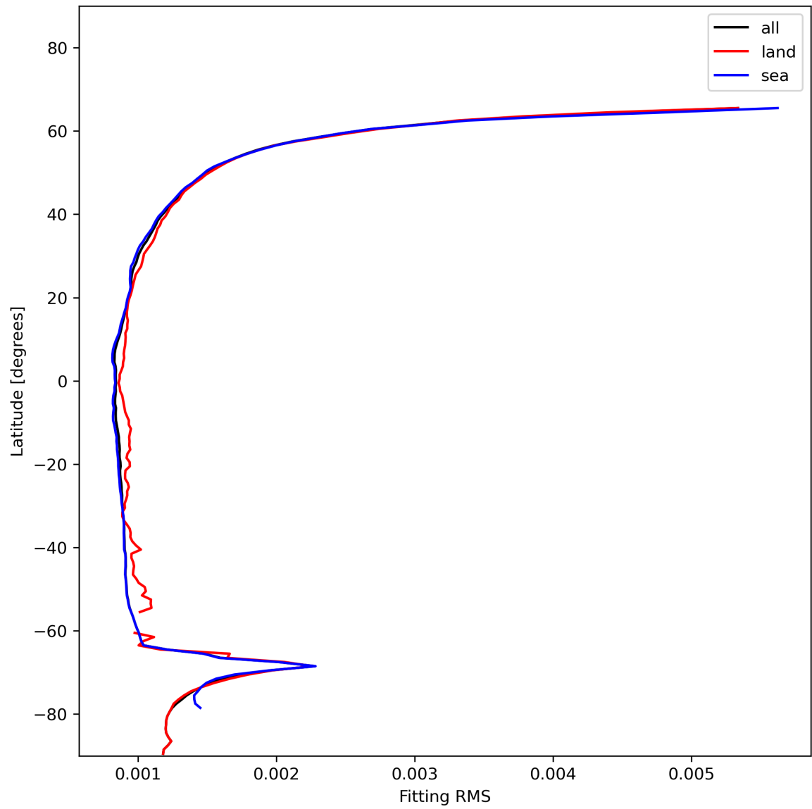
Figure 16: Zonal average of “Fitting RMS” for 2023-12-12 to 2023-12-14.
