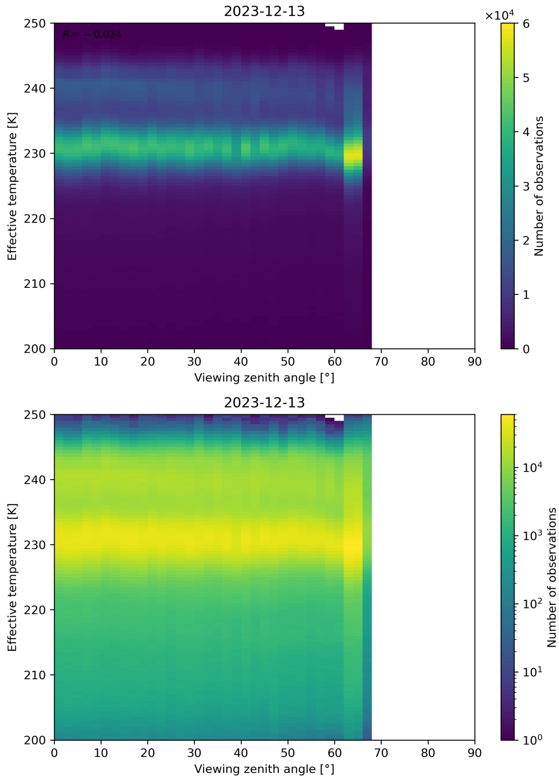
Figure 50: Scatter density plot of “Viewing zenith angle” against “Effective temperature” for 2023-12-12 to 2023-12-14.
