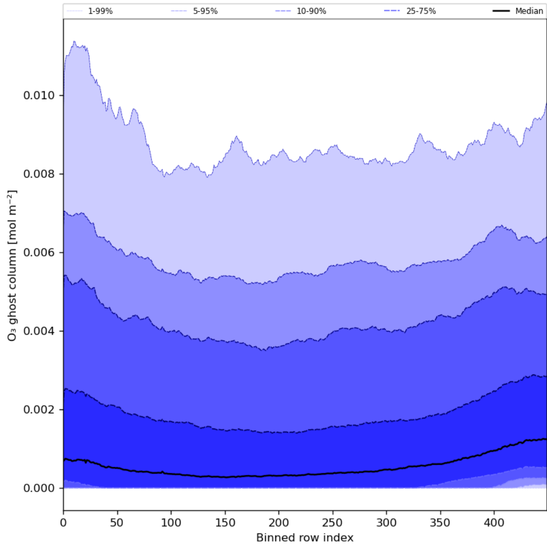
Figure 32: Along track statistics of “O 3 ghost column” for 2023-12-12 to 2023-12-14
