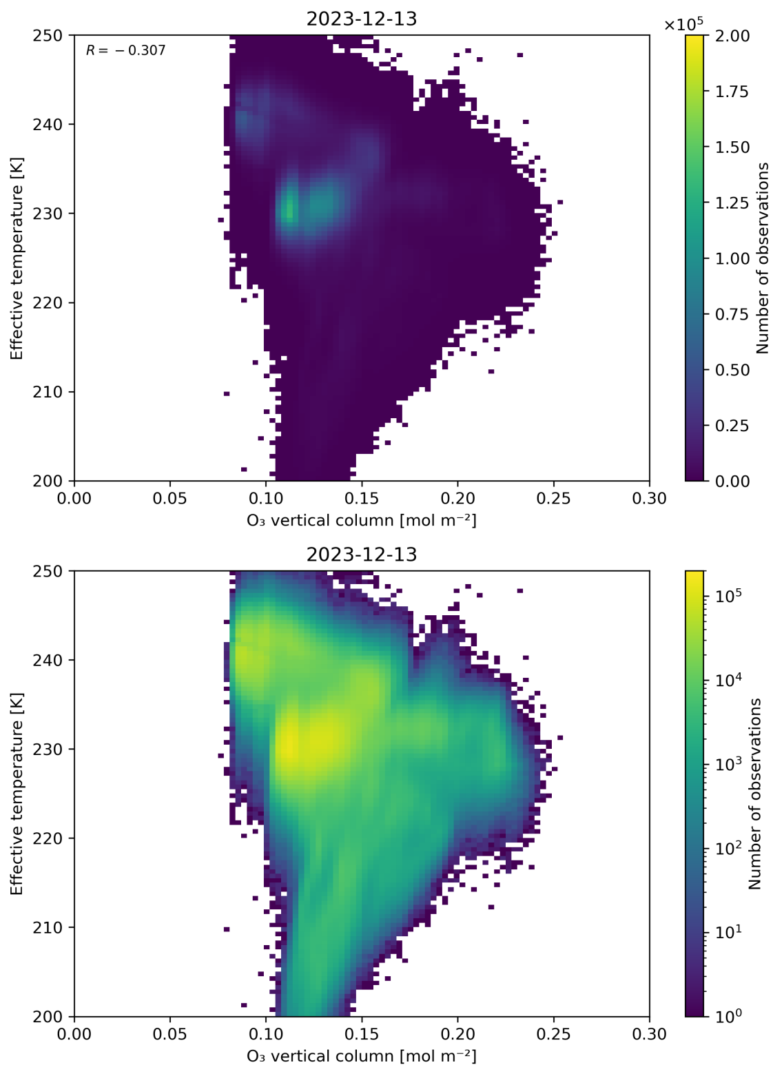
Figure 39: Scatter density plot of “O 3 vertical column” against “Effective temperature” for 2023-12-12 to 2023-12-14.
