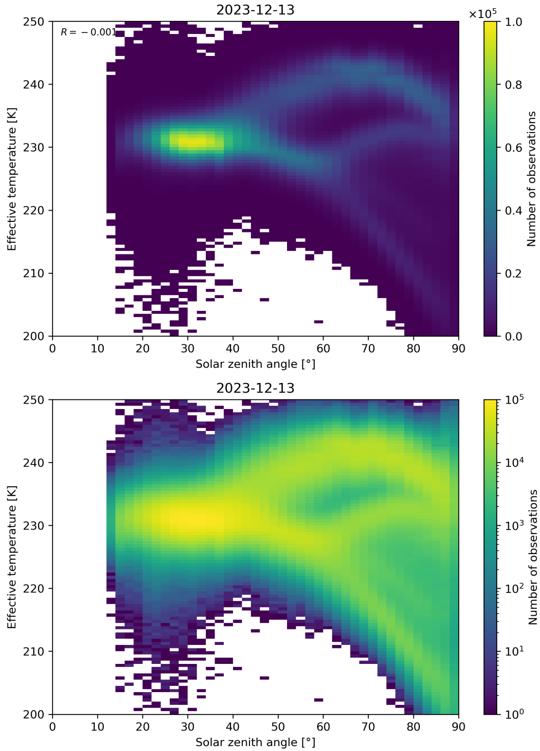
Figure 45: Scatter density plot of “Solar zenith angle” against “Effective temperature” for 2023-12-12 to 2023-12-14.
