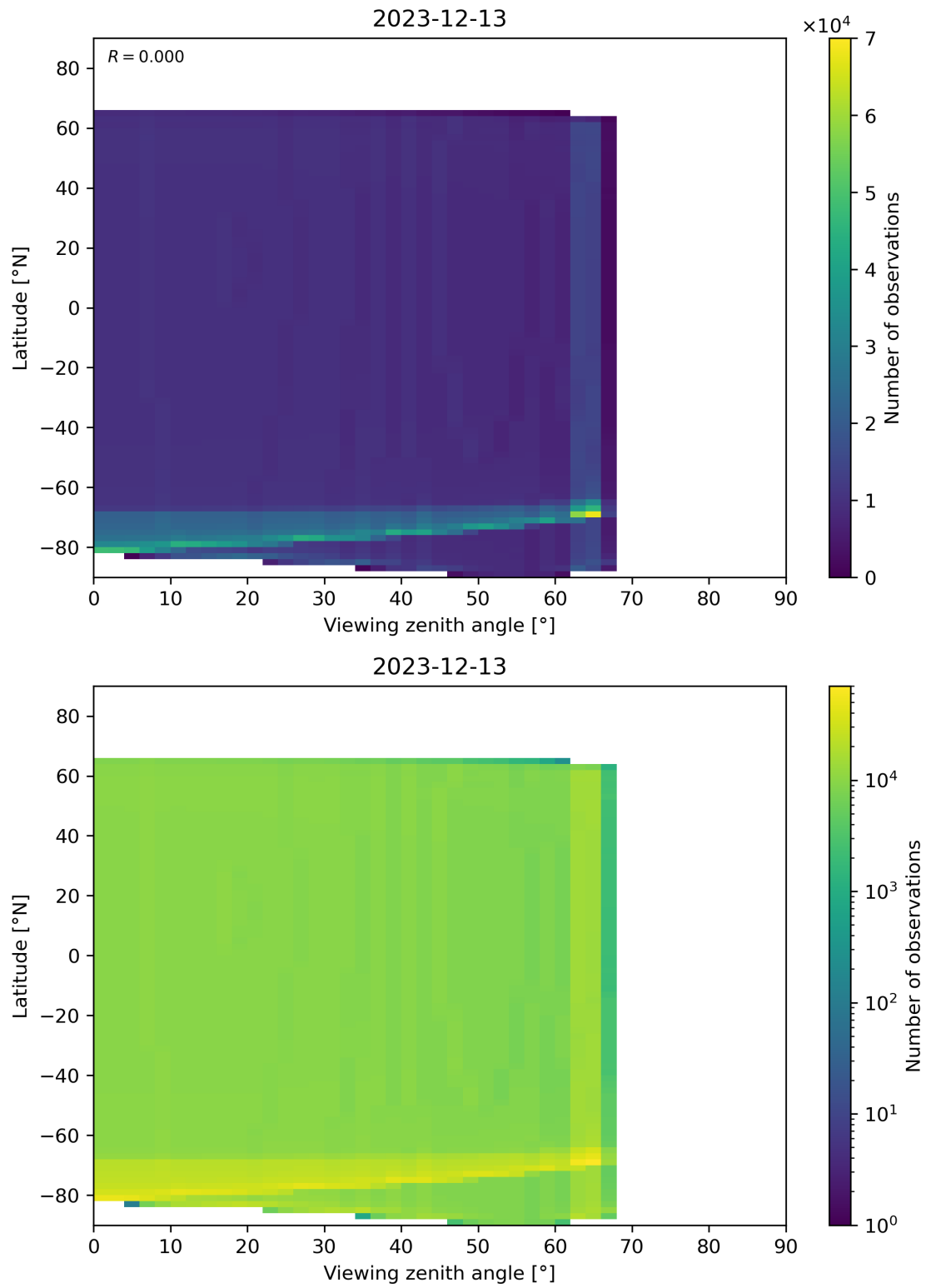
Figure 49: Scatter density plot of “Viewing zenith angle” against “Latitude” for 2023-12-12 to 2023-12-14.
