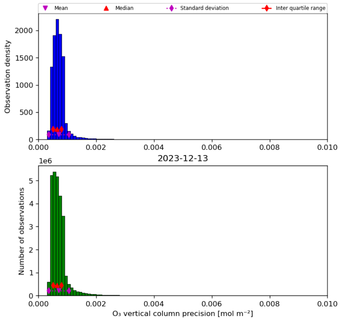
Figure 22: Histogram of “O 3 vertical column precision” for 2023-12-12 to 2023-12-14
