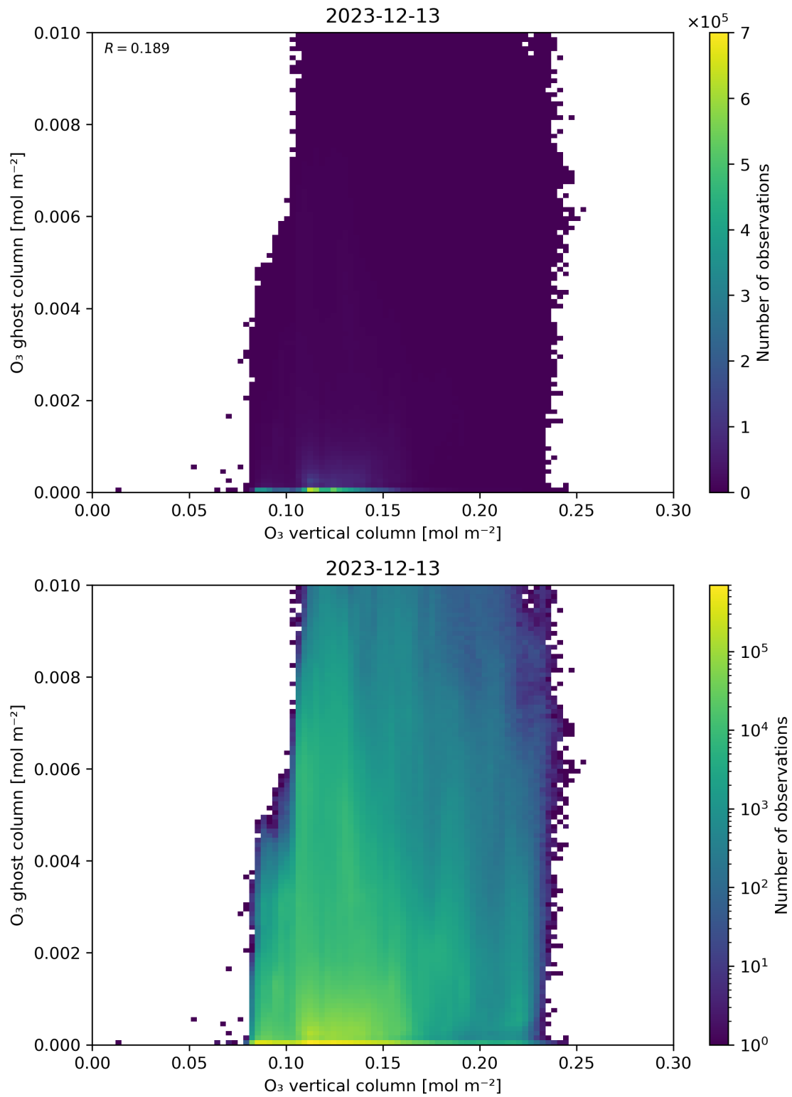
Figure 40: Scatter density plot of “O 3 vertical column” against “O 3 ghost column” for 2023-12-12 to 2023-12-14.
