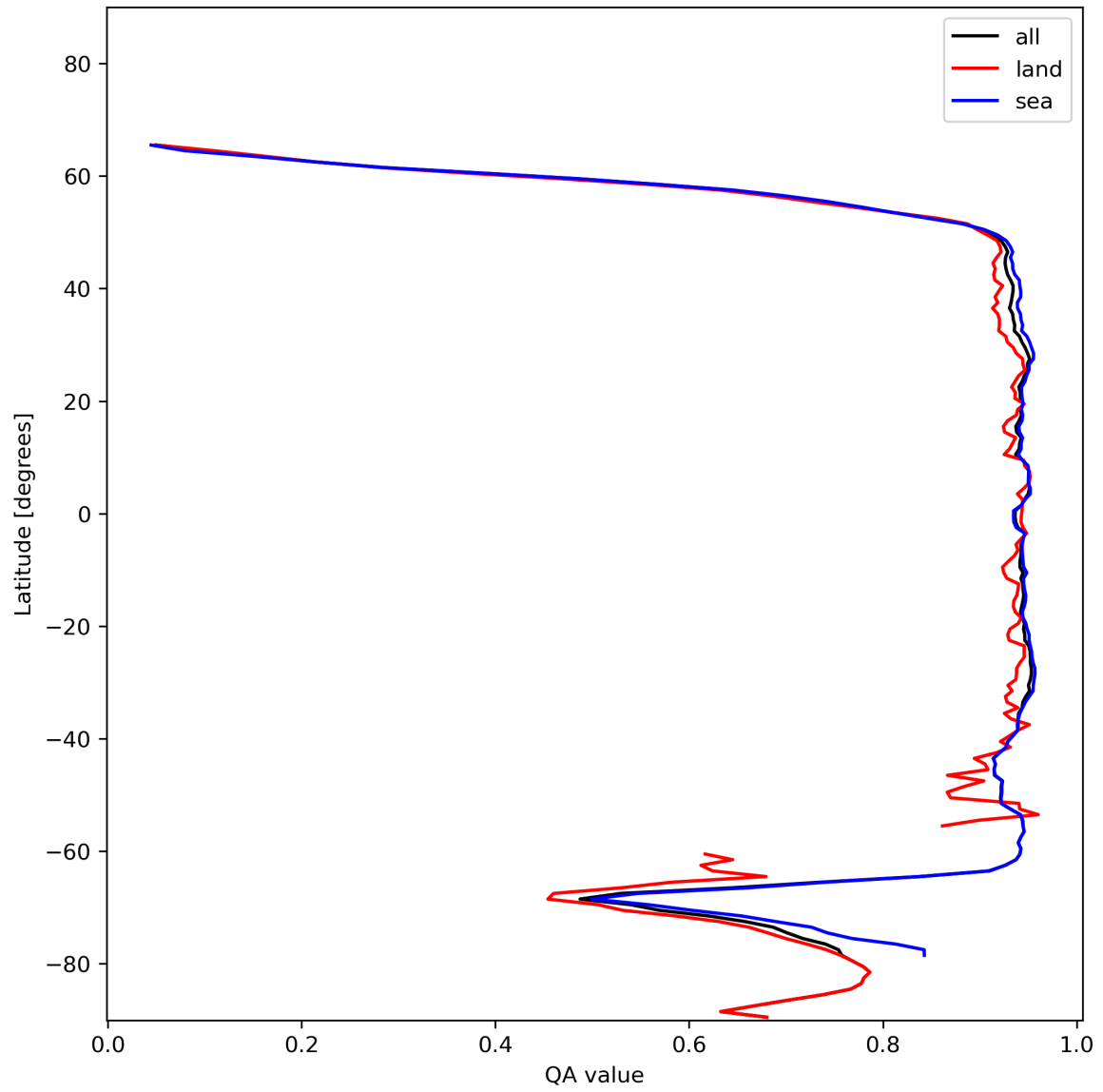
Figure 13: Zonal average of “QA value” for 2023-12-12 to 2023-12-14.
