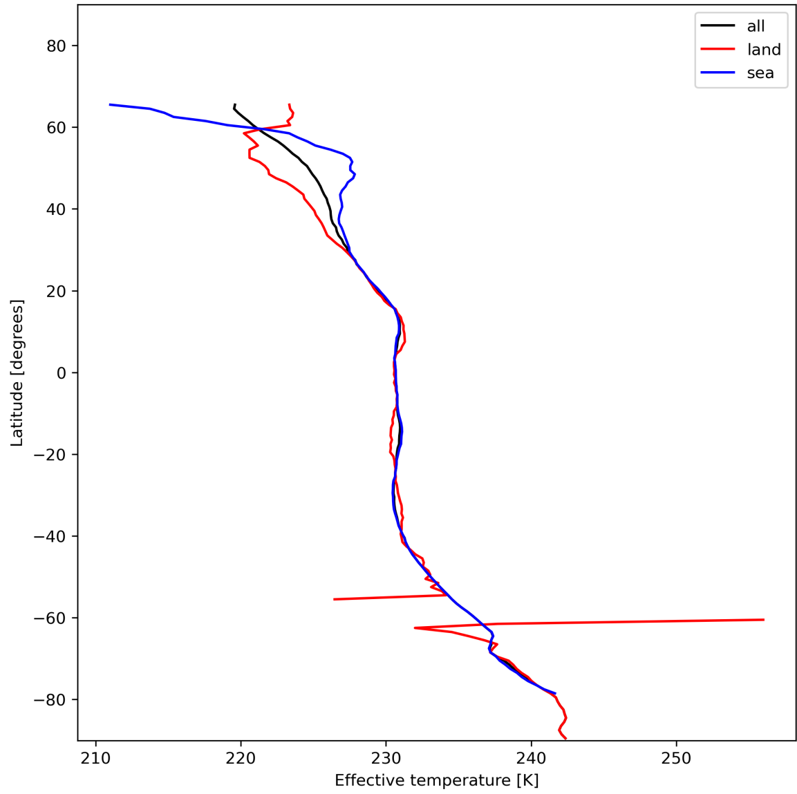
Figure 17: Zonal average of “Effective temperature” for 2023-12-12 to 2023-12-14.
