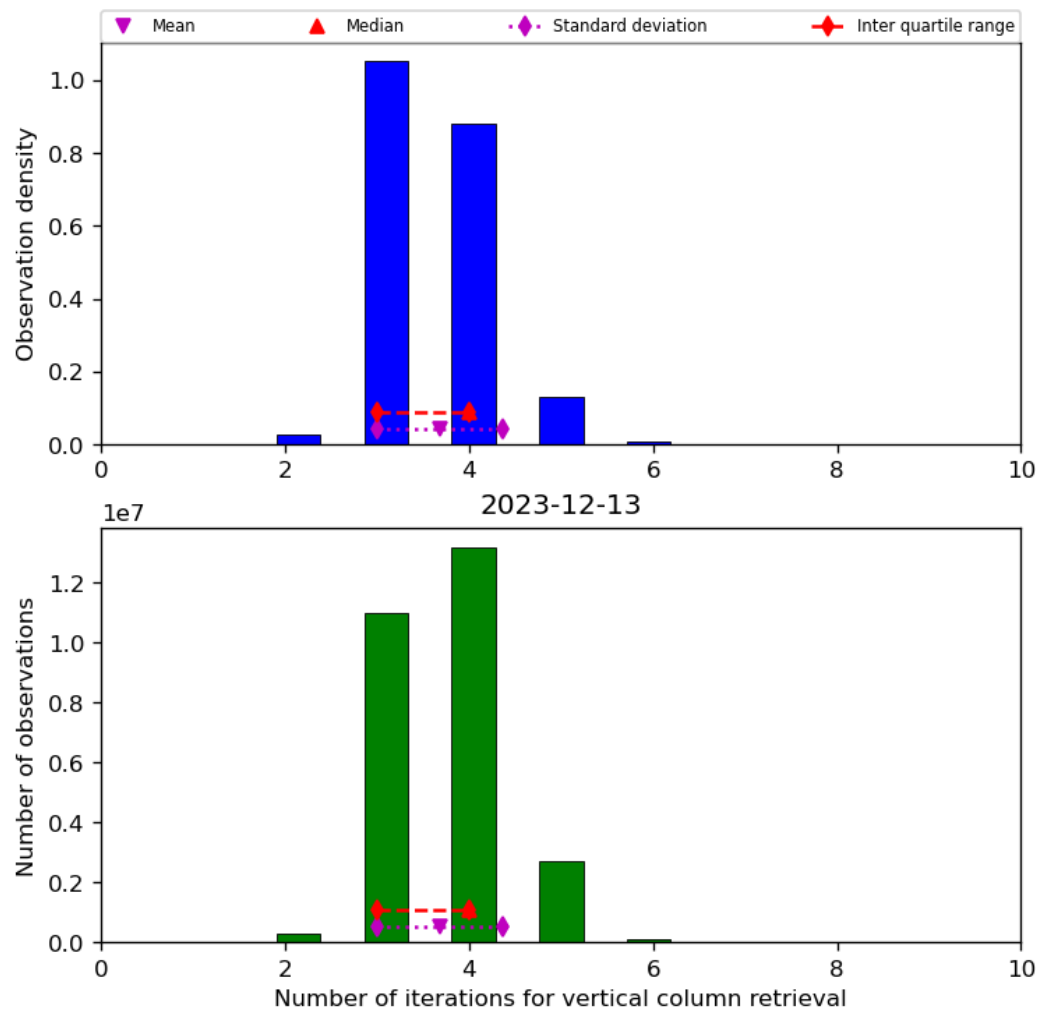
Figure 26: Histogram of “Number of iterations for vertical column retrieval” for 2023-12-12 to 2023-12-14
