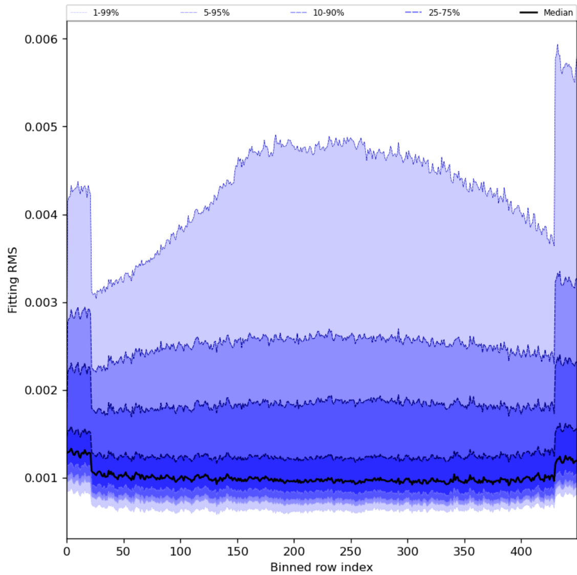
Figure 30: Along track statistics of “Fitting RMS” for 2023-12-12 to 2023-12-14
