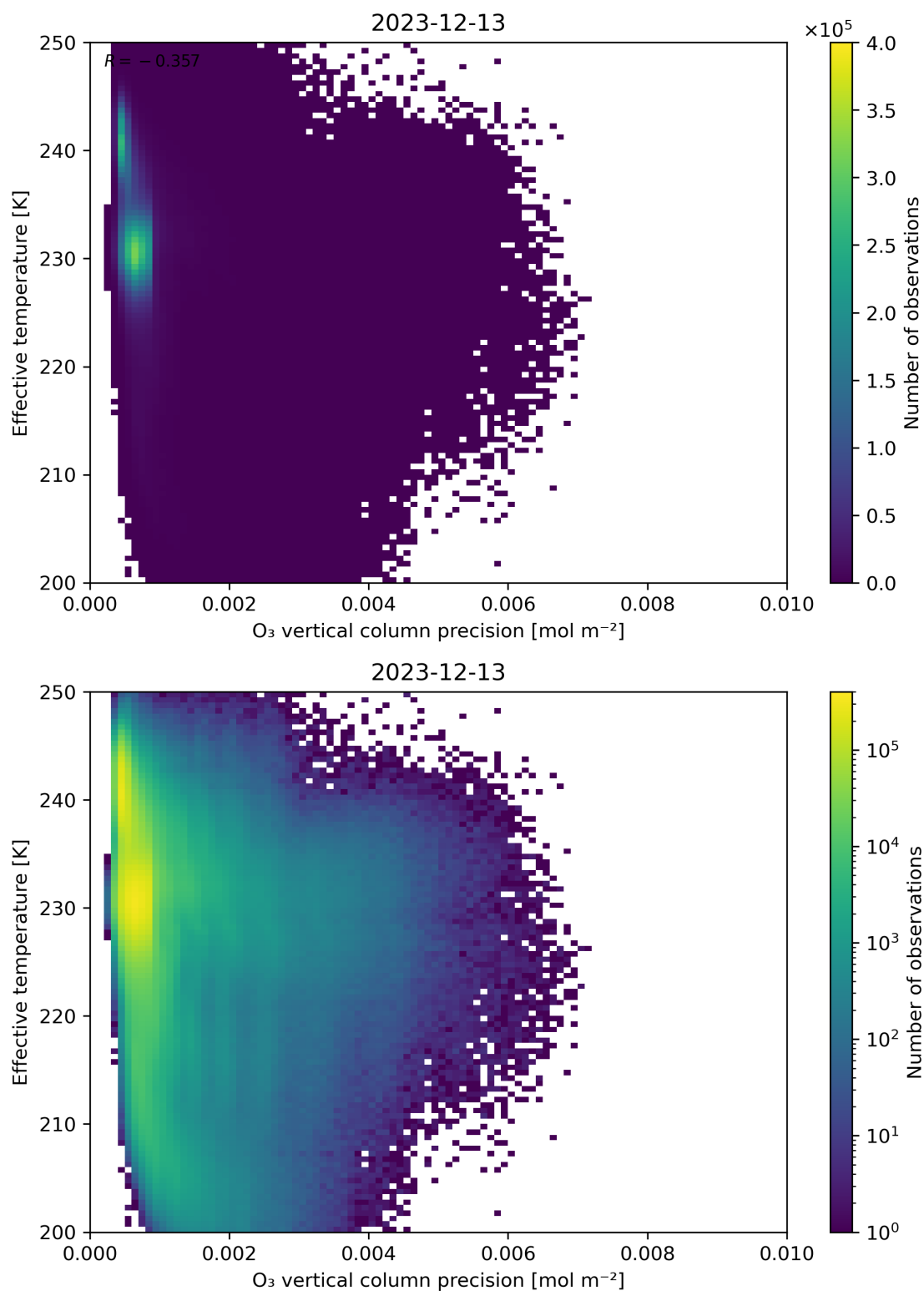
Figure 42: Scatter density plot of “O 3 vertical column precision” against “Effective temperature” for 2023-12-12 to 2023-12-14.
