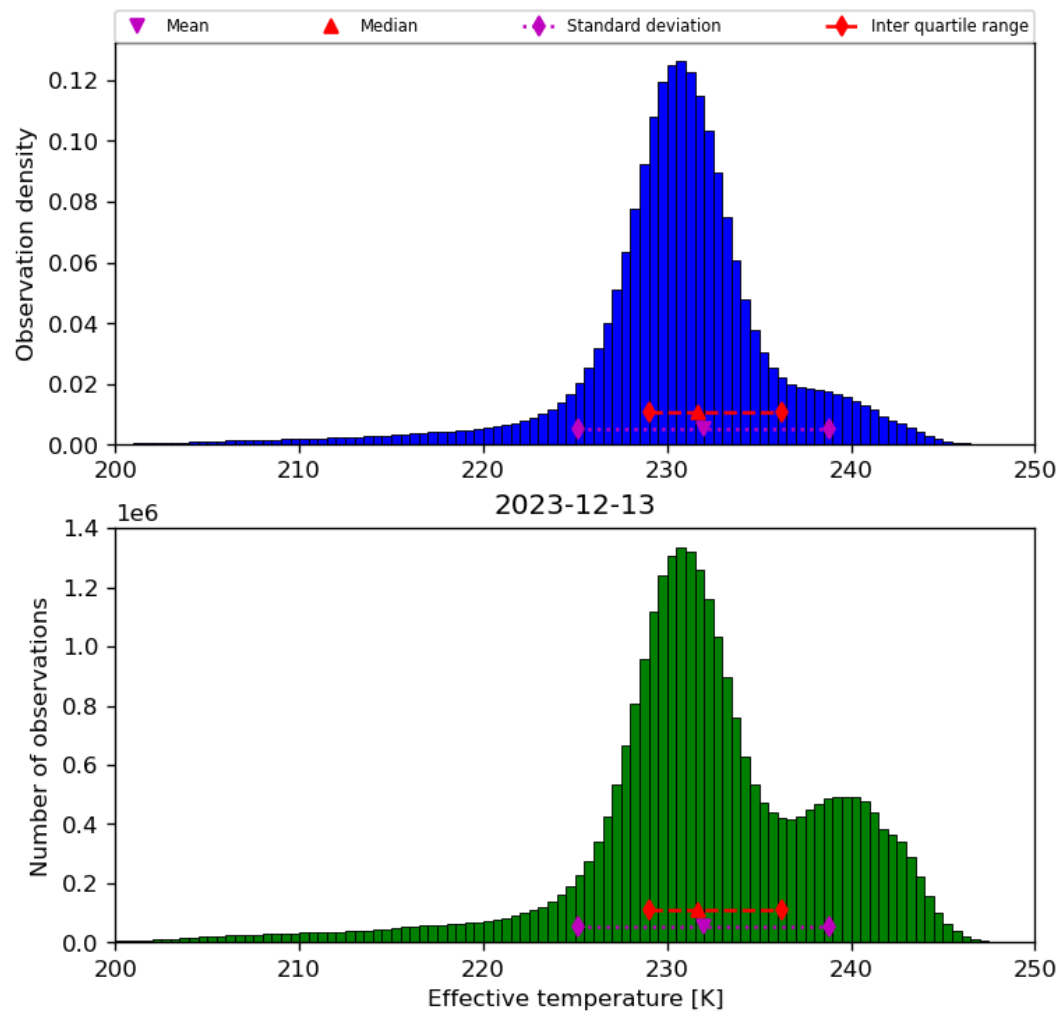
Figure 24: Histogram of “Effective temperature” for 2023-12-12 to 2023-12-14
