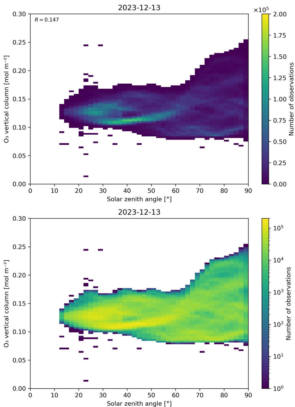
Figure 47: Scatter density plot of “Solar zenith angle” against “O 3 vertical column” for 2023-12-12 to 2023-12-14.
