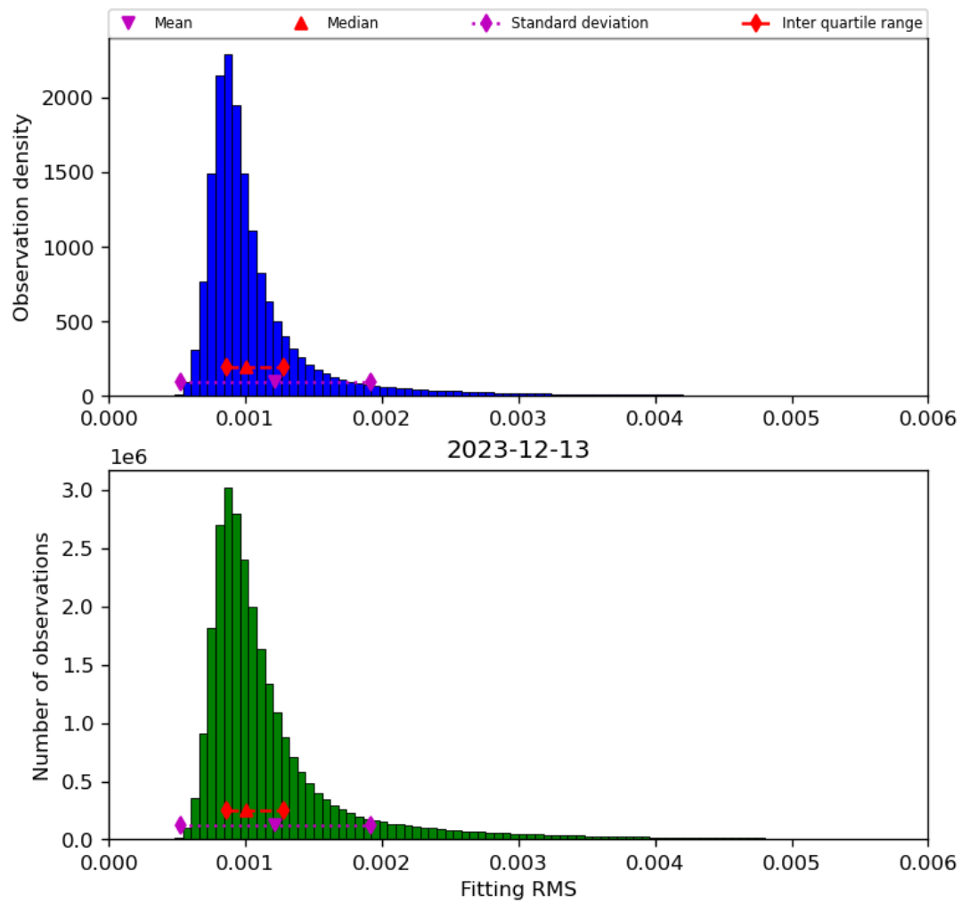
Figure 23: Histogram of “Fitting RMS” for 2023-12-12 to 2023-12-14
