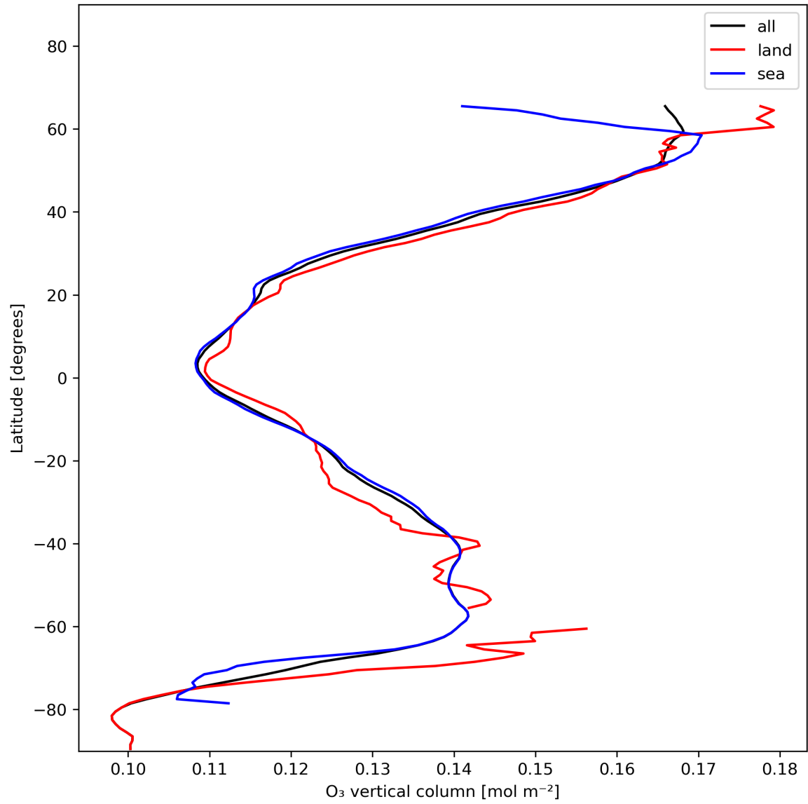
Figure 14: Zonal average of “O 3 vertical column” for 2023-12-12 to 2023-12-14.
