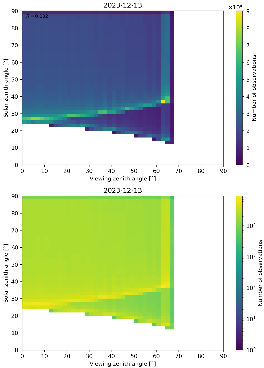
Figure 54: Scatter density plot of “Viewing zenith angle” against “Solar zenith angle” for 2023-12-12 to 2023-12-14.
