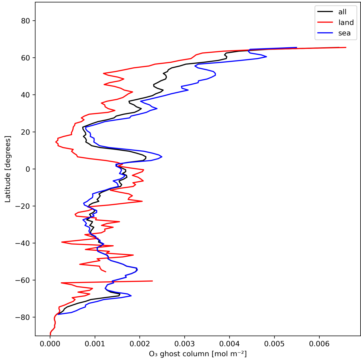
Figure 18: Zonal average of "O 3 ghost column" for 2023-12-12 to 2023-12-14.
