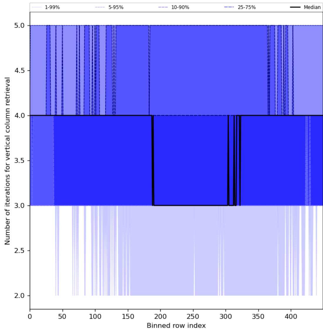
Figure 33: Along track statistics of “Number of iterations for vertical column retrieval” for 2023-12-12 to 2023-12-14
