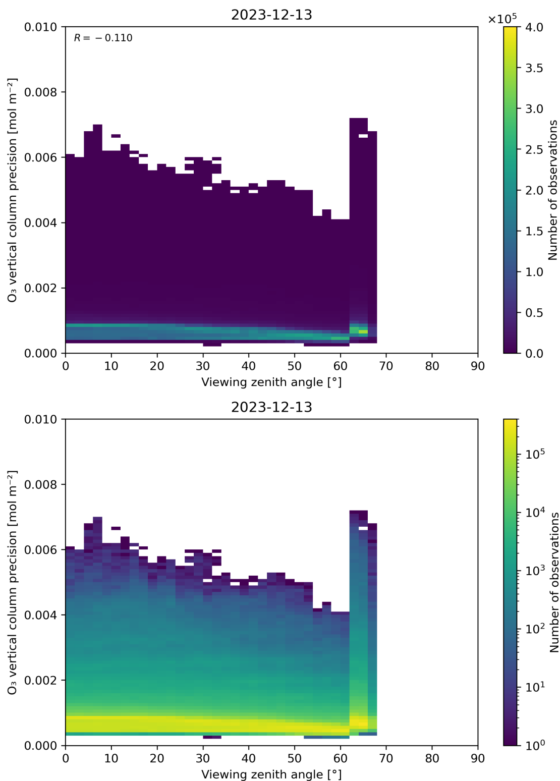
Figure 53: Scatter density plot of “Viewing zenith angle” against “O 3 vertical column precision” for 2023-12-12 to 2023-12-14.
