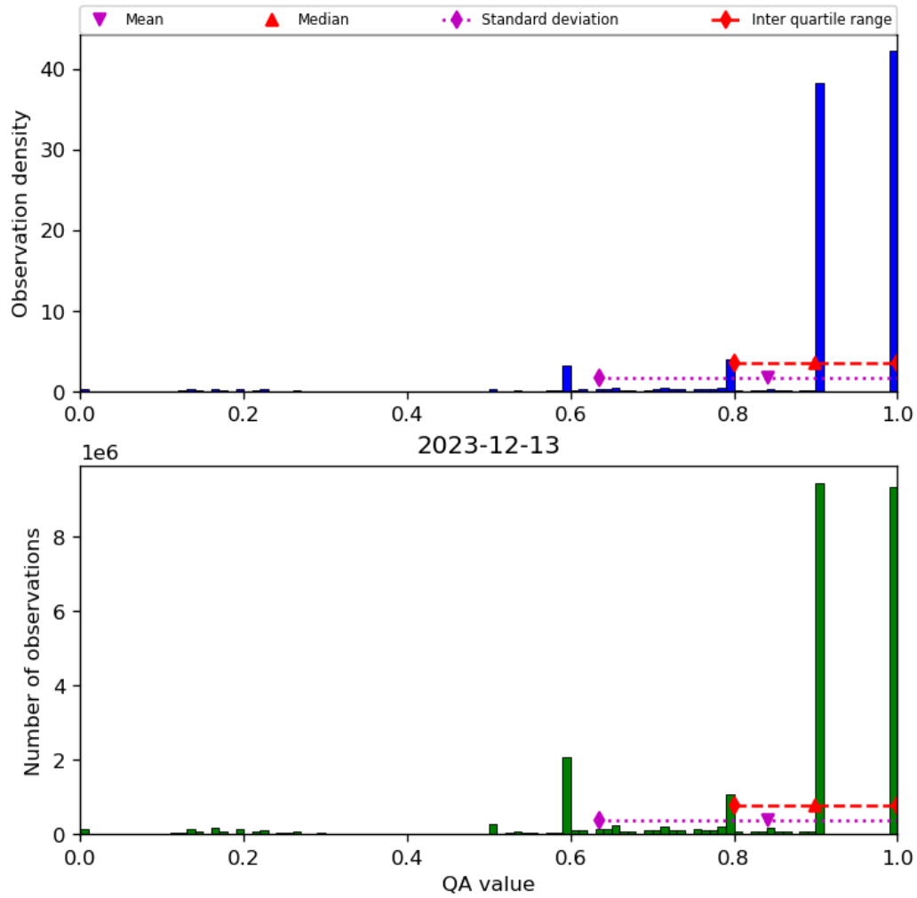
Figure 20: Histogram of “QA value” for 2023-12-12 to 2023-12-14
