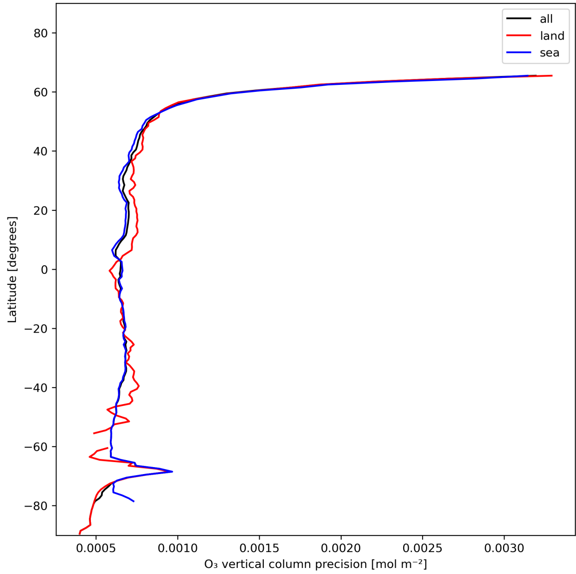
Figure 15: Zonal average of “O 3 vertical column precision” for 2023-12-12 to 2023-12-14.
