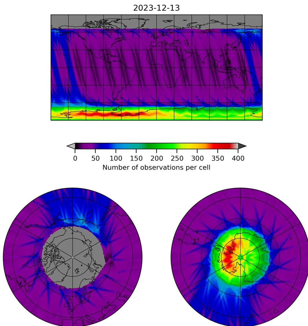
Figure 12: Map of the number of observations for 2023-12-12 to 2023-12-14
