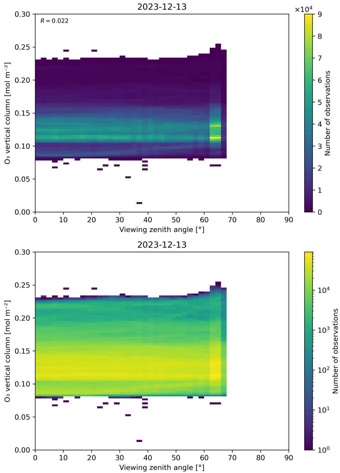
Figure 52: Scatter density plot of “Viewing zenith angle” against “O 3 vertical column” for 2023-12-12 to 2023-12-14.
