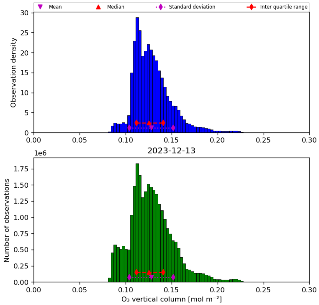
Figure 21: Histogram of “O 3 vertical column” for 2023-12-12 to 2023-12-14
