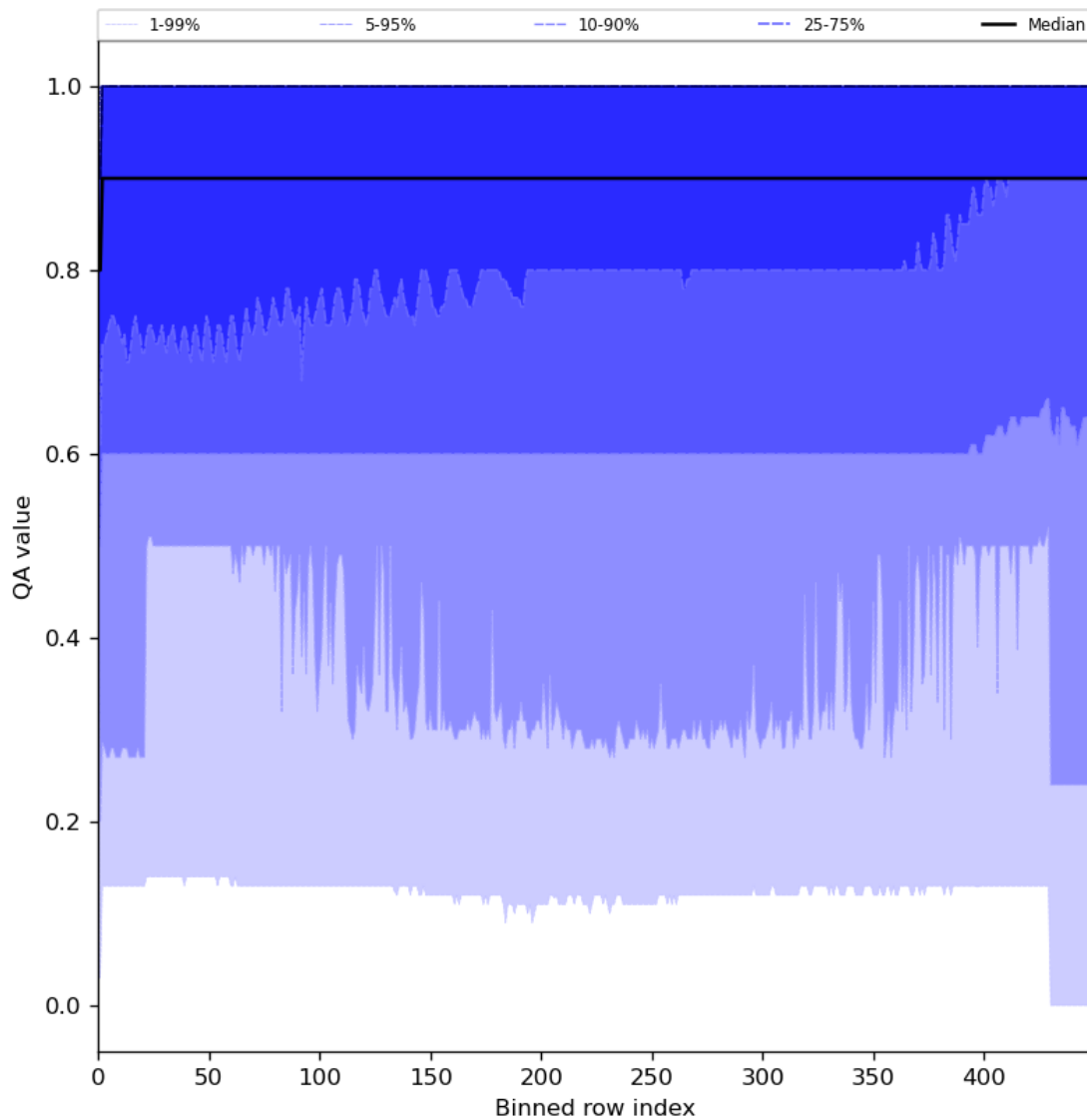
Figure 27: Along track statistics of “QA value” for 2023-12-12 to 2023-12-14
