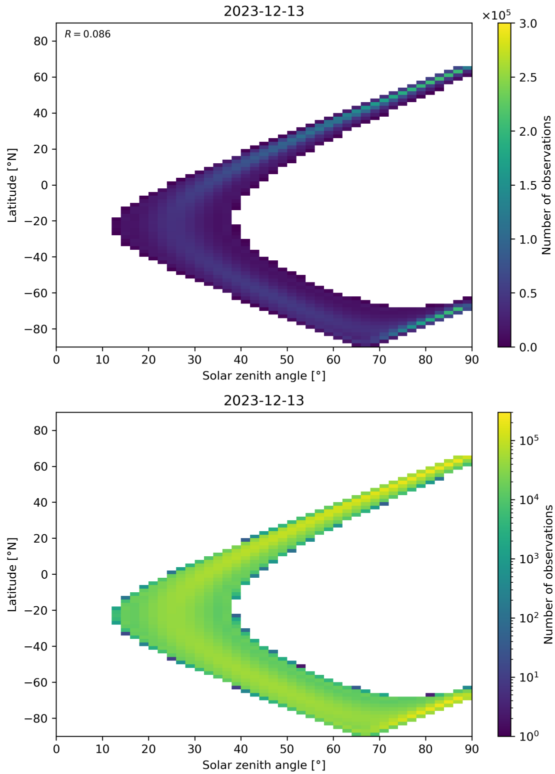
Figure 44: Scatter density plot of “Solar zenith angle” against “Latitude” for 2023-12-12 to 2023-12-14.
