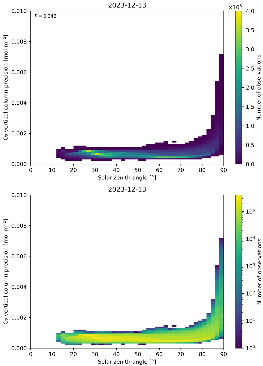
Figure 48: Scatter density plot of “Solar zenith angle” against “O 3 vertical column precision” for 2023-12-12 to 2023-12-14.
