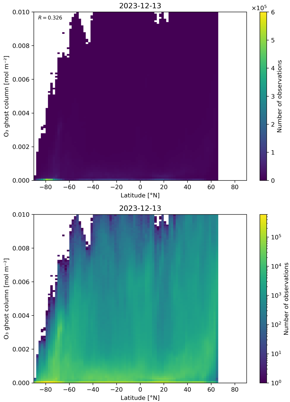
Figure 35: Scatter density plot of “Latitude” against “O 3 ghost column” for 2023-12-12 to 2023-12-14.
