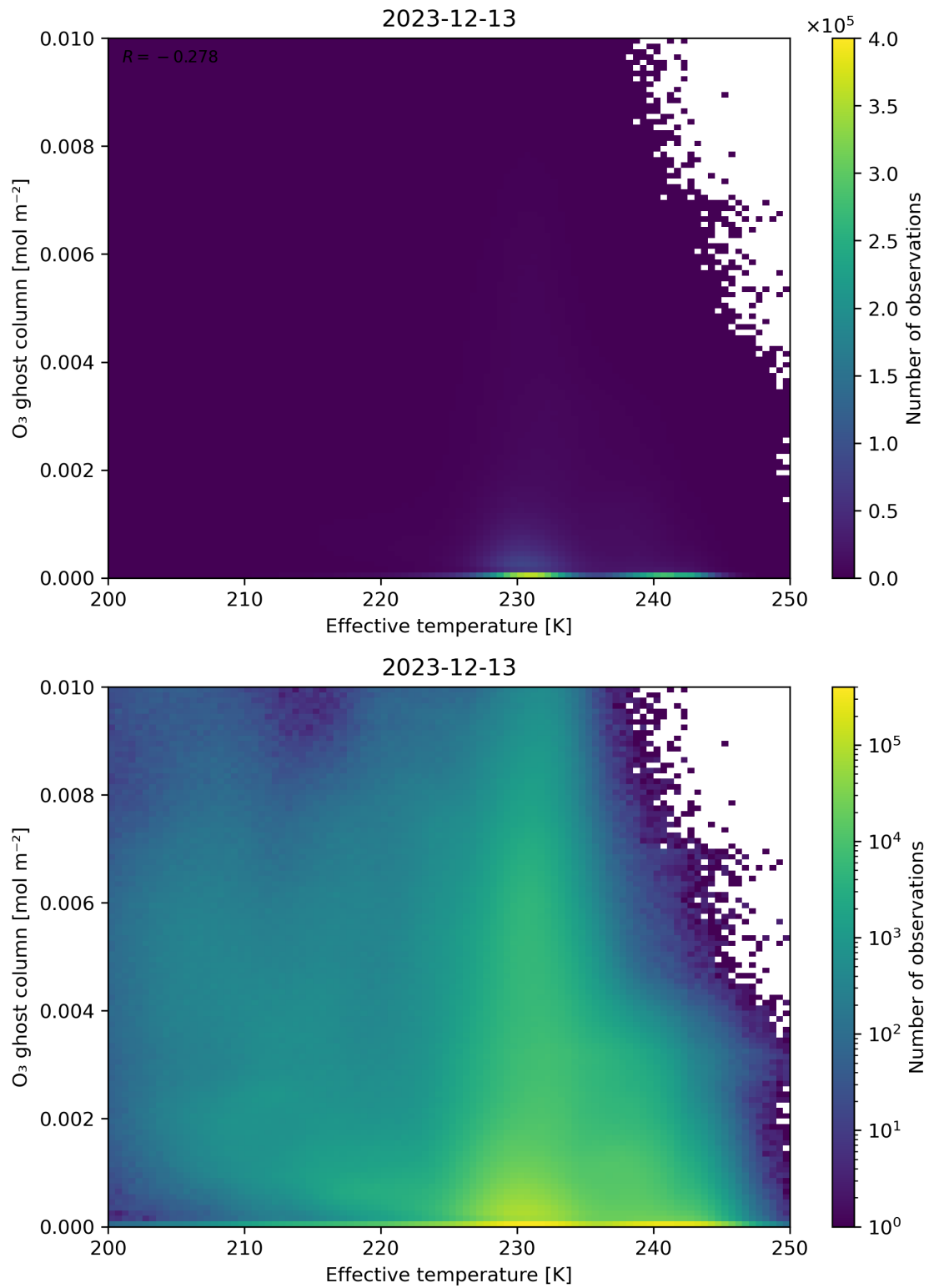
Figure 38: Scatter density plot of “Effective temperature” against “O 3 ghost column” for 2023-12-12 to 2023-12-14.
