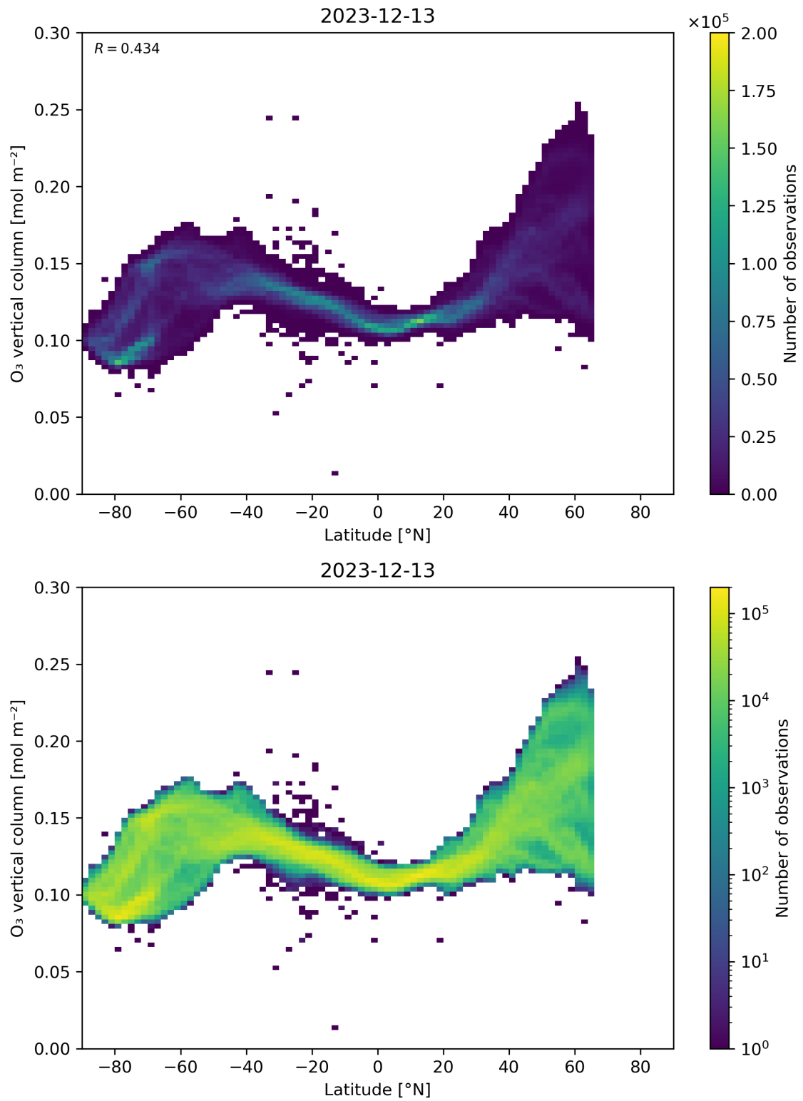
Figure 36: Scatter density plot of “Latitude” against “O 3 vertical column” for 2023-12-12 to 2023-12-14.
