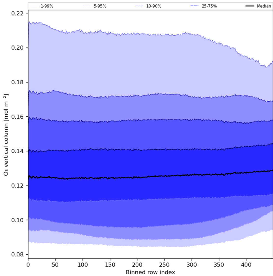
Figure 28: Along track statistics of “O 3 vertical column” for 2023-12-12 to 2023-12-14
