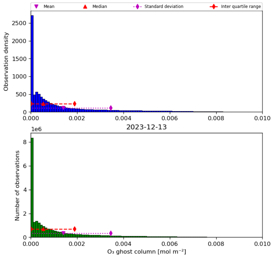
Figure 25: Histogram of “O 3 ghost column” for 2023-12-12 to 2023-12-14
