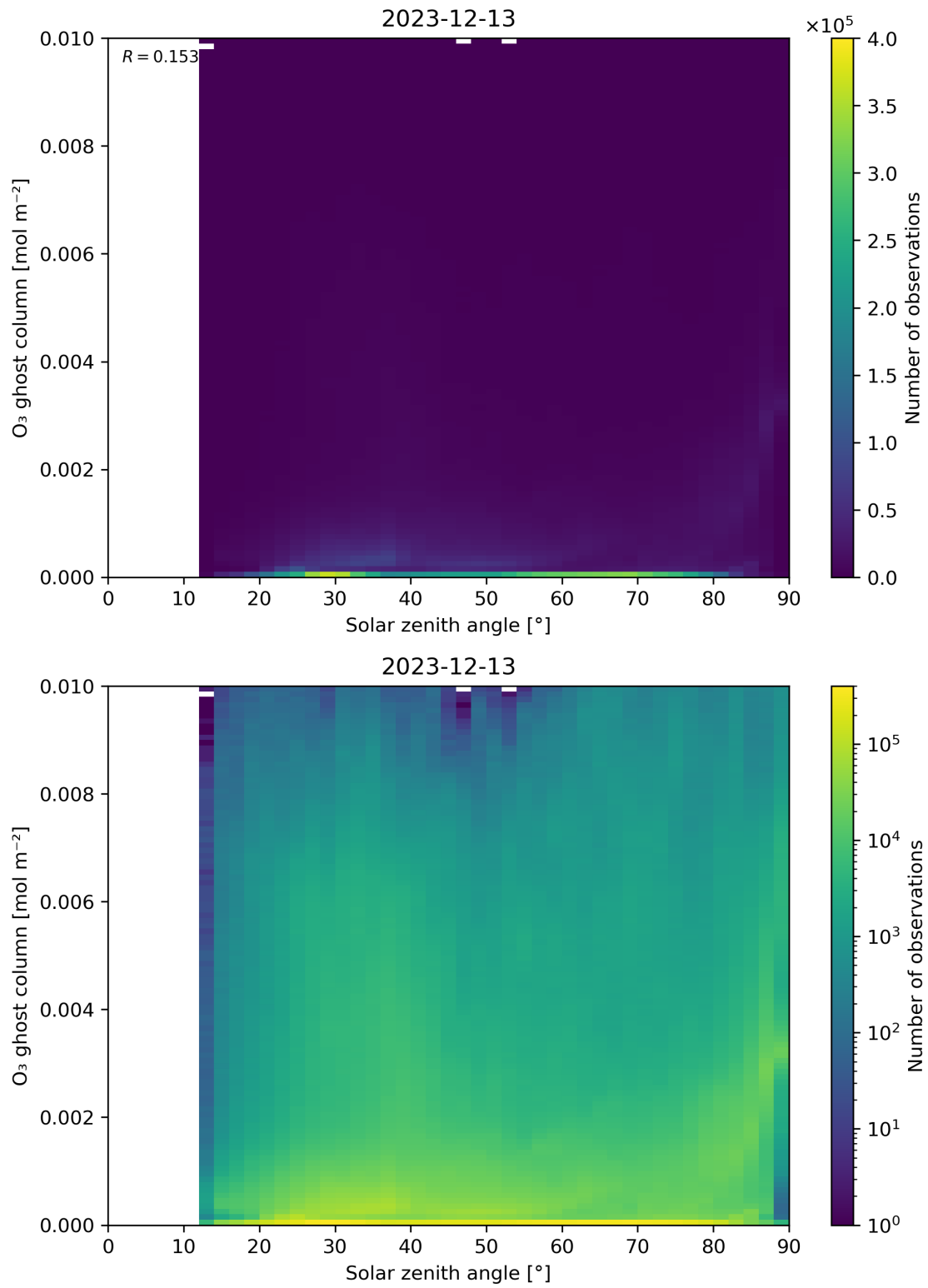
Figure 46: Scatter density plot of “Solar zenith angle” against “O 3 ghost column” for 2023-12-12 to 2023-12-14.
