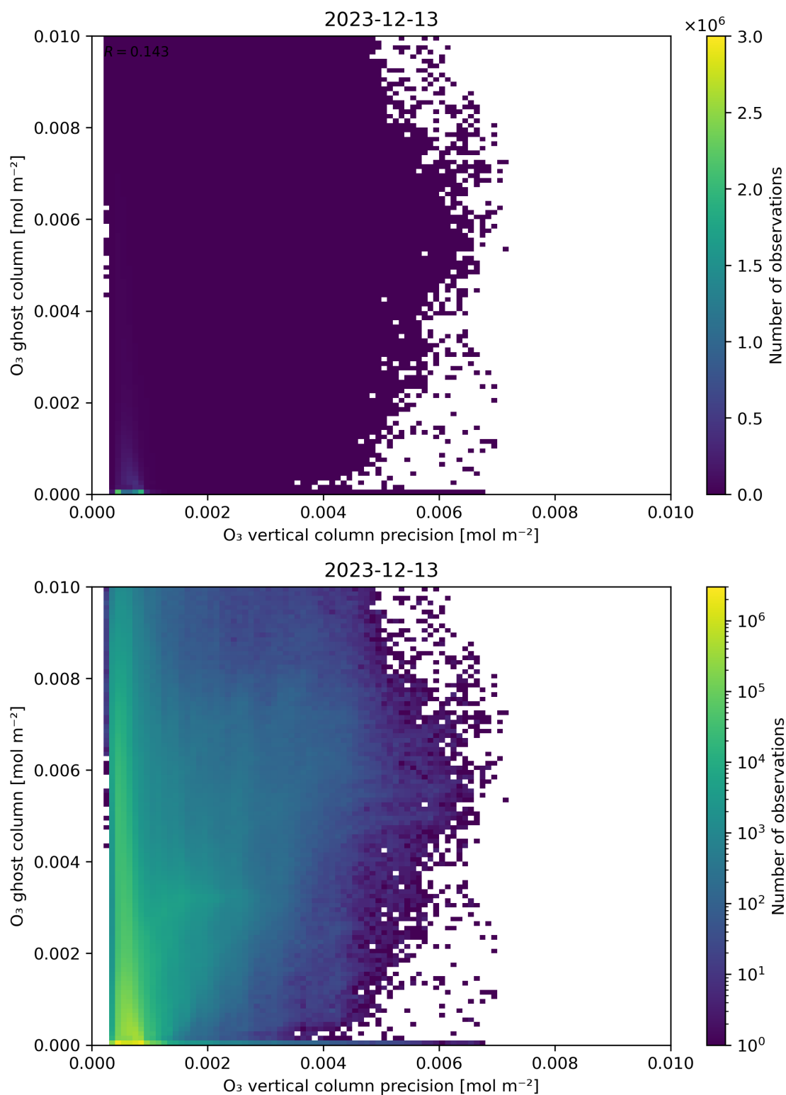
Figure 43: Scatter density plot of “ O_3 vertical column precision” against “ O_3 ghost column” for 2023-12-12 to 2023-12-14.
