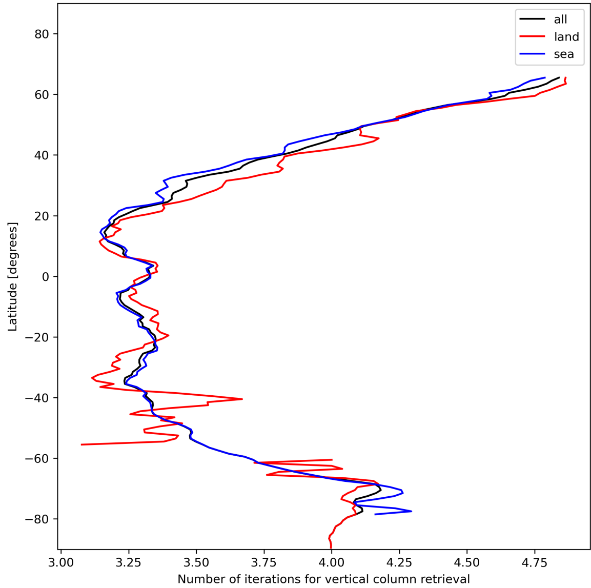
Figure 19: Zonal average of “Number of iterations for vertical column retrieval” for 2023-12-12 to 2023-12-14.
