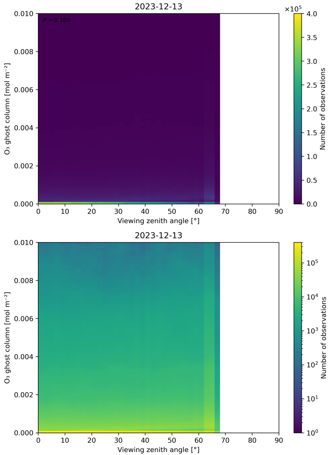
Figure 51: Scatter density plot of “Viewing zenith angle” against “O 3 ghost column” for 2023-12-12 to 2023-12-14.
