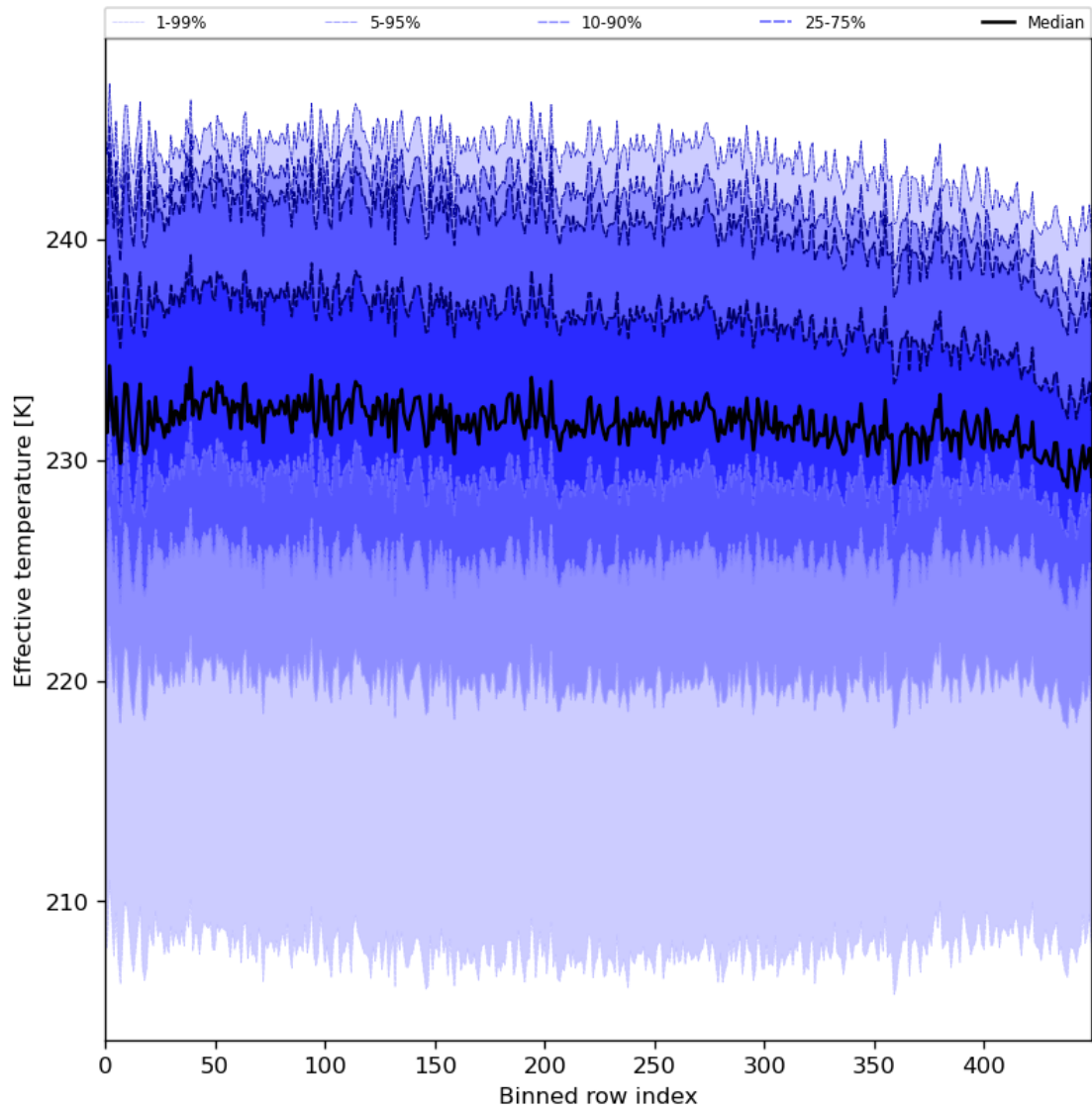
Figure 31: Along track statistics of “Effective temperature” for 2023-12-12 to 2023-12-14
