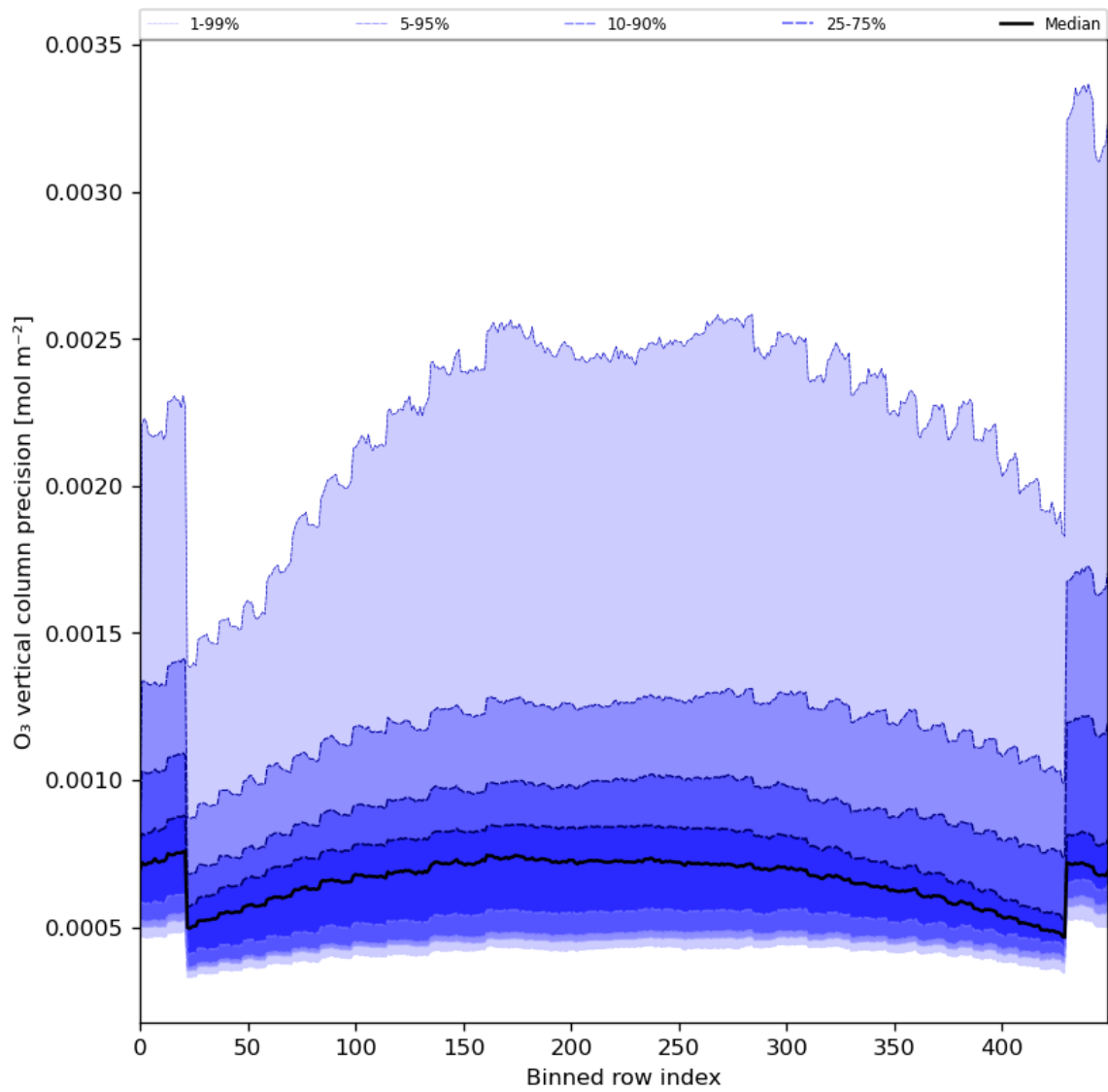
Figure 29: Along track statistics of “O 3 vertical column precision” for 2023-12-12 to 2023-12-14
