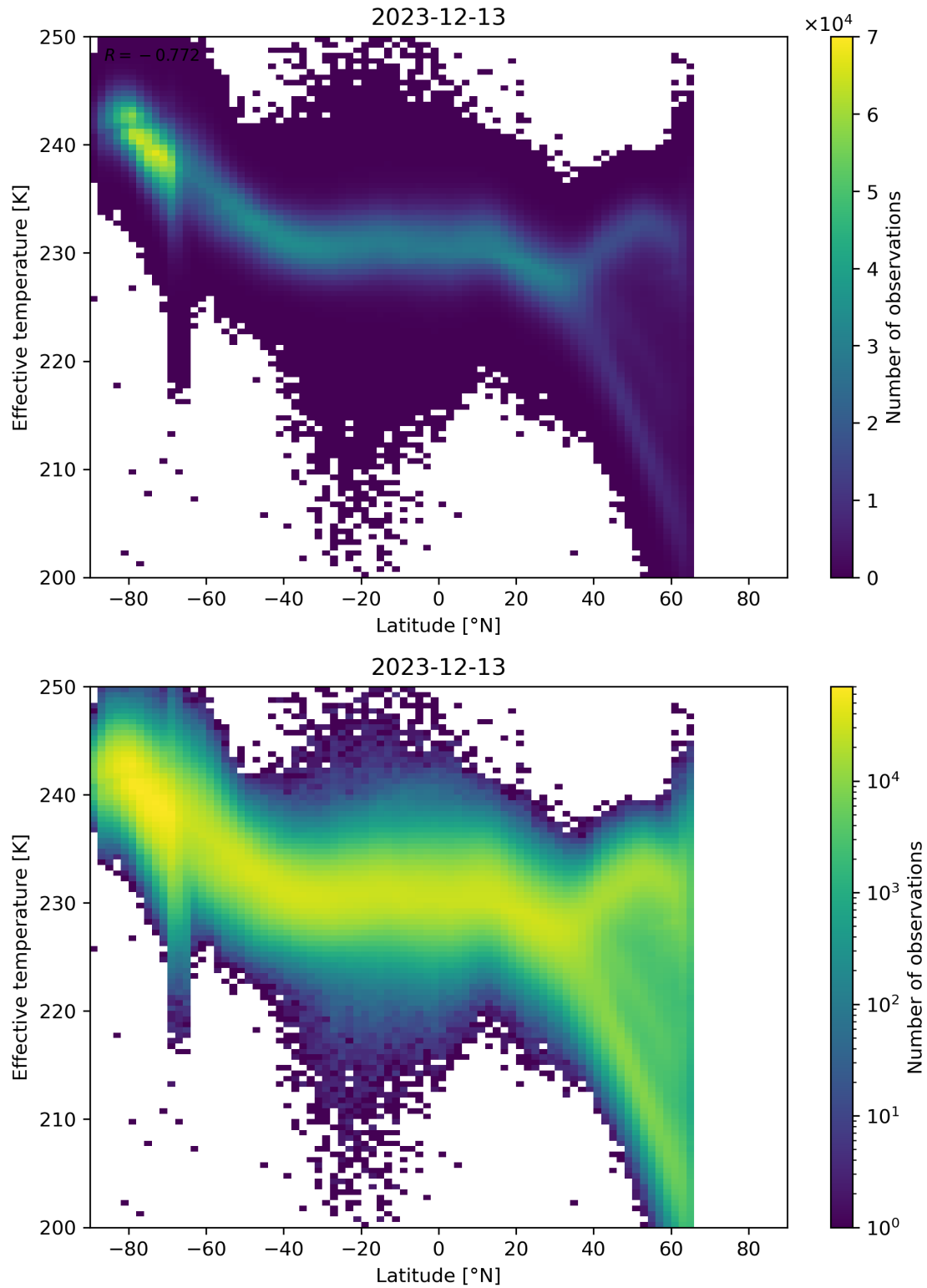
Figure 34: Scatter density plot of “Latitude” against “Effective temperature” for 2023-12-12 to 2023-12-14.
