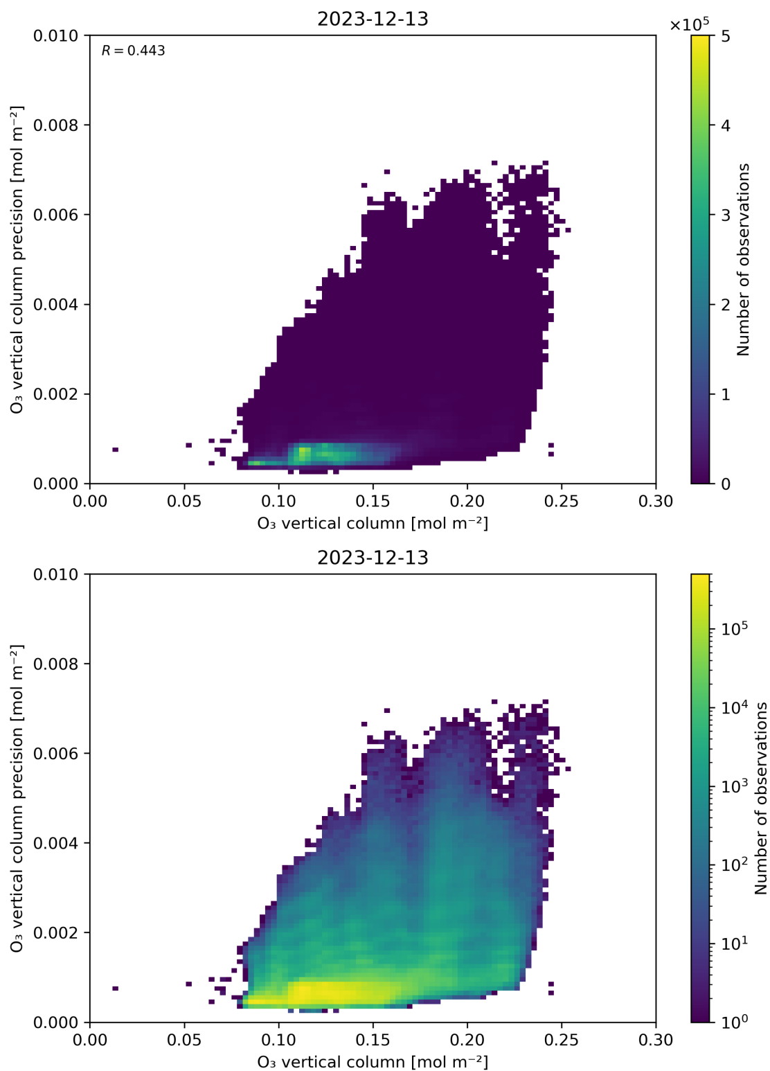
Figure 41: Scatter density plot of “O 3 vertical column” against “O 3 vertical column precision” for 2023-12-12 to 2023-12-14.
