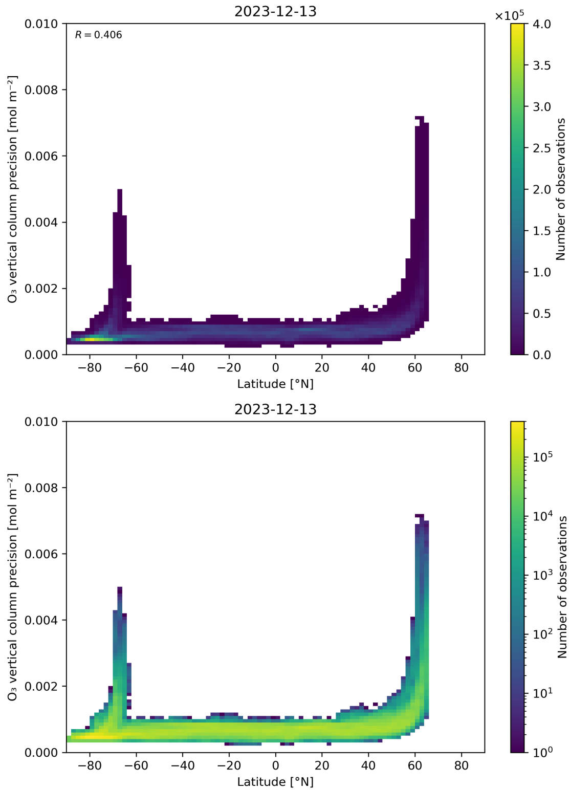
Figure 37: Scatter density plot of “Latitude” against “O 3 vertical column precision” for 2023-12-12 to 2023-12-14.
