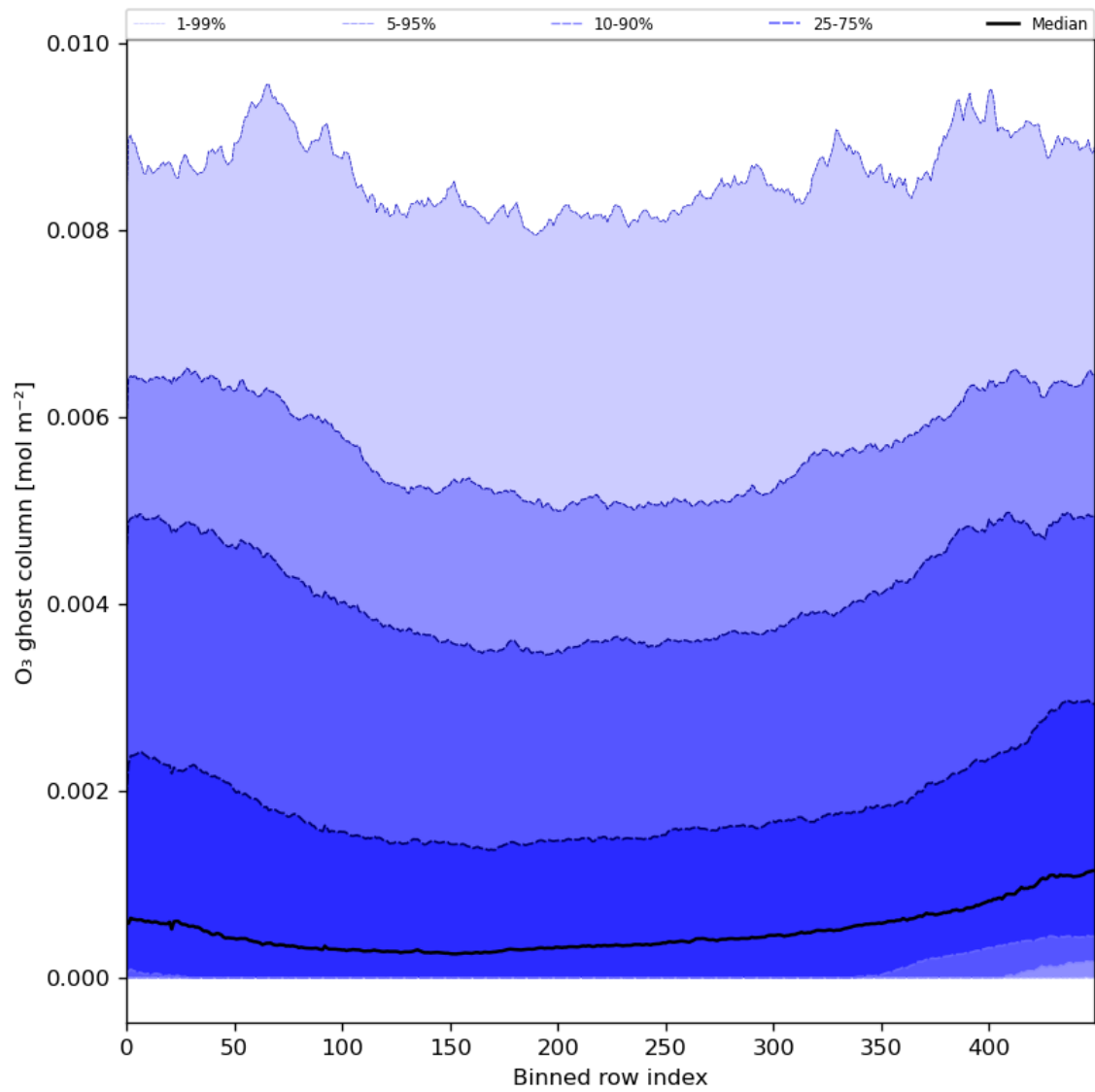
Figure 32: Along track statistics of “O 3 ghost column” for 2023-12-14 to 2023-12-15
