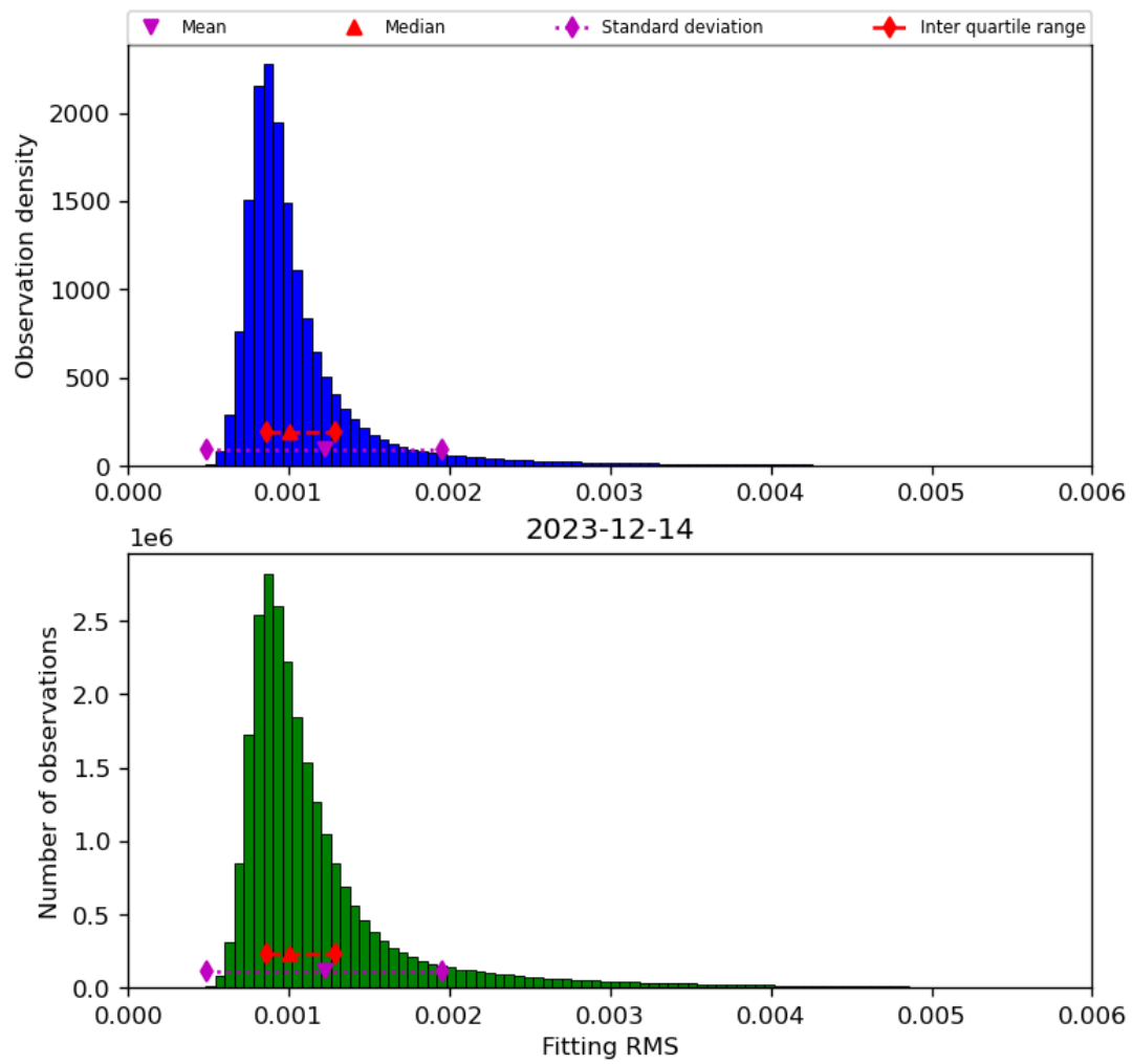
Figure 23: Histogram of “Fitting RMS” for 2023-12-14 to 2023-12-15
