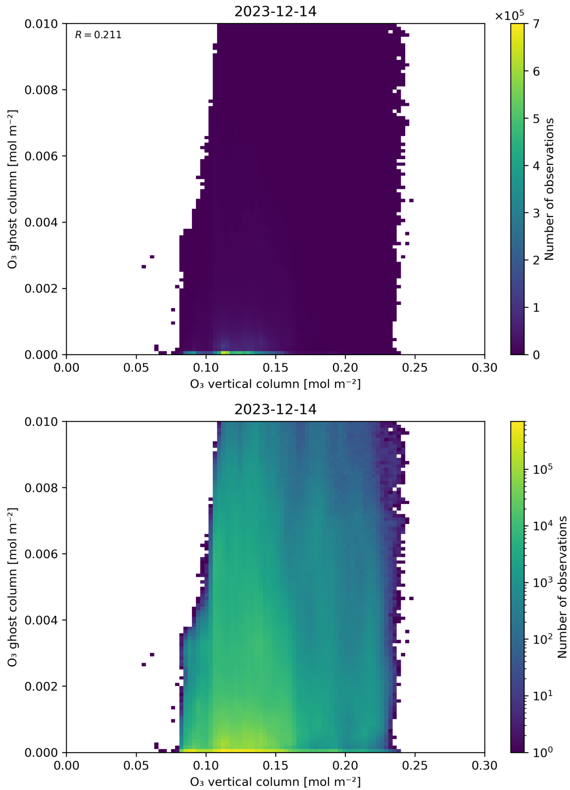
Figure 40: Scatter density plot of “O 3 vertical column” against “O 3 ghost column” for 2023-12-14 to 2023-12-15.
