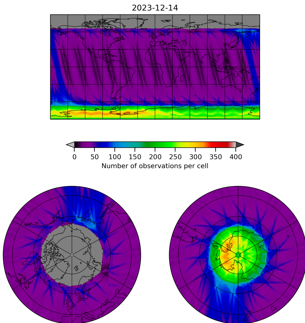
Figure 12: Map of the number of observations for 2023-12-14 to 2023-12-15
