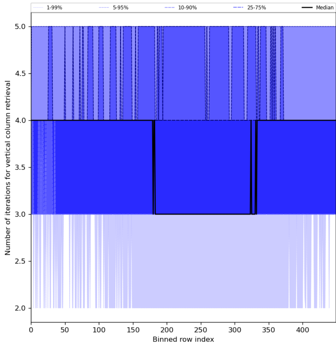
Figure 33: Along track statistics of “Number of iterations for vertical column retrieval” for 2023-12-14 to 2023-12-15
