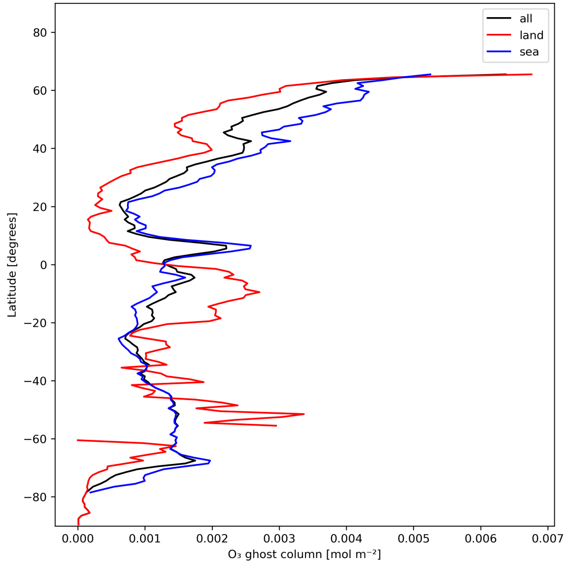
Figure 18: Zonal average of “O 3 ghost column” for 2023-12-14 to 2023-12-15.
