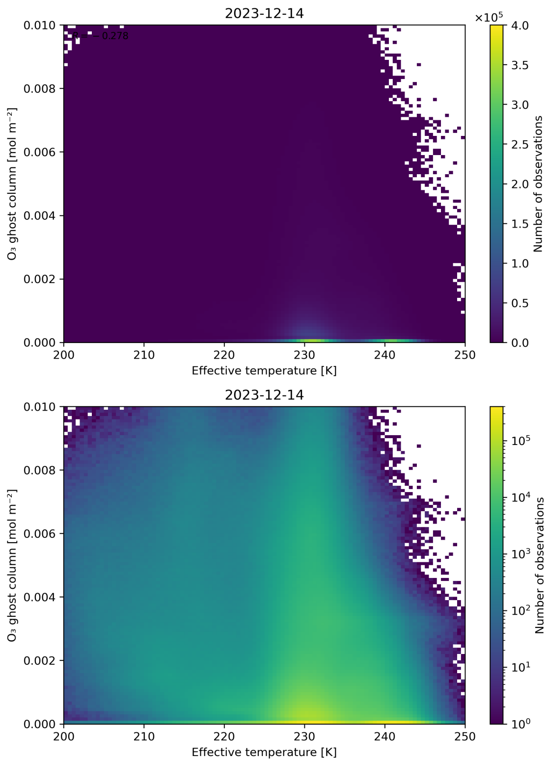
Figure 38: Scatter density plot of “Effective temperature” against “O 3 ghost column” for 2023-12-14 to 2023-12-15.
