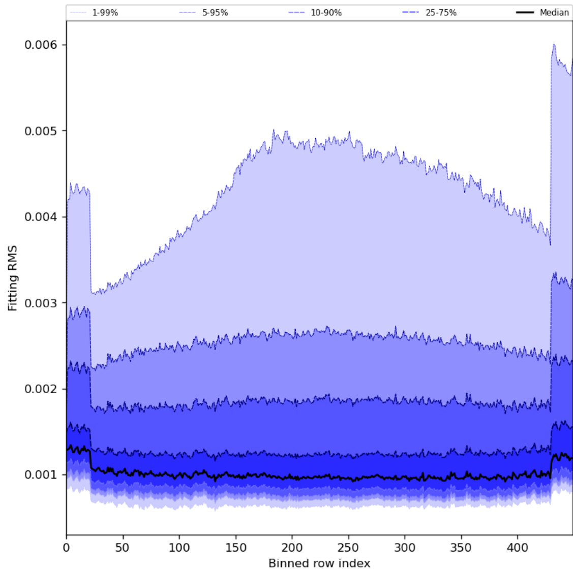
Figure 30: Along track statistics of “Fitting RMS” for 2023-12-14 to 2023-12-15
