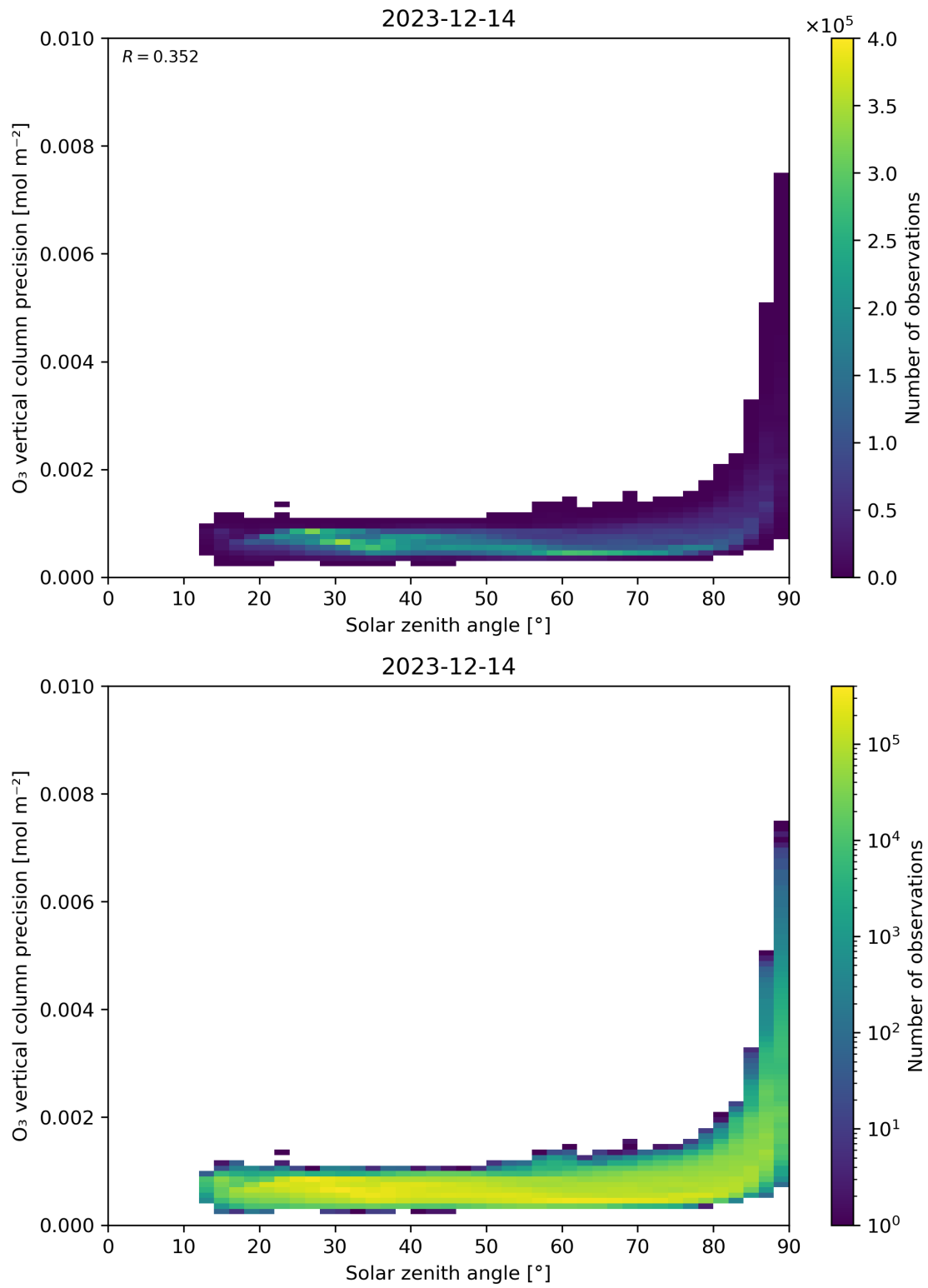
Figure 48: Scatter density plot of “Solar zenith angle” against “O 3 vertical column precision” for 2023-12-14 to 2023-12-15.
