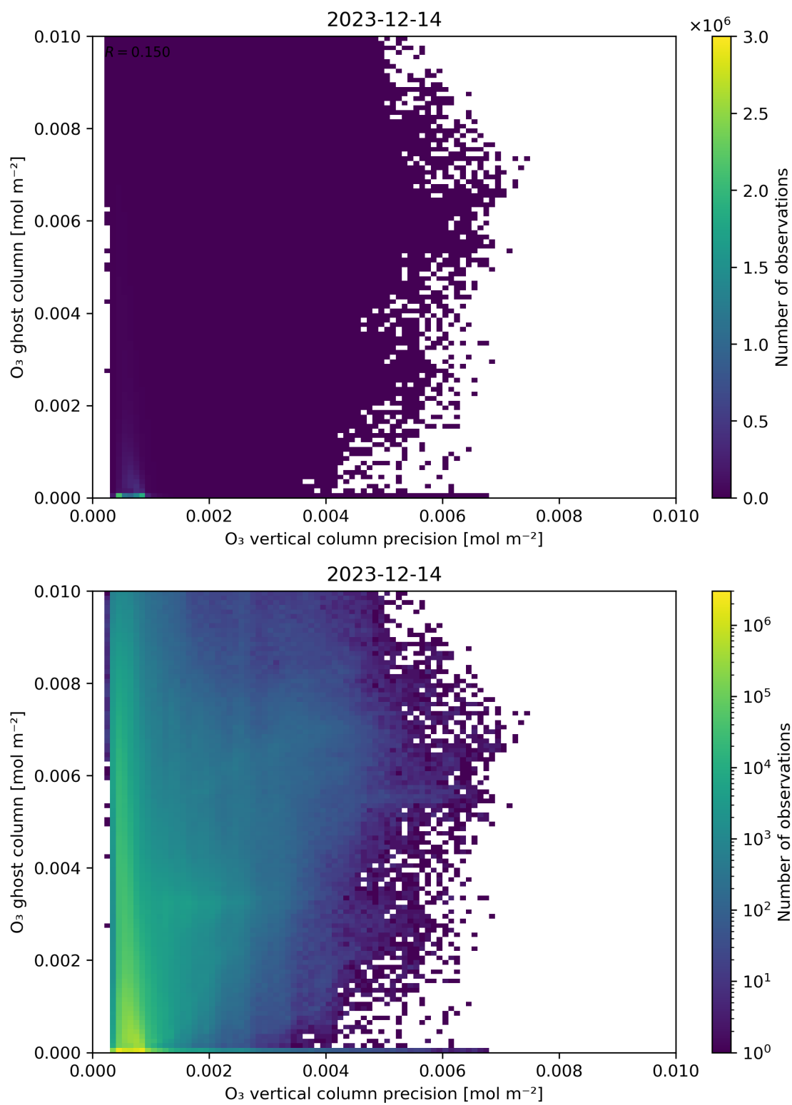
Figure 43: Scatter density plot of “ \text{O}_3 vertical column precision” against “ \text{O}_3 ghost column” for 2023-12-14 to 2023-12-15.
