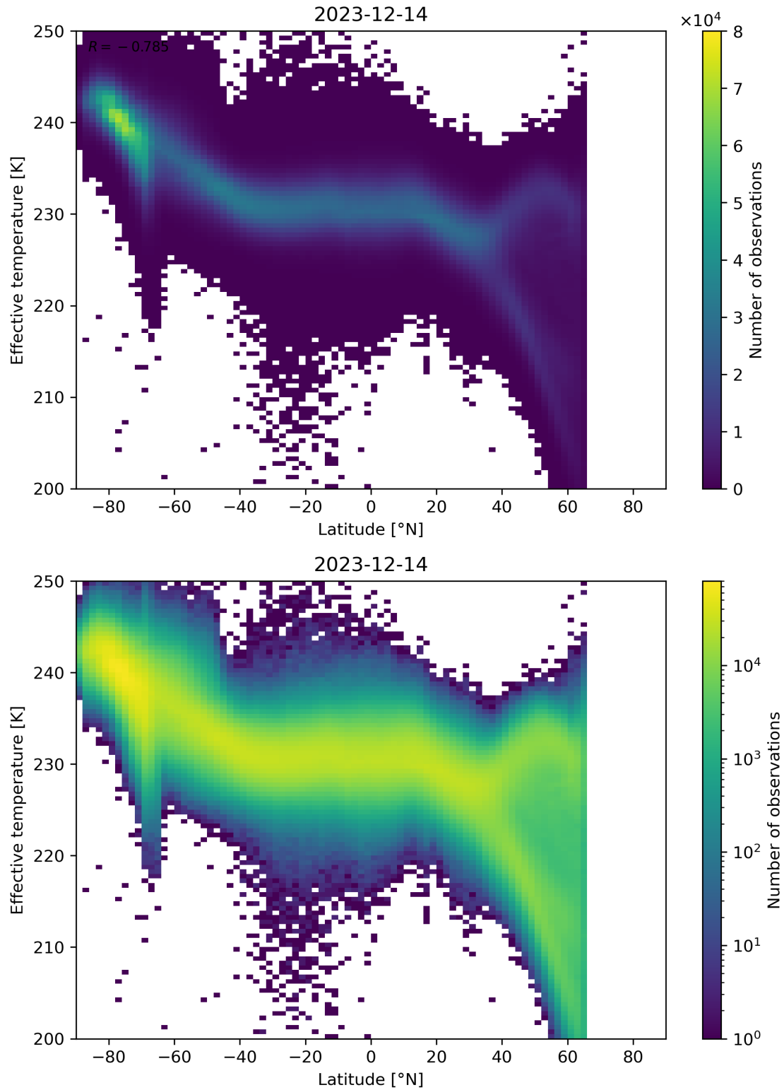
Figure 34: Scatter density plot of “Latitude” against “Effective temperature” for 2023-12-14 to 2023-12-15.
