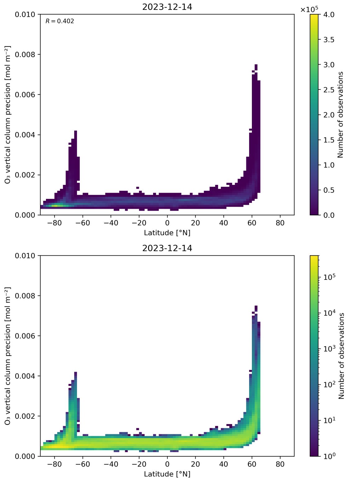
Figure 37: Scatter density plot of “Latitude” against “O 3 vertical column precision” for 2023-12-14 to 2023-12-15.
