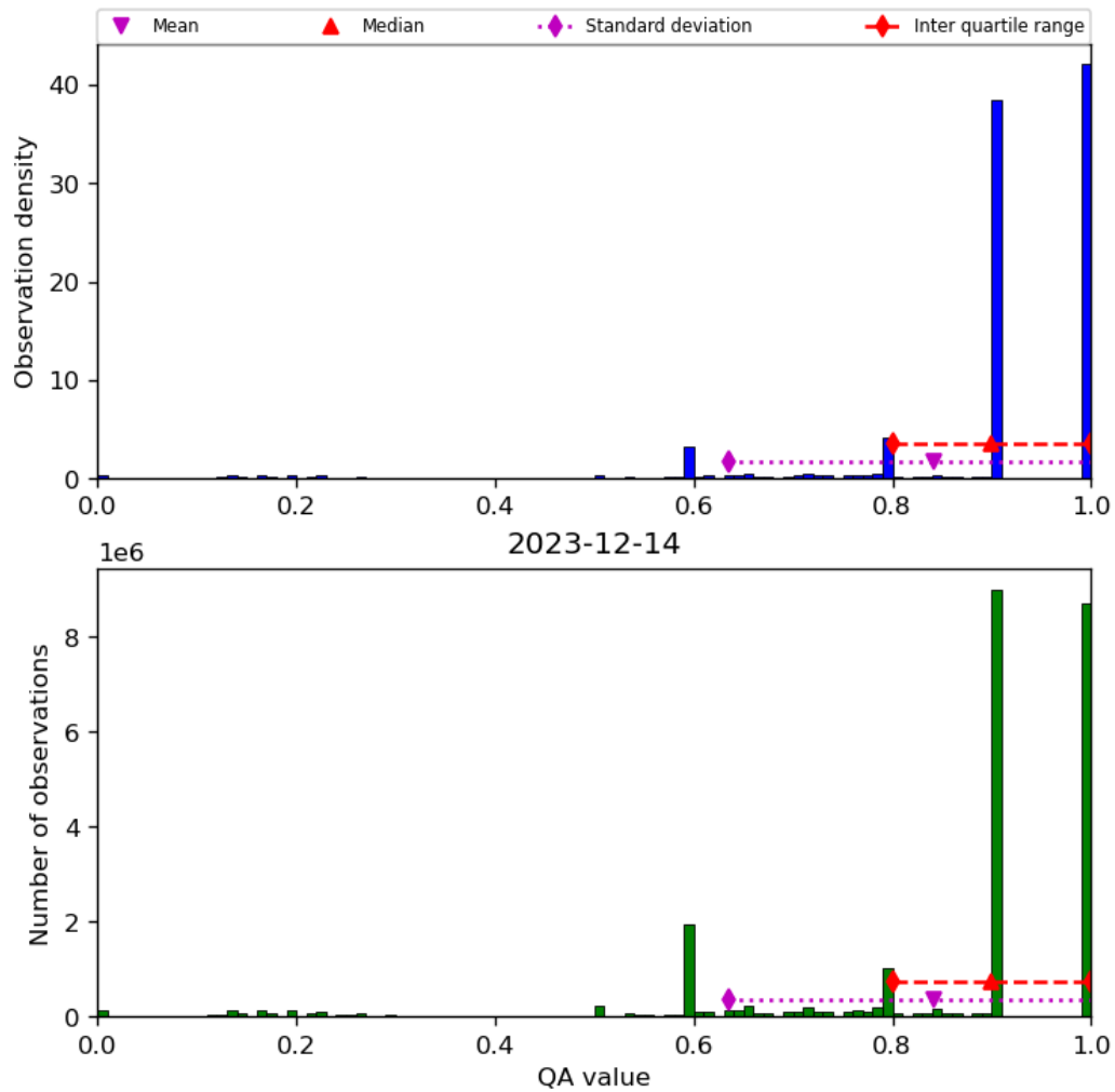
Figure 20: Histogram of “QA value” for 2023-12-14 to 2023-12-15
