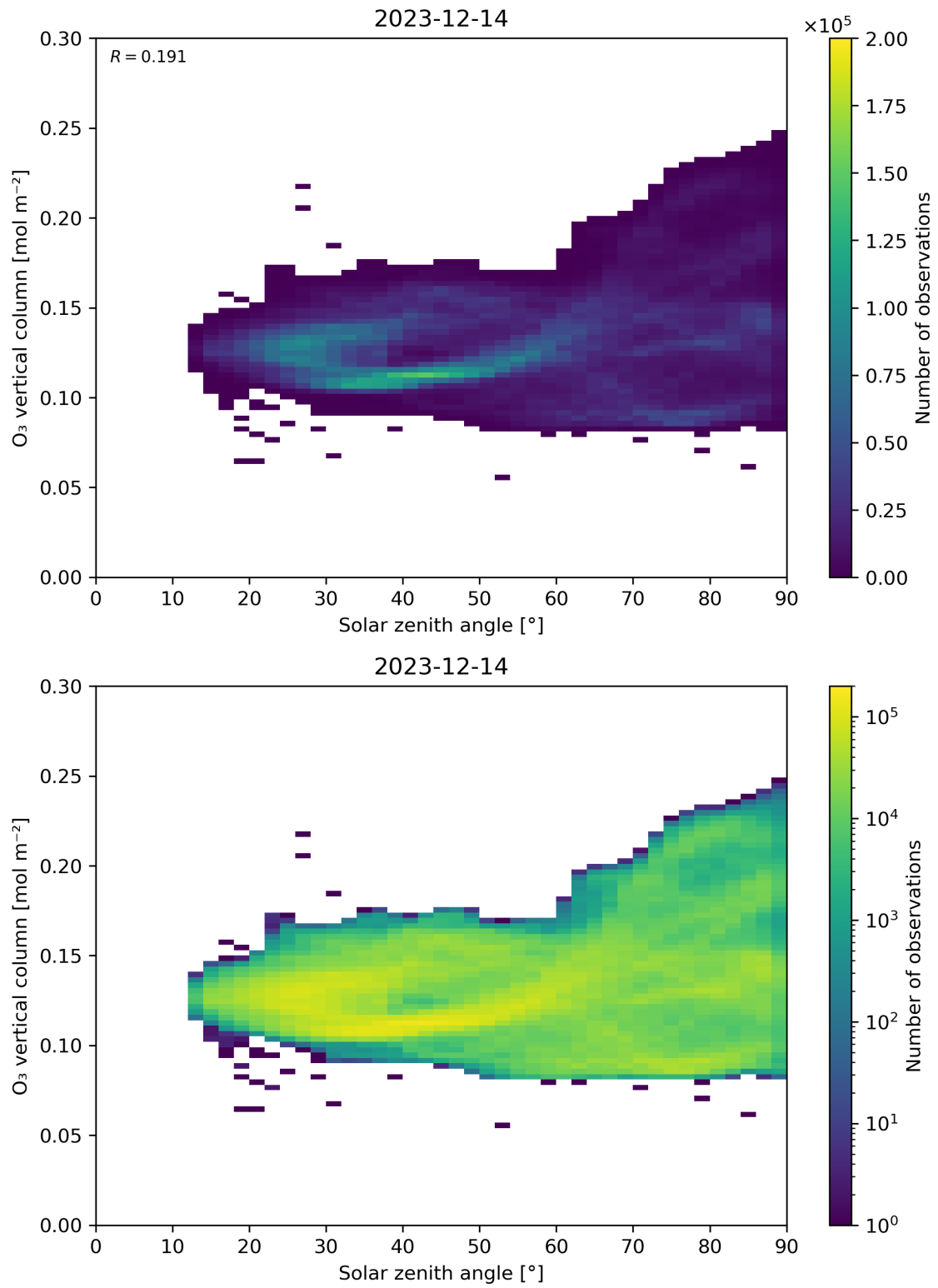
Figure 47: Scatter density plot of “Solar zenith angle” against “O 3 vertical column” for 2023-12-14 to 2023-12-15.
