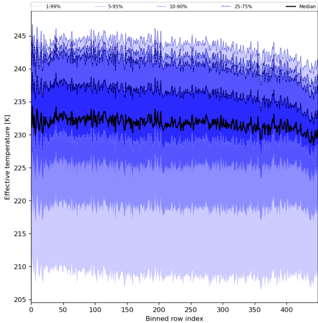
Figure 31: Along track statistics of “Effective temperature” for 2023-12-14 to 2023-12-15
