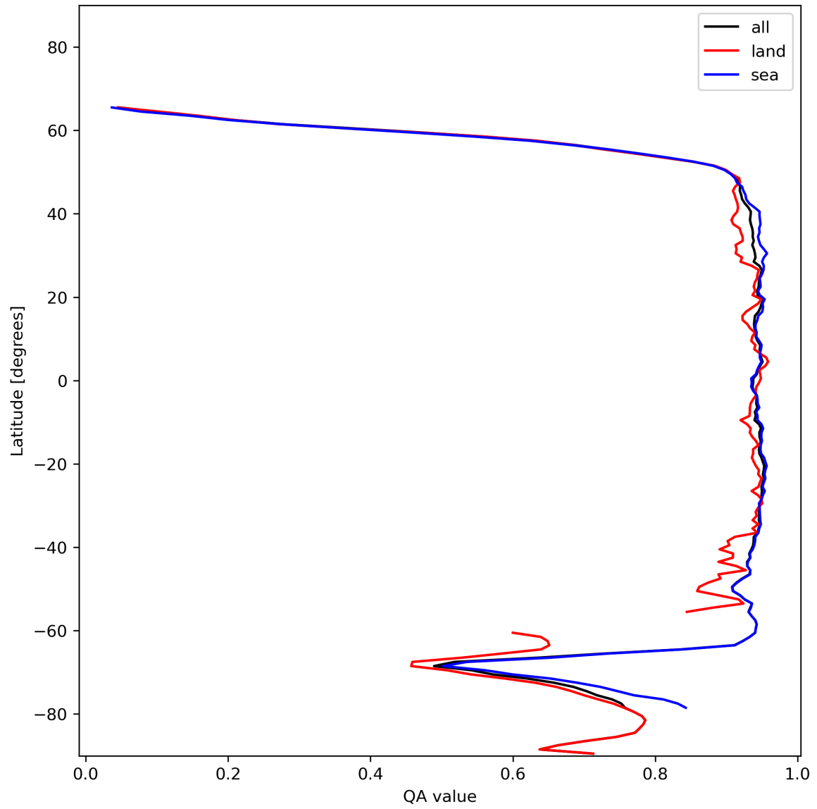
Figure 13: Zonal average of “QA value” for 2023-12-14 to 2023-12-15.
