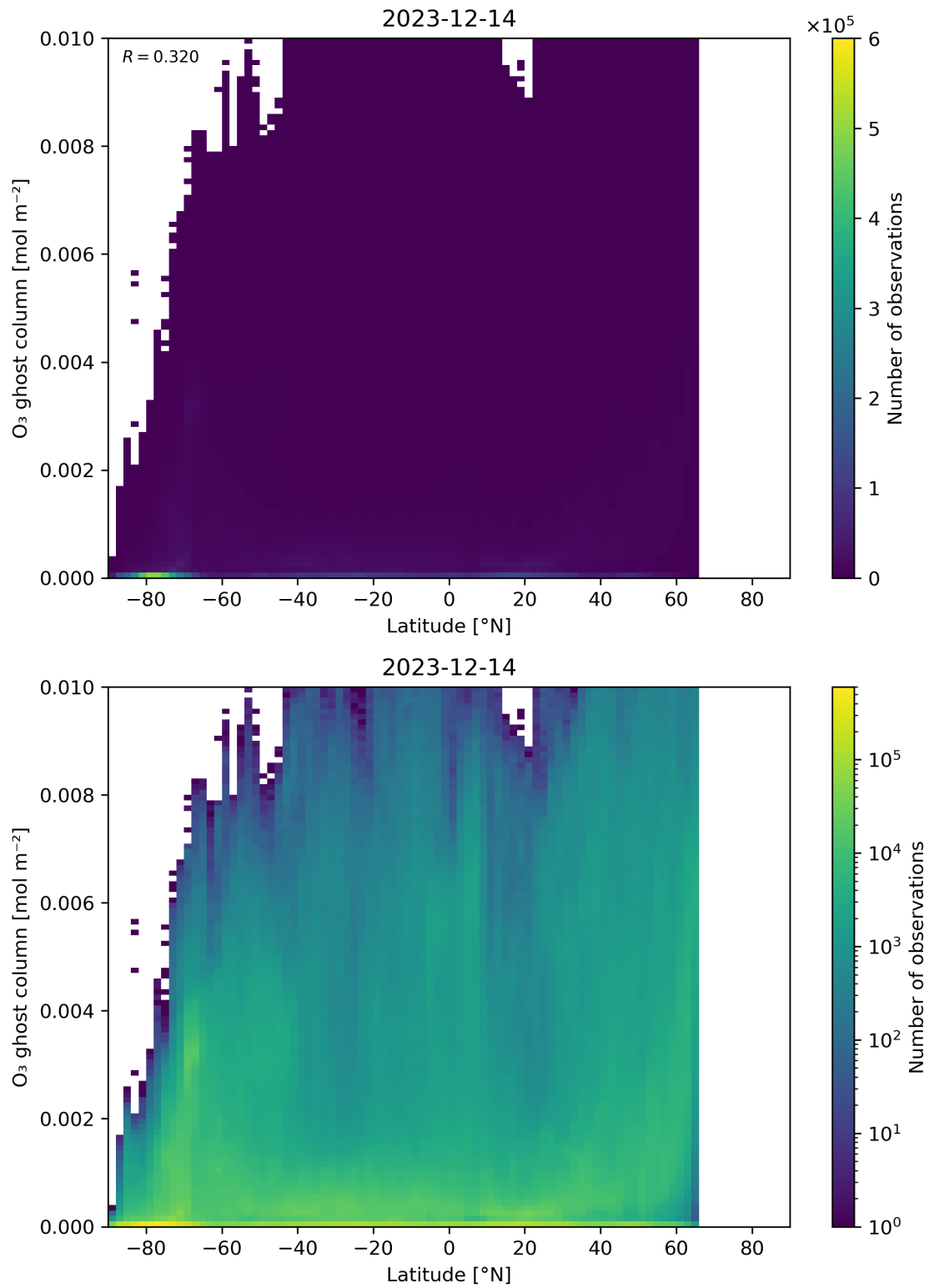
Figure 35: Scatter density plot of “Latitude” against “O 3 ghost column” for 2023-12-14 to 2023-12-15.
