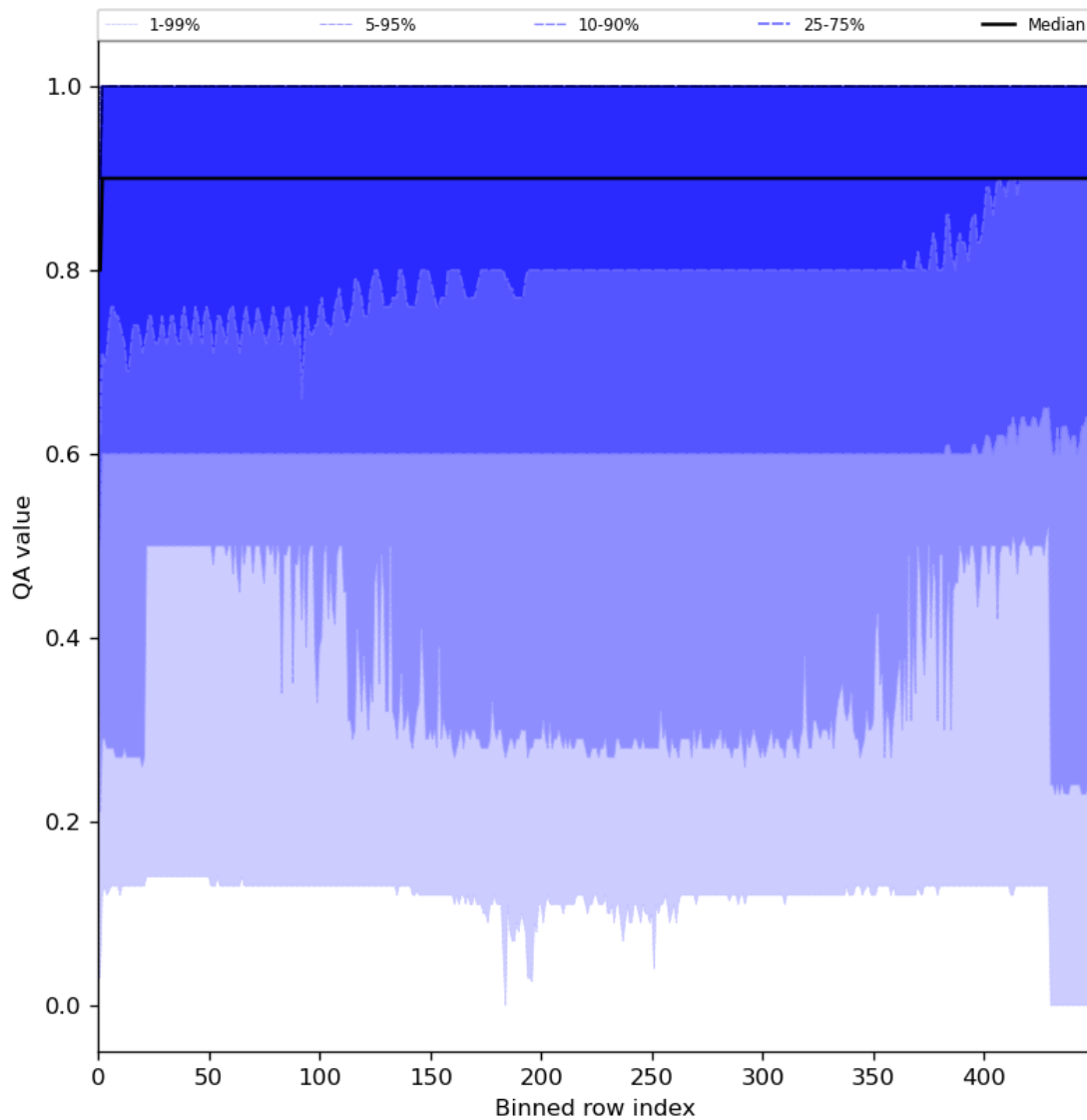
Figure 27: Along track statistics of “QA value” for 2023-12-14 to 2023-12-15
