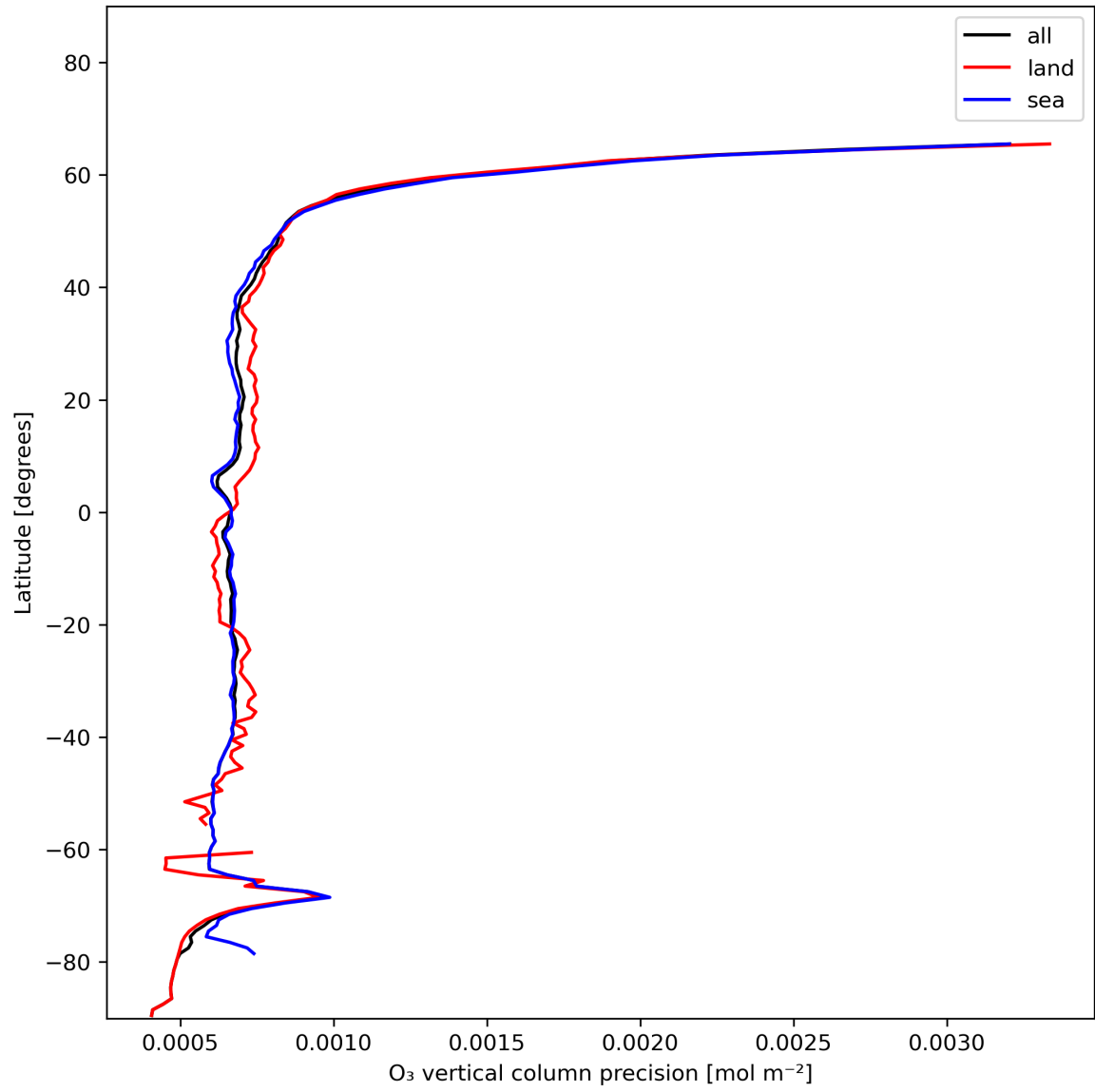
Figure 15: Zonal average of “O 3 vertical column precision” for 2023-12-14 to 2023-12-15.
