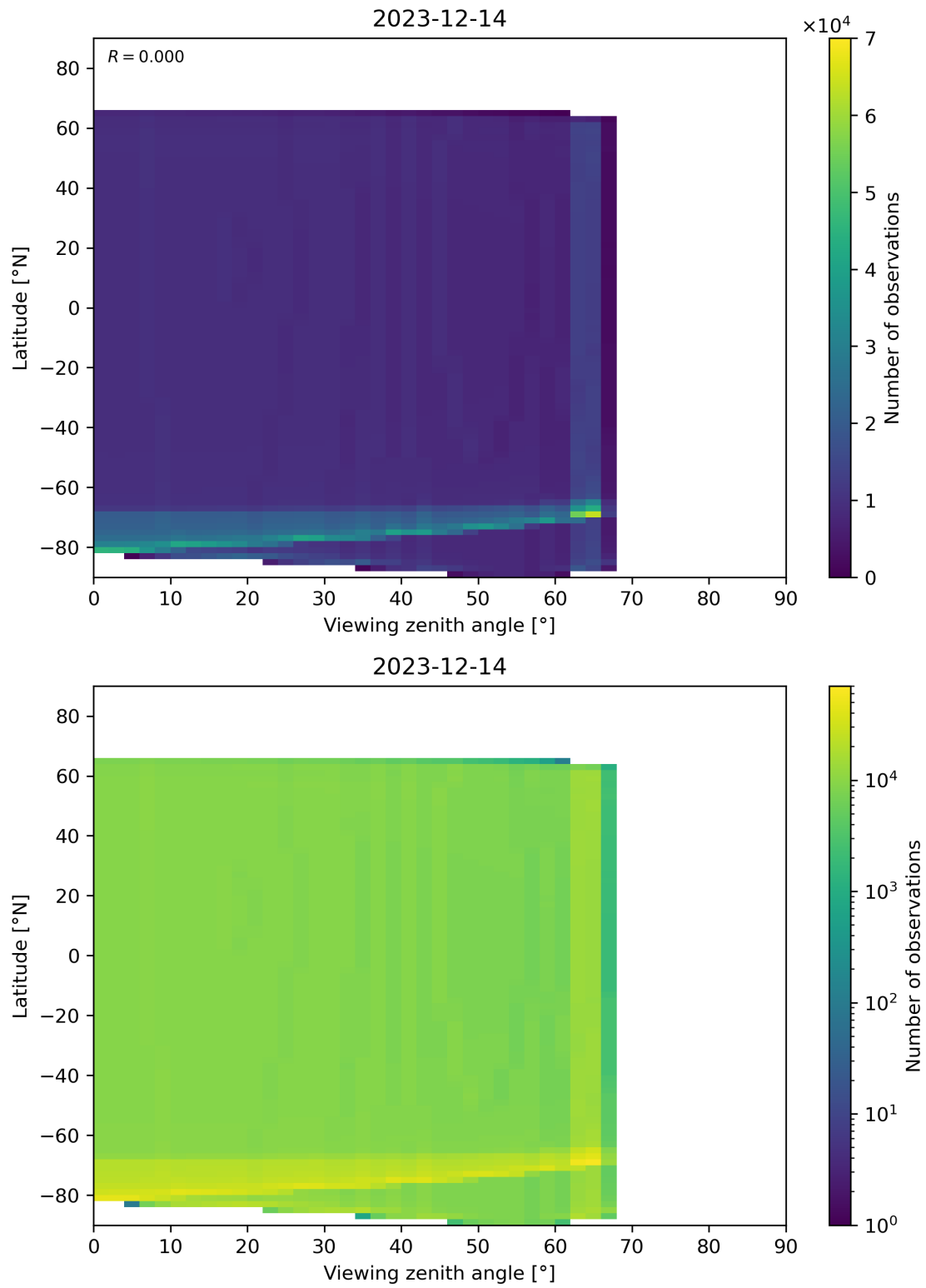
Figure 49: Scatter density plot of “Viewing zenith angle” against “Latitude” for 2023-12-14 to 2023-12-15.
