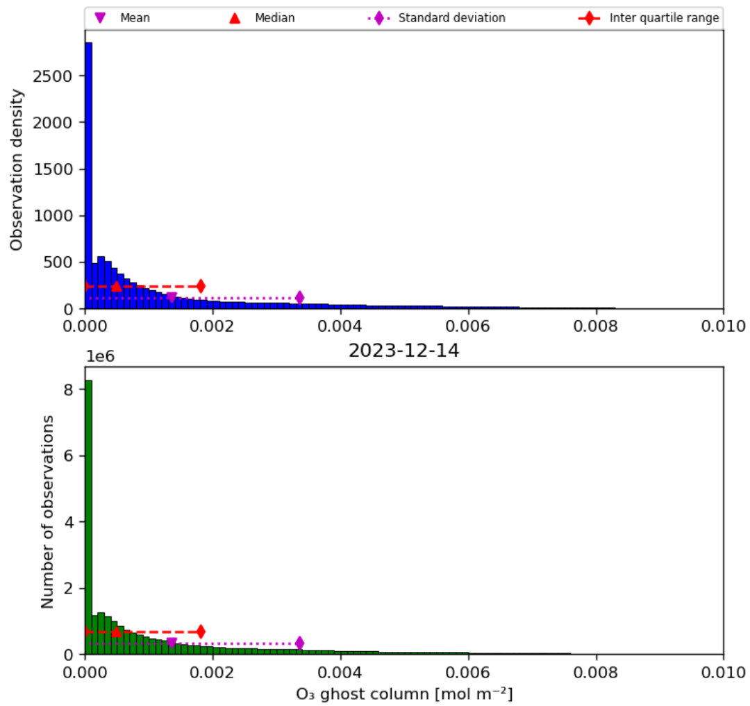
Figure 25: Histogram of “O 3 ghost column” for 2023-12-14 to 2023-12-15
