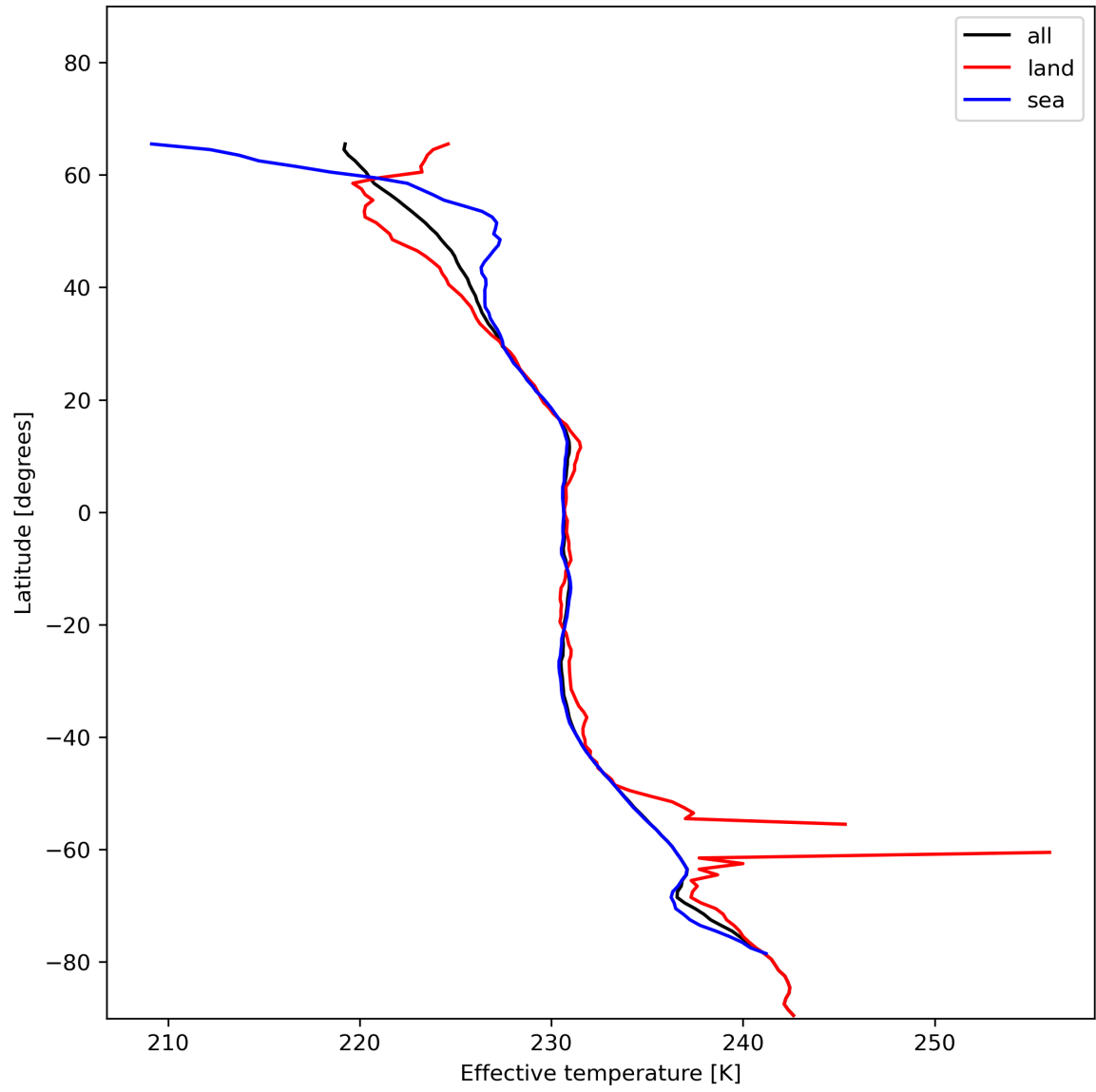
Figure 17: Zonal average of “Effective temperature” for 2023-12-14 to 2023-12-15.
