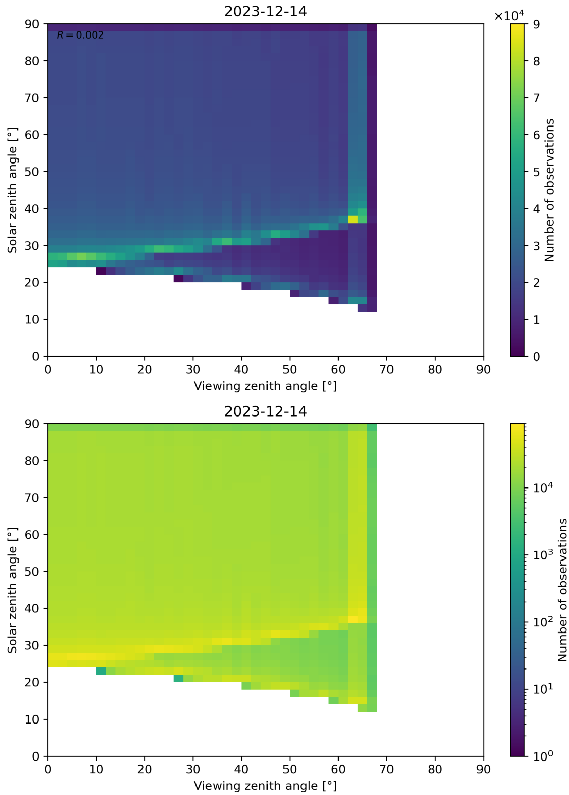
Figure 54: Scatter density plot of “Viewing zenith angle” against “Solar zenith angle” for 2023-12-14 to 2023-12-15.
