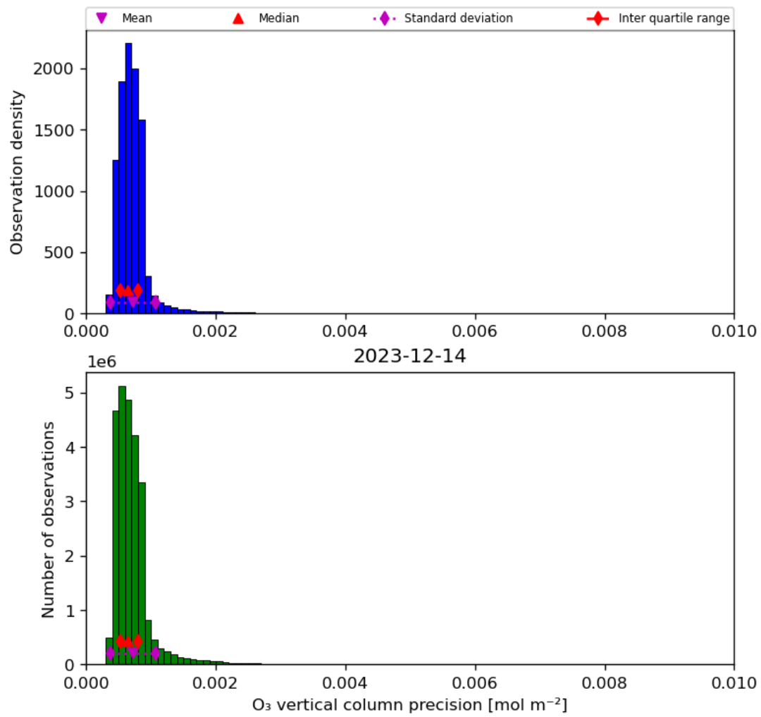
Figure 22: Histogram of “O 3 vertical column precision” for 2023-12-14 to 2023-12-15
