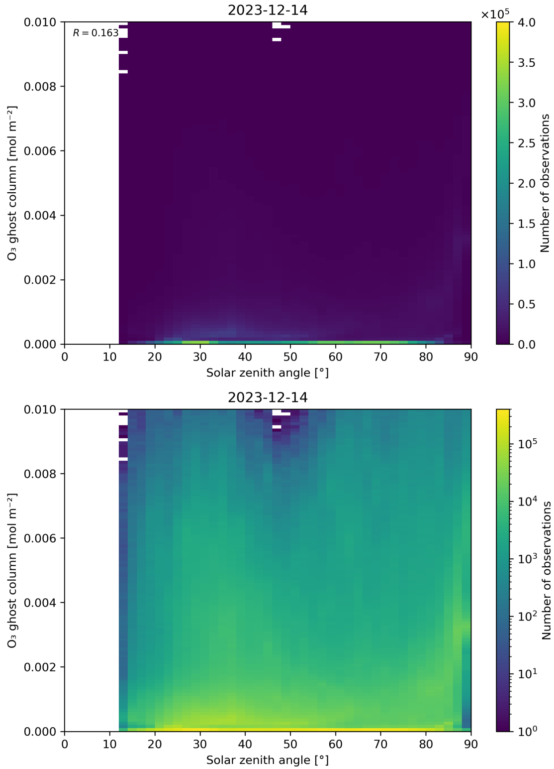
Figure 46: Scatter density plot of “Solar zenith angle” against “O 3 ghost column” for 2023-12-14 to 2023-12-15.
