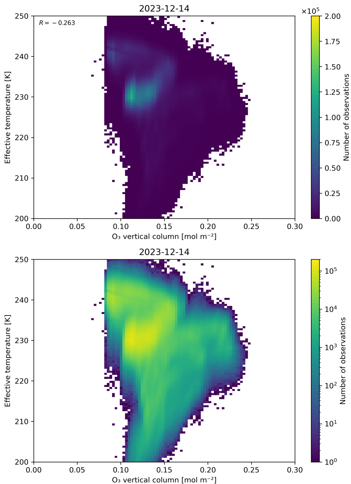
Figure 39: Scatter density plot of “O 3 vertical column” against “Effective temperature” for 2023-12-14 to 2023-12-15.
