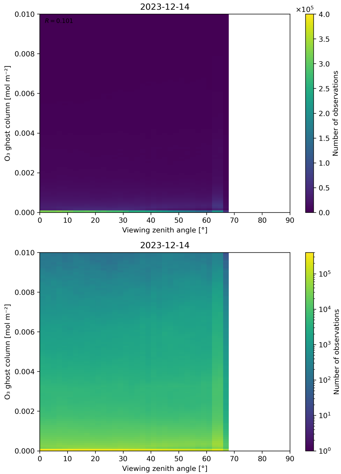
Figure 51: Scatter density plot of “Viewing zenith angle” against “O 3 ghost column” for 2023-12-14 to 2023-12-15.
