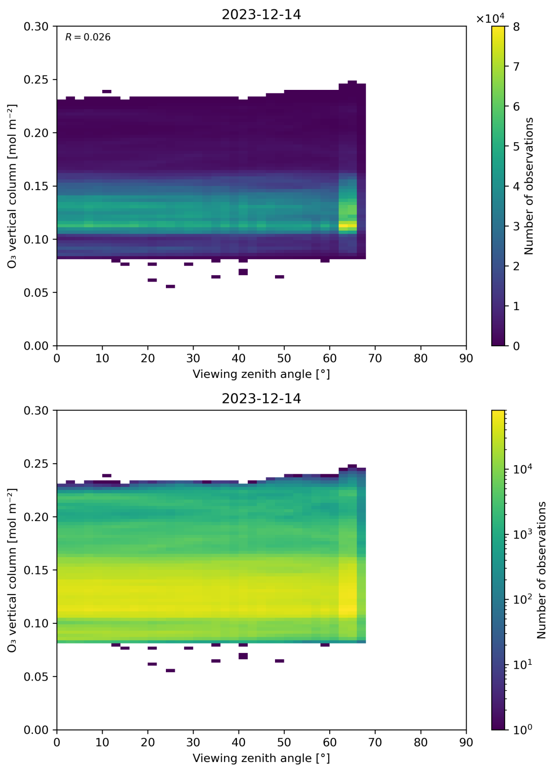
Figure 52: Scatter density plot of “Viewing zenith angle” against “O 3 vertical column” for 2023-12-14 to 2023-12-15.
