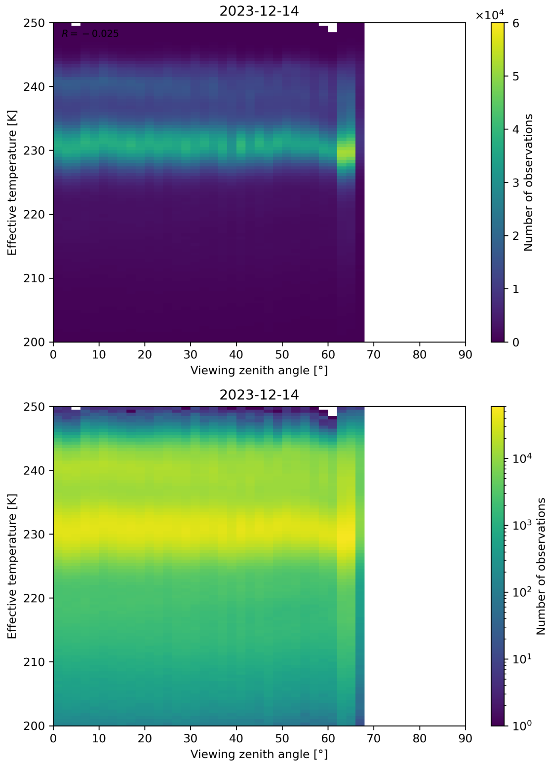
Figure 50: Scatter density plot of “Viewing zenith angle” against “Effective temperature” for 2023-12-14 to 2023-12-15.
