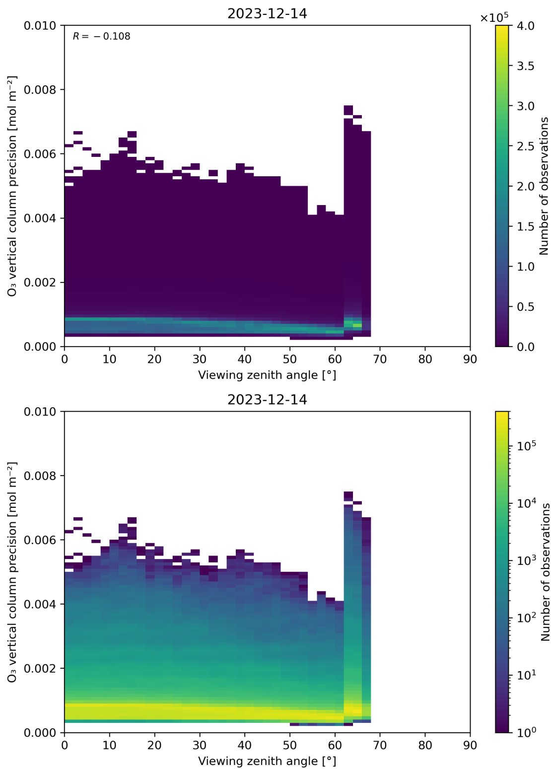
Figure 53: Scatter density plot of “Viewing zenith angle” against “O 3 vertical column precision” for 2023-12-14 to 2023-12-15.
