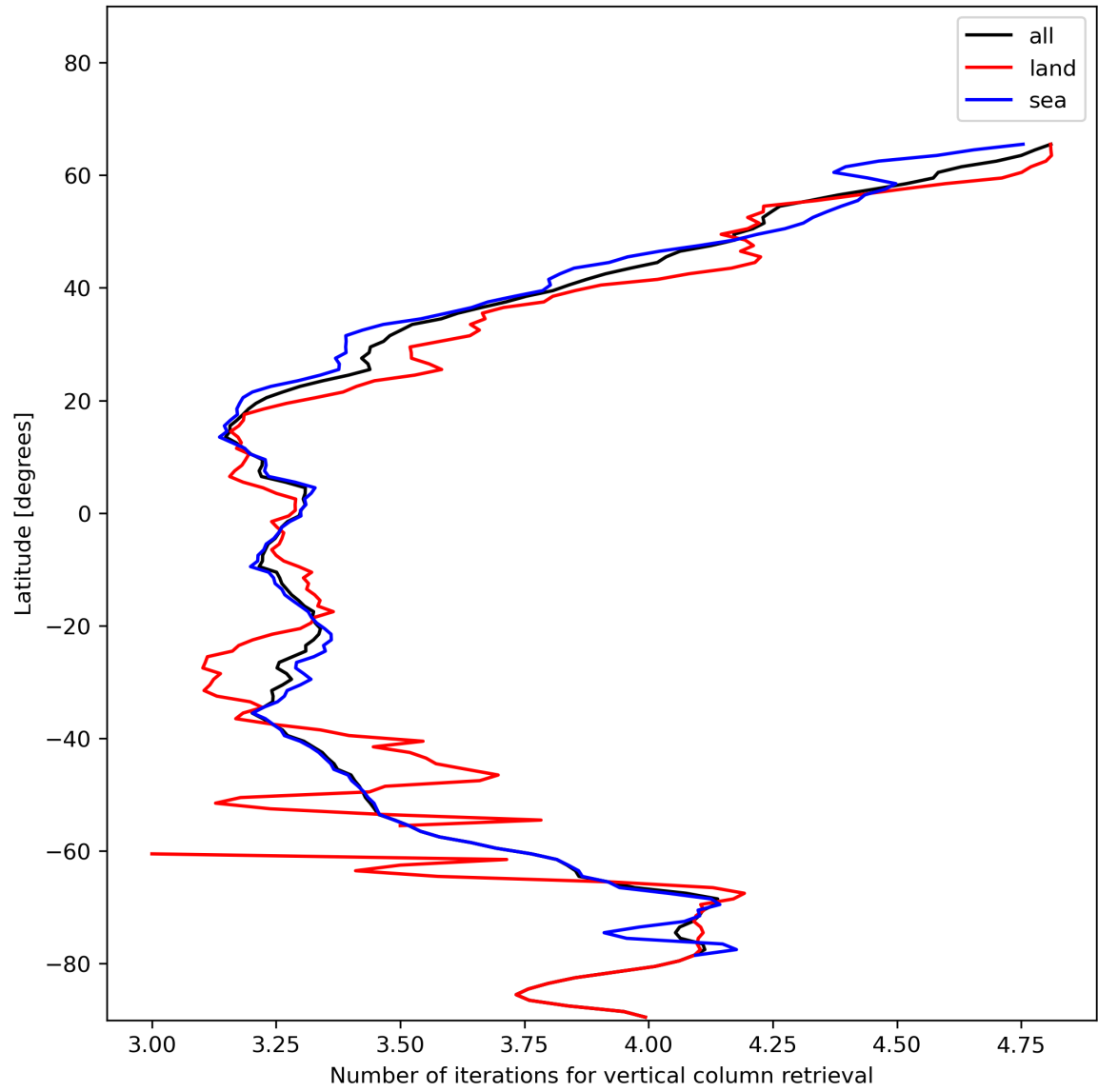
Figure 19: Zonal average of “Number of iterations for vertical column retrieval” for 2023-12-14 to 2023-12-15.
