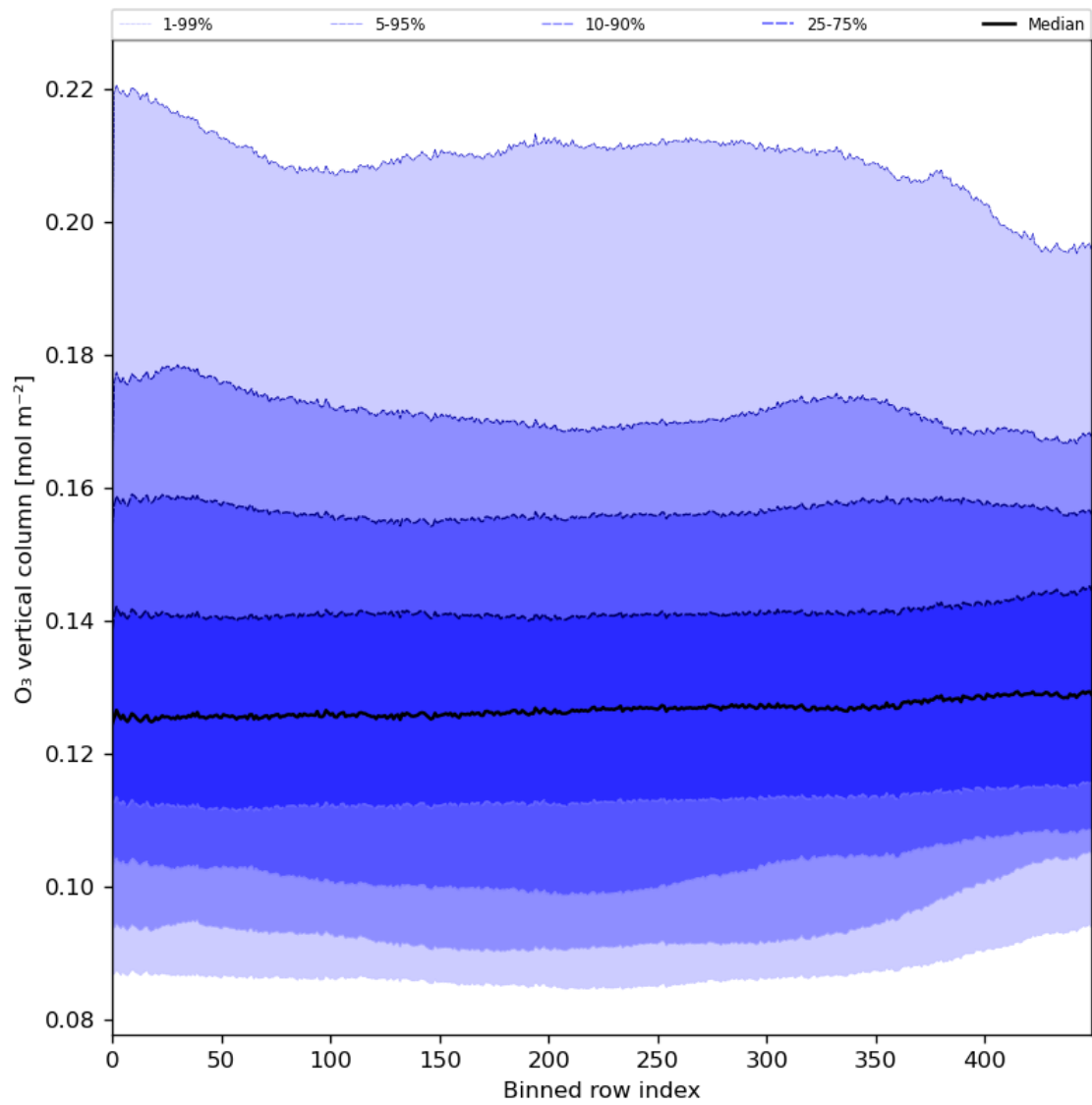
Figure 28: Along track statistics of “O 3 vertical column” for 2023-12-14 to 2023-12-15
