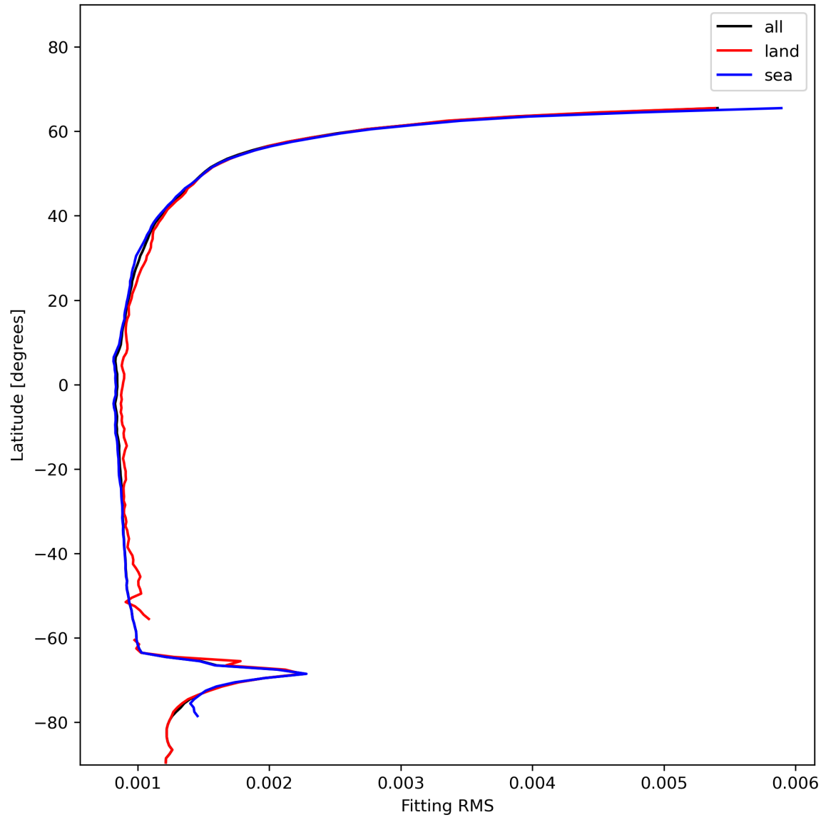
Figure 16: Zonal average of “Fitting RMS” for 2023-12-14 to 2023-12-15.
