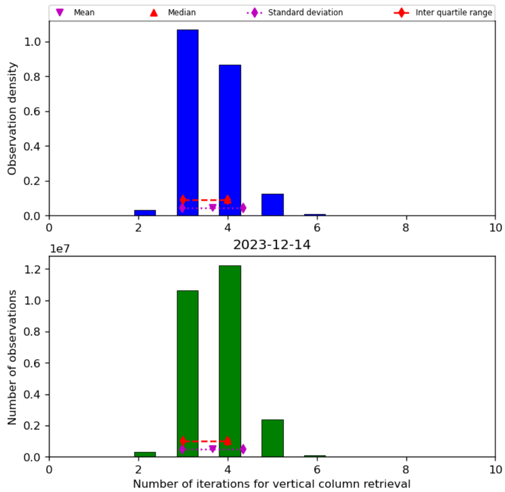
Figure 26: Histogram of “Number of iterations for vertical column retrieval” for 2023-12-14 to 2023-12-15
