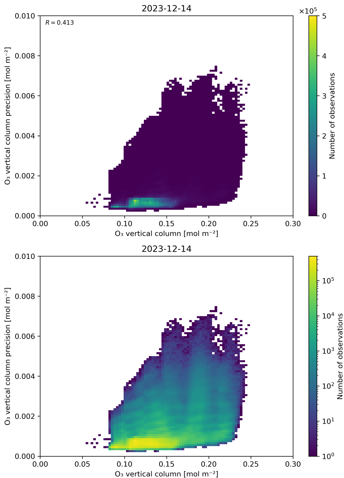
Figure 41: Scatter density plot of “O 3 vertical column” against “O 3 vertical column precision” for 2023-12-14 to 2023-12-15.
