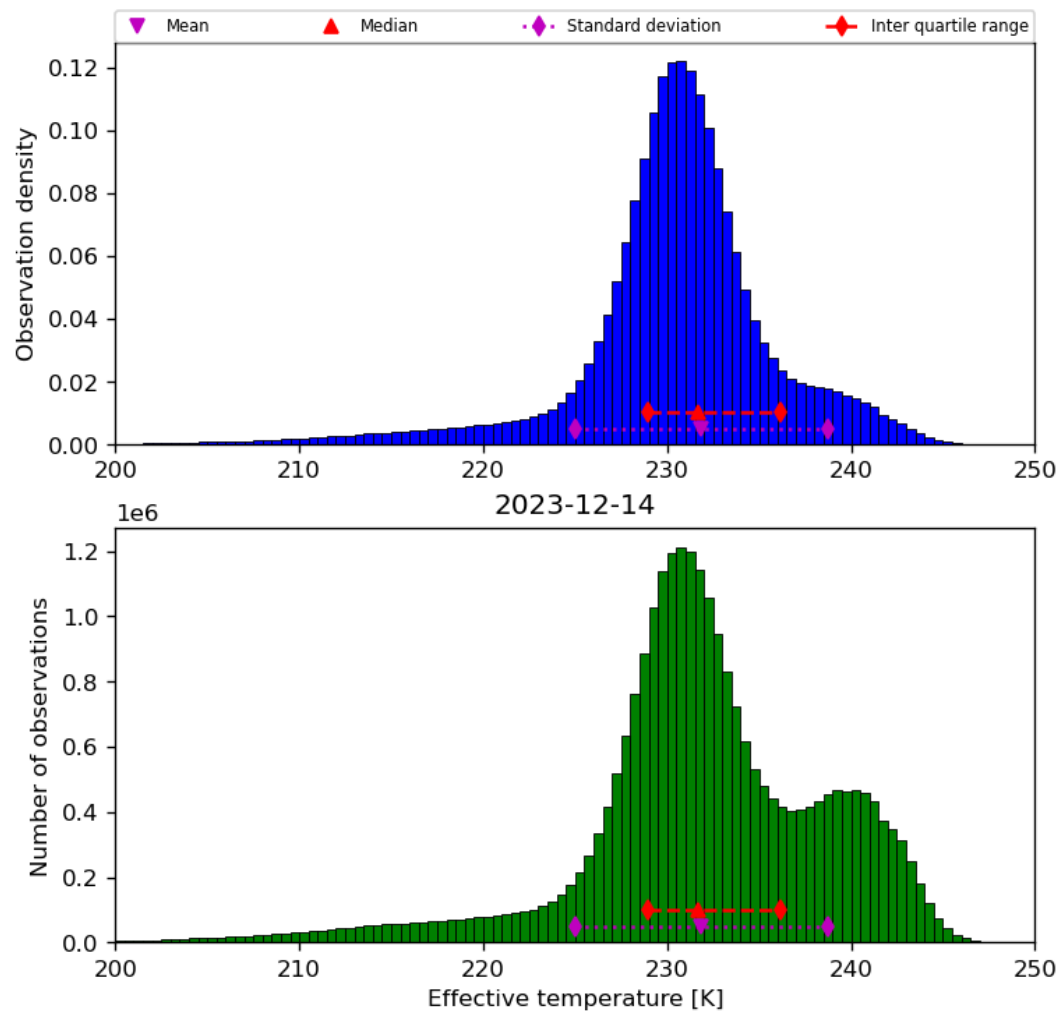
Figure 24: Histogram of “Effective temperature” for 2023-12-14 to 2023-12-15
