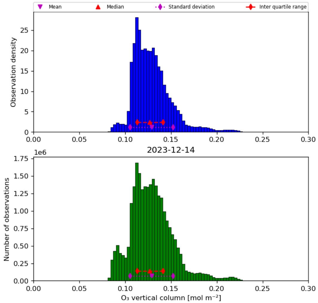
Figure 21: Histogram of “O 3 vertical column” for 2023-12-14 to 2023-12-15
