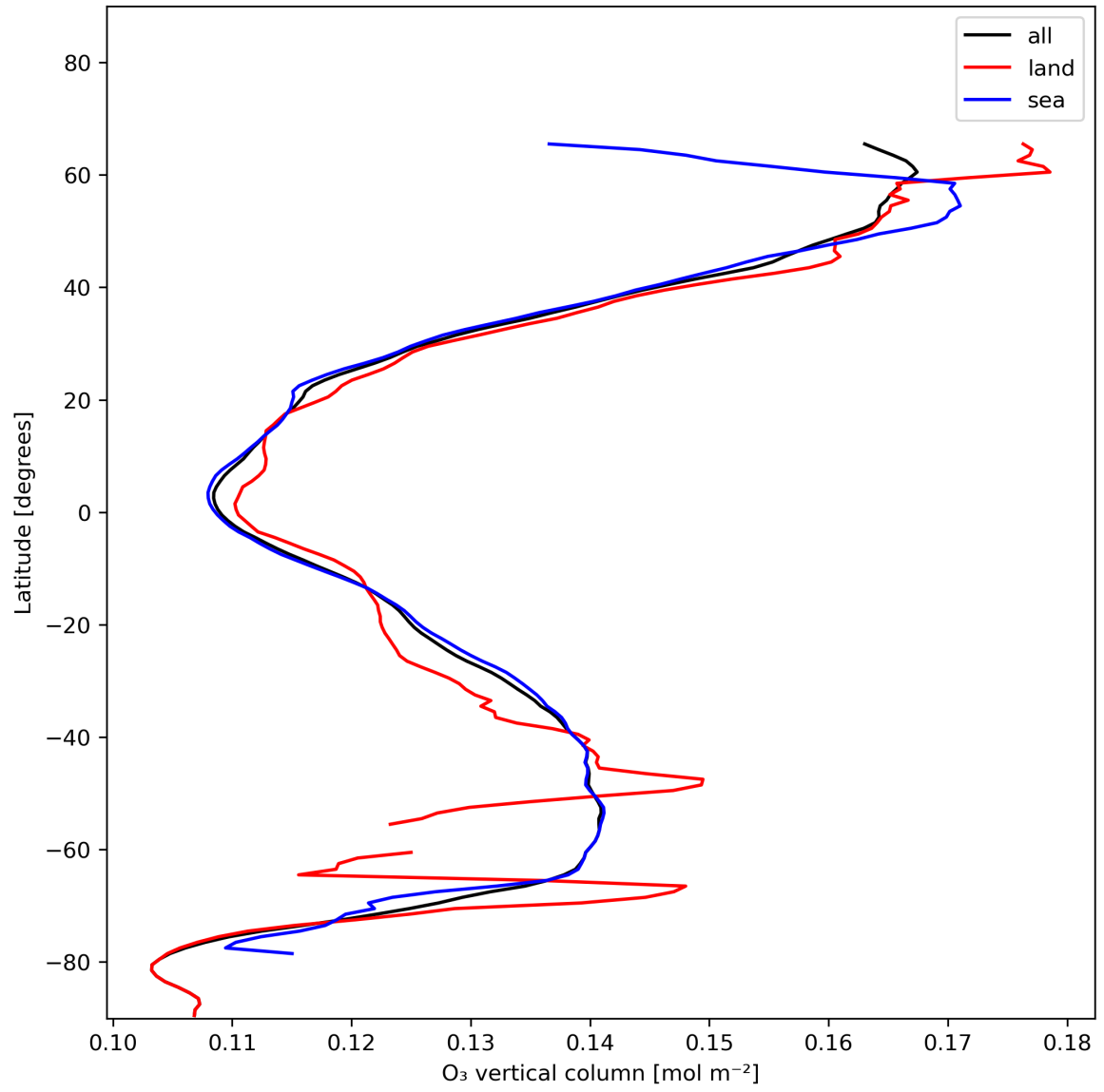
Figure 14: Zonal average of “O 3 vertical column” for 2023-12-14 to 2023-12-15.
