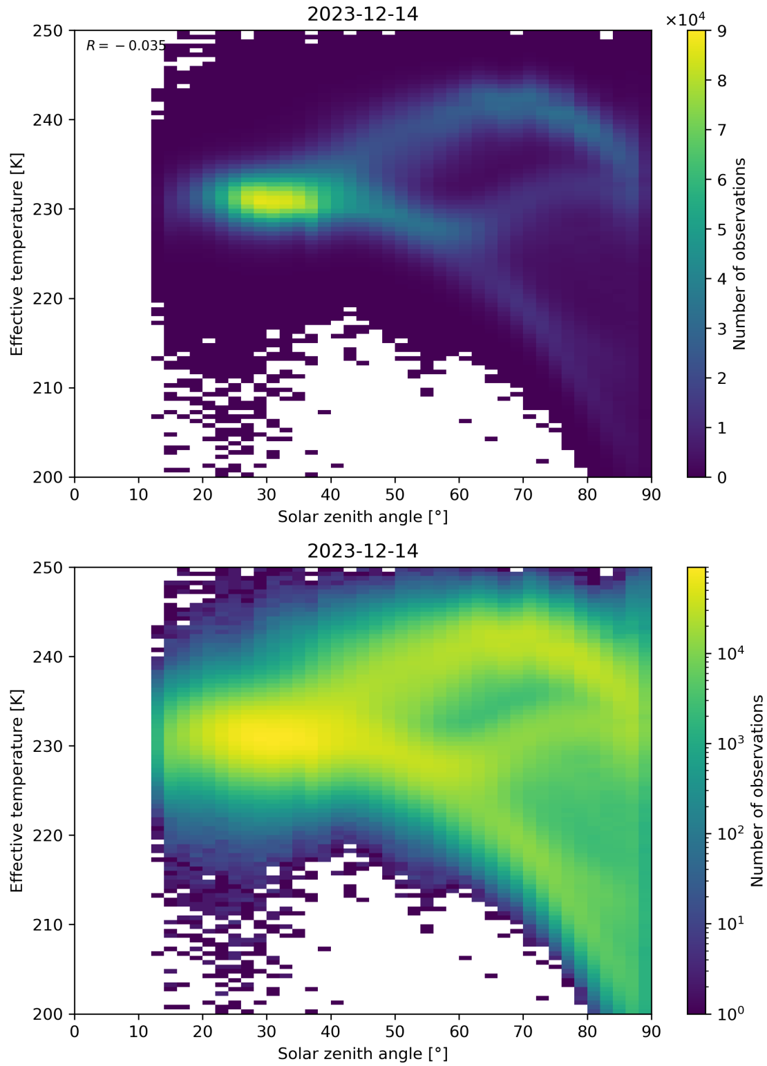
Figure 45: Scatter density plot of “Solar zenith angle” against “Effective temperature” for 2023-12-14 to 2023-12-15.
