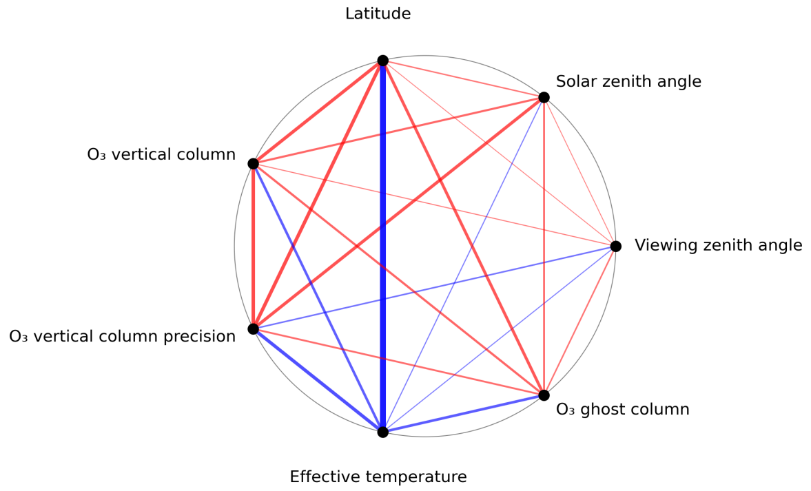
Figure 1: Map of correlation graph for 2023-12-14 to 2023-12-15.
