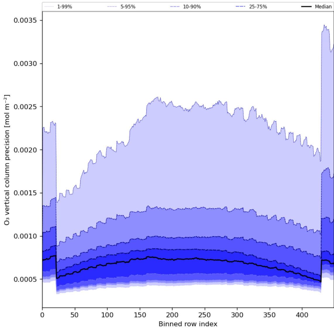
Figure 29: Along track statistics of “O 3 vertical column precision” for 2023-12-14 to 2023-12-15
