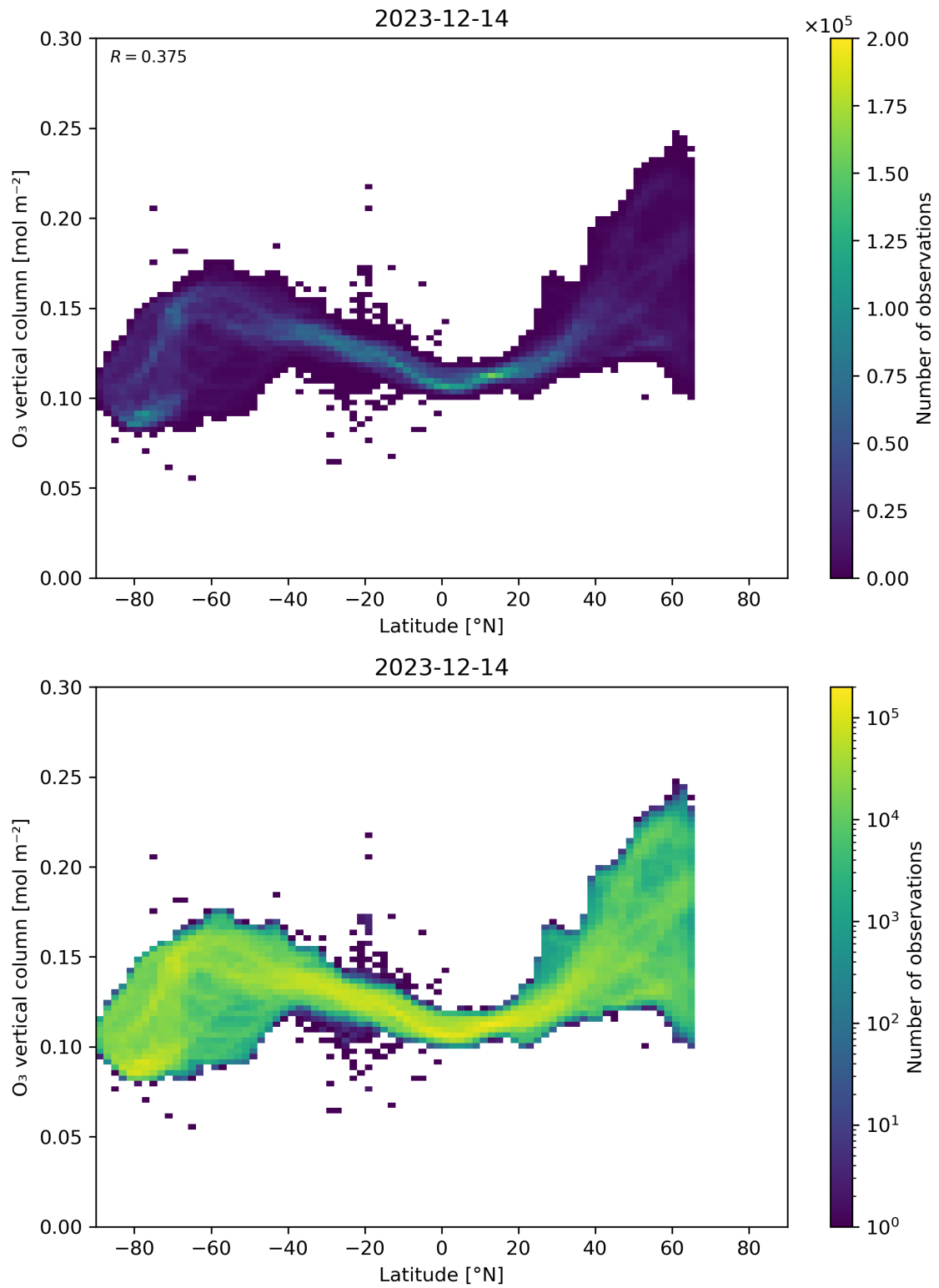
Figure 36: Scatter density plot of “Latitude” against “O 3 vertical column” for 2023-12-14 to 2023-12-15.
