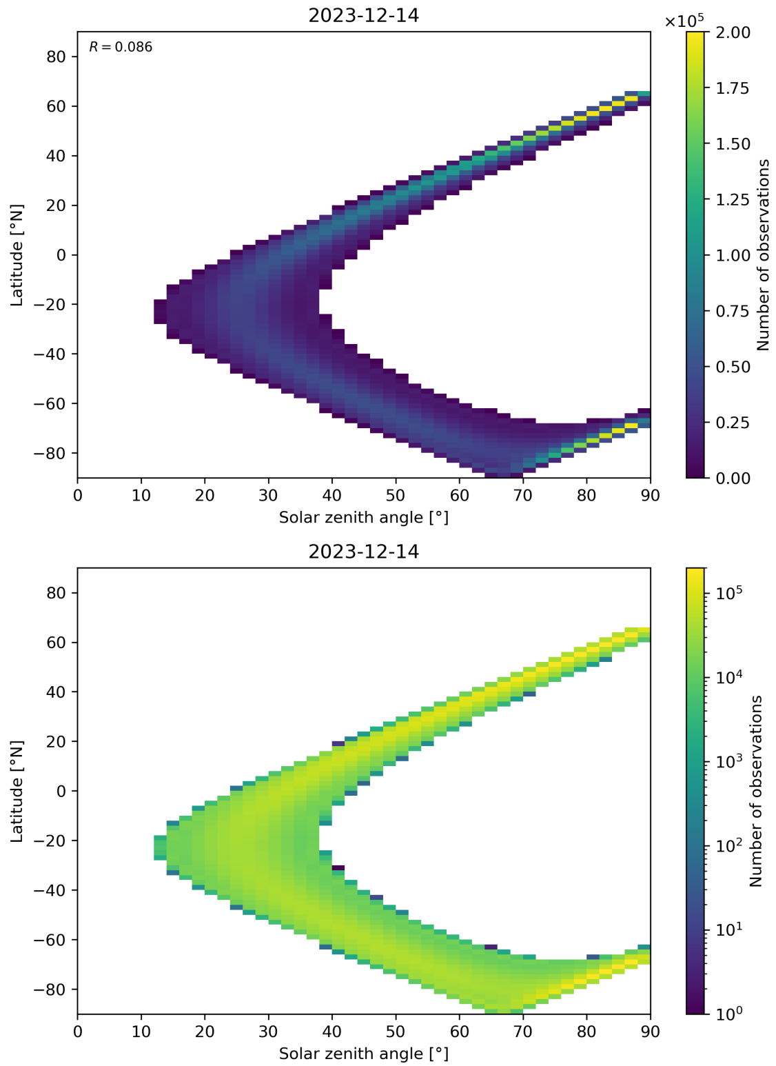
Figure 44: Scatter density plot of “Solar zenith angle” against “Latitude” for 2023-12-14 to 2023-12-15.
