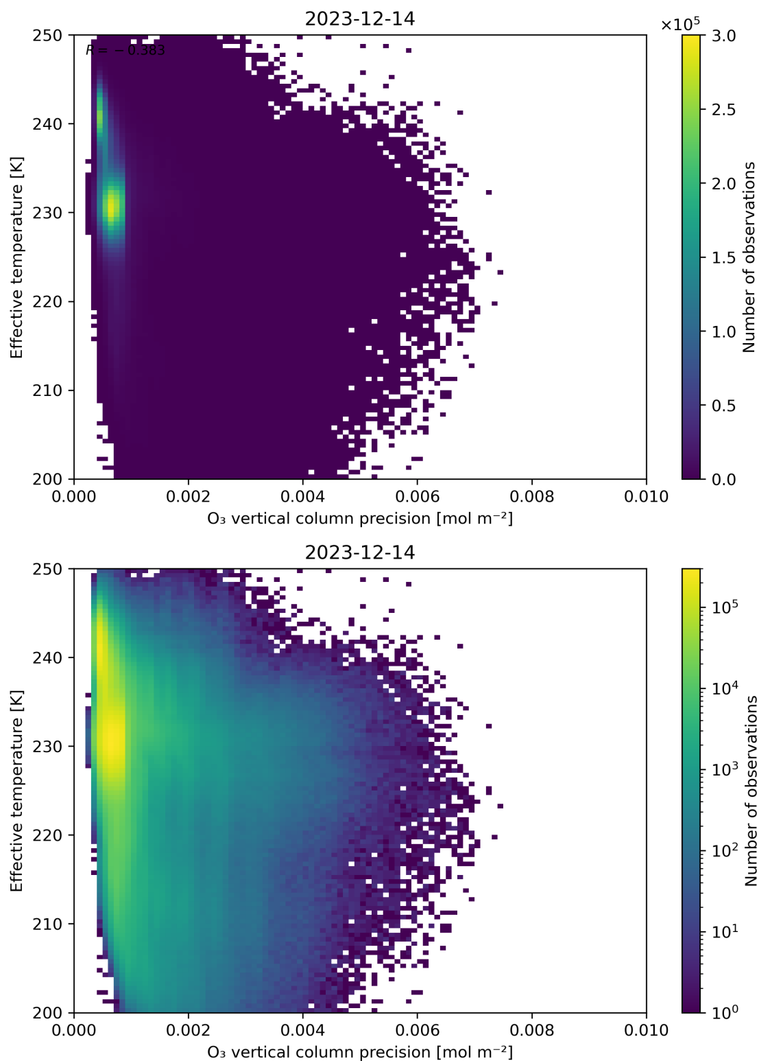
Figure 42: Scatter density plot of “O 3 vertical column precision” against “Effective temperature” for 2023-12-14 to 2023-12-15.
