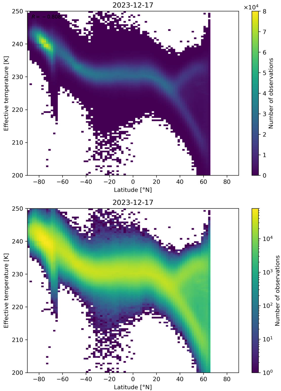
Figure 34: Scatter density plot of “Latitude” against “Effective temperature” for 2023-12-16 to 2023-12-18.
