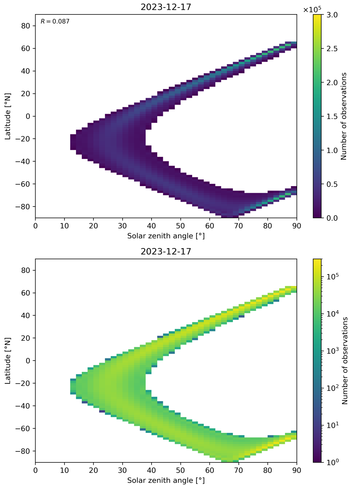
Figure 44: Scatter density plot of “Solar zenith angle” against “Latitude” for 2023-12-16 to 2023-12-18.
