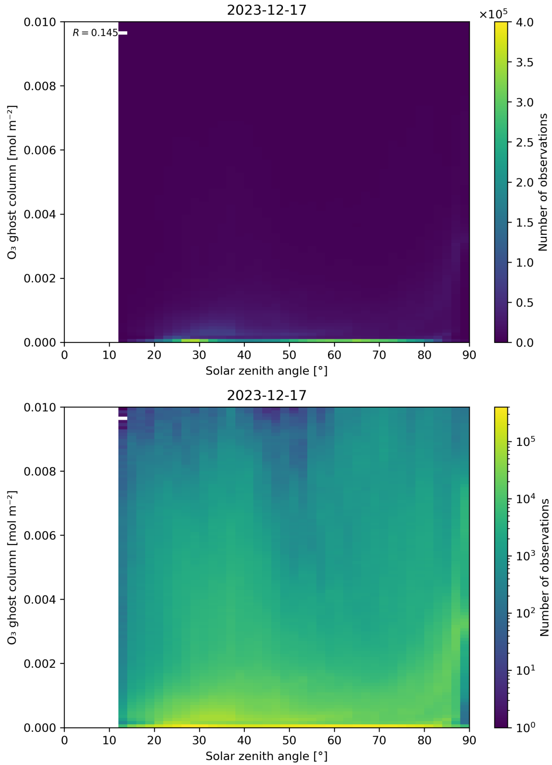
Figure 46: Scatter density plot of “Solar zenith angle” against “O 3 ghost column” for 2023-12-16 to 2023-12-18.
