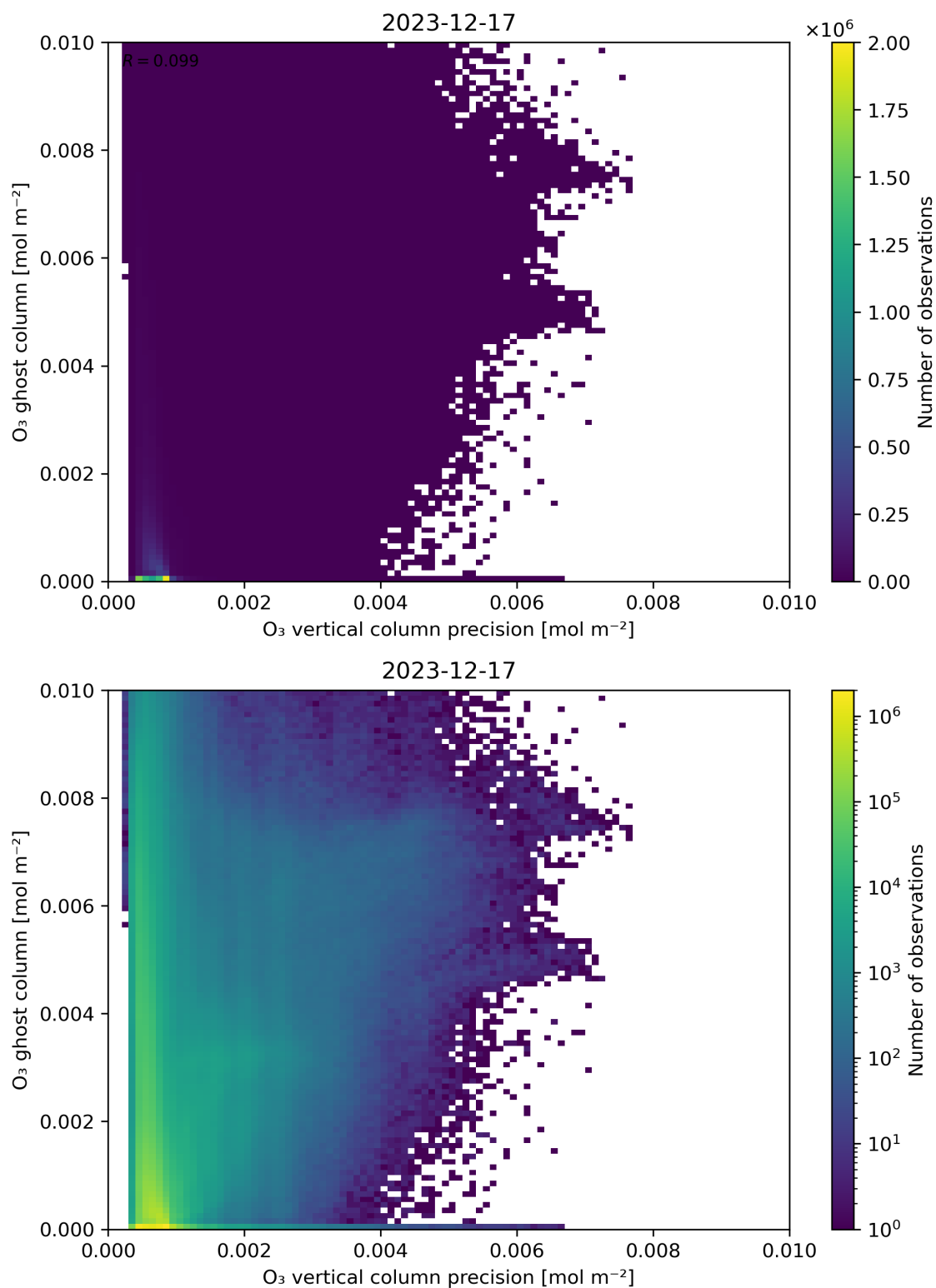
Figure 43: Scatter density plot of “ \text{O}_3 vertical column precision” against “ \text{O}_3 ghost column” for 2023-12-16 to 2023-12-18.
