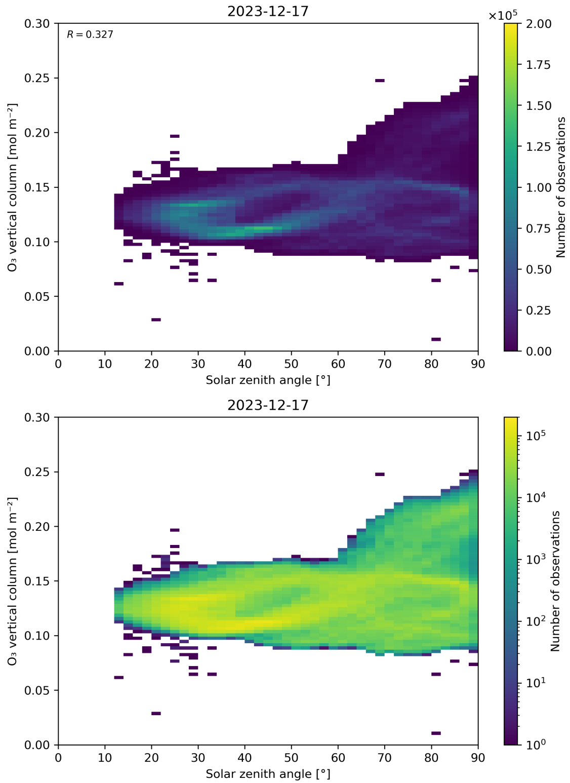
Figure 47: Scatter density plot of “Solar zenith angle” against “O 3 vertical column” for 2023-12-16 to 2023-12-18.
