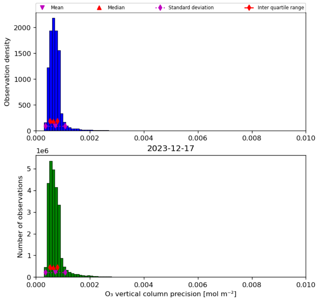
Figure 22: Histogram of “O 3 vertical column precision” for 2023-12-16 to 2023-12-18
