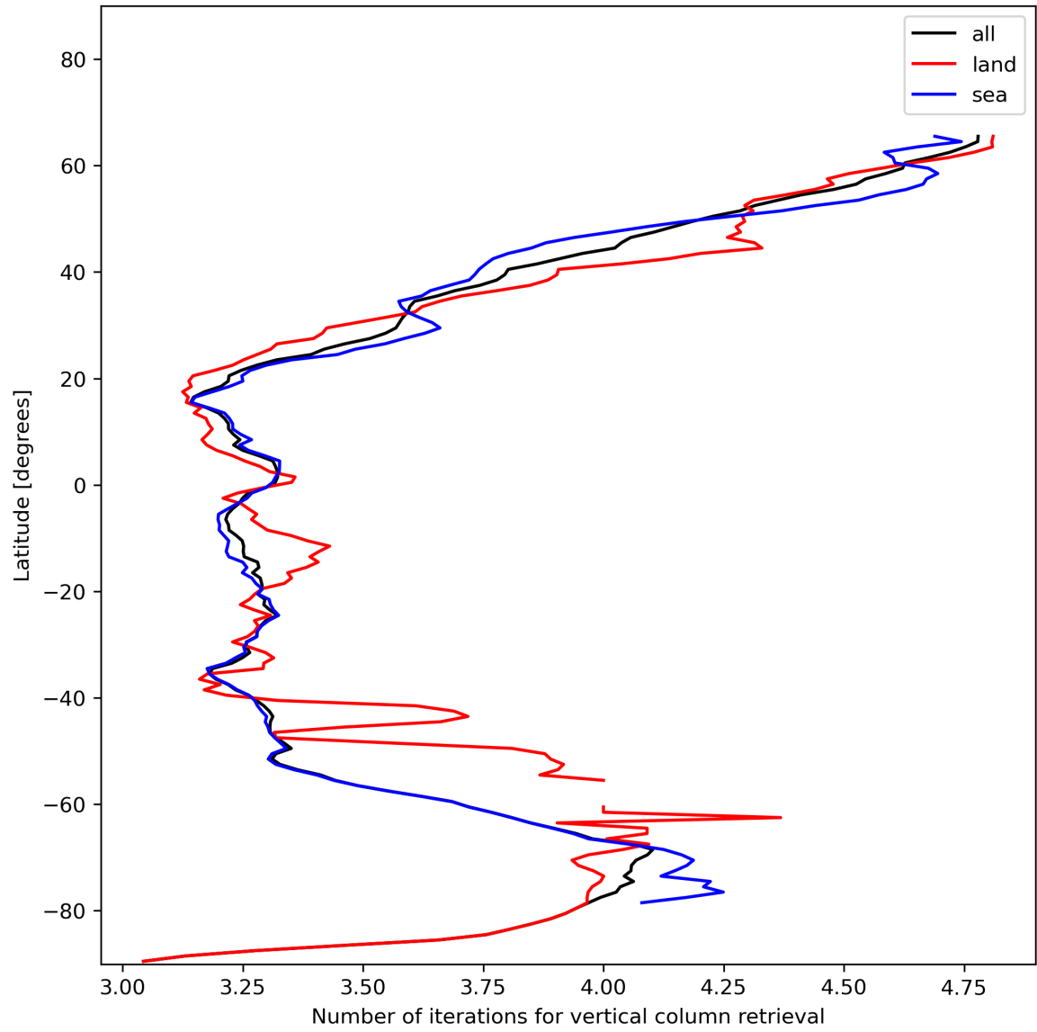
Figure 19: Zonal average of “Number of iterations for vertical column retrieval” for 2023-12-16 to 2023-12-18.
