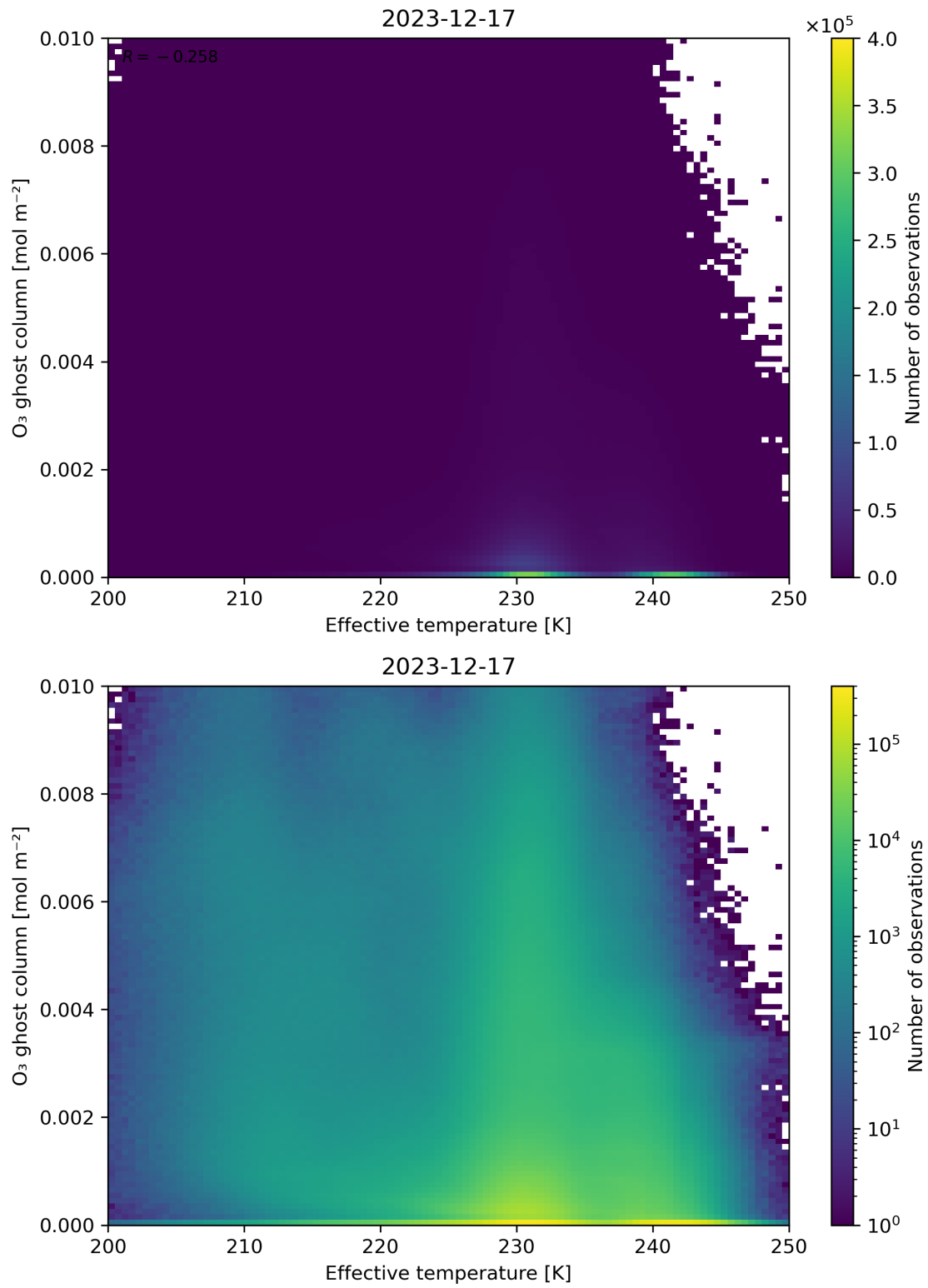
Figure 38: Scatter density plot of “Effective temperature” against “O 3 ghost column” for 2023-12-16 to 2023-12-18.
