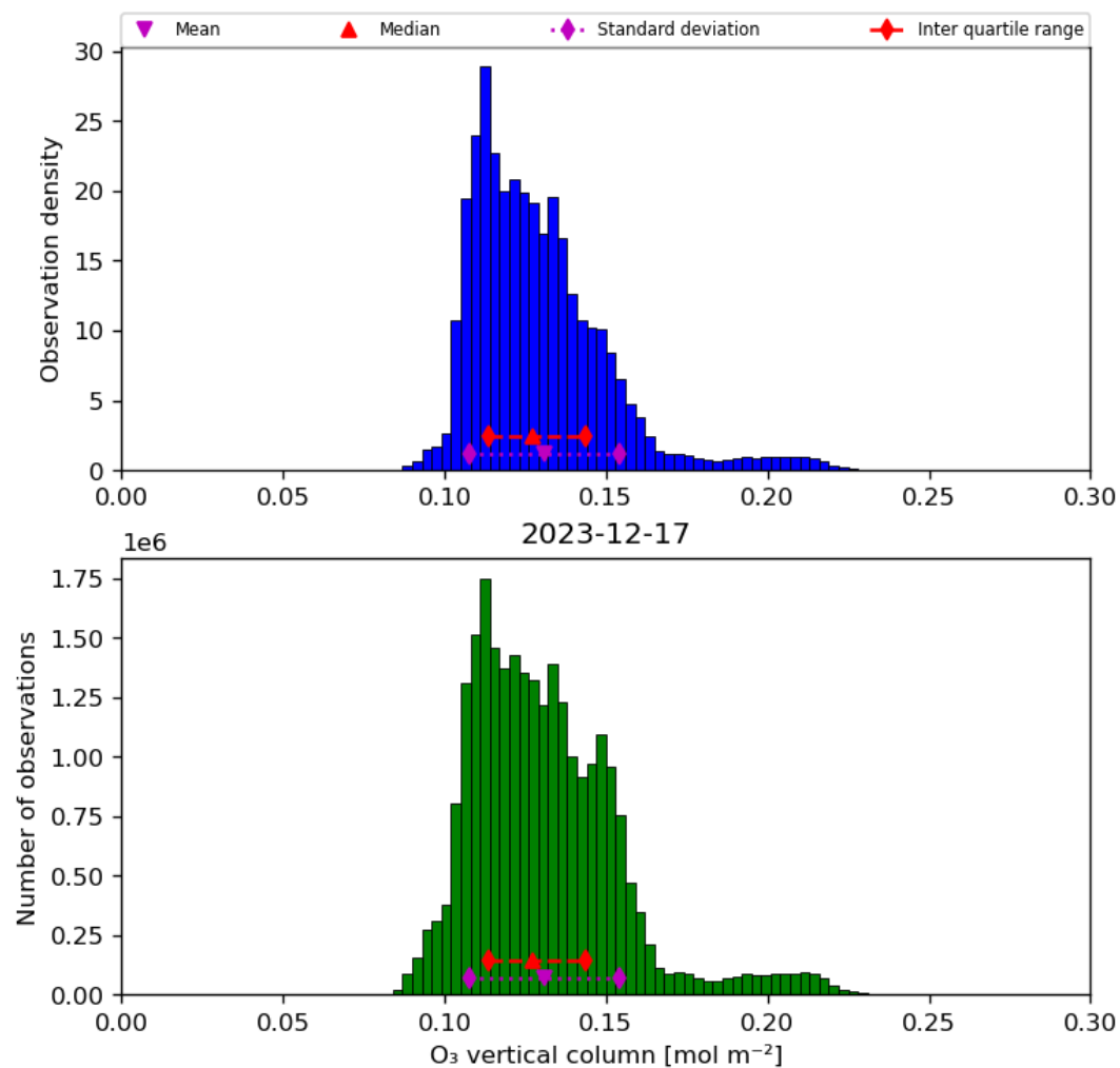
Figure 21: Histogram of “O 3 vertical column” for 2023-12-16 to 2023-12-18
