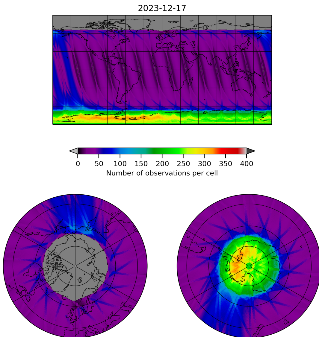
Figure 12: Map of the number of observations for 2023-12-16 to 2023-12-18
