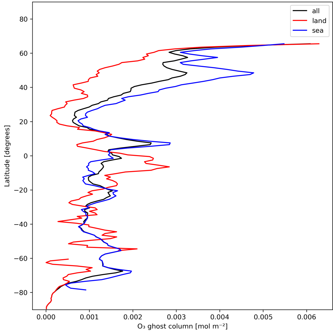
Figure 18: Zonal average of “O 3 ghost column” for 2023-12-16 to 2023-12-18.
