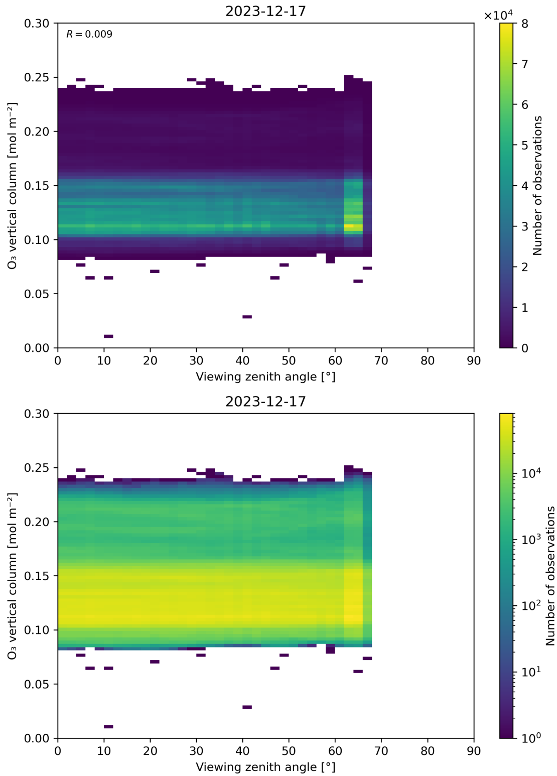
Figure 52: Scatter density plot of “Viewing zenith angle” against “O 3 vertical column” for 2023-12-16 to 2023-12-18.
