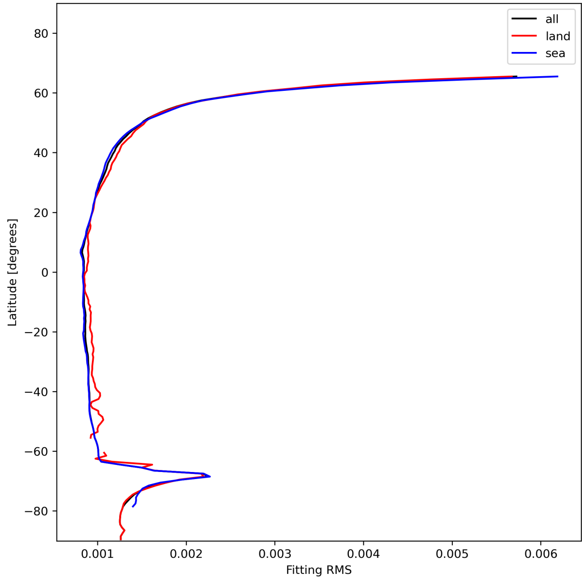
Figure 16: Zonal average of “Fitting RMS” for 2023-12-16 to 2023-12-18.
