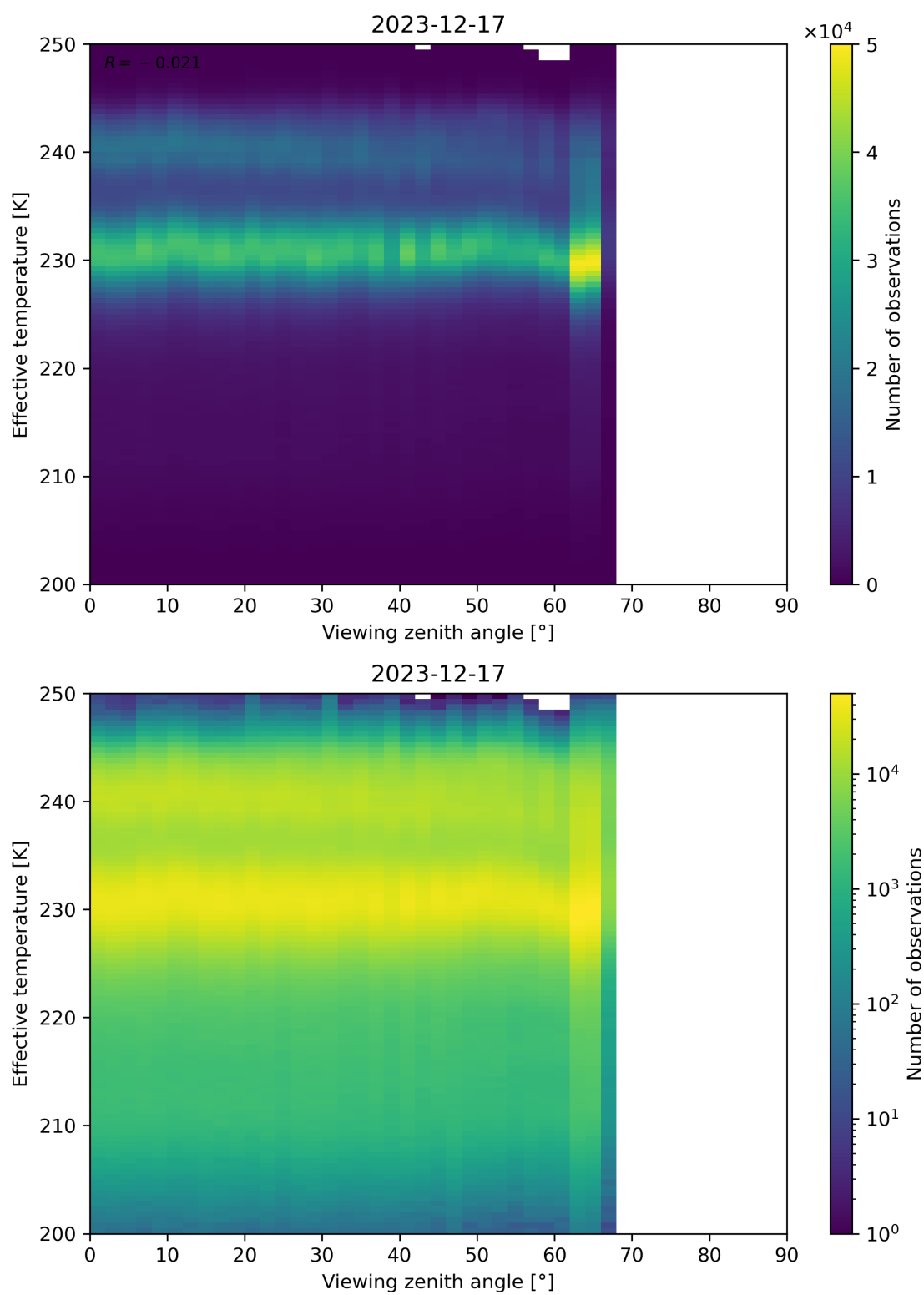
Figure 50: Scatter density plot of “Viewing zenith angle” against “Effective temperature” for 2023-12-16 to 2023-12-18.
