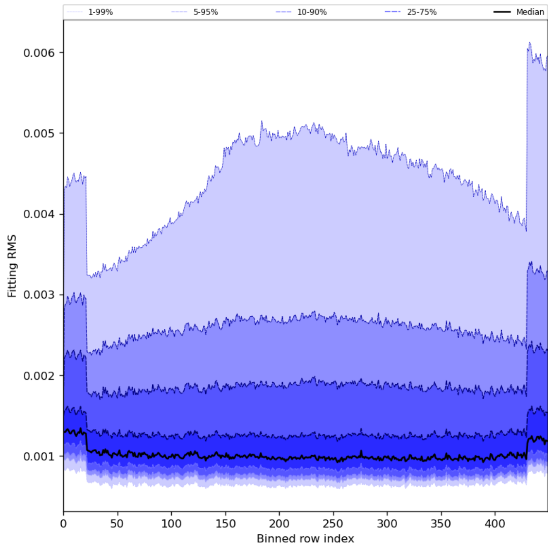
Figure 30: Along track statistics of “Fitting RMS” for 2023-12-16 to 2023-12-18
