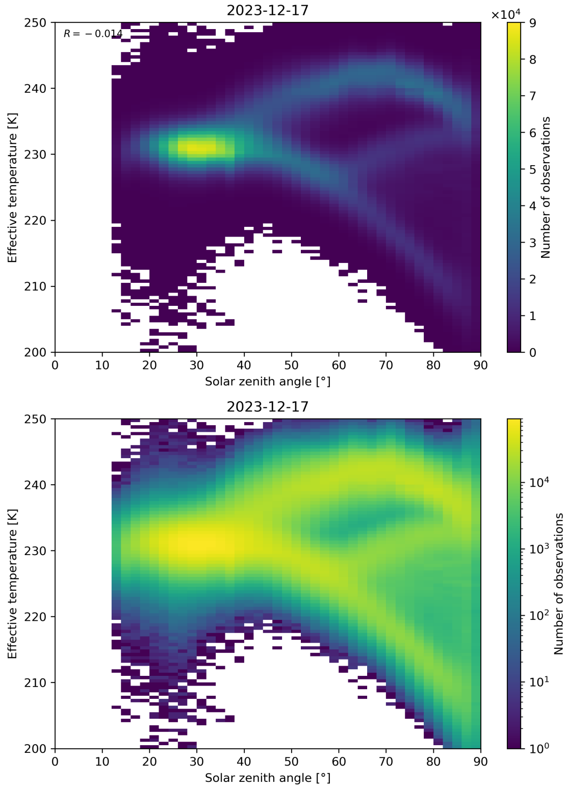
Figure 45: Scatter density plot of “Solar zenith angle” against “Effective temperature” for 2023-12-16 to 2023-12-18.
