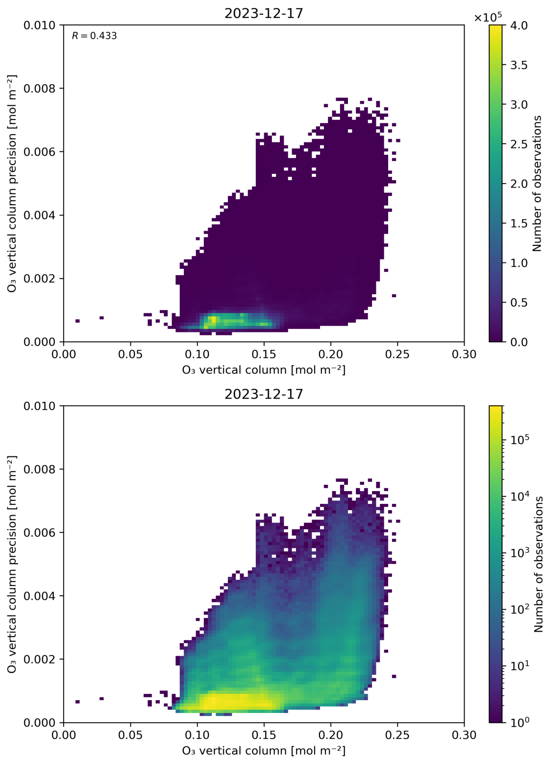
Figure 41: Scatter density plot of “O 3 vertical column” against “O 3 vertical column precision” for 2023-12-16 to 2023-12-18.
