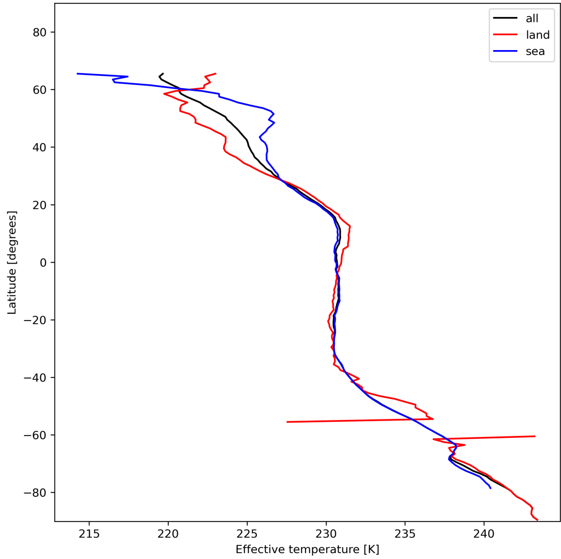
Figure 17: Zonal average of “Effective temperature” for 2023-12-16 to 2023-12-18.
