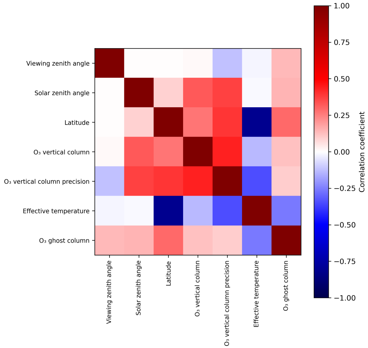
Figure 2: Map of correlation matrix for 2023-12-16 to 2023-12-18.
