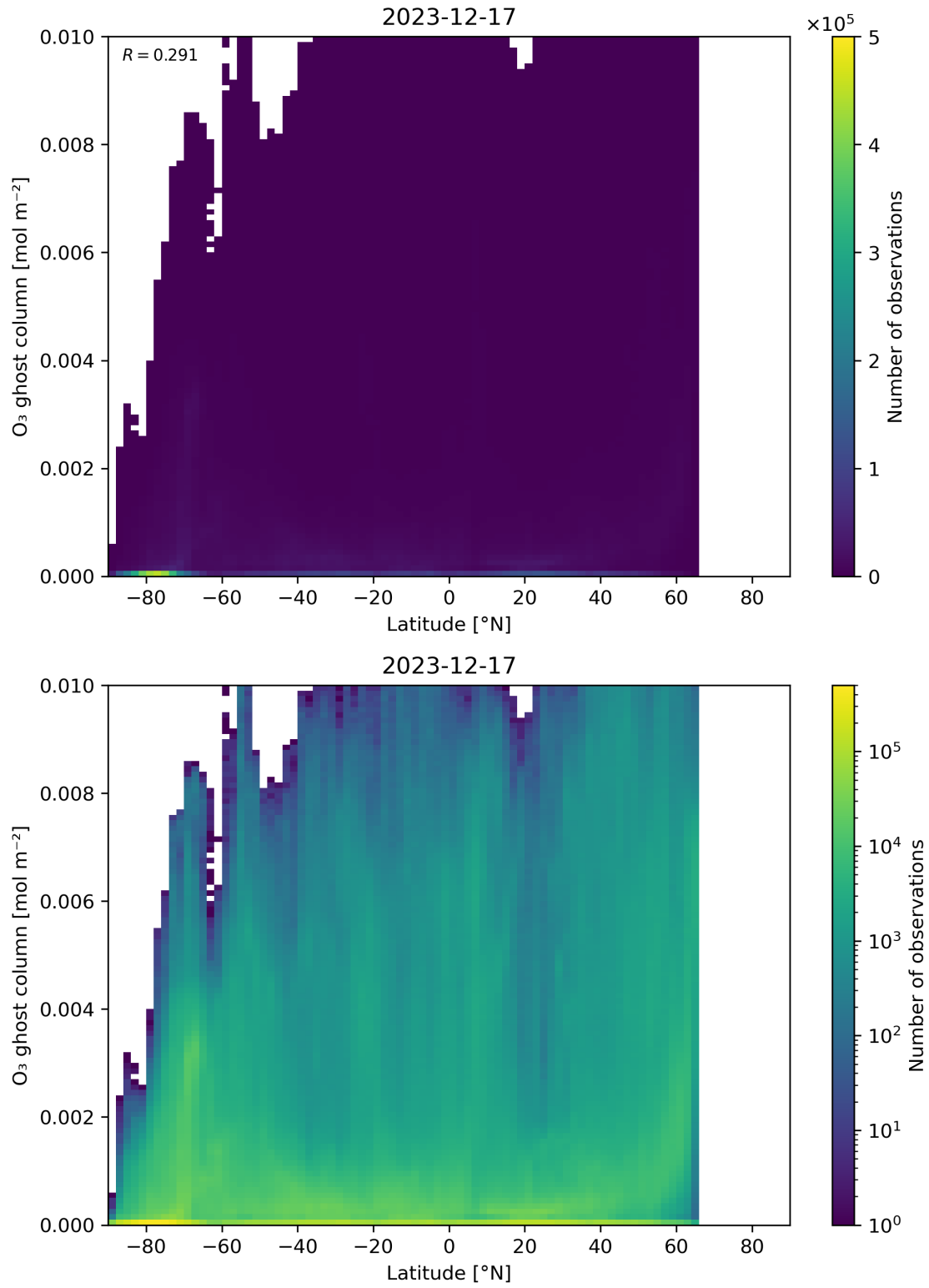
Figure 35: Scatter density plot of “Latitude” against “O 3 ghost column” for 2023-12-16 to 2023-12-18.
