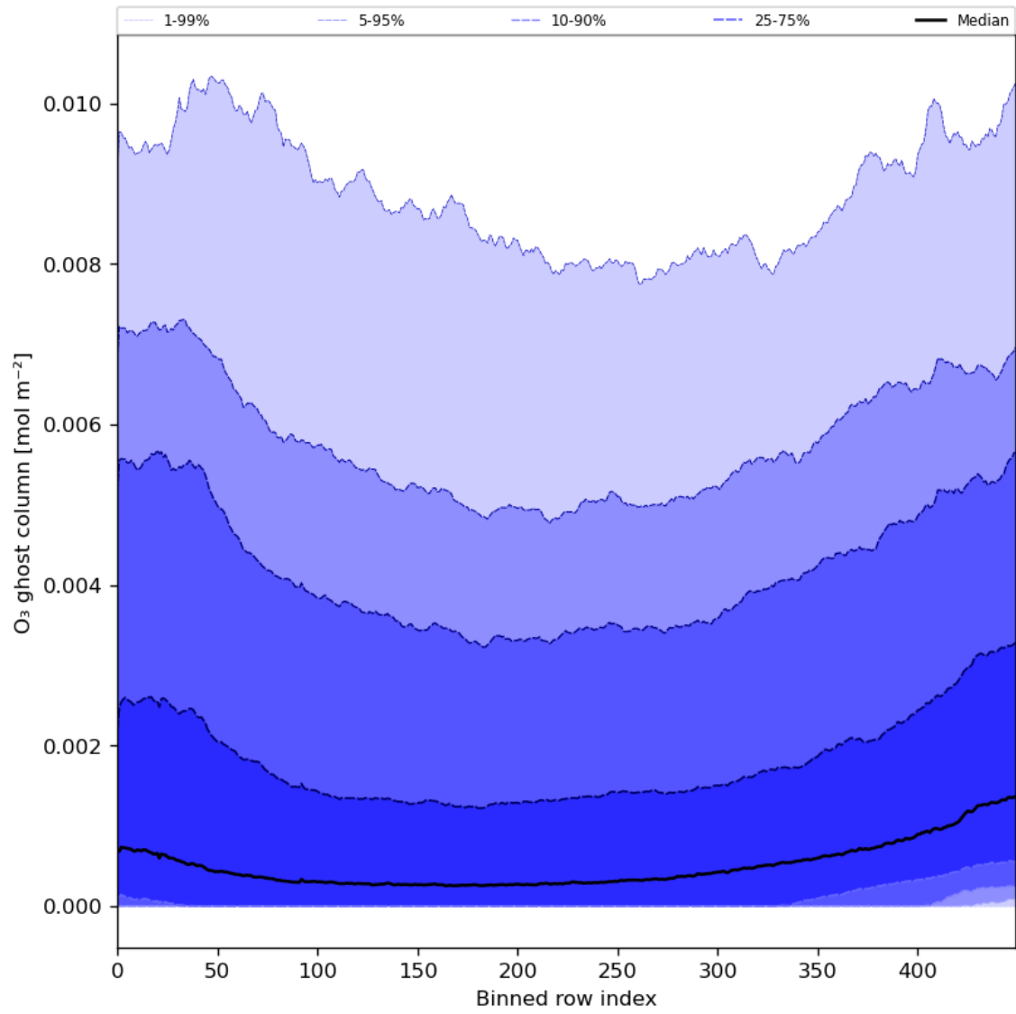
Figure 32: Along track statistics of “O 3 ghost column” for 2023-12-16 to 2023-12-18
