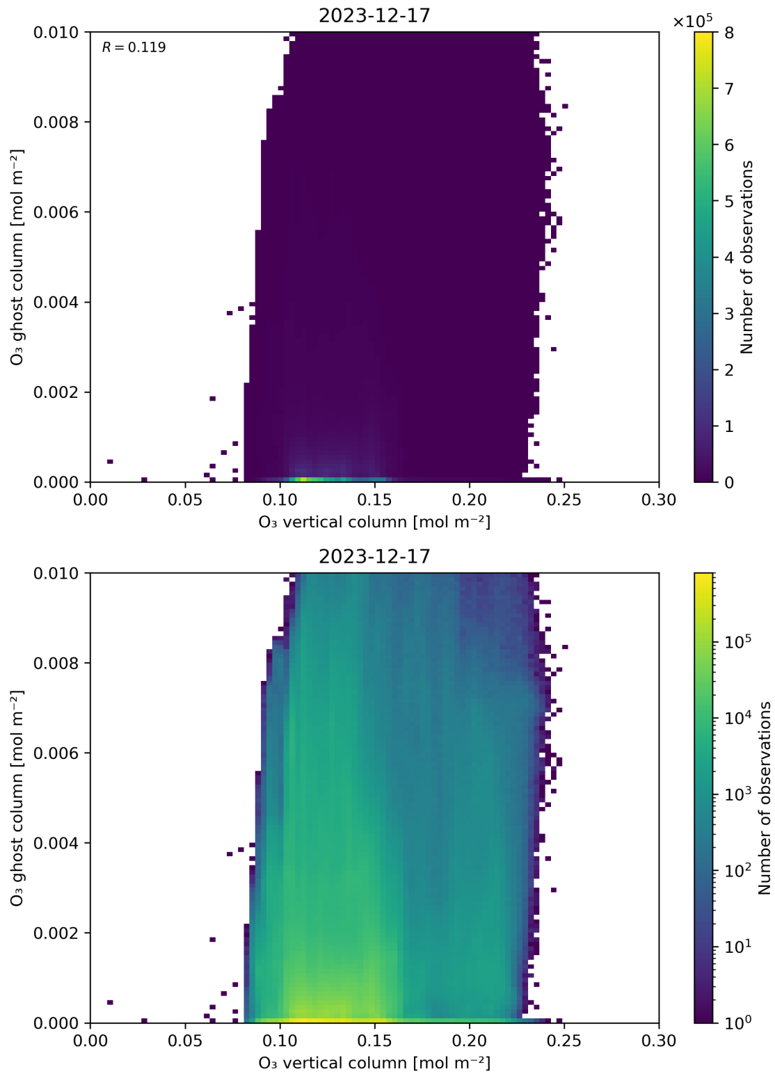
Figure 40: Scatter density plot of “O 3 vertical column” against “O 3 ghost column” for 2023-12-16 to 2023-12-18.
