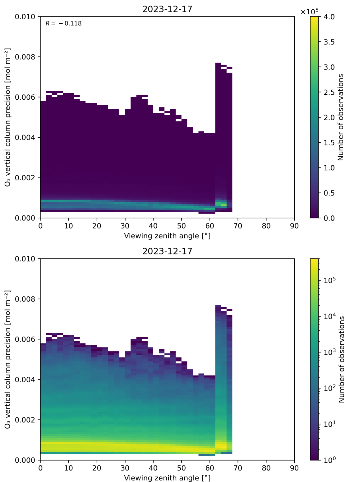
Figure 53: Scatter density plot of “Viewing zenith angle” against “O 3 vertical column precision” for 2023-12-16 to 2023-12-18.
