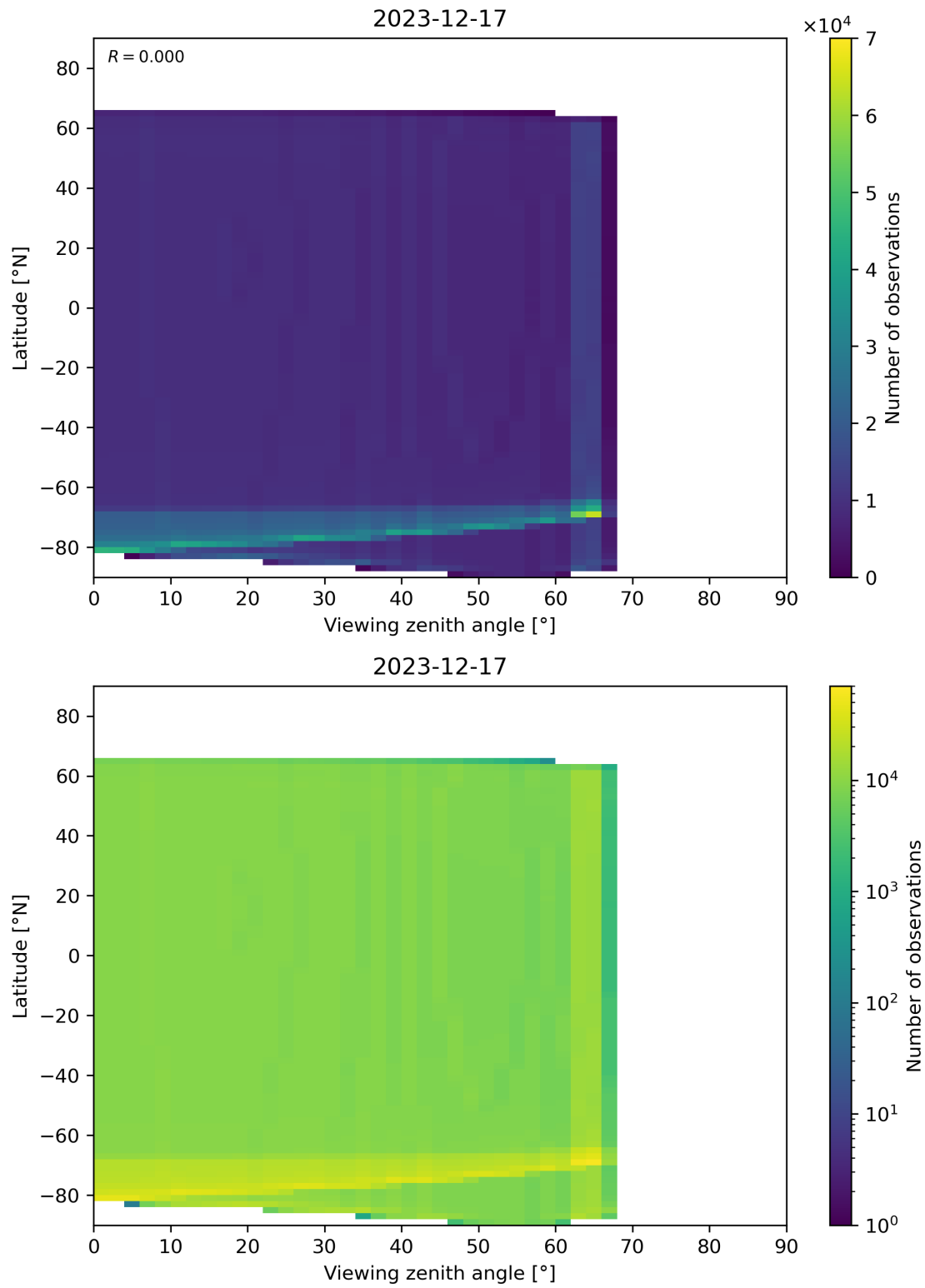
Figure 49: Scatter density plot of “Viewing zenith angle” against “Latitude” for 2023-12-16 to 2023-12-18.
