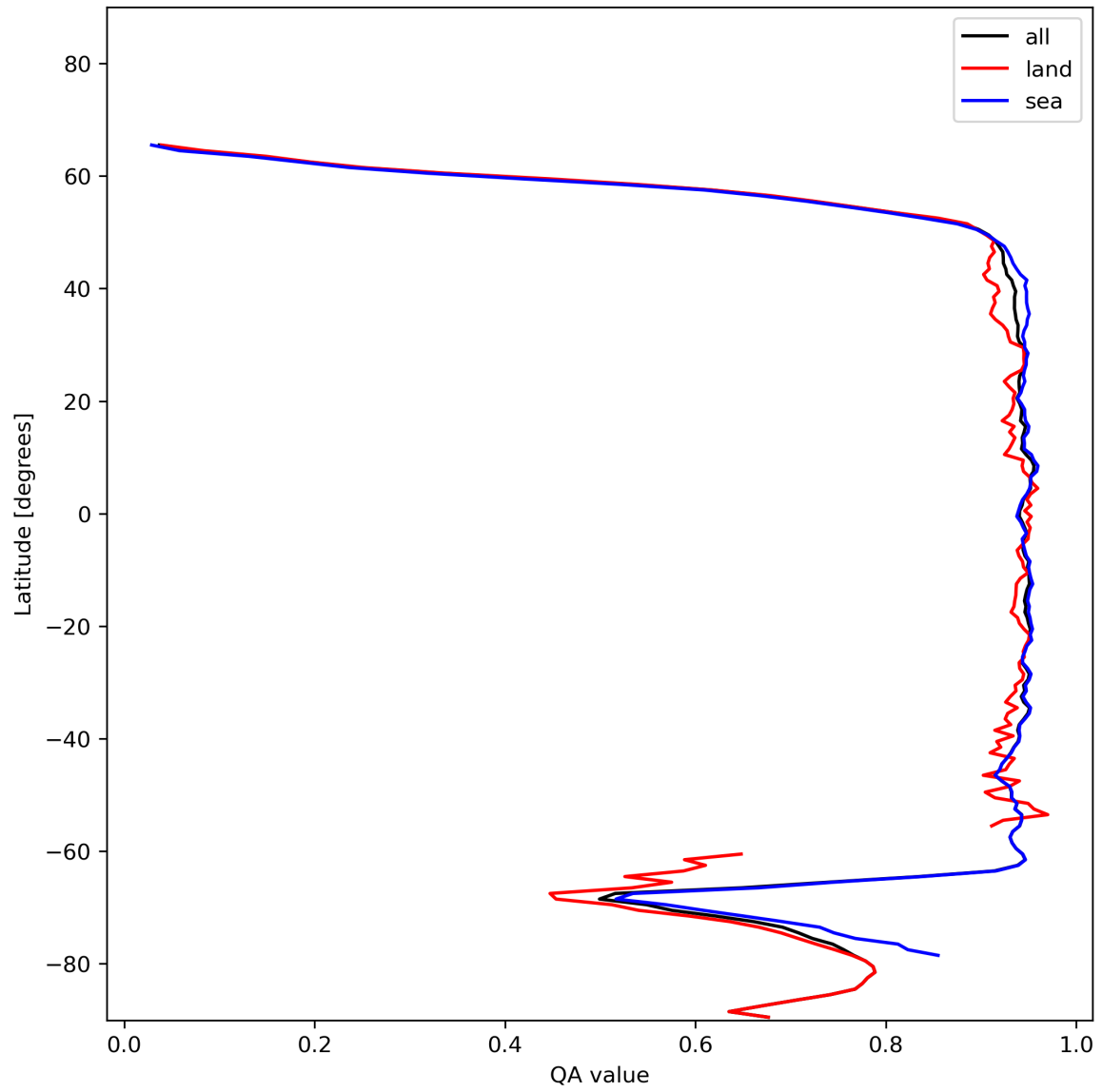
Figure 13: Zonal average of “QA value” for 2023-12-16 to 2023-12-18.
