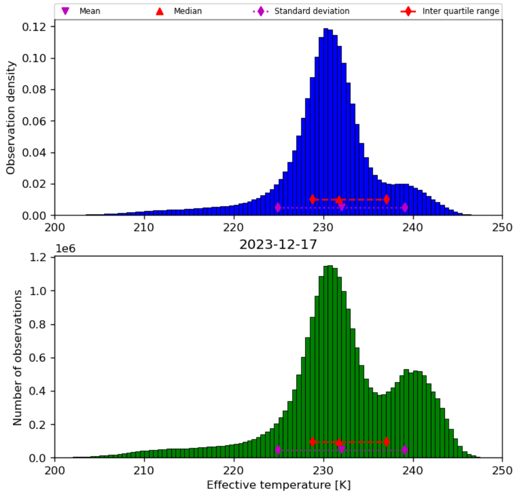
Figure 24: Histogram of “Effective temperature” for 2023-12-16 to 2023-12-18
