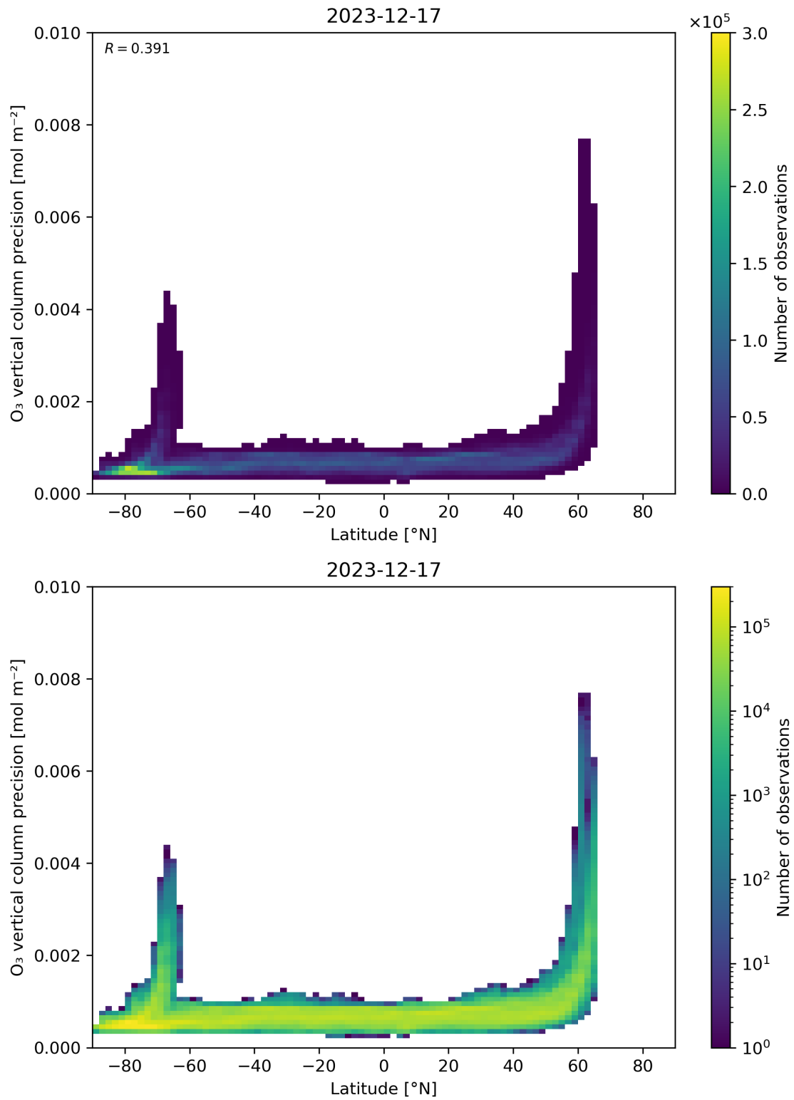
Figure 37: Scatter density plot of “Latitude” against “O 3 vertical column precision” for 2023-12-16 to 2023-12-18.
