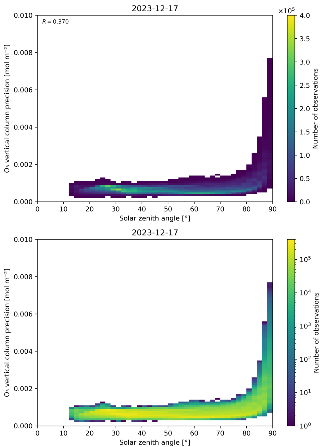
Figure 48: Scatter density plot of “Solar zenith angle” against “O 3 vertical column precision” for 2023-12-16 to 2023-12-18.
