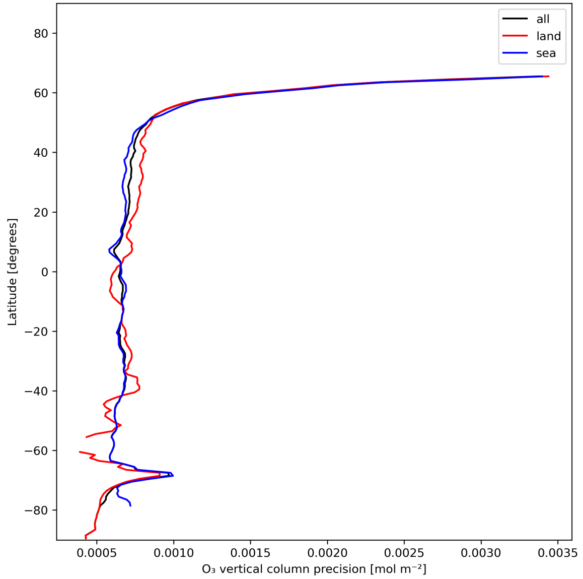
Figure 15: Zonal average of “O 3 vertical column precision” for 2023-12-16 to 2023-12-18.
