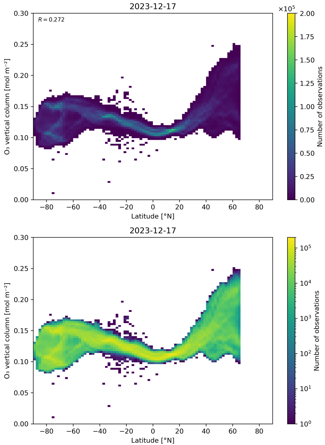
Figure 36: Scatter density plot of “Latitude” against “O 3 vertical column” for 2023-12-16 to 2023-12-18.
