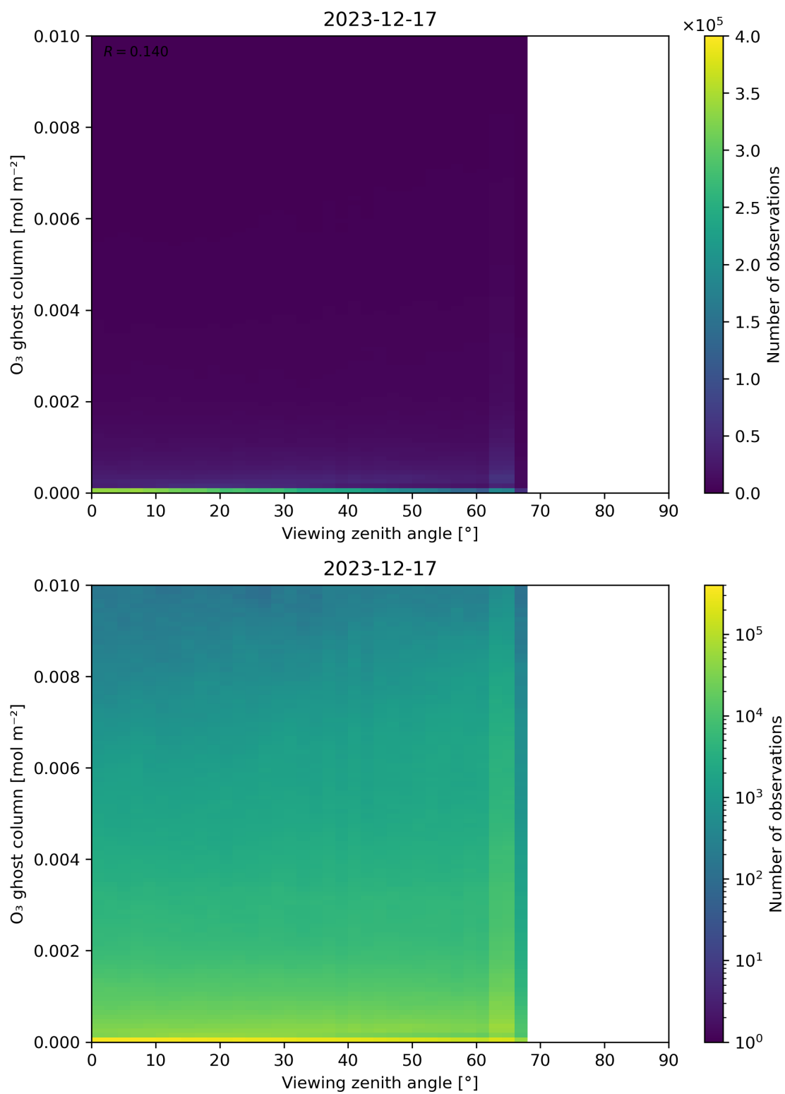
Figure 51: Scatter density plot of “Viewing zenith angle” against “O 3 ghost column” for 2023-12-16 to 2023-12-18.
