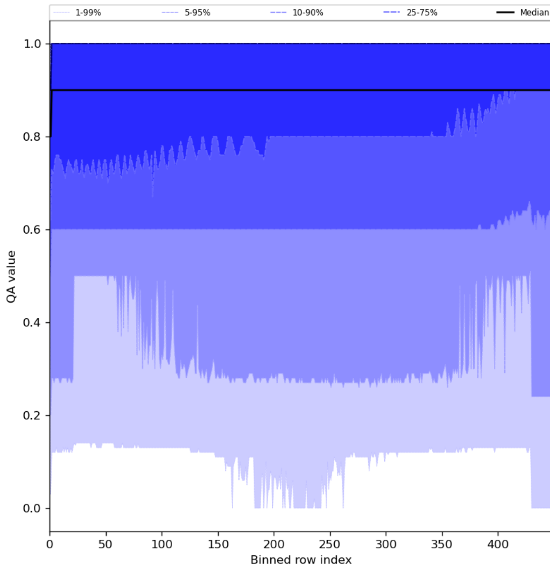
Figure 27: Along track statistics of “QA value” for 2023-12-16 to 2023-12-18
