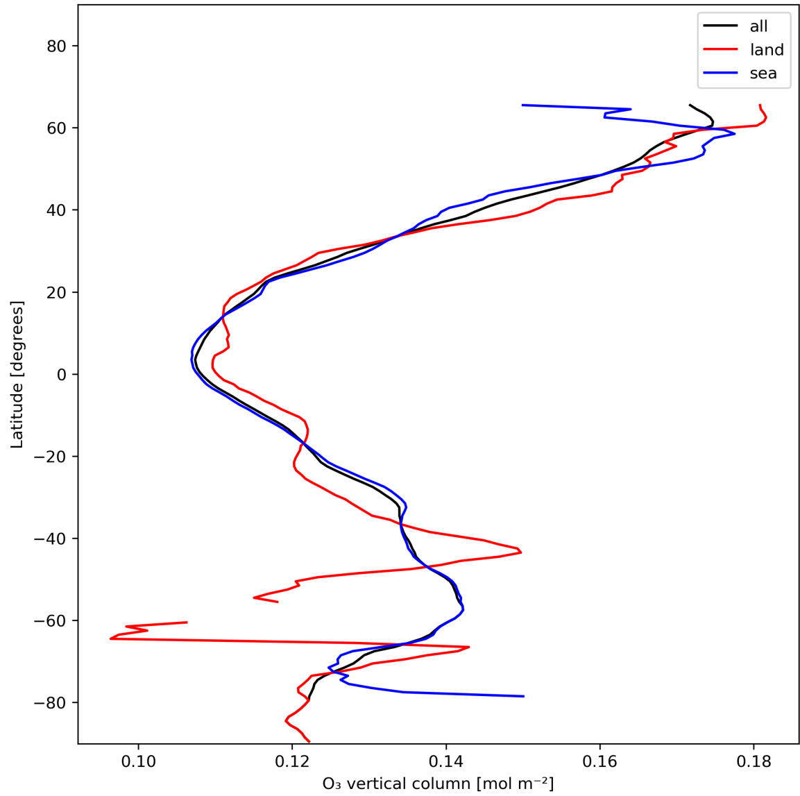
Figure 14: Zonal average of “O 3 vertical column” for 2023-12-16 to 2023-12-18.
