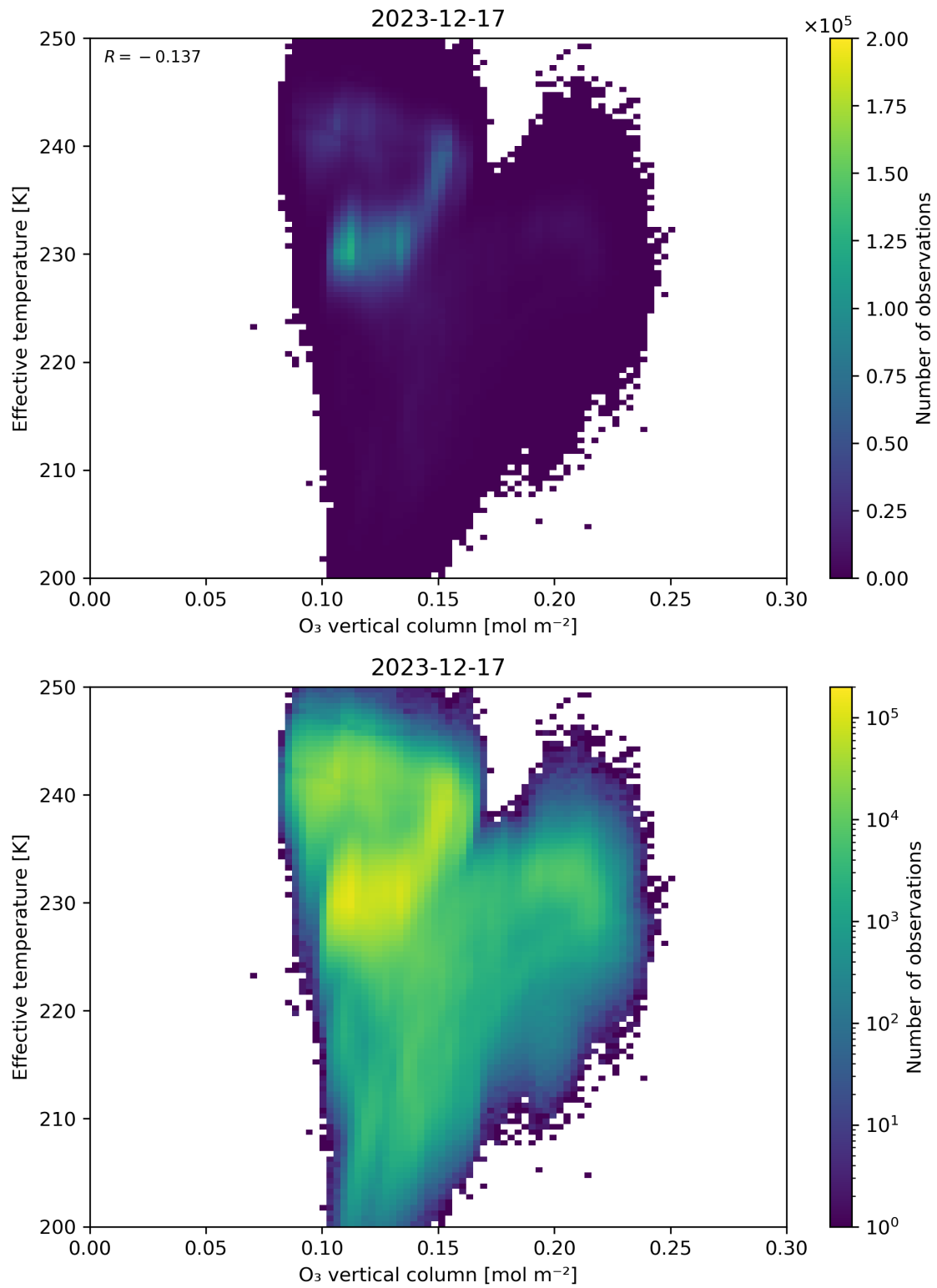
Figure 39: Scatter density plot of “O 3 vertical column” against “Effective temperature” for 2023-12-16 to 2023-12-18.
