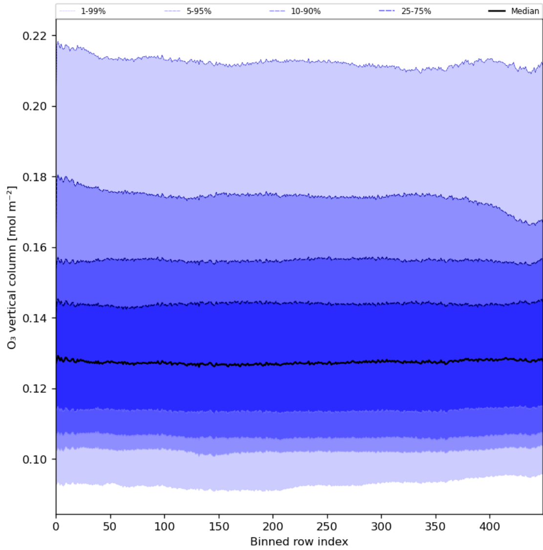
Figure 28: Along track statistics of “O 3 vertical column” for 2023-12-16 to 2023-12-18
