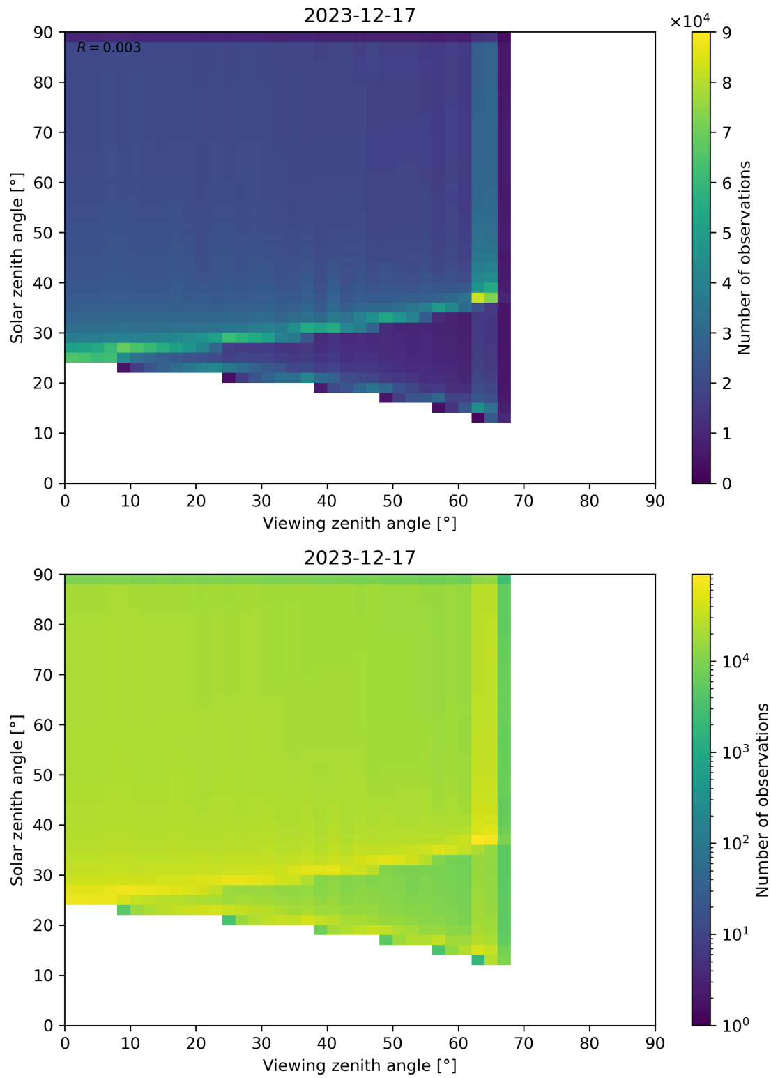
Figure 54: Scatter density plot of “Viewing zenith angle” against “Solar zenith angle” for 2023-12-16 to 2023-12-18.
