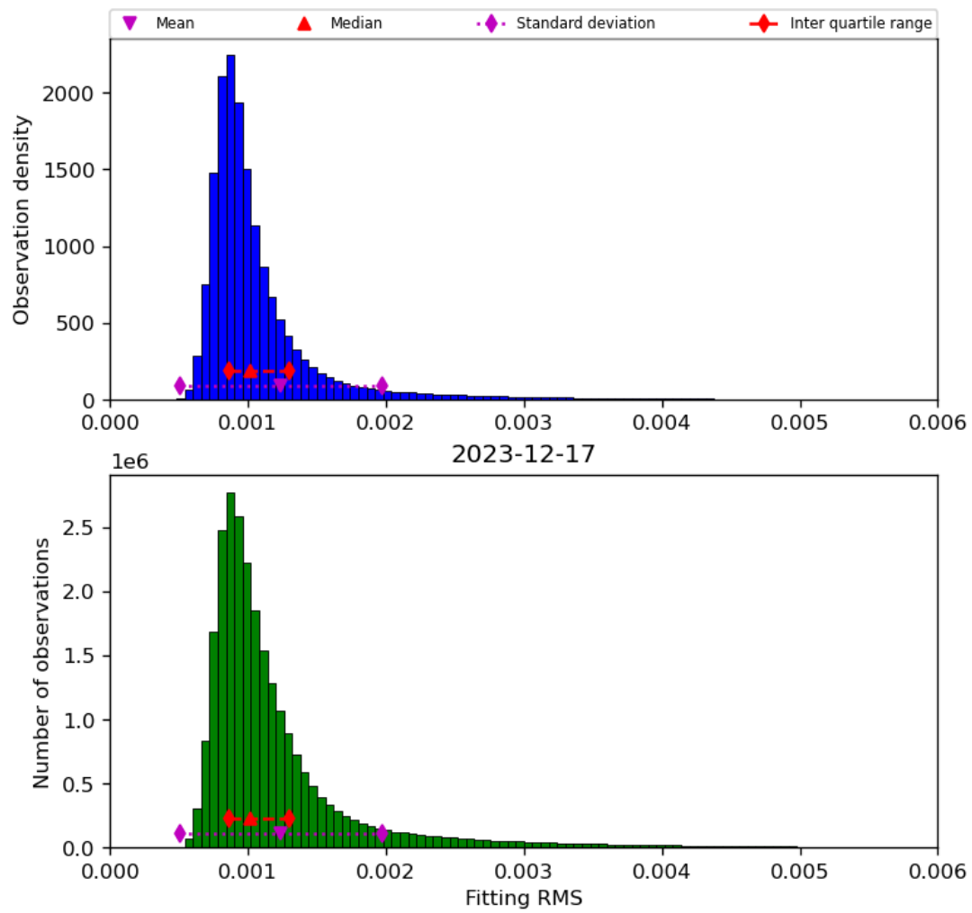
Figure 23: Histogram of “Fitting RMS” for 2023-12-16 to 2023-12-18
