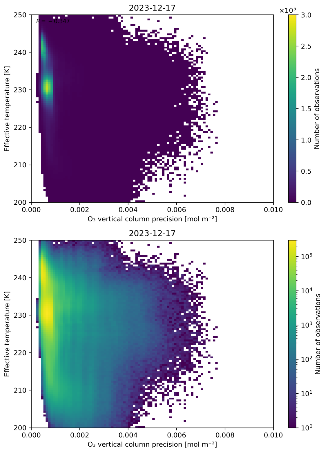
Figure 42: Scatter density plot of “O 3 vertical column precision” against “Effective temperature” for 2023-12-16 to 2023-12-18.
