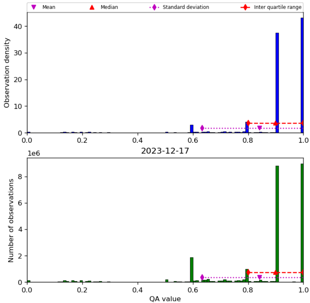
Figure 20: Histogram of “QA value” for 2023-12-16 to 2023-12-18
