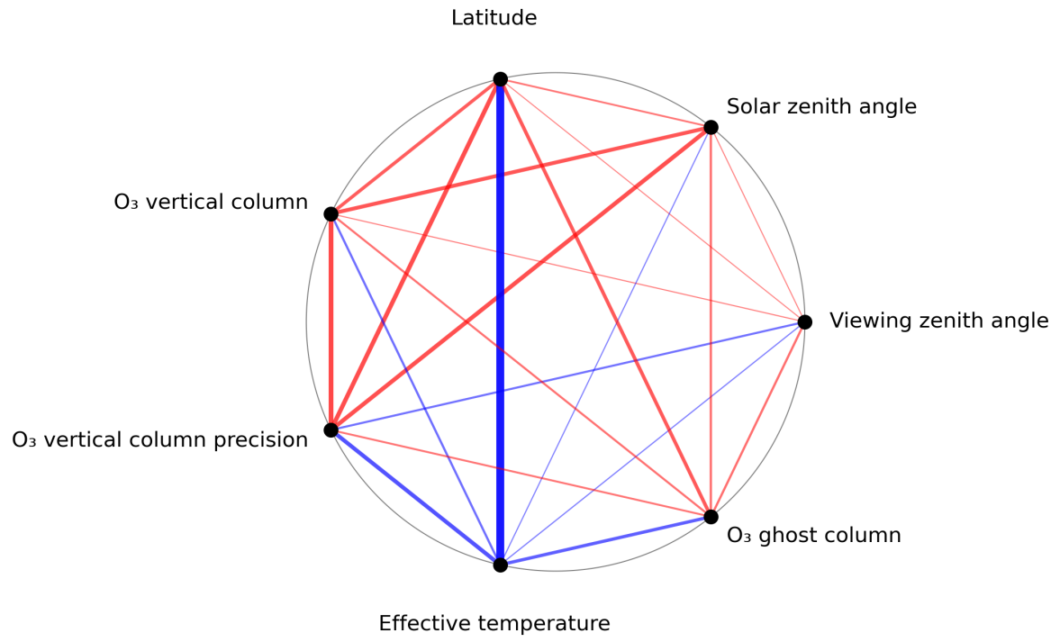
Figure 1: Map of correlation graph for 2023-12-16 to 2023-12-18.
