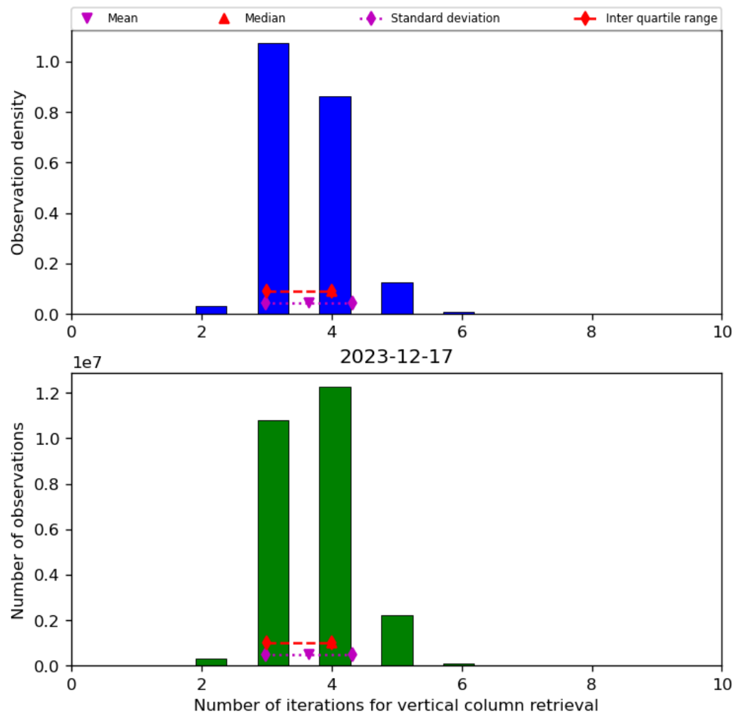
Figure 26: Histogram of “Number of iterations for vertical column retrieval” for 2023-12-16 to 2023-12-18
