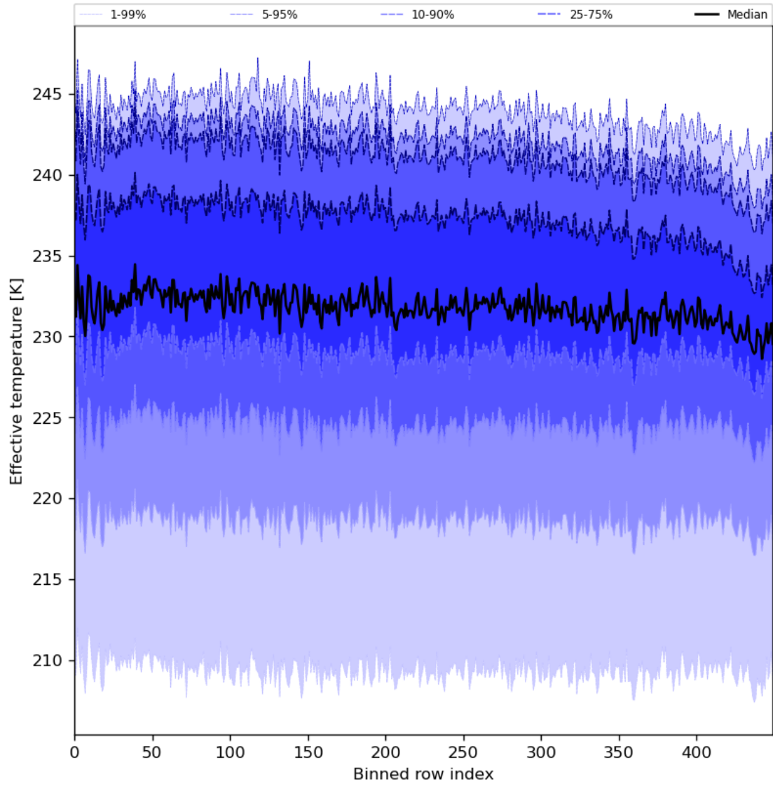
Figure 31: Along track statistics of “Effective temperature” for 2023-12-16 to 2023-12-18
