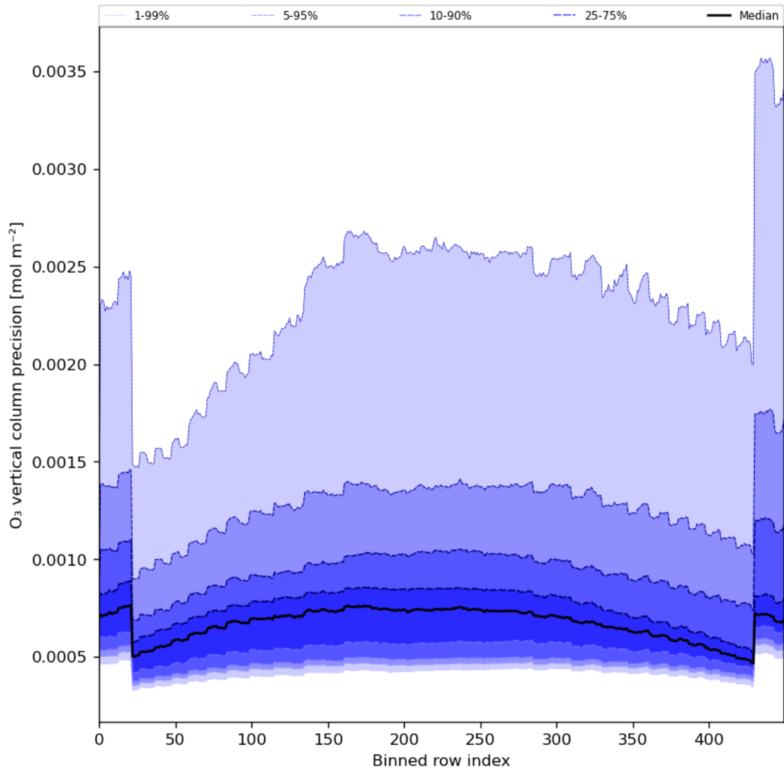
Figure 29: Along track statistics of “O 3 vertical column precision” for 2023-12-16 to 2023-12-18
