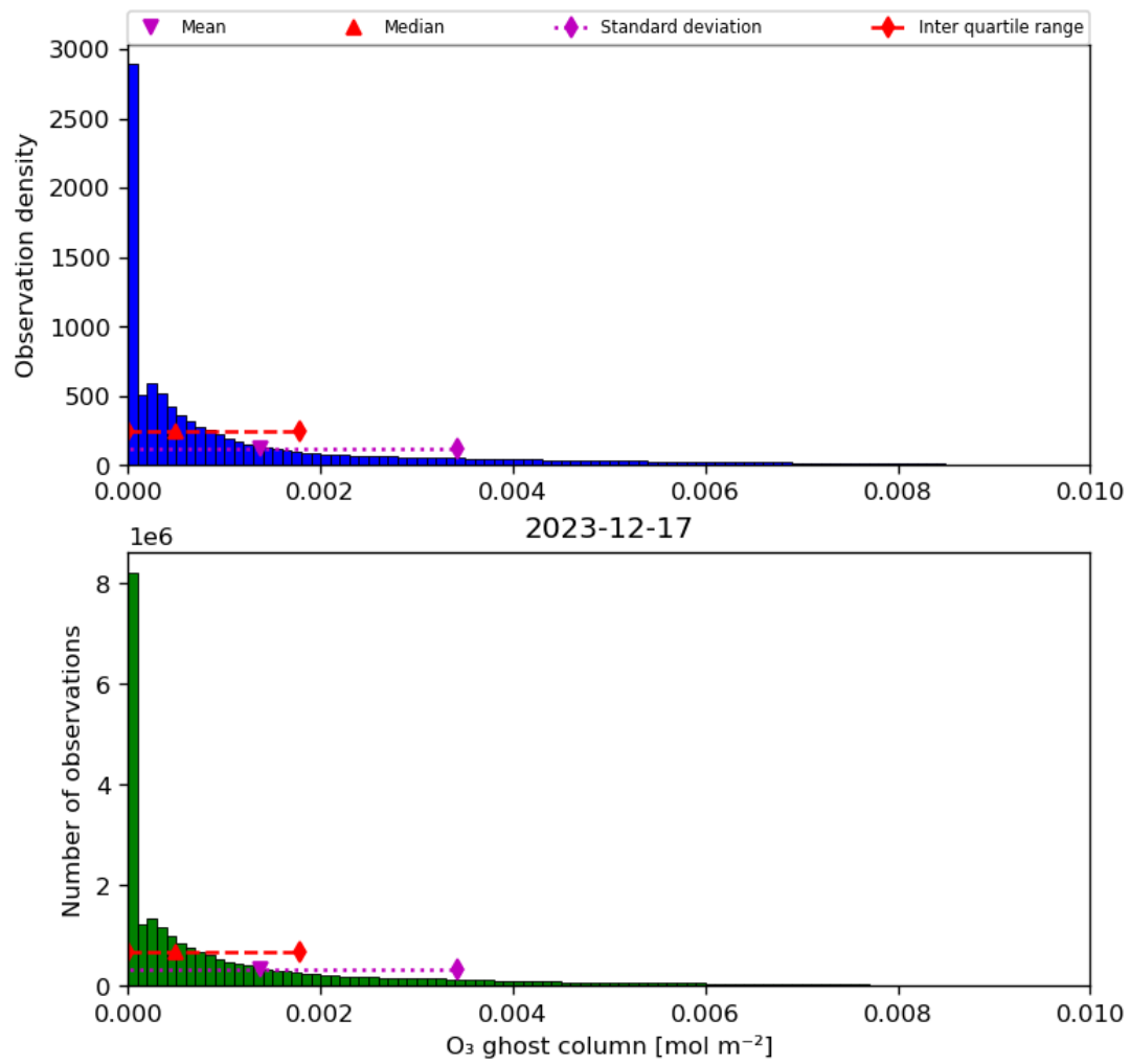
Figure 25: Histogram of “O 3 ghost column” for 2023-12-16 to 2023-12-18
