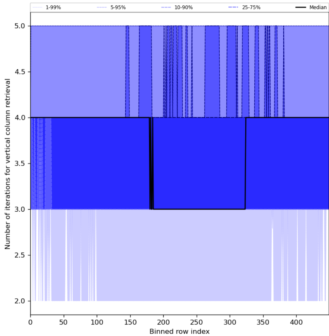
Figure 33: Along track statistics of “Number of iterations for vertical column retrieval” for 2023-12-16 to 2023-12-18
