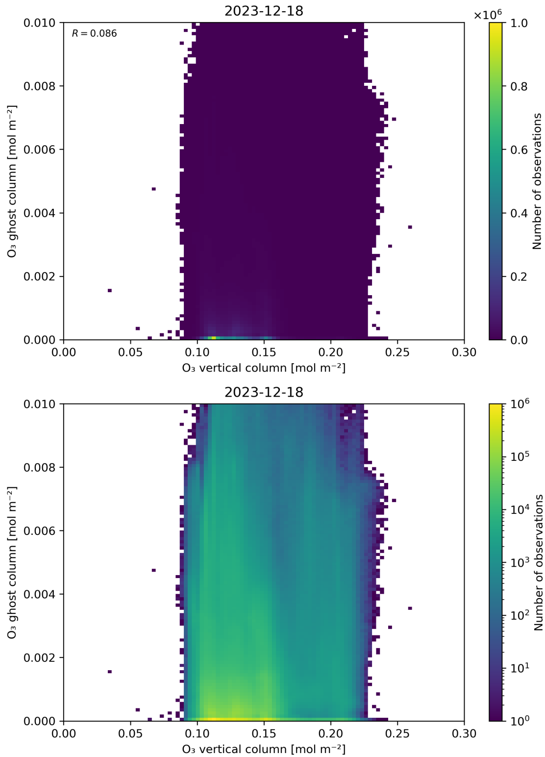
Figure 40: Scatter density plot of “O 3 vertical column” against “O 3 ghost column” for 2023-12-17 to 2023-12-19.
