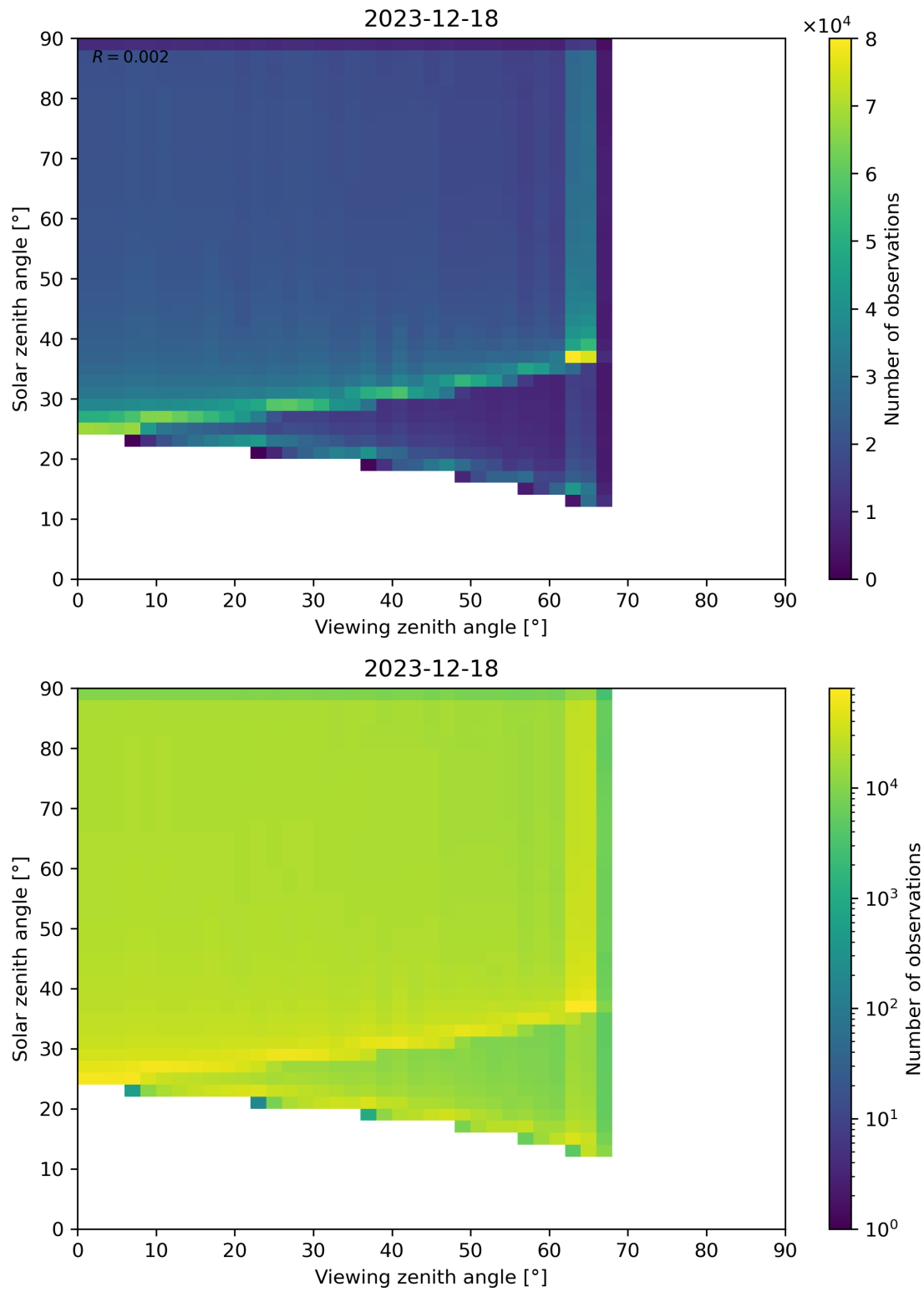
Figure 54: Scatter density plot of “Viewing zenith angle” against “Solar zenith angle” for 2023-12-17 to 2023-12-19.
