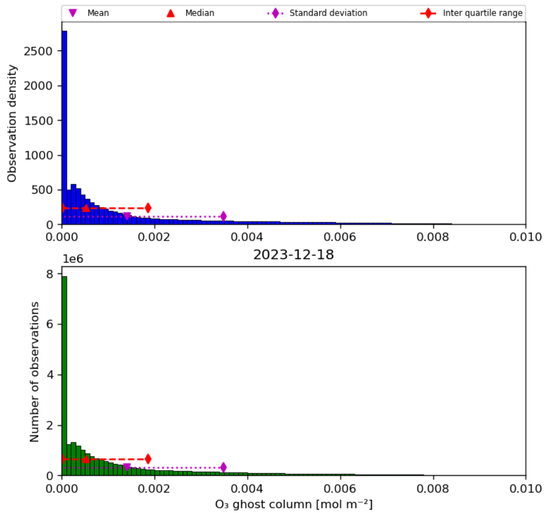
Figure 25: Histogram of “O 3 ghost column” for 2023-12-17 to 2023-12-19
