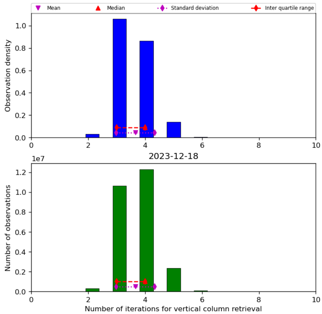
Figure 26: Histogram of “Number of iterations for vertical column retrieval” for 2023-12-17 to 2023-12-19
