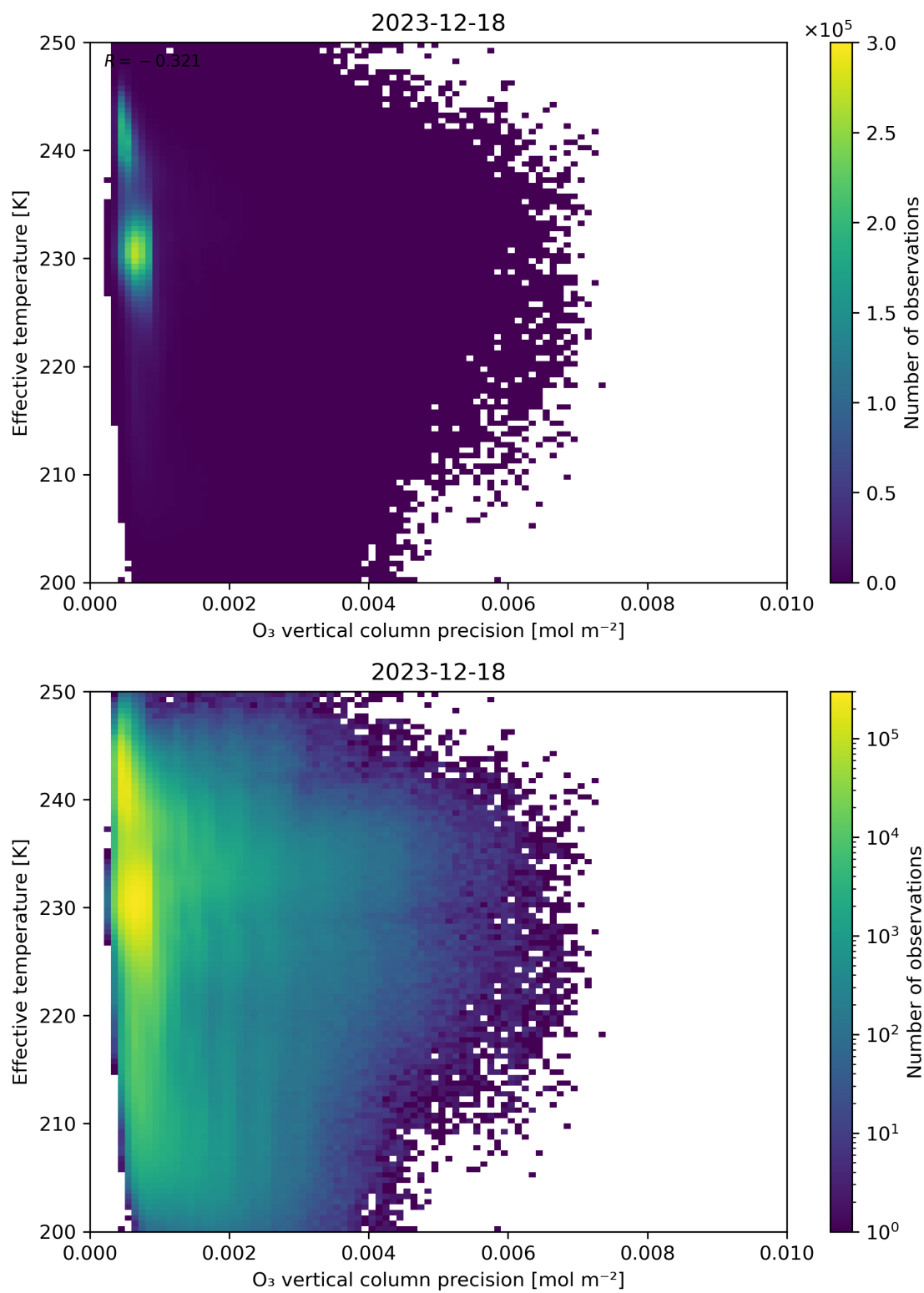
Figure 42: Scatter density plot of “O 3 vertical column precision” against “Effective temperature” for 2023-12-17 to 2023-12-19.
