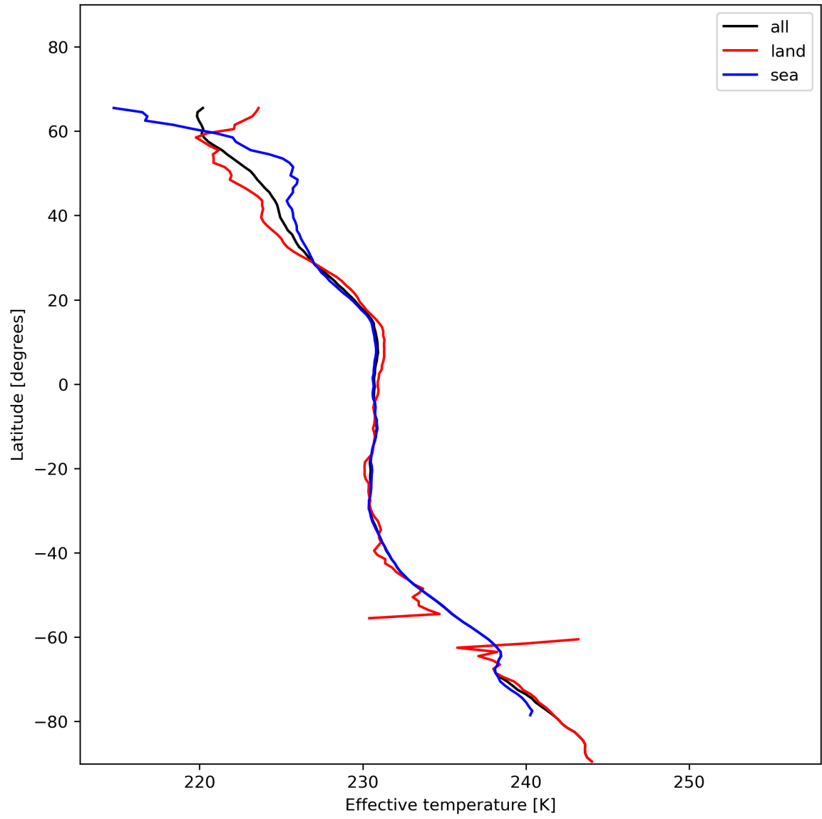
Figure 17: Zonal average of "Effective temperature" for 2023-12-17 to 2023-12-19.
