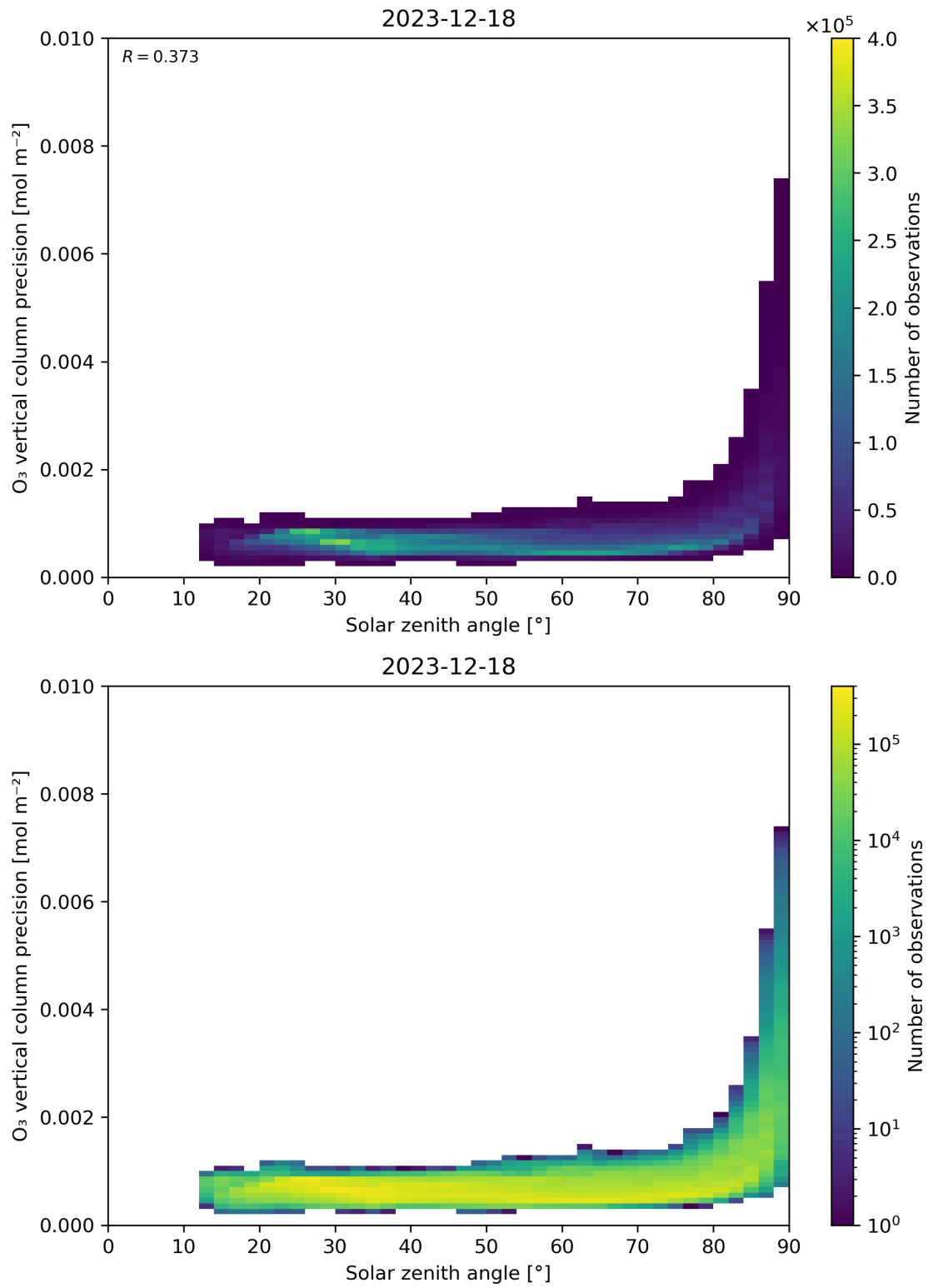
Figure 48: Scatter density plot of “Solar zenith angle” against “O 3 vertical column precision” for 2023-12-17 to 2023-12-19.
