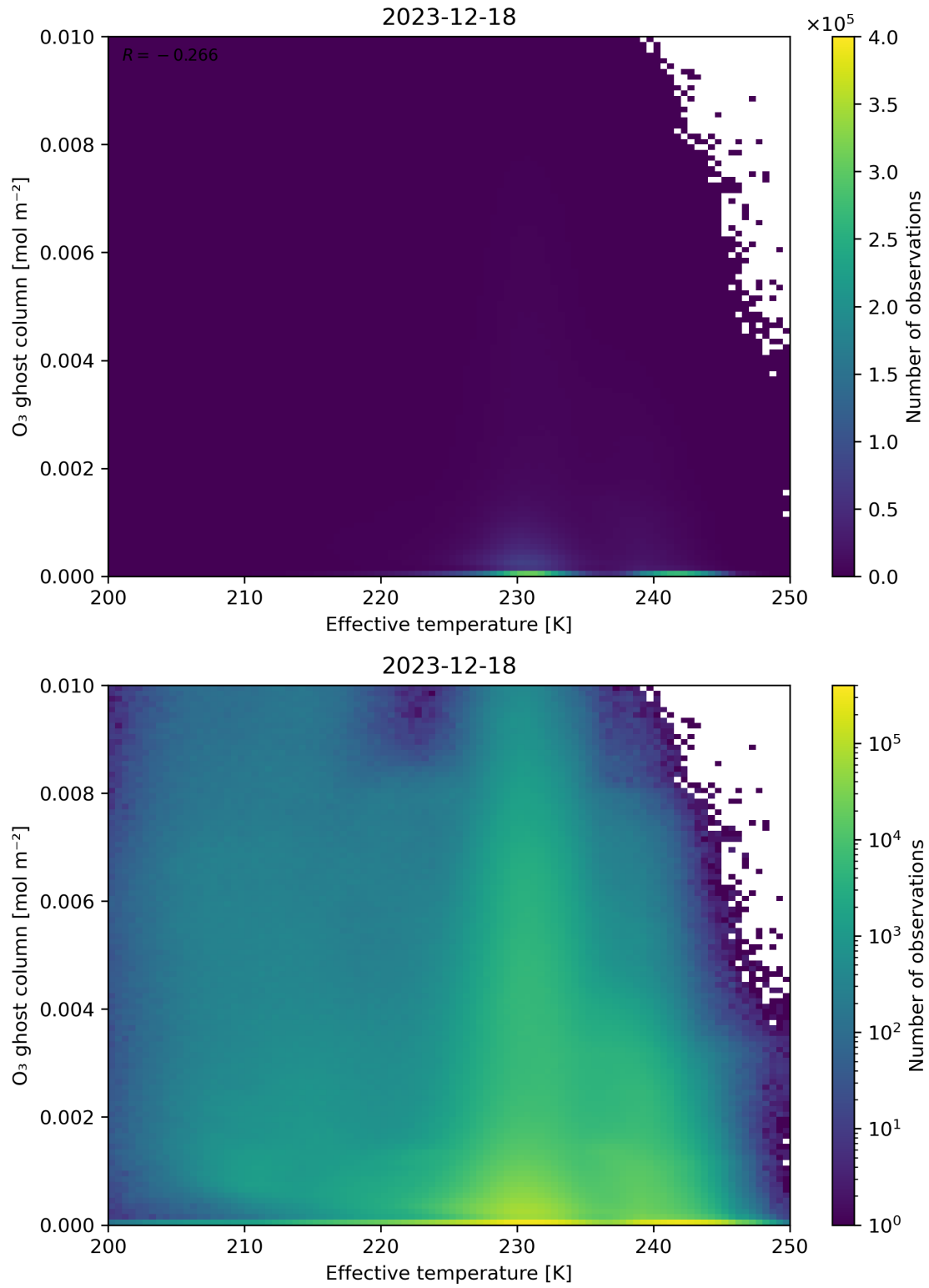
Figure 38: Scatter density plot of “Effective temperature” against “O 3 ghost column” for 2023-12-17 to 2023-12-19.
