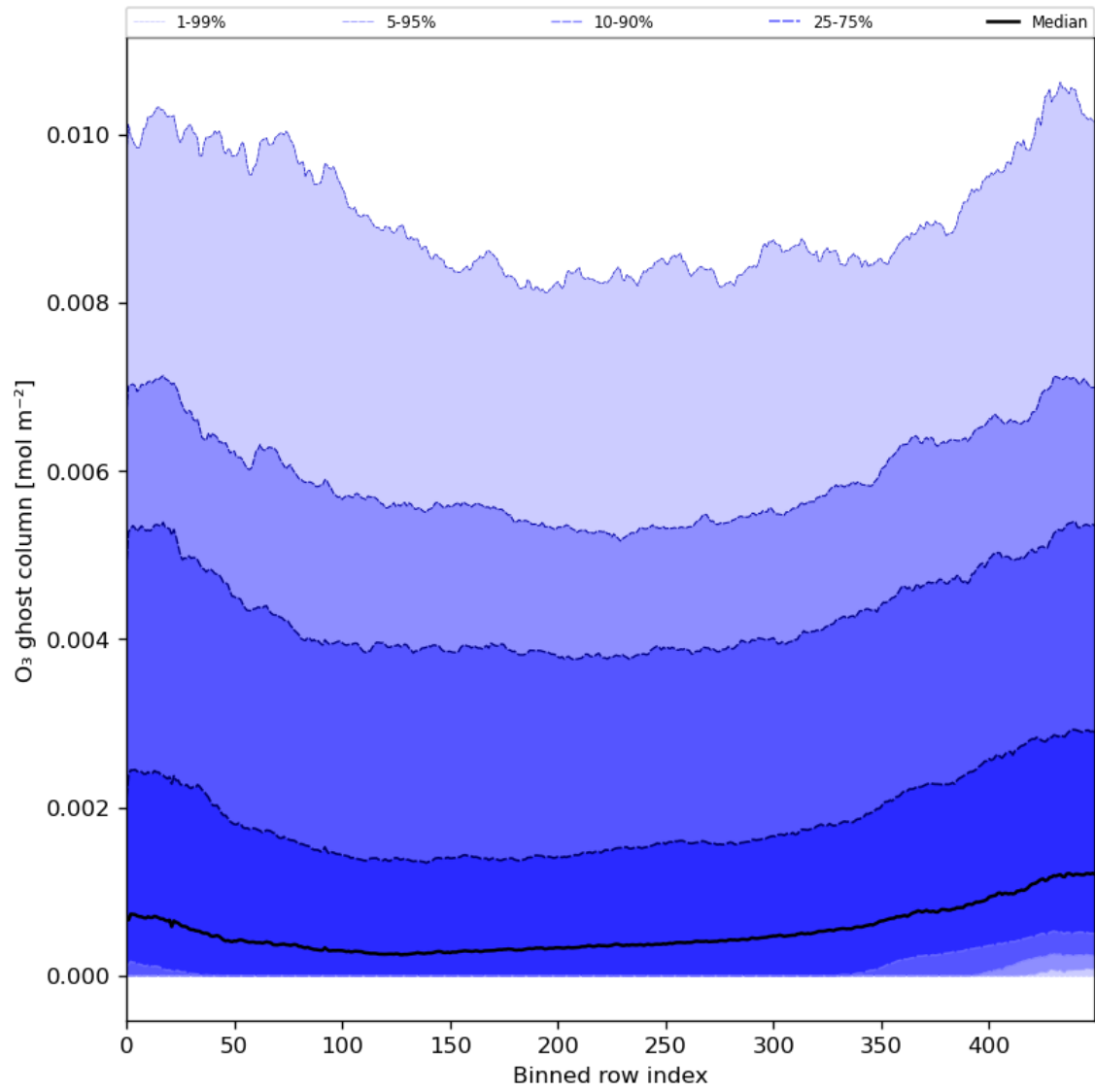
Figure 32: Along track statistics of “O 3 ghost column” for 2023-12-17 to 2023-12-19
