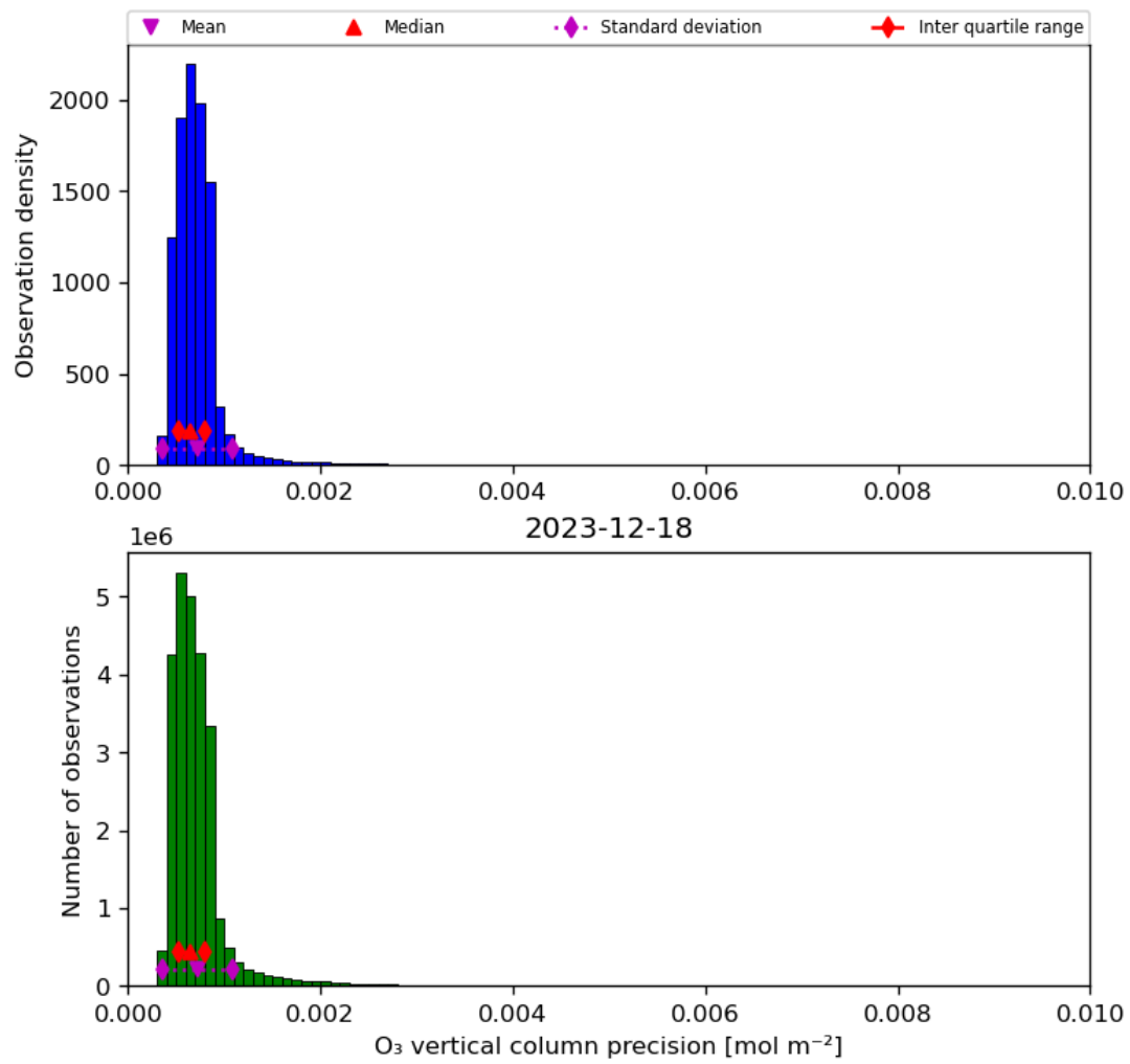
Figure 22: Histogram of “O 3 vertical column precision” for 2023-12-17 to 2023-12-19
