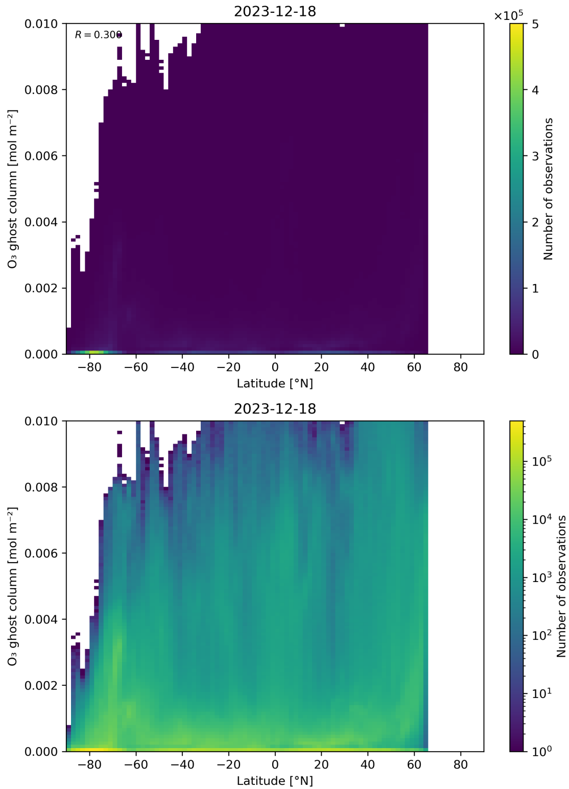
Figure 35: Scatter density plot of “Latitude” against “O 3 ghost column” for 2023-12-17 to 2023-12-19.
