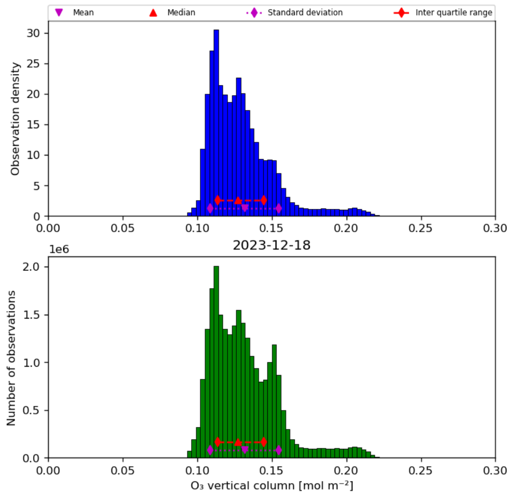
Figure 21: Histogram of “O 3 vertical column” for 2023-12-17 to 2023-12-19
