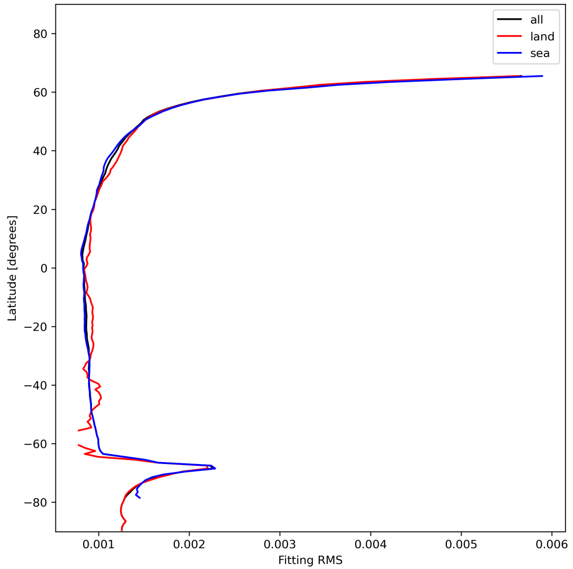
Figure 16: Zonal average of “Fitting RMS” for 2023-12-17 to 2023-12-19.
