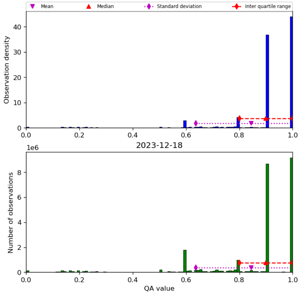
Figure 20: Histogram of “QA value” for 2023-12-17 to 2023-12-19
