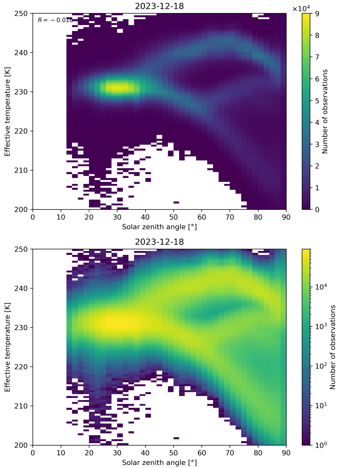
Figure 45: Scatter density plot of “Solar zenith angle” against “Effective temperature” for 2023-12-17 to 2023-12-19.
