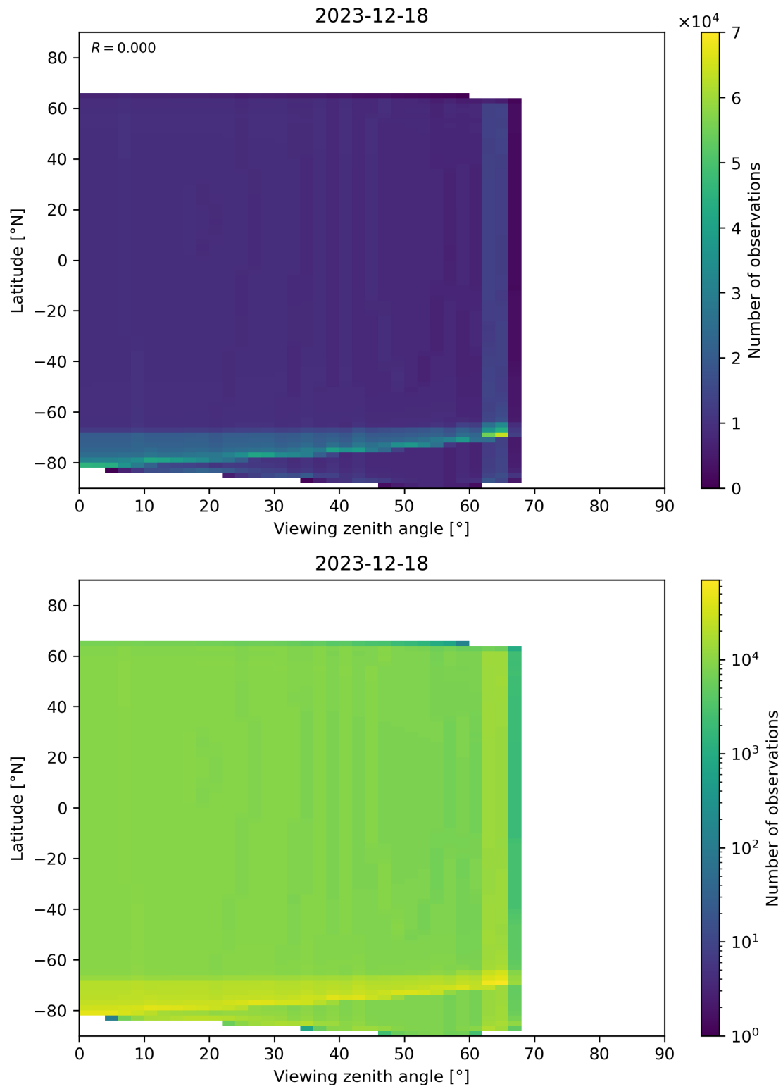
Figure 49: Scatter density plot of “Viewing zenith angle” against “Latitude” for 2023-12-17 to 2023-12-19.
