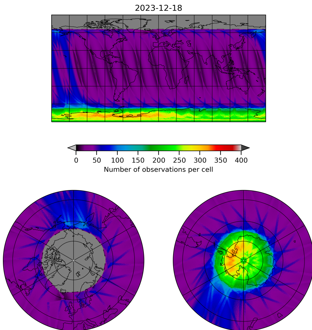
Figure 12: Map of the number of observations for 2023-12-17 to 2023-12-19
