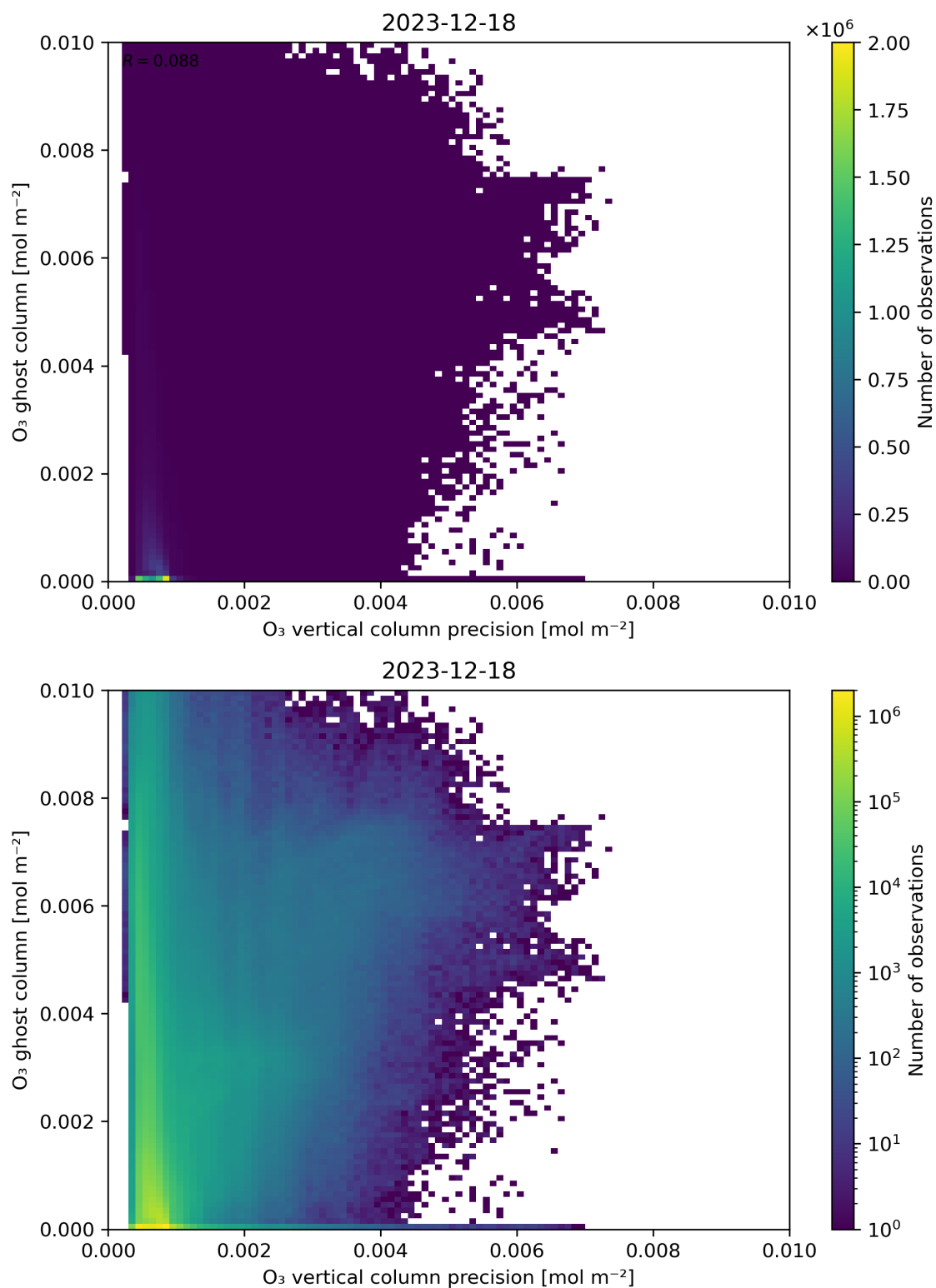
Figure 43: Scatter density plot of “O 3 vertical column precision” against “O 3 ghost column” for 2023-12-17 to 2023-12-19.
