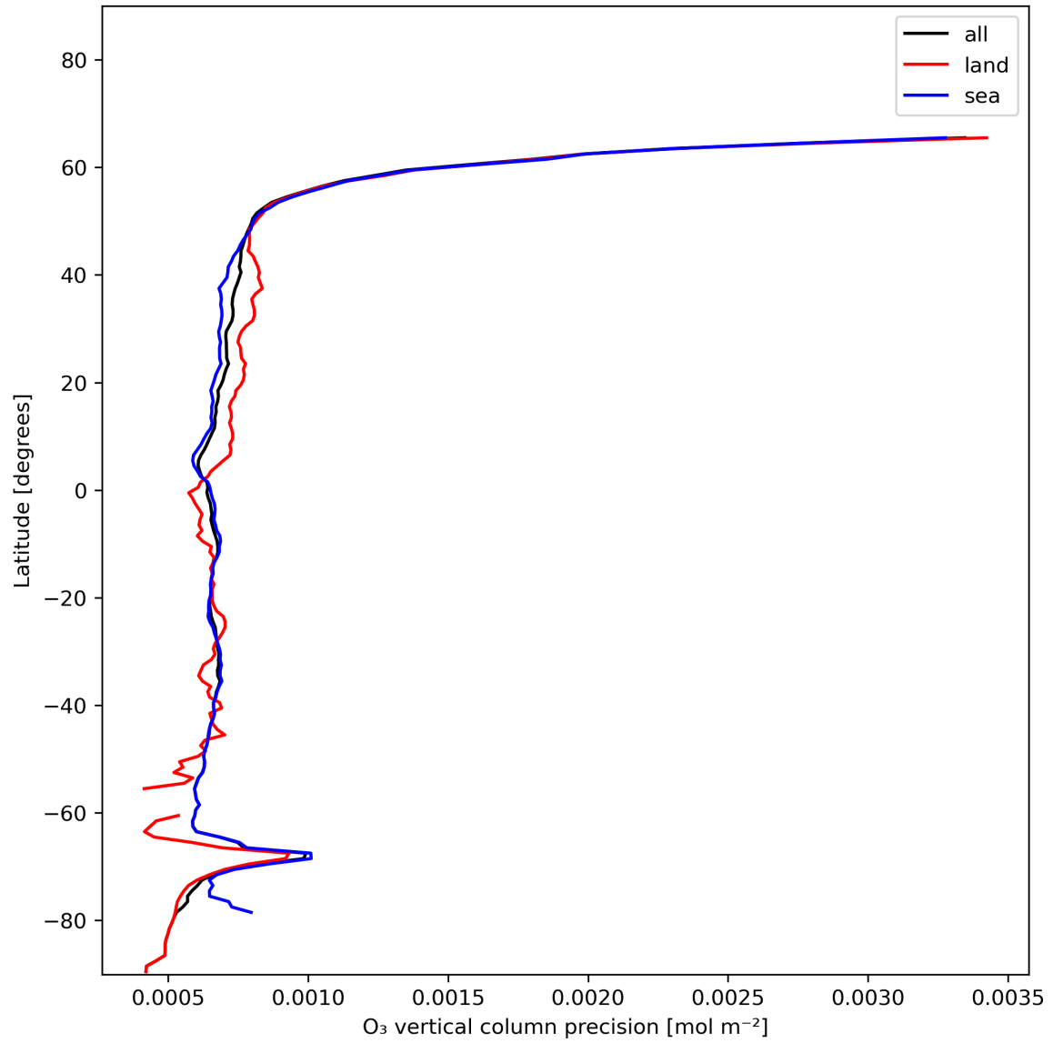
Figure 15: Zonal average of “O 3 vertical column precision” for 2023-12-17 to 2023-12-19.
