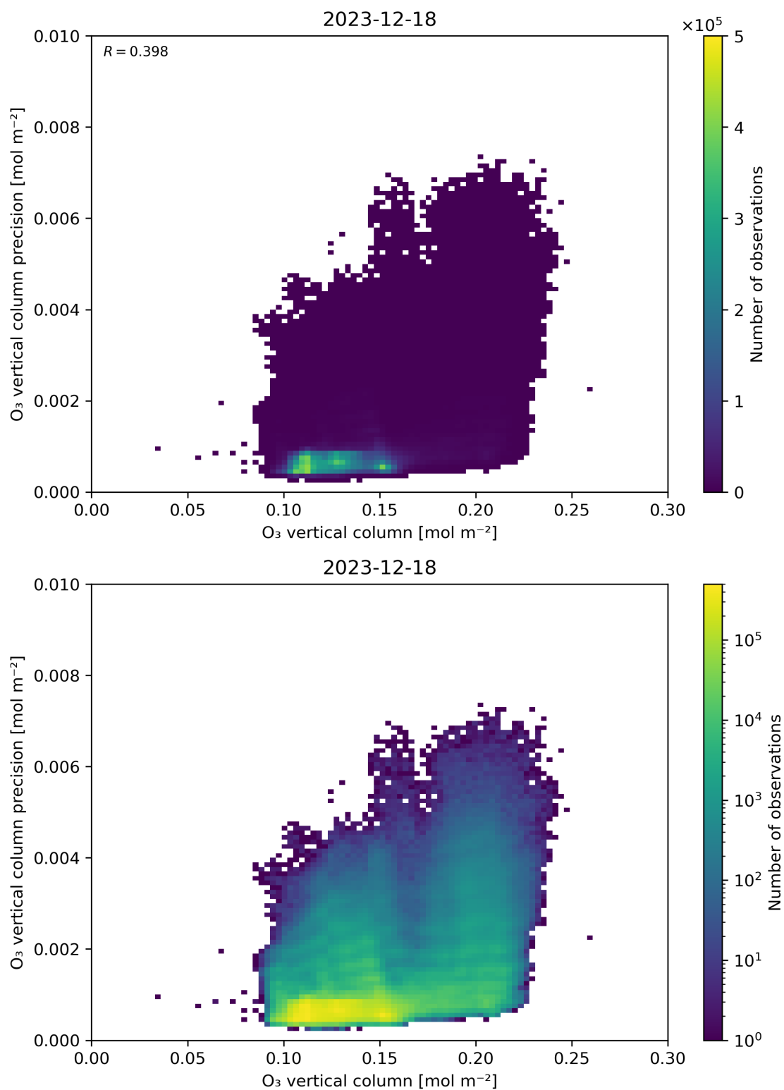
Figure 41: Scatter density plot of “O 3 vertical column” against “O 3 vertical column precision” for 2023-12-17 to 2023-12-19.
