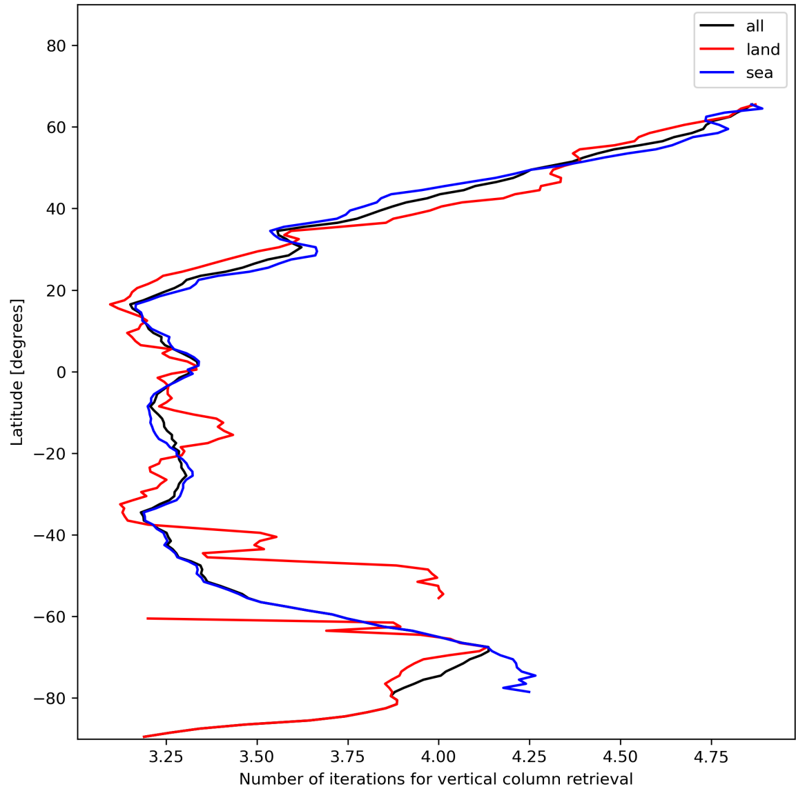
Figure 19: Zonal average of “Number of iterations for vertical column retrieval” for 2023-12-17 to 2023-12-19.
