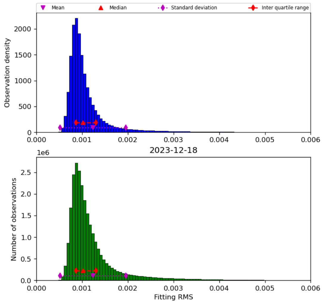
Figure 23: Histogram of “Fitting RMS” for 2023-12-17 to 2023-12-19
