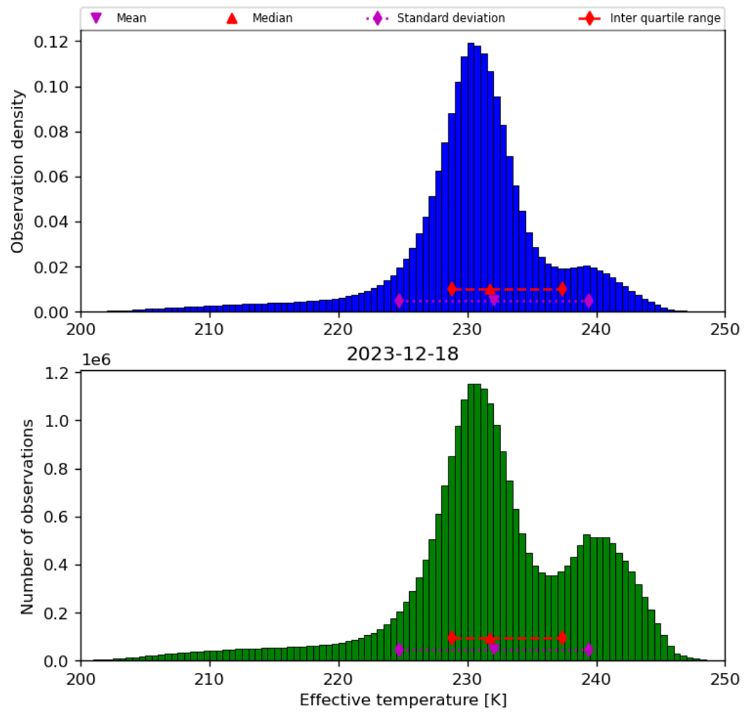
Figure 24: Histogram of “Effective temperature” for 2023-12-17 to 2023-12-19
