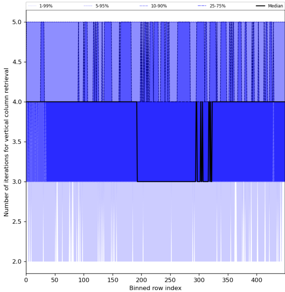
Figure 33: Along track statistics of “Number of iterations for vertical column retrieval” for 2023-12-17 to 2023-12-19
