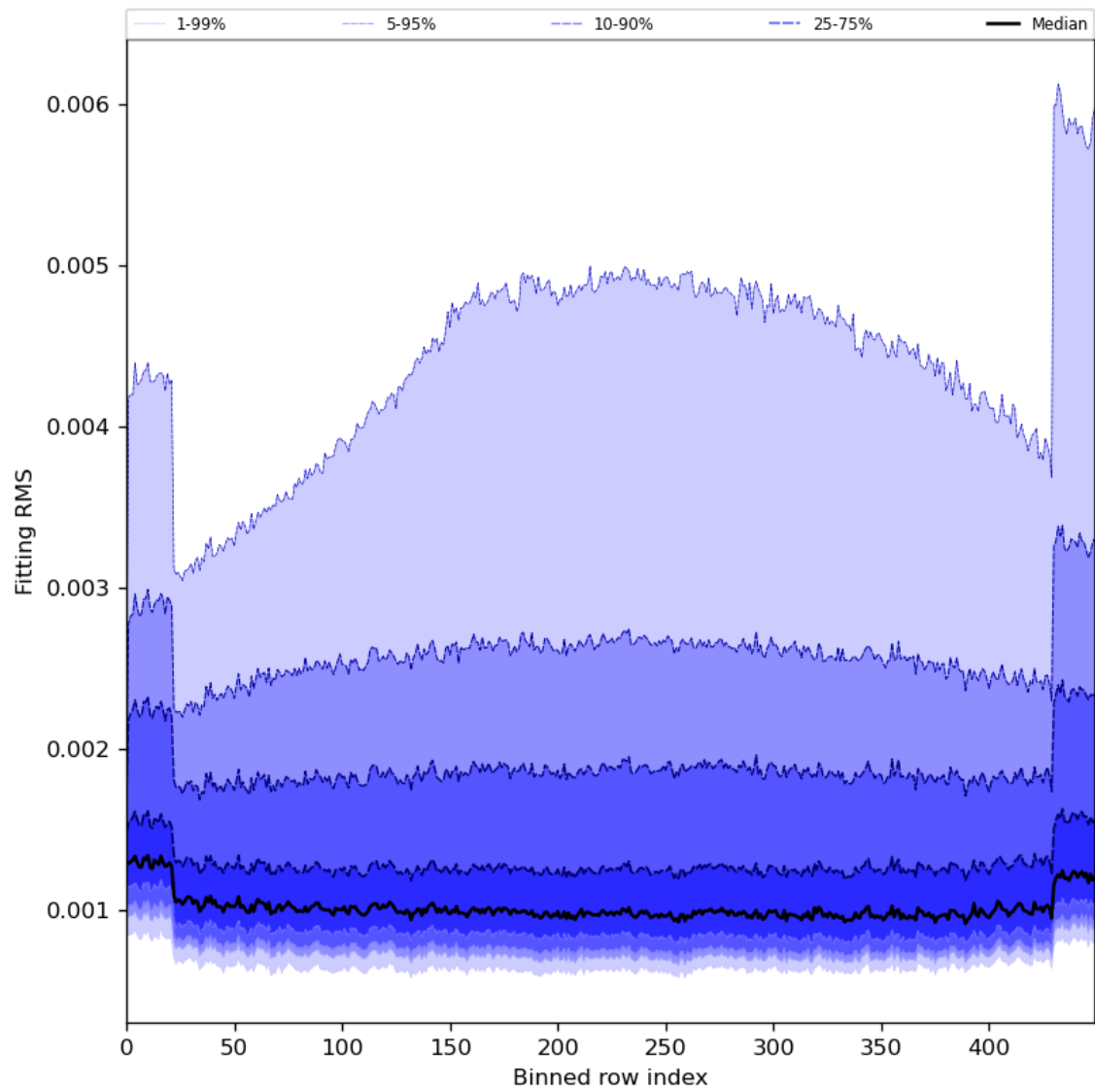
Figure 30: Along track statistics of “Fitting RMS” for 2023-12-17 to 2023-12-19
