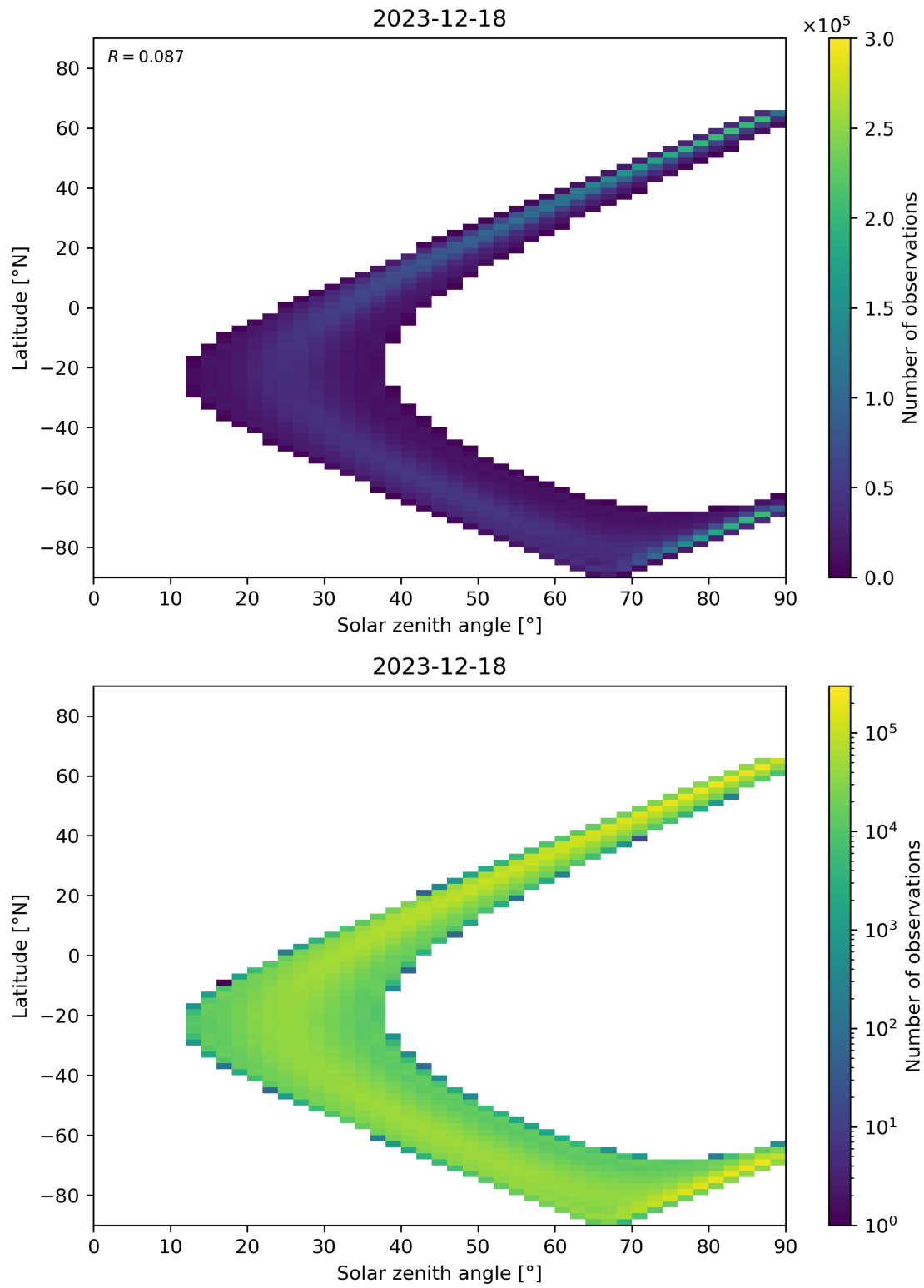
Figure 44: Scatter density plot of “Solar zenith angle” against “Latitude” for 2023-12-17 to 2023-12-19.
