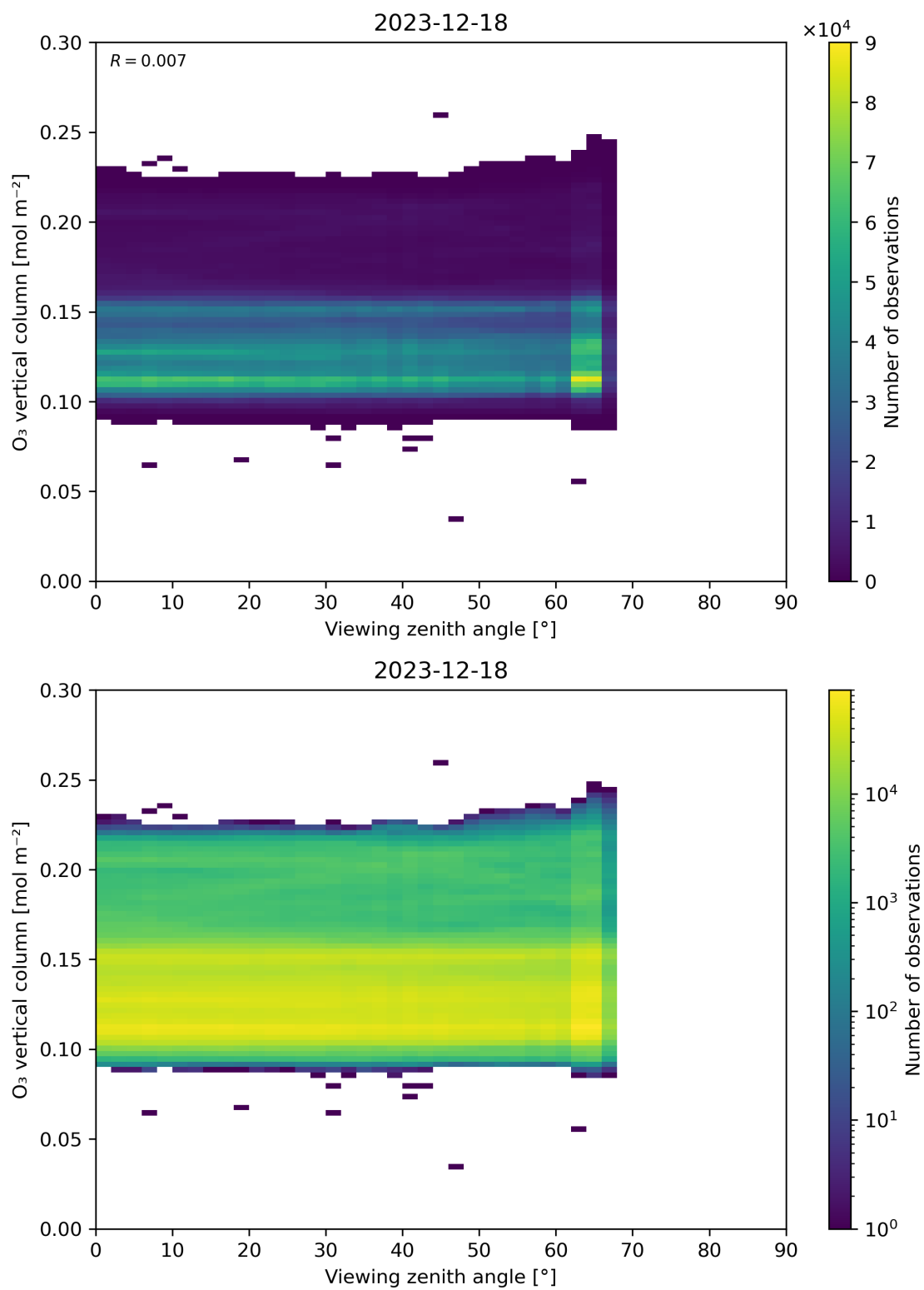
Figure 52: Scatter density plot of “Viewing zenith angle” against “O 3 vertical column” for 2023-12-17 to 2023-12-19.
