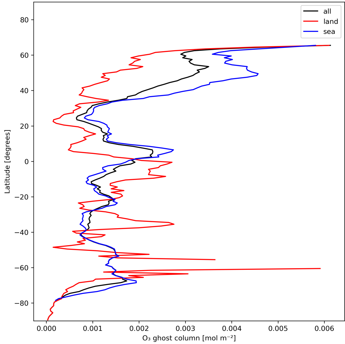
Figure 18: Zonal average of “O 3 ghost column” for 2023-12-17 to 2023-12-19.
