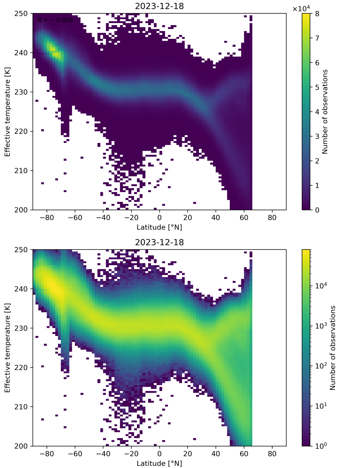
Figure 34: Scatter density plot of “Latitude” against “Effective temperature” for 2023-12-17 to 2023-12-19.
