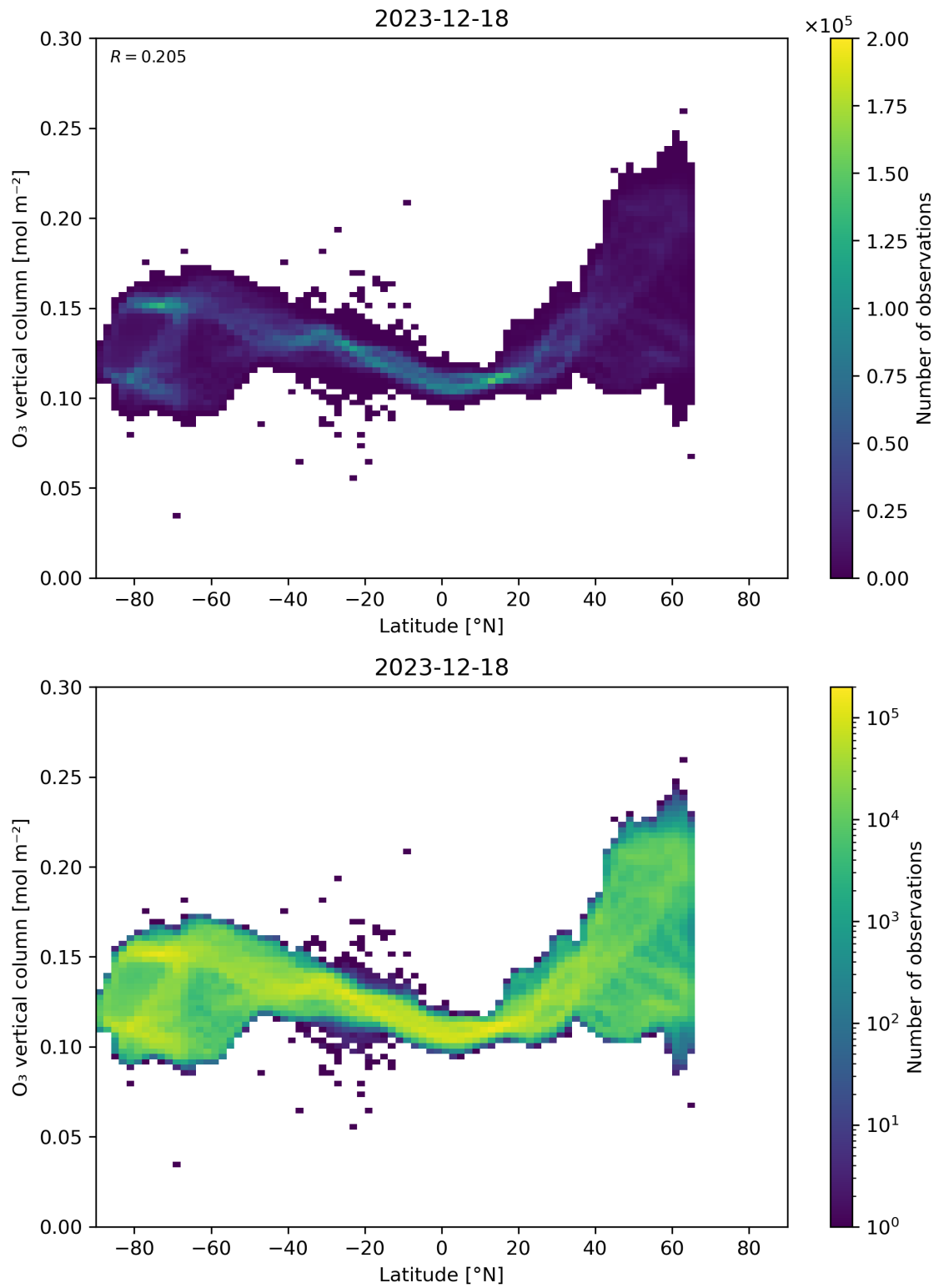
Figure 36: Scatter density plot of “Latitude” against “O 3 vertical column” for 2023-12-17 to 2023-12-19.
