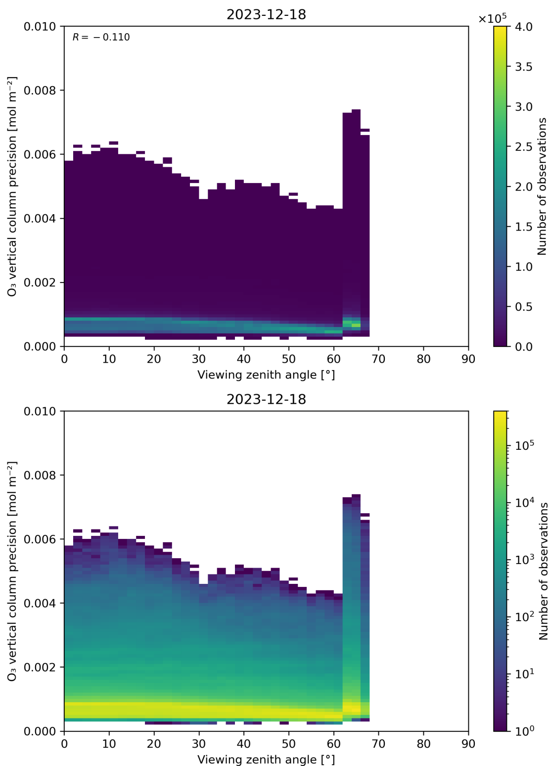
Figure 53: Scatter density plot of “Viewing zenith angle” against “O 3 vertical column precision” for 2023-12-17 to 2023-12-19.
