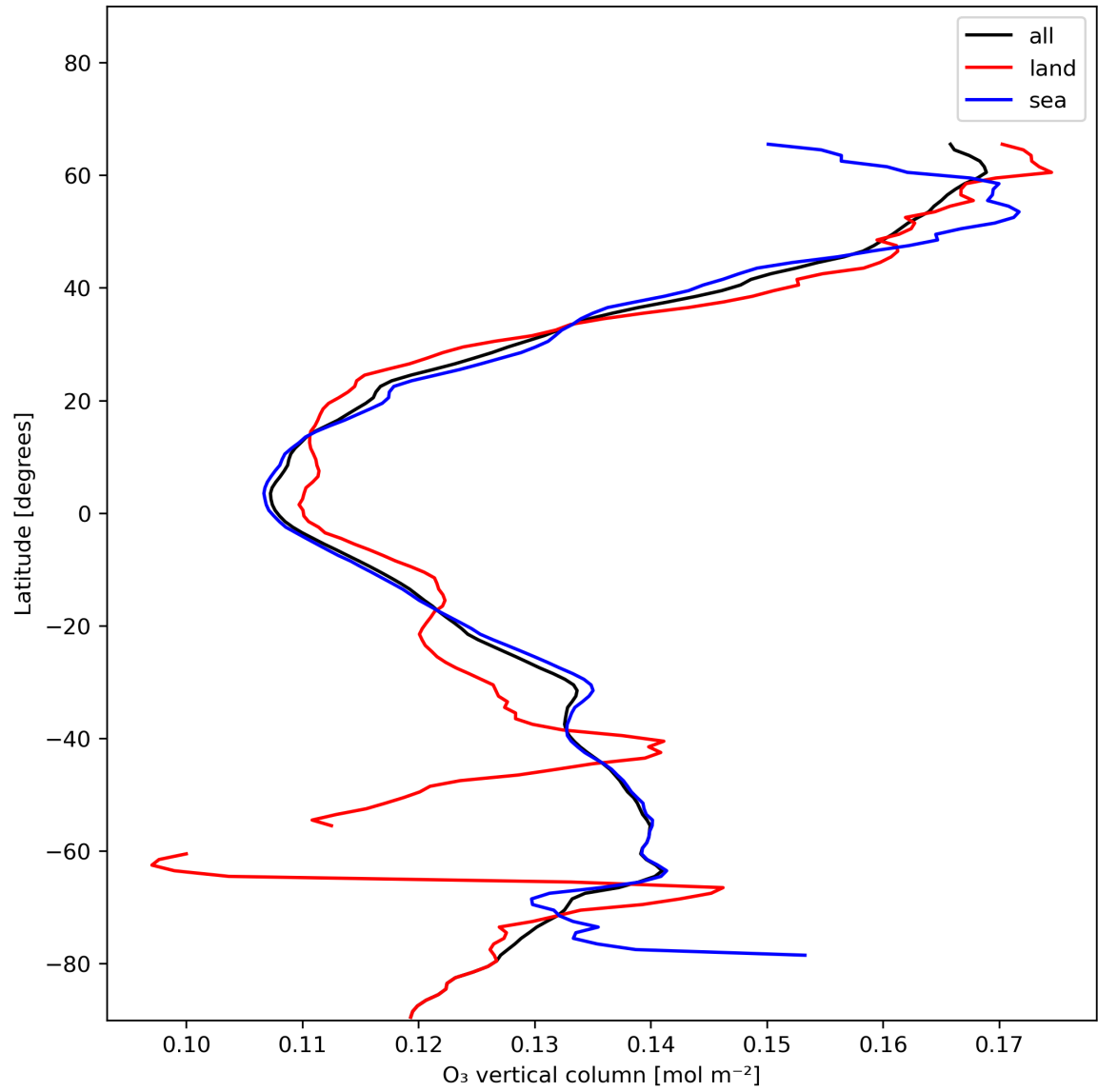
Figure 14: Zonal average of “O 3 vertical column” for 2023-12-17 to 2023-12-19.
