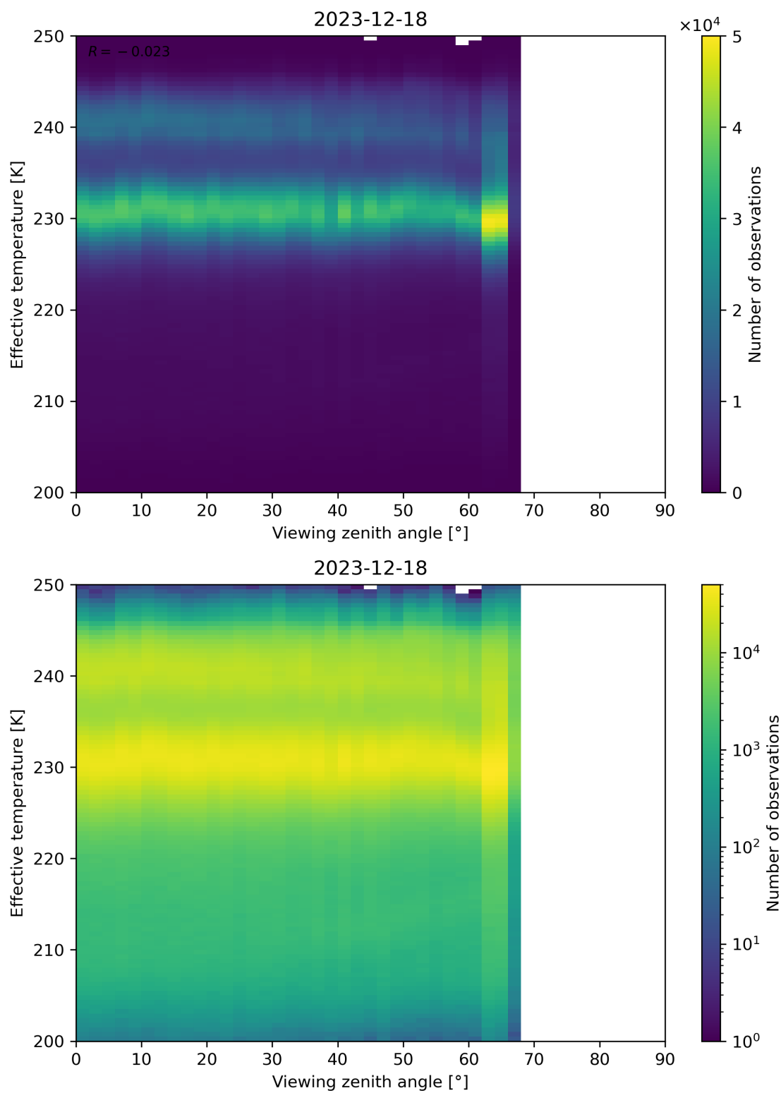
Figure 50: Scatter density plot of “Viewing zenith angle” against “Effective temperature” for 2023-12-17 to 2023-12-19.
