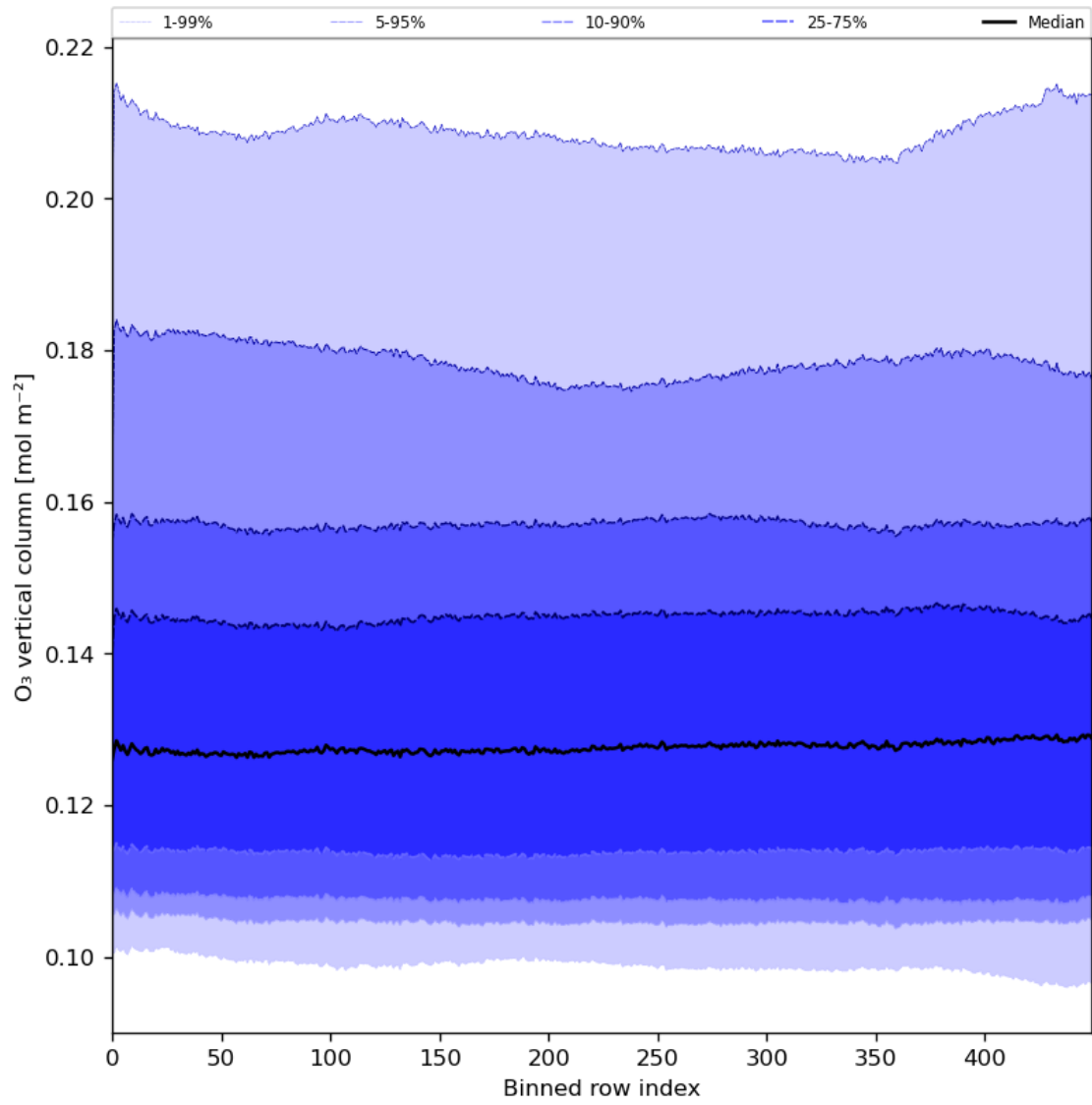
Figure 28: Along track statistics of “O 3 vertical column” for 2023-12-17 to 2023-12-19
