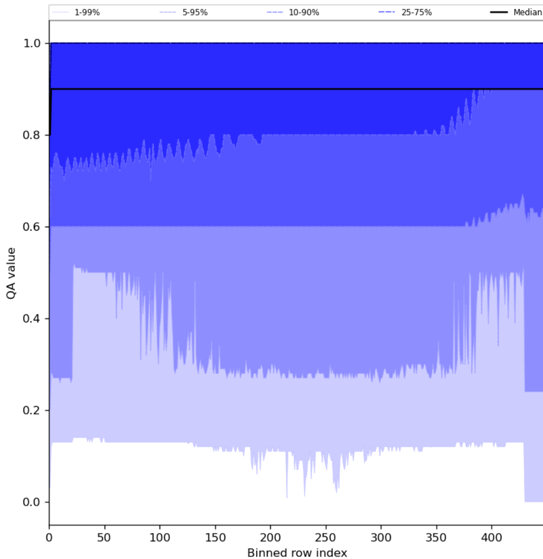
Figure 27: Along track statistics of “QA value” for 2023-12-17 to 2023-12-19
