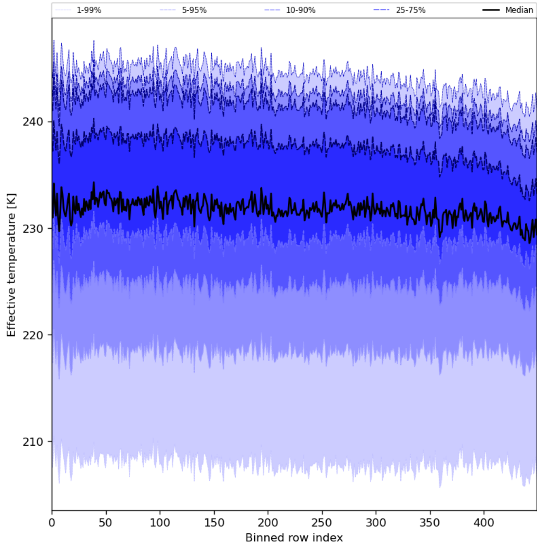
Figure 31: Along track statistics of “Effective temperature” for 2023-12-17 to 2023-12-19
