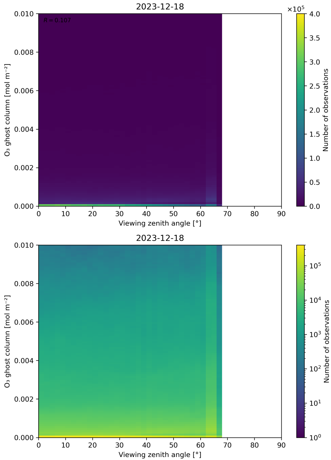
Figure 51: Scatter density plot of “Viewing zenith angle” against “O 3 ghost column” for 2023-12-17 to 2023-12-19.
