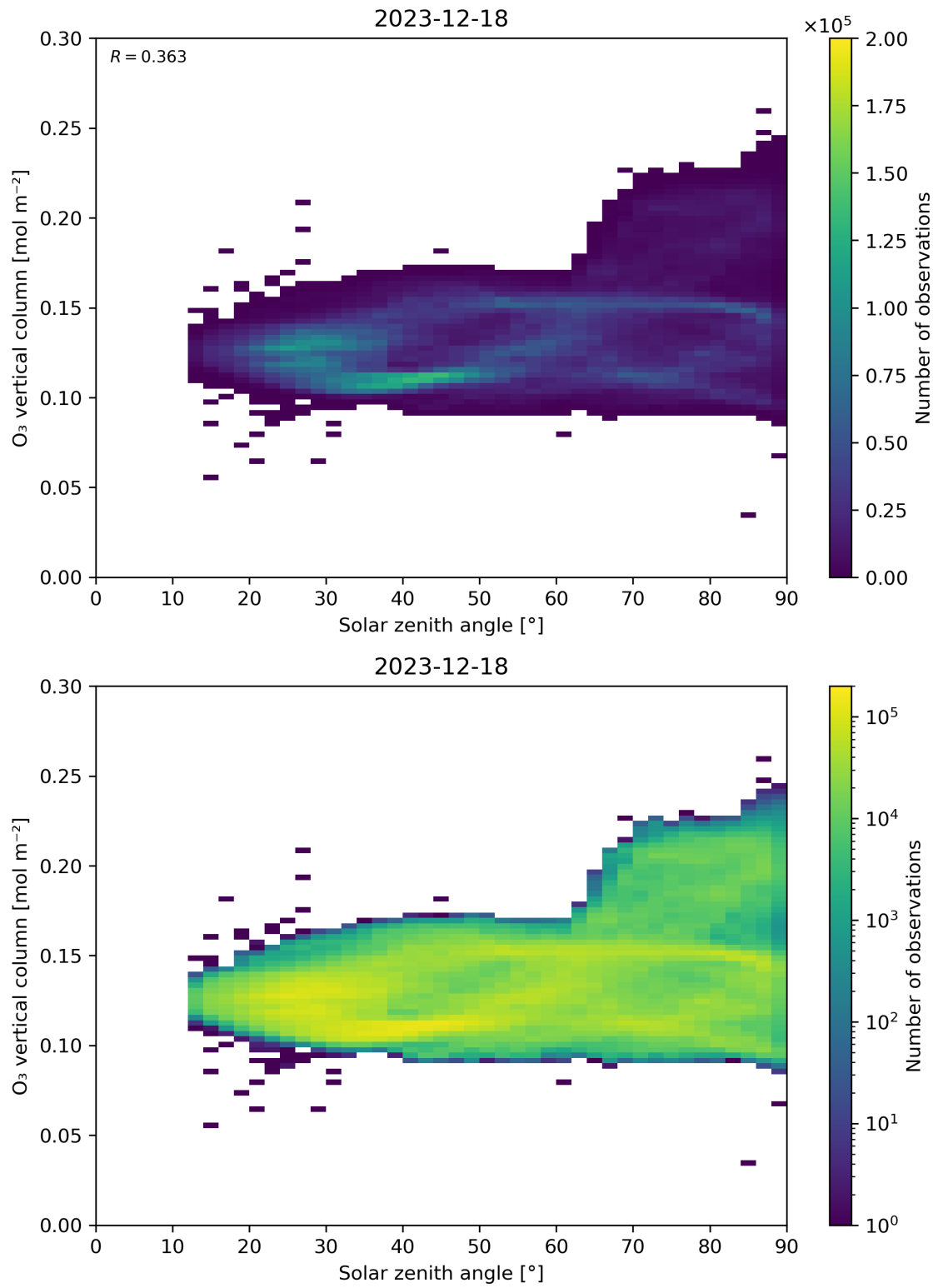
Figure 47: Scatter density plot of “Solar zenith angle” against “O 3 vertical column” for 2023-12-17 to 2023-12-19.
