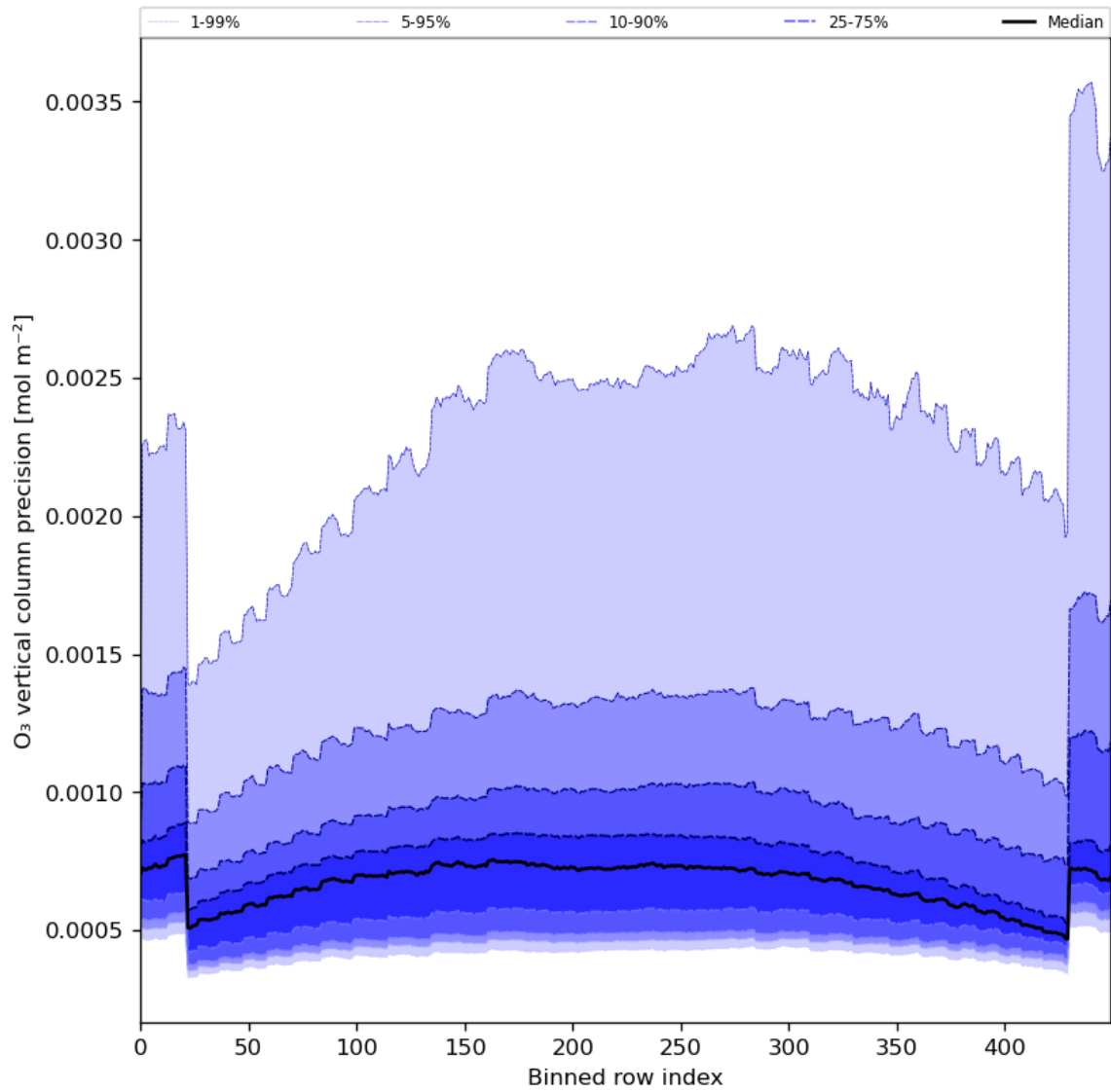
Figure 29: Along track statistics of “O 3 vertical column precision” for 2023-12-17 to 2023-12-19
