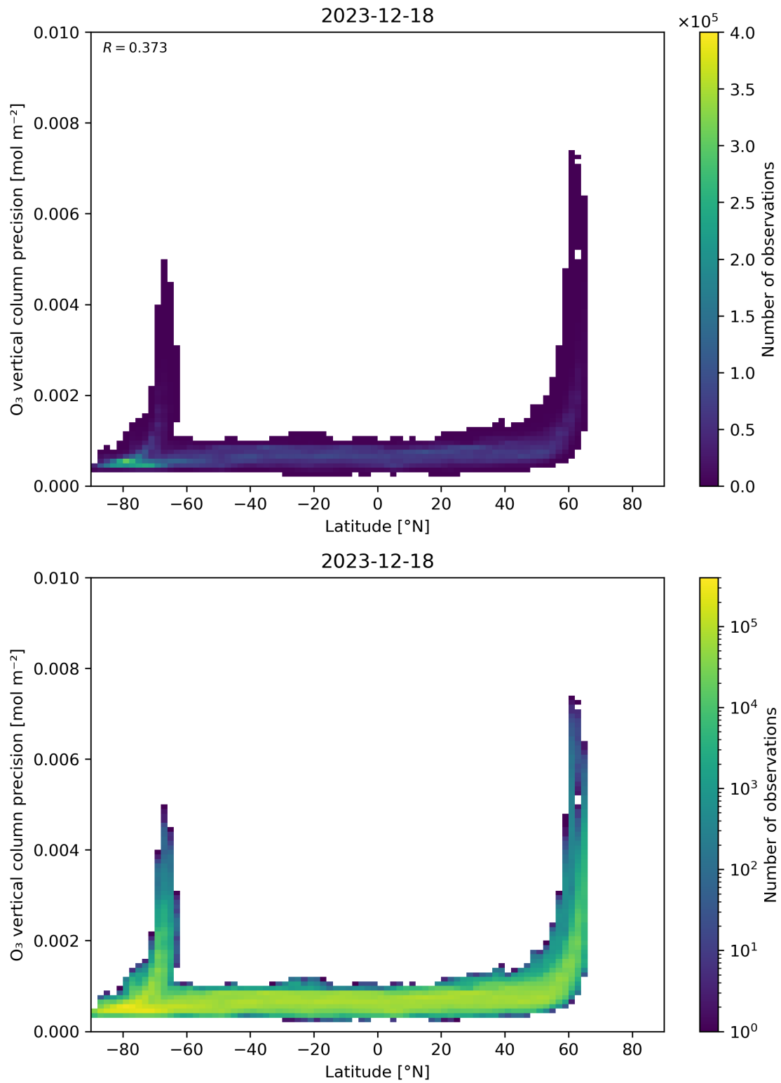
Figure 37: Scatter density plot of “Latitude” against “O 3 vertical column precision” for 2023-12-17 to 2023-12-19.
