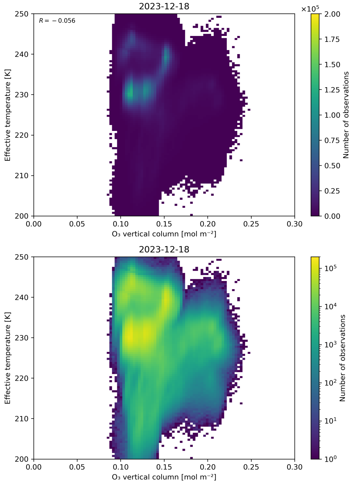
Figure 39: Scatter density plot of “O 3 vertical column” against “Effective temperature” for 2023-12-17 to 2023-12-19.
