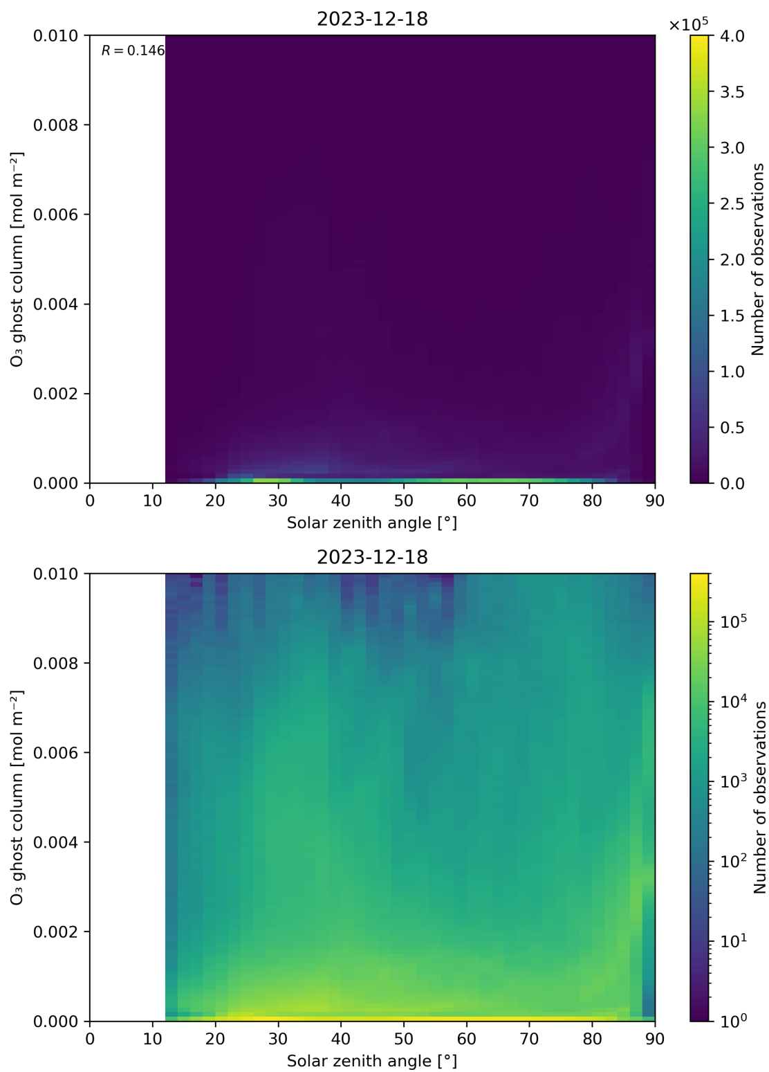
Figure 46: Scatter density plot of “Solar zenith angle” against “O 3 ghost column” for 2023-12-17 to 2023-12-19.
