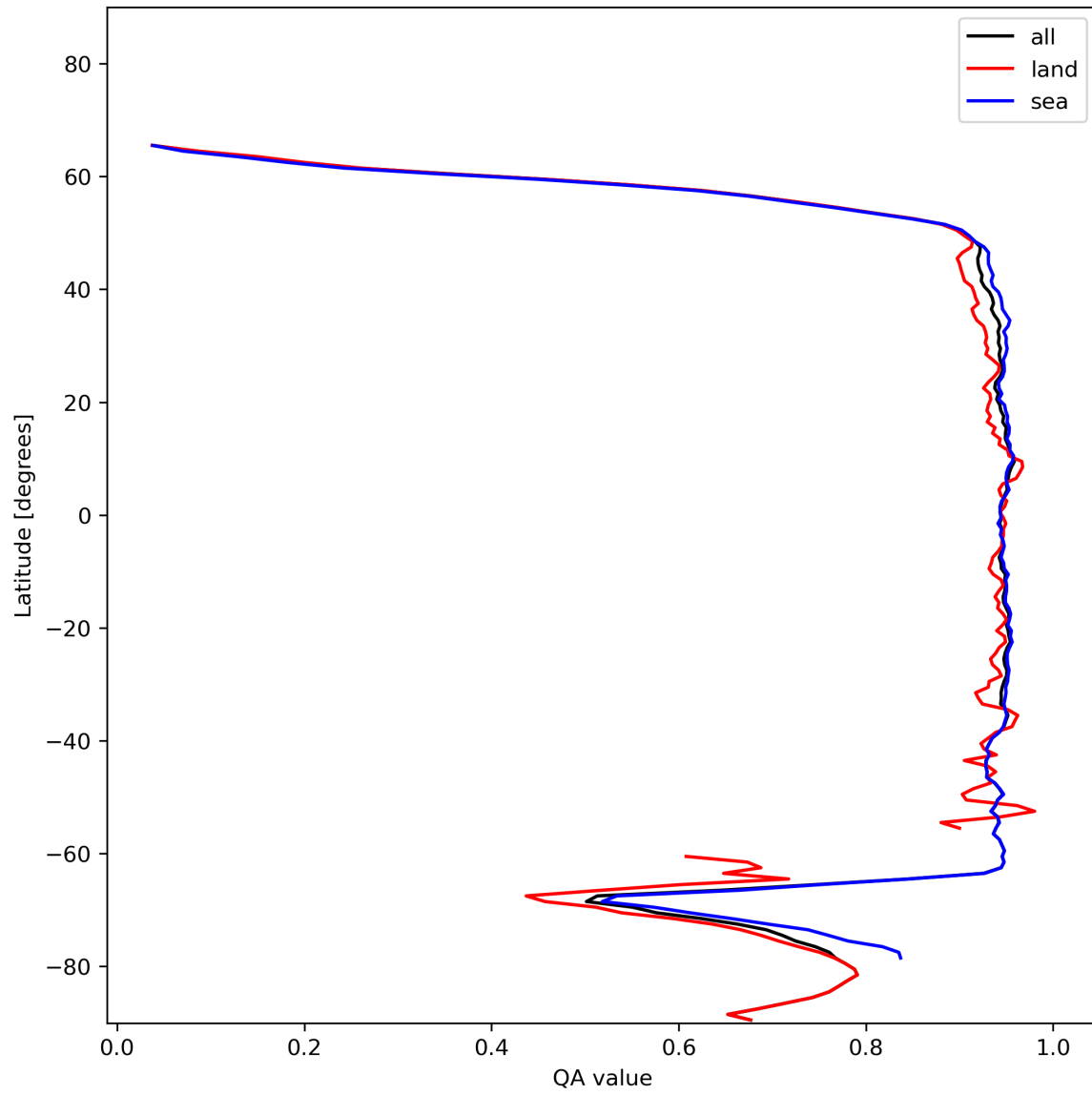
Figure 13: Zonal average of “QA value” for 2023-12-17 to 2023-12-19.
