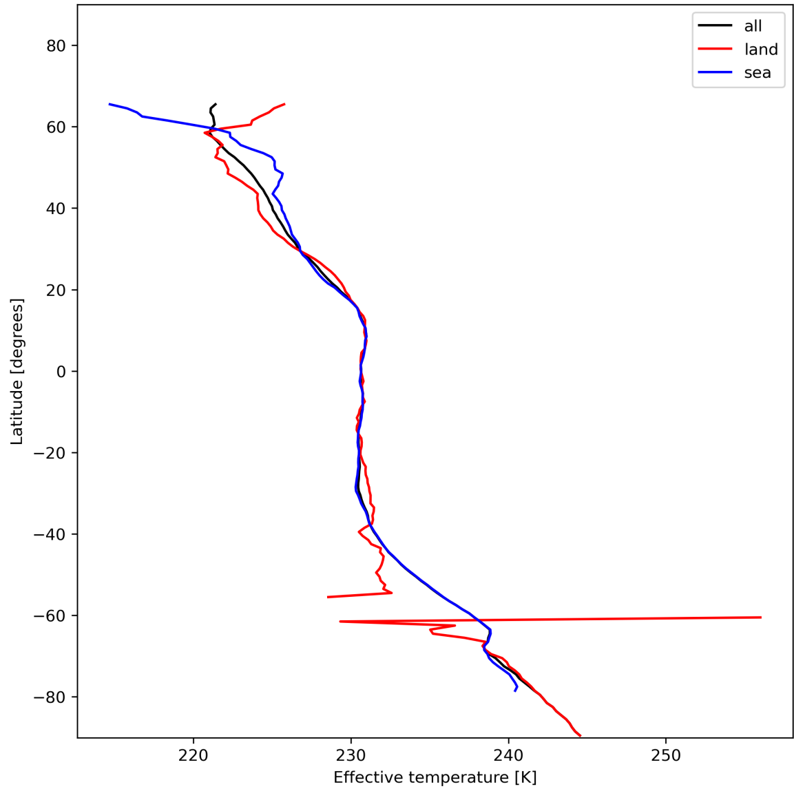
Figure 17: Zonal average of “Effective temperature” for 2023-12-18 to 2023-12-20.
