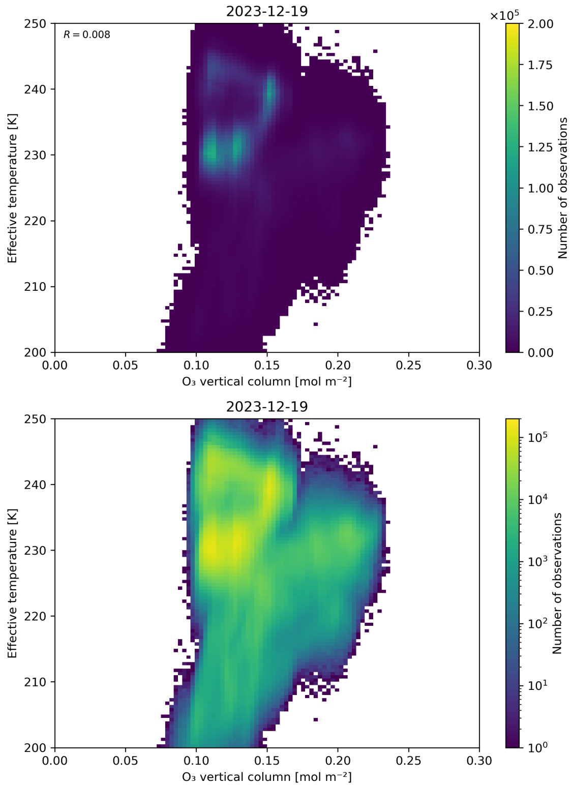
Figure 39: Scatter density plot of “O 3 vertical column” against “Effective temperature” for 2023-12-18 to 2023-12-20.
