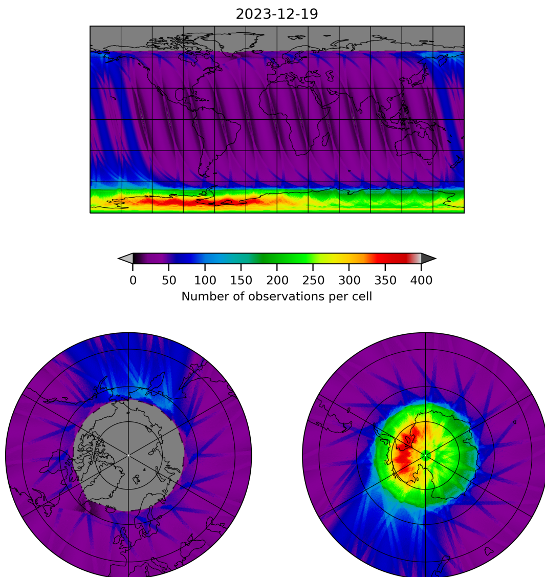
Figure 12: Map of the number of observations for 2023-12-18 to 2023-12-20
