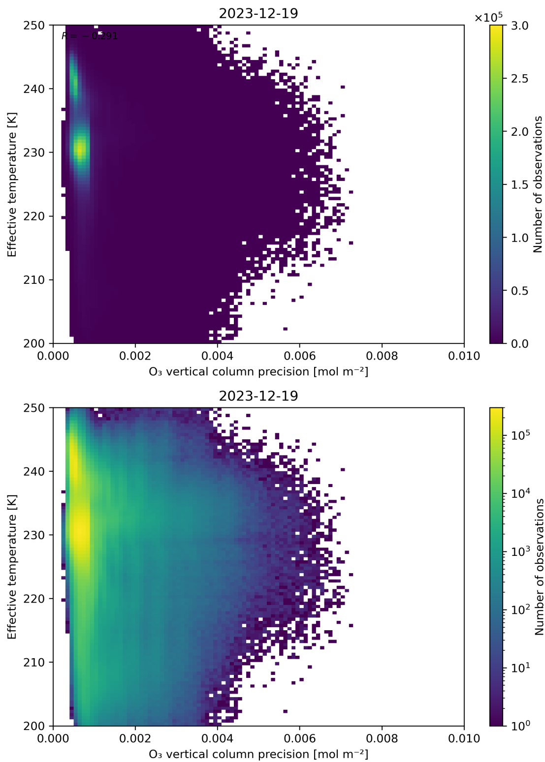
Figure 42: Scatter density plot of “O 3 vertical column precision” against “Effective temperature” for 2023-12-18 to 2023-12-20.
