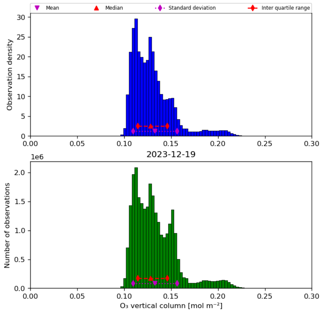
Figure 21: Histogram of “O 3 vertical column” for 2023-12-18 to 2023-12-20
