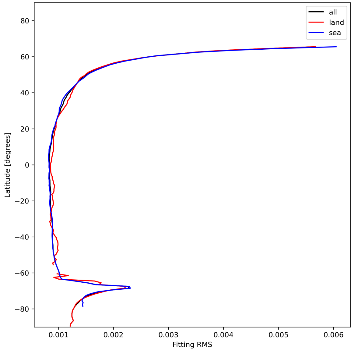
Figure 16: Zonal average of “Fitting RMS” for 2023-12-18 to 2023-12-20.
