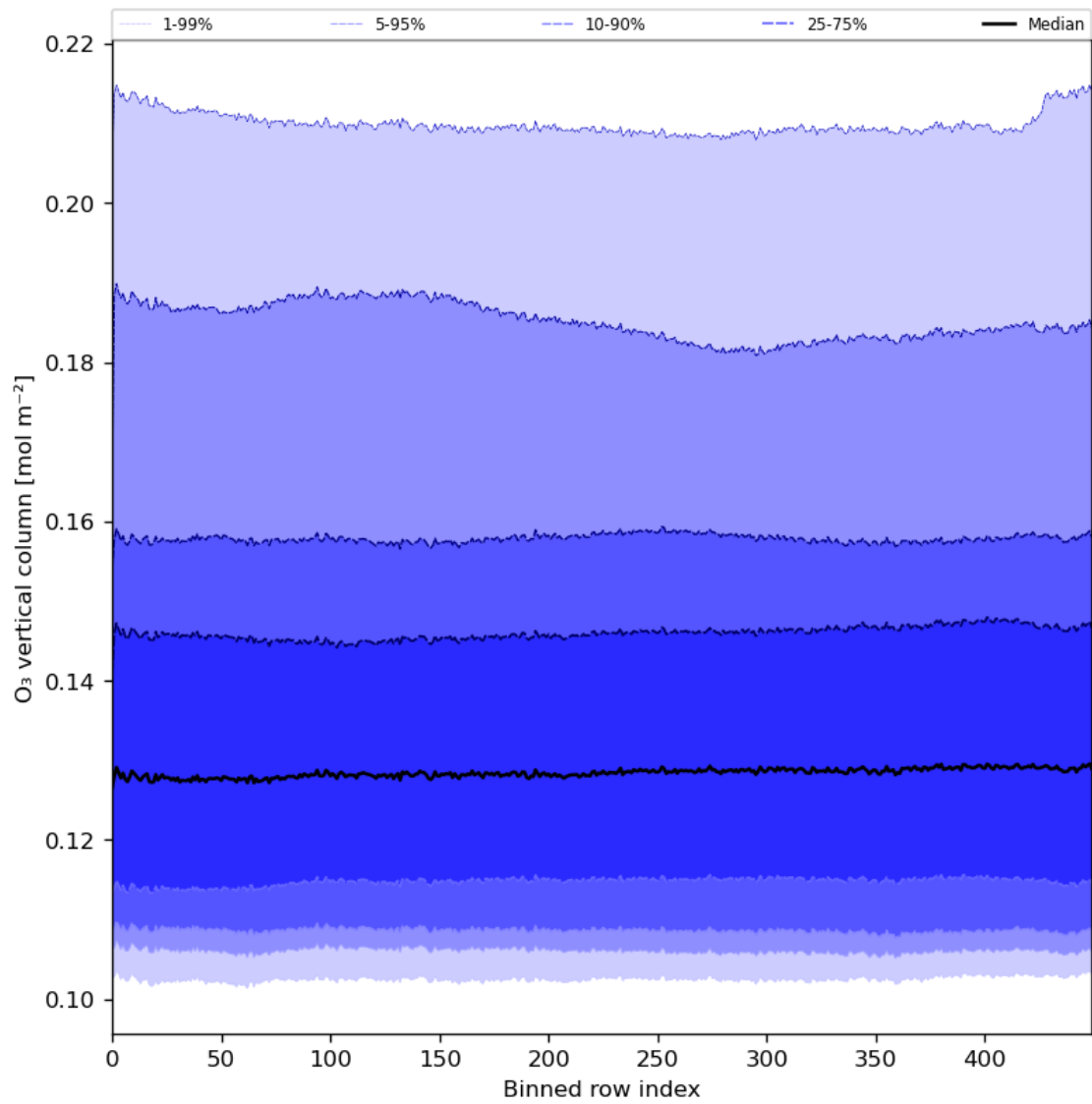
Figure 28: Along track statistics of “O 3 vertical column” for 2023-12-18 to 2023-12-20
