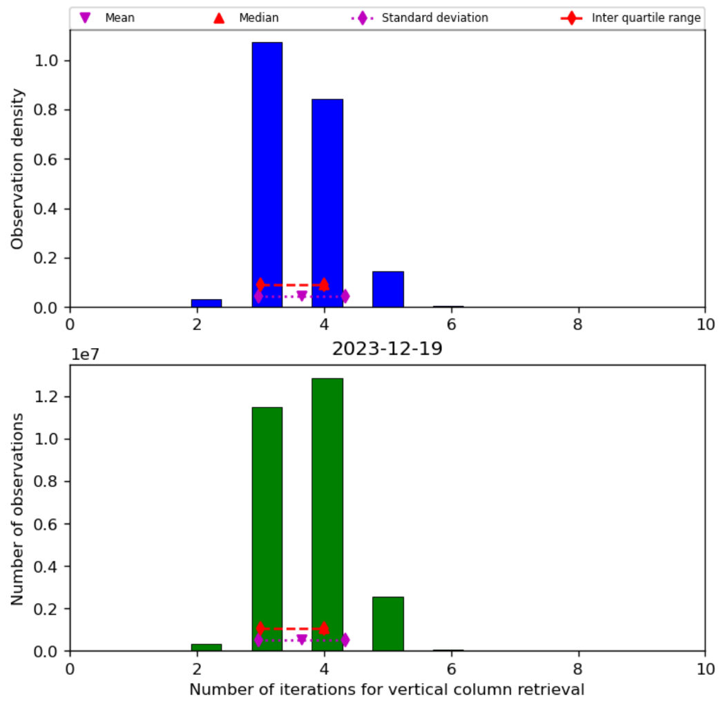
Figure 26: Histogram of “Number of iterations for vertical column retrieval” for 2023-12-18 to 2023-12-20
