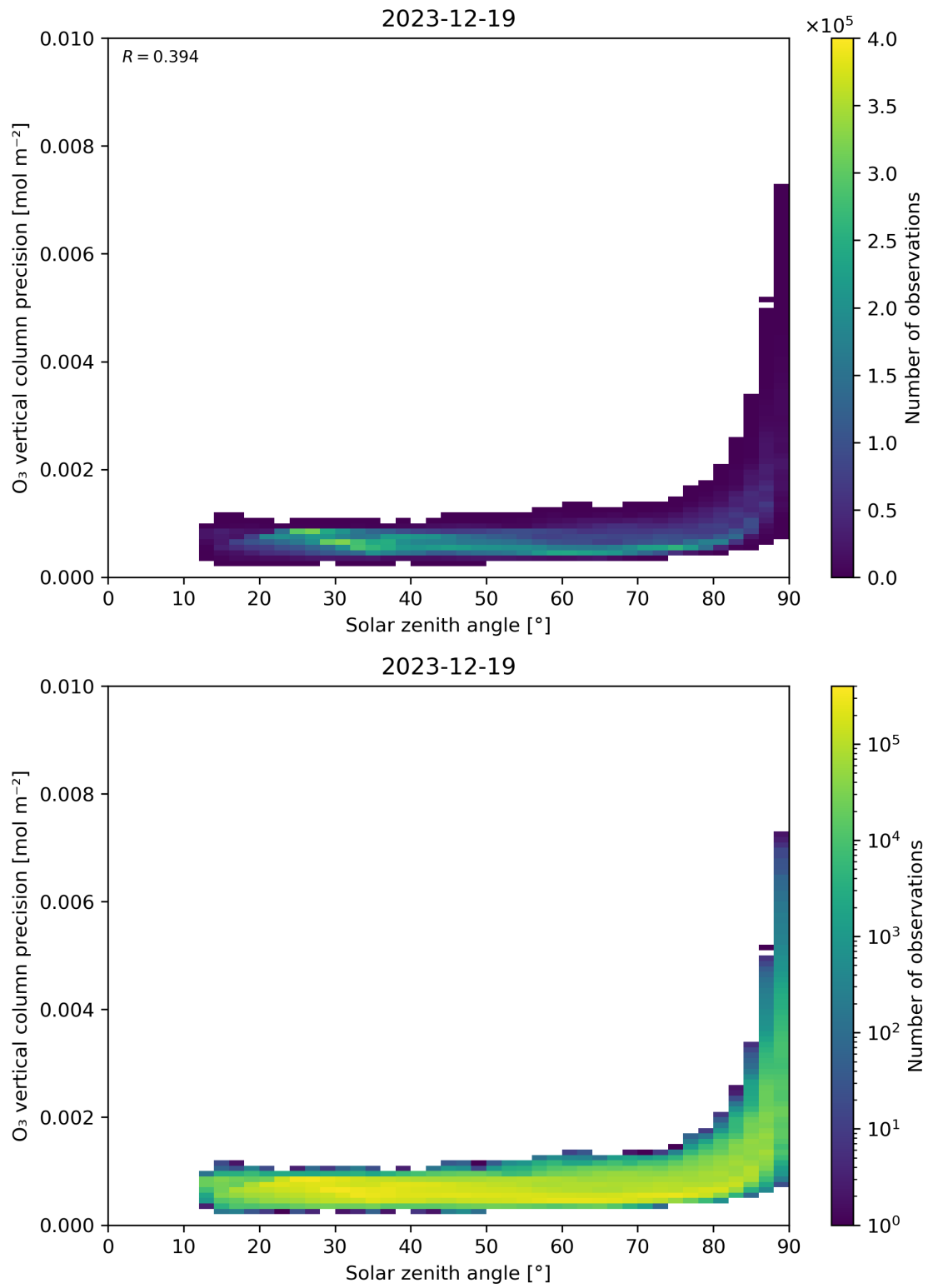
Figure 48: Scatter density plot of “Solar zenith angle” against “O 3 vertical column precision” for 2023-12-18 to 2023-12-20.
