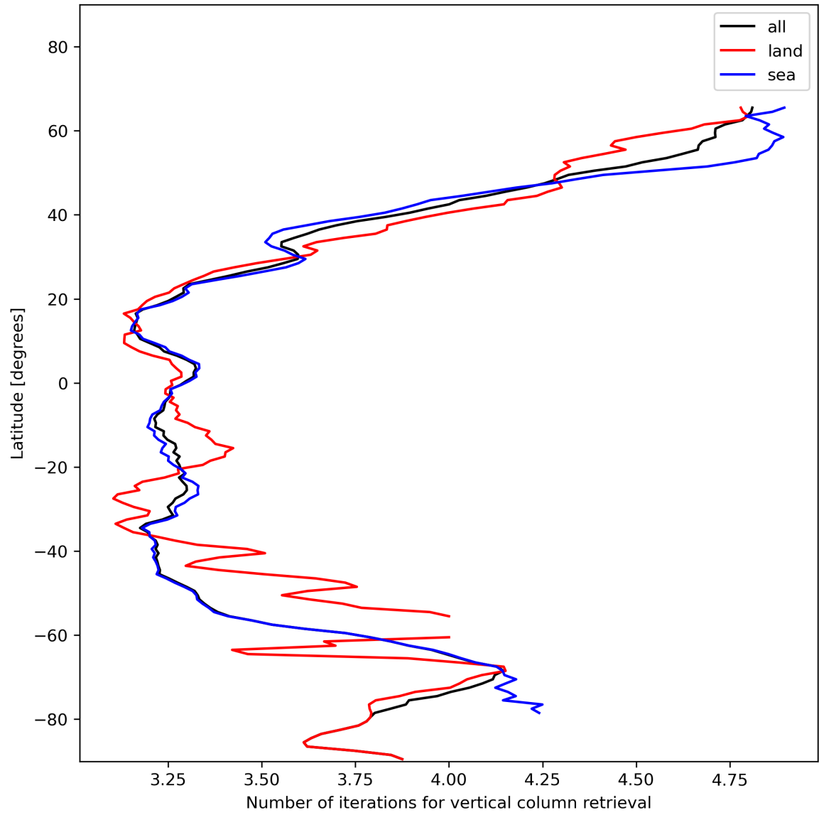
Figure 19: Zonal average of “Number of iterations for vertical column retrieval” for 2023-12-18 to 2023-12-20.
