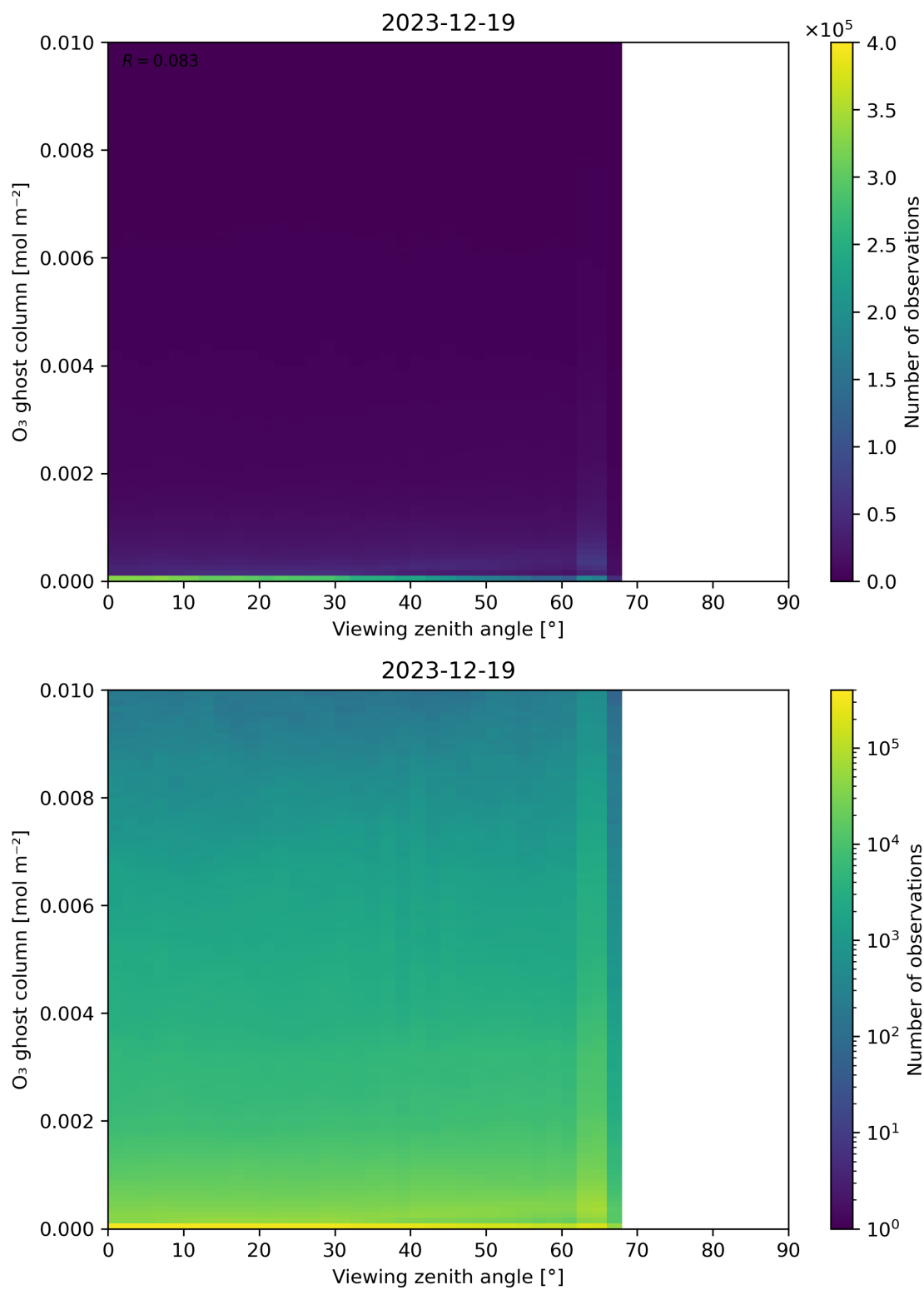
Figure 51: Scatter density plot of “Viewing zenith angle” against “O 3 ghost column” for 2023-12-18 to 2023-12-20.
