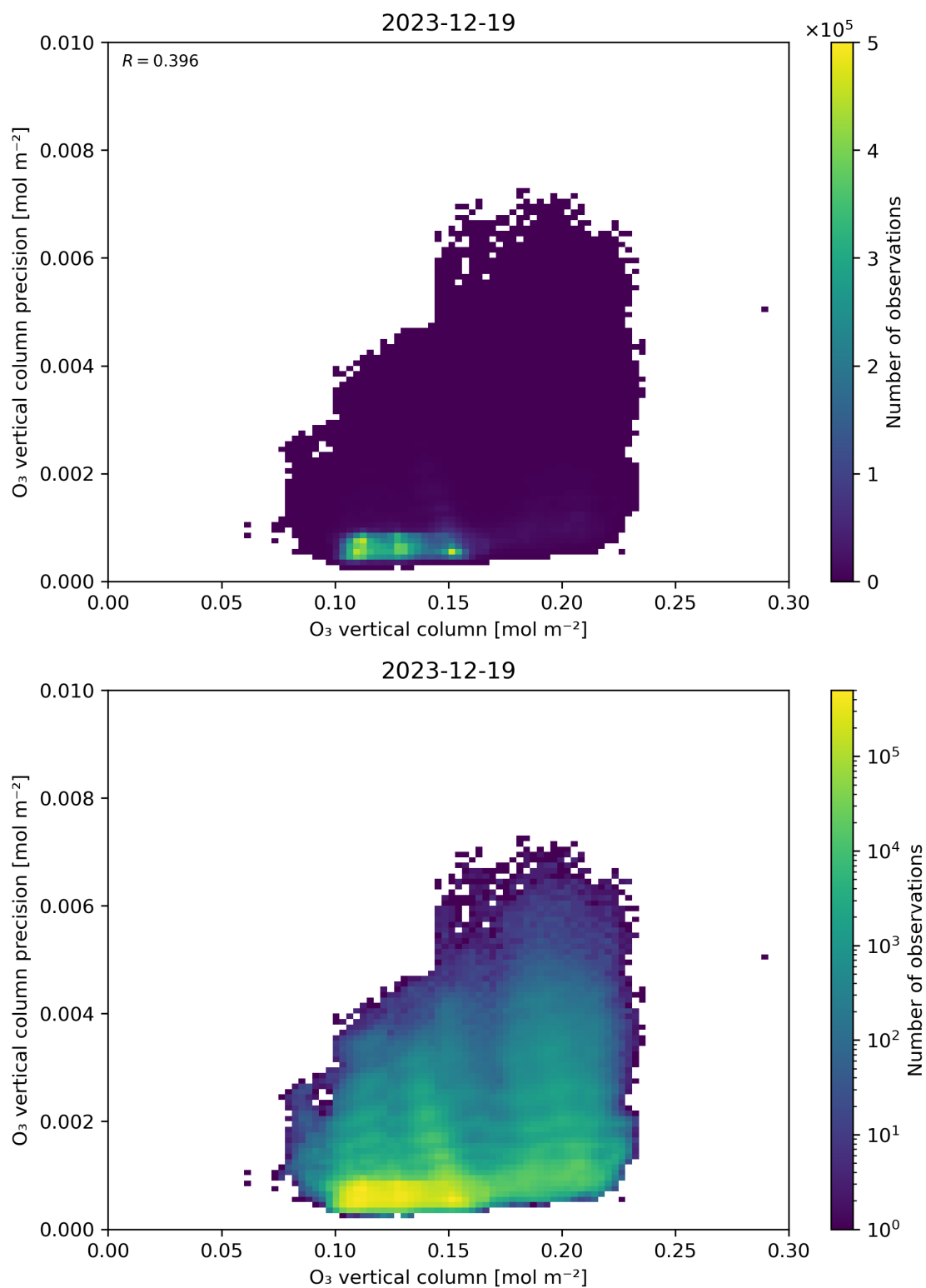
Figure 41: Scatter density plot of “O 3 vertical column” against “O 3 vertical column precision” for 2023-12-18 to 2023-12-20.
