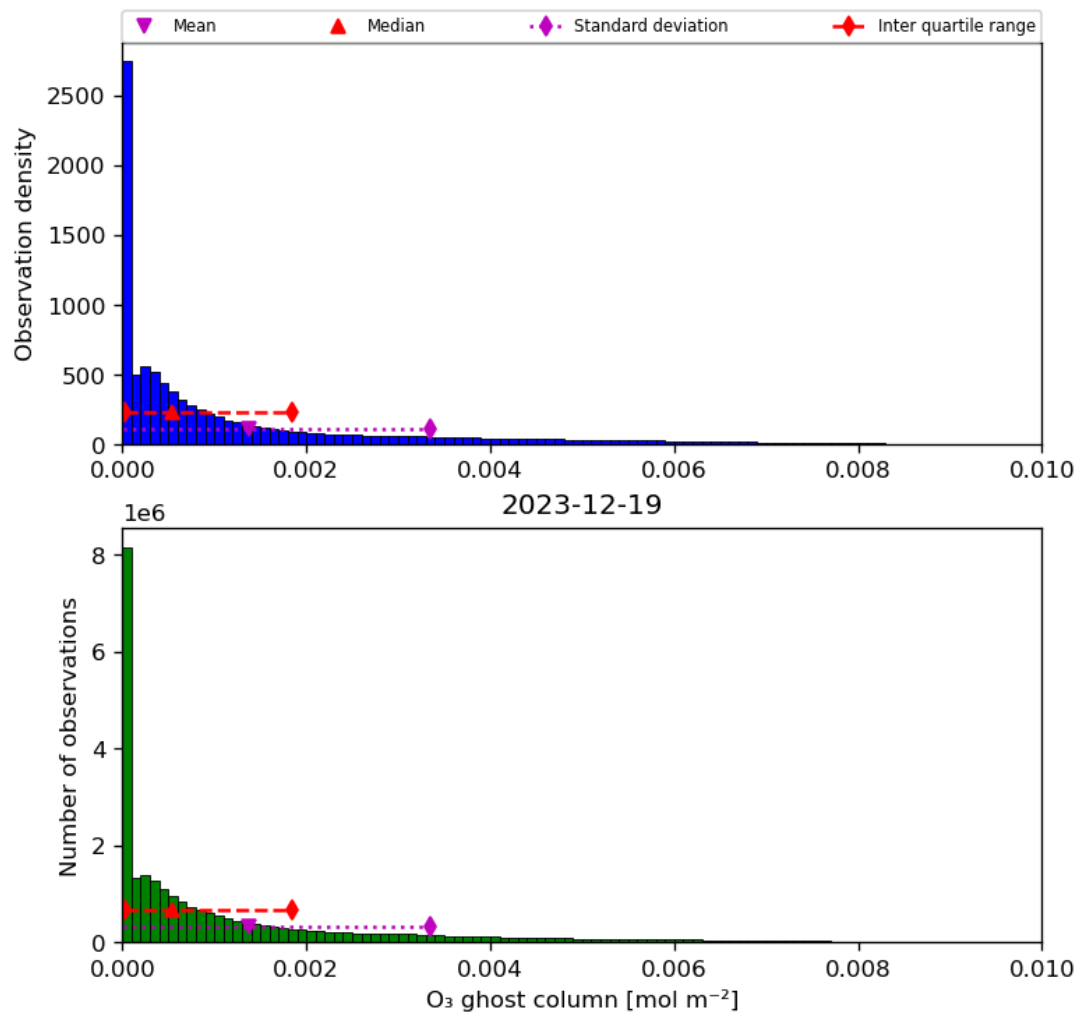
Figure 25: Histogram of “O 3 ghost column” for 2023-12-18 to 2023-12-20
