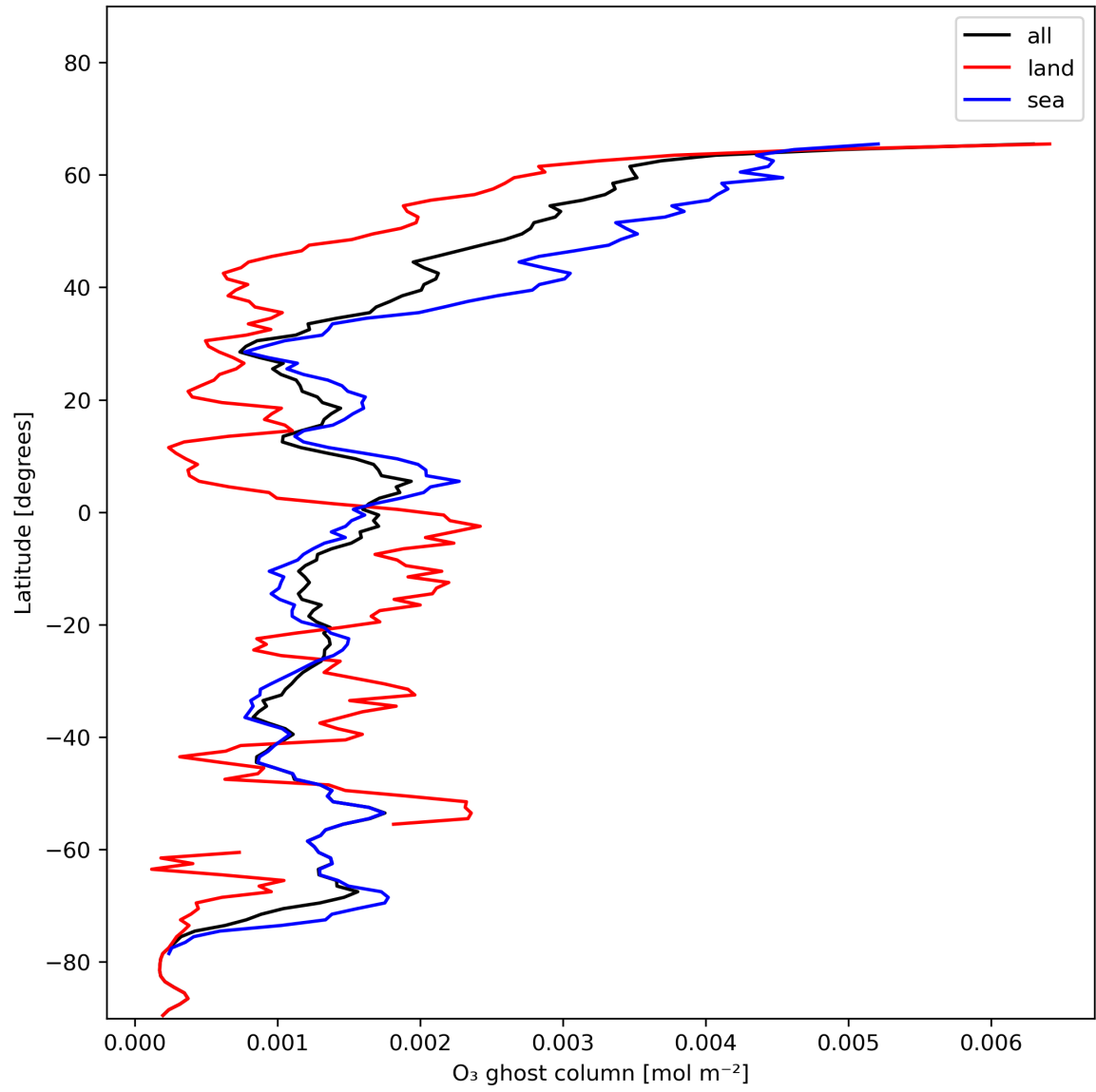
Figure 18: Zonal average of “O 3 ghost column” for 2023-12-18 to 2023-12-20.
