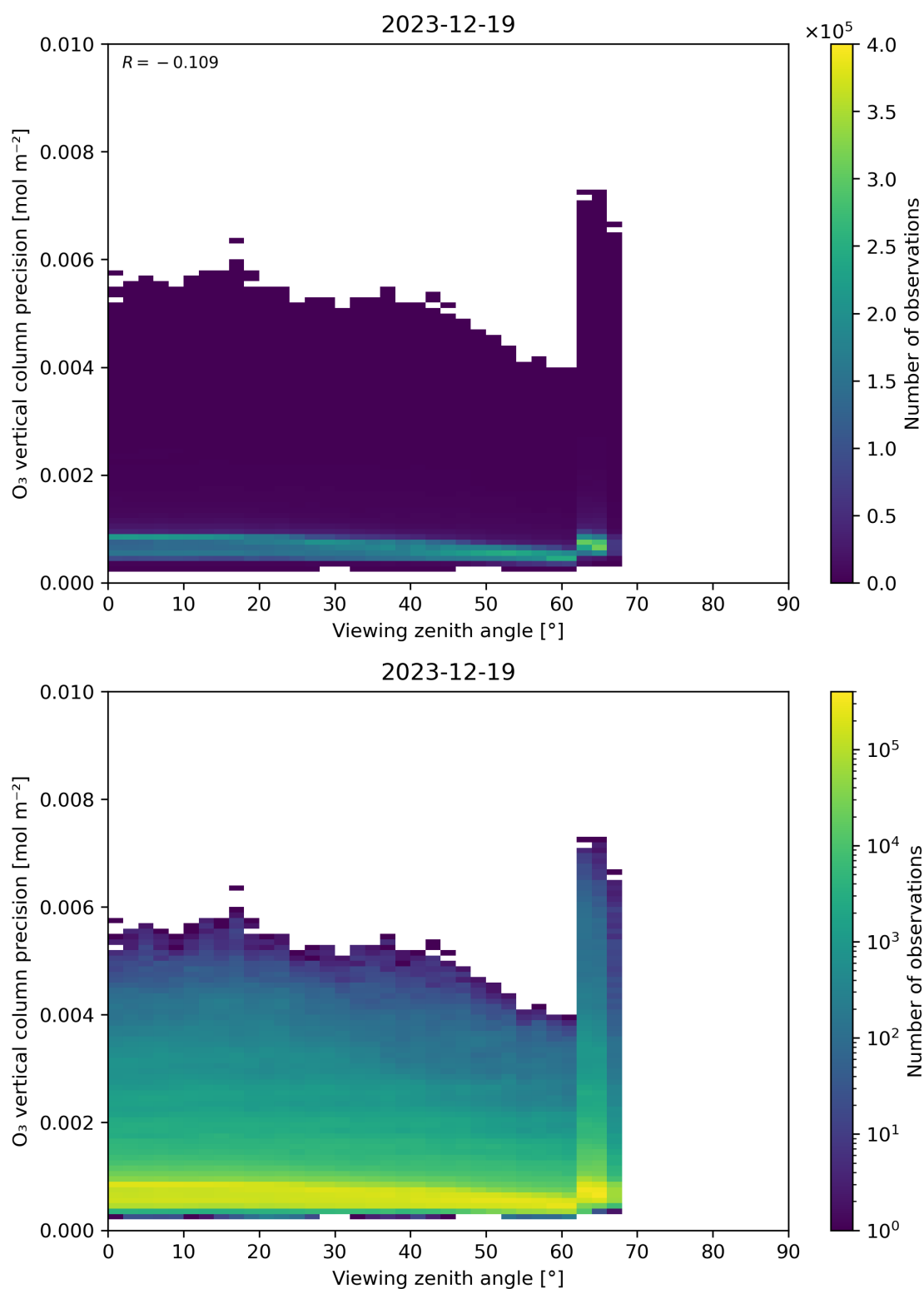
Figure 53: Scatter density plot of “Viewing zenith angle” against “O 3 vertical column precision” for 2023-12-18 to 2023-12-20.
