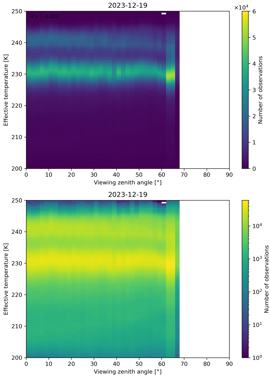
Figure 50: Scatter density plot of “Viewing zenith angle” against “Effective temperature” for 2023-12-18 to 2023-12-20.
