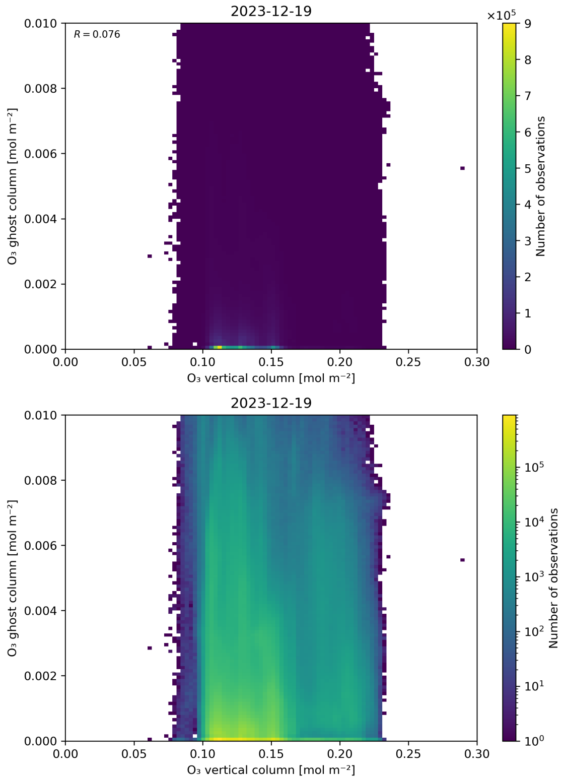
Figure 40: Scatter density plot of “O 3 vertical column” against “O 3 ghost column” for 2023-12-18 to 2023-12-20.
