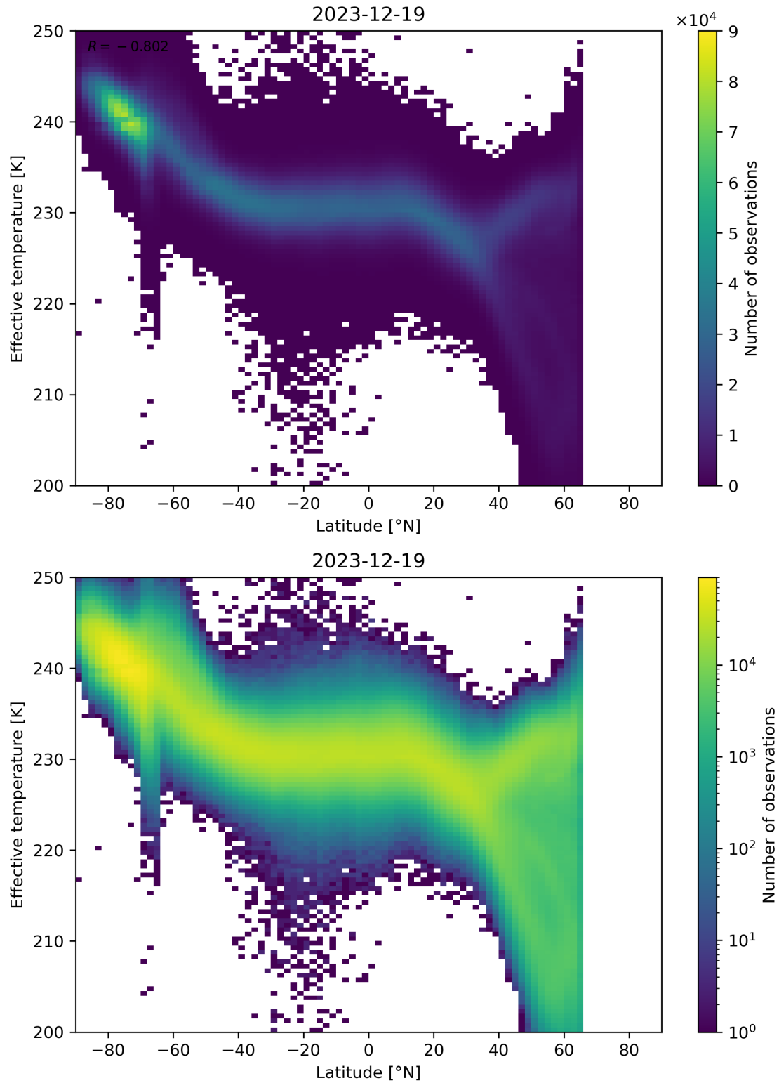
Figure 34: Scatter density plot of “Latitude” against “Effective temperature” for 2023-12-18 to 2023-12-20.
