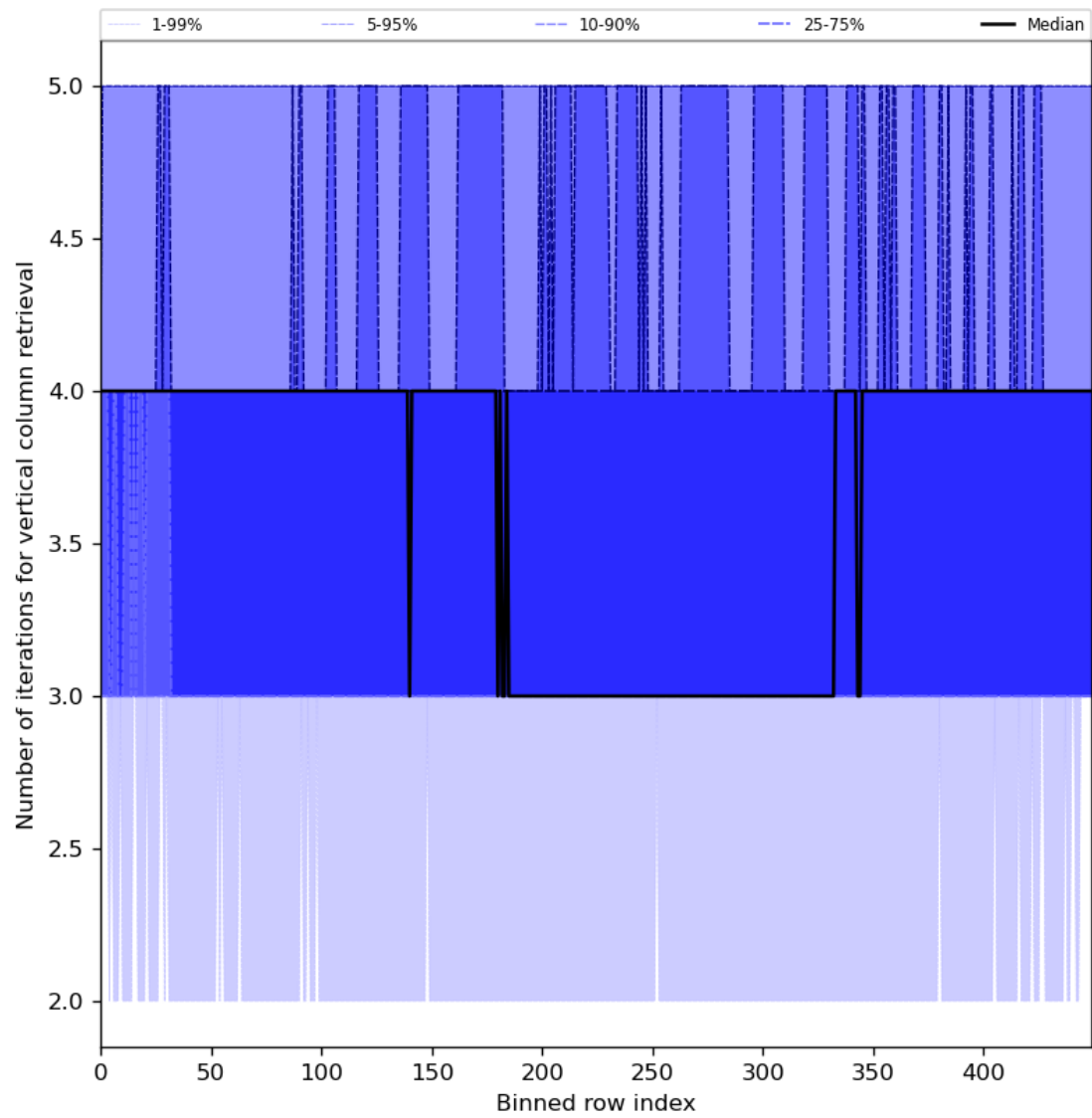
Figure 33: Along track statistics of “Number of iterations for vertical column retrieval” for 2023-12-18 to 2023-12-20
