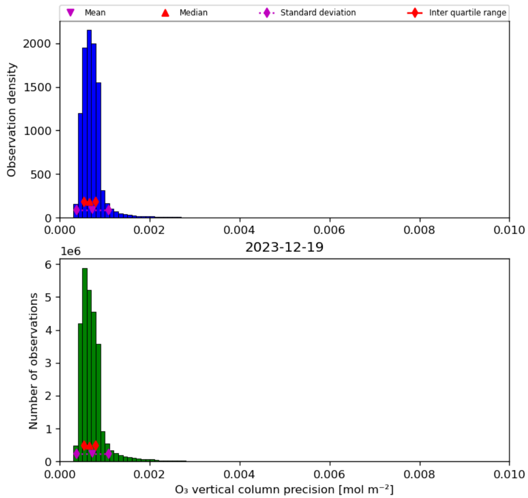
Figure 22: Histogram of “O 3 vertical column precision” for 2023-12-18 to 2023-12-20
