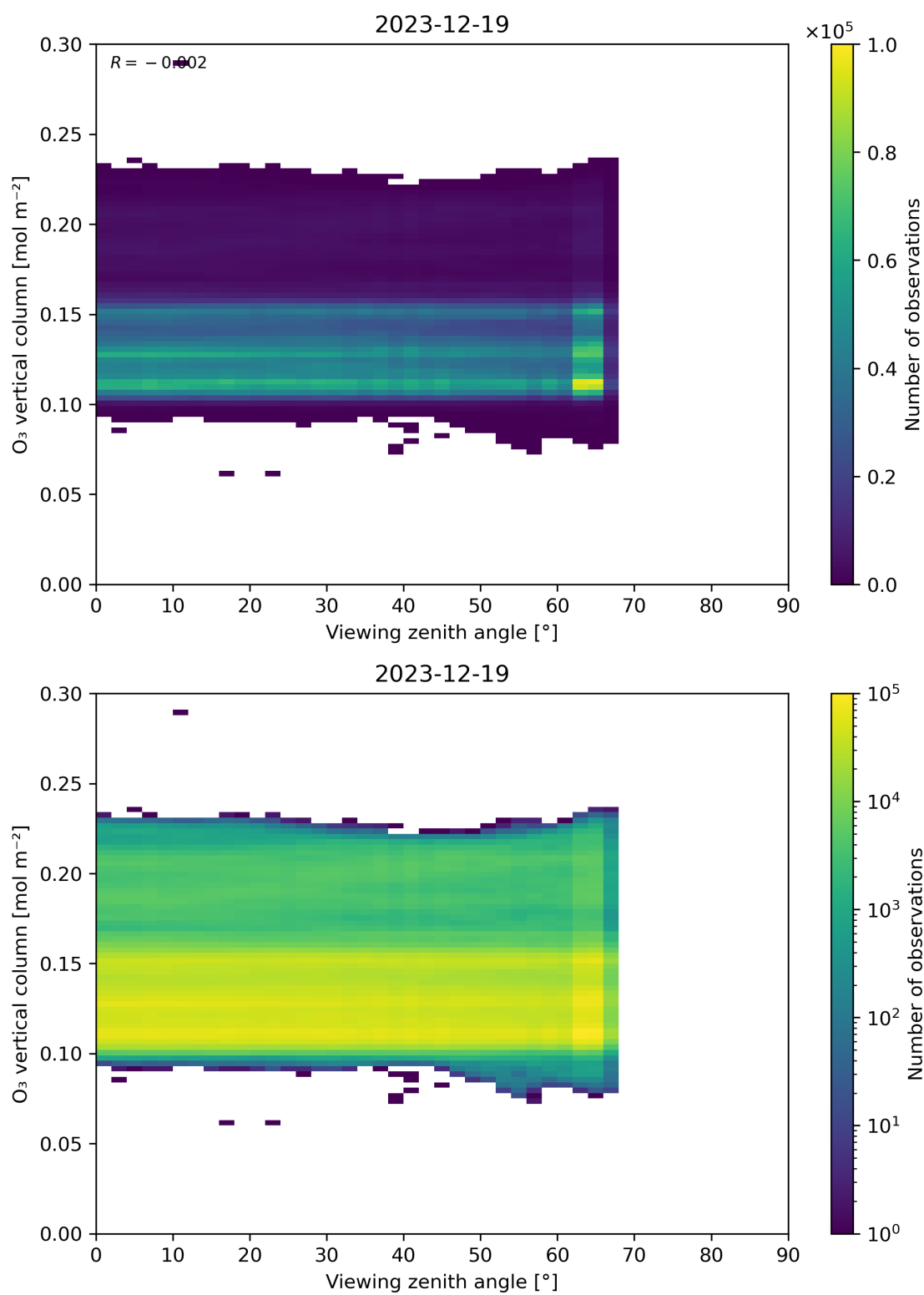
Figure 52: Scatter density plot of “Viewing zenith angle” against “O 3 vertical column” for 2023-12-18 to 2023-12-20.
