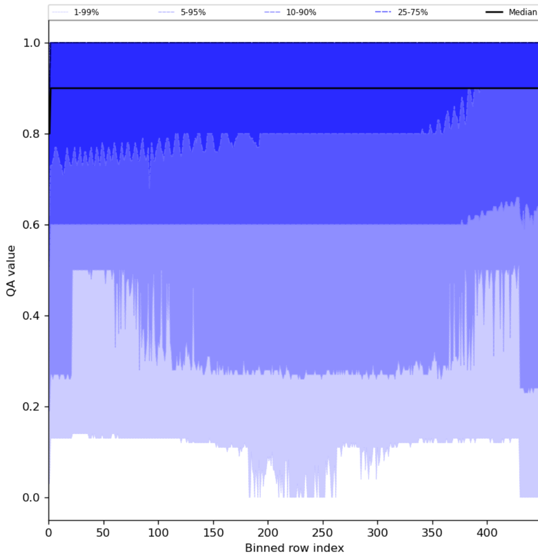
Figure 27: Along track statistics of “QA value” for 2023-12-18 to 2023-12-20
