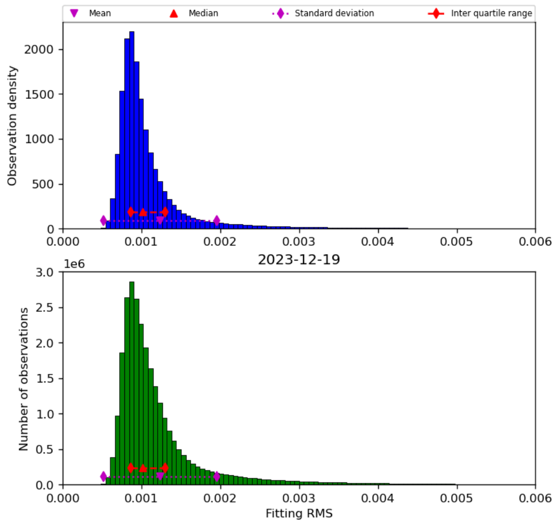
Figure 23: Histogram of “Fitting RMS” for 2023-12-18 to 2023-12-20
