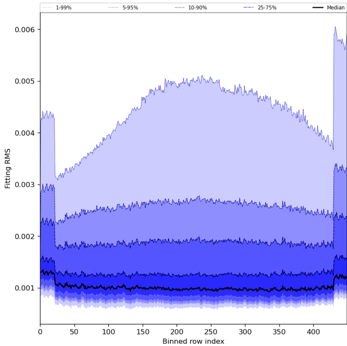
Figure 30: Along track statistics of “Fitting RMS” for 2023-12-18 to 2023-12-20
