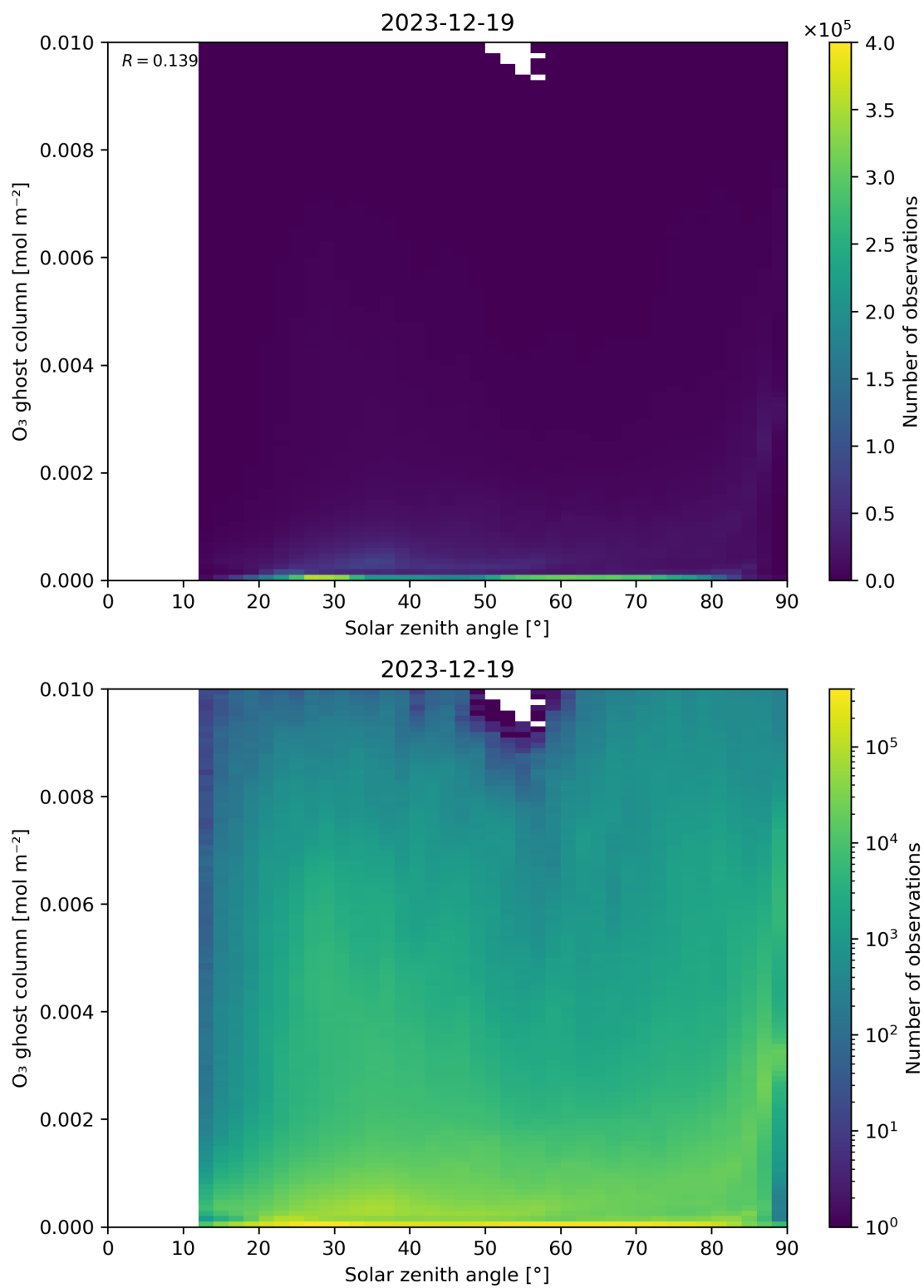
Figure 46: Scatter density plot of “Solar zenith angle” against “O 3 ghost column” for 2023-12-18 to 2023-12-20.
