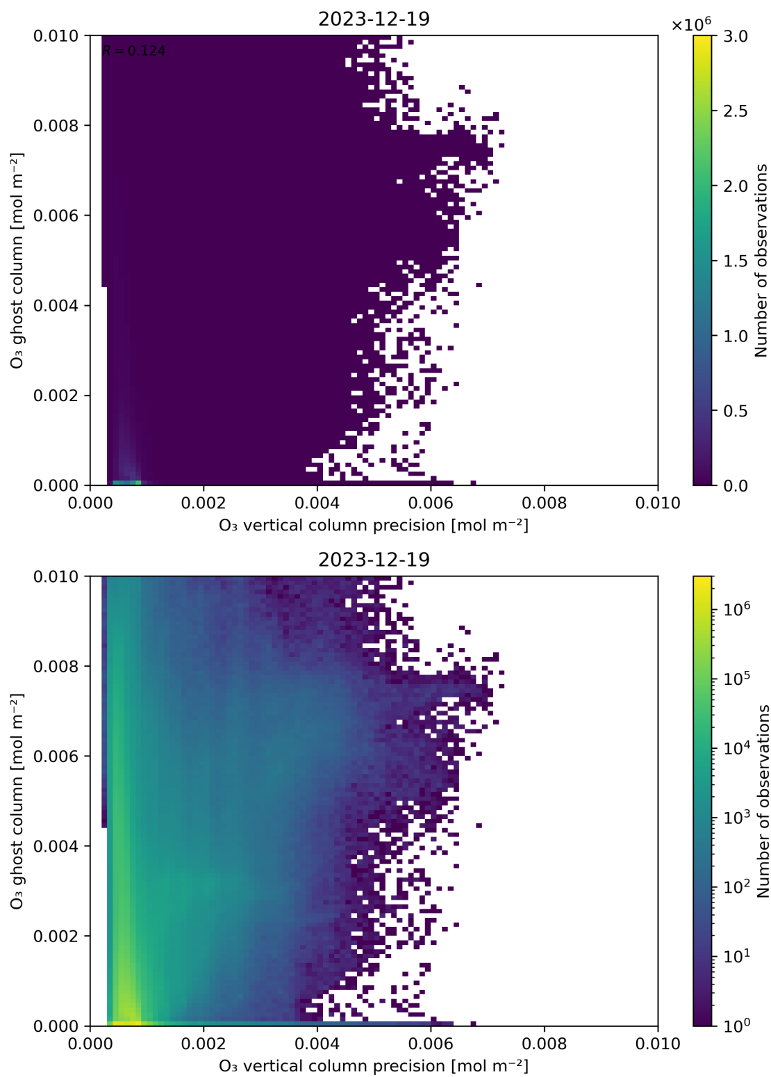
Figure 43: Scatter density plot of “ \text{O}_3 vertical column precision” against “ \text{O}_3 ghost column” for 2023-12-18 to 2023-12-20.
