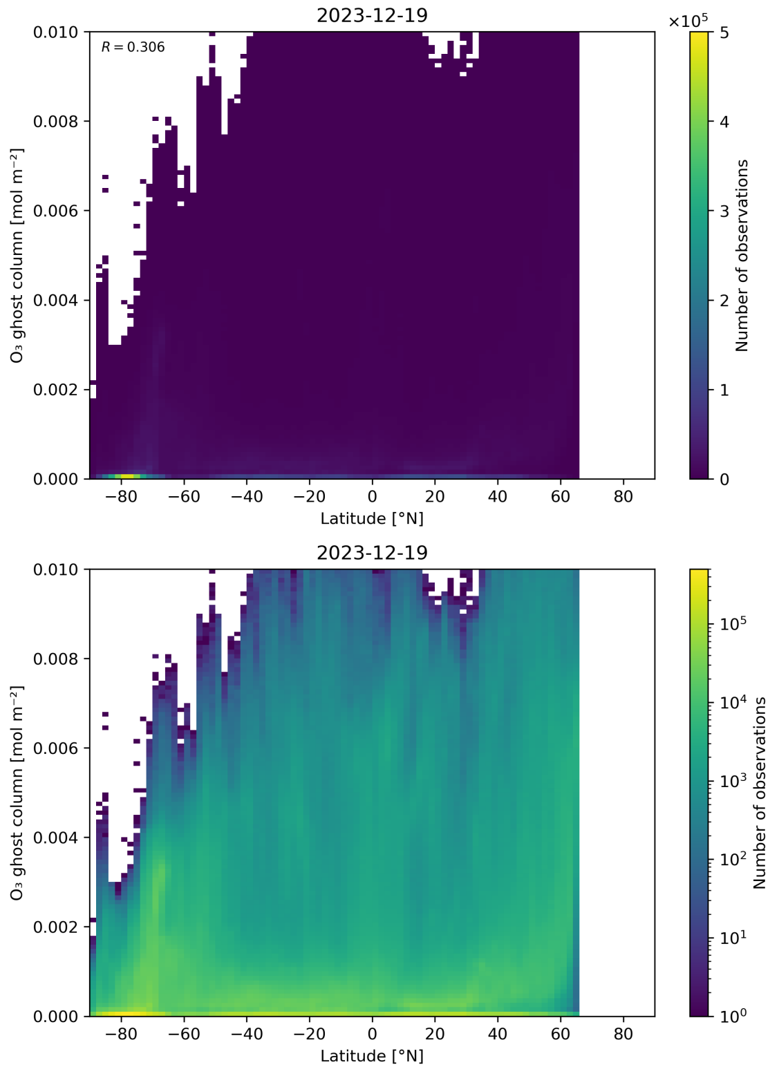
Figure 35: Scatter density plot of “Latitude” against “O 3 ghost column” for 2023-12-18 to 2023-12-20.
