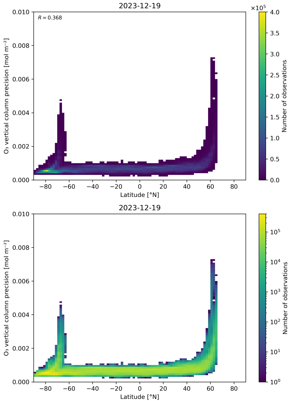
Figure 37: Scatter density plot of “Latitude” against “O 3 vertical column precision” for 2023-12-18 to 2023-12-20.
