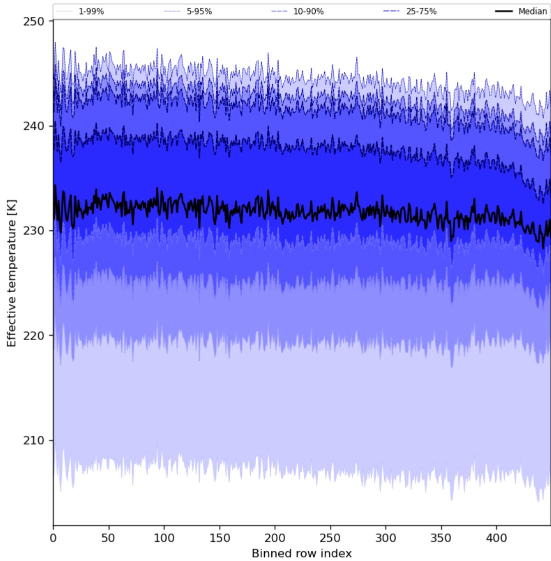
Figure 31: Along track statistics of “Effective temperature” for 2023-12-18 to 2023-12-20
