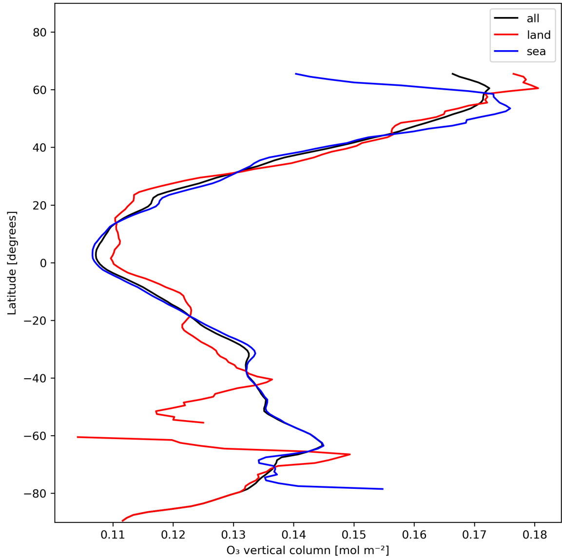
Figure 14: Zonal average of “O 3 vertical column” for 2023-12-18 to 2023-12-20.
