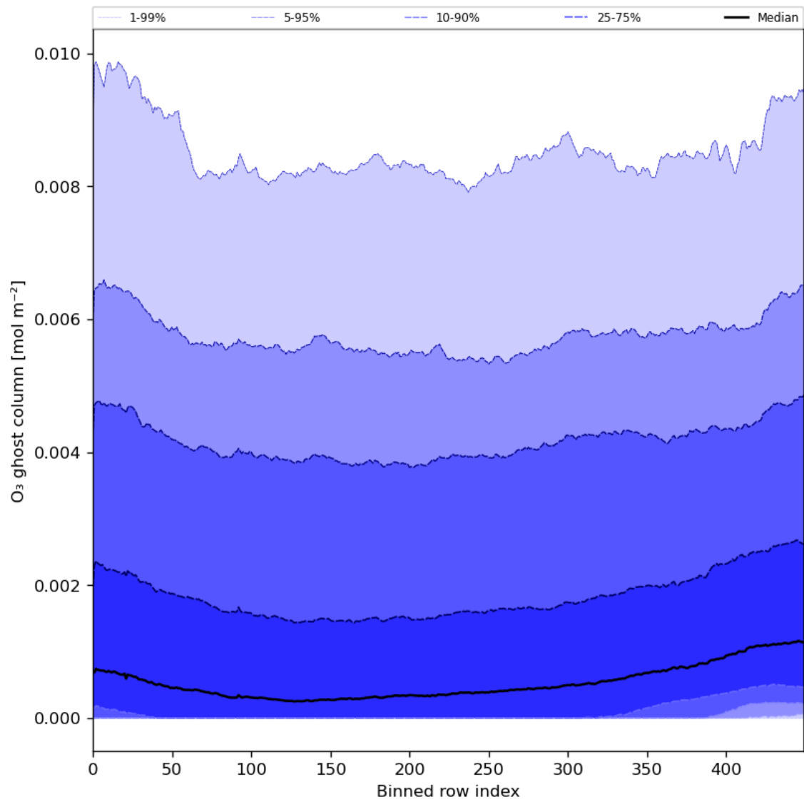
Figure 32: Along track statistics of “O 3 ghost column” for 2023-12-18 to 2023-12-20
