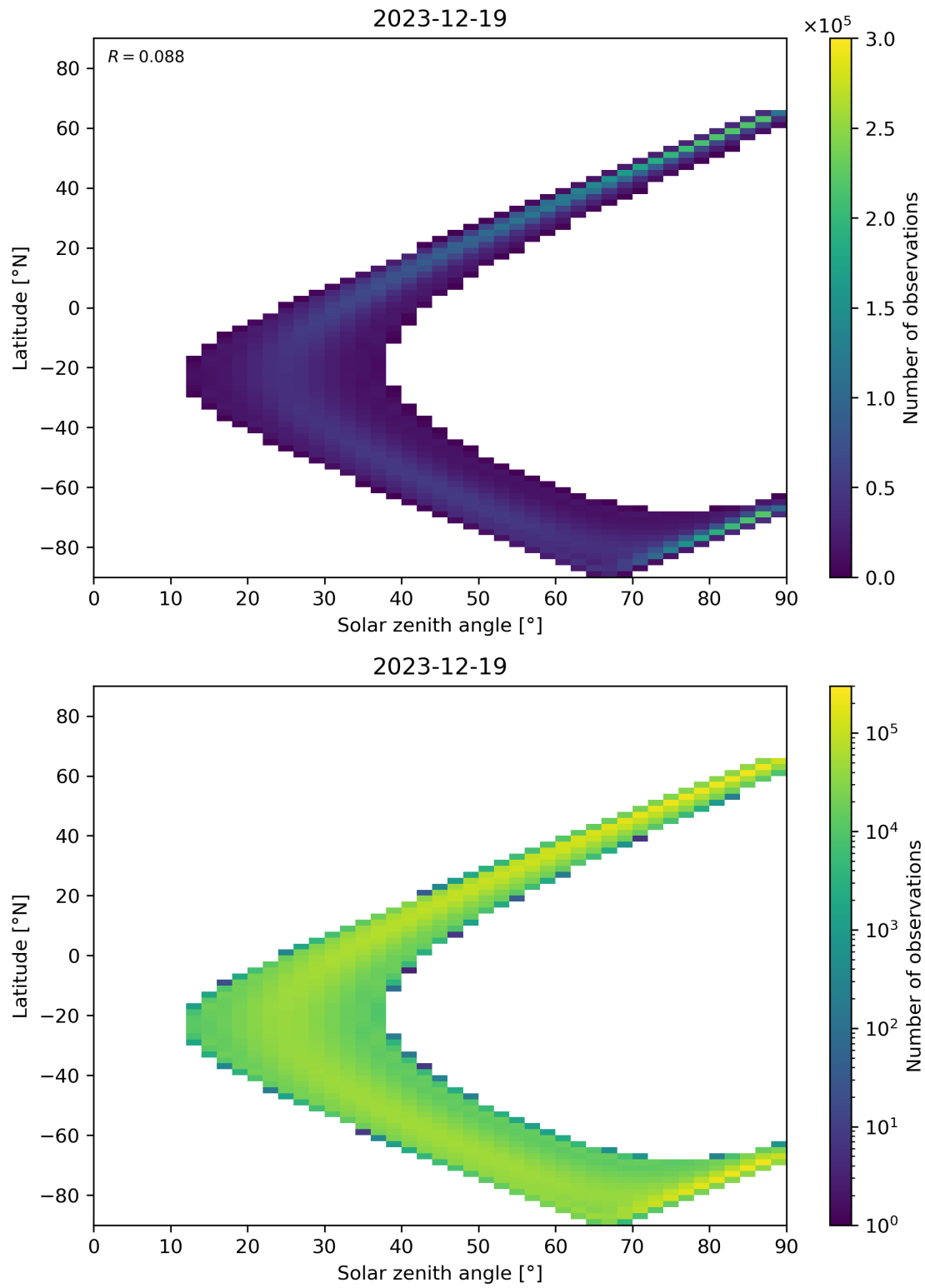
Figure 44: Scatter density plot of “Solar zenith angle” against “Latitude” for 2023-12-18 to 2023-12-20.
