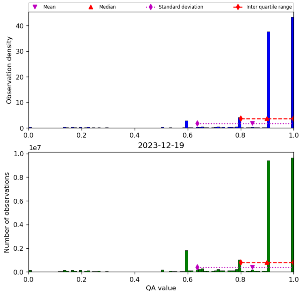
Figure 20: Histogram of “QA value” for 2023-12-18 to 2023-12-20
