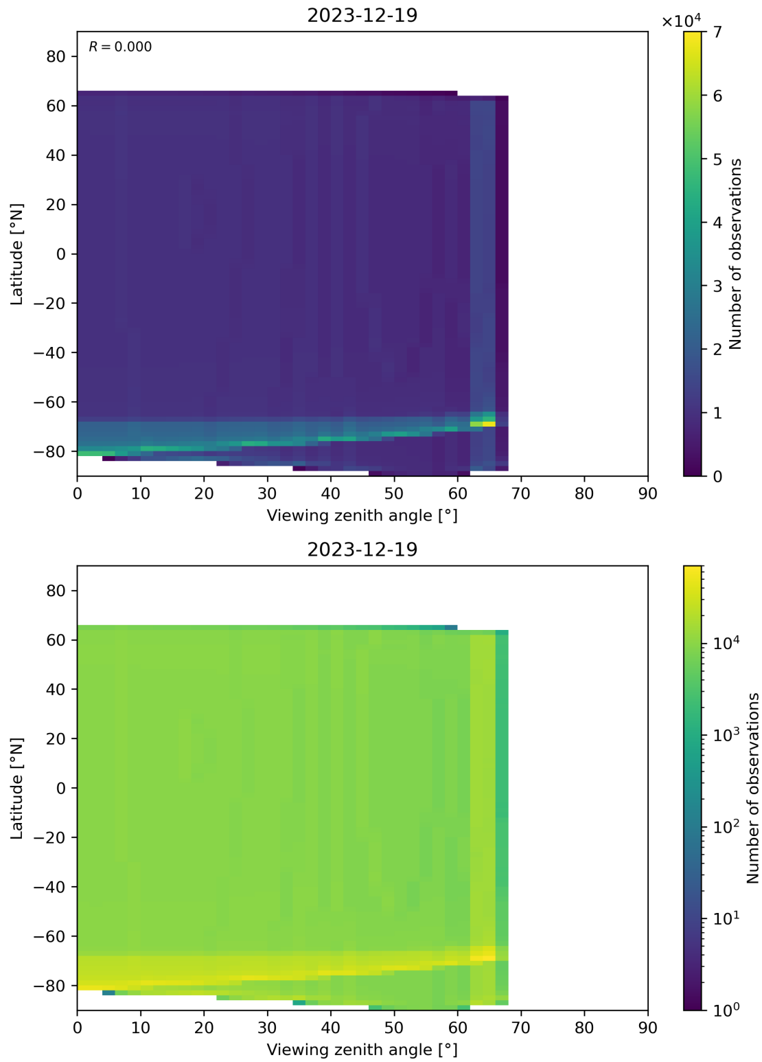
Figure 49: Scatter density plot of “Viewing zenith angle” against “Latitude” for 2023-12-18 to 2023-12-20.
