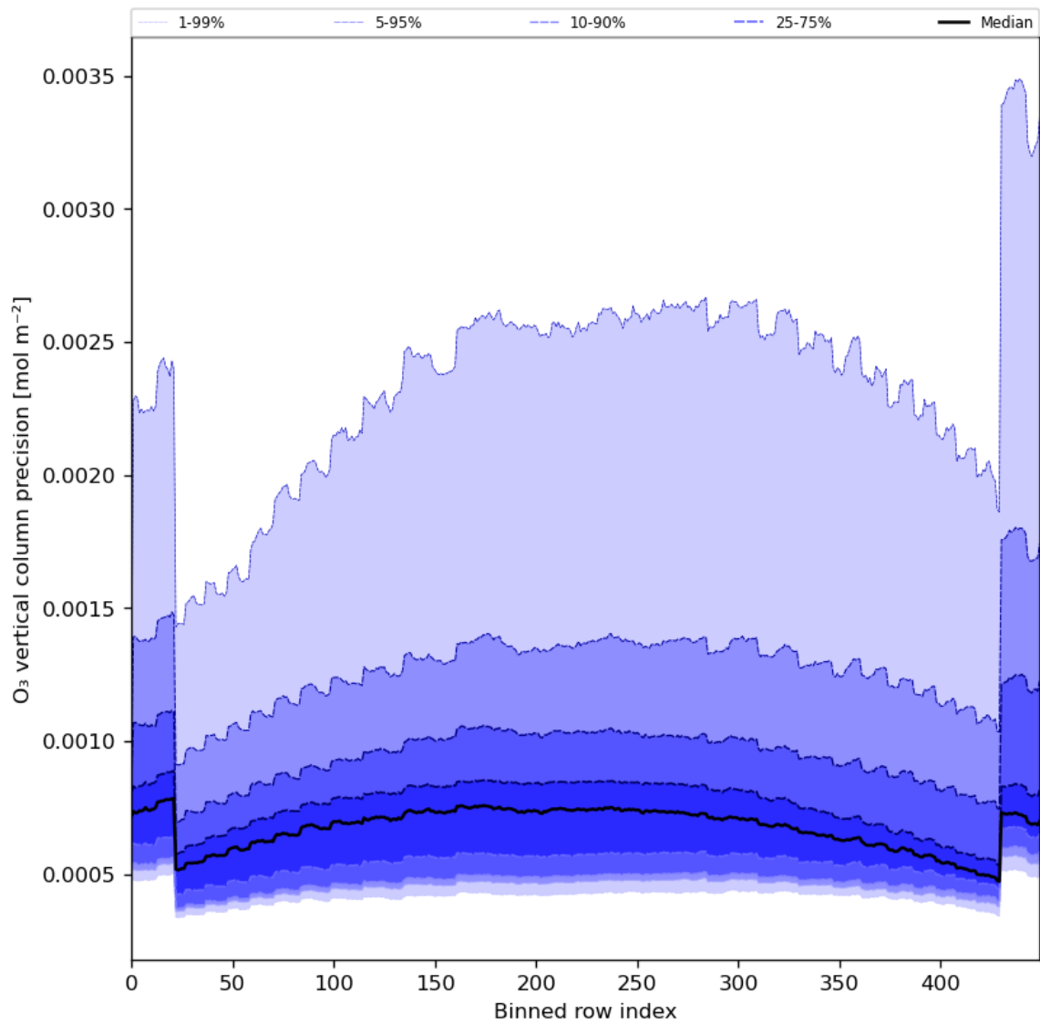
Figure 29: Along track statistics of “O 3 vertical column precision” for 2023-12-18 to 2023-12-20
