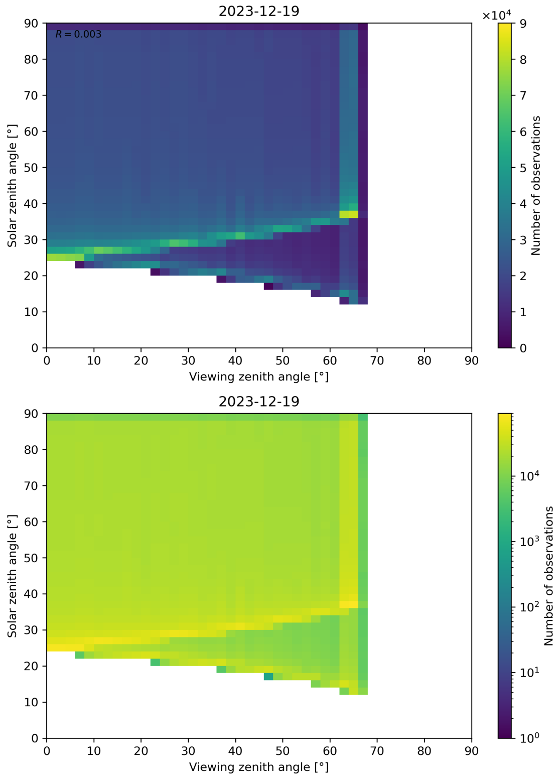
Figure 54: Scatter density plot of “Viewing zenith angle” against “Solar zenith angle” for 2023-12-18 to 2023-12-20.
