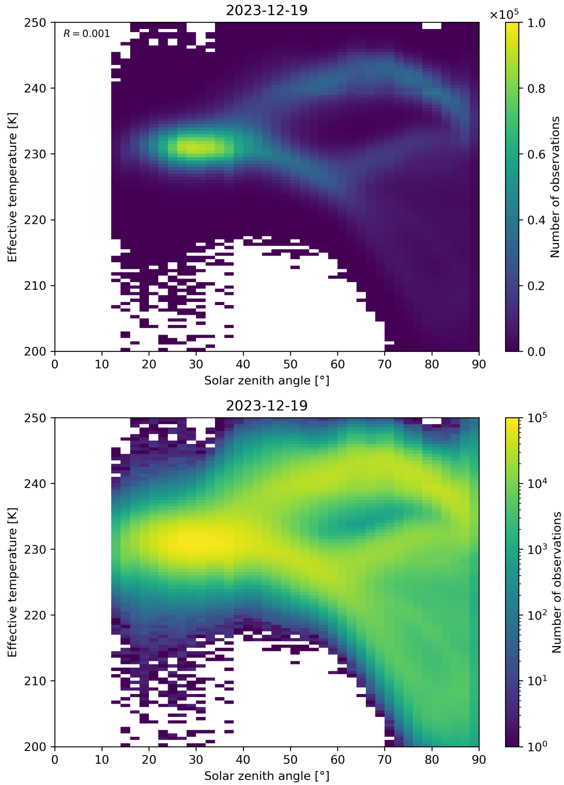
Figure 45: Scatter density plot of “Solar zenith angle” against “Effective temperature” for 2023-12-18 to 2023-12-20.
