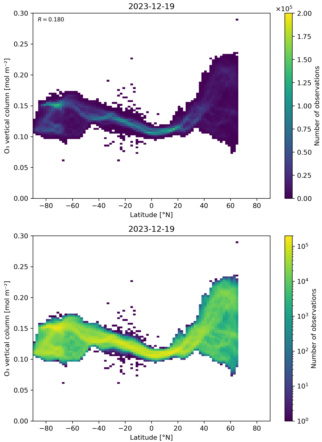
Figure 36: Scatter density plot of “Latitude” against “O 3 vertical column” for 2023-12-18 to 2023-12-20.
