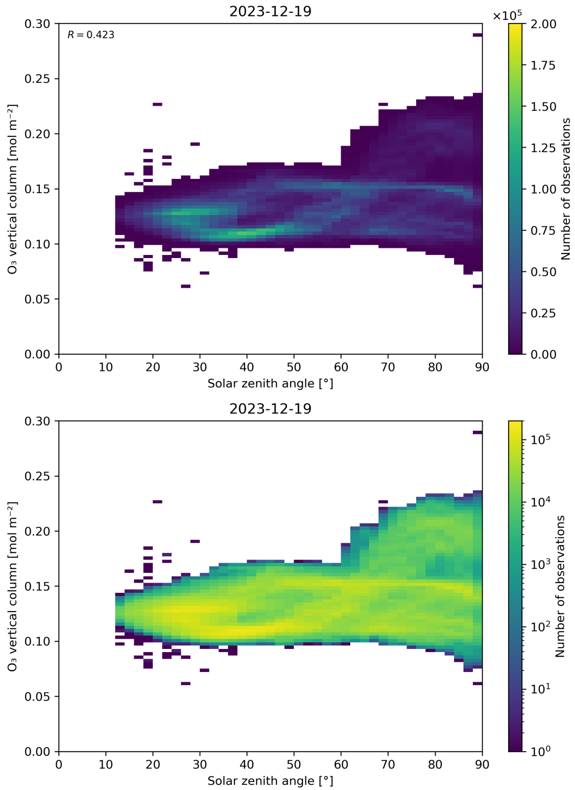
Figure 47: Scatter density plot of “Solar zenith angle” against “O 3 vertical column” for 2023-12-18 to 2023-12-20.
