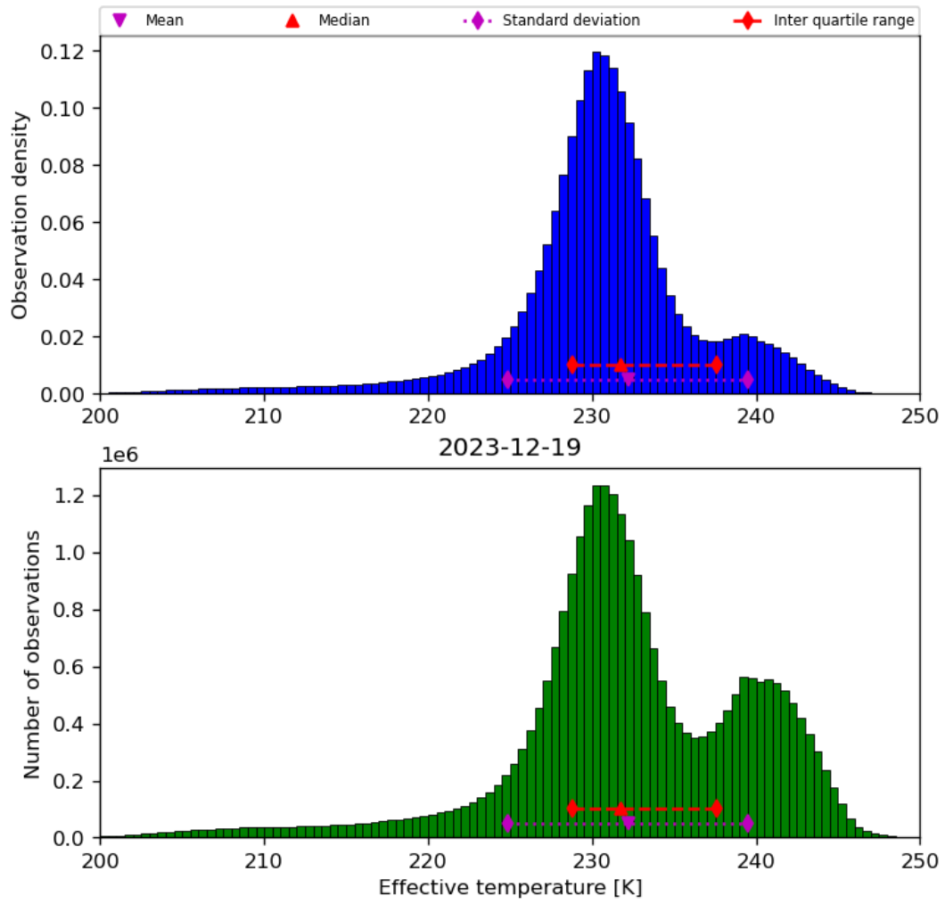
Figure 24: Histogram of “Effective temperature” for 2023-12-18 to 2023-12-20
