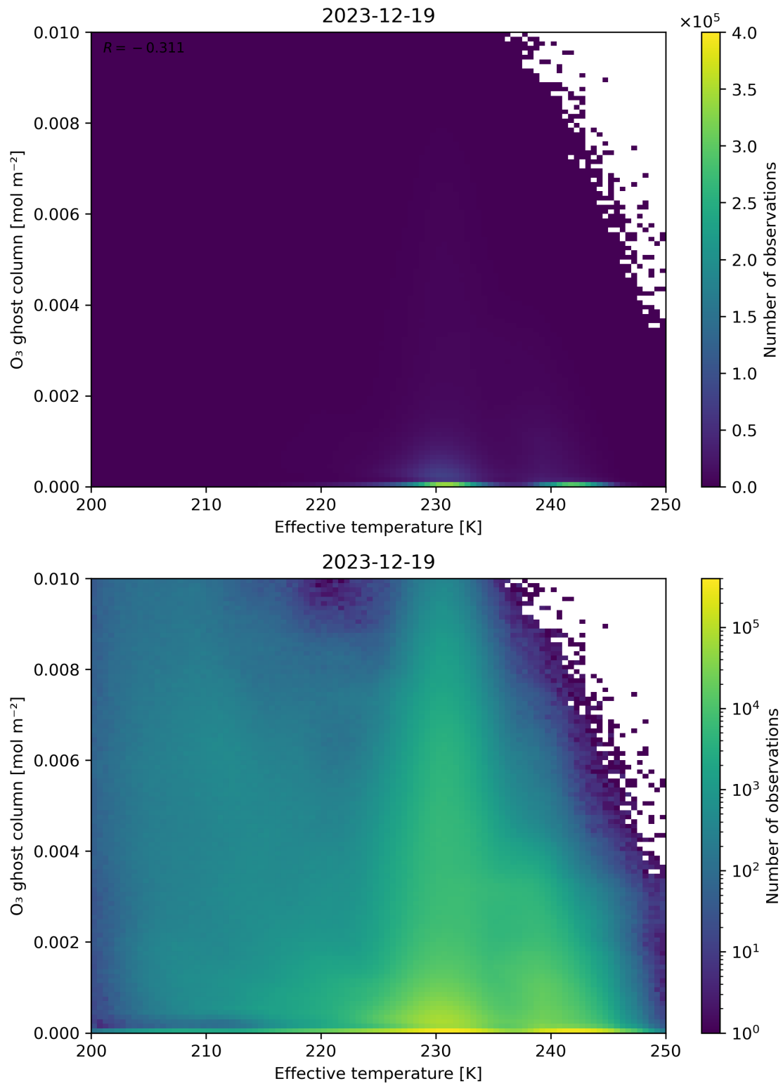
Figure 38: Scatter density plot of “Effective temperature” against “O 3 ghost column” for 2023-12-18 to 2023-12-20.
