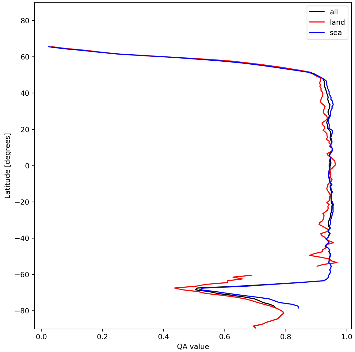
Figure 13: Zonal average of “QA value” for 2023-12-18 to 2023-12-20.
