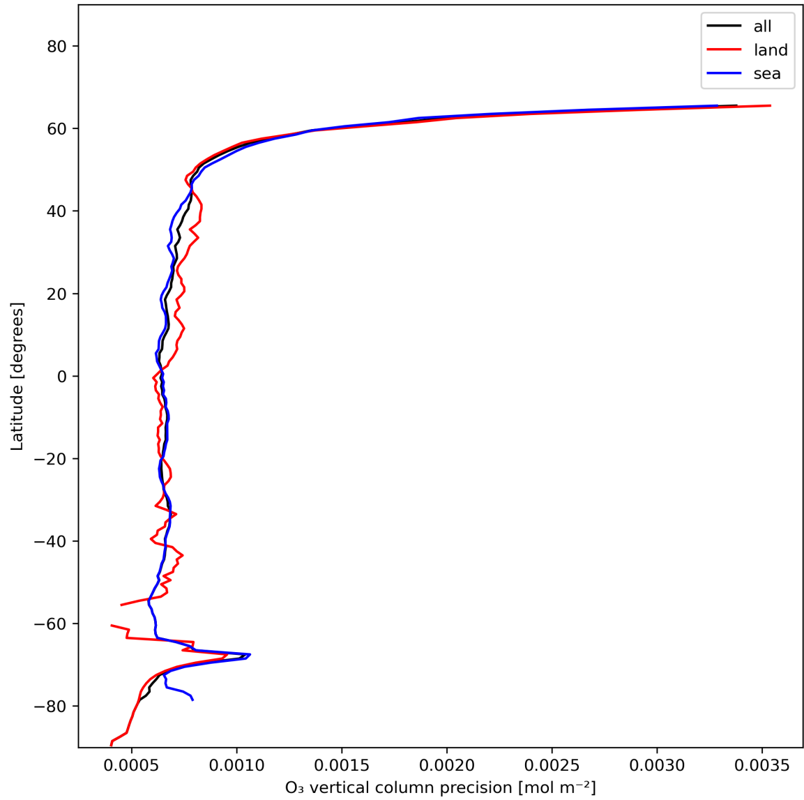
Figure 15: Zonal average of “O 3 vertical column precision” for 2023-12-18 to 2023-12-20.
