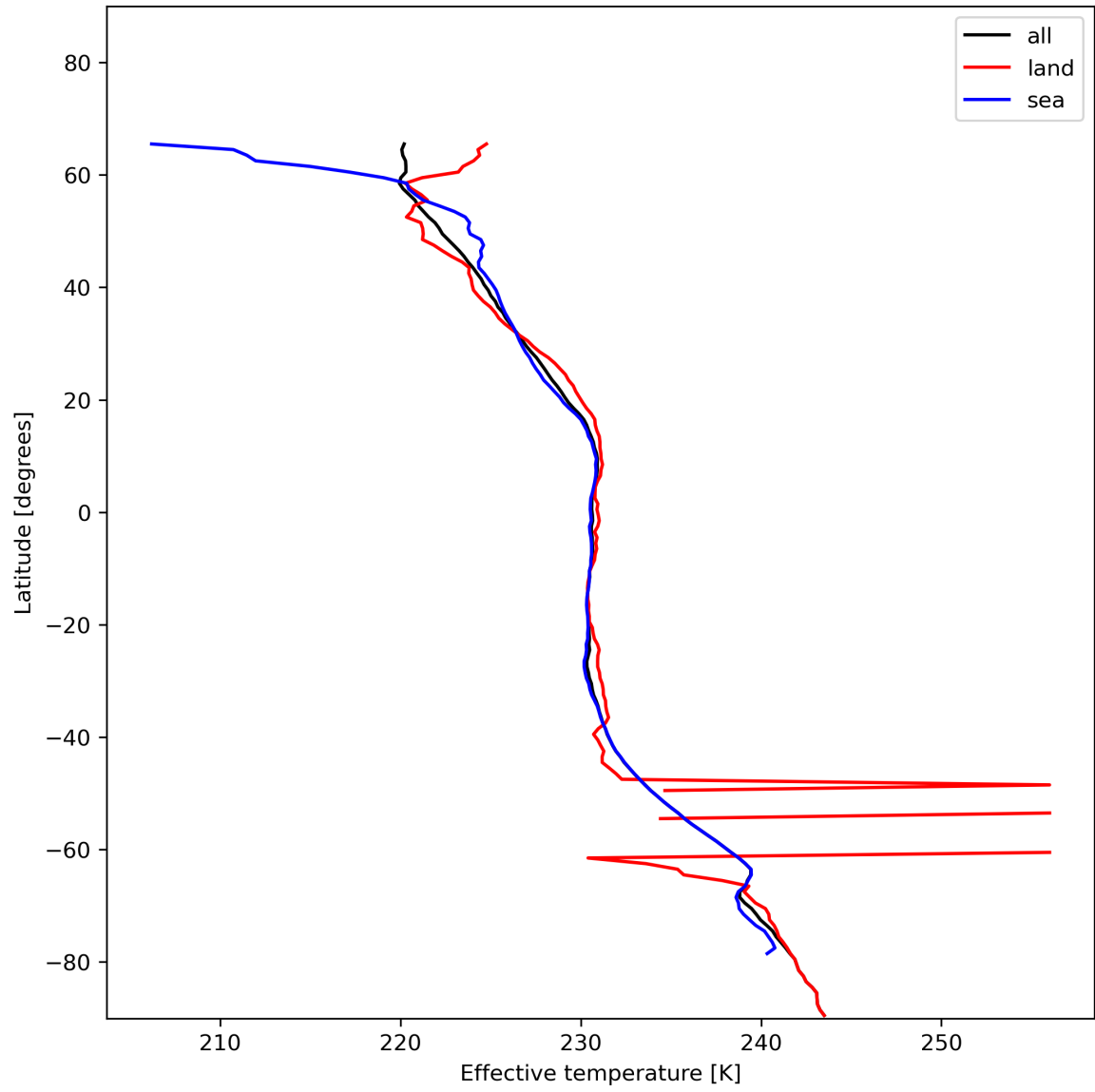
Figure 17: Zonal average of “Effective temperature” for 2023-12-20 to 2023-12-21.
