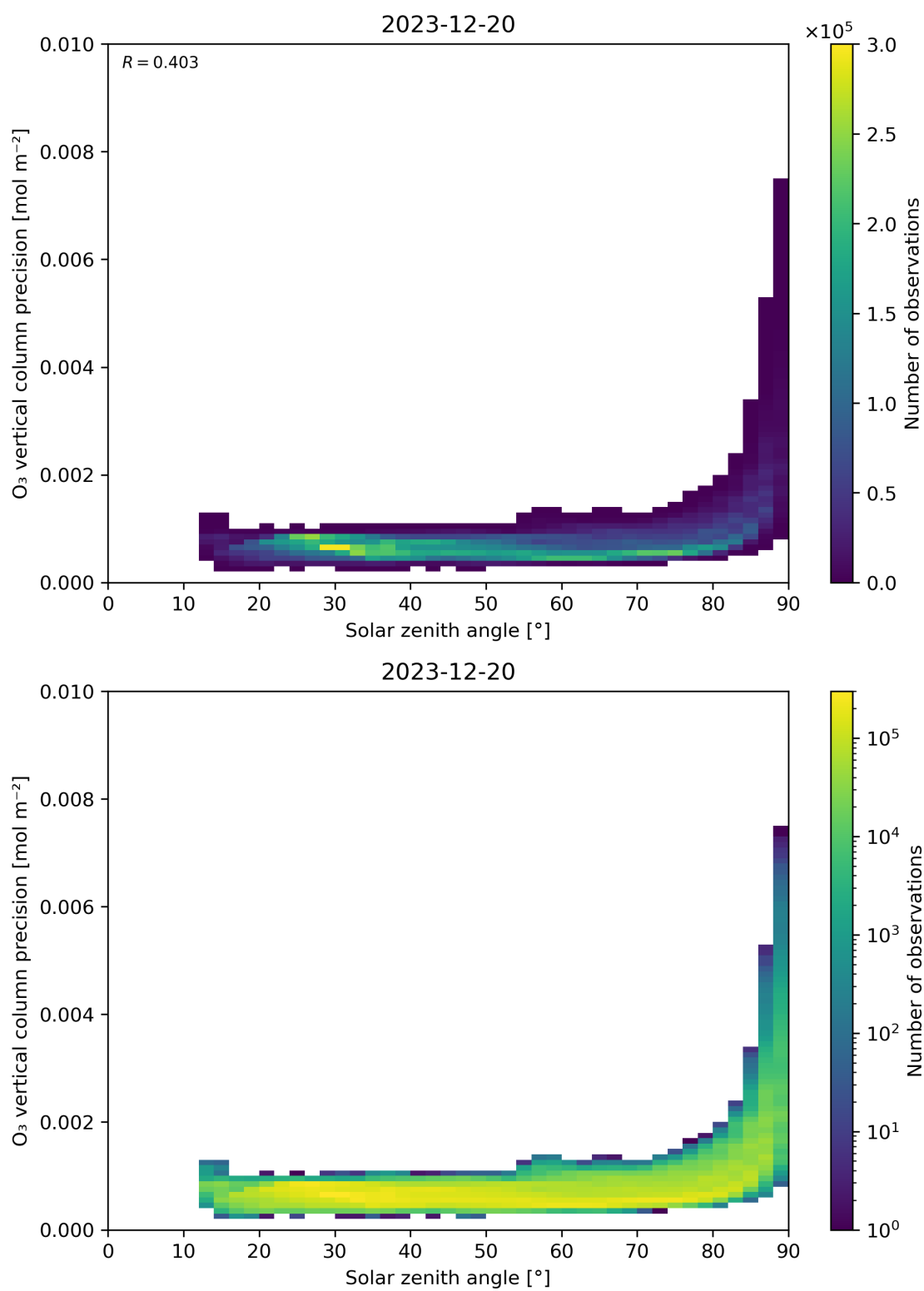
Figure 48: Scatter density plot of “Solar zenith angle” against “O 3 vertical column precision” for 2023-12-20 to 2023-12-21.
