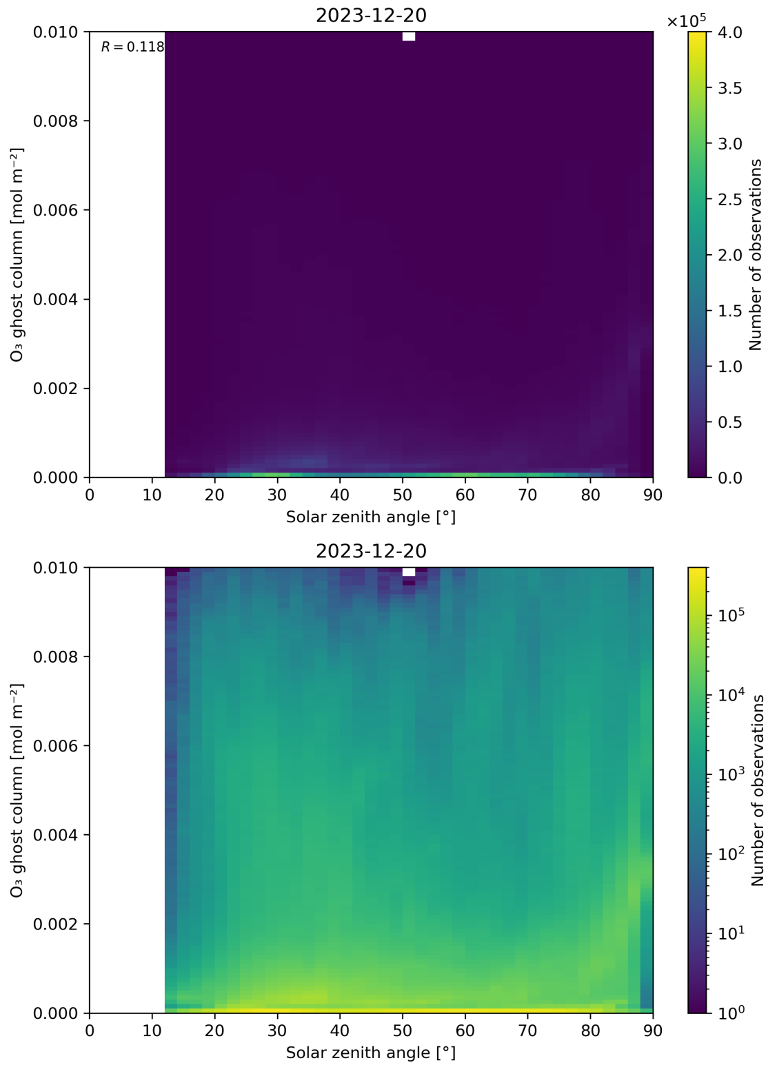
Figure 46: Scatter density plot of “Solar zenith angle” against “O 3 ghost column” for 2023-12-20 to 2023-12-21.
