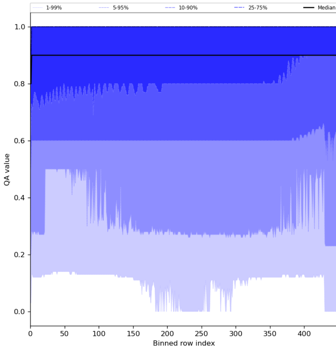
Figure 27: Along track statistics of “QA value” for 2023-12-20 to 2023-12-21
