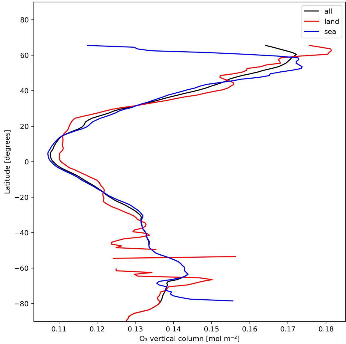
Figure 14: Zonal average of “O 3 vertical column” for 2023-12-20 to 2023-12-21.
