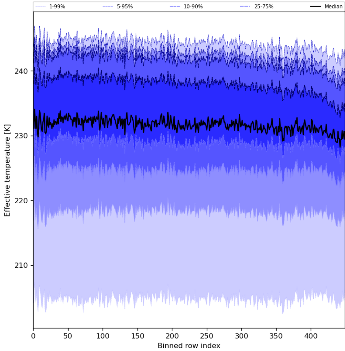
Figure 31: Along track statistics of “Effective temperature” for 2023-12-20 to 2023-12-21
