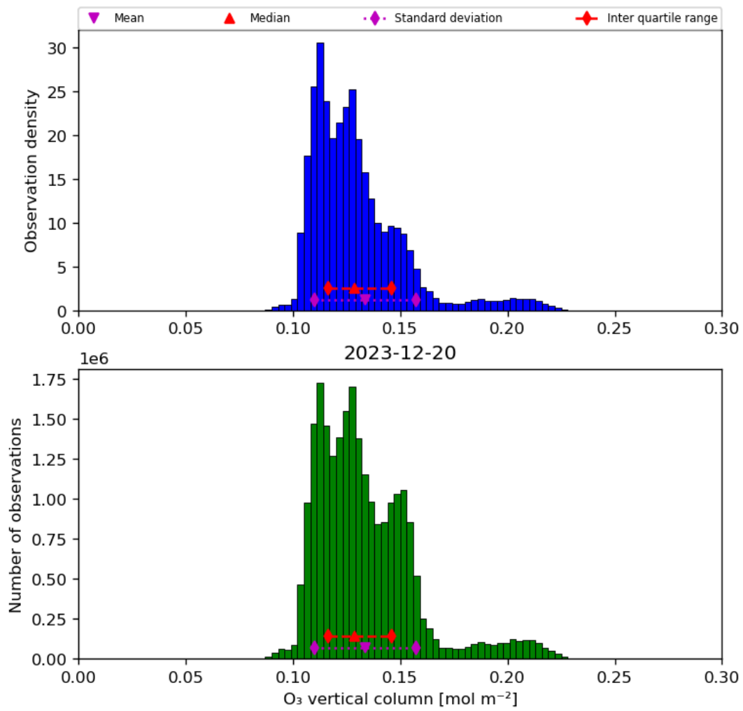
Figure 21: Histogram of “O 3 vertical column” for 2023-12-20 to 2023-12-21
