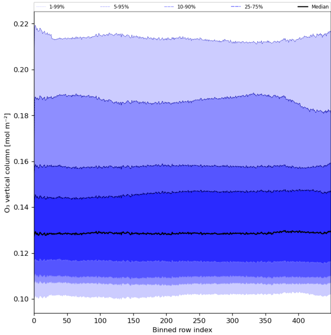
Figure 28: Along track statistics of “O 3 vertical column” for 2023-12-20 to 2023-12-21
