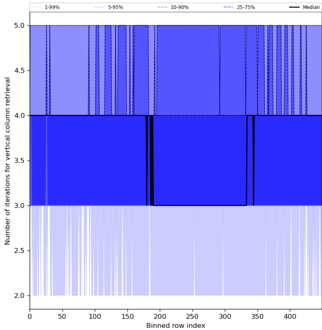
Figure 33: Along track statistics of “Number of iterations for vertical column retrieval” for 2023-12-20 to 2023-12-21
