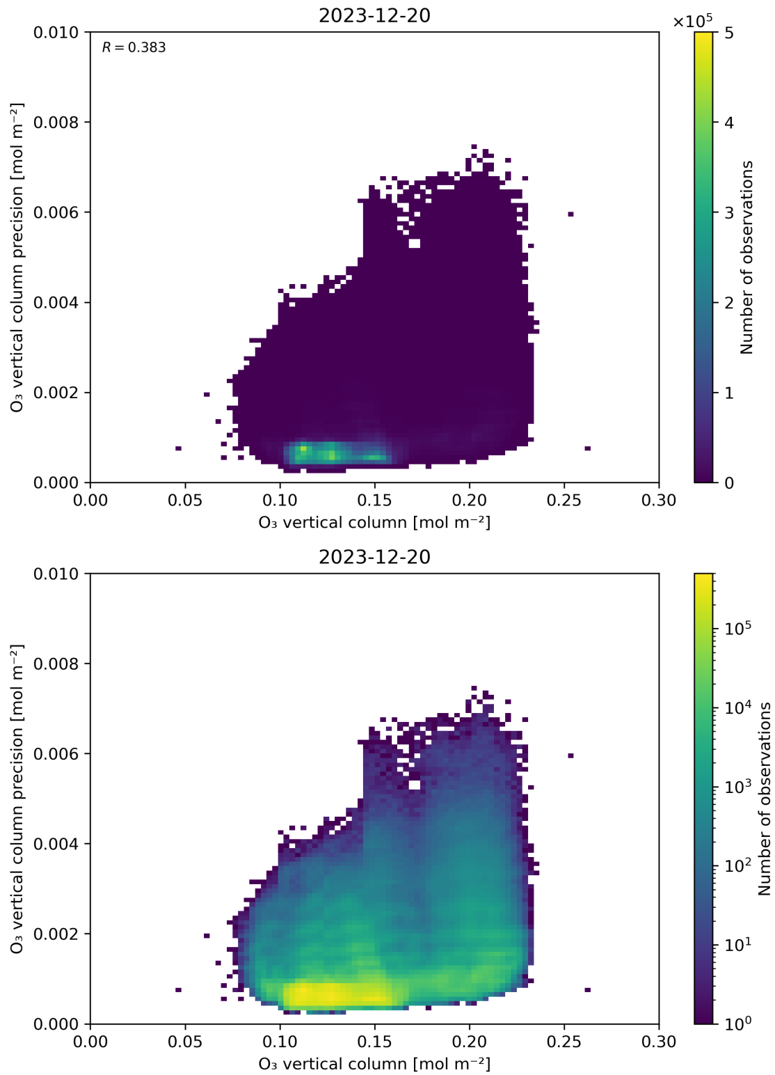
Figure 41: Scatter density plot of “O 3 vertical column” against “O 3 vertical column precision” for 2023-12-20 to 2023-12-21.
