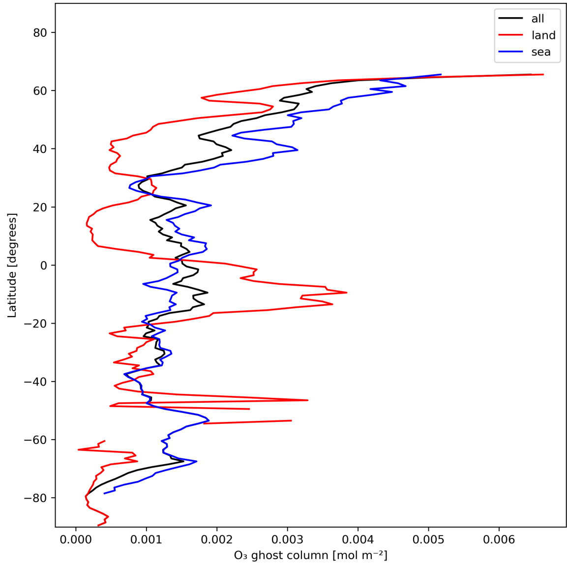
Figure 18: Zonal average of “O 3 ghost column” for 2023-12-20 to 2023-12-21.
