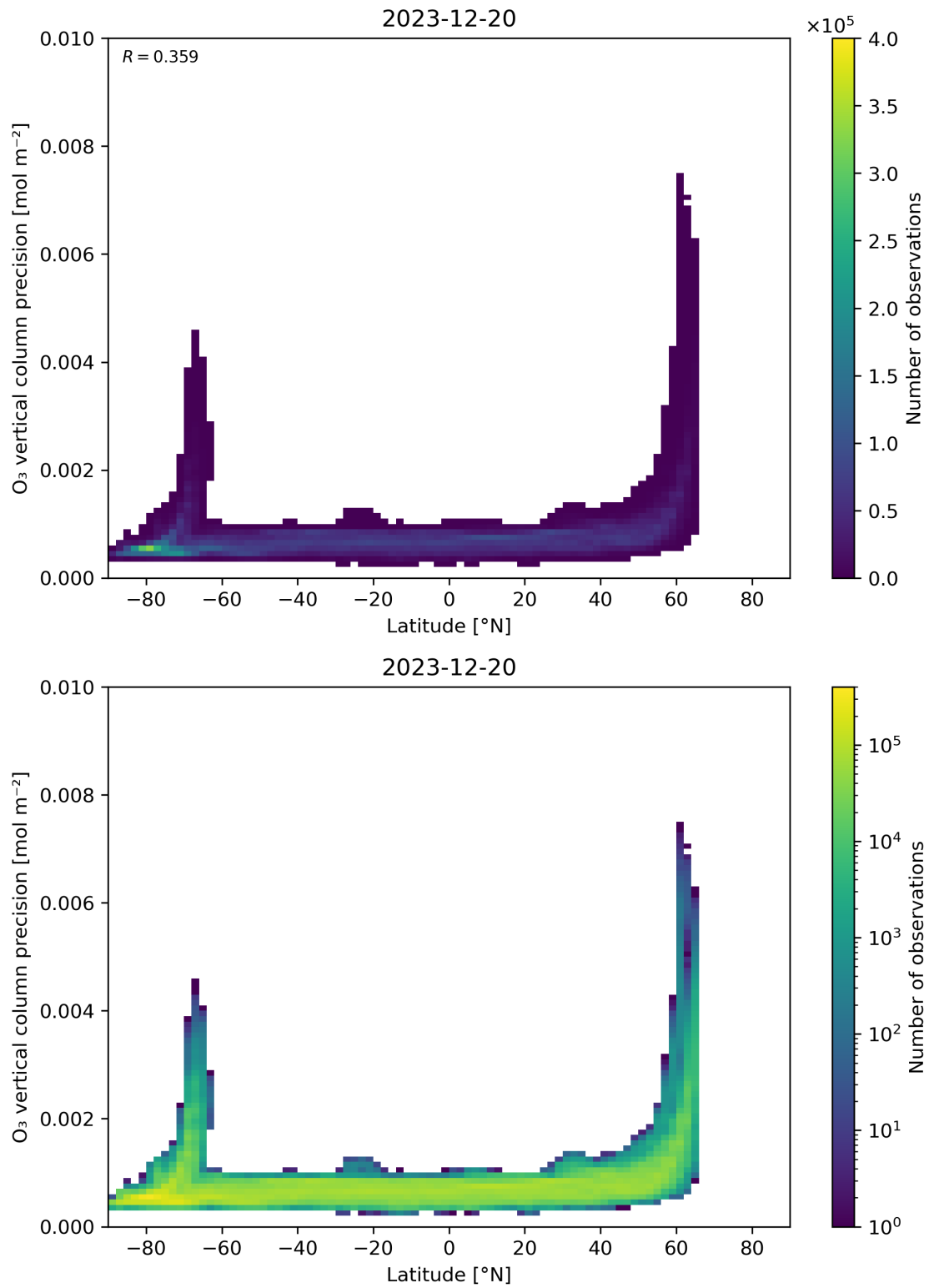
Figure 37: Scatter density plot of “Latitude” against “O 3 vertical column precision” for 2023-12-20 to 2023-12-21.
