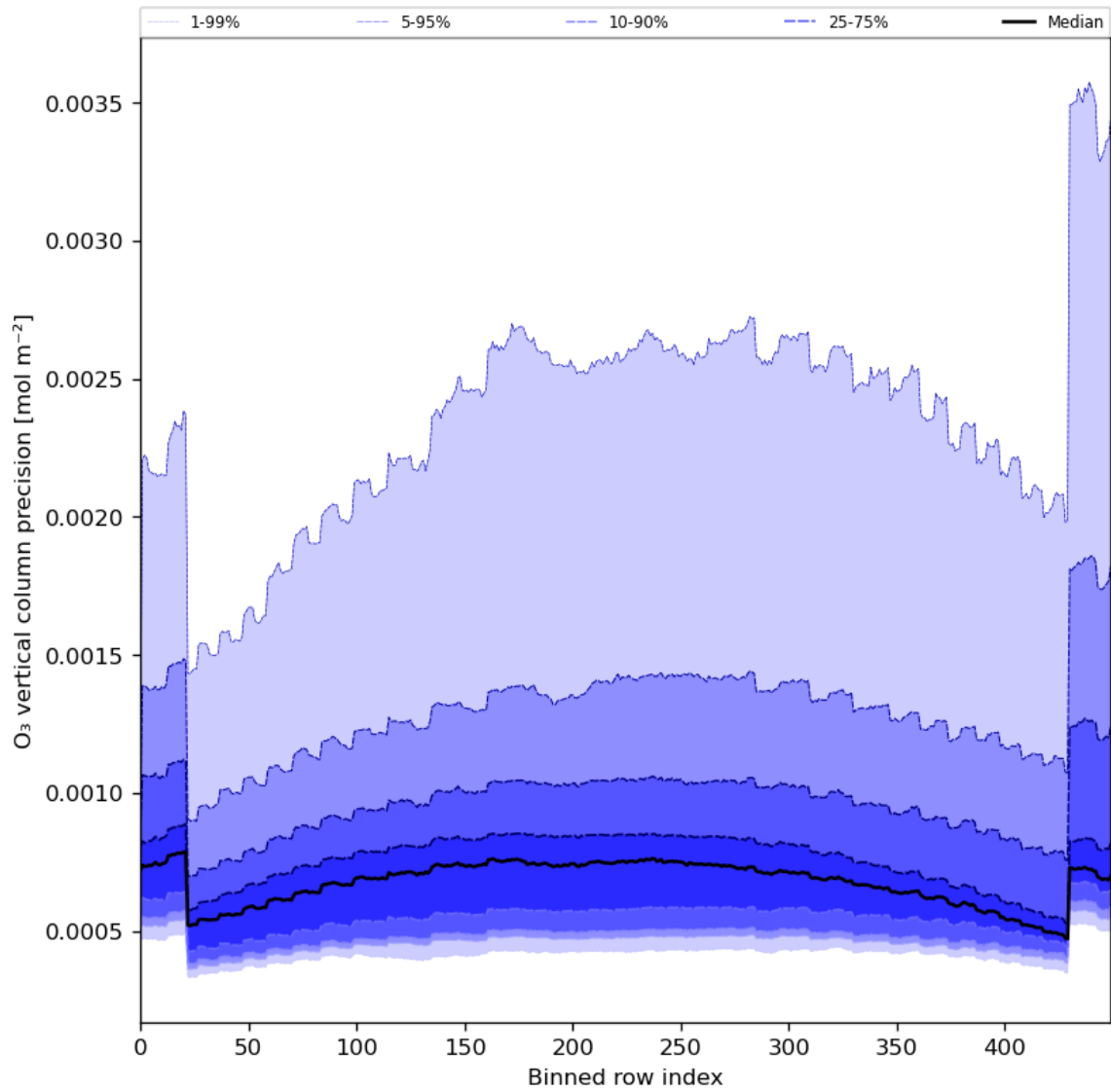
Figure 29: Along track statistics of “O 3 vertical column precision” for 2023-12-20 to 2023-12-21
