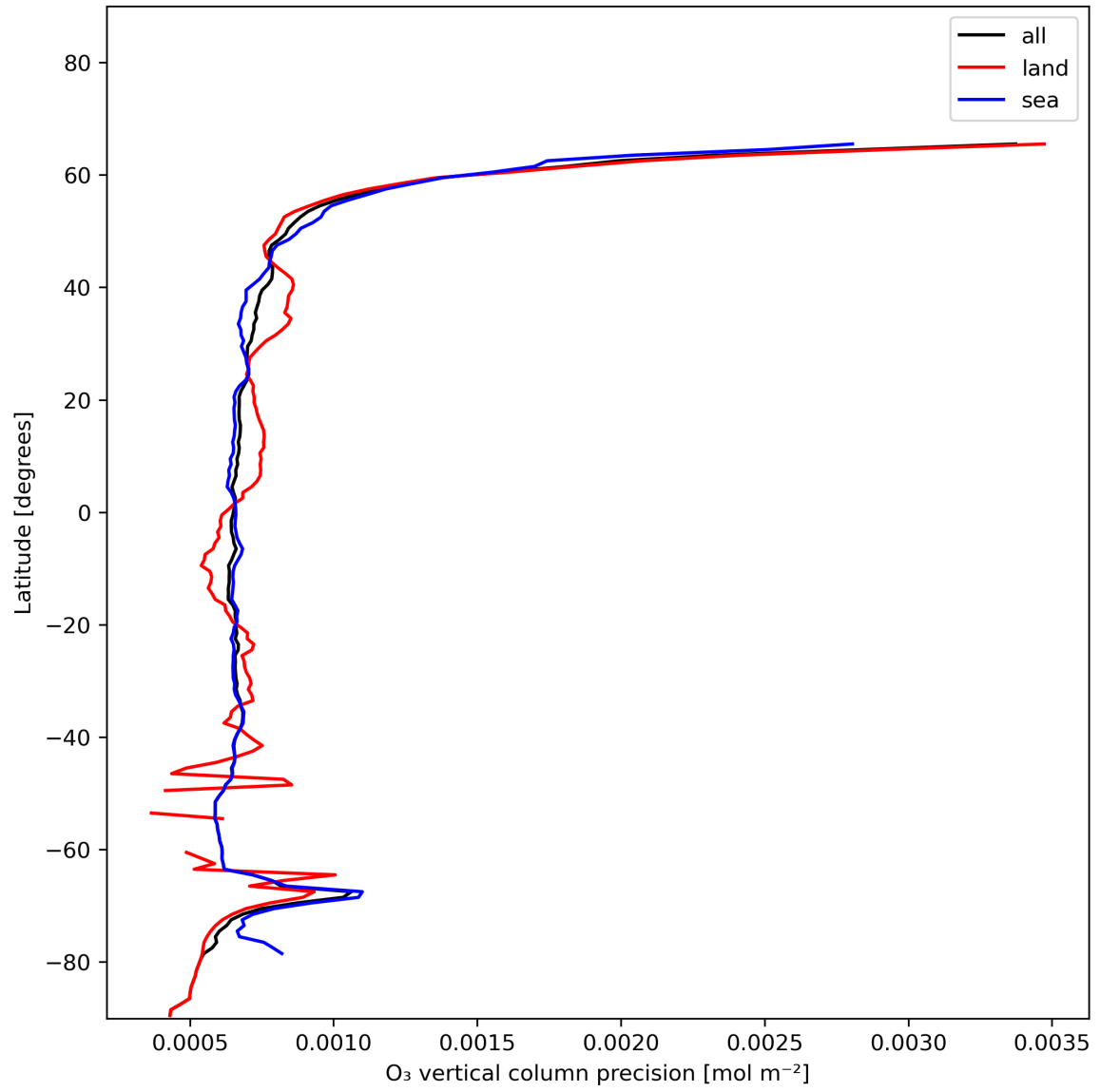
Figure 15: Zonal average of “O 3 vertical column precision” for 2023-12-20 to 2023-12-21.
