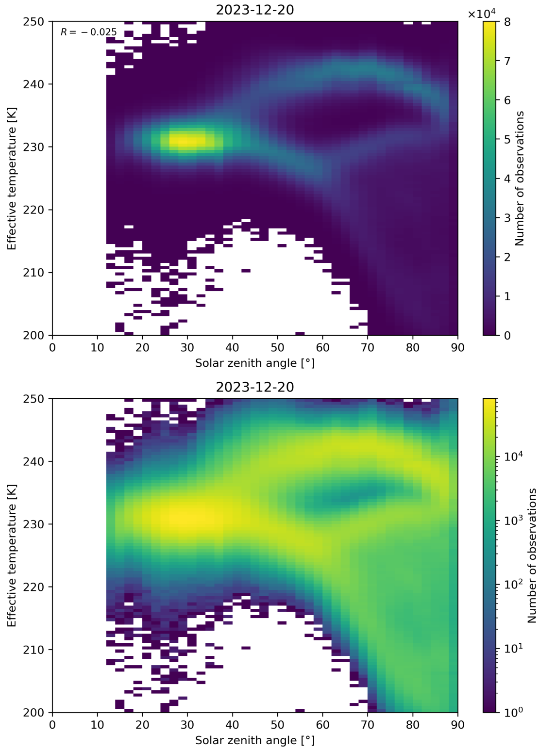
Figure 45: Scatter density plot of “Solar zenith angle” against “Effective temperature” for 2023-12-20 to 2023-12-21.
