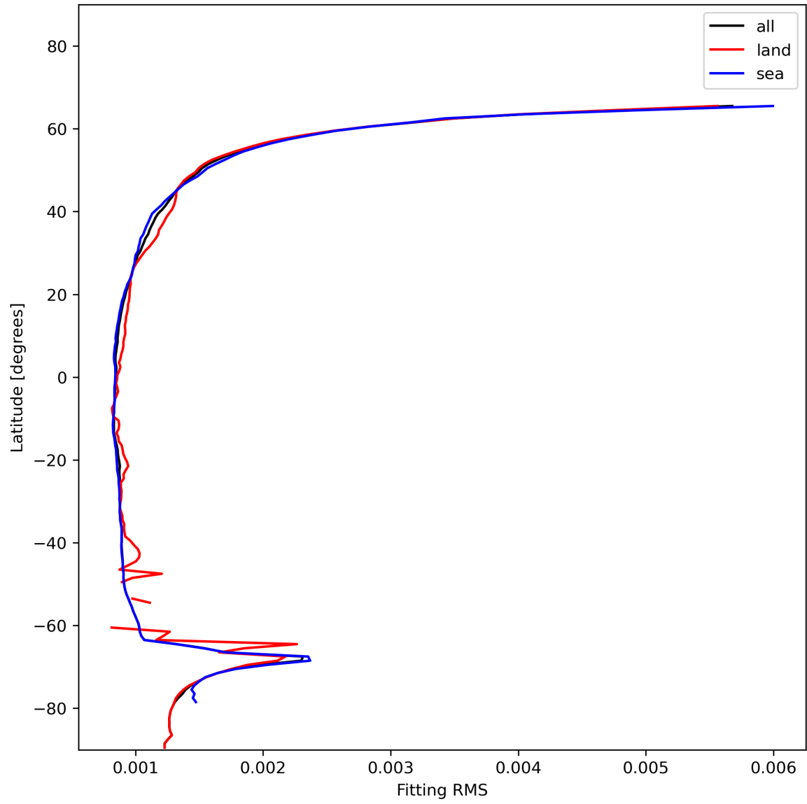
Figure 16: Zonal average of “Fitting RMS” for 2023-12-20 to 2023-12-21.
