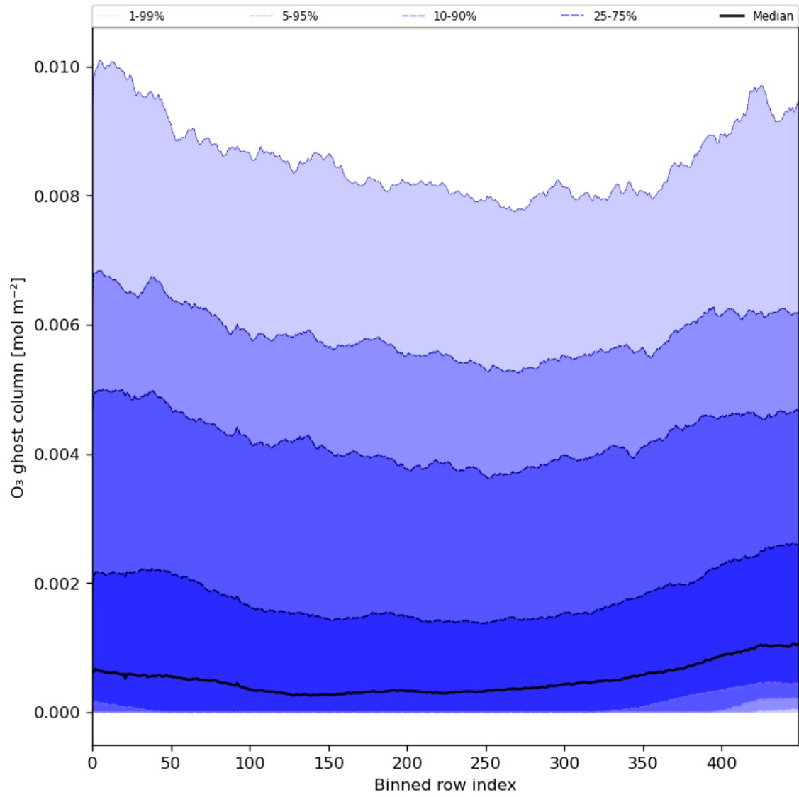
Figure 32: Along track statistics of "O 3 ghost column" for 2023-12-20 to 2023-12-21
