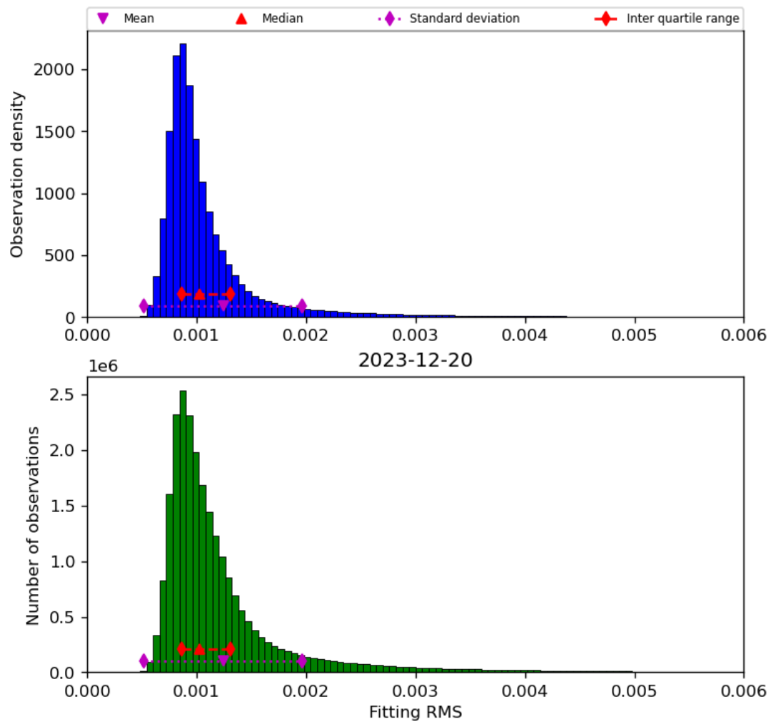
Figure 23: Histogram of “Fitting RMS” for 2023-12-20 to 2023-12-21
