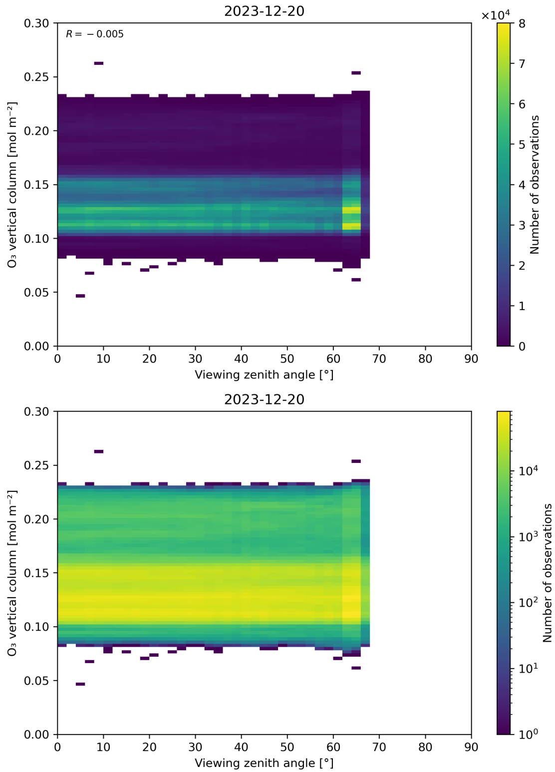
Figure 52: Scatter density plot of “Viewing zenith angle” against “O 3 vertical column” for 2023-12-20 to 2023-12-21.
