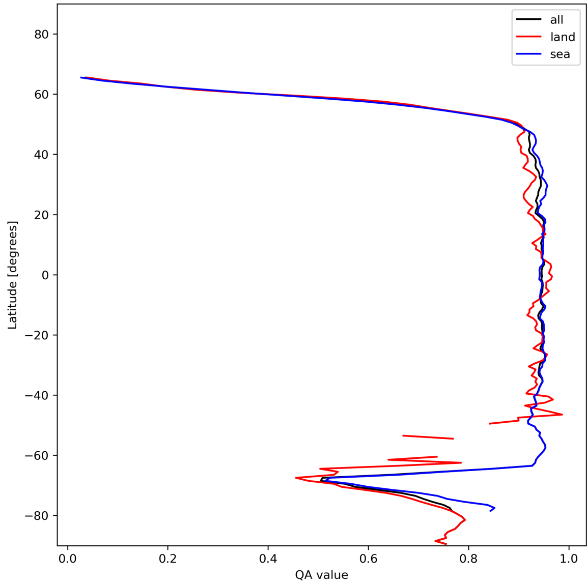
Figure 13: Zonal average of “QA value” for 2023-12-20 to 2023-12-21.
