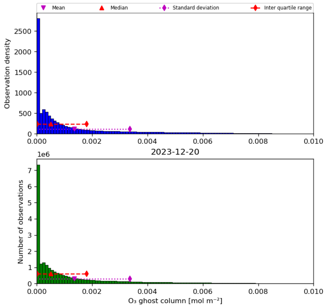
Figure 25: Histogram of “O 3 ghost column” for 2023-12-20 to 2023-12-21
