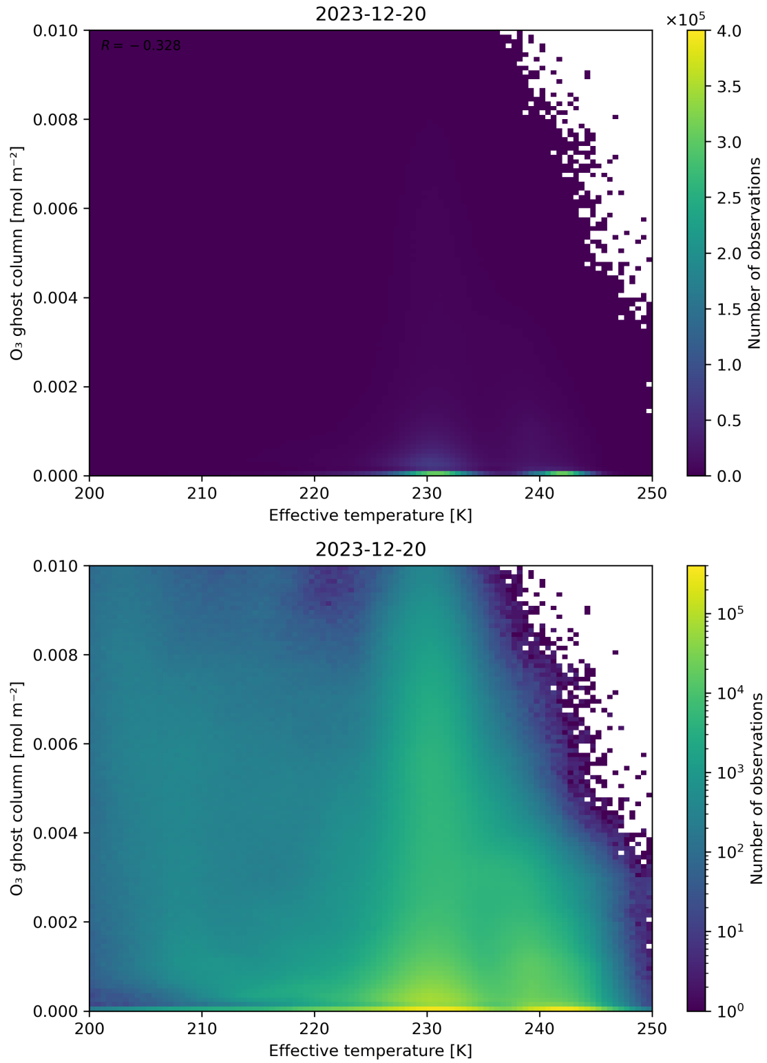
Figure 38: Scatter density plot of “Effective temperature” against “O 3 ghost column” for 2023-12-20 to 2023-12-21.
