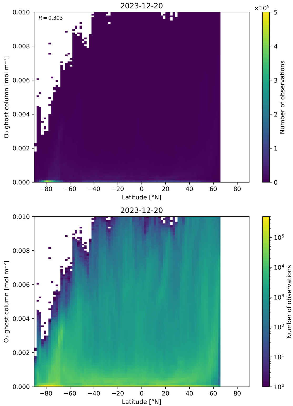
Figure 35: Scatter density plot of “Latitude” against “O 3 ghost column” for 2023-12-20 to 2023-12-21.
