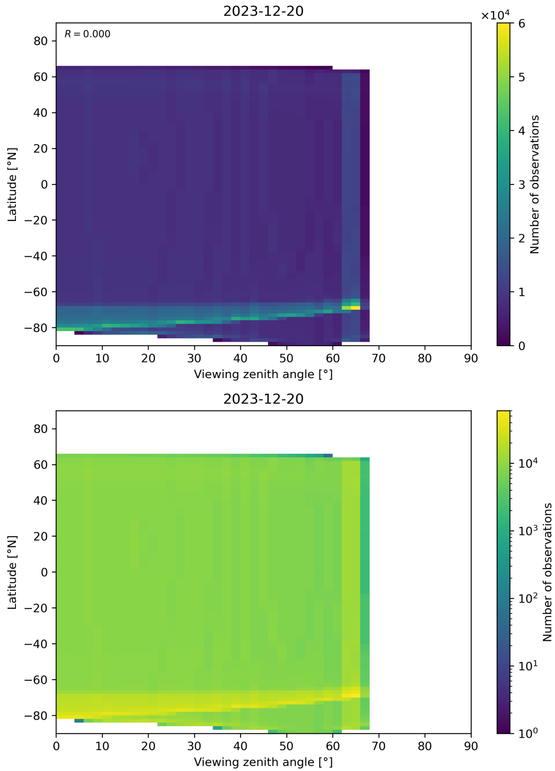
Figure 49: Scatter density plot of “Viewing zenith angle” against “Latitude” for 2023-12-20 to 2023-12-21.
