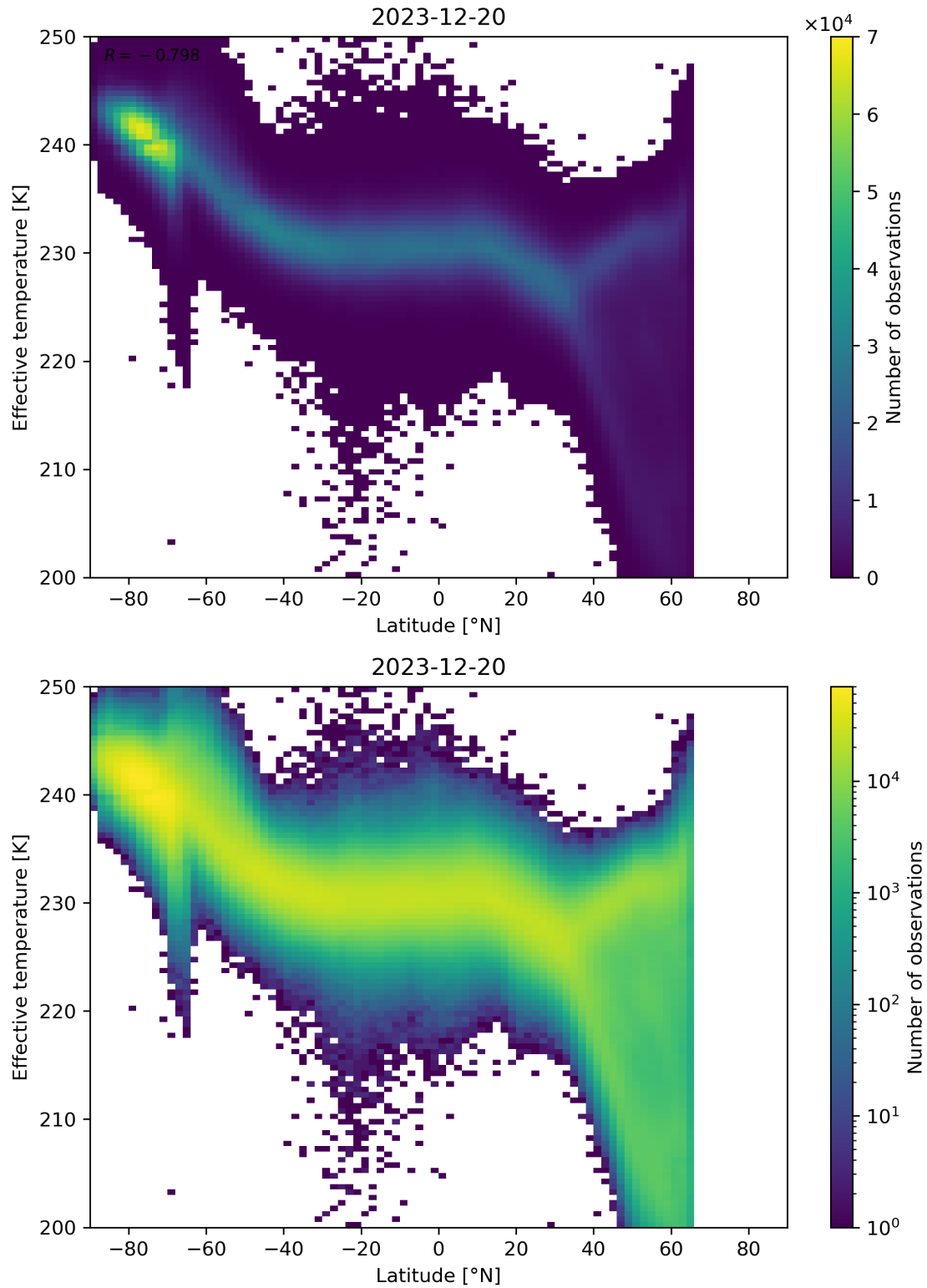
Figure 34: Scatter density plot of “Latitude” against “Effective temperature” for 2023-12-20 to 2023-12-21.
