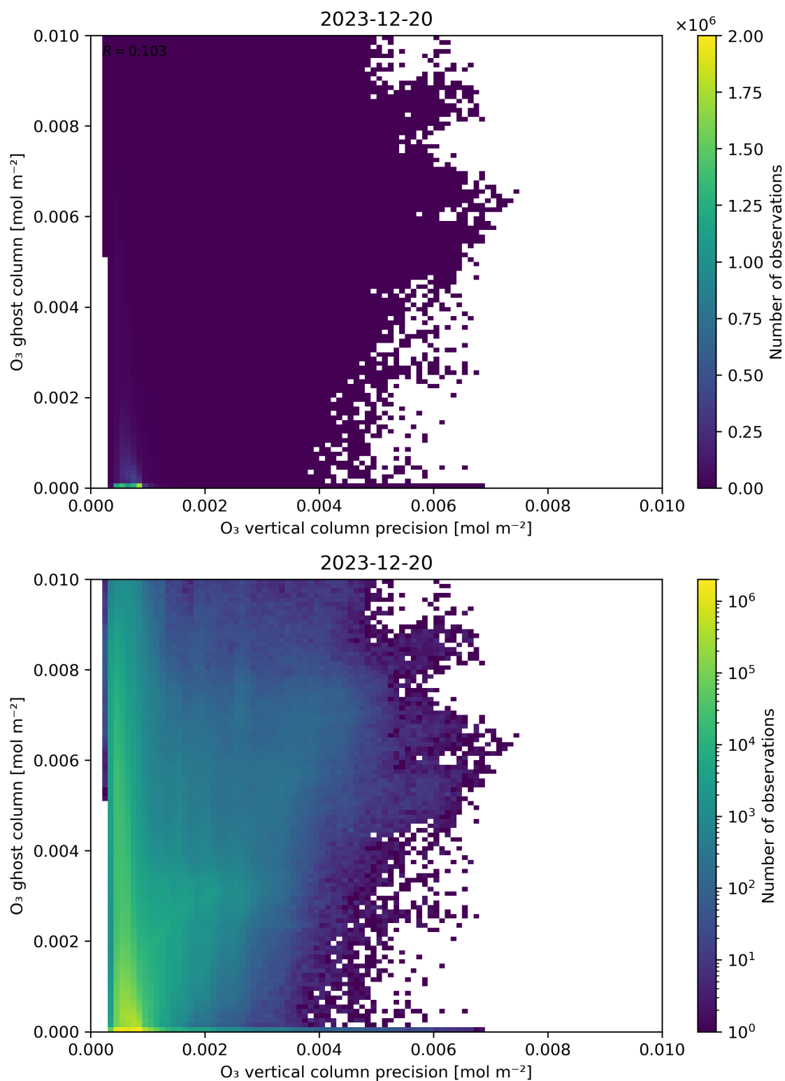
Figure 43: Scatter density plot of “ O_3 vertical column precision” against “ O_3 ghost column” for 2023-12-20 to 2023-12-21.
