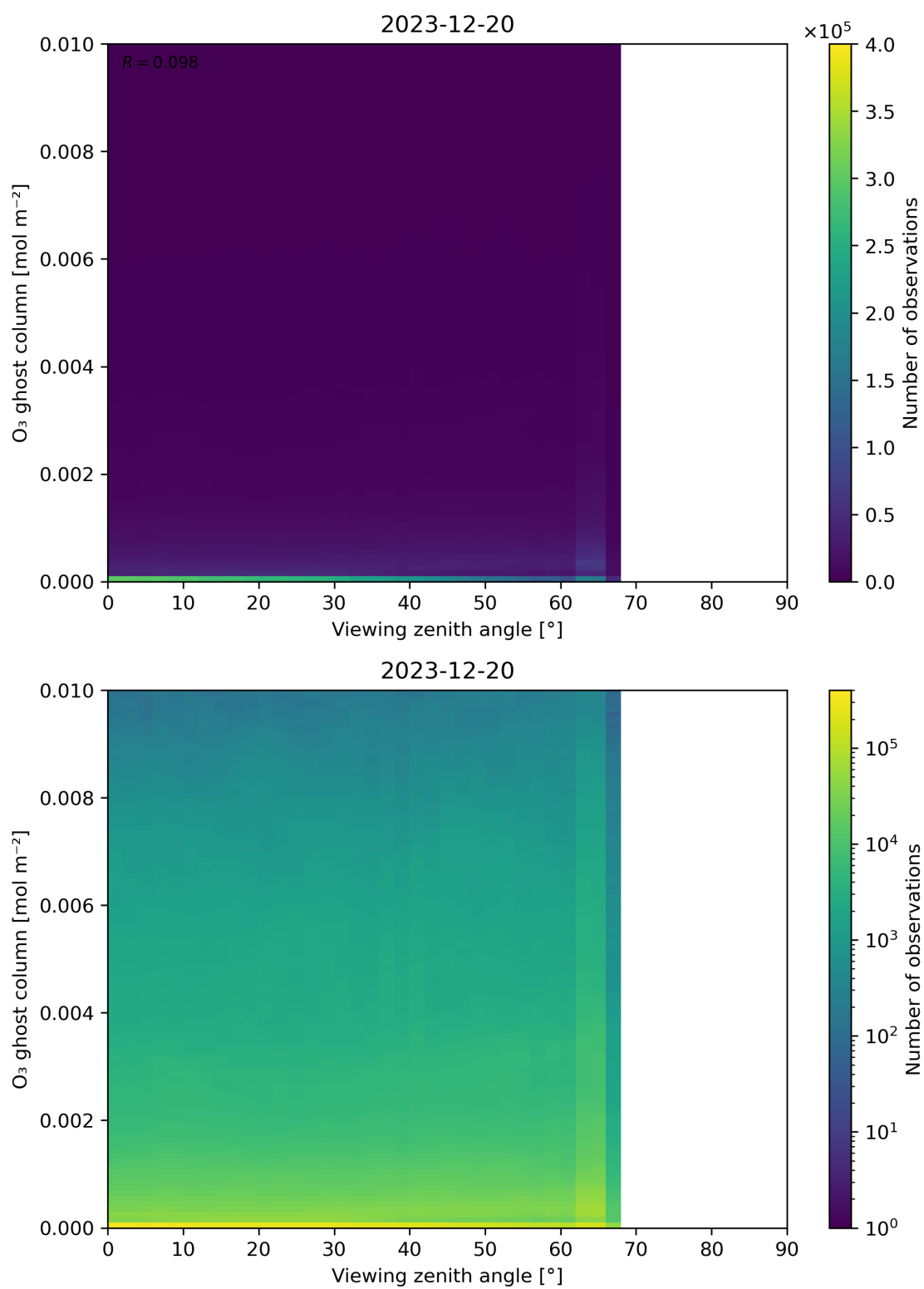
Figure 51: Scatter density plot of “Viewing zenith angle” against “O 3 ghost column” for 2023-12-20 to 2023-12-21.
