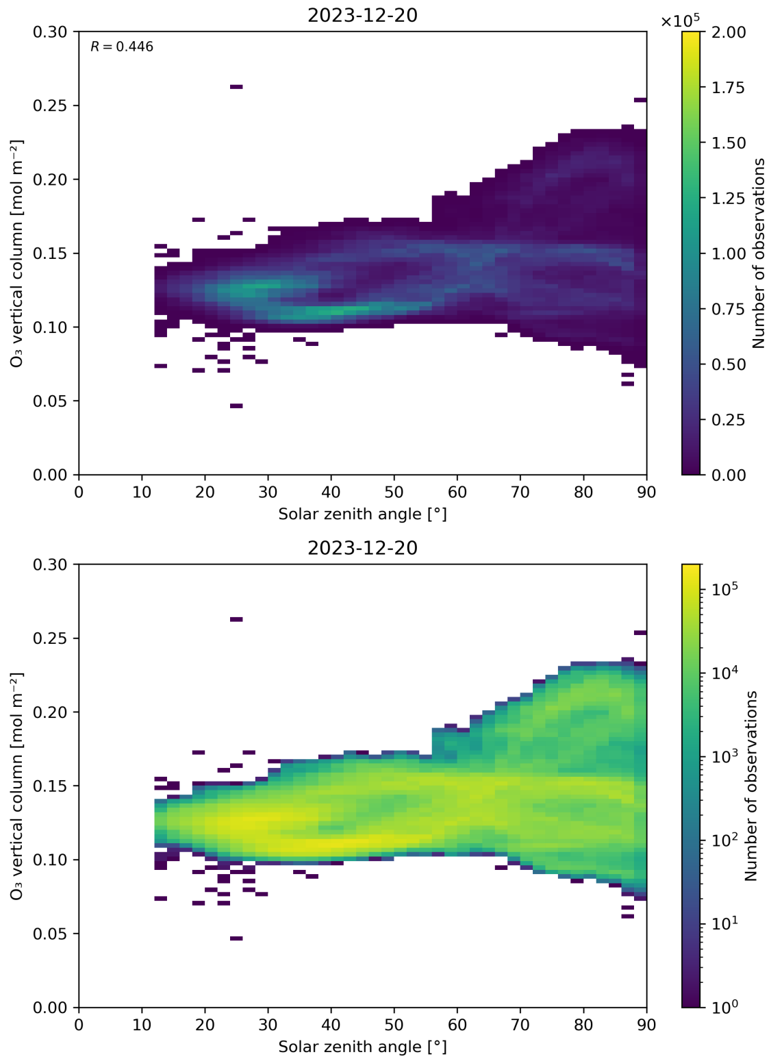
Figure 47: Scatter density plot of “Solar zenith angle” against “O 3 vertical column” for 2023-12-20 to 2023-12-21.
