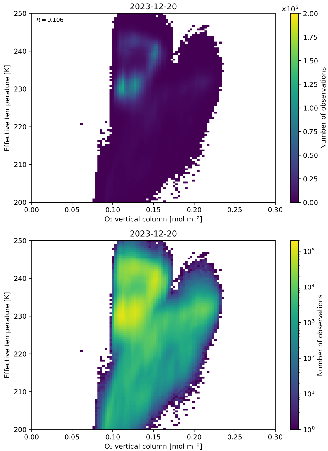
Figure 39: Scatter density plot of “O 3 vertical column” against “Effective temperature” for 2023-12-20 to 2023-12-21.
