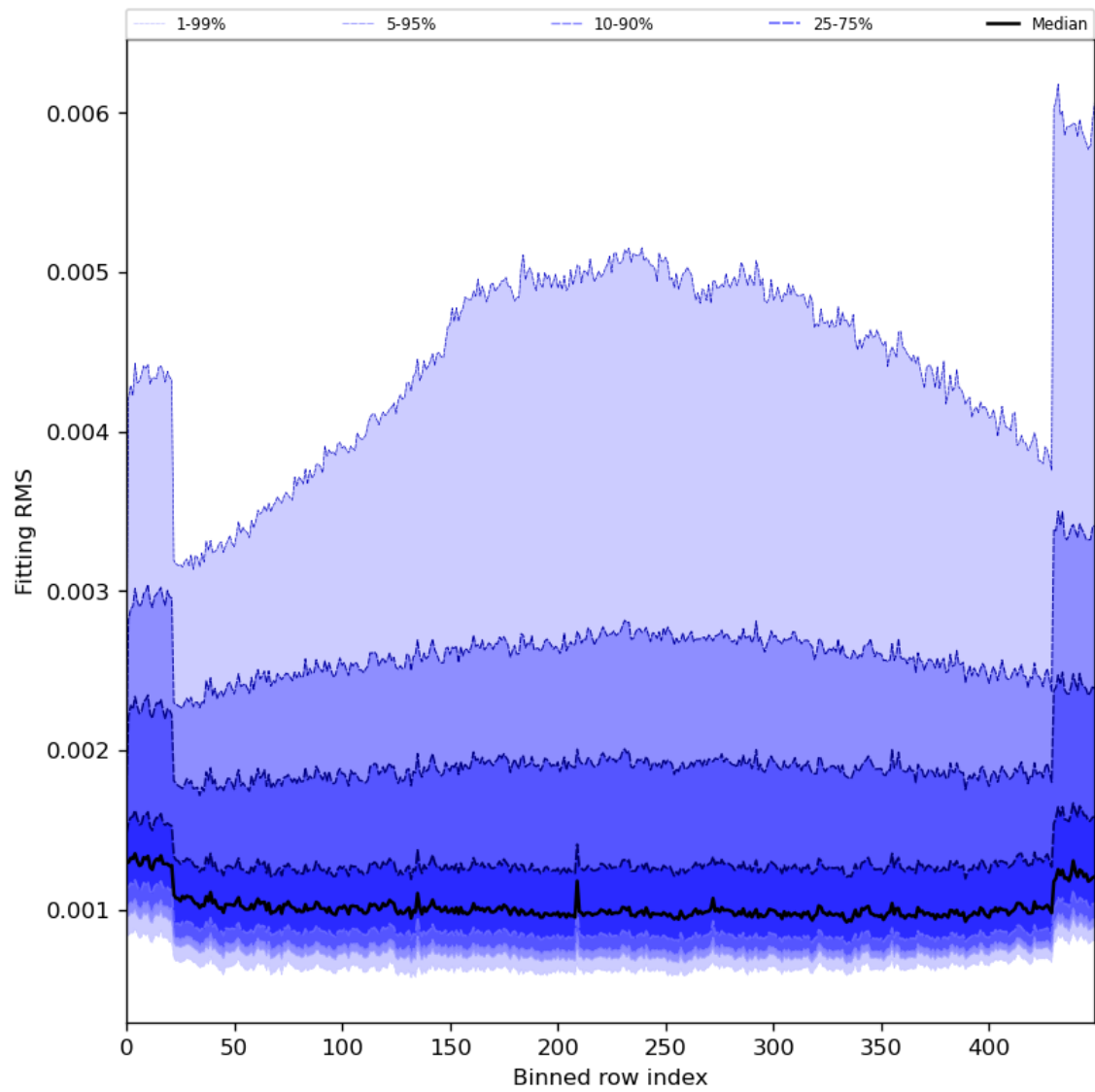
Figure 30: Along track statistics of “Fitting RMS” for 2023-12-20 to 2023-12-21
