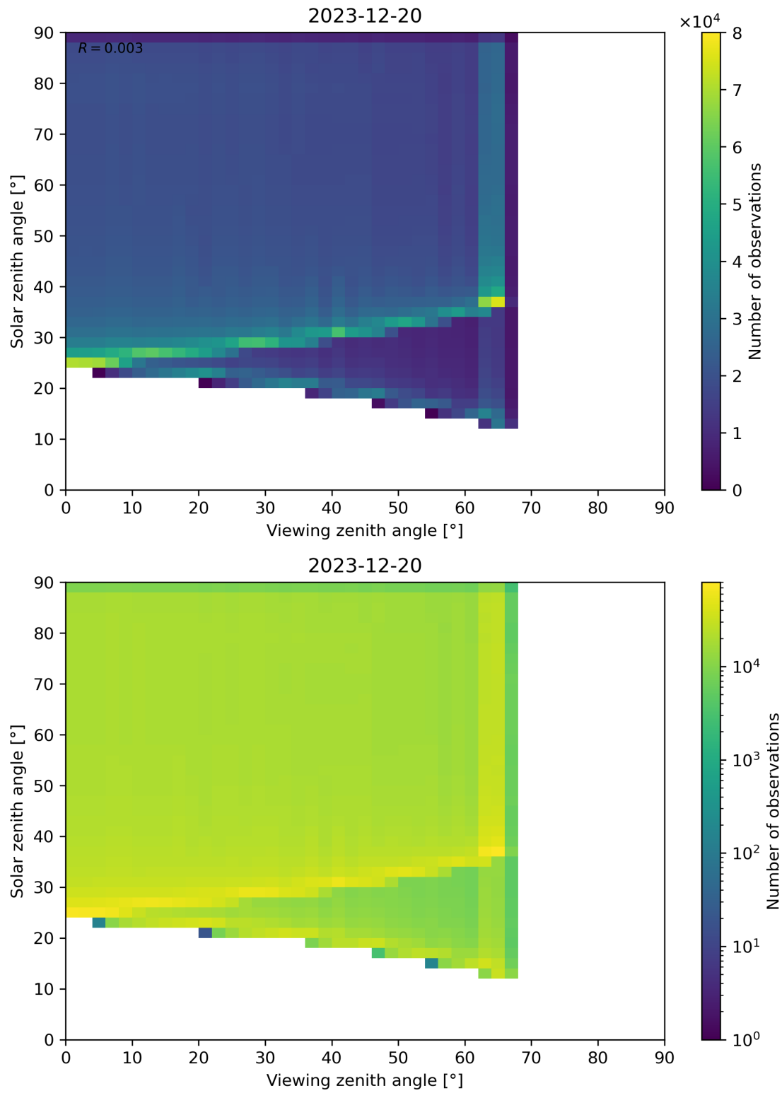
Figure 54: Scatter density plot of “Viewing zenith angle” against “Solar zenith angle” for 2023-12-20 to 2023-12-21.
