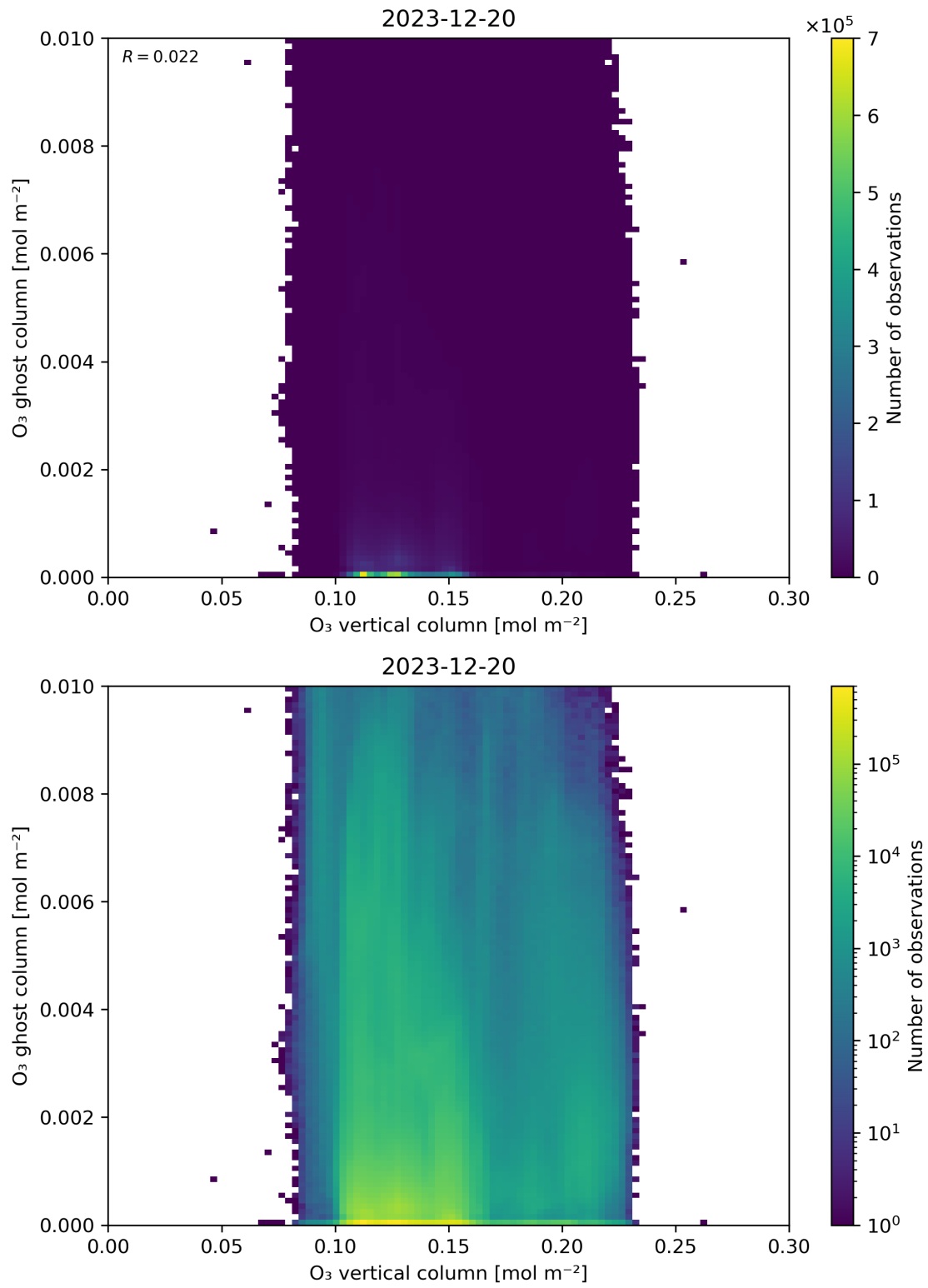
Figure 40: Scatter density plot of “O 3 vertical column” against “O 3 ghost column” for 2023-12-20 to 2023-12-21.
