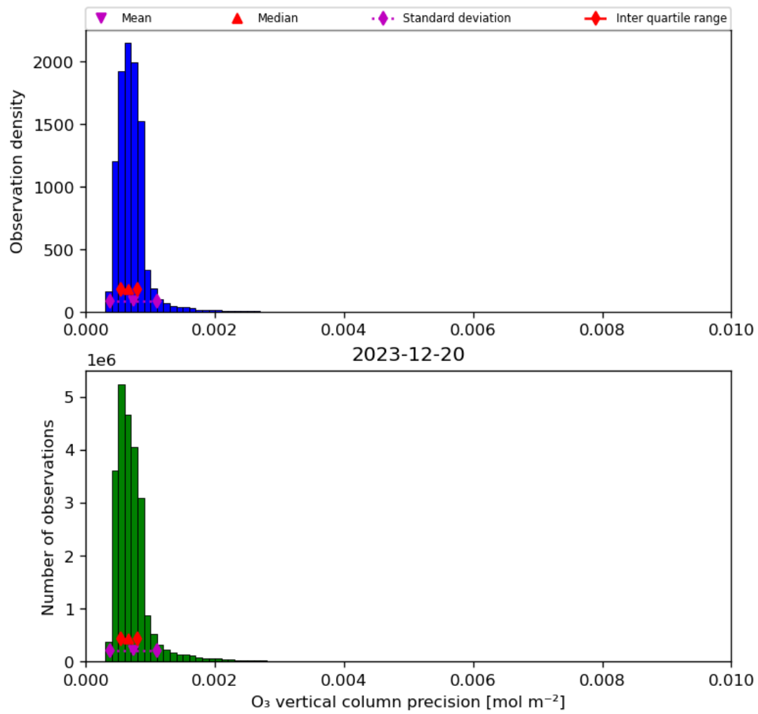
Figure 22: Histogram of “O 3 vertical column precision” for 2023-12-20 to 2023-12-21
