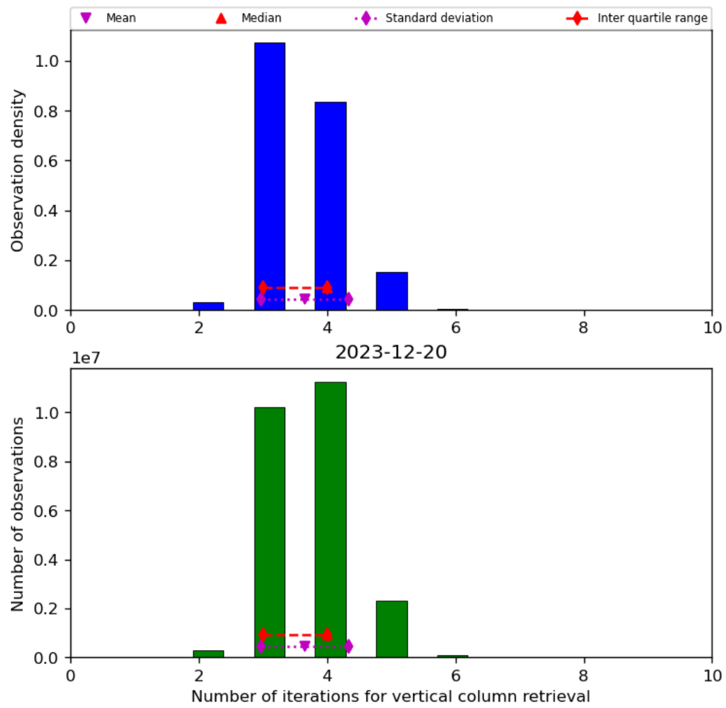
Figure 26: Histogram of “Number of iterations for vertical column retrieval” for 2023-12-20 to 2023-12-21
