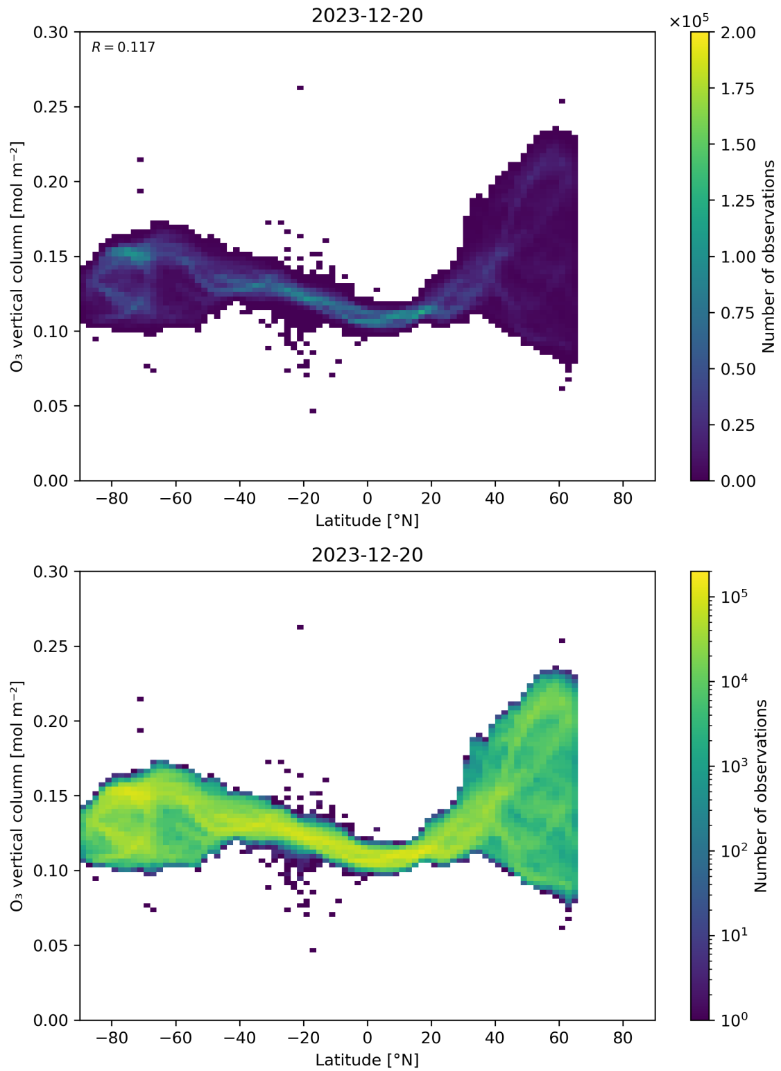
Figure 36: Scatter density plot of “Latitude” against “O 3 vertical column” for 2023-12-20 to 2023-12-21.
