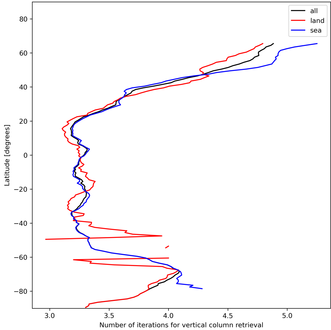
Figure 19: Zonal average of “Number of iterations for vertical column retrieval” for 2023-12-20 to 2023-12-21.
