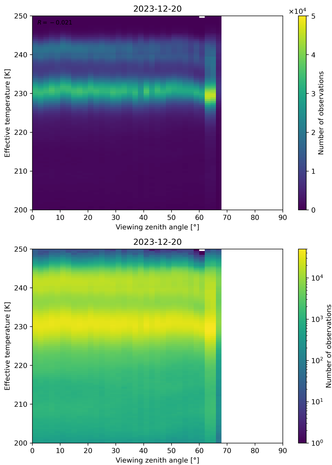
Figure 50: Scatter density plot of “Viewing zenith angle” against “Effective temperature” for 2023-12-20 to 2023-12-21.
