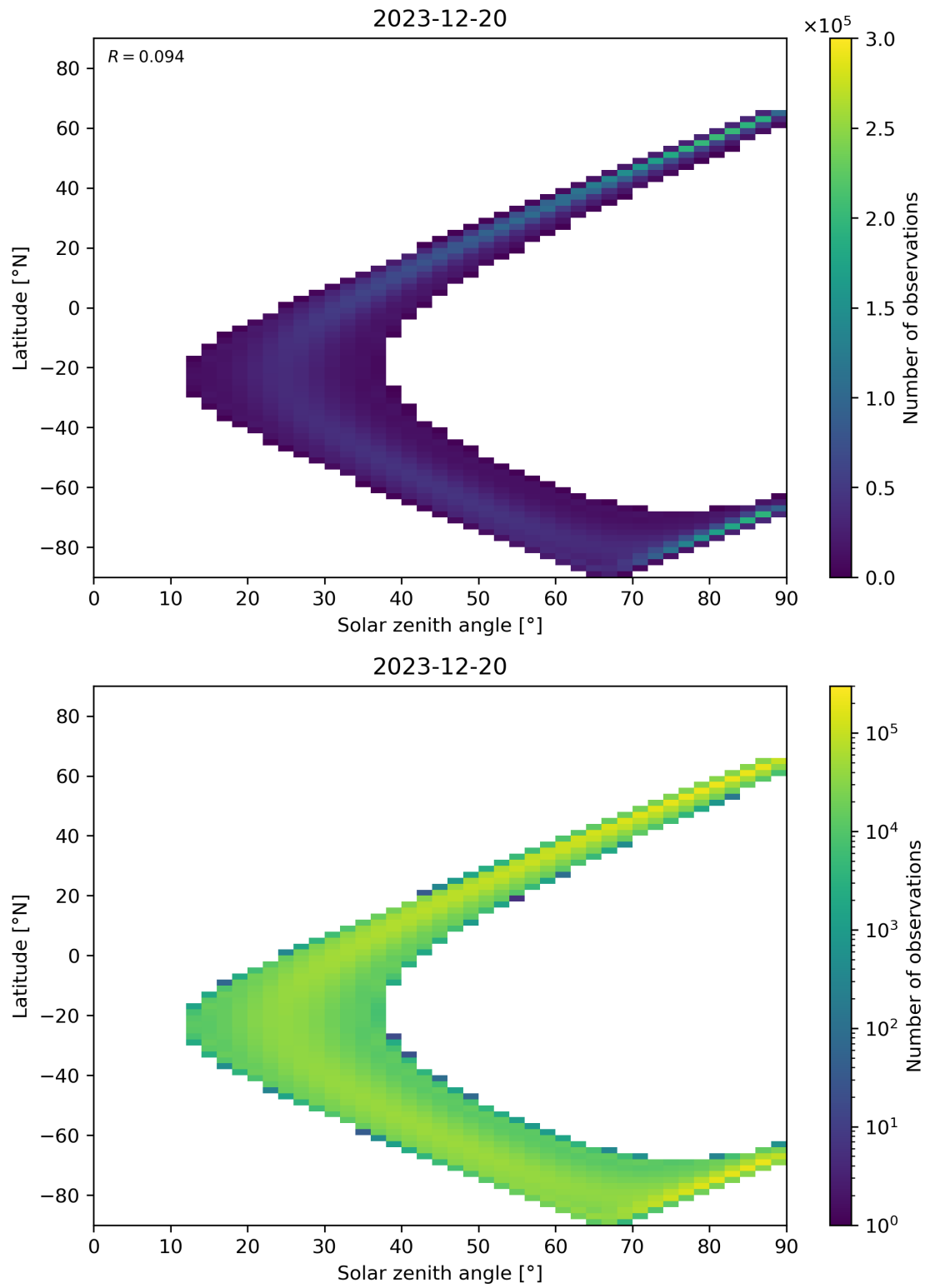
Figure 44: Scatter density plot of “Solar zenith angle” against “Latitude” for 2023-12-20 to 2023-12-21.
