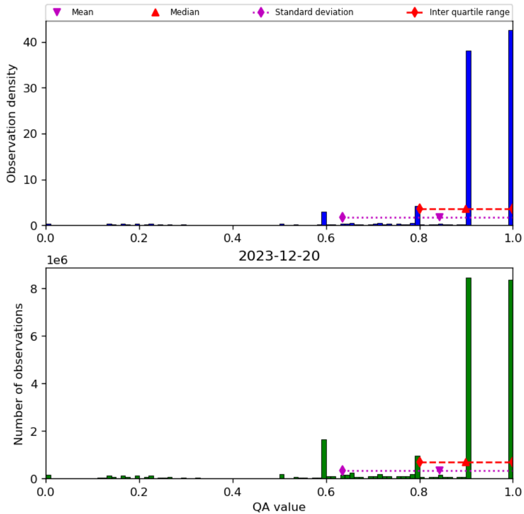
Figure 20: Histogram of “QA value” for 2023-12-20 to 2023-12-21
