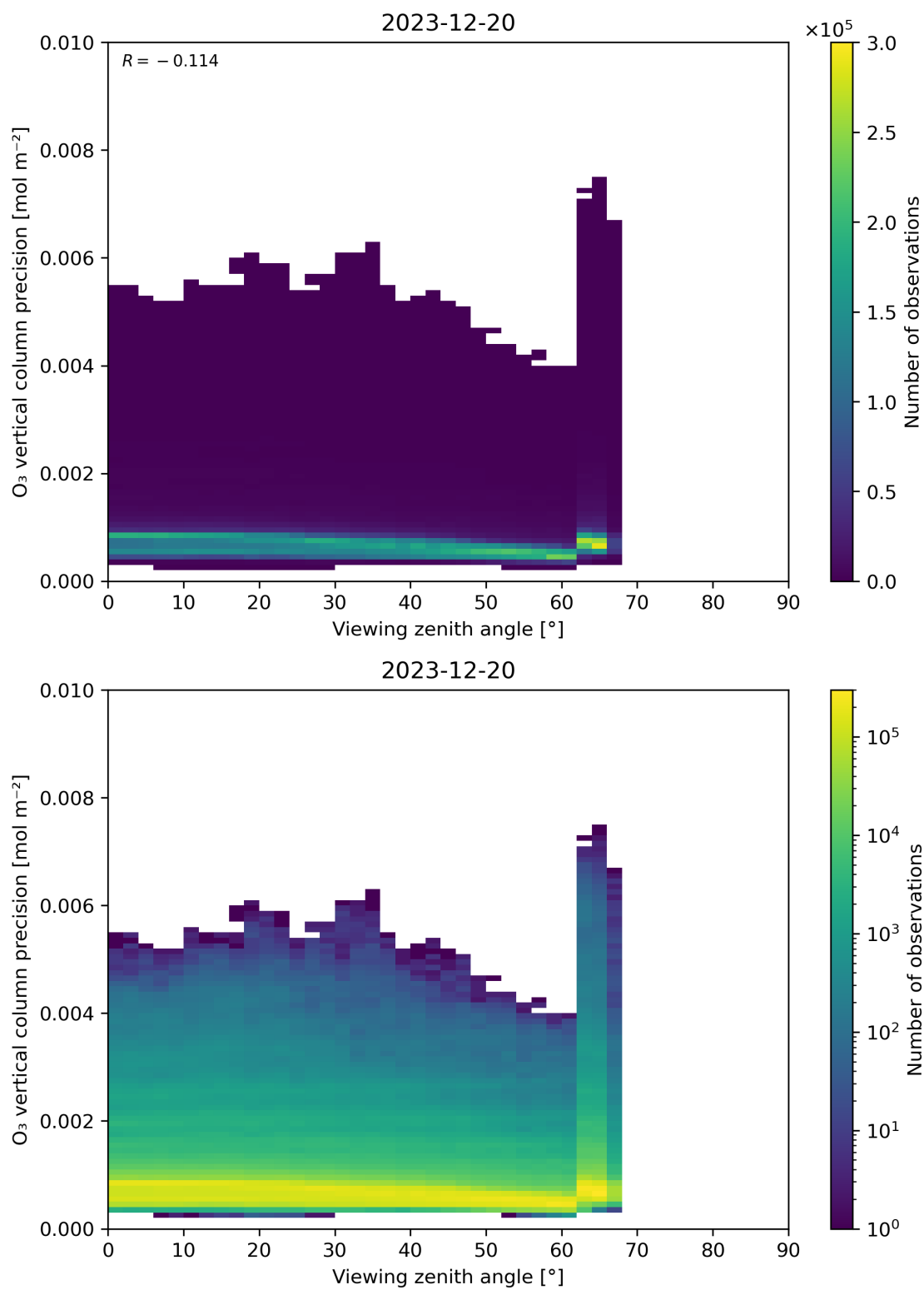
Figure 53: Scatter density plot of “Viewing zenith angle” against “O 3 vertical column precision” for 2023-12-20 to 2023-12-21.
