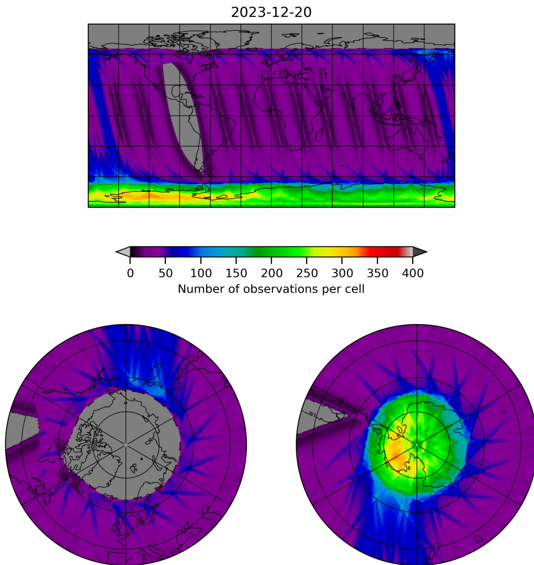
Figure 12: Map of the number of observations for 2023-12-20 to 2023-12-21
