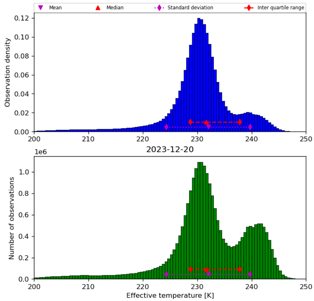
Figure 24: Histogram of “Effective temperature” for 2023-12-20 to 2023-12-21
