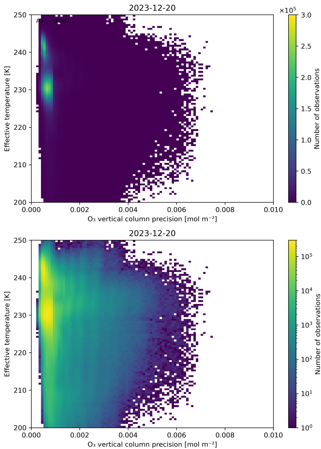
Figure 42: Scatter density plot of “O 3 vertical column precision” against “Effective temperature” for 2023-12-20 to 2023-12-21.
