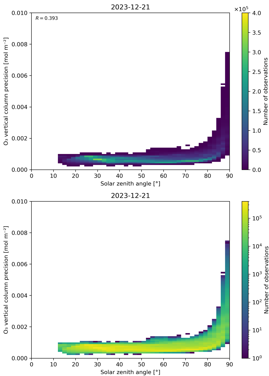
Figure 48: Scatter density plot of “Solar zenith angle” against “O 3 vertical column precision” for 2023-12-20 to 2023-12-22.
