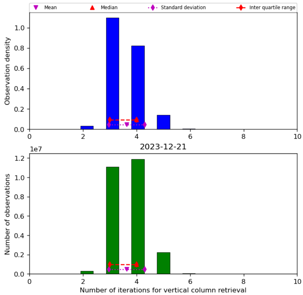
Figure 26: Histogram of “Number of iterations for vertical column retrieval” for 2023-12-20 to 2023-12-22
