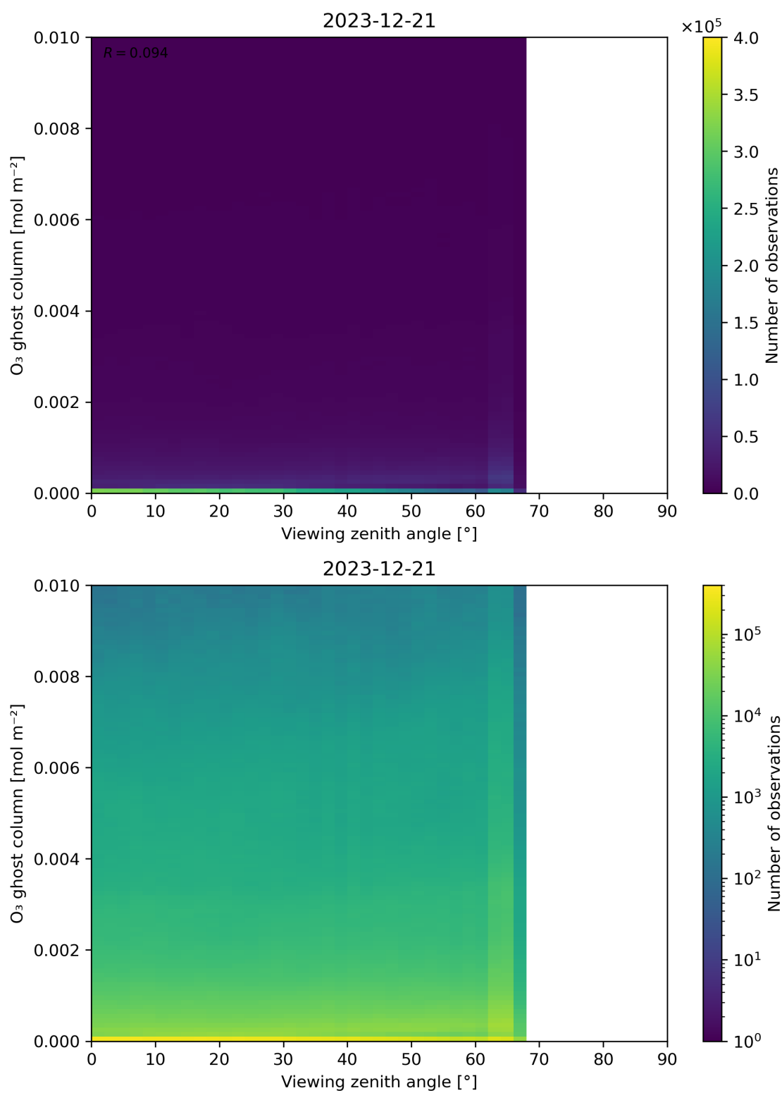
Figure 51: Scatter density plot of “Viewing zenith angle” against “O 3 ghost column” for 2023-12-20 to 2023-12-22.
