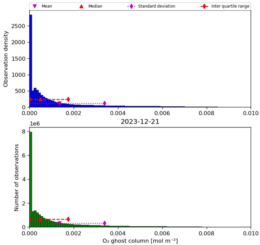
Figure 25: Histogram of “O 3 ghost column” for 2023-12-20 to 2023-12-22
