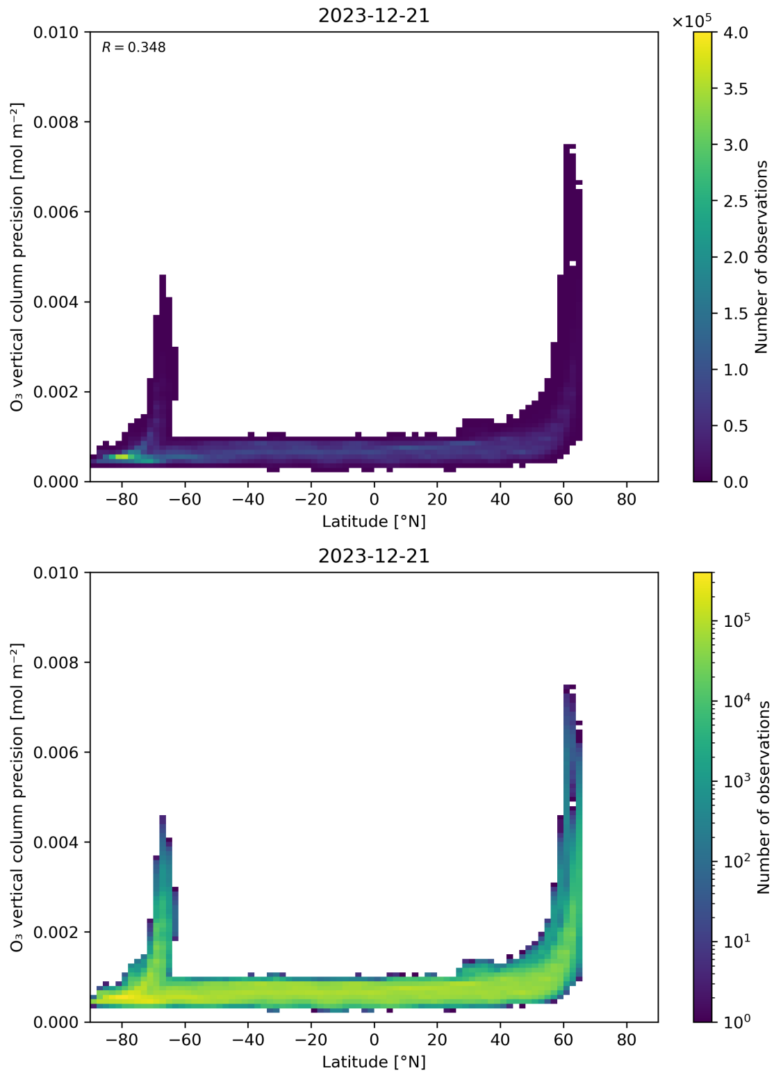
Figure 37: Scatter density plot of “Latitude” against “O 3 vertical column precision” for 2023-12-20 to 2023-12-22.
