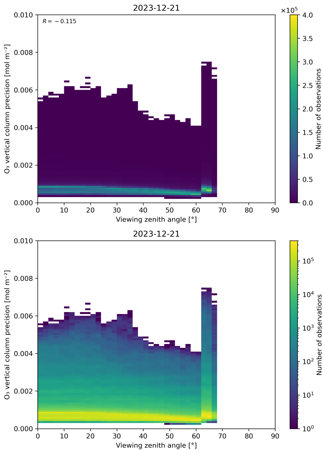
Figure 53: Scatter density plot of “Viewing zenith angle” against “O 3 vertical column precision” for 2023-12-20 to 2023-12-22.
