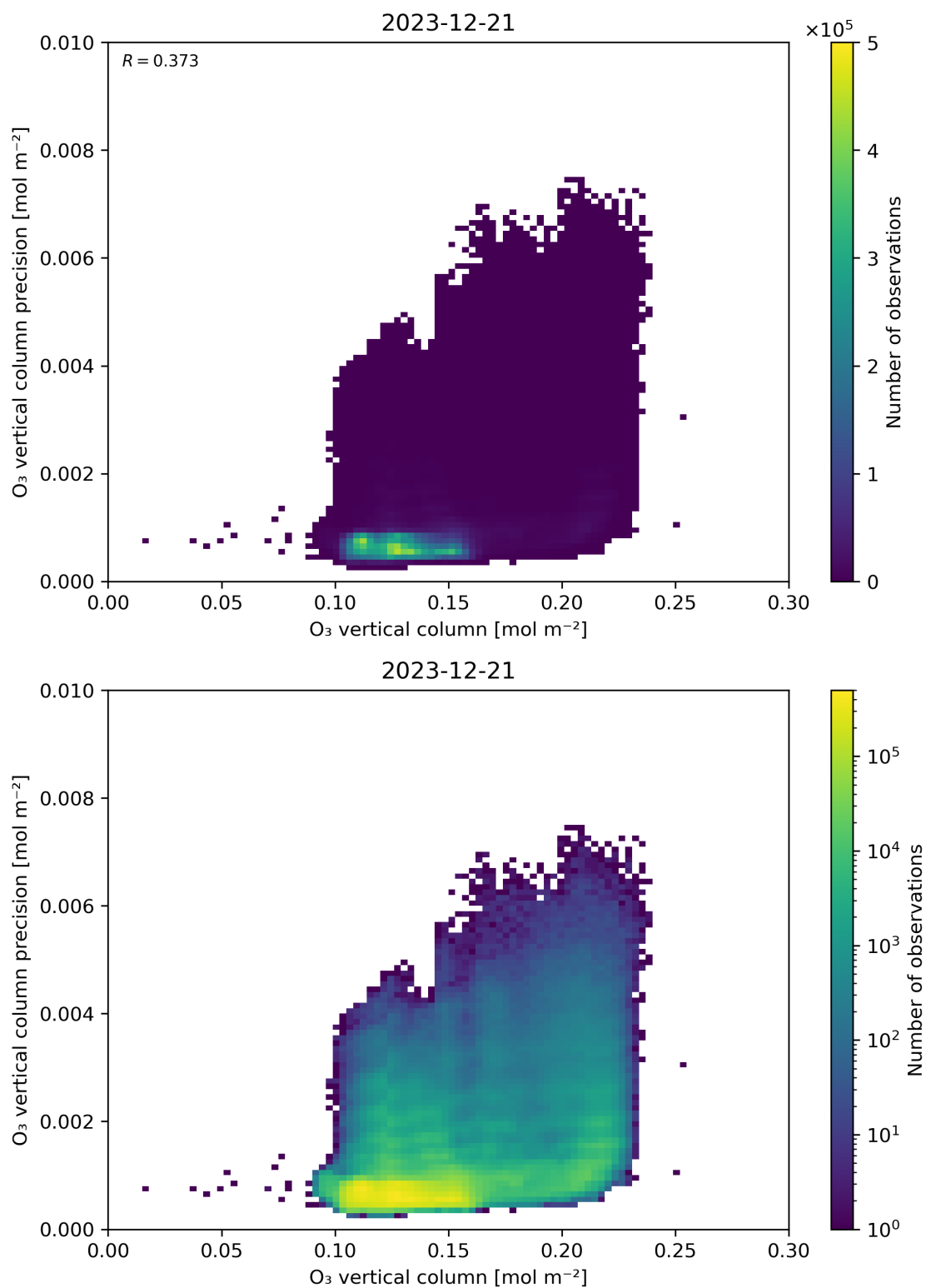
Figure 41: Scatter density plot of “O 3 vertical column” against “O 3 vertical column precision” for 2023-12-20 to 2023-12-22.
