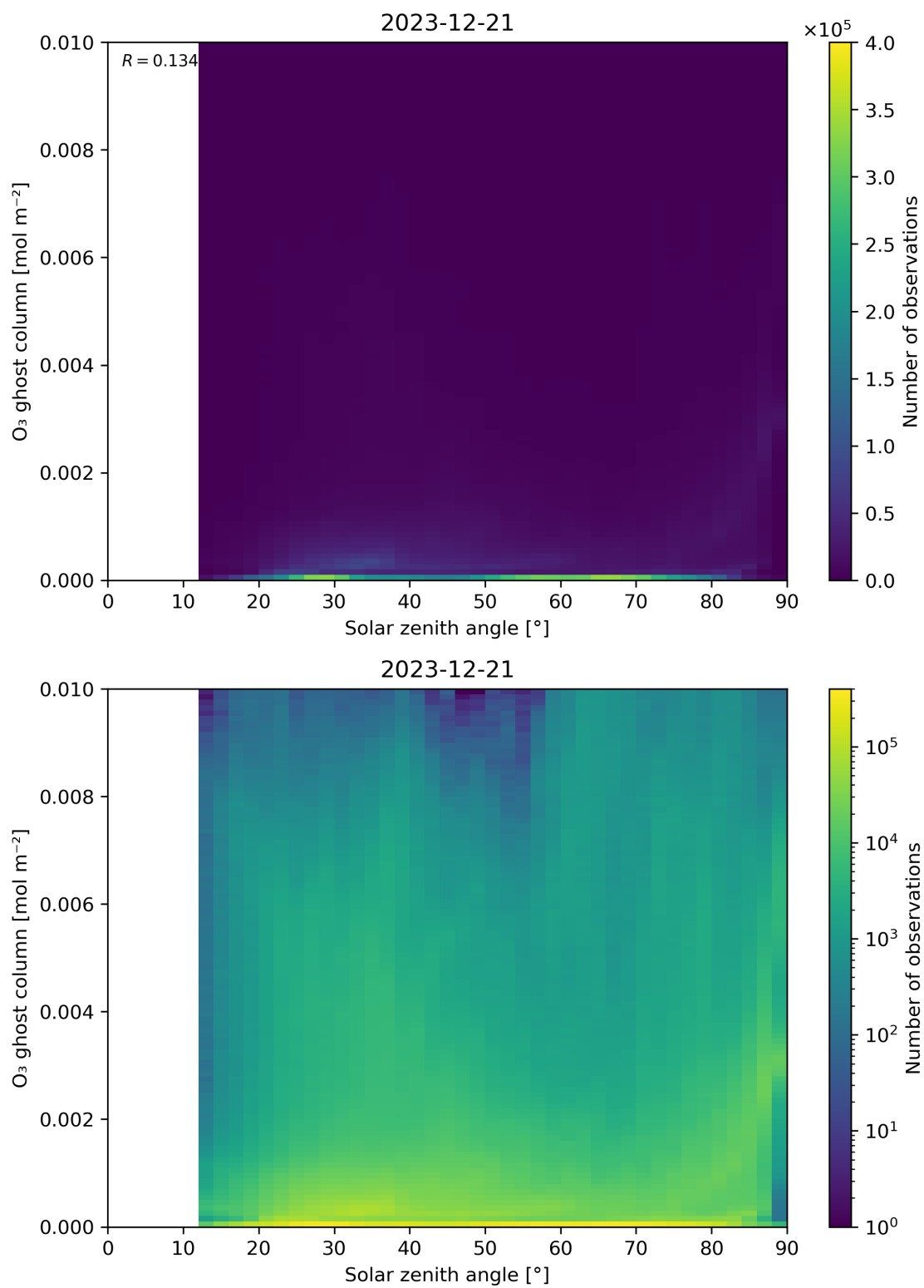
Figure 46: Scatter density plot of “Solar zenith angle” against “O 3 ghost column” for 2023-12-20 to 2023-12-22.
