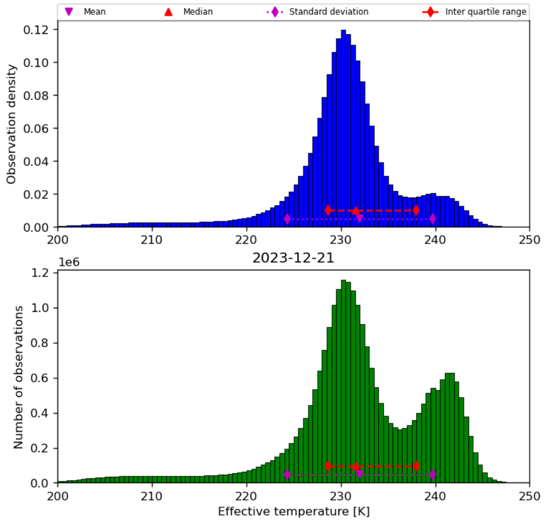
Figure 24: Histogram of “Effective temperature” for 2023-12-20 to 2023-12-22
