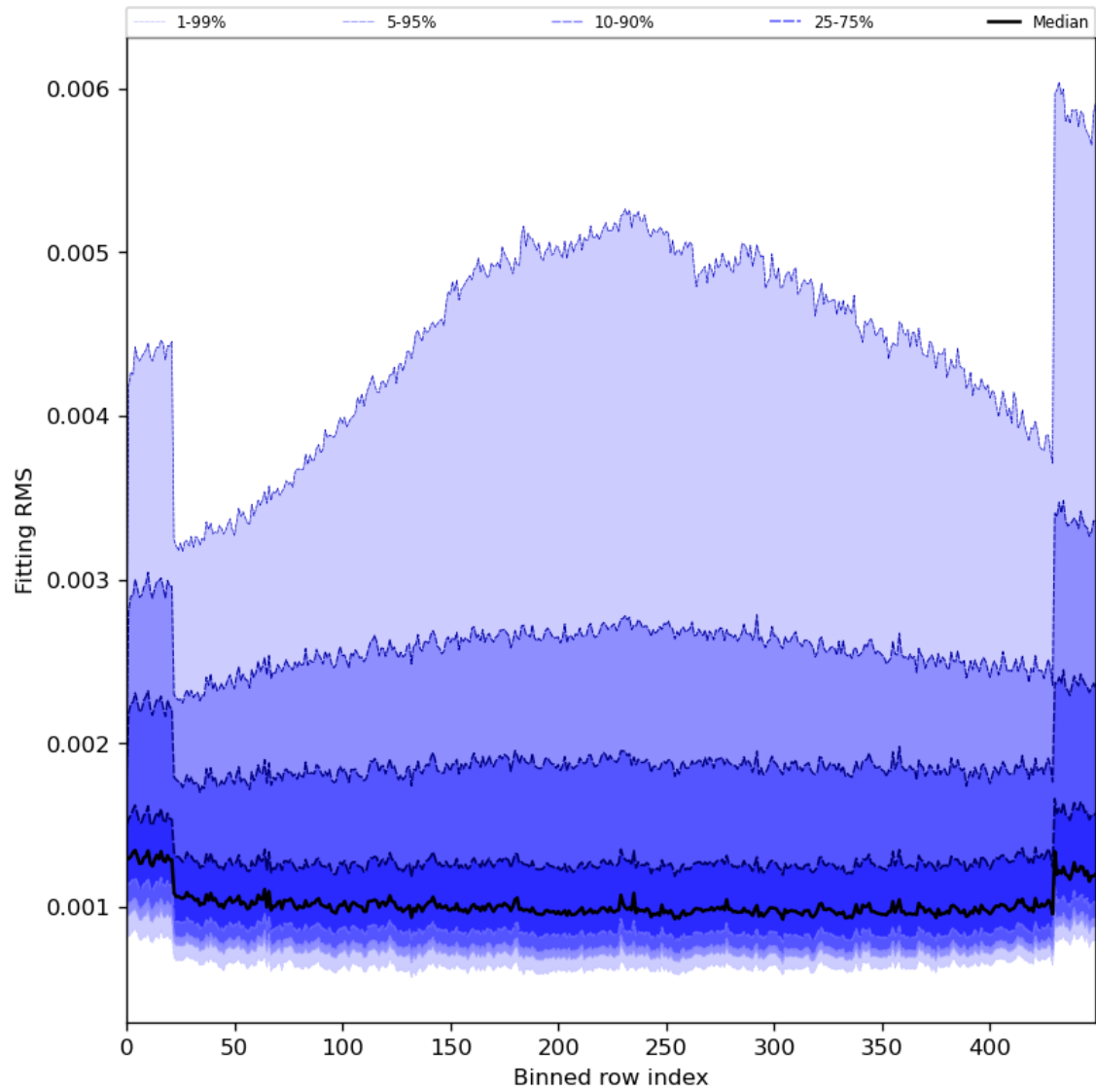
Figure 30: Along track statistics of “Fitting RMS” for 2023-12-20 to 2023-12-22
