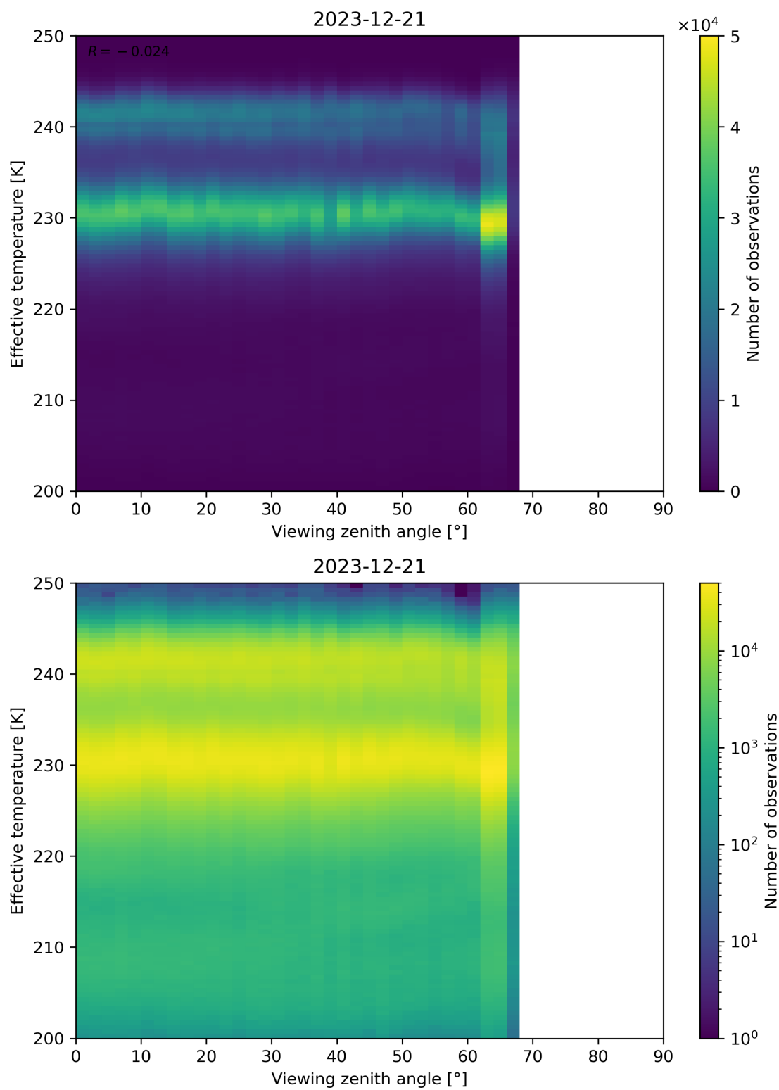
Figure 50: Scatter density plot of “Viewing zenith angle” against “Effective temperature” for 2023-12-20 to 2023-12-22.
