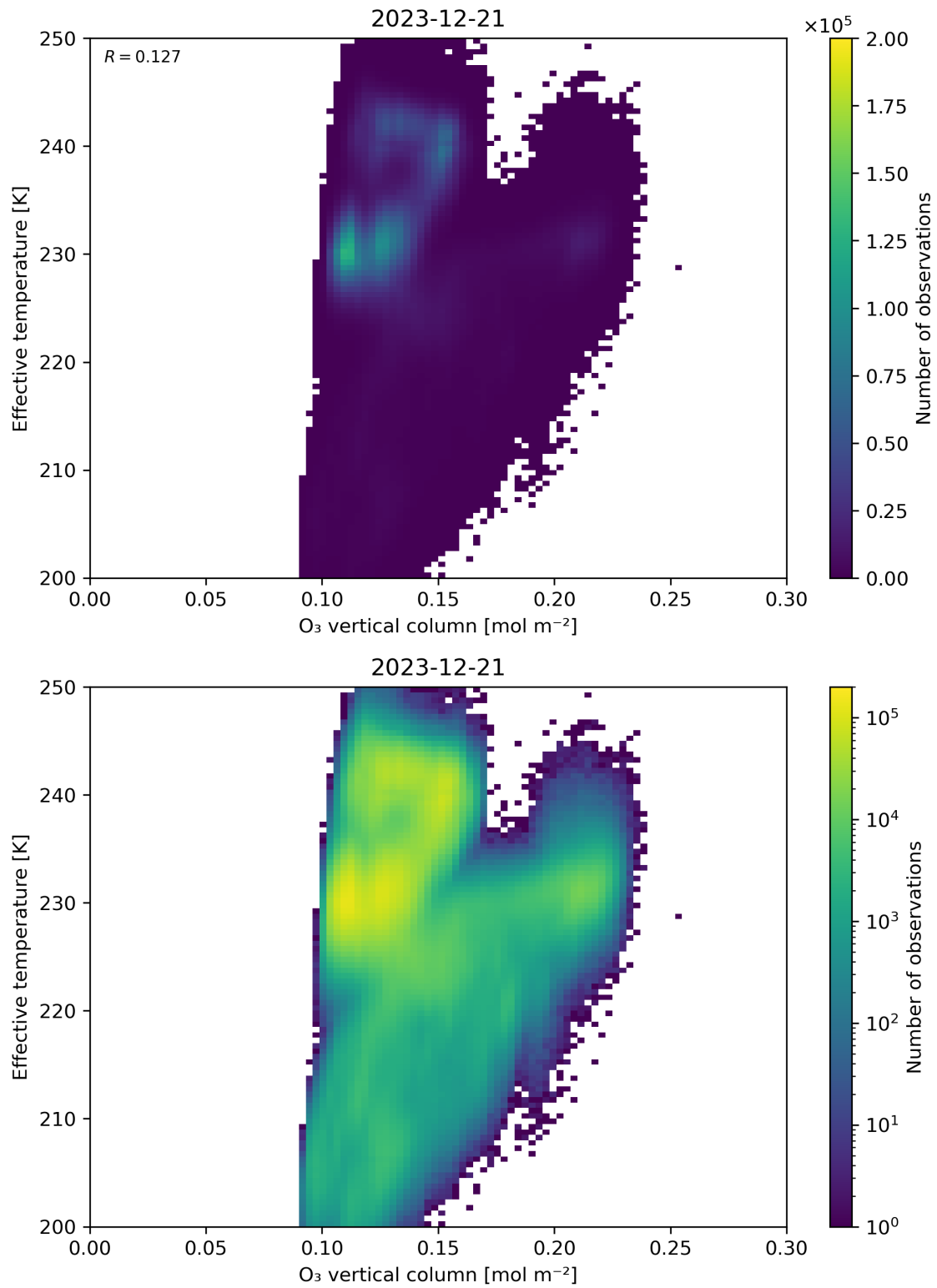
Figure 39: Scatter density plot of “O 3 vertical column” against “Effective temperature” for 2023-12-20 to 2023-12-22.
