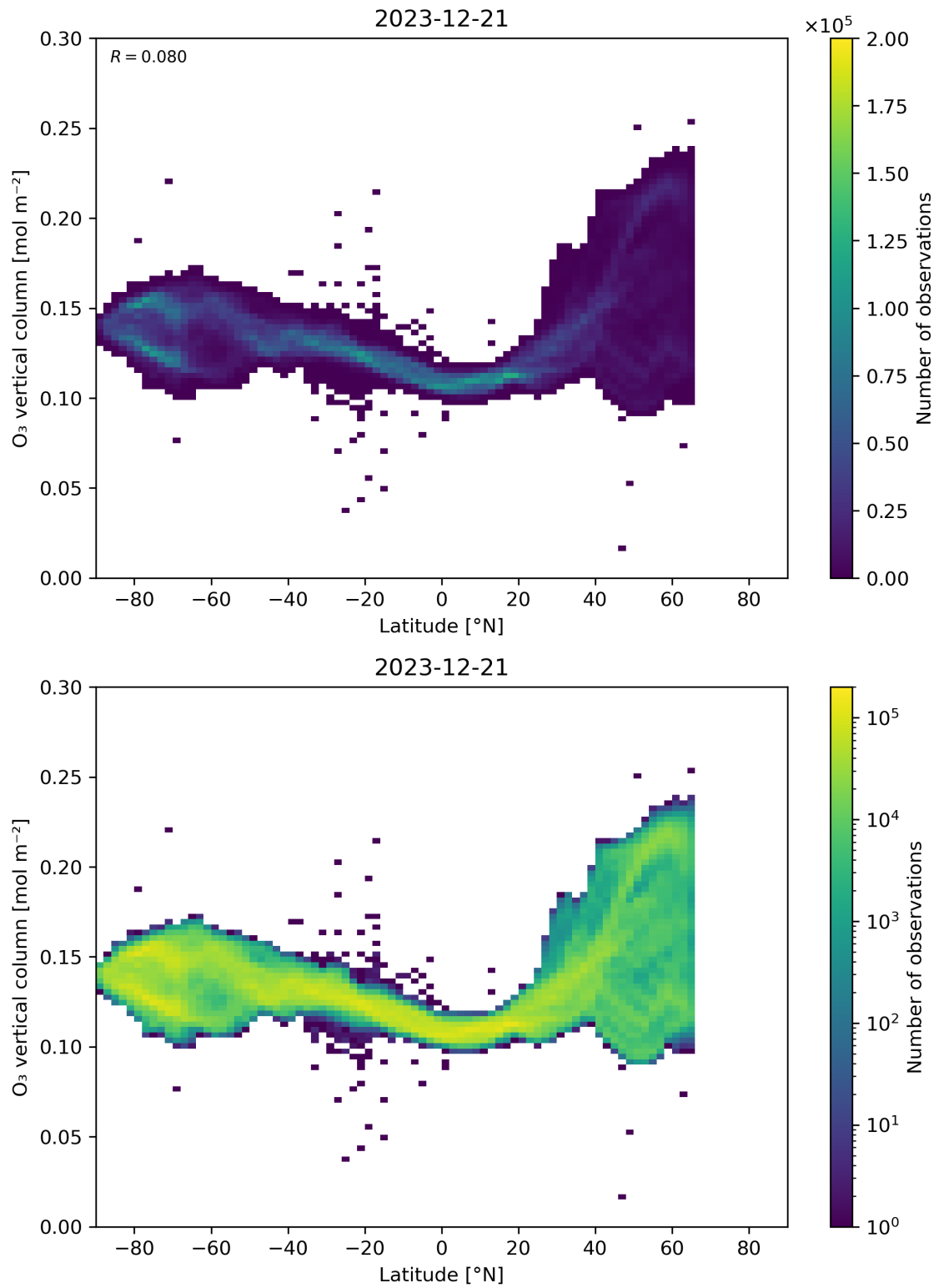
Figure 36: Scatter density plot of “Latitude” against “O 3 vertical column” for 2023-12-20 to 2023-12-22.
