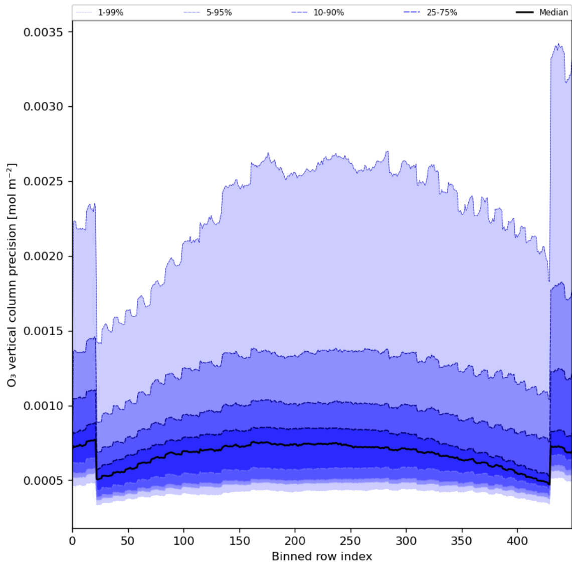
Figure 29: Along track statistics of “O 3 vertical column precision” for 2023-12-20 to 2023-12-22
