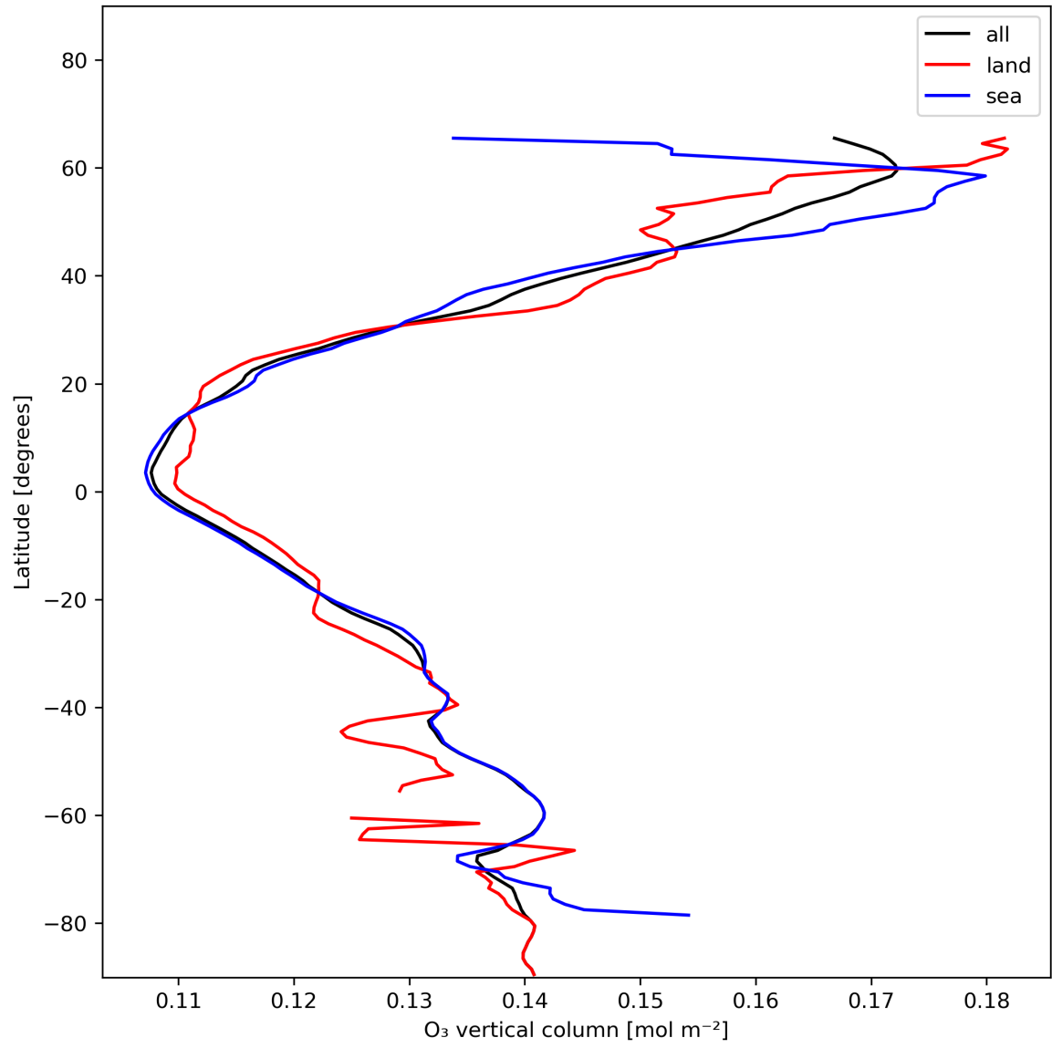
Figure 14: Zonal average of “O 3 vertical column” for 2023-12-20 to 2023-12-22.
