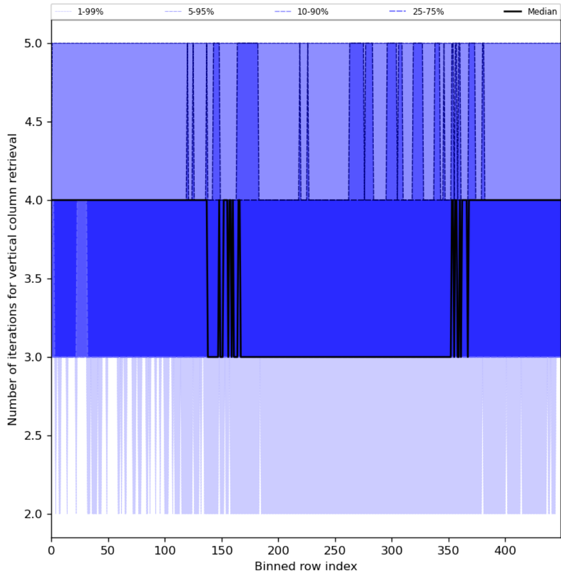
Figure 33: Along track statistics of “Number of iterations for vertical column retrieval” for 2023-12-20 to 2023-12-22
