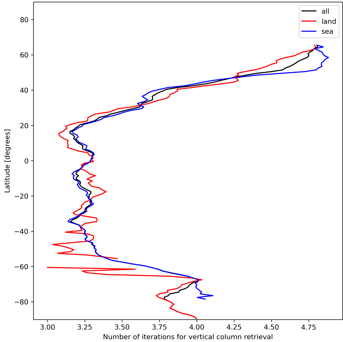
Figure 19: Zonal average of “Number of iterations for vertical column retrieval” for 2023-12-20 to 2023-12-22.
