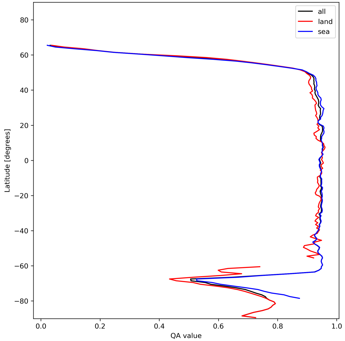
Figure 13: Zonal average of “QA value” for 2023-12-20 to 2023-12-22.
