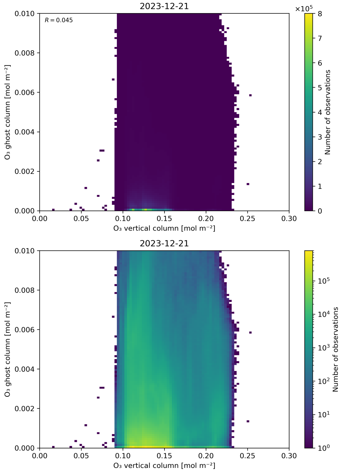
Figure 40: Scatter density plot of “O 3 vertical column” against “O 3 ghost column” for 2023-12-20 to 2023-12-22.
