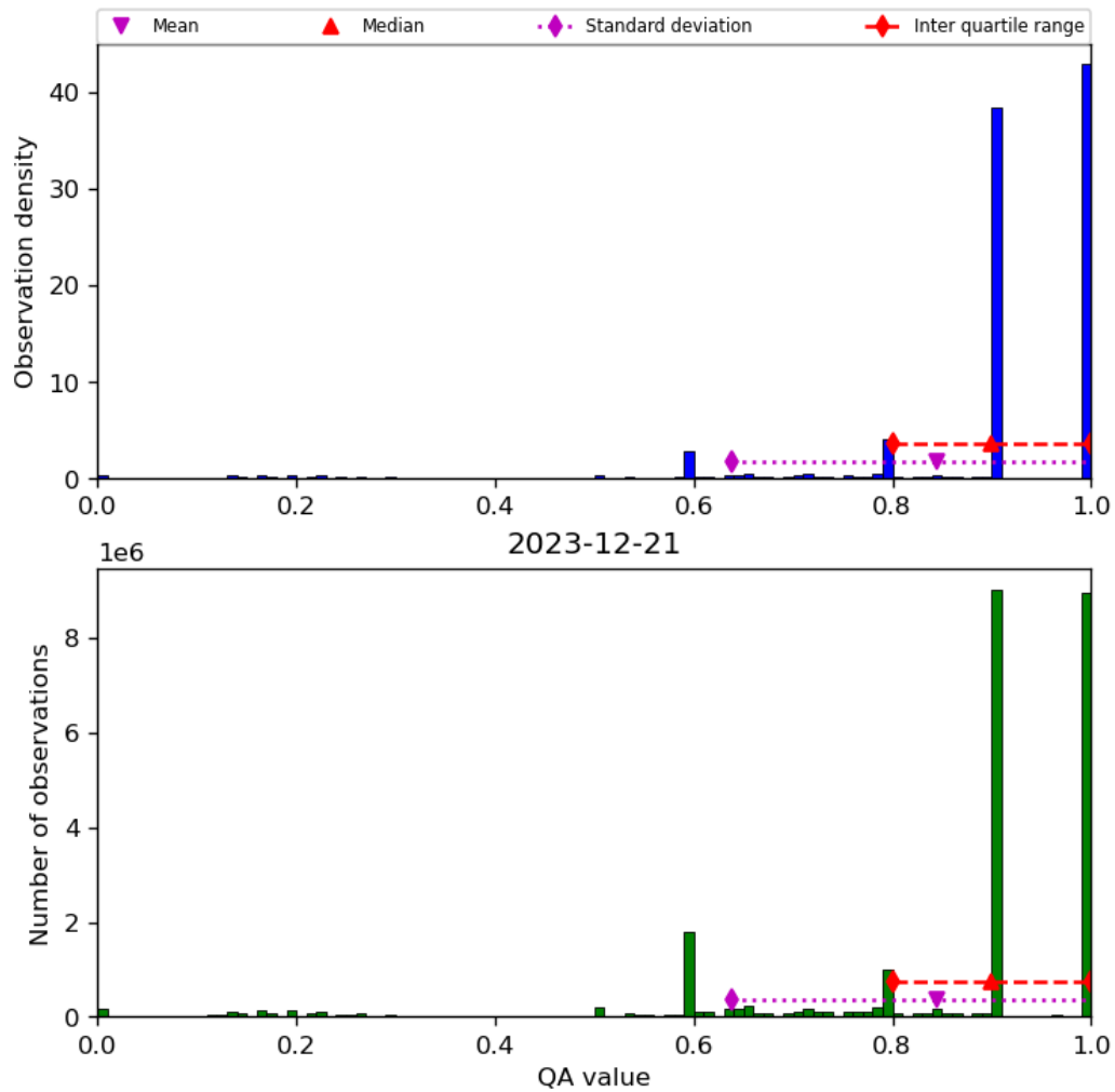
Figure 20: Histogram of “QA value” for 2023-12-20 to 2023-12-22
