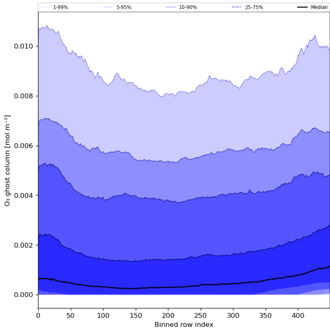
Figure 32: Along track statistics of “O 3 ghost column” for 2023-12-20 to 2023-12-22
