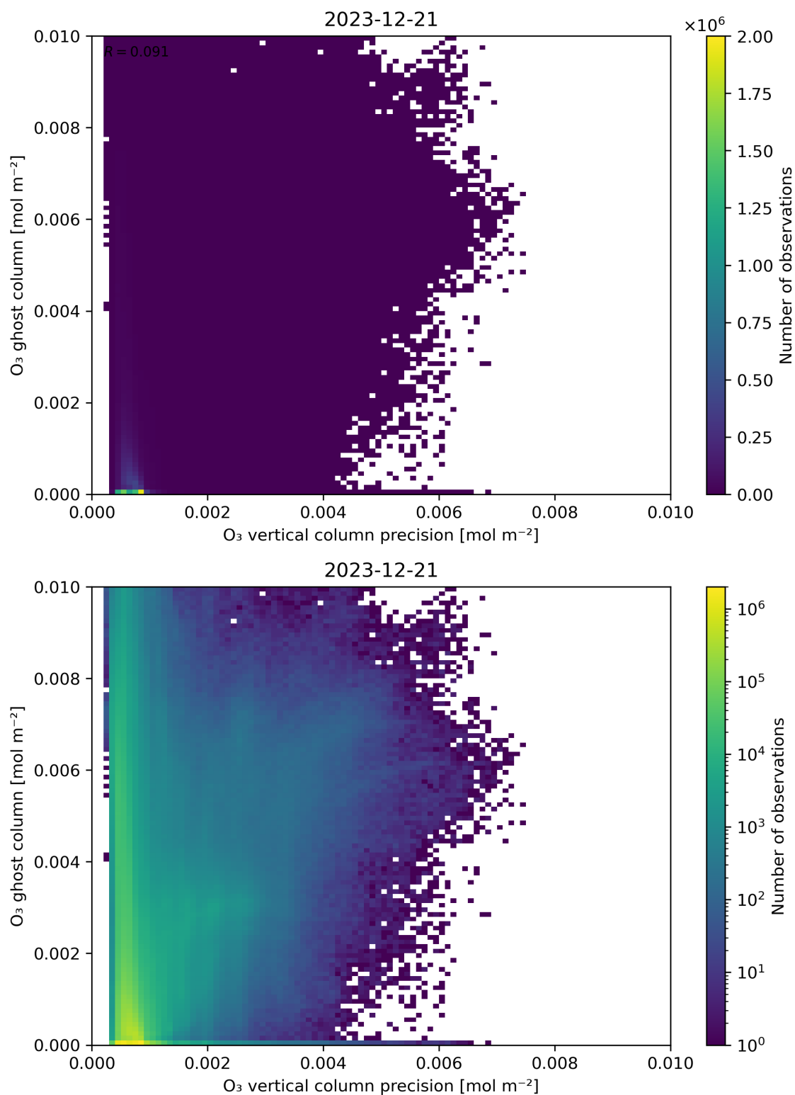
Figure 43: Scatter density plot of “ \text{O}_3 vertical column precision” against “ \text{O}_3 ghost column” for 2023-12-20 to 2023-12-22.
