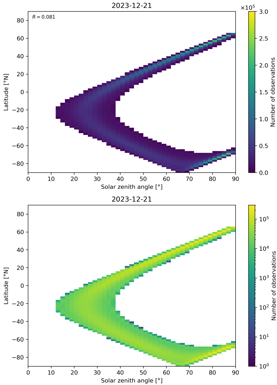
Figure 44: Scatter density plot of “Solar zenith angle” against “Latitude” for 2023-12-20 to 2023-12-22.
