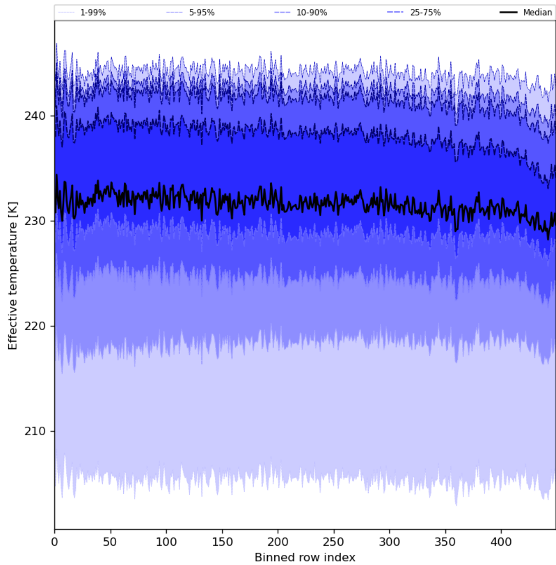
Figure 31: Along track statistics of “Effective temperature” for 2023-12-20 to 2023-12-22
