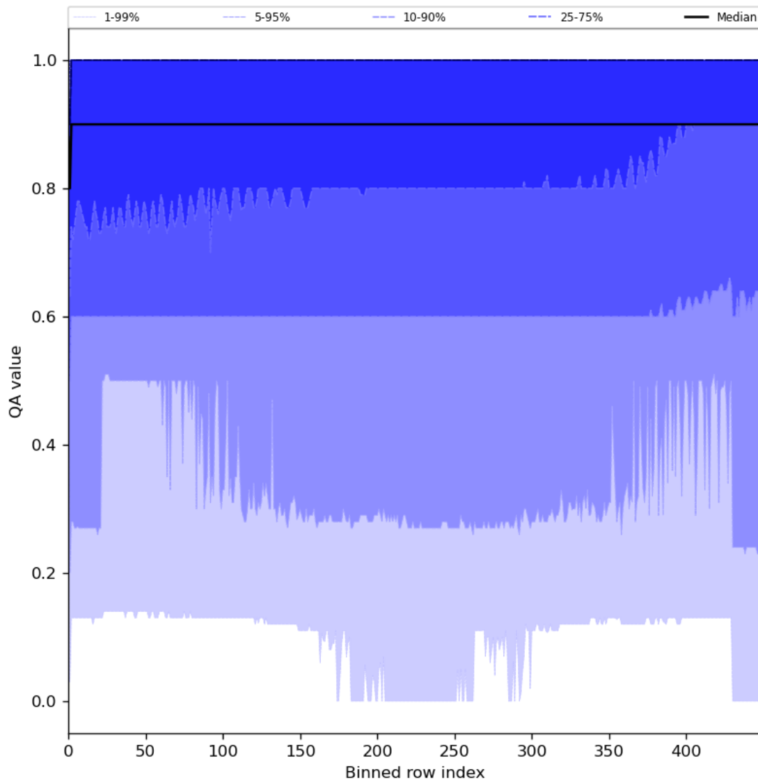
Figure 27: Along track statistics of “QA value” for 2023-12-20 to 2023-12-22
