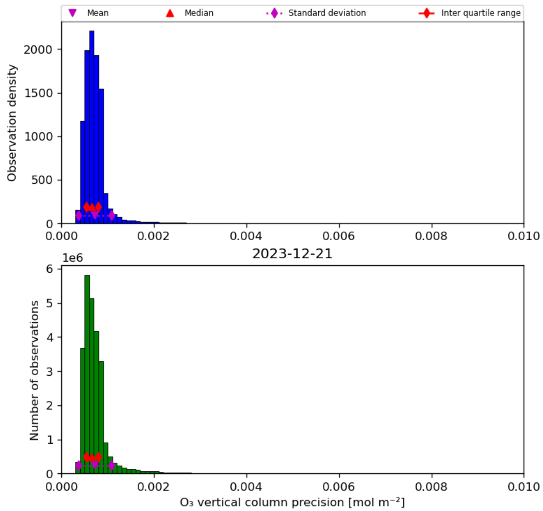
Figure 22: Histogram of “O 3 vertical column precision” for 2023-12-20 to 2023-12-22
