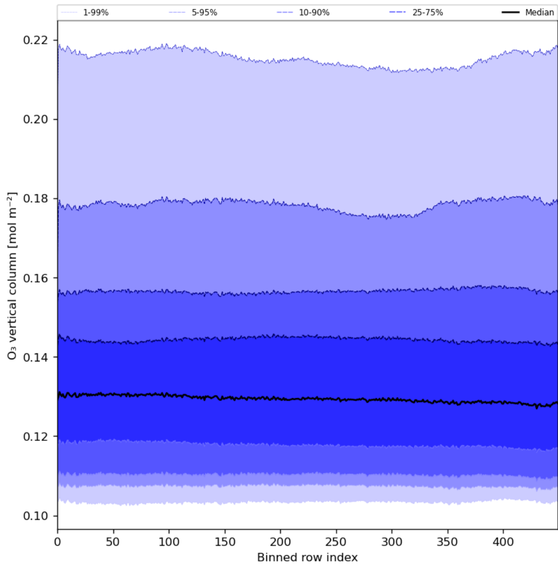
Figure 28: Along track statistics of “O 3 vertical column” for 2023-12-20 to 2023-12-22
