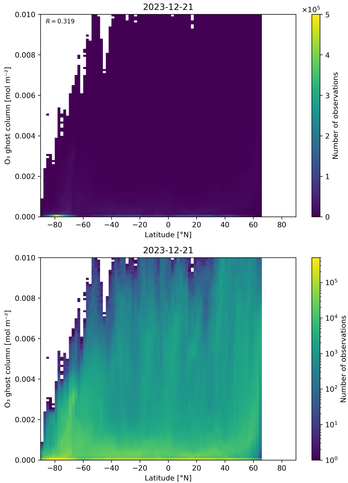
Figure 35: Scatter density plot of “Latitude” against “O 3 ghost column” for 2023-12-20 to 2023-12-22.
