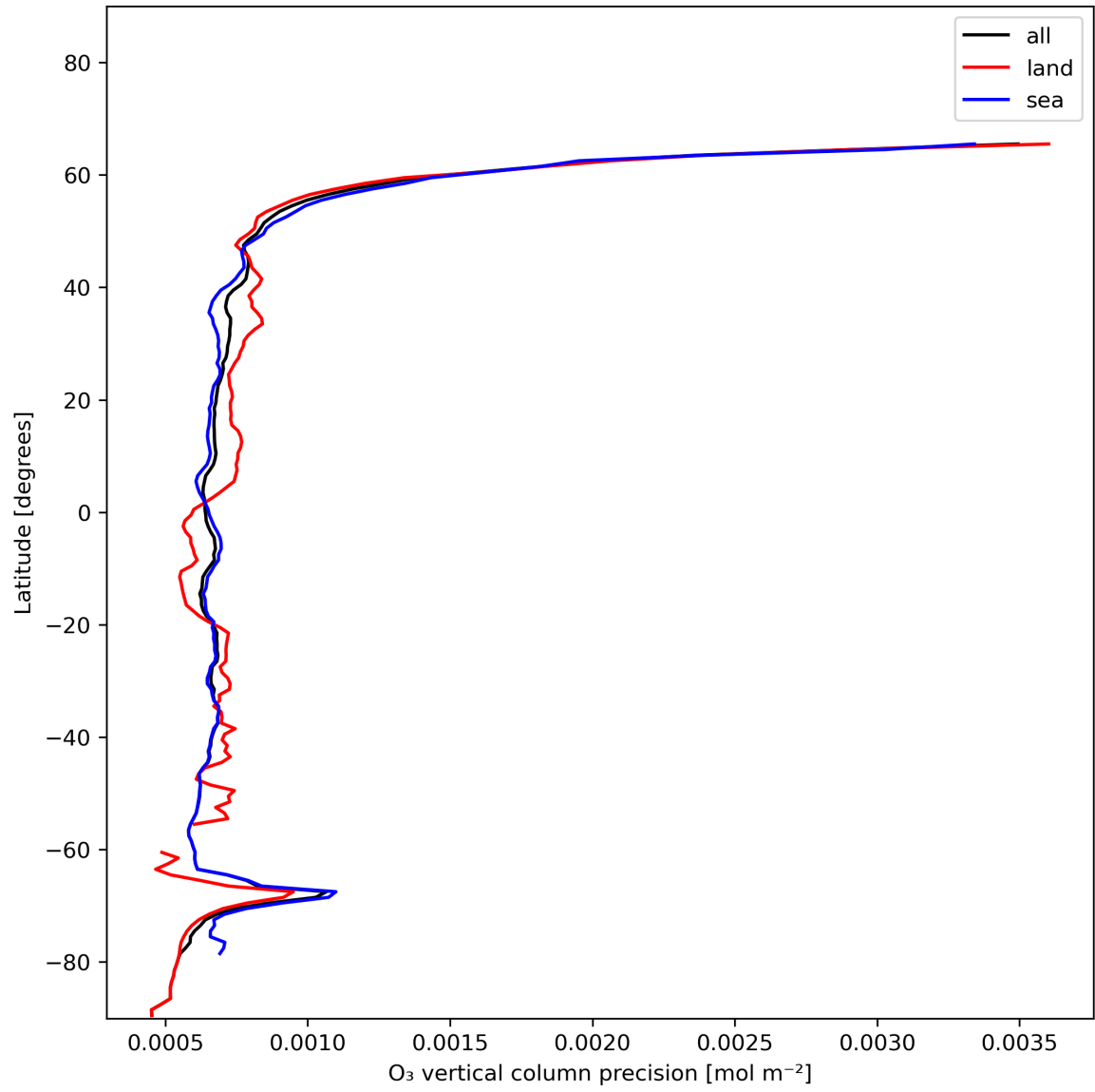
Figure 15: Zonal average of “O 3 vertical column precision” for 2023-12-20 to 2023-12-22.
