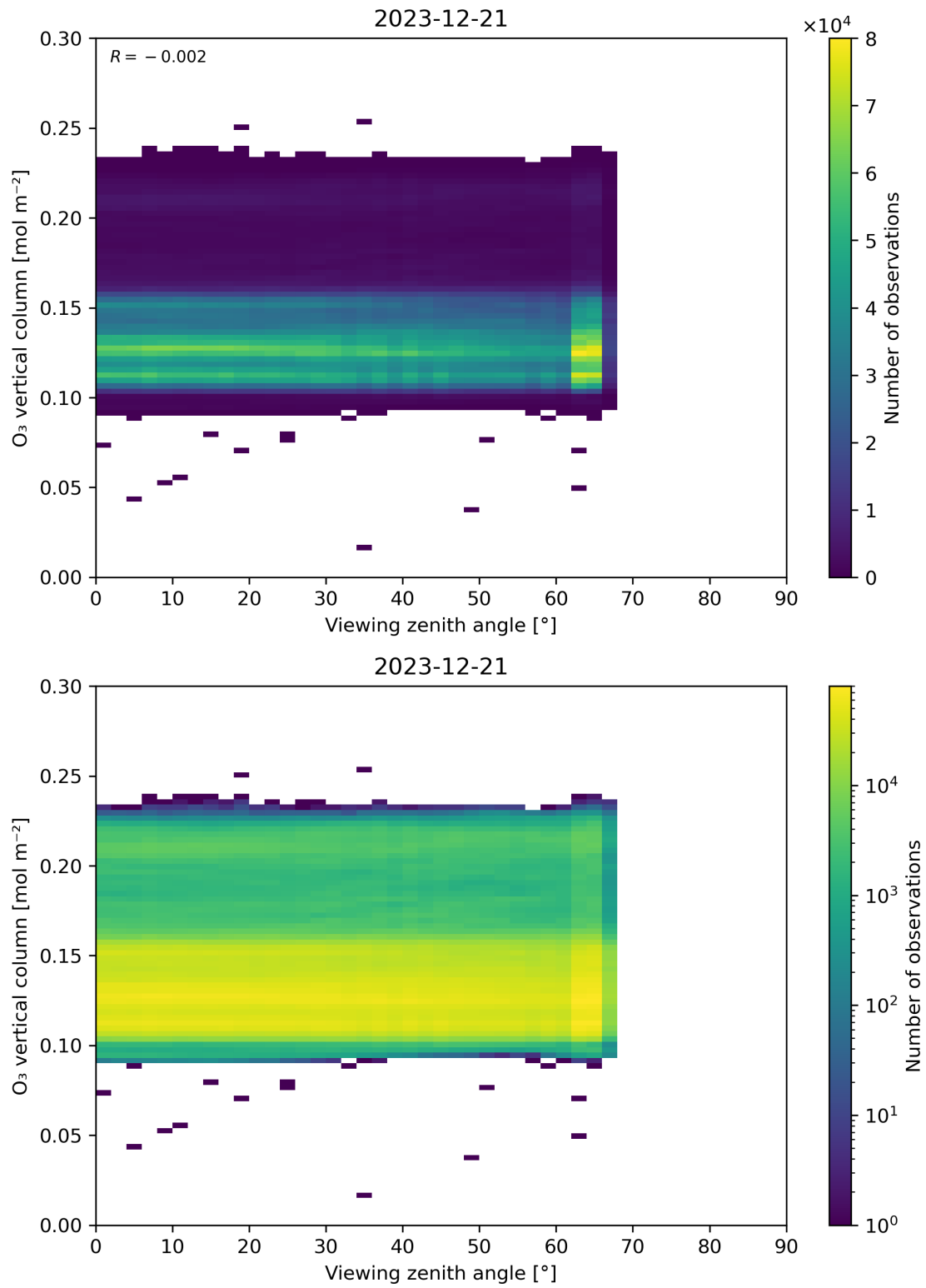
Figure 52: Scatter density plot of “Viewing zenith angle” against “O 3 vertical column” for 2023-12-20 to 2023-12-22.
