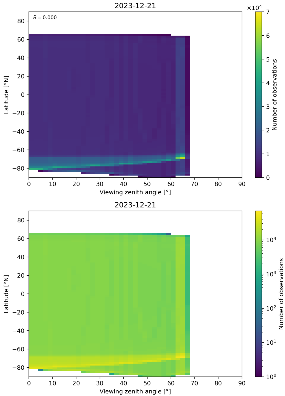
Figure 49: Scatter density plot of “Viewing zenith angle” against “Latitude” for 2023-12-20 to 2023-12-22.
