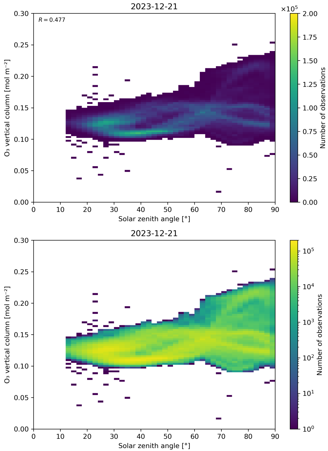
Figure 47: Scatter density plot of “Solar zenith angle” against “O 3 vertical column” for 2023-12-20 to 2023-12-22.
