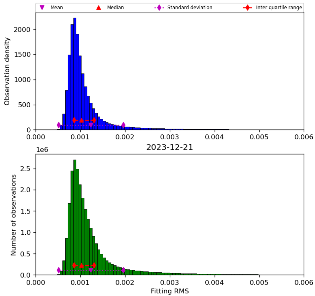
Figure 23: Histogram of “Fitting RMS” for 2023-12-20 to 2023-12-22
