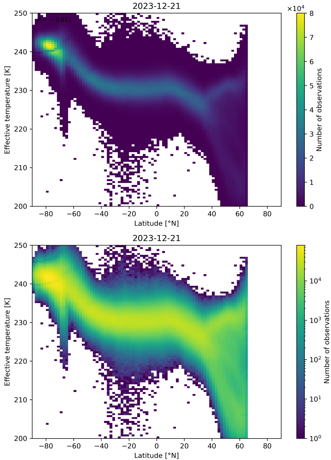
Figure 34: Scatter density plot of “Latitude” against “Effective temperature” for 2023-12-20 to 2023-12-22.
