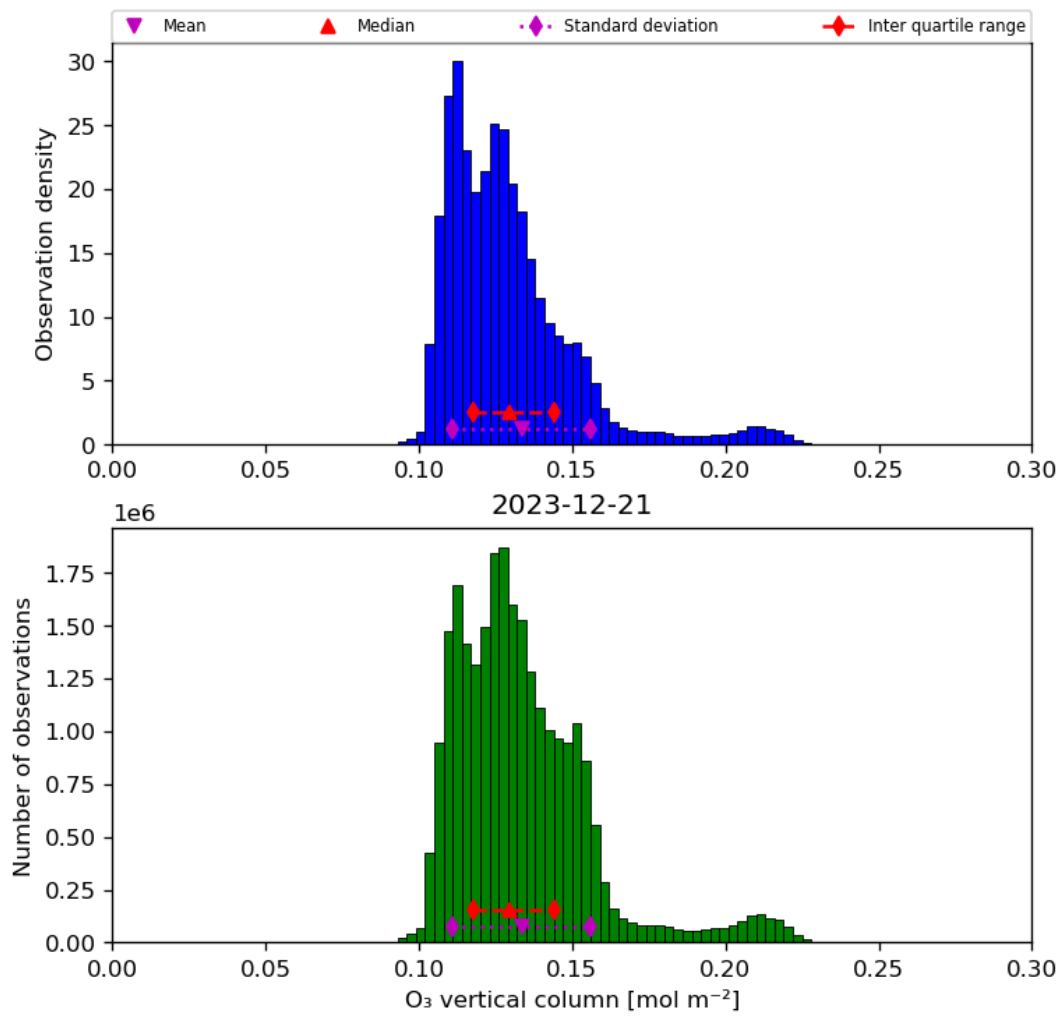
Figure 21: Histogram of “O 3 vertical column” for 2023-12-20 to 2023-12-22
