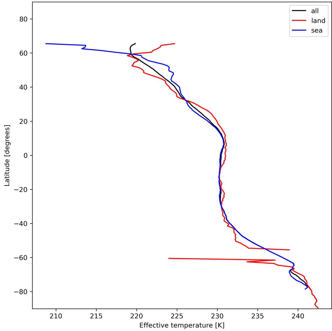
Figure 17: Zonal average of “Effective temperature” for 2023-12-20 to 2023-12-22.
