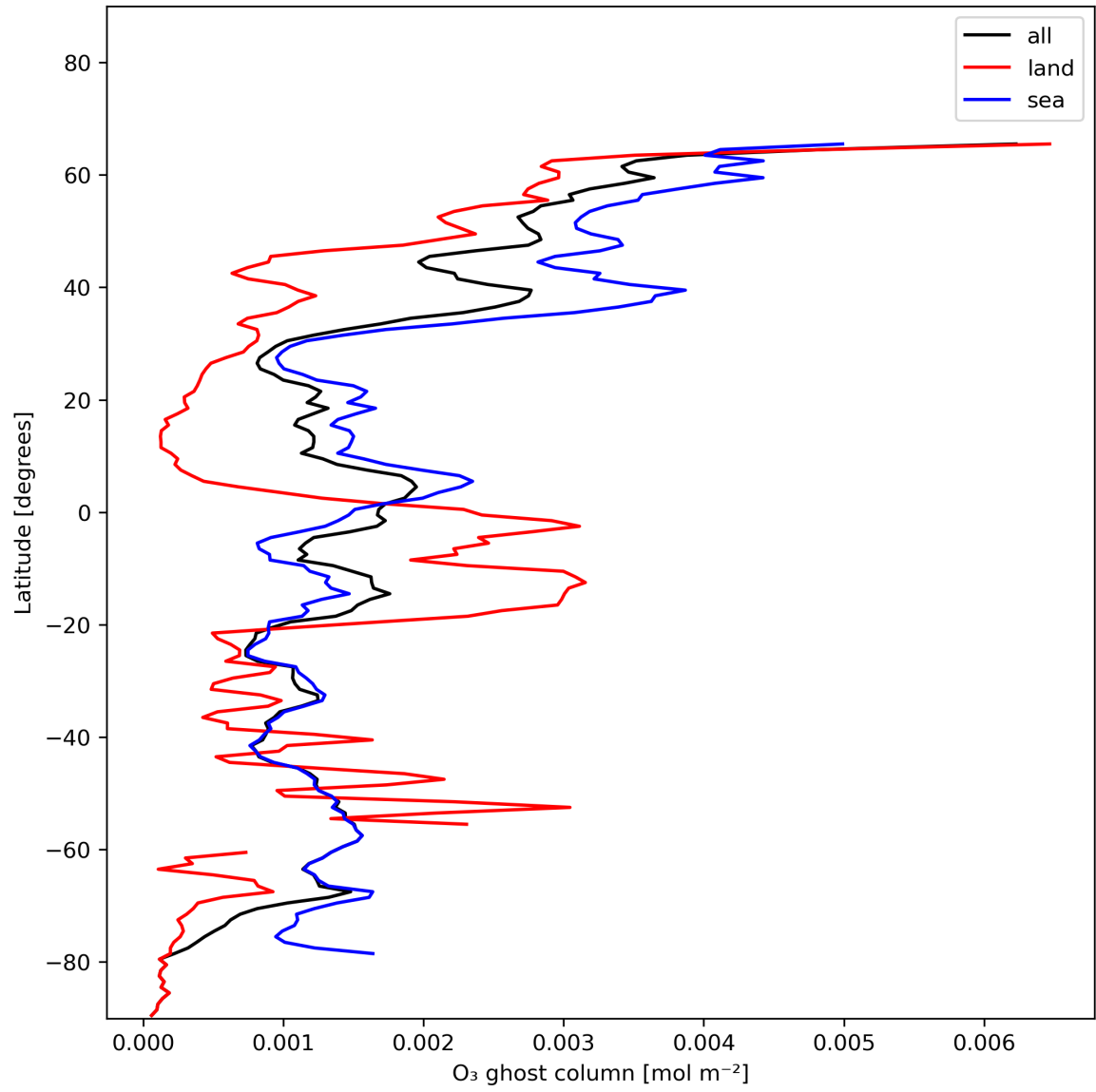
Figure 18: Zonal average of “O 3 ghost column” for 2023-12-20 to 2023-12-22.
