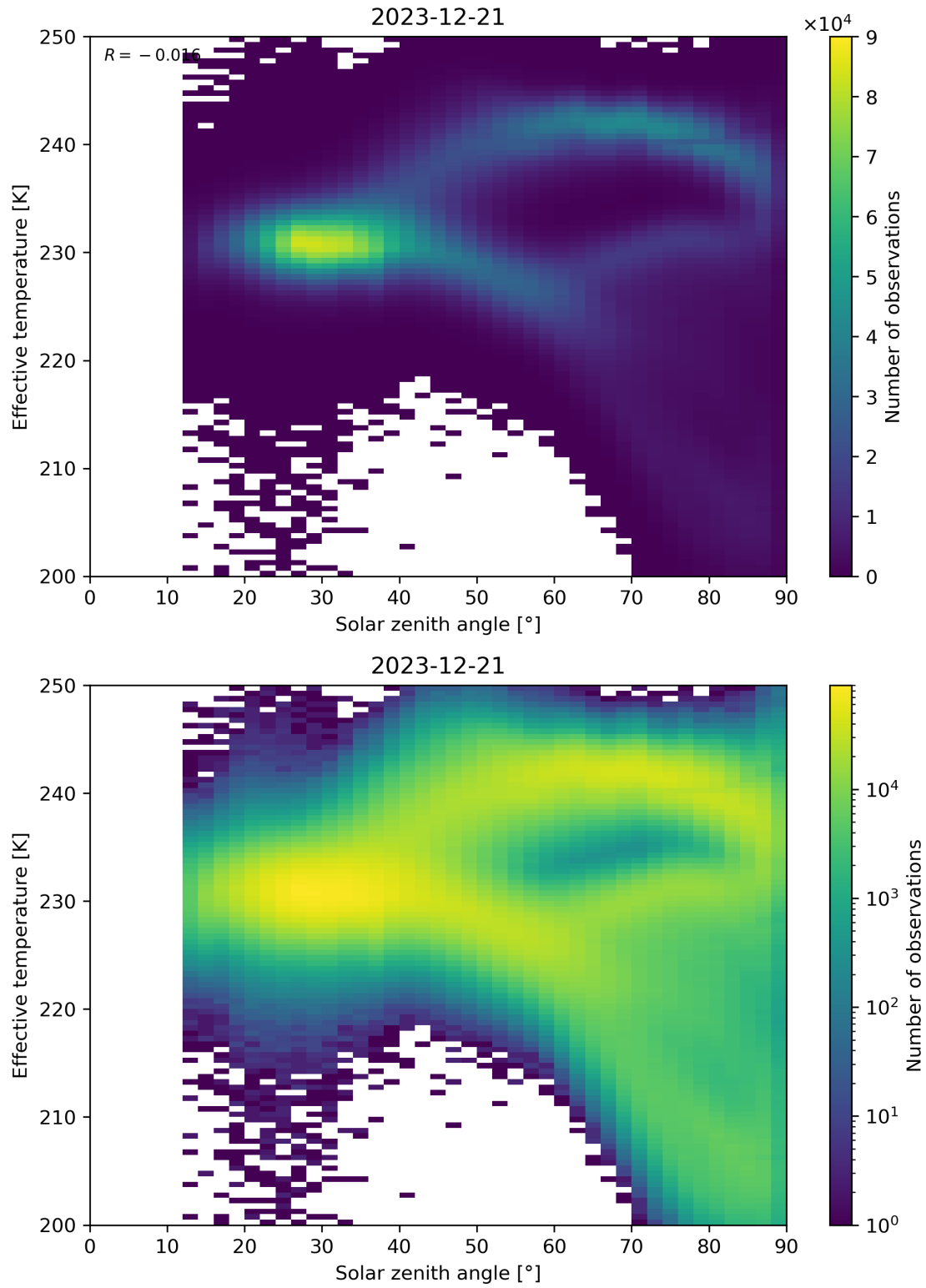
Figure 45: Scatter density plot of “Solar zenith angle” against “Effective temperature” for 2023-12-20 to 2023-12-22.
