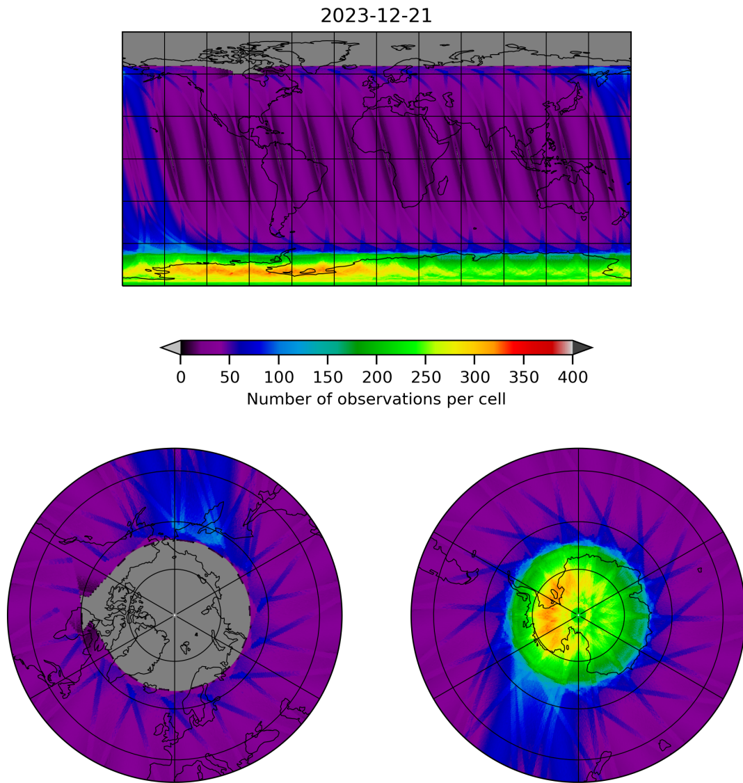
Figure 12: Map of the number of observations for 2023-12-20 to 2023-12-22
