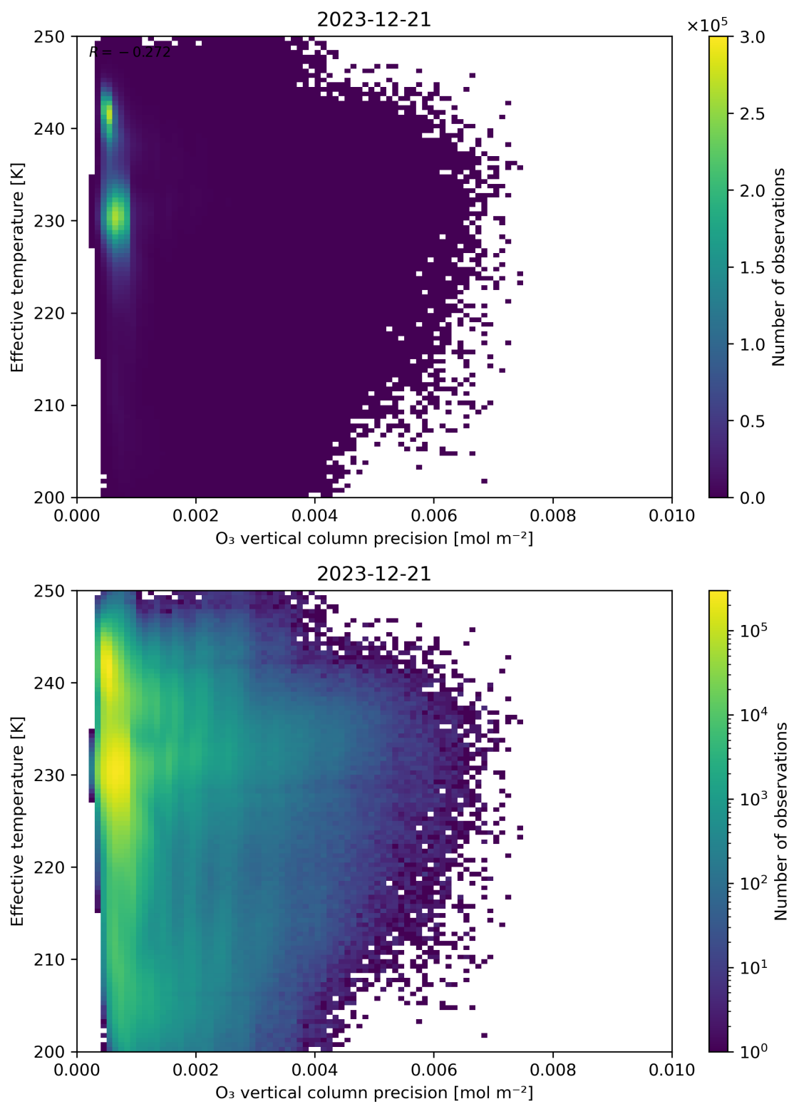
Figure 42: Scatter density plot of “O 3 vertical column precision” against “Effective temperature” for 2023-12-20 to 2023-12-22.
