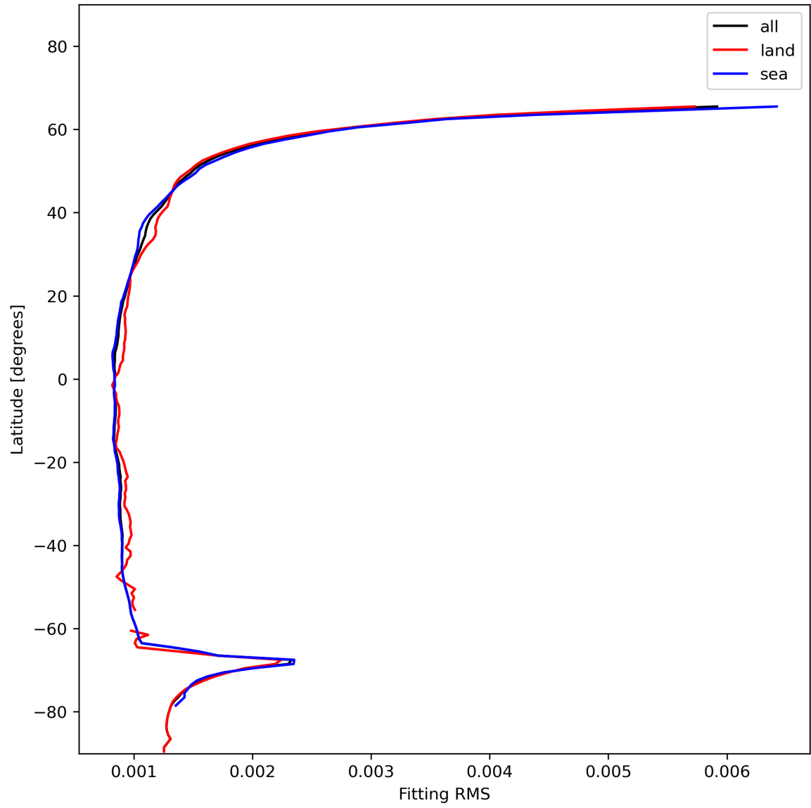
Figure 16: Zonal average of “Fitting RMS” for 2023-12-20 to 2023-12-22.
