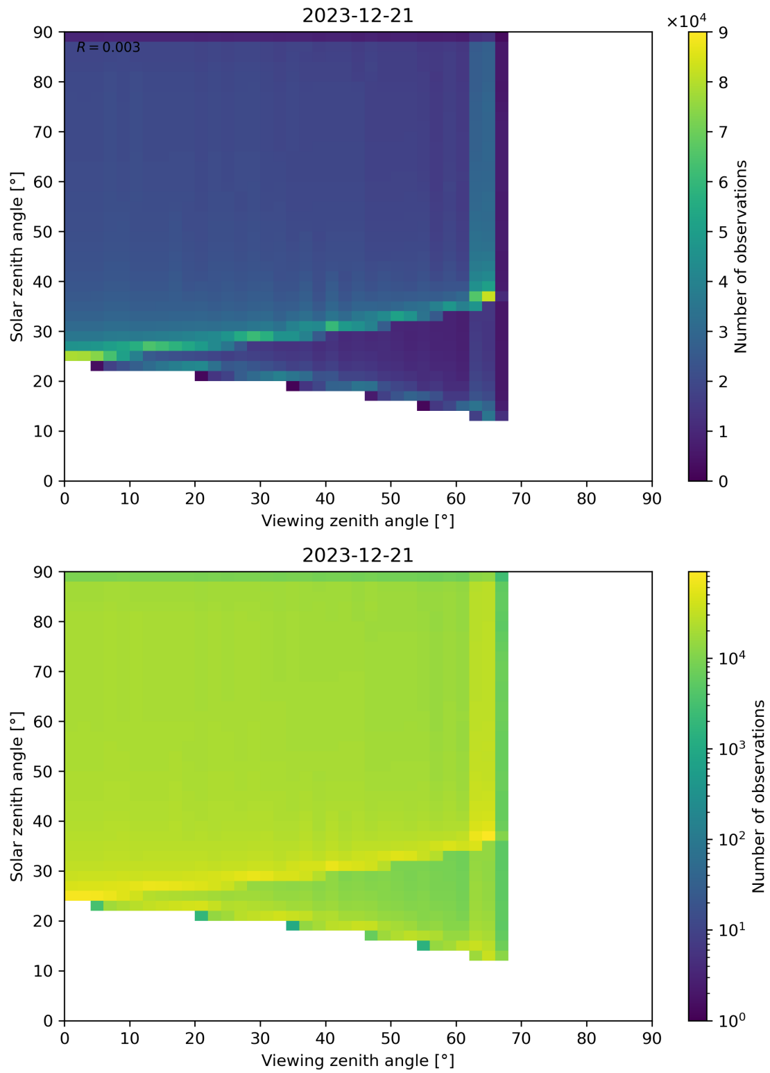
Figure 54: Scatter density plot of “Viewing zenith angle” against “Solar zenith angle” for 2023-12-20 to 2023-12-22.
