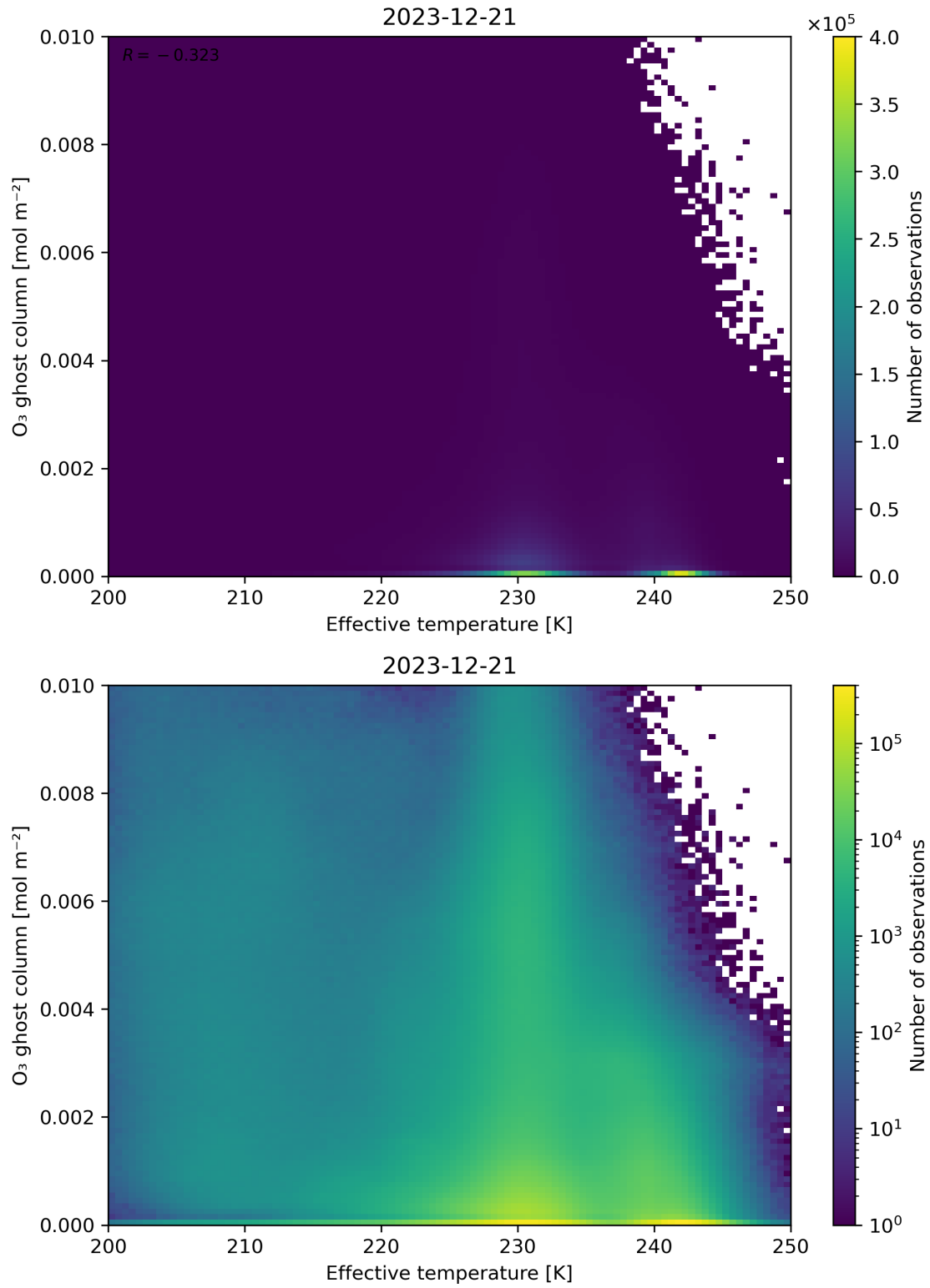
Figure 38: Scatter density plot of “Effective temperature” against “O 3 ghost column” for 2023-12-20 to 2023-12-22.
