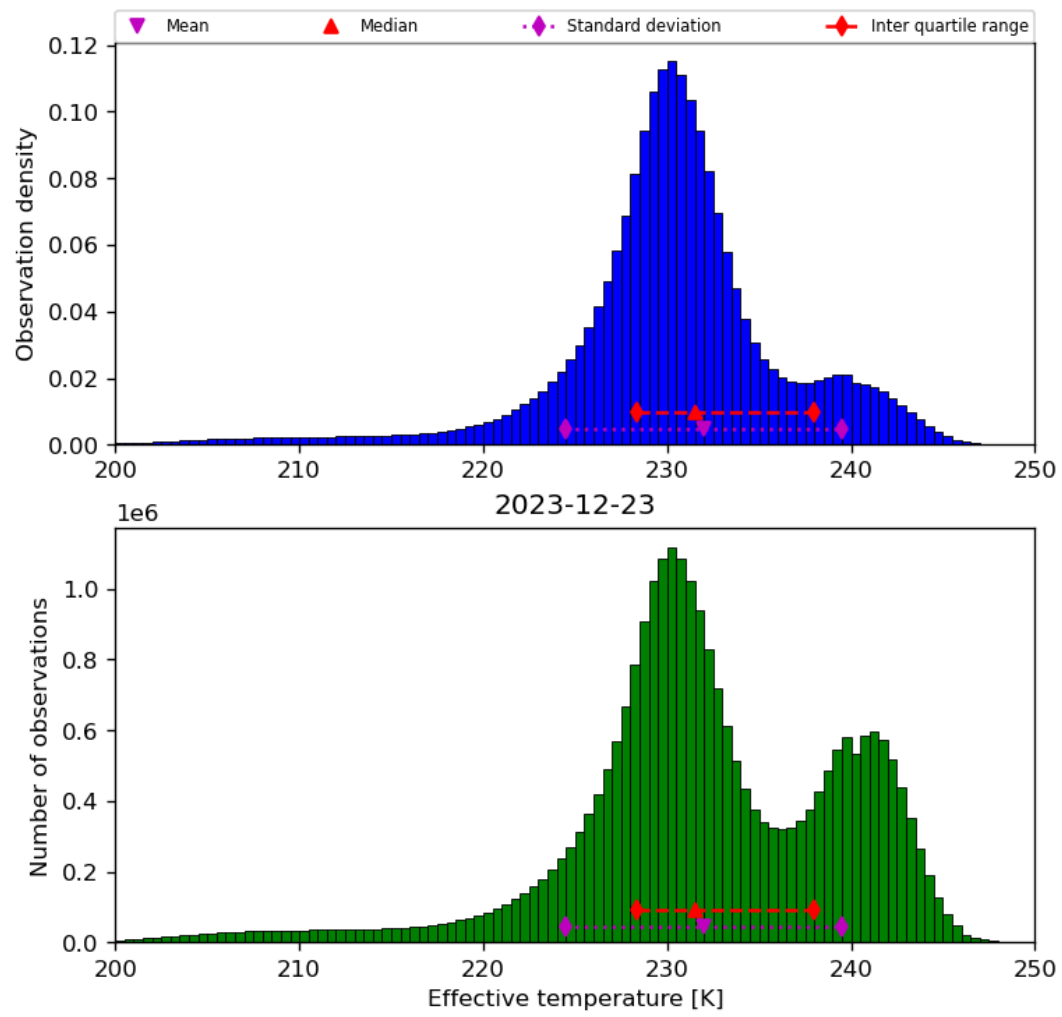
Figure 24: Histogram of “Effective temperature” for 2023-12-22 to 2023-12-24
