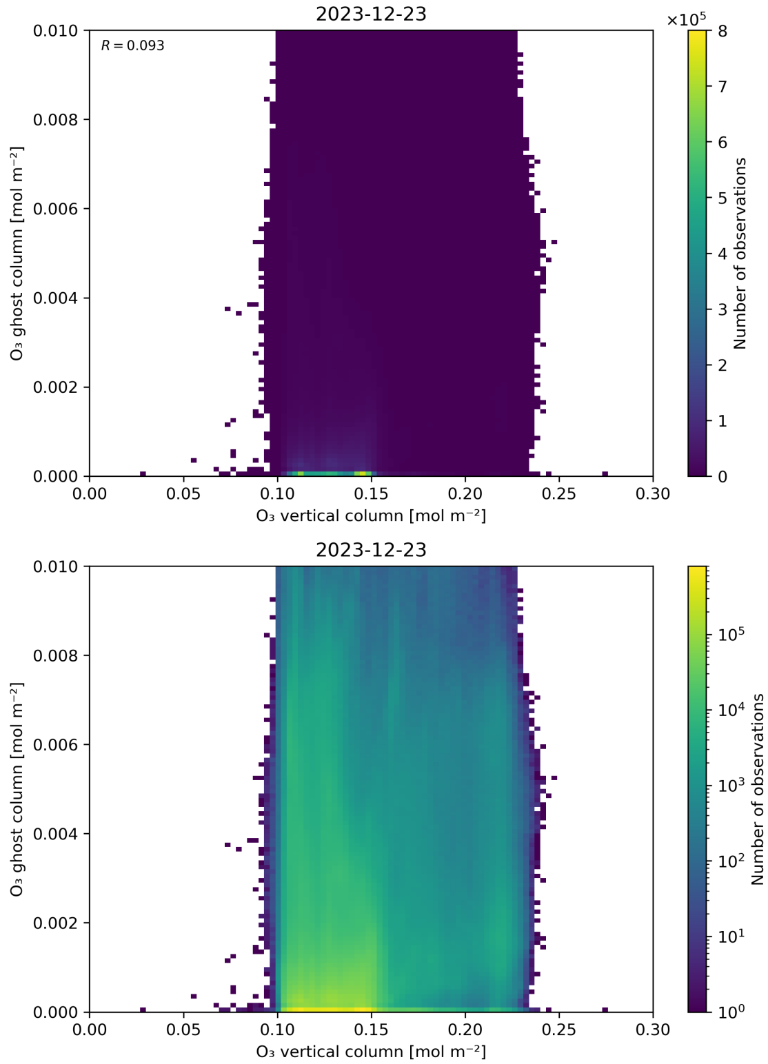
Figure 40: Scatter density plot of “O 3 vertical column” against “O 3 ghost column” for 2023-12-22 to 2023-12-24.
