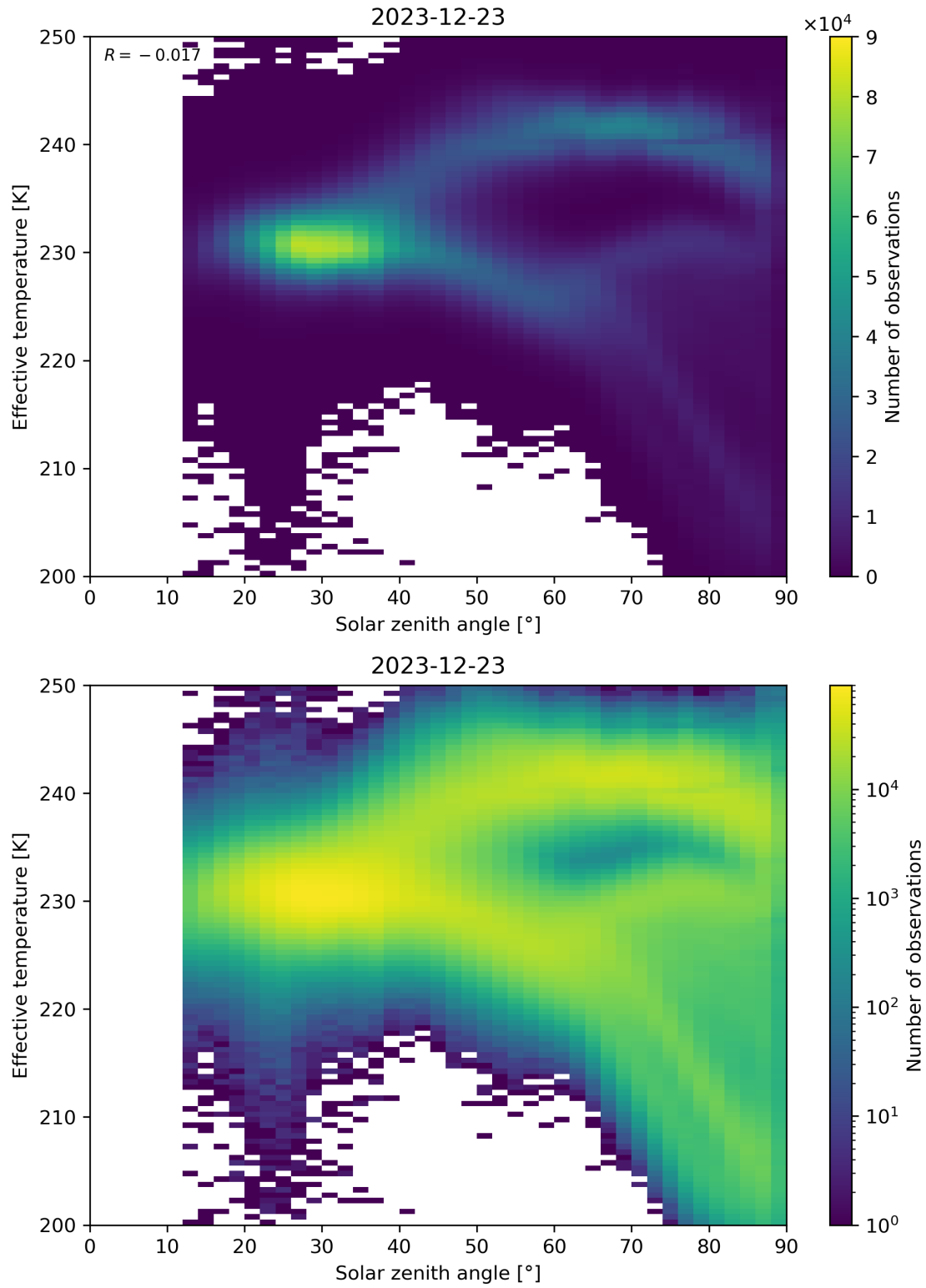
Figure 45: Scatter density plot of “Solar zenith angle” against “Effective temperature” for 2023-12-22 to 2023-12-24.
