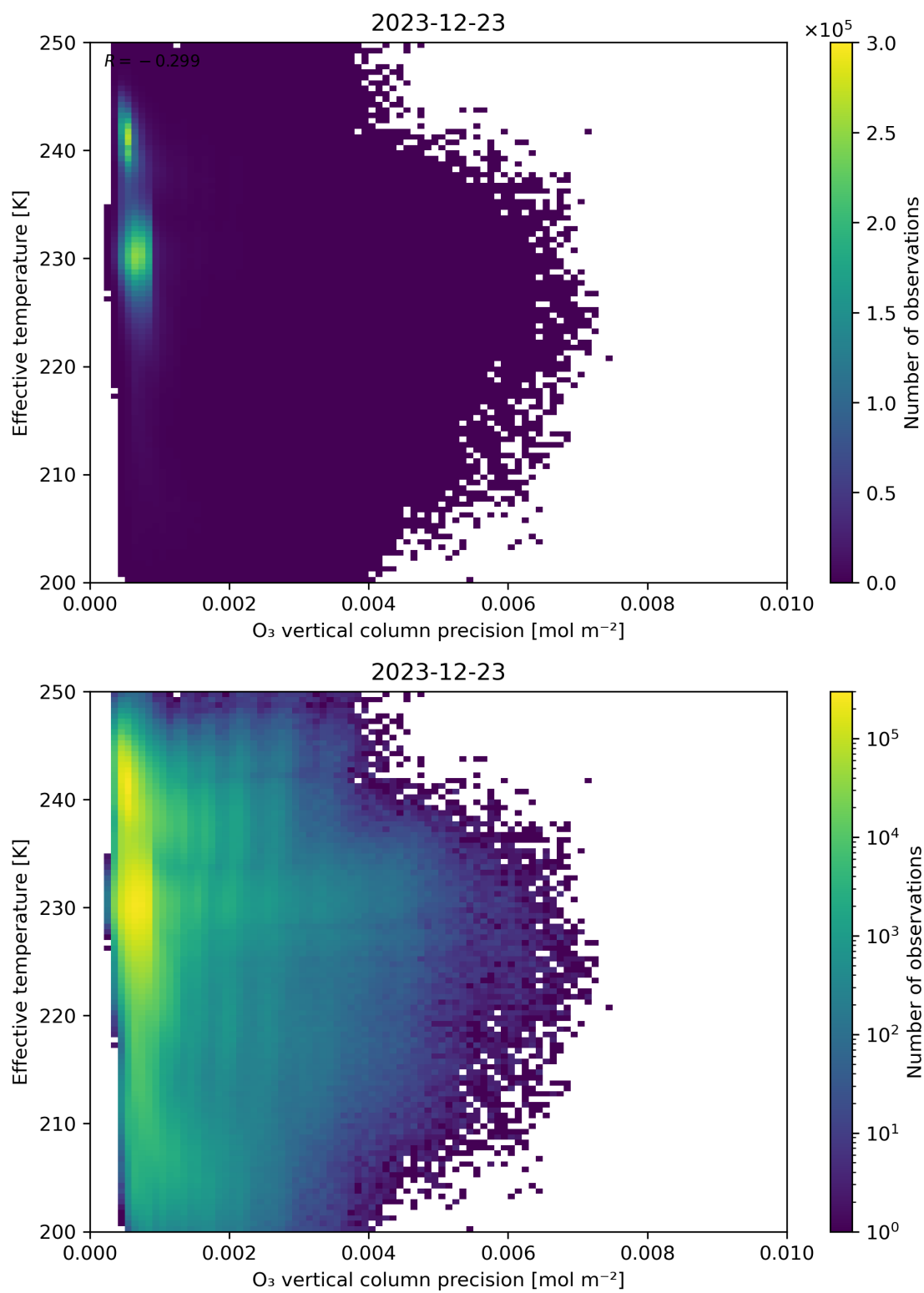
Figure 42: Scatter density plot of “O 3 vertical column precision” against “Effective temperature” for 2023-12-22 to 2023-12-24.
