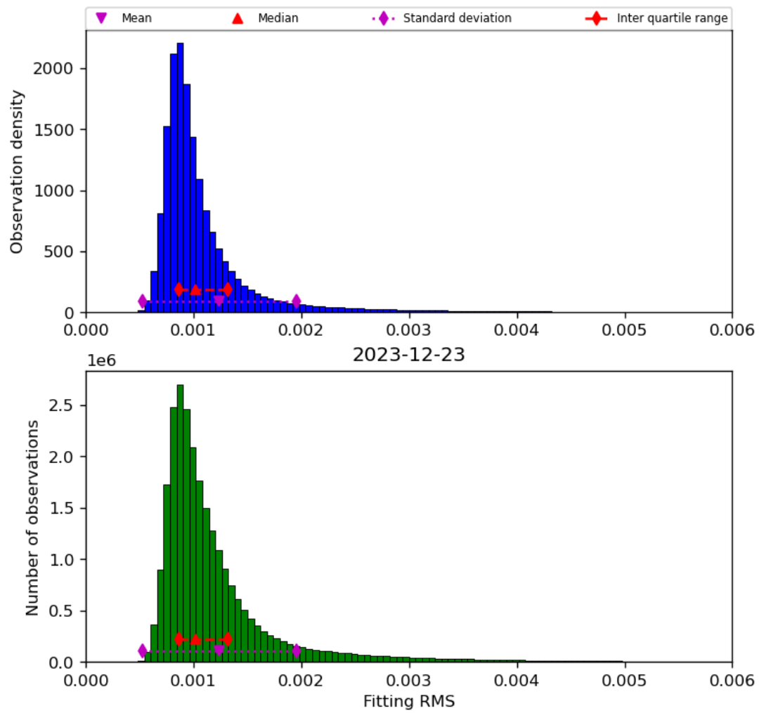
Figure 23: Histogram of “Fitting RMS” for 2023-12-22 to 2023-12-24
