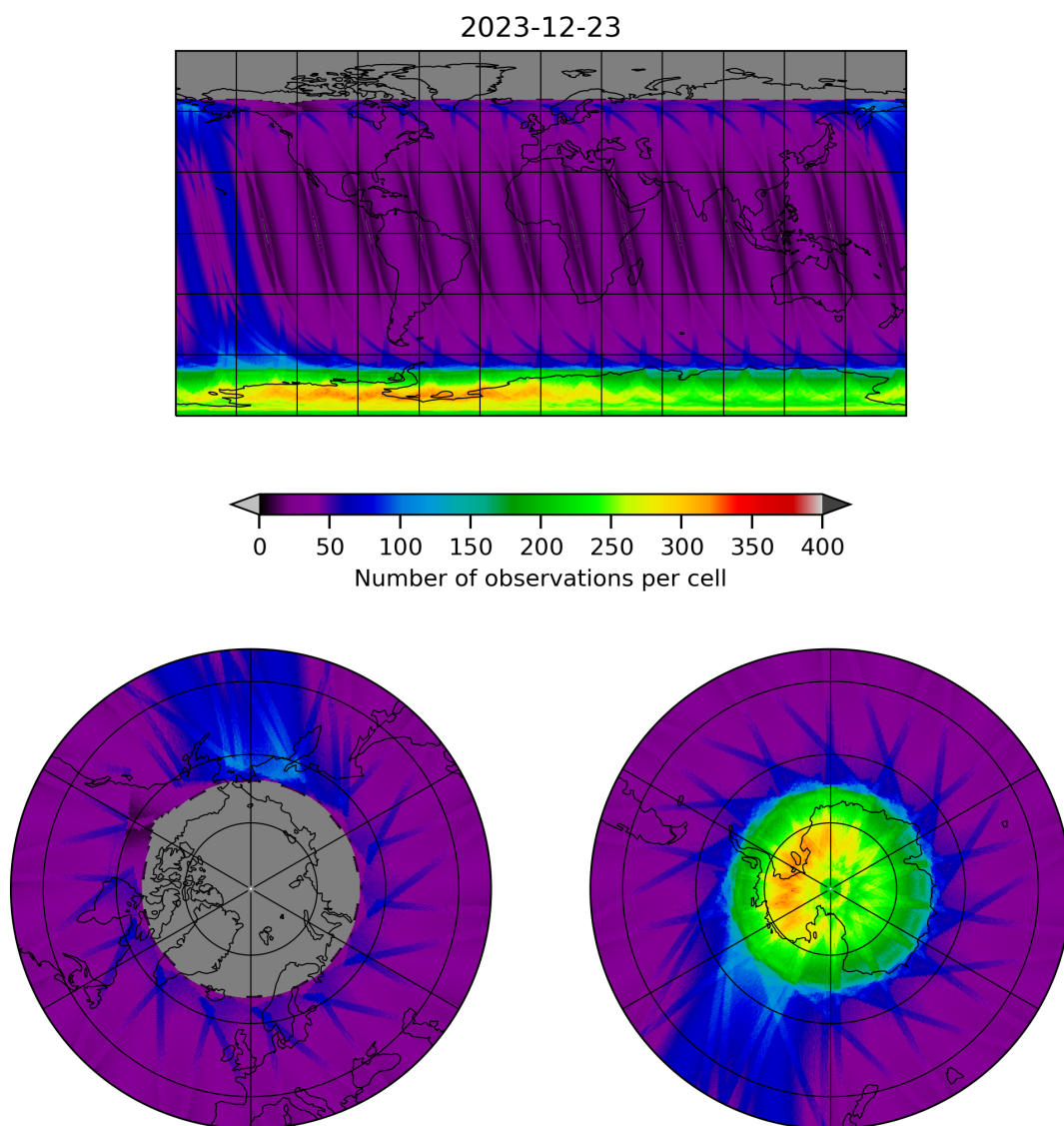
Figure 12: Map of the number of observations for 2023-12-22 to 2023-12-24
