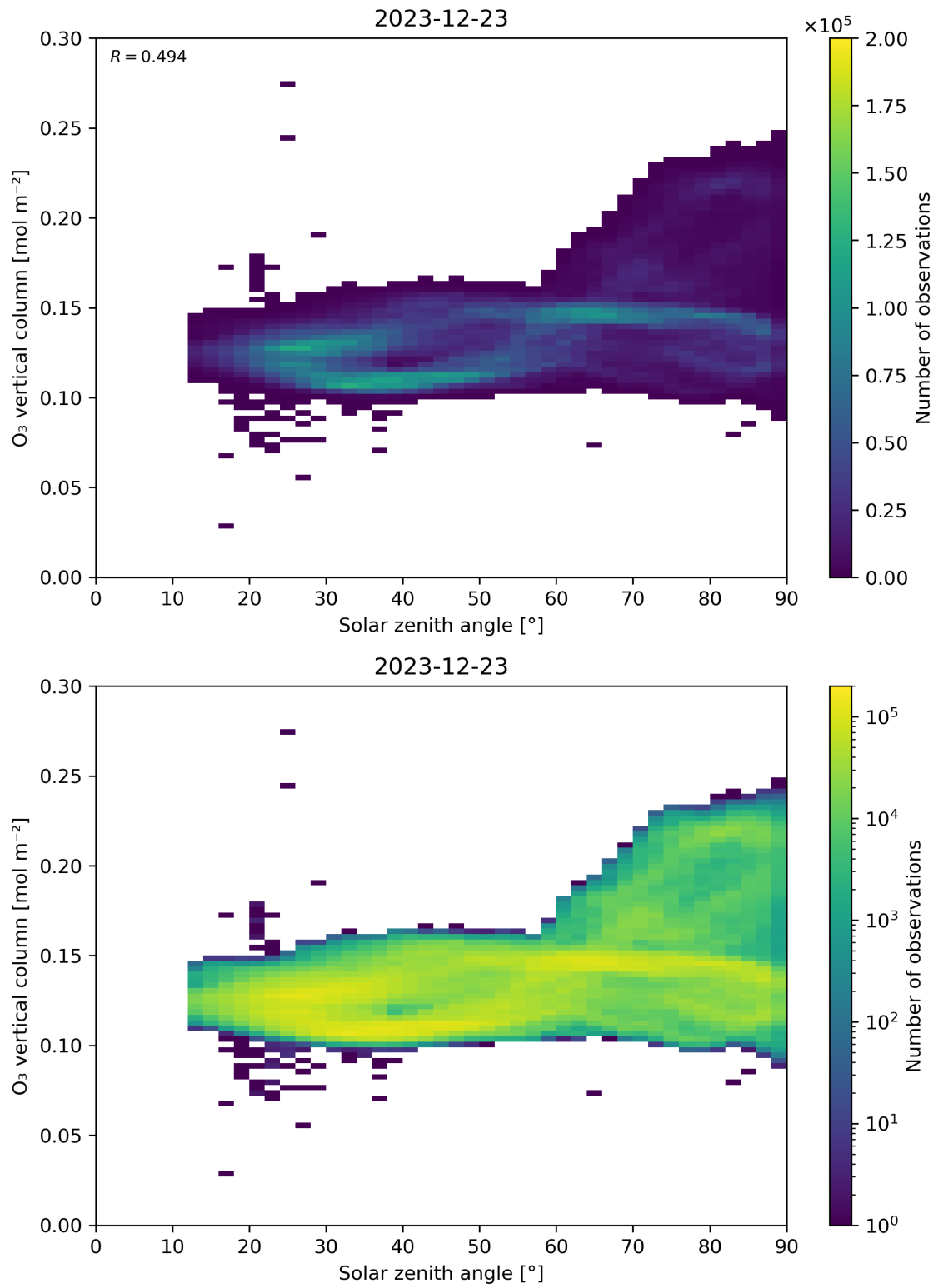
Figure 47: Scatter density plot of “Solar zenith angle” against “O 3 vertical column” for 2023-12-22 to 2023-12-24.
