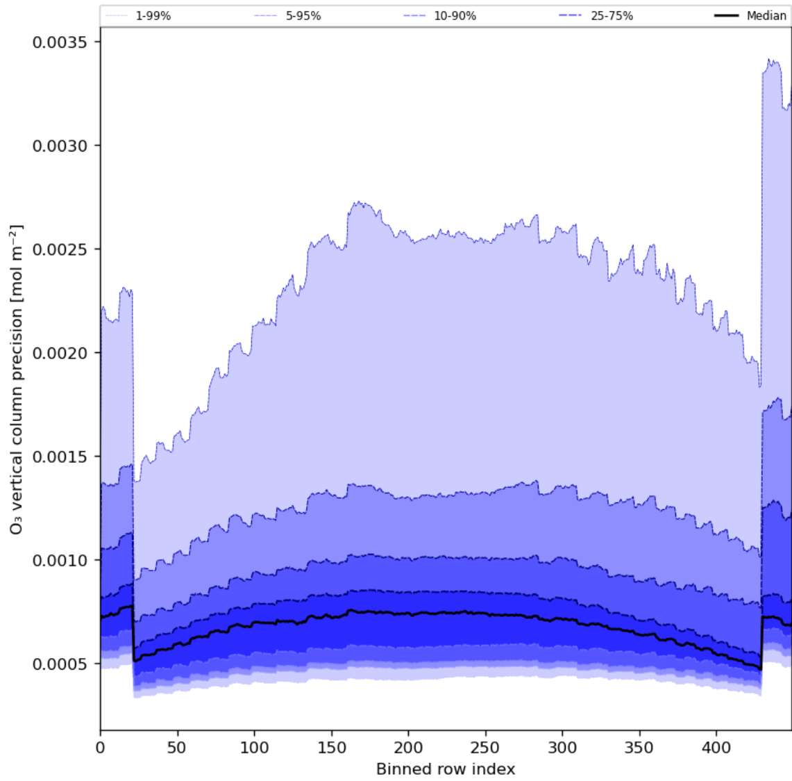
Figure 29: Along track statistics of “O 3 vertical column precision” for 2023-12-22 to 2023-12-24
