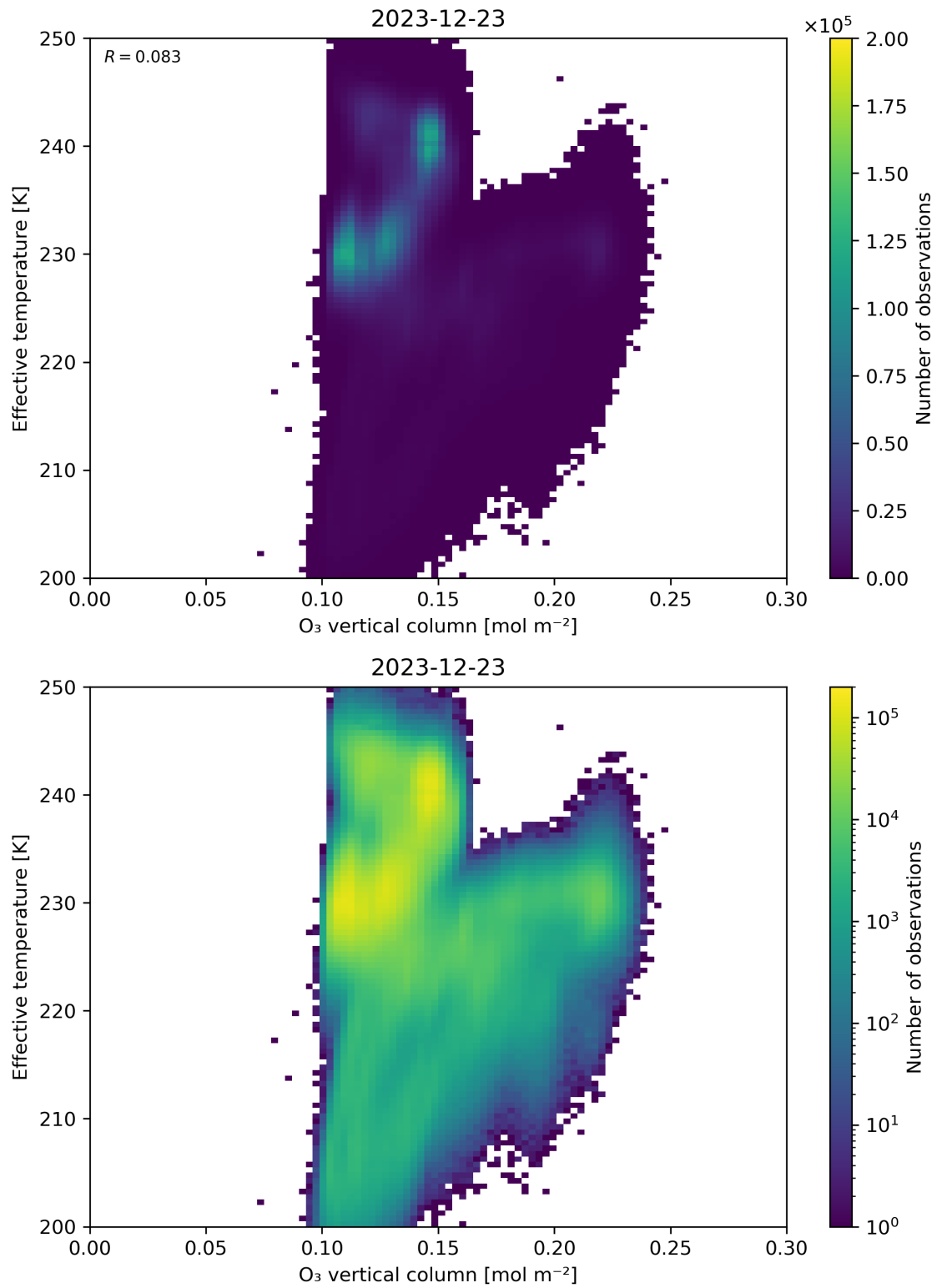
Figure 39: Scatter density plot of “O 3 vertical column” against “Effective temperature” for 2023-12-22 to 2023-12-24.
