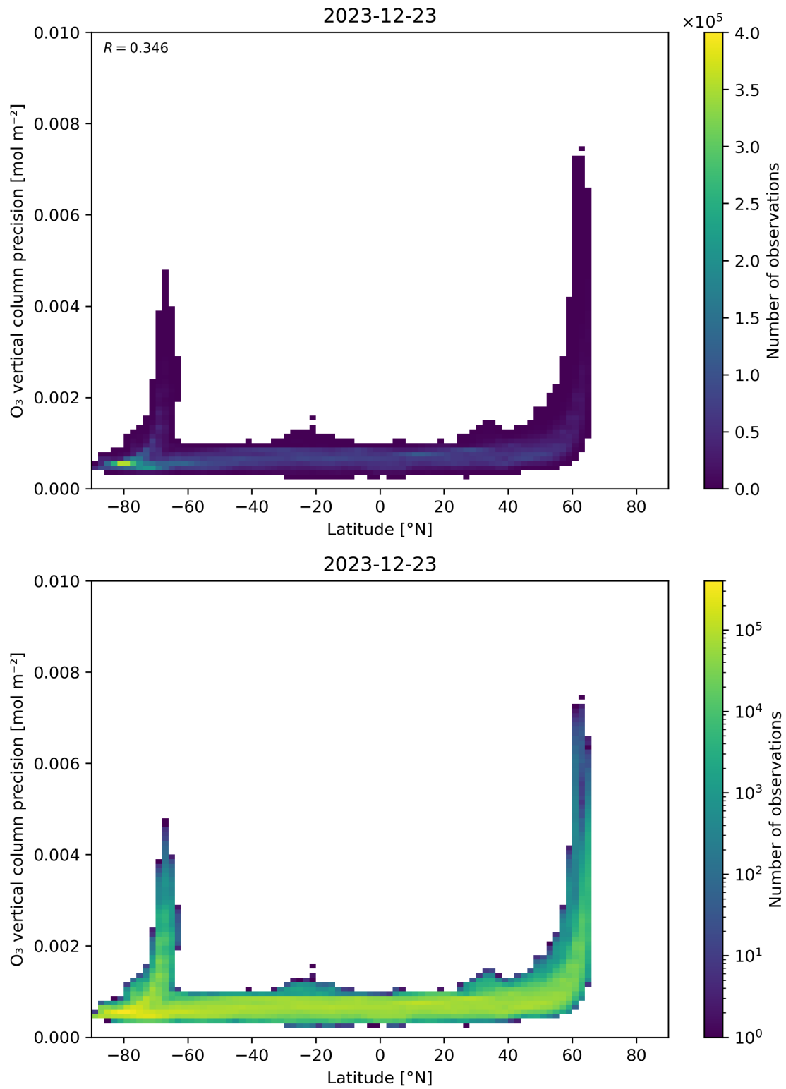
Figure 37: Scatter density plot of “Latitude” against “O 3 vertical column precision” for 2023-12-22 to 2023-12-24.
