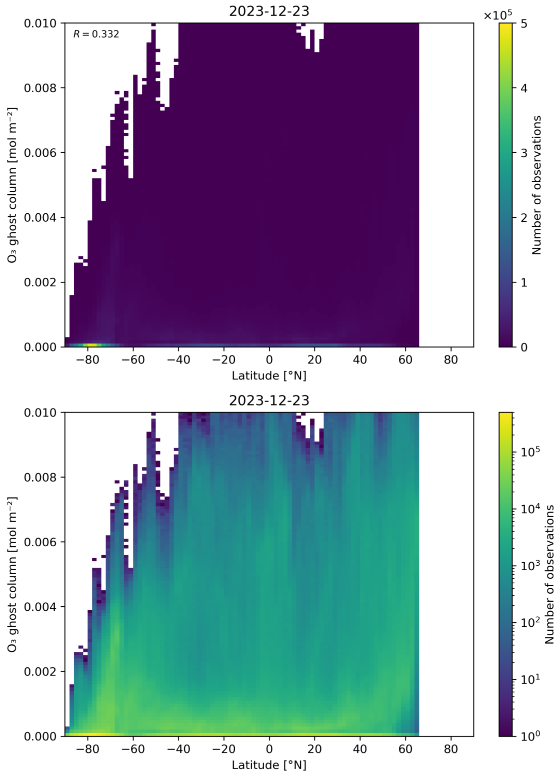
Figure 35: Scatter density plot of “Latitude” against “O 3 ghost column” for 2023-12-22 to 2023-12-24.
