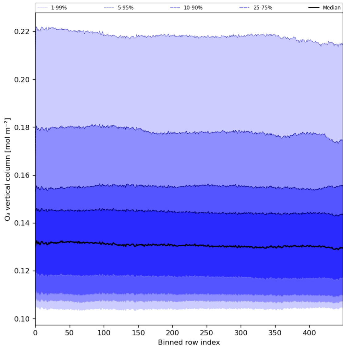
Figure 28: Along track statistics of “O 3 vertical column” for 2023-12-22 to 2023-12-24
