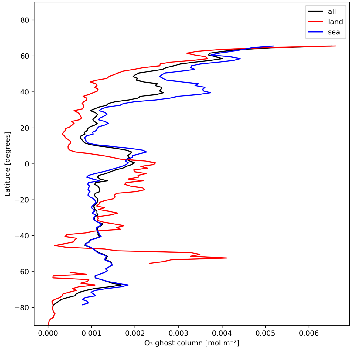
Figure 18: Zonal average of “O 3 ghost column” for 2023-12-22 to 2023-12-24.
