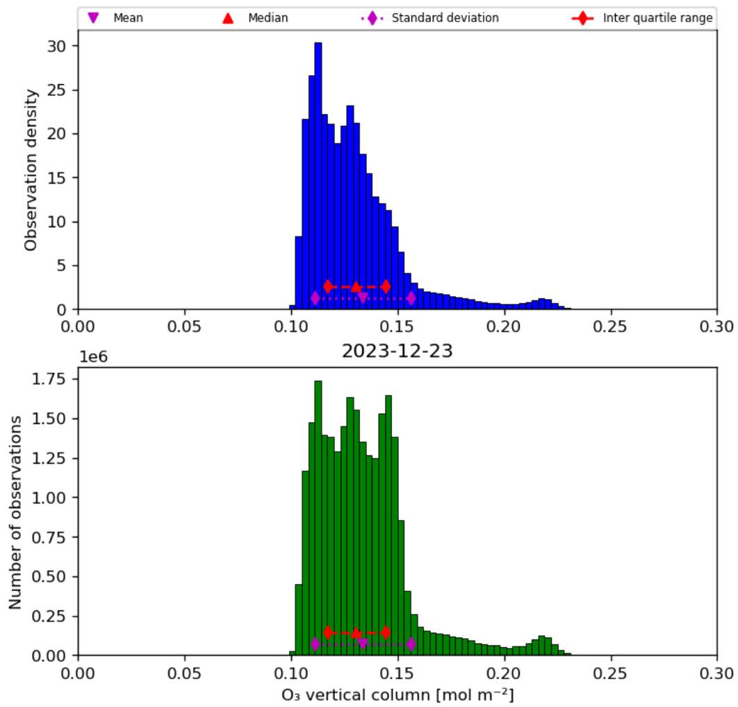
Figure 21: Histogram of “O 3 vertical column” for 2023-12-22 to 2023-12-24
