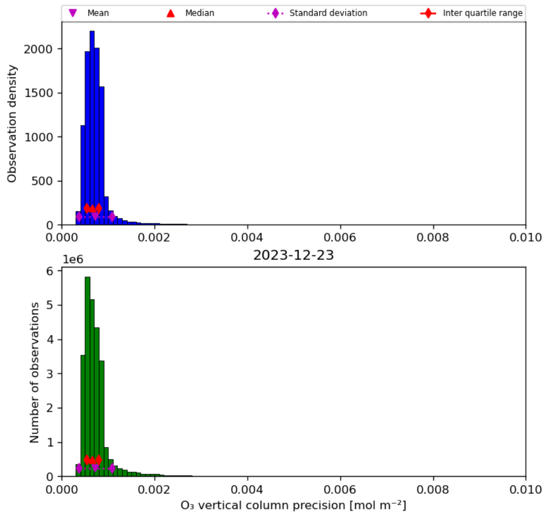
Figure 22: Histogram of “O 3 vertical column precision” for 2023-12-22 to 2023-12-24
