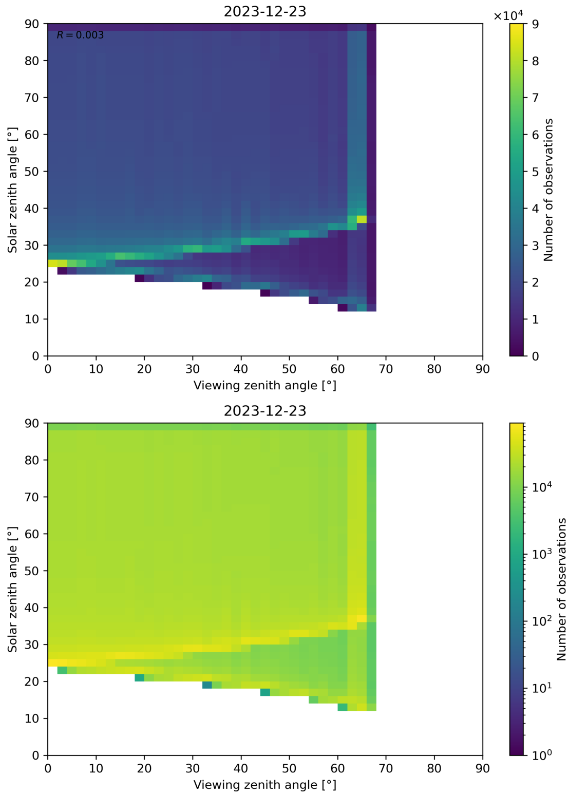
Figure 54: Scatter density plot of “Viewing zenith angle” against “Solar zenith angle” for 2023-12-22 to 2023-12-24.
