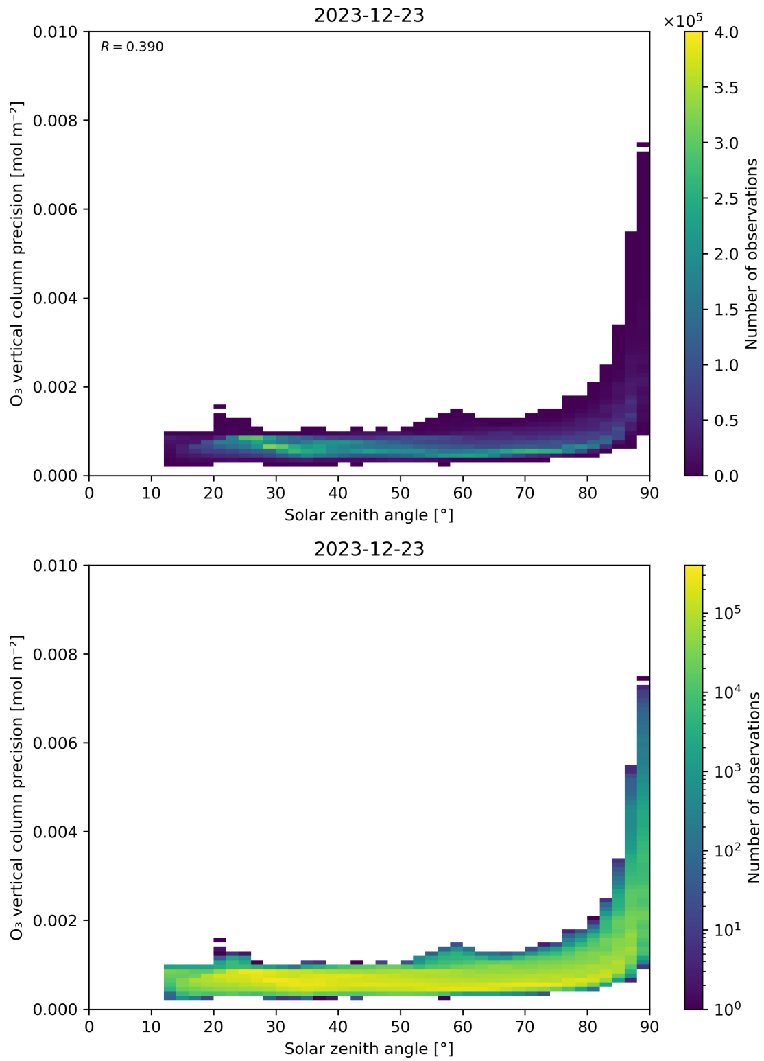
Figure 48: Scatter density plot of “Solar zenith angle” against “O 3 vertical column precision” for 2023-12-22 to 2023-12-24.
