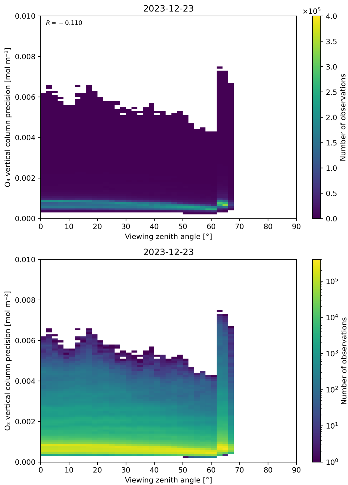
Figure 53: Scatter density plot of “Viewing zenith angle” against “O 3 vertical column precision” for 2023-12-22 to 2023-12-24.
