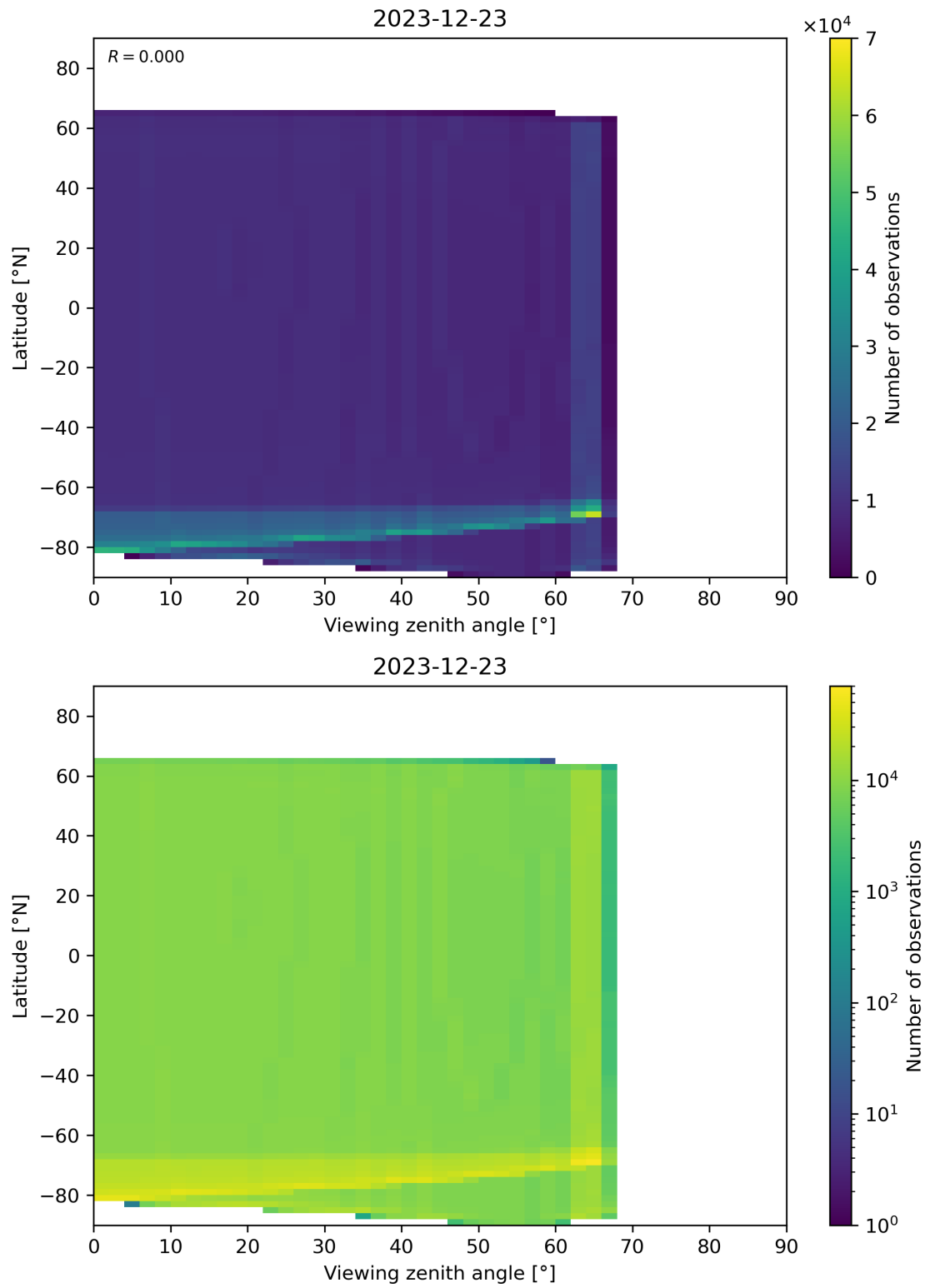
Figure 49: Scatter density plot of “Viewing zenith angle” against “Latitude” for 2023-12-22 to 2023-12-24.
