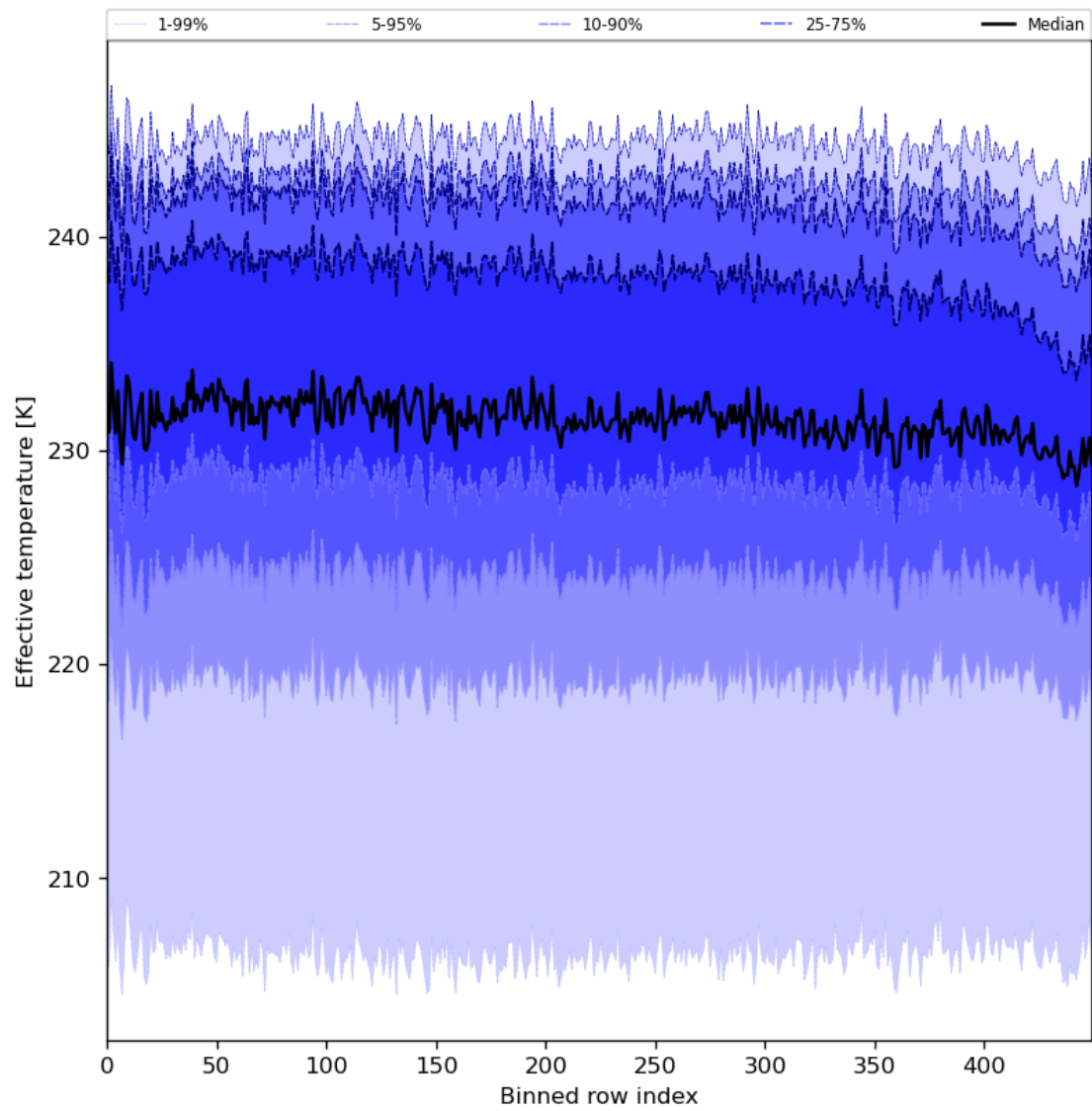
Figure 31: Along track statistics of “Effective temperature” for 2023-12-22 to 2023-12-24
