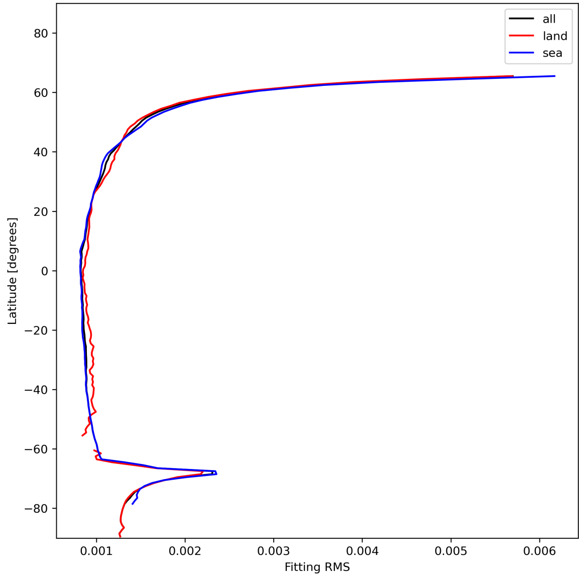
Figure 16: Zonal average of “Fitting RMS” for 2023-12-22 to 2023-12-24.
