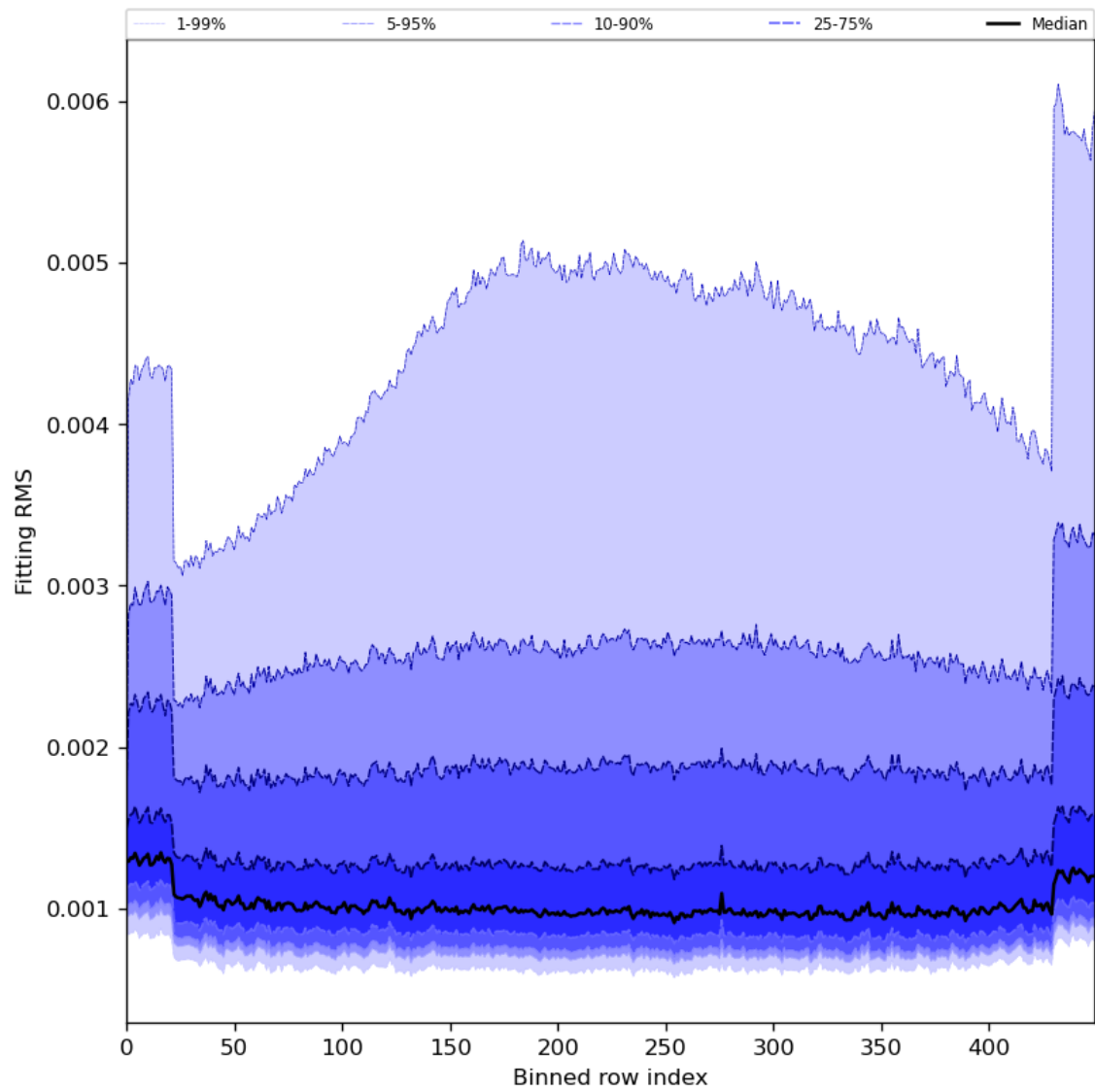
Figure 30: Along track statistics of “Fitting RMS” for 2023-12-22 to 2023-12-24
