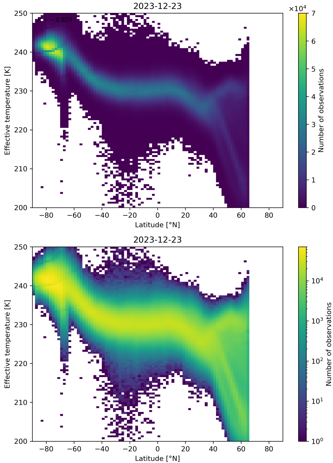
Figure 34: Scatter density plot of “Latitude” against “Effective temperature” for 2023-12-22 to 2023-12-24.
