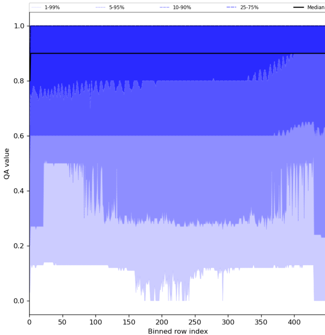
Figure 27: Along track statistics of “QA value” for 2023-12-22 to 2023-12-24
