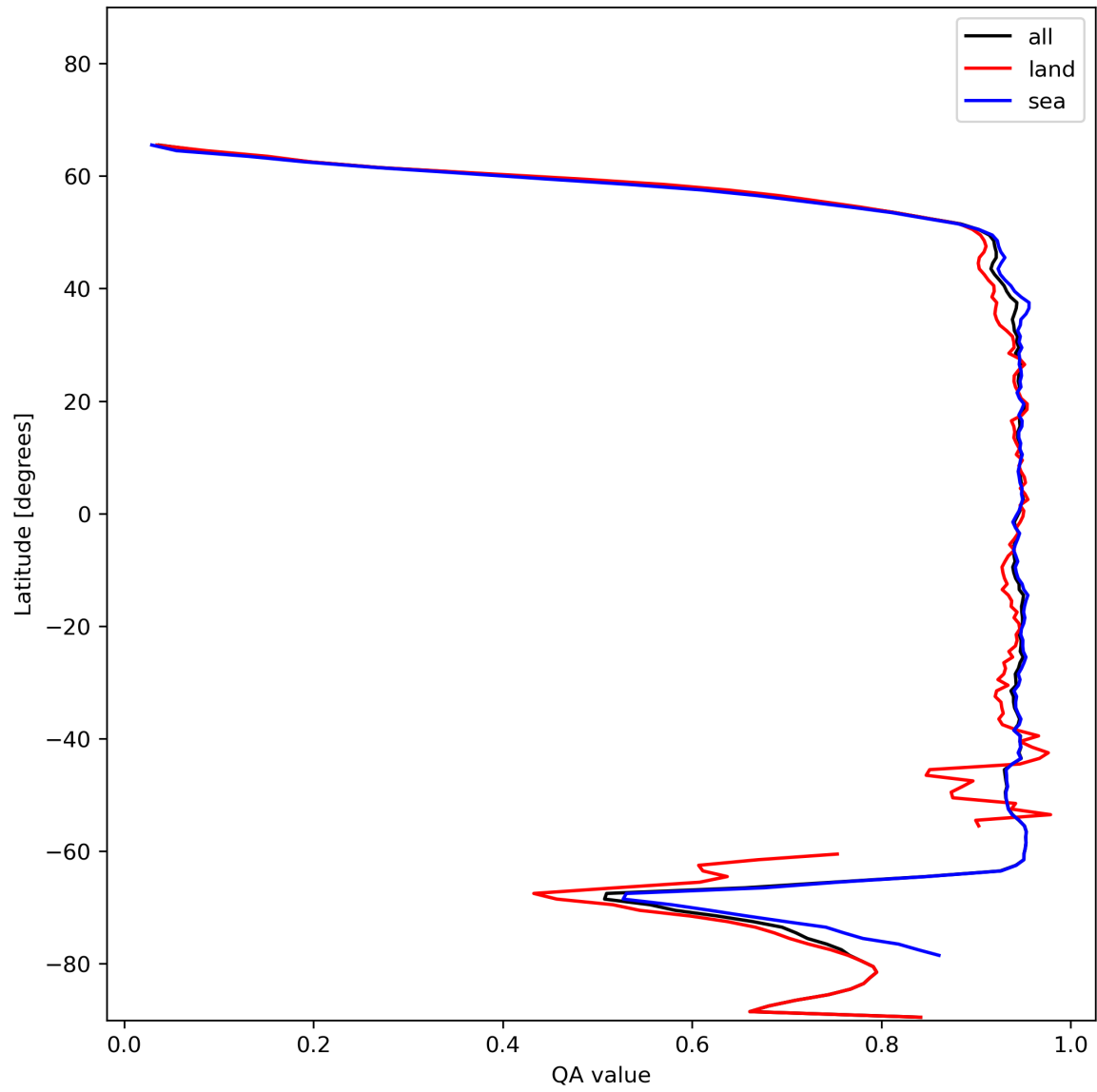
Figure 13: Zonal average of “QA value” for 2023-12-22 to 2023-12-24.
