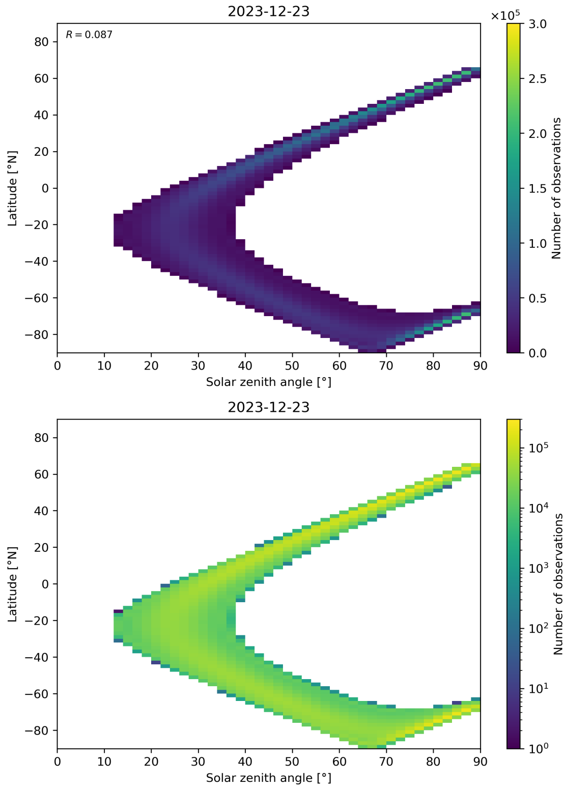
Figure 44: Scatter density plot of “Solar zenith angle” against “Latitude” for 2023-12-22 to 2023-12-24.
