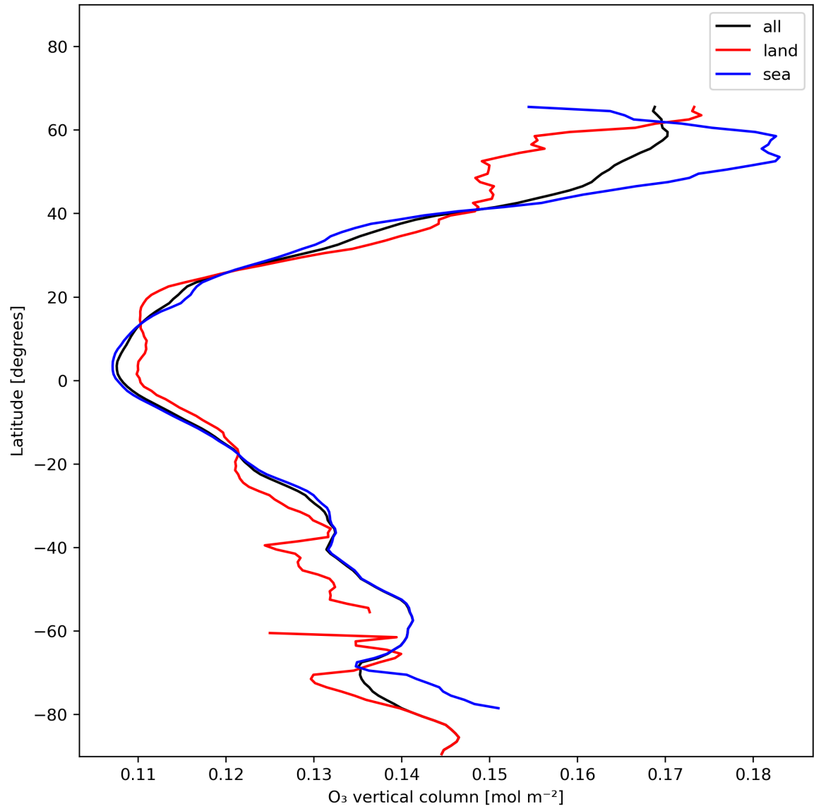
Figure 14: Zonal average of “O 3 vertical column” for 2023-12-22 to 2023-12-24.
