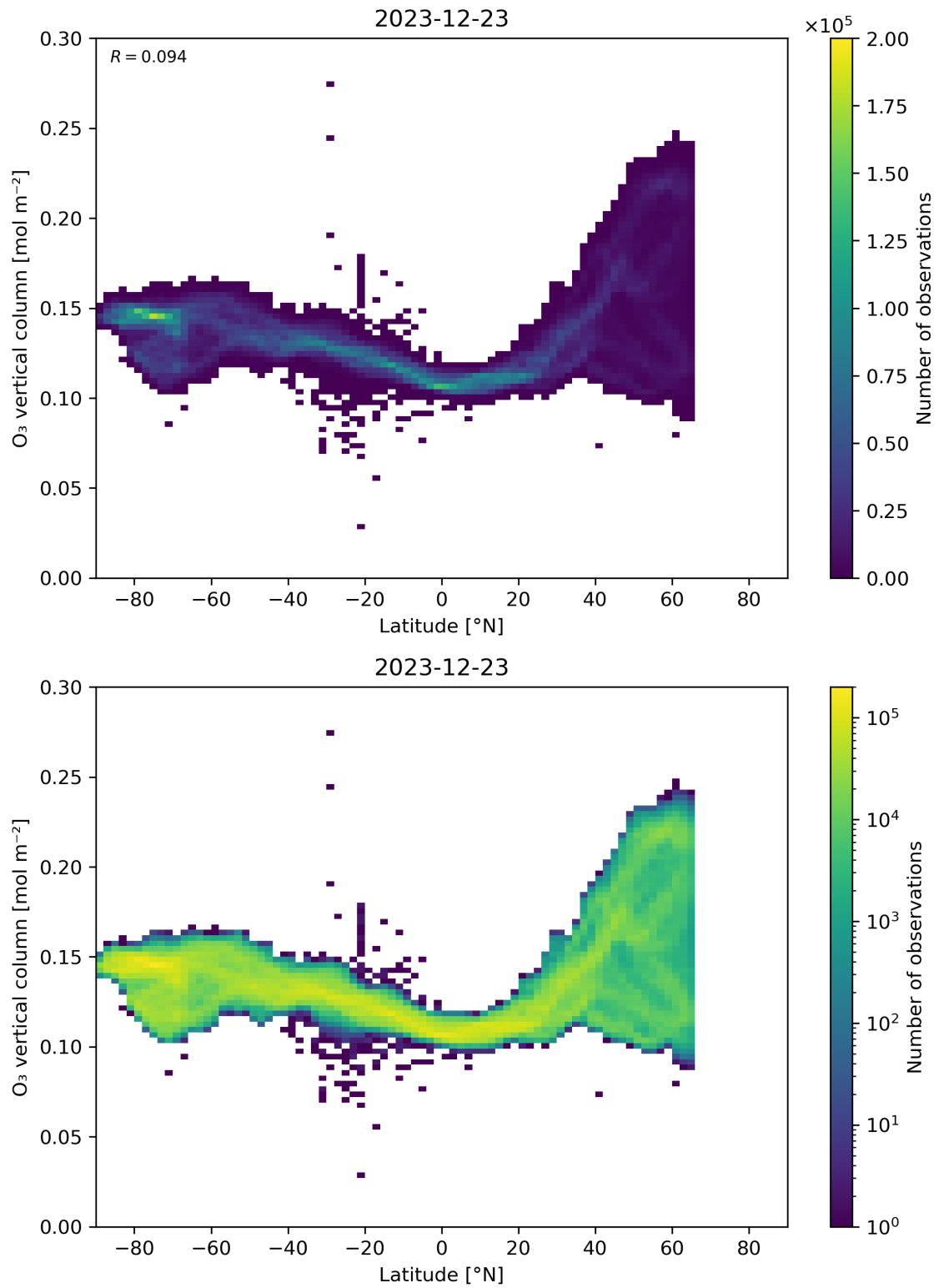
Figure 36: Scatter density plot of “Latitude” against “O 3 vertical column” for 2023-12-22 to 2023-12-24.
