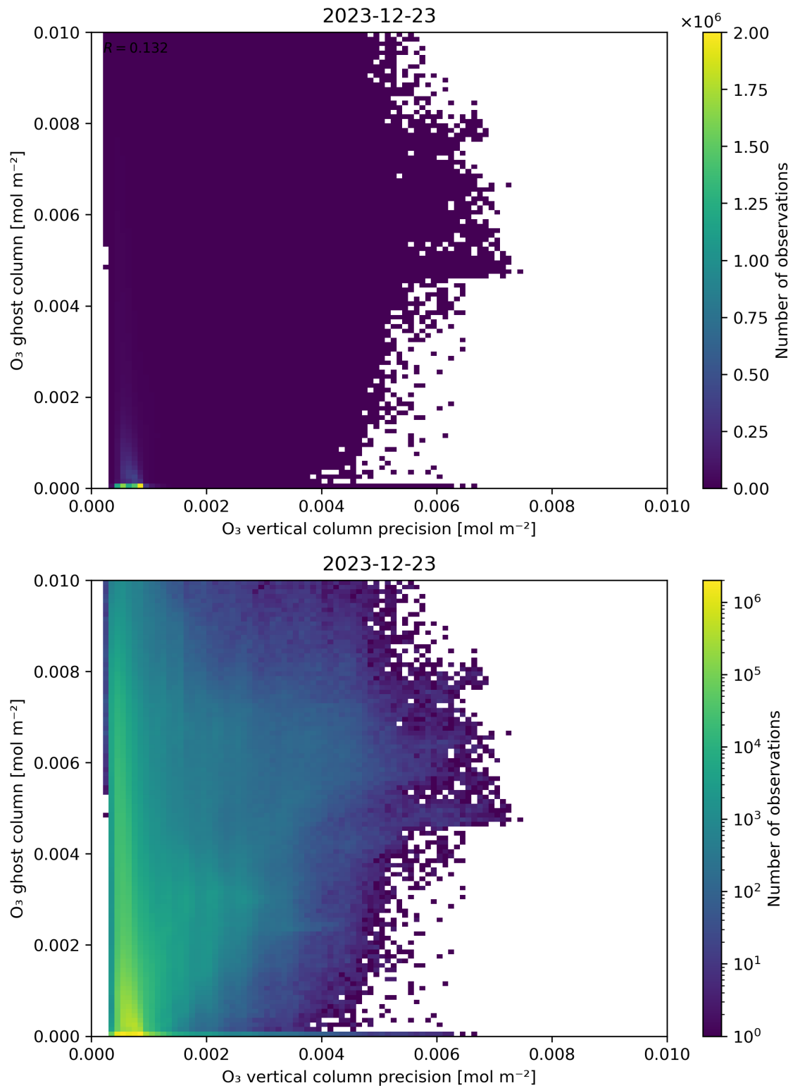
Figure 43: Scatter density plot of “ O_3 vertical column precision” against “ O_3 ghost column” for 2023-12-22 to 2023-12-24.
