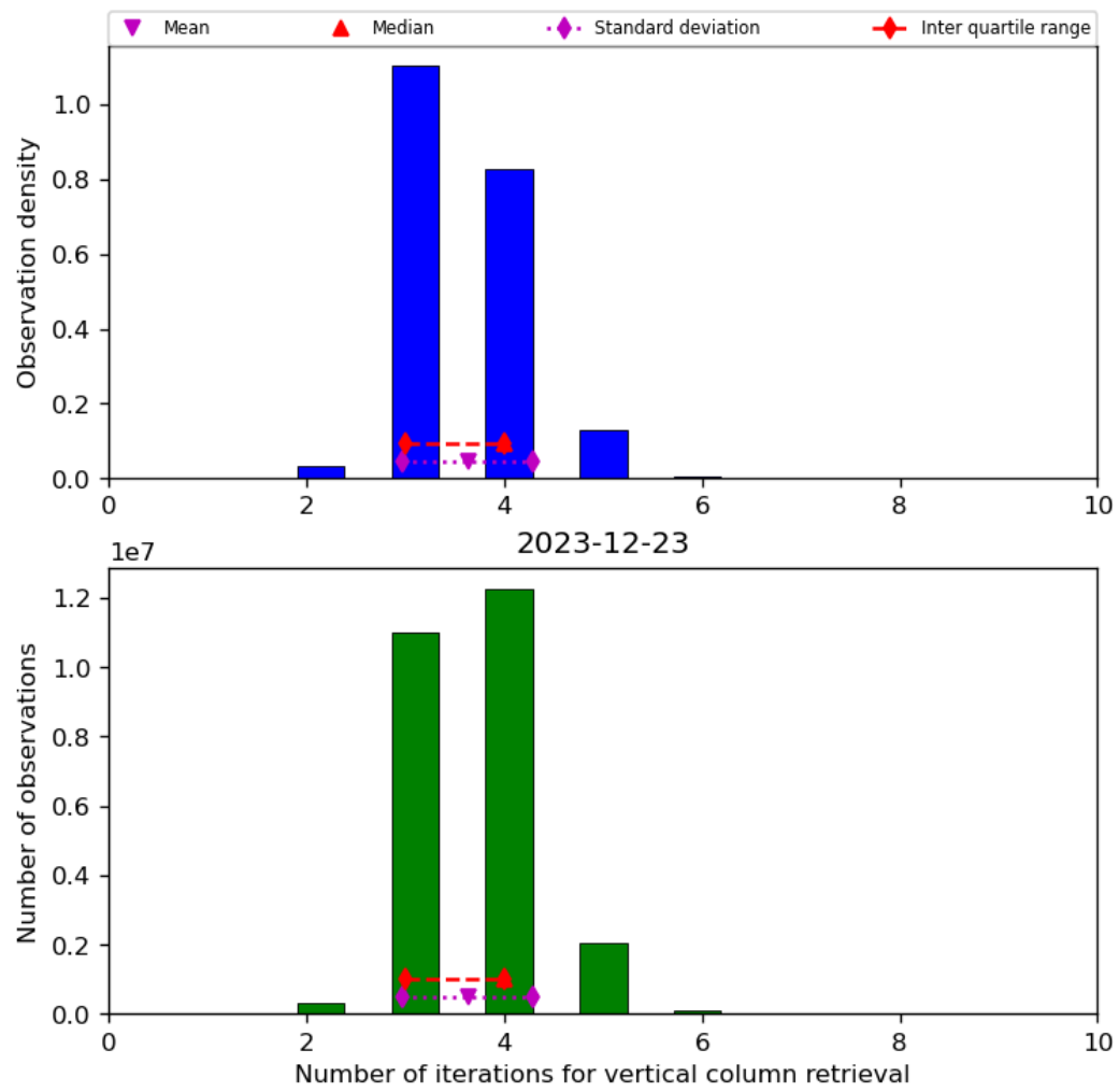
Figure 26: Histogram of “Number of iterations for vertical column retrieval” for 2023-12-22 to 2023-12-24
