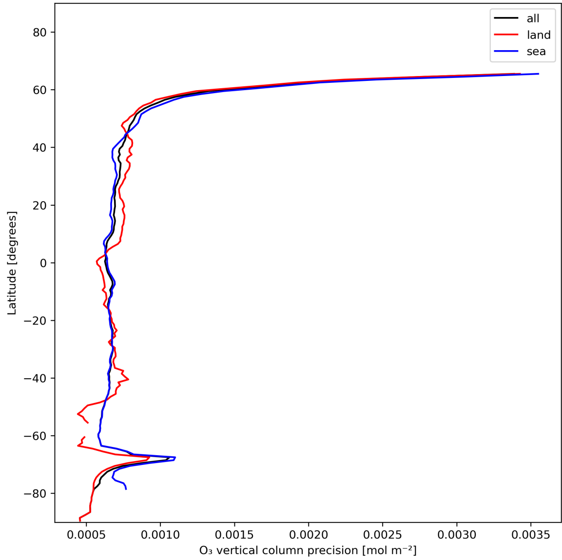
Figure 15: Zonal average of “O 3 vertical column precision” for 2023-12-22 to 2023-12-24.
