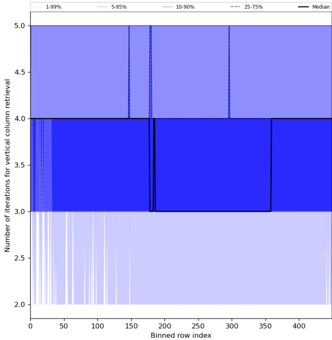
Figure 33: Along track statistics of “Number of iterations for vertical column retrieval” for 2023-12-22 to 2023-12-24
