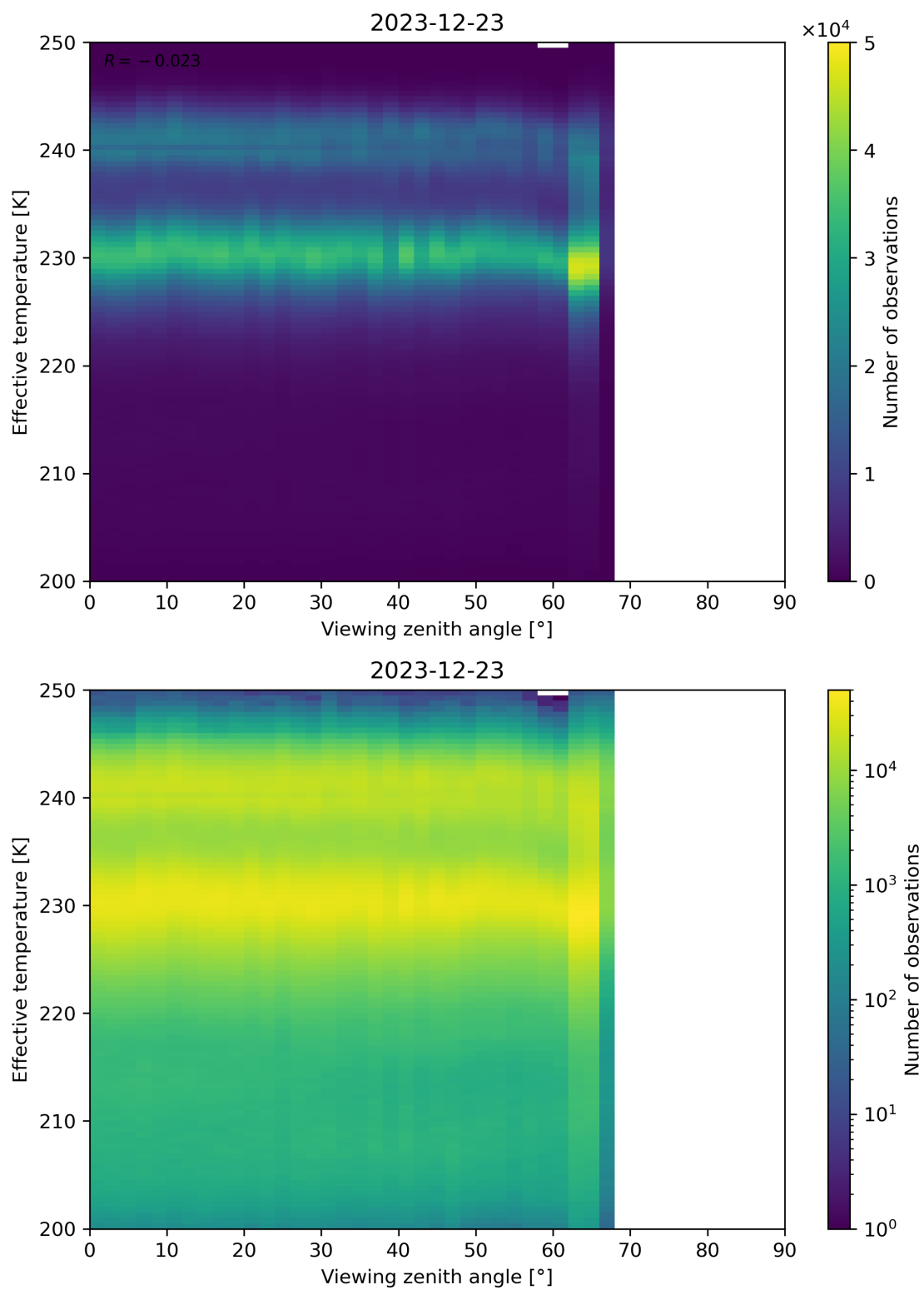
Figure 50: Scatter density plot of “Viewing zenith angle” against “Effective temperature” for 2023-12-22 to 2023-12-24.
