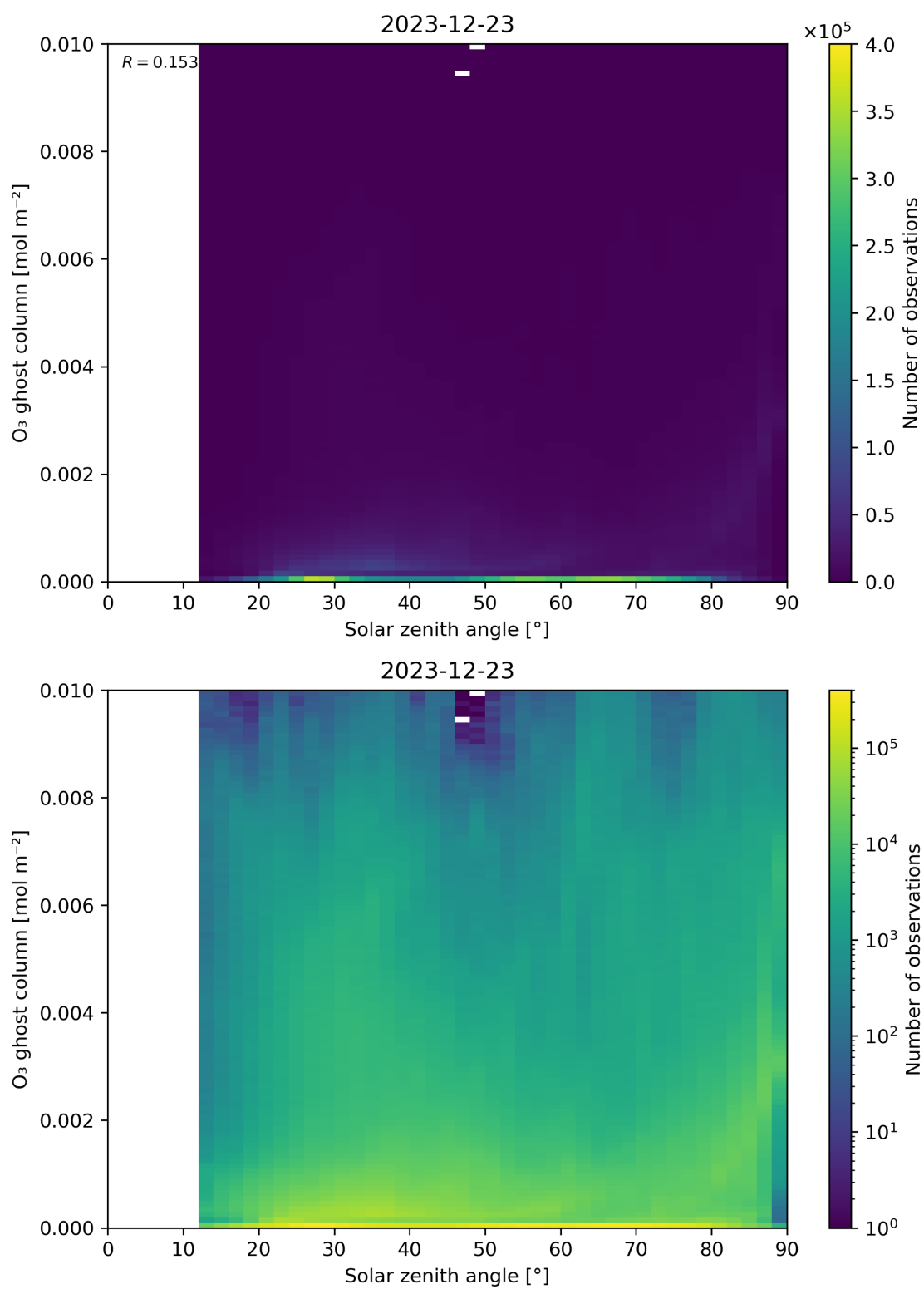
Figure 46: Scatter density plot of “Solar zenith angle” against “O 3 ghost column” for 2023-12-22 to 2023-12-24.
