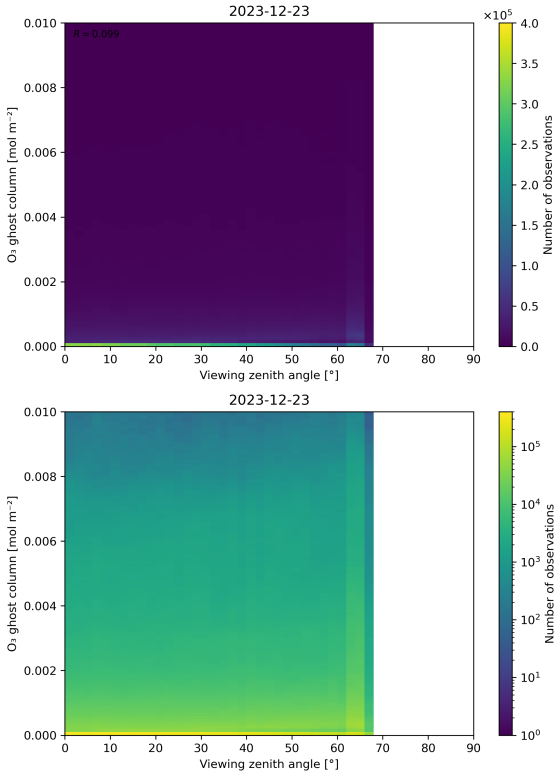
Figure 51: Scatter density plot of “Viewing zenith angle” against “O 3 ghost column” for 2023-12-22 to 2023-12-24.
