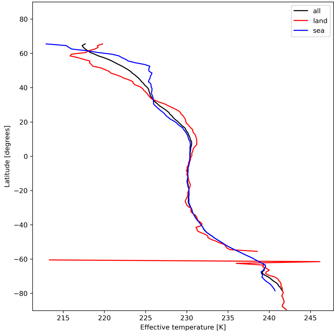
Figure 17: Zonal average of “Effective temperature” for 2023-12-22 to 2023-12-24.
