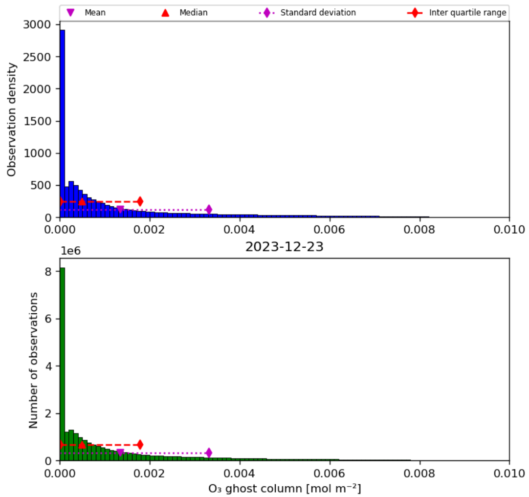
Figure 25: Histogram of “O 3 ghost column” for 2023-12-22 to 2023-12-24
