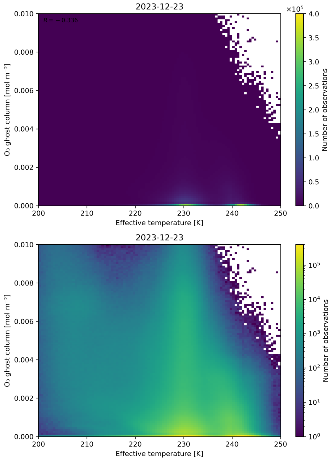
Figure 38: Scatter density plot of “Effective temperature” against “O 3 ghost column” for 2023-12-22 to 2023-12-24.
