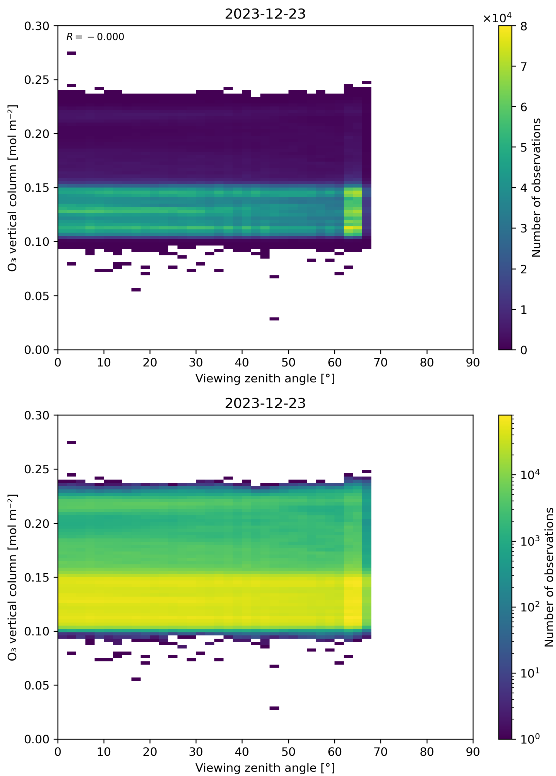
Figure 52: Scatter density plot of “Viewing zenith angle” against “O 3 vertical column” for 2023-12-22 to 2023-12-24.
