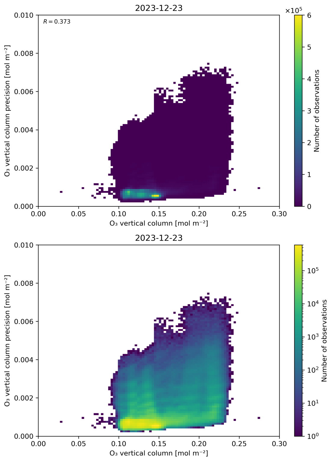
Figure 41: Scatter density plot of “O 3 vertical column” against “O 3 vertical column precision” for 2023-12-22 to 2023-12-24.
