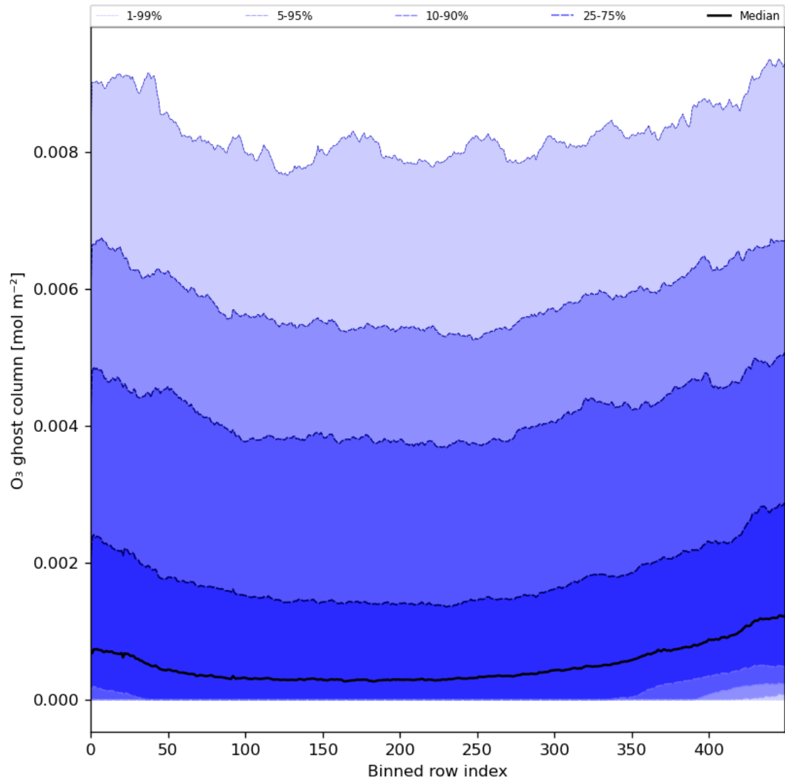
Figure 32: Along track statistics of “O 3 ghost column” for 2023-12-22 to 2023-12-24
