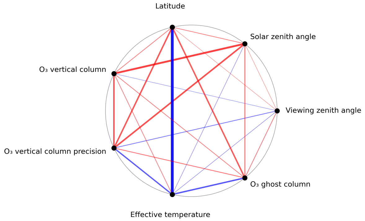
Figure 1: Map of correlation graph for 2023-12-22 to 2023-12-24.
