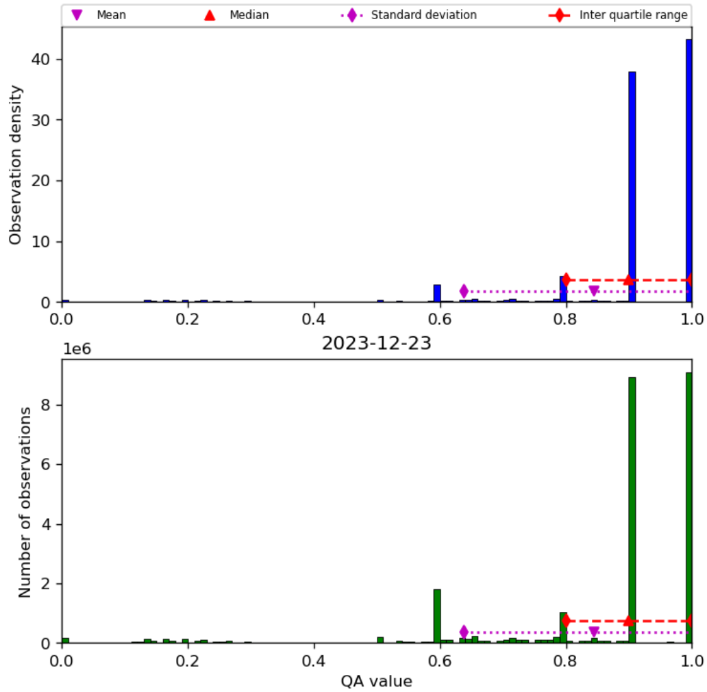
Figure 20: Histogram of “QA value” for 2023-12-22 to 2023-12-24
