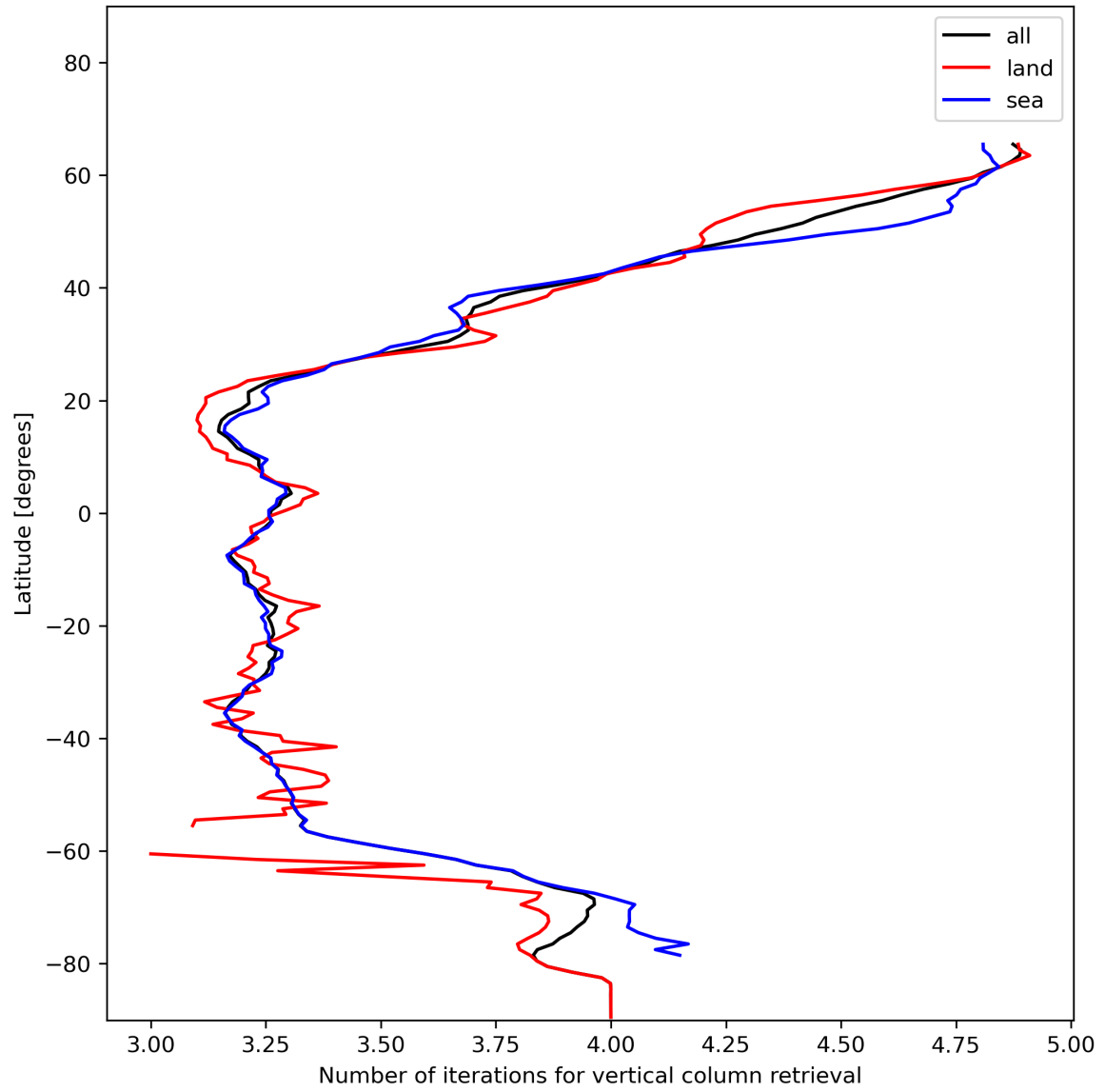
Figure 19: Zonal average of “Number of iterations for vertical column retrieval” for 2023-12-22 to 2023-12-24.
