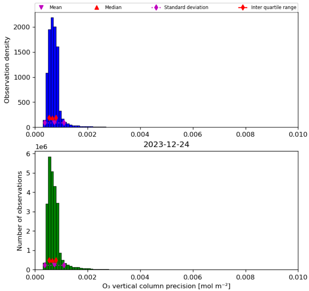
Figure 22: Histogram of “O 3 vertical column precision” for 2023-12-23 to 2023-12-25
