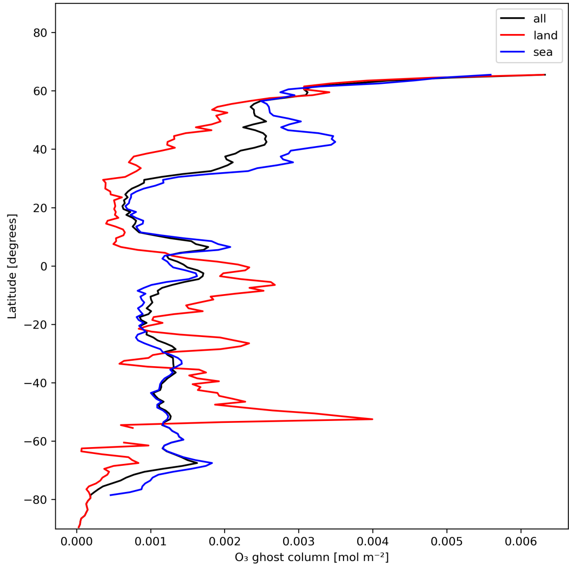
Figure 18: Zonal average of “O 3 ghost column” for 2023-12-23 to 2023-12-25.
