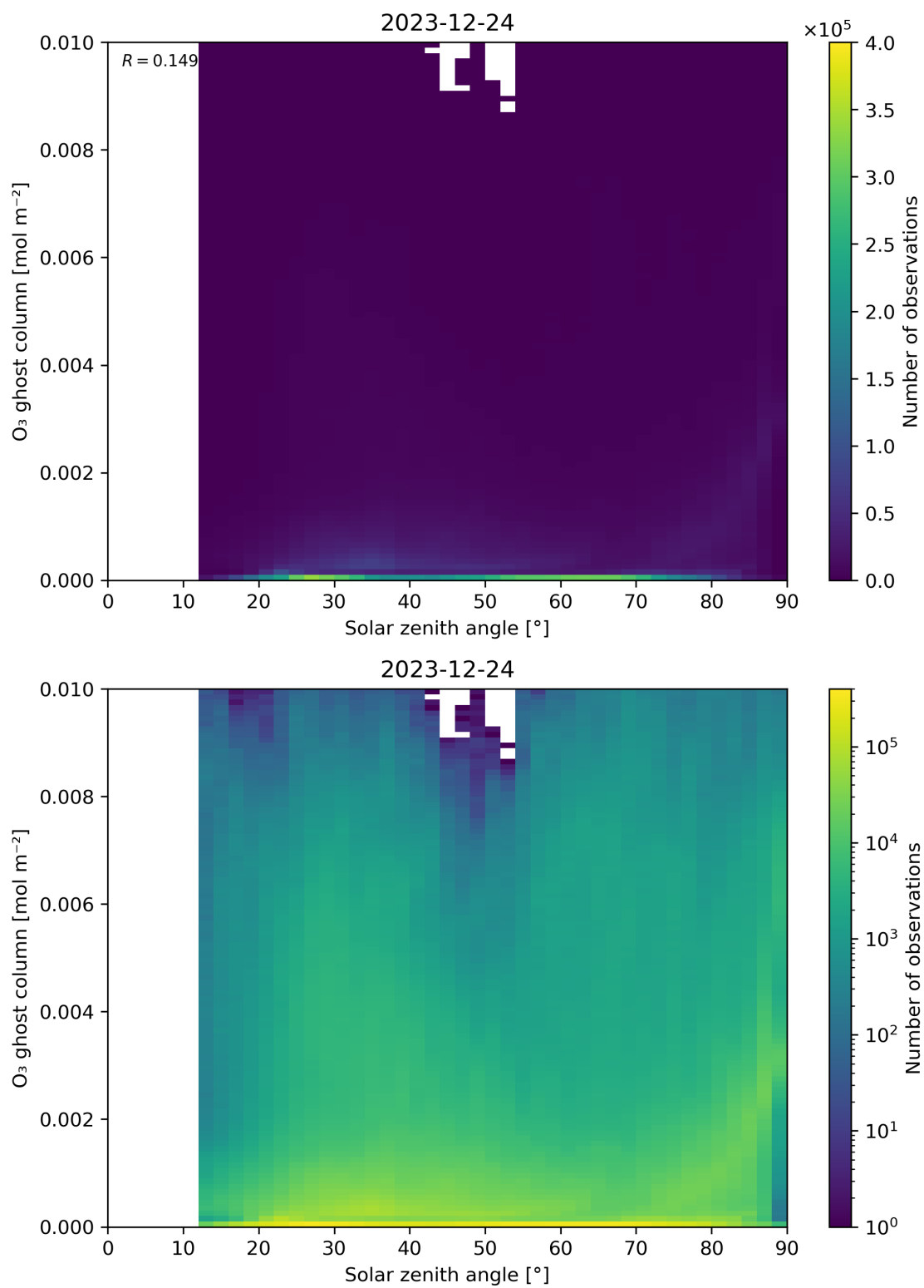
Figure 46: Scatter density plot of “Solar zenith angle” against “O 3 ghost column” for 2023-12-23 to 2023-12-25.
