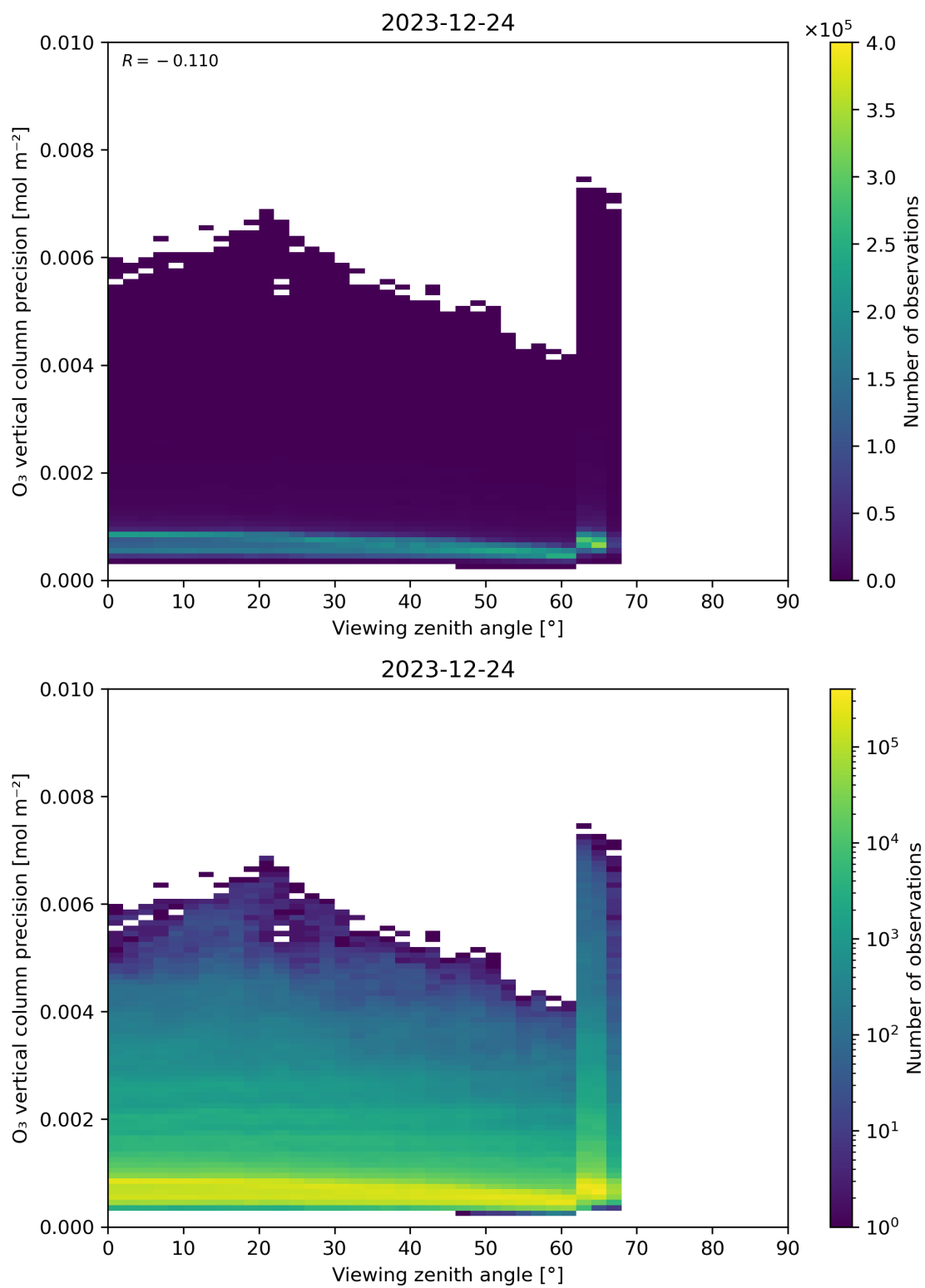
Figure 53: Scatter density plot of “Viewing zenith angle” against “O 3 vertical column precision” for 2023-12-23 to 2023-12-25.
