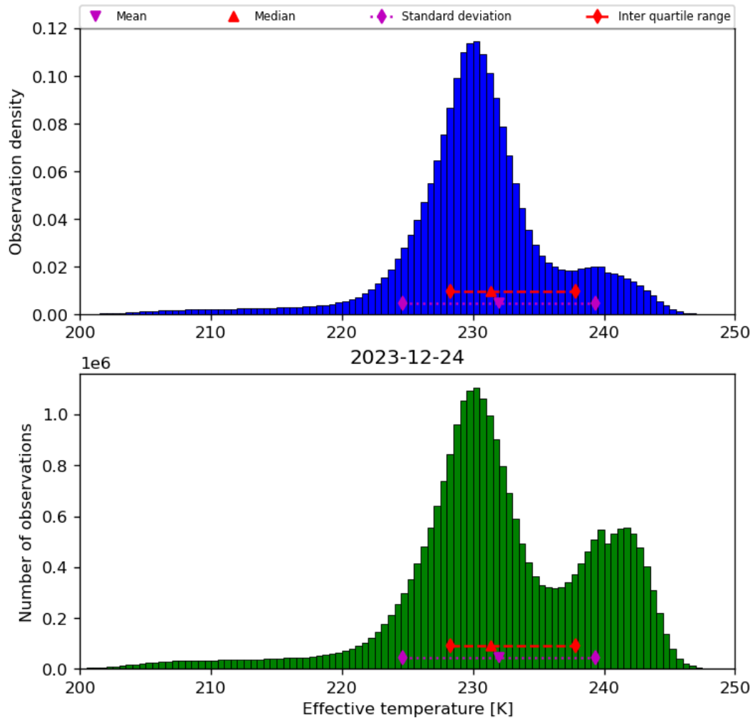
Figure 24: Histogram of “Effective temperature” for 2023-12-23 to 2023-12-25
