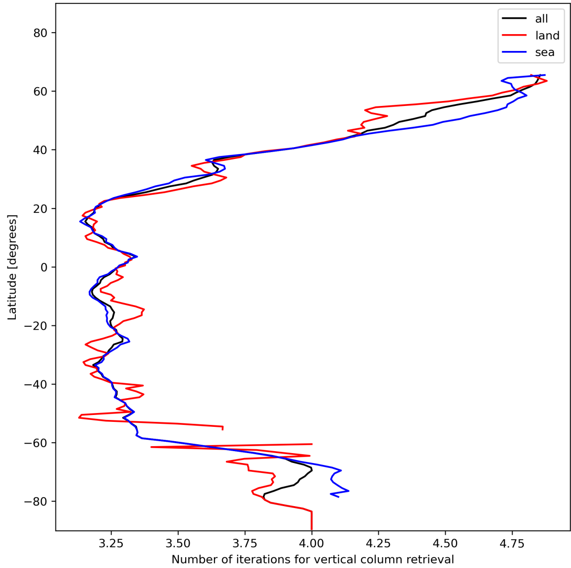
Figure 19: Zonal average of “Number of iterations for vertical column retrieval” for 2023-12-23 to 2023-12-25.
