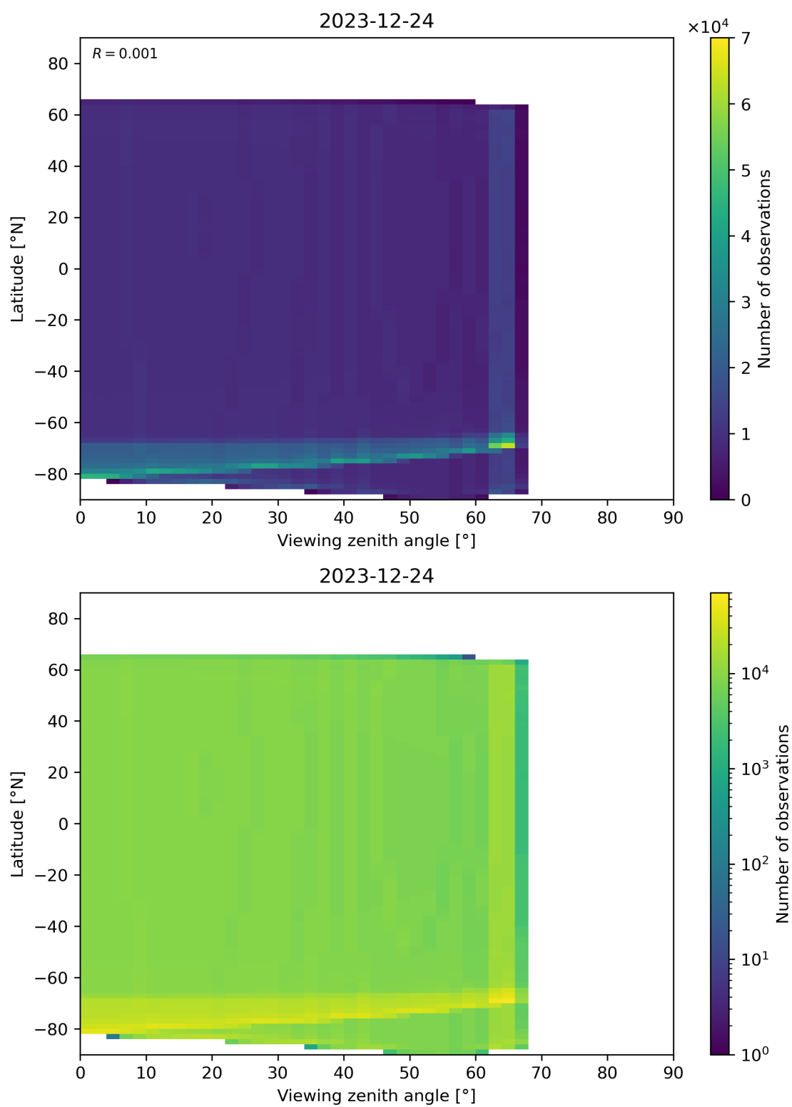
Figure 49: Scatter density plot of “Viewing zenith angle” against “Latitude” for 2023-12-23 to 2023-12-25.
