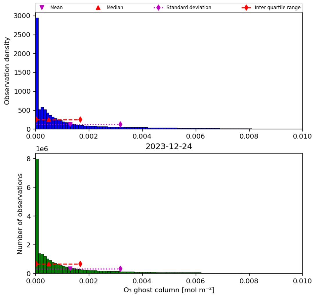
Figure 25: Histogram of “O 3 ghost column” for 2023-12-23 to 2023-12-25
