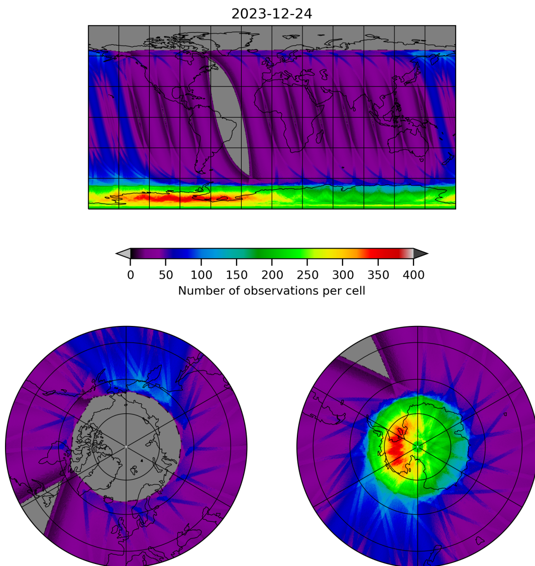
Figure 12: Map of the number of observations for 2023-12-23 to 2023-12-25
