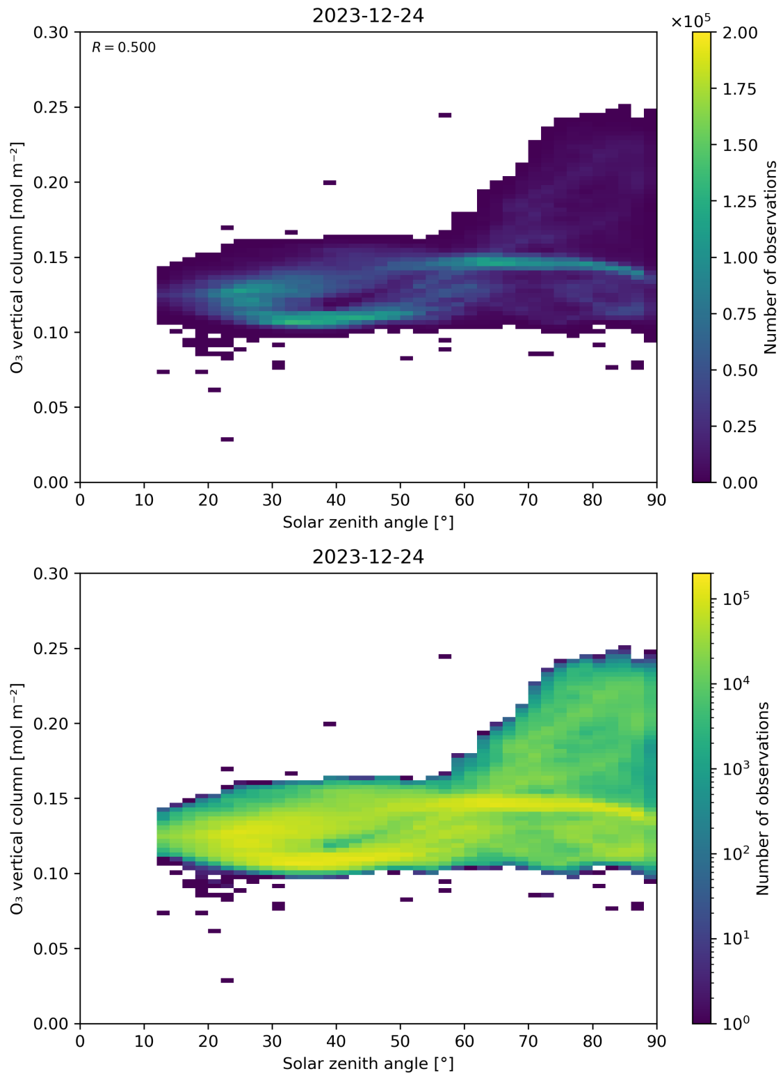
Figure 47: Scatter density plot of “Solar zenith angle” against “O 3 vertical column” for 2023-12-23 to 2023-12-25.
