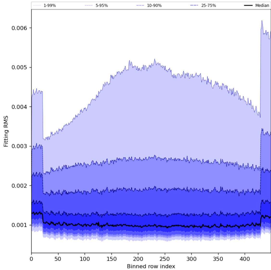
Figure 30: Along track statistics of “Fitting RMS” for 2023-12-23 to 2023-12-25
