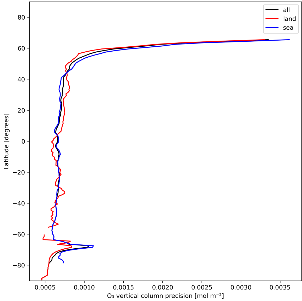
Figure 15: Zonal average of “O 3 vertical column precision” for 2023-12-23 to 2023-12-25.
