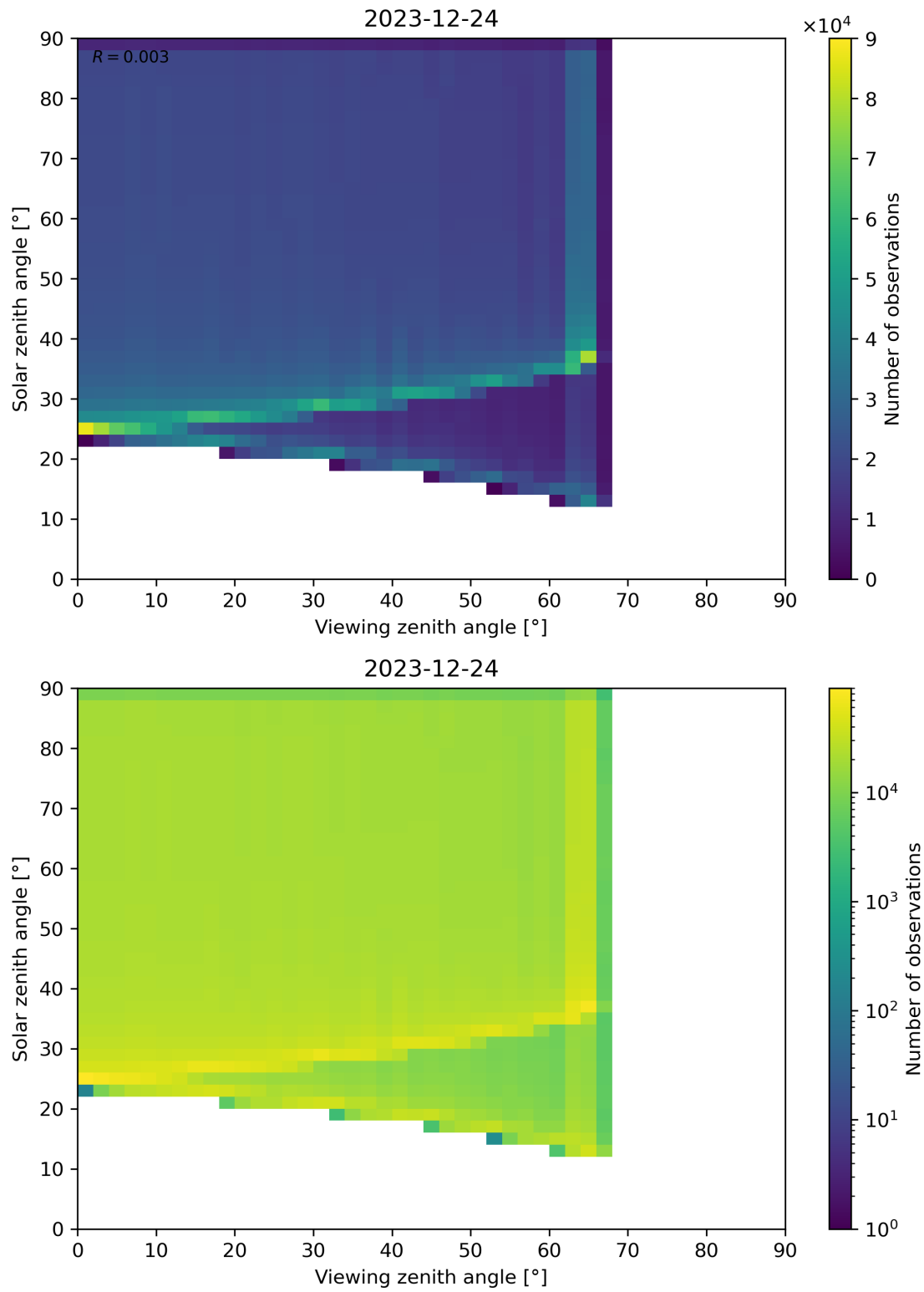
Figure 54: Scatter density plot of “Viewing zenith angle” against “Solar zenith angle” for 2023-12-23 to 2023-12-25.
