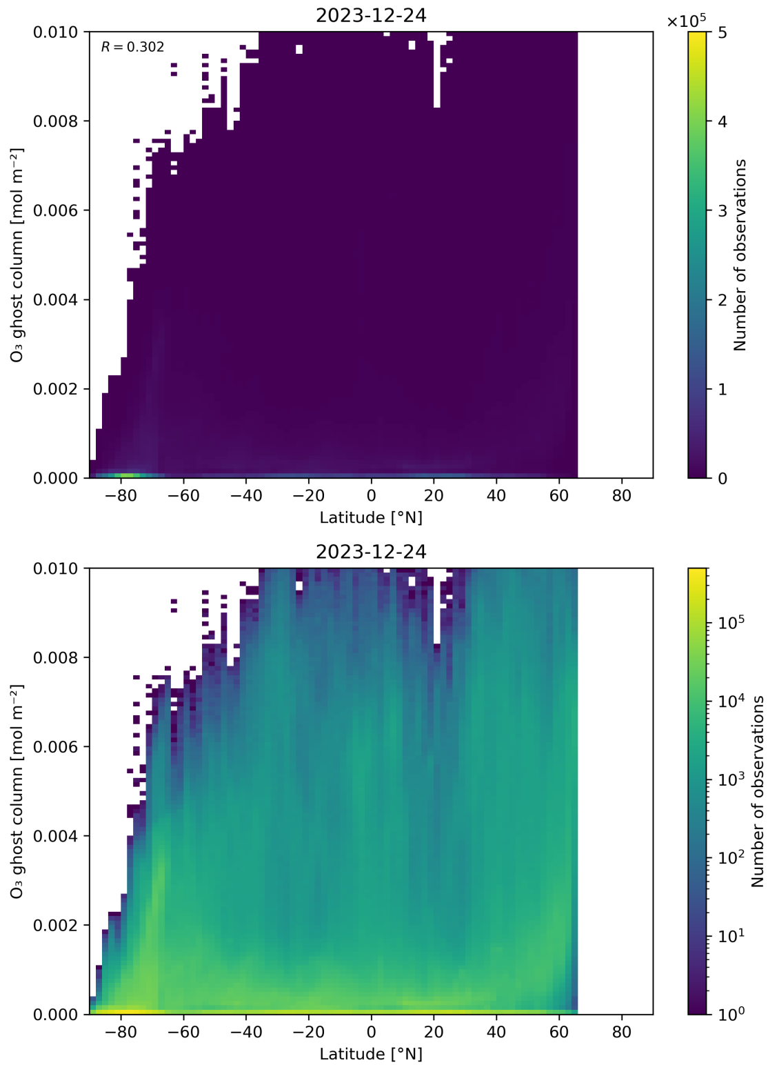
Figure 35: Scatter density plot of “Latitude” against “O 3 ghost column” for 2023-12-23 to 2023-12-25.
