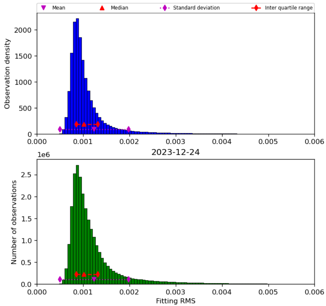
Figure 23: Histogram of “Fitting RMS” for 2023-12-23 to 2023-12-25
