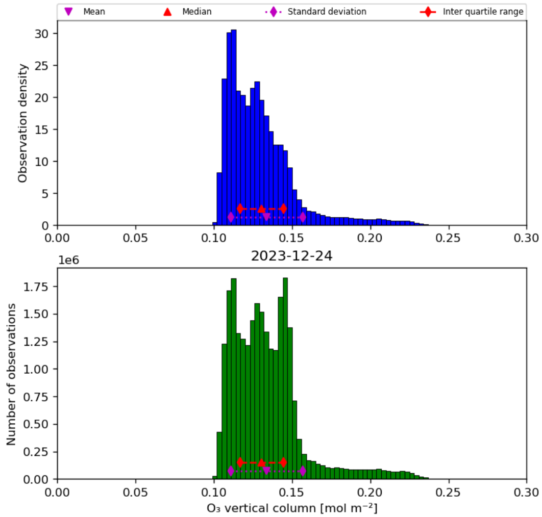
Figure 21: Histogram of “O 3 vertical column” for 2023-12-23 to 2023-12-25
