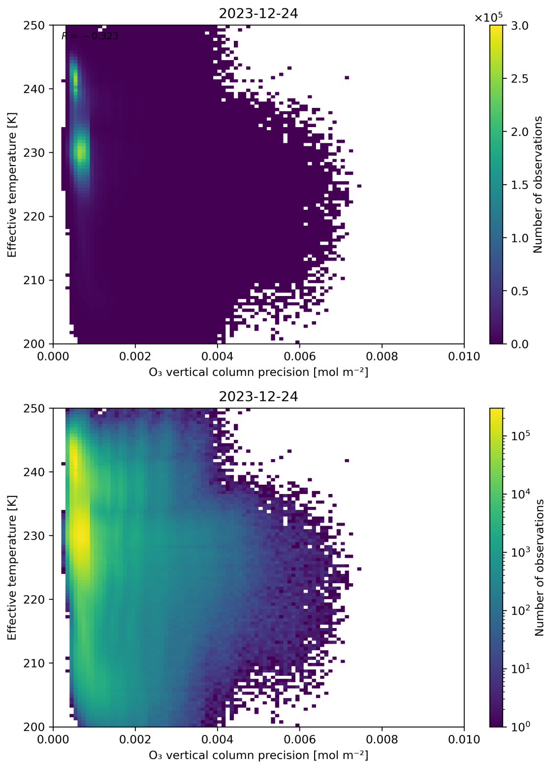
Figure 42: Scatter density plot of “O 3 vertical column precision” against “Effective temperature” for 2023-12-23 to 2023-12-25.
