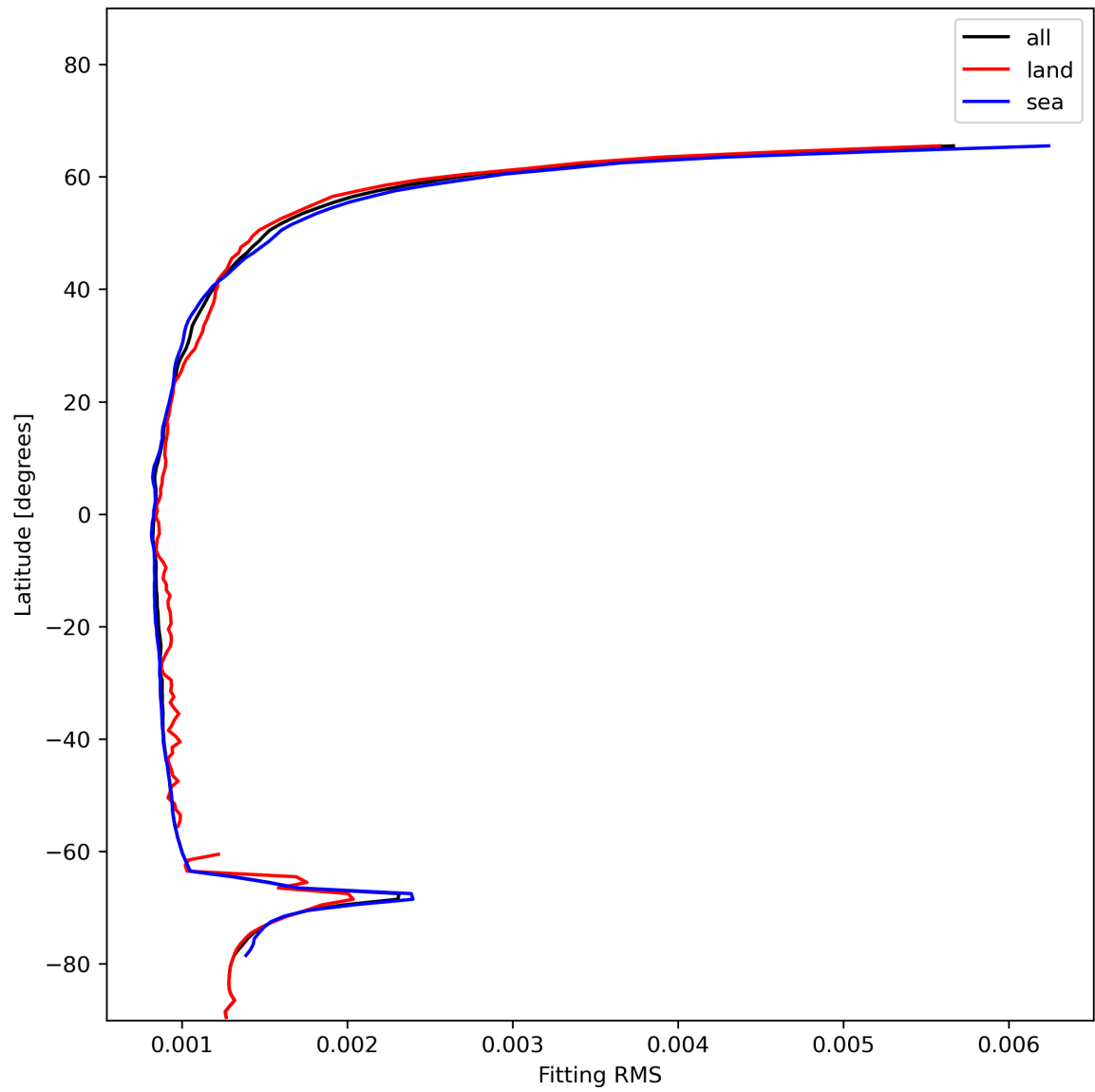
Figure 16: Zonal average of “Fitting RMS” for 2023-12-23 to 2023-12-25.
