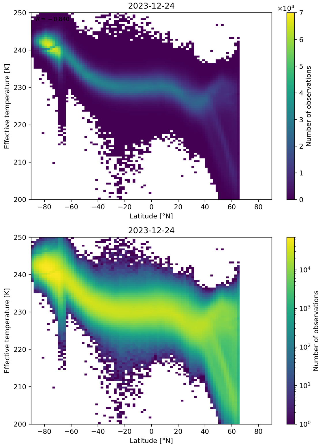
Figure 34: Scatter density plot of “Latitude” against “Effective temperature” for 2023-12-23 to 2023-12-25.
