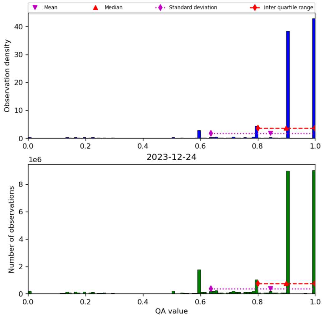
Figure 20: Histogram of “QA value” for 2023-12-23 to 2023-12-25
