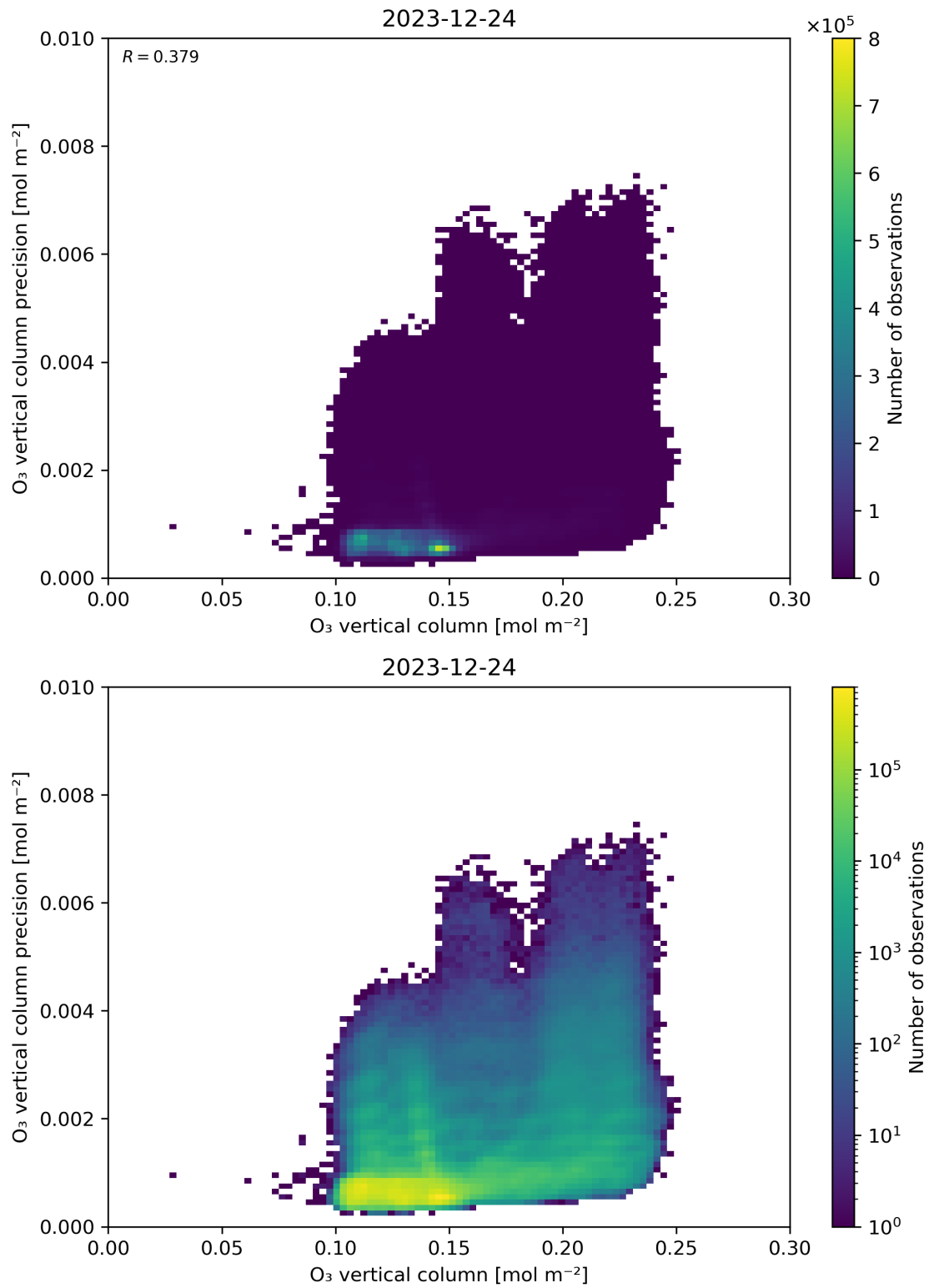
Figure 41: Scatter density plot of “O 3 vertical column” against “O 3 vertical column precision” for 2023-12-23 to 2023-12-25.
