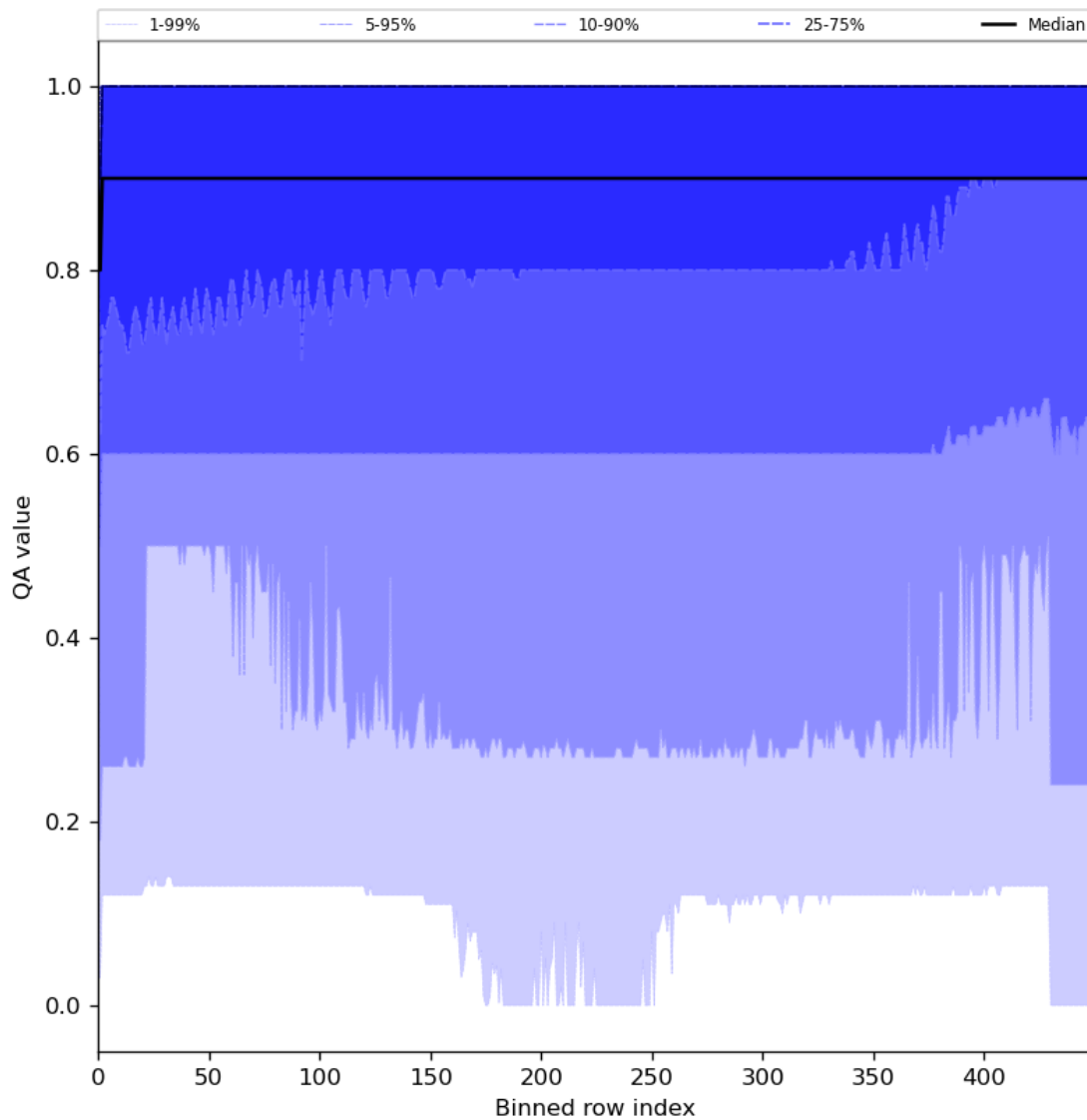
Figure 27: Along track statistics of “QA value” for 2023-12-23 to 2023-12-25
