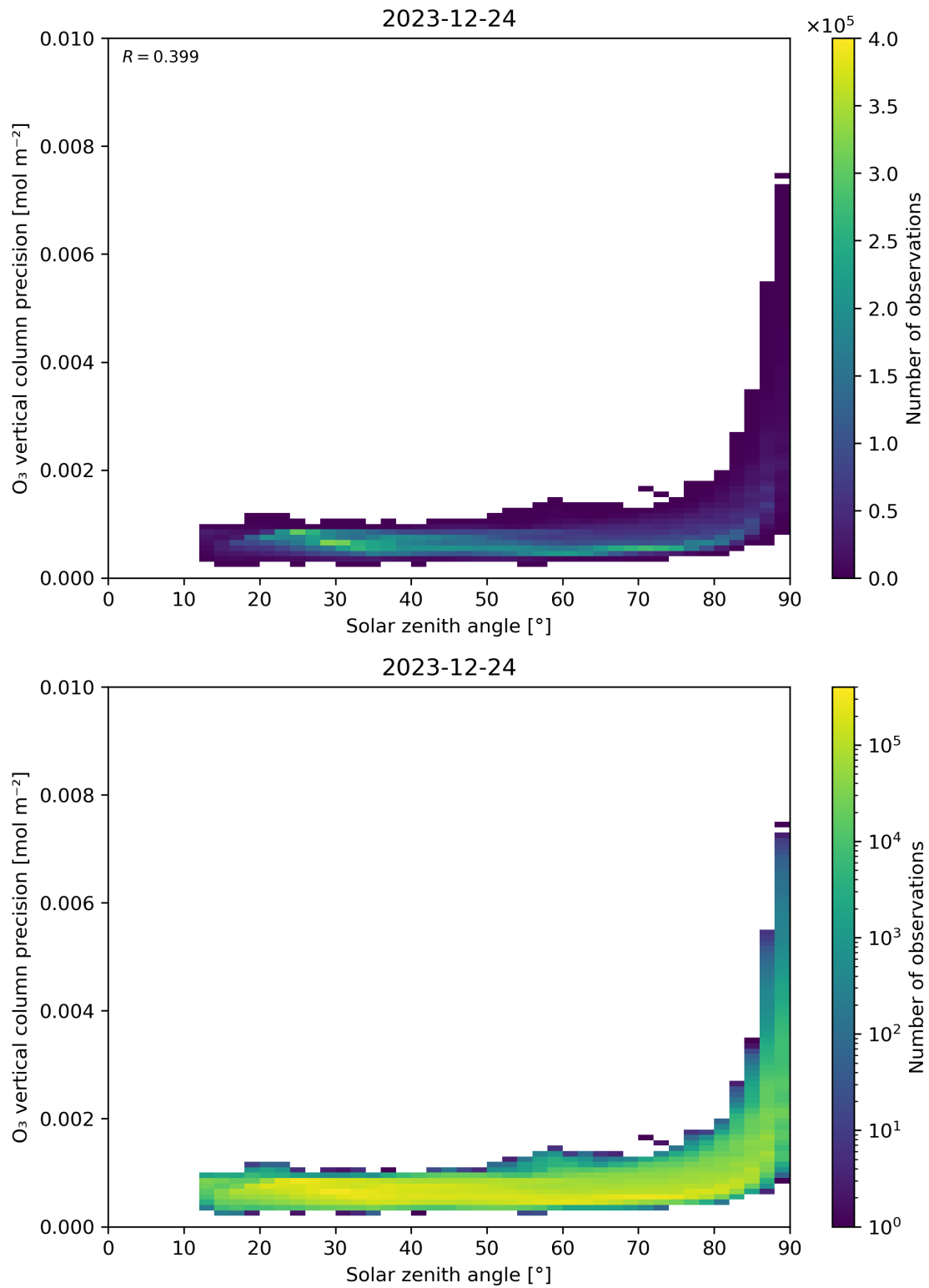
Figure 48: Scatter density plot of “Solar zenith angle” against “O 3 vertical column precision” for 2023-12-23 to 2023-12-25.
