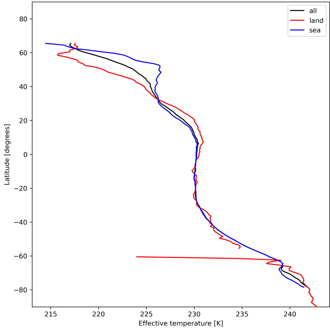
Figure 17: Zonal average of “Effective temperature” for 2023-12-23 to 2023-12-25.
