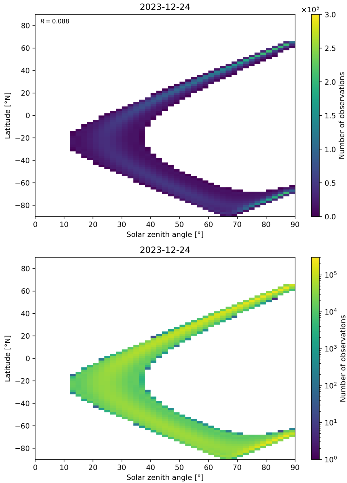
Figure 44: Scatter density plot of “Solar zenith angle” against “Latitude” for 2023-12-23 to 2023-12-25.
