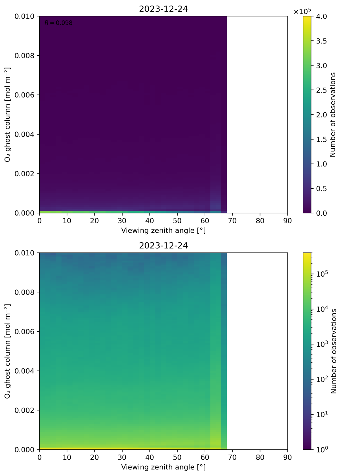
Figure 51: Scatter density plot of “Viewing zenith angle” against “O 3 ghost column” for 2023-12-23 to 2023-12-25.
