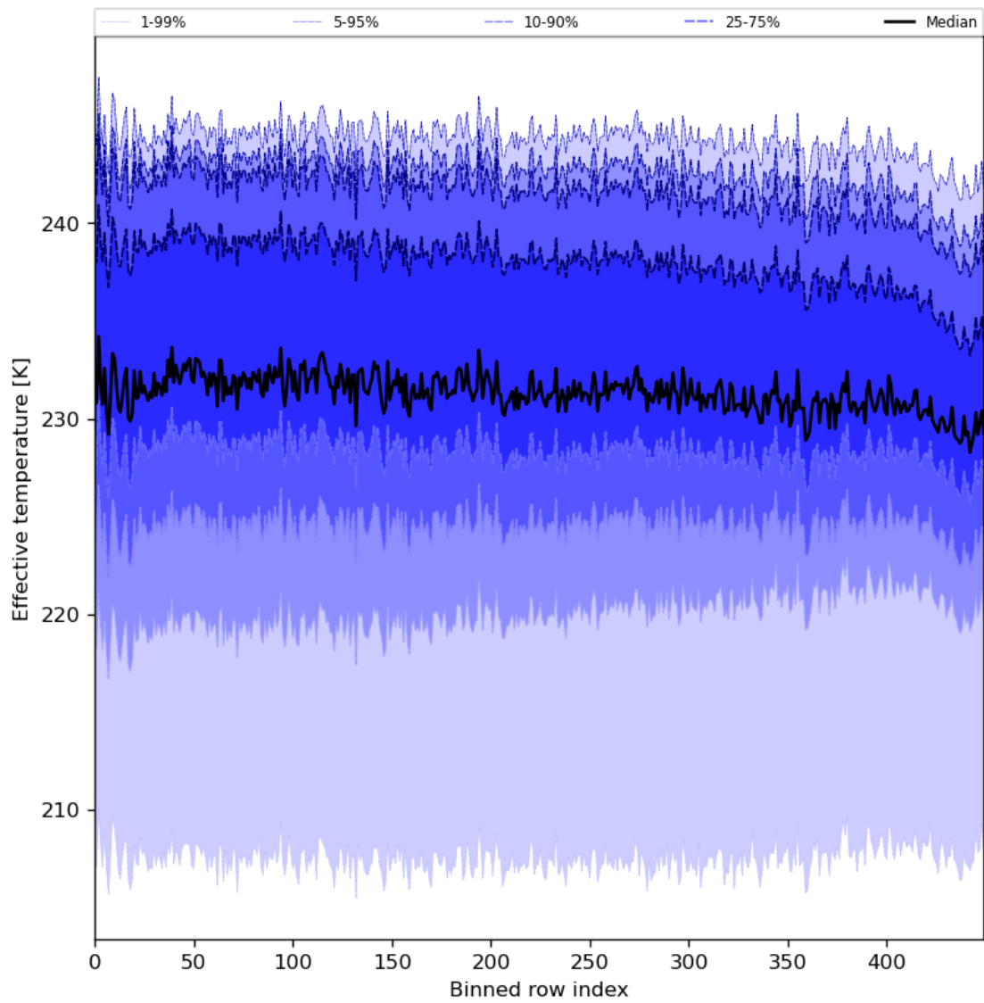
Figure 31: Along track statistics of “Effective temperature” for 2023-12-23 to 2023-12-25
