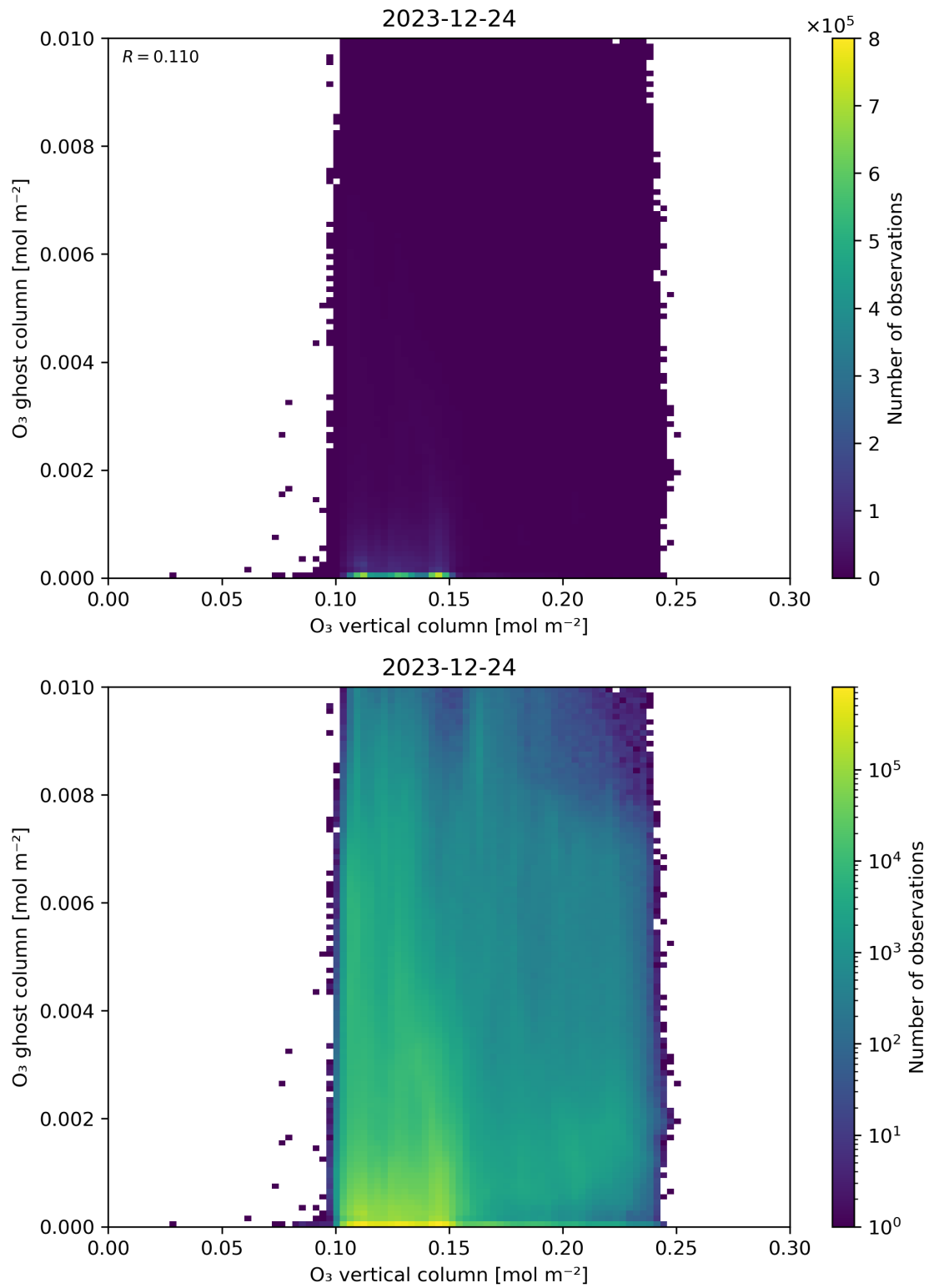
Figure 40: Scatter density plot of “O 3 vertical column” against “O 3 ghost column” for 2023-12-23 to 2023-12-25.
