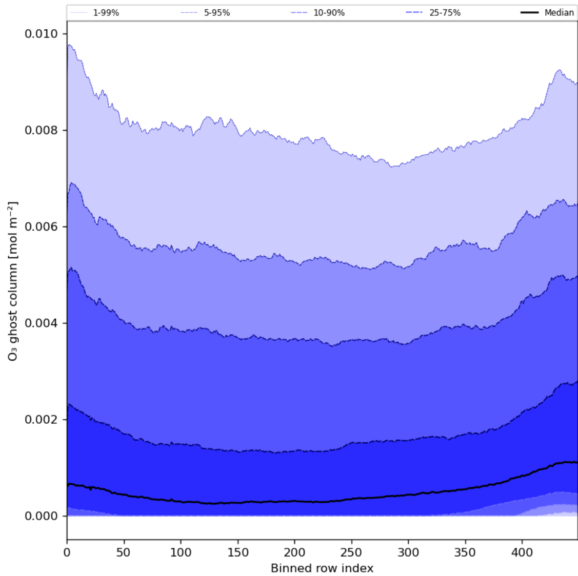
Figure 32: Along track statistics of “O 3 ghost column” for 2023-12-23 to 2023-12-25
