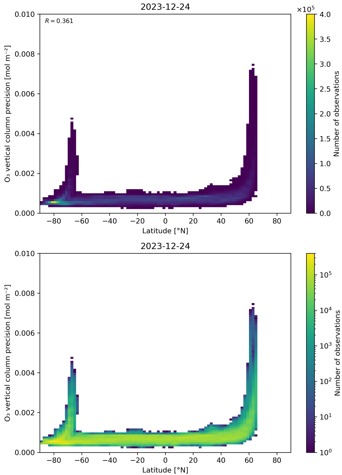
Figure 37: Scatter density plot of “Latitude” against “O 3 vertical column precision” for 2023-12-23 to 2023-12-25.
