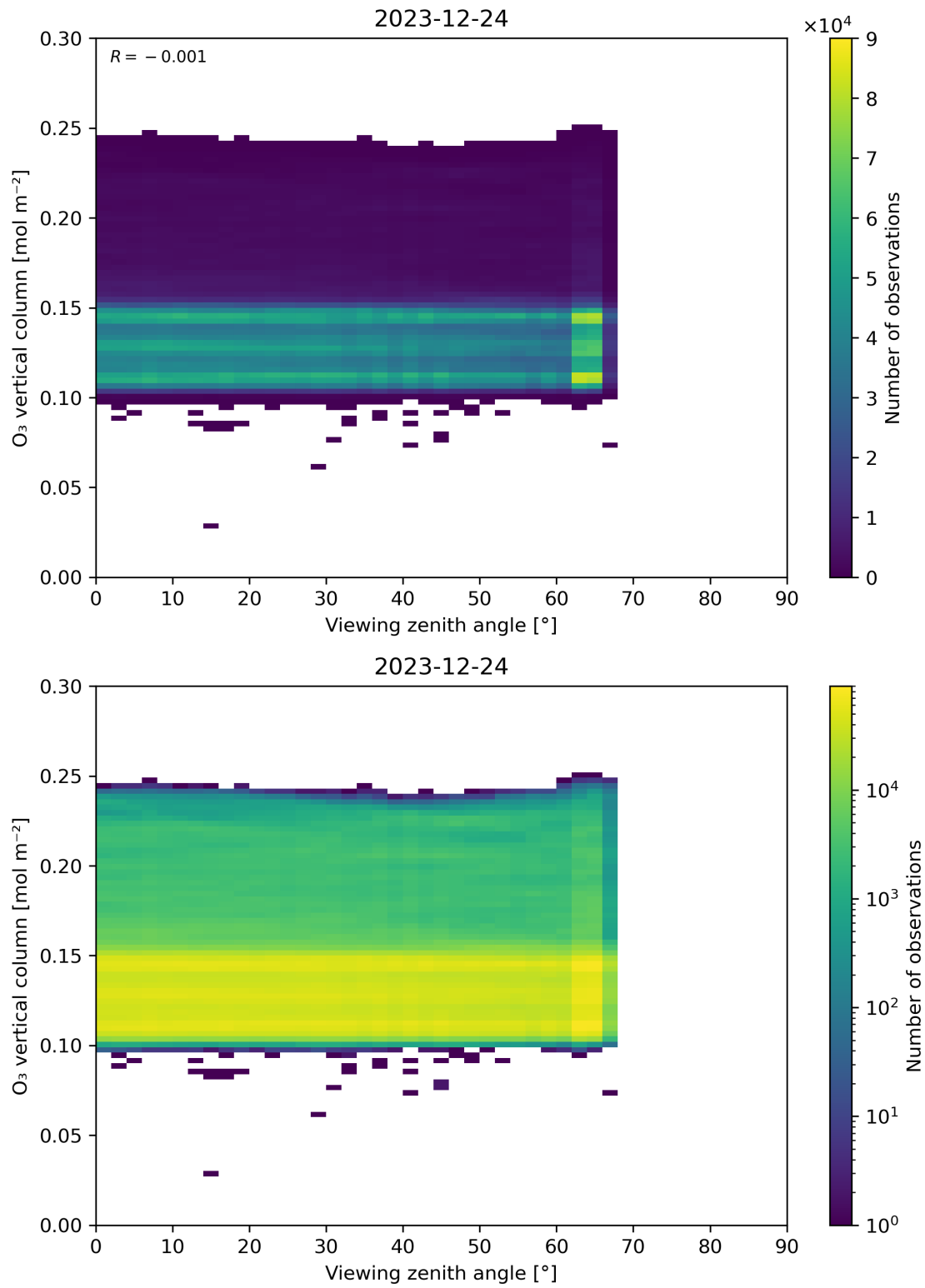
Figure 52: Scatter density plot of “Viewing zenith angle” against “O 3 vertical column” for 2023-12-23 to 2023-12-25.
