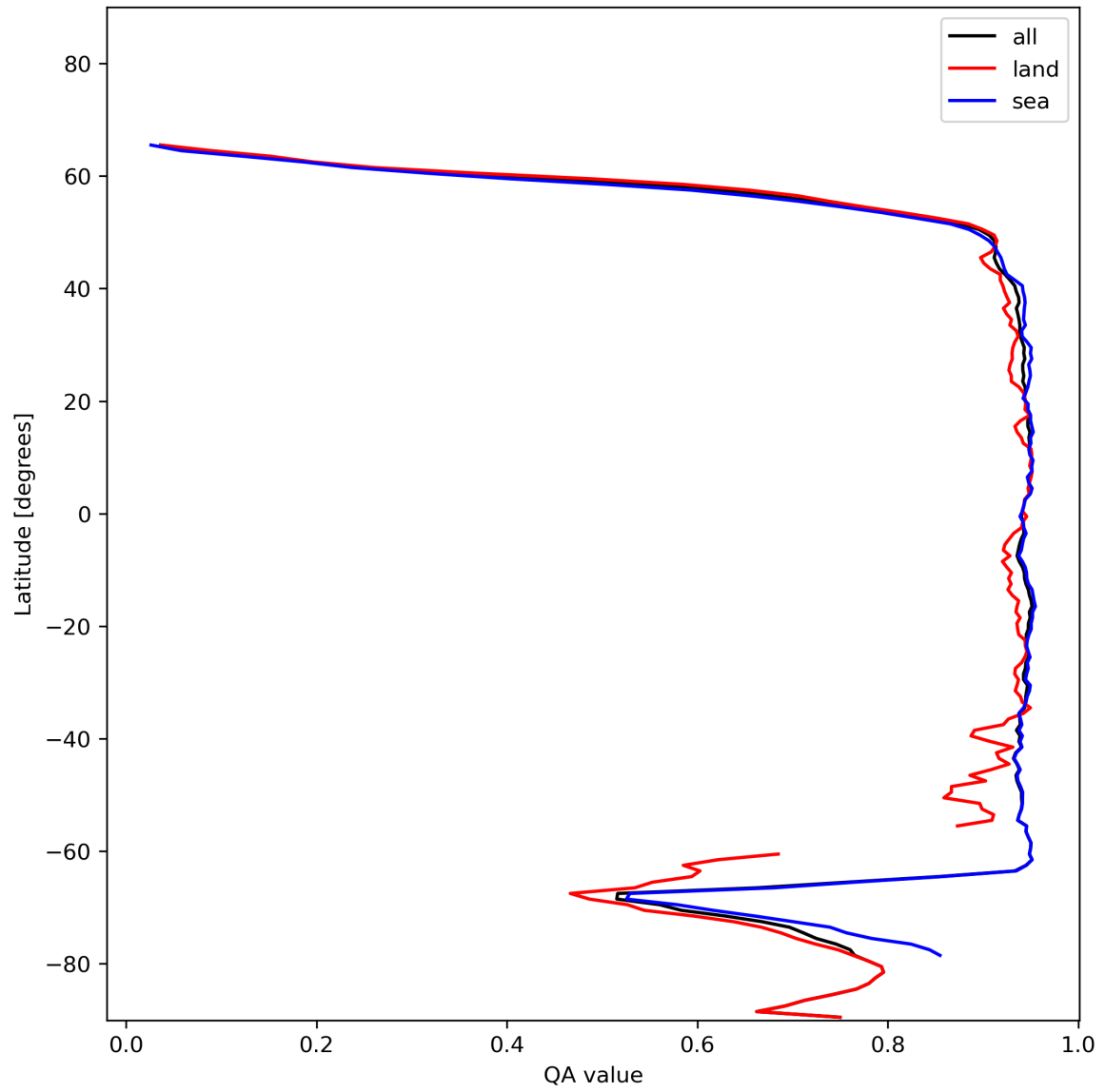
Figure 13: Zonal average of “QA value” for 2023-12-23 to 2023-12-25.
