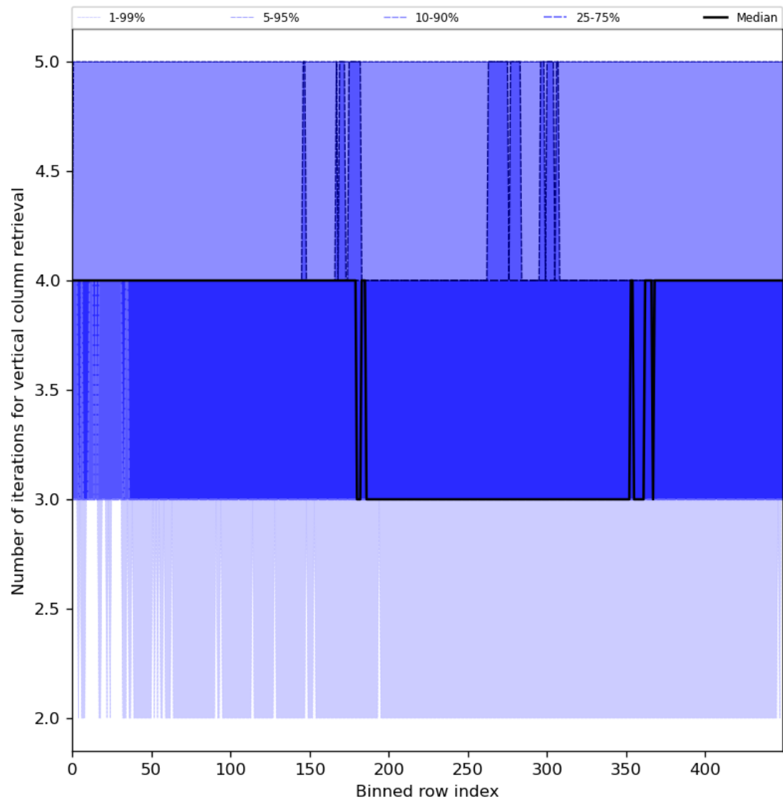
Figure 33: Along track statistics of “Number of iterations for vertical column retrieval” for 2023-12-23 to 2023-12-25
