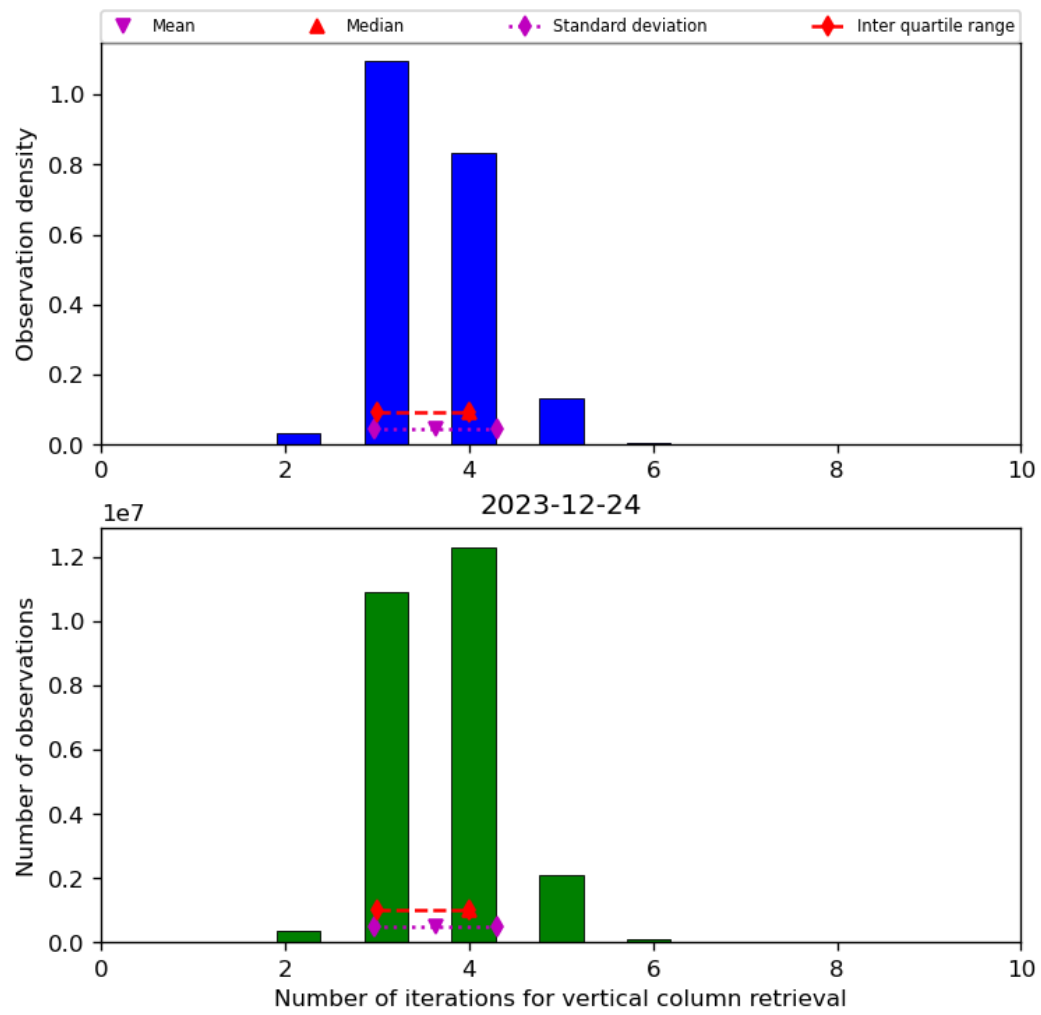
Figure 26: Histogram of “Number of iterations for vertical column retrieval” for 2023-12-23 to 2023-12-25
