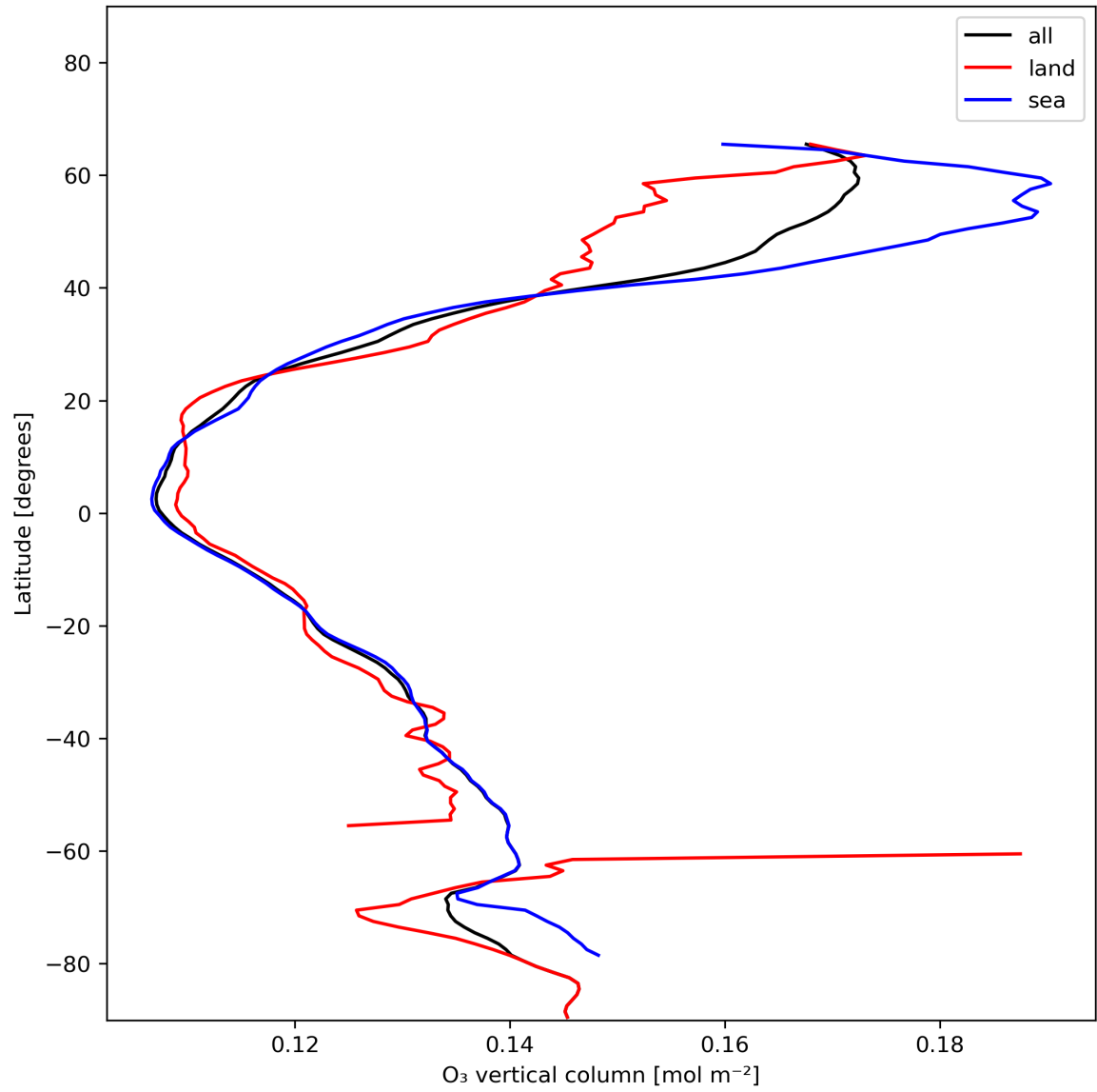
Figure 14: Zonal average of “O 3 vertical column” for 2023-12-23 to 2023-12-25.
