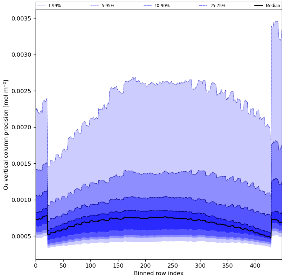
Figure 29: Along track statistics of “O 3 vertical column precision” for 2023-12-23 to 2023-12-25
