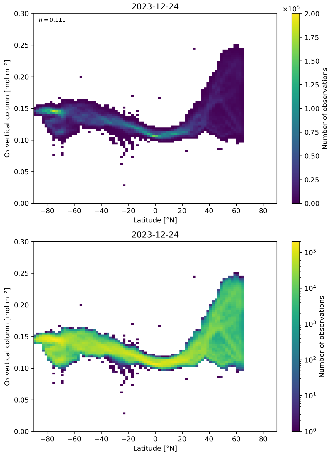
Figure 36: Scatter density plot of “Latitude” against “O 3 vertical column” for 2023-12-23 to 2023-12-25.
