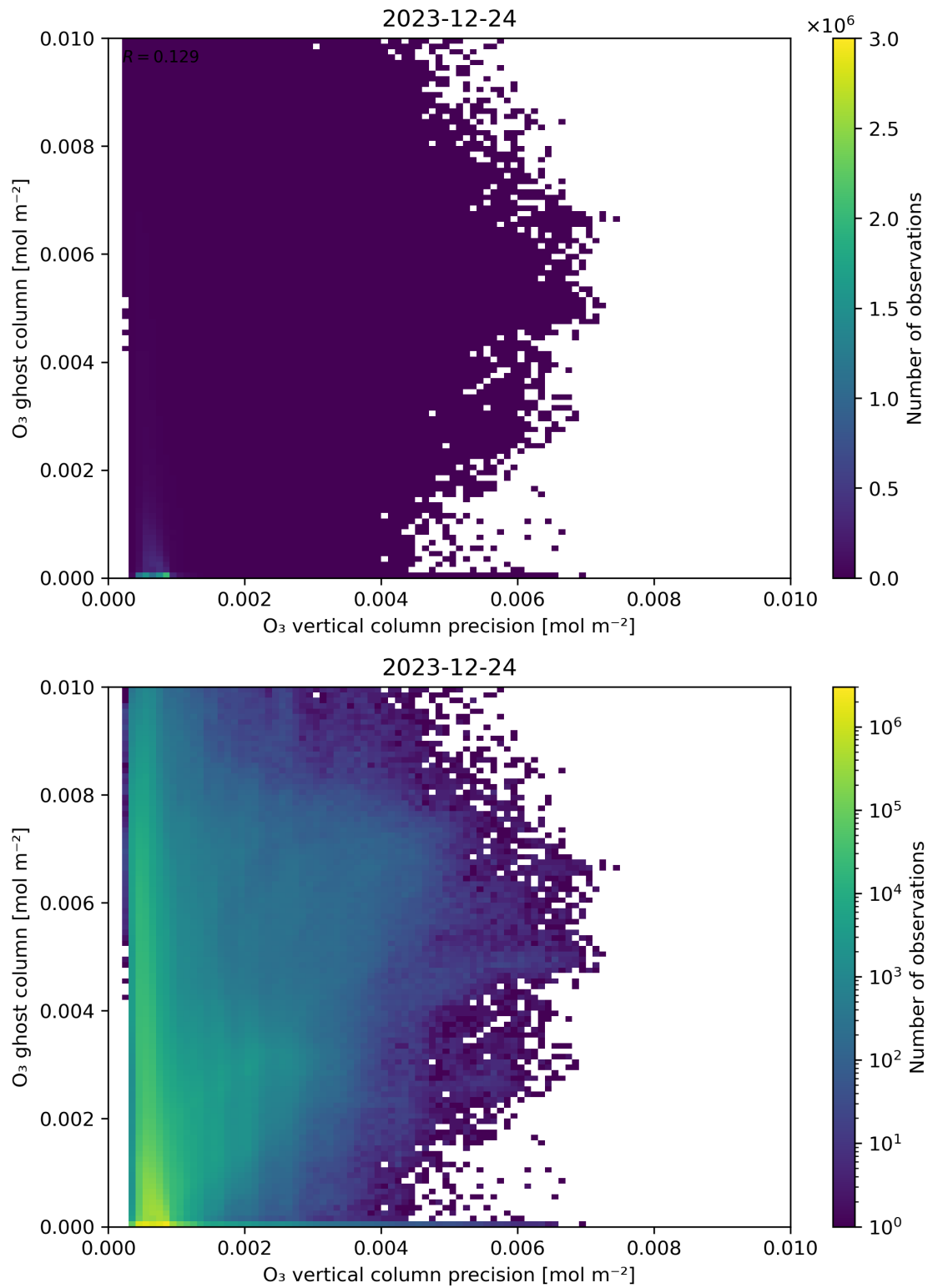
Figure 43: Scatter density plot of “ O_3 vertical column precision” against “ O_3 ghost column” for 2023-12-23 to 2023-12-25.
