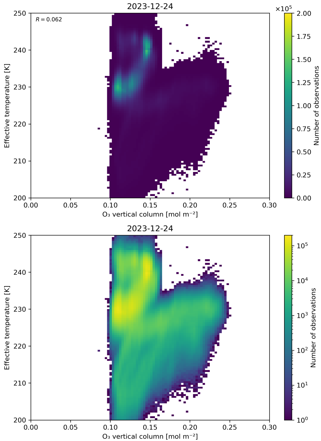
Figure 39: Scatter density plot of “O 3 vertical column” against “Effective temperature” for 2023-12-23 to 2023-12-25.
