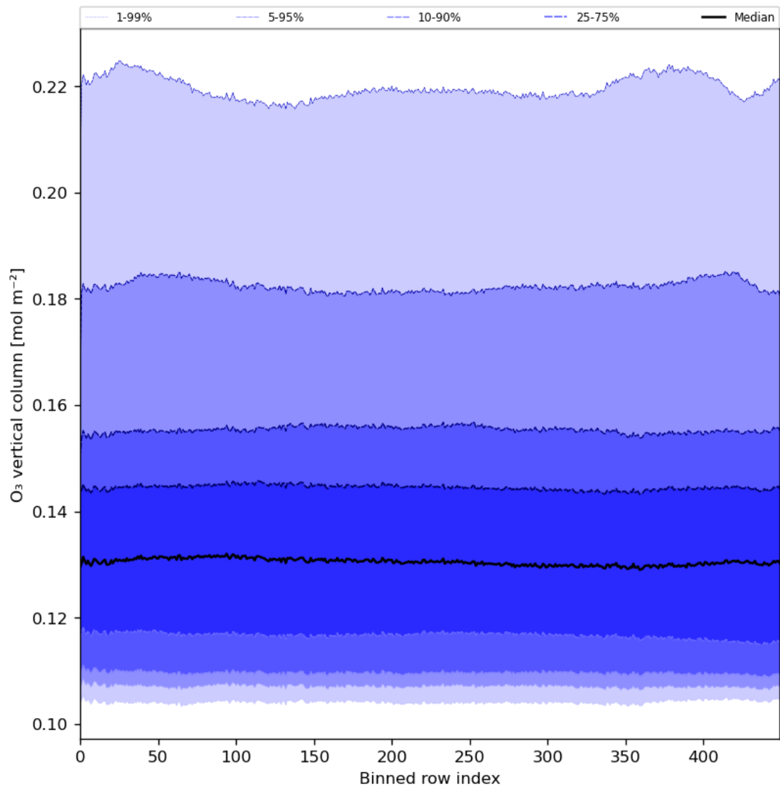
Figure 28: Along track statistics of “O 3 vertical column” for 2023-12-23 to 2023-12-25
