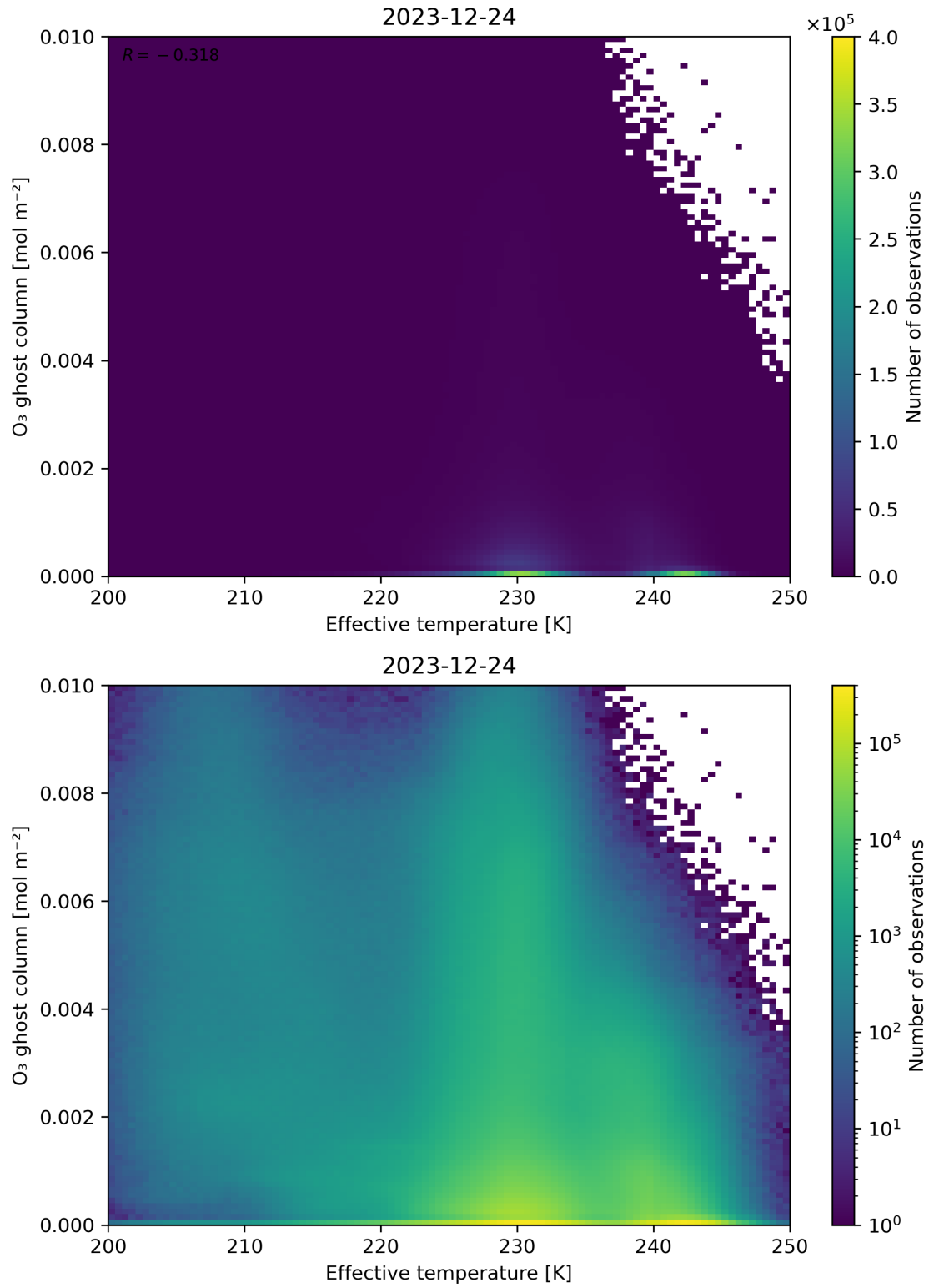
Figure 38: Scatter density plot of “Effective temperature” against “O 3 ghost column” for 2023-12-23 to 2023-12-25.
