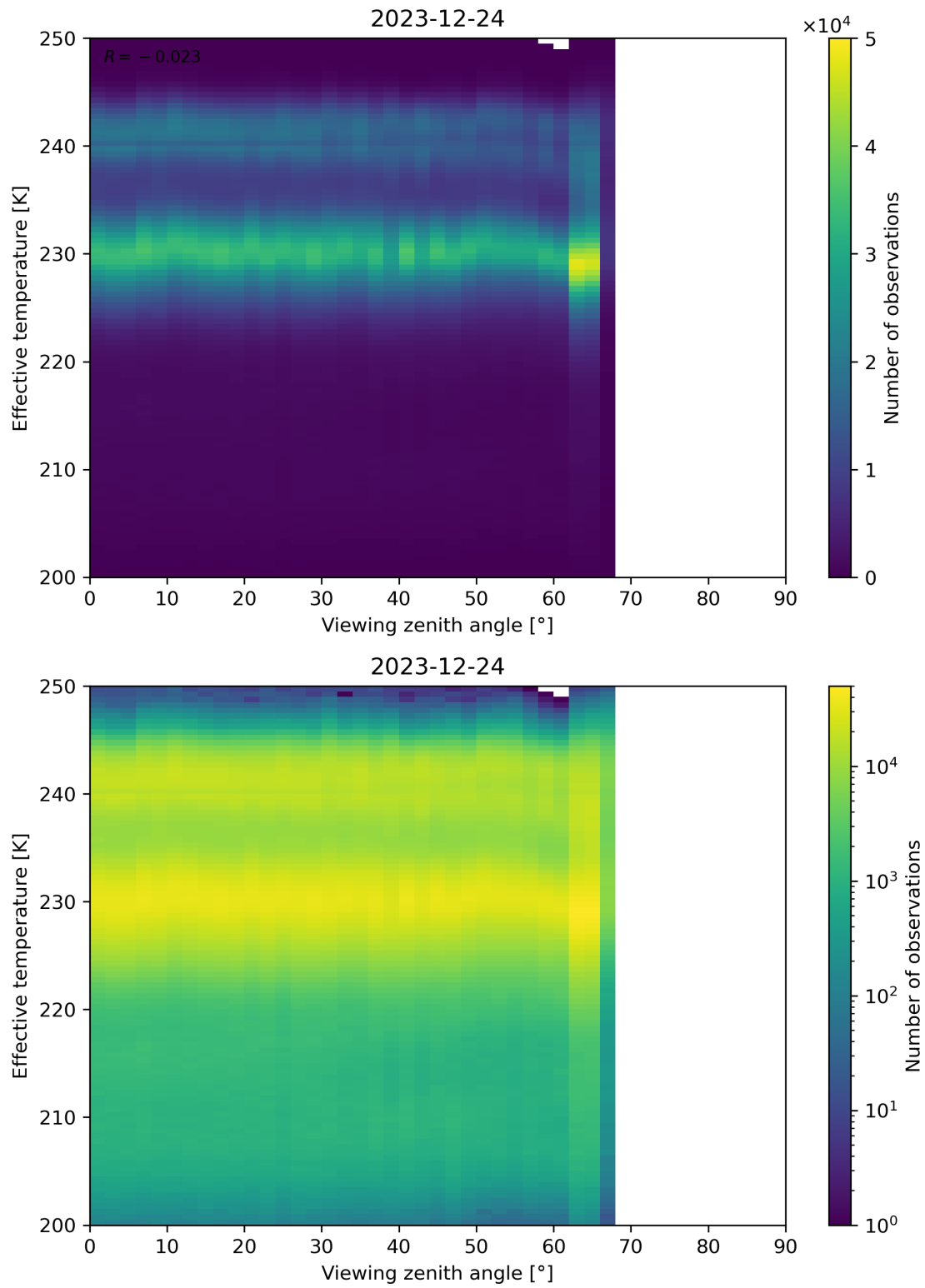
Figure 50: Scatter density plot of “Viewing zenith angle” against “Effective temperature” for 2023-12-23 to 2023-12-25.
