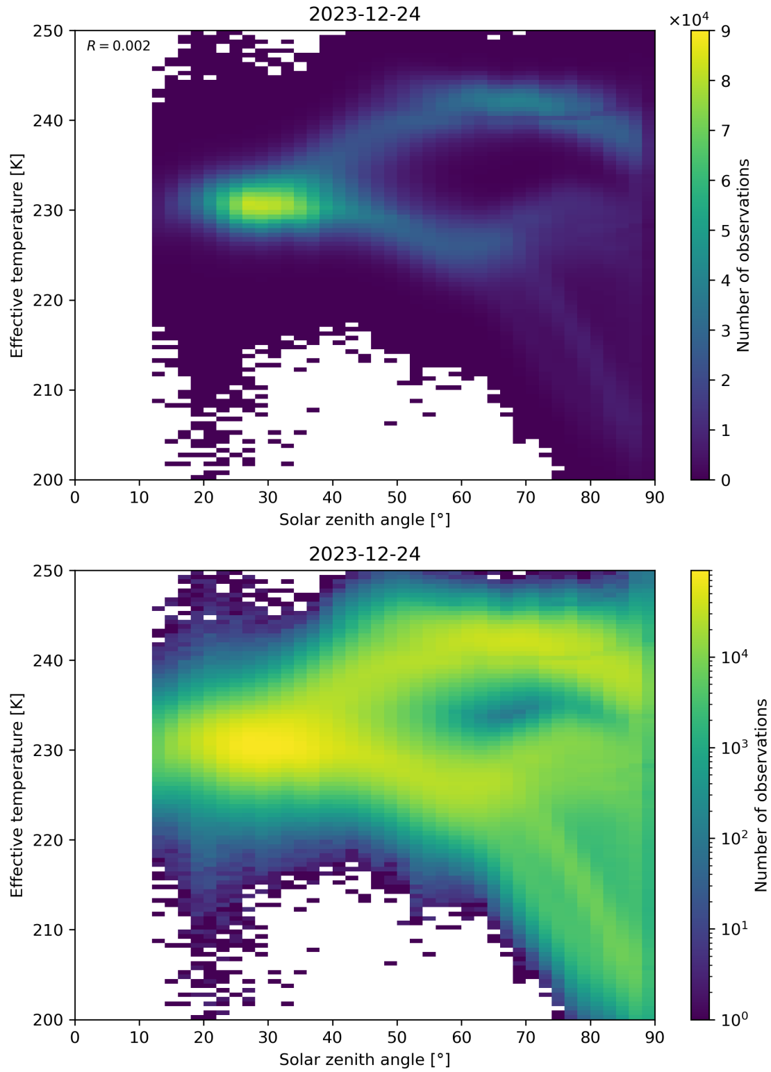
Figure 45: Scatter density plot of “Solar zenith angle” against “Effective temperature” for 2023-12-23 to 2023-12-25.
