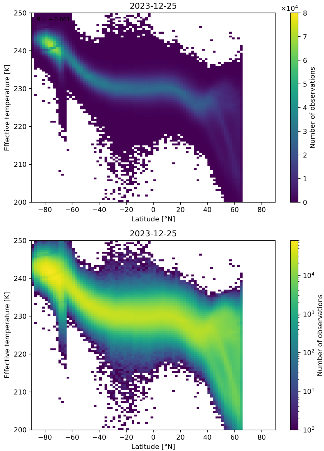
Figure 34: Scatter density plot of “Latitude” against “Effective temperature” for 2023-12-25 to 2023-12-26.
