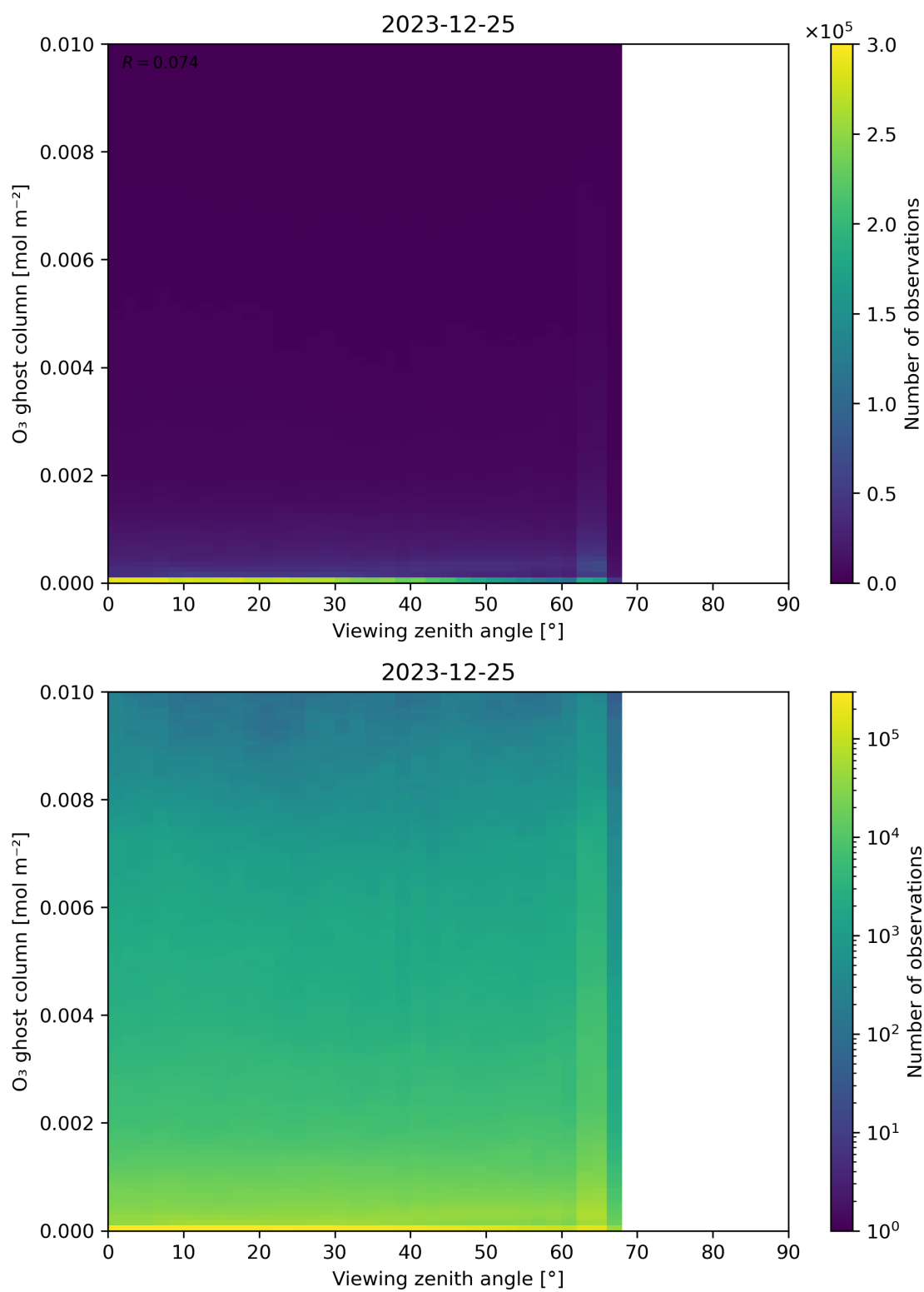
Figure 51: Scatter density plot of “Viewing zenith angle” against “O 3 ghost column” for 2023-12-25 to 2023-12-26.
