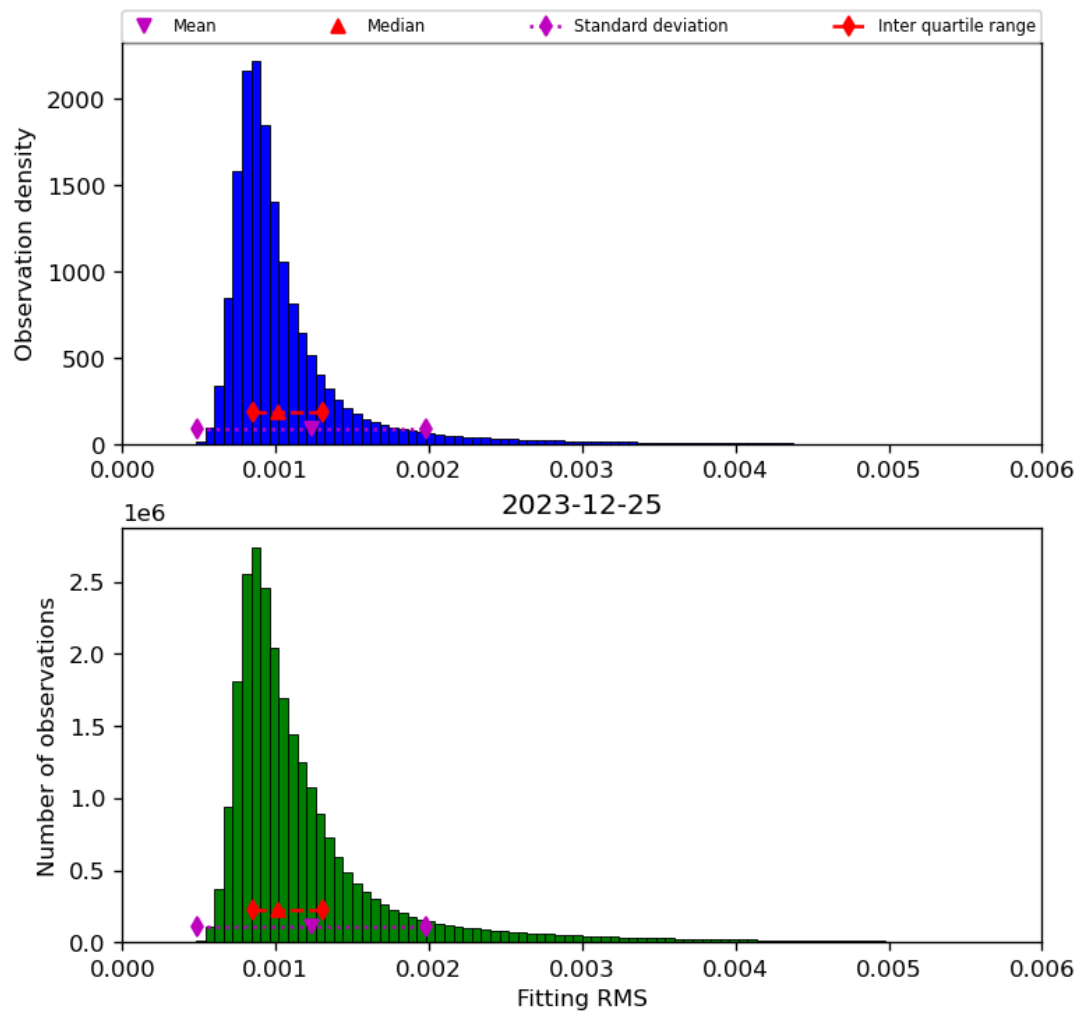
Figure 23: Histogram of “Fitting RMS” for 2023-12-25 to 2023-12-26
