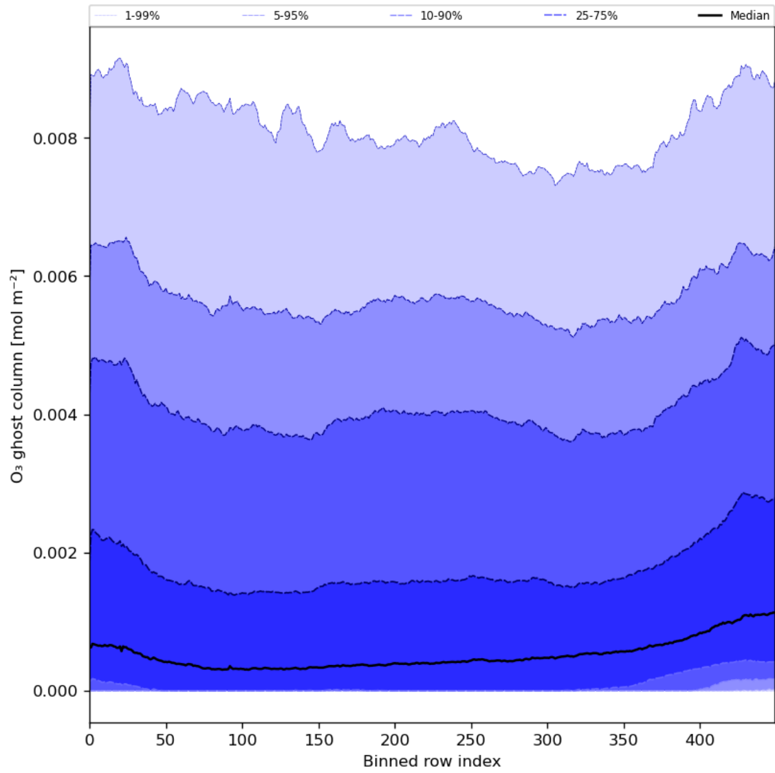
Figure 32: Along track statistics of “O 3 ghost column” for 2023-12-25 to 2023-12-26
