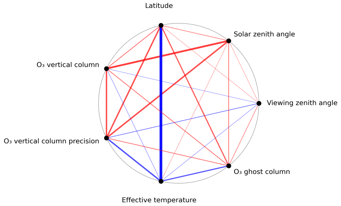
Figure 1: Map of correlation graph for 2023-12-25 to 2023-12-26.
