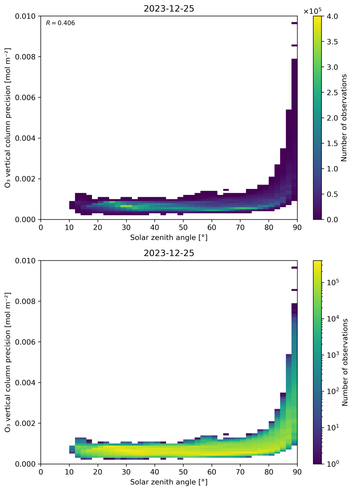
Figure 48: Scatter density plot of “Solar zenith angle” against “O 3 vertical column precision” for 2023-12-25 to 2023-12-26.
