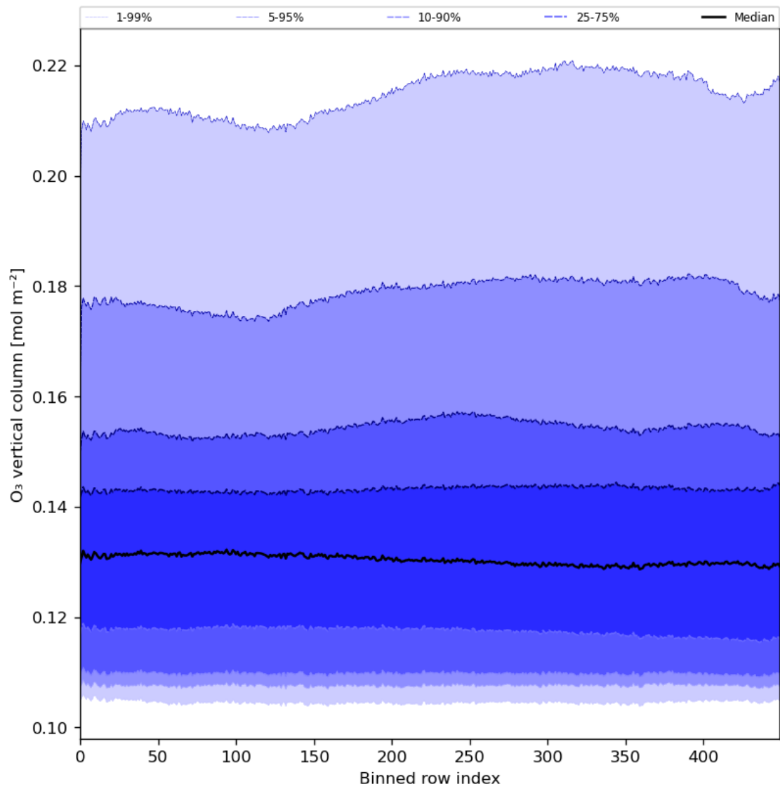
Figure 28: Along track statistics of “O 3 vertical column” for 2023-12-25 to 2023-12-26
