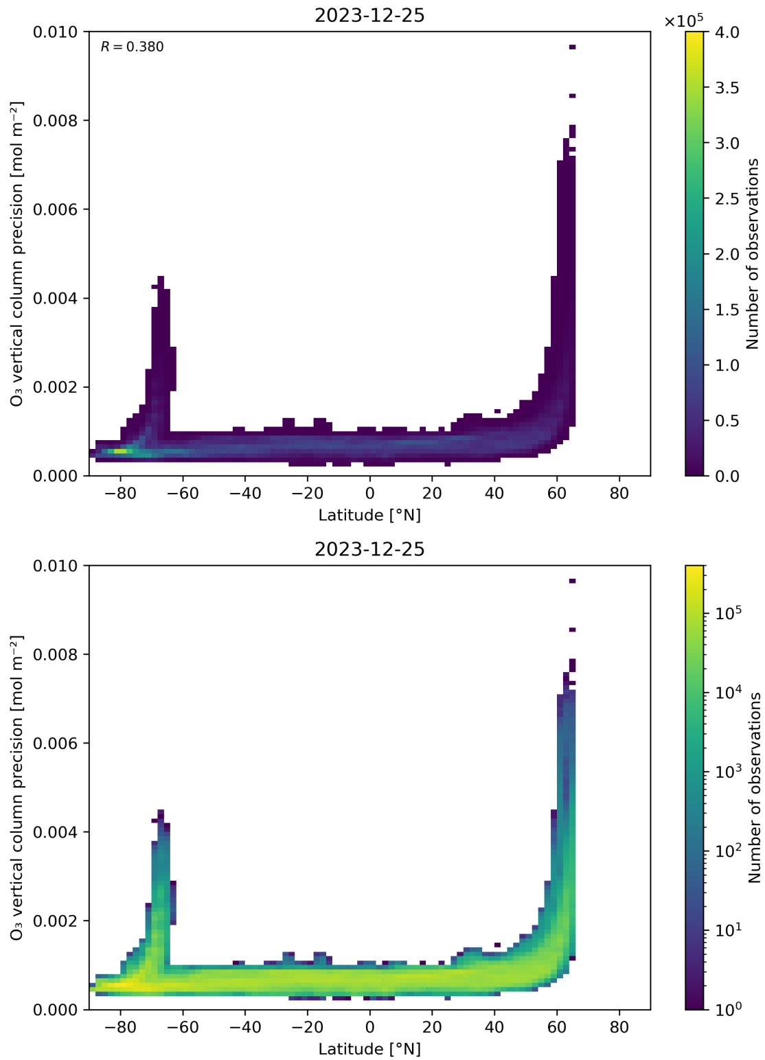
Figure 37: Scatter density plot of “Latitude” against “O 3 vertical column precision” for 2023-12-25 to 2023-12-26.
