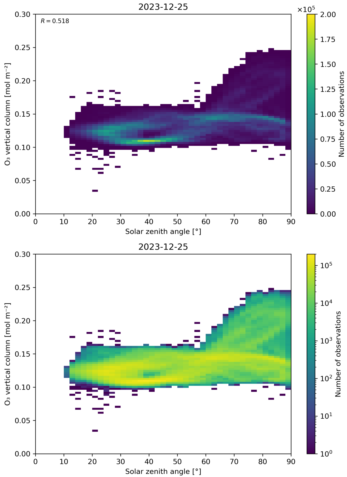
Figure 47: Scatter density plot of “Solar zenith angle” against “O 3 vertical column” for 2023-12-25 to 2023-12-26.
