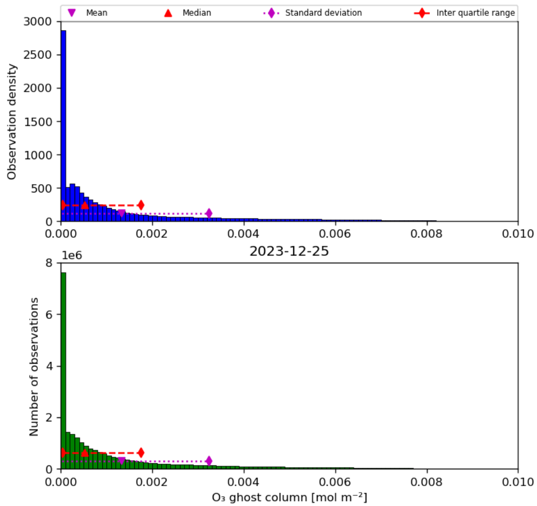
Figure 25: Histogram of “O 3 ghost column” for 2023-12-25 to 2023-12-26
