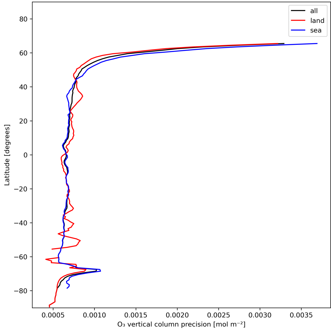
Figure 15: Zonal average of “O 3 vertical column precision” for 2023-12-25 to 2023-12-26.
