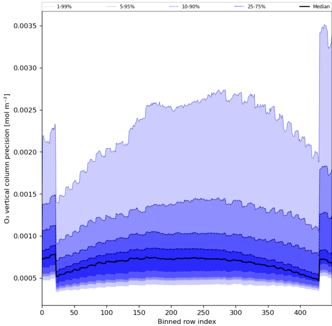
Figure 29: Along track statistics of “O 3 vertical column precision” for 2023-12-25 to 2023-12-26
