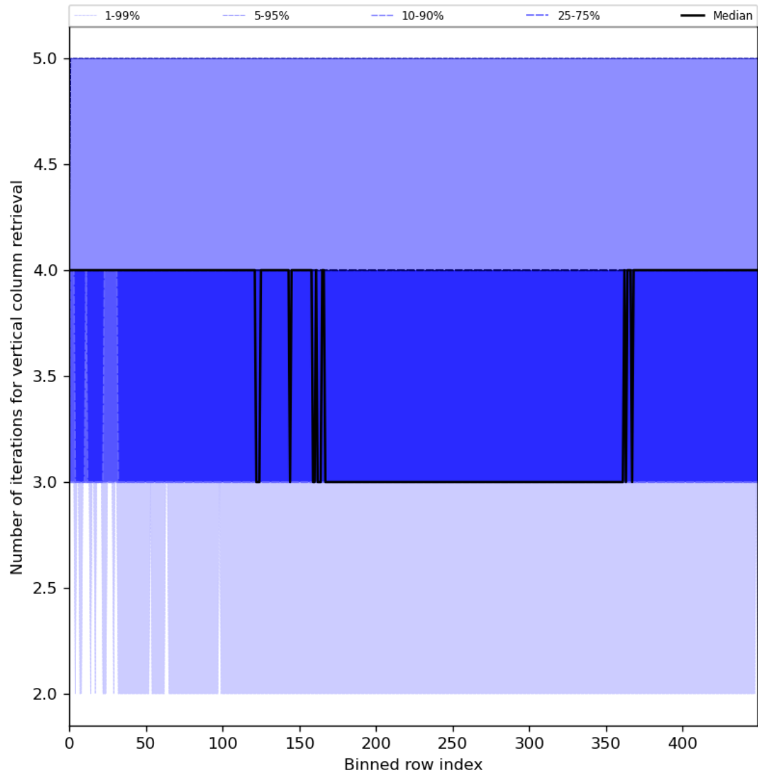
Figure 33: Along track statistics of “Number of iterations for vertical column retrieval” for 2023-12-25 to 2023-12-26
