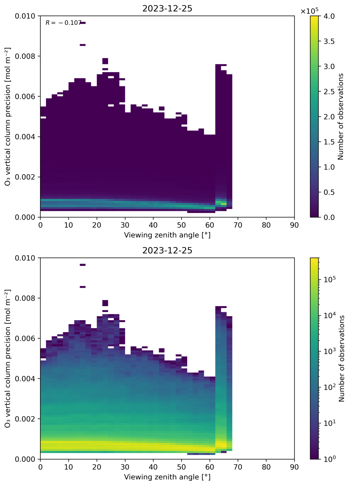
Figure 53: Scatter density plot of “Viewing zenith angle” against “O 3 vertical column precision” for 2023-12-25 to 2023-12-26.
