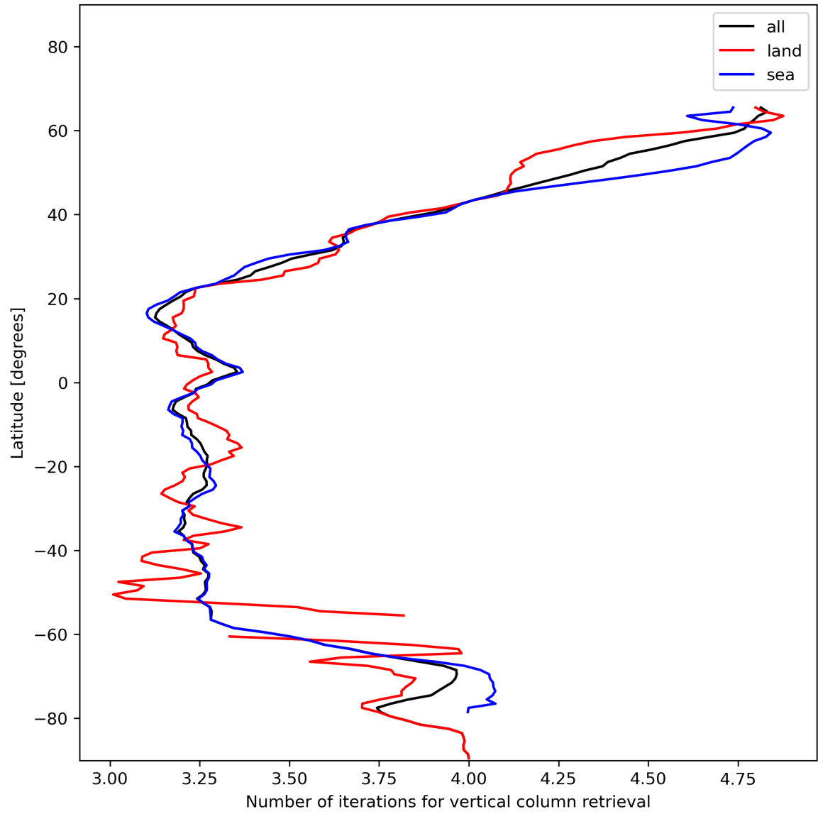
Figure 19: Zonal average of “Number of iterations for vertical column retrieval” for 2023-12-25 to 2023-12-26.
