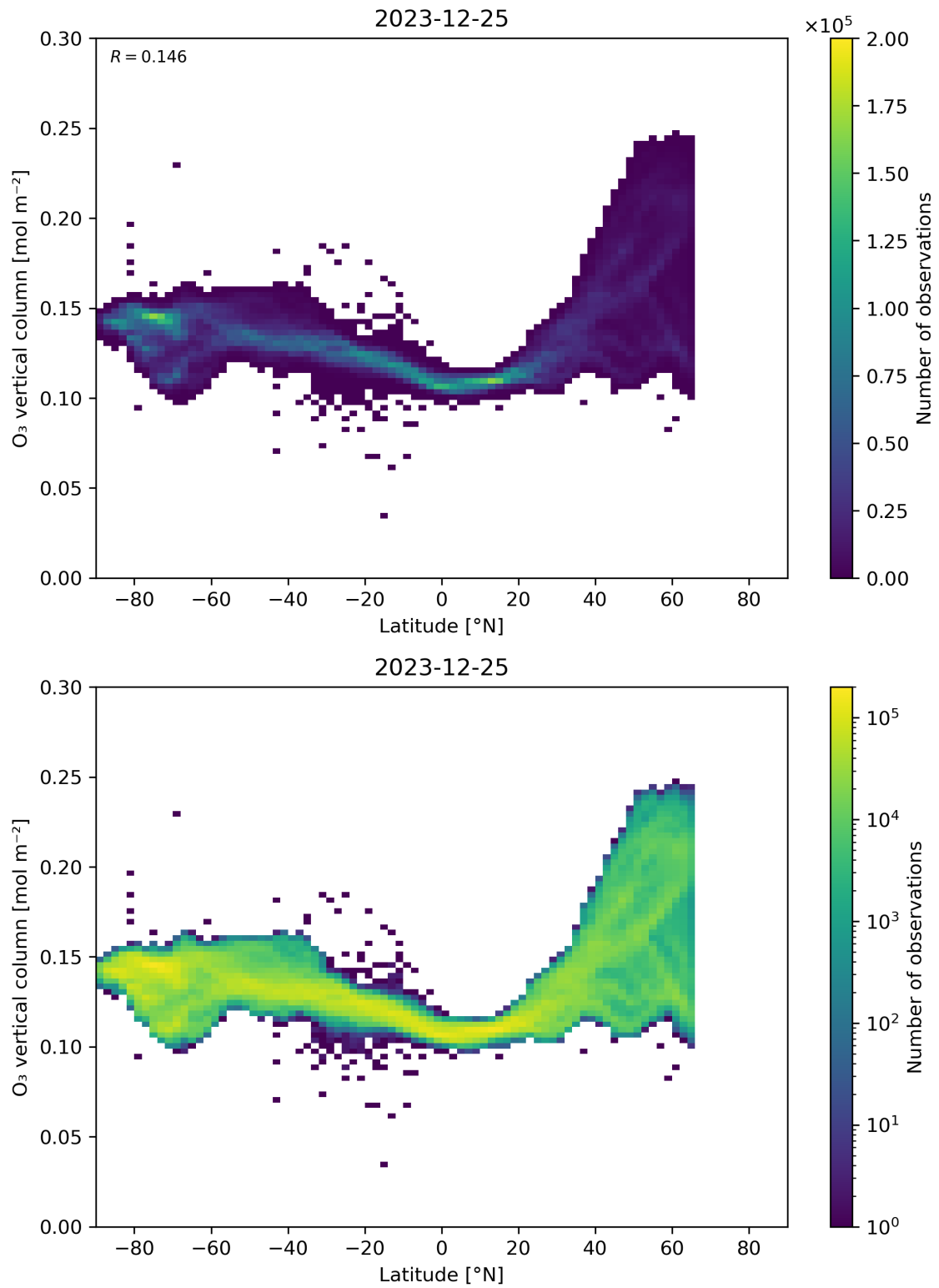
Figure 36: Scatter density plot of “Latitude” against “O 3 vertical column” for 2023-12-25 to 2023-12-26.
