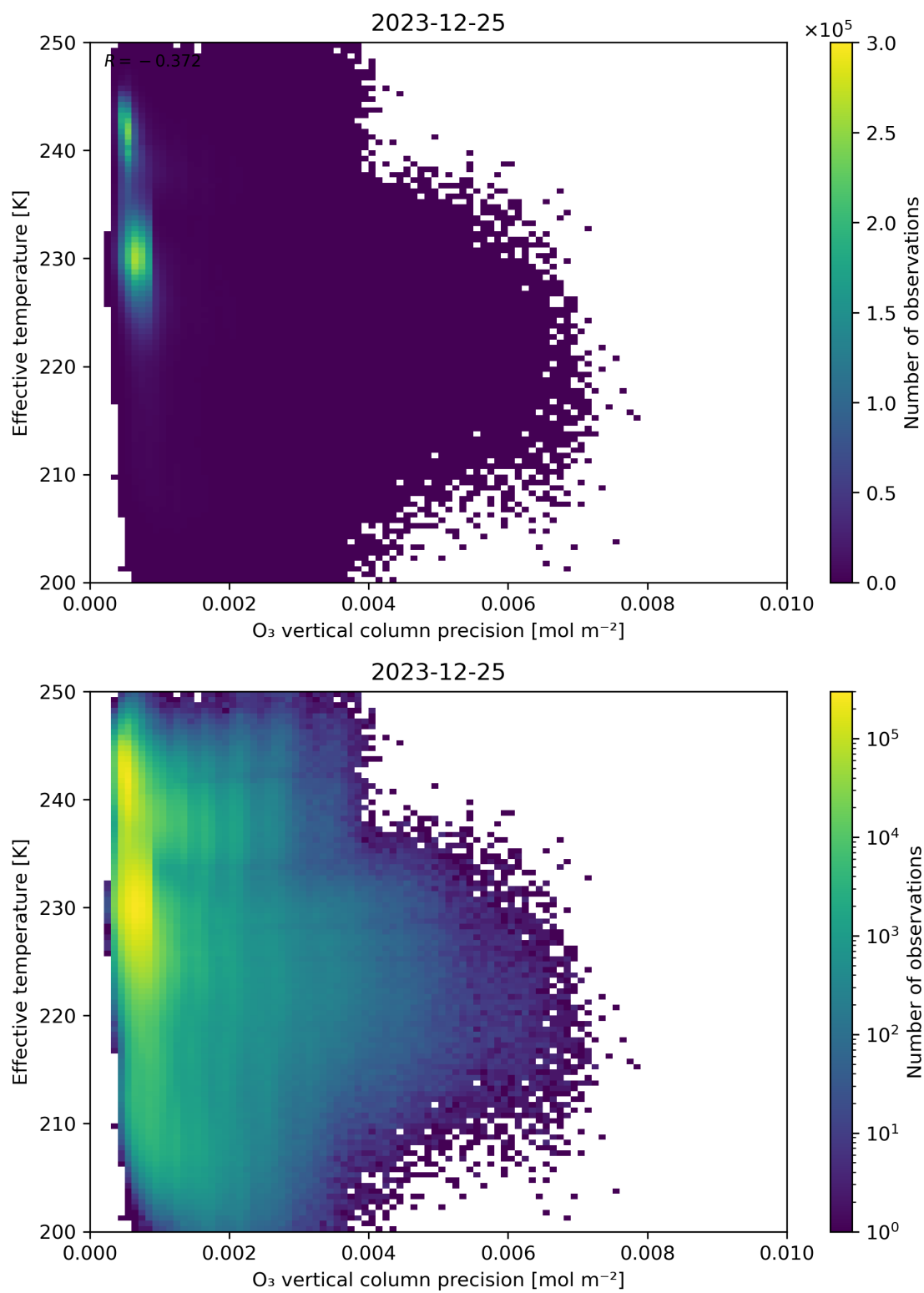
Figure 42: Scatter density plot of “O 3 vertical column precision” against “Effective temperature” for 2023-12-25 to 2023-12-26.
