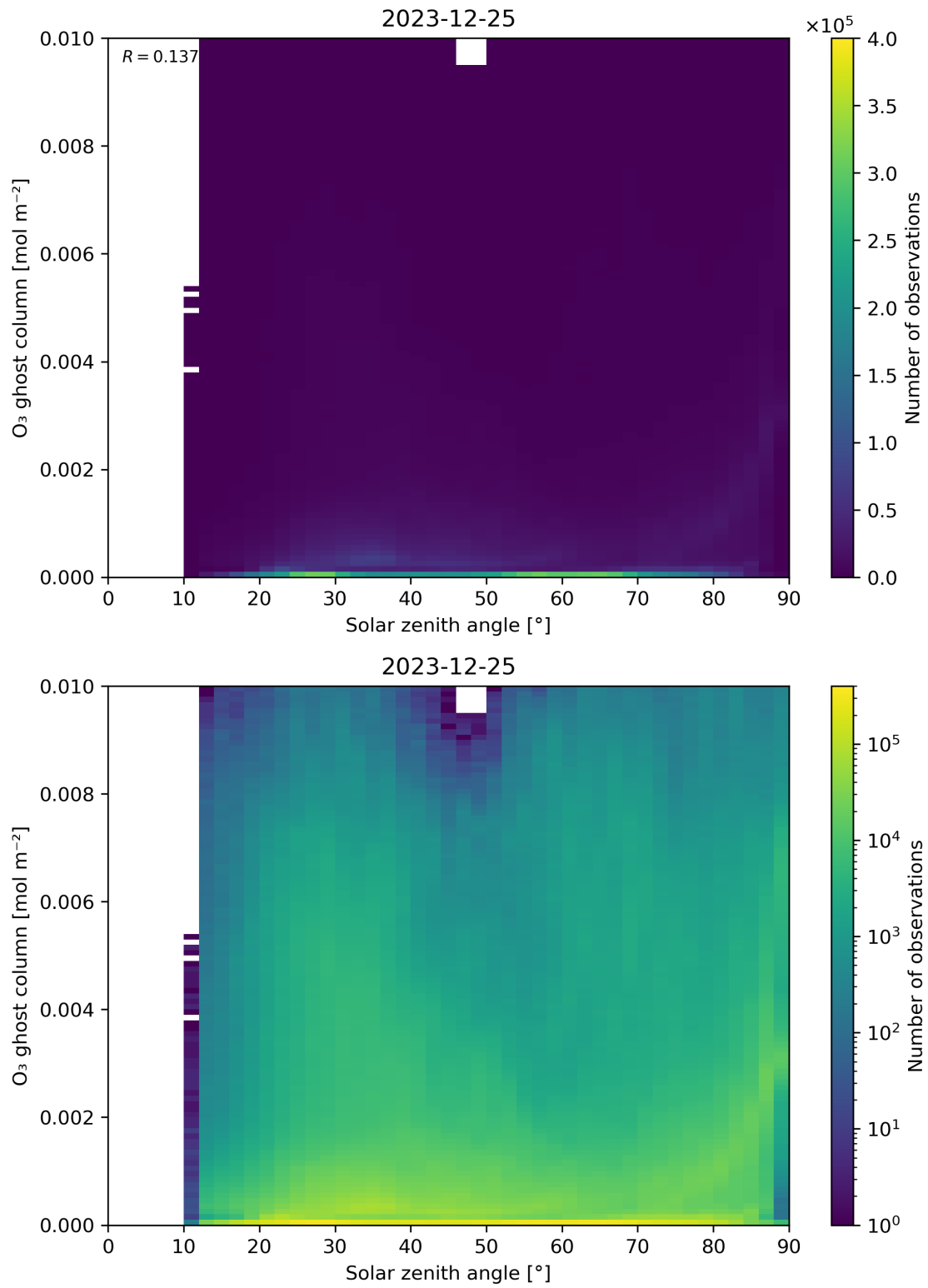
Figure 46: Scatter density plot of “Solar zenith angle” against “O 3 ghost column” for 2023-12-25 to 2023-12-26.
