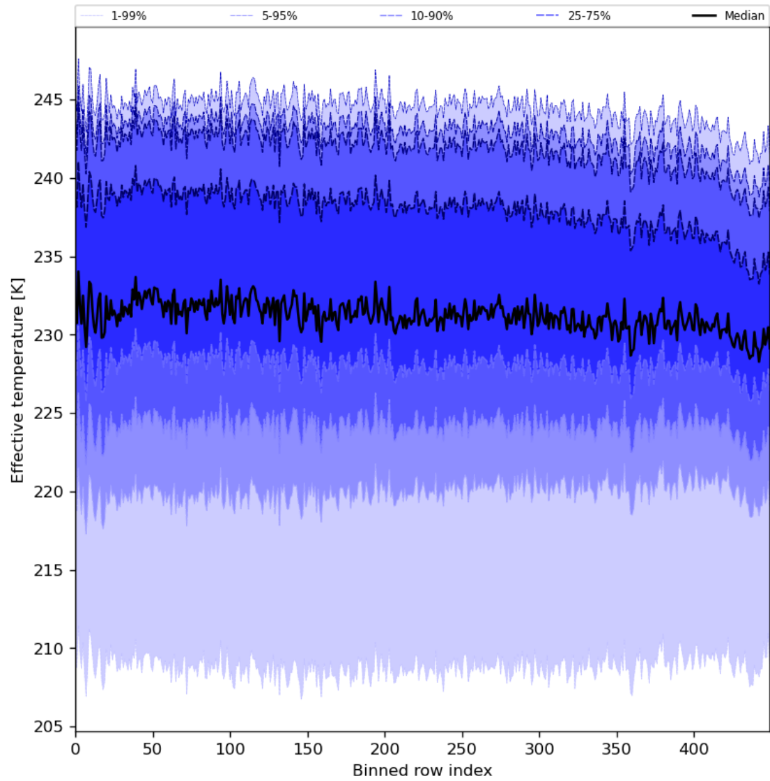
Figure 31: Along track statistics of “Effective temperature” for 2023-12-25 to 2023-12-26
