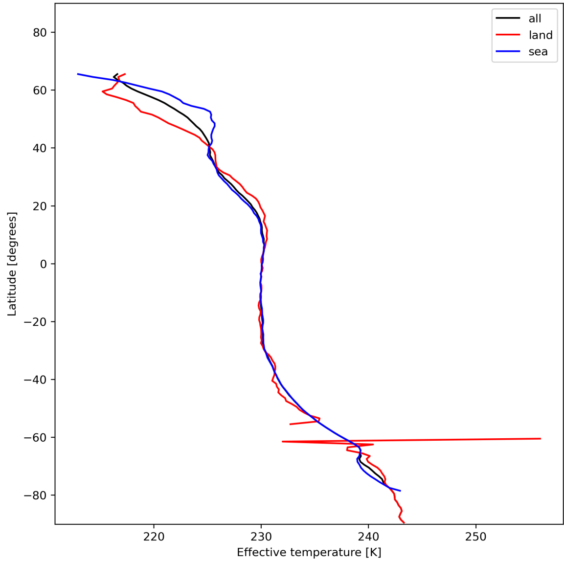
Figure 17: Zonal average of “Effective temperature” for 2023-12-25 to 2023-12-26.
