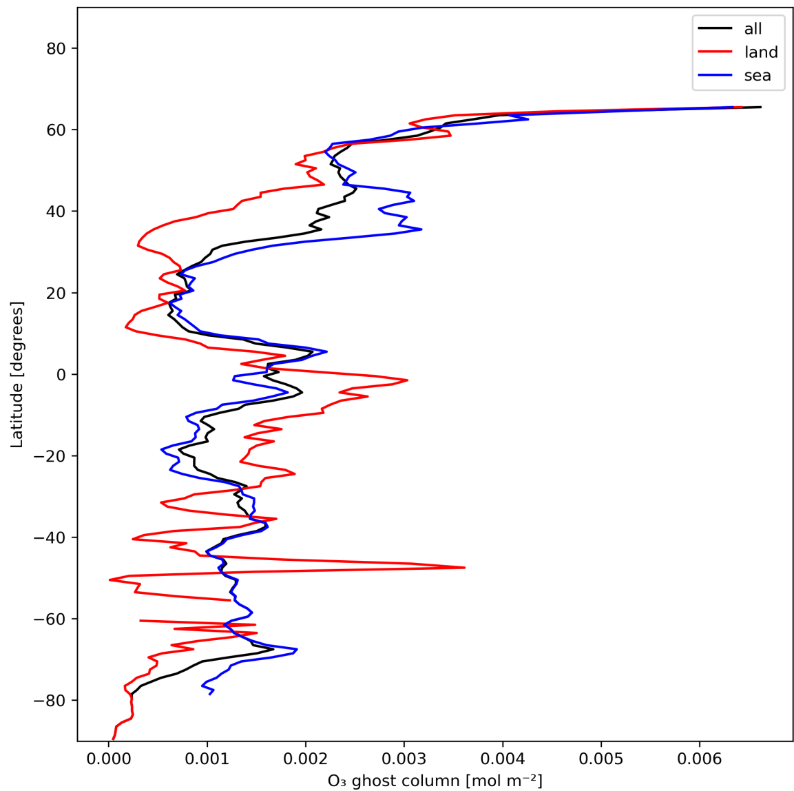
Figure 18: Zonal average of “O 3 ghost column” for 2023-12-25 to 2023-12-26.
