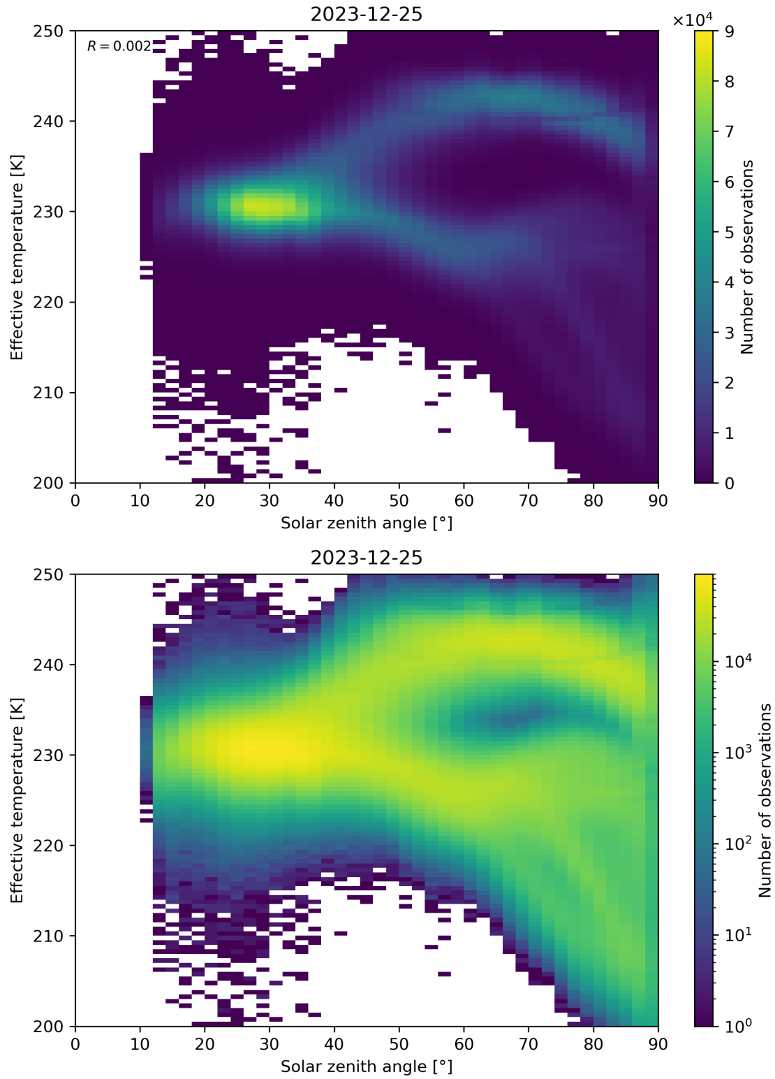
Figure 45: Scatter density plot of “Solar zenith angle” against “Effective temperature” for 2023-12-25 to 2023-12-26.
