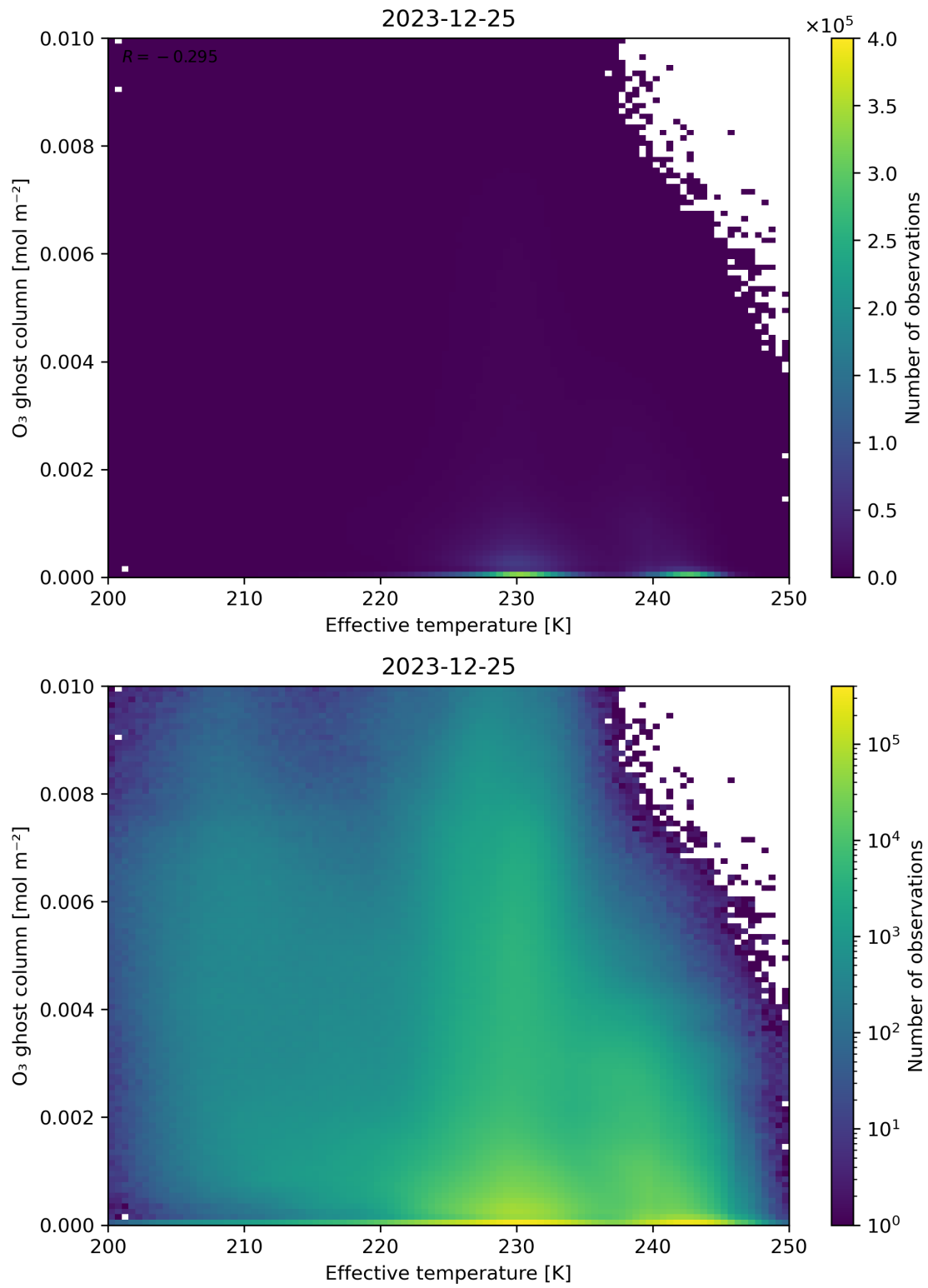
Figure 38: Scatter density plot of “Effective temperature” against “O 3 ghost column” for 2023-12-25 to 2023-12-26.
