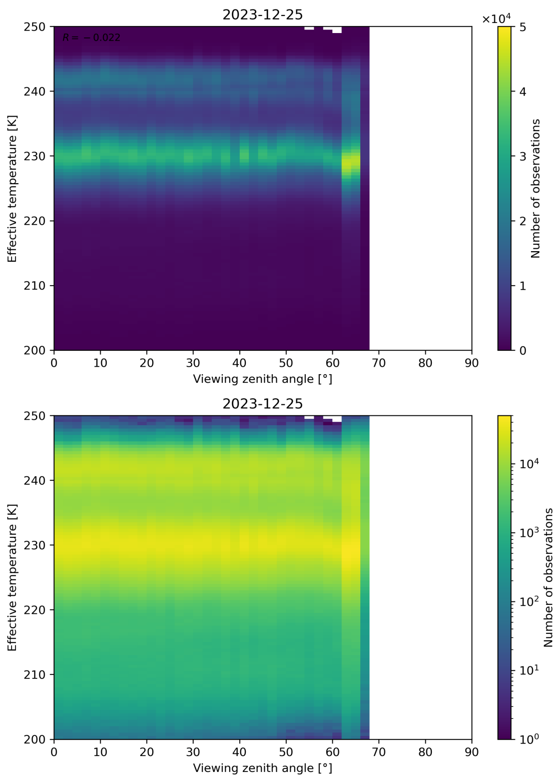
Figure 50: Scatter density plot of “Viewing zenith angle” against “Effective temperature” for 2023-12-25 to 2023-12-26.
