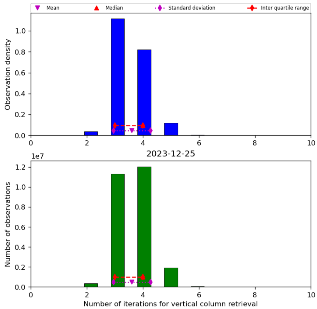
Figure 26: Histogram of “Number of iterations for vertical column retrieval” for 2023-12-25 to 2023-12-26
