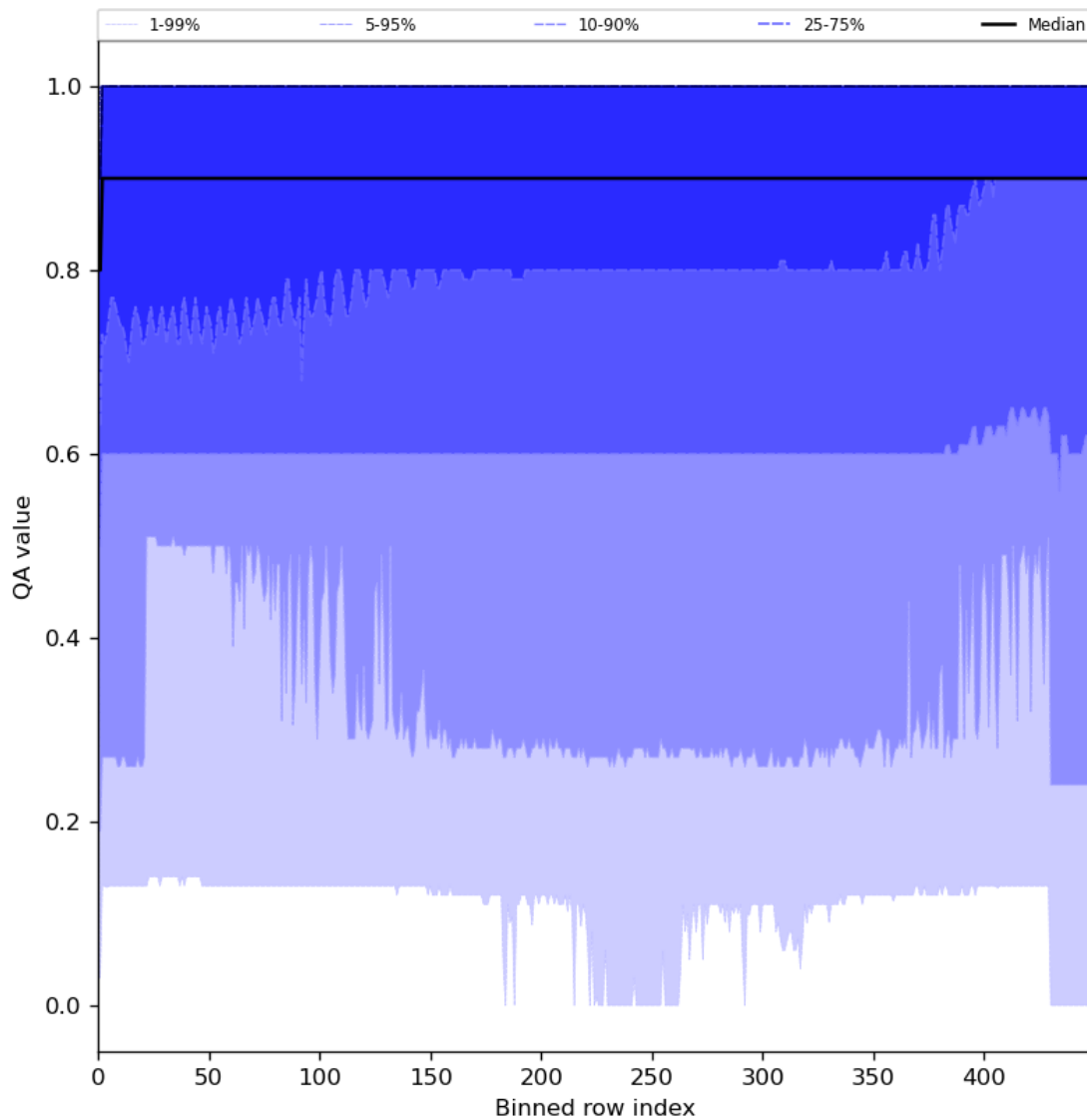
Figure 27: Along track statistics of “QA value” for 2023-12-25 to 2023-12-26
