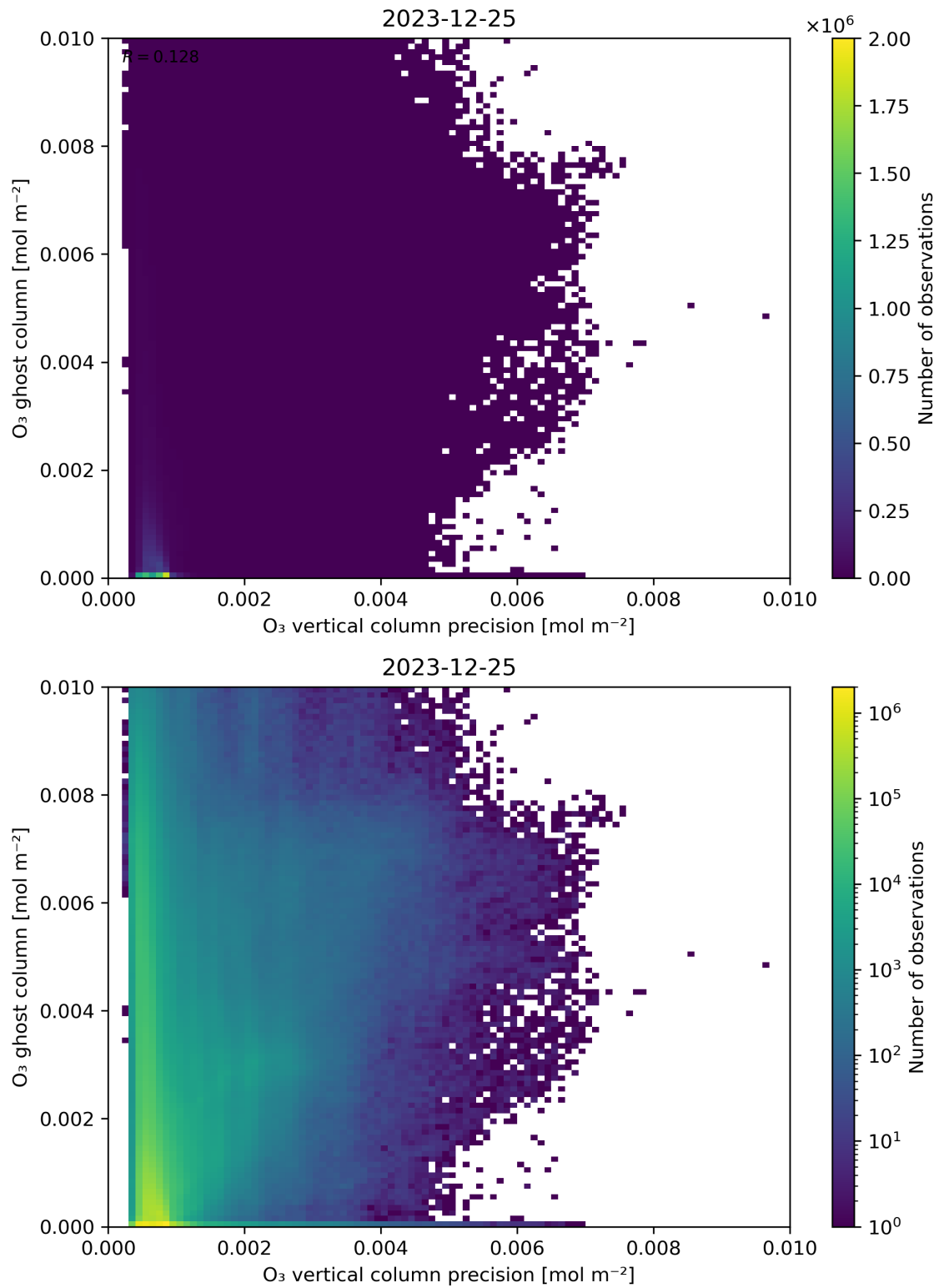
Figure 43: Scatter density plot of “O 3 vertical column precision” against “O 3 ghost column” for 2023-12-25 to 2023-12-26.
