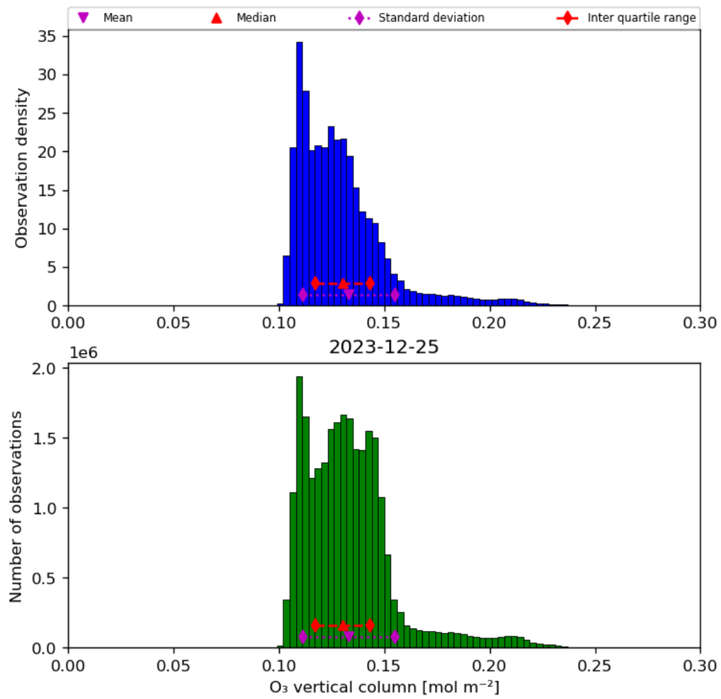
Figure 21: Histogram of “O 3 vertical column” for 2023-12-25 to 2023-12-26
