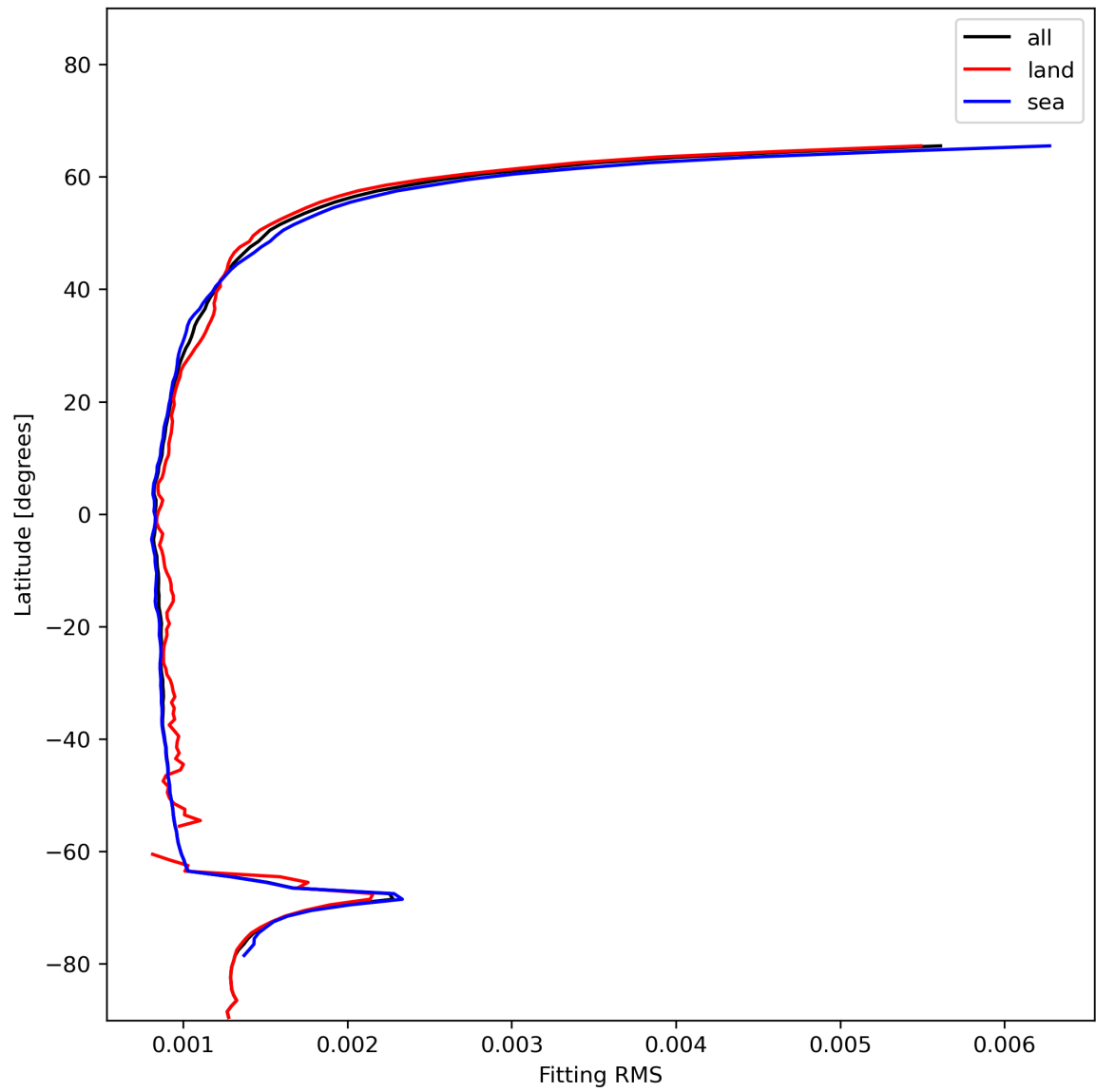
Figure 16: Zonal average of “Fitting RMS” for 2023-12-25 to 2023-12-26.
