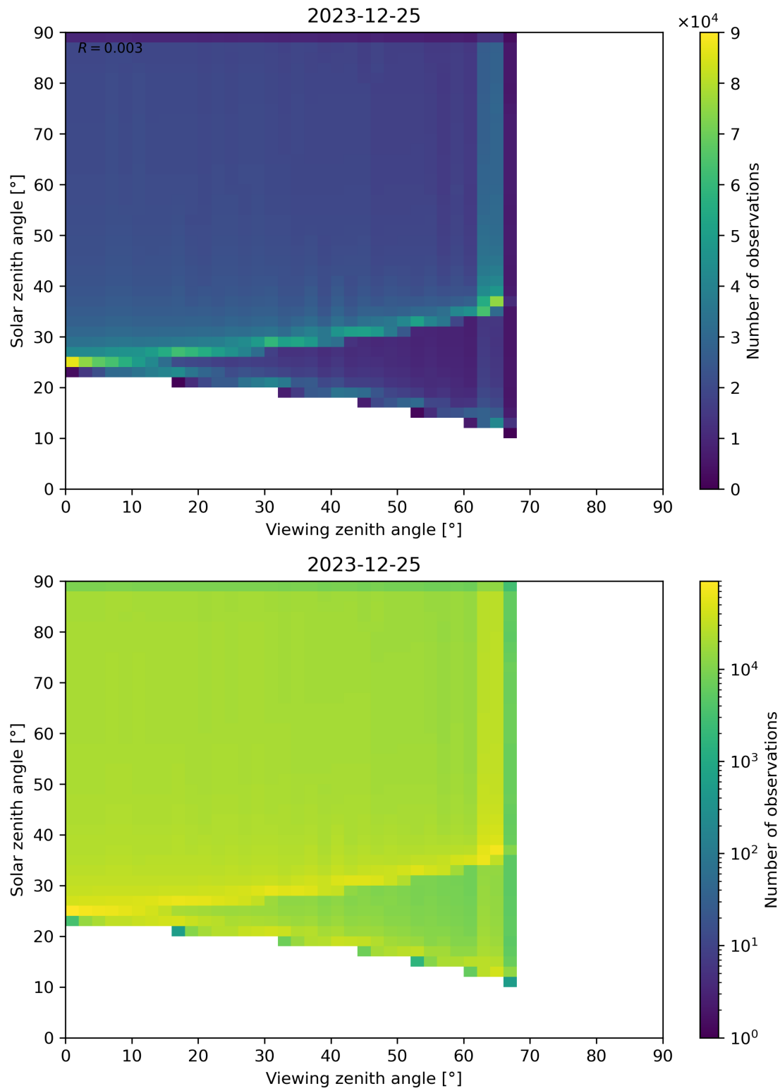
Figure 54: Scatter density plot of “Viewing zenith angle” against “Solar zenith angle” for 2023-12-25 to 2023-12-26.
