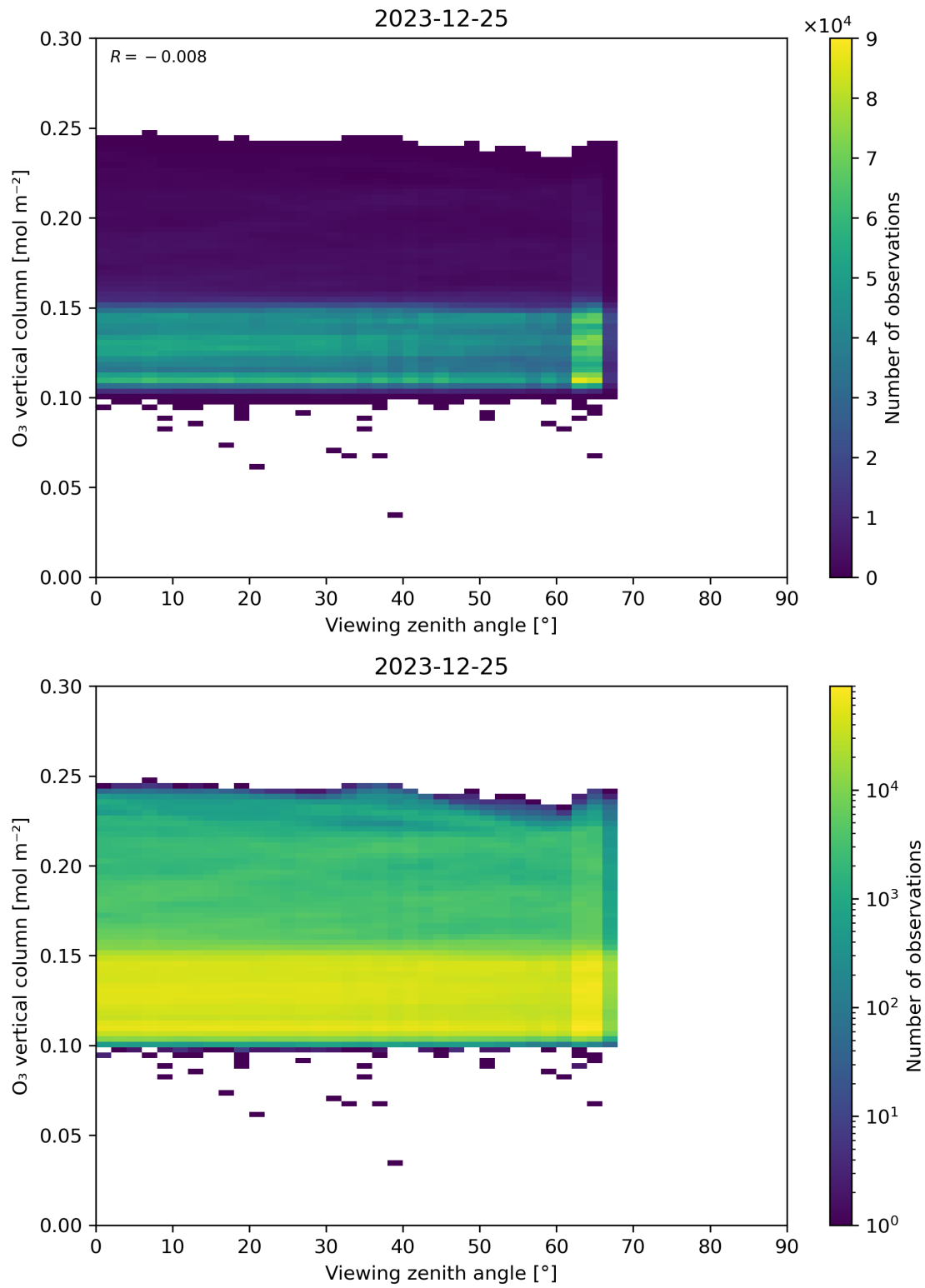
Figure 52: Scatter density plot of “Viewing zenith angle” against “O 3 vertical column” for 2023-12-25 to 2023-12-26.
