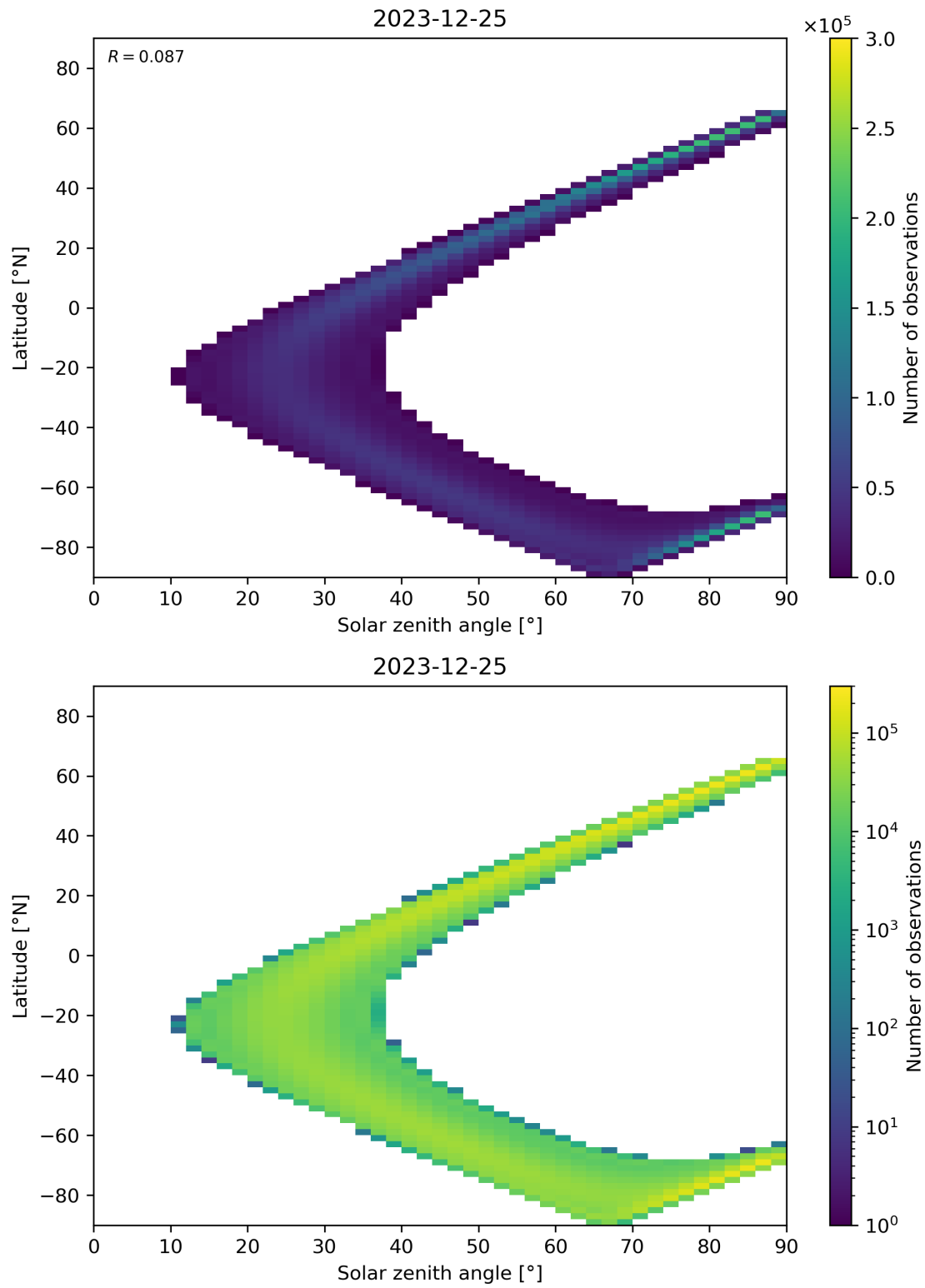
Figure 44: Scatter density plot of “Solar zenith angle” against “Latitude” for 2023-12-25 to 2023-12-26.
