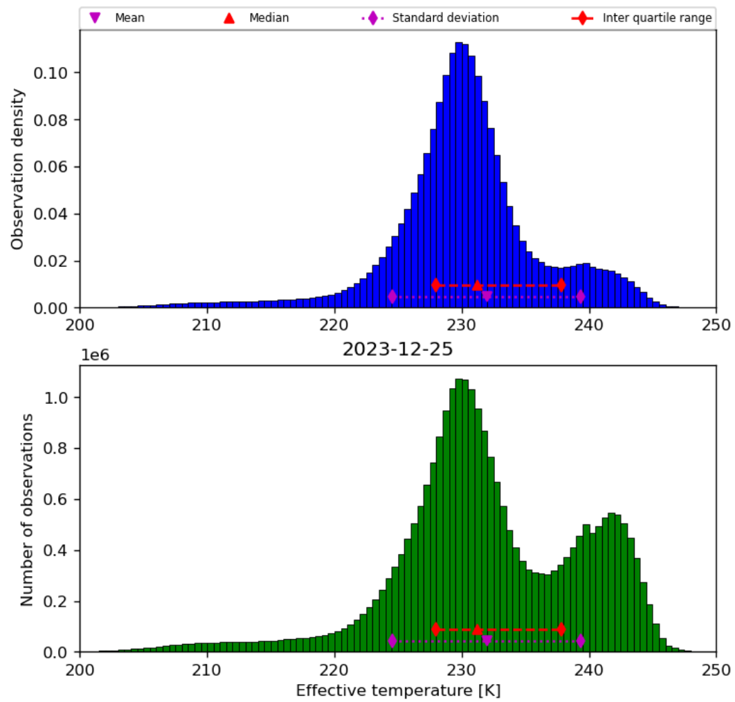
Figure 24: Histogram of “Effective temperature” for 2023-12-25 to 2023-12-26
