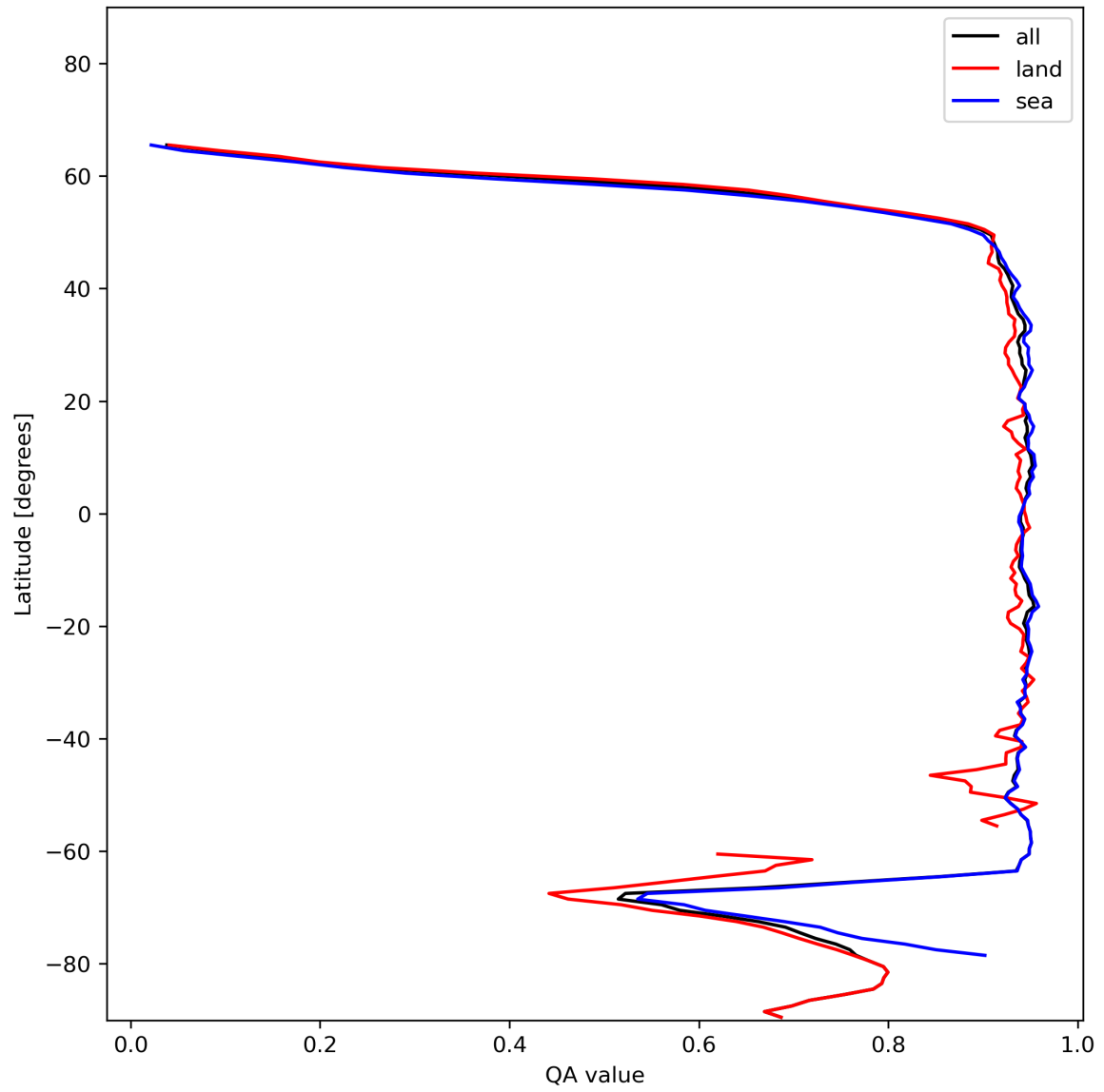
Figure 13: Zonal average of “QA value” for 2023-12-25 to 2023-12-26.
