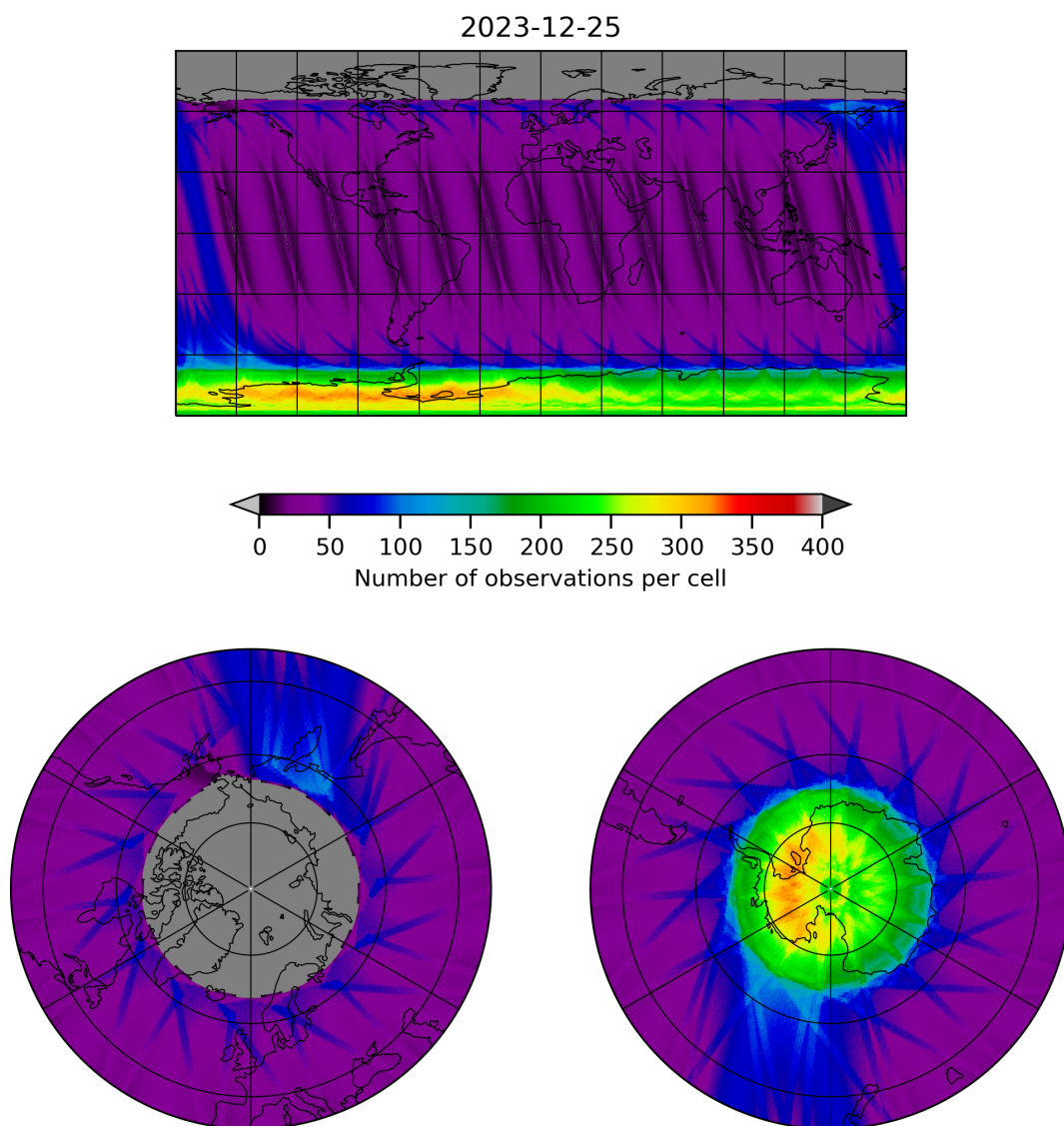
Figure 12: Map of the number of observations for 2023-12-25 to 2023-12-26
