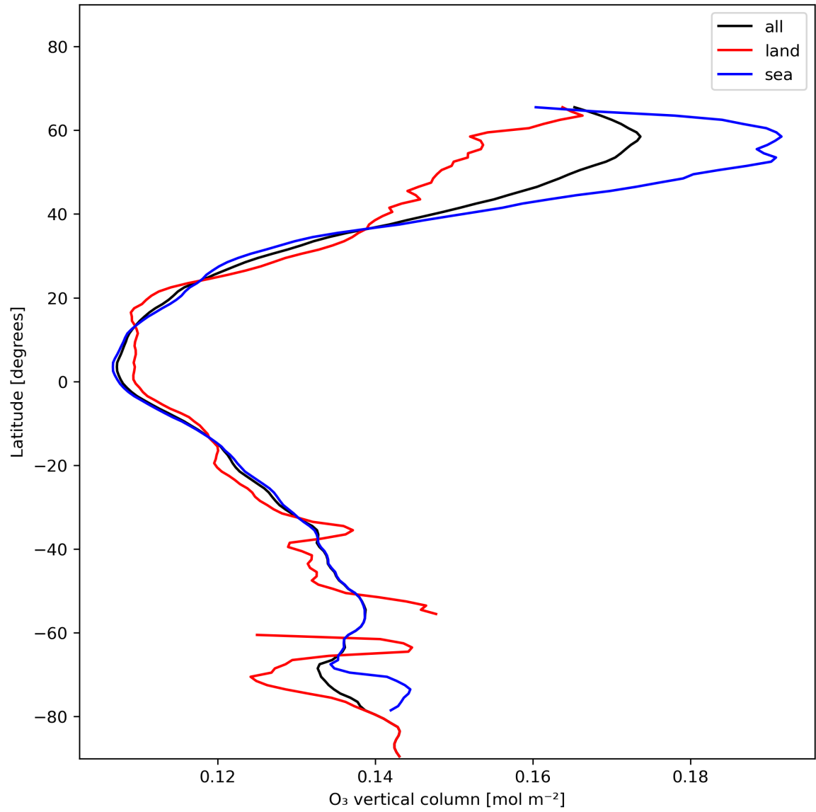
Figure 14: Zonal average of “O 3 vertical column” for 2023-12-25 to 2023-12-26.
