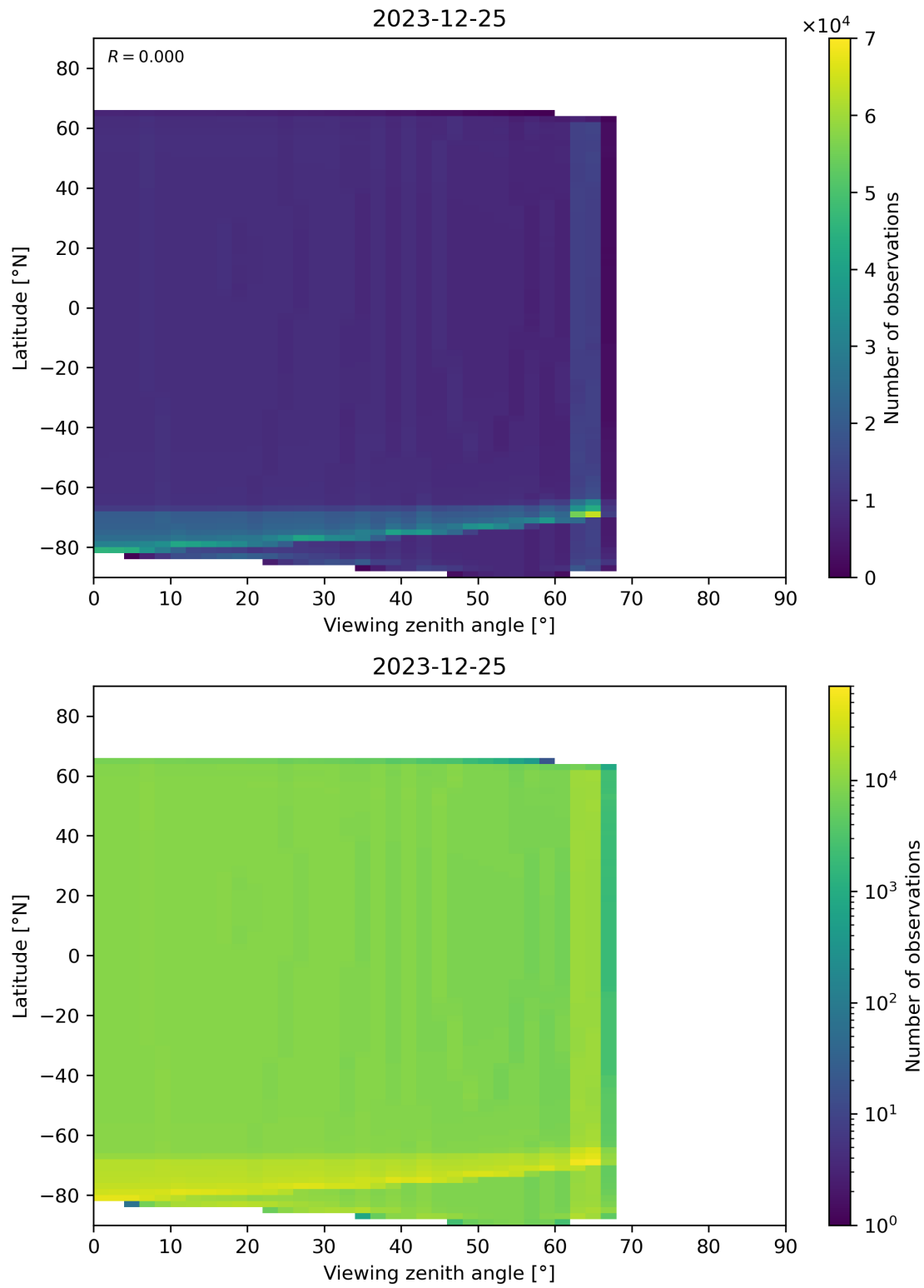
Figure 49: Scatter density plot of “Viewing zenith angle” against “Latitude” for 2023-12-25 to 2023-12-26.
