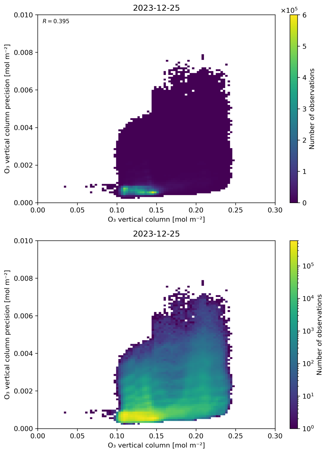
Figure 41: Scatter density plot of “O 3 vertical column” against “O 3 vertical column precision” for 2023-12-25 to 2023-12-26.
