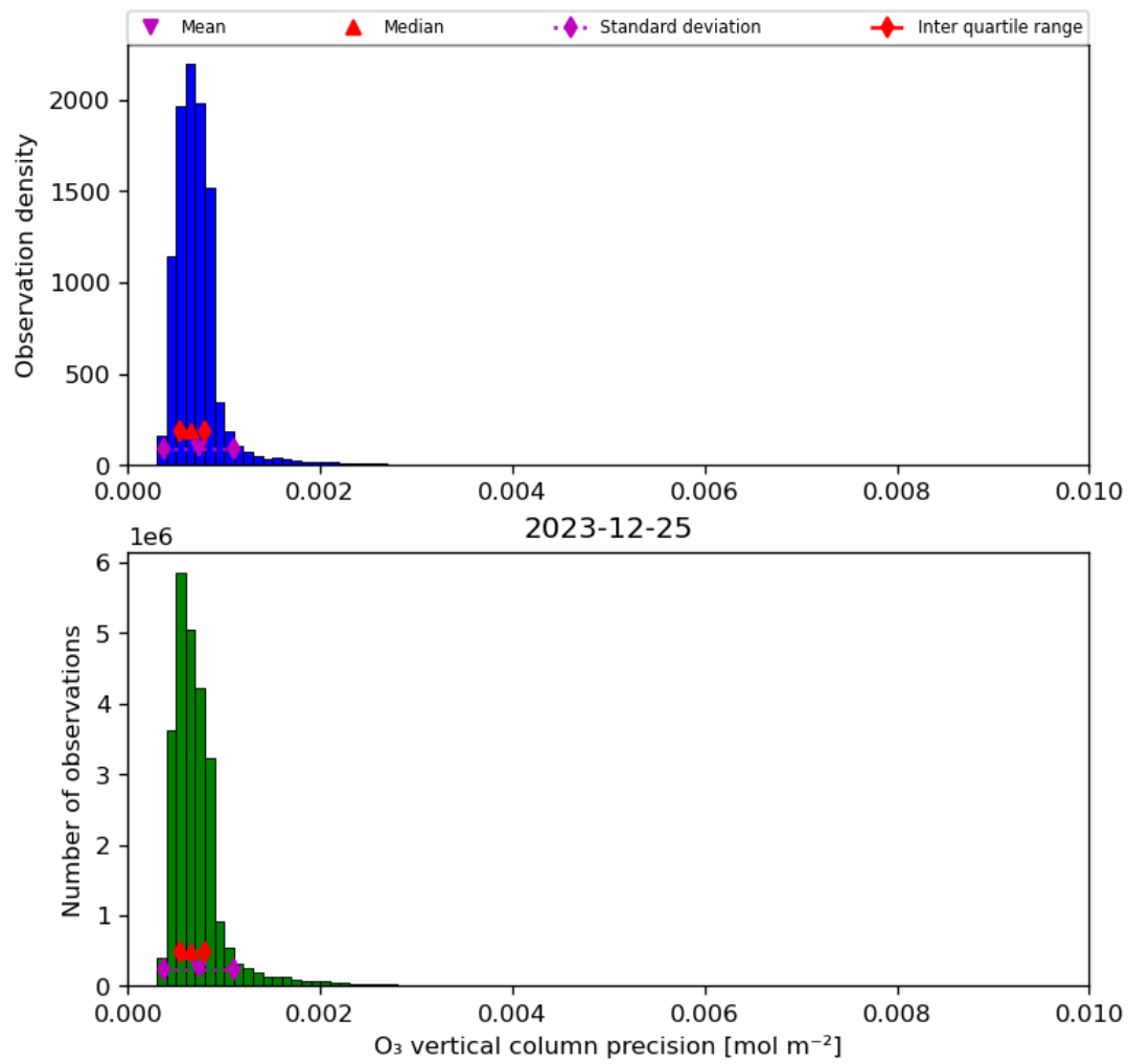
Figure 22: Histogram of “O 3 vertical column precision” for 2023-12-25 to 2023-12-26
