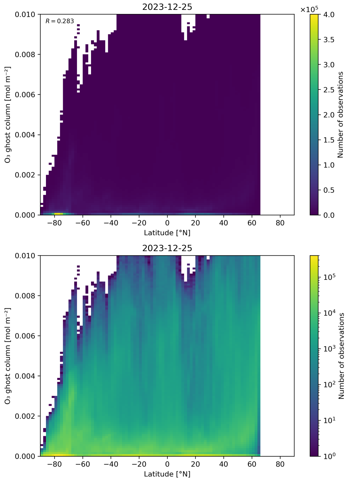
Figure 35: Scatter density plot of “Latitude” against “O 3 ghost column” for 2023-12-25 to 2023-12-26.
