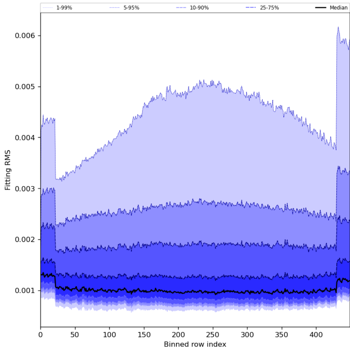
Figure 30: Along track statistics of “Fitting RMS” for 2023-12-25 to 2023-12-26
