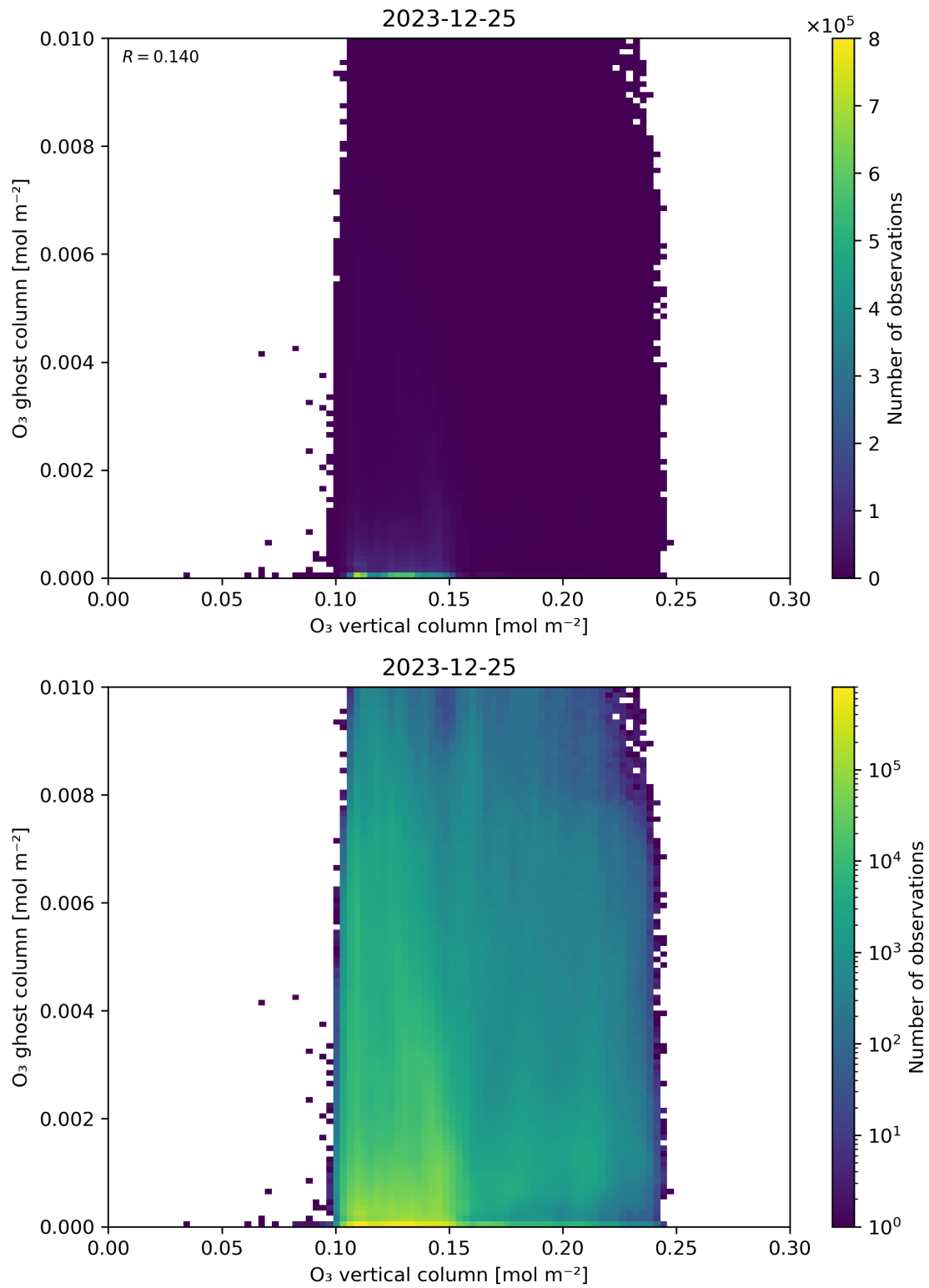
Figure 40: Scatter density plot of “O 3 vertical column” against “O 3 ghost column” for 2023-12-25 to 2023-12-26.
