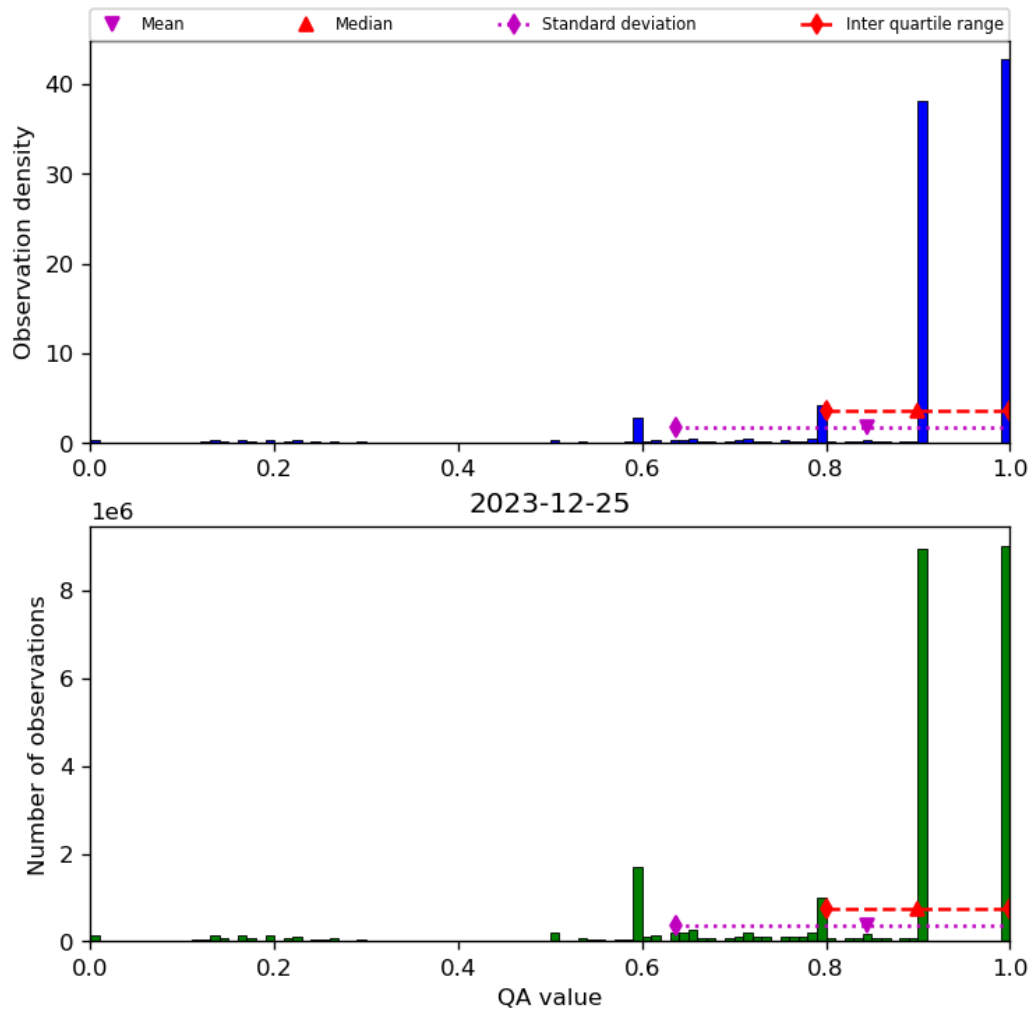
Figure 20: Histogram of “QA value” for 2023-12-25 to 2023-12-26
