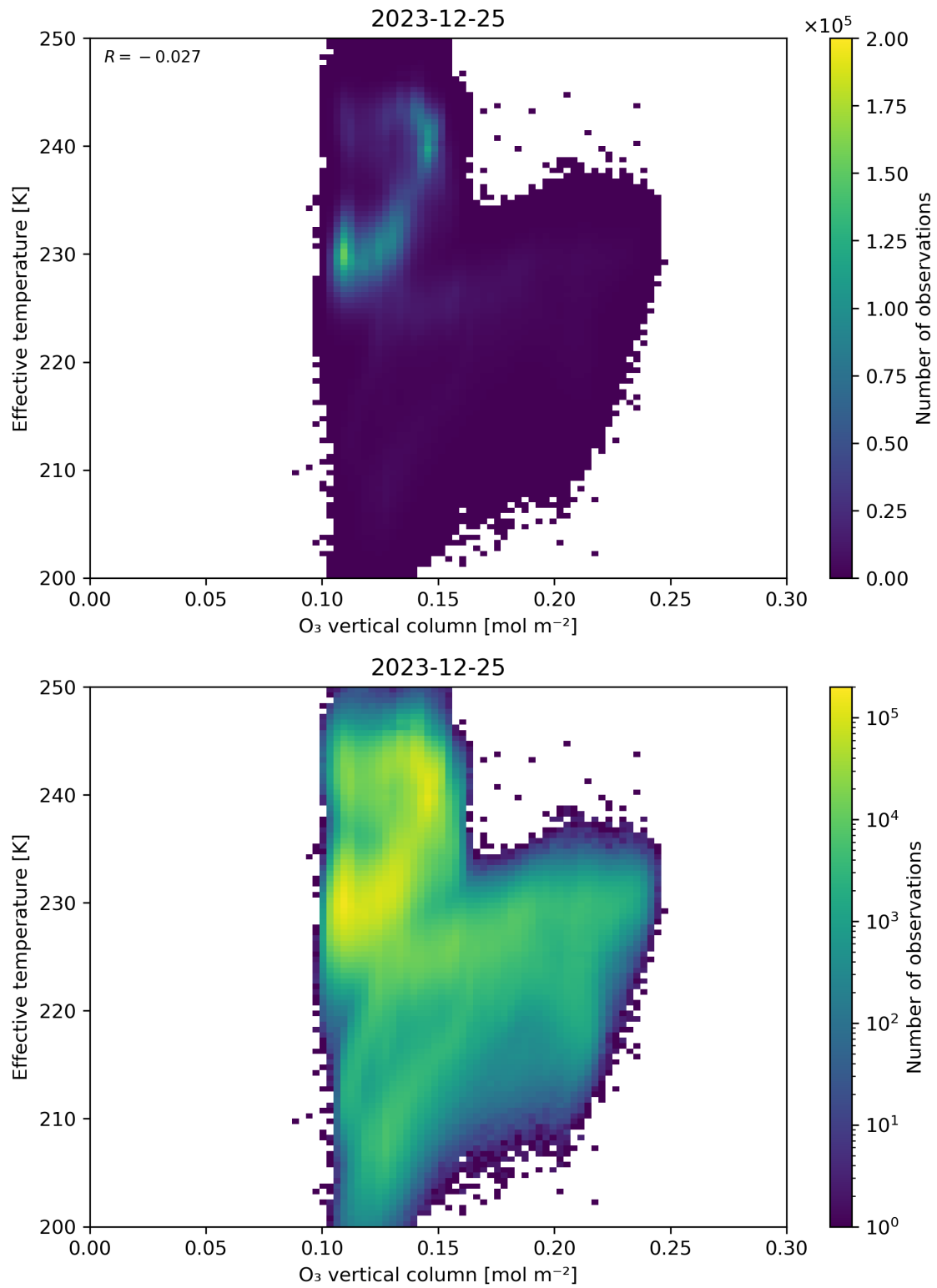
Figure 39: Scatter density plot of “O 3 vertical column” against “Effective temperature” for 2023-12-25 to 2023-12-26.
