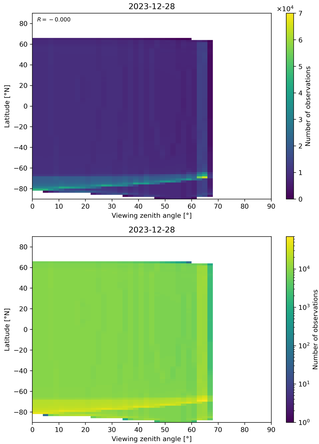
Figure 49: Scatter density plot of “Viewing zenith angle” against “Latitude” for 2023-12-27 to 2023-12-29.
