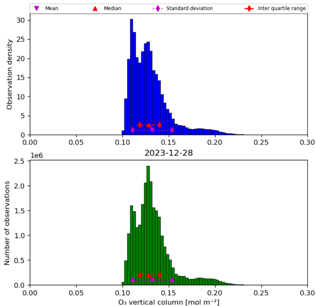
Figure 21: Histogram of “O 3 vertical column” for 2023-12-27 to 2023-12-29
