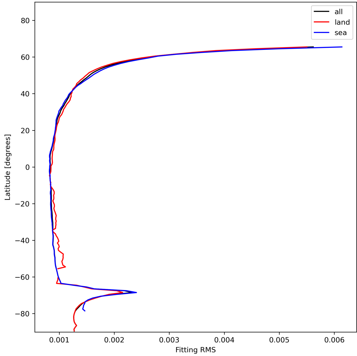
Figure 16: Zonal average of “Fitting RMS” for 2023-12-27 to 2023-12-29.
