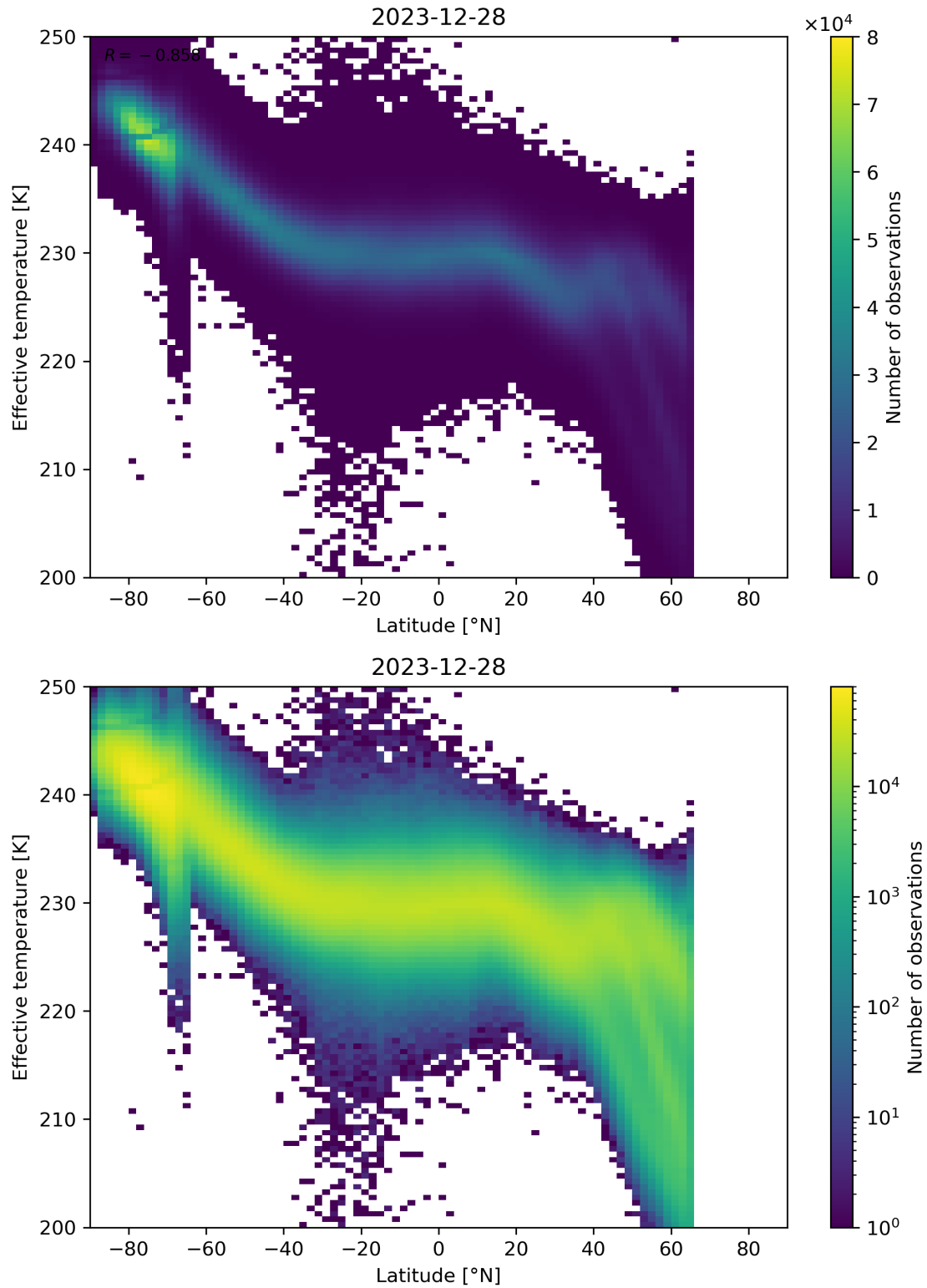
Figure 34: Scatter density plot of “Latitude” against “Effective temperature” for 2023-12-27 to 2023-12-29.
