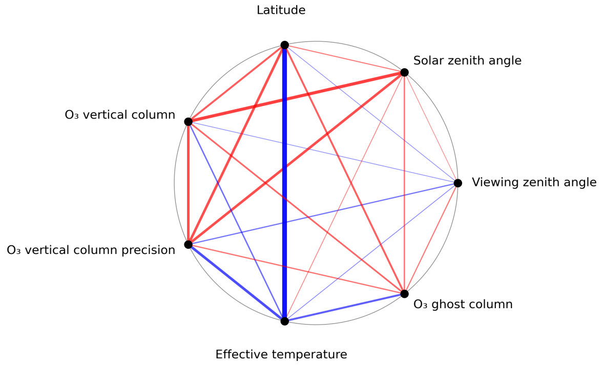
Figure 1: Map of correlation graph for 2023-12-27 to 2023-12-29.
