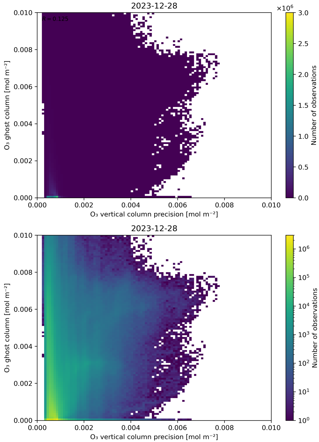
Figure 43: Scatter density plot of “ \text{O}_3 vertical column precision” against “ \text{O}_3 ghost column” for 2023-12-27 to 2023-12-29.
