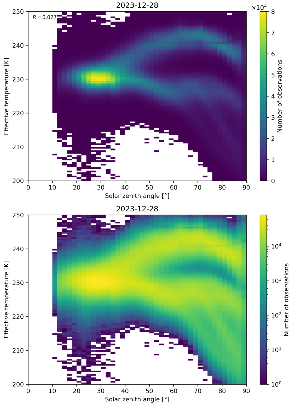
Figure 45: Scatter density plot of “Solar zenith angle” against “Effective temperature” for 2023-12-27 to 2023-12-29.
