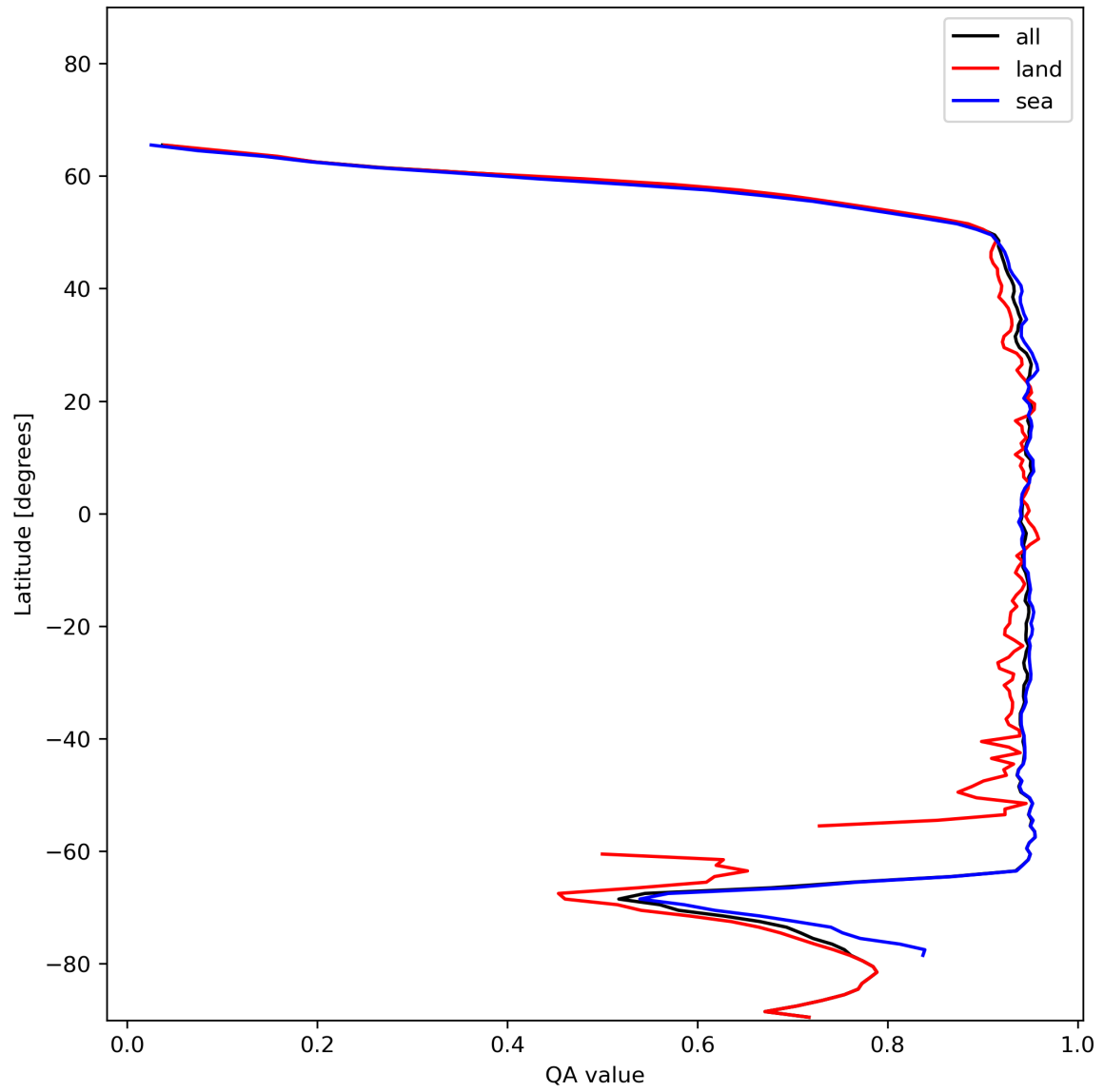
Figure 13: Zonal average of “QA value” for 2023-12-27 to 2023-12-29.
