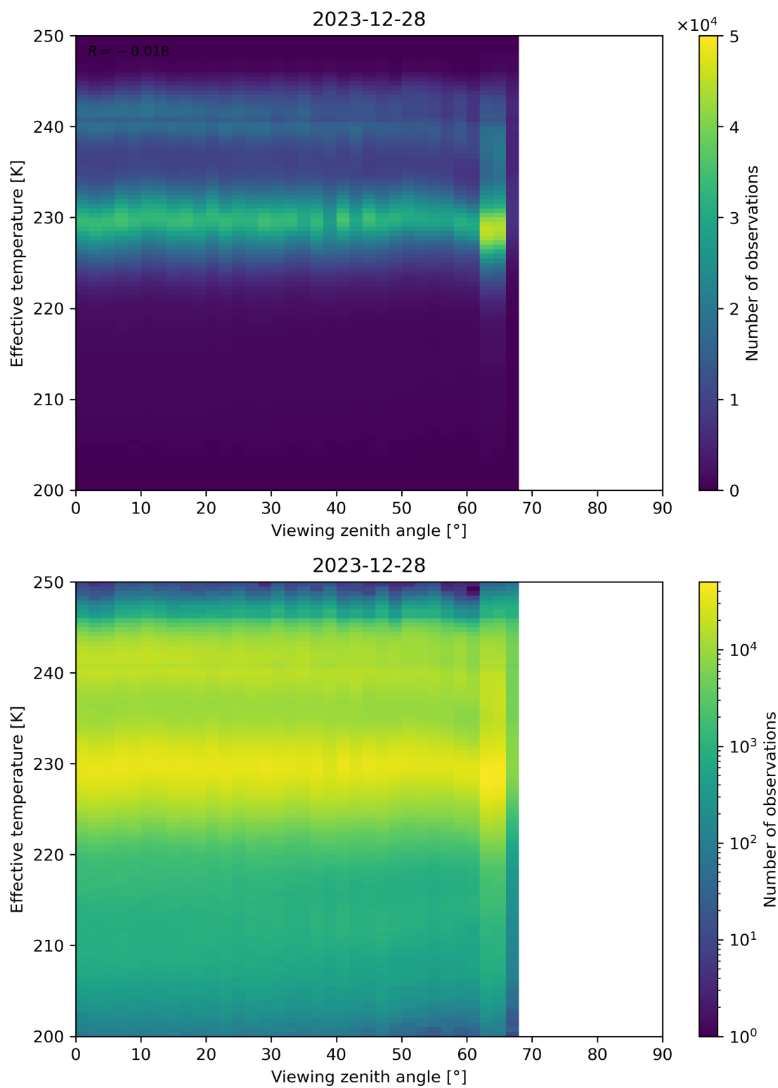
Figure 50: Scatter density plot of “Viewing zenith angle” against “Effective temperature” for 2023-12-27 to 2023-12-29.
