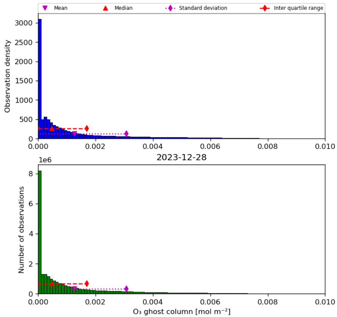
Figure 25: Histogram of “O 3 ghost column” for 2023-12-27 to 2023-12-29
