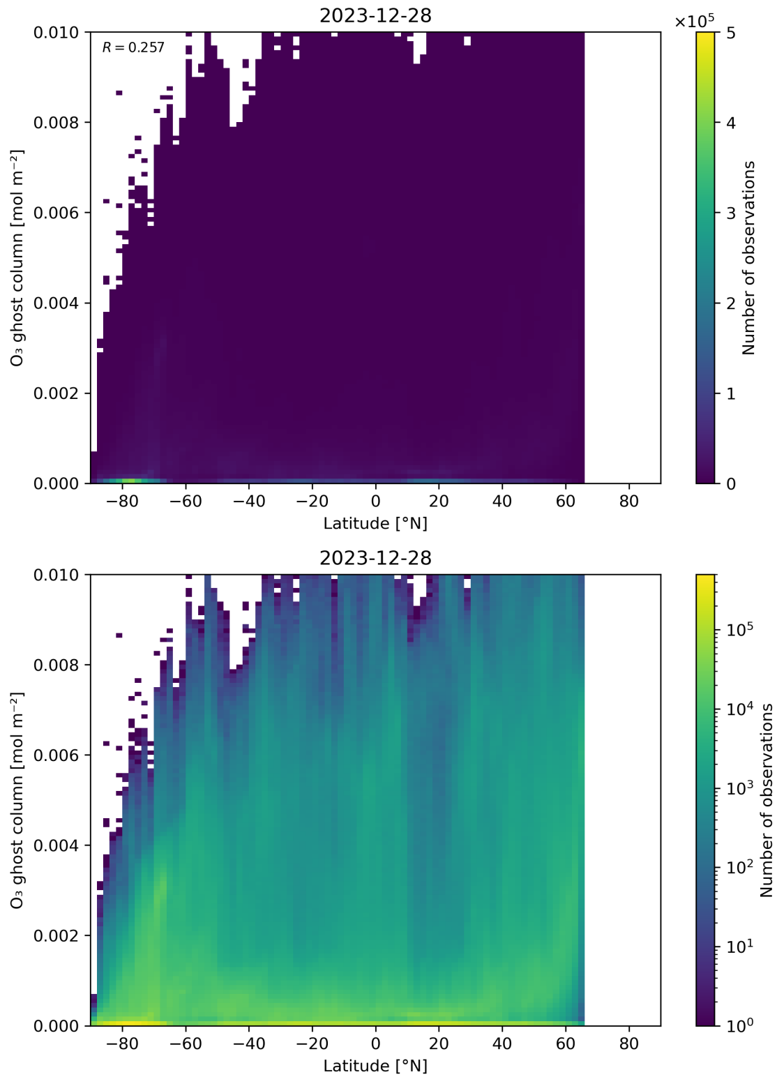
Figure 35: Scatter density plot of “Latitude” against “O 3 ghost column” for 2023-12-27 to 2023-12-29.
