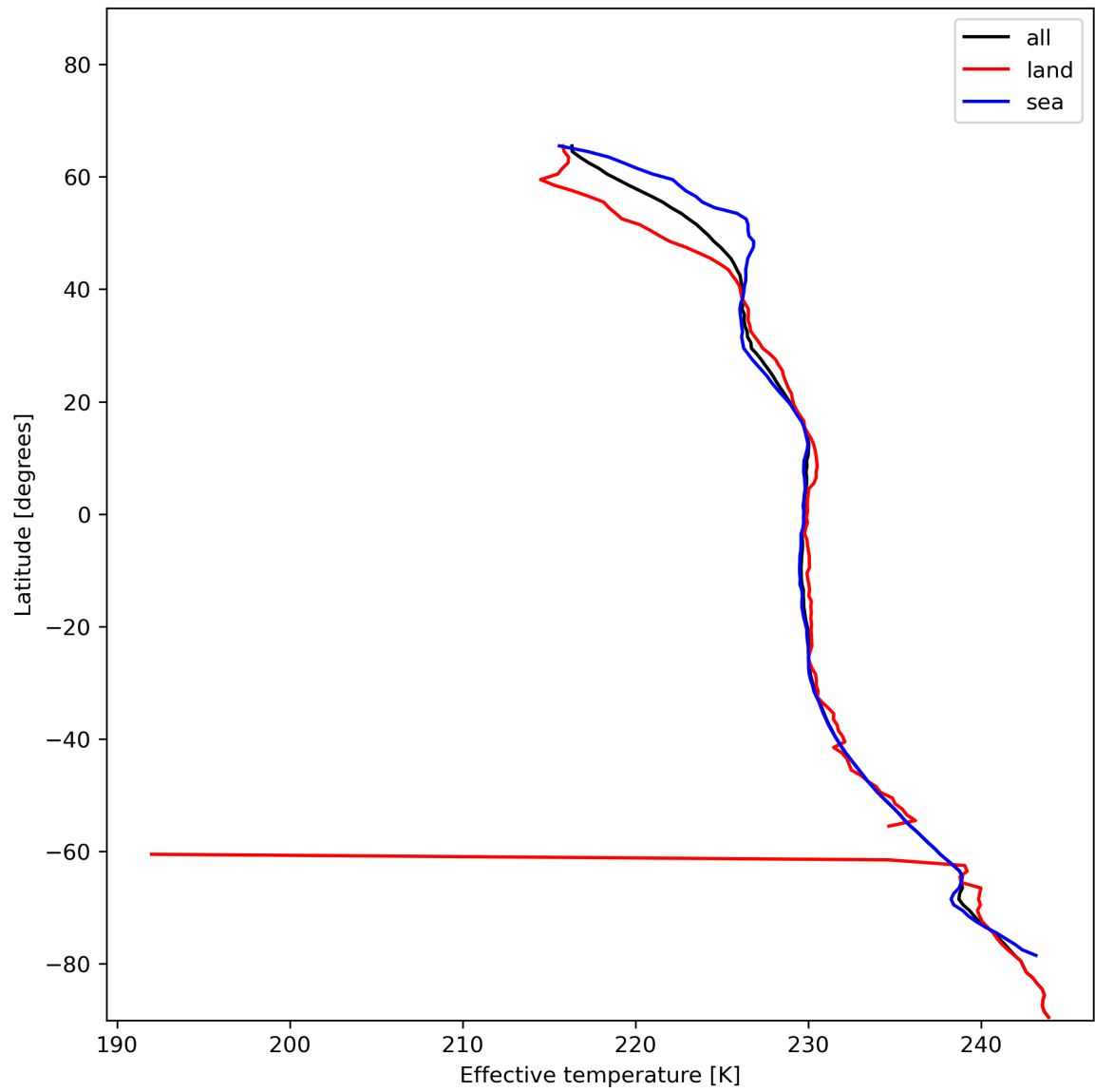
Figure 17: Zonal average of “Effective temperature” for 2023-12-27 to 2023-12-29.
