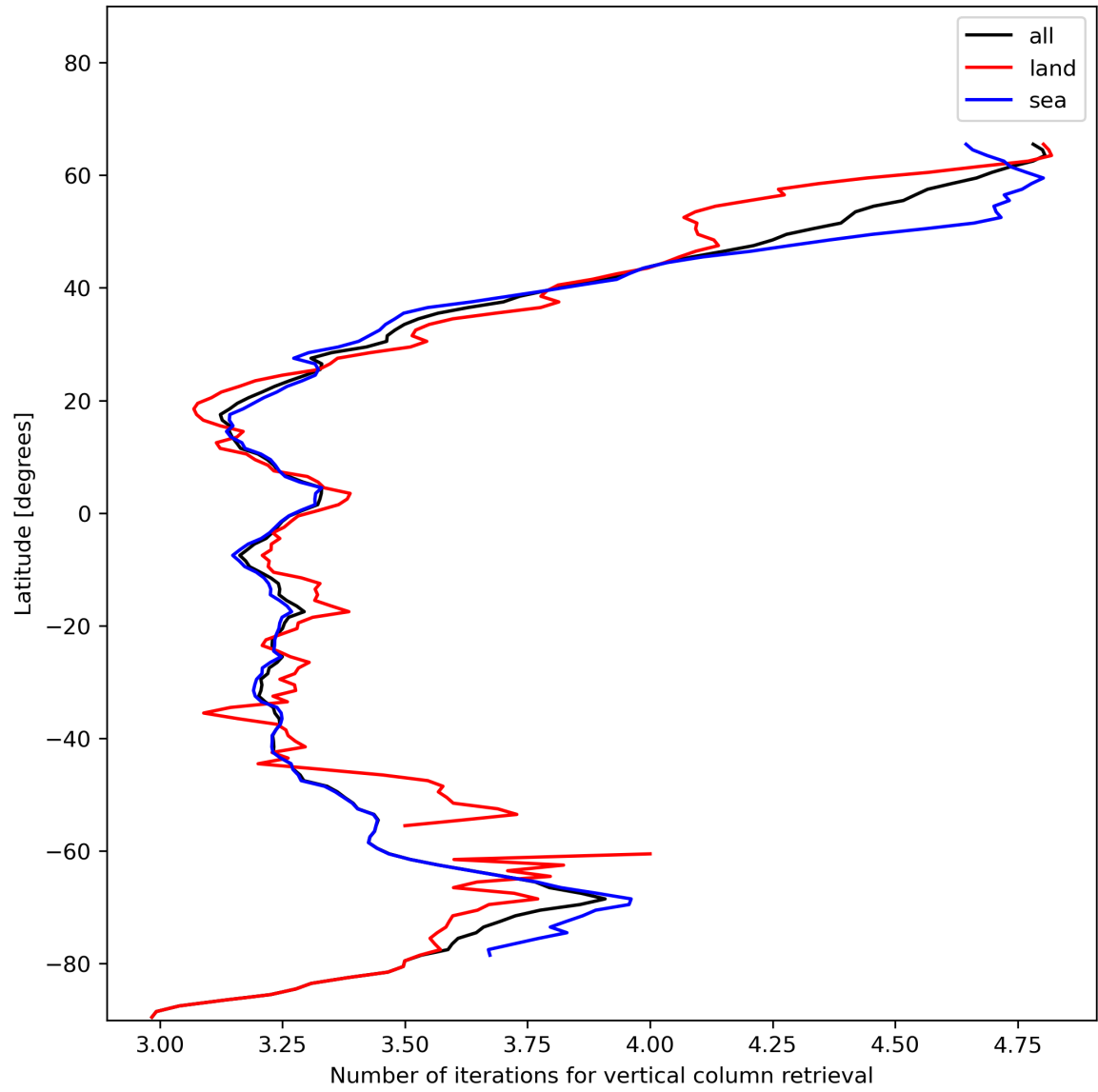
Figure 19: Zonal average of “Number of iterations for vertical column retrieval” for 2023-12-27 to 2023-12-29.
