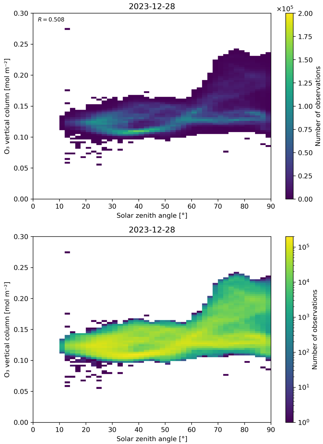
Figure 47: Scatter density plot of “Solar zenith angle” against “O 3 vertical column” for 2023-12-27 to 2023-12-29.
