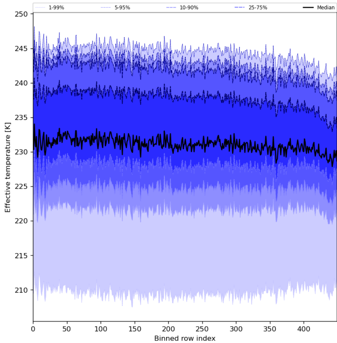
Figure 31: Along track statistics of “Effective temperature” for 2023-12-27 to 2023-12-29
