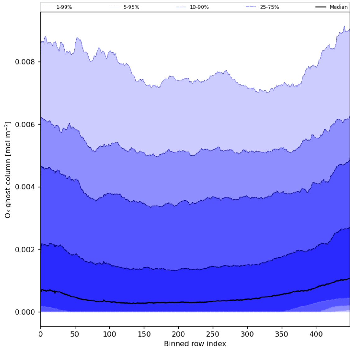
Figure 32: Along track statistics of “O 3 ghost column” for 2023-12-27 to 2023-12-29
