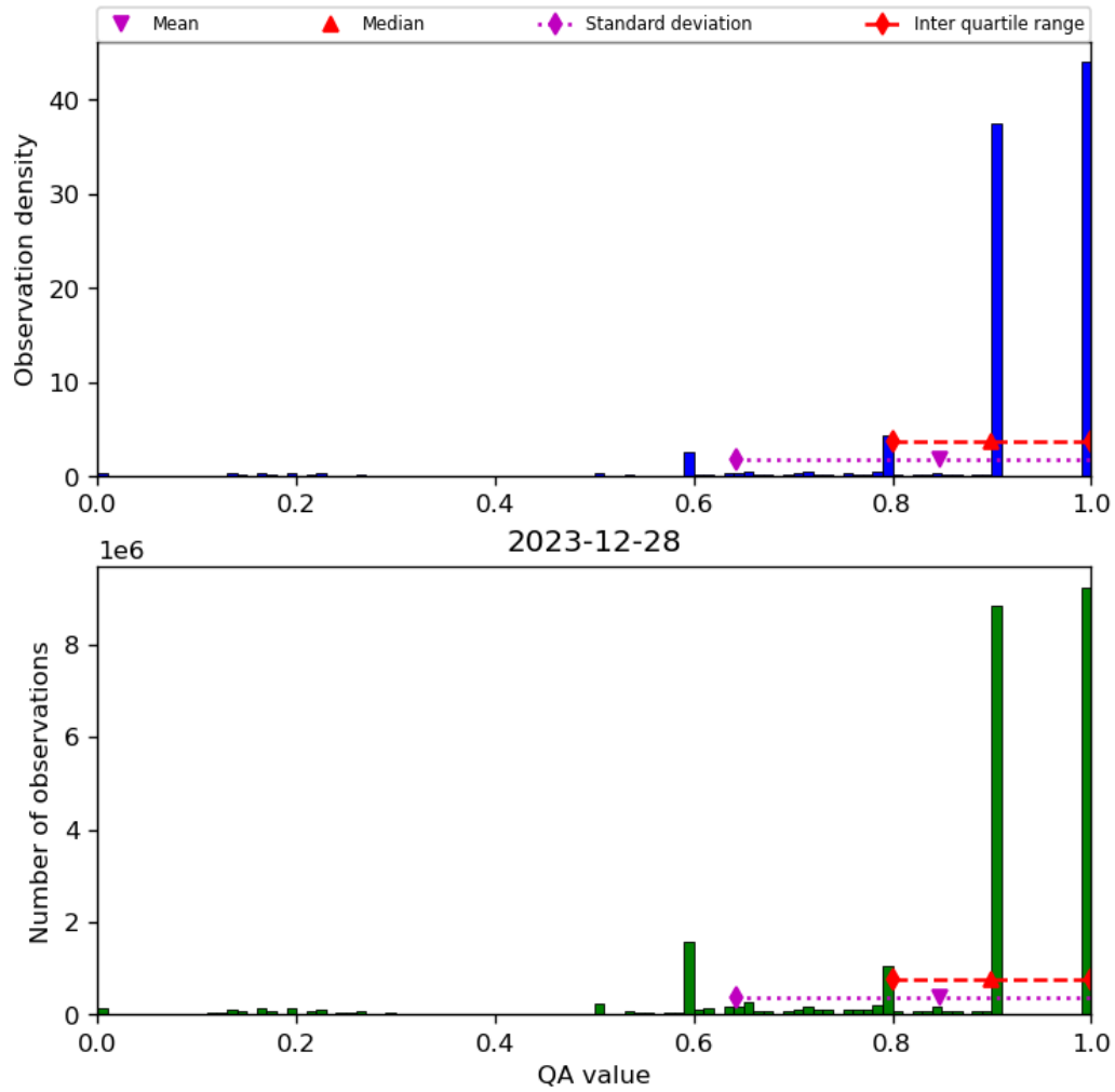
Figure 20: Histogram of “QA value” for 2023-12-27 to 2023-12-29
