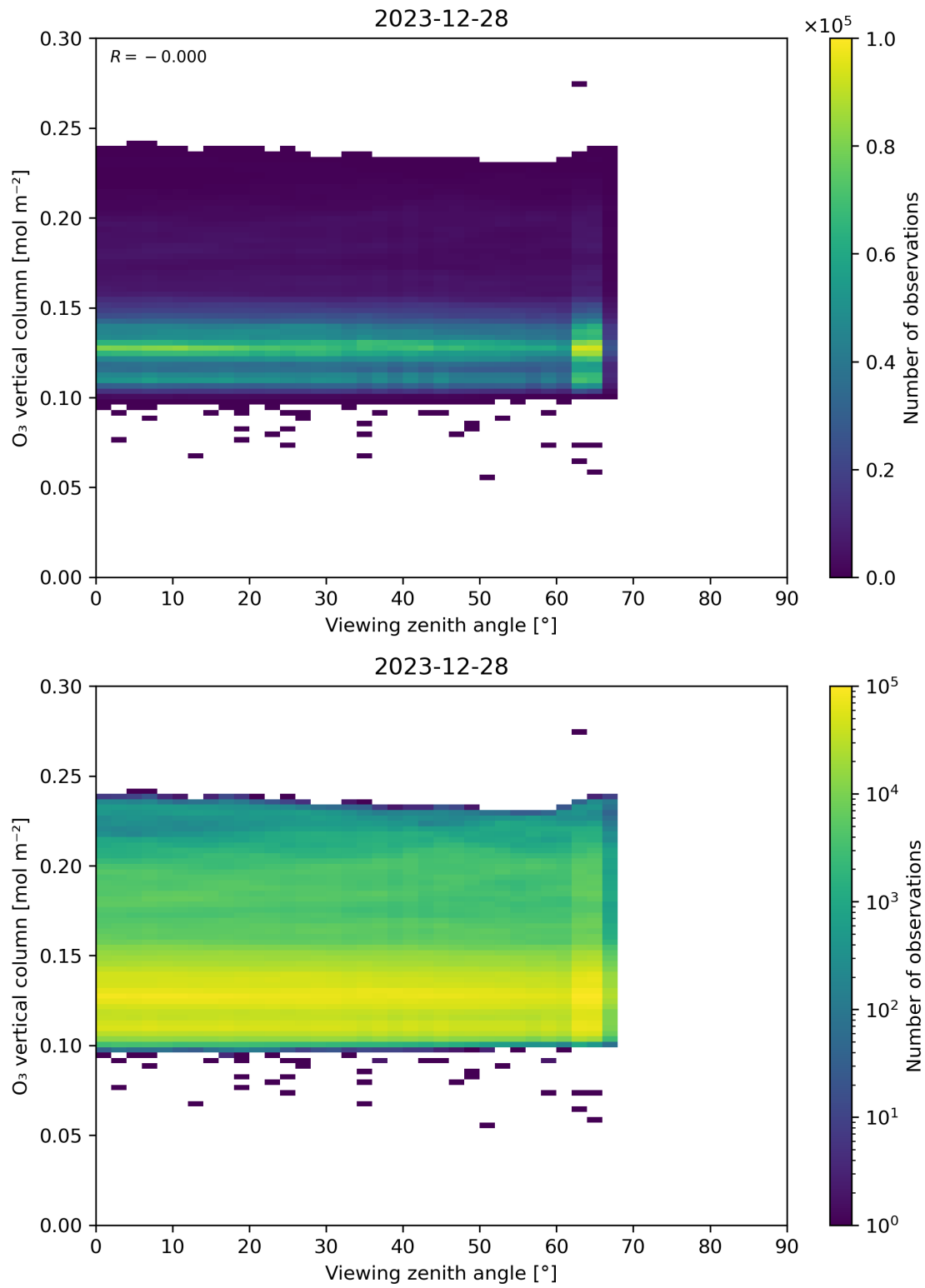
Figure 52: Scatter density plot of “Viewing zenith angle” against “O 3 vertical column” for 2023-12-27 to 2023-12-29.
