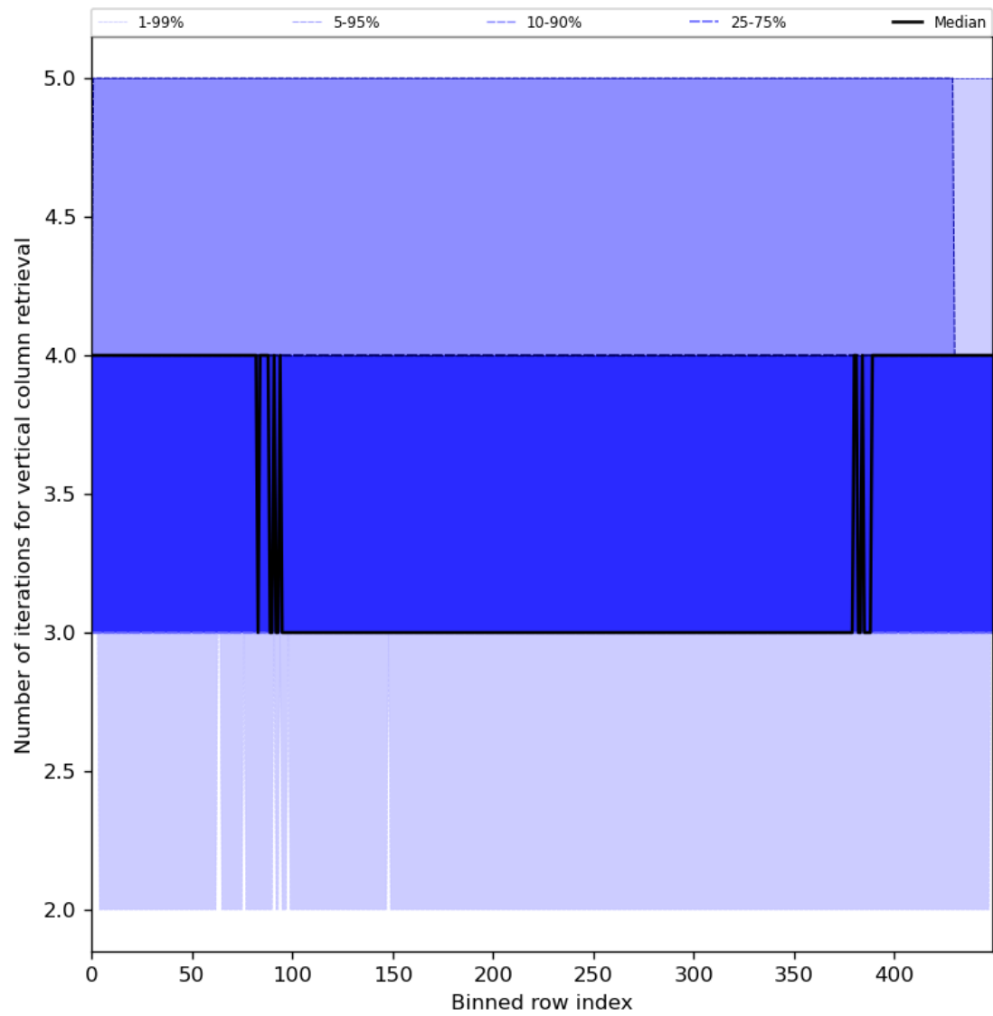
Figure 33: Along track statistics of “Number of iterations for vertical column retrieval” for 2023-12-27 to 2023-12-29
