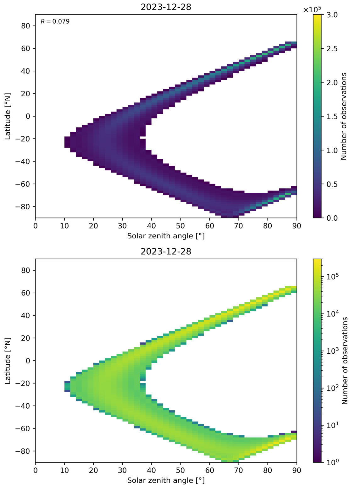
Figure 44: Scatter density plot of “Solar zenith angle” against “Latitude” for 2023-12-27 to 2023-12-29.
