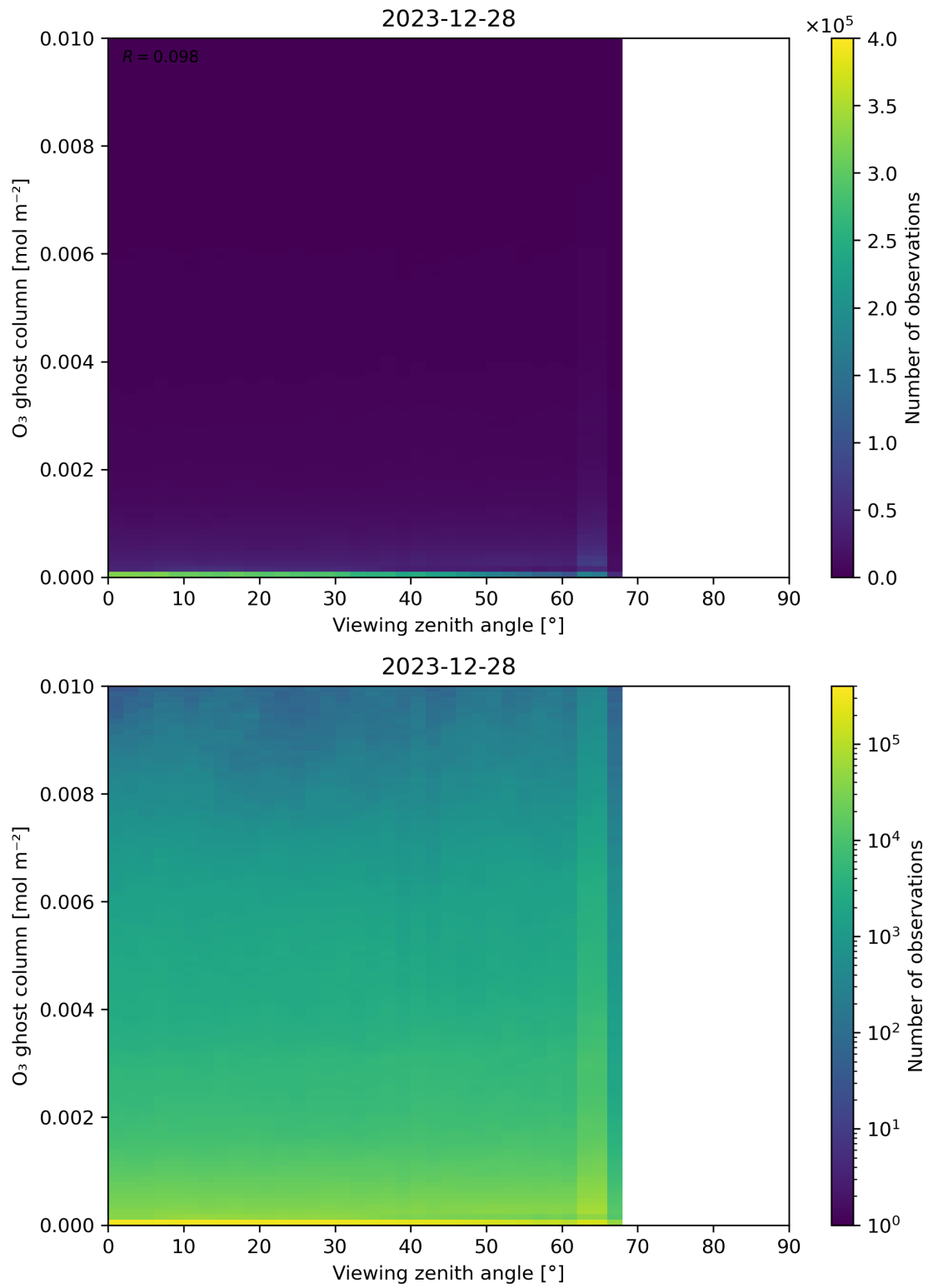
Figure 51: Scatter density plot of “Viewing zenith angle” against “O 3 ghost column” for 2023-12-27 to 2023-12-29.
