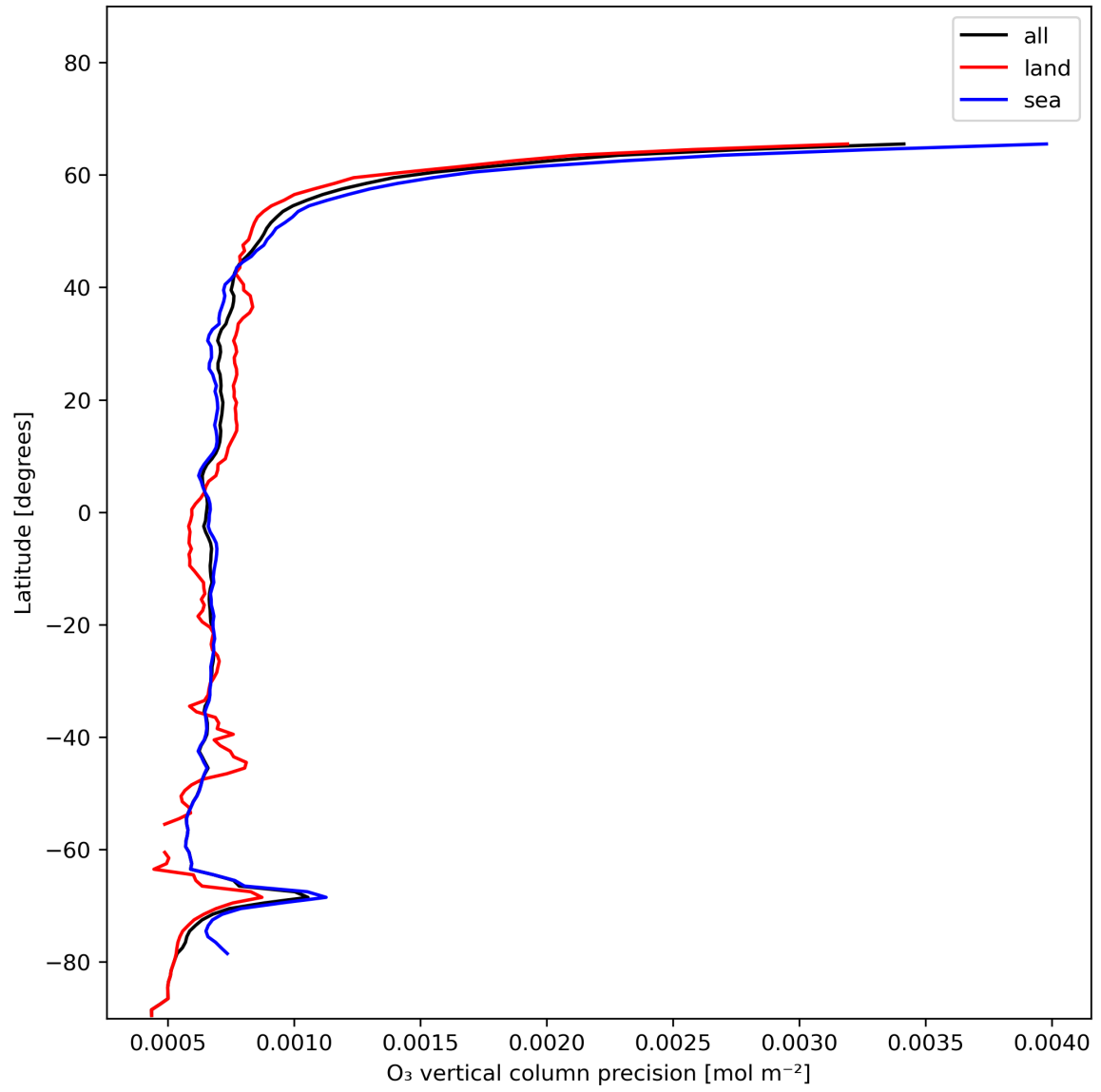
Figure 15: Zonal average of “O 3 vertical column precision” for 2023-12-27 to 2023-12-29.
