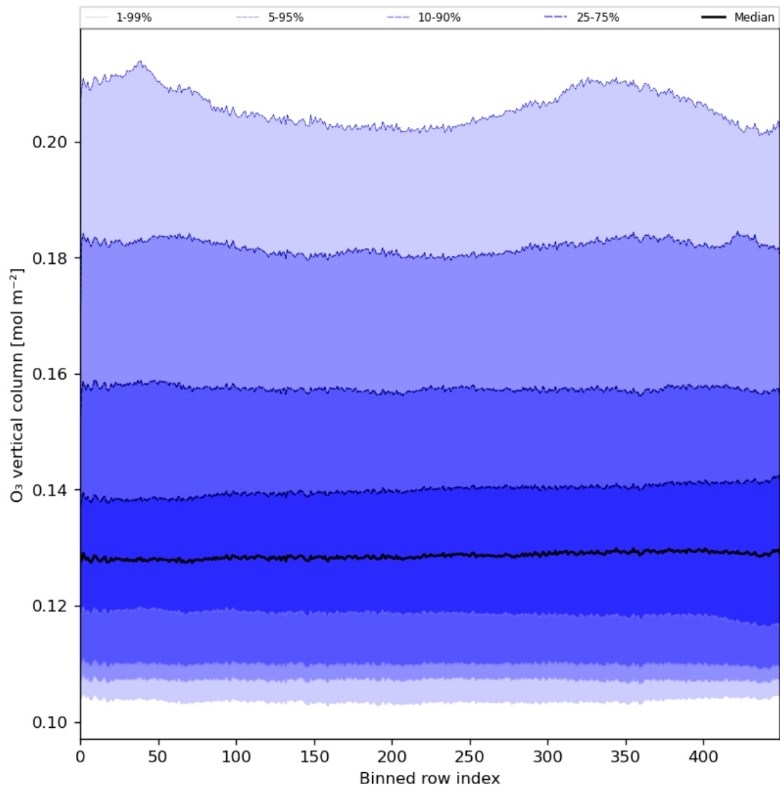
Figure 28: Along track statistics of “O 3 vertical column” for 2023-12-27 to 2023-12-29
