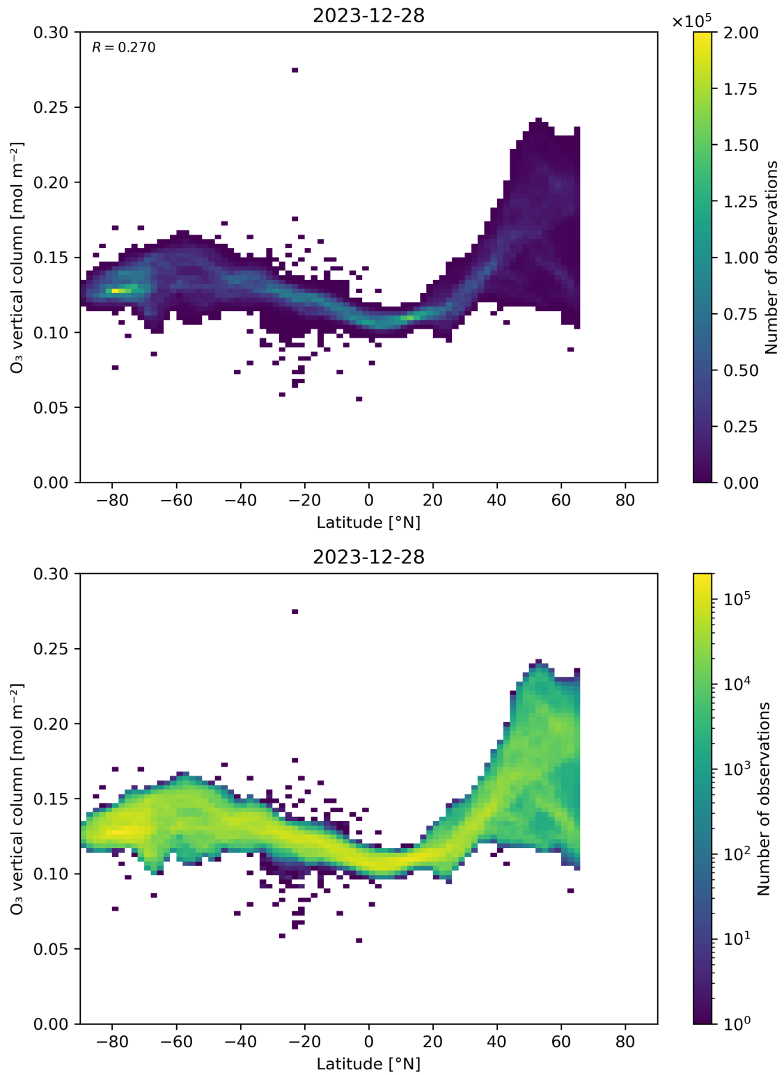
Figure 36: Scatter density plot of “Latitude” against “O 3 vertical column” for 2023-12-27 to 2023-12-29.
