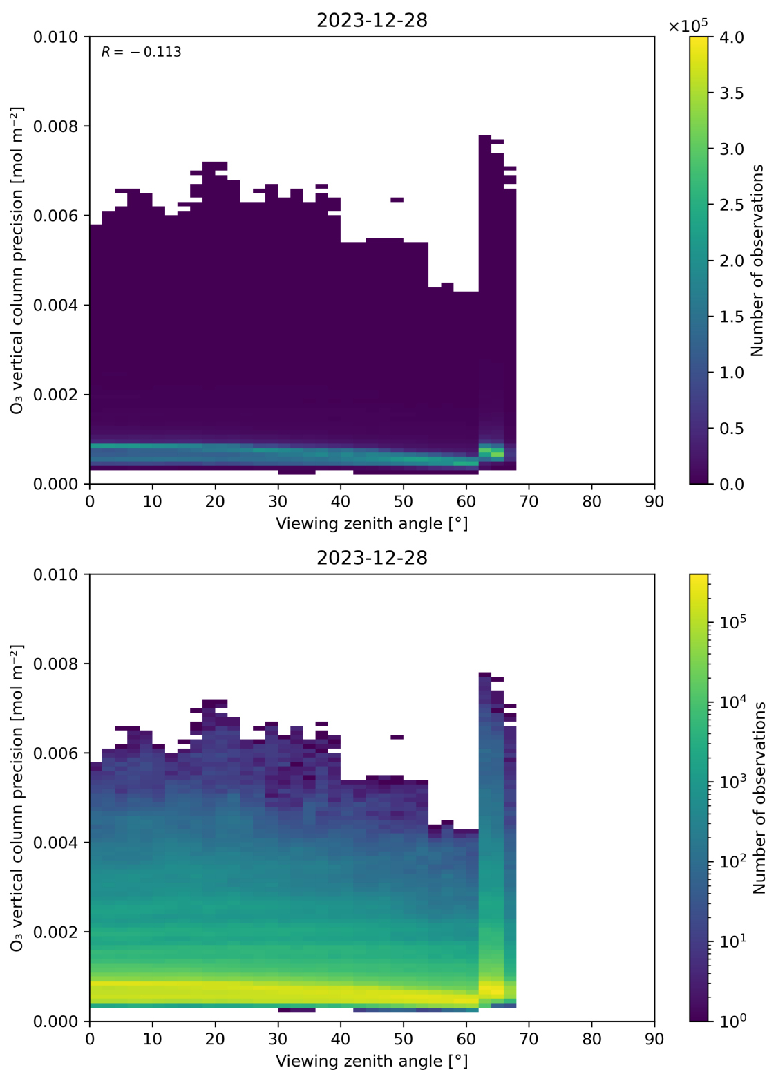
Figure 53: Scatter density plot of “Viewing zenith angle” against “O 3 vertical column precision” for 2023-12-27 to 2023-12-29.
