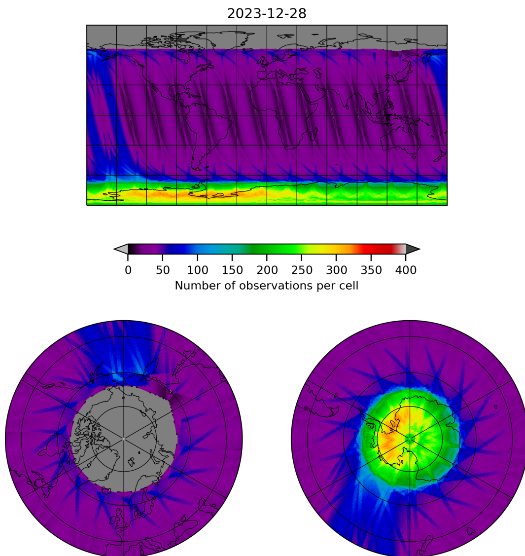
Figure 12: Map of the number of observations for 2023-12-27 to 2023-12-29
