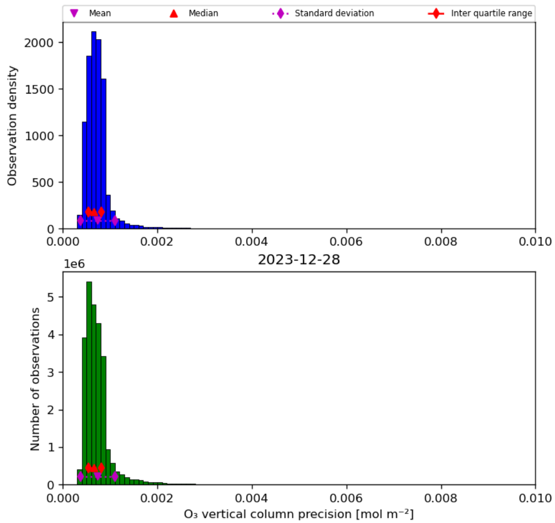
Figure 22: Histogram of “O 3 vertical column precision” for 2023-12-27 to 2023-12-29
