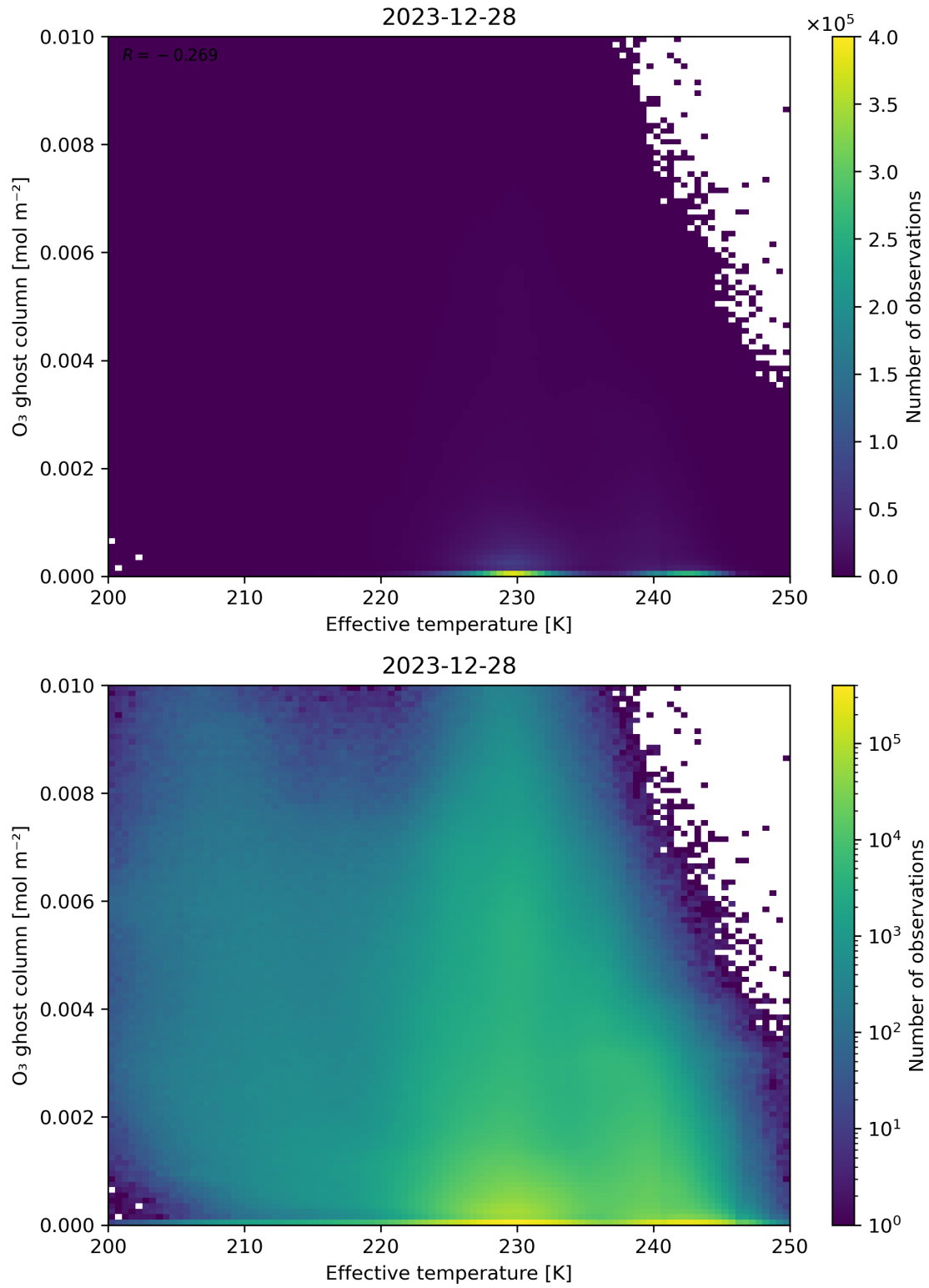
Figure 38: Scatter density plot of “Effective temperature” against “O 3 ghost column” for 2023-12-27 to 2023-12-29.
