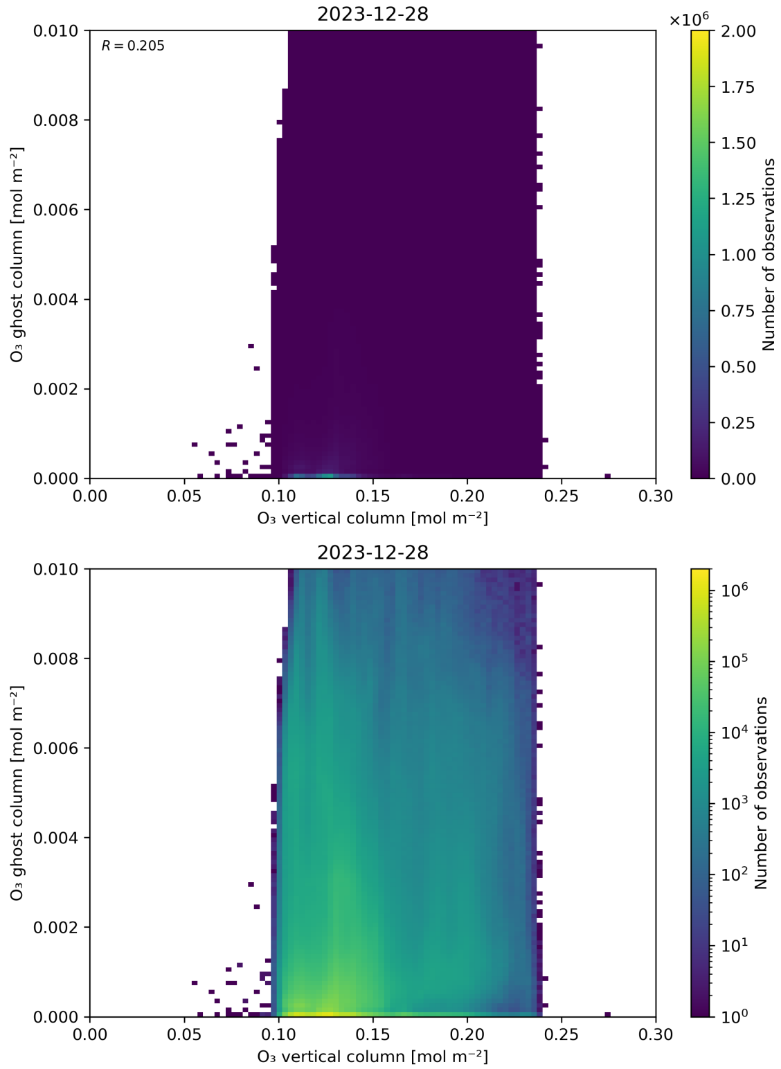
Figure 40: Scatter density plot of “O 3 vertical column” against “O 3 ghost column” for 2023-12-27 to 2023-12-29.
