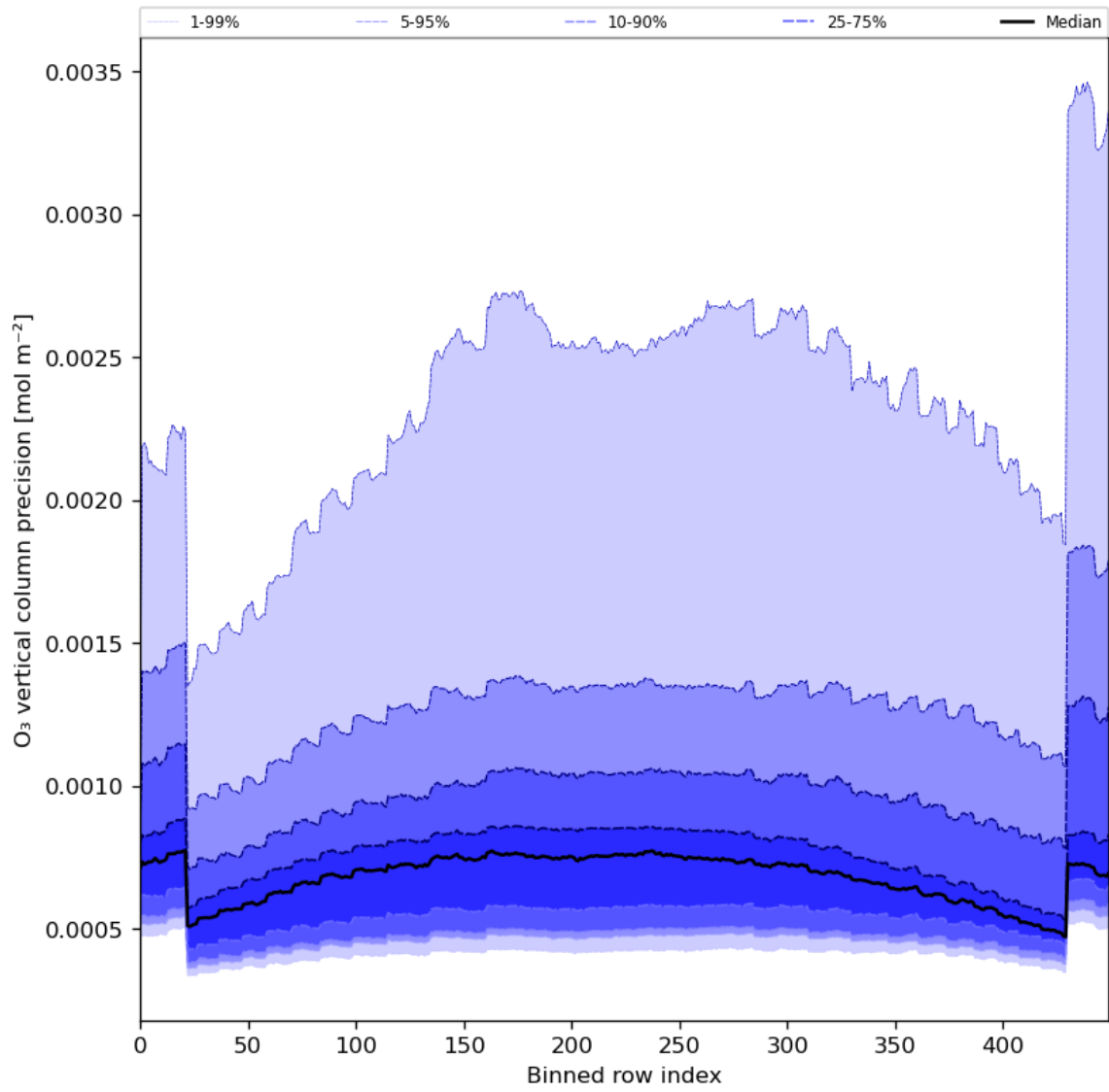
Figure 29: Along track statistics of “O 3 vertical column precision” for 2023-12-27 to 2023-12-29
