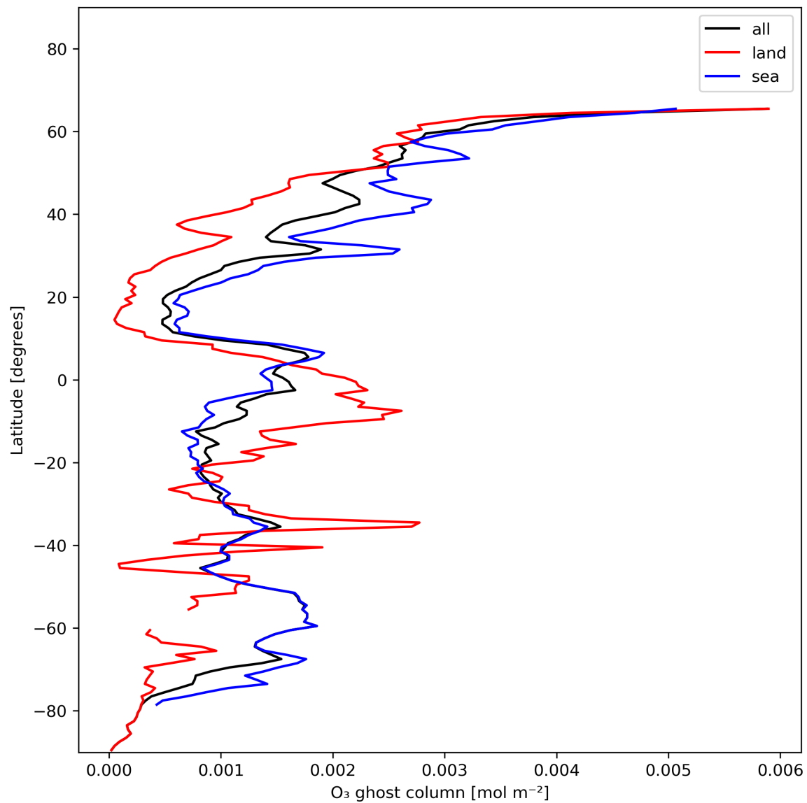
Figure 18: Zonal average of “O 3 ghost column” for 2023-12-27 to 2023-12-29.
