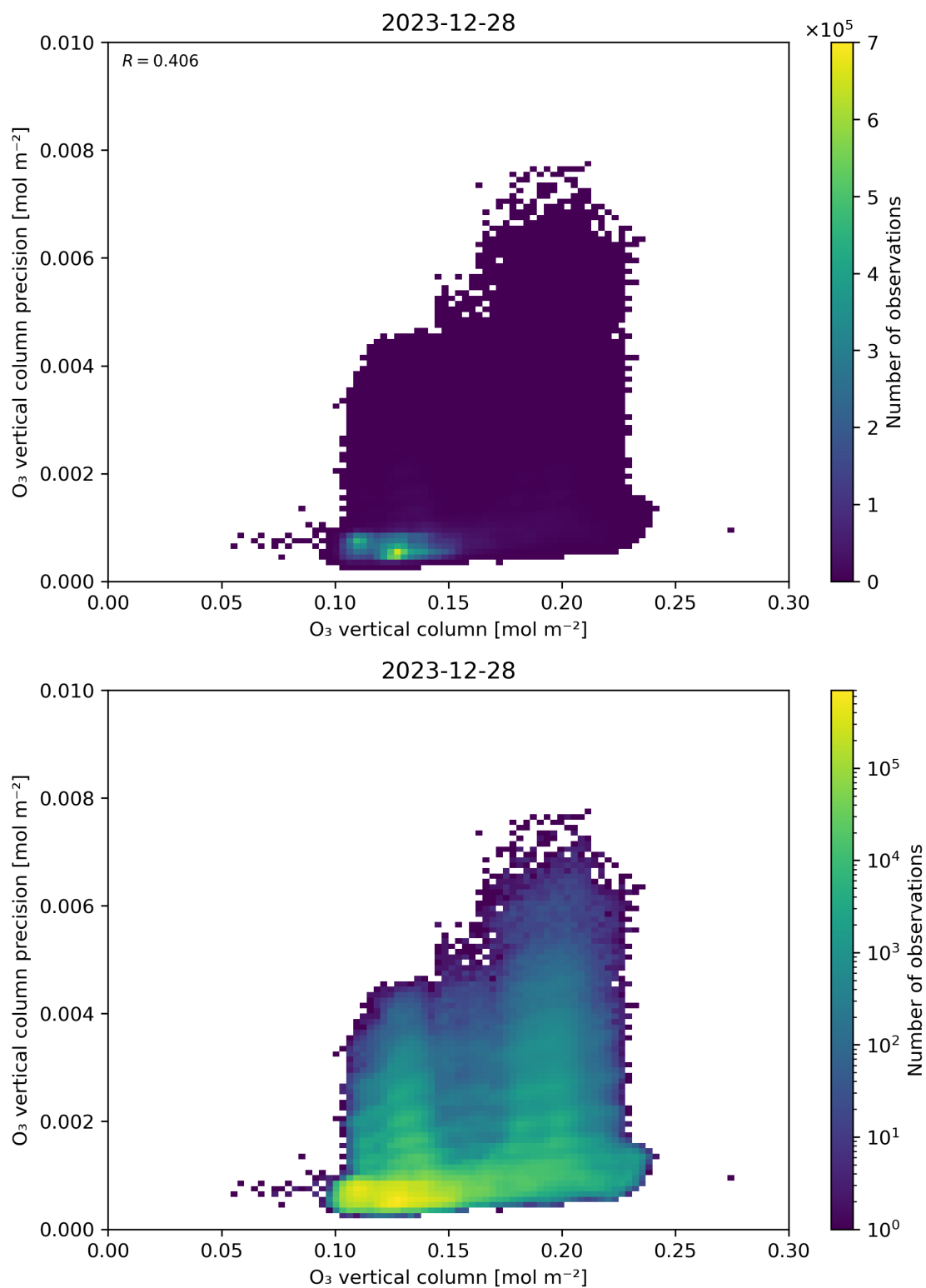
Figure 41: Scatter density plot of “O 3 vertical column” against “O 3 vertical column precision” for 2023-12-27 to 2023-12-29.
