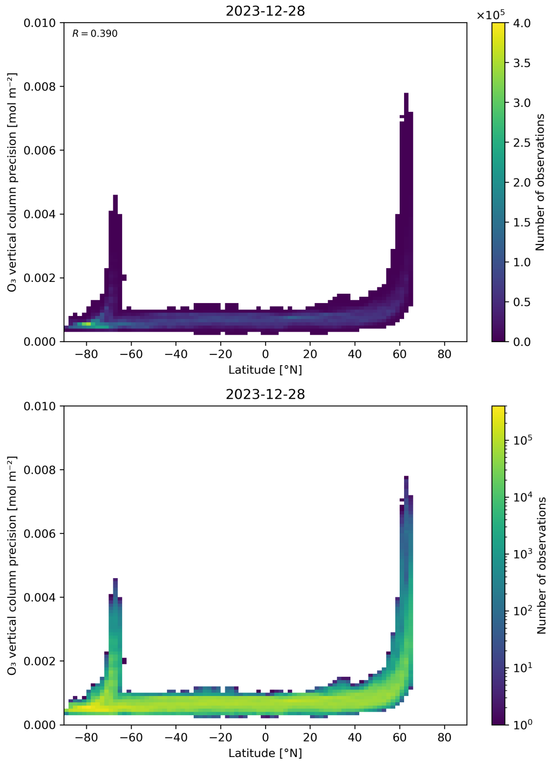
Figure 37: Scatter density plot of “Latitude” against “O 3 vertical column precision” for 2023-12-27 to 2023-12-29.
