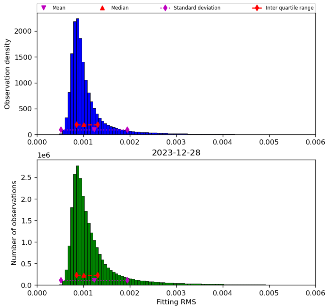
Figure 23: Histogram of “Fitting RMS” for 2023-12-27 to 2023-12-29
