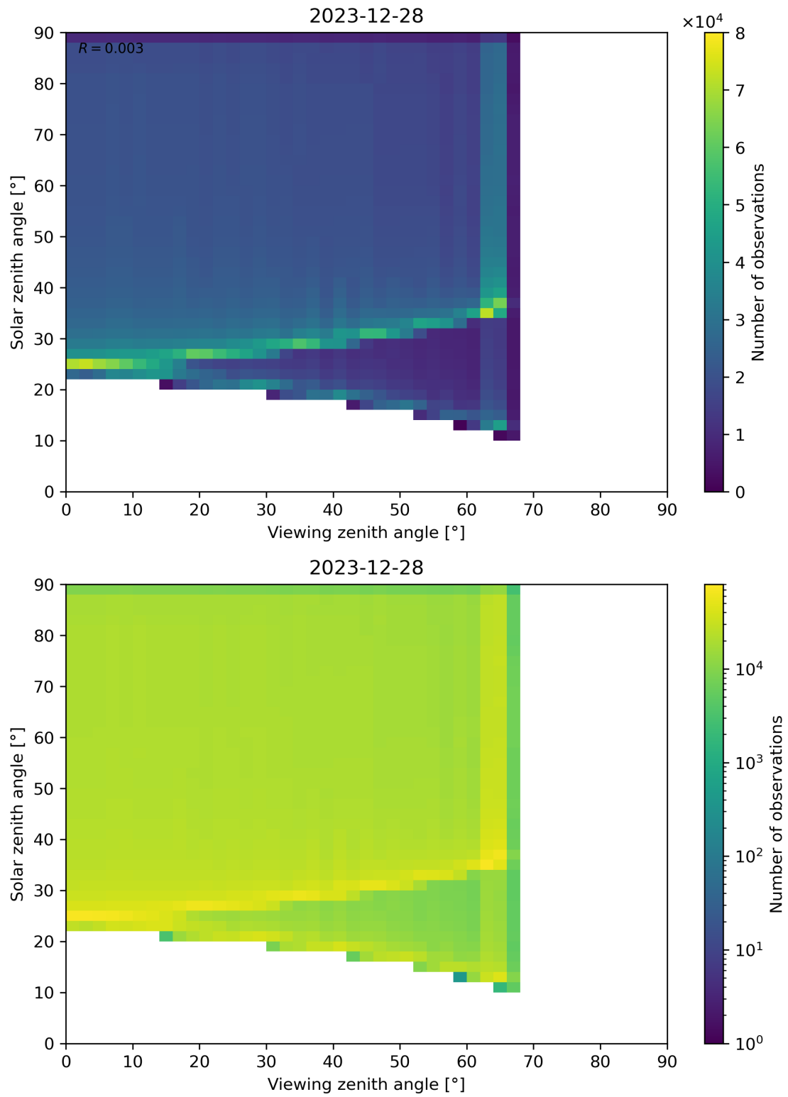
Figure 54: Scatter density plot of “Viewing zenith angle” against “Solar zenith angle” for 2023-12-27 to 2023-12-29.
