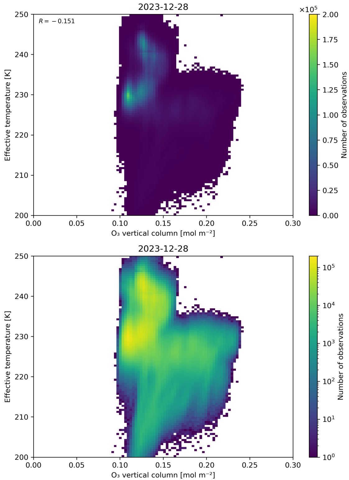
Figure 39: Scatter density plot of “O 3 vertical column” against “Effective temperature” for 2023-12-27 to 2023-12-29.
