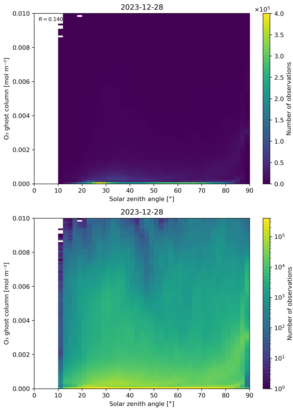
Figure 46: Scatter density plot of “Solar zenith angle” against “O 3 ghost column” for 2023-12-27 to 2023-12-29.
