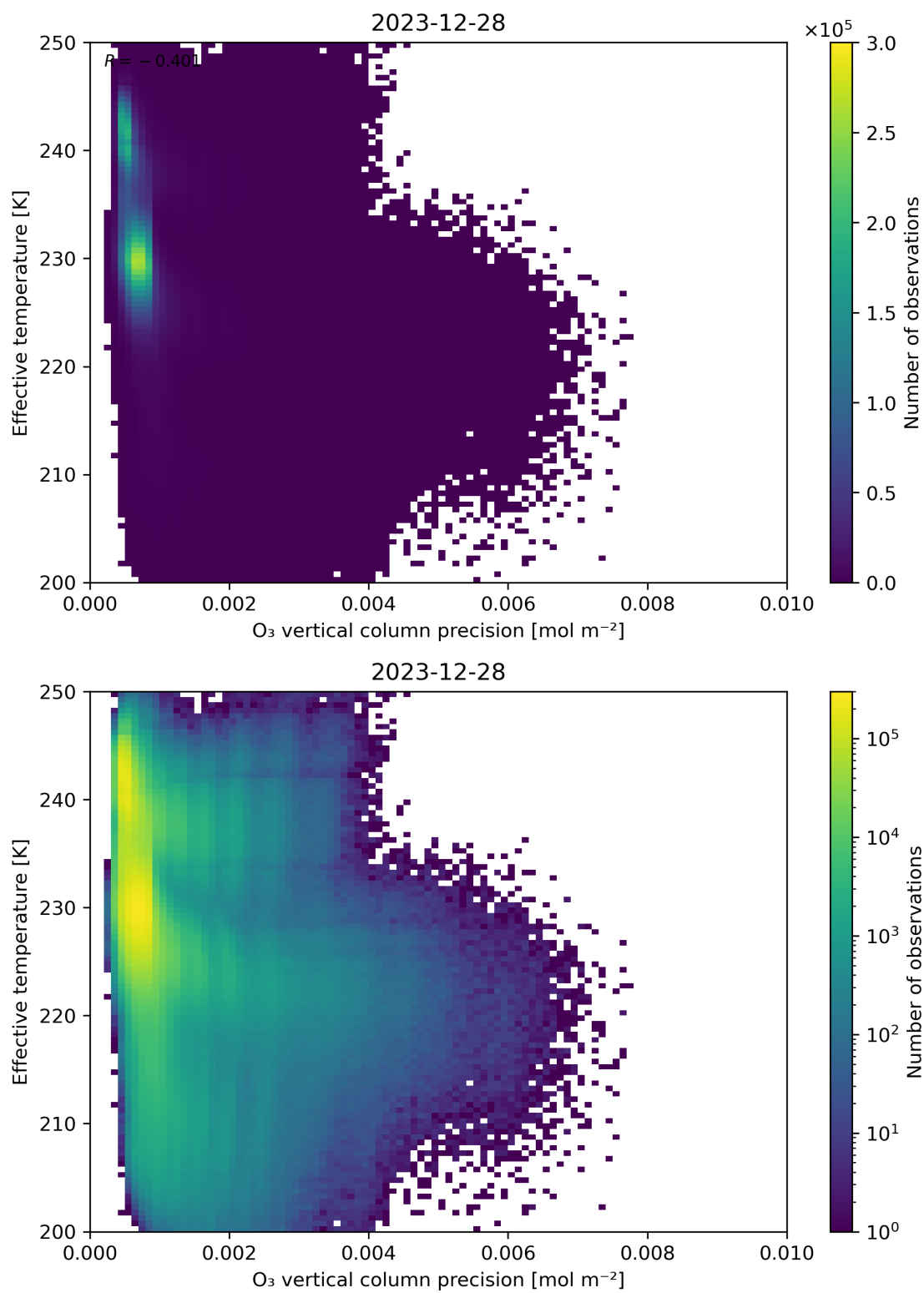
Figure 42: Scatter density plot of “O 3 vertical column precision” against “Effective temperature” for 2023-12-27 to 2023-12-29.
