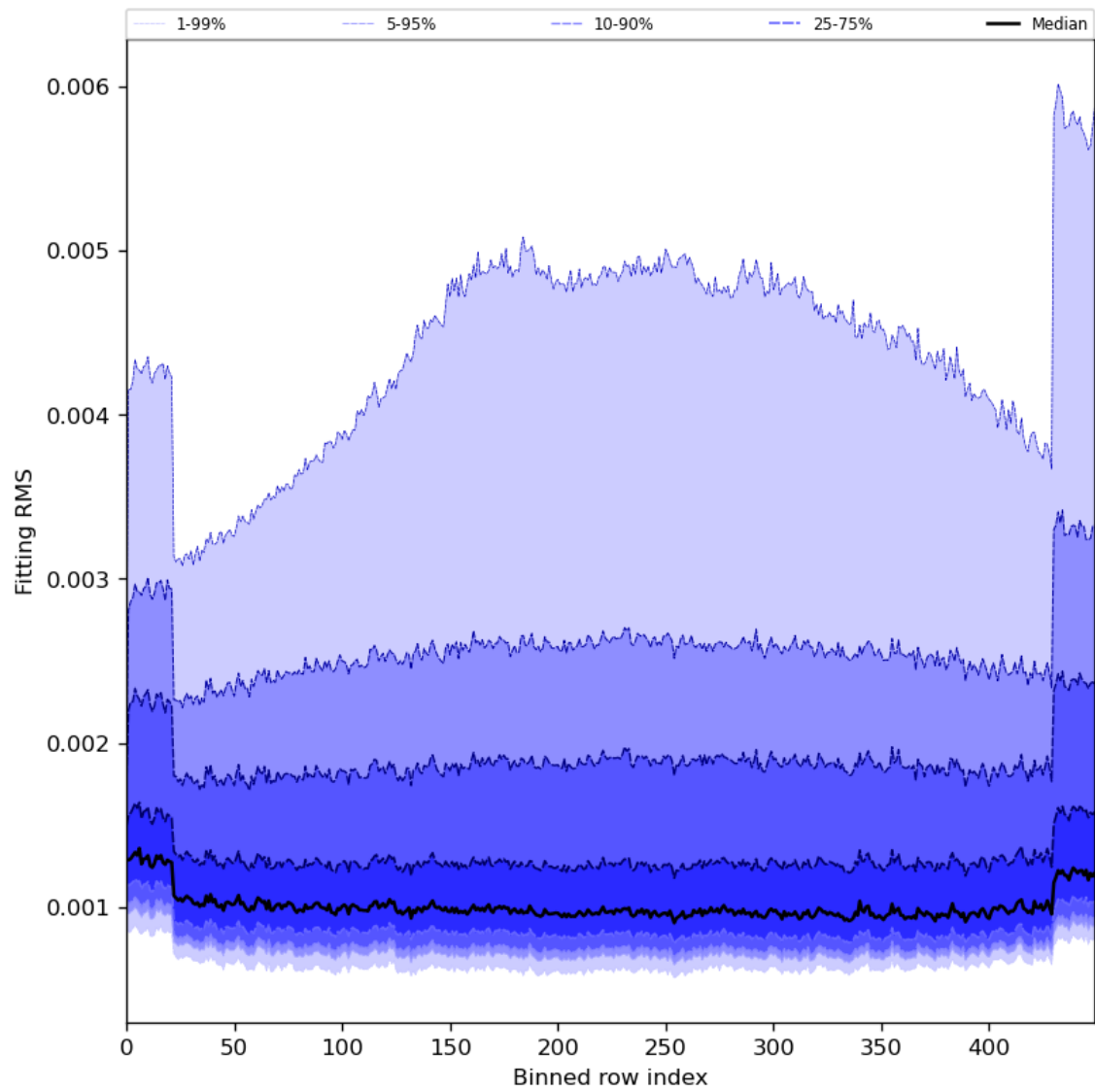
Figure 30: Along track statistics of “Fitting RMS” for 2023-12-27 to 2023-12-29
