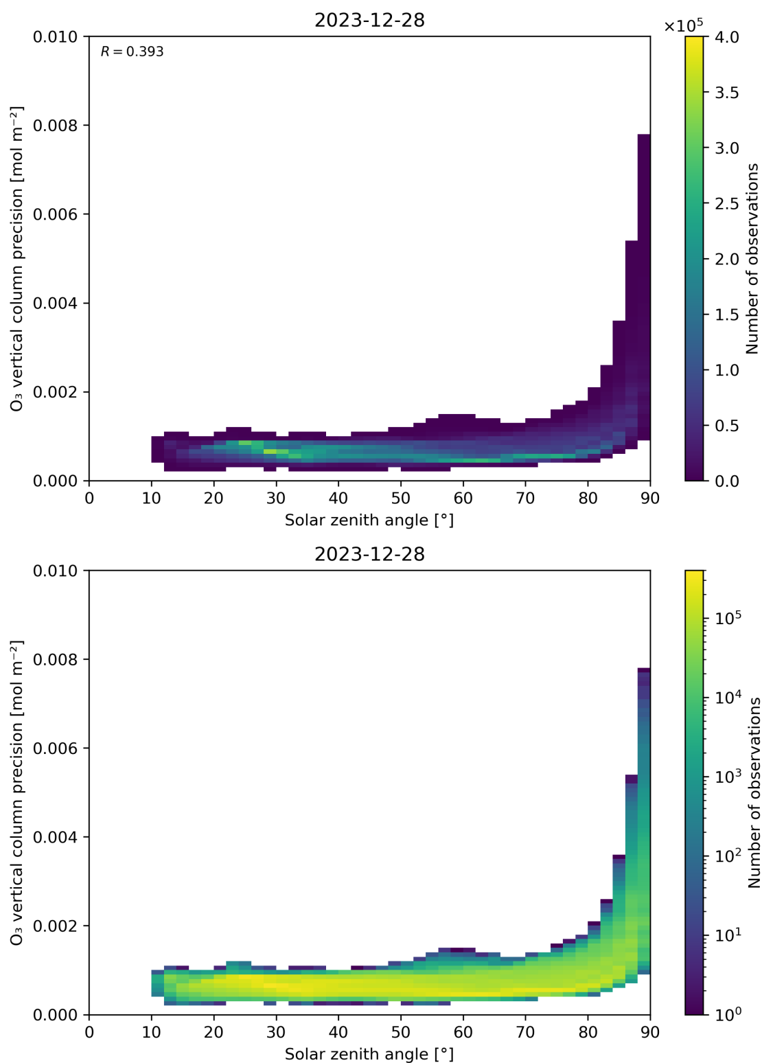
Figure 48: Scatter density plot of “Solar zenith angle” against “O 3 vertical column precision” for 2023-12-27 to 2023-12-29.
