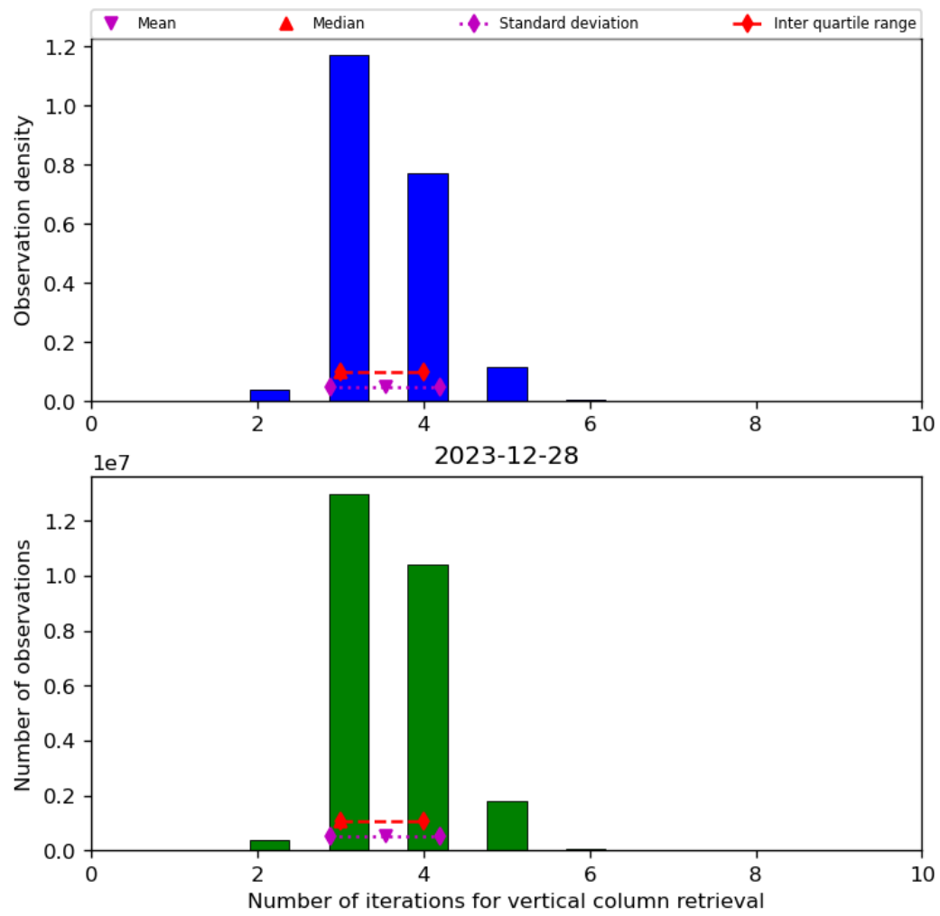
Figure 26: Histogram of “Number of iterations for vertical column retrieval” for 2023-12-27 to 2023-12-29
