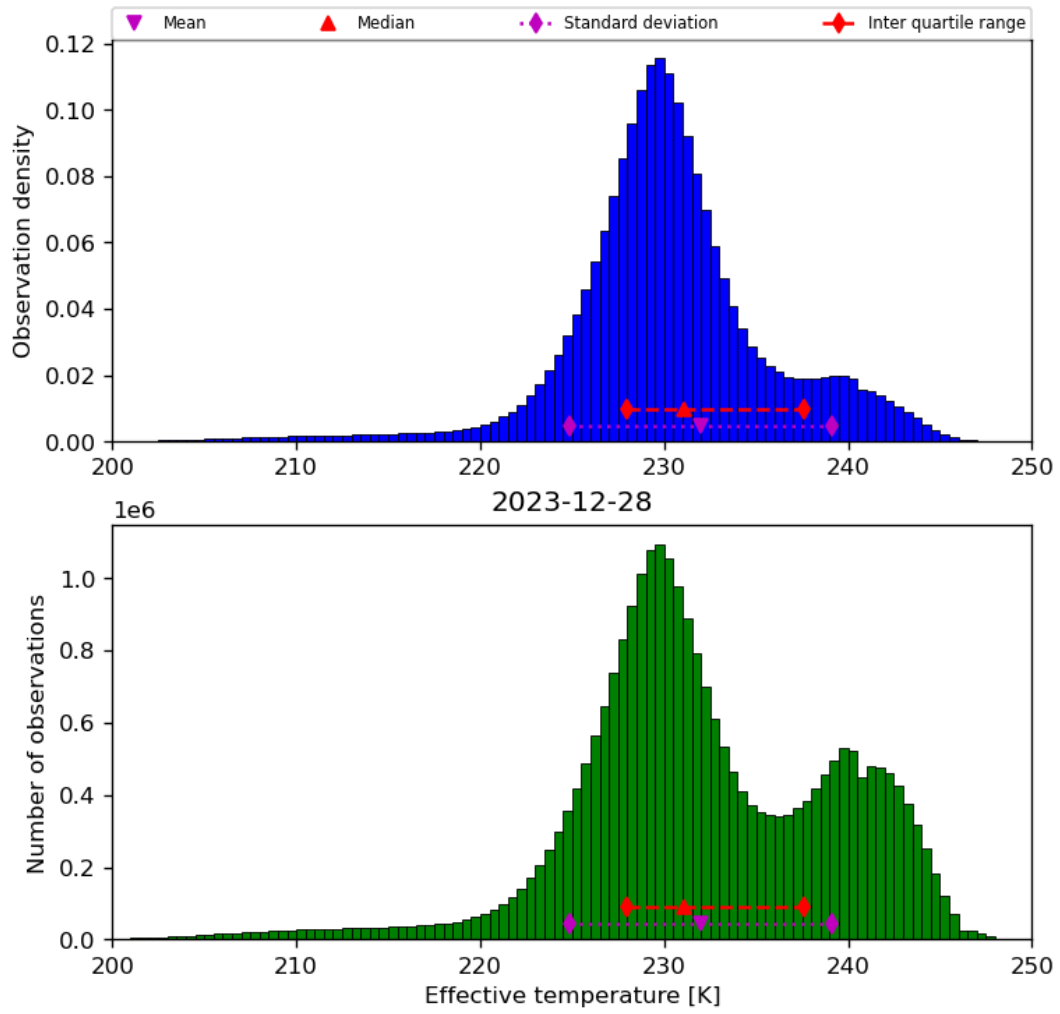
Figure 24: Histogram of “Effective temperature” for 2023-12-27 to 2023-12-29
