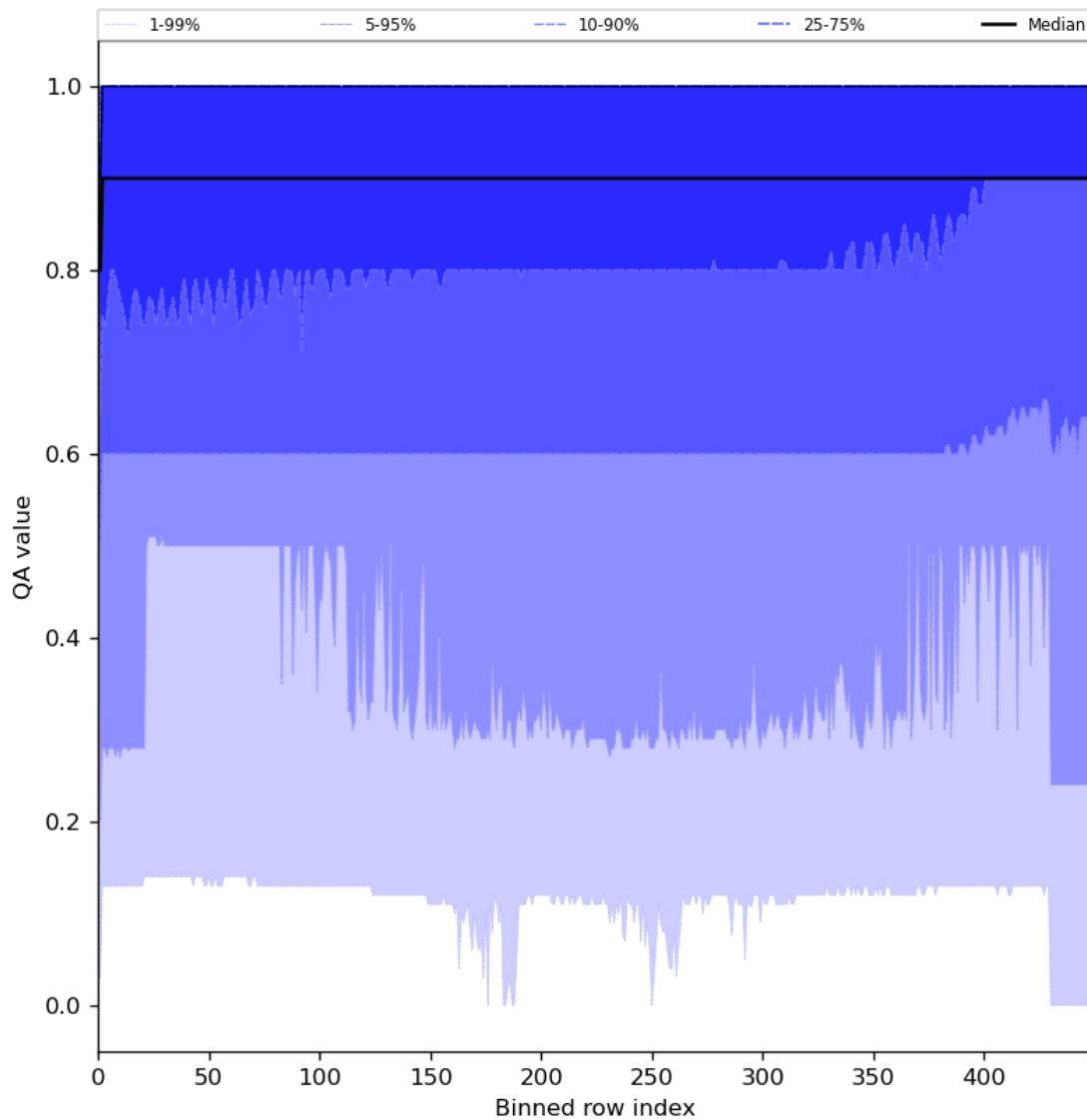
Figure 27: Along track statistics of “QA value” for 2023-12-27 to 2023-12-29
