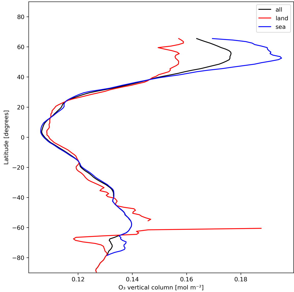
Figure 14: Zonal average of “O 3 vertical column” for 2023-12-27 to 2023-12-29.
