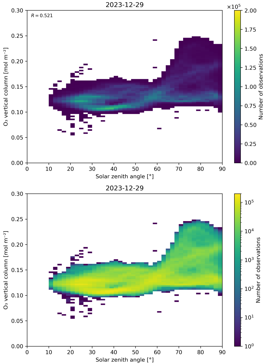
Figure 47: Scatter density plot of “Solar zenith angle” against “O 3 vertical column” for 2023-12-28 to 2023-12-30.
