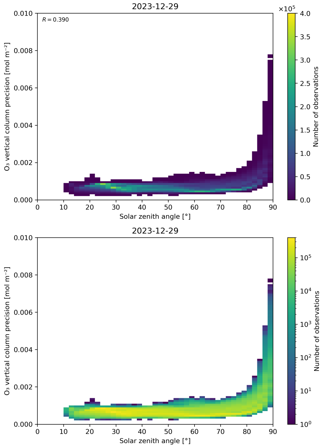
Figure 48: Scatter density plot of “Solar zenith angle” against “O 3 vertical column precision” for 2023-12-28 to 2023-12-30.
