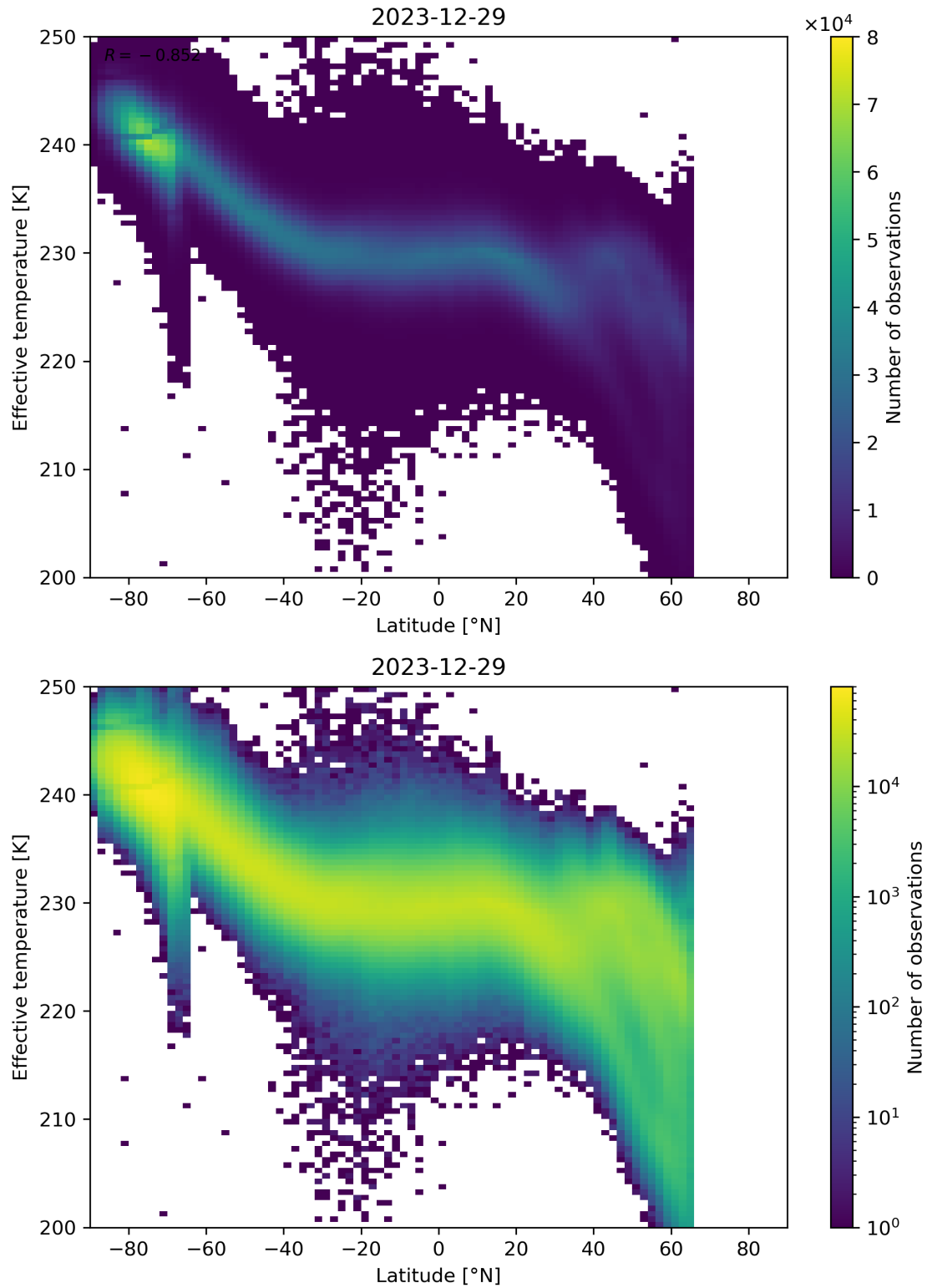
Figure 34: Scatter density plot of “Latitude” against “Effective temperature” for 2023-12-28 to 2023-12-30.
