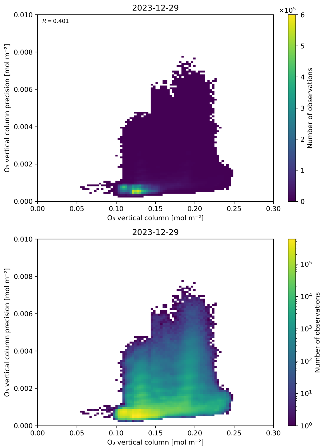
Figure 41: Scatter density plot of “O 3 vertical column” against “O 3 vertical column precision” for 2023-12-28 to 2023-12-30.
