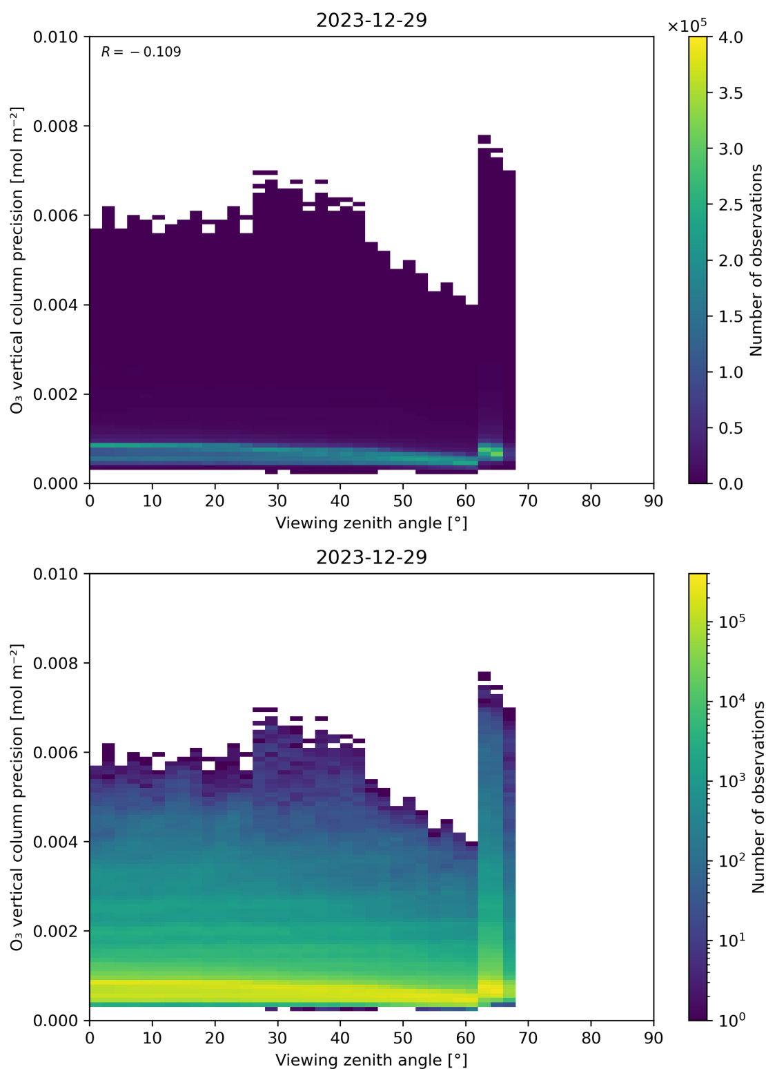
Figure 53: Scatter density plot of “Viewing zenith angle” against “O 3 vertical column precision” for 2023-12-28 to 2023-12-30.
