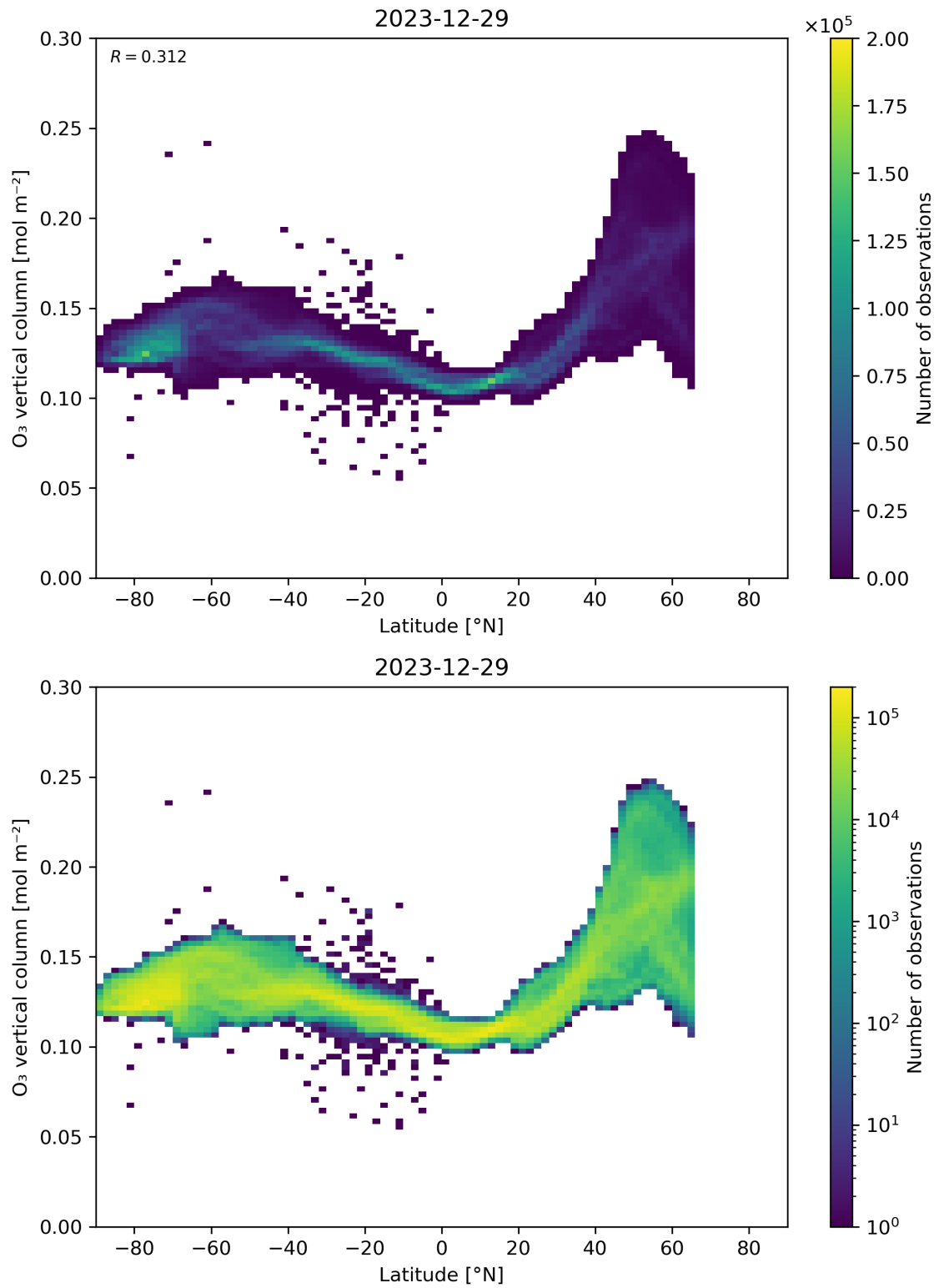
Figure 36: Scatter density plot of “Latitude” against “O 3 vertical column” for 2023-12-28 to 2023-12-30.
