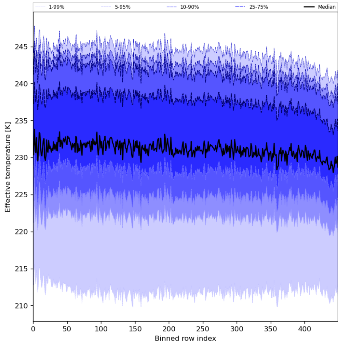
Figure 31: Along track statistics of “Effective temperature” for 2023-12-28 to 2023-12-30
