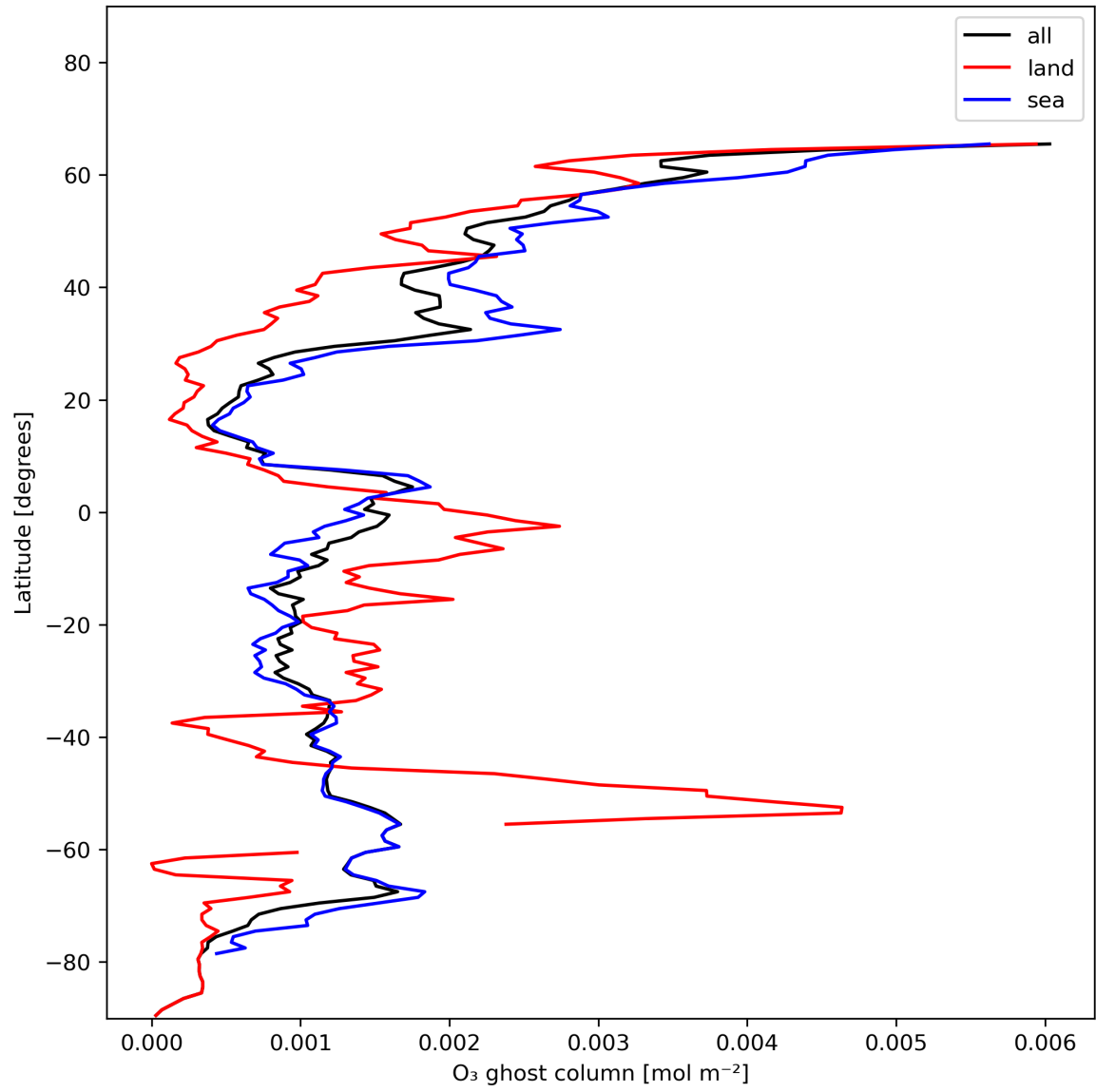
Figure 18: Zonal average of “O 3 ghost column” for 2023-12-28 to 2023-12-30.
