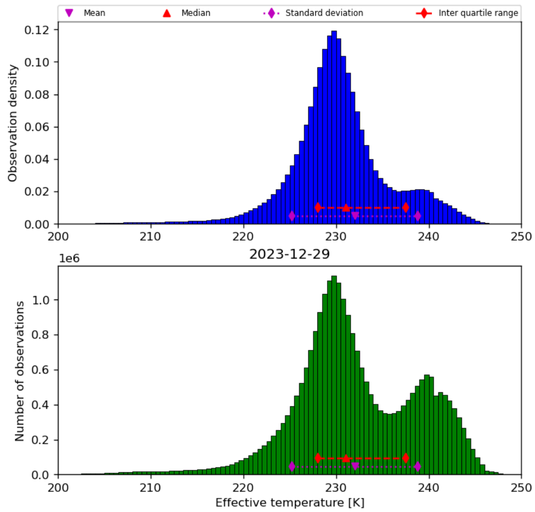
Figure 24: Histogram of “Effective temperature” for 2023-12-28 to 2023-12-30
