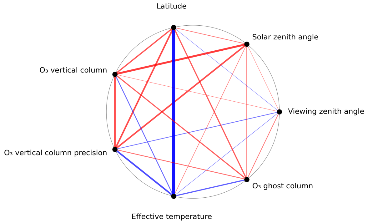
Figure 1: Map of correlation graph for 2023-12-28 to 2023-12-30.
