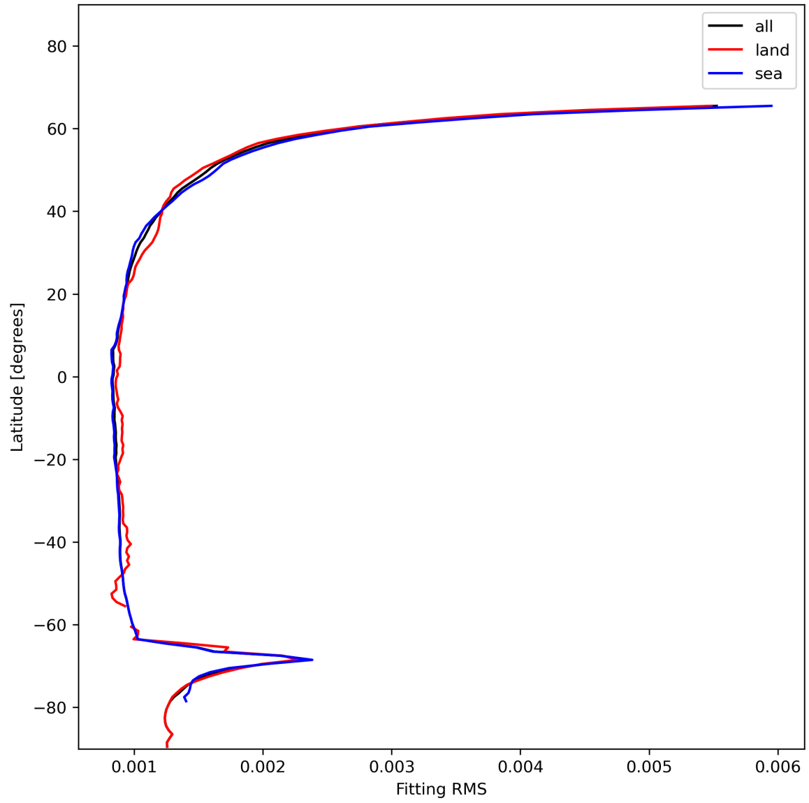
Figure 16: Zonal average of “Fitting RMS” for 2023-12-28 to 2023-12-30.
