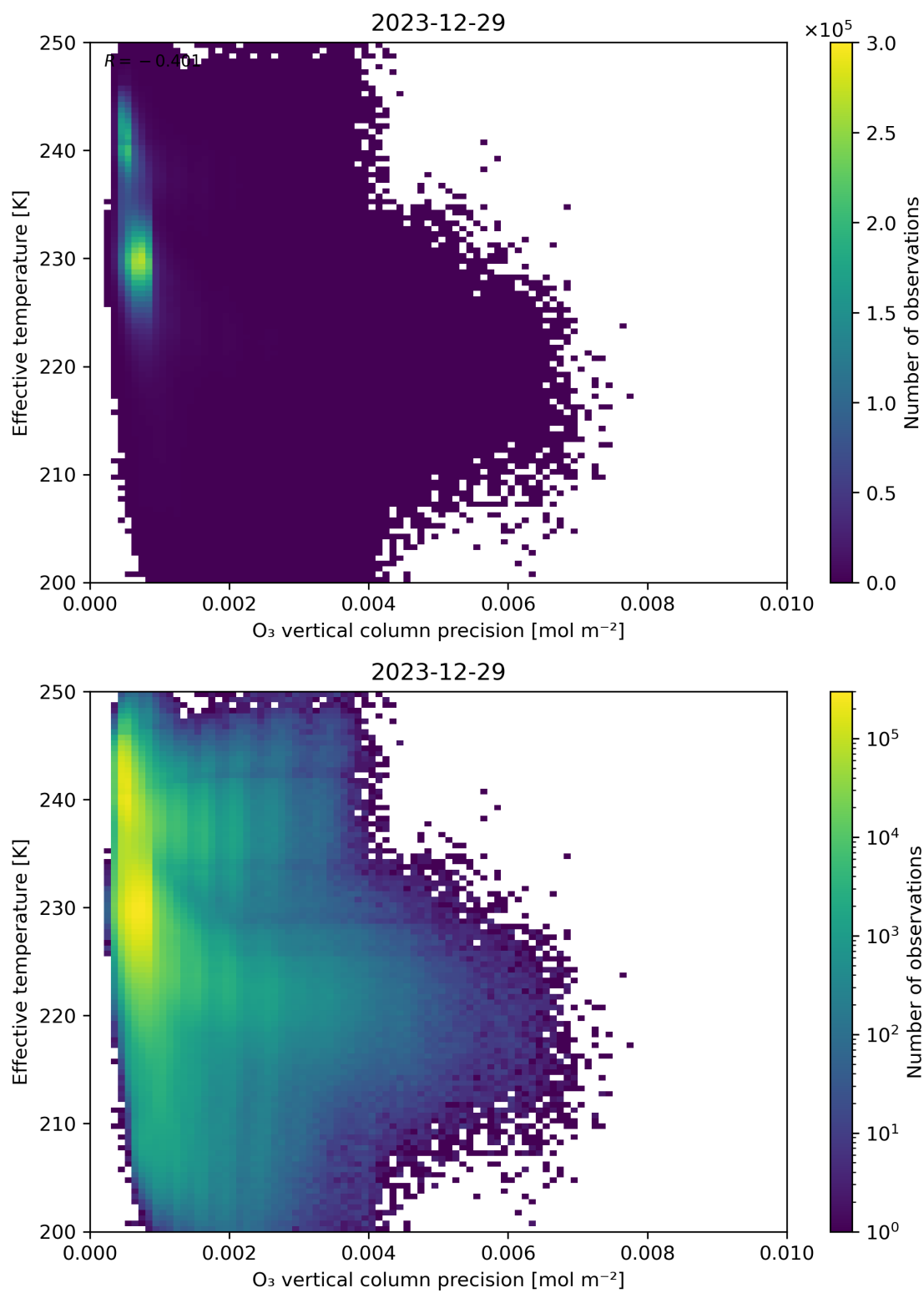
Figure 42: Scatter density plot of “O 3 vertical column precision” against “Effective temperature” for 2023-12-28 to 2023-12-30.
