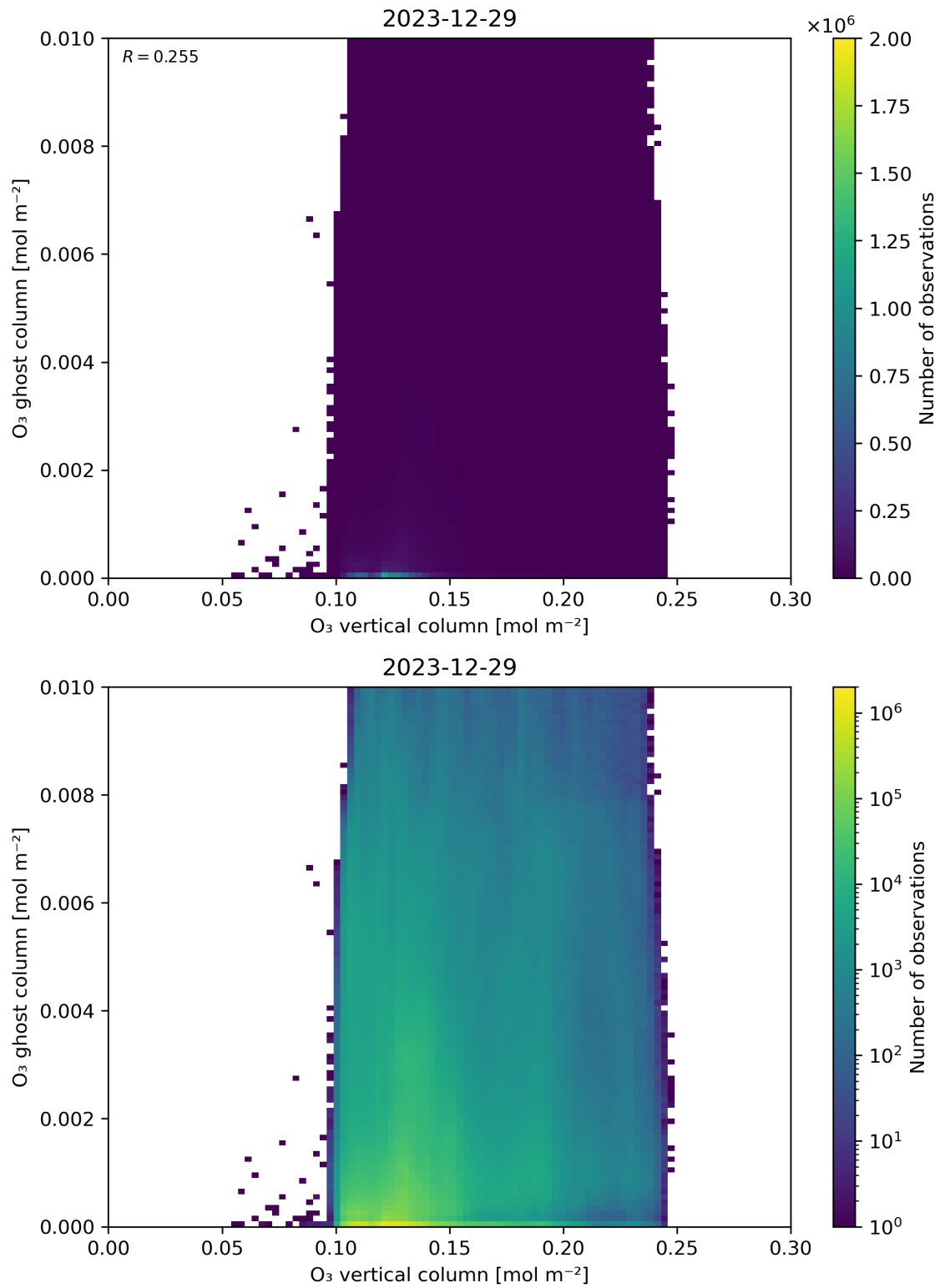
Figure 40: Scatter density plot of “O 3 vertical column” against “O 3 ghost column” for 2023-12-28 to 2023-12-30.
