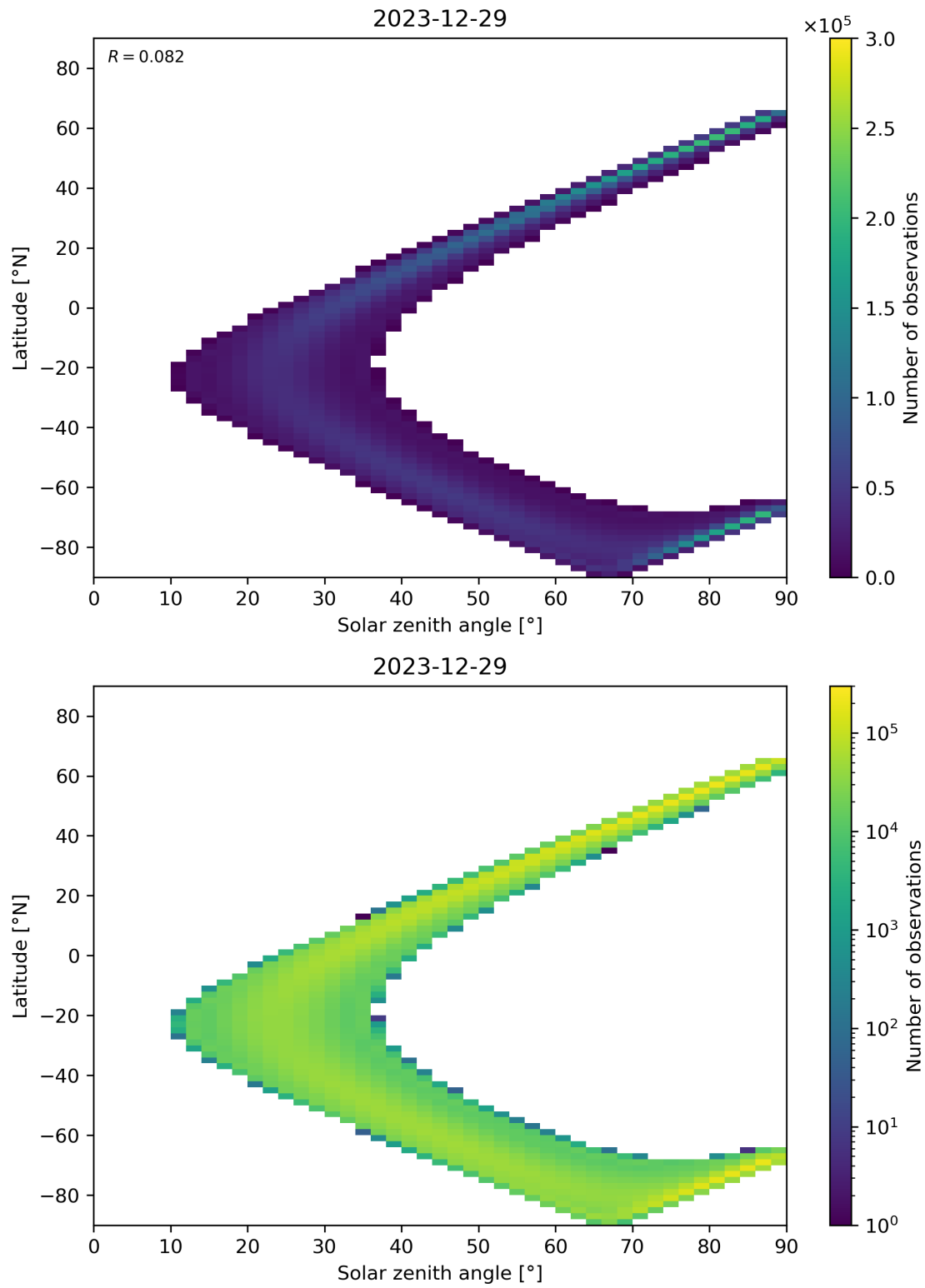
Figure 44: Scatter density plot of “Solar zenith angle” against “Latitude” for 2023-12-28 to 2023-12-30.
