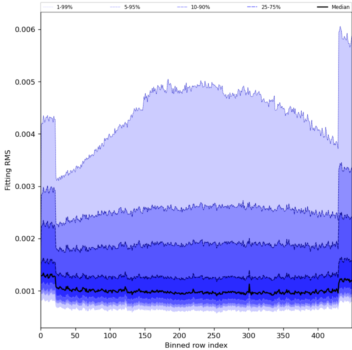
Figure 30: Along track statistics of “Fitting RMS” for 2023-12-28 to 2023-12-30
