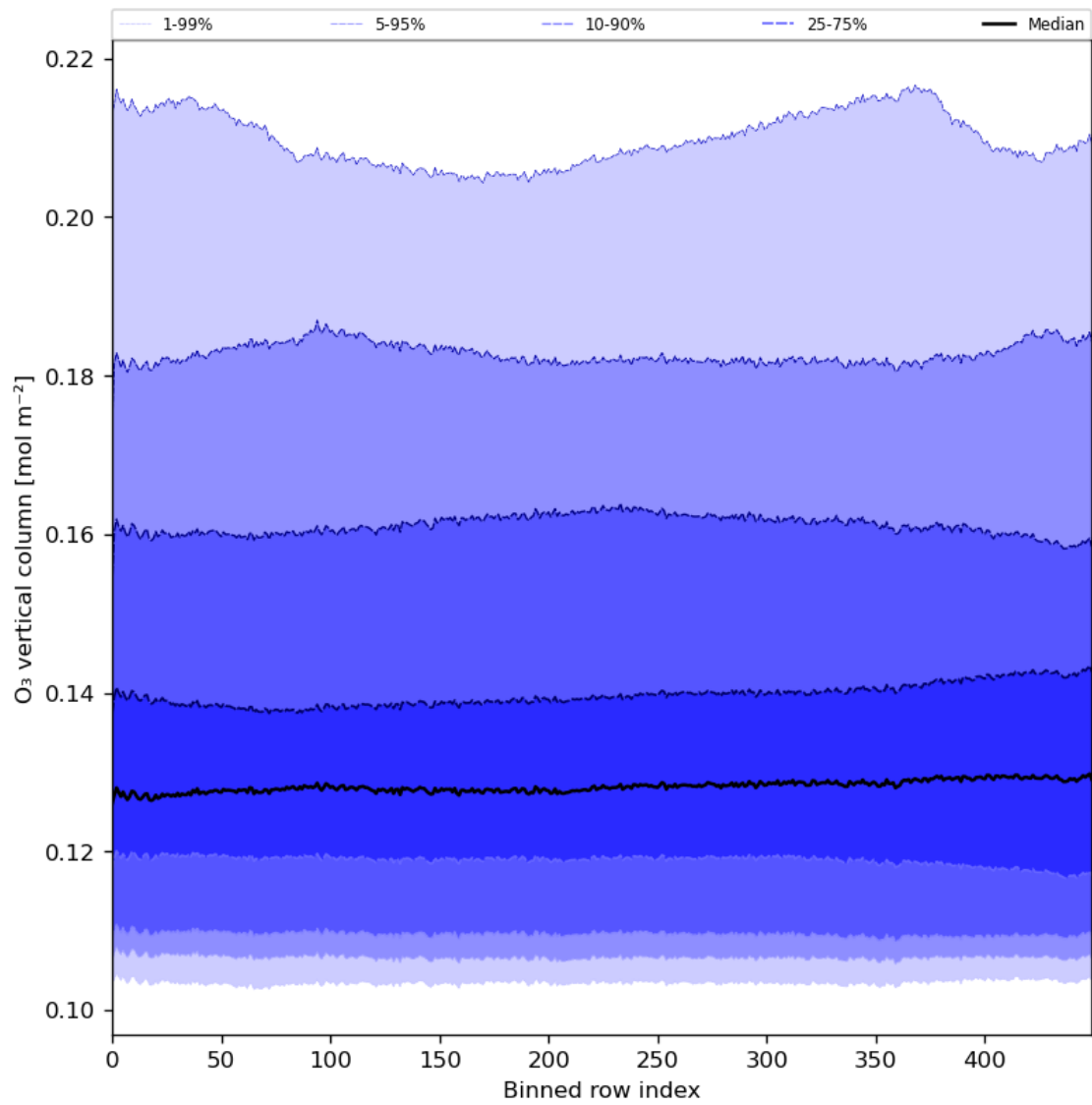
Figure 28: Along track statistics of “O 3 vertical column” for 2023-12-28 to 2023-12-30
