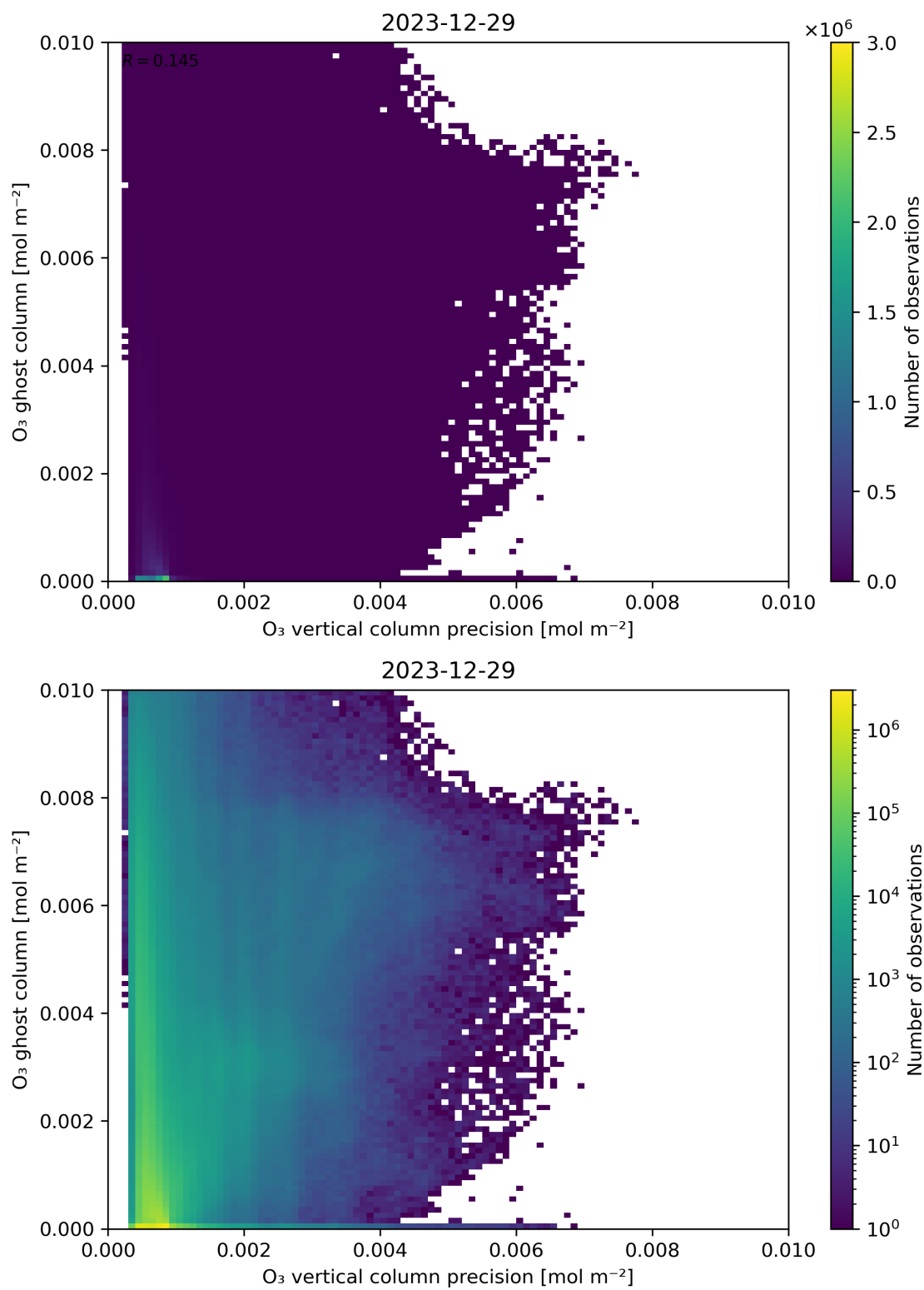
Figure 43: Scatter density plot of “ \text{O}_3 vertical column precision” against “ \text{O}_3 ghost column” for 2023-12-28 to 2023-12-30.
