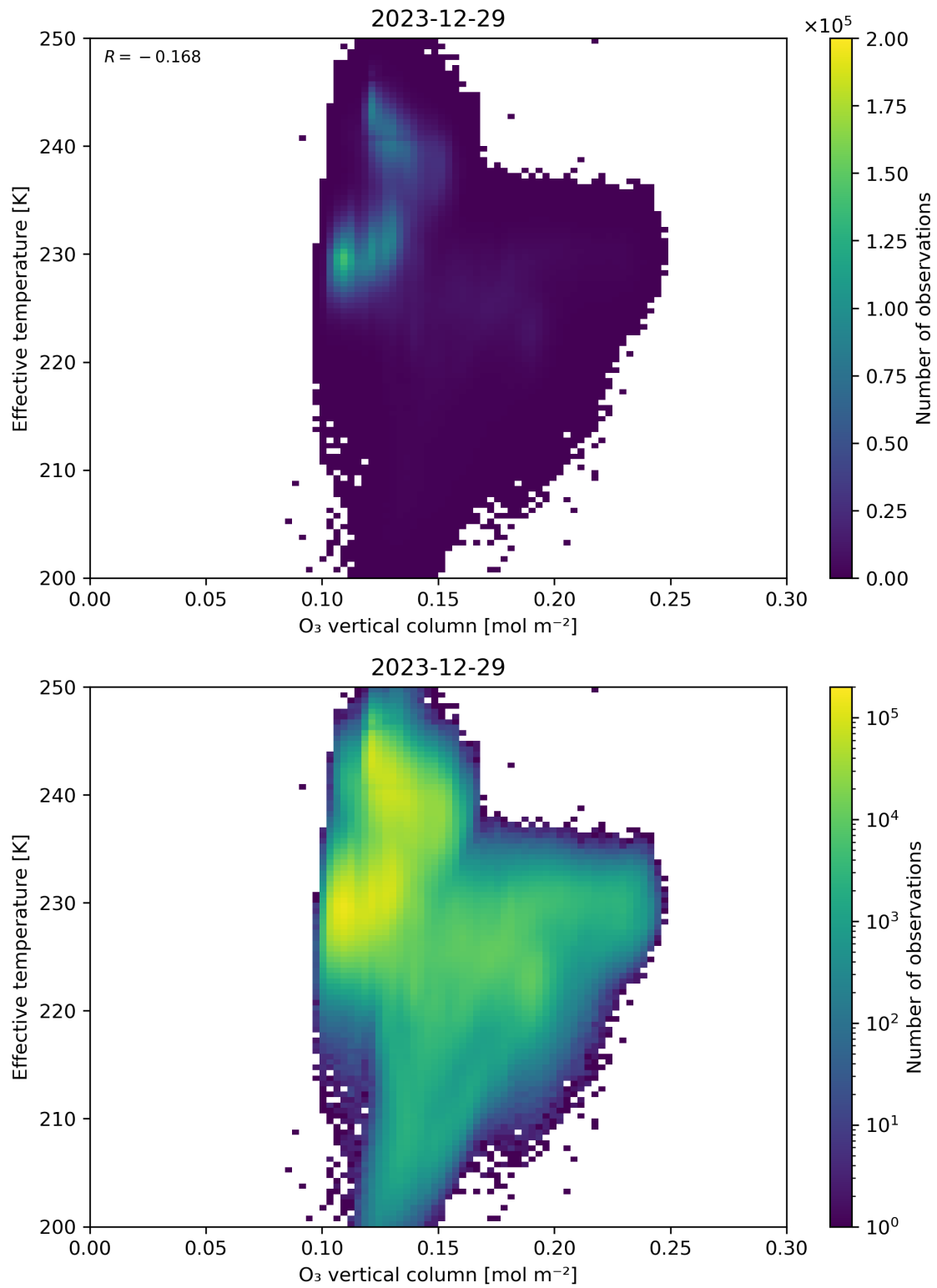
Figure 39: Scatter density plot of “O 3 vertical column” against “Effective temperature” for 2023-12-28 to 2023-12-30.
