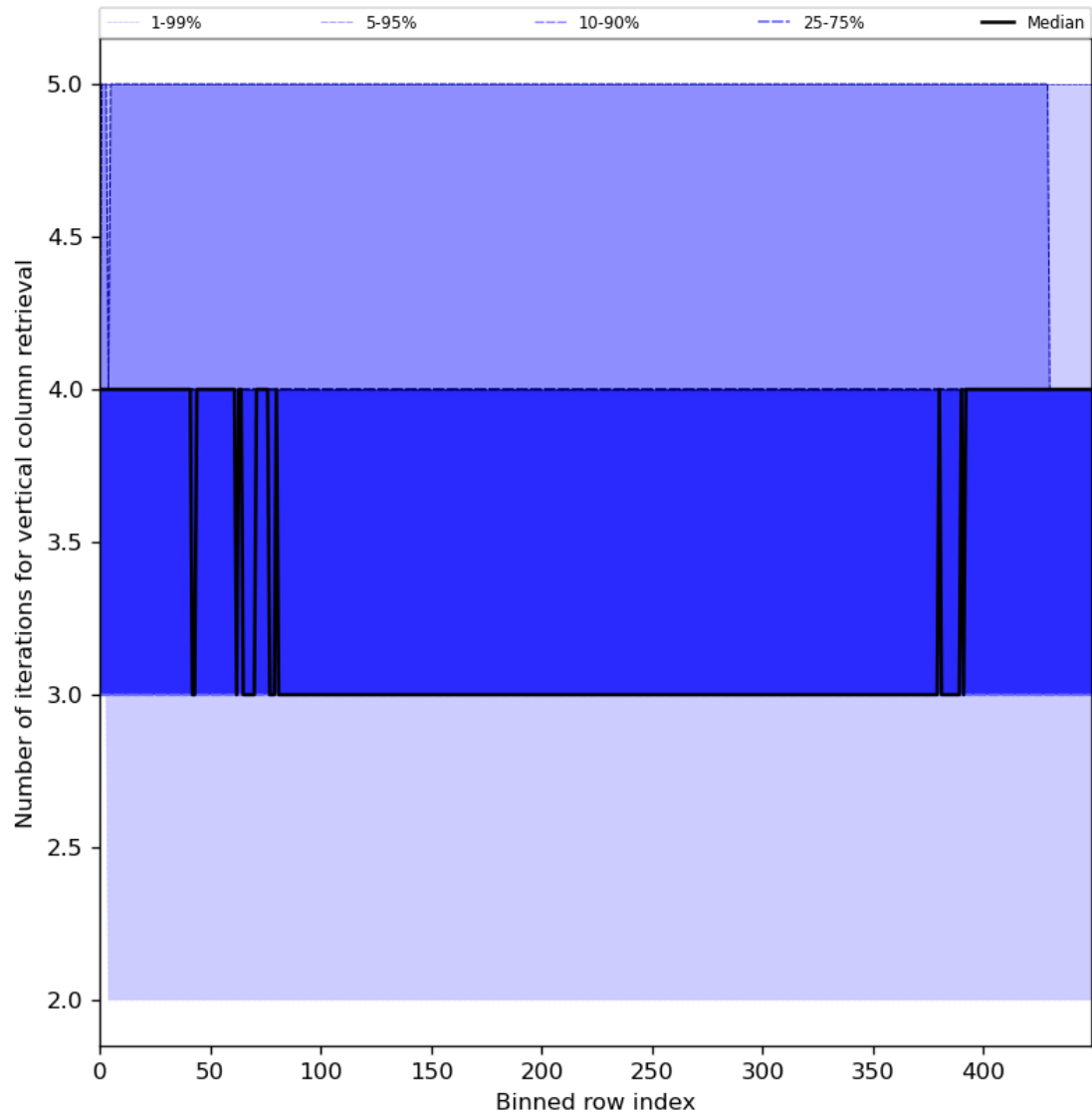
Figure 33: Along track statistics of “Number of iterations for vertical column retrieval” for 2023-12-28 to 2023-12-30
