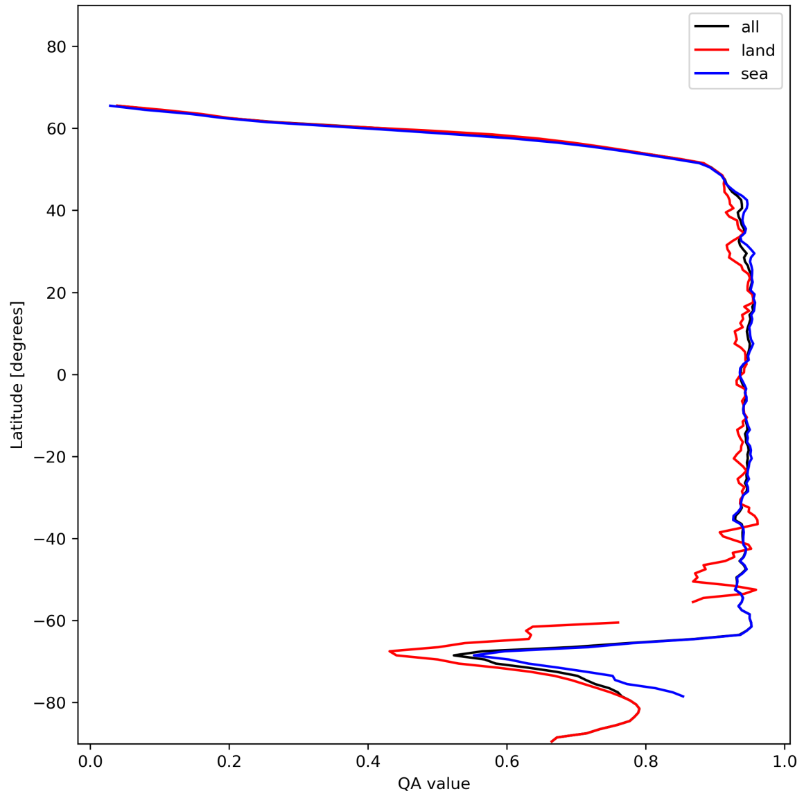
Figure 13: Zonal average of “QA value” for 2023-12-28 to 2023-12-30.
