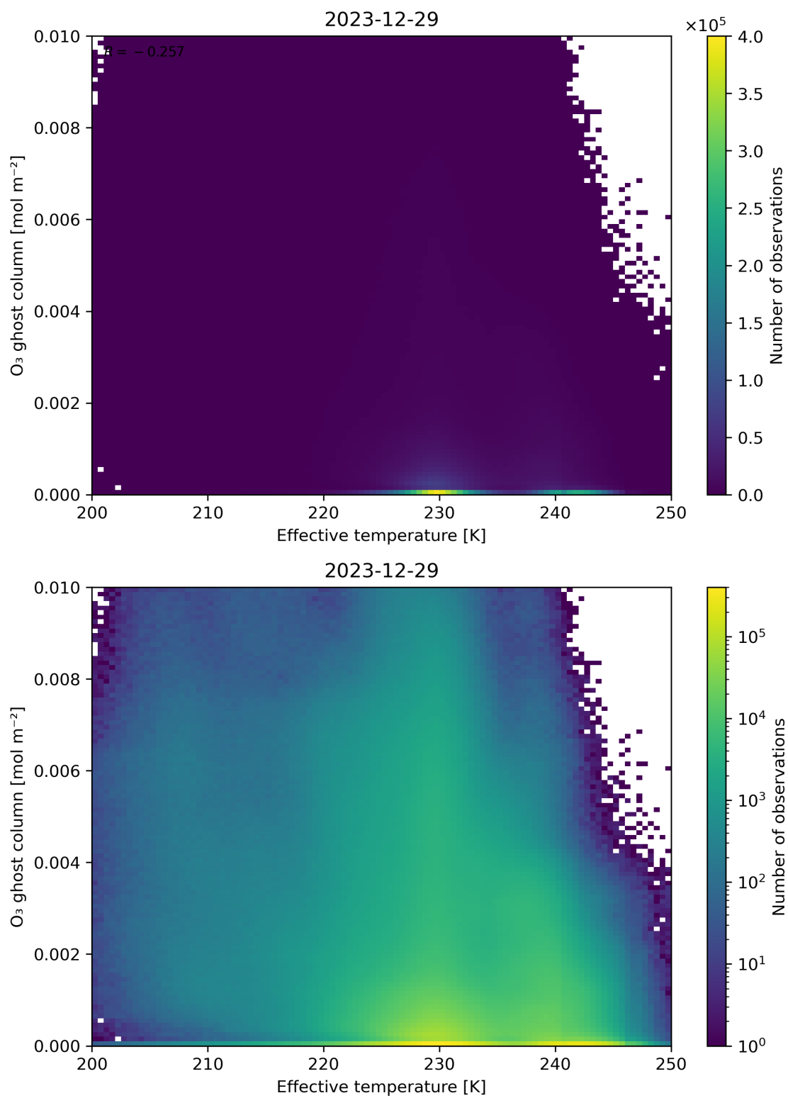
Figure 38: Scatter density plot of “Effective temperature” against “O 3 ghost column” for 2023-12-28 to 2023-12-30.
