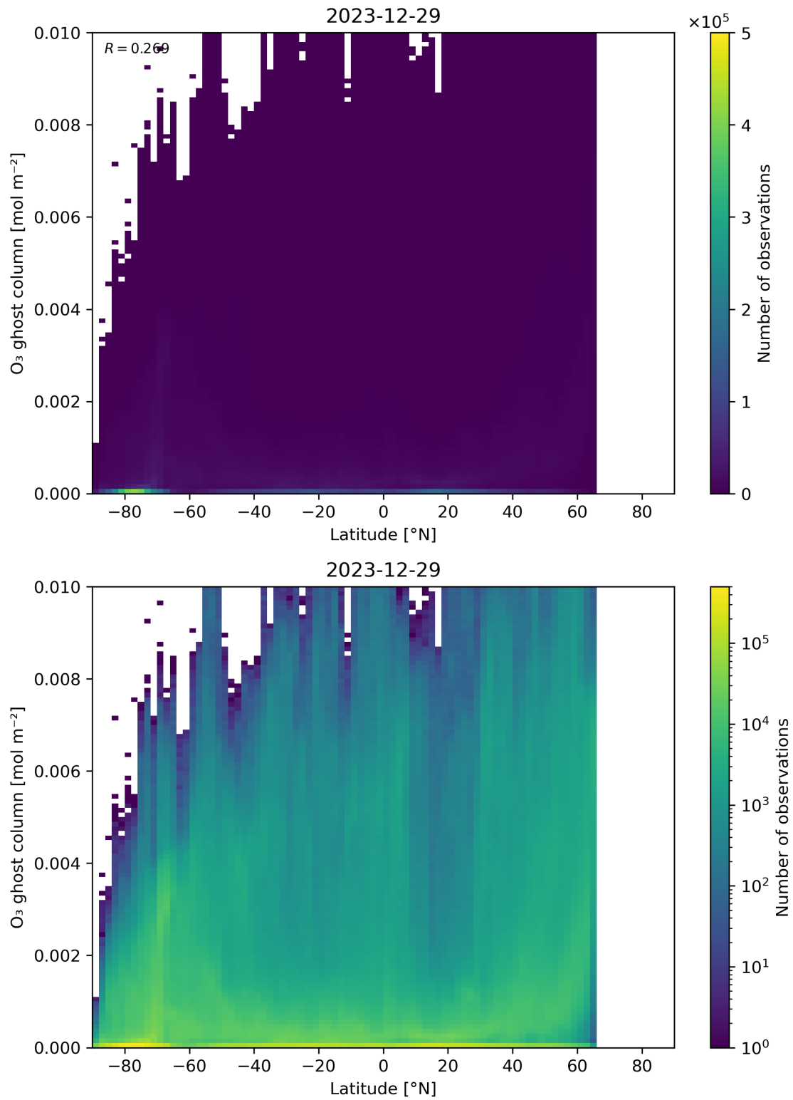
Figure 35: Scatter density plot of “Latitude” against “O 3 ghost column” for 2023-12-28 to 2023-12-30.
