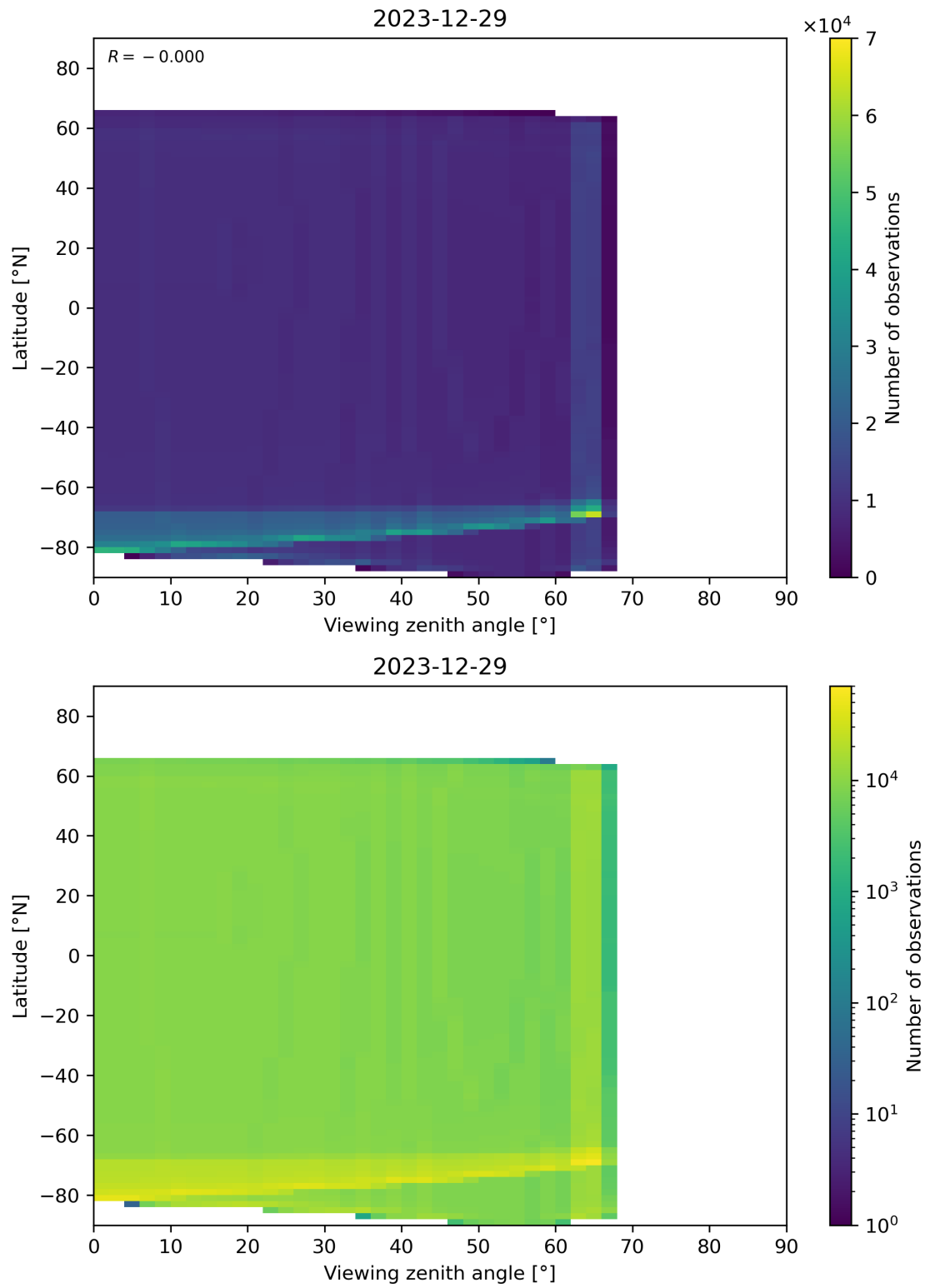
Figure 49: Scatter density plot of “Viewing zenith angle” against “Latitude” for 2023-12-28 to 2023-12-30.
