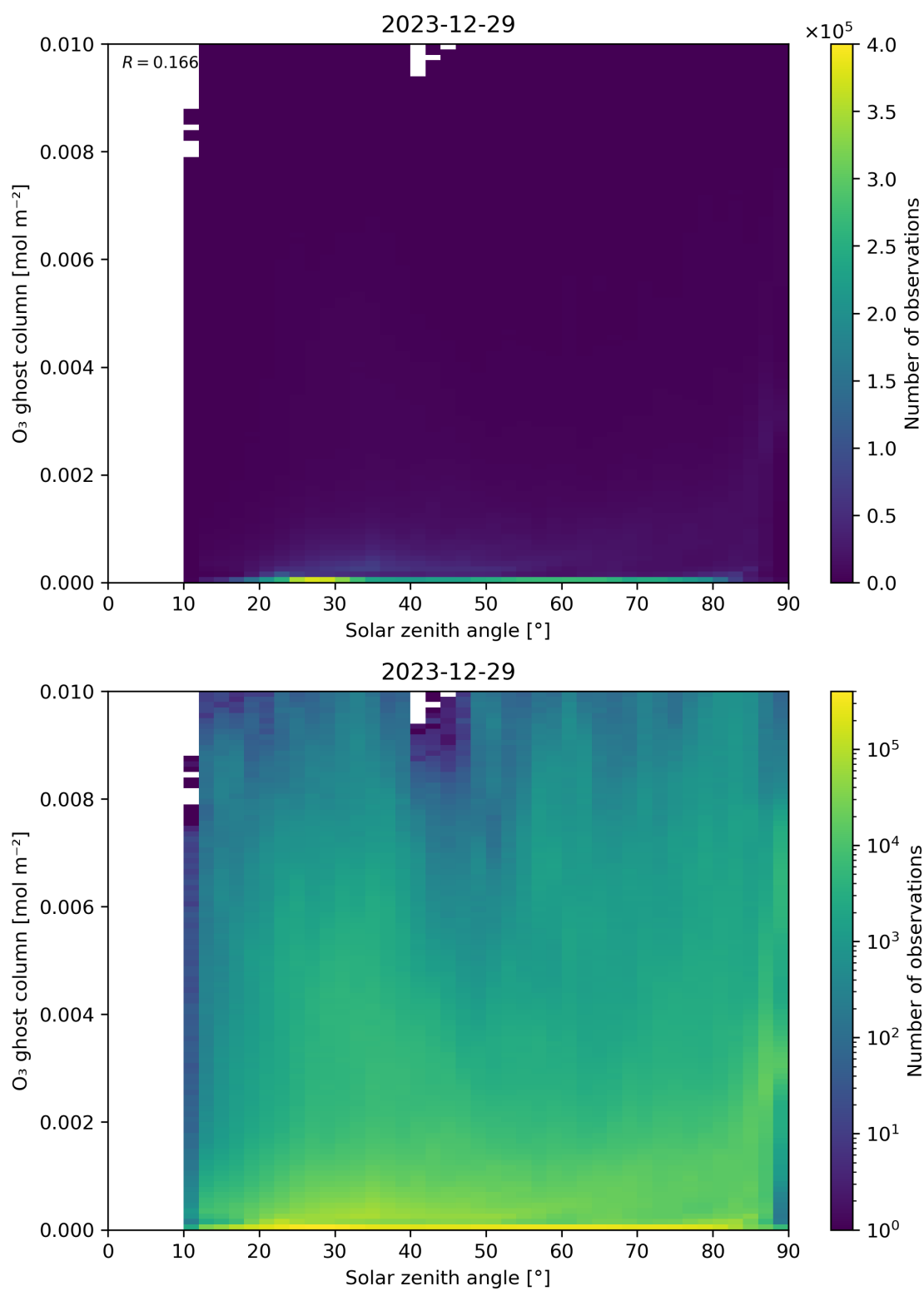
Figure 46: Scatter density plot of “Solar zenith angle” against “O 3 ghost column” for 2023-12-28 to 2023-12-30.
