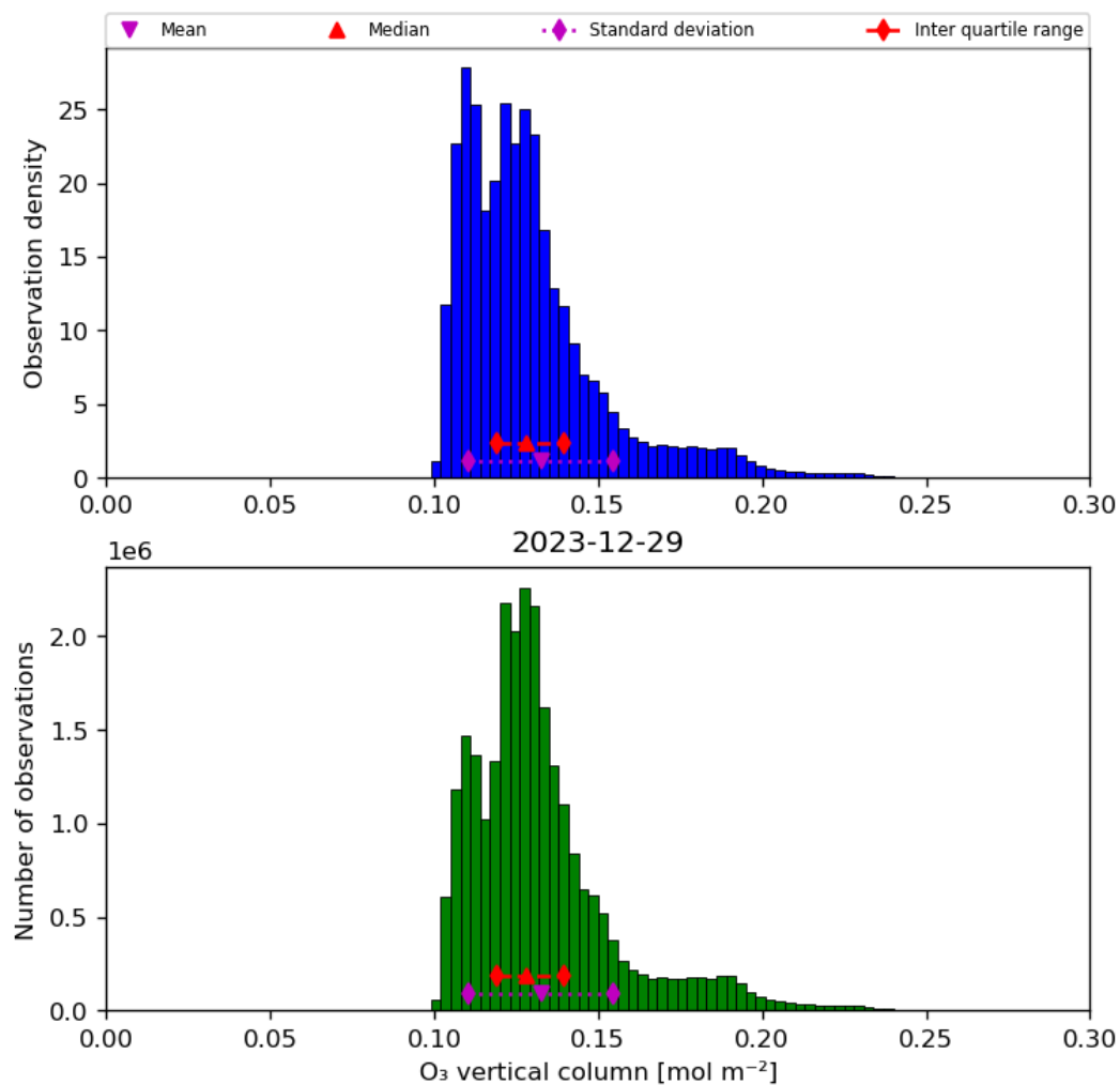
Figure 21: Histogram of “O 3 vertical column” for 2023-12-28 to 2023-12-30
