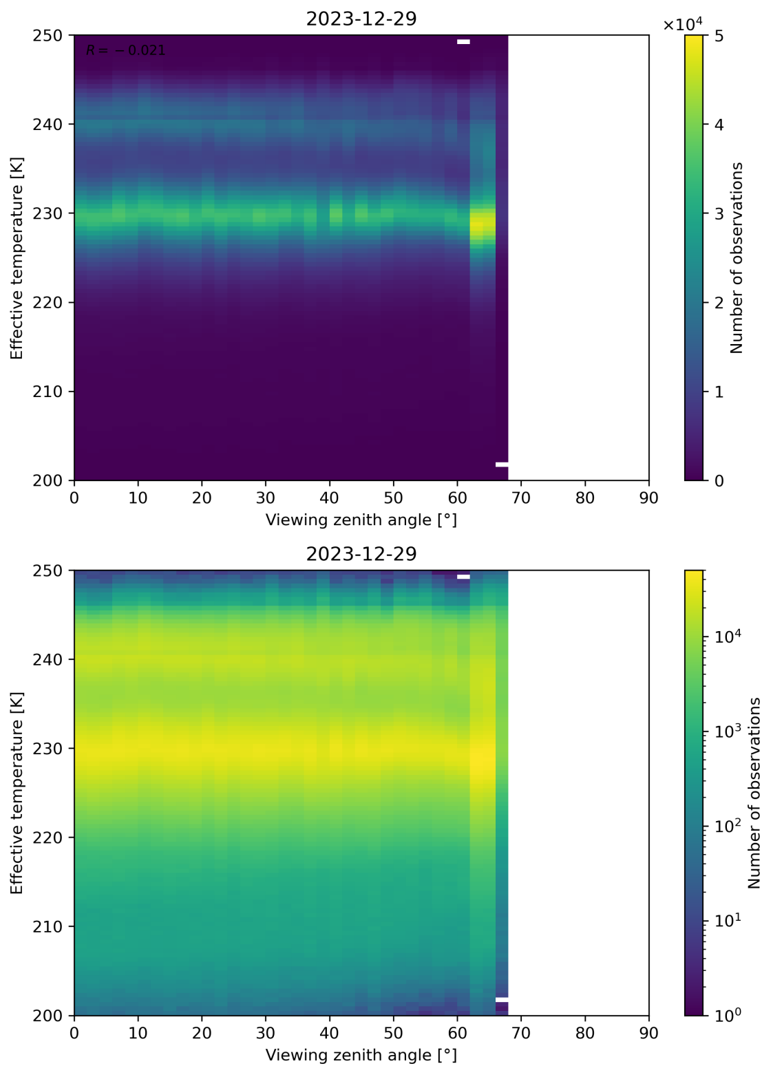
Figure 50: Scatter density plot of “Viewing zenith angle” against “Effective temperature” for 2023-12-28 to 2023-12-30.
