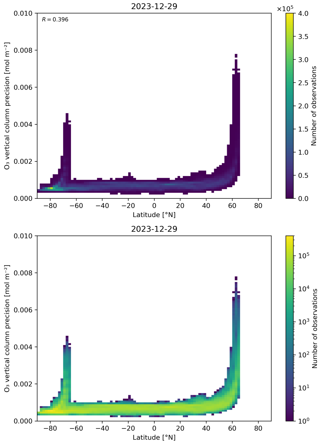
Figure 37: Scatter density plot of “Latitude” against “O 3 vertical column precision” for 2023-12-28 to 2023-12-30.
