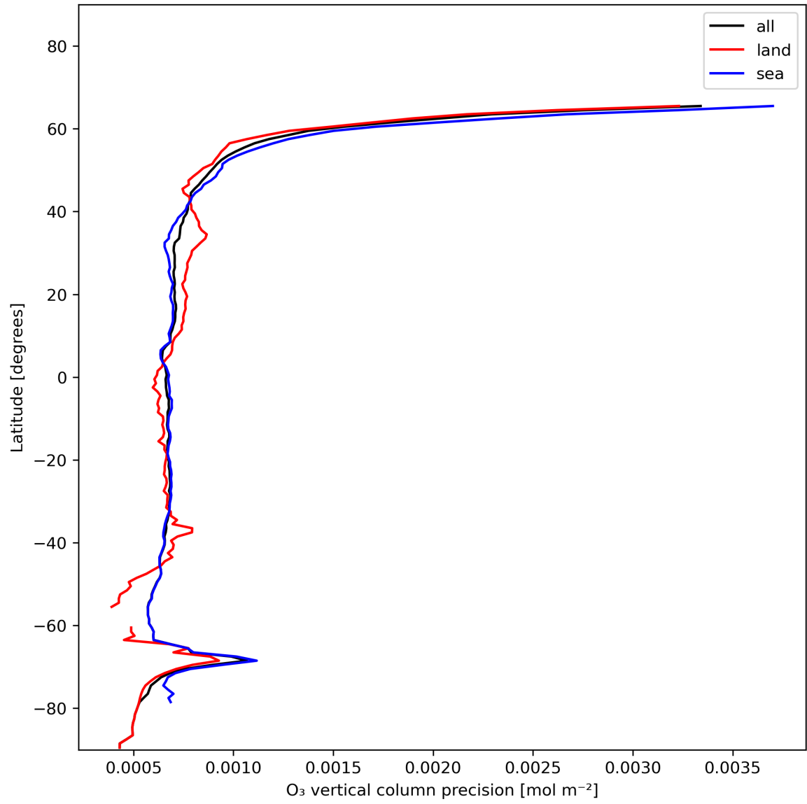
Figure 15: Zonal average of “O 3 vertical column precision” for 2023-12-28 to 2023-12-30.
