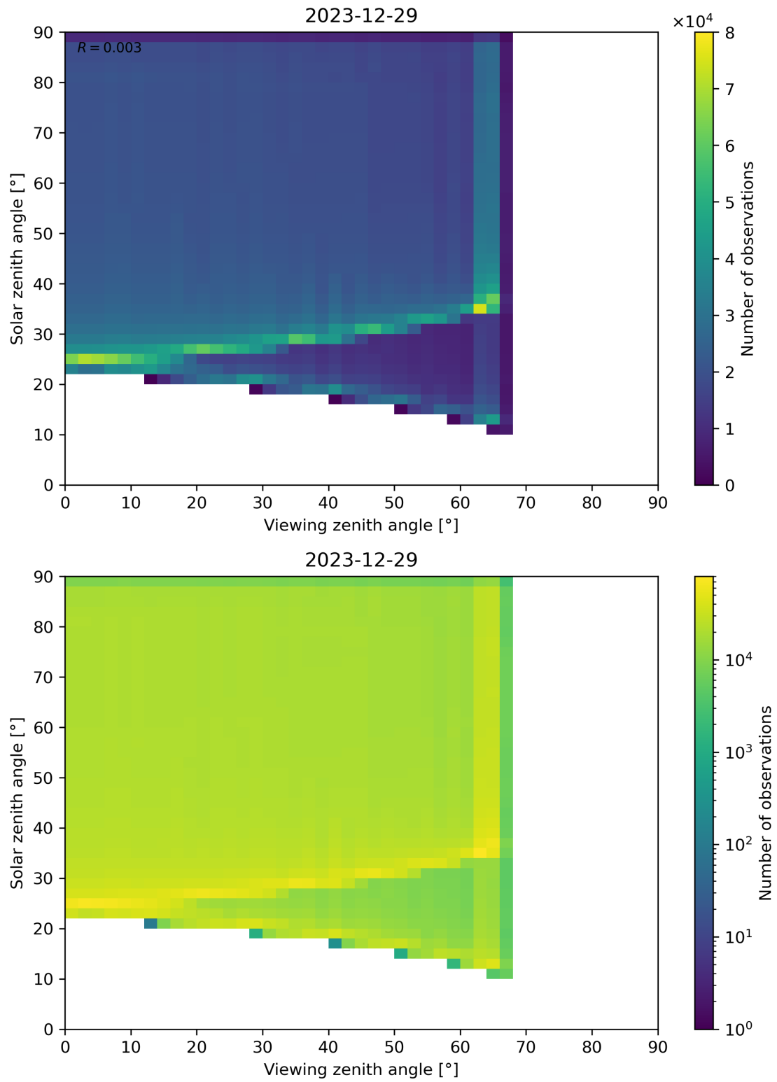
Figure 54: Scatter density plot of “Viewing zenith angle” against “Solar zenith angle” for 2023-12-28 to 2023-12-30.
