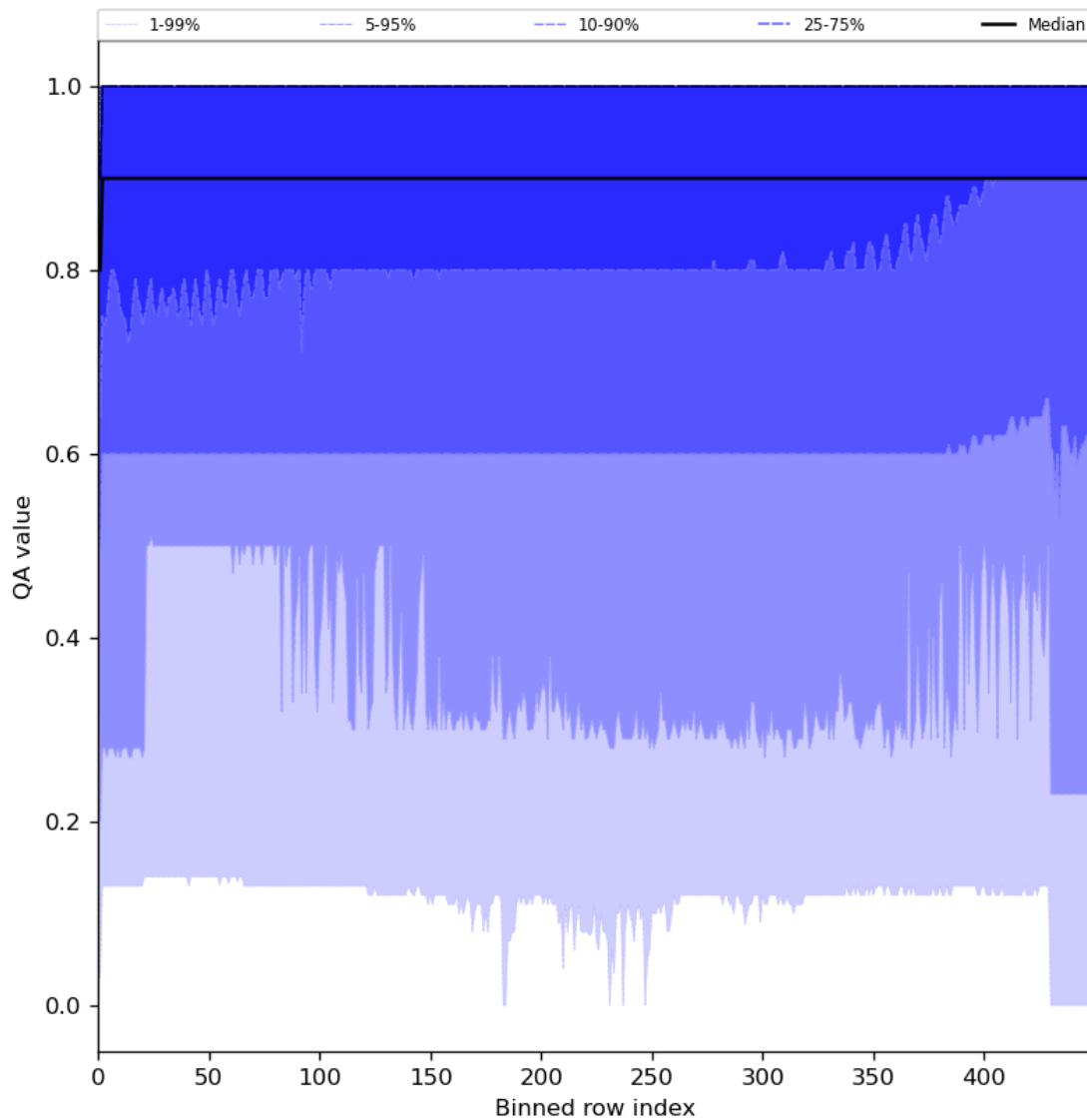
Figure 27: Along track statistics of “QA value” for 2023-12-28 to 2023-12-30
