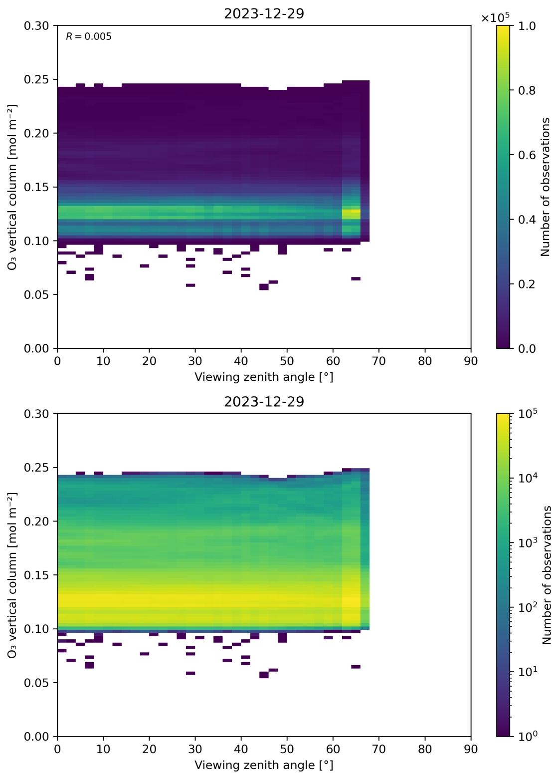
Figure 52: Scatter density plot of “Viewing zenith angle” against “O 3 vertical column” for 2023-12-28 to 2023-12-30.
