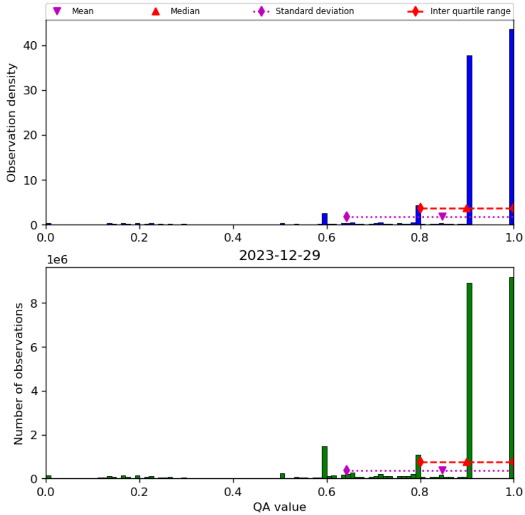
Figure 20: Histogram of “QA value” for 2023-12-28 to 2023-12-30
