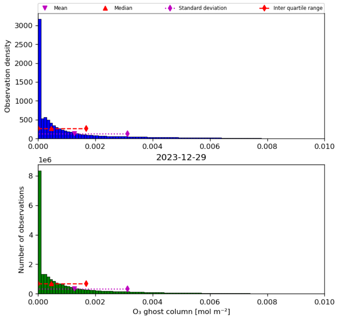
Figure 25: Histogram of "O 3 ghost column" for 2023-12-28 to 2023-12-30
