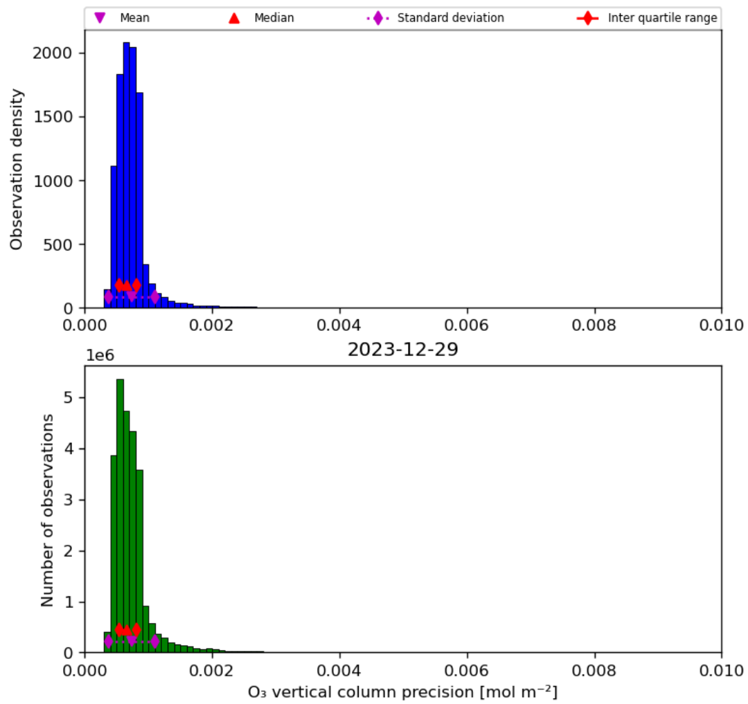
Figure 22: Histogram of “O 3 vertical column precision” for 2023-12-28 to 2023-12-30
