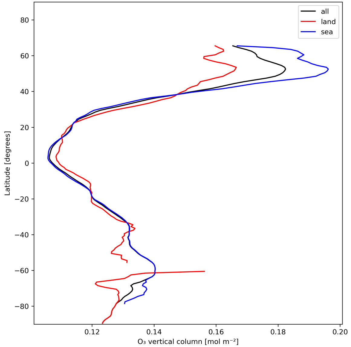
Figure 14: Zonal average of “O 3 vertical column” for 2023-12-28 to 2023-12-30.
