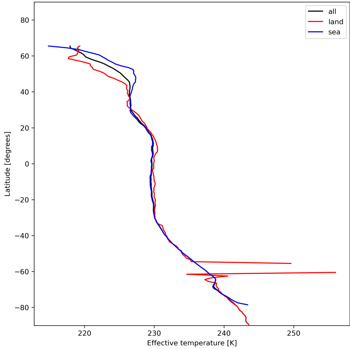
Figure 17: Zonal average of “Effective temperature” for 2023-12-28 to 2023-12-30.
