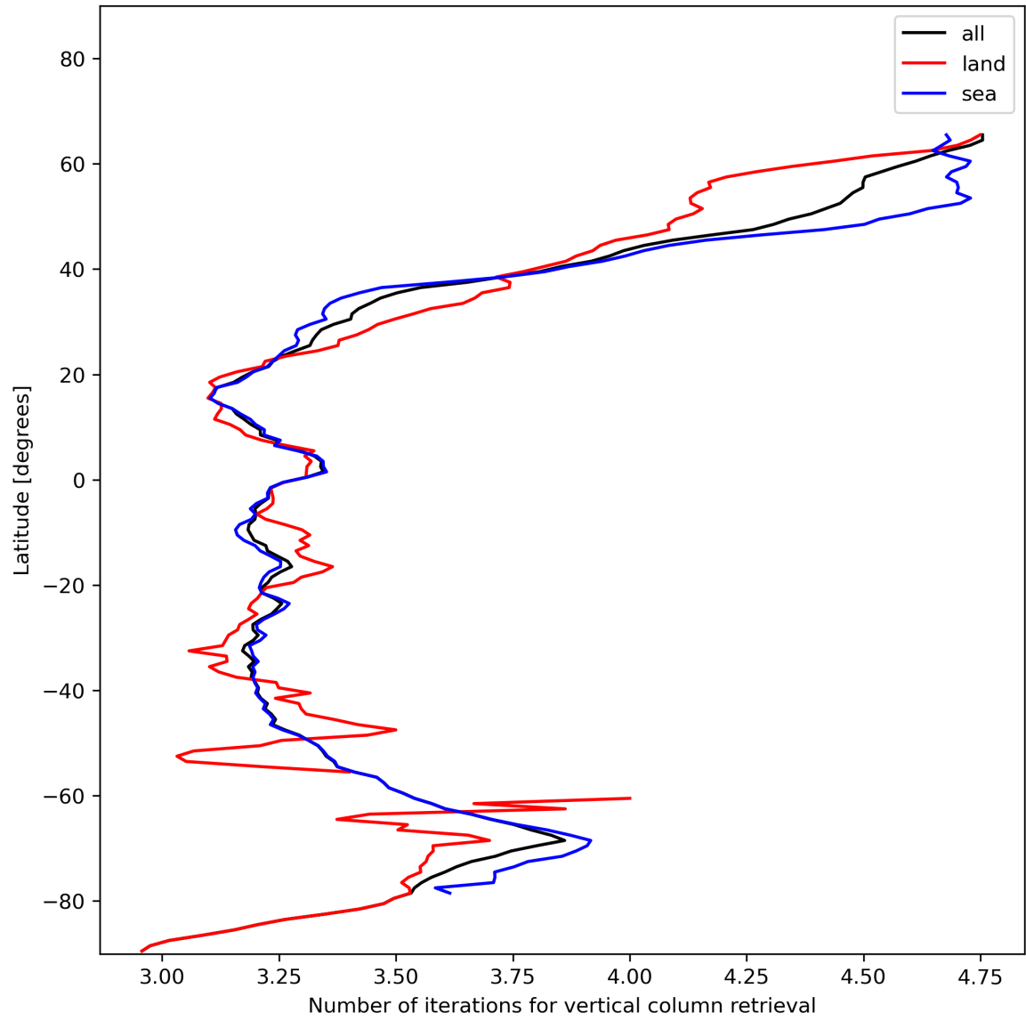
Figure 19: Zonal average of “Number of iterations for vertical column retrieval” for 2023-12-28 to 2023-12-30.
