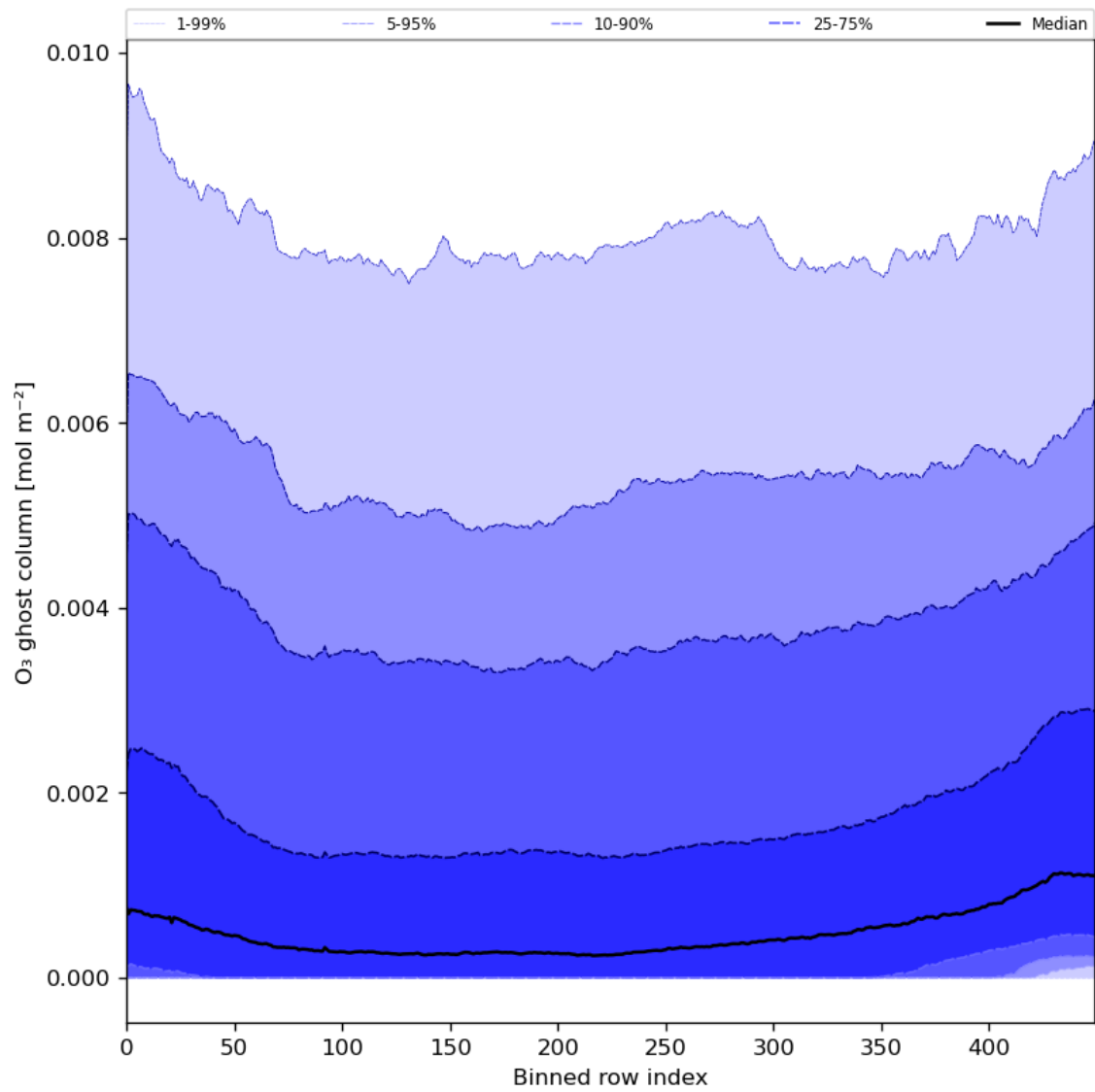
Figure 32: Along track statistics of “O 3 ghost column” for 2023-12-28 to 2023-12-30
