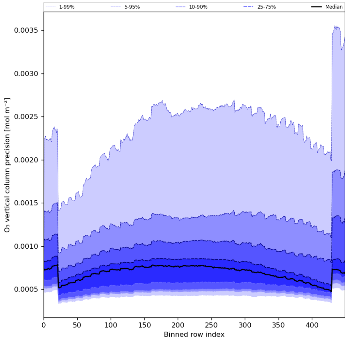
Figure 29: Along track statistics of “O 3 vertical column precision” for 2023-12-28 to 2023-12-30
