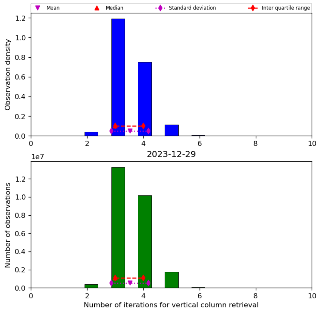
Figure 26: Histogram of “Number of iterations for vertical column retrieval” for 2023-12-28 to 2023-12-30
