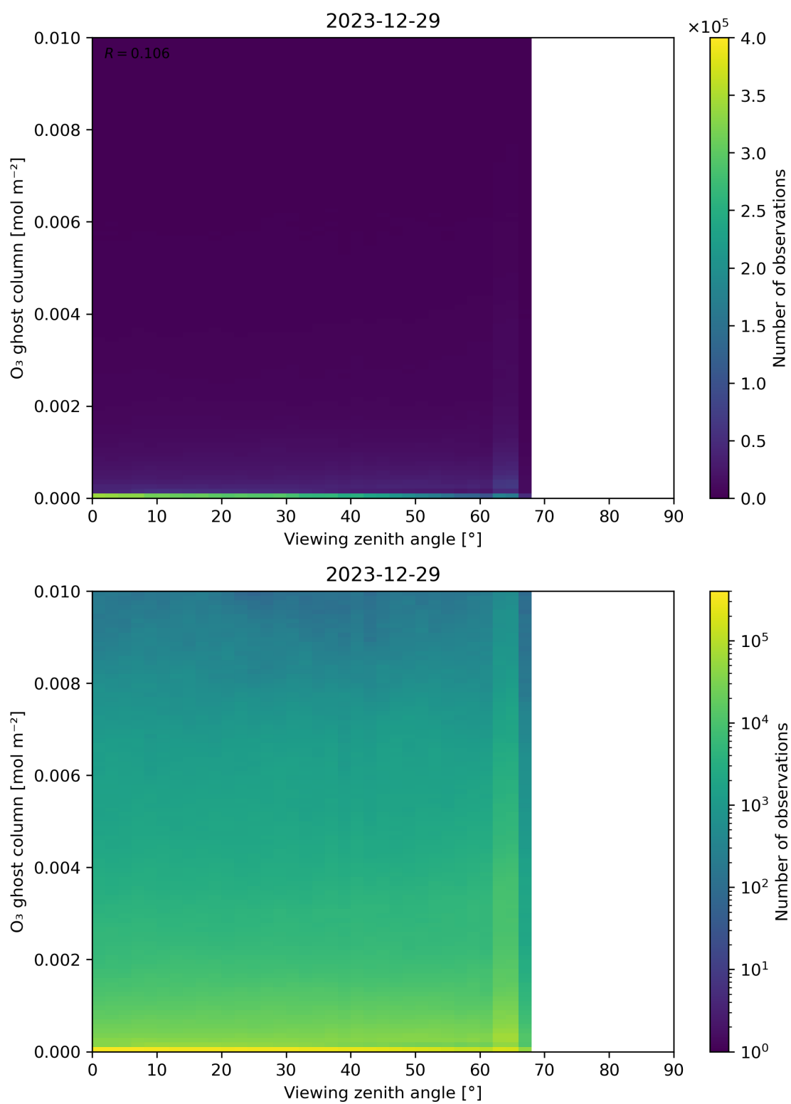
Figure 51: Scatter density plot of “Viewing zenith angle” against “O 3 ghost column” for 2023-12-28 to 2023-12-30.
