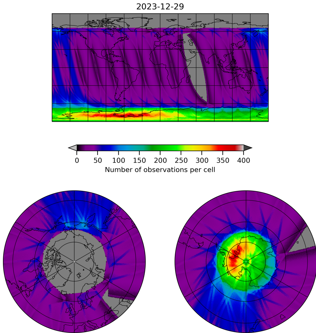
Figure 12: Map of the number of observations for 2023-12-28 to 2023-12-30
