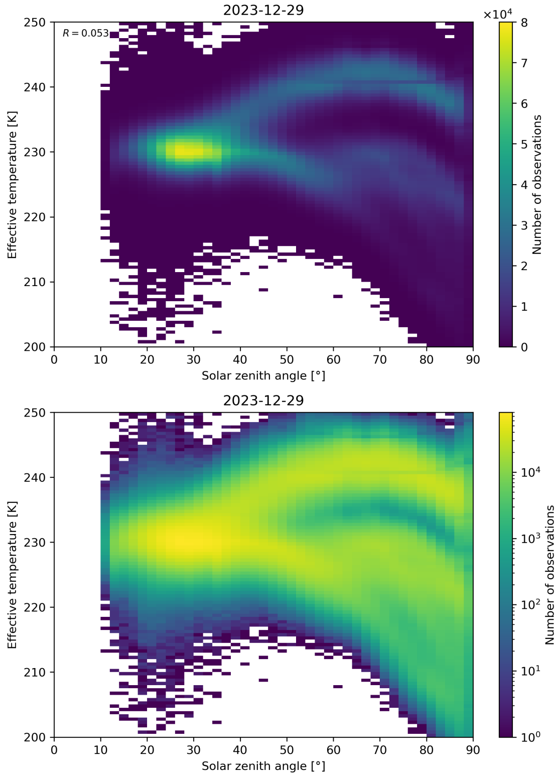
Figure 45: Scatter density plot of “Solar zenith angle” against “Effective temperature” for 2023-12-28 to 2023-12-30.
