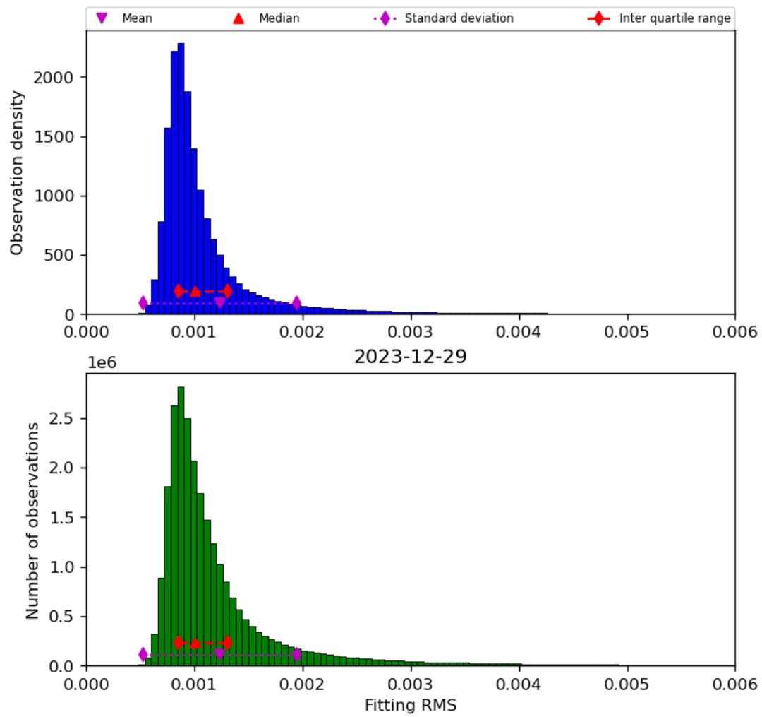
Figure 23: Histogram of “Fitting RMS” for 2023-12-28 to 2023-12-30
