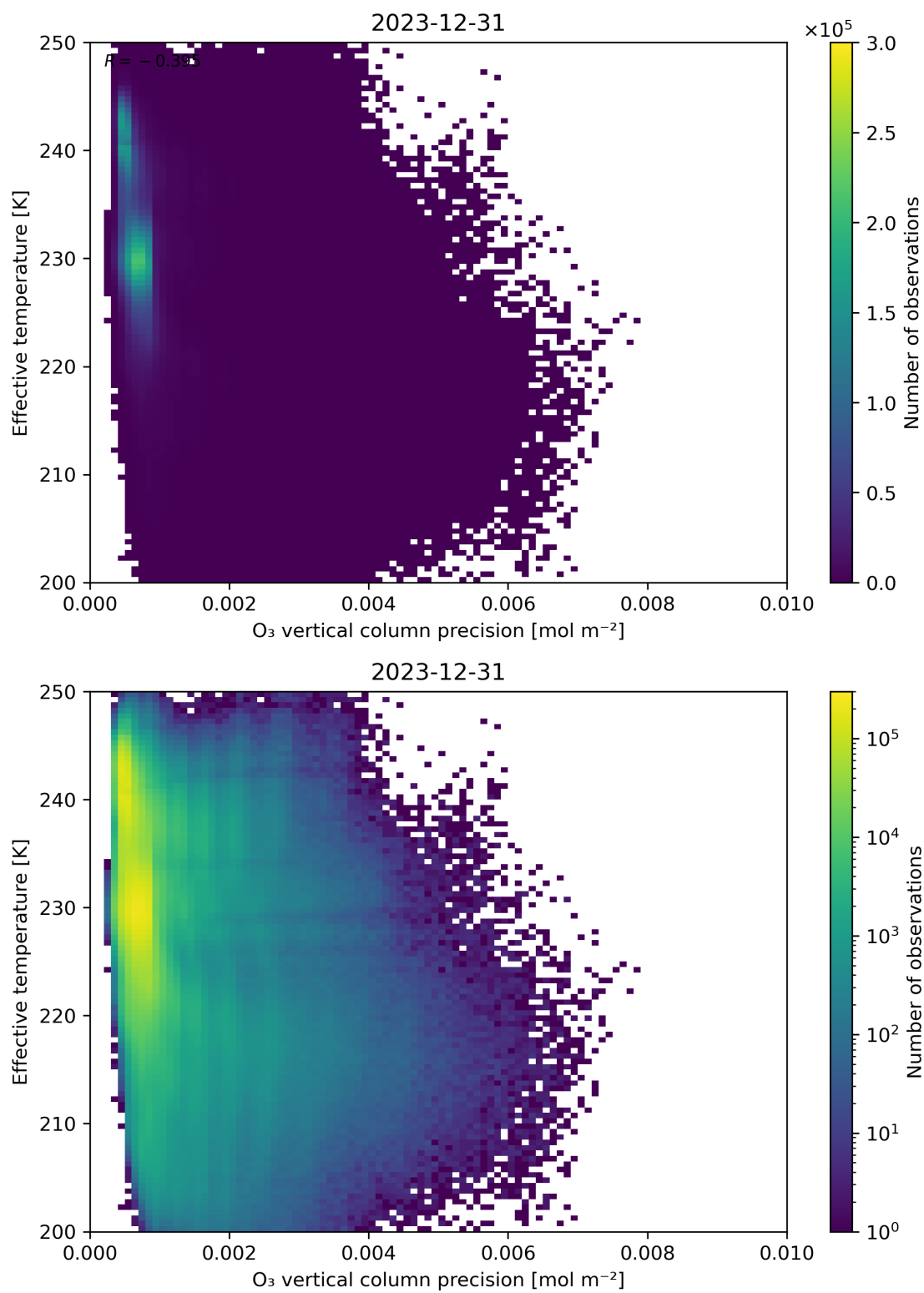
Figure 42: Scatter density plot of “O 3 vertical column precision” against “Effective temperature” for 2023-12-30 to 2023-12-31.
