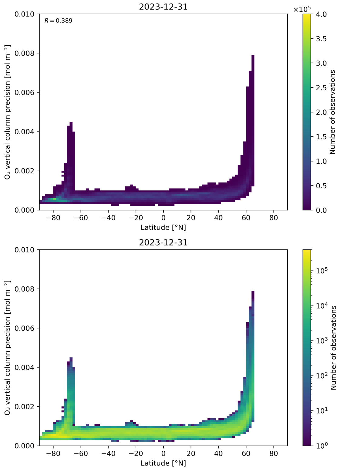
Figure 37: Scatter density plot of “Latitude” against “O 3 vertical column precision” for 2023-12-30 to 2023-12-31.
