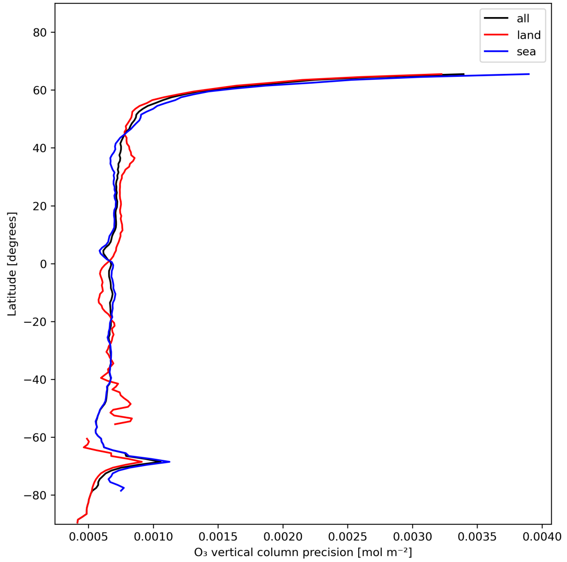
Figure 15: Zonal average of “O 3 vertical column precision” for 2023-12-30 to 2023-12-31.
