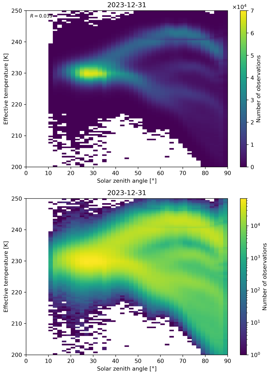
Figure 45: Scatter density plot of “Solar zenith angle” against “Effective temperature” for 2023-12-30 to 2023-12-31.
