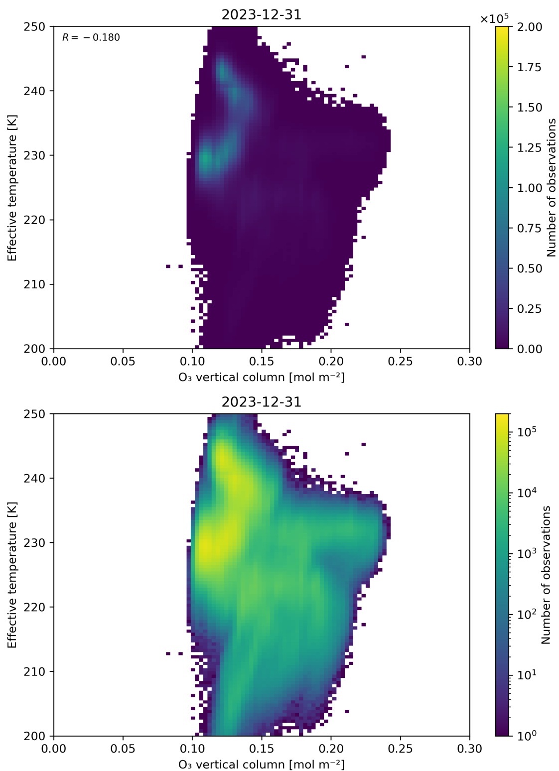
Figure 39: Scatter density plot of “O 3 vertical column” against “Effective temperature” for 2023-12-30 to 2023-12-31.
