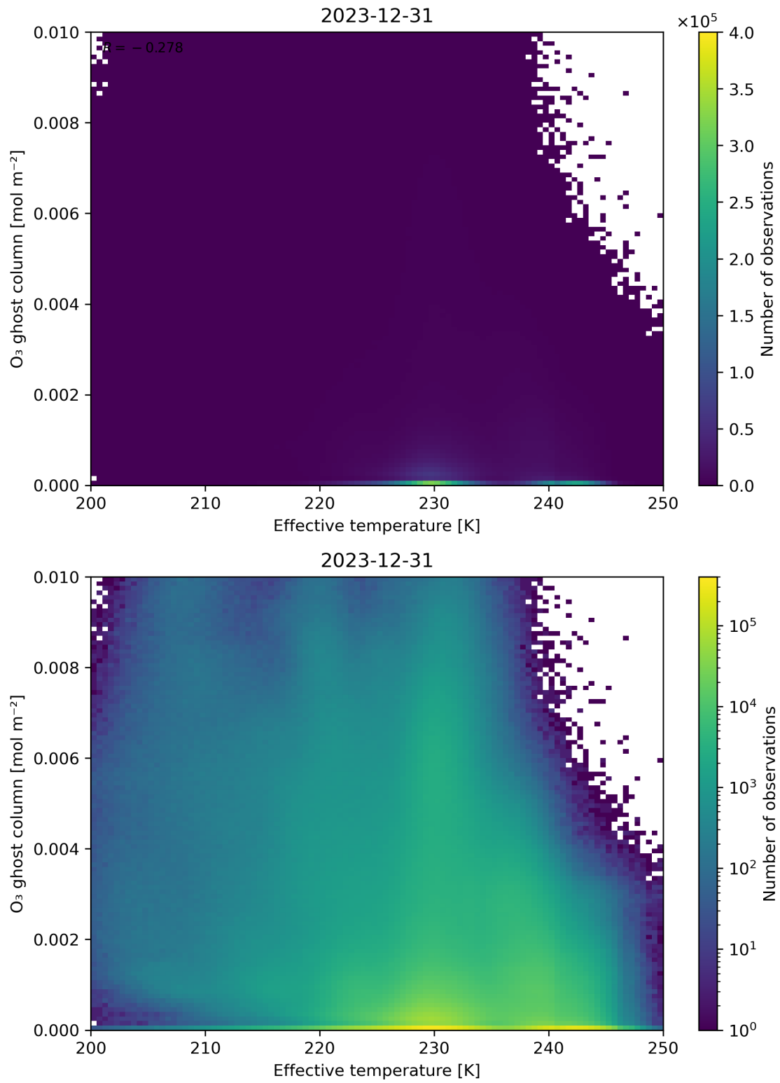
Figure 38: Scatter density plot of “Effective temperature” against “O 3 ghost column” for 2023-12-30 to 2023-12-31.
