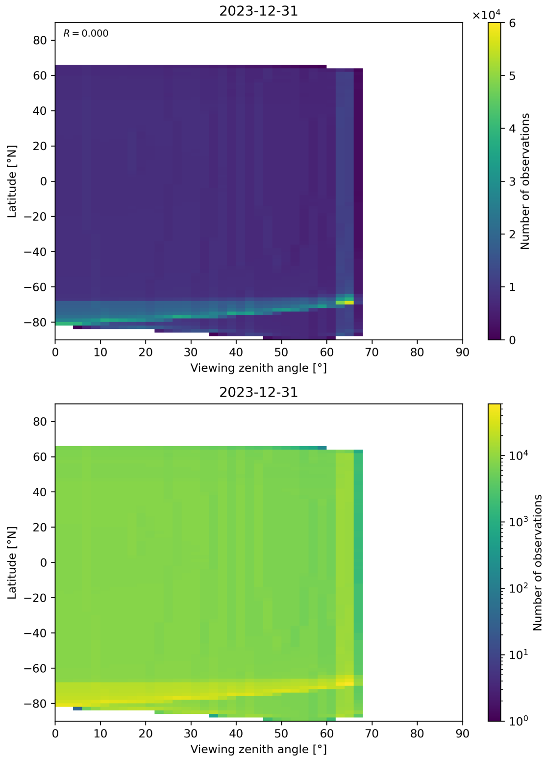
Figure 49: Scatter density plot of “Viewing zenith angle” against “Latitude” for 2023-12-30 to 2023-12-31.
