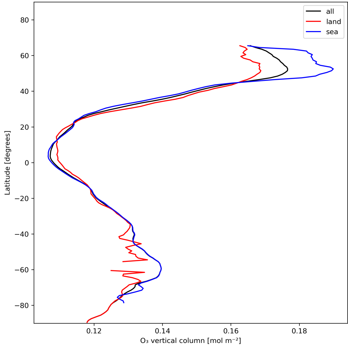
Figure 14: Zonal average of “O 3 vertical column” for 2023-12-30 to 2023-12-31.
