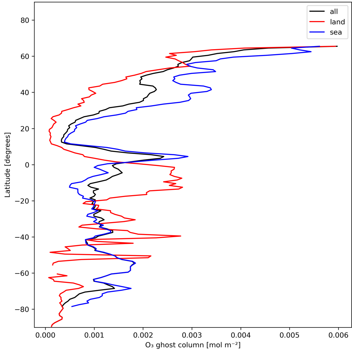
Figure 18: Zonal average of “O 3 ghost column” for 2023-12-30 to 2023-12-31.
