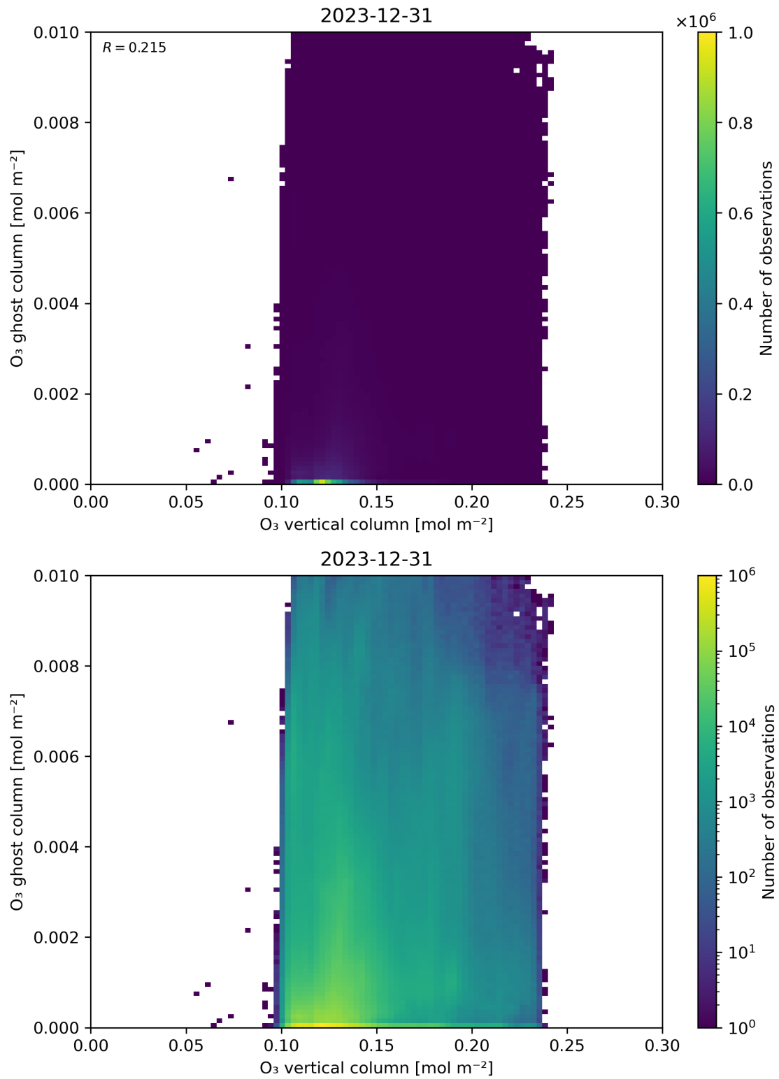
Figure 40: Scatter density plot of “O 3 vertical column” against “O 3 ghost column” for 2023-12-30 to 2023-12-31.
