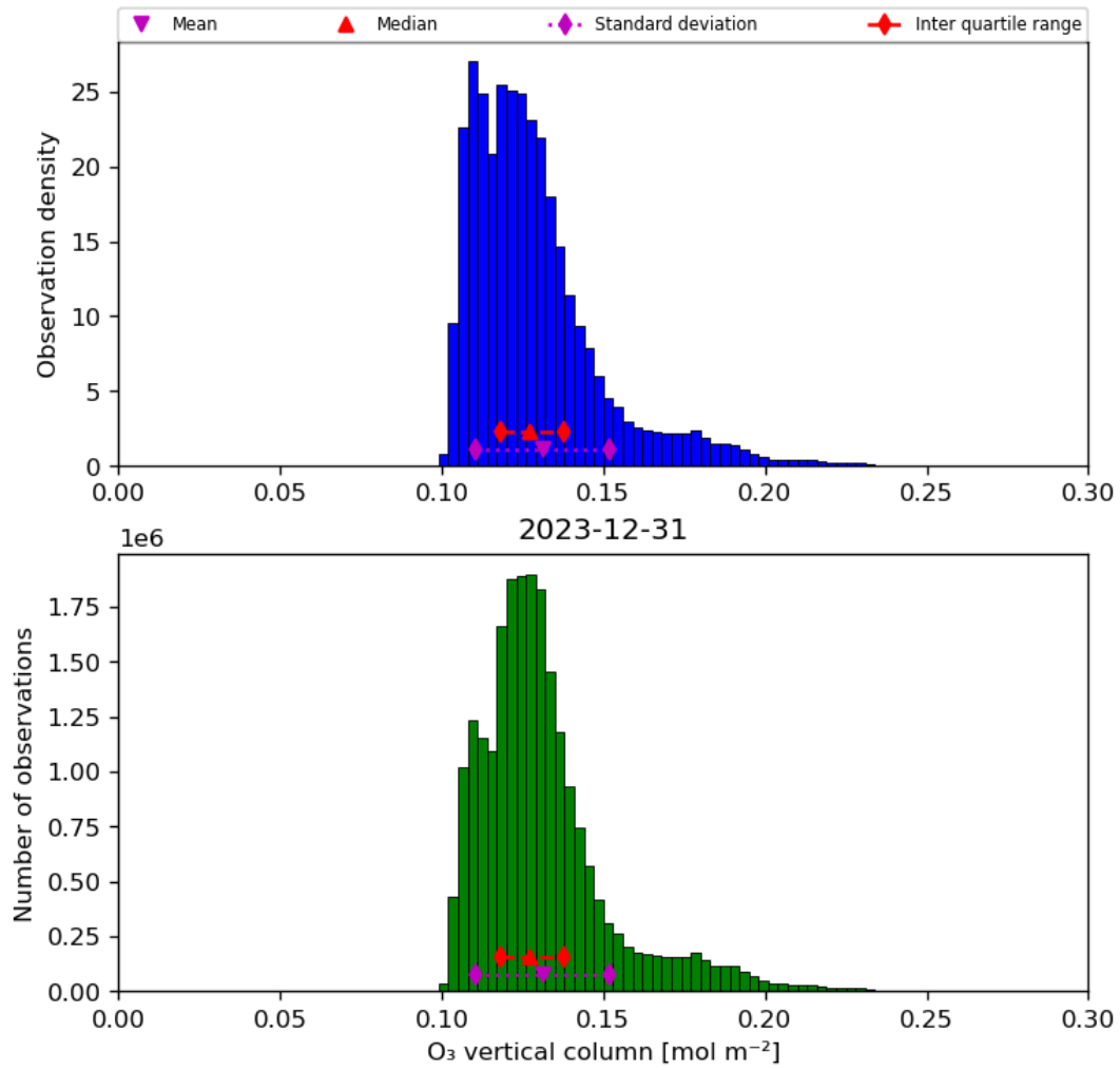
Figure 21: Histogram of “O 3 vertical column” for 2023-12-30 to 2023-12-31
