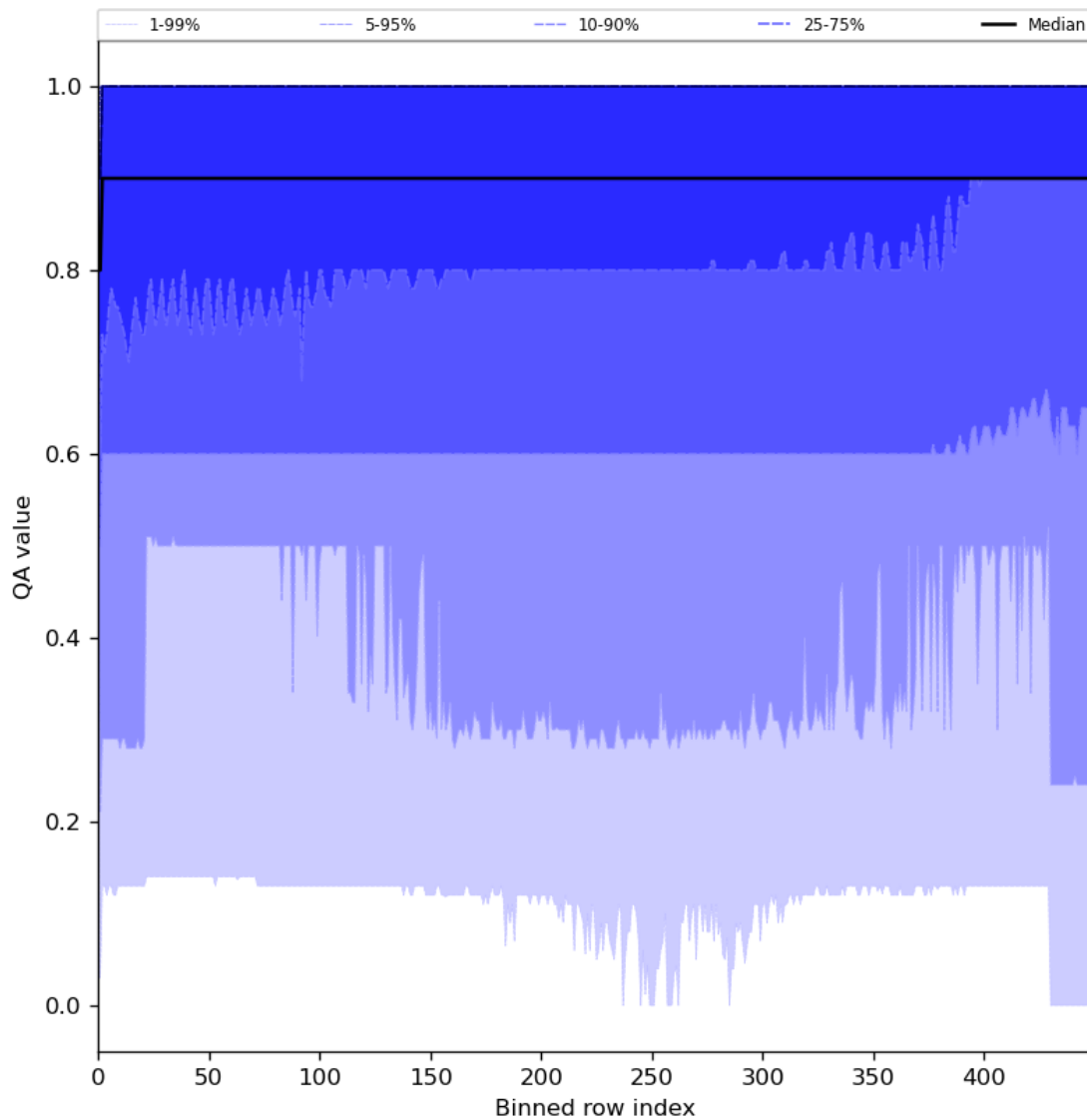
Figure 27: Along track statistics of “QA value” for 2023-12-30 to 2023-12-31
