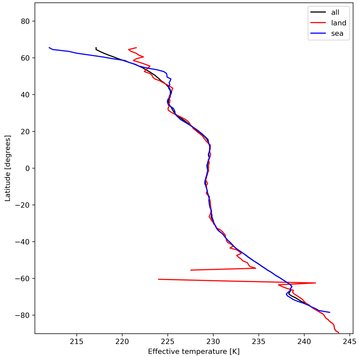
Figure 17: Zonal average of “Effective temperature” for 2023-12-30 to 2023-12-31.
