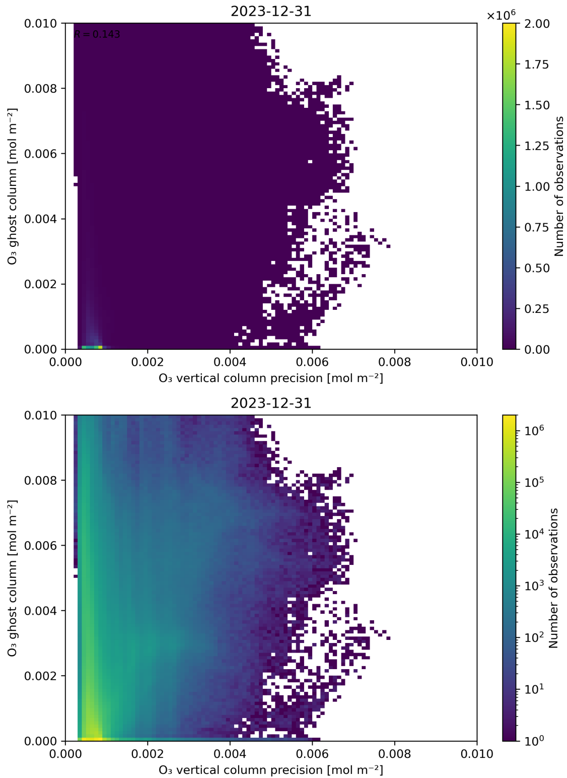
Figure 43: Scatter density plot of “ \text{O}_3 vertical column precision” against “ \text{O}_3 ghost column” for 2023-12-30 to 2023-12-31.
