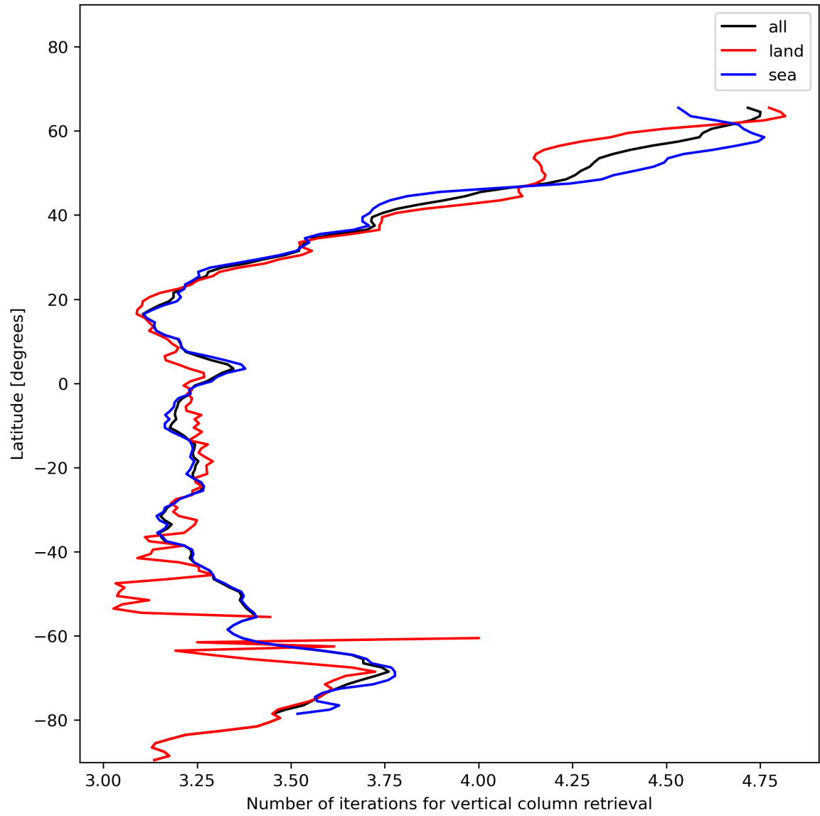
Figure 19: Zonal average of “Number of iterations for vertical column retrieval” for 2023-12-30 to 2023-12-31.
