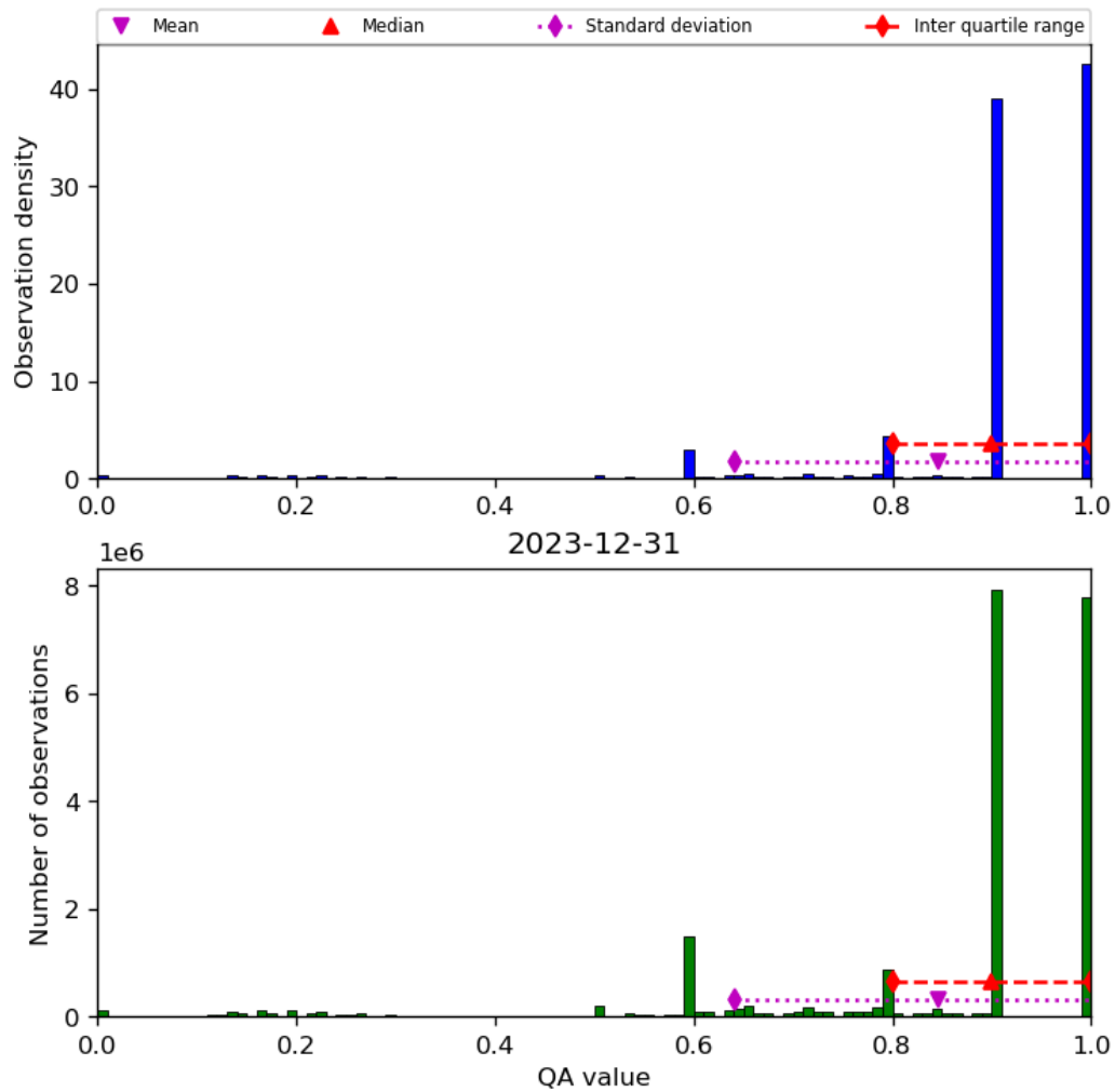
Figure 20: Histogram of “QA value” for 2023-12-30 to 2023-12-31
