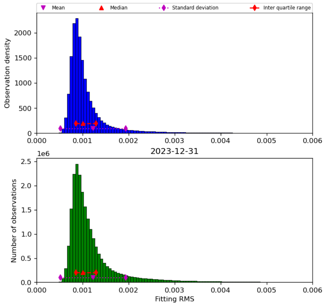
Figure 23: Histogram of “Fitting RMS” for 2023-12-30 to 2023-12-31
