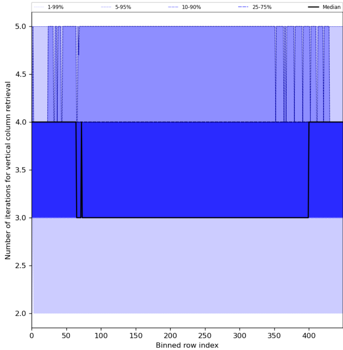
Figure 33: Along track statistics of “Number of iterations for vertical column retrieval” for 2023-12-30 to 2023-12-31
