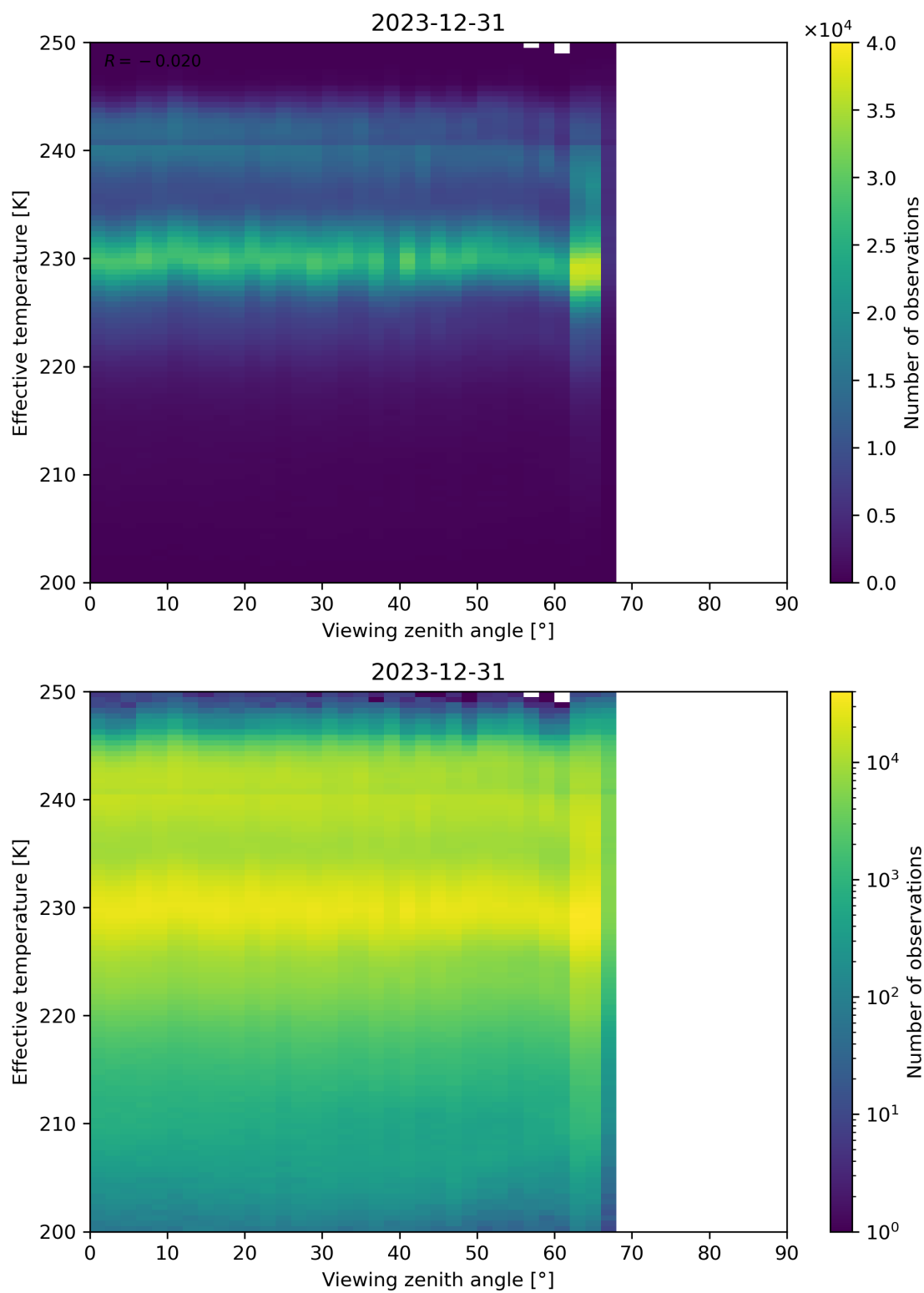
Figure 50: Scatter density plot of “Viewing zenith angle” against “Effective temperature” for 2023-12-30 to 2023-12-31.
