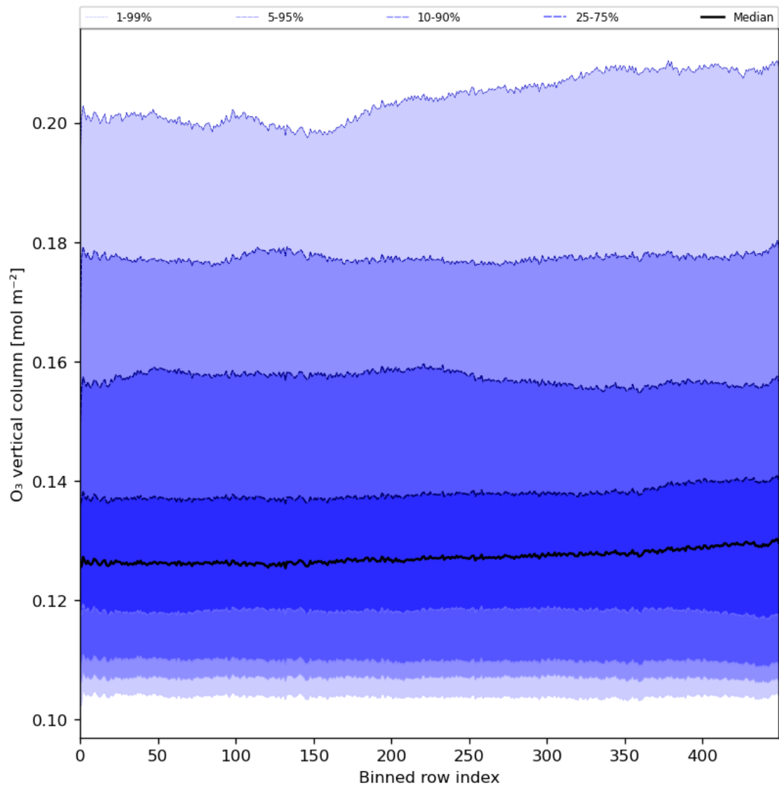
Figure 28: Along track statistics of “O 3 vertical column” for 2023-12-30 to 2023-12-31
