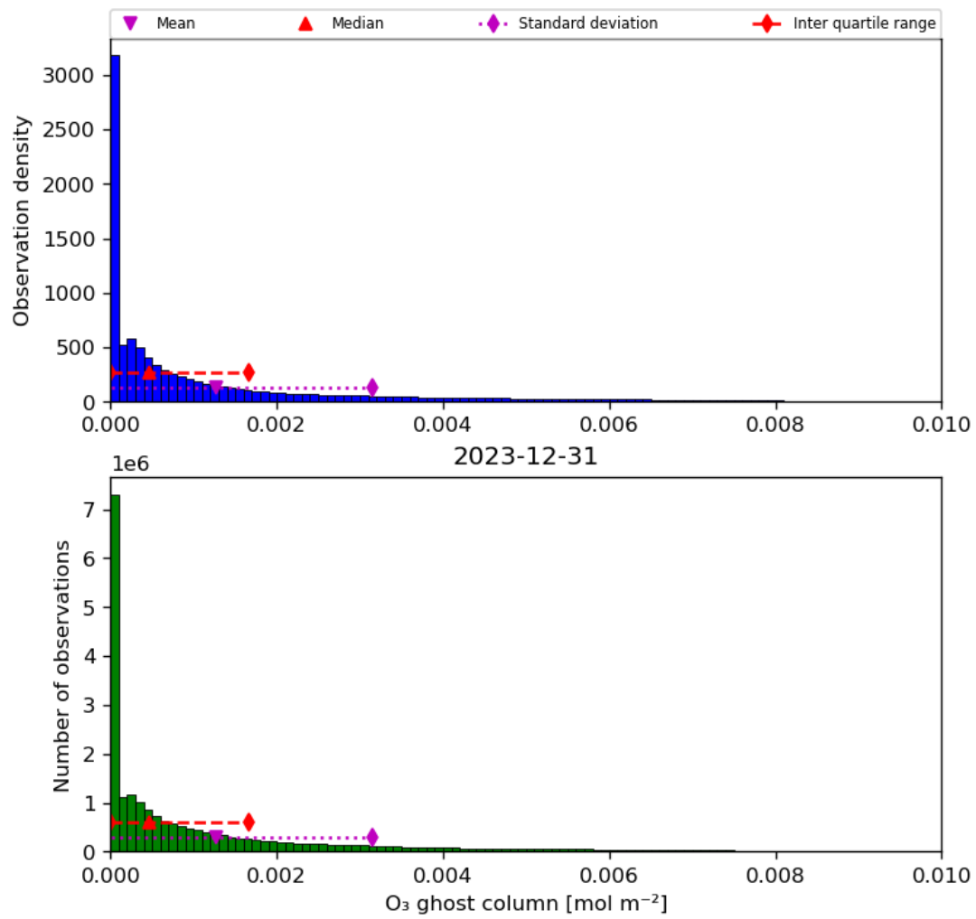
Figure 25: Histogram of “O 3 ghost column” for 2023-12-30 to 2023-12-31
