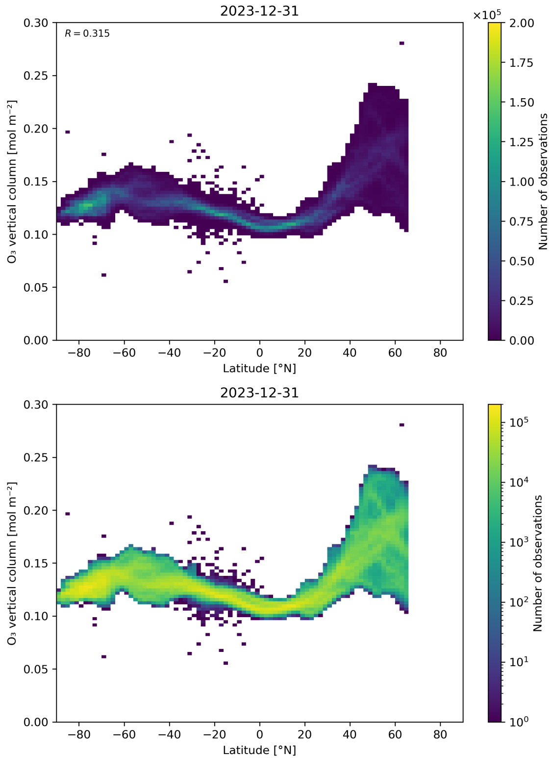
Figure 36: Scatter density plot of “Latitude” against “O 3 vertical column” for 2023-12-30 to 2023-12-31.
