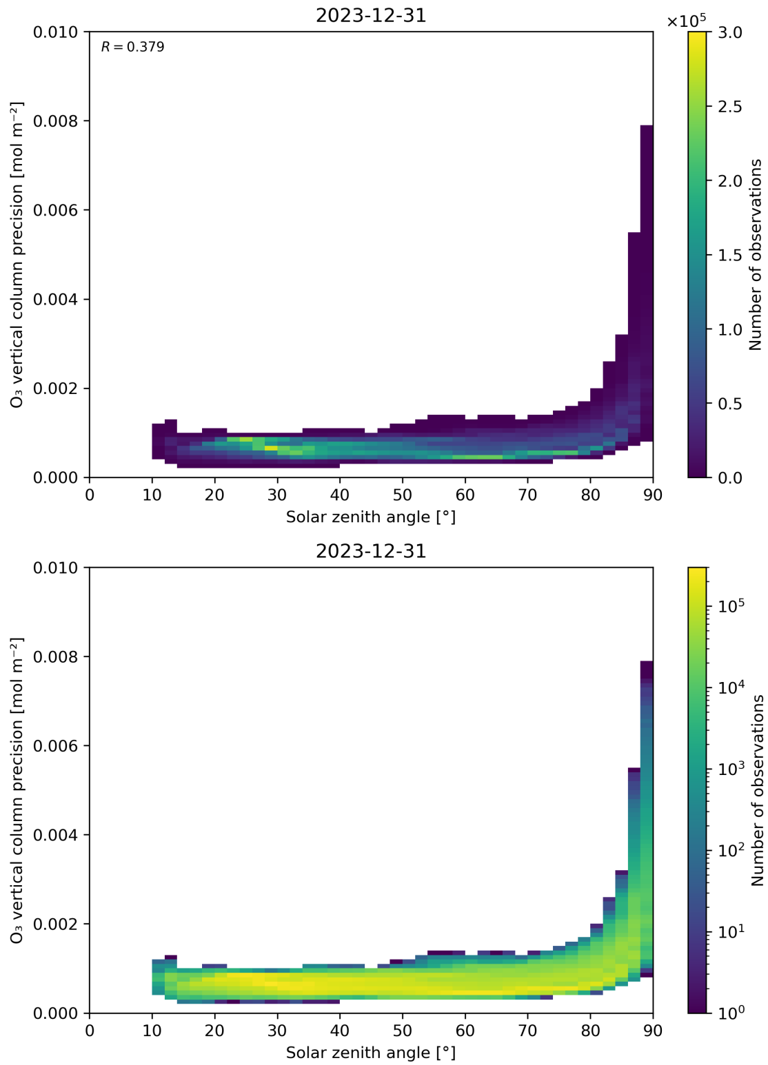
Figure 48: Scatter density plot of “Solar zenith angle” against “O 3 vertical column precision” for 2023-12-30 to 2023-12-31.
