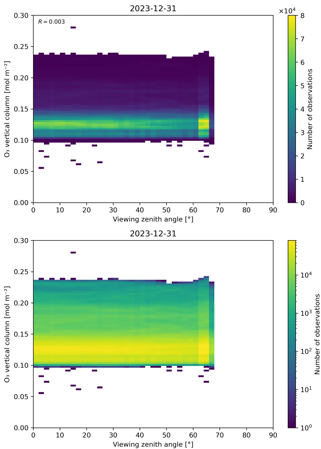
Figure 52: Scatter density plot of “Viewing zenith angle” against “O 3 vertical column” for 2023-12-30 to 2023-12-31.
