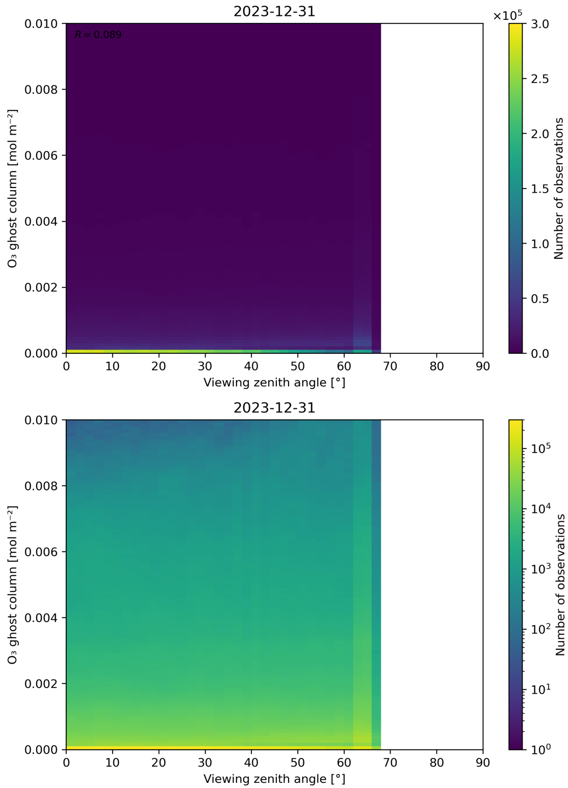
Figure 51: Scatter density plot of “Viewing zenith angle” against “O 3 ghost column” for 2023-12-30 to 2023-12-31.
