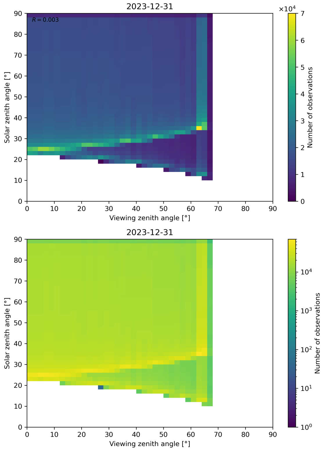
Figure 54: Scatter density plot of “Viewing zenith angle” against “Solar zenith angle” for 2023-12-30 to 2023-12-31.
