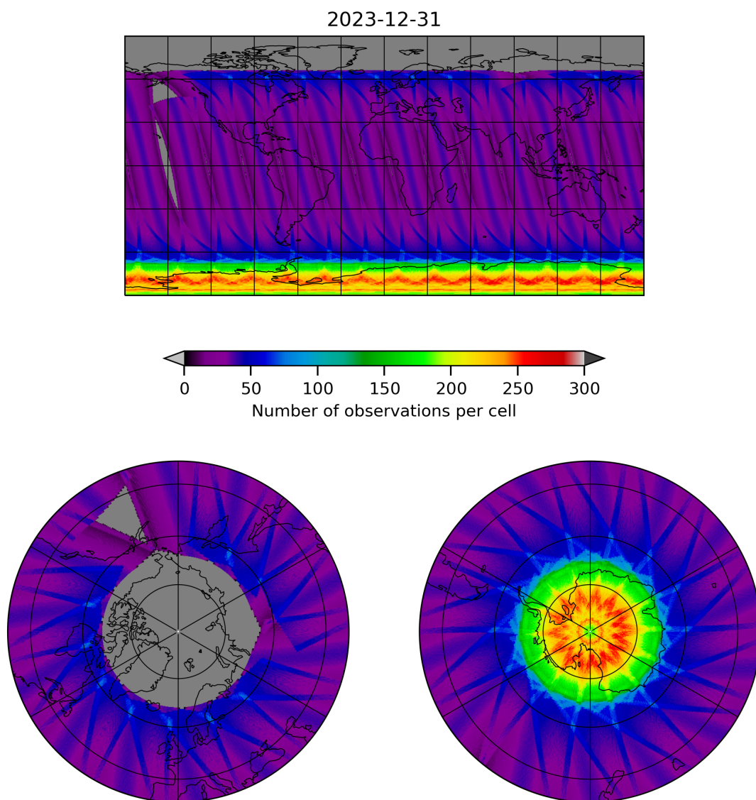
Figure 12: Map of the number of observations for 2023-12-30 to 2023-12-31
