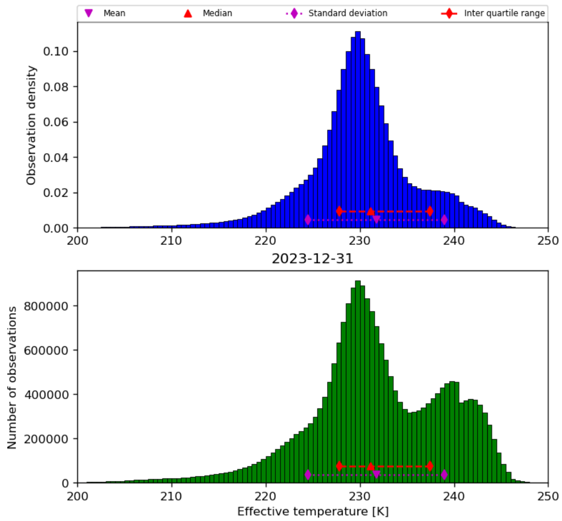
Figure 24: Histogram of “Effective temperature” for 2023-12-30 to 2023-12-31
