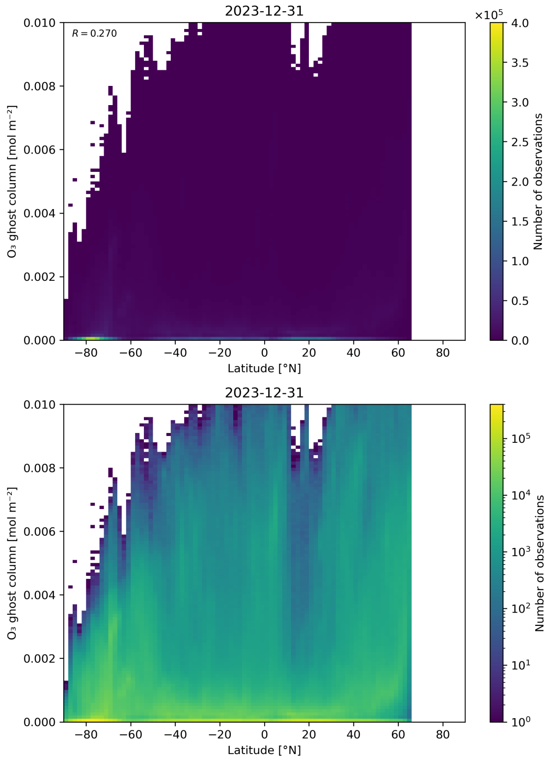
Figure 35: Scatter density plot of “Latitude” against “O 3 ghost column” for 2023-12-30 to 2023-12-31.
