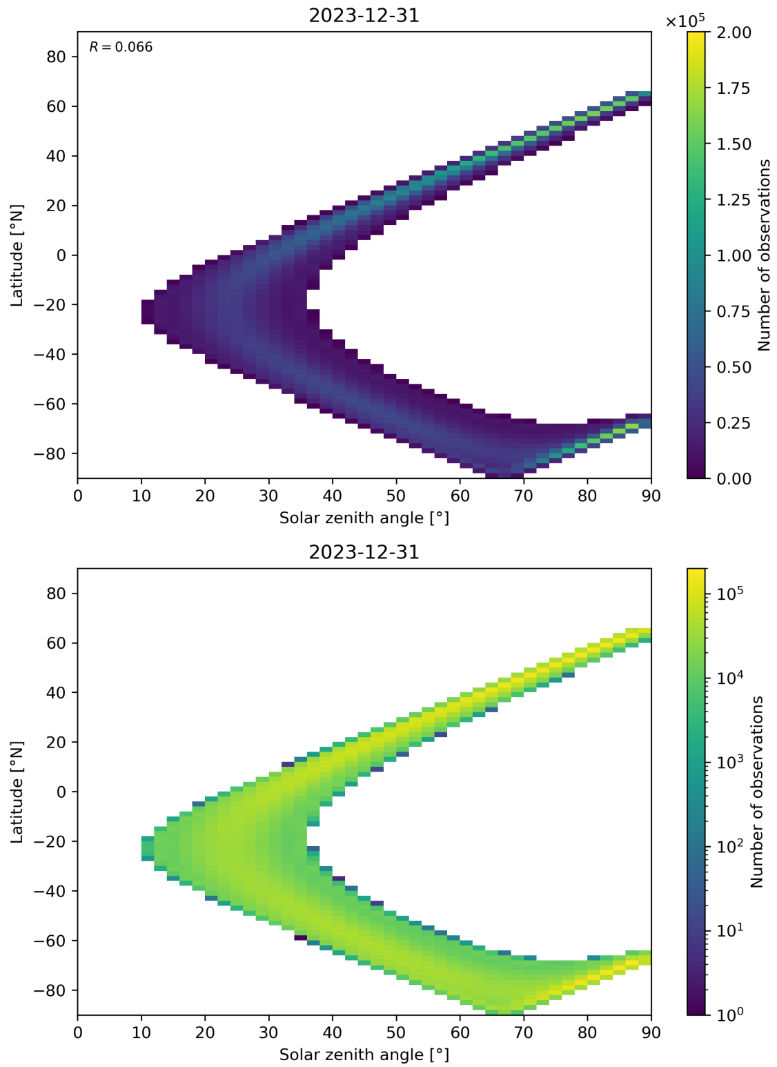
Figure 44: Scatter density plot of “Solar zenith angle” against “Latitude” for 2023-12-30 to 2023-12-31.
