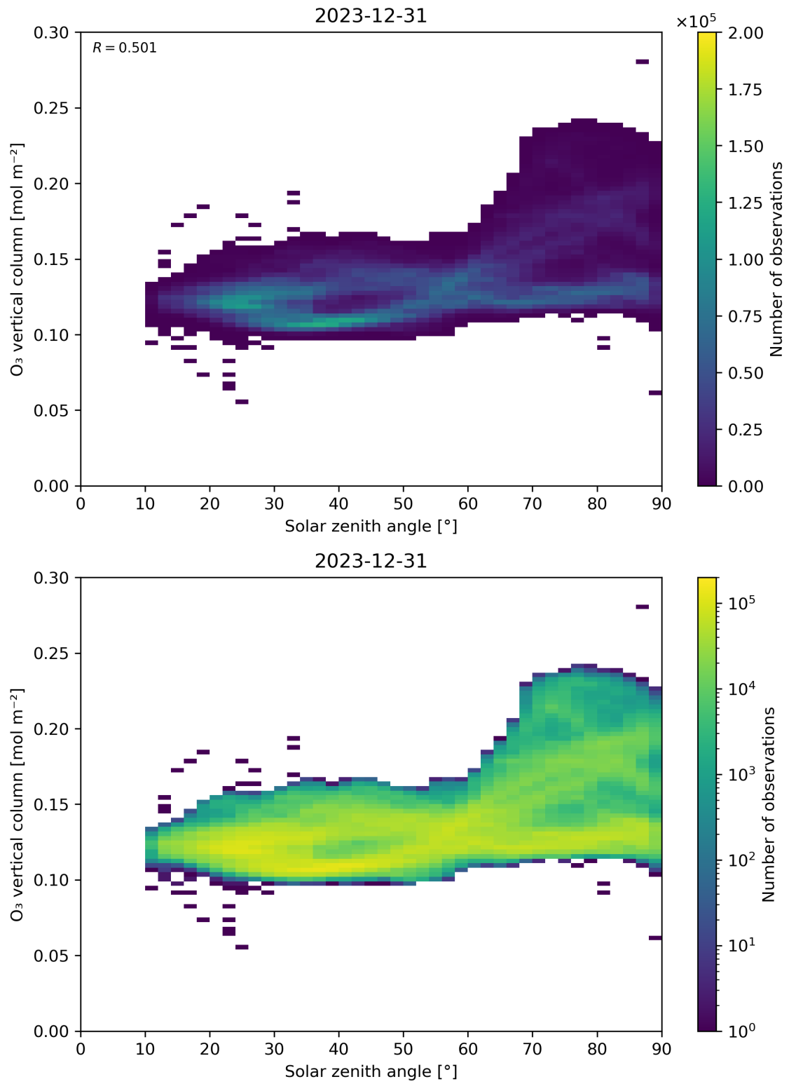
Figure 47: Scatter density plot of “Solar zenith angle” against “O 3 vertical column” for 2023-12-30 to 2023-12-31.
