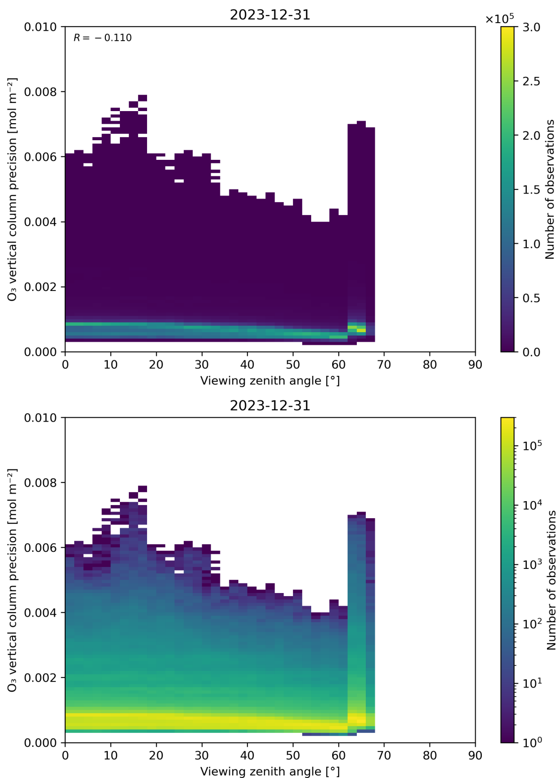
Figure 53: Scatter density plot of “Viewing zenith angle” against “O 3 vertical column precision” for 2023-12-30 to 2023-12-31.
