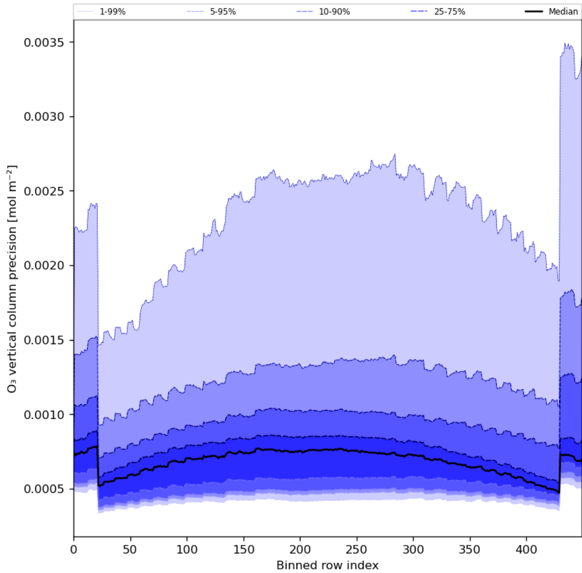
Figure 29: Along track statistics of “O 3 vertical column precision” for 2023-12-30 to 2023-12-31
