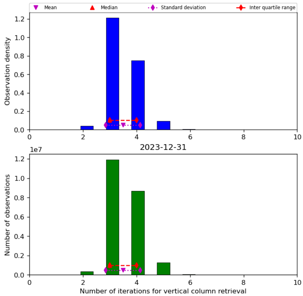
Figure 26: Histogram of “Number of iterations for vertical column retrieval” for 2023-12-30 to 2023-12-31
