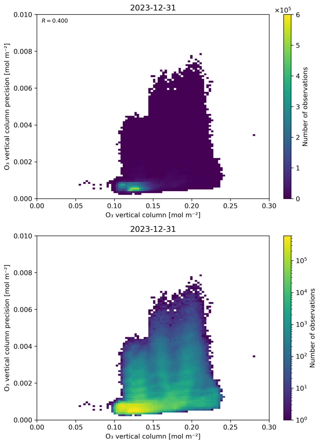
Figure 41: Scatter density plot of “O 3 vertical column” against “O 3 vertical column precision” for 2023-12-30 to 2023-12-31.
