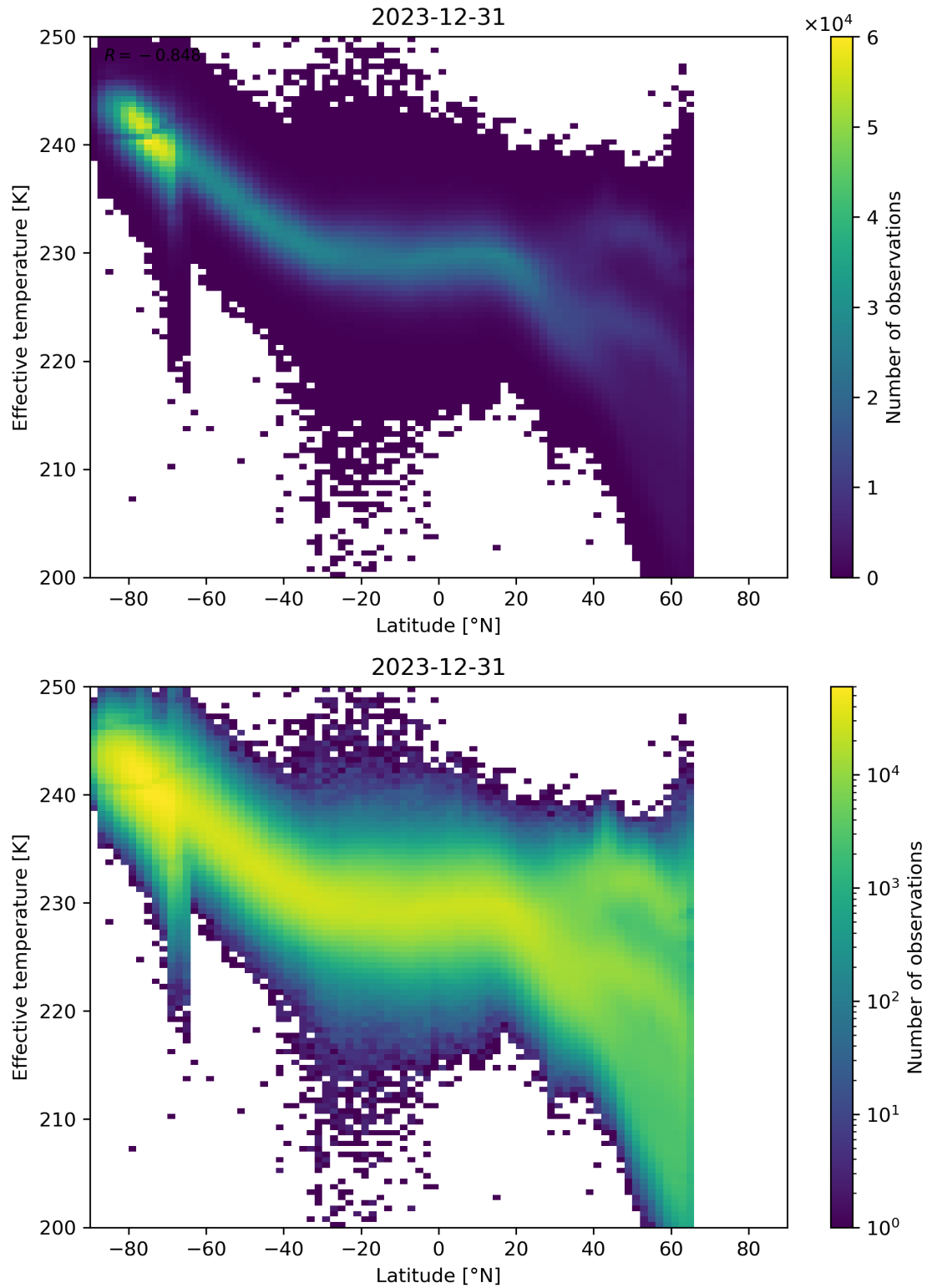
Figure 34: Scatter density plot of “Latitude” against “Effective temperature” for 2023-12-30 to 2023-12-31.
