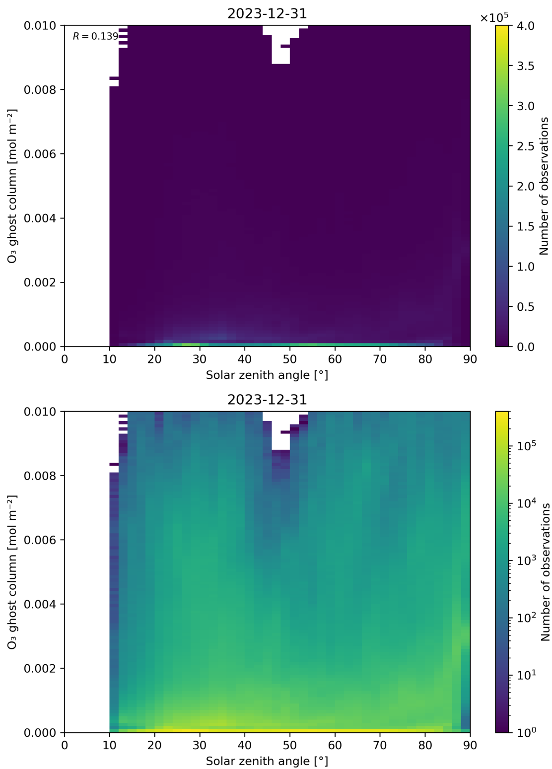
Figure 46: Scatter density plot of “Solar zenith angle” against “O 3 ghost column” for 2023-12-30 to 2023-12-31.
