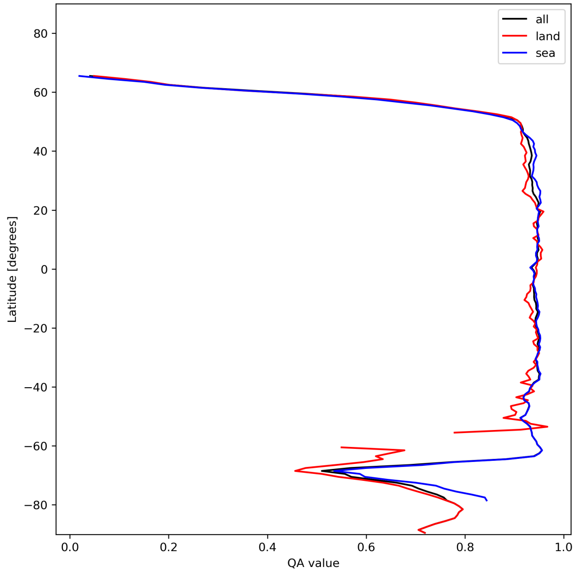
Figure 13: Zonal average of “QA value” for 2023-12-30 to 2023-12-31.
