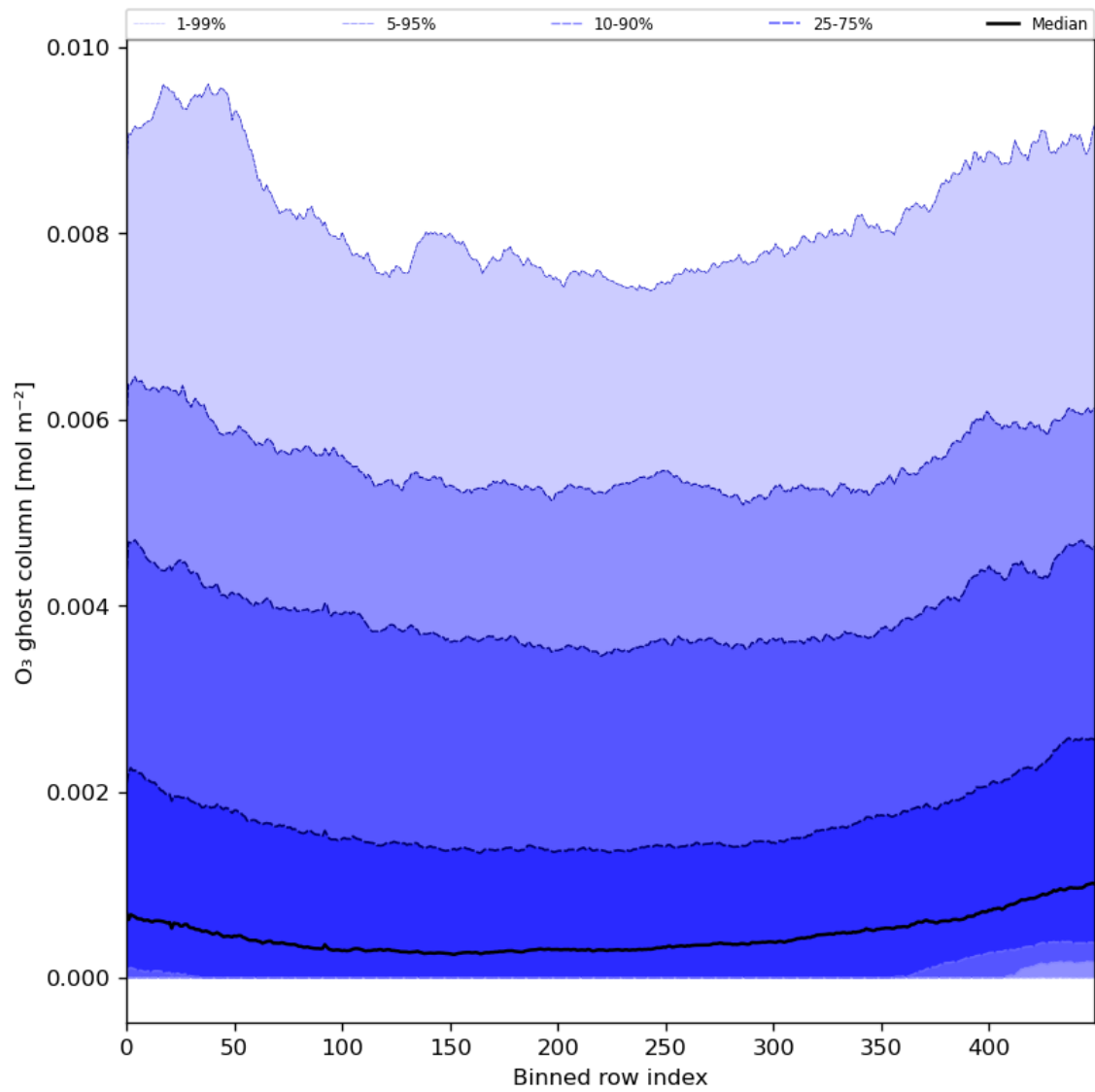
Figure 32: Along track statistics of “O 3 ghost column” for 2023-12-30 to 2023-12-31
