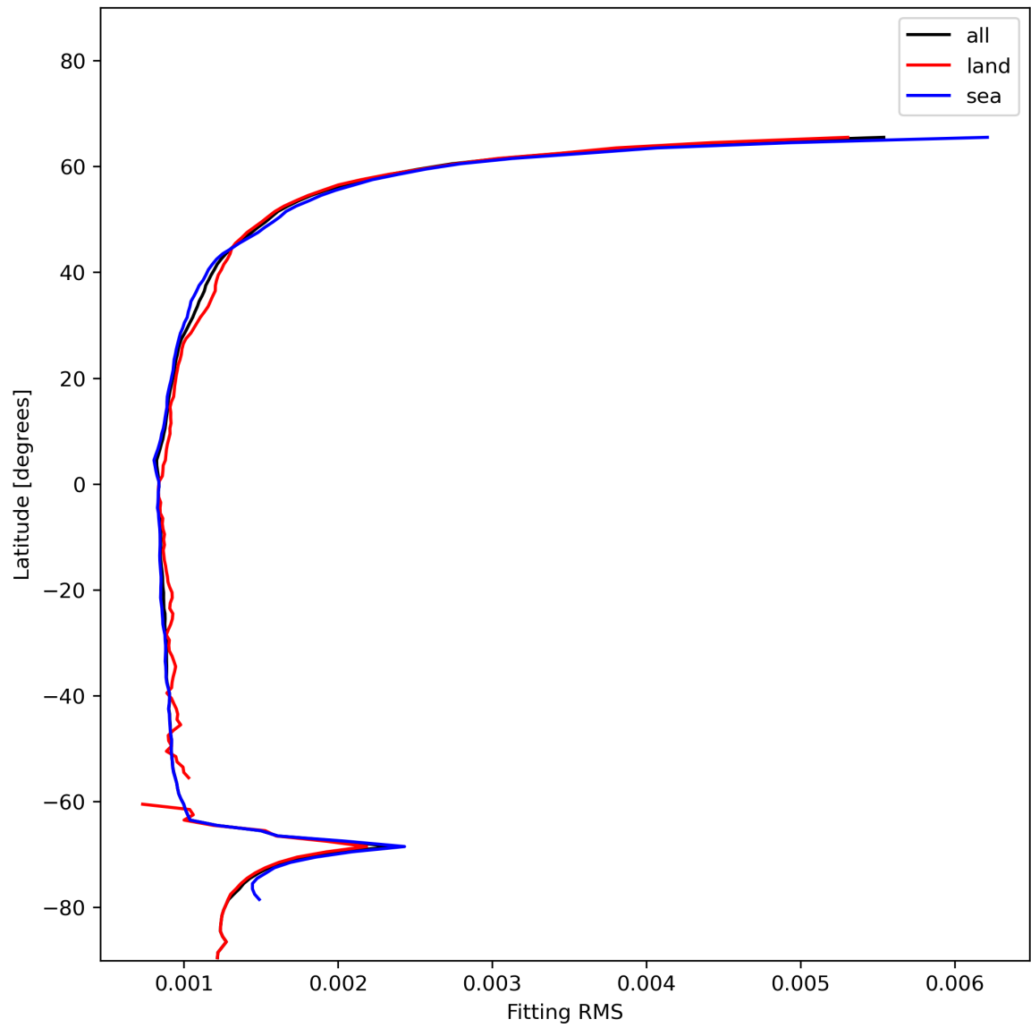
Figure 16: Zonal average of “Fitting RMS” for 2023-12-30 to 2023-12-31.
