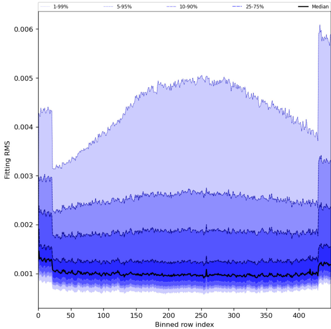
Figure 30: Along track statistics of “Fitting RMS” for 2023-12-30 to 2023-12-31
