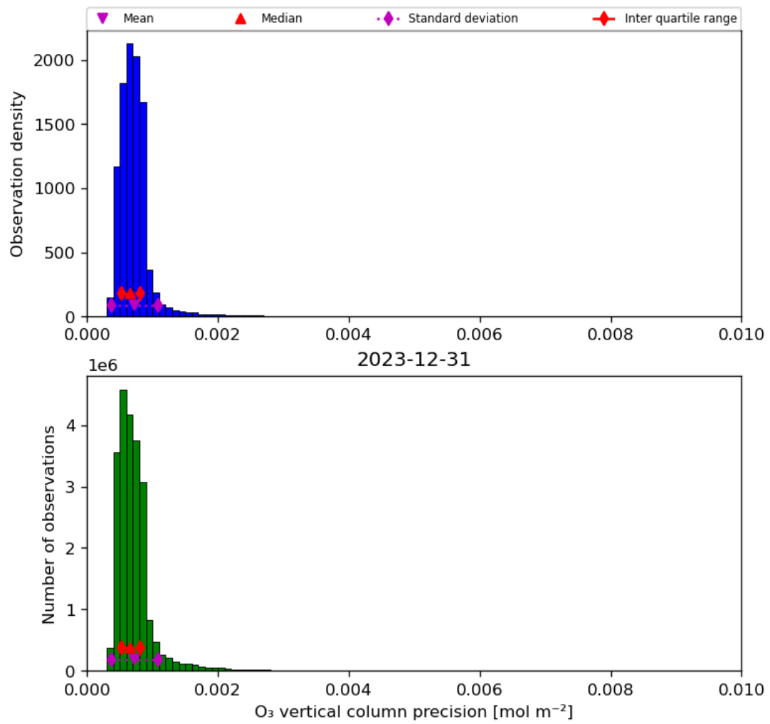
Figure 22: Histogram of “O 3 vertical column precision” for 2023-12-30 to 2023-12-31
