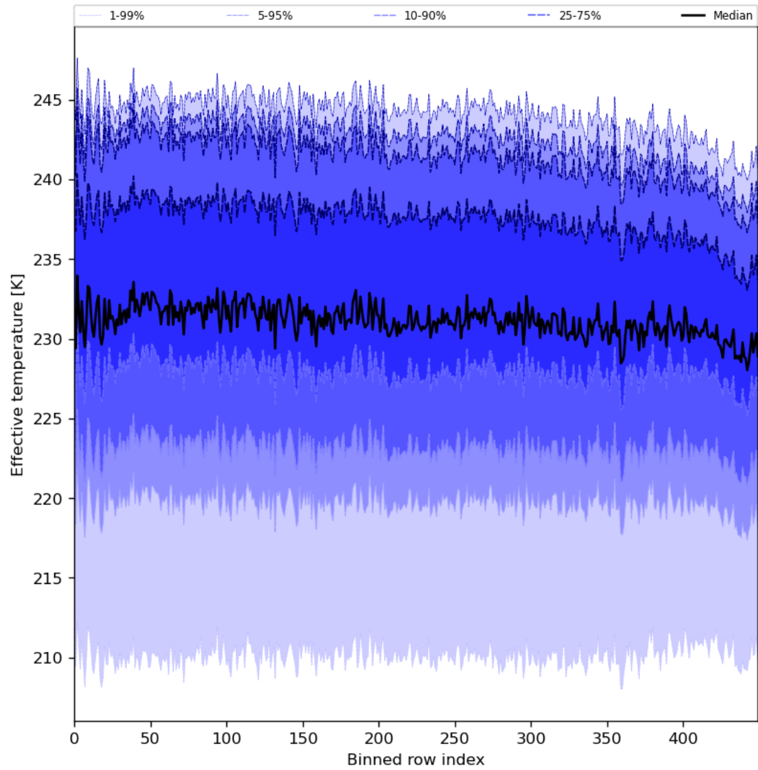
Figure 31: Along track statistics of “Effective temperature” for 2023-12-30 to 2023-12-31
