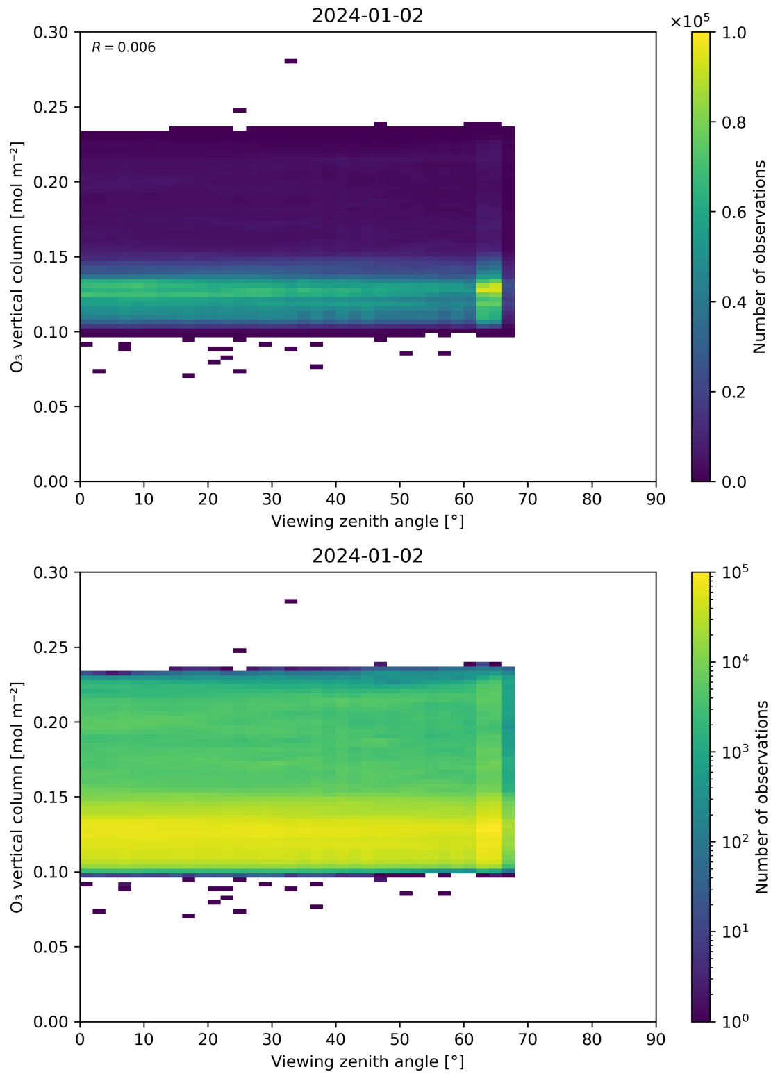
Figure 52: Scatter density plot of “Viewing zenith angle” against “O 3 vertical column” for 2024-01-01 to 2024-01-03.
