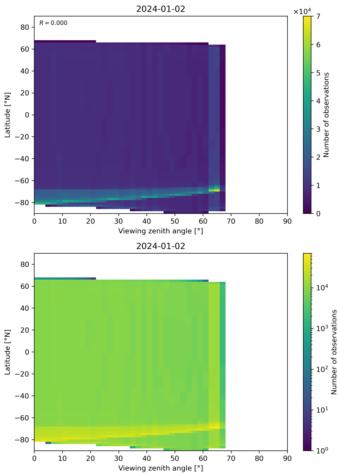
Figure 49: Scatter density plot of “Viewing zenith angle” against “Latitude” for 2024-01-01 to 2024-01-03.
