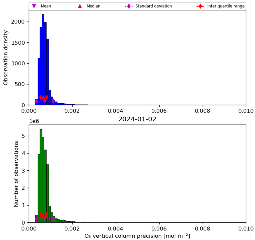
Figure 22: Histogram of “O 3 vertical column precision” for 2024-01-01 to 2024-01-03
