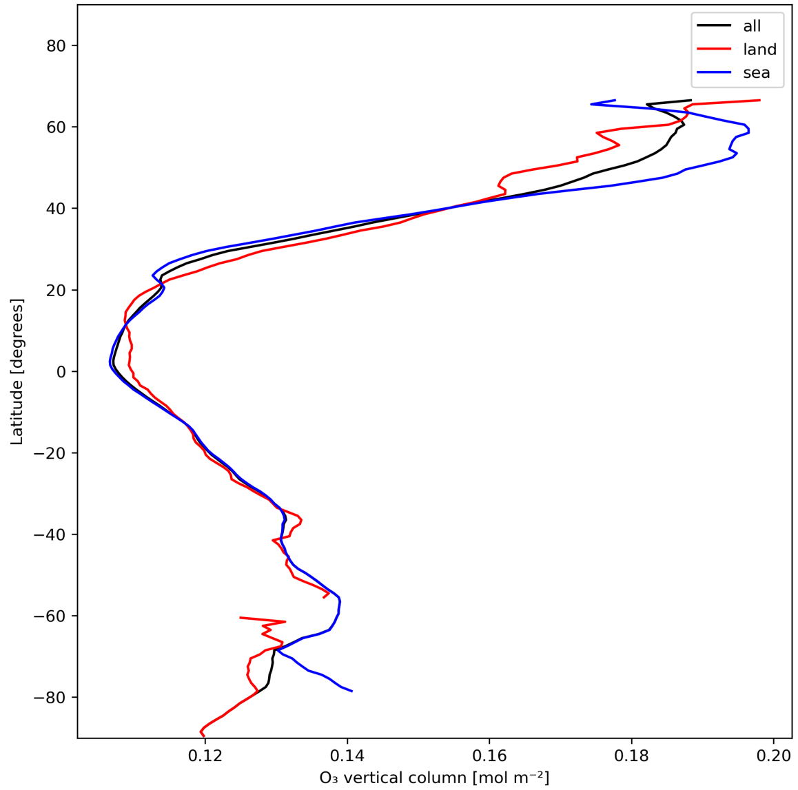
Figure 14: Zonal average of “O 3 vertical column” for 2024-01-01 to 2024-01-03.
