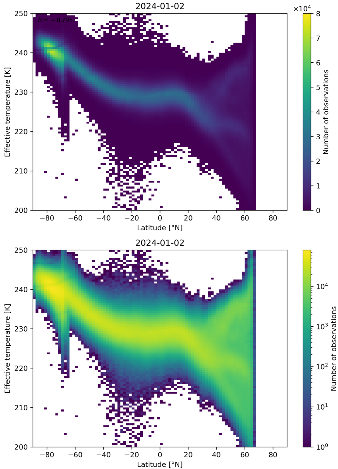
Figure 34: Scatter density plot of “Latitude” against “Effective temperature” for 2024-01-01 to 2024-01-03.
