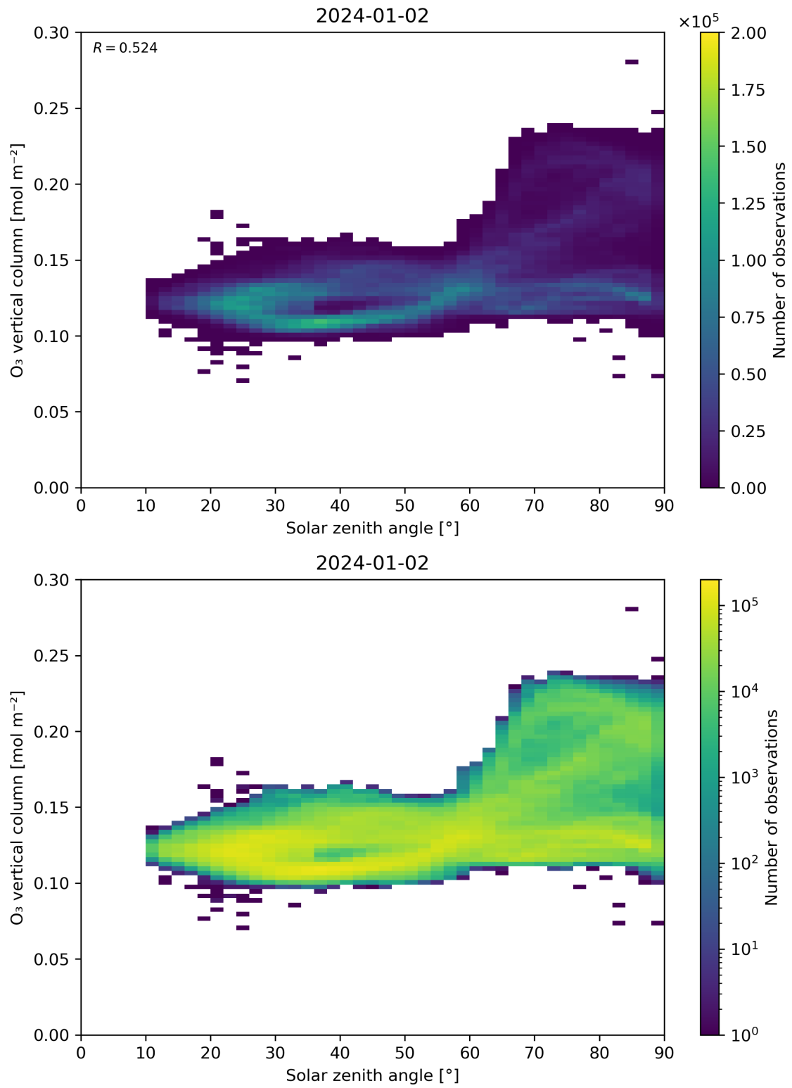
Figure 47: Scatter density plot of “Solar zenith angle” against “O 3 vertical column” for 2024-01-01 to 2024-01-03.
