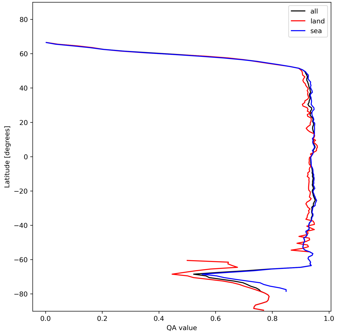
Figure 13: Zonal average of “QA value” for 2024-01-01 to 2024-01-03.
