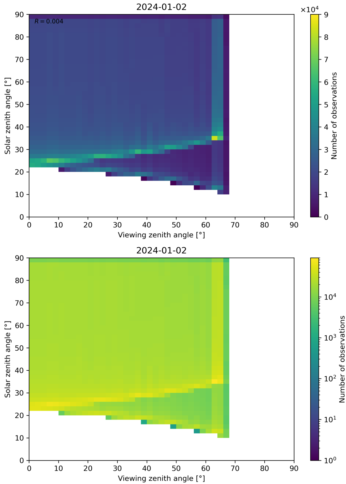
Figure 54: Scatter density plot of “Viewing zenith angle” against “Solar zenith angle” for 2024-01-01 to 2024-01-03.
