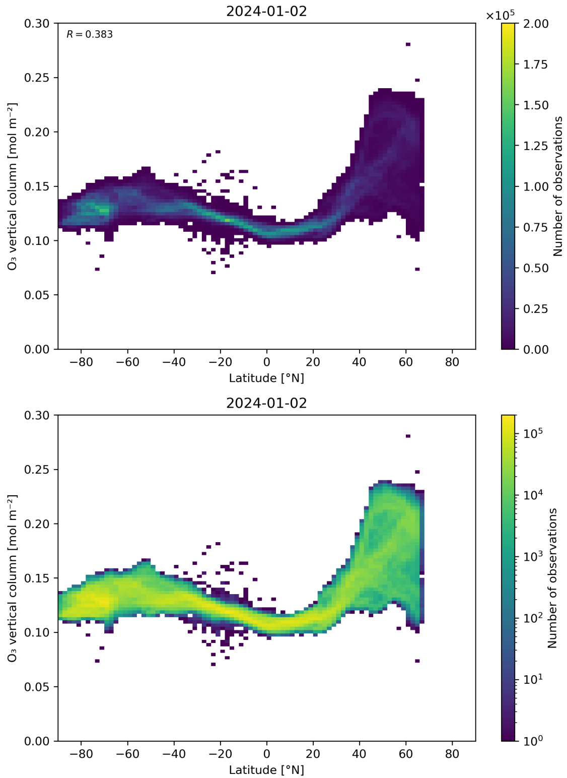
Figure 36: Scatter density plot of “Latitude” against “O 3 vertical column” for 2024-01-01 to 2024-01-03.
