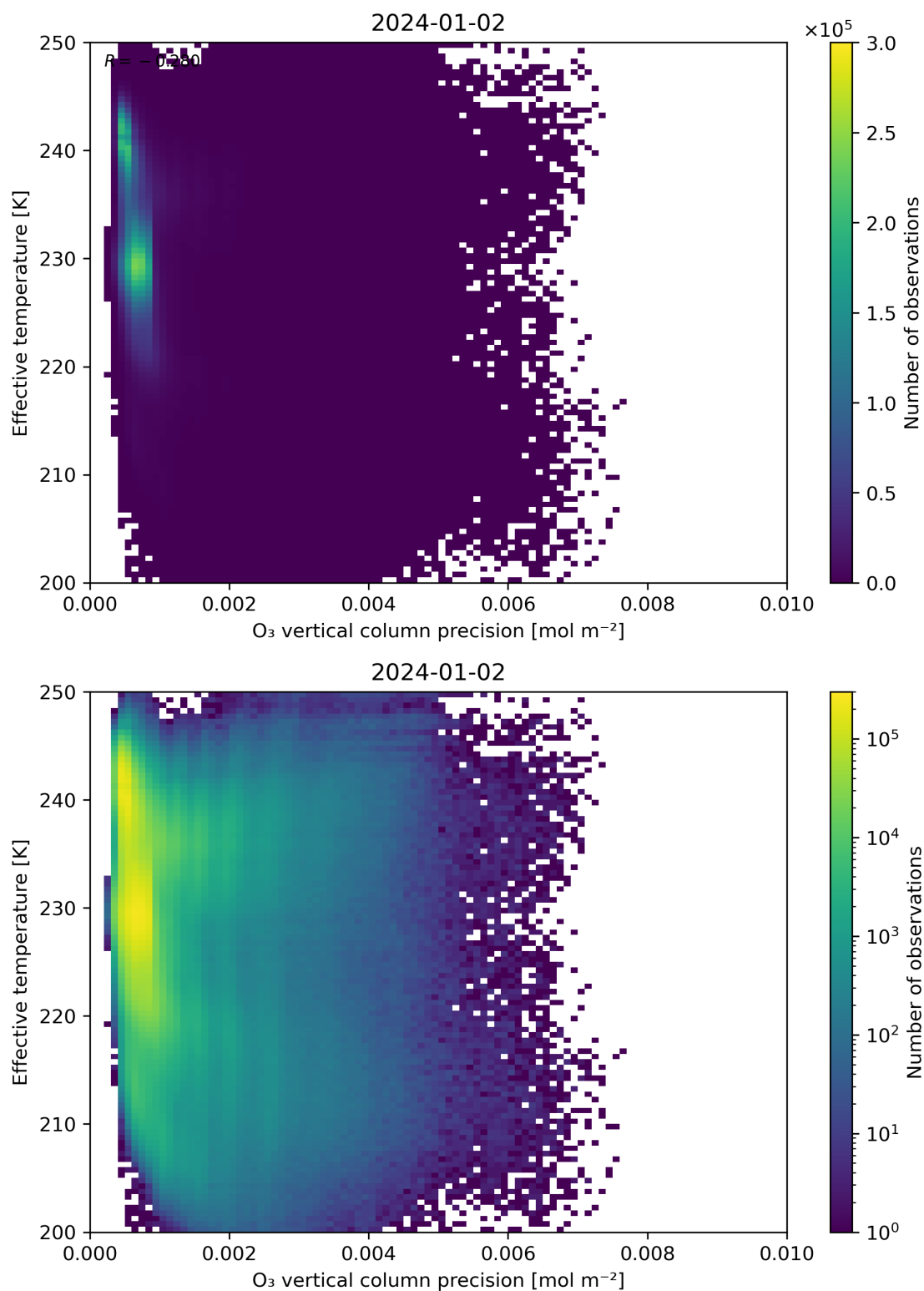
Figure 42: Scatter density plot of “O 3 vertical column precision” against “Effective temperature” for 2024-01-01 to 2024-01-03.
