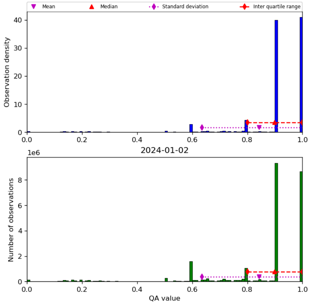
Figure 20: Histogram of “QA value” for 2024-01-01 to 2024-01-03
