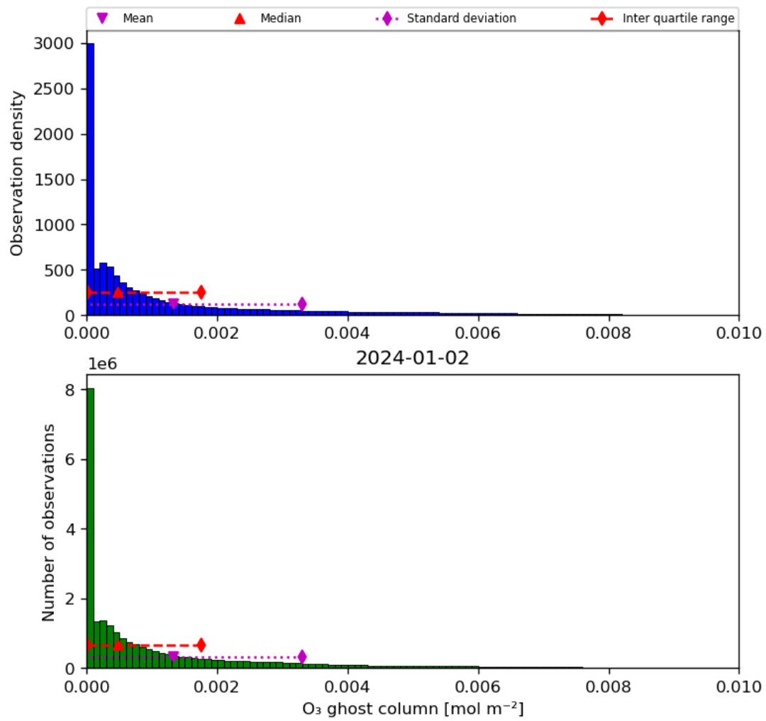
Figure 25: Histogram of “O 3 ghost column” for 2024-01-01 to 2024-01-03
