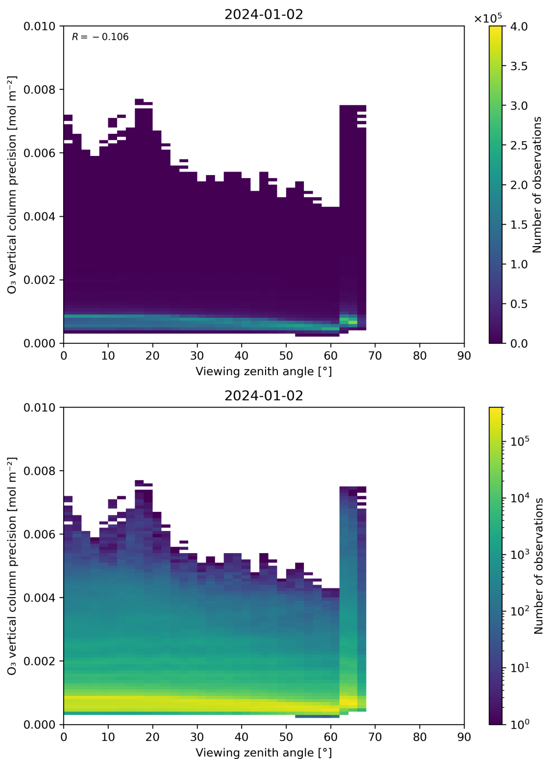
Figure 53: Scatter density plot of “Viewing zenith angle” against “O 3 vertical column precision” for 2024-01-01 to 2024-01-03.
