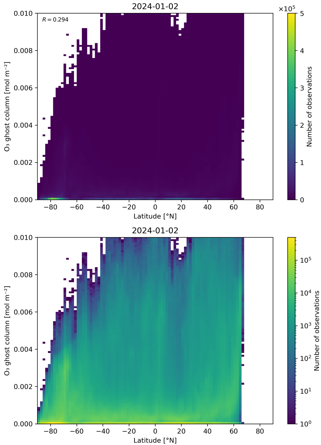
Figure 35: Scatter density plot of “Latitude” against “O 3 ghost column” for 2024-01-01 to 2024-01-03.
