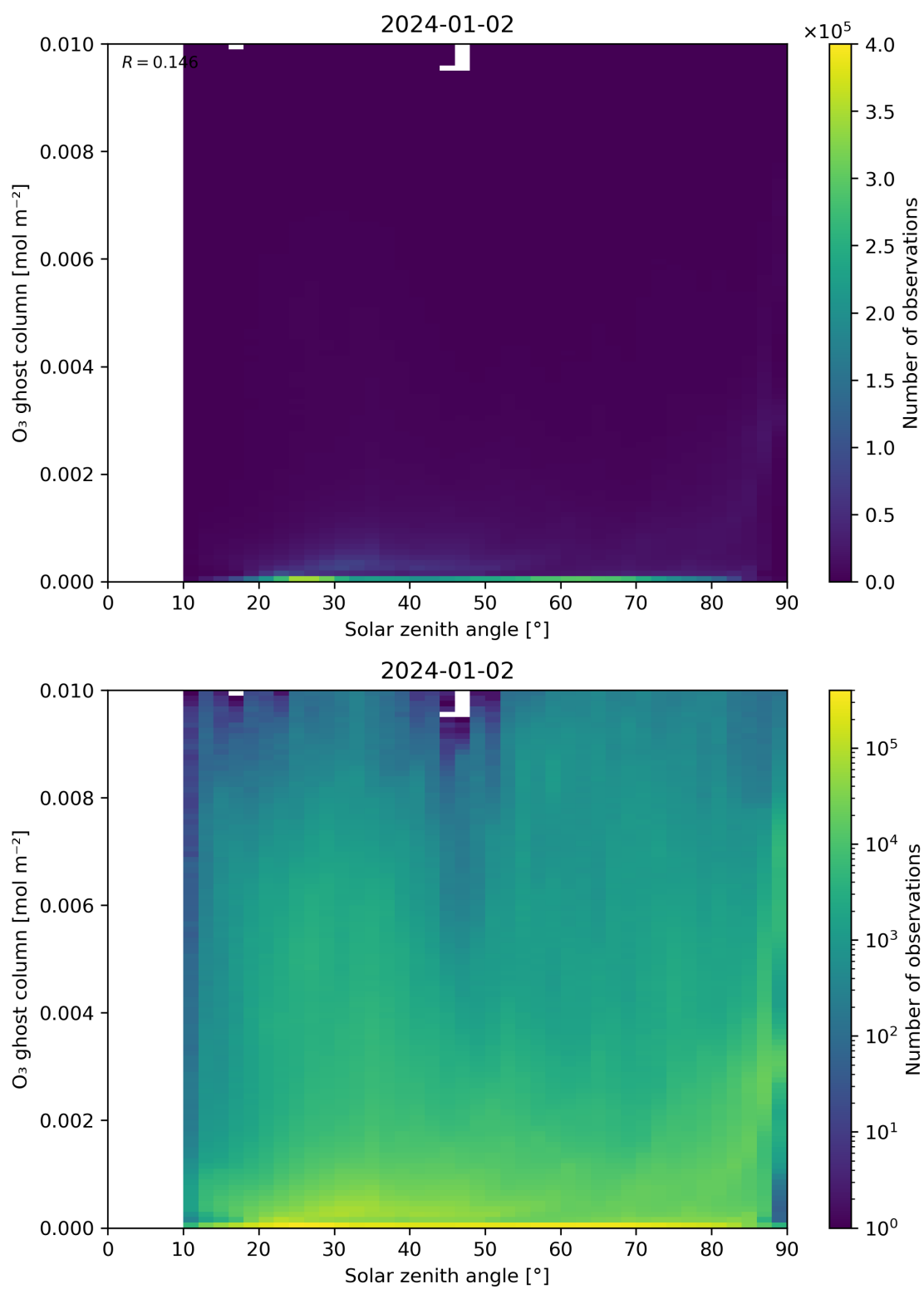
Figure 46: Scatter density plot of “Solar zenith angle” against “O 3 ghost column” for 2024-01-01 to 2024-01-03.
