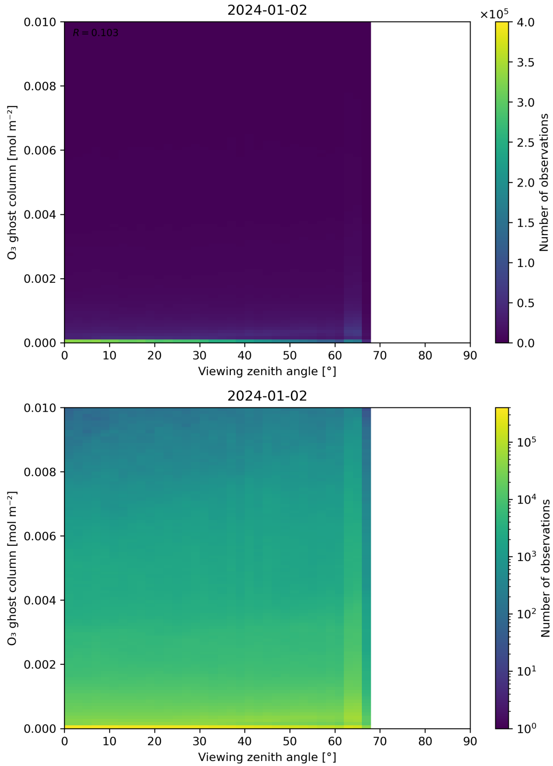
Figure 51: Scatter density plot of “Viewing zenith angle” against “O 3 ghost column” for 2024-01-01 to 2024-01-03.
