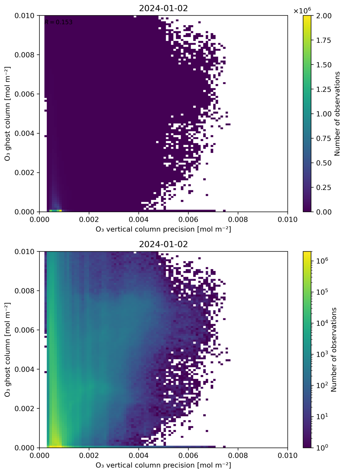
Figure 43: Scatter density plot of “ \text{O}_3 vertical column precision” against “ \text{O}_3 ghost column” for 2024-01-01 to 2024-01-03.
