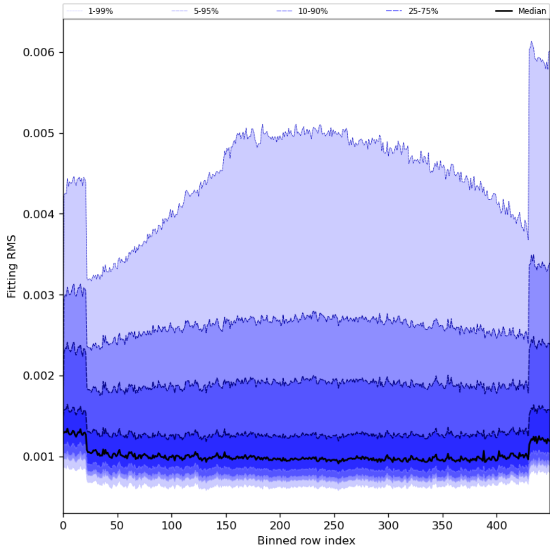
Figure 30: Along track statistics of “Fitting RMS” for 2024-01-01 to 2024-01-03
