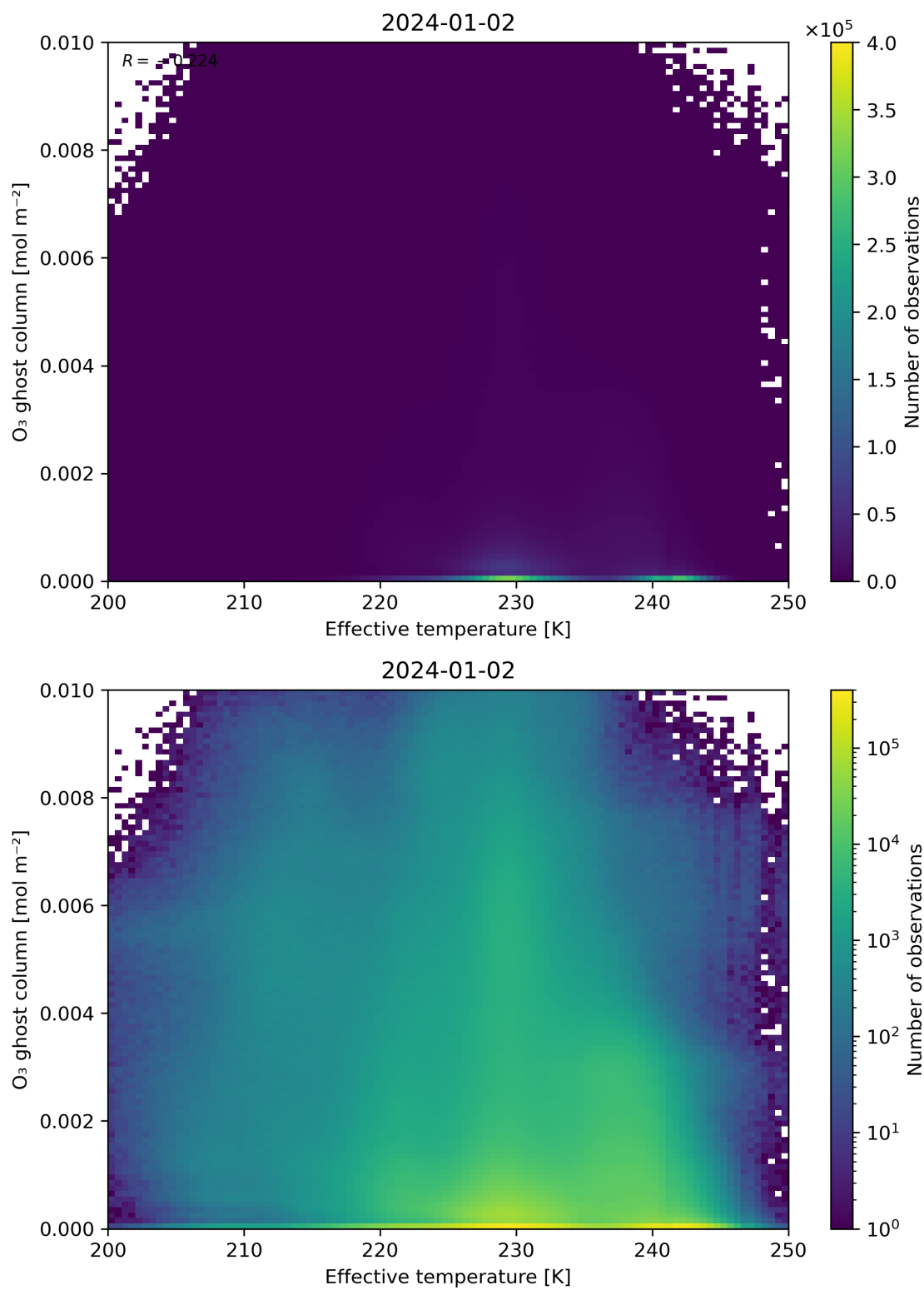
Figure 38: Scatter density plot of “Effective temperature” against “O 3 ghost column” for 2024-01-01 to 2024-01-03.
