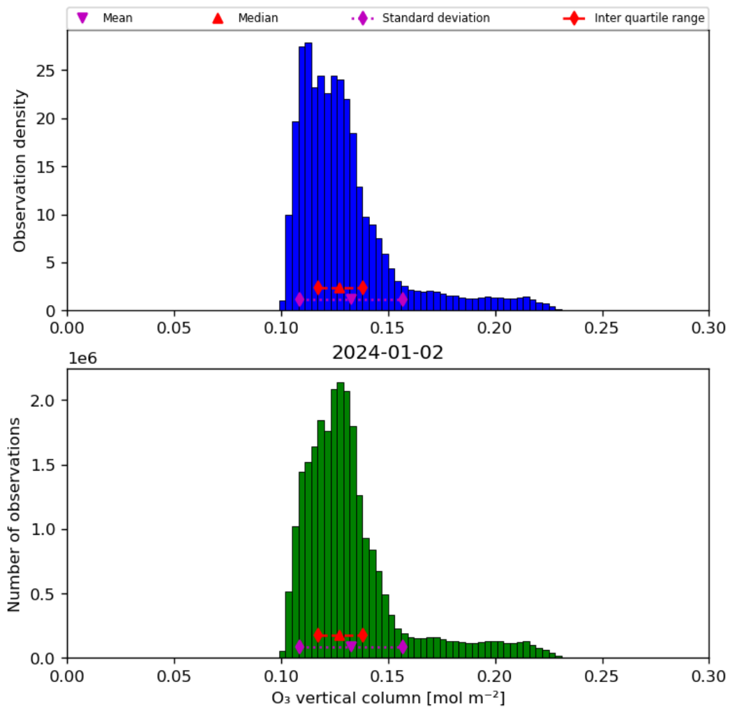
Figure 21: Histogram of “O 3 vertical column” for 2024-01-01 to 2024-01-03
