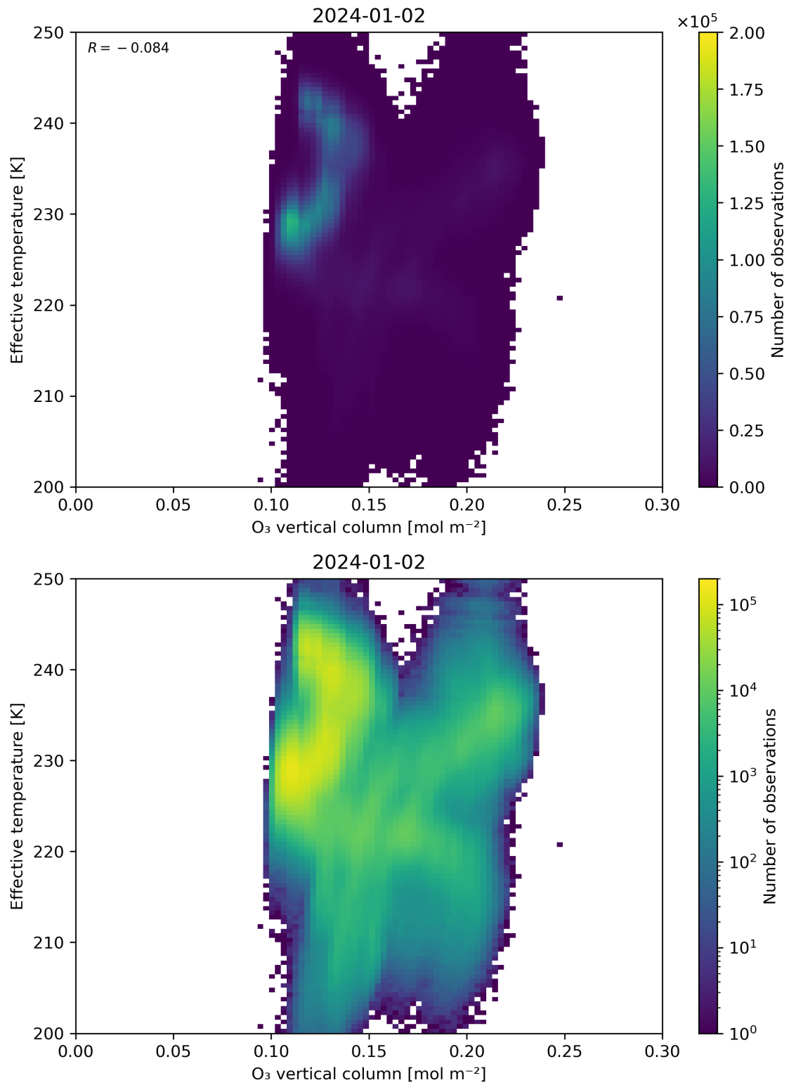
Figure 39: Scatter density plot of “O 3 vertical column” against “Effective temperature” for 2024-01-01 to 2024-01-03.
