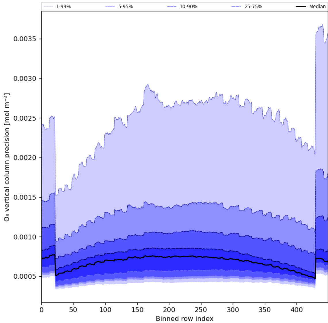
Figure 29: Along track statistics of “O 3 vertical column precision” for 2024-01-01 to 2024-01-03
