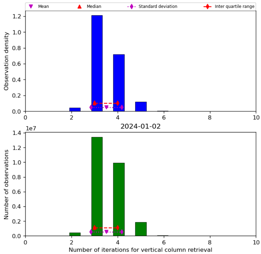
Figure 26: Histogram of “Number of iterations for vertical column retrieval” for 2024-01-01 to 2024-01-03
