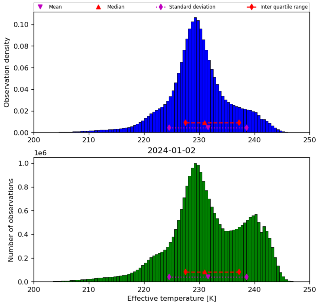
Figure 24: Histogram of “Effective temperature” for 2024-01-01 to 2024-01-03
