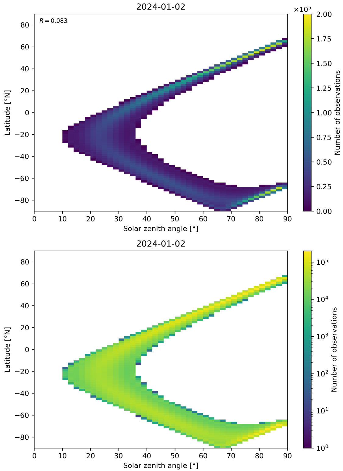
Figure 44: Scatter density plot of “Solar zenith angle” against “Latitude” for 2024-01-01 to 2024-01-03.
