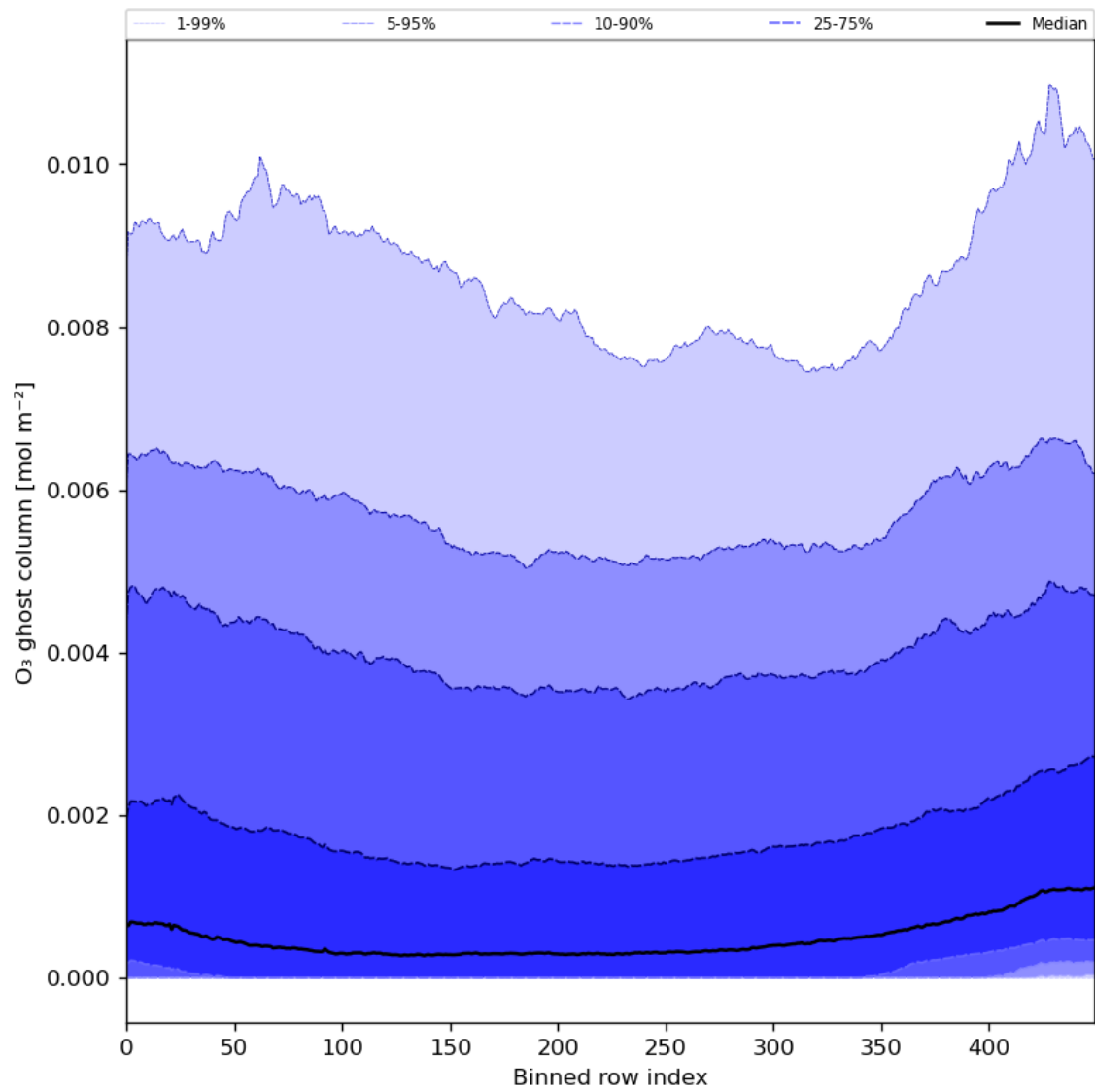
Figure 32: Along track statistics of “O 3 ghost column” for 2024-01-01 to 2024-01-03
