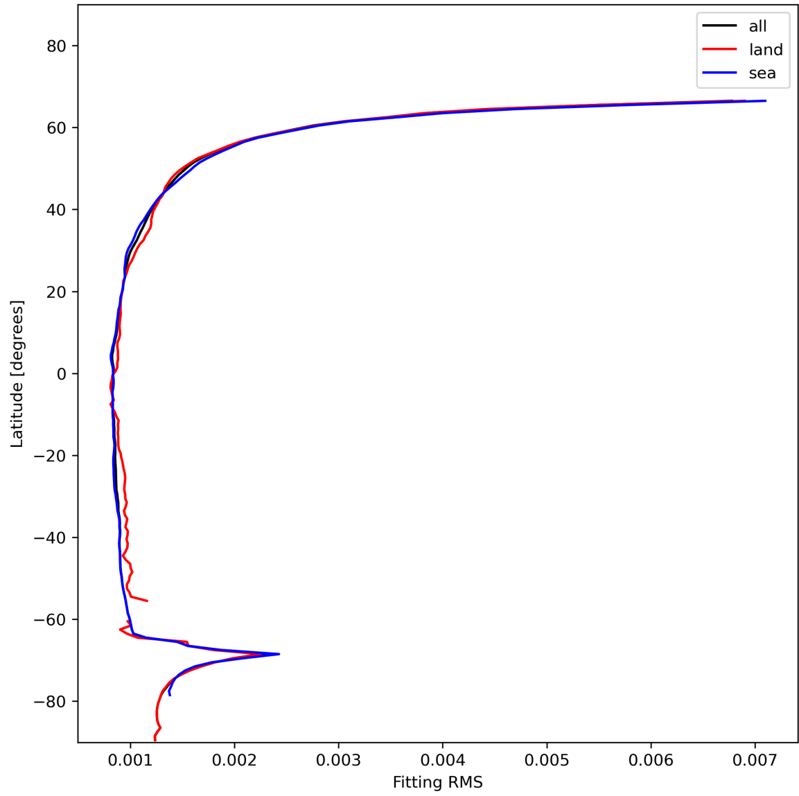
Figure 16: Zonal average of “Fitting RMS” for 2024-01-01 to 2024-01-03.
