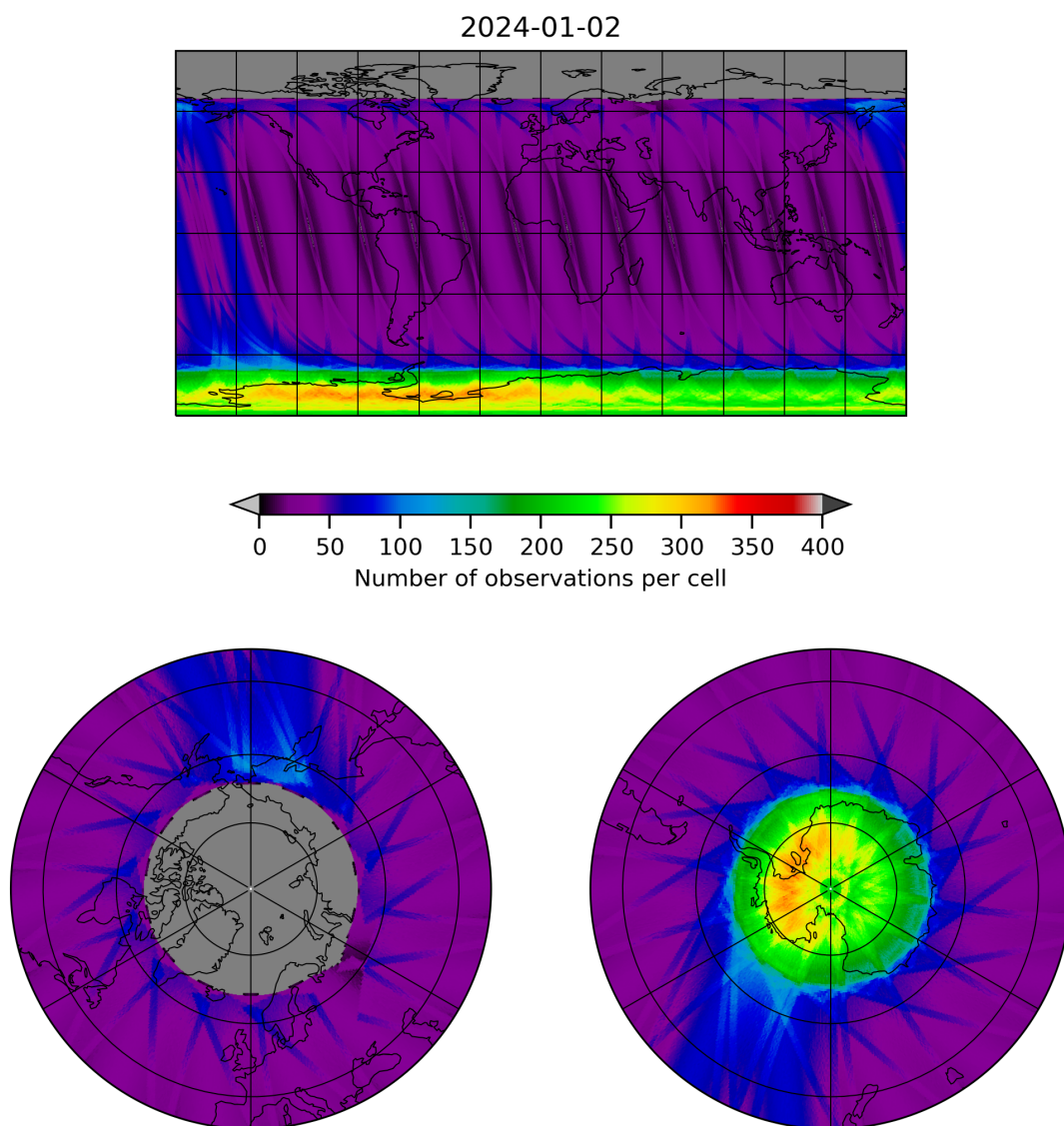
Figure 12: Map of the number of observations for 2024-01-01 to 2024-01-03
