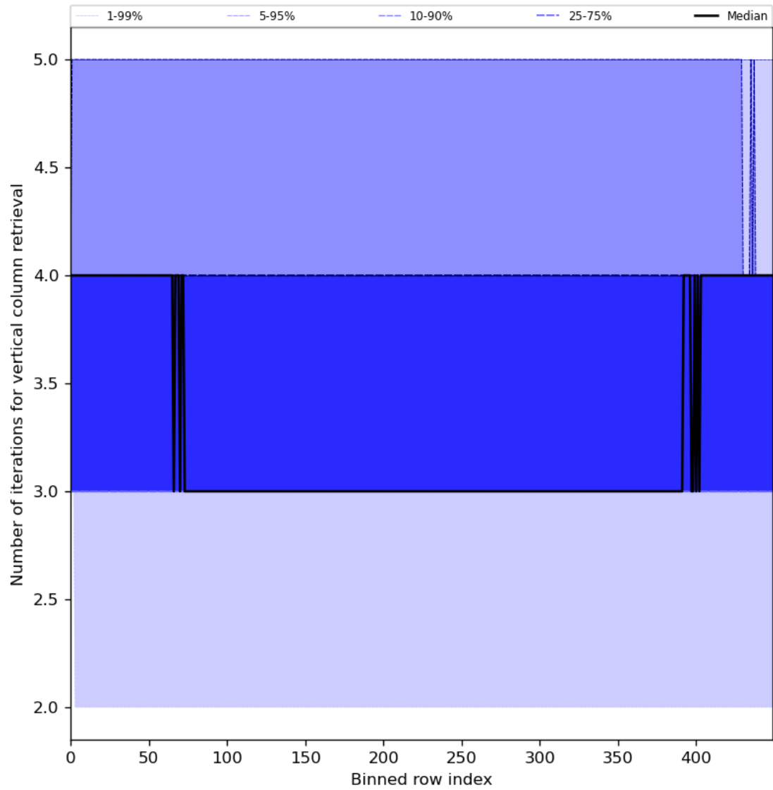
Figure 33: Along track statistics of “Number of iterations for vertical column retrieval” for 2024-01-01 to 2024-01-03
