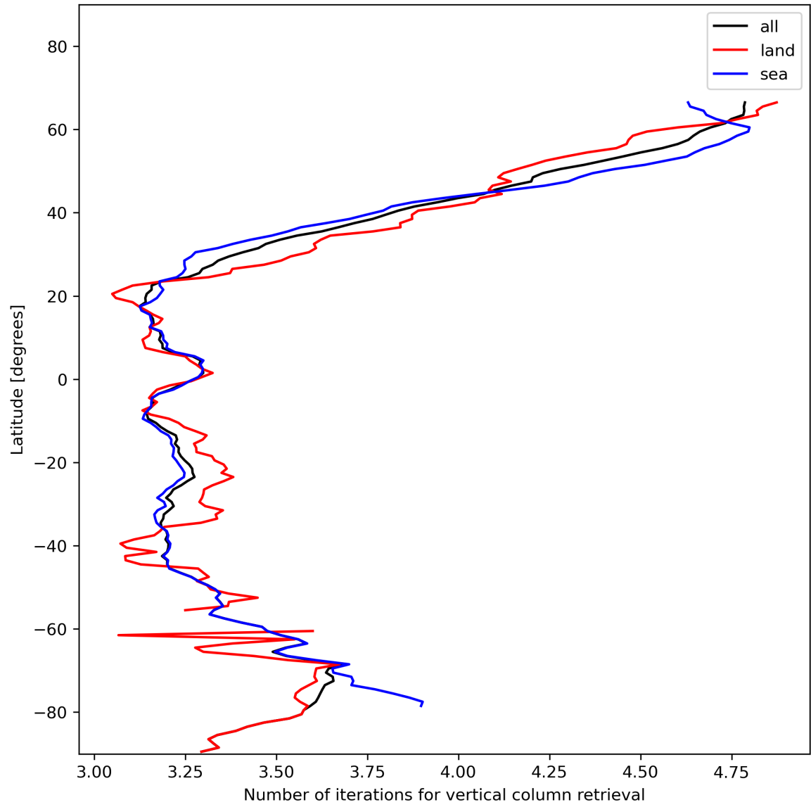
Figure 19: Zonal average of “Number of iterations for vertical column retrieval” for 2024-01-01 to 2024-01-03.
