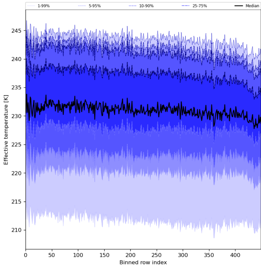
Figure 31: Along track statistics of “Effective temperature” for 2024-01-01 to 2024-01-03
