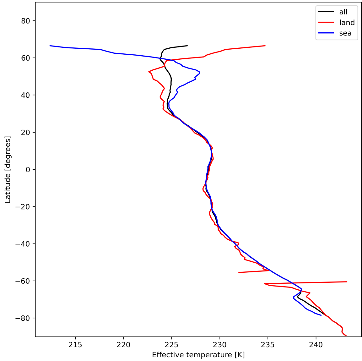
Figure 17: Zonal average of "Effective temperature" for 2024-01-01 to 2024-01-03.
