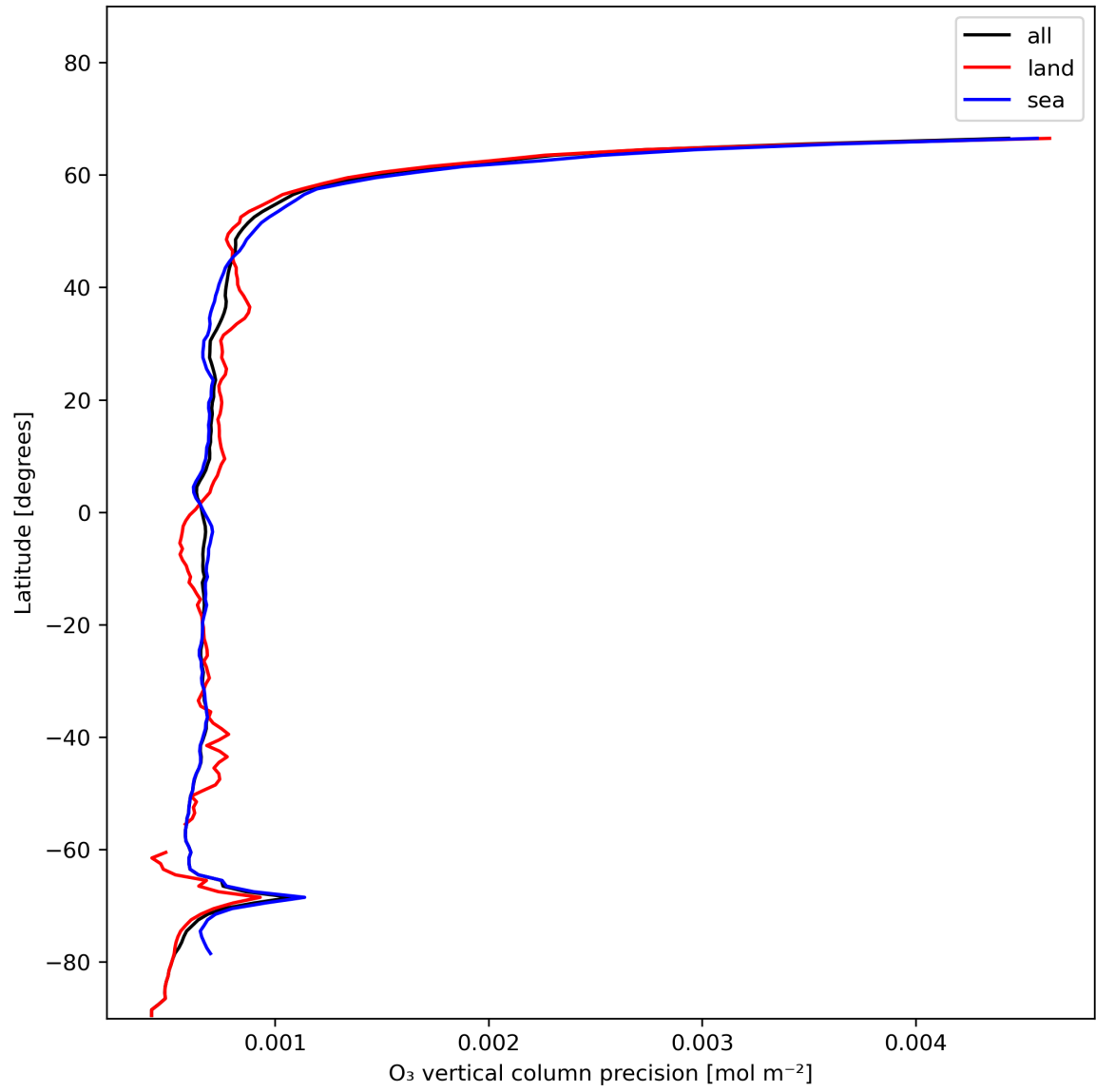
Figure 15: Zonal average of "O 3 vertical column precision" for 2024-01-01 to 2024-01-03.
