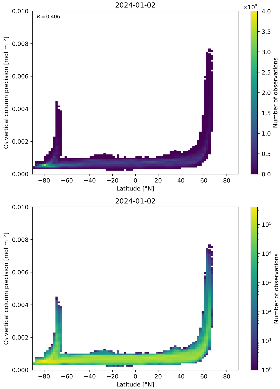
Figure 37: Scatter density plot of “Latitude” against “O 3 vertical column precision” for 2024-01-01 to 2024-01-03.
