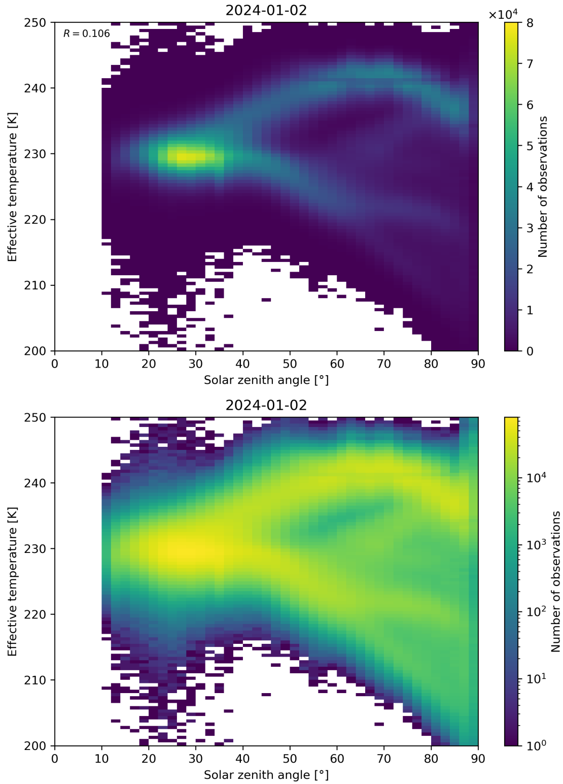
Figure 45: Scatter density plot of “Solar zenith angle” against “Effective temperature” for 2024-01-01 to 2024-01-03.
