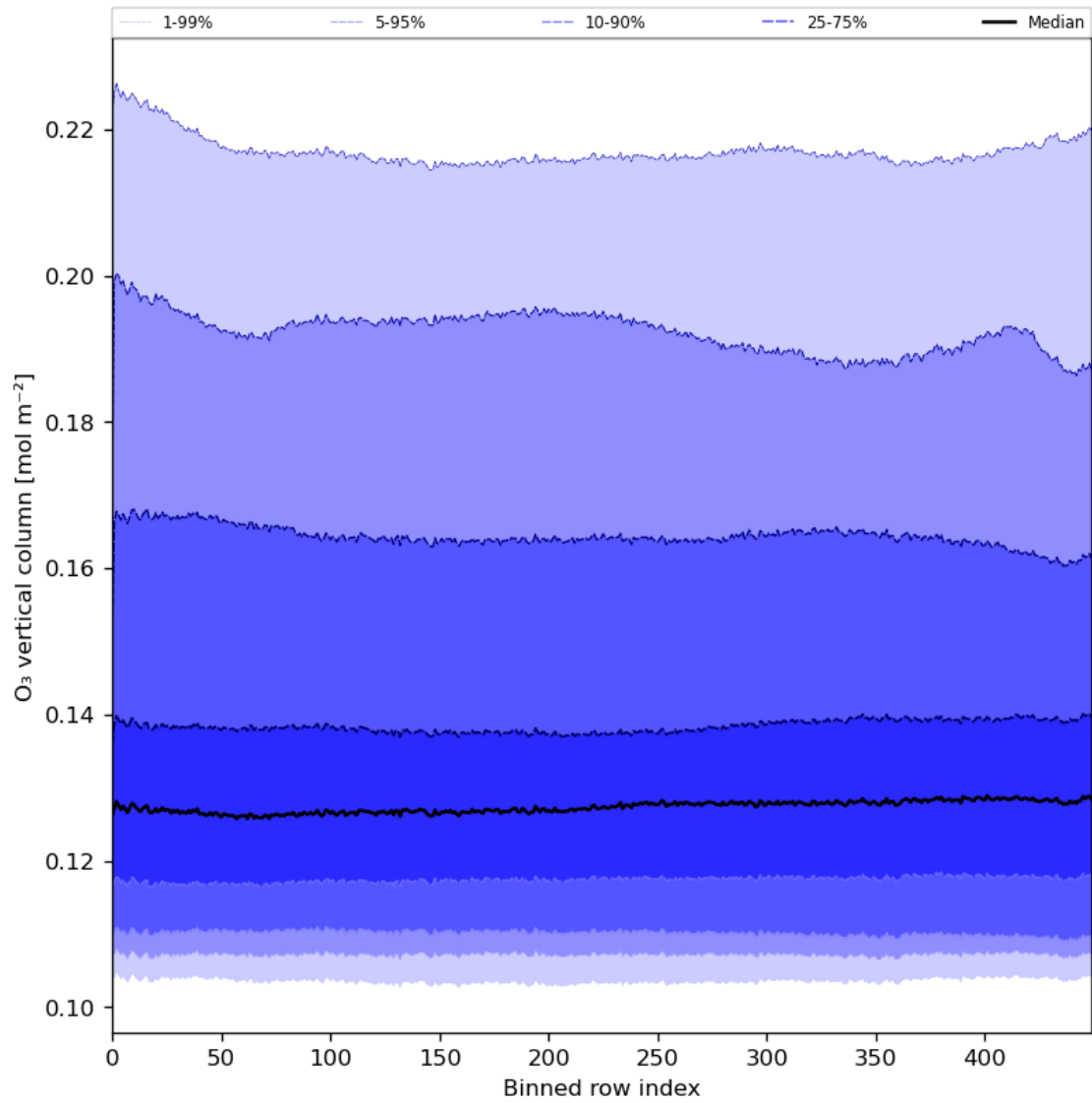
Figure 28: Along track statistics of “O 3 vertical column” for 2024-01-01 to 2024-01-03
