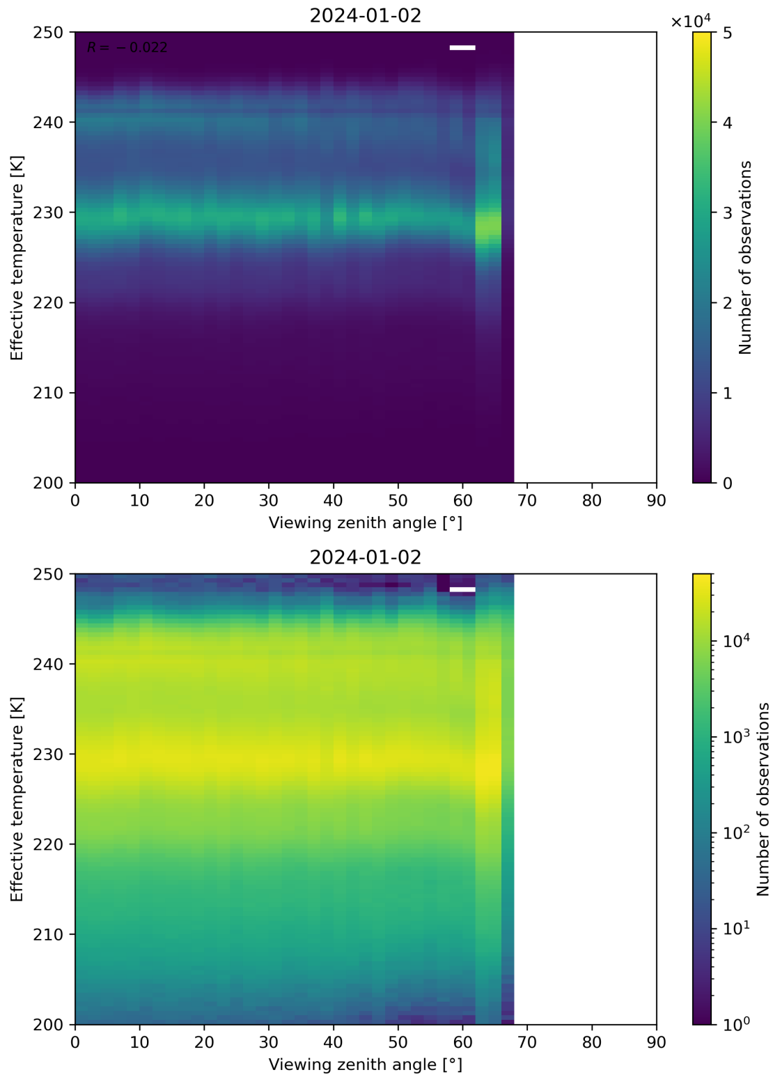
Figure 50: Scatter density plot of “Viewing zenith angle” against “Effective temperature” for 2024-01-01 to 2024-01-03.
