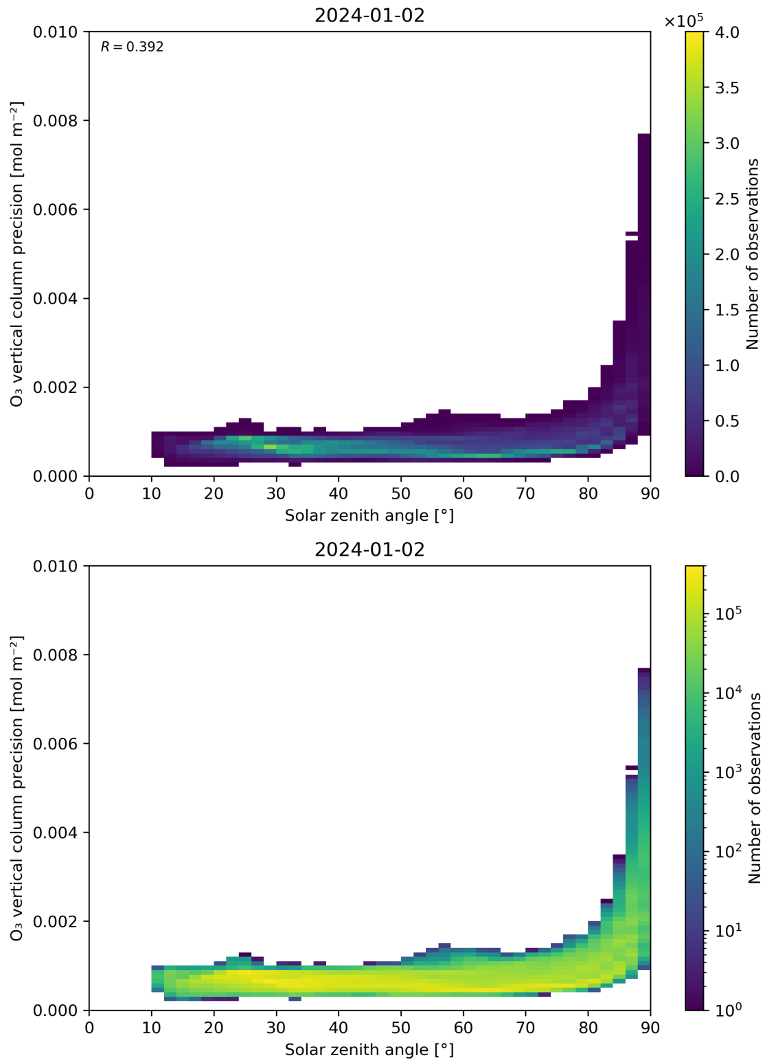
Figure 48: Scatter density plot of “Solar zenith angle” against “O 3 vertical column precision” for 2024-01-01 to 2024-01-03.
