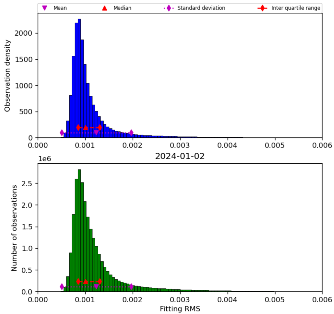
Figure 23: Histogram of “Fitting RMS” for 2024-01-01 to 2024-01-03
