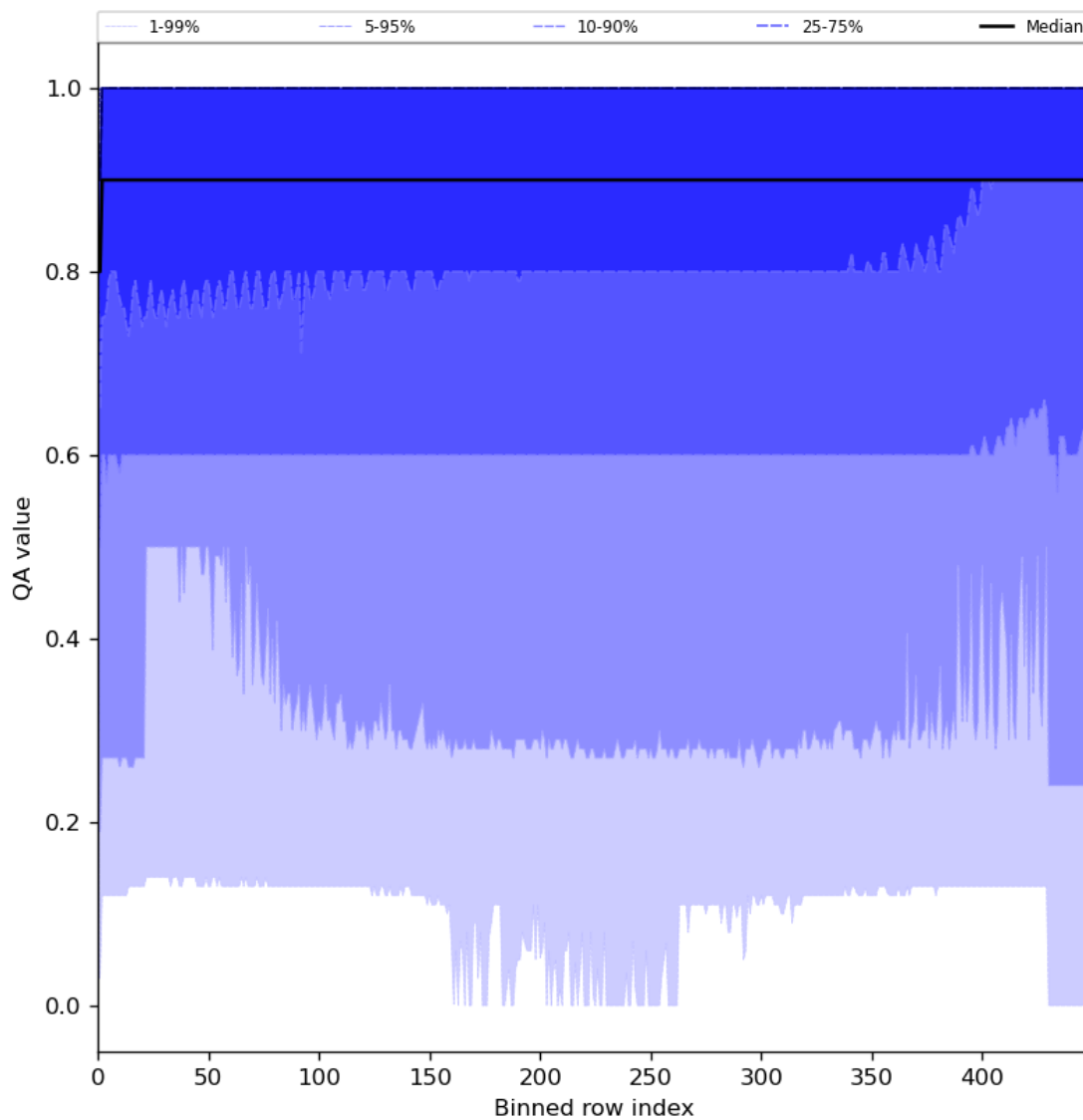
Figure 27: Along track statistics of “QA value” for 2024-01-01 to 2024-01-03
