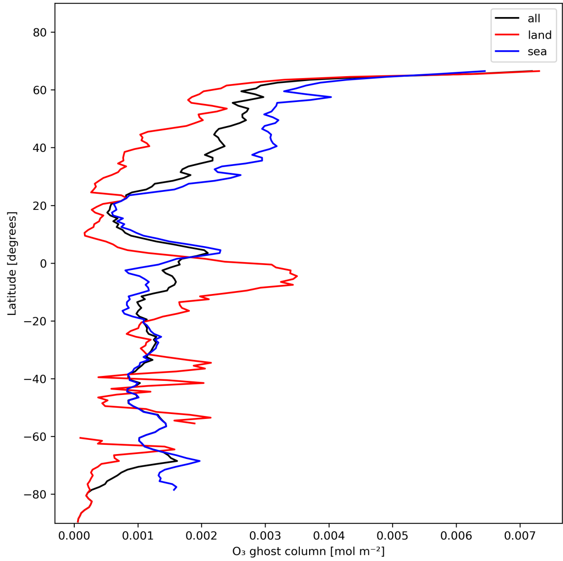
Figure 18: Zonal average of “O 3 ghost column” for 2024-01-01 to 2024-01-03.
