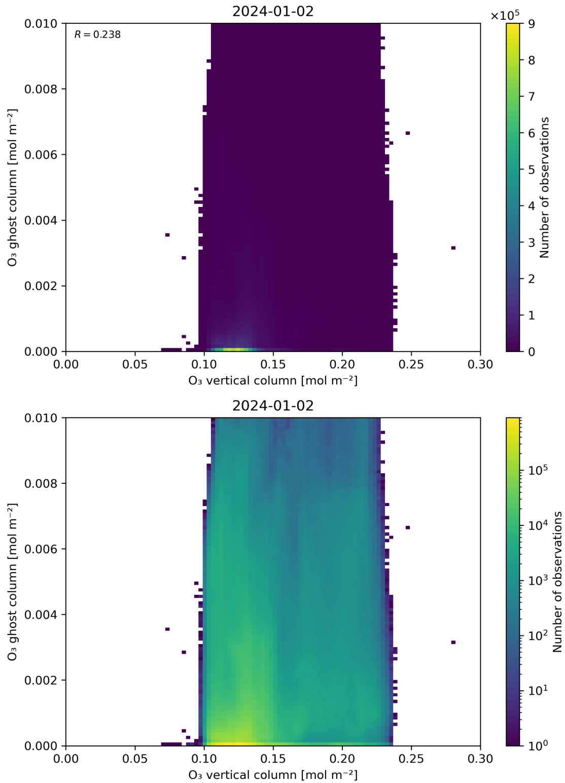
Figure 40: Scatter density plot of “O 3 vertical column” against “O 3 ghost column” for 2024-01-01 to 2024-01-03.
