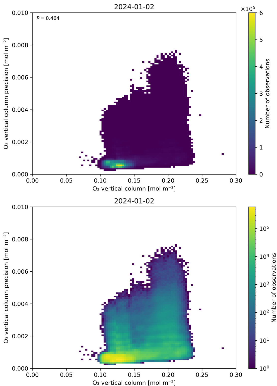
Figure 41: Scatter density plot of “O 3 vertical column” against “O 3 vertical column precision” for 2024-01-01 to 2024-01-03.
