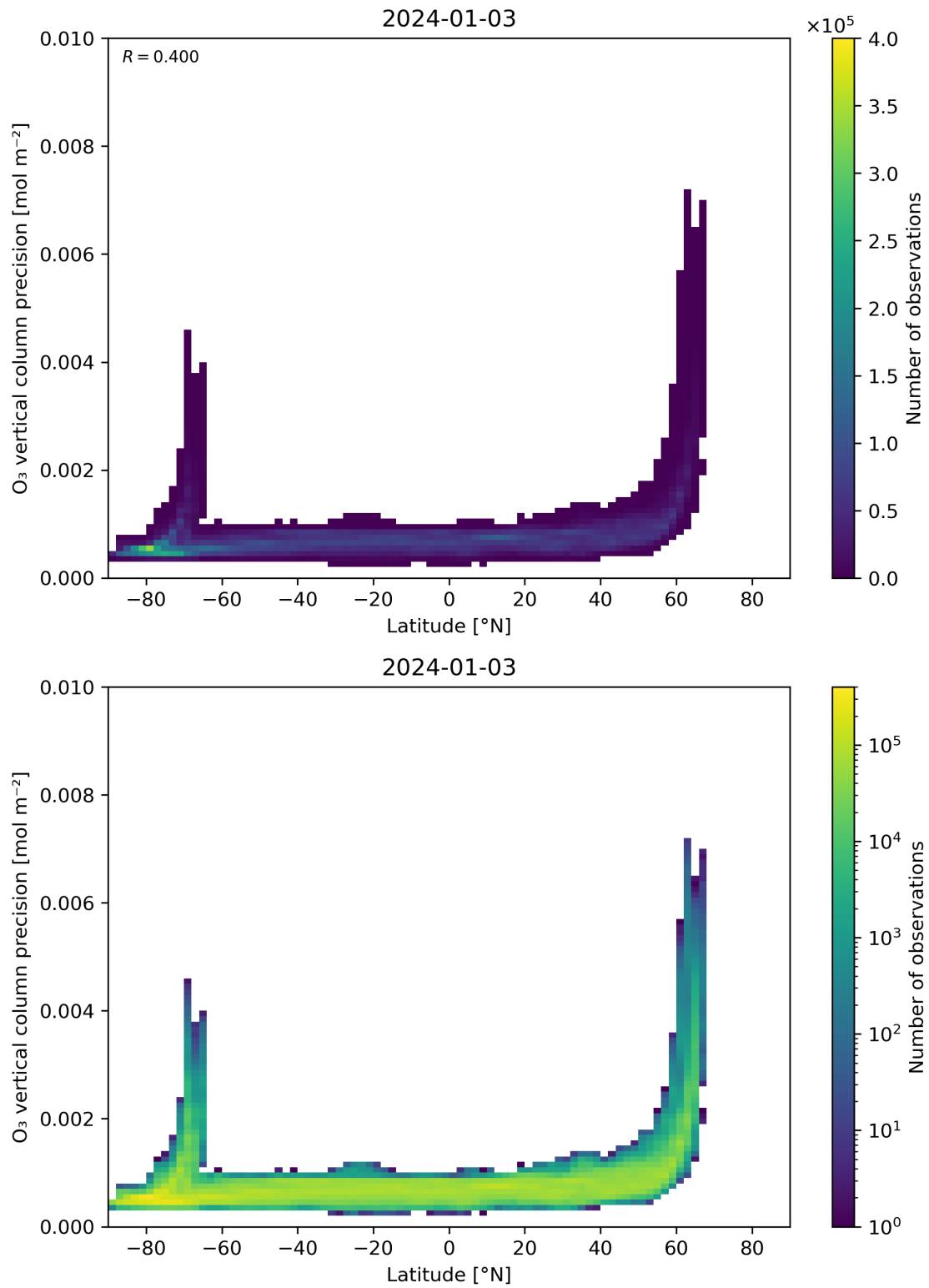
Figure 37: Scatter density plot of “Latitude” against “O 3 vertical column precision” for 2024-01-02 to 2024-01-04.
