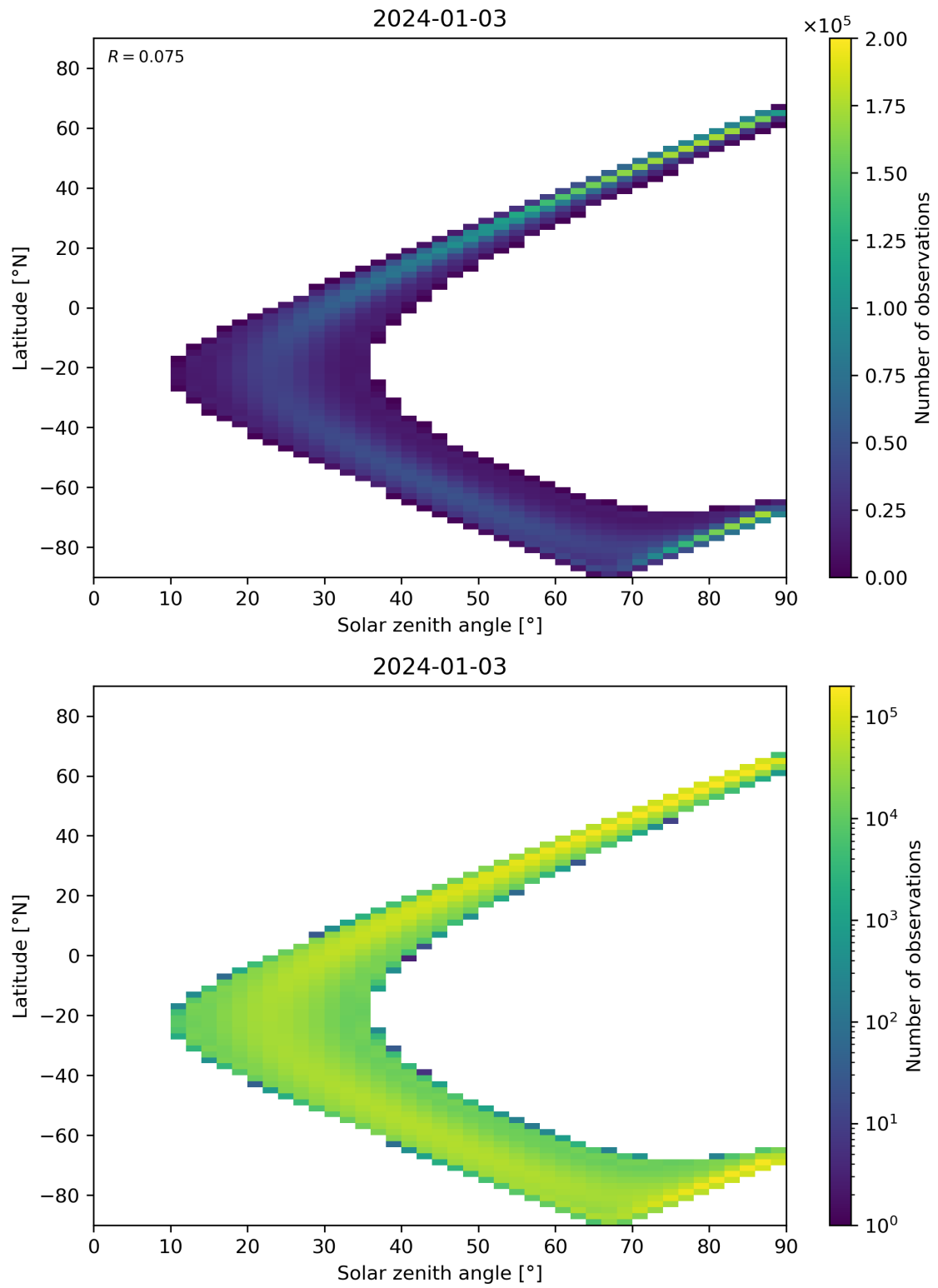
Figure 44: Scatter density plot of “Solar zenith angle” against “Latitude” for 2024-01-02 to 2024-01-04.
