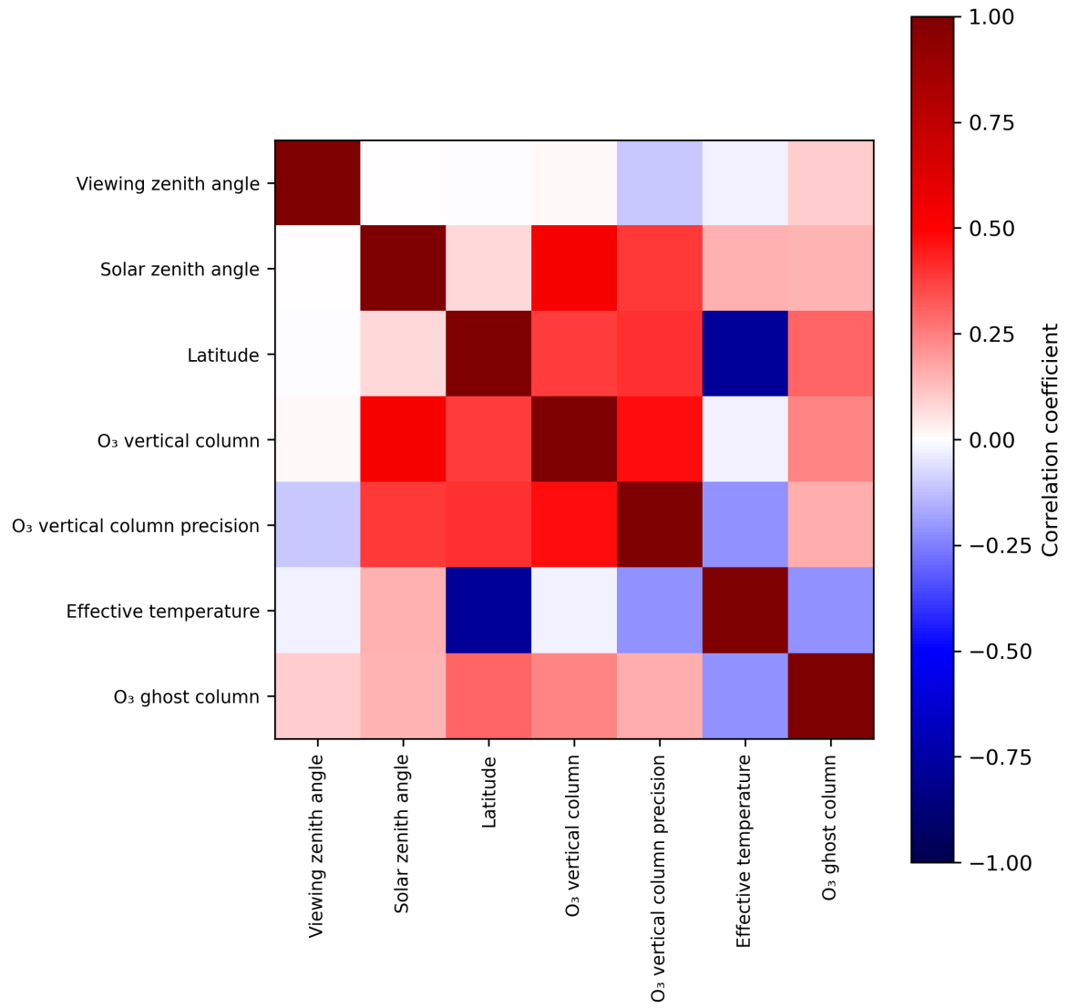
Figure 2: Map of correlation matrix for 2024-01-02 to 2024-01-04.
