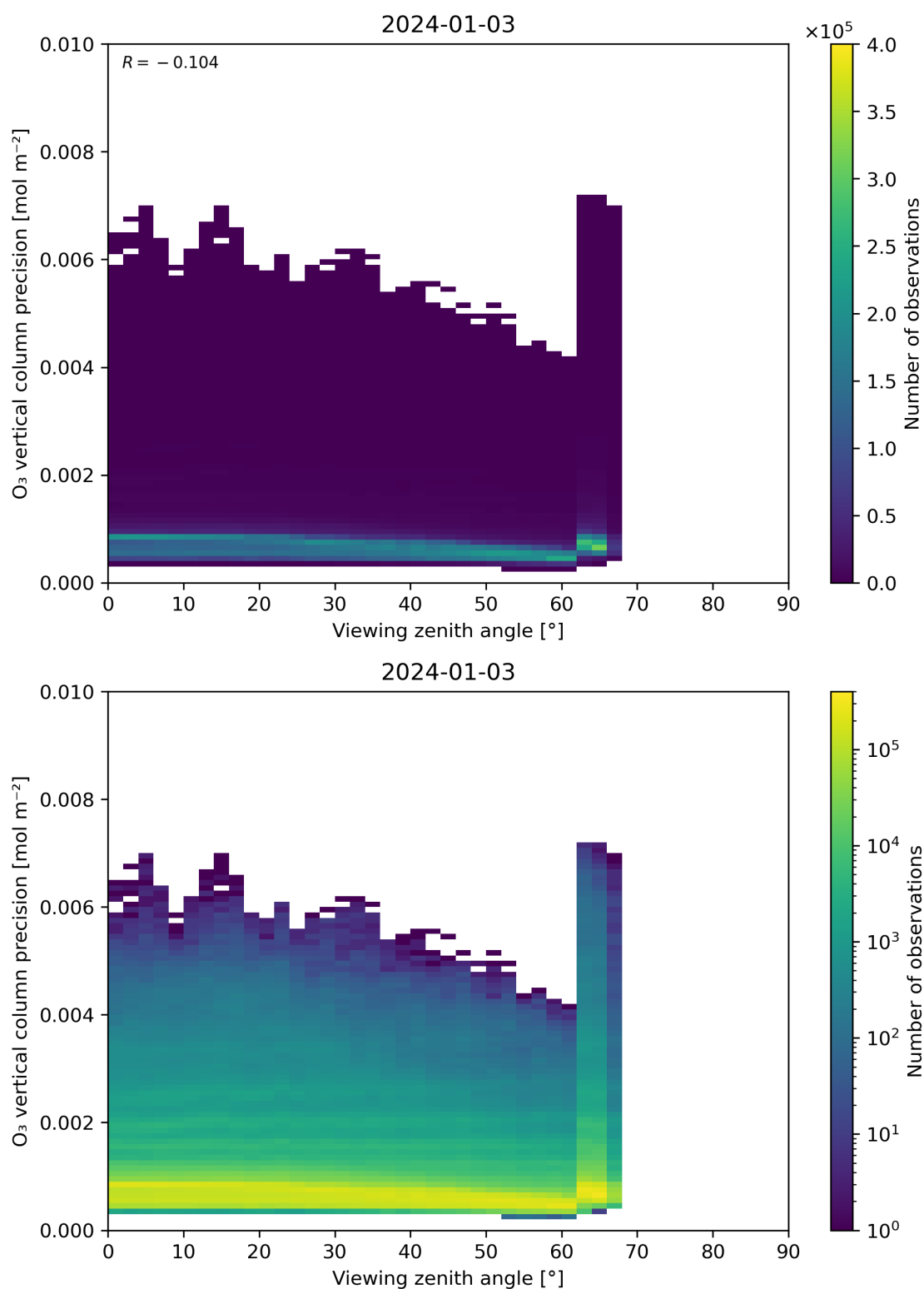
Figure 53: Scatter density plot of “Viewing zenith angle” against “O 3 vertical column precision” for 2024-01-02 to 2024-01-04.
