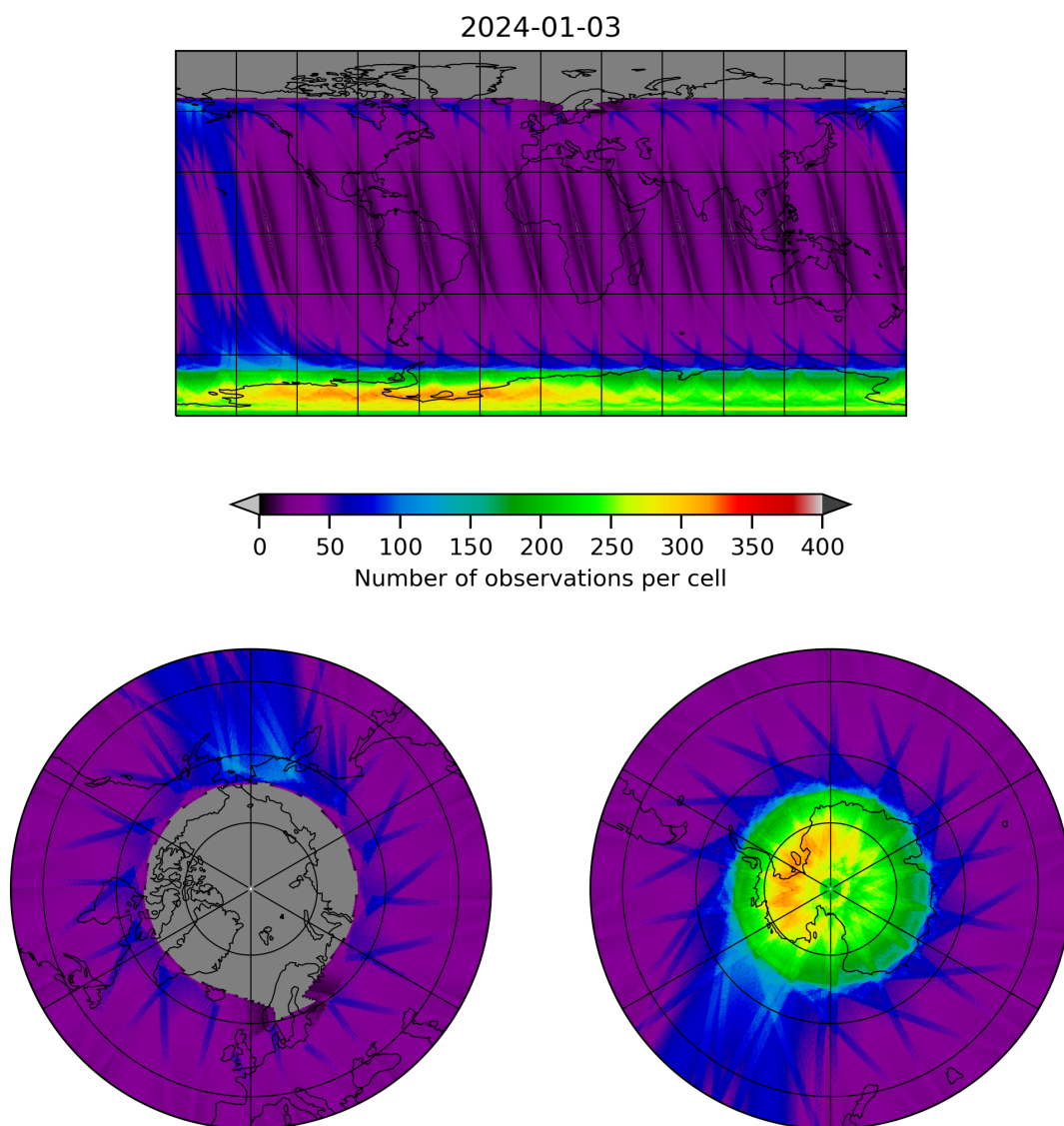
Figure 12: Map of the number of observations for 2024-01-02 to 2024-01-04
