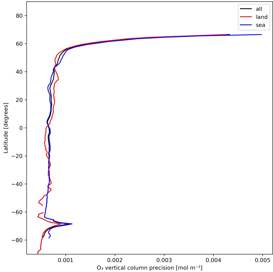
Figure 15: Zonal average of “O 3 vertical column precision” for 2024-01-02 to 2024-01-04.
