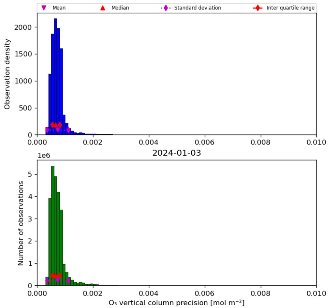
Figure 22: Histogram of “O 3 vertical column precision” for 2024-01-02 to 2024-01-04
