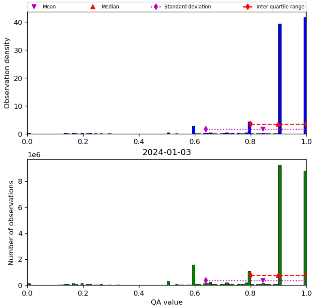
Figure 20: Histogram of “QA value” for 2024-01-02 to 2024-01-04
