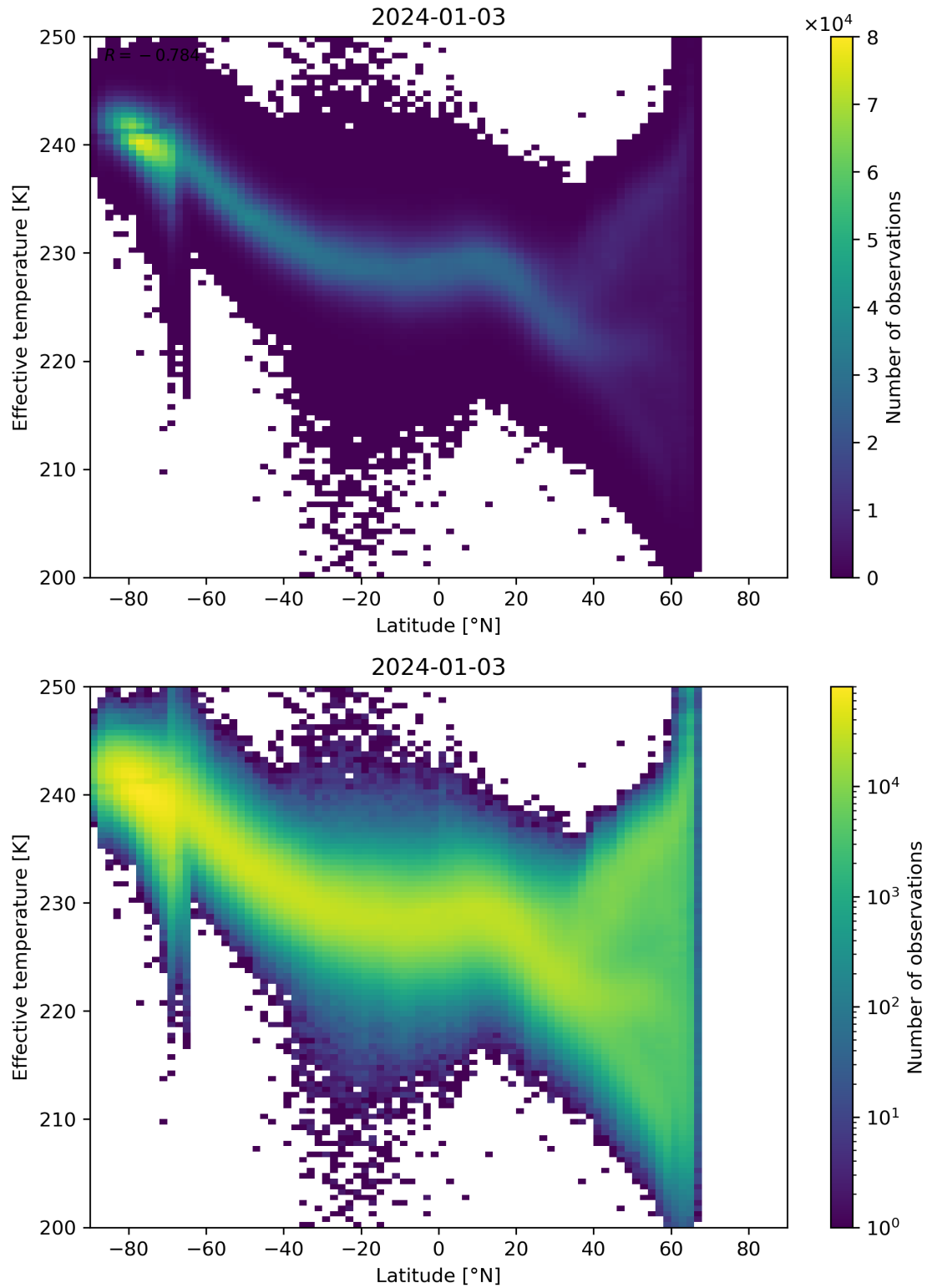
Figure 34: Scatter density plot of “Latitude” against “Effective temperature” for 2024-01-02 to 2024-01-04.
