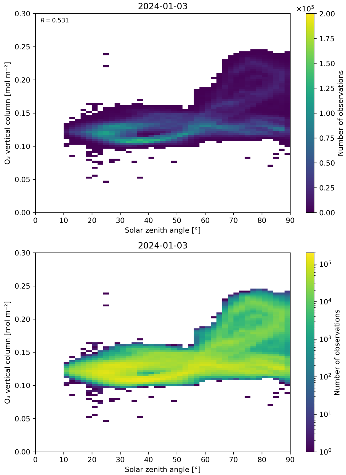
Figure 47: Scatter density plot of “Solar zenith angle” against “O 3 vertical column” for 2024-01-02 to 2024-01-04.
