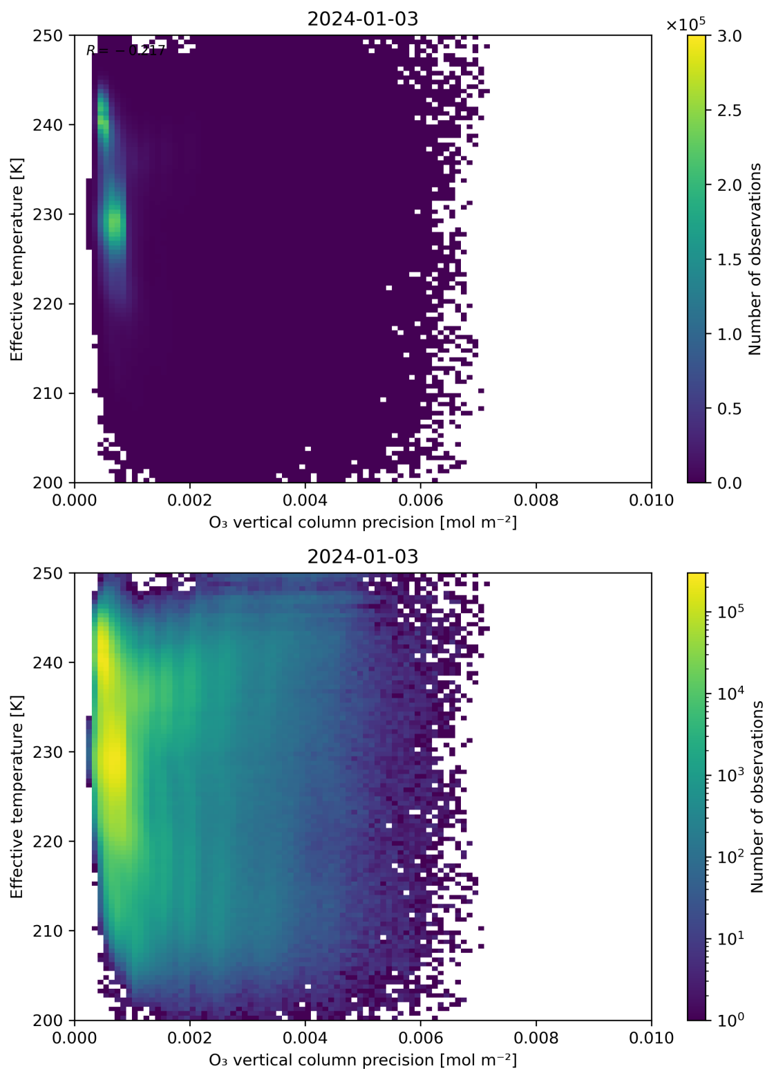
Figure 42: Scatter density plot of “O 3 vertical column precision” against “Effective temperature” for 2024-01-02 to 2024-01-04.
