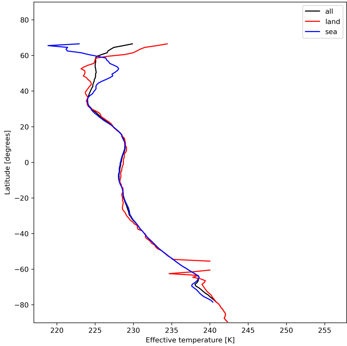
Figure 17: Zonal average of "Effective temperature" for 2024-01-02 to 2024-01-04.
