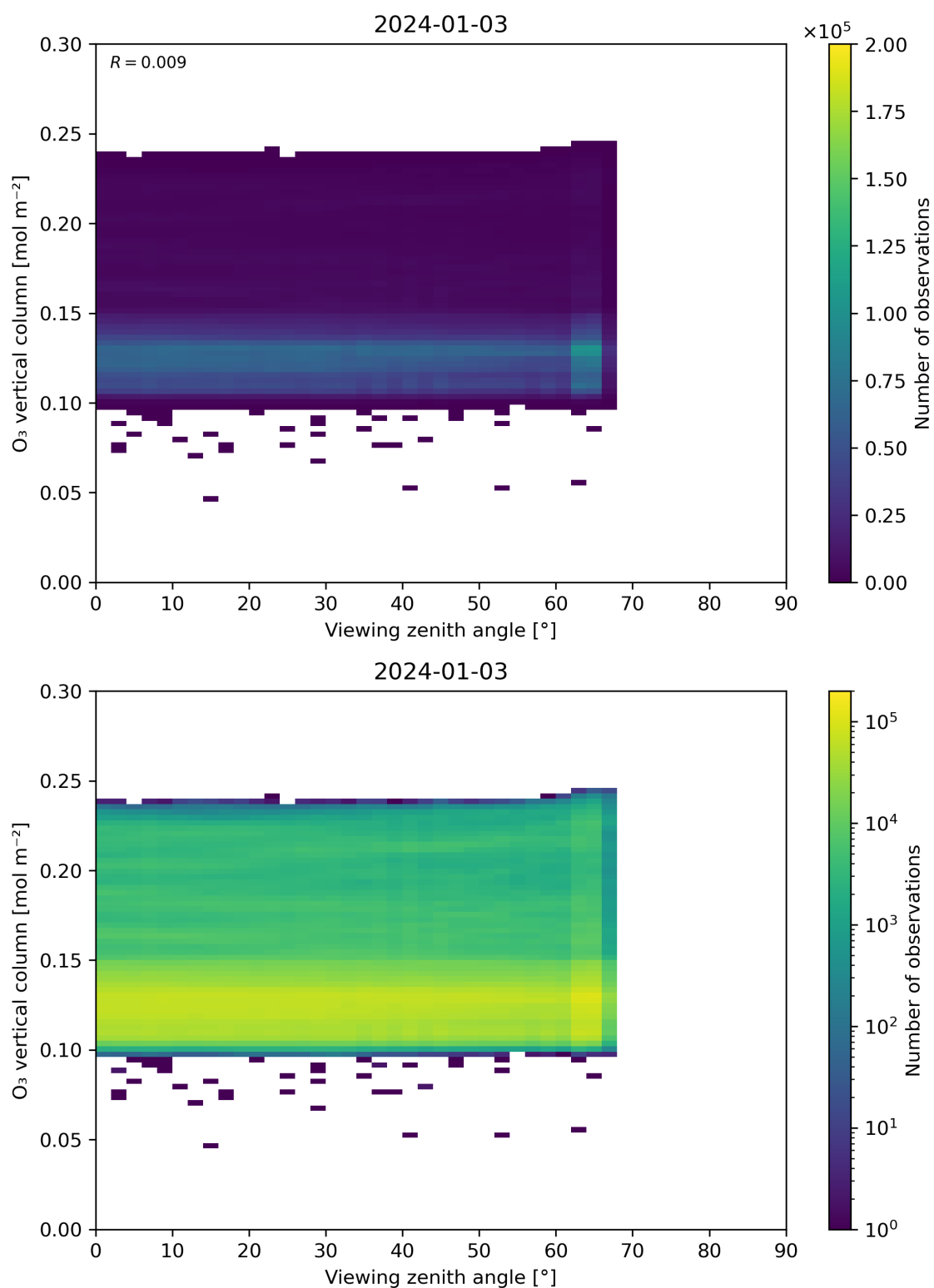
Figure 52: Scatter density plot of “Viewing zenith angle” against “O 3 vertical column” for 2024-01-02 to 2024-01-04.
