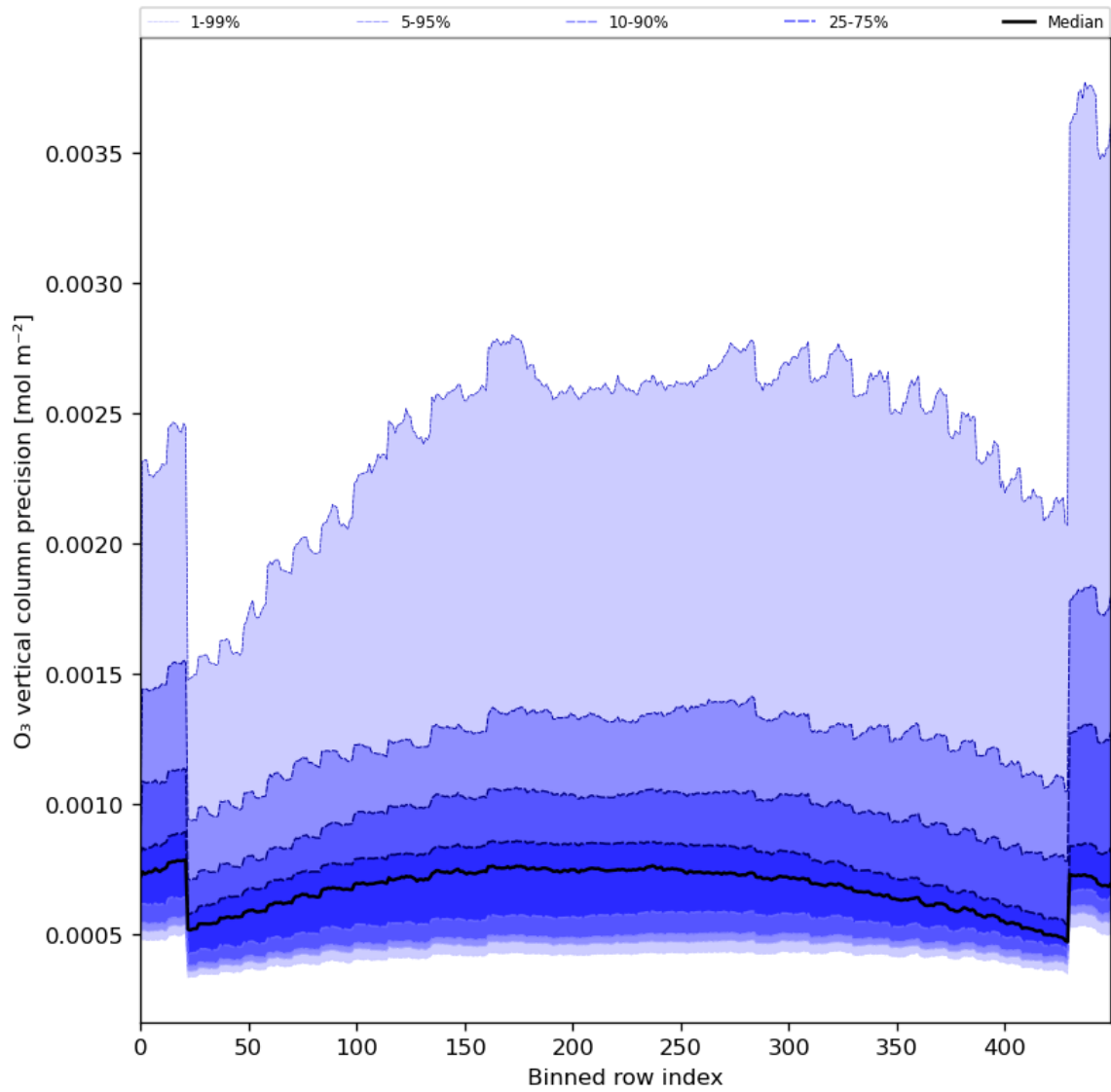
Figure 29: Along track statistics of “O 3 vertical column precision” for 2024-01-02 to 2024-01-04
