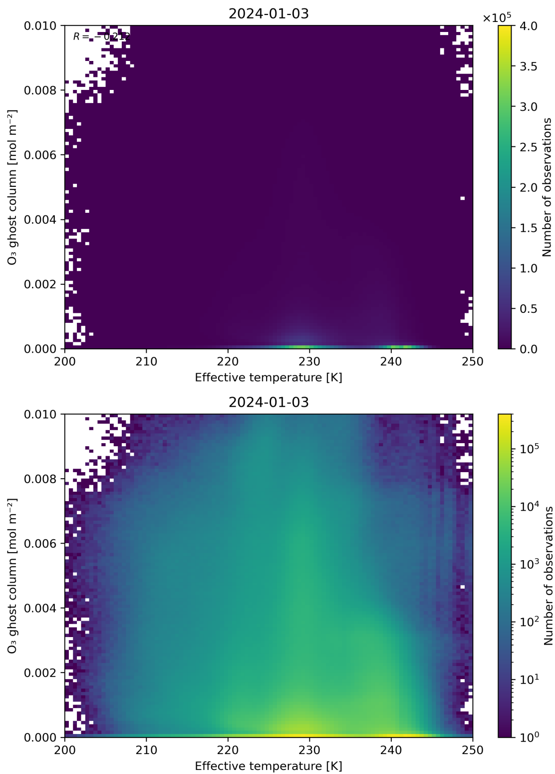
Figure 38: Scatter density plot of “Effective temperature” against “O 3 ghost column” for 2024-01-02 to 2024-01-04.
