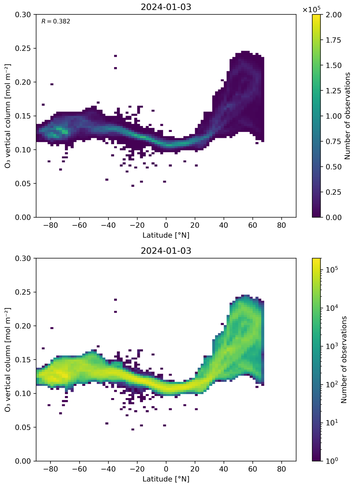
Figure 36: Scatter density plot of “Latitude” against “O 3 vertical column” for 2024-01-02 to 2024-01-04.
