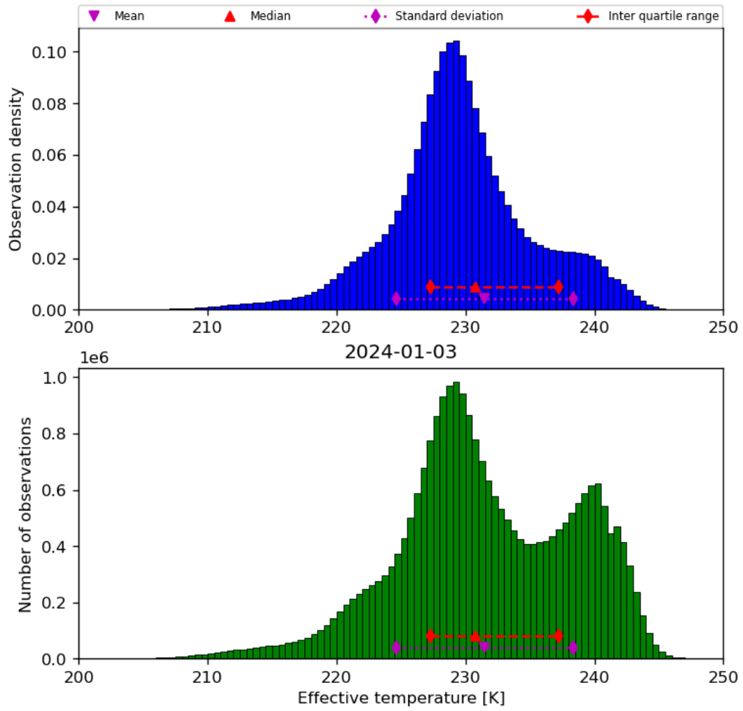
Figure 24: Histogram of “Effective temperature” for 2024-01-02 to 2024-01-04
