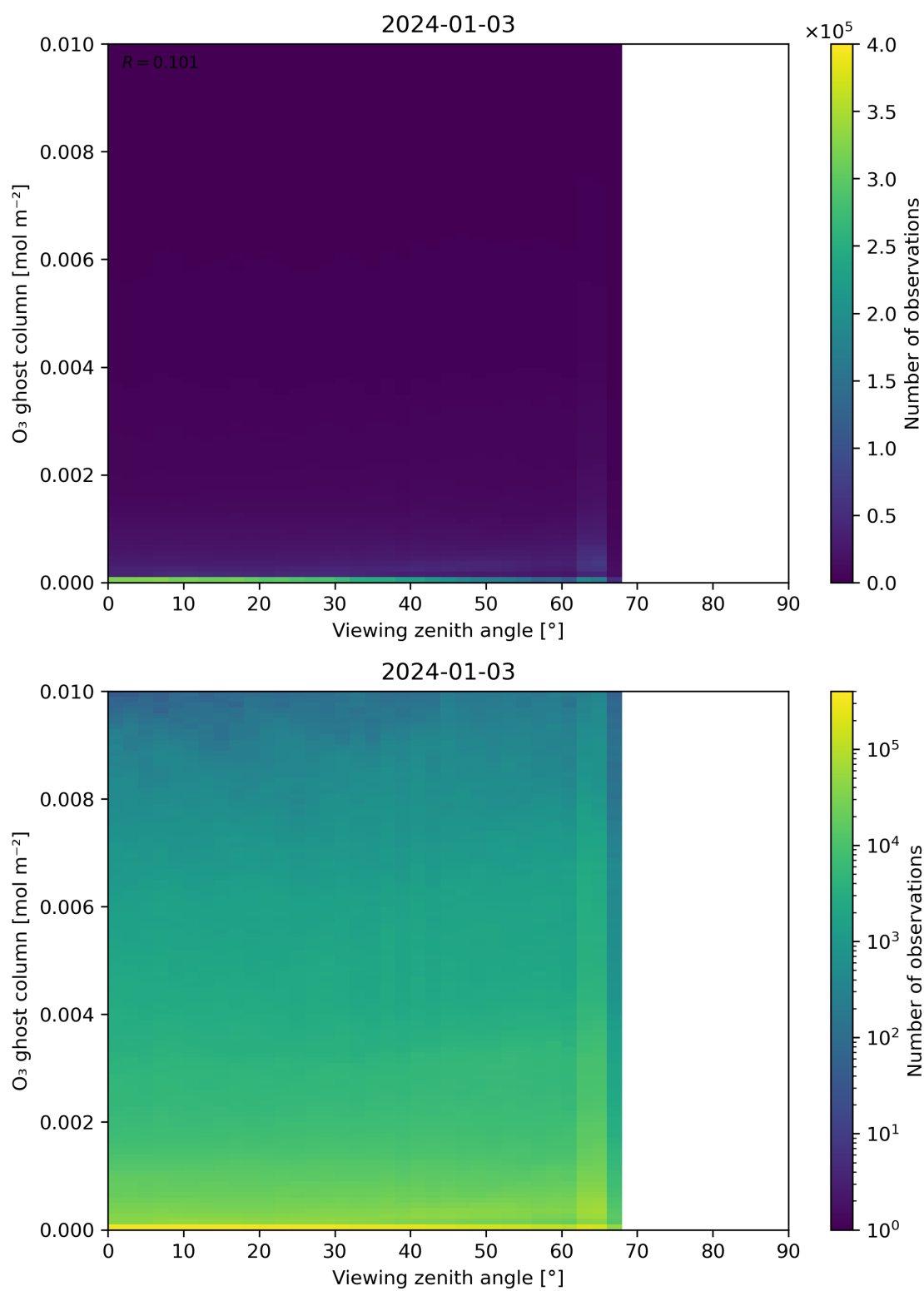
Figure 51: Scatter density plot of “Viewing zenith angle” against “O 3 ghost column” for 2024-01-02 to 2024-01-04.
