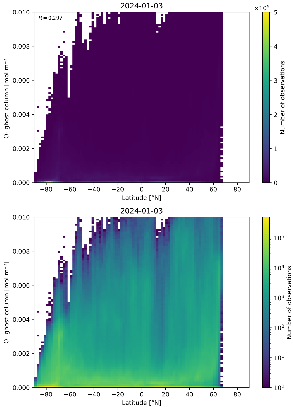
Figure 35: Scatter density plot of “Latitude” against “O 3 ghost column” for 2024-01-02 to 2024-01-04.
