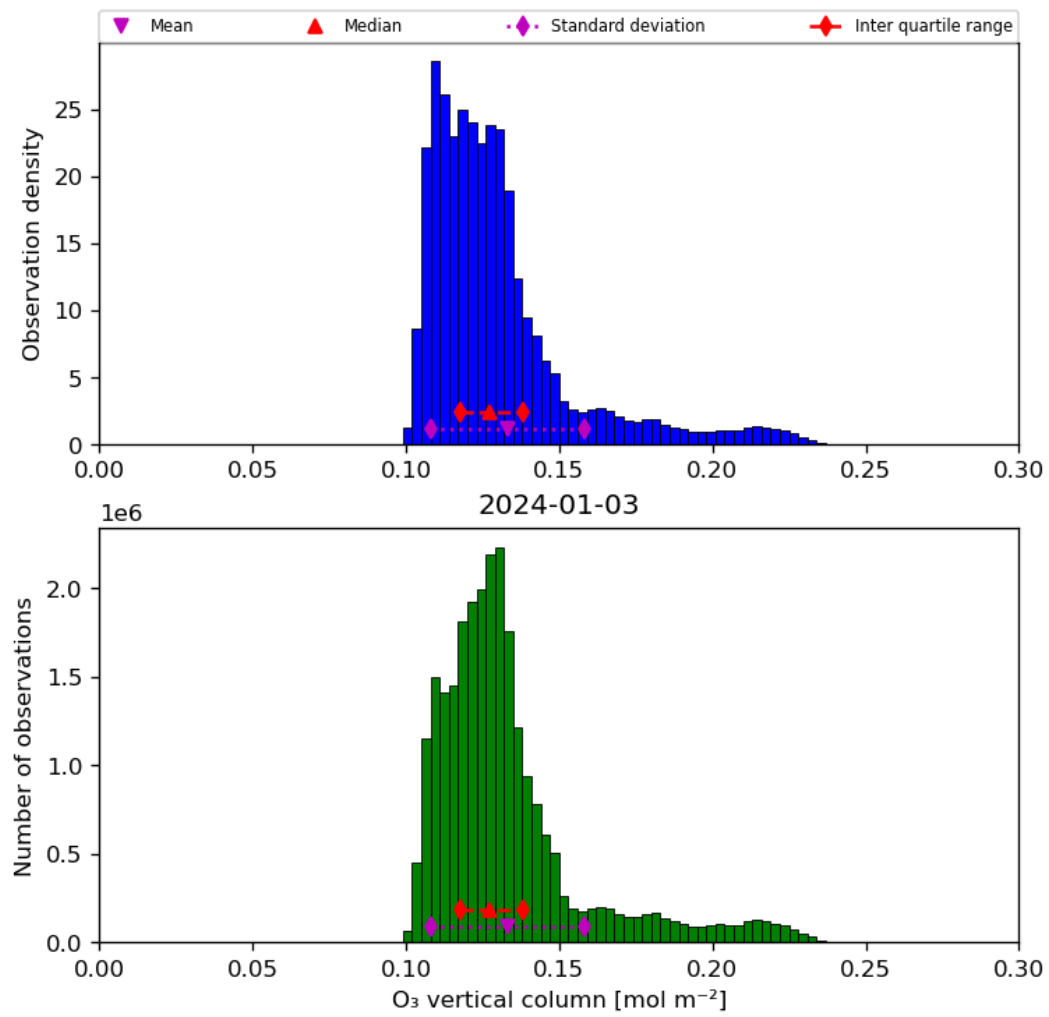
Figure 21: Histogram of “O 3 vertical column” for 2024-01-02 to 2024-01-04
