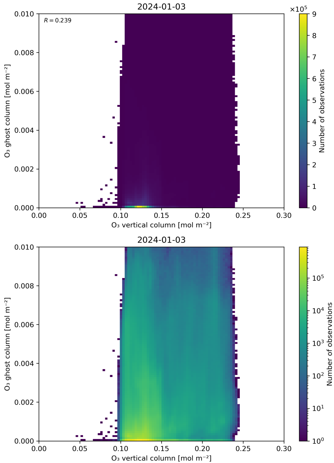
Figure 40: Scatter density plot of “O 3 vertical column” against “O 3 ghost column” for 2024-01-02 to 2024-01-04.
