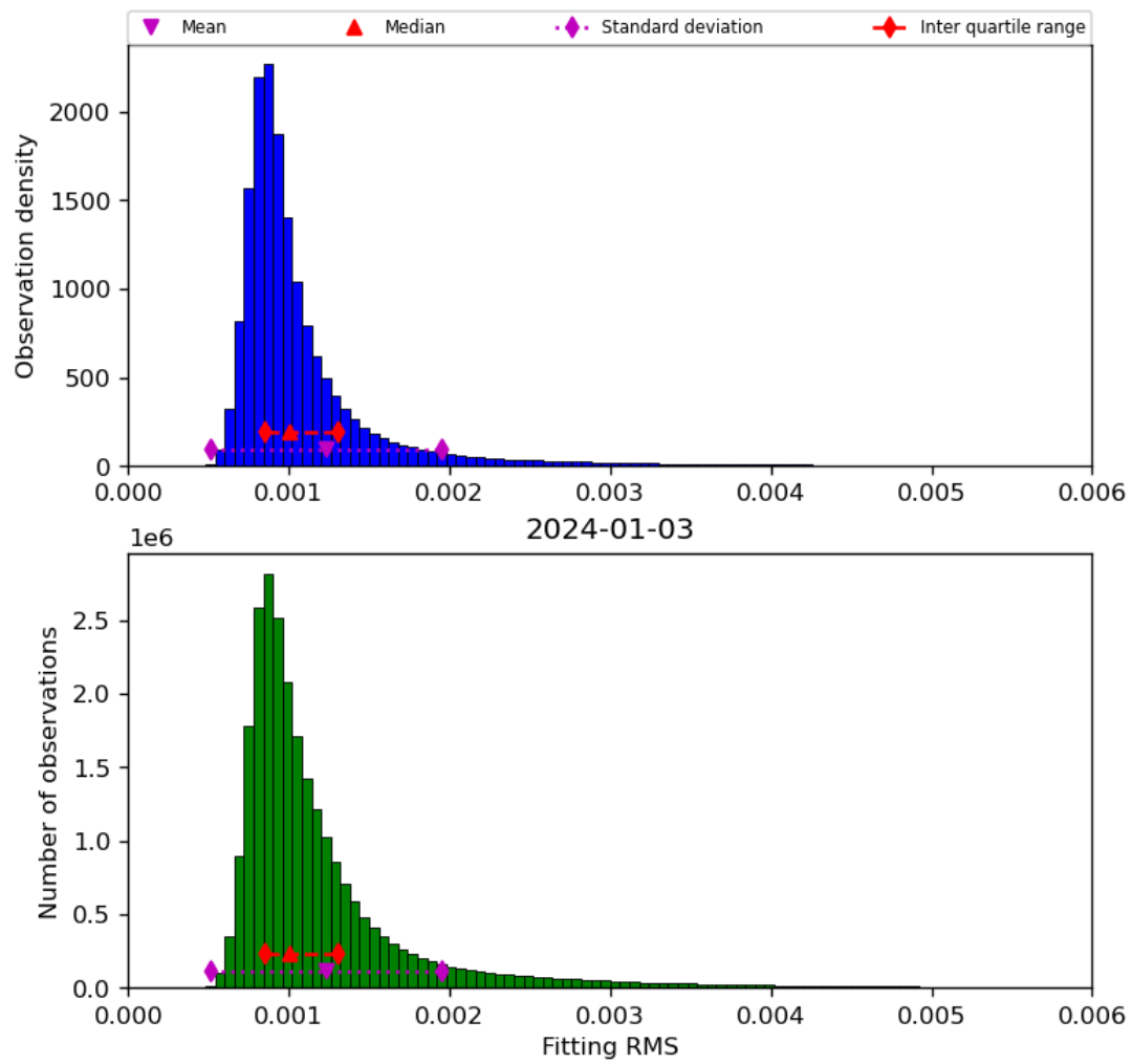
Figure 23: Histogram of “Fitting RMS” for 2024-01-02 to 2024-01-04
