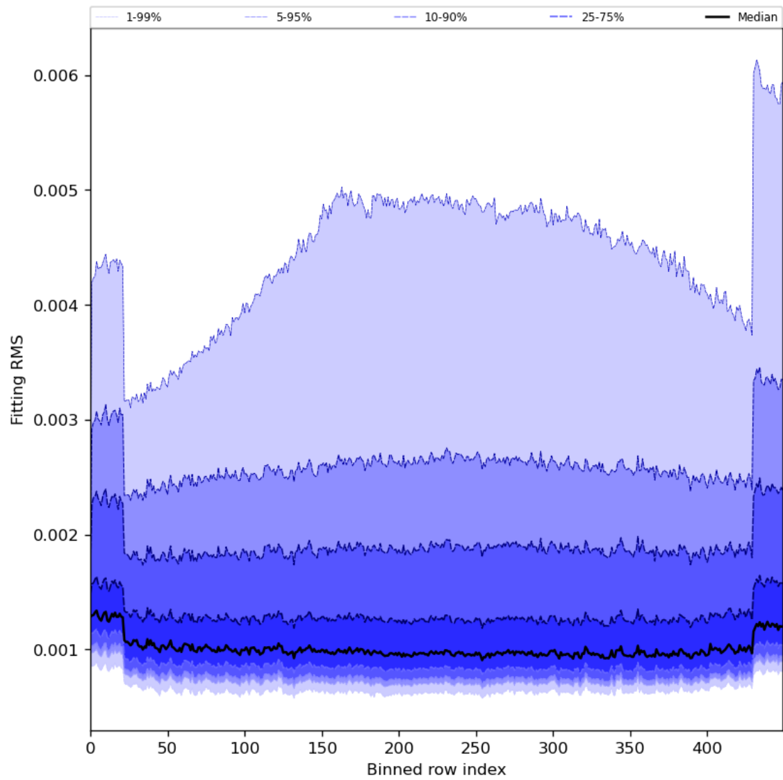
Figure 30: Along track statistics of “Fitting RMS” for 2024-01-02 to 2024-01-04
