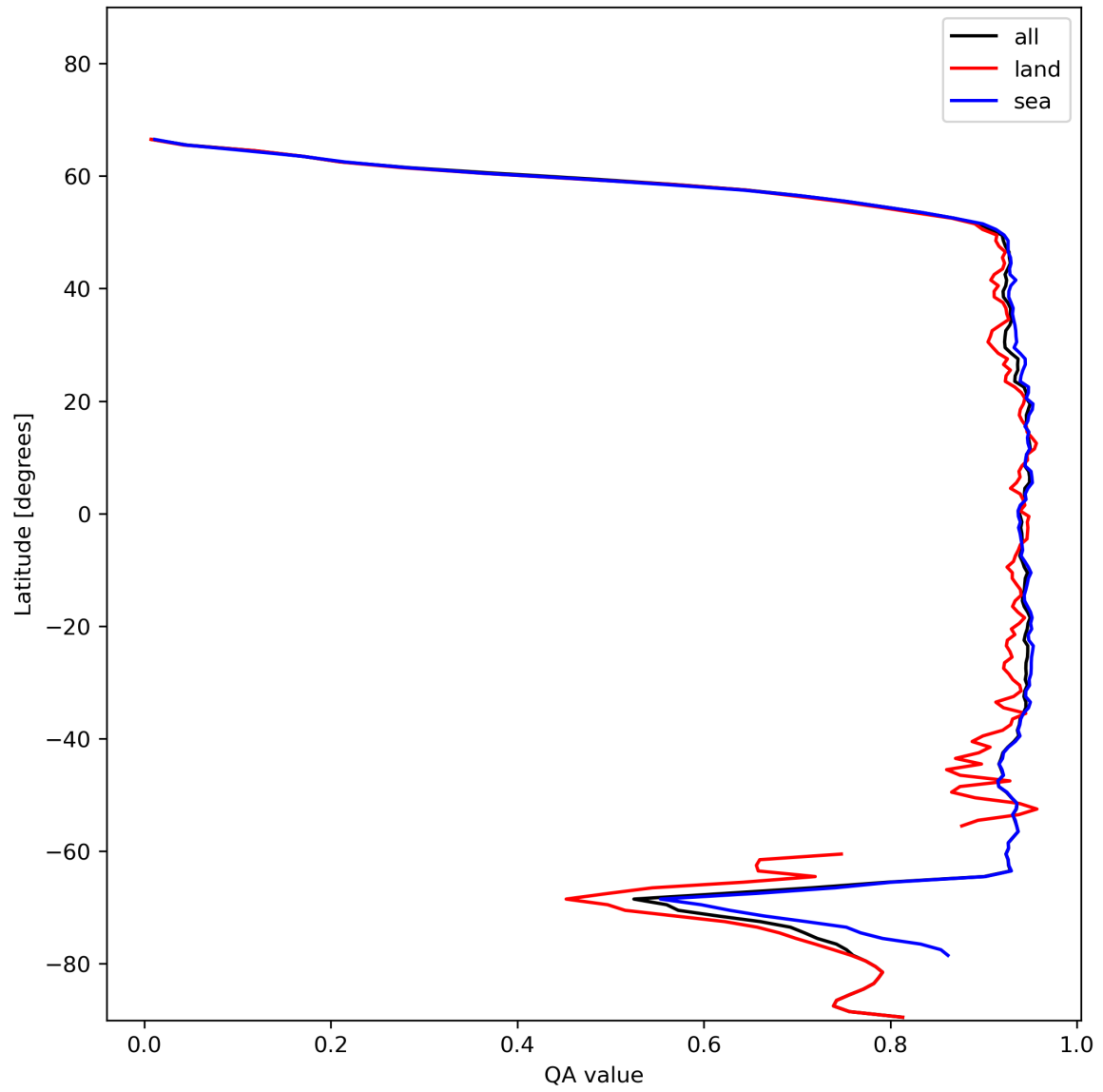
Figure 13: Zonal average of “QA value” for 2024-01-02 to 2024-01-04.
