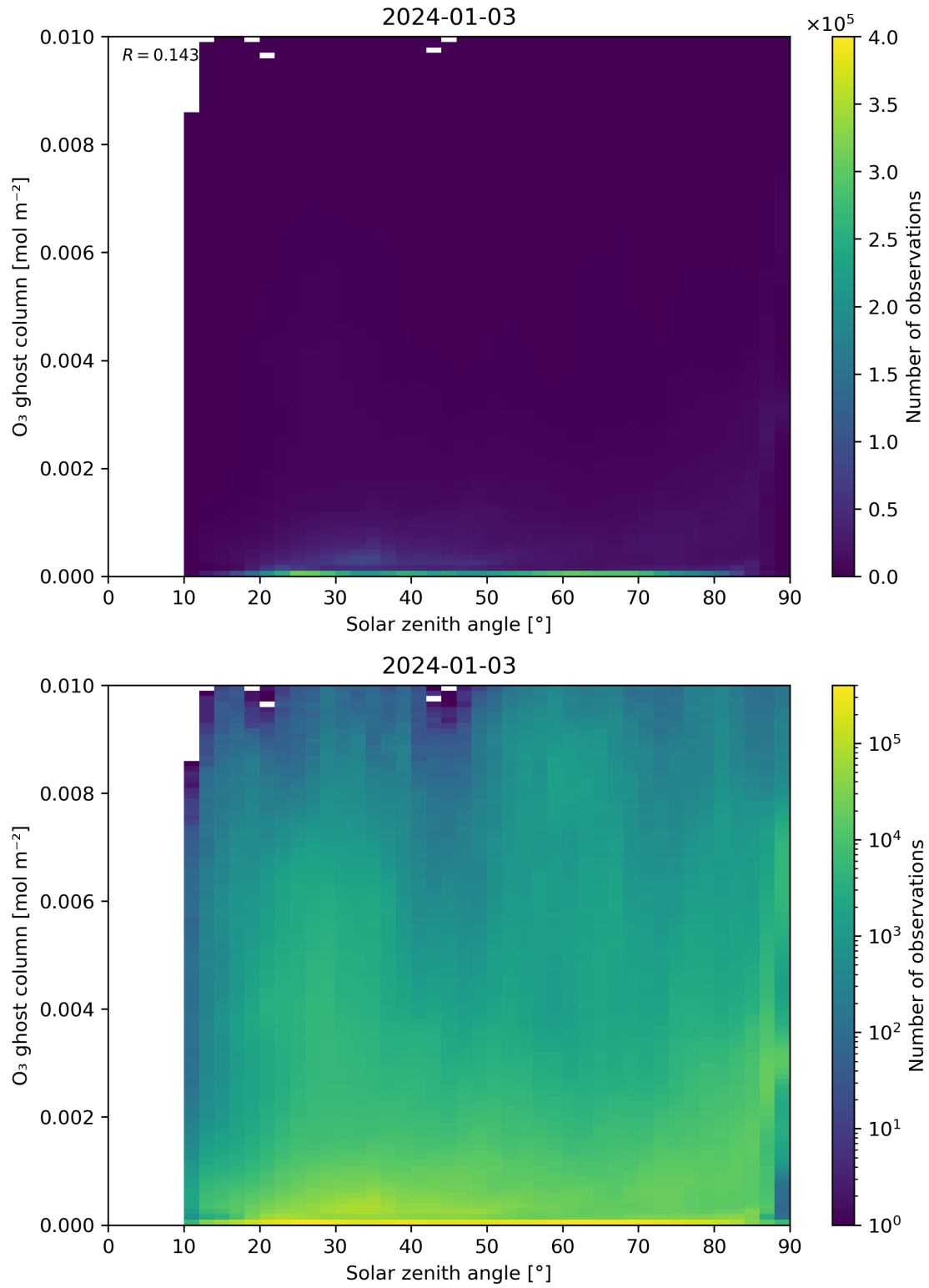
Figure 46: Scatter density plot of “Solar zenith angle” against “O 3 ghost column” for 2024-01-02 to 2024-01-04.
