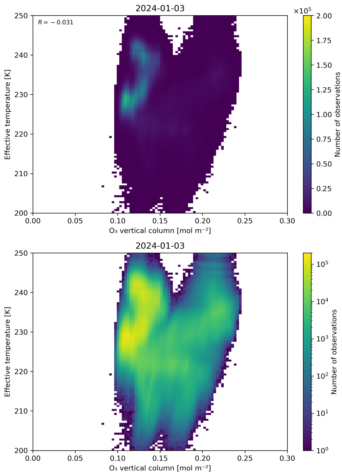
Figure 39: Scatter density plot of “O 3 vertical column” against “Effective temperature” for 2024-01-02 to 2024-01-04.
