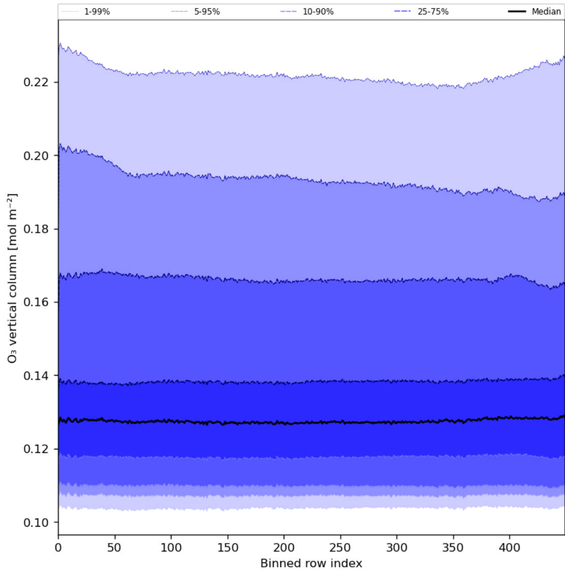
Figure 28: Along track statistics of “O 3 vertical column” for 2024-01-02 to 2024-01-04
