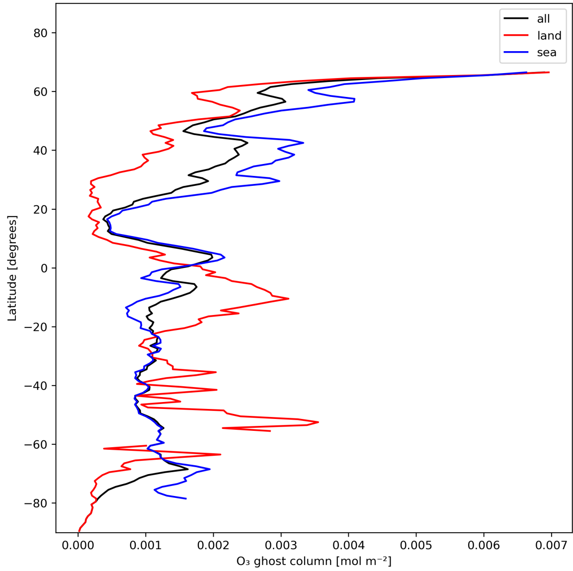
Figure 18: Zonal average of “O 3 ghost column” for 2024-01-02 to 2024-01-04.
