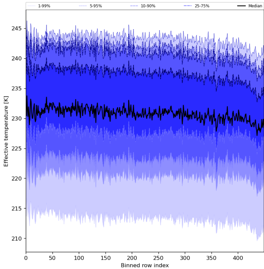
Figure 31: Along track statistics of “Effective temperature” for 2024-01-02 to 2024-01-04
