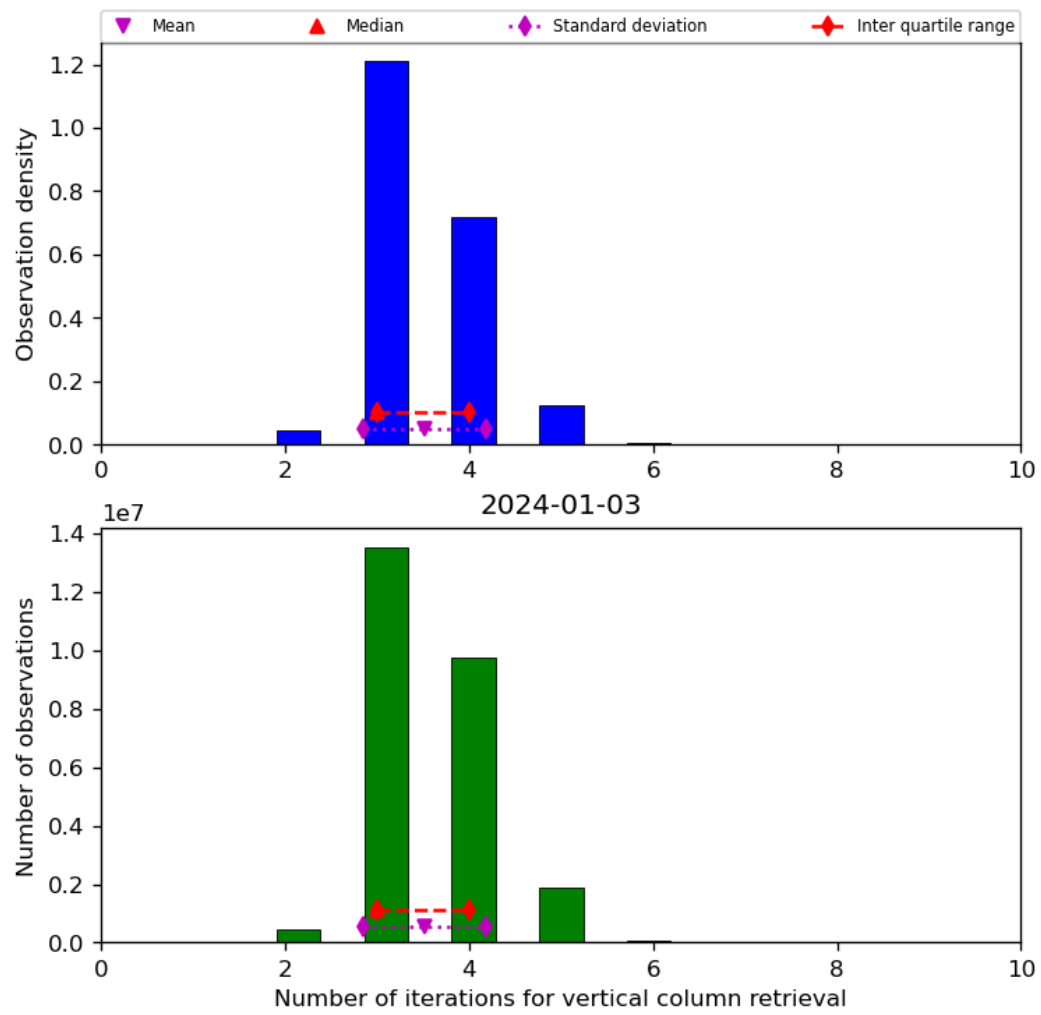
Figure 26: Histogram of “Number of iterations for vertical column retrieval” for 2024-01-02 to 2024-01-04
