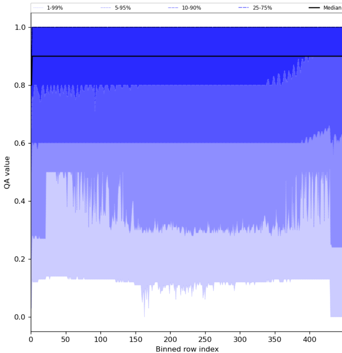
Figure 27: Along track statistics of “QA value” for 2024-01-02 to 2024-01-04
