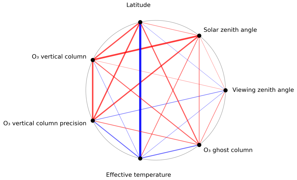
Figure 1: Map of correlation graph for 2024-01-02 to 2024-01-04.
