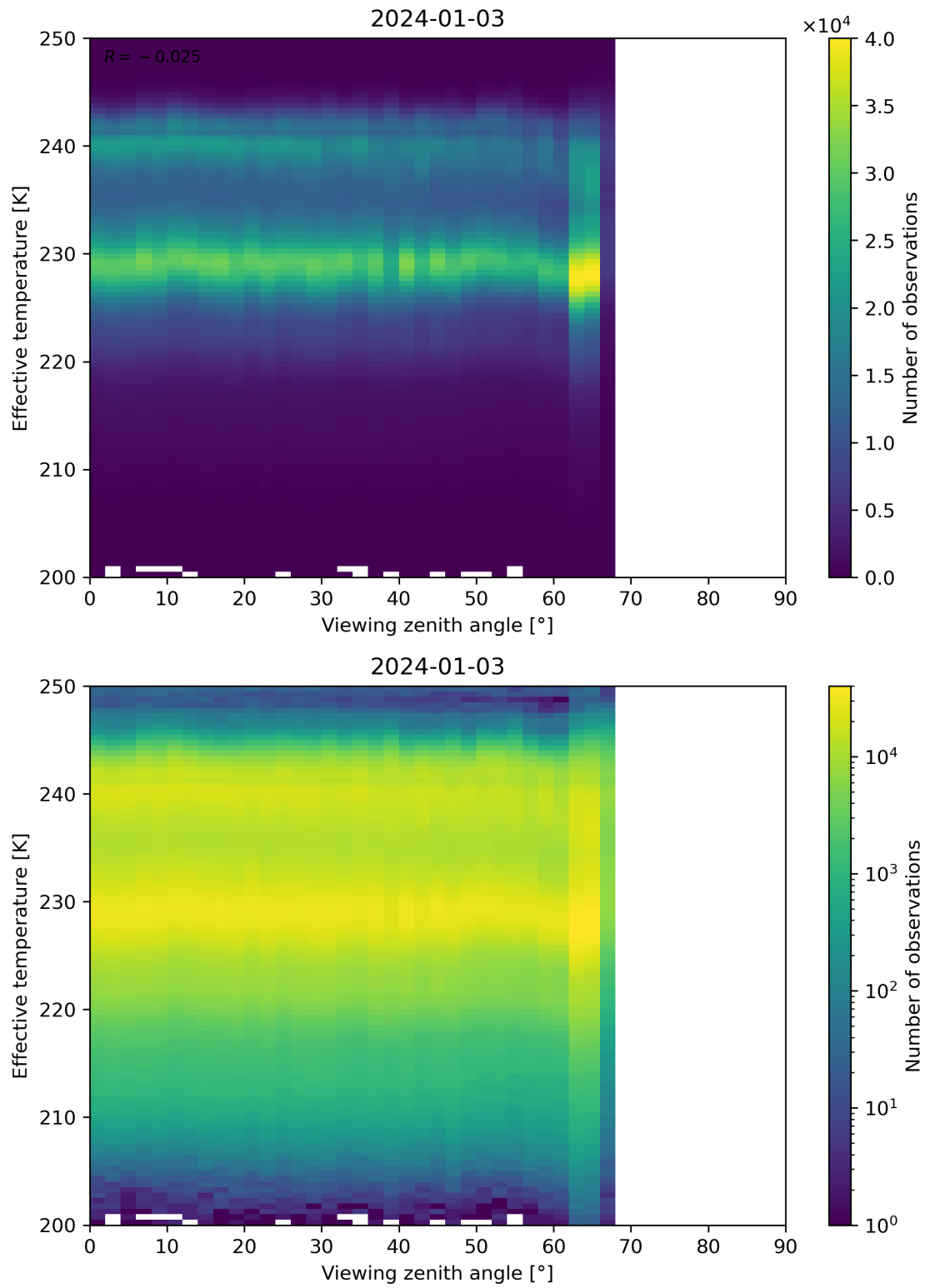
Figure 50: Scatter density plot of “Viewing zenith angle” against “Effective temperature” for 2024-01-02 to 2024-01-04.
