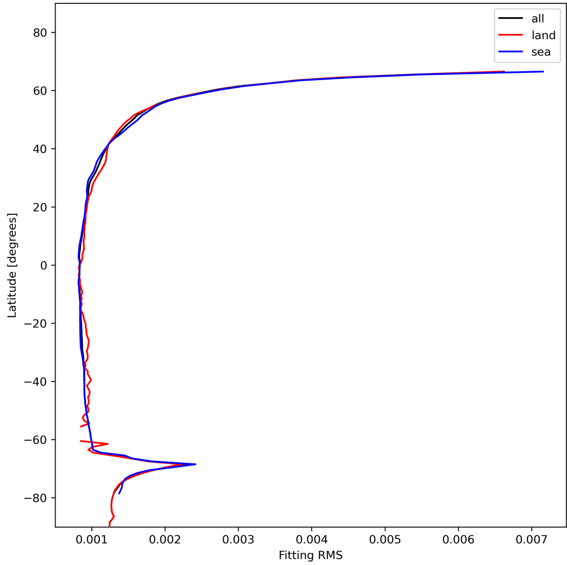
Figure 16: Zonal average of “Fitting RMS” for 2024-01-02 to 2024-01-04.
