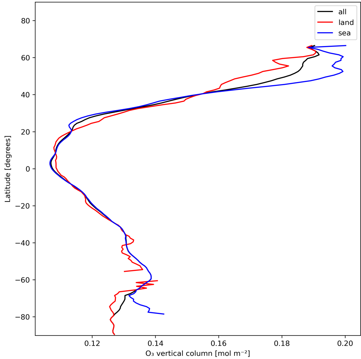
Figure 14: Zonal average of “O 3 vertical column” for 2024-01-02 to 2024-01-04.
