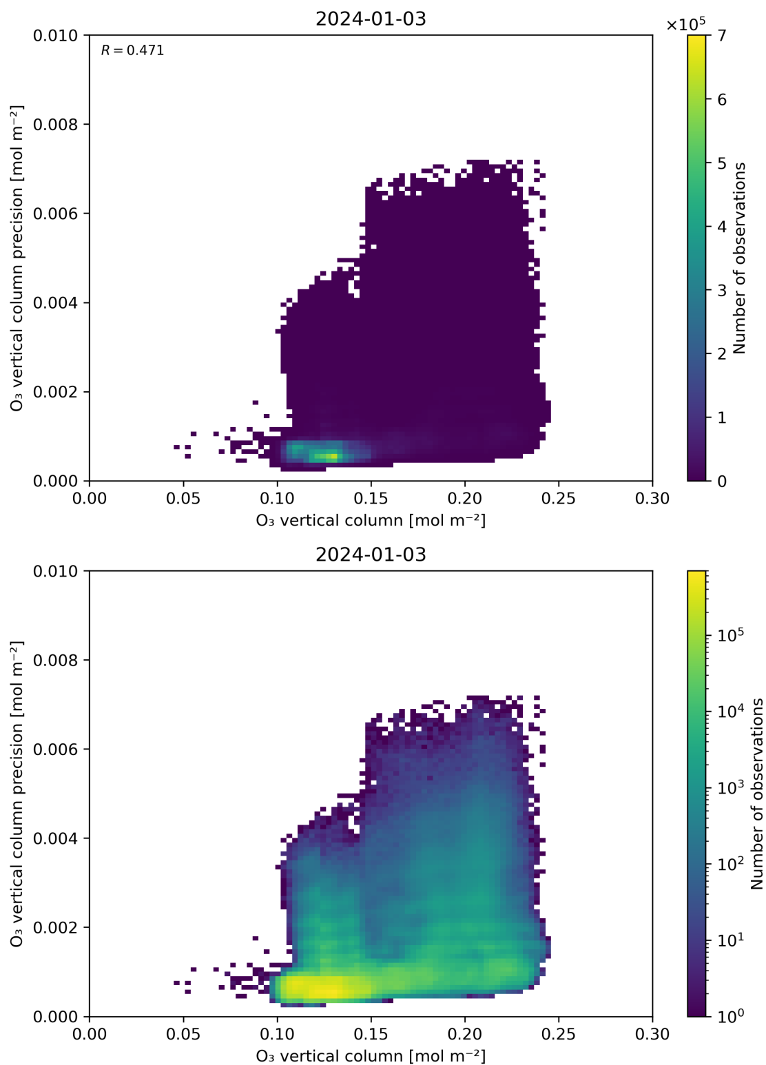
Figure 41: Scatter density plot of “O 3 vertical column” against “O 3 vertical column precision” for 2024-01-02 to 2024-01-04.
