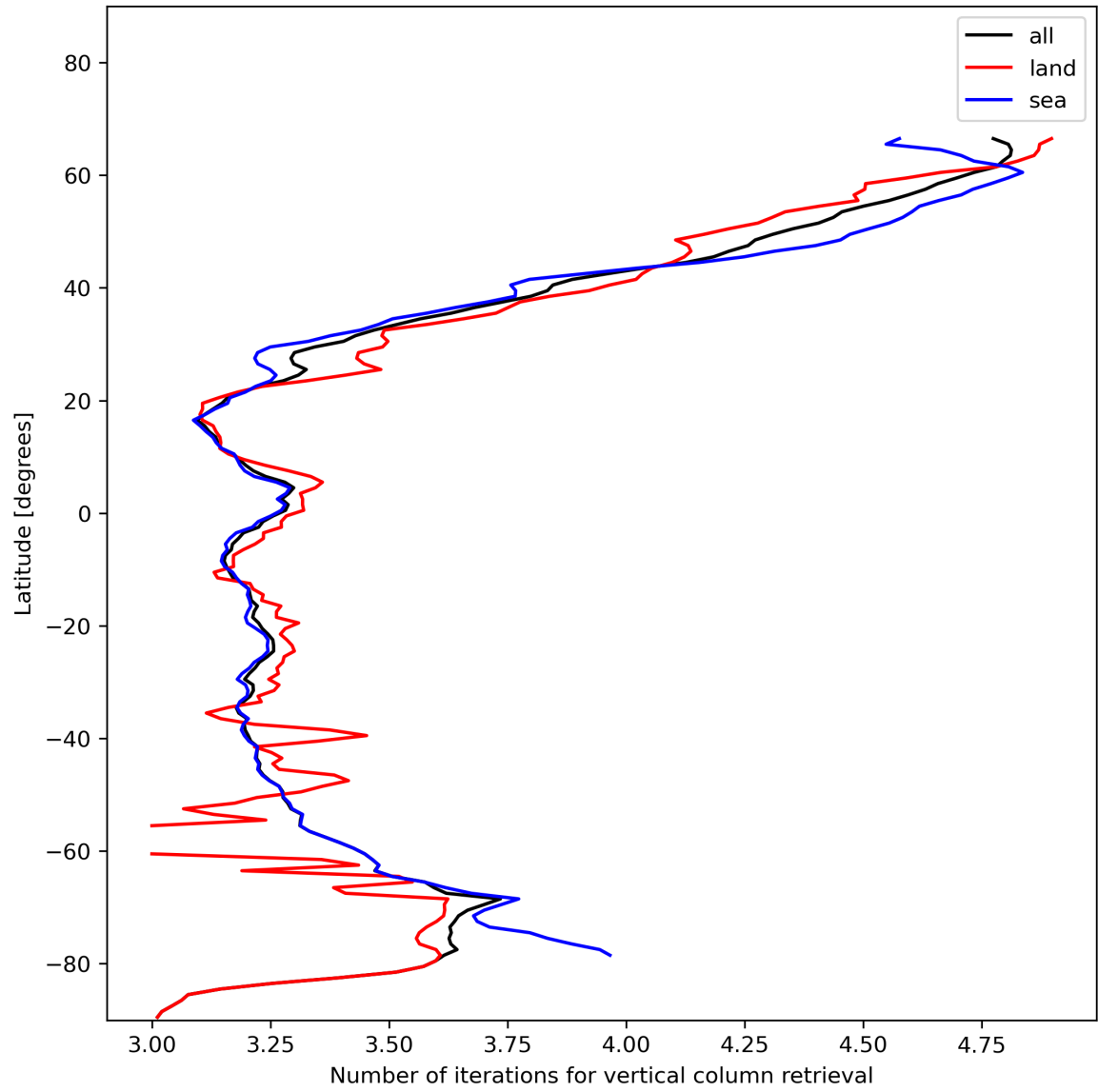
Figure 19: Zonal average of “Number of iterations for vertical column retrieval” for 2024-01-02 to 2024-01-04.
