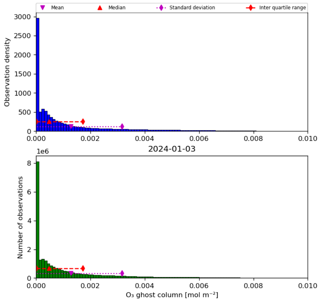
Figure 25: Histogram of “O 3 ghost column” for 2024-01-02 to 2024-01-04
