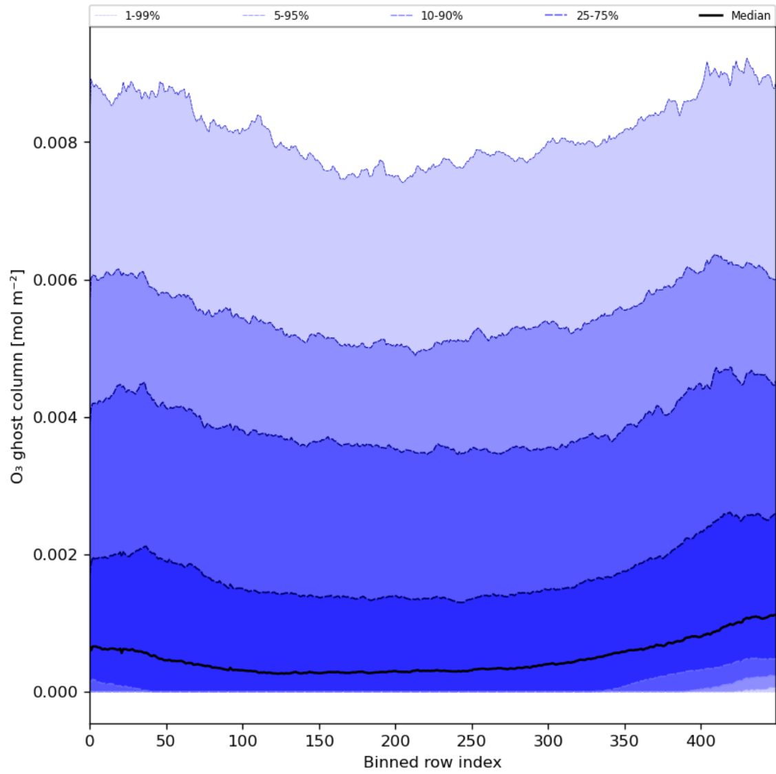
Figure 32: Along track statistics of “O 3 ghost column” for 2024-01-02 to 2024-01-04
