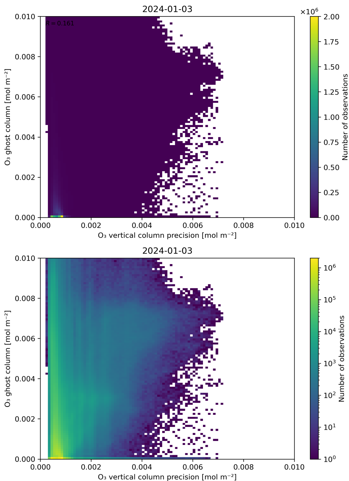
Figure 43: Scatter density plot of “ \text{O}_3 vertical column precision” against “ \text{O}_3 ghost column” for 2024-01-02 to 2024-01-04.
