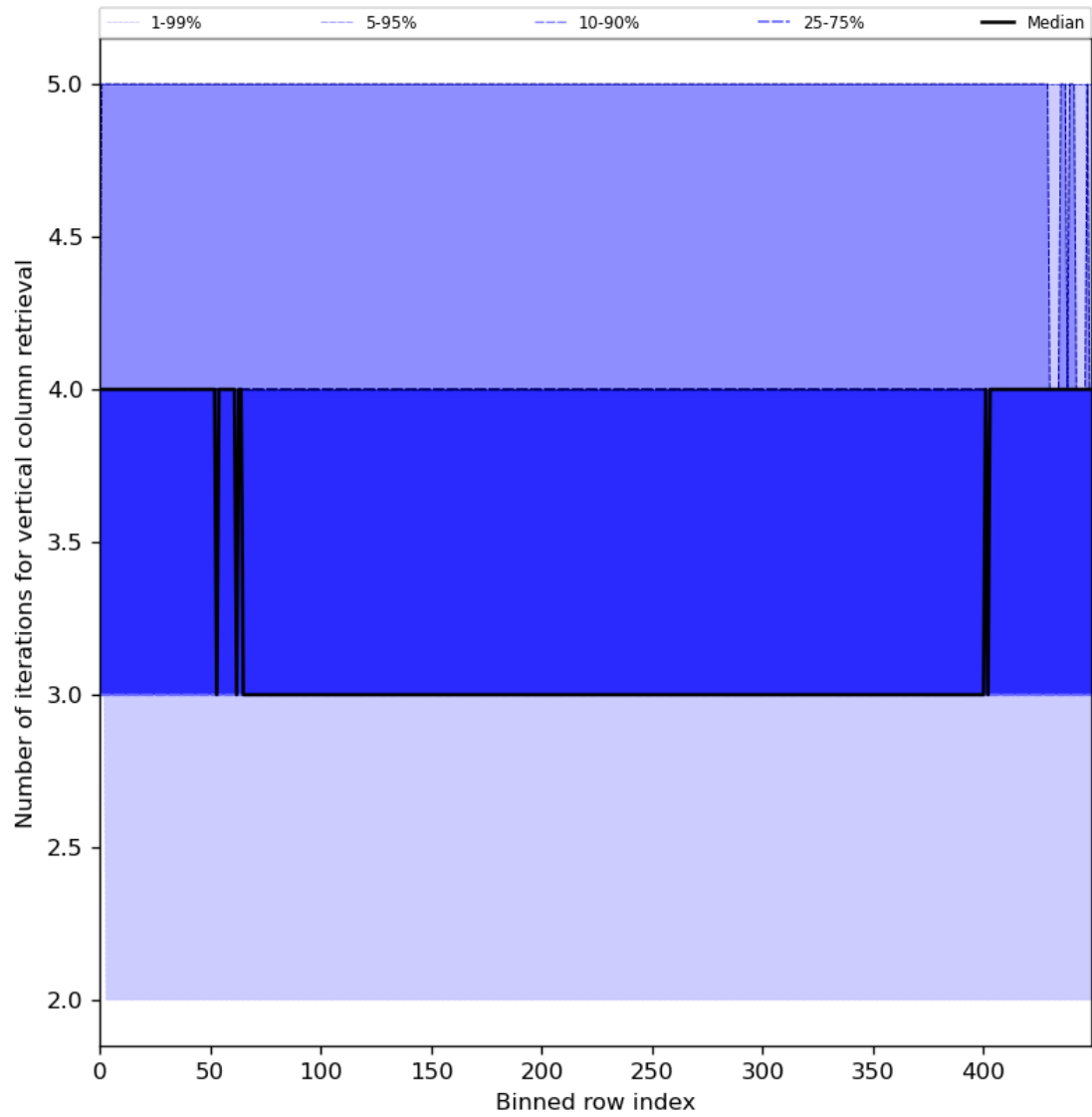
Figure 33: Along track statistics of “Number of iterations for vertical column retrieval” for 2024-01-02 to 2024-01-04
