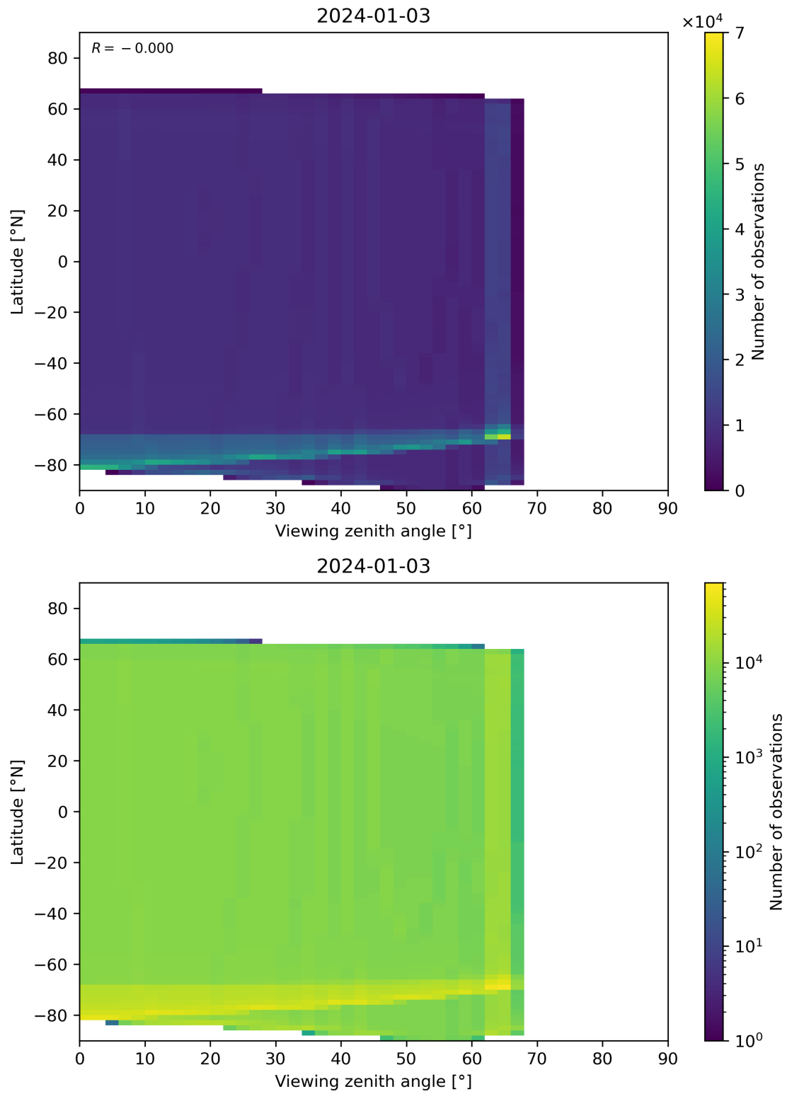
Figure 49: Scatter density plot of “Viewing zenith angle” against “Latitude” for 2024-01-02 to 2024-01-04.
