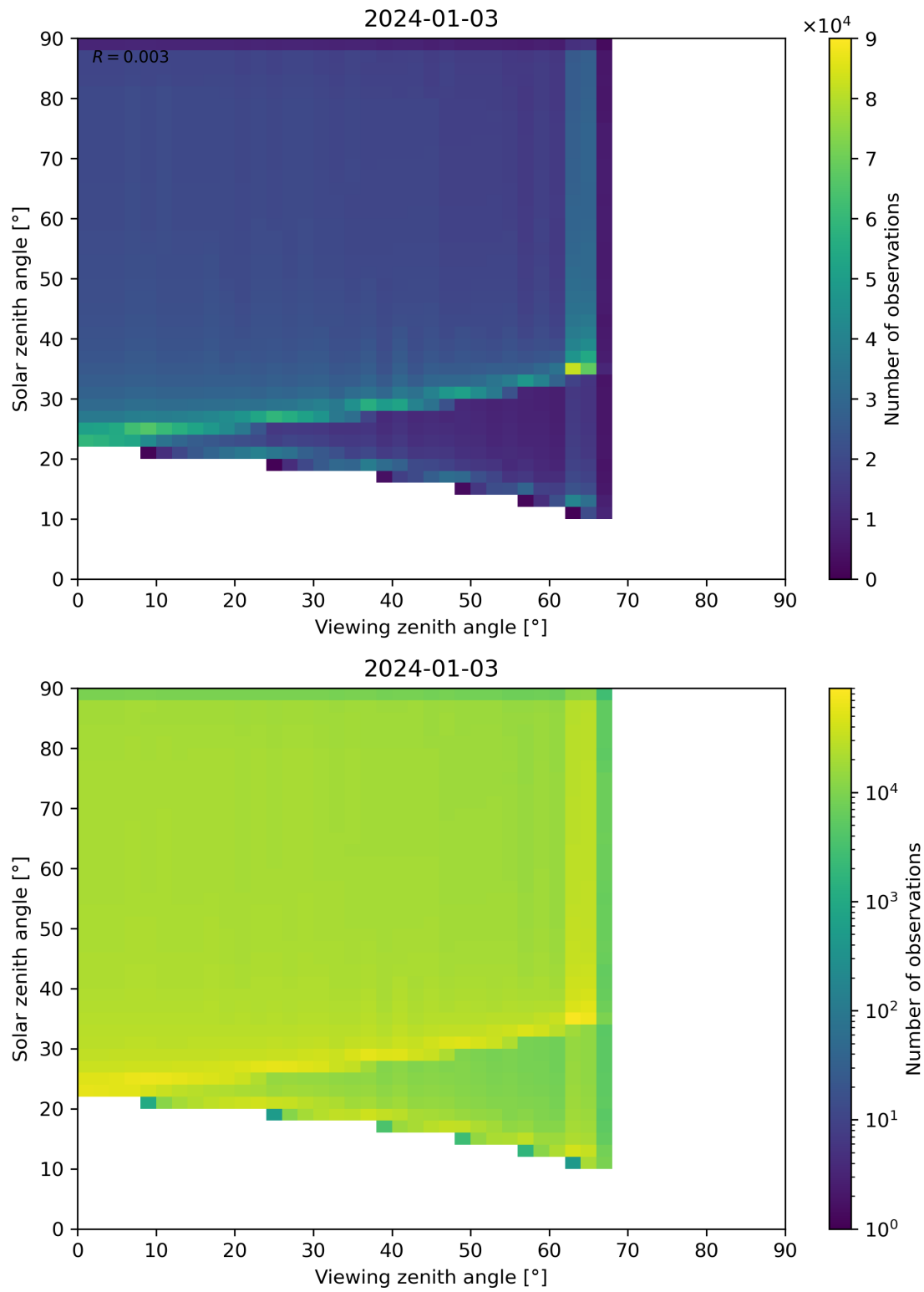
Figure 54: Scatter density plot of “Viewing zenith angle” against “Solar zenith angle” for 2024-01-02 to 2024-01-04.
