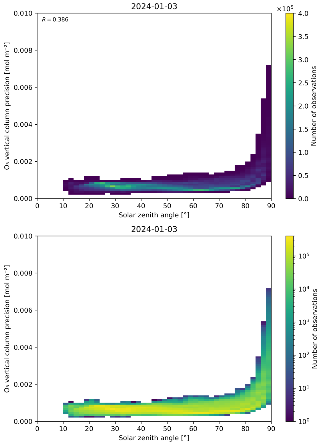
Figure 48: Scatter density plot of “Solar zenith angle” against “O 3 vertical column precision” for 2024-01-02 to 2024-01-04.
