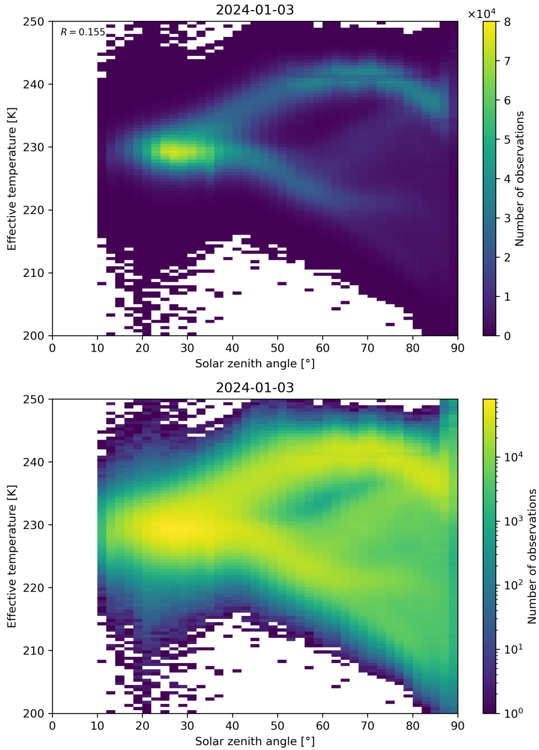
Figure 45: Scatter density plot of “Solar zenith angle” against “Effective temperature” for 2024-01-02 to 2024-01-04.
