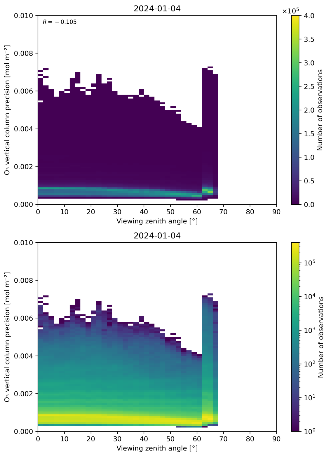
Figure 53: Scatter density plot of “Viewing zenith angle” against “O 3 vertical column precision” for 2024-01-03 to 2024-01-05.
