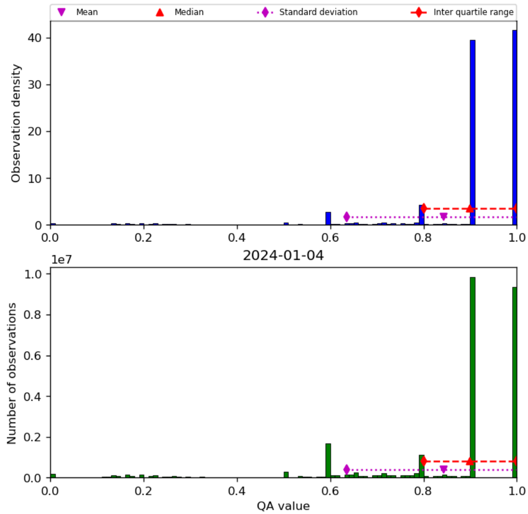
Figure 20: Histogram of “QA value” for 2024-01-03 to 2024-01-05
