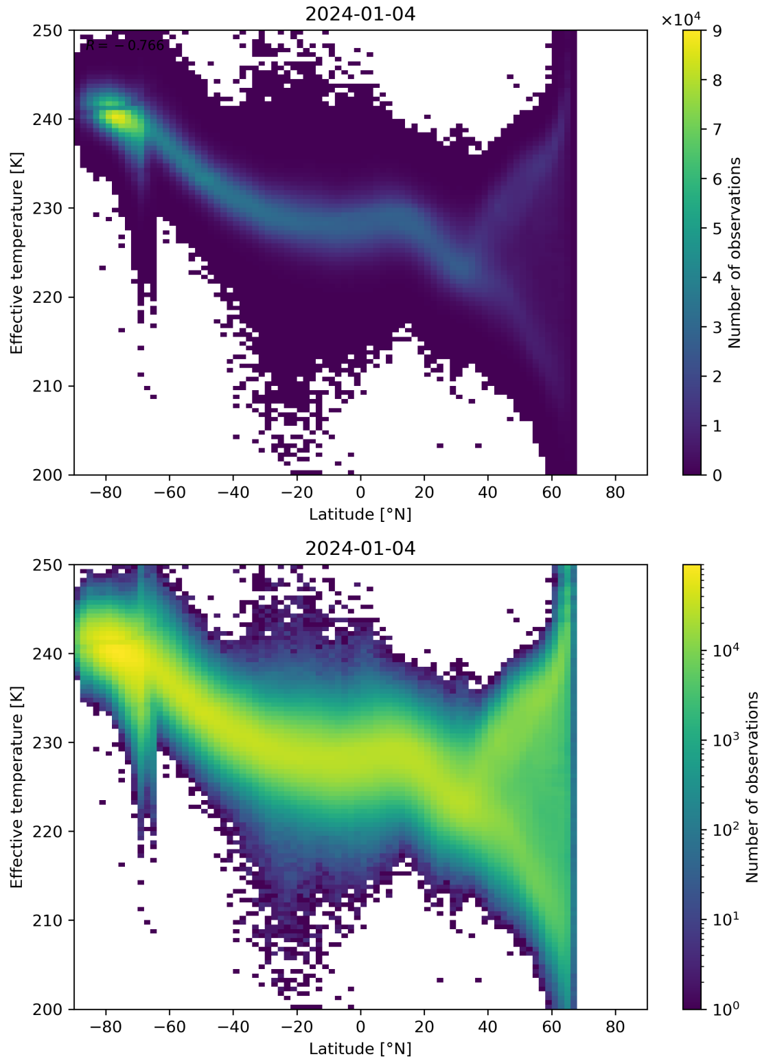
Figure 34: Scatter density plot of “Latitude” against “Effective temperature” for 2024-01-03 to 2024-01-05.
