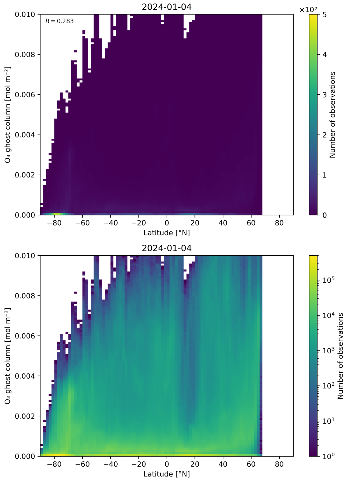
Figure 35: Scatter density plot of “Latitude” against “O 3 ghost column” for 2024-01-03 to 2024-01-05.
