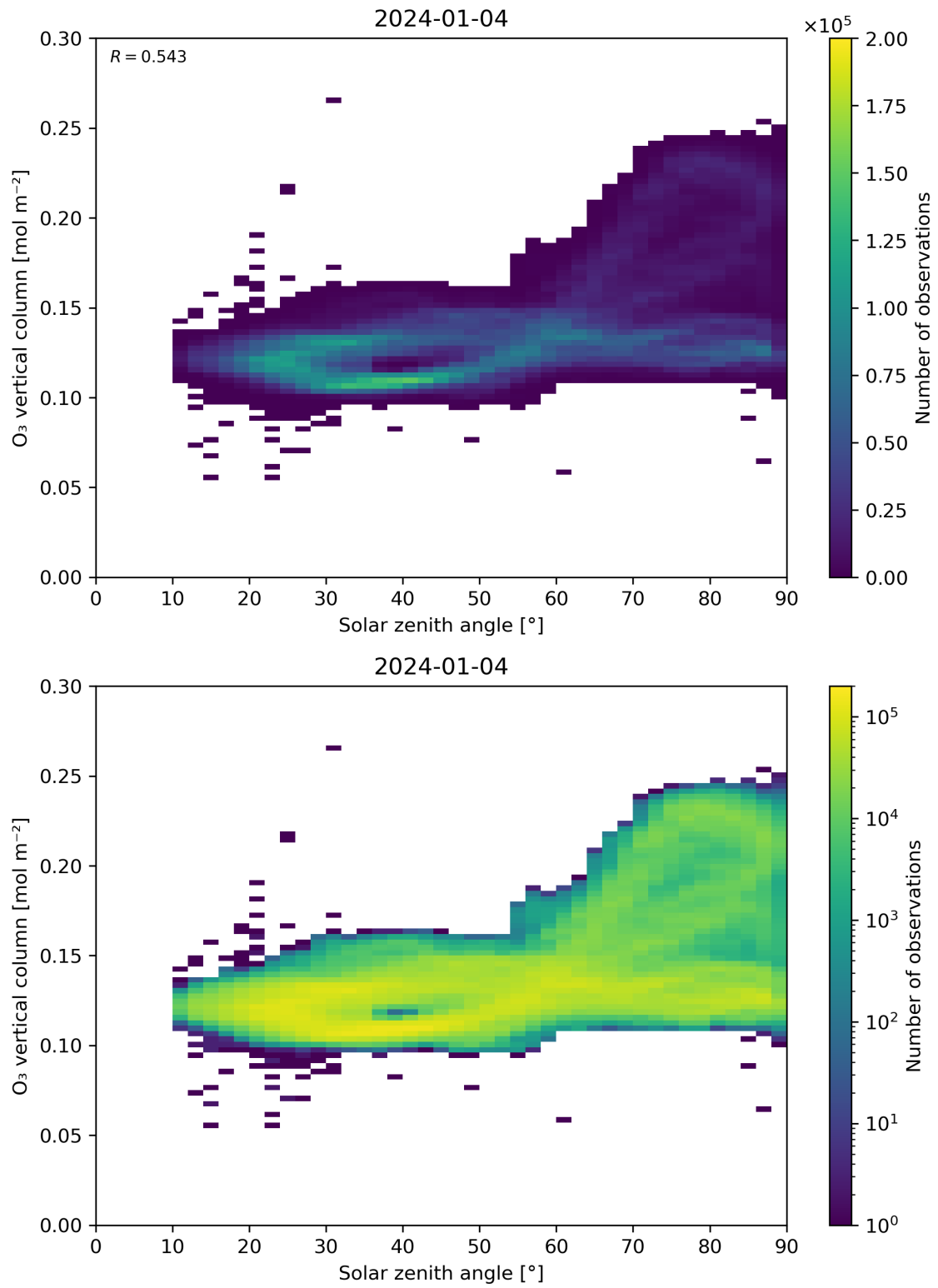
Figure 47: Scatter density plot of “Solar zenith angle” against “O 3 vertical column” for 2024-01-03 to 2024-01-05.
