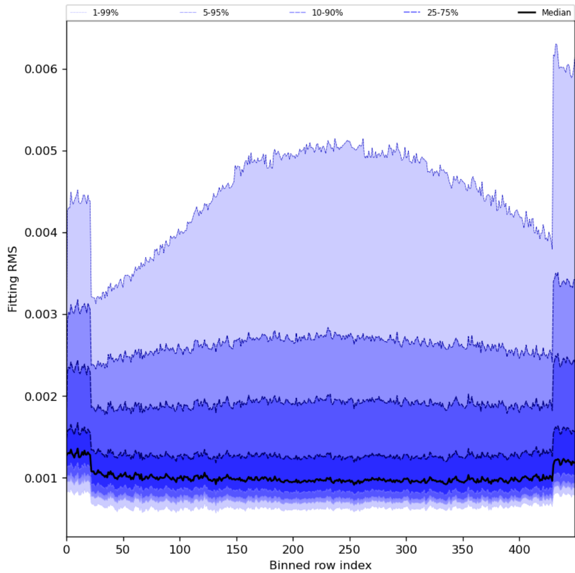
Figure 30: Along track statistics of “Fitting RMS” for 2024-01-03 to 2024-01-05
