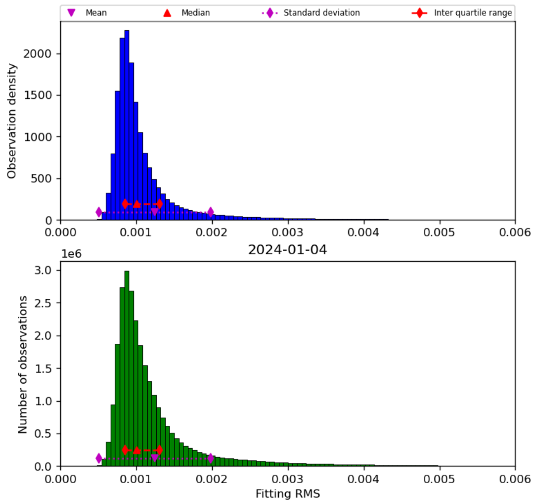
Figure 23: Histogram of “Fitting RMS” for 2024-01-03 to 2024-01-05
