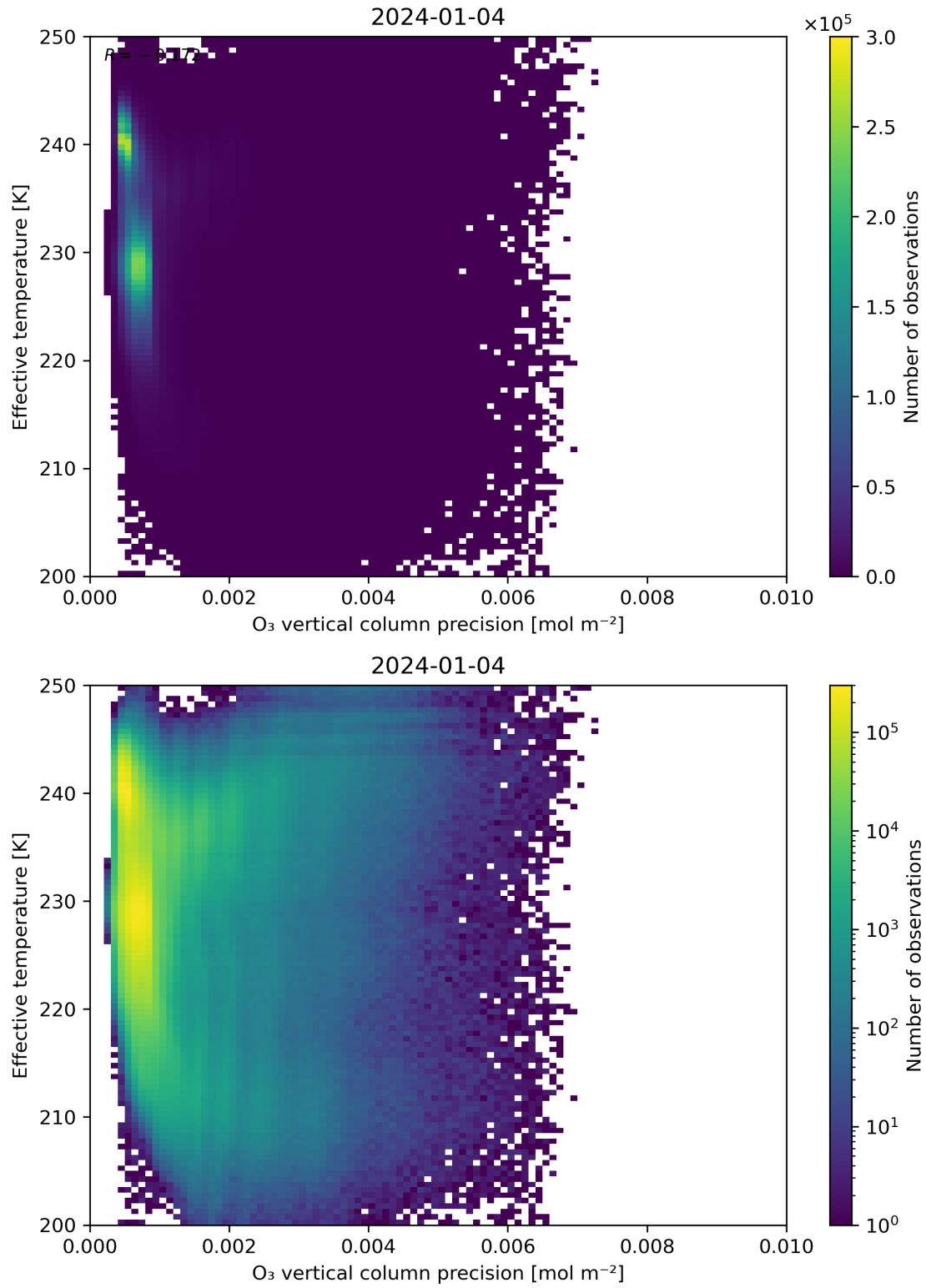
Figure 42: Scatter density plot of “O 3 vertical column precision” against “Effective temperature” for 2024-01-03 to 2024-01-05.
