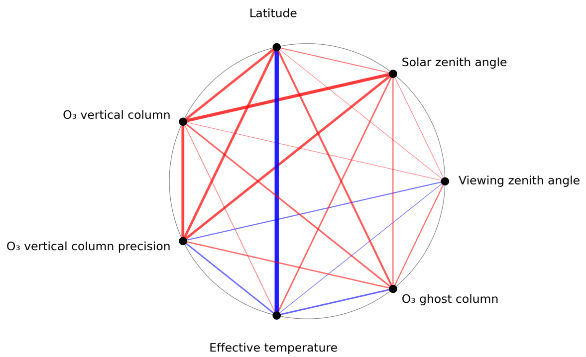
Figure 1: Map of correlation graph for 2024-01-03 to 2024-01-05.
