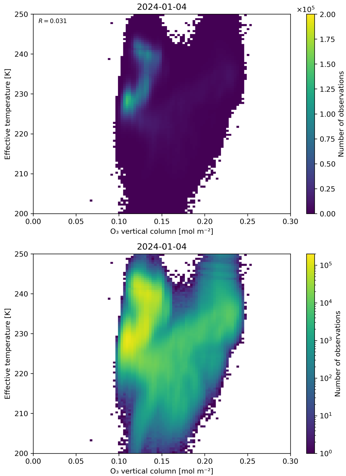
Figure 39: Scatter density plot of “O 3 vertical column” against “Effective temperature” for 2024-01-03 to 2024-01-05.
