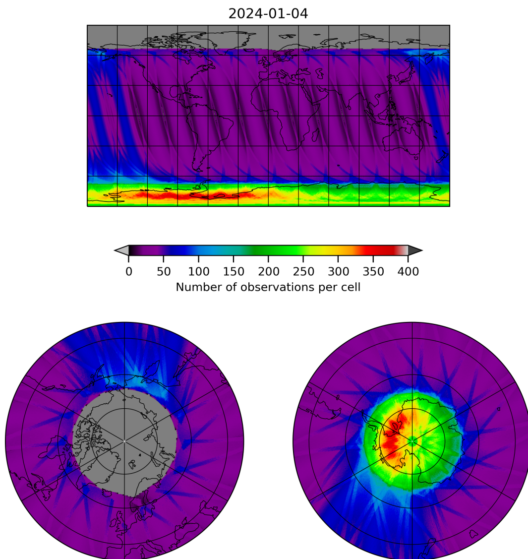
Figure 12: Map of the number of observations for 2024-01-03 to 2024-01-05
