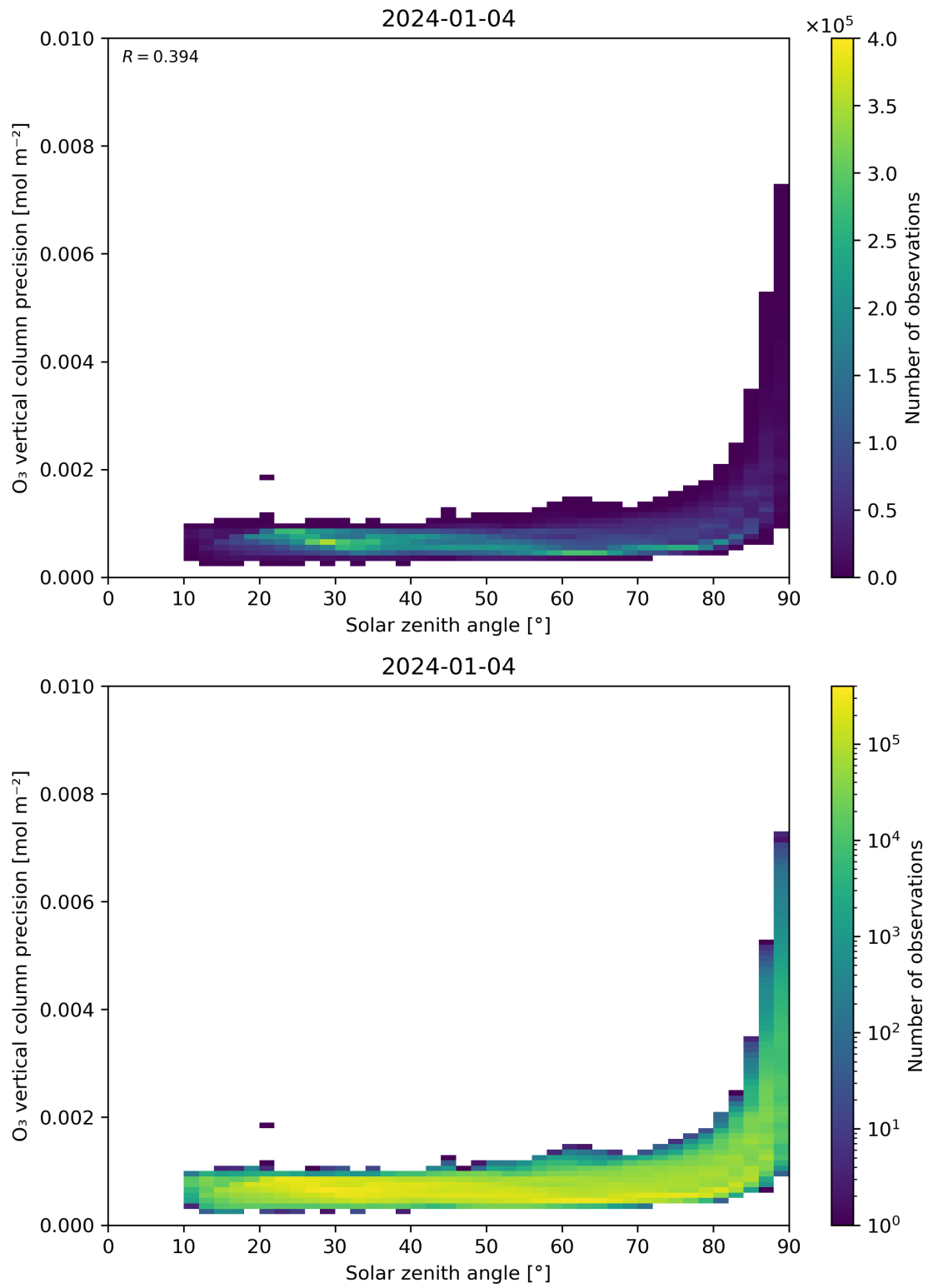
Figure 48: Scatter density plot of “Solar zenith angle” against “O 3 vertical column precision” for 2024-01-03 to 2024-01-05.
