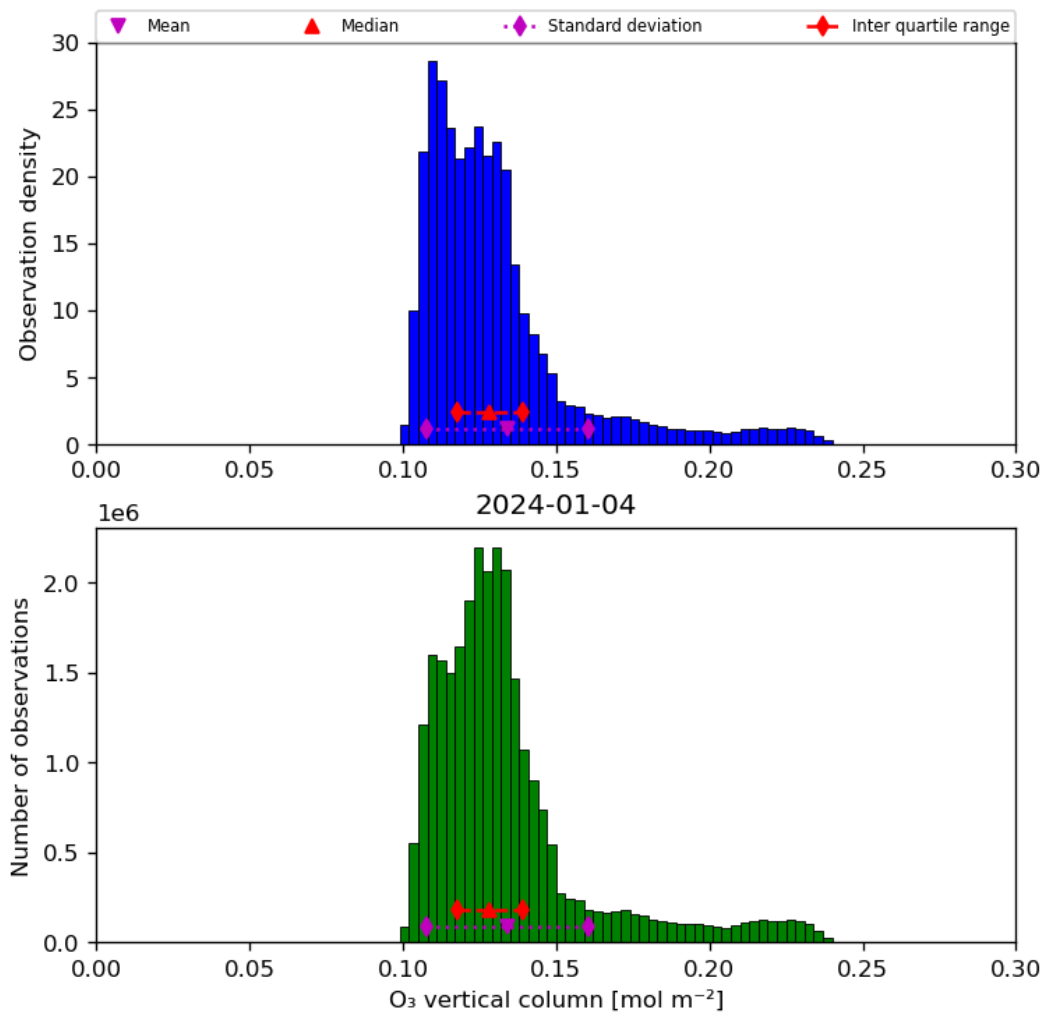
Figure 21: Histogram of “O 3 vertical column” for 2024-01-03 to 2024-01-05
