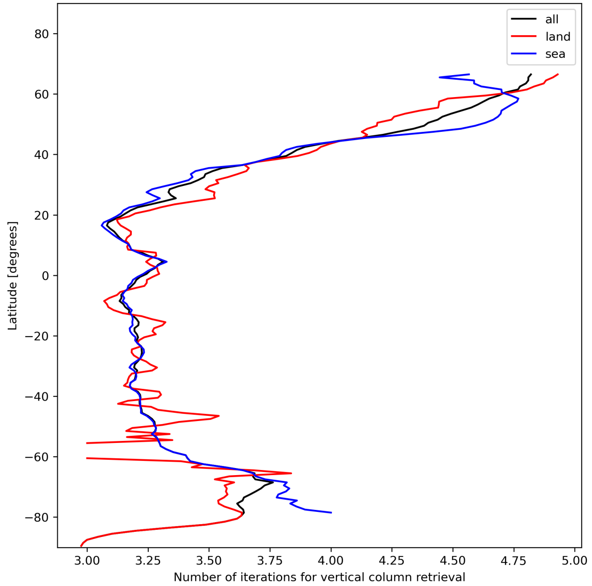
Figure 19: Zonal average of “Number of iterations for vertical column retrieval” for 2024-01-03 to 2024-01-05.
