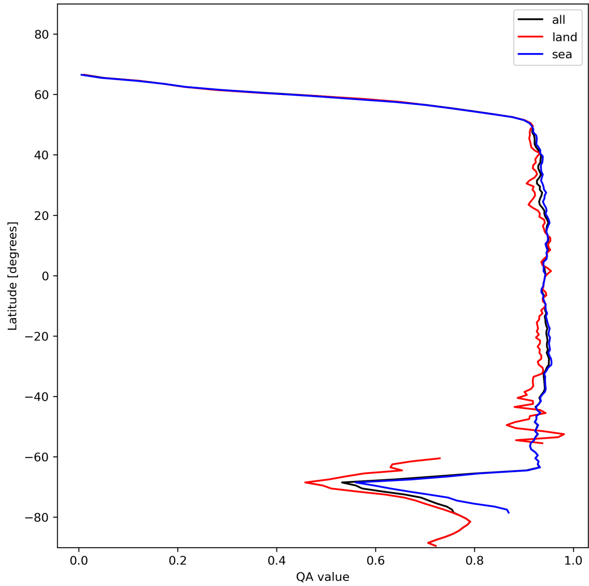
Figure 13: Zonal average of “QA value” for 2024-01-03 to 2024-01-05.
