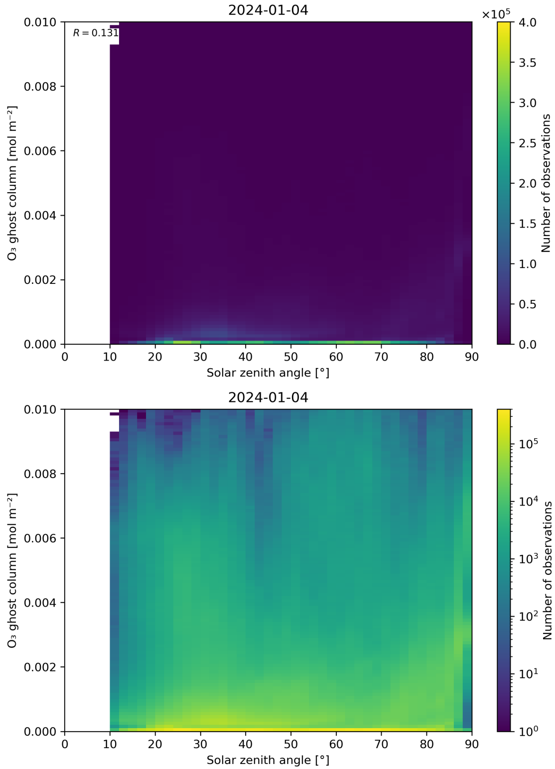
Figure 46: Scatter density plot of “Solar zenith angle” against “O 3 ghost column” for 2024-01-03 to 2024-01-05.
