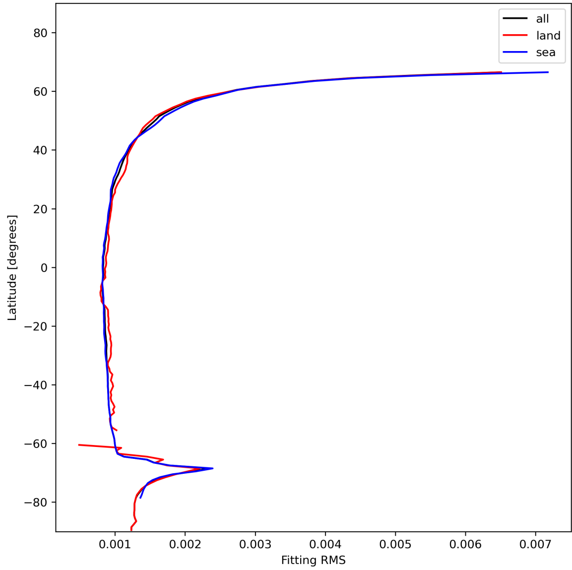
Figure 16: Zonal average of “Fitting RMS” for 2024-01-03 to 2024-01-05.
