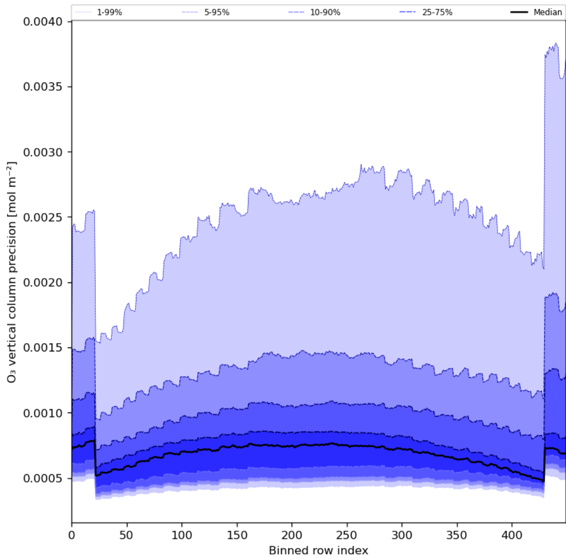
Figure 29: Along track statistics of “O 3 vertical column precision” for 2024-01-03 to 2024-01-05
