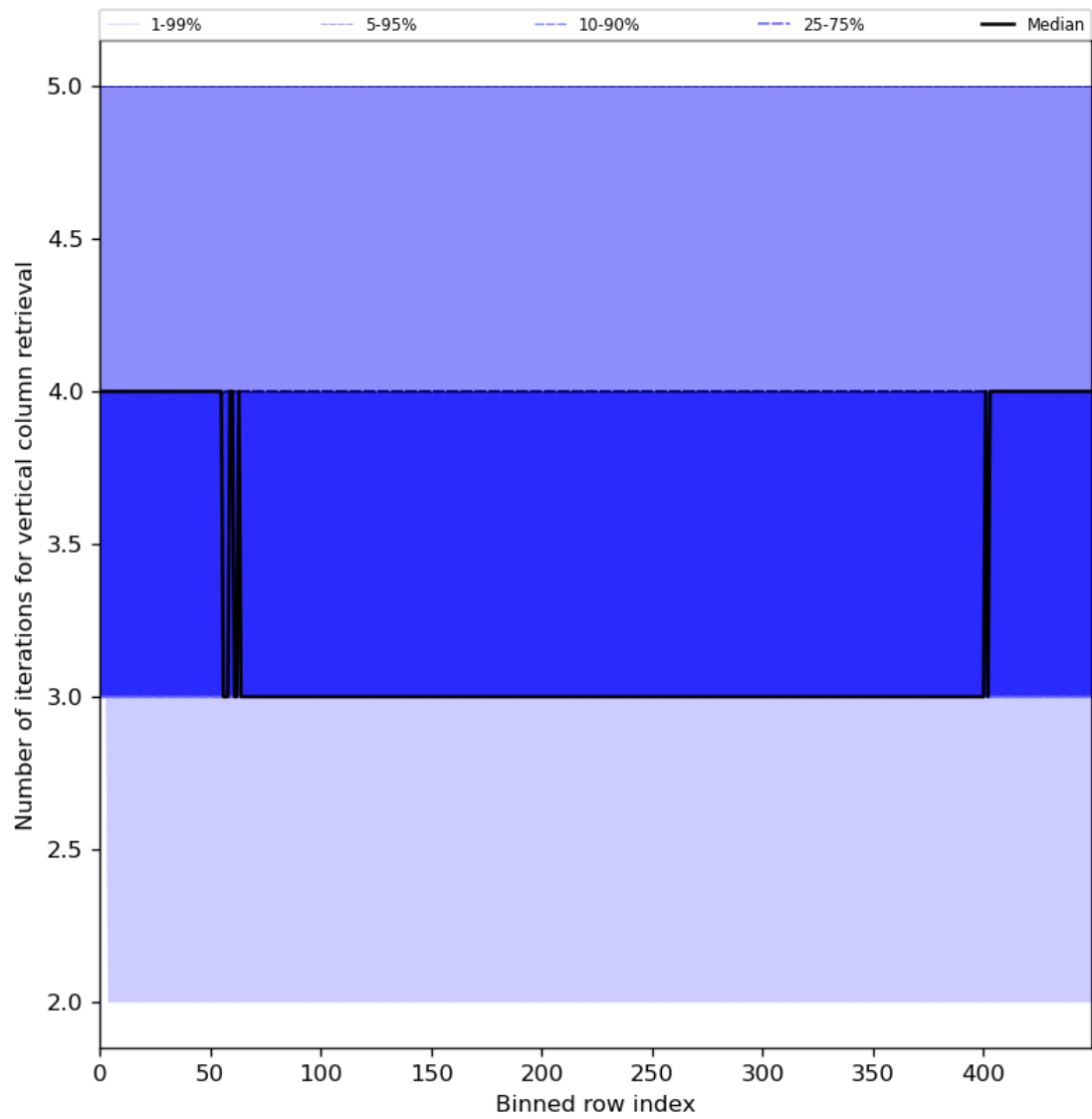
Figure 33: Along track statistics of “Number of iterations for vertical column retrieval” for 2024-01-03 to 2024-01-05
