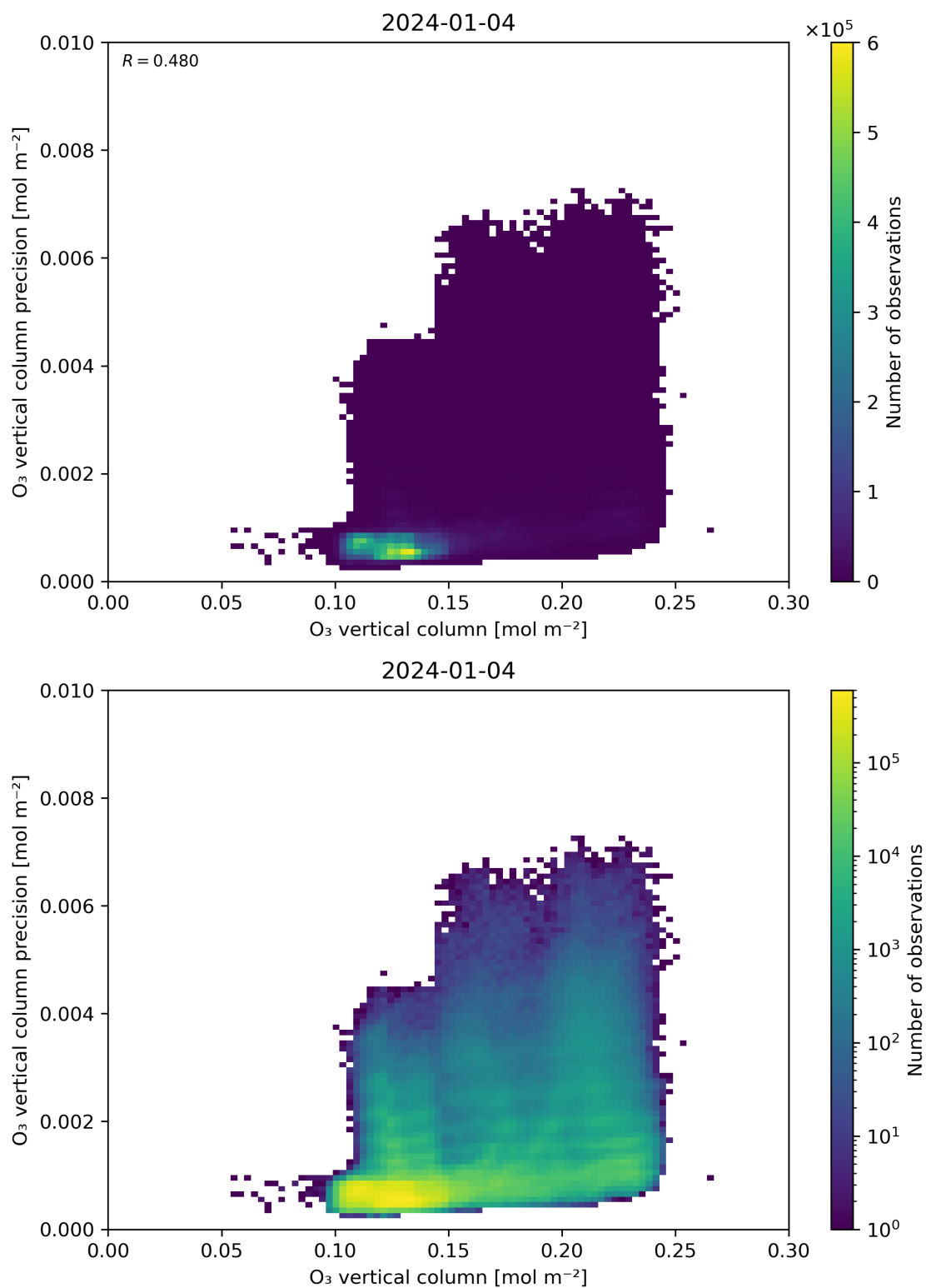
Figure 41: Scatter density plot of “O 3 vertical column” against “O 3 vertical column precision” for 2024-01-03 to 2024-01-05.
