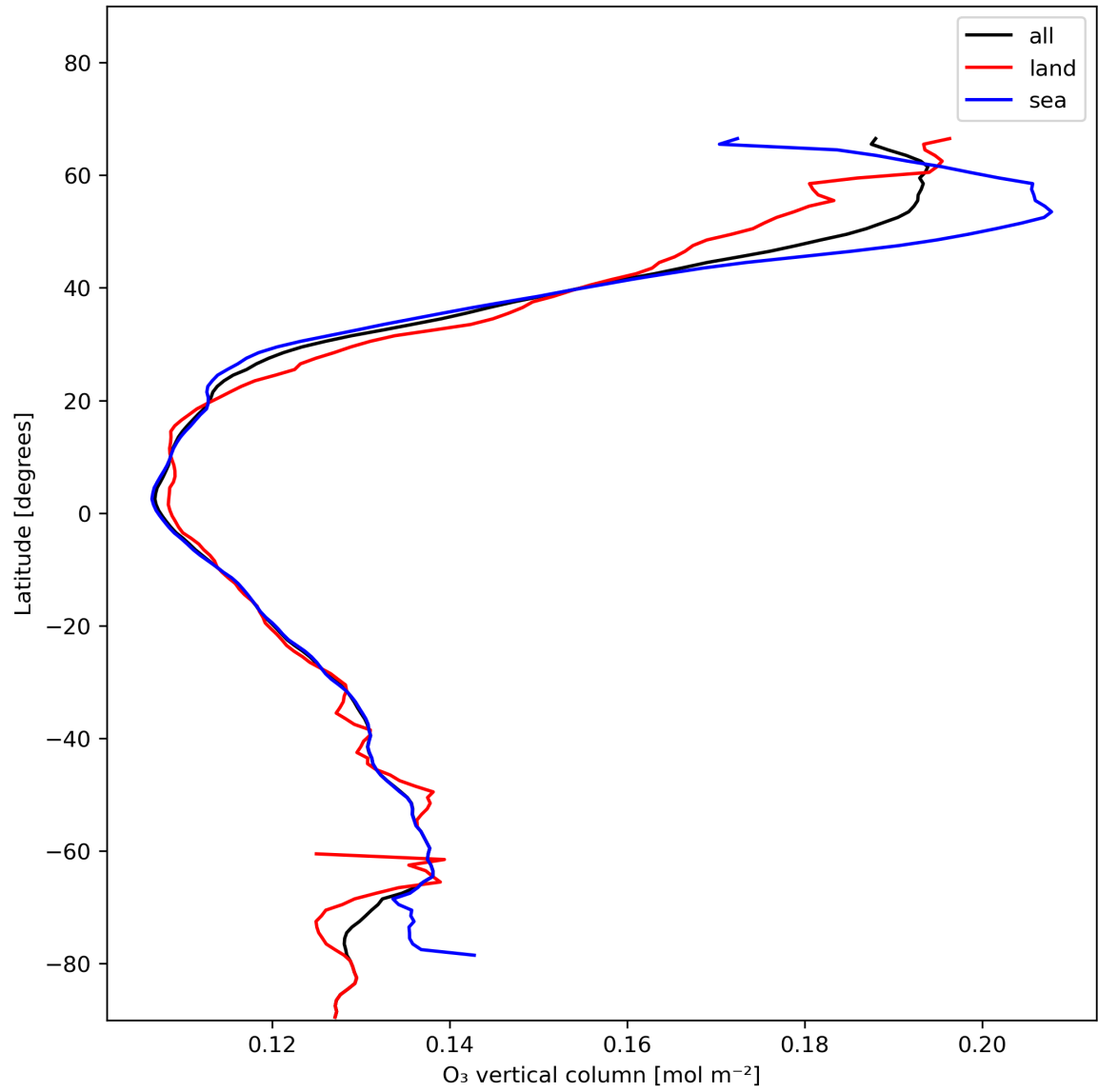
Figure 14: Zonal average of “O 3 vertical column” for 2024-01-03 to 2024-01-05.
