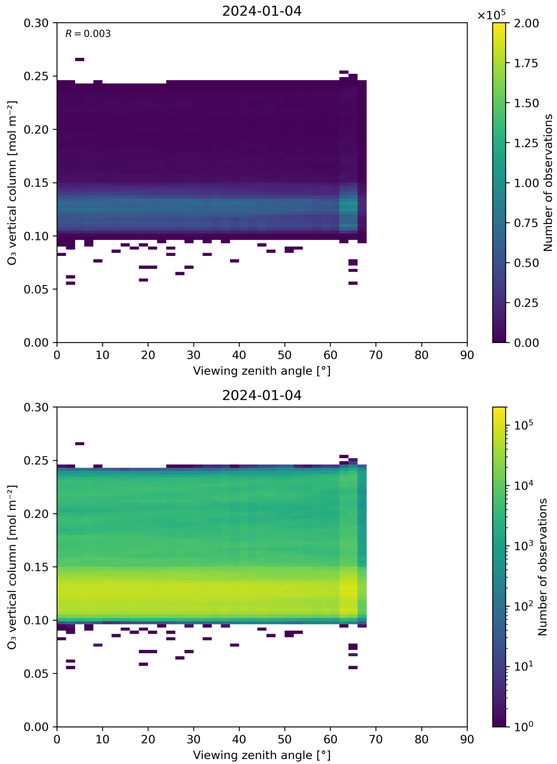
Figure 52: Scatter density plot of “Viewing zenith angle” against “O 3 vertical column” for 2024-01-03 to 2024-01-05.
