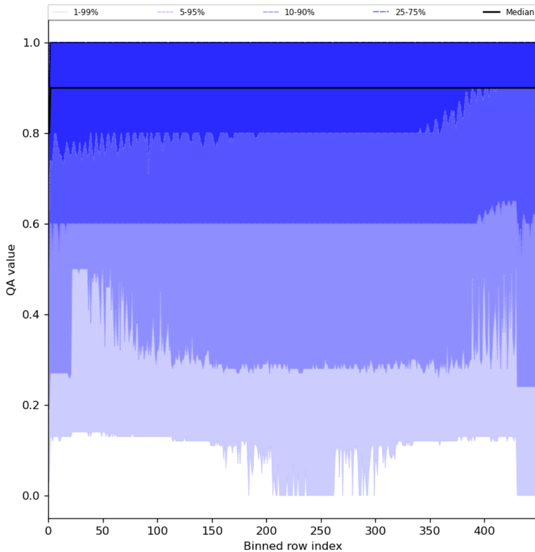
Figure 27: Along track statistics of “QA value” for 2024-01-03 to 2024-01-05
