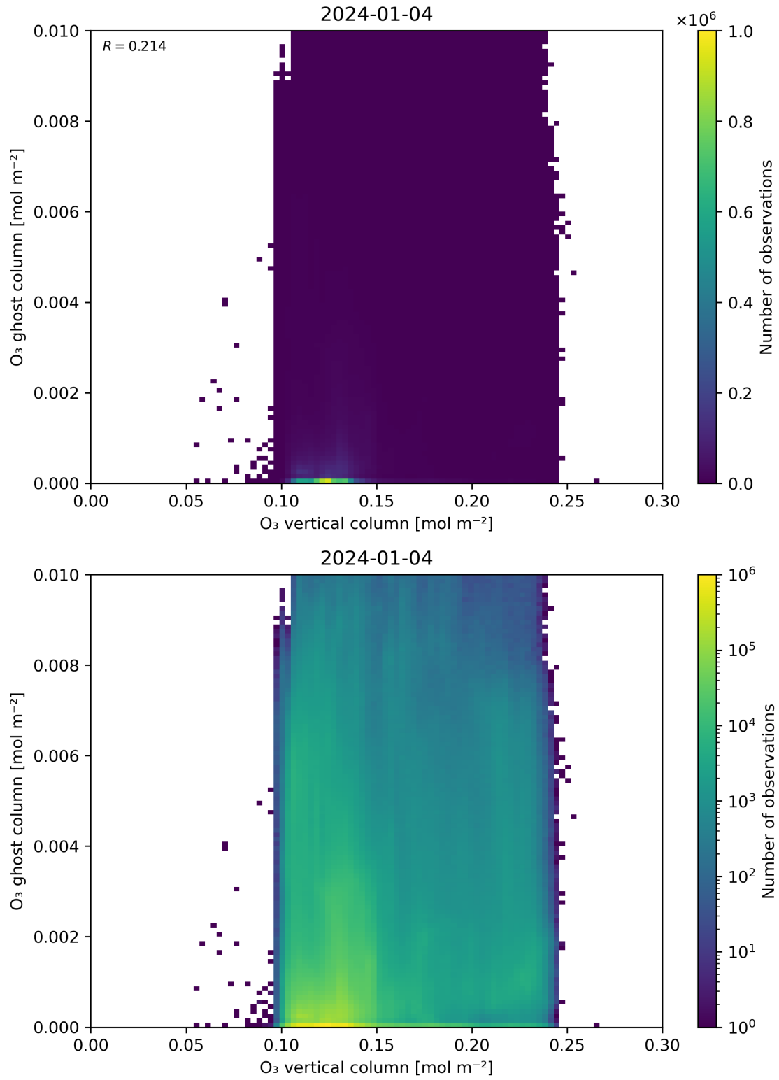
Figure 40: Scatter density plot of “O 3 vertical column” against “O 3 ghost column” for 2024-01-03 to 2024-01-05.
