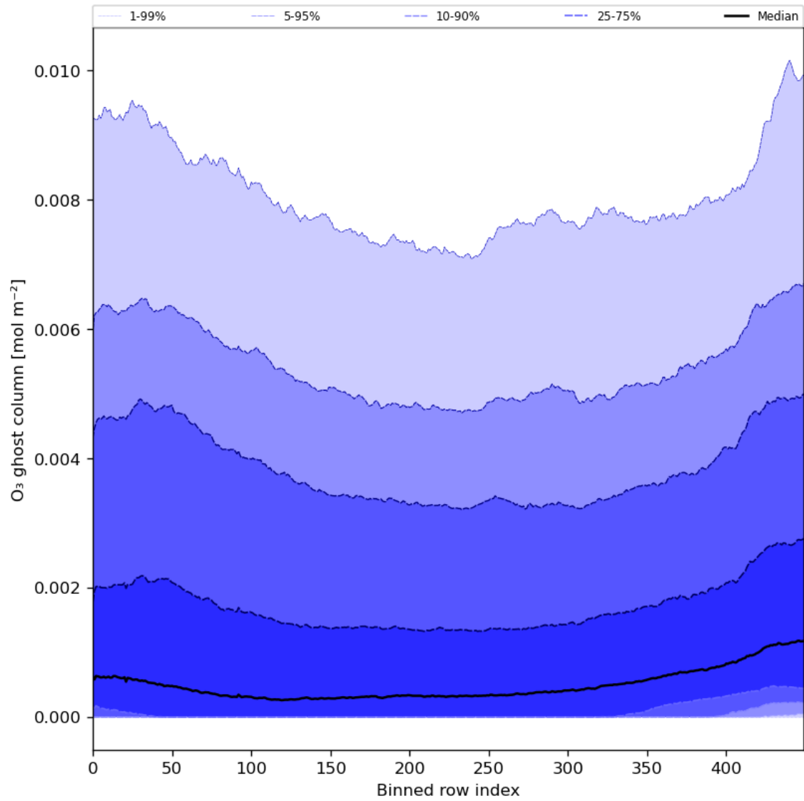
Figure 32: Along track statistics of “O 3 ghost column” for 2024-01-03 to 2024-01-05
