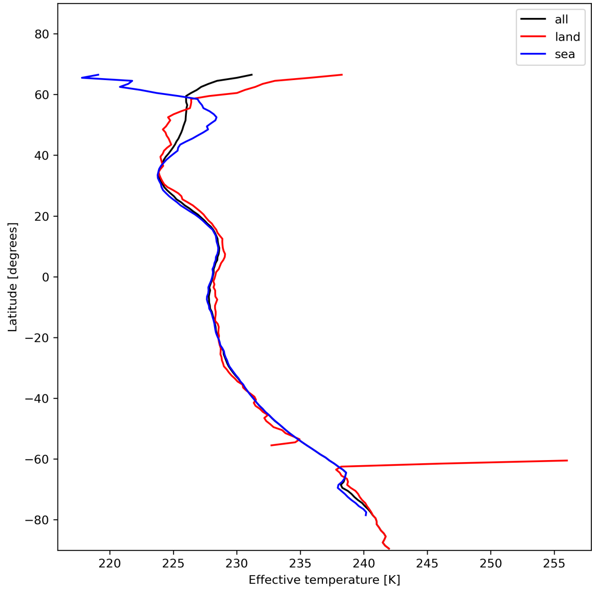
Figure 17: Zonal average of “Effective temperature” for 2024-01-03 to 2024-01-05.
