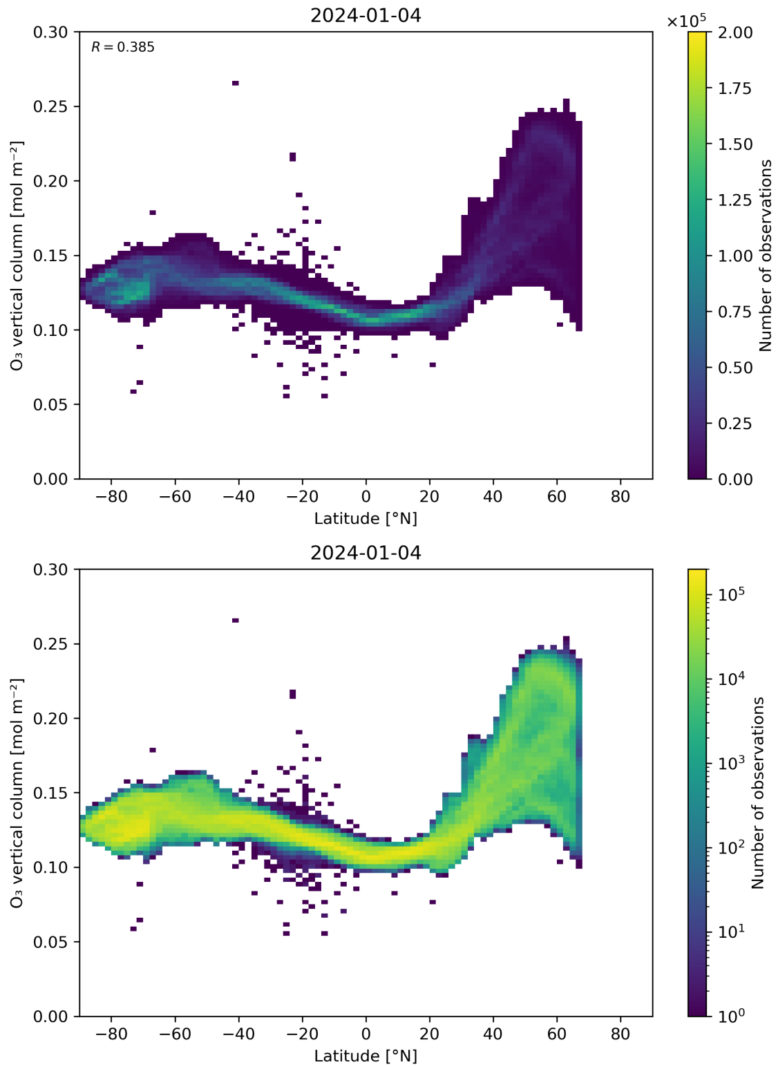
Figure 36: Scatter density plot of “Latitude” against “O 3 vertical column” for 2024-01-03 to 2024-01-05.
