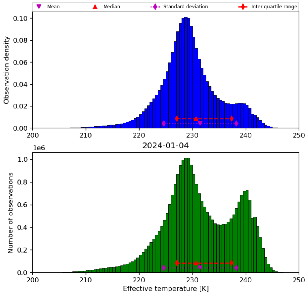
Figure 24: Histogram of “Effective temperature” for 2024-01-03 to 2024-01-05
