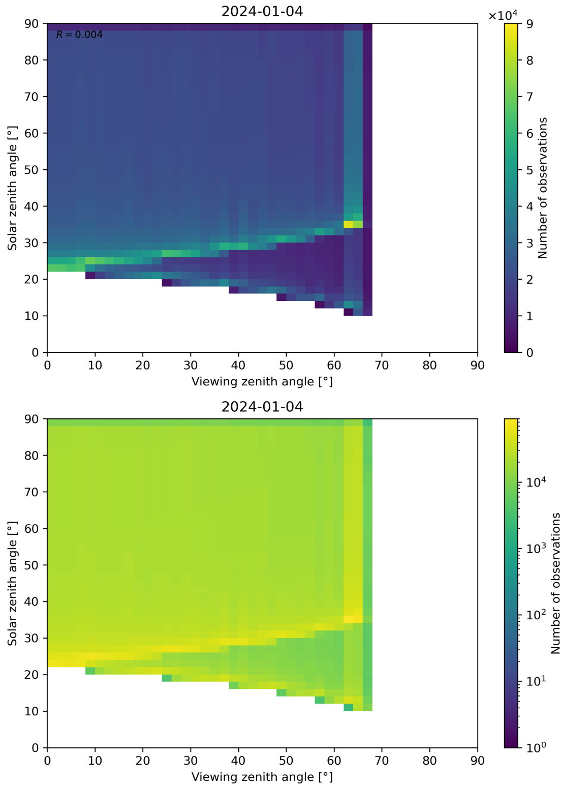
Figure 54: Scatter density plot of “Viewing zenith angle” against “Solar zenith angle” for 2024-01-03 to 2024-01-05.
