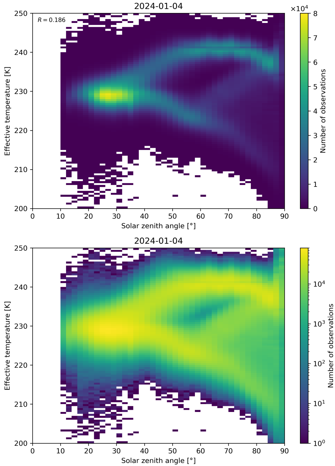
Figure 45: Scatter density plot of “Solar zenith angle” against “Effective temperature” for 2024-01-03 to 2024-01-05.
