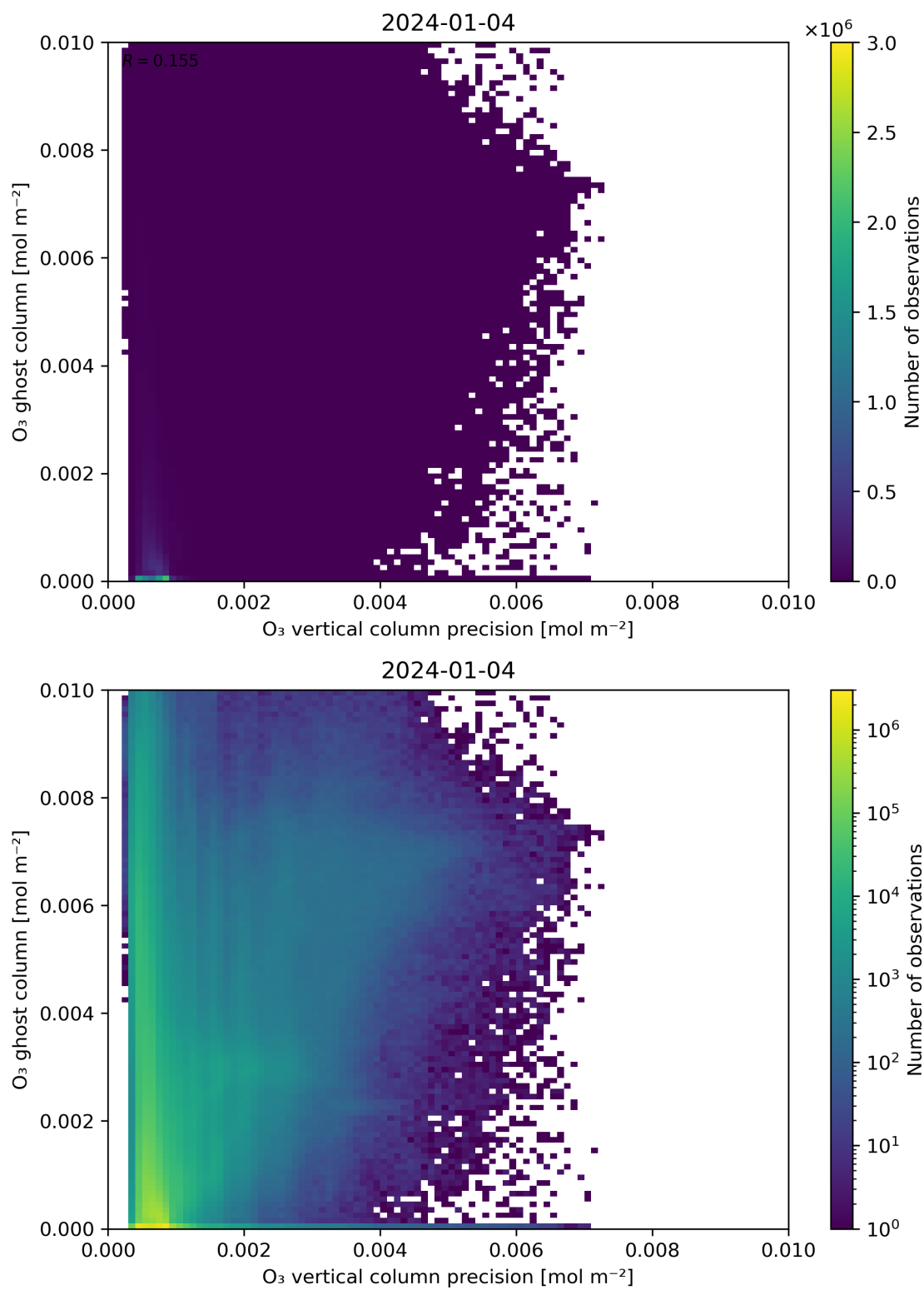
Figure 43: Scatter density plot of “ \text{O}_3 vertical column precision” against “ \text{O}_3 ghost column” for 2024-01-03 to 2024-01-05.
