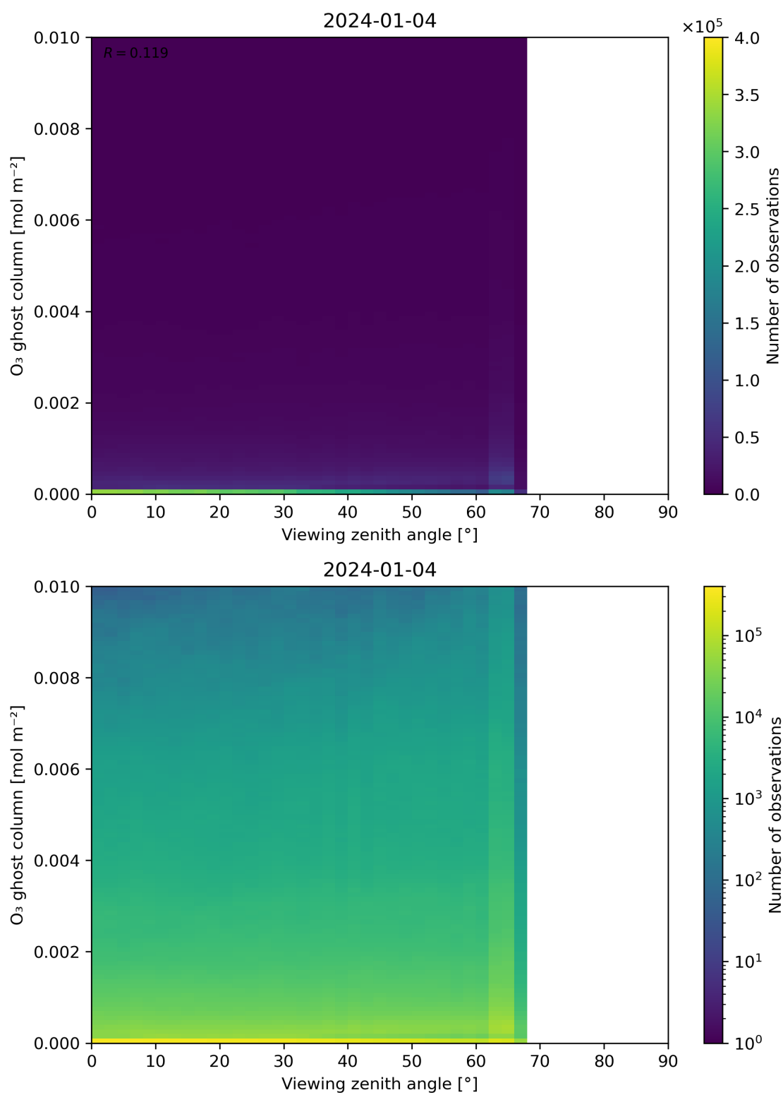
Figure 51: Scatter density plot of “Viewing zenith angle” against “O 3 ghost column” for 2024-01-03 to 2024-01-05.
