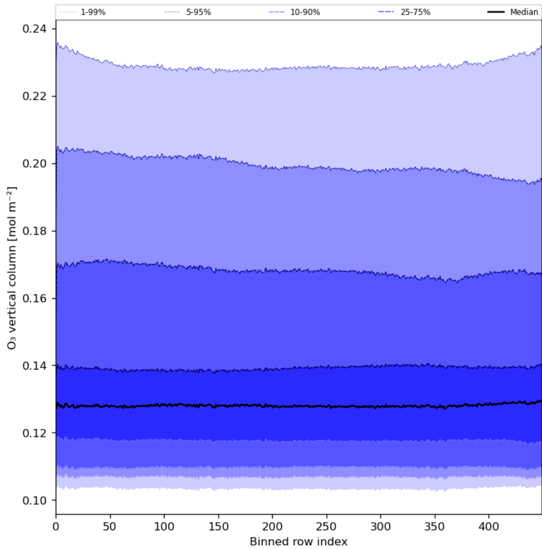
Figure 28: Along track statistics of “O 3 vertical column” for 2024-01-03 to 2024-01-05
