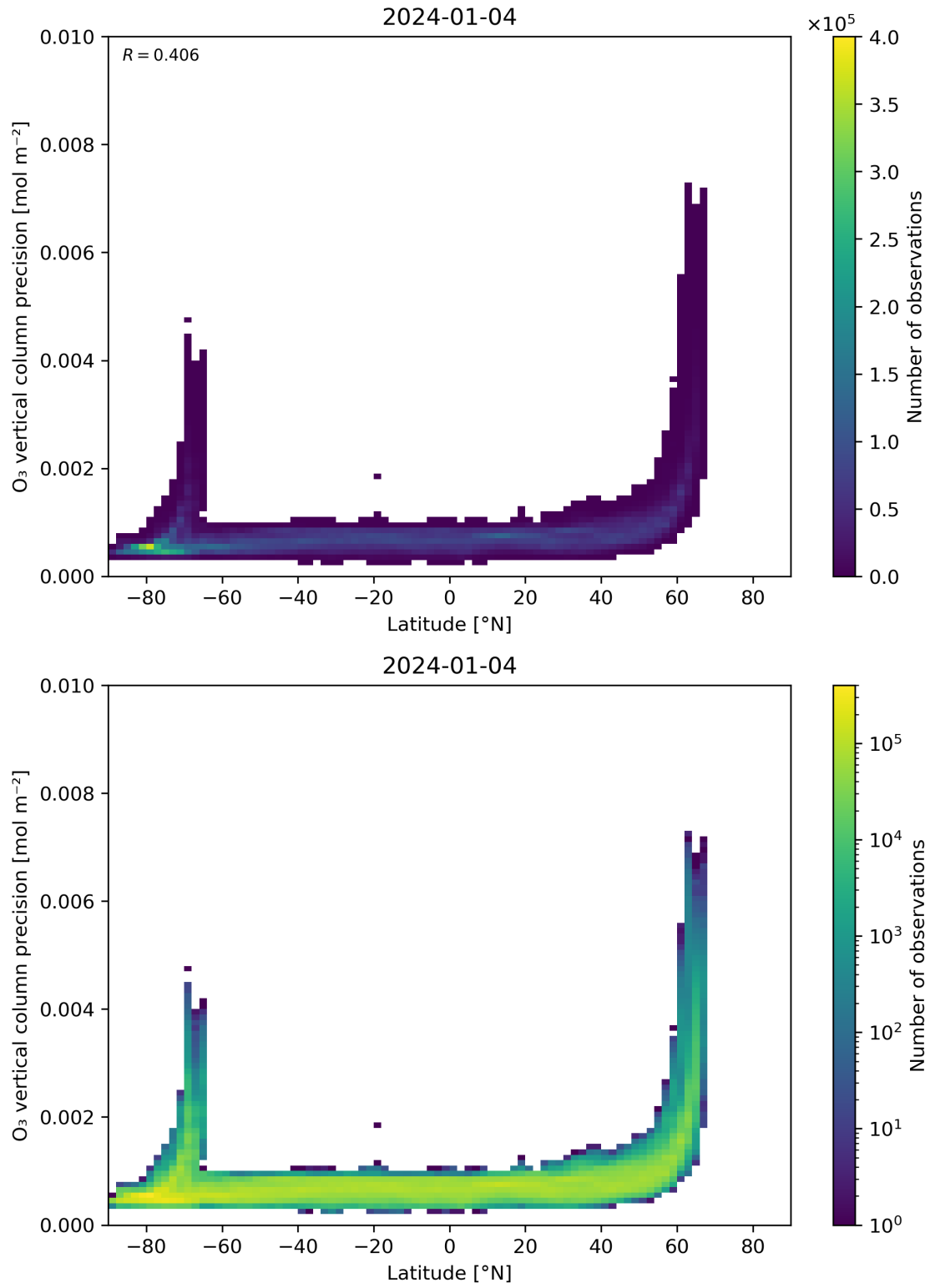
Figure 37: Scatter density plot of “Latitude” against “O 3 vertical column precision” for 2024-01-03 to 2024-01-05.
