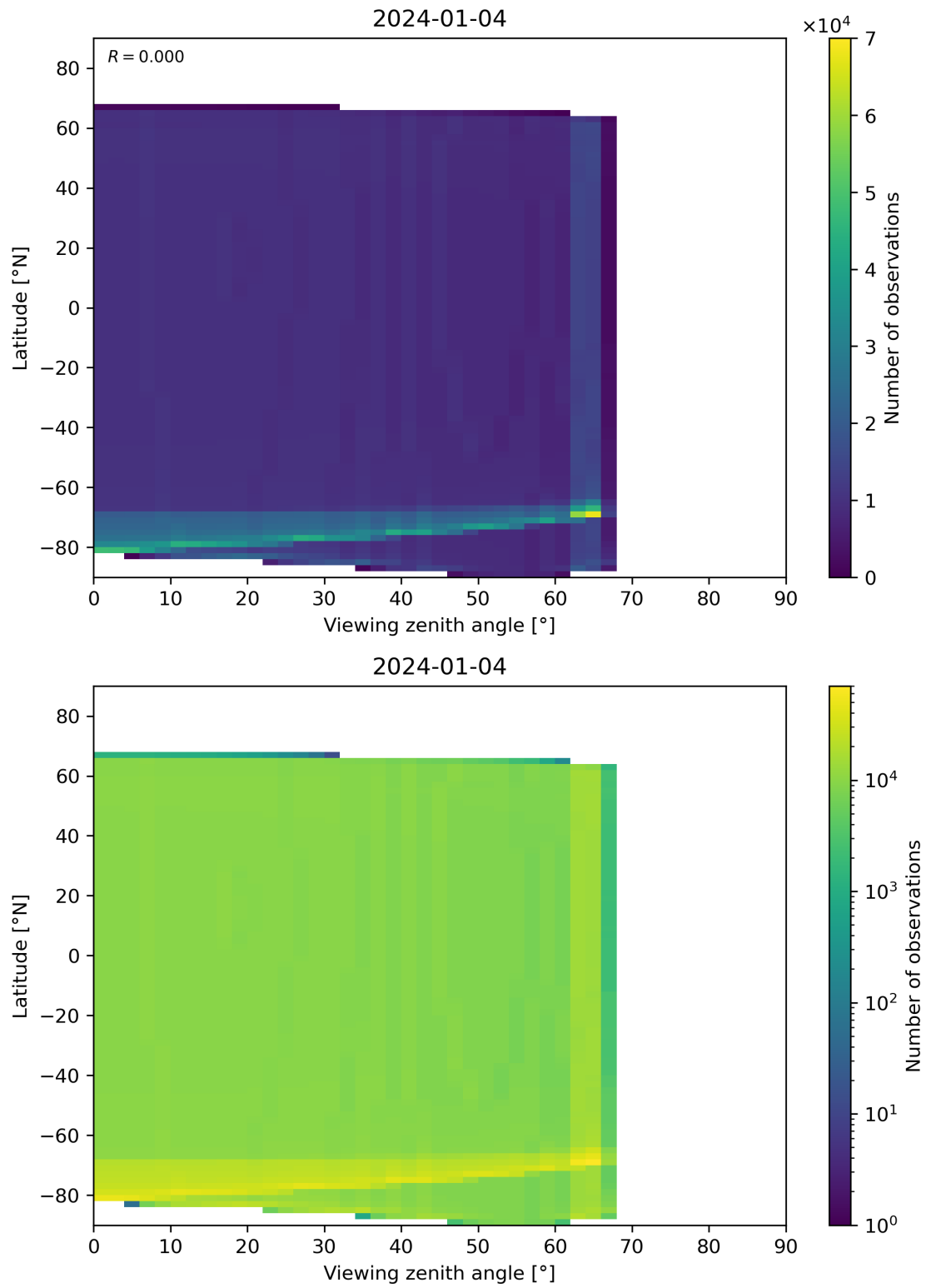
Figure 49: Scatter density plot of “Viewing zenith angle” against “Latitude” for 2024-01-03 to 2024-01-05.
