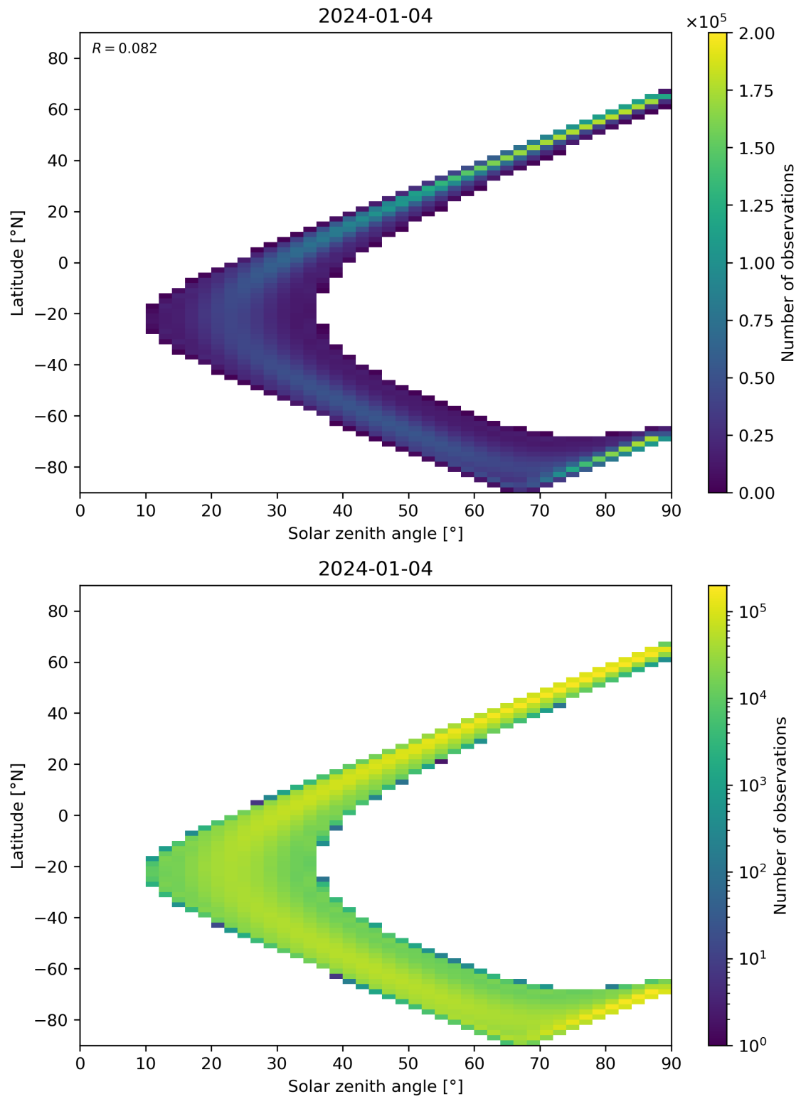
Figure 44: Scatter density plot of “Solar zenith angle” against “Latitude” for 2024-01-03 to 2024-01-05.
