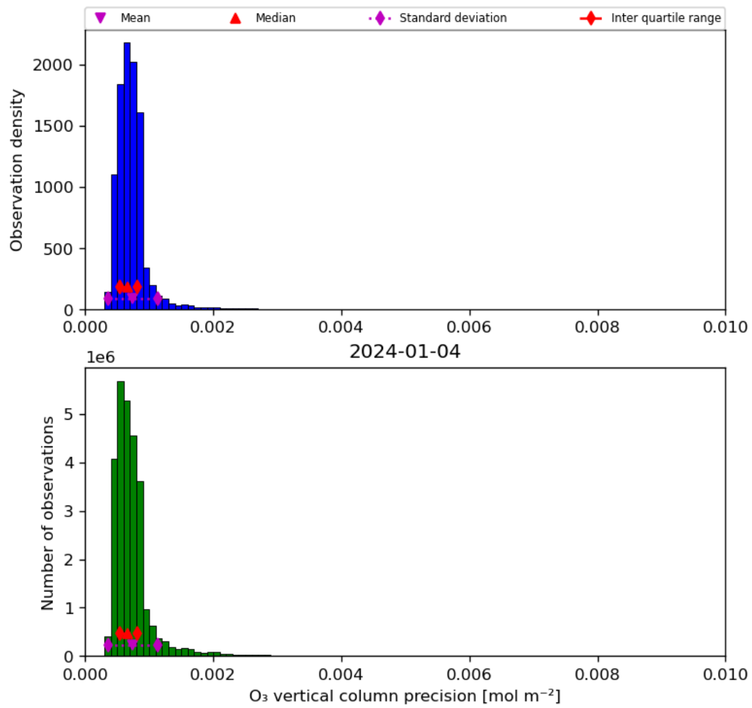
Figure 22: Histogram of “O 3 vertical column precision” for 2024-01-03 to 2024-01-05
