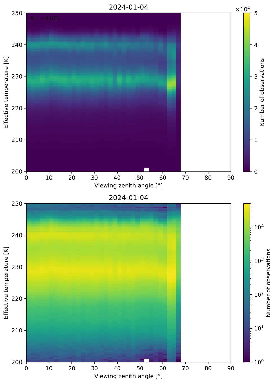
Figure 50: Scatter density plot of “Viewing zenith angle” against “Effective temperature” for 2024-01-03 to 2024-01-05.
