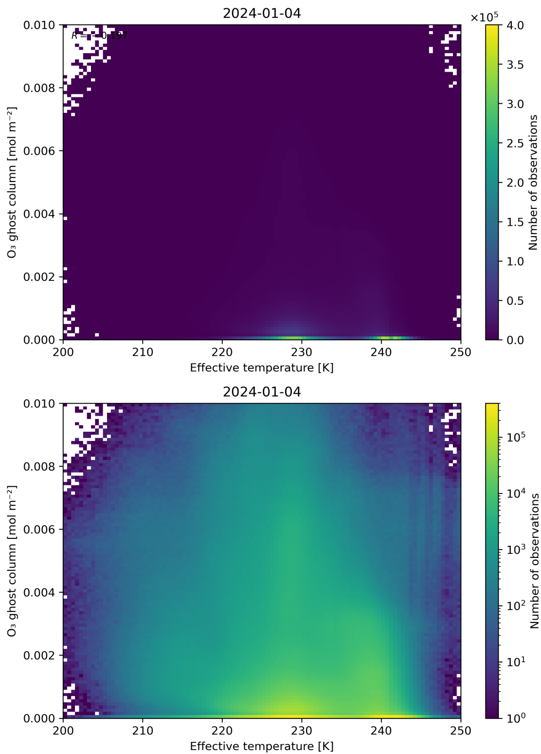
Figure 38: Scatter density plot of “Effective temperature” against “O 3 ghost column” for 2024-01-03 to 2024-01-05.
