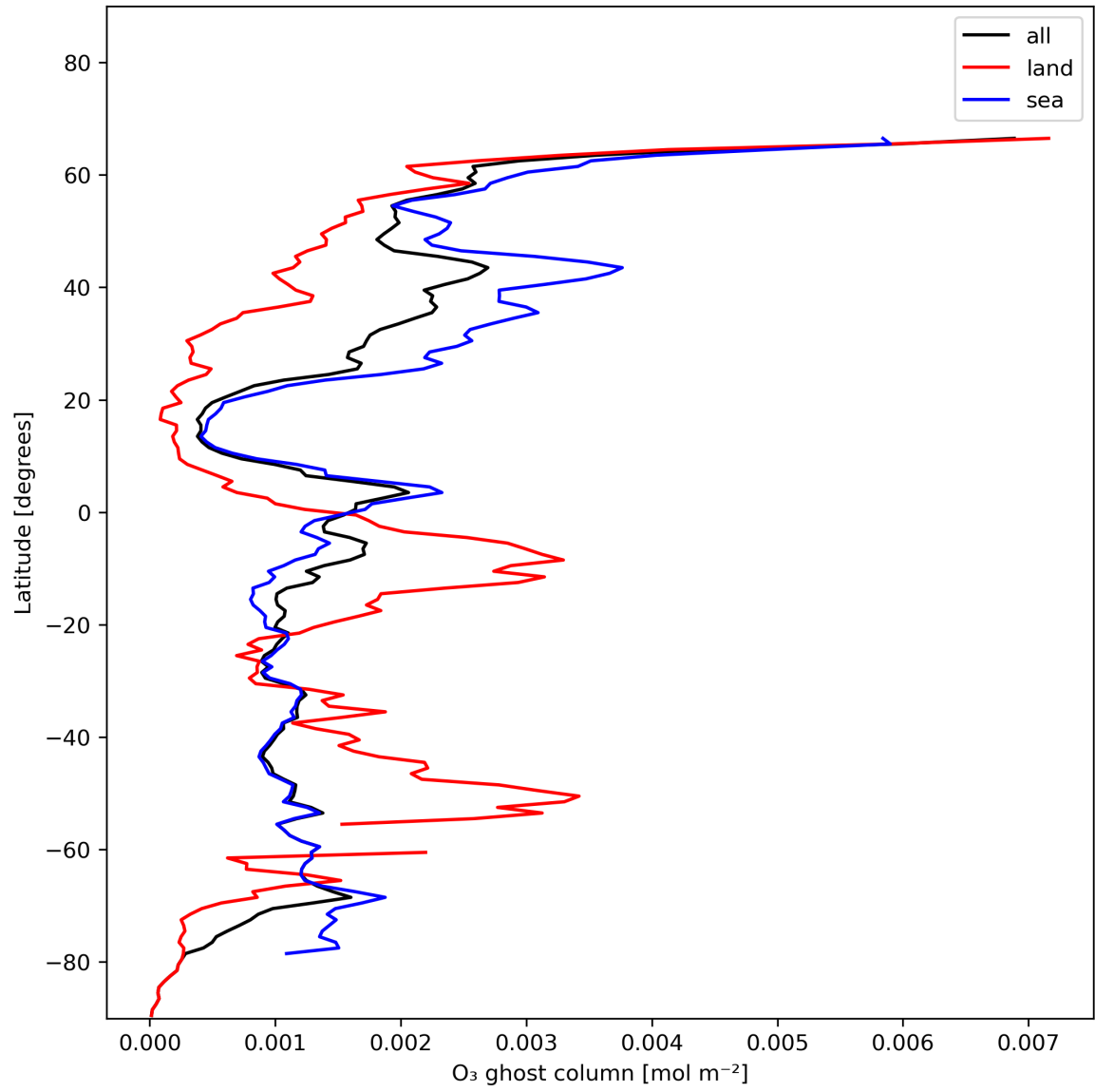
Figure 18: Zonal average of “O 3 ghost column” for 2024-01-03 to 2024-01-05.
