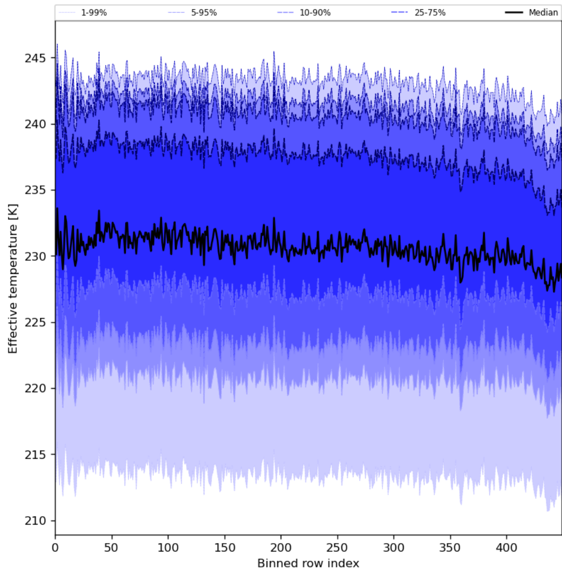
Figure 31: Along track statistics of “Effective temperature” for 2024-01-03 to 2024-01-05
