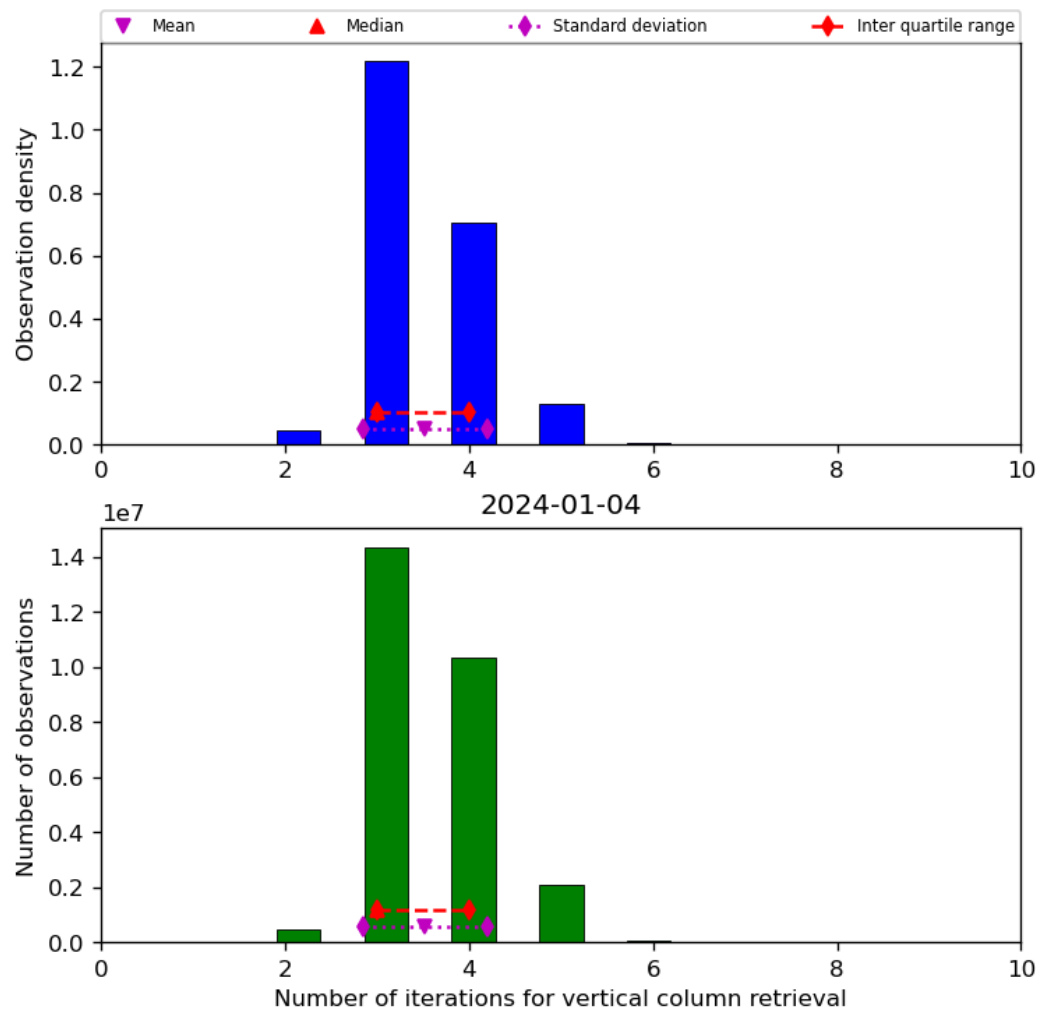
Figure 26: Histogram of “Number of iterations for vertical column retrieval” for 2024-01-03 to 2024-01-05
