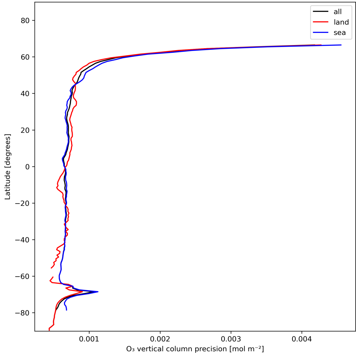
Figure 15: Zonal average of “O 3 vertical column precision” for 2024-01-03 to 2024-01-05.
