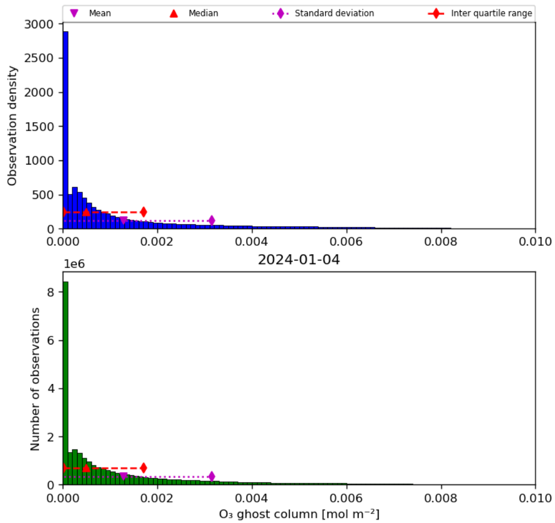
Figure 25: Histogram of “O 3 ghost column” for 2024-01-03 to 2024-01-05
