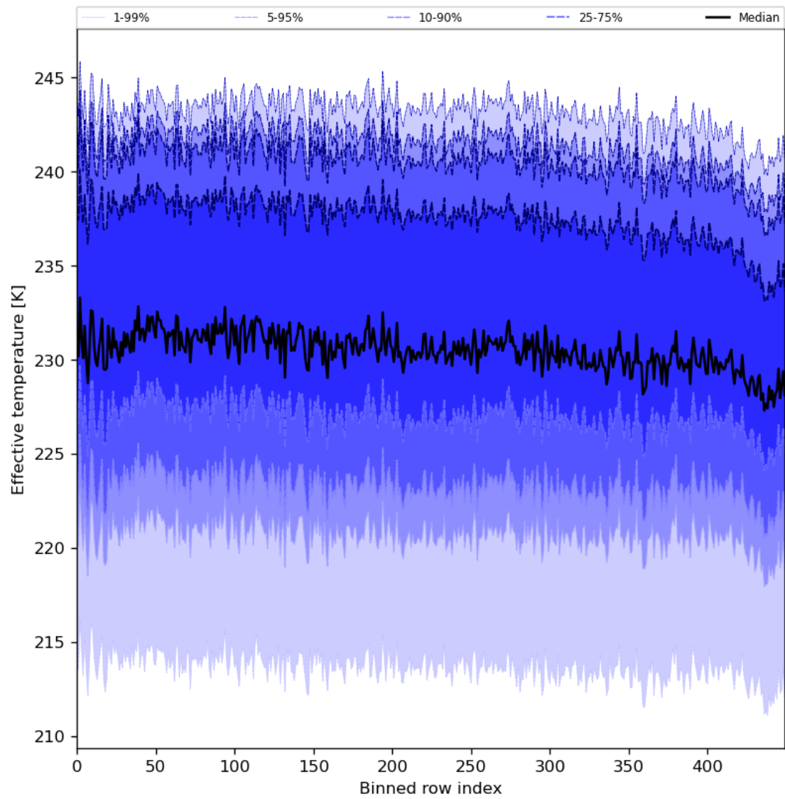
Figure 31: Along track statistics of “Effective temperature” for 2024-01-05 to 2024-01-06
