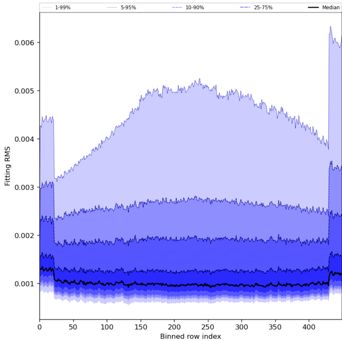
Figure 30: Along track statistics of “Fitting RMS” for 2024-01-05 to 2024-01-06
