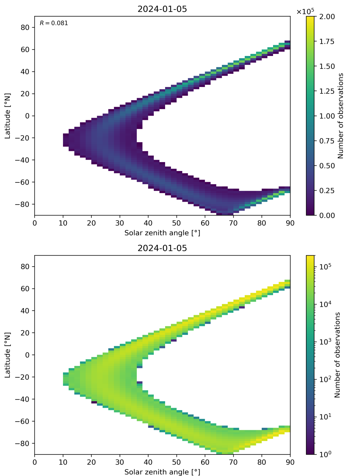
Figure 44: Scatter density plot of “Solar zenith angle” against “Latitude” for 2024-01-05 to 2024-01-06.
