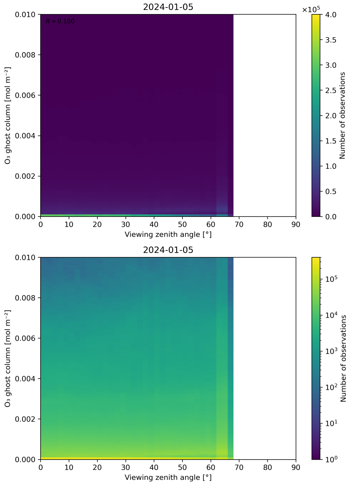
Figure 51: Scatter density plot of “Viewing zenith angle” against “O 3 ghost column” for 2024-01-05 to 2024-01-06.
