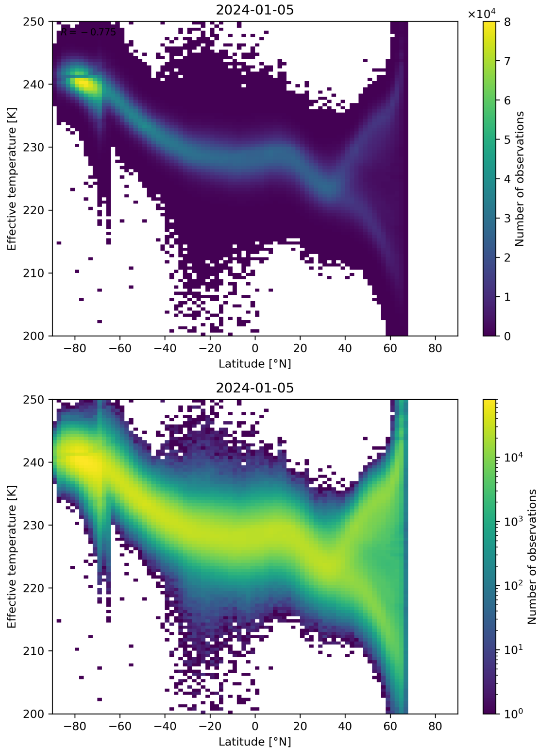
Figure 34: Scatter density plot of “Latitude” against “Effective temperature” for 2024-01-05 to 2024-01-06.
