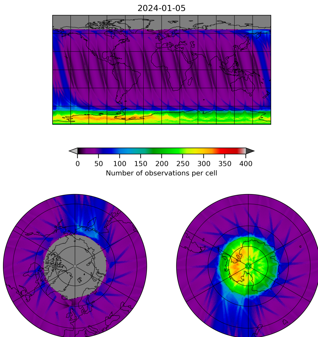
Figure 12: Map of the number of observations for 2024-01-05 to 2024-01-06
