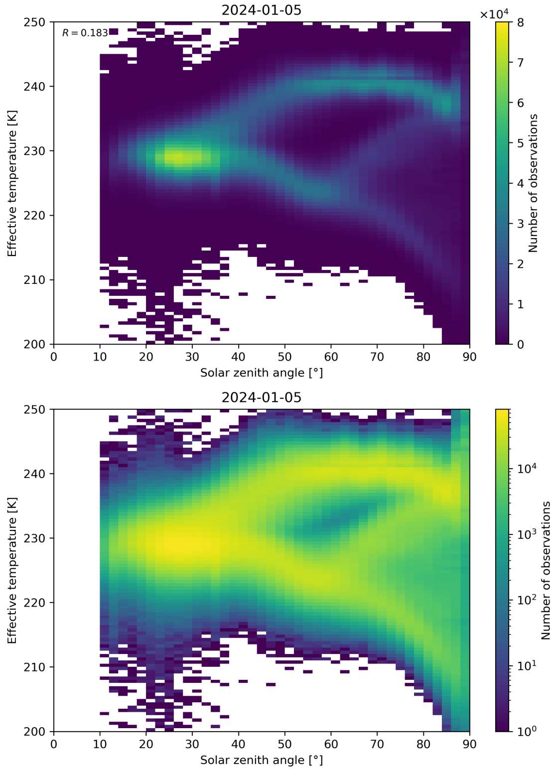
Figure 45: Scatter density plot of “Solar zenith angle” against “Effective temperature” for 2024-01-05 to 2024-01-06.
