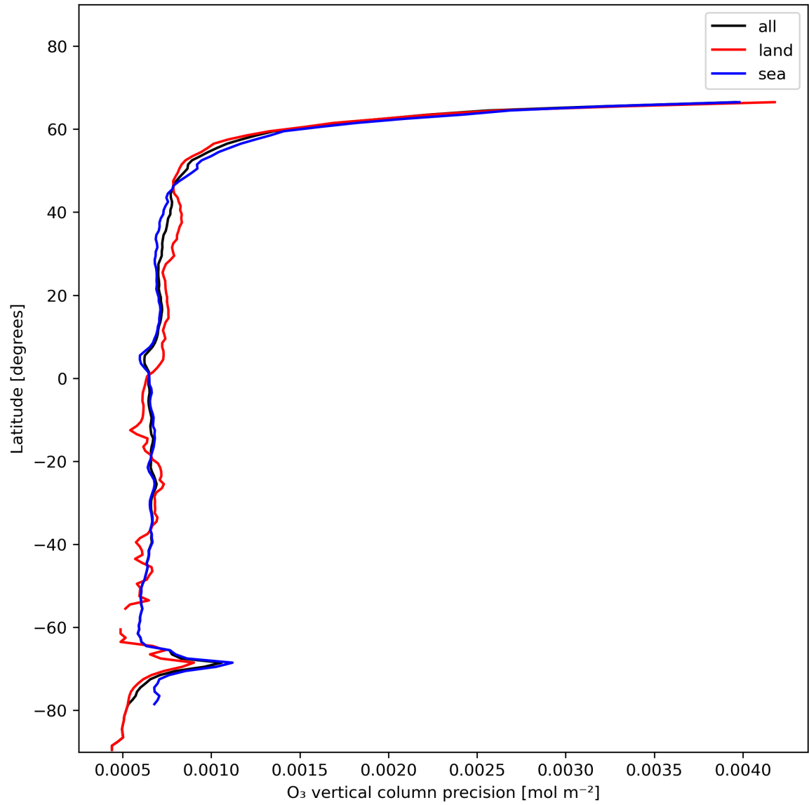
Figure 15: Zonal average of “O 3 vertical column precision” for 2024-01-05 to 2024-01-06.
