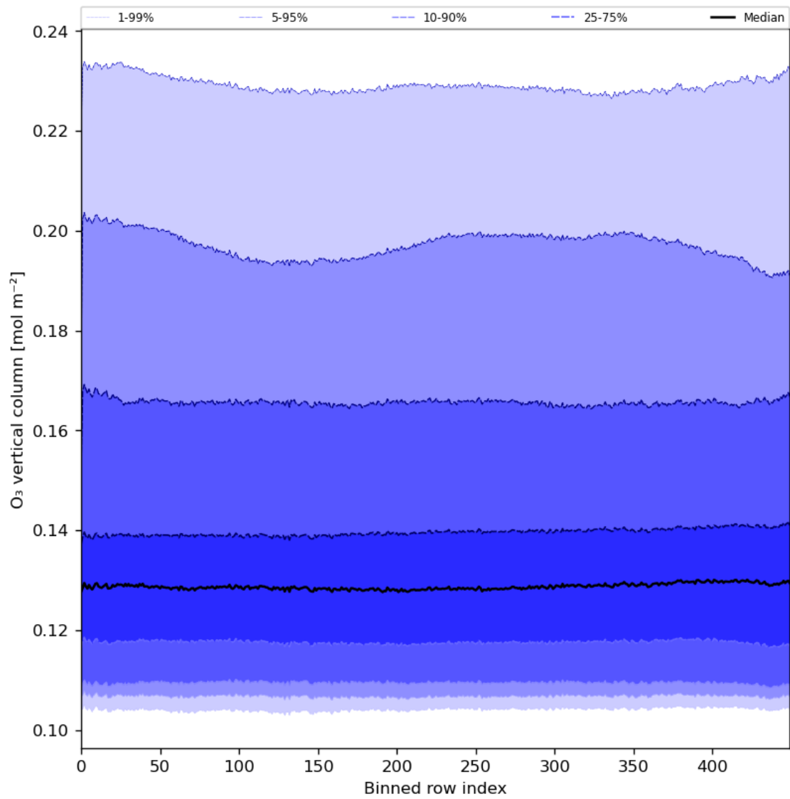
Figure 28: Along track statistics of “O 3 vertical column” for 2024-01-05 to 2024-01-06
