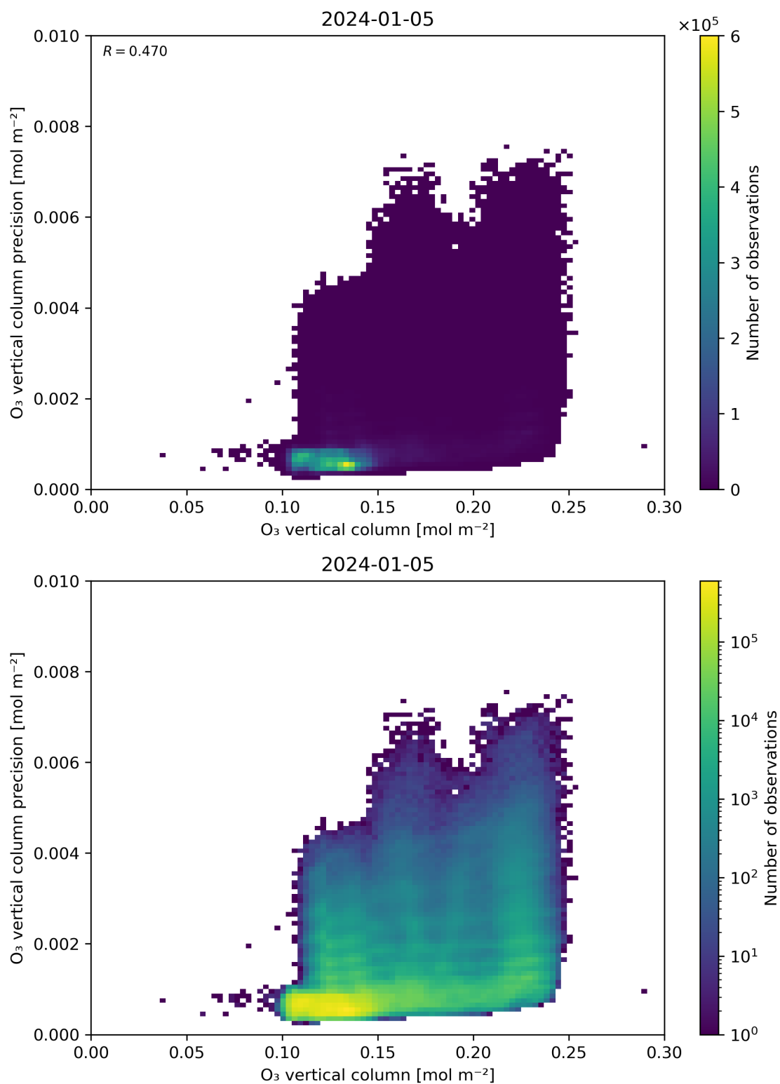
Figure 41: Scatter density plot of “O 3 vertical column” against “O 3 vertical column precision” for 2024-01-05 to 2024-01-06.
