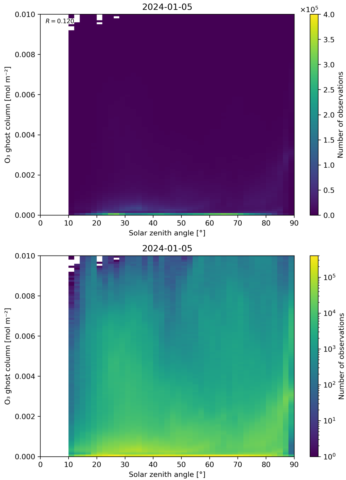
Figure 46: Scatter density plot of “Solar zenith angle” against “O 3 ghost column” for 2024-01-05 to 2024-01-06.
