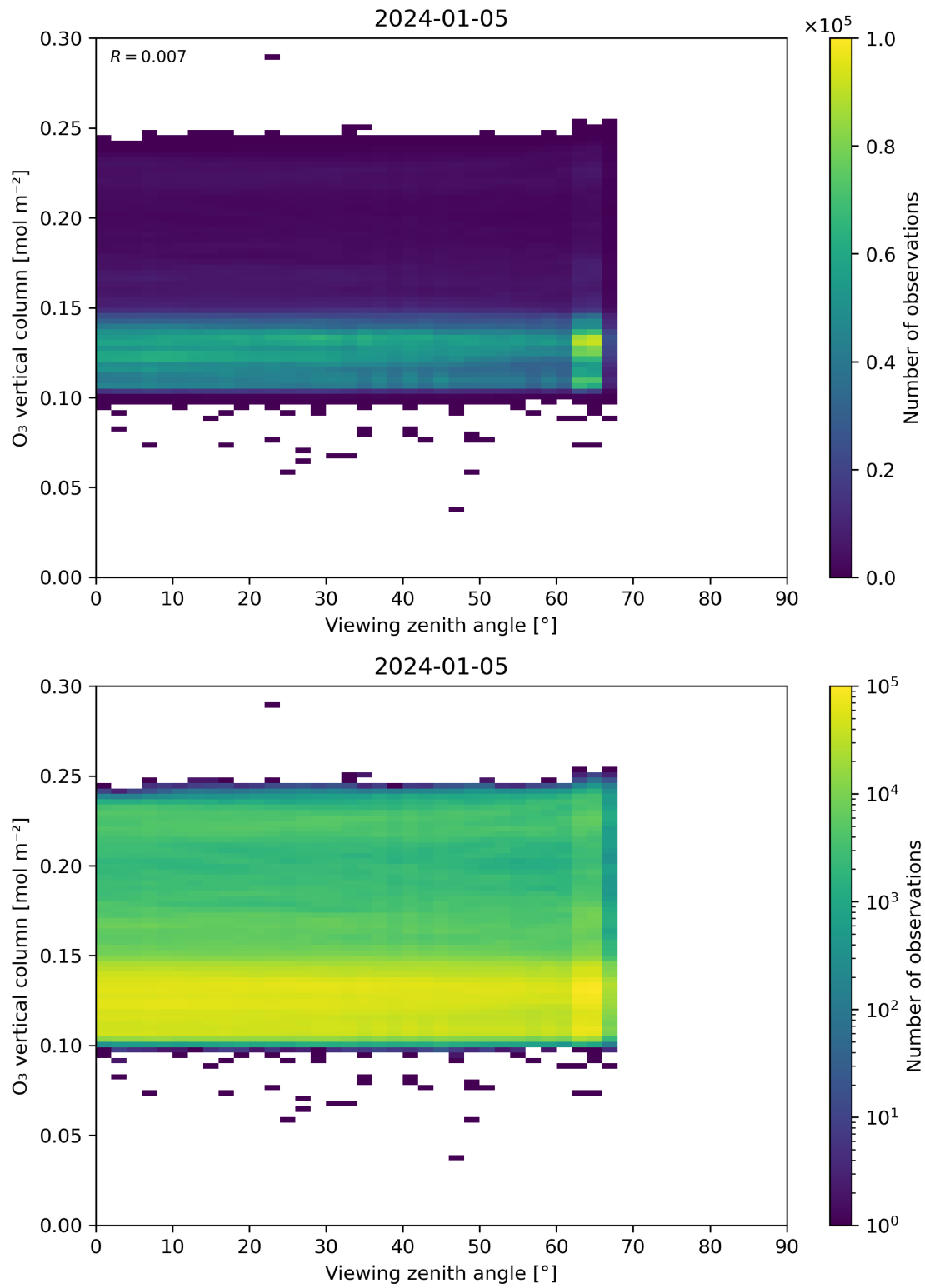
Figure 52: Scatter density plot of “Viewing zenith angle” against “O 3 vertical column” for 2024-01-05 to 2024-01-06.
