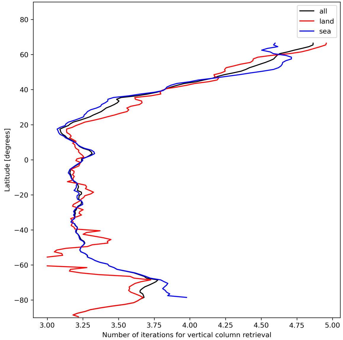
Figure 19: Zonal average of “Number of iterations for vertical column retrieval” for 2024-01-05 to 2024-01-06.
