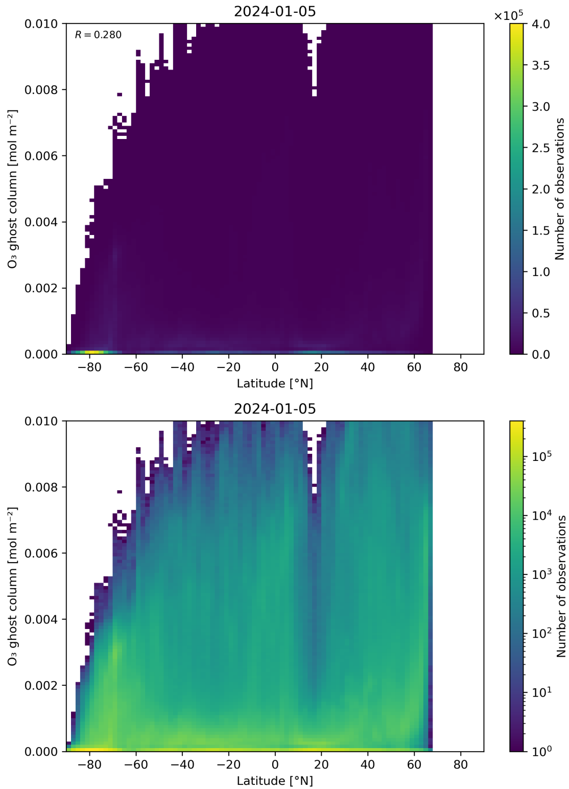
Figure 35: Scatter density plot of “Latitude” against “O 3 ghost column” for 2024-01-05 to 2024-01-06.
