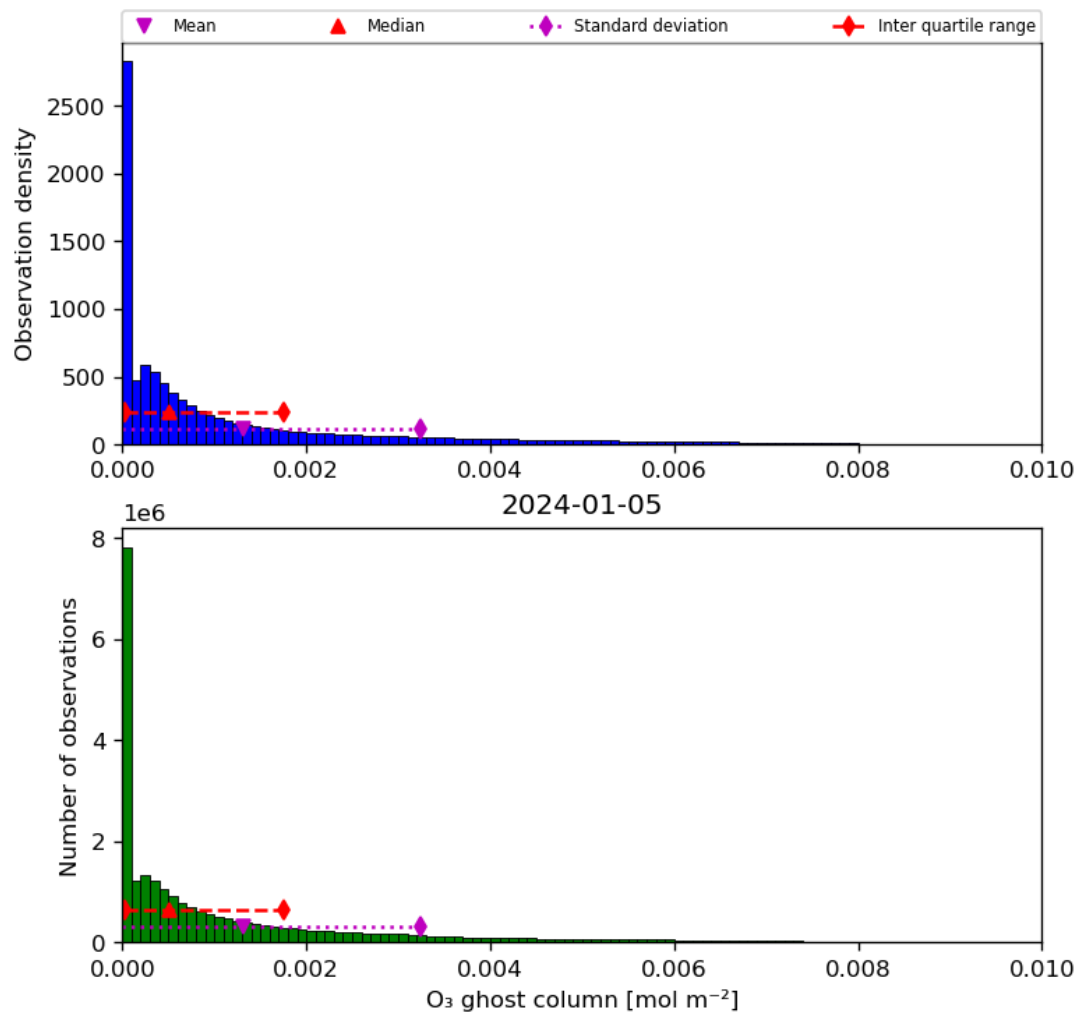
Figure 25: Histogram of “O 3 ghost column” for 2024-01-05 to 2024-01-06
