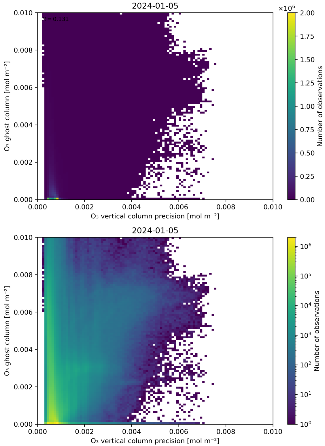
Figure 43: Scatter density plot of “ \text{O}_3 vertical column precision” against “ \text{O}_3 ghost column” for 2024-01-05 to 2024-01-06.
