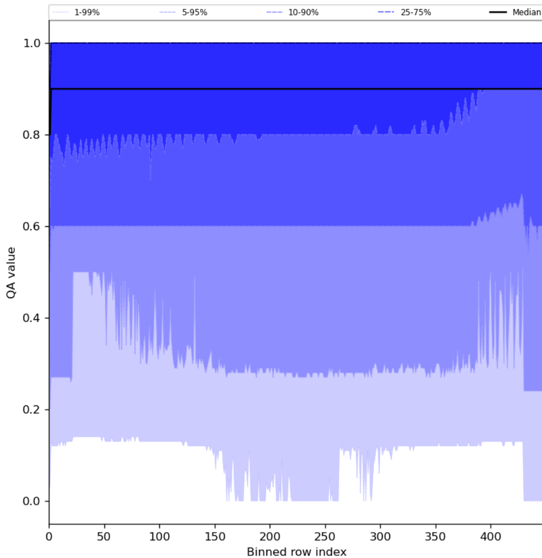
Figure 27: Along track statistics of “QA value” for 2024-01-05 to 2024-01-06
