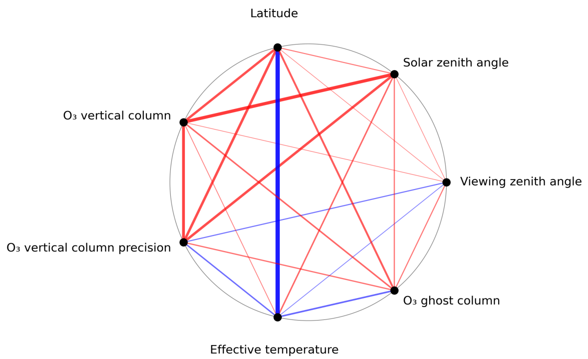
Figure 1: Map of correlation graph for 2024-01-05 to 2024-01-06.
