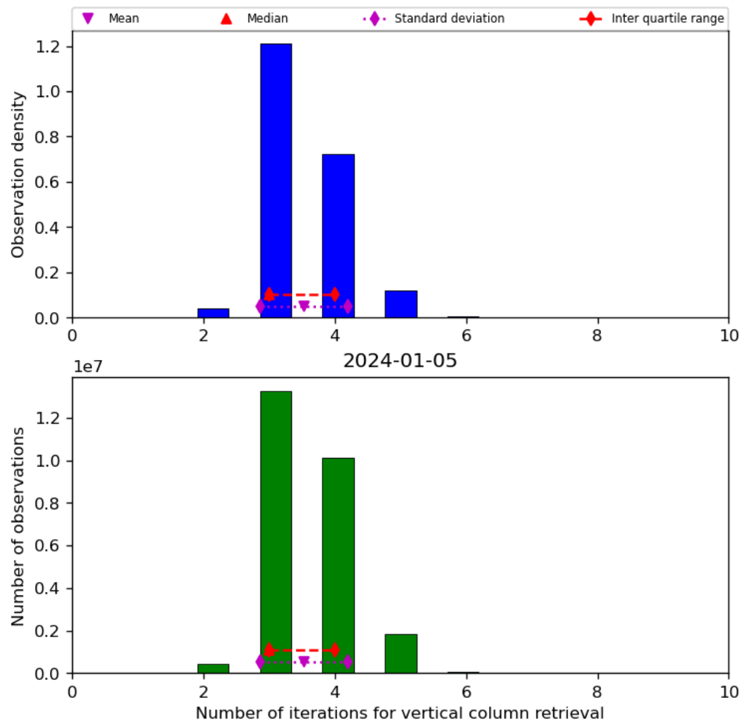
Figure 26: Histogram of “Number of iterations for vertical column retrieval” for 2024-01-05 to 2024-01-06
