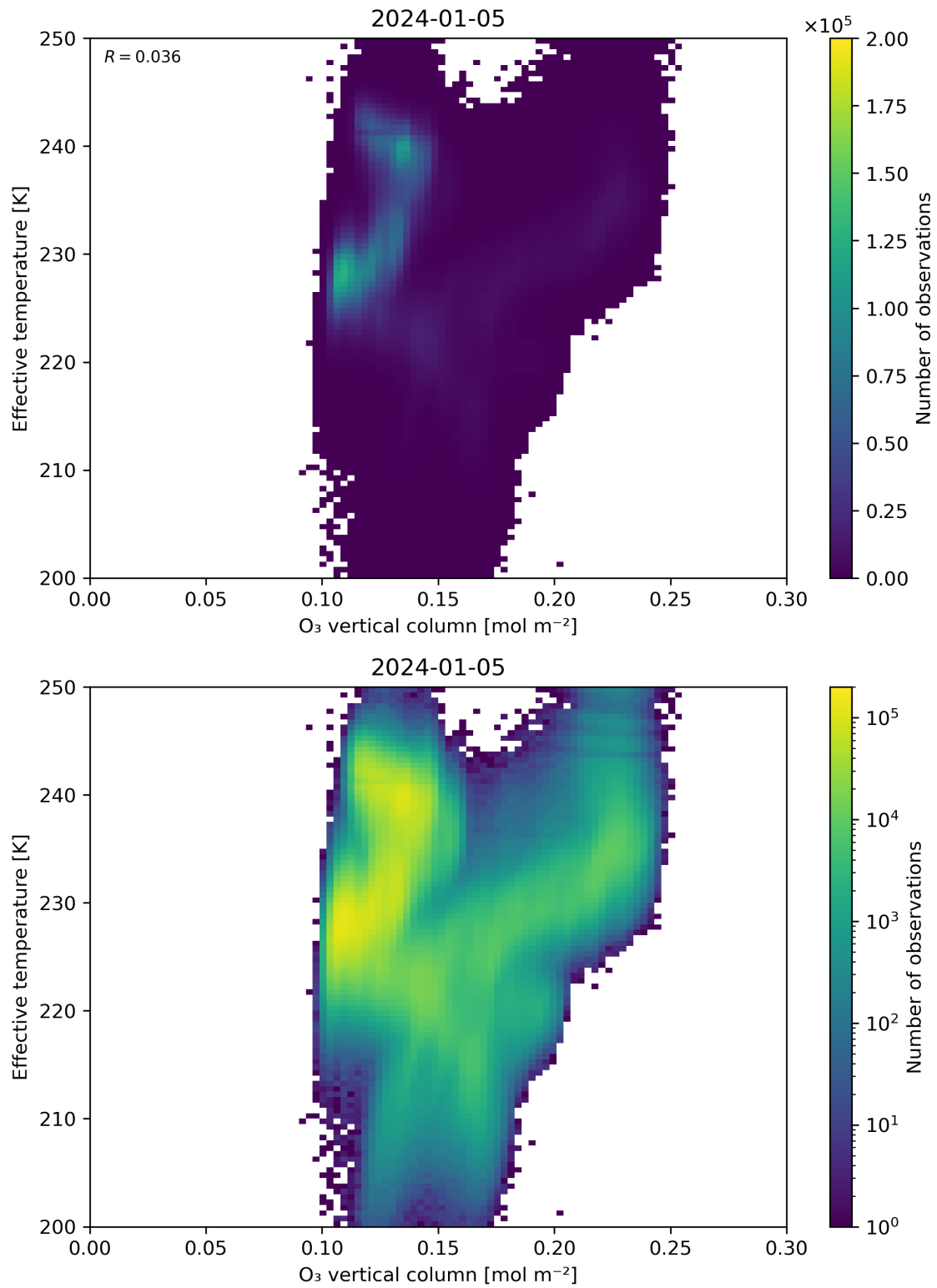
Figure 39: Scatter density plot of “O 3 vertical column” against “Effective temperature” for 2024-01-05 to 2024-01-06.
