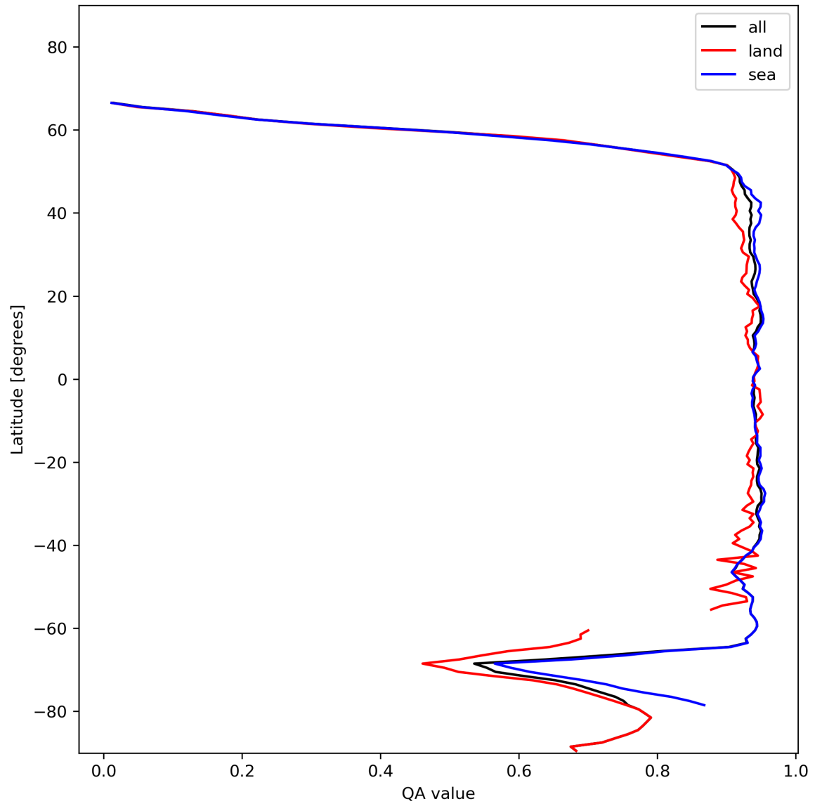
Figure 13: Zonal average of “QA value” for 2024-01-05 to 2024-01-06.
