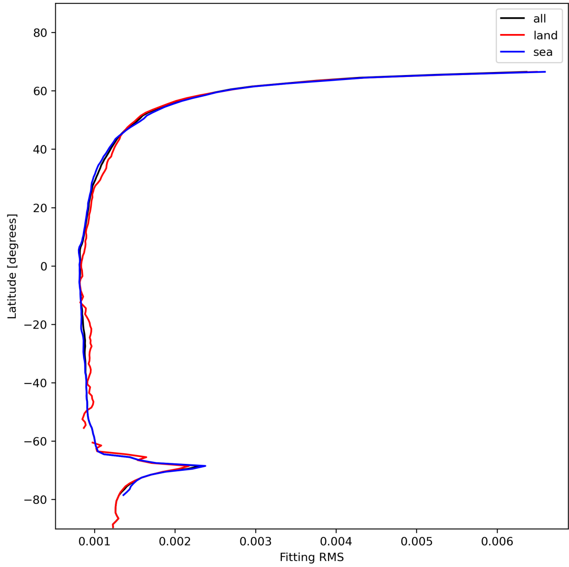
Figure 16: Zonal average of “Fitting RMS” for 2024-01-05 to 2024-01-06.
