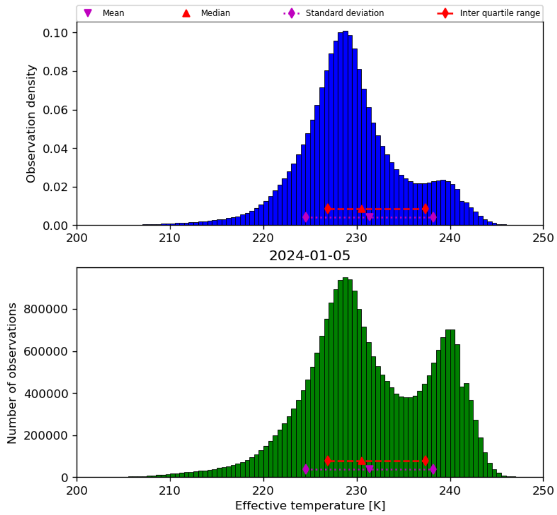
Figure 24: Histogram of “Effective temperature” for 2024-01-05 to 2024-01-06
