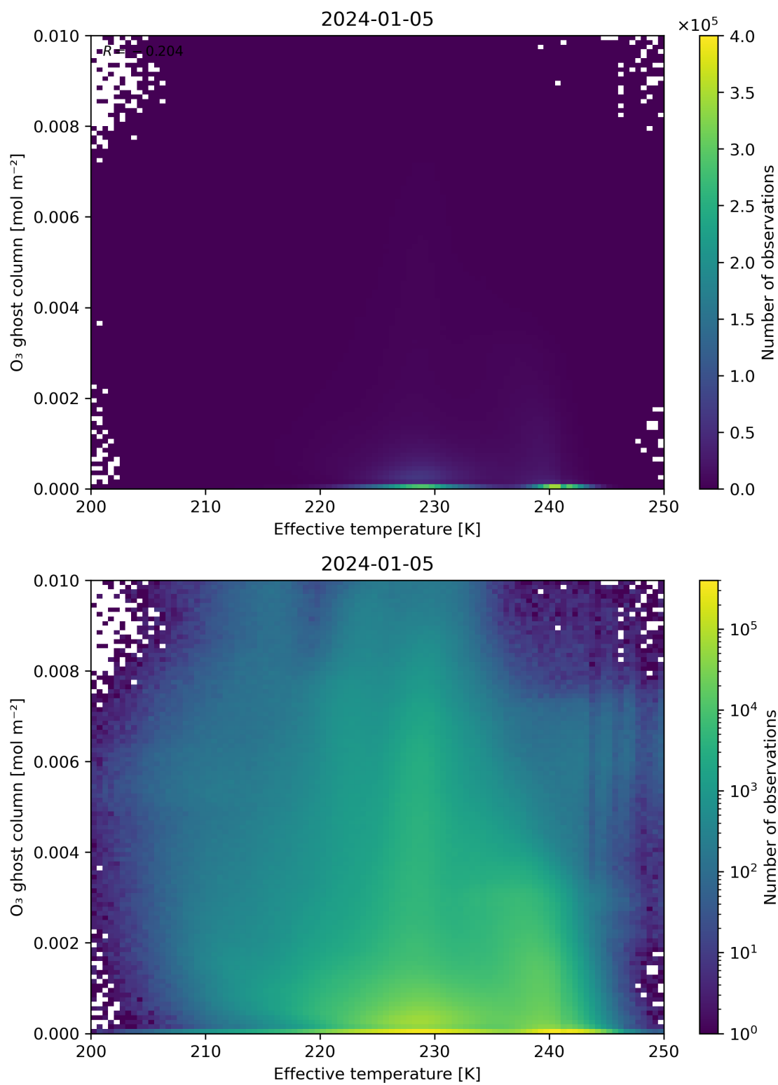
Figure 38: Scatter density plot of “Effective temperature” against “O 3 ghost column” for 2024-01-05 to 2024-01-06.
