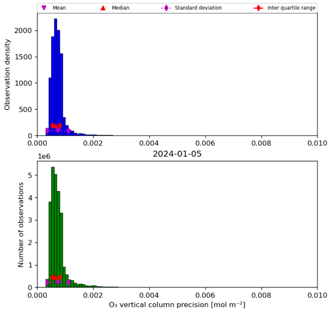
Figure 22: Histogram of “O 3 vertical column precision” for 2024-01-05 to 2024-01-06
