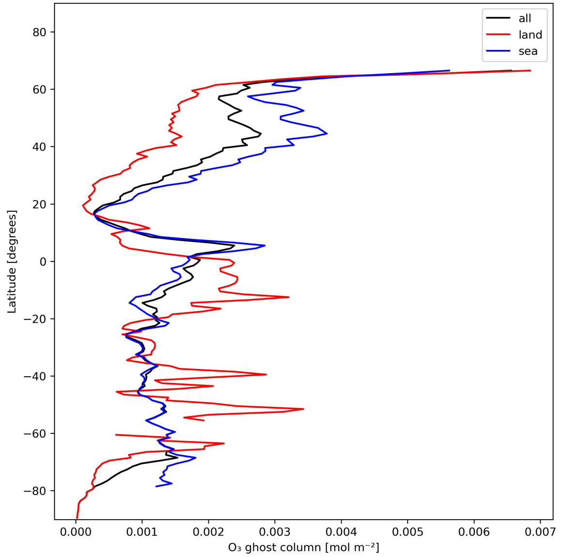
Figure 18: Zonal average of “O 3 ghost column” for 2024-01-05 to 2024-01-06.
