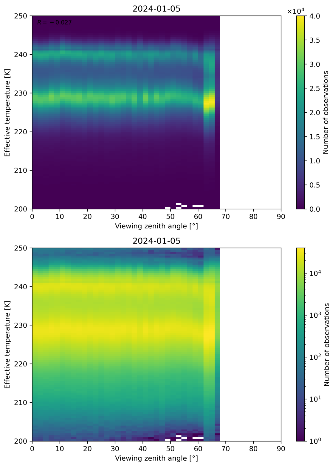
Figure 50: Scatter density plot of “Viewing zenith angle” against “Effective temperature” for 2024-01-05 to 2024-01-06.
