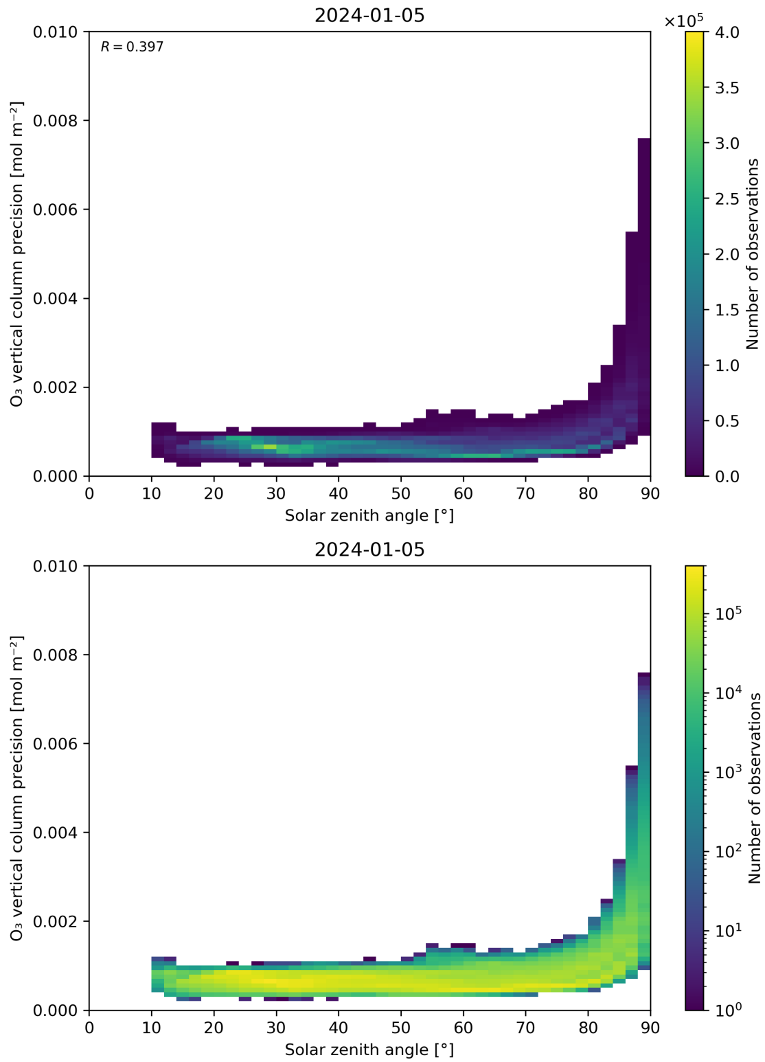
Figure 48: Scatter density plot of “Solar zenith angle” against “O 3 vertical column precision” for 2024-01-05 to 2024-01-06.
