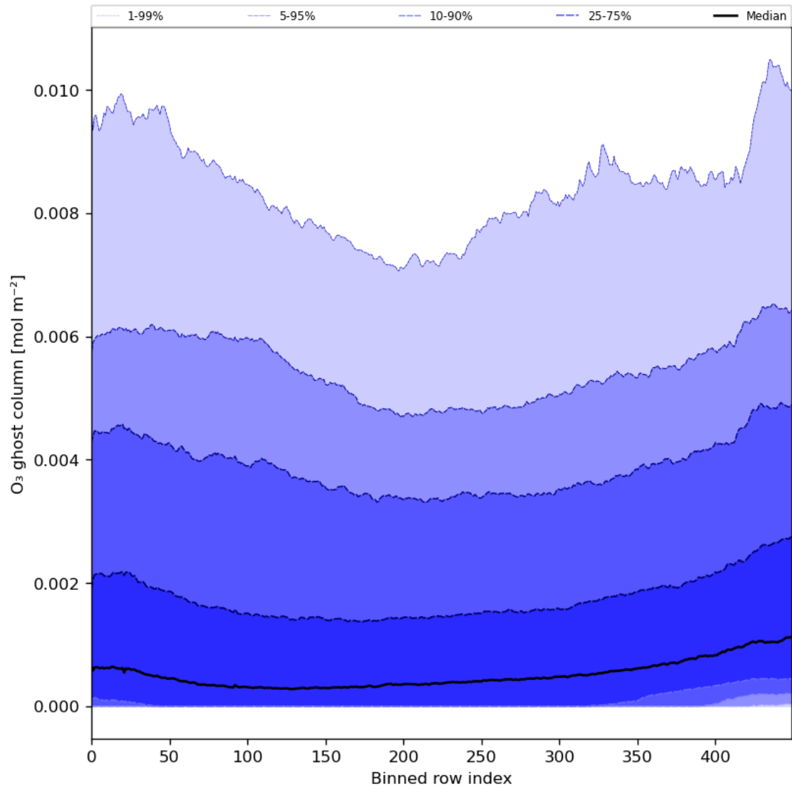
Figure 32: Along track statistics of “O 3 ghost column” for 2024-01-05 to 2024-01-06
