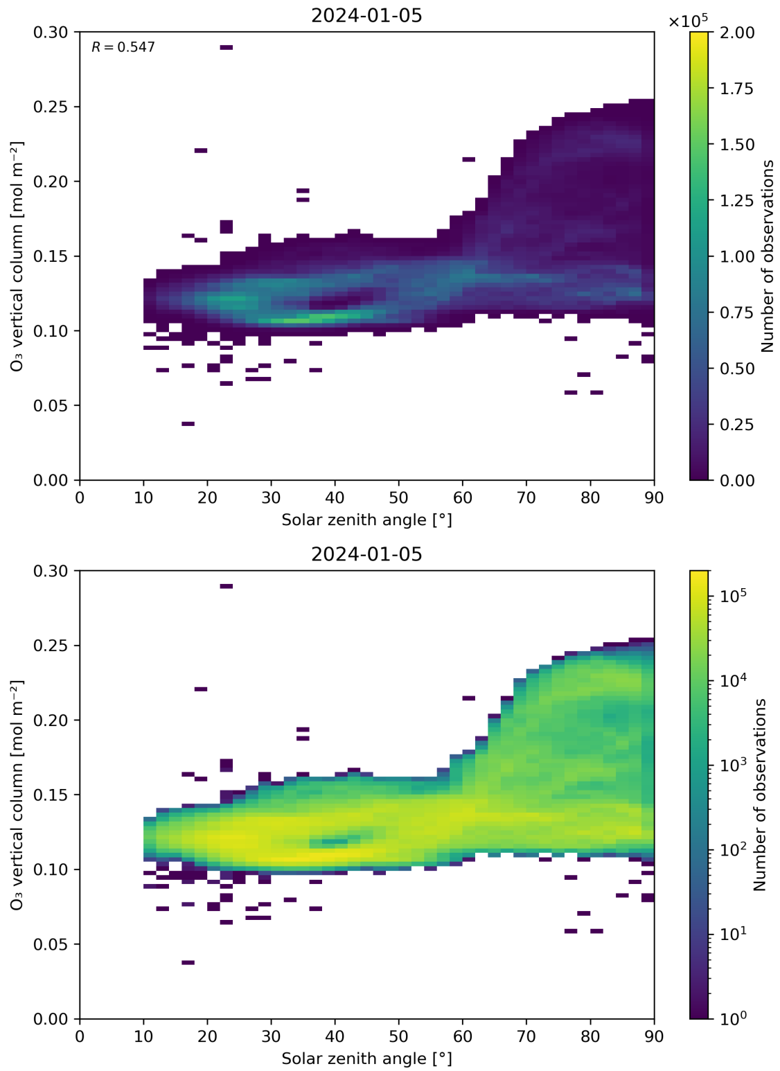
Figure 47: Scatter density plot of “Solar zenith angle” against “O 3 vertical column” for 2024-01-05 to 2024-01-06.
