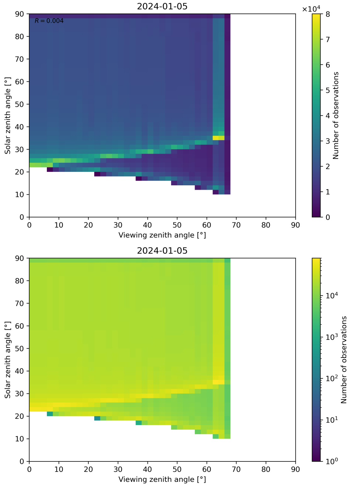
Figure 54: Scatter density plot of “Viewing zenith angle” against “Solar zenith angle” for 2024-01-05 to 2024-01-06.
