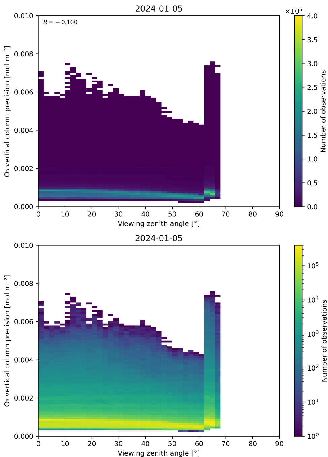
Figure 53: Scatter density plot of “Viewing zenith angle” against “O 3 vertical column precision” for 2024-01-05 to 2024-01-06.
