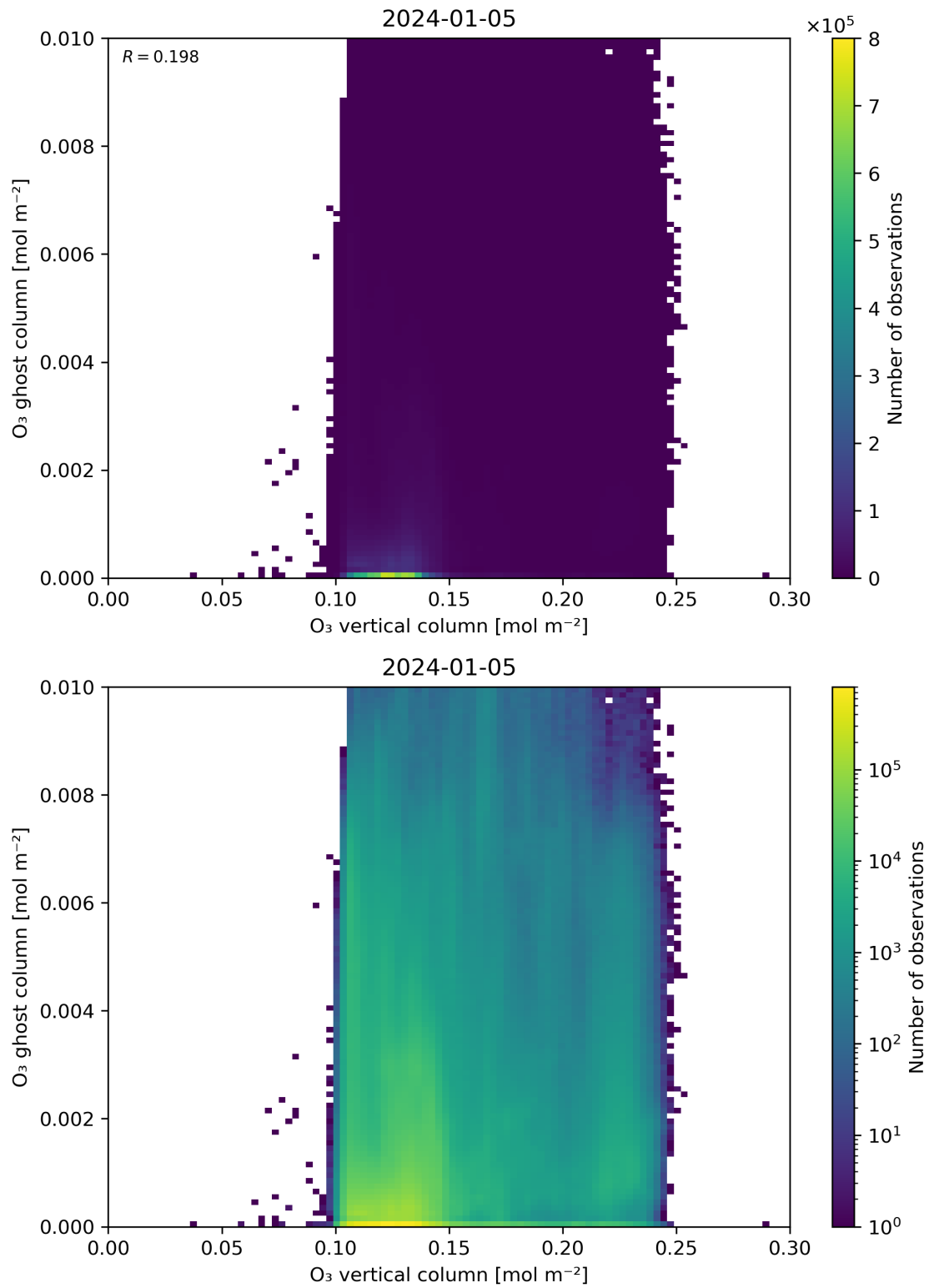
Figure 40: Scatter density plot of “O 3 vertical column” against “O 3 ghost column” for 2024-01-05 to 2024-01-06.
