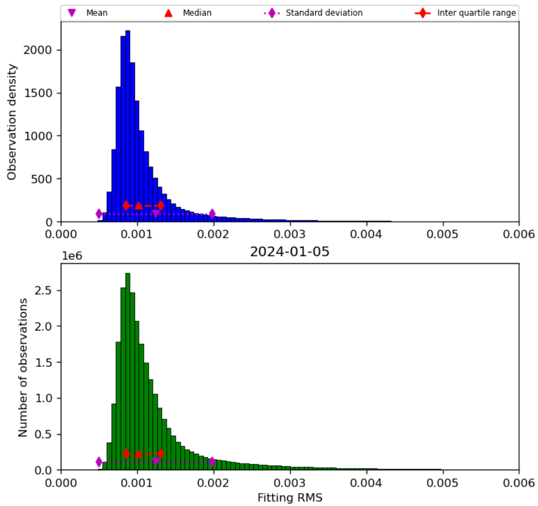
Figure 23: Histogram of “Fitting RMS” for 2024-01-05 to 2024-01-06
