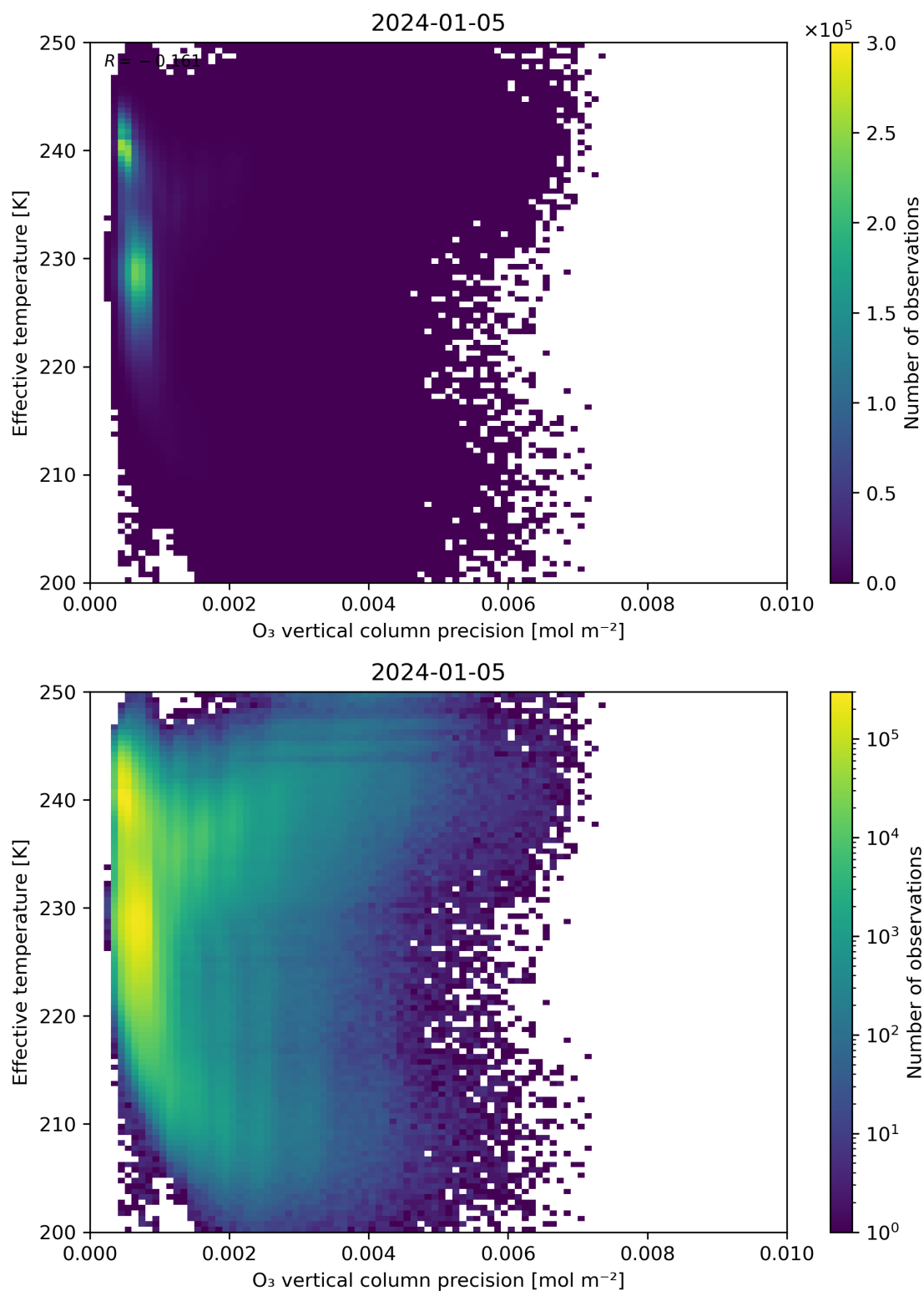
Figure 42: Scatter density plot of “O 3 vertical column precision” against “Effective temperature” for 2024-01-05 to 2024-01-06.
