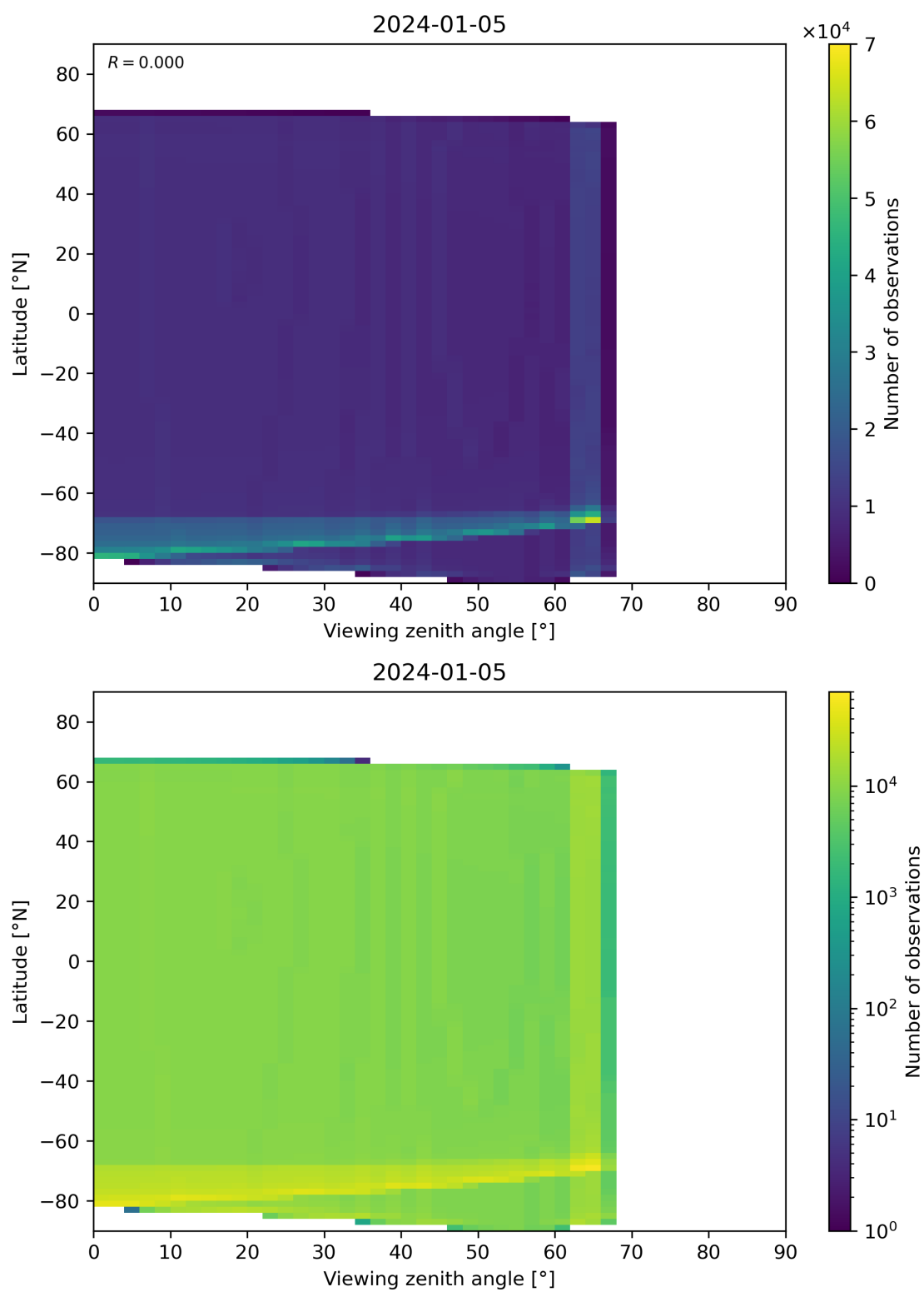
Figure 49: Scatter density plot of “Viewing zenith angle” against “Latitude” for 2024-01-05 to 2024-01-06.
