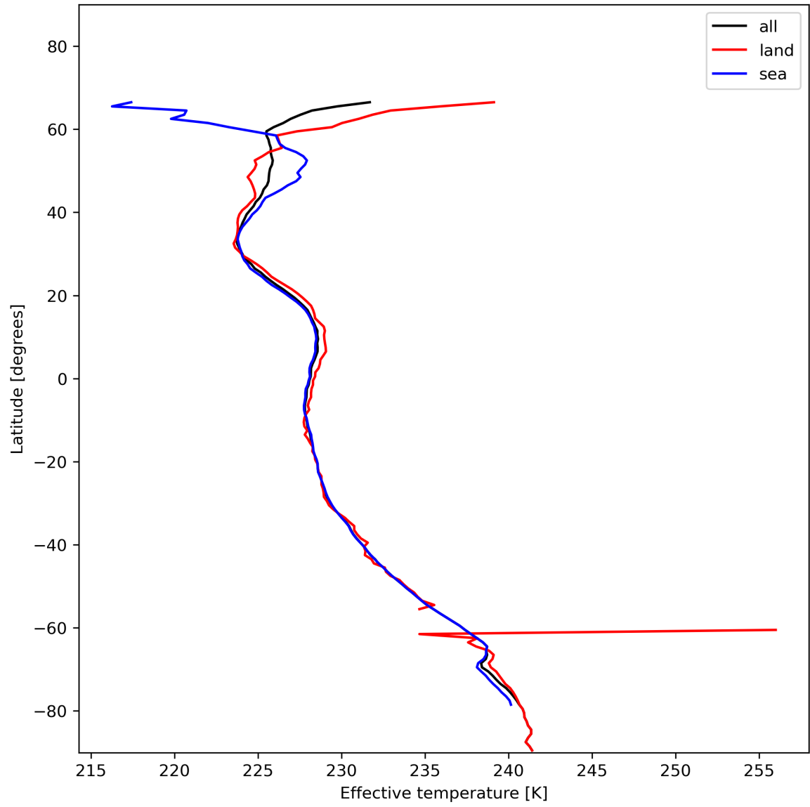
Figure 17: Zonal average of “Effective temperature” for 2024-01-05 to 2024-01-06.
