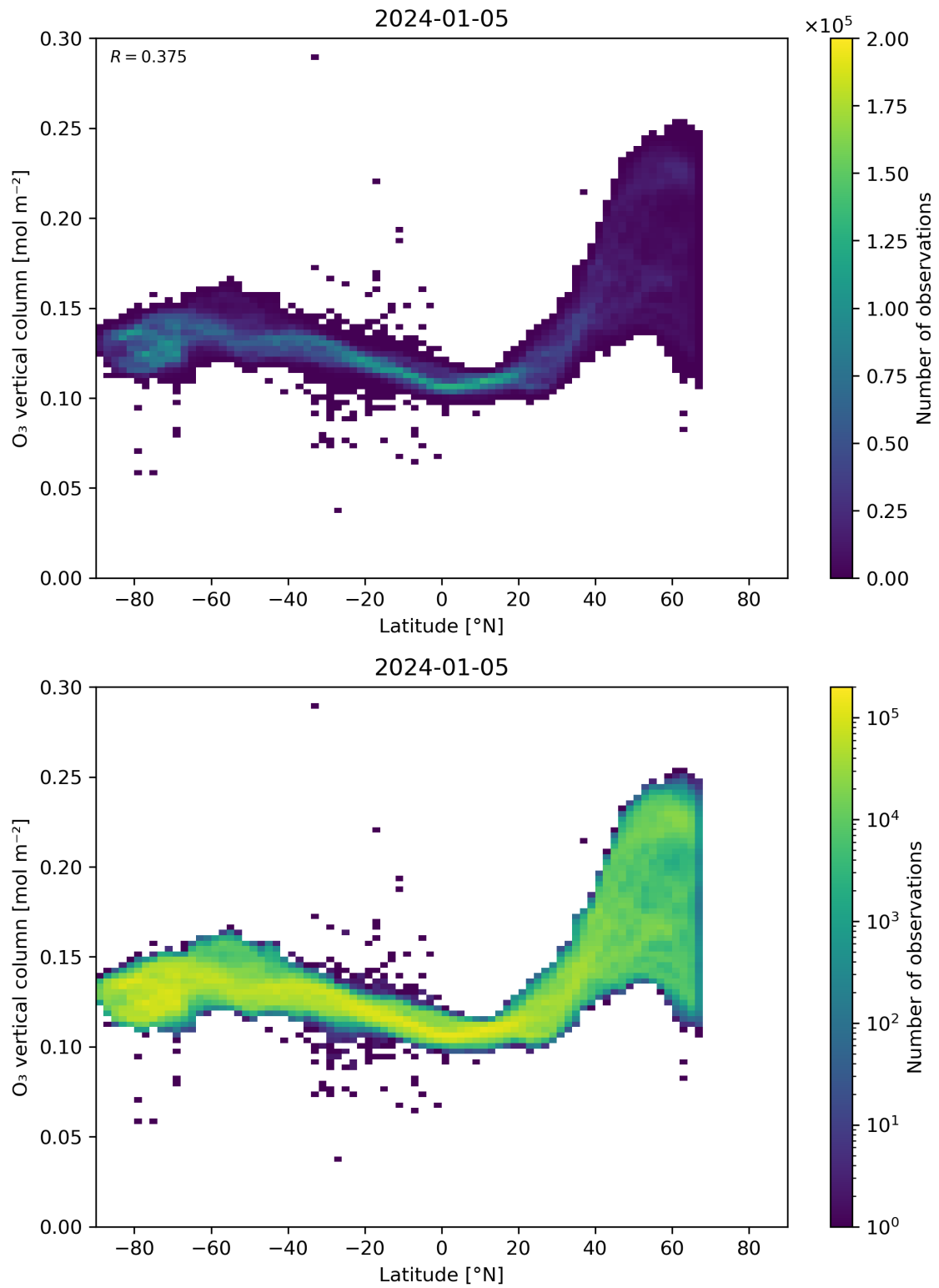
Figure 36: Scatter density plot of “Latitude” against “O 3 vertical column” for 2024-01-05 to 2024-01-06.
