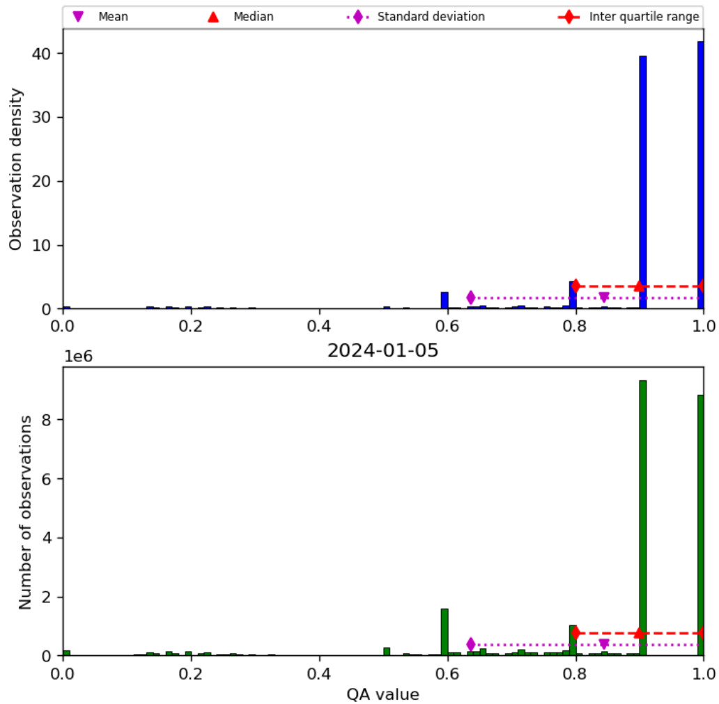
Figure 20: Histogram of “QA value” for 2024-01-05 to 2024-01-06
