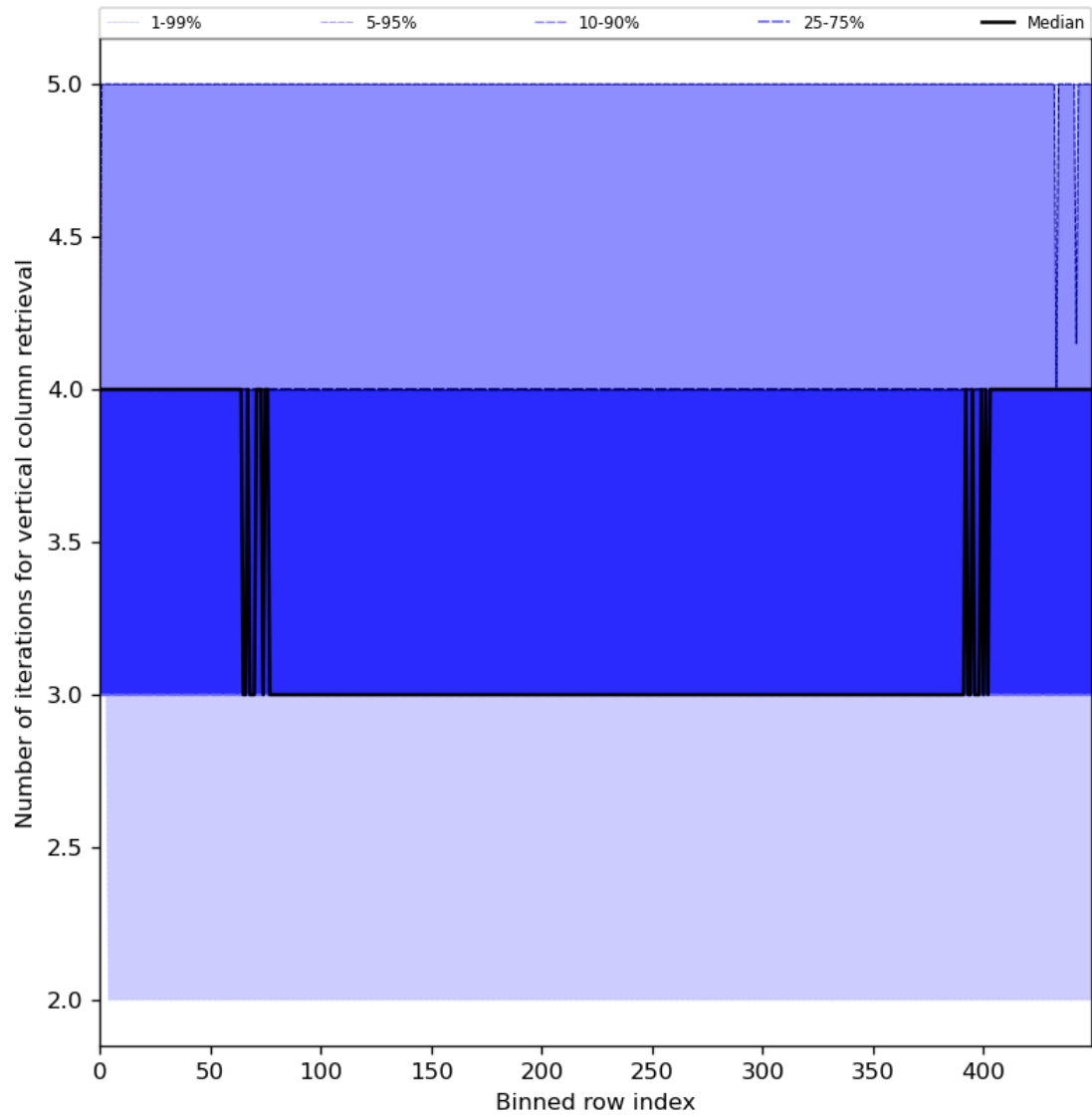
Figure 33: Along track statistics of “Number of iterations for vertical column retrieval” for 2024-01-05 to 2024-01-06
