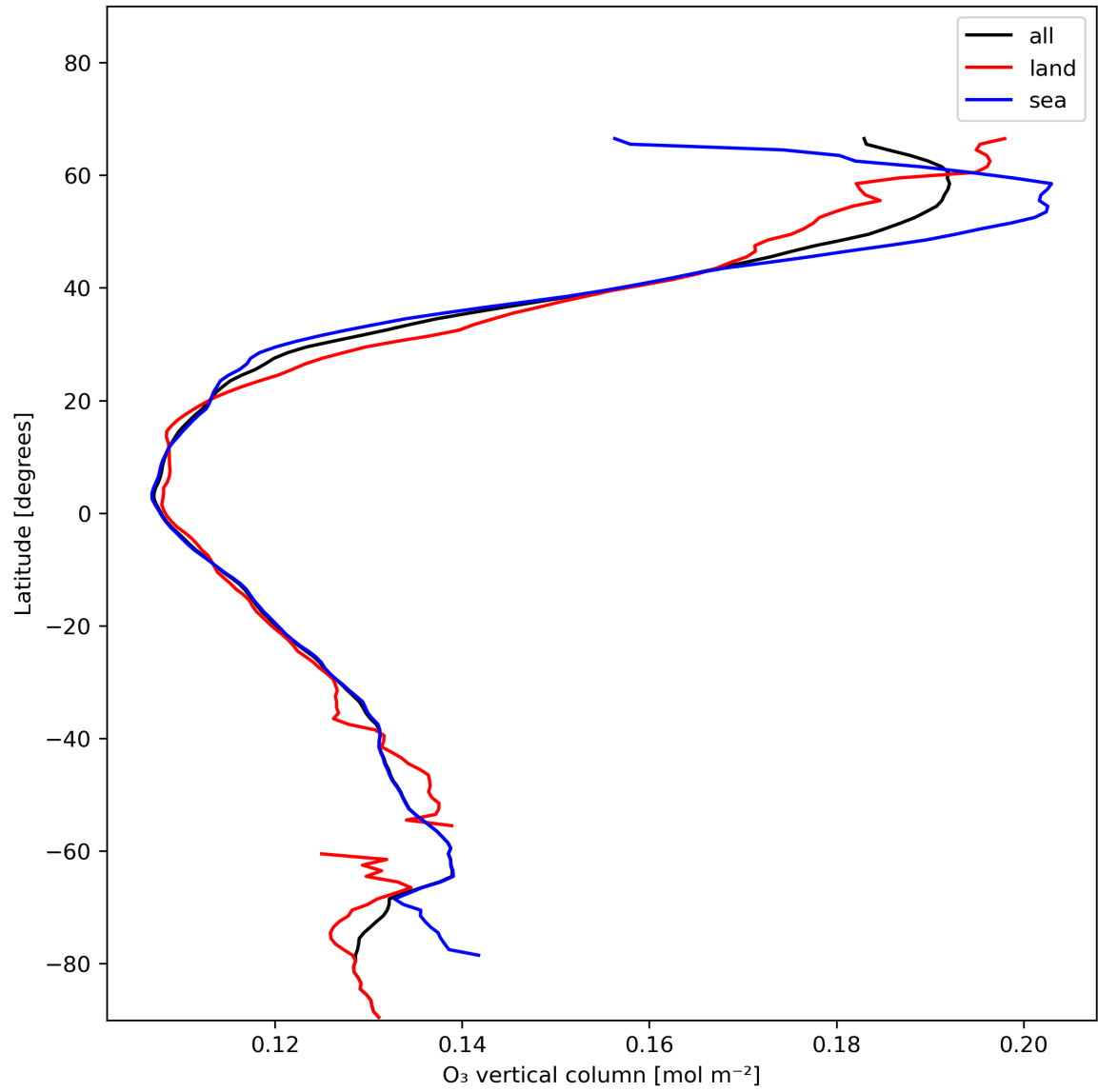
Figure 14: Zonal average of “O 3 vertical column” for 2024-01-05 to 2024-01-06.
