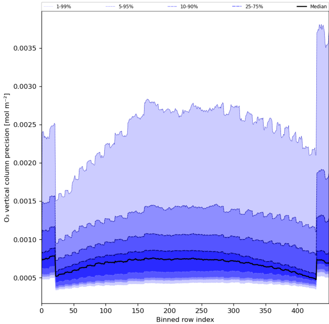
Figure 29: Along track statistics of “O 3 vertical column precision” for 2024-01-05 to 2024-01-06
