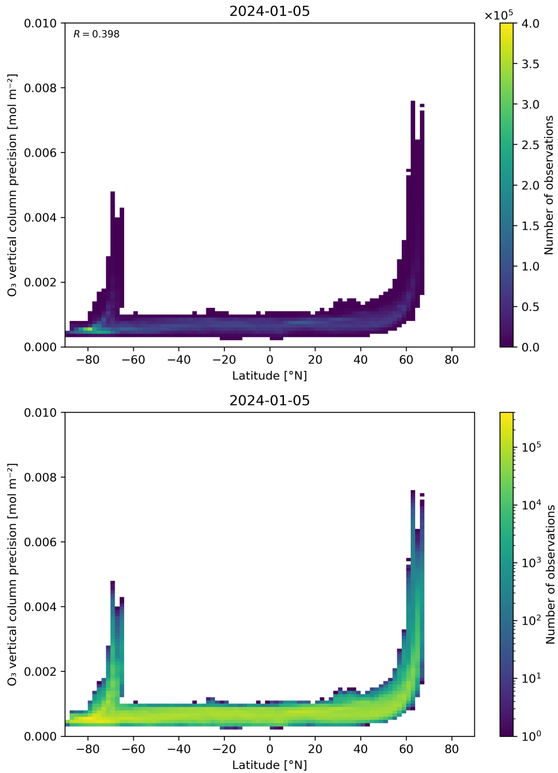
Figure 37: Scatter density plot of “Latitude” against “O 3 vertical column precision” for 2024-01-05 to 2024-01-06.
