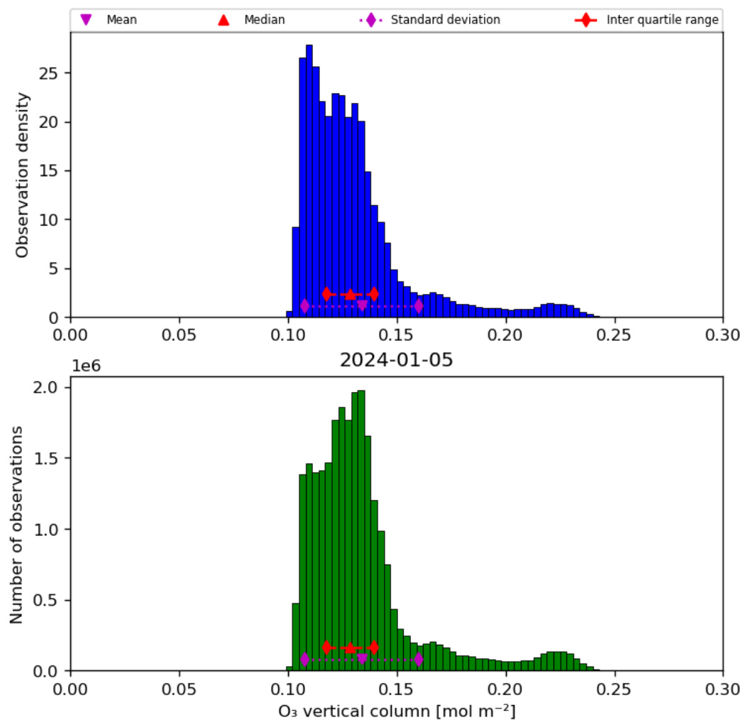
Figure 21: Histogram of “O 3 vertical column” for 2024-01-05 to 2024-01-06
