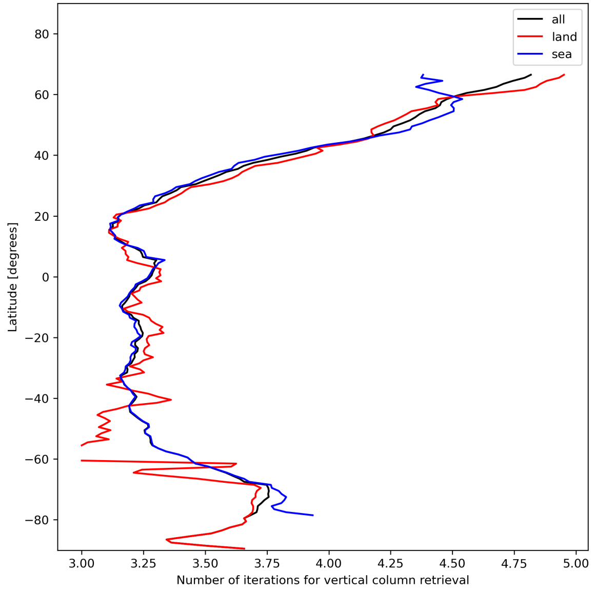
Figure 19: Zonal average of “Number of iterations for vertical column retrieval” for 2024-01-05 to 2024-01-07.
