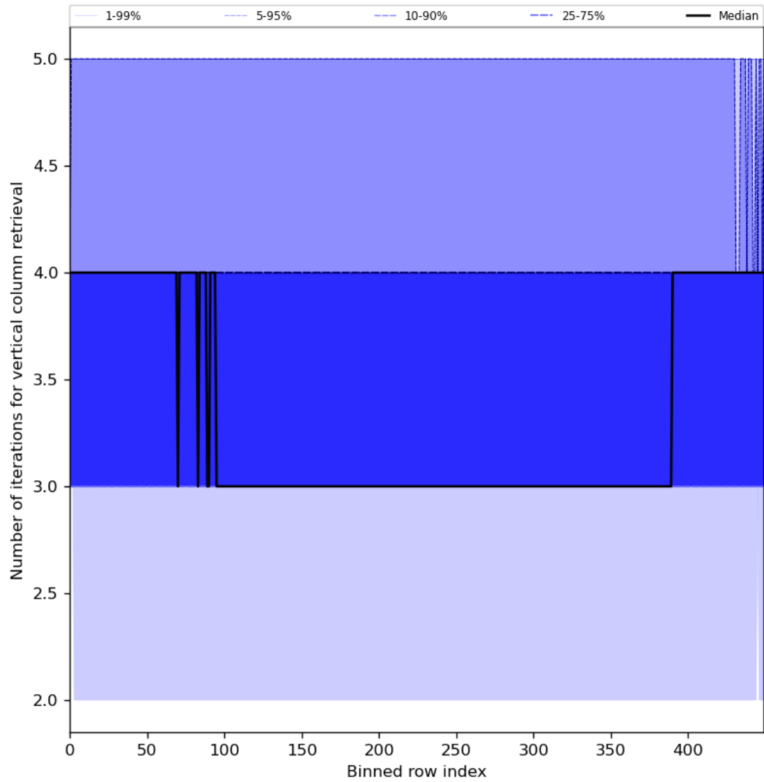
Figure 33: Along track statistics of “Number of iterations for vertical column retrieval” for 2024-01-05 to 2024-01-07
