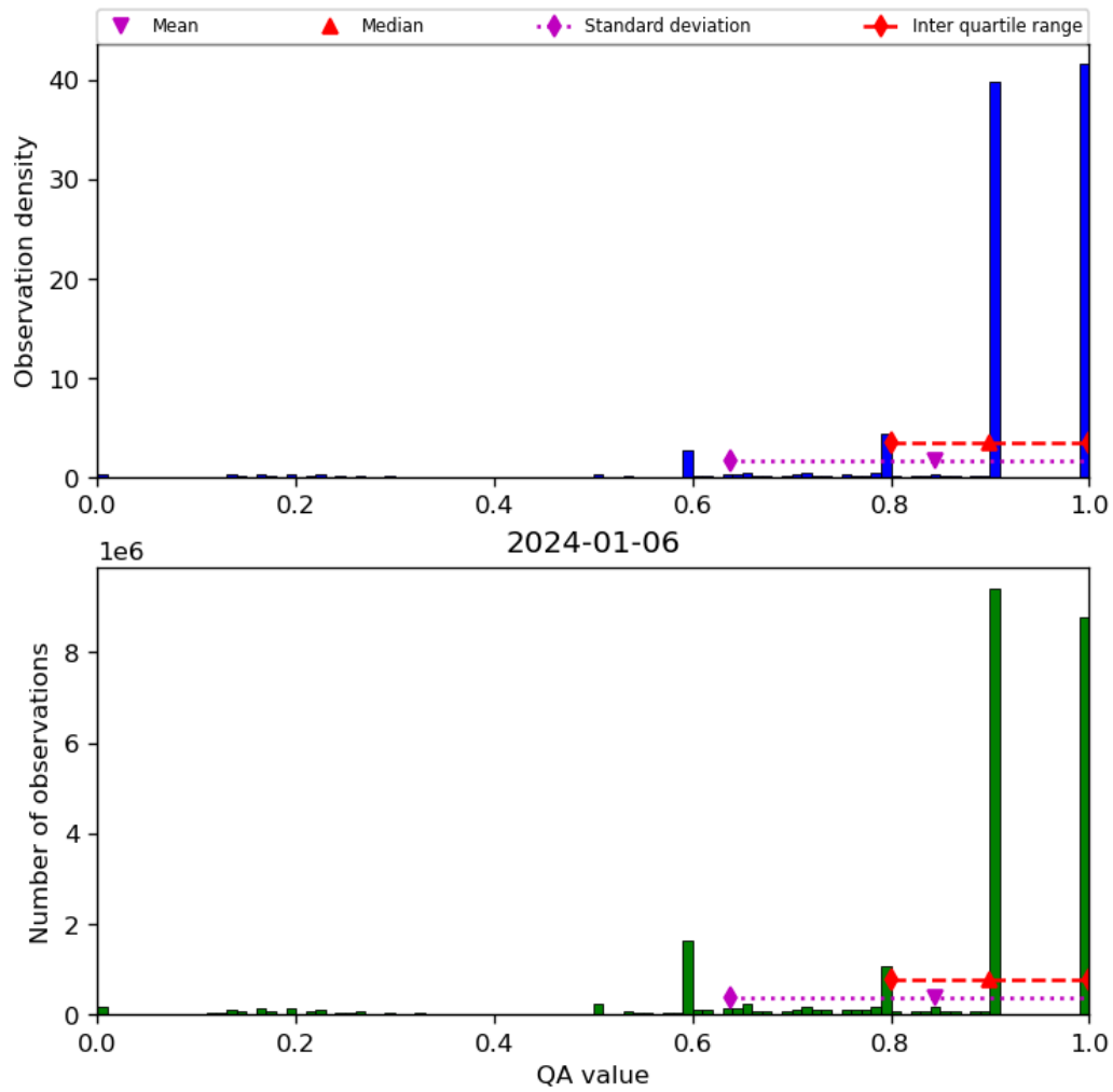
Figure 20: Histogram of “QA value” for 2024-01-05 to 2024-01-07
