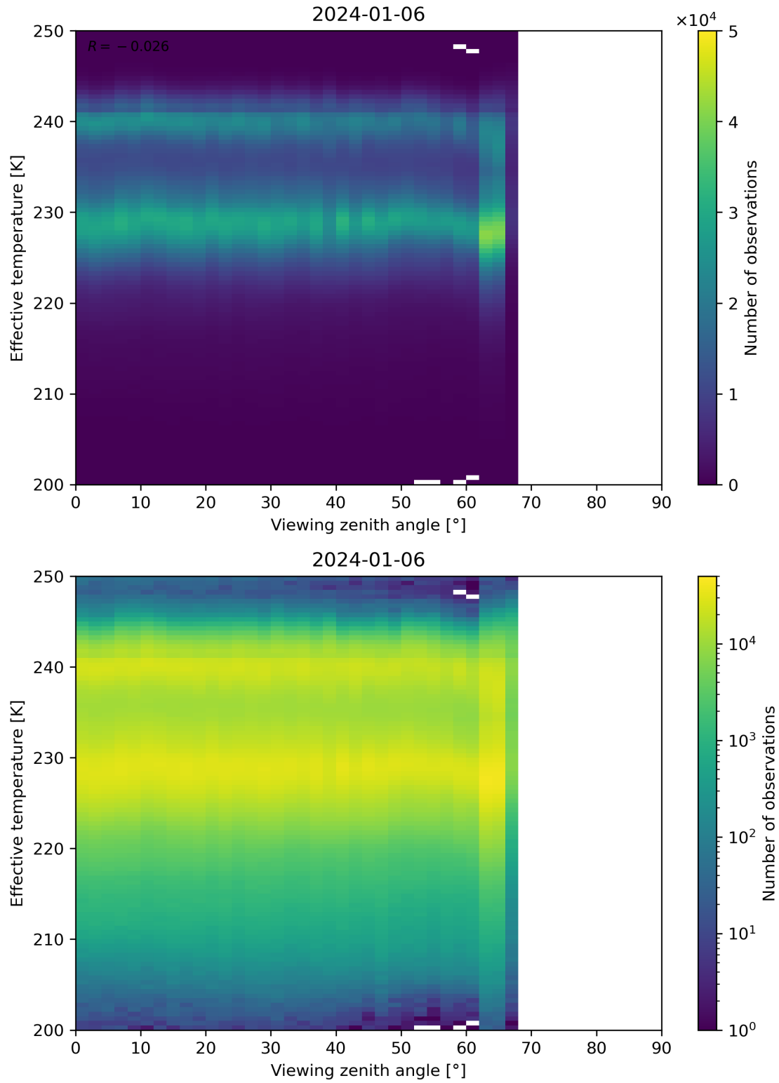
Figure 50: Scatter density plot of “Viewing zenith angle” against “Effective temperature” for 2024-01-05 to 2024-01-07.
