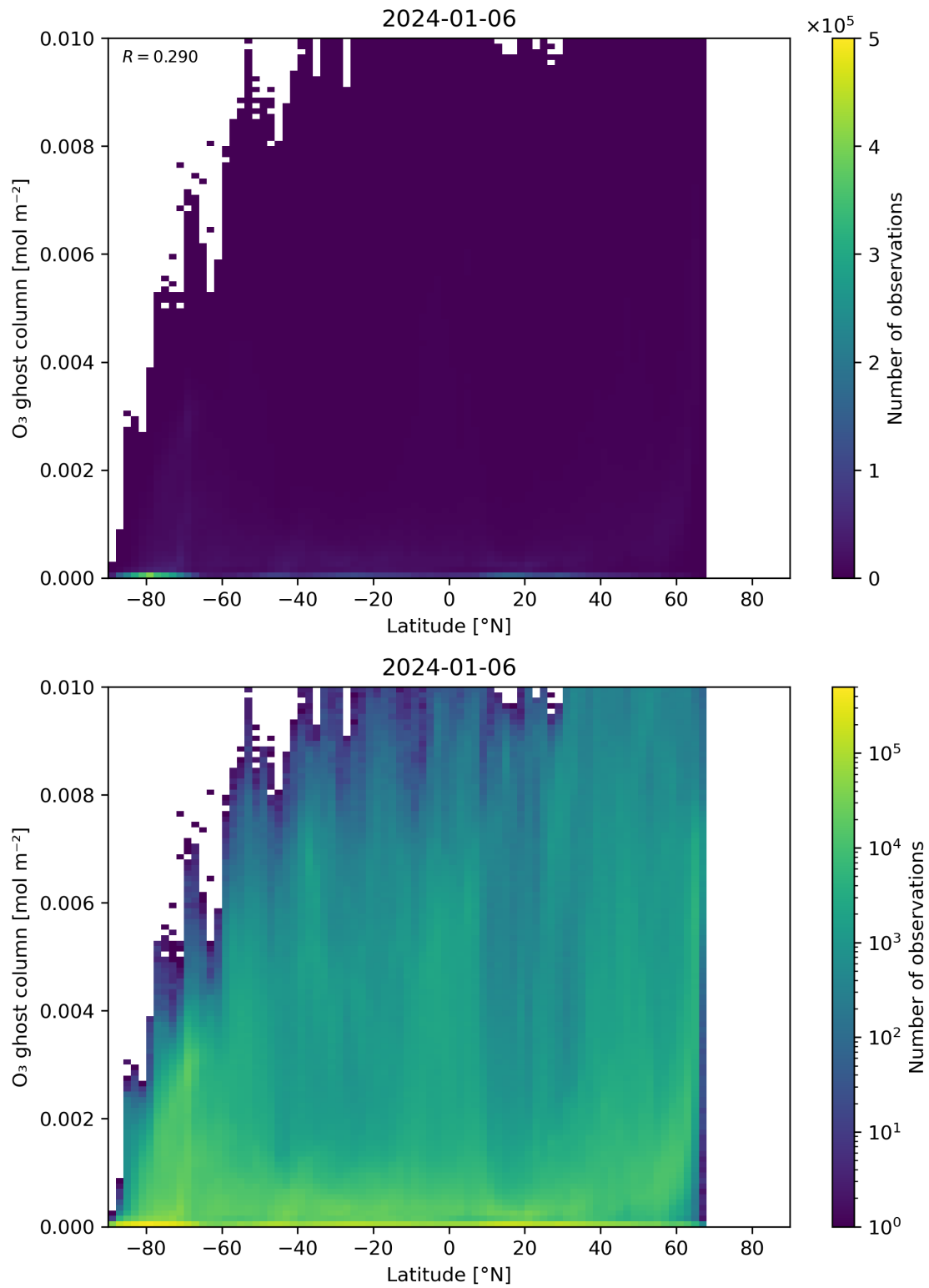
Figure 35: Scatter density plot of “Latitude” against “O 3 ghost column” for 2024-01-05 to 2024-01-07.
