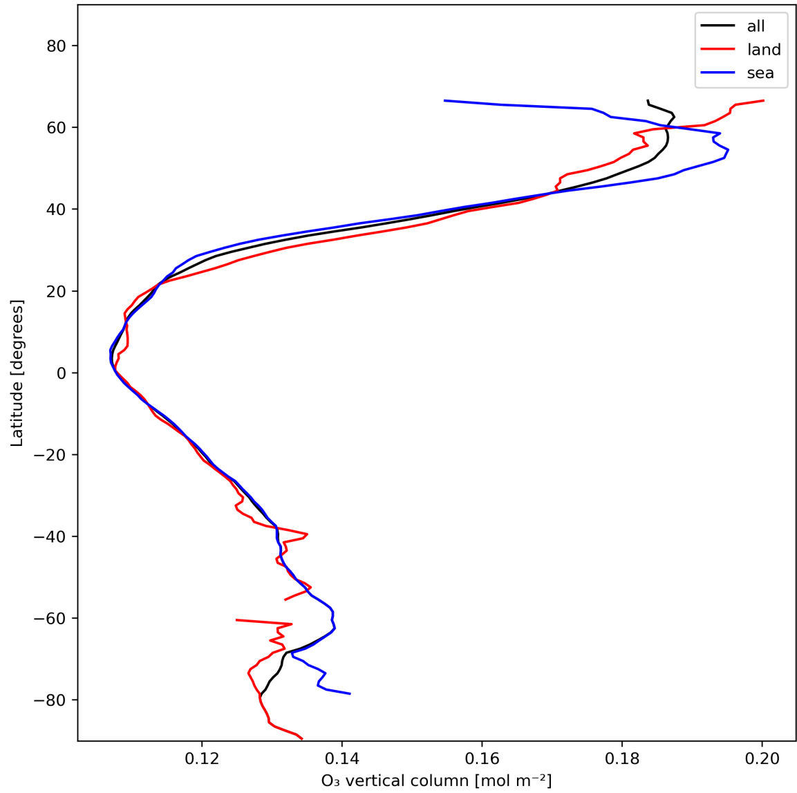
Figure 14: Zonal average of “O 3 vertical column” for 2024-01-05 to 2024-01-07.
