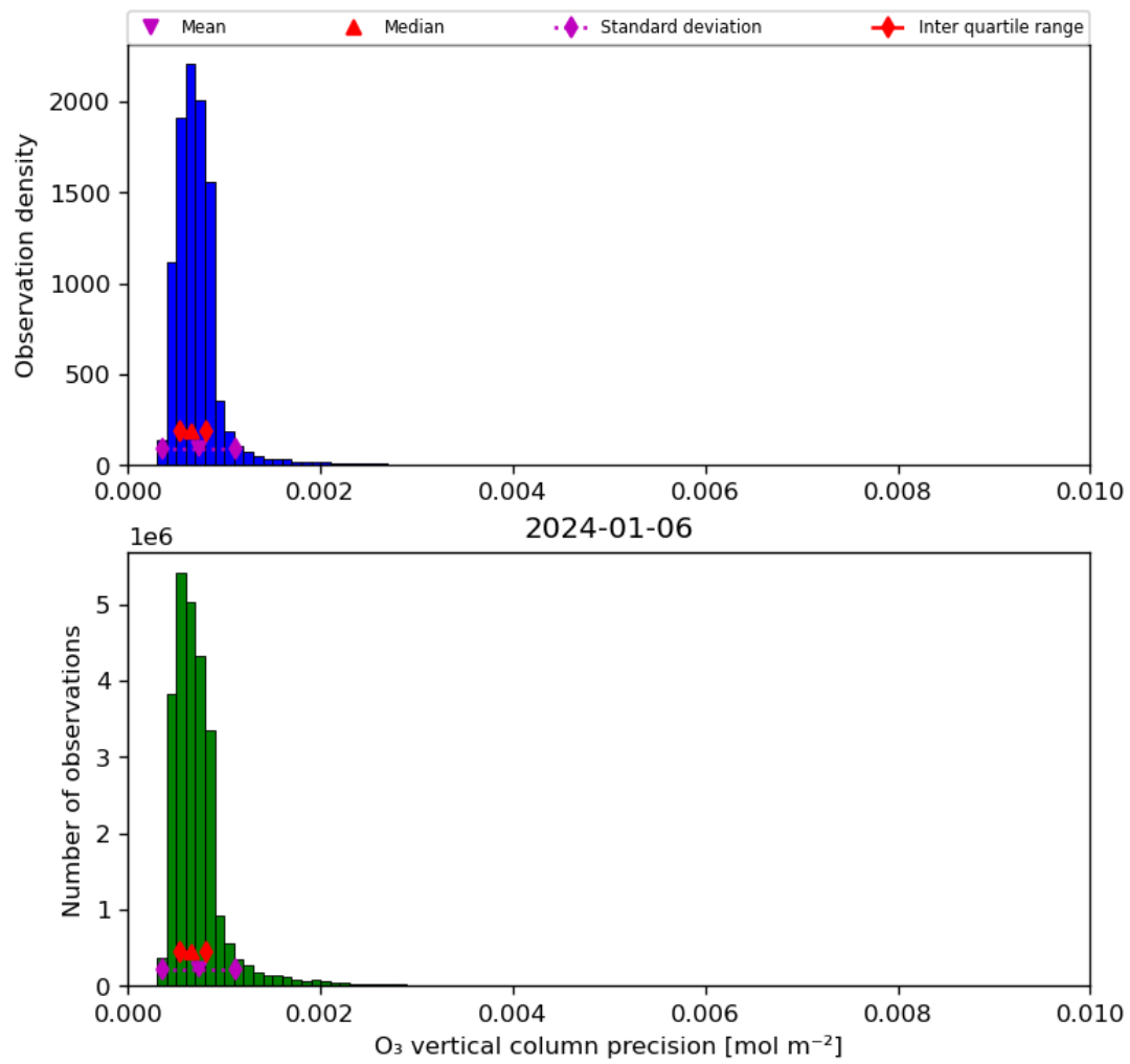
Figure 22: Histogram of “O 3 vertical column precision” for 2024-01-05 to 2024-01-07
