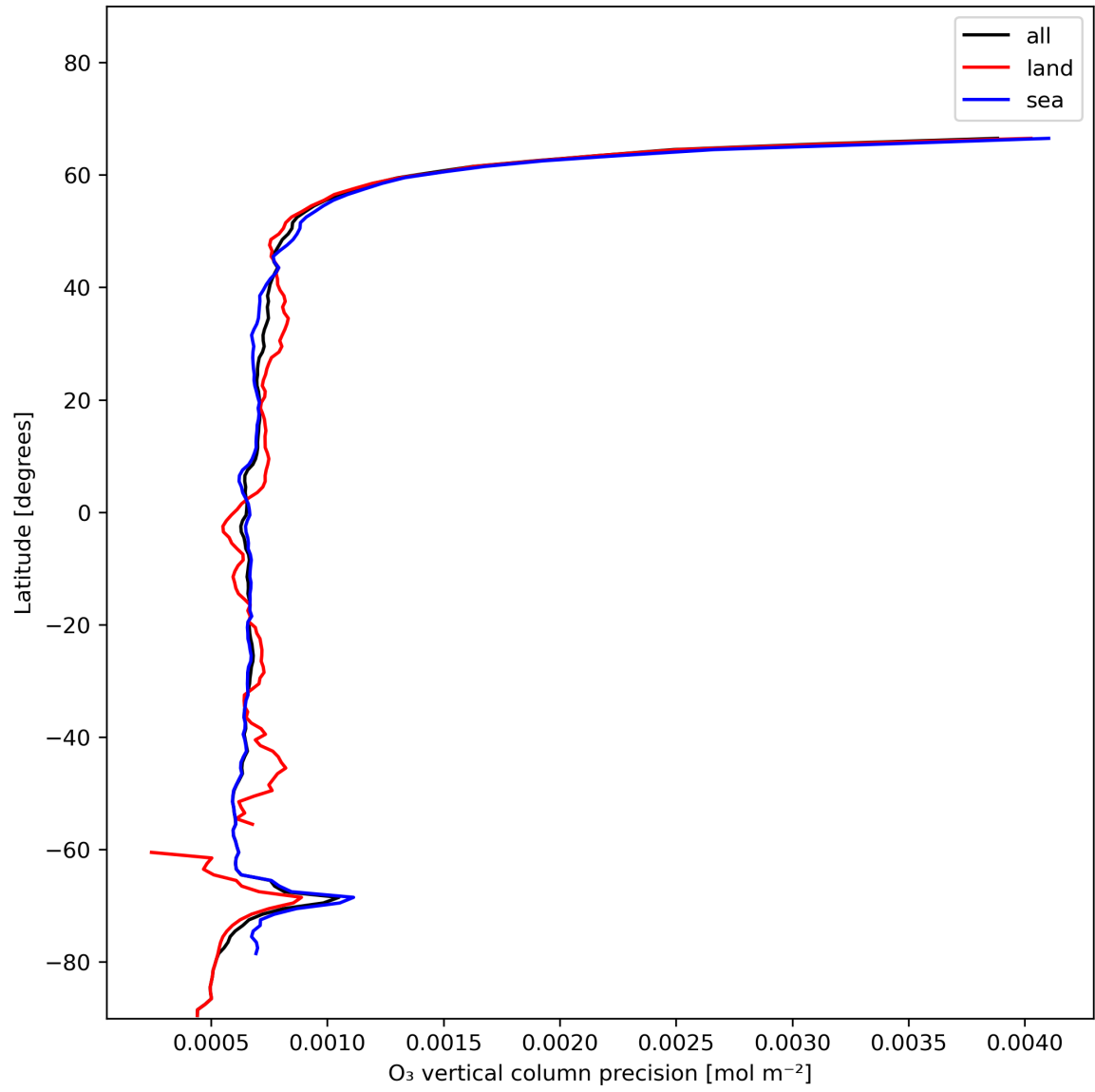
Figure 15: Zonal average of “O 3 vertical column precision” for 2024-01-05 to 2024-01-07.
