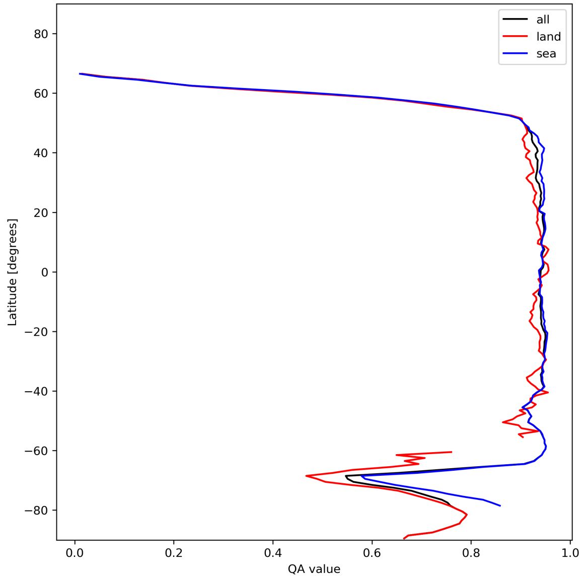
Figure 13: Zonal average of “QA value” for 2024-01-05 to 2024-01-07.
