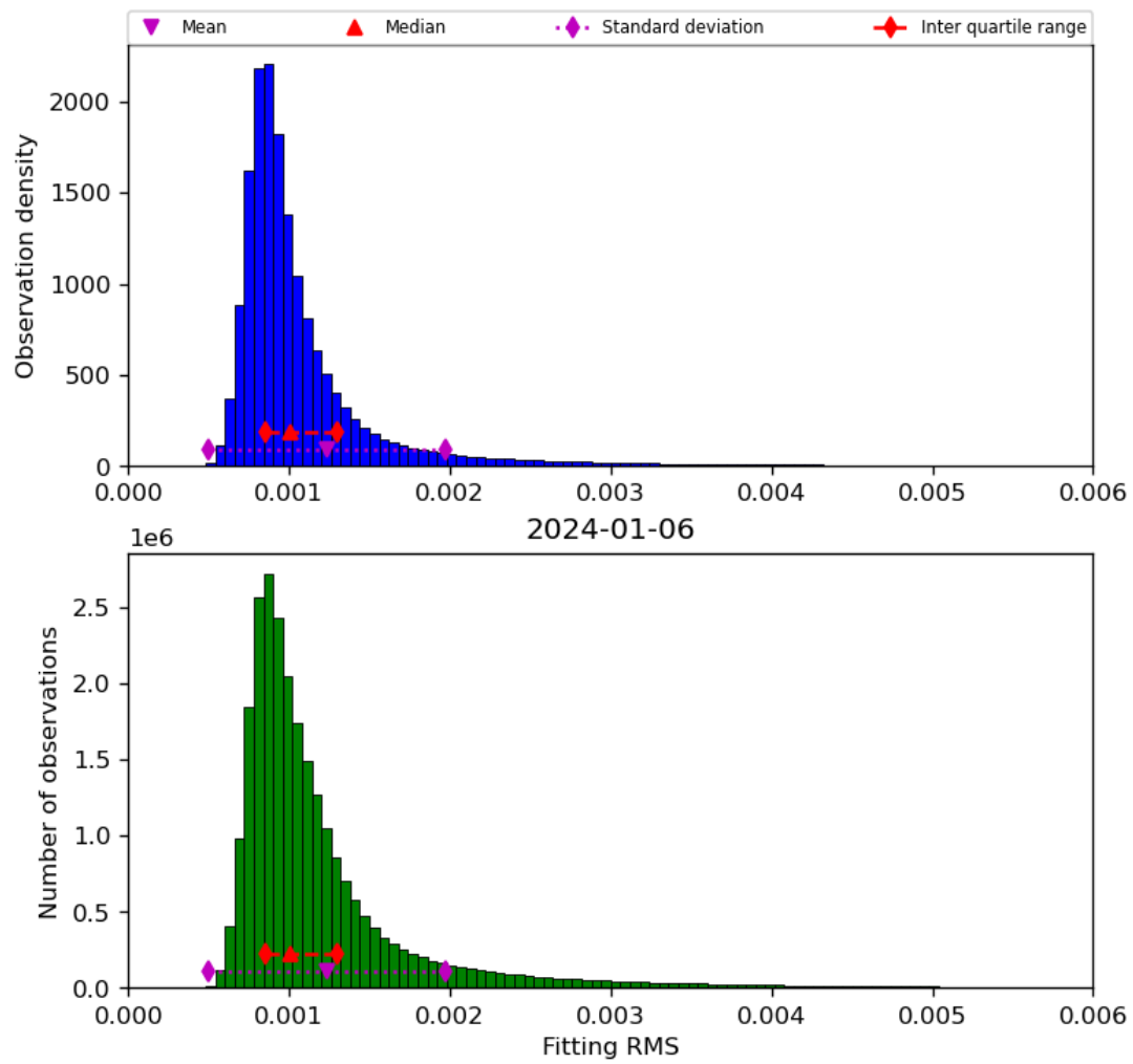
Figure 23: Histogram of “Fitting RMS” for 2024-01-05 to 2024-01-07
