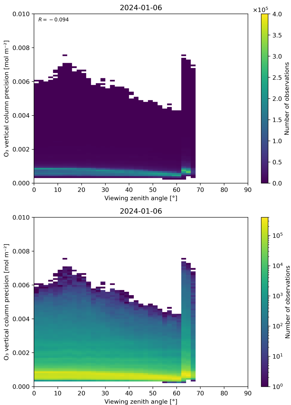
Figure 53: Scatter density plot of “Viewing zenith angle” against “O 3 vertical column precision” for 2024-01-05 to 2024-01-07.
