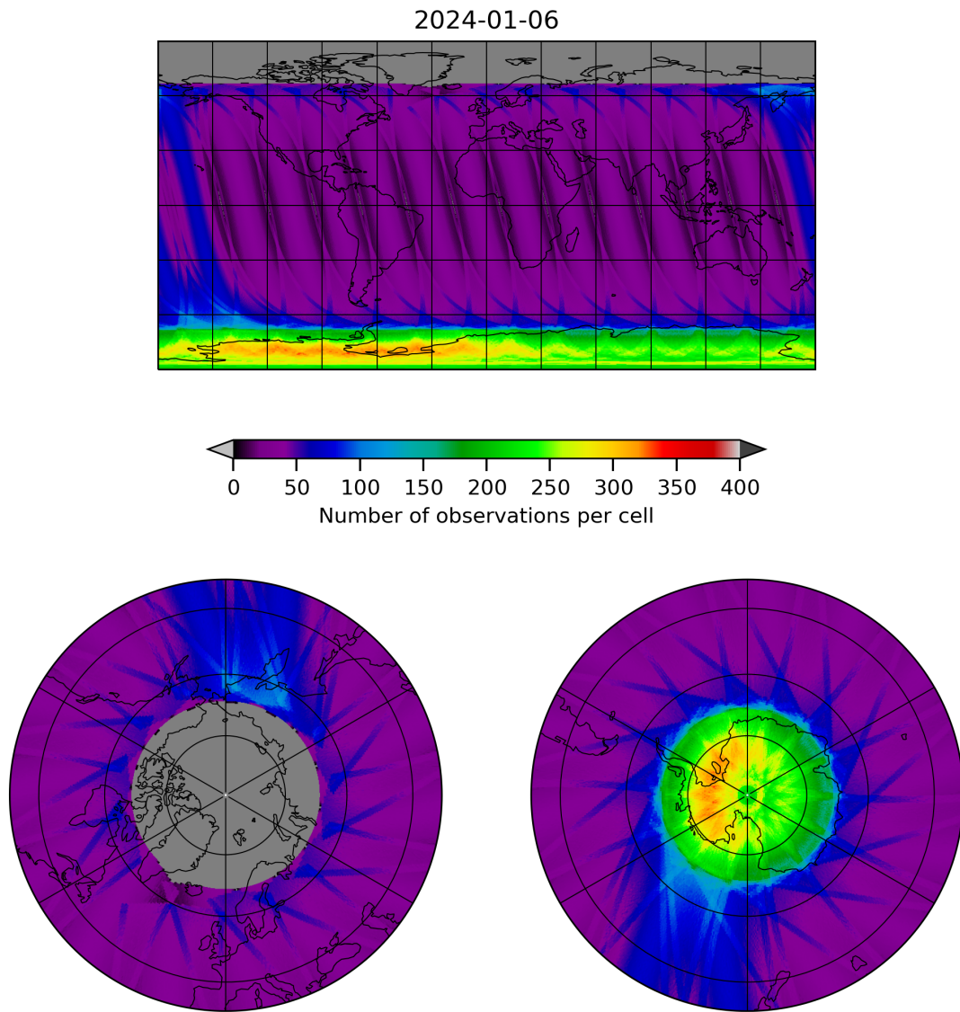
Figure 12: Map of the number of observations for 2024-01-05 to 2024-01-07
