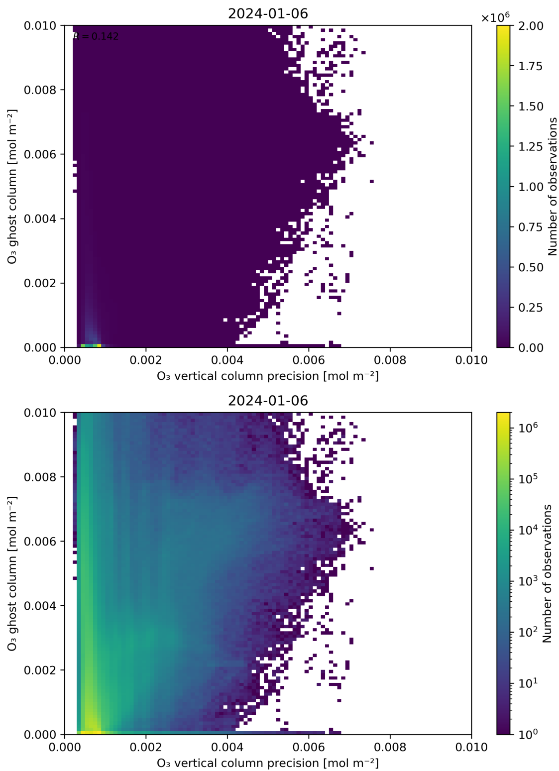
Figure 43: Scatter density plot of “ \text{O}_3 vertical column precision” against “ \text{O}_3 ghost column” for 2024-01-05 to 2024-01-07.
