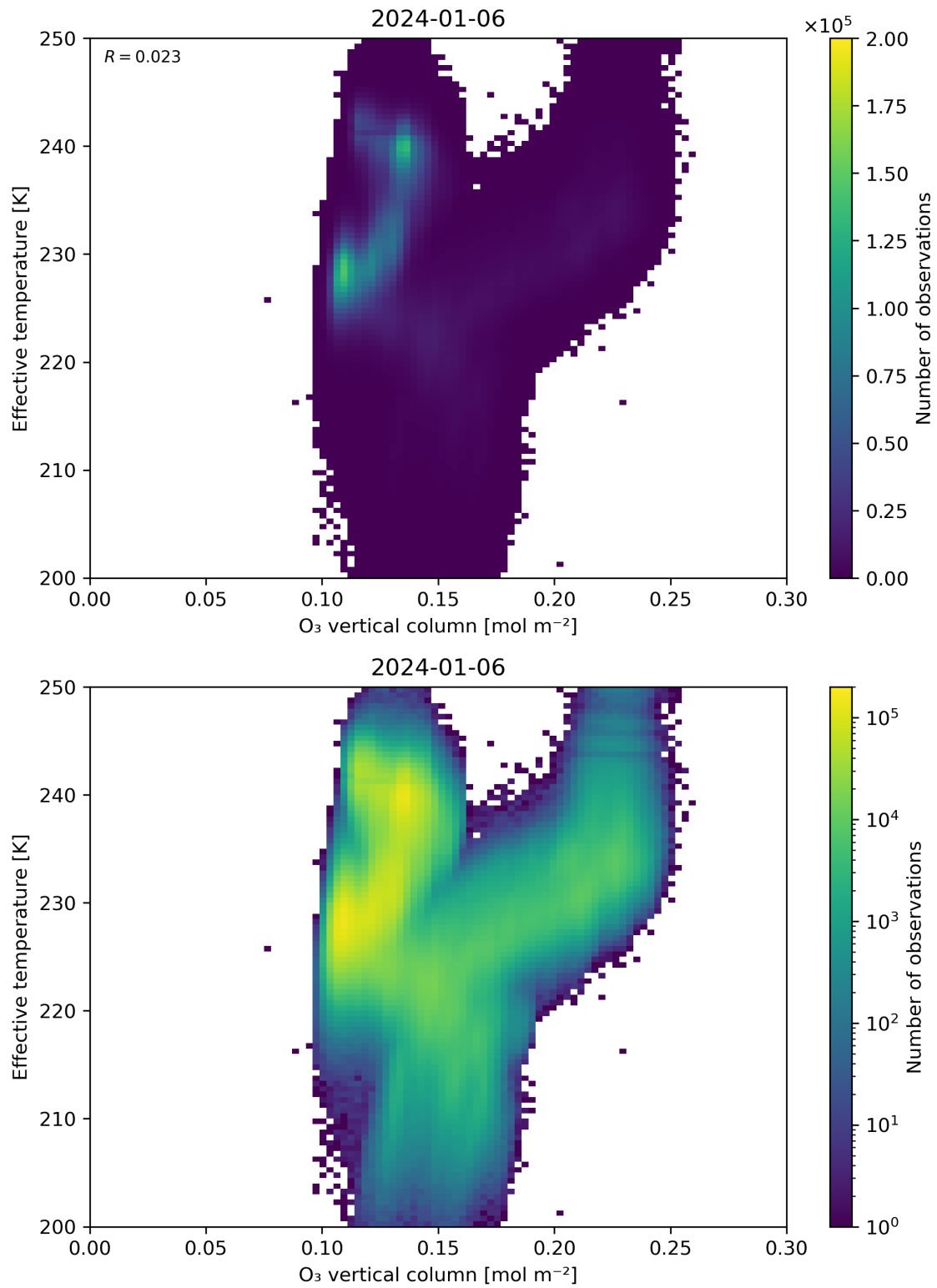
Figure 39: Scatter density plot of “O 3 vertical column” against “Effective temperature” for 2024-01-05 to 2024-01-07.
