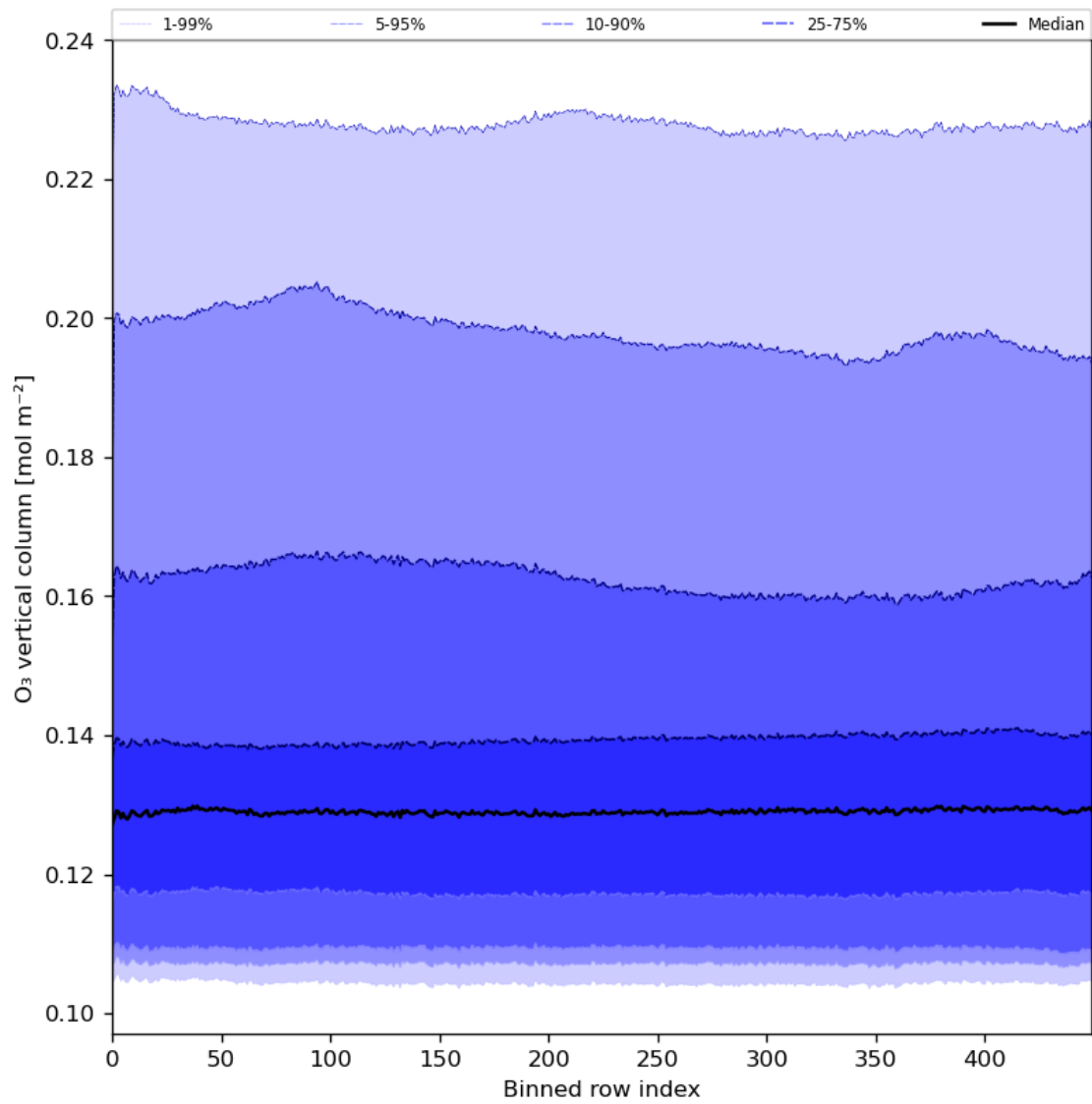
Figure 28: Along track statistics of “O 3 vertical column” for 2024-01-05 to 2024-01-07
