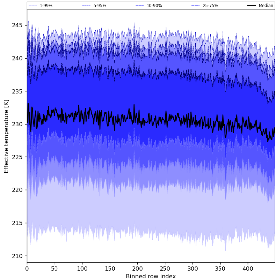
Figure 31: Along track statistics of “Effective temperature” for 2024-01-05 to 2024-01-07
