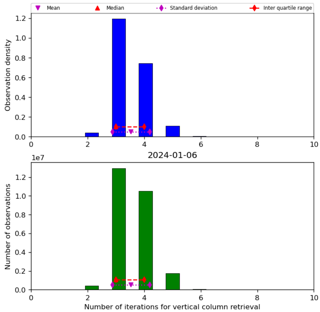
Figure 26: Histogram of “Number of iterations for vertical column retrieval” for 2024-01-05 to 2024-01-07
