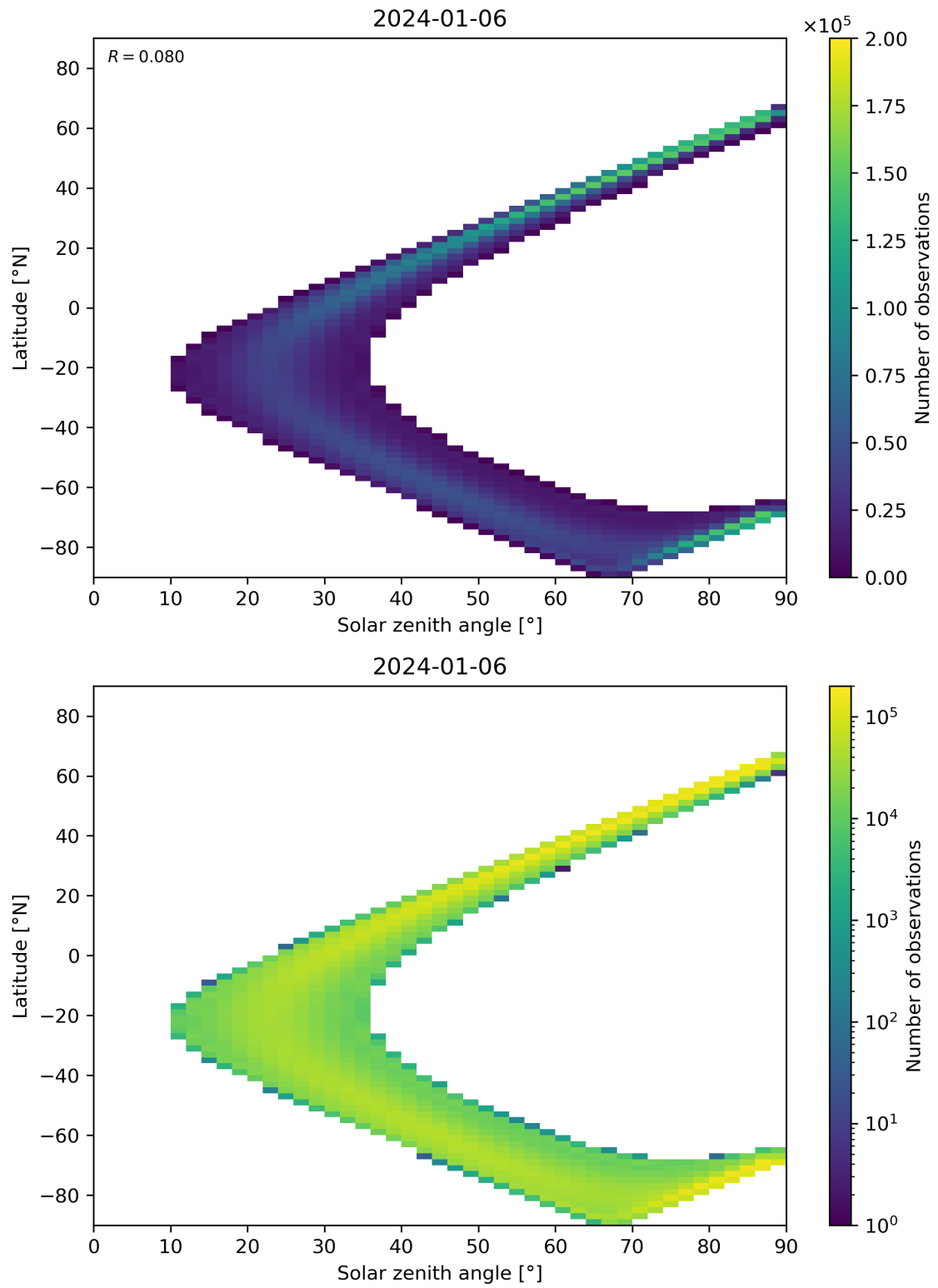
Figure 44: Scatter density plot of “Solar zenith angle” against “Latitude” for 2024-01-05 to 2024-01-07.
