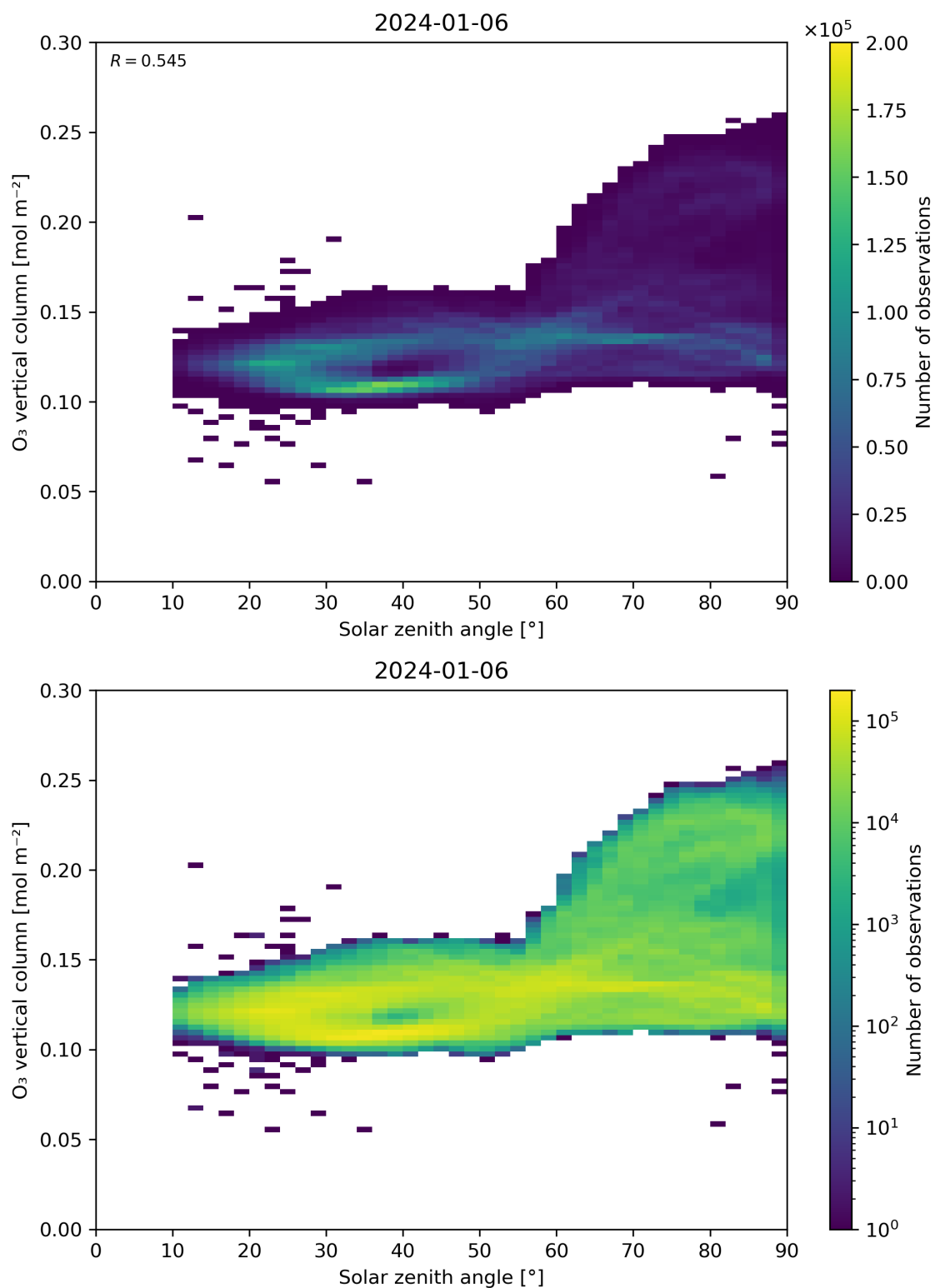
Figure 47: Scatter density plot of “Solar zenith angle” against “O 3 vertical column” for 2024-01-05 to 2024-01-07.
