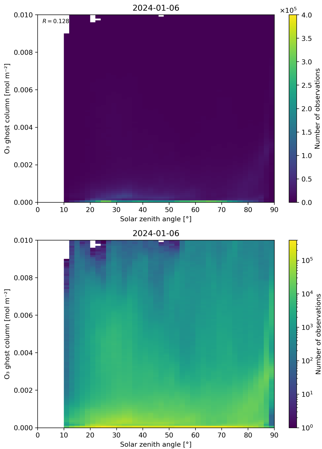
Figure 46: Scatter density plot of “Solar zenith angle” against “O 3 ghost column” for 2024-01-05 to 2024-01-07.
