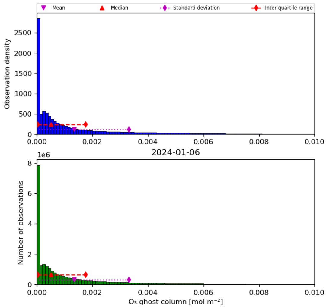
Figure 25: Histogram of “O 3 ghost column” for 2024-01-05 to 2024-01-07
