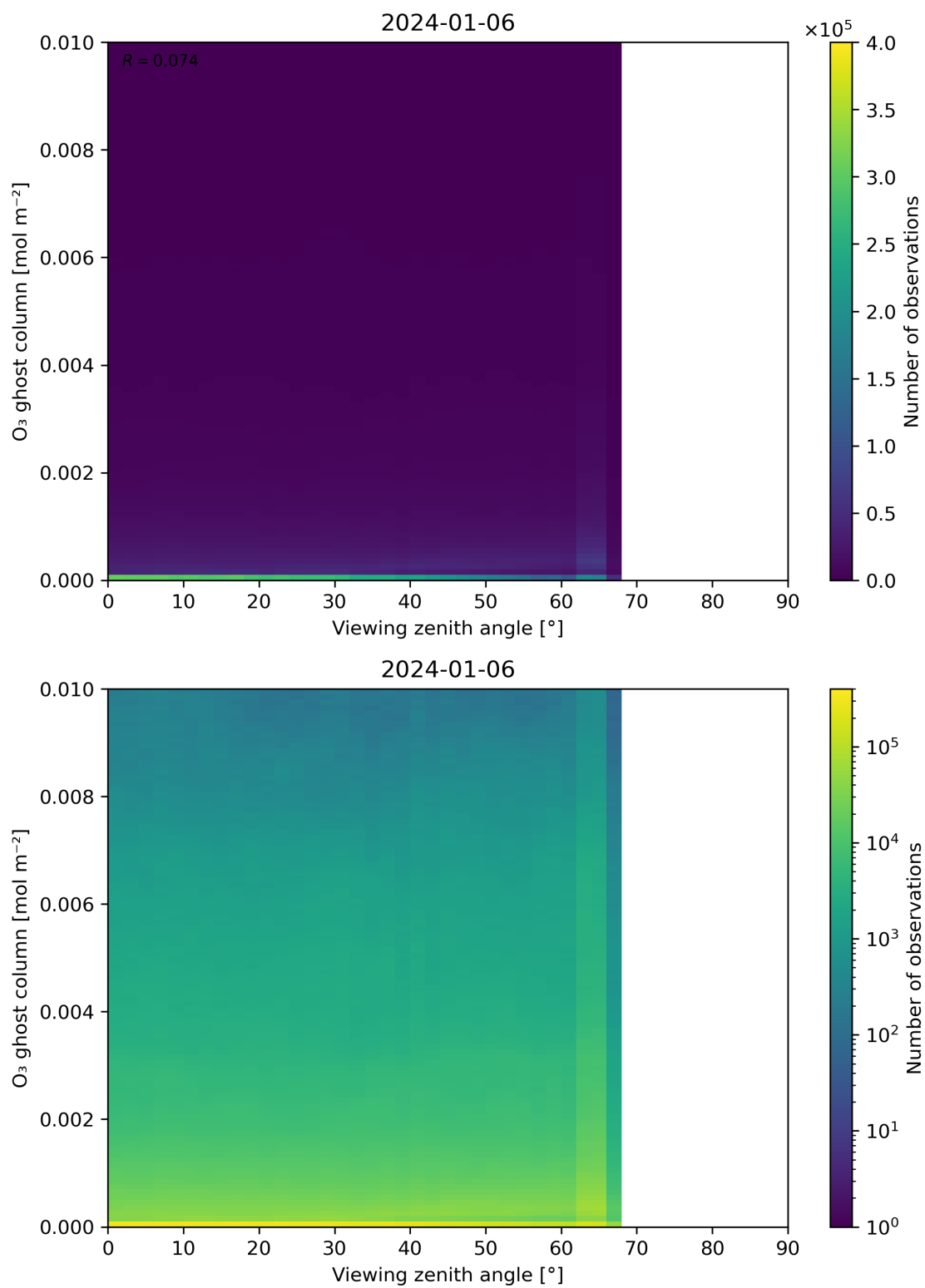
Figure 51: Scatter density plot of “Viewing zenith angle” against “O 3 ghost column” for 2024-01-05 to 2024-01-07.
