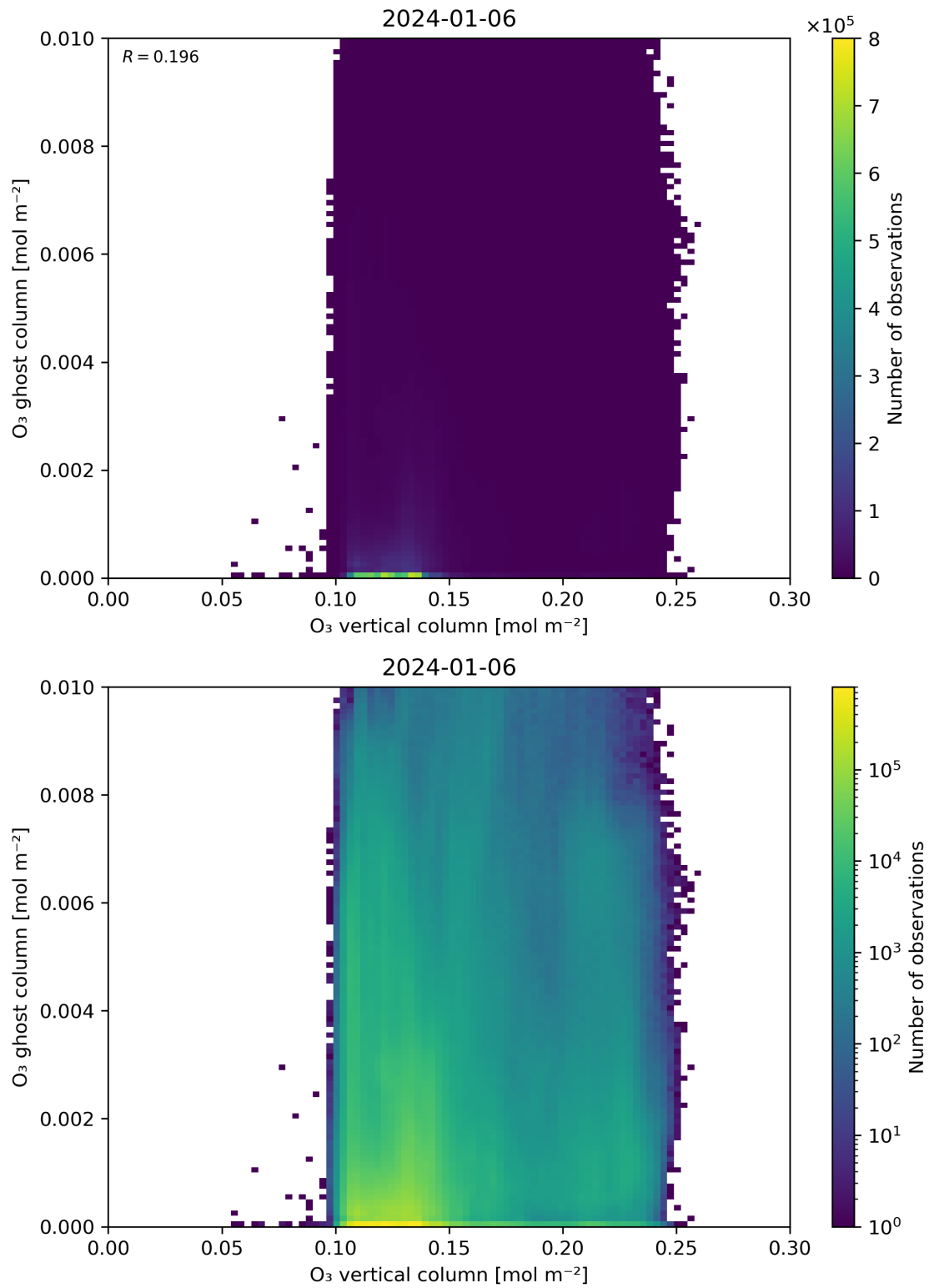
Figure 40: Scatter density plot of “O 3 vertical column” against “O 3 ghost column” for 2024-01-05 to 2024-01-07.
