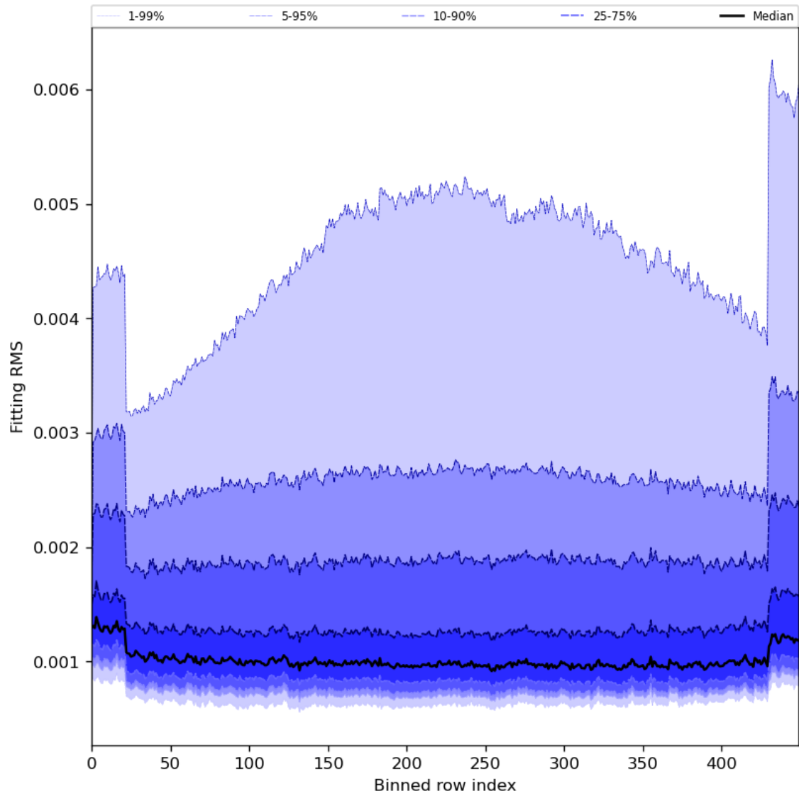
Figure 30: Along track statistics of “Fitting RMS” for 2024-01-05 to 2024-01-07
