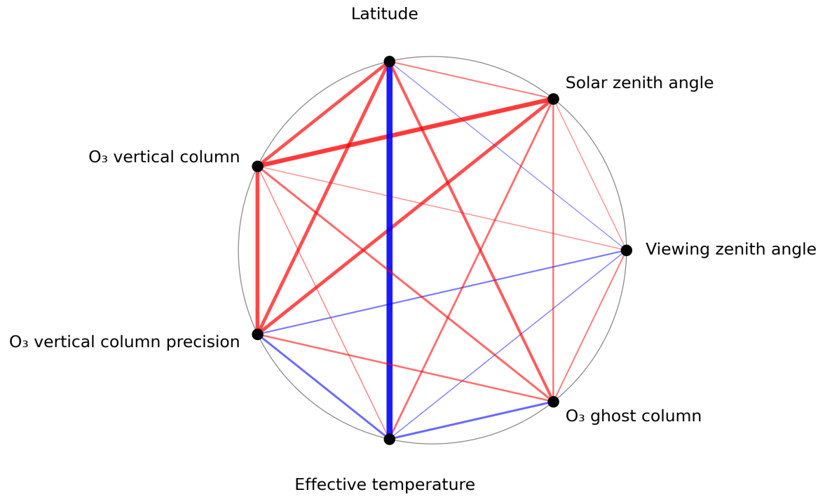
Figure 1: Map of correlation graph for 2024-01-05 to 2024-01-07.
