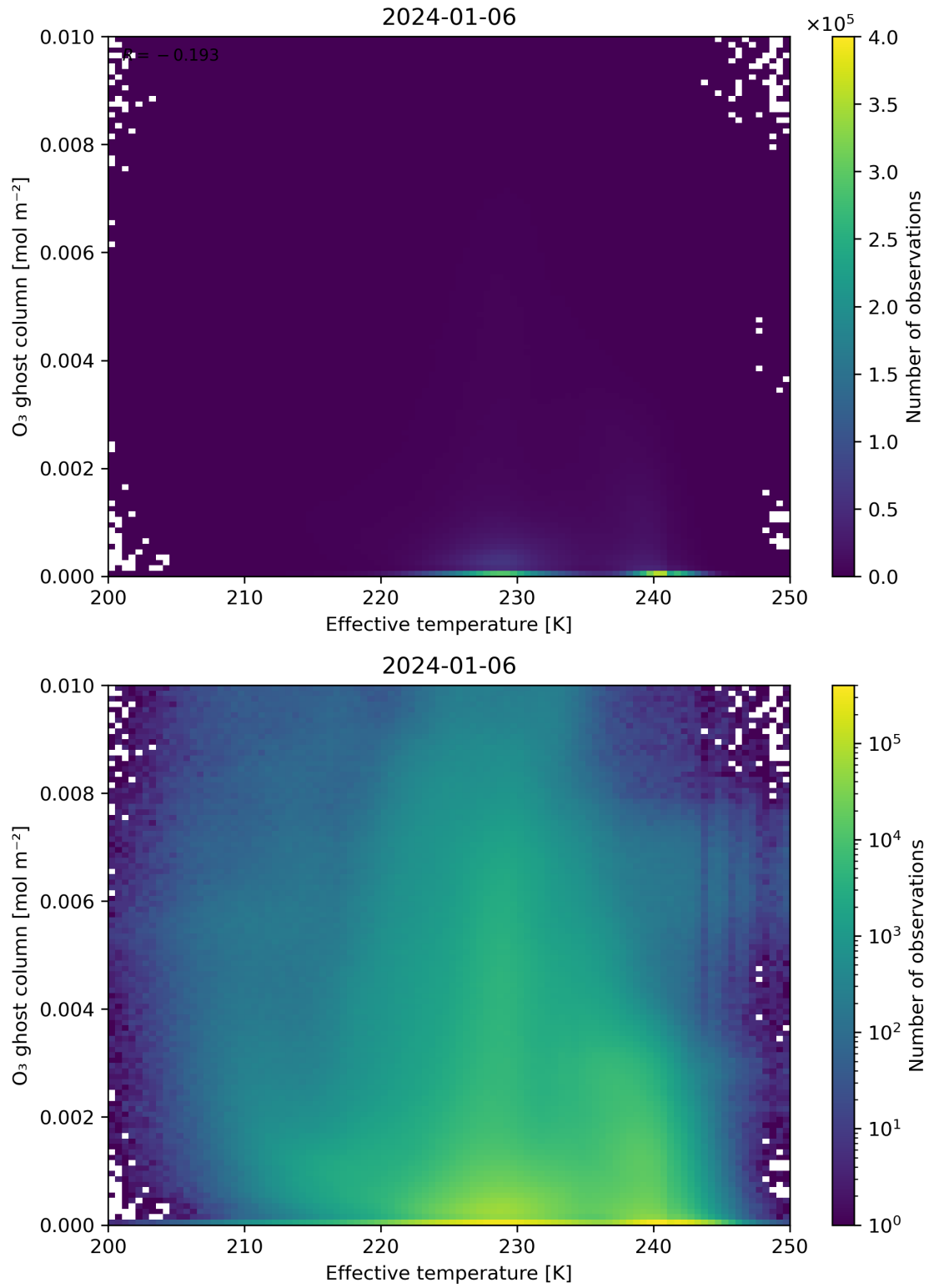
Figure 38: Scatter density plot of “Effective temperature” against “O 3 ghost column” for 2024-01-05 to 2024-01-07.
