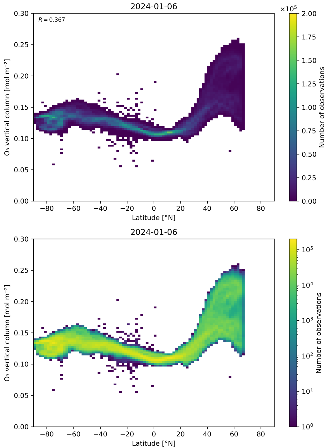
Figure 36: Scatter density plot of “Latitude” against “O 3 vertical column” for 2024-01-05 to 2024-01-07.
