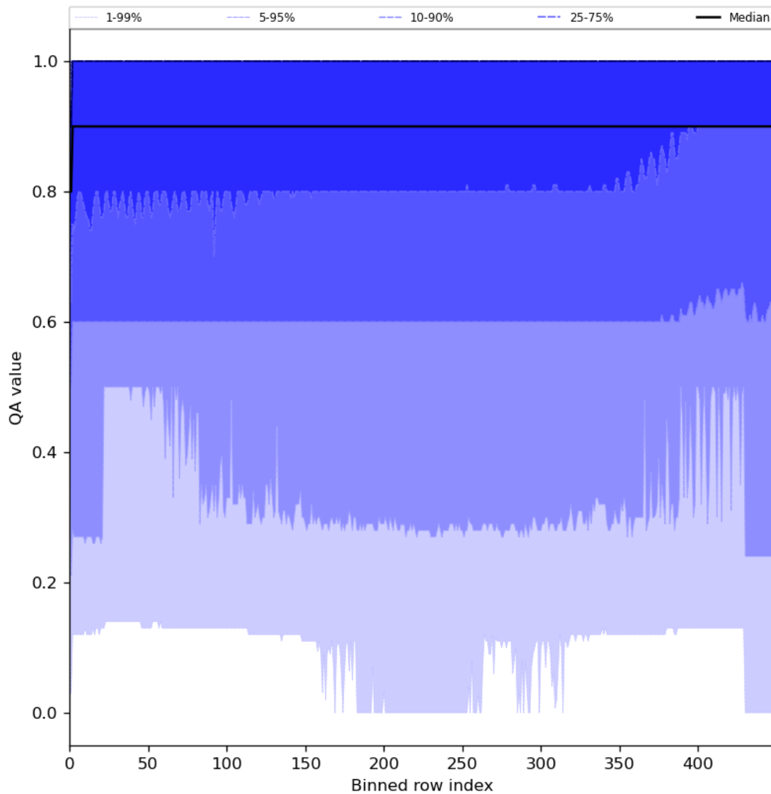
Figure 27: Along track statistics of “QA value” for 2024-01-05 to 2024-01-07
