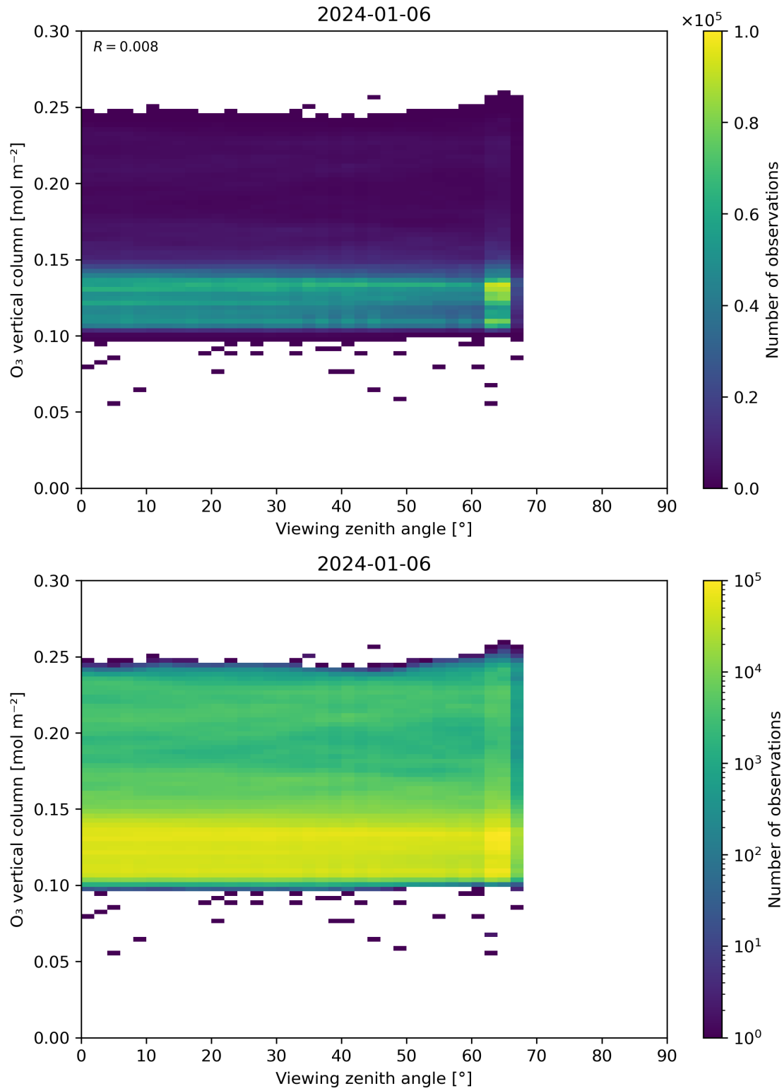
Figure 52: Scatter density plot of “Viewing zenith angle” against “O 3 vertical column” for 2024-01-05 to 2024-01-07.
