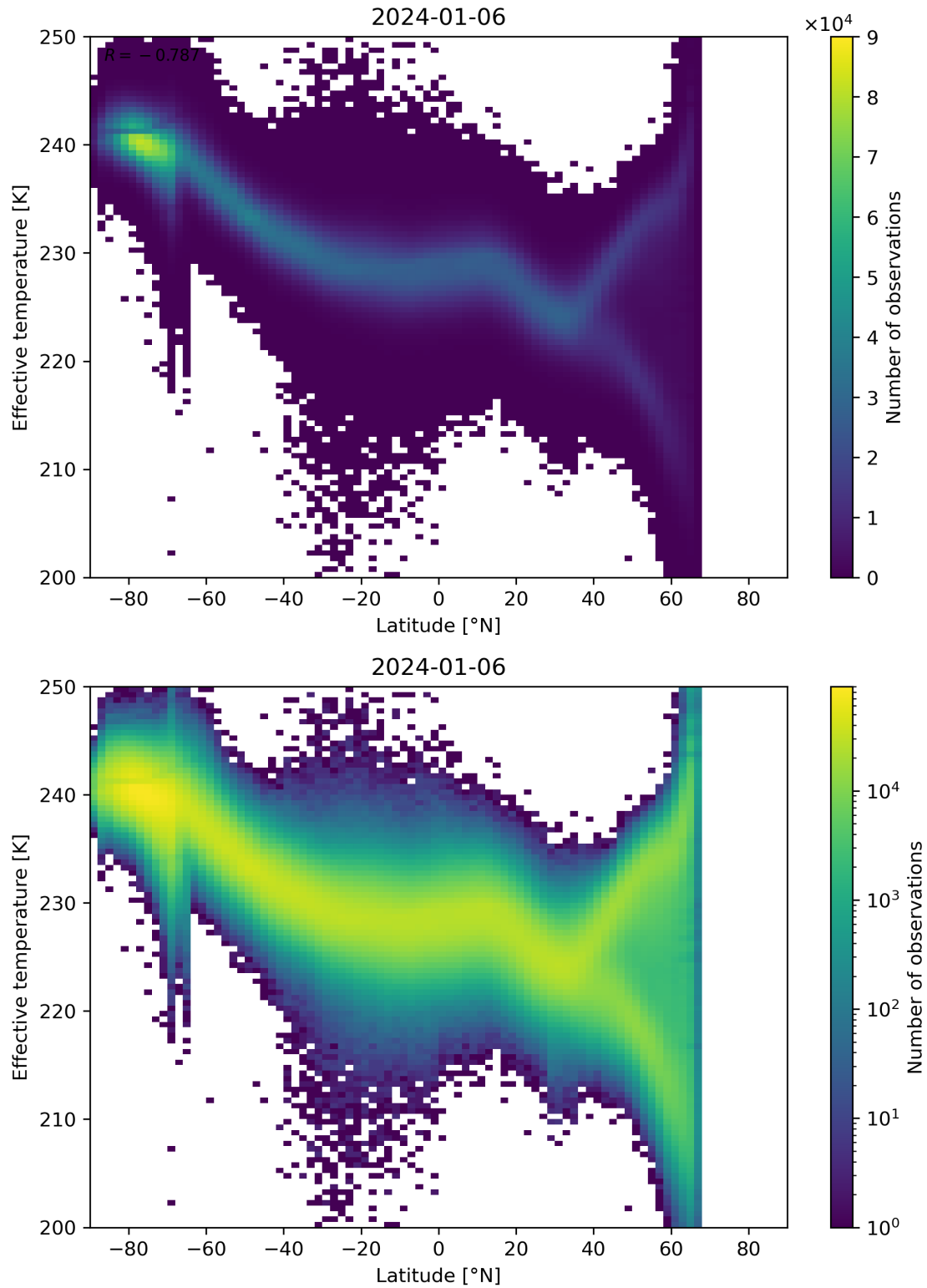
Figure 34: Scatter density plot of “Latitude” against “Effective temperature” for 2024-01-05 to 2024-01-07.
