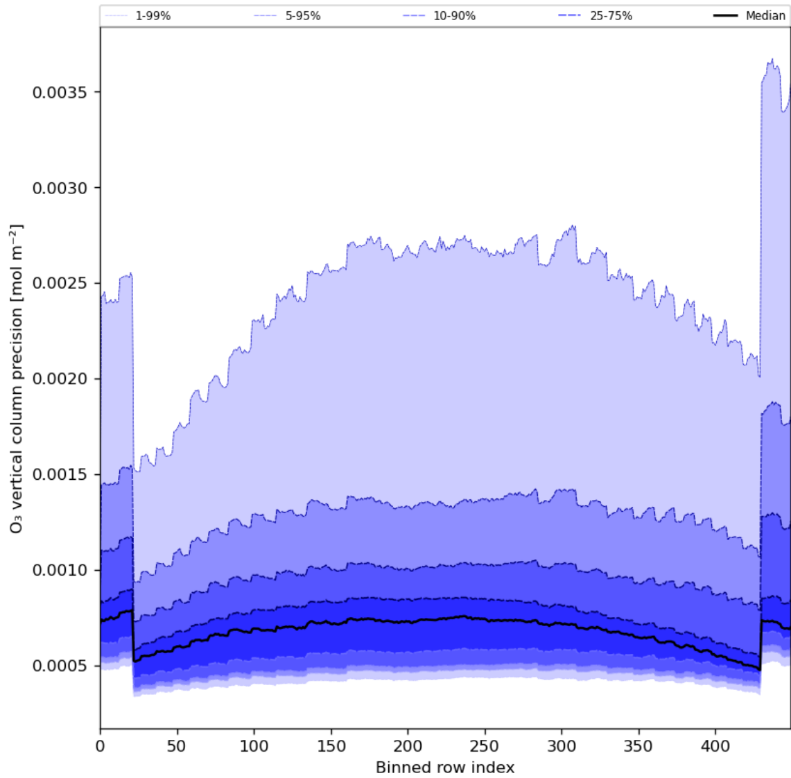
Figure 29: Along track statistics of “O 3 vertical column precision” for 2024-01-05 to 2024-01-07
