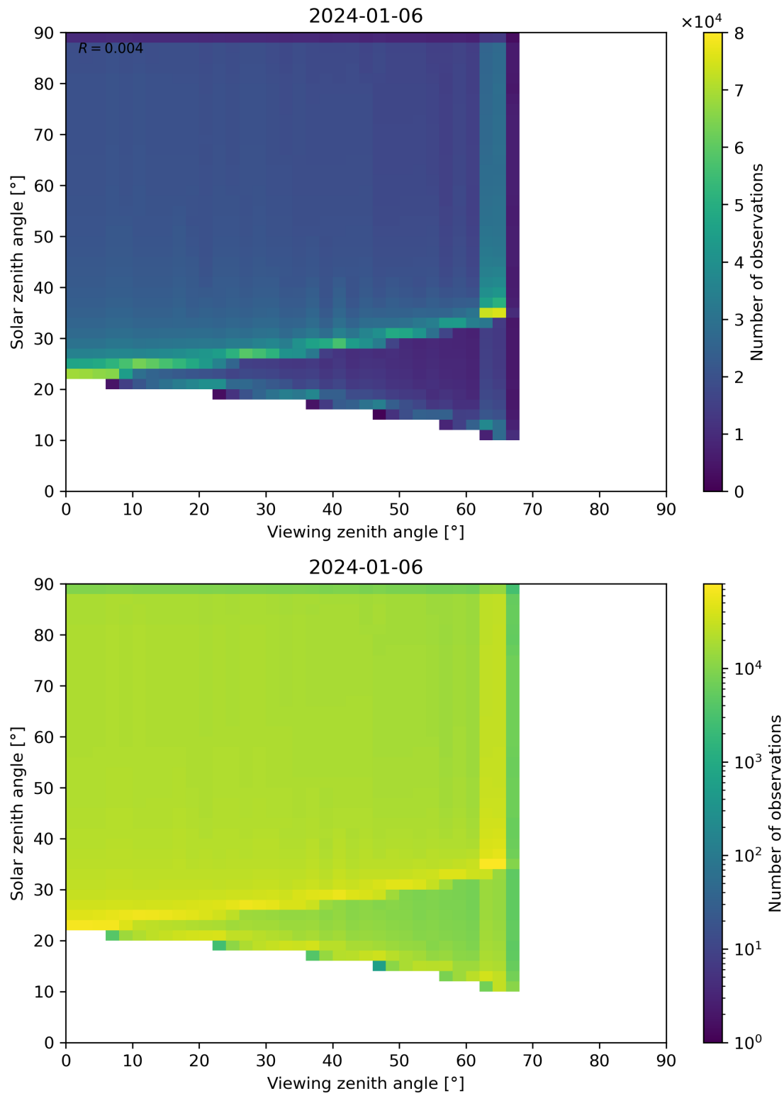
Figure 54: Scatter density plot of “Viewing zenith angle” against “Solar zenith angle” for 2024-01-05 to 2024-01-07.
