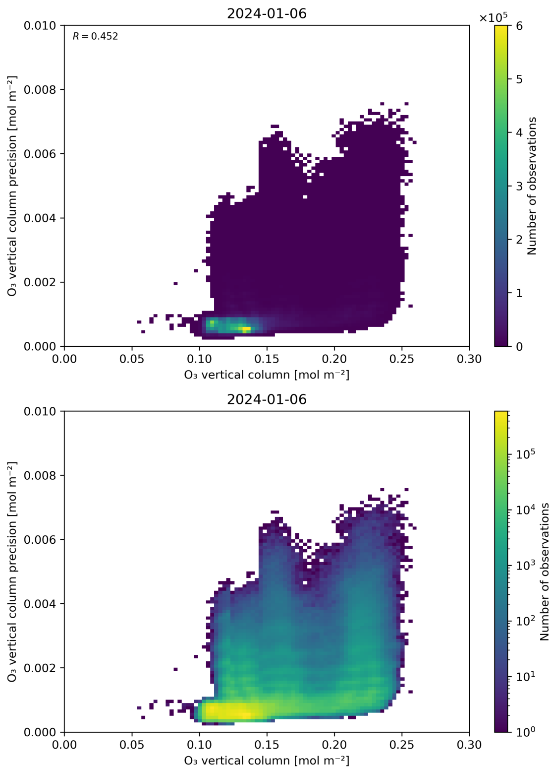
Figure 41: Scatter density plot of “O 3 vertical column” against “O 3 vertical column precision” for 2024-01-05 to 2024-01-07.
