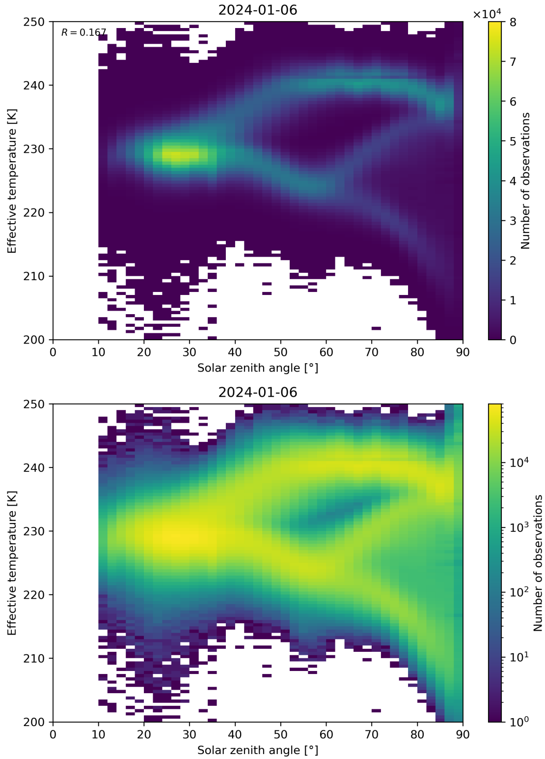
Figure 45: Scatter density plot of “Solar zenith angle” against “Effective temperature” for 2024-01-05 to 2024-01-07.
