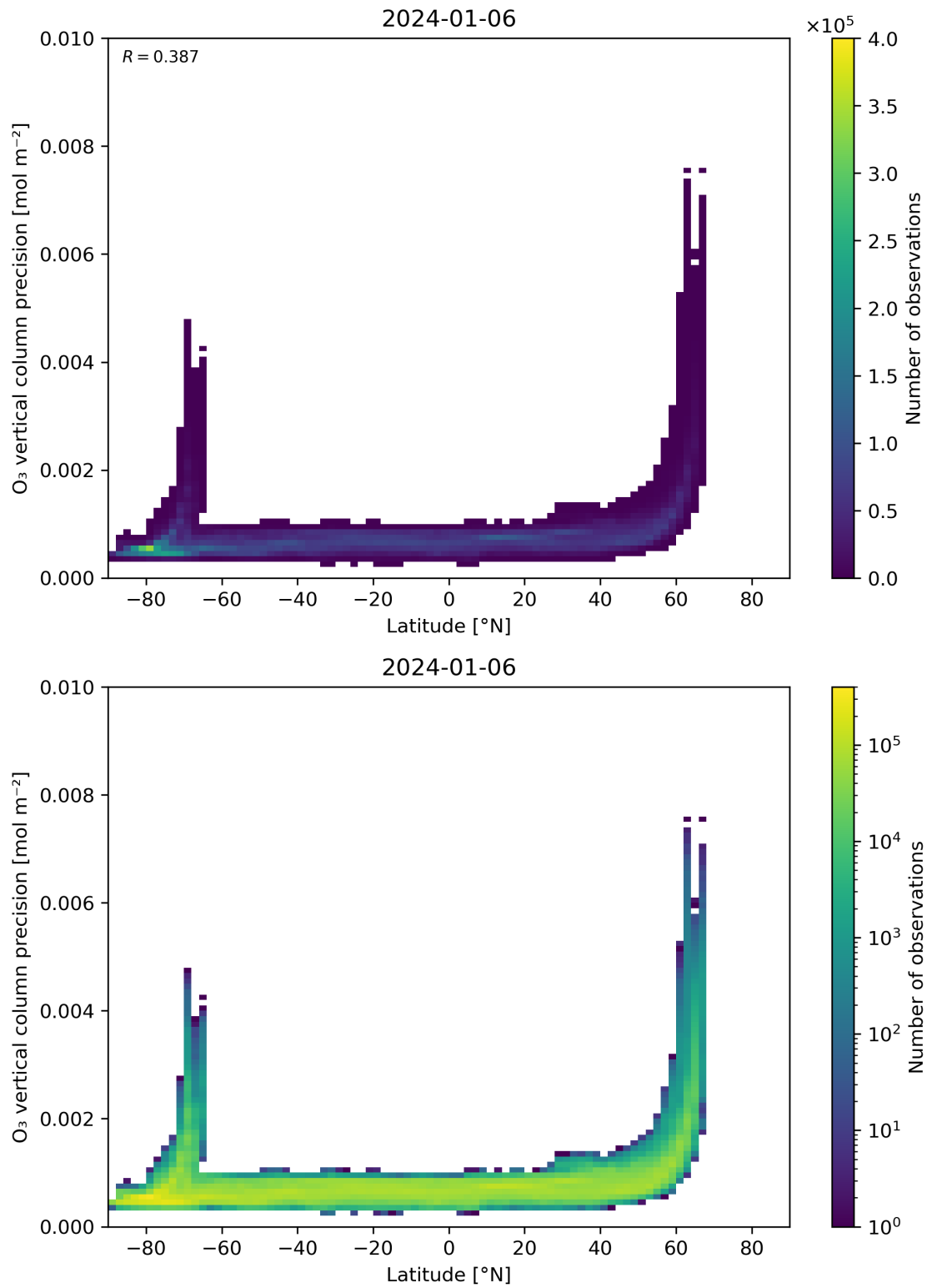
Figure 37: Scatter density plot of “Latitude” against “O 3 vertical column precision” for 2024-01-05 to 2024-01-07.
