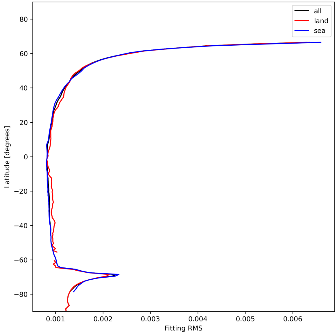
Figure 16: Zonal average of “Fitting RMS” for 2024-01-05 to 2024-01-07.
