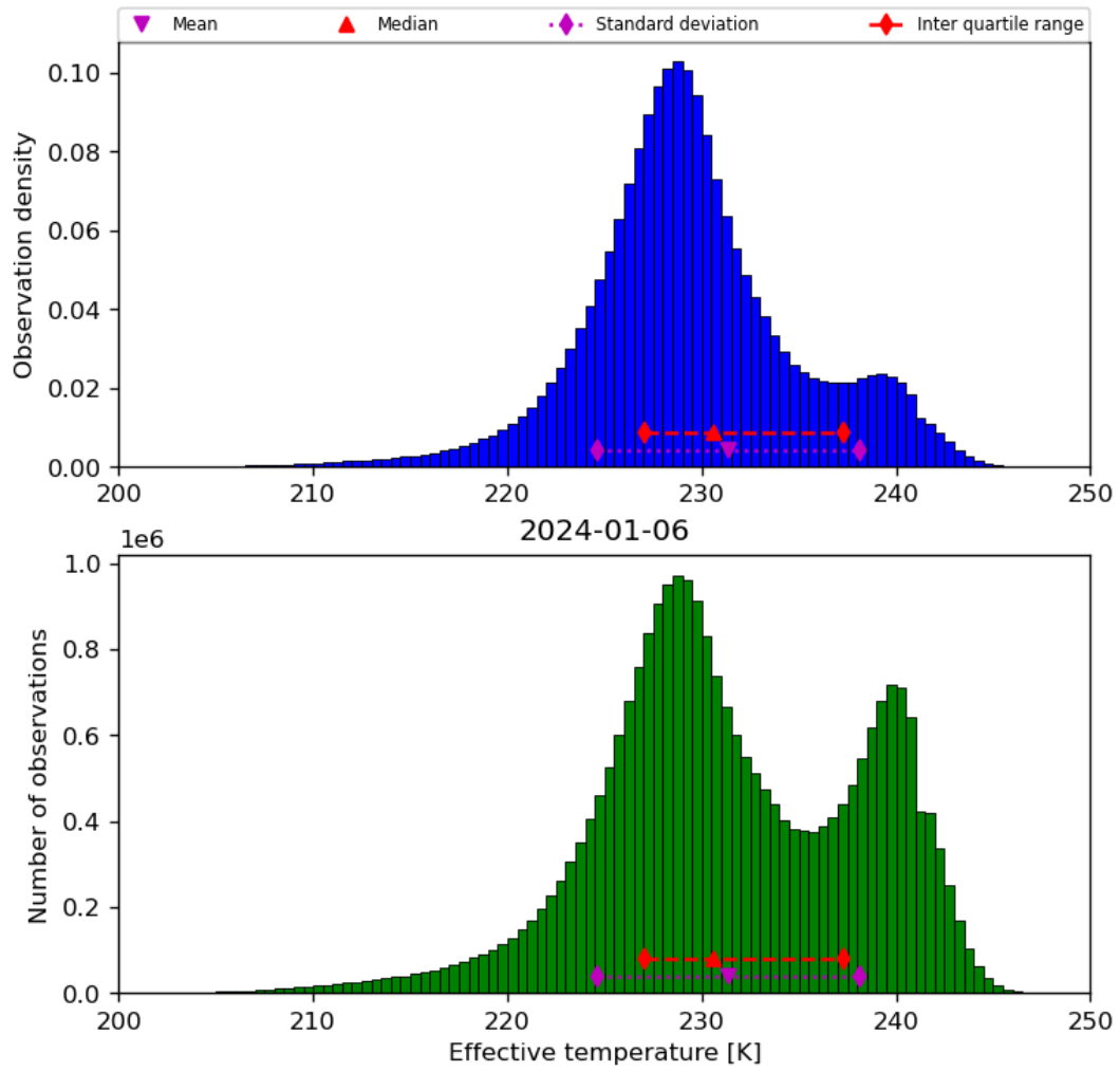
Figure 24: Histogram of “Effective temperature” for 2024-01-05 to 2024-01-07
