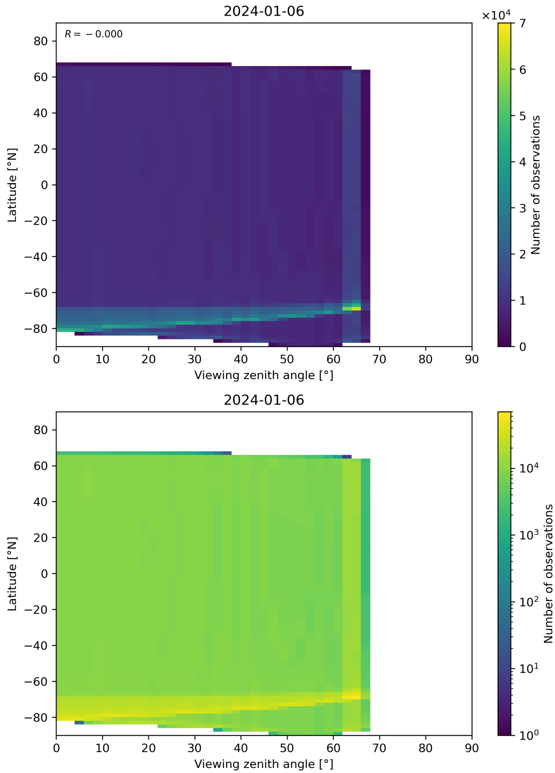
Figure 49: Scatter density plot of “Viewing zenith angle” against “Latitude” for 2024-01-05 to 2024-01-07.
