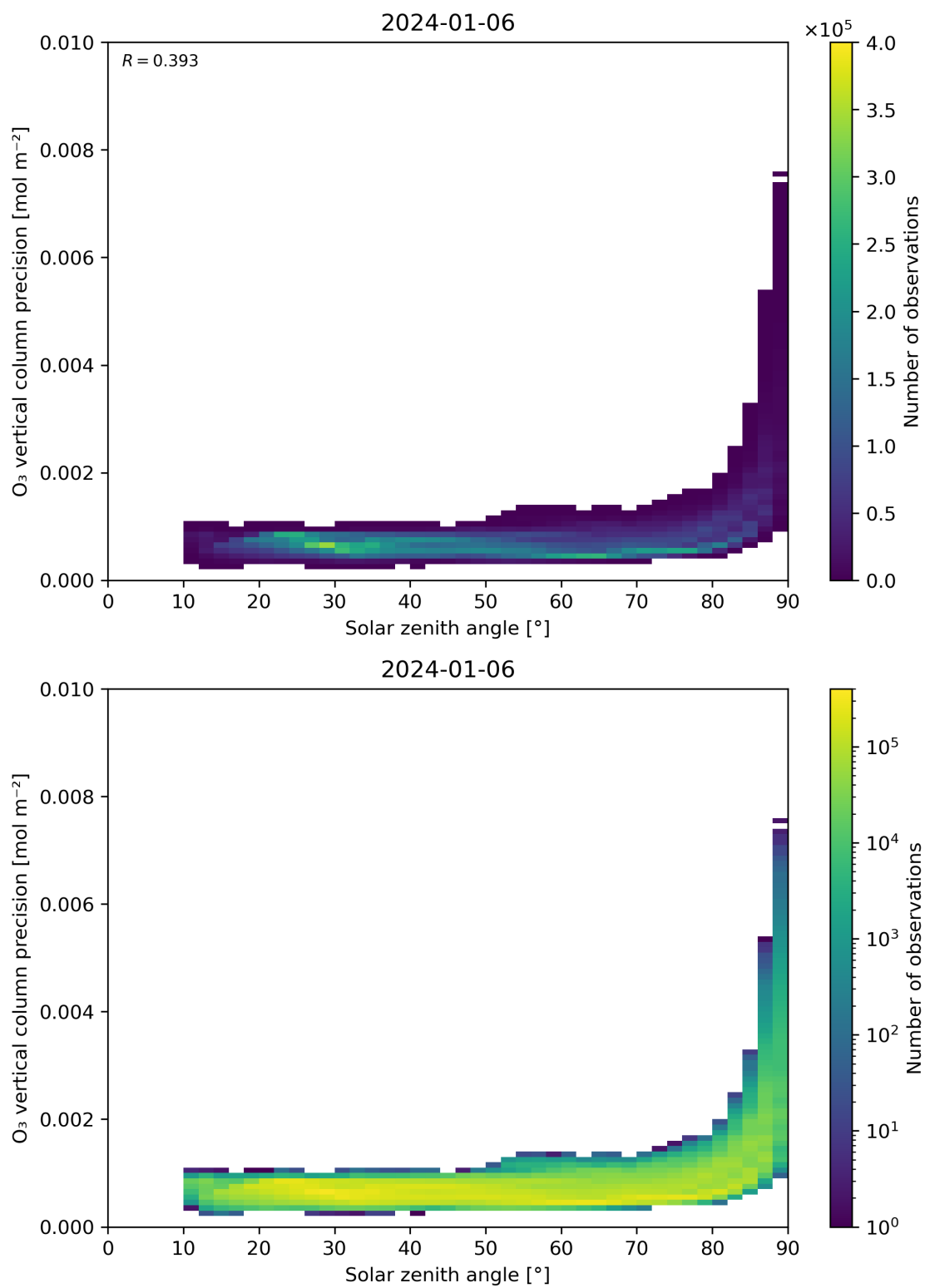
Figure 48: Scatter density plot of “Solar zenith angle” against “O 3 vertical column precision” for 2024-01-05 to 2024-01-07.
