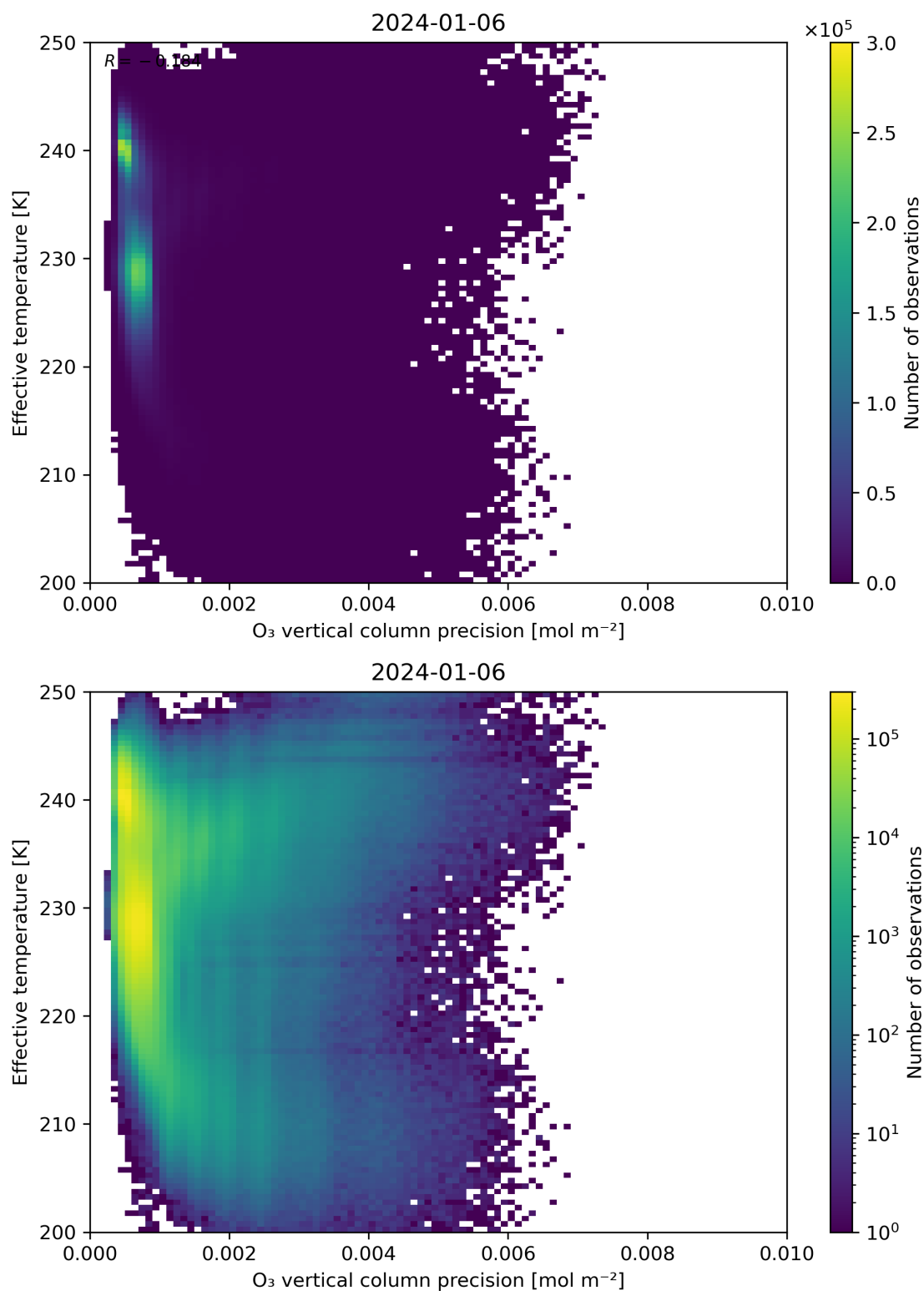
Figure 42: Scatter density plot of “O 3 vertical column precision” against “Effective temperature” for 2024-01-05 to 2024-01-07.
