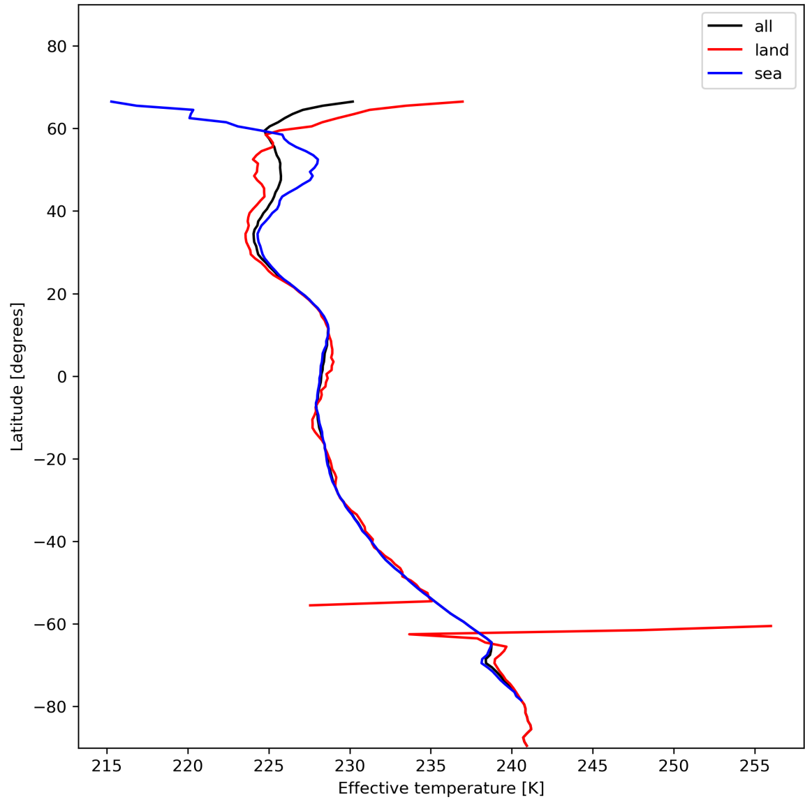
Figure 17: Zonal average of “Effective temperature” for 2024-01-05 to 2024-01-07.
