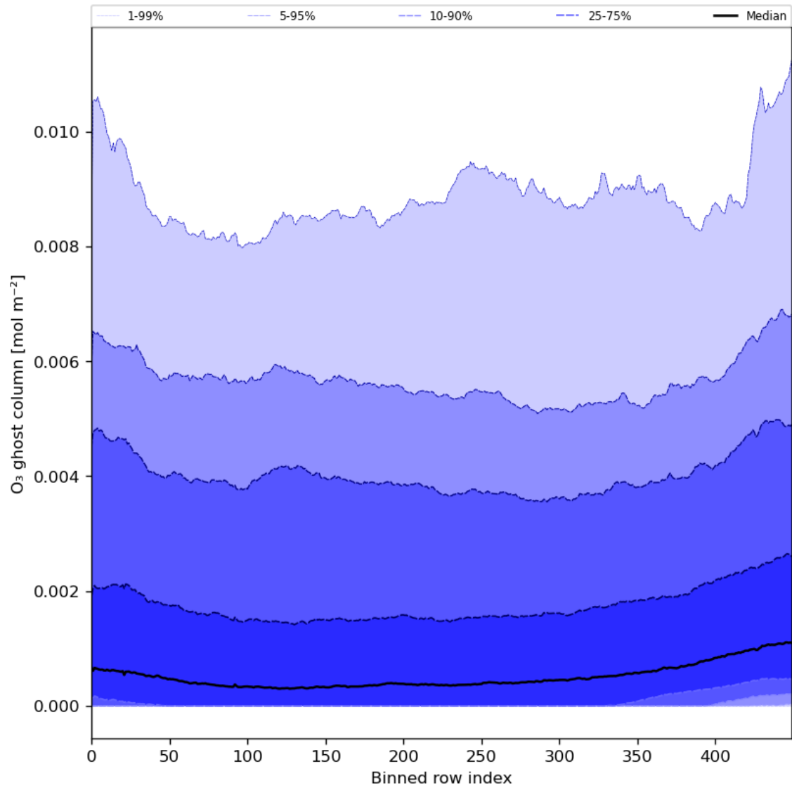
Figure 32: Along track statistics of “O 3 ghost column” for 2024-01-05 to 2024-01-07
