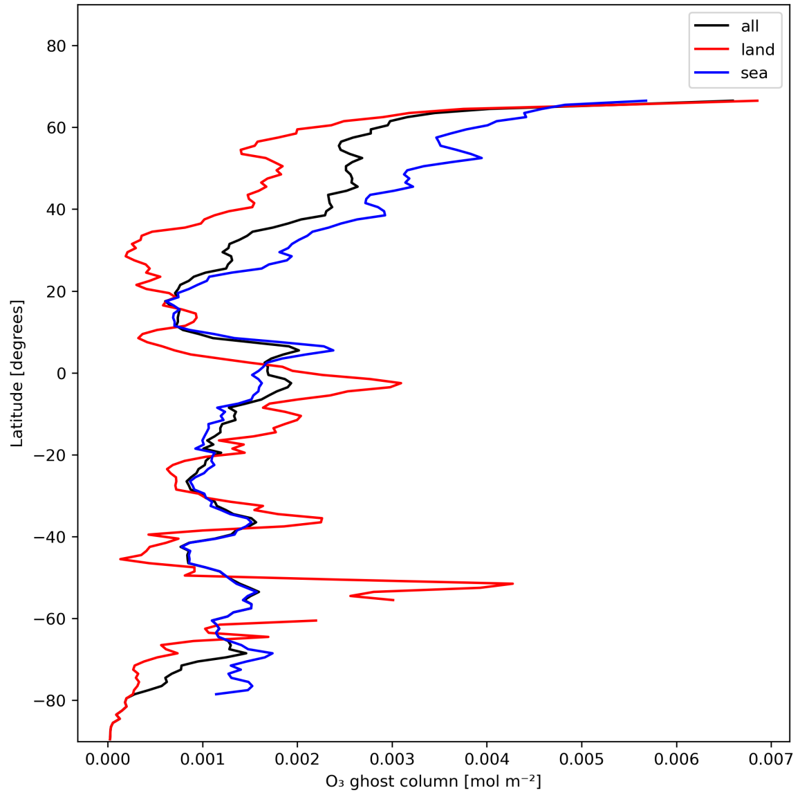
Figure 18: Zonal average of "O 3 ghost column" for 2024-01-05 to 2024-01-07.
