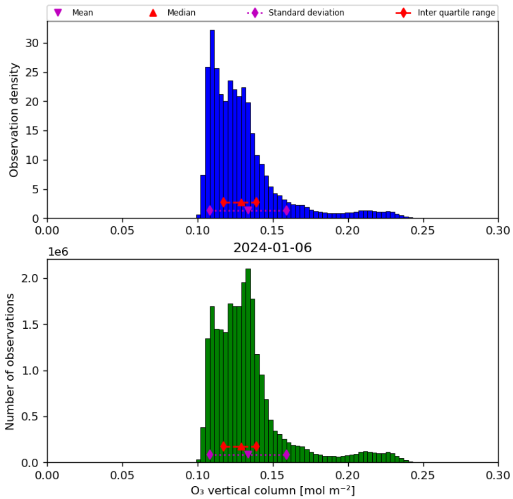
Figure 21: Histogram of “O 3 vertical column” for 2024-01-05 to 2024-01-07
