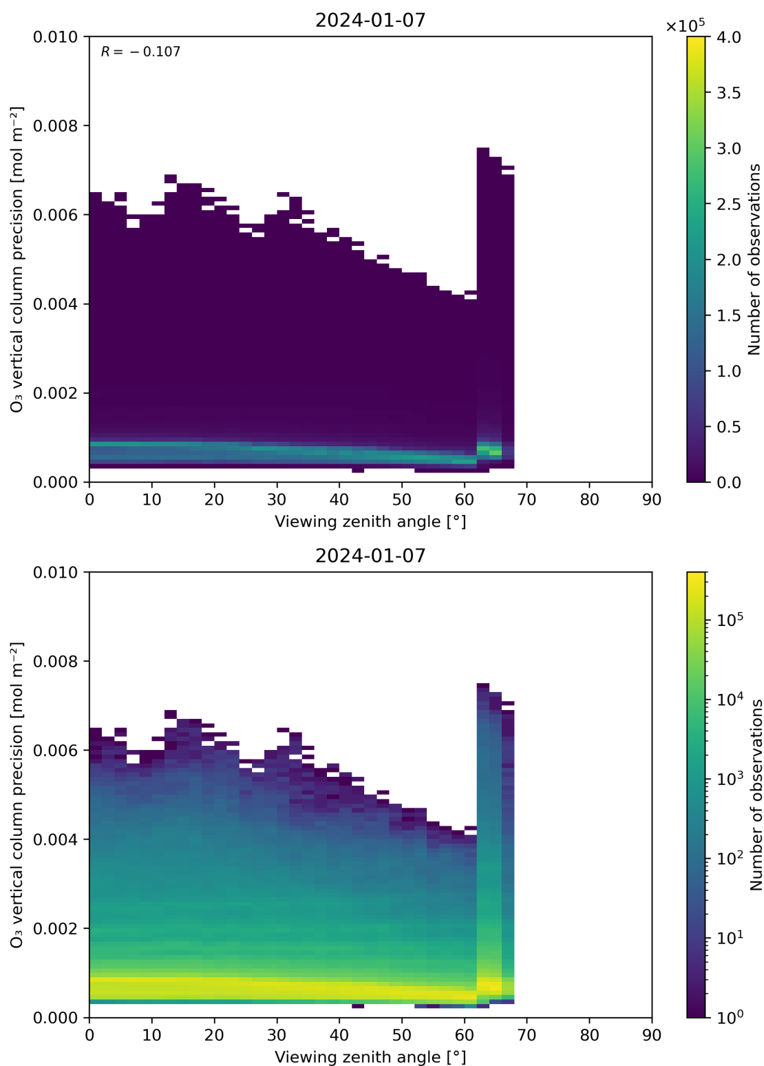
Figure 53: Scatter density plot of “Viewing zenith angle” against “O 3 vertical column precision” for 2024-01-06 to 2024-01-08.
