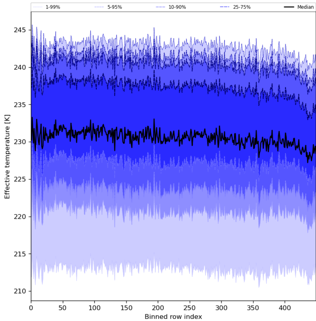
Figure 31: Along track statistics of “Effective temperature” for 2024-01-06 to 2024-01-08
