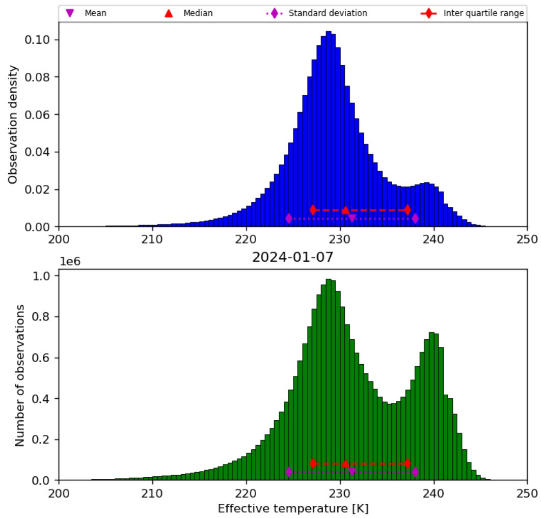
Figure 24: Histogram of “Effective temperature” for 2024-01-06 to 2024-01-08
