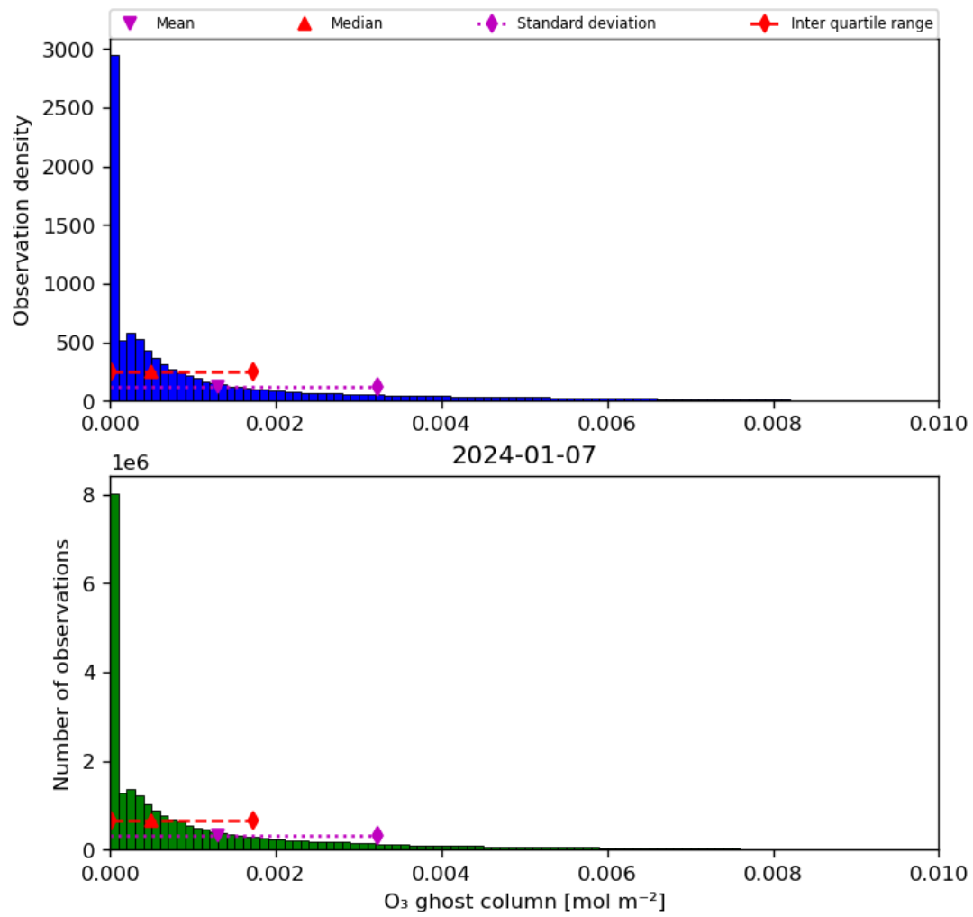
Figure 25: Histogram of “O 3 ghost column” for 2024-01-06 to 2024-01-08
