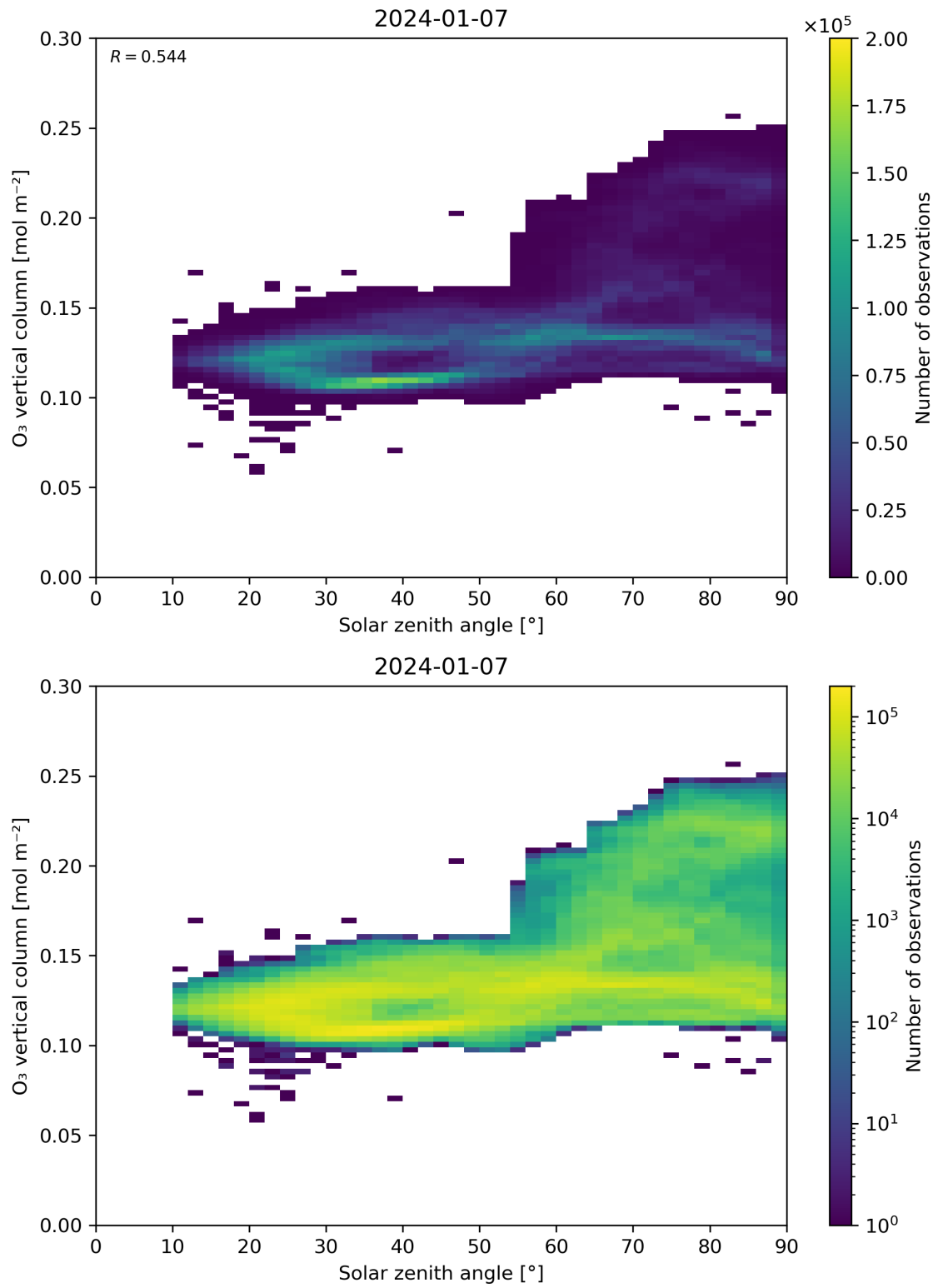
Figure 47: Scatter density plot of “Solar zenith angle” against “O 3 vertical column” for 2024-01-06 to 2024-01-08.
