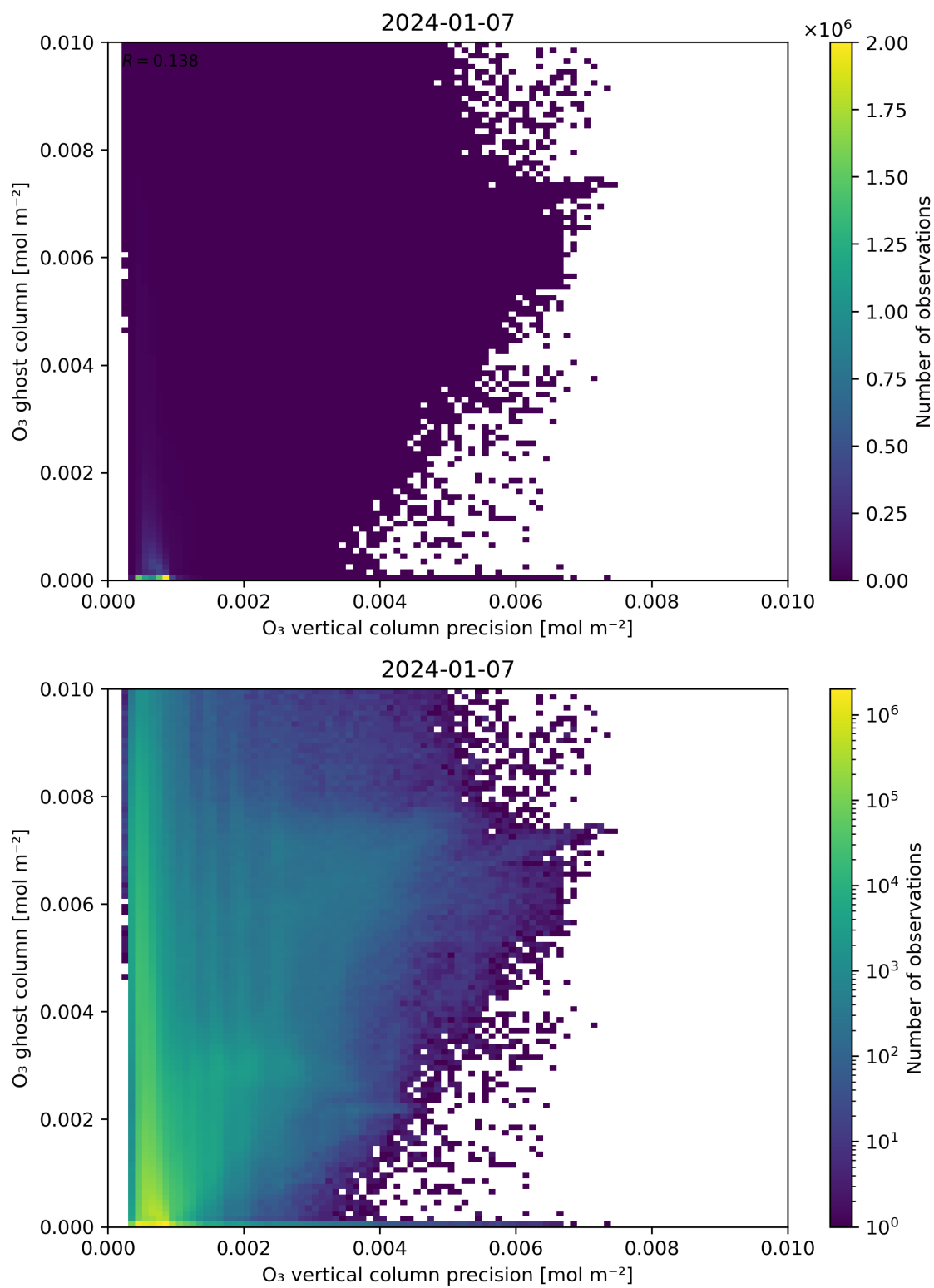
Figure 43: Scatter density plot of “ \text{O}_3 vertical column precision” against “ \text{O}_3 ghost column” for 2024-01-06 to 2024-01-08.
