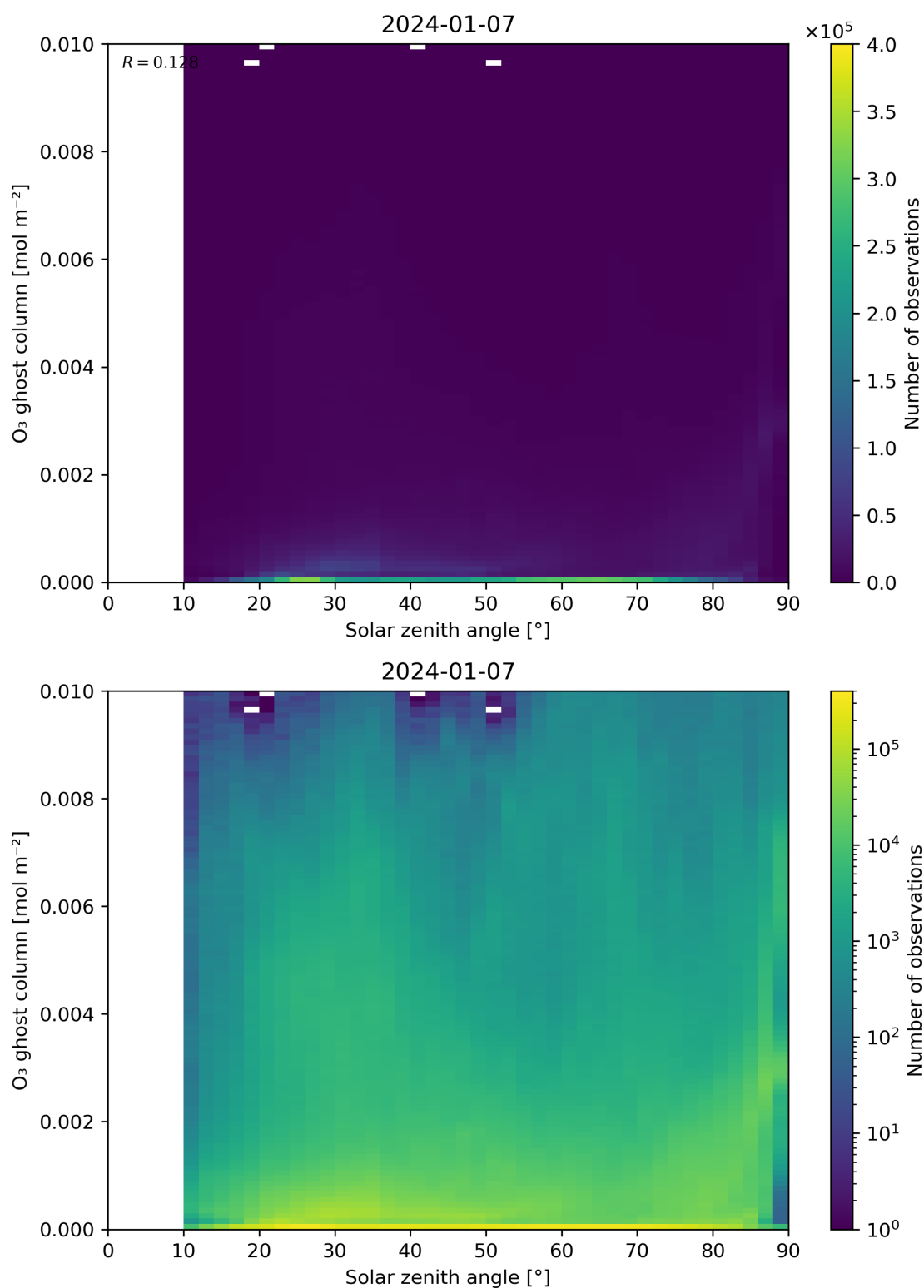
Figure 46: Scatter density plot of “Solar zenith angle” against “O 3 ghost column” for 2024-01-06 to 2024-01-08.
