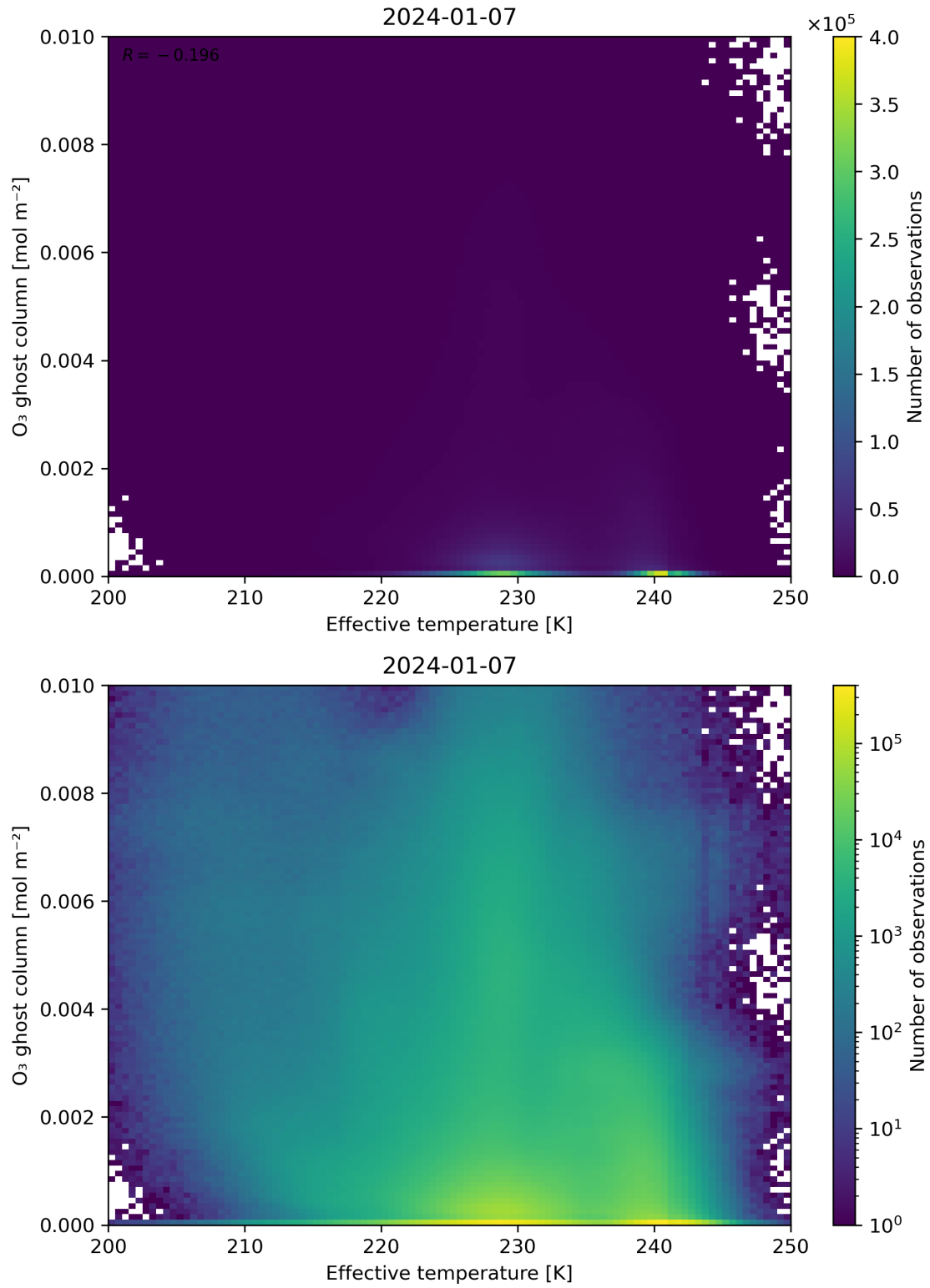
Figure 38: Scatter density plot of “Effective temperature” against “O 3 ghost column” for 2024-01-06 to 2024-01-08.
