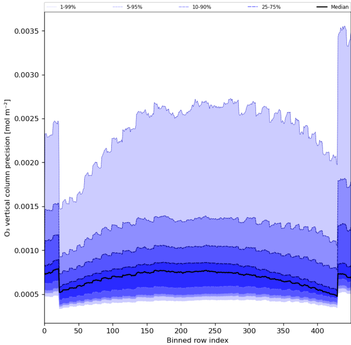
Figure 29: Along track statistics of “O 3 vertical column precision” for 2024-01-06 to 2024-01-08
