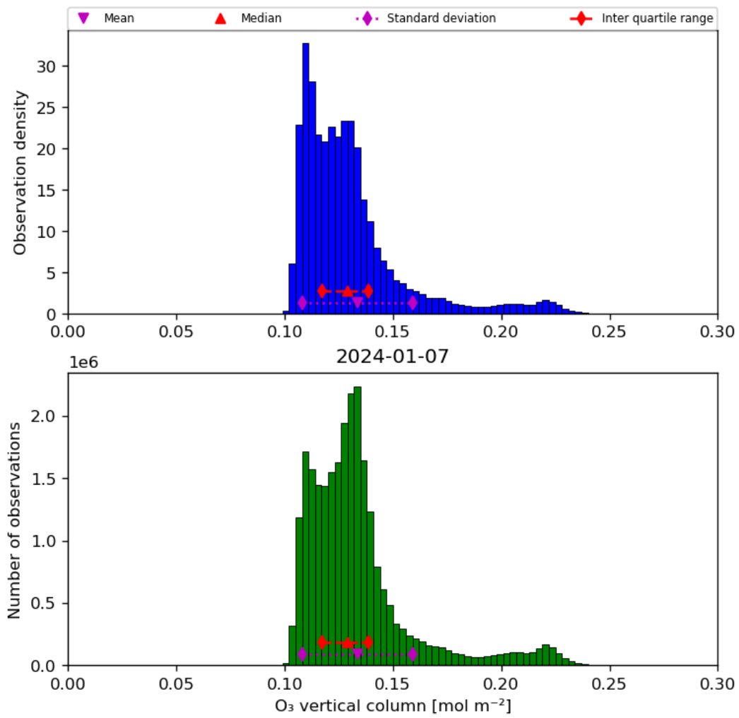
Figure 21: Histogram of “O 3 vertical column” for 2024-01-06 to 2024-01-08
