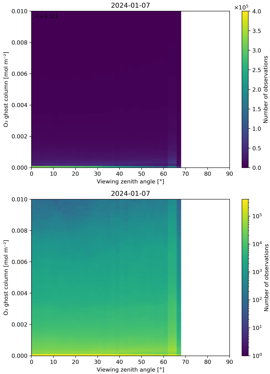
Figure 51: Scatter density plot of “Viewing zenith angle” against “O 3 ghost column” for 2024-01-06 to 2024-01-08.
