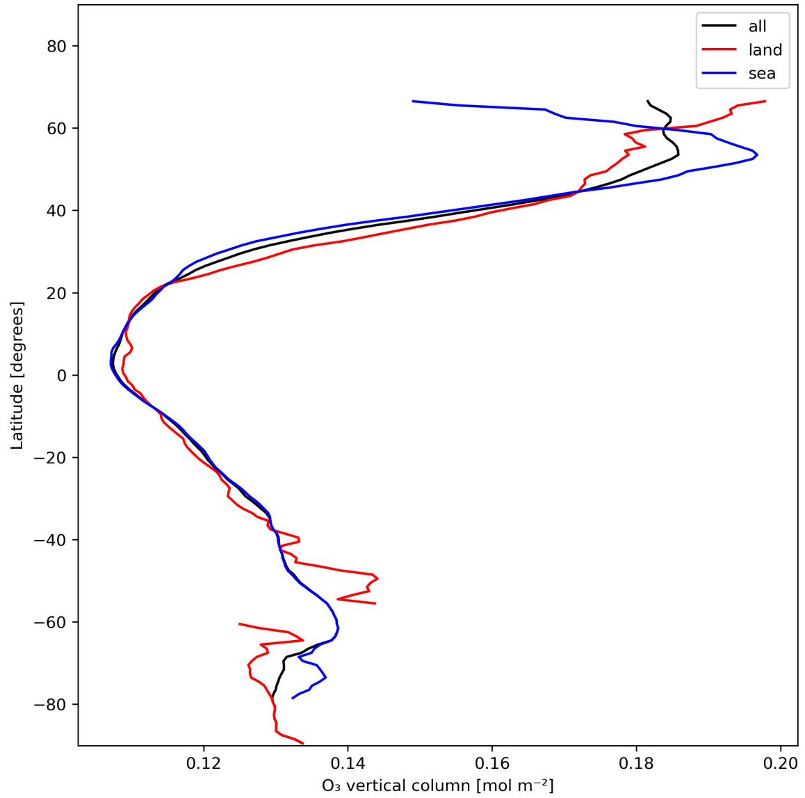
Figure 14: Zonal average of “O 3 vertical column” for 2024-01-06 to 2024-01-08.
