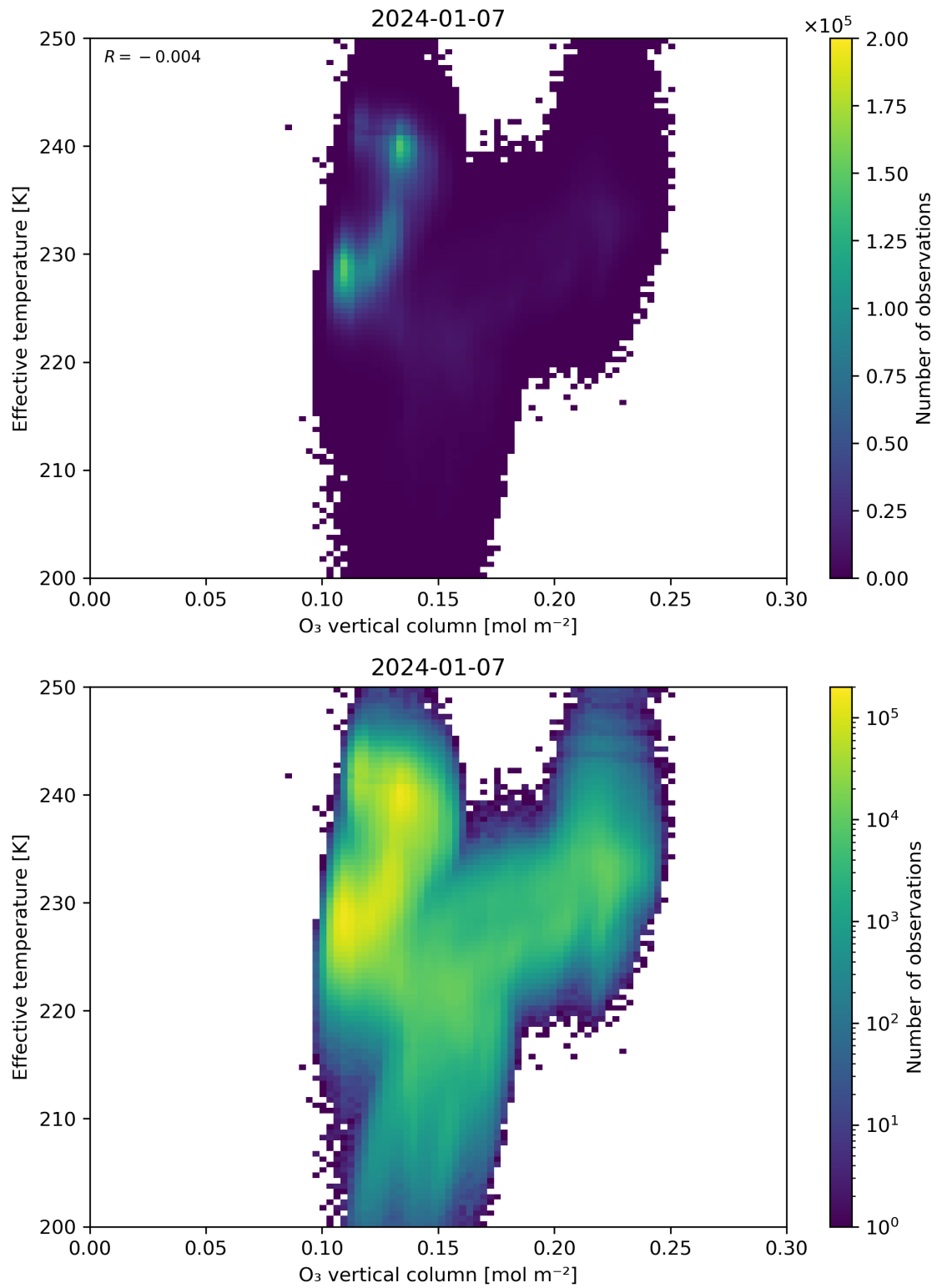
Figure 39: Scatter density plot of “O 3 vertical column” against “Effective temperature” for 2024-01-06 to 2024-01-08.
