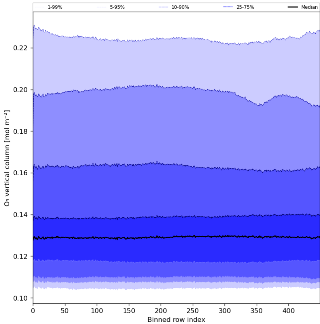
Figure 28: Along track statistics of “O 3 vertical column” for 2024-01-06 to 2024-01-08
