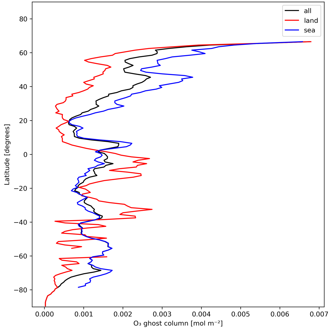
Figure 18: Zonal average of “O 3 ghost column” for 2024-01-06 to 2024-01-08.
