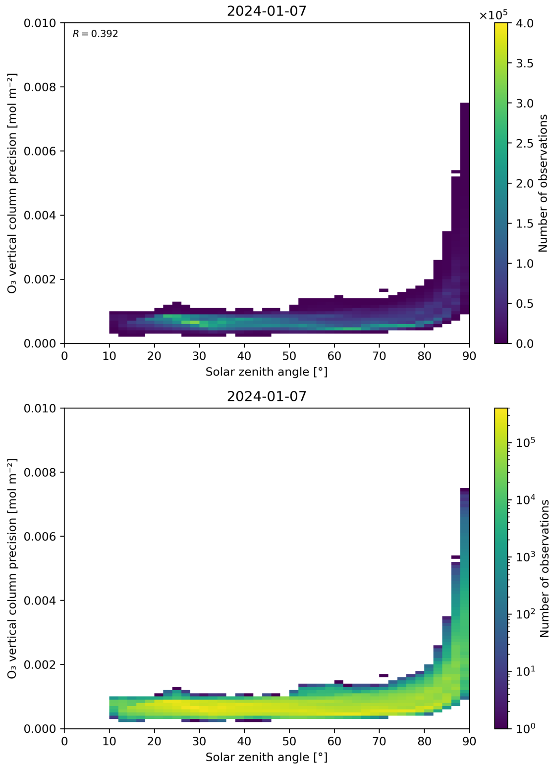
Figure 48: Scatter density plot of “Solar zenith angle” against “O 3 vertical column precision” for 2024-01-06 to 2024-01-08.
