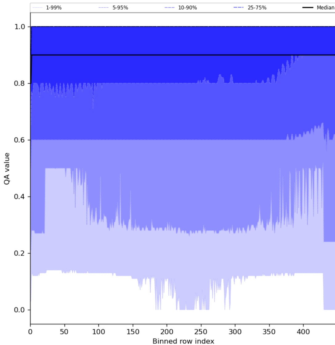
Figure 27: Along track statistics of “QA value” for 2024-01-06 to 2024-01-08
