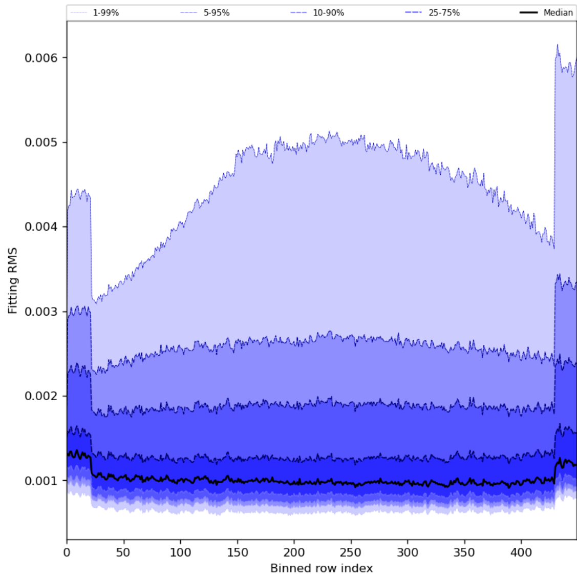
Figure 30: Along track statistics of “Fitting RMS” for 2024-01-06 to 2024-01-08
