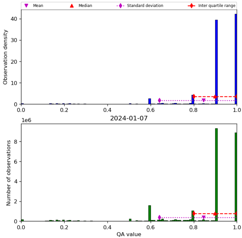
Figure 20: Histogram of “QA value” for 2024-01-06 to 2024-01-08
