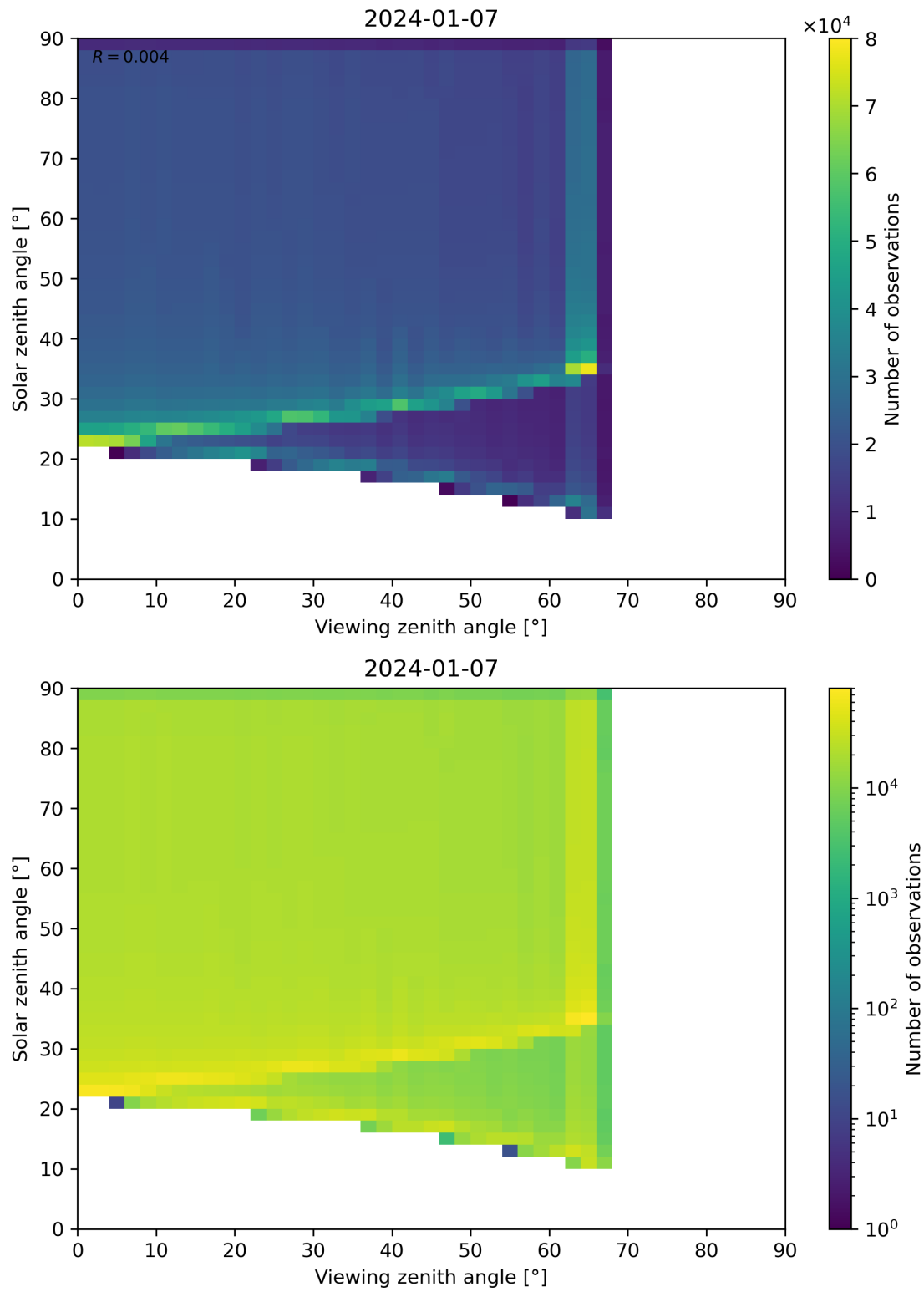
Figure 54: Scatter density plot of “Viewing zenith angle” against “Solar zenith angle” for 2024-01-06 to 2024-01-08.
