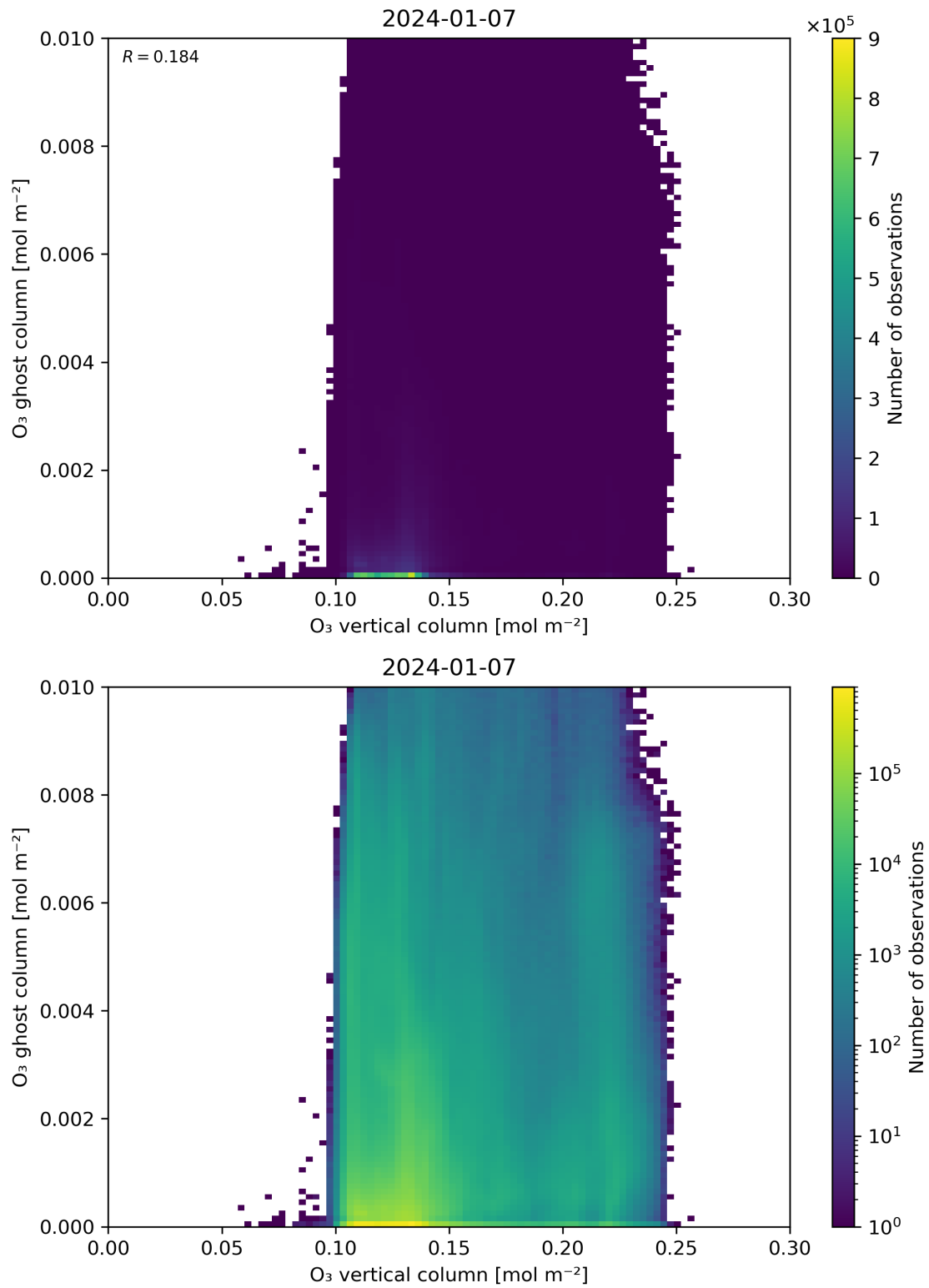
Figure 40: Scatter density plot of “O 3 vertical column” against “O 3 ghost column” for 2024-01-06 to 2024-01-08.
