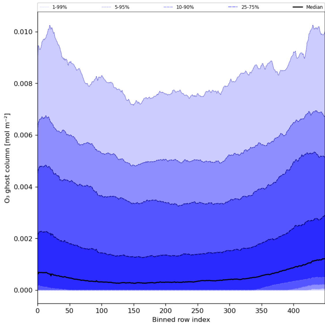
Figure 32: Along track statistics of “O 3 ghost column” for 2024-01-06 to 2024-01-08
