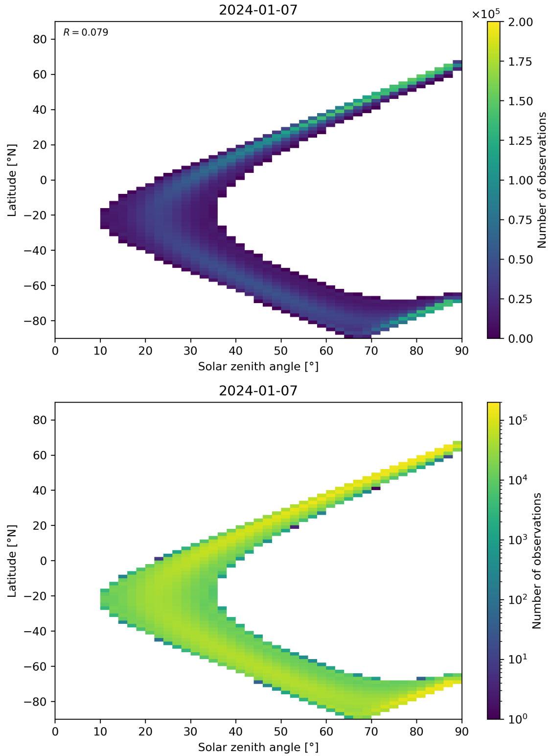
Figure 44: Scatter density plot of “Solar zenith angle” against “Latitude” for 2024-01-06 to 2024-01-08.
