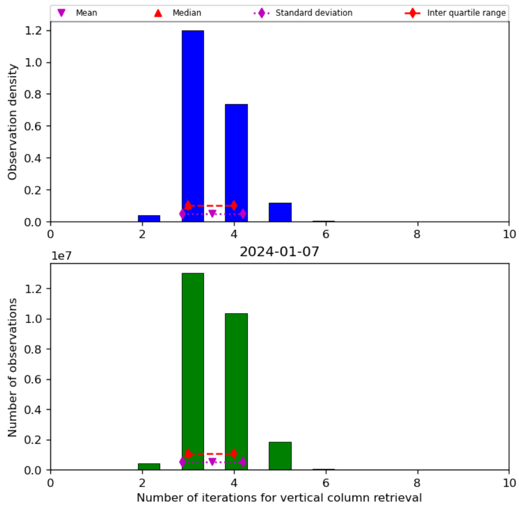
Figure 26: Histogram of “Number of iterations for vertical column retrieval” for 2024-01-06 to 2024-01-08
