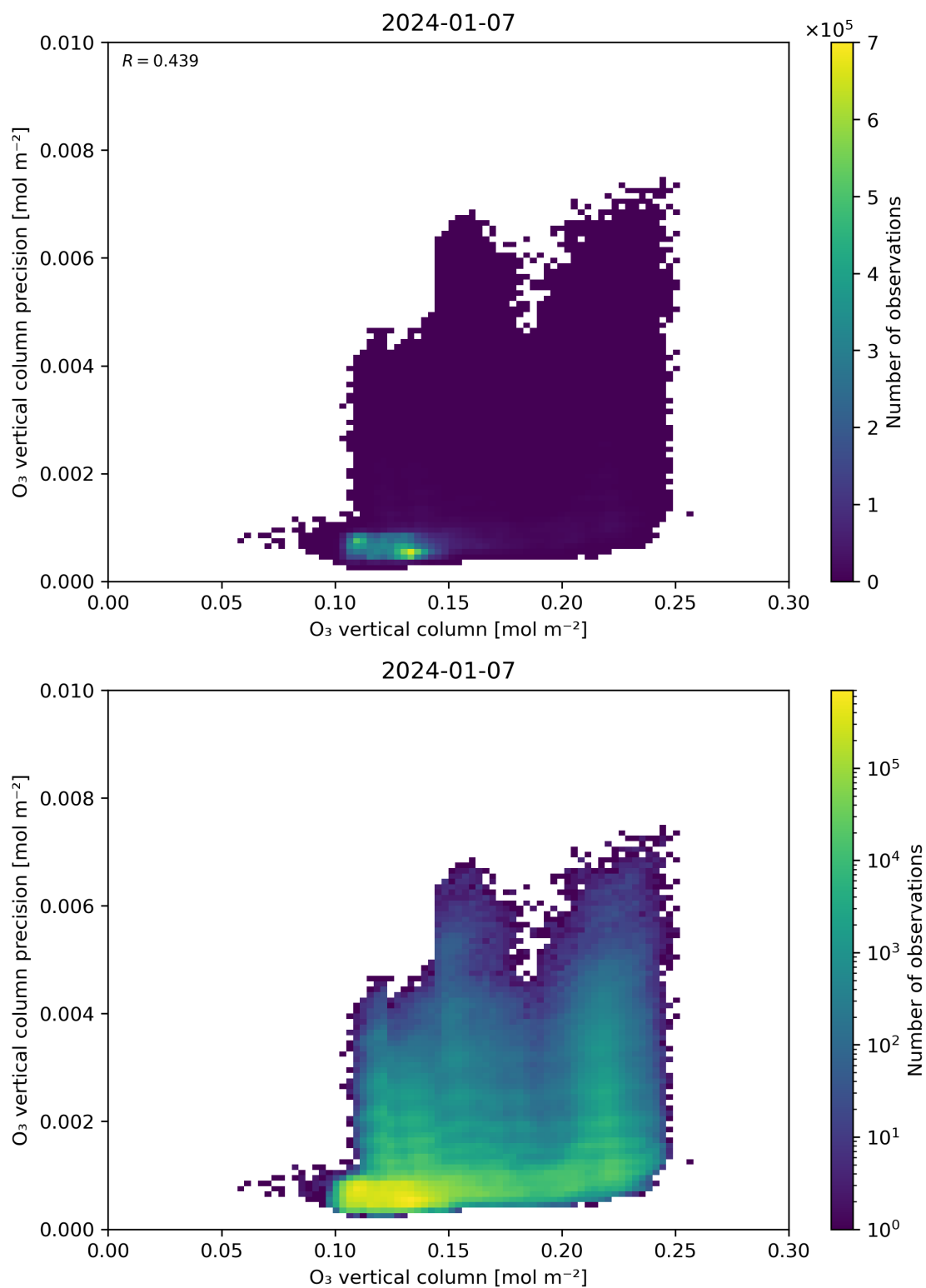
Figure 41: Scatter density plot of “O 3 vertical column” against “O 3 vertical column precision” for 2024-01-06 to 2024-01-08.
