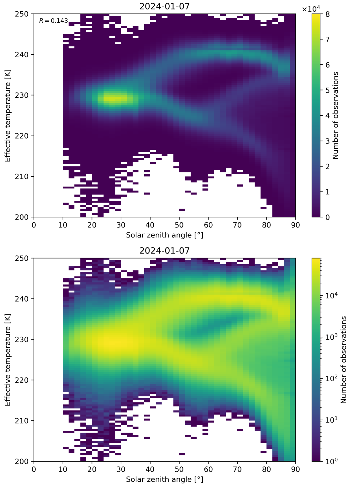
Figure 45: Scatter density plot of “Solar zenith angle” against “Effective temperature” for 2024-01-06 to 2024-01-08.
