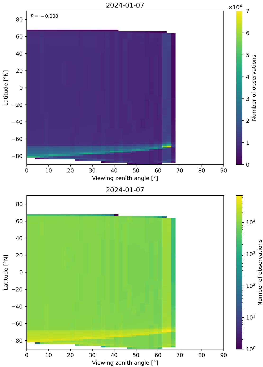
Figure 49: Scatter density plot of “Viewing zenith angle” against “Latitude” for 2024-01-06 to 2024-01-08.
