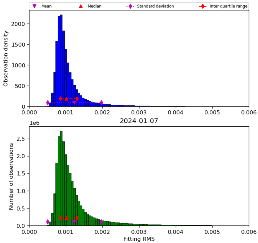
Figure 23: Histogram of “Fitting RMS” for 2024-01-06 to 2024-01-08
