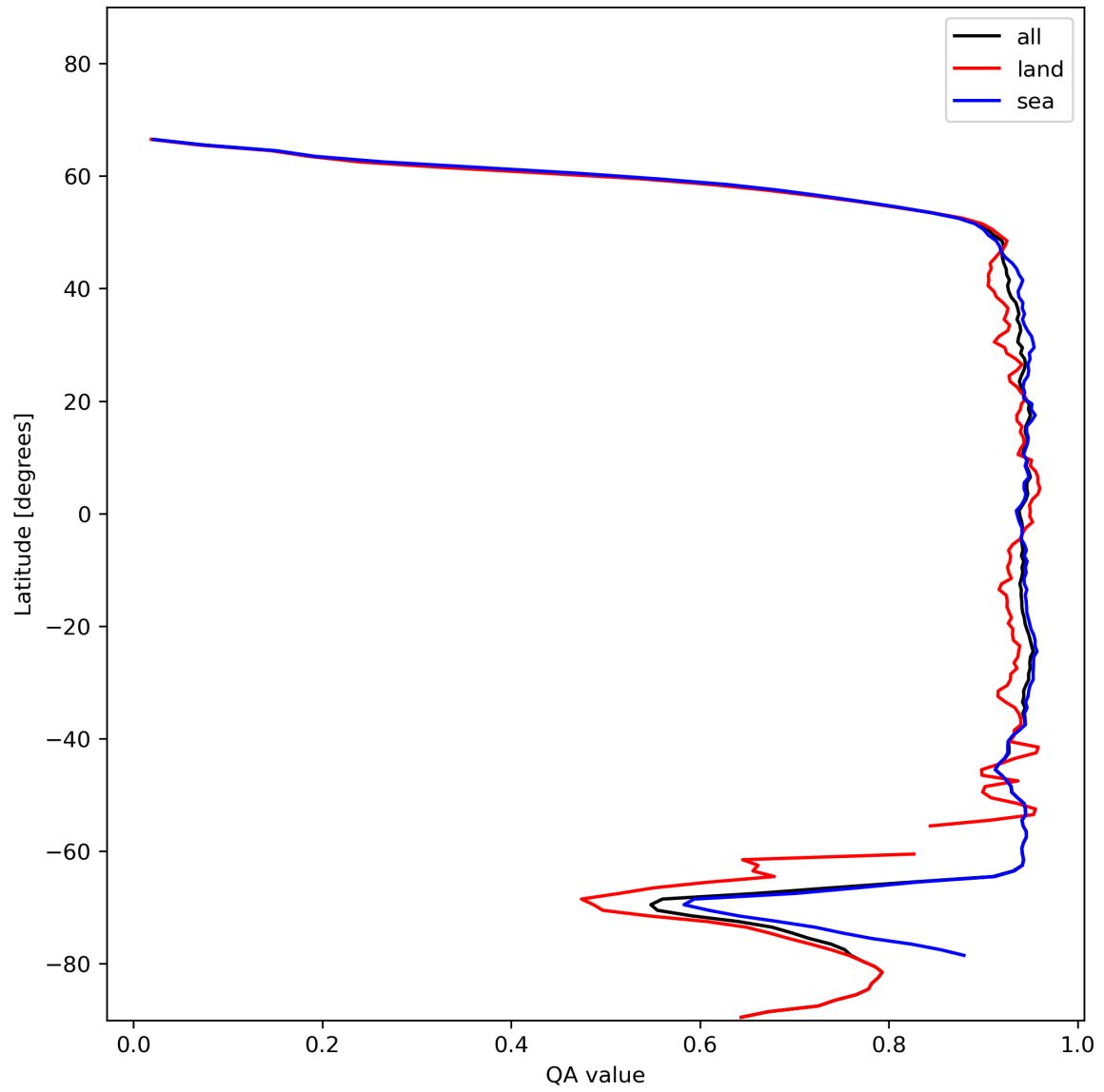
Figure 13: Zonal average of “QA value” for 2024-01-06 to 2024-01-08.
