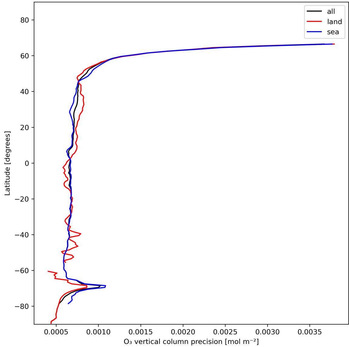
Figure 15: Zonal average of “O 3 vertical column precision” for 2024-01-06 to 2024-01-08.
