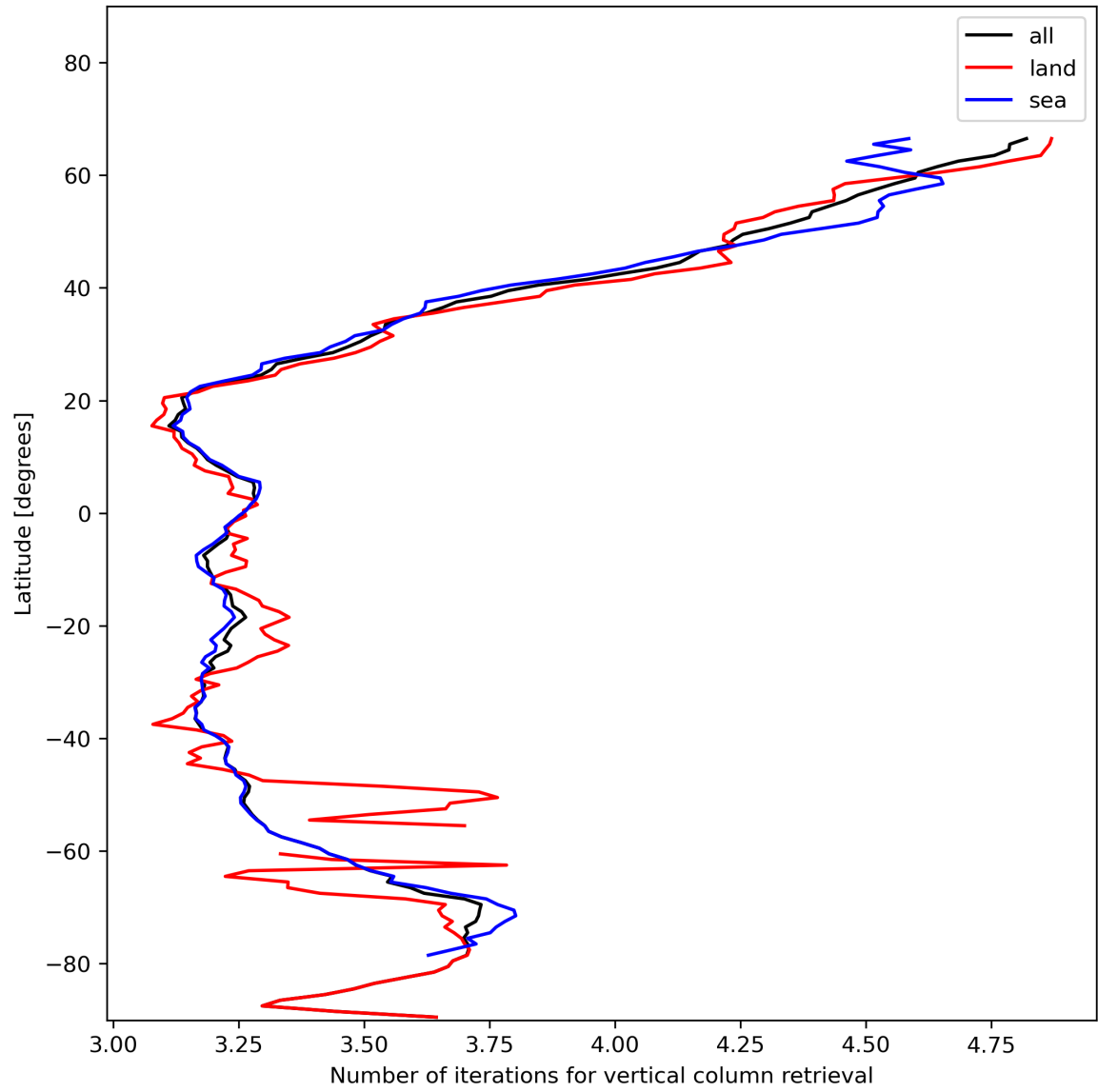
Figure 19: Zonal average of “Number of iterations for vertical column retrieval” for 2024-01-06 to 2024-01-08.
