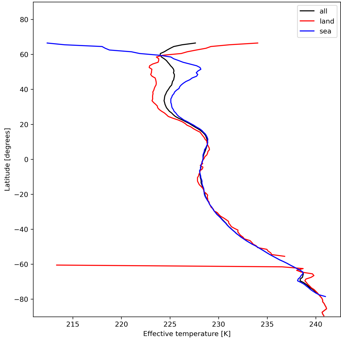
Figure 17: Zonal average of "Effective temperature" for 2024-01-06 to 2024-01-08.
