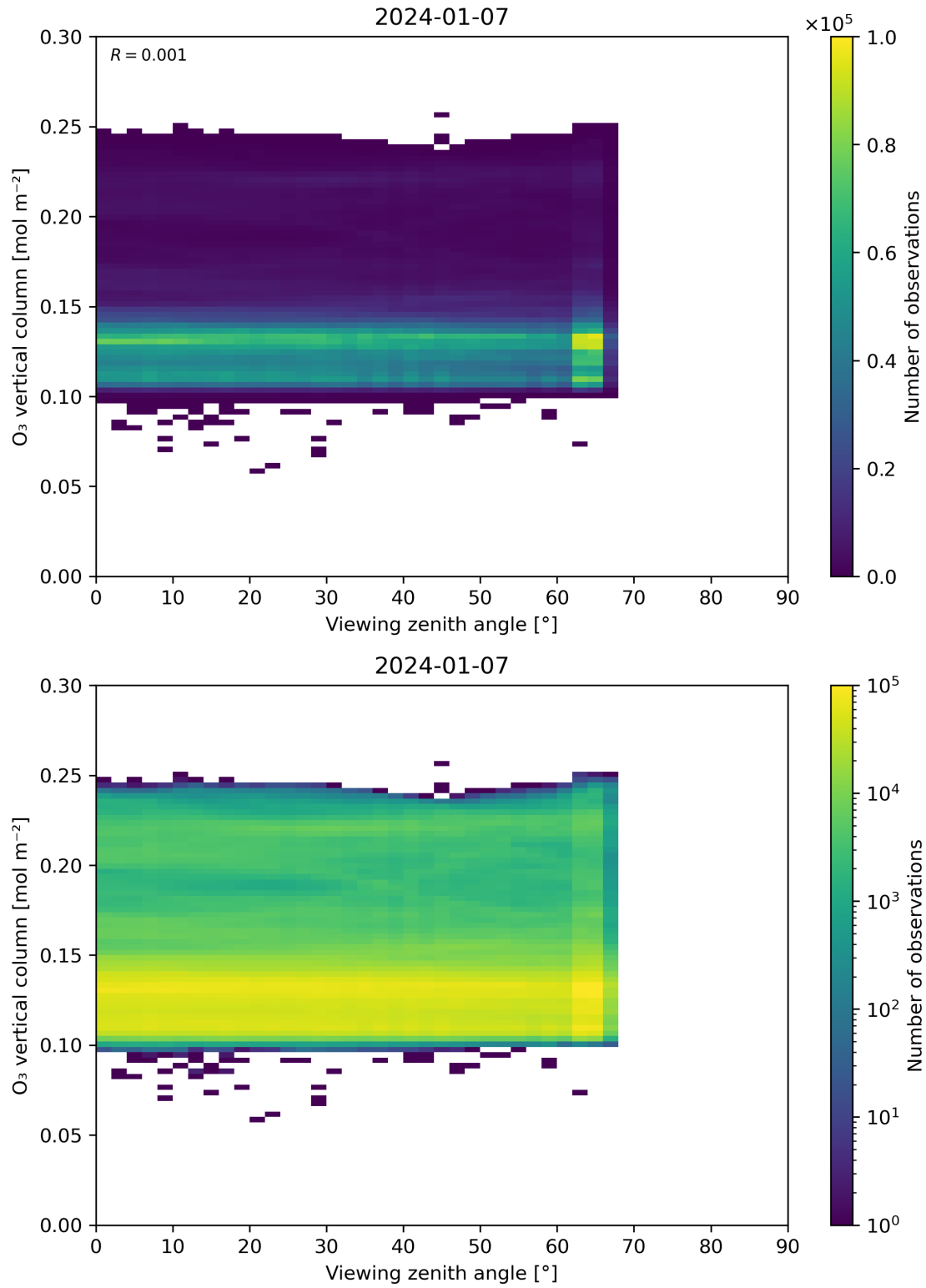
Figure 52: Scatter density plot of “Viewing zenith angle” against “O 3 vertical column” for 2024-01-06 to 2024-01-08.
