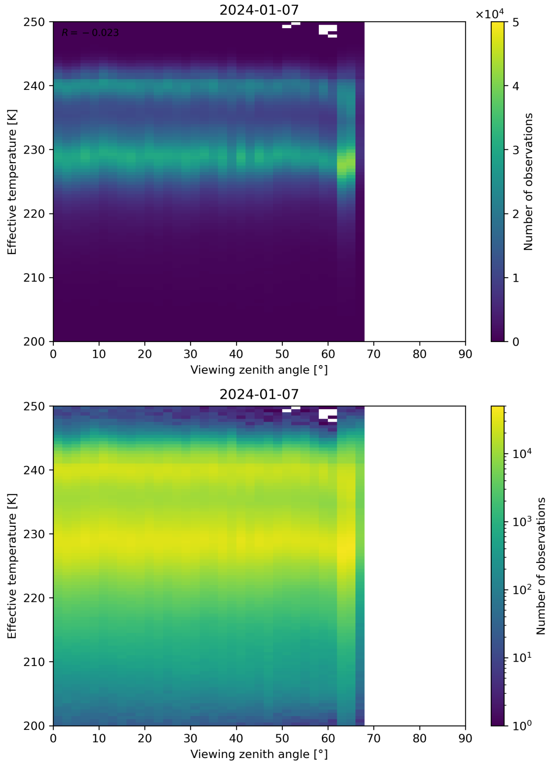
Figure 50: Scatter density plot of “Viewing zenith angle” against “Effective temperature” for 2024-01-06 to 2024-01-08.
