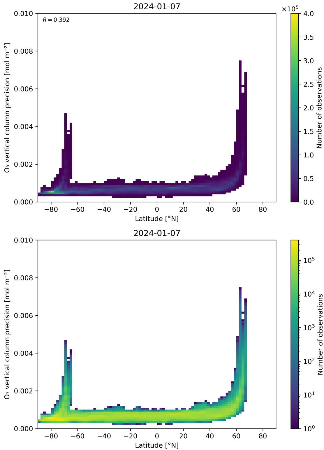
Figure 37: Scatter density plot of “Latitude” against “O 3 vertical column precision” for 2024-01-06 to 2024-01-08.
