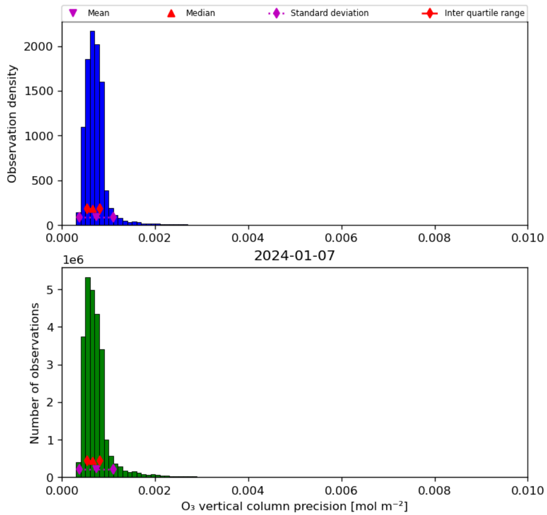
Figure 22: Histogram of “O 3 vertical column precision” for 2024-01-06 to 2024-01-08
