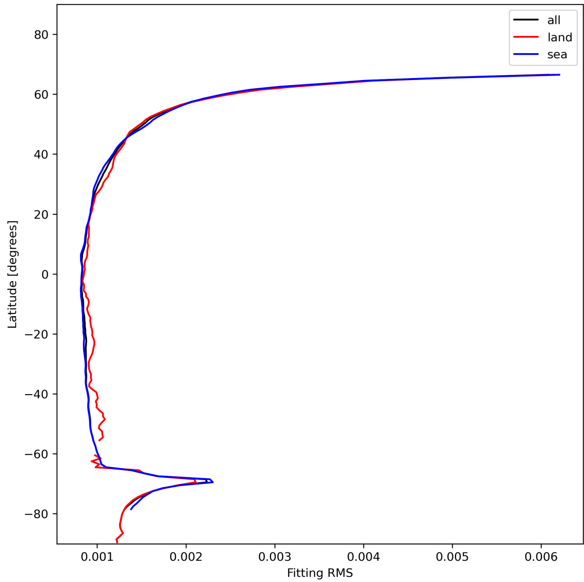
Figure 16: Zonal average of “Fitting RMS” for 2024-01-06 to 2024-01-08.
