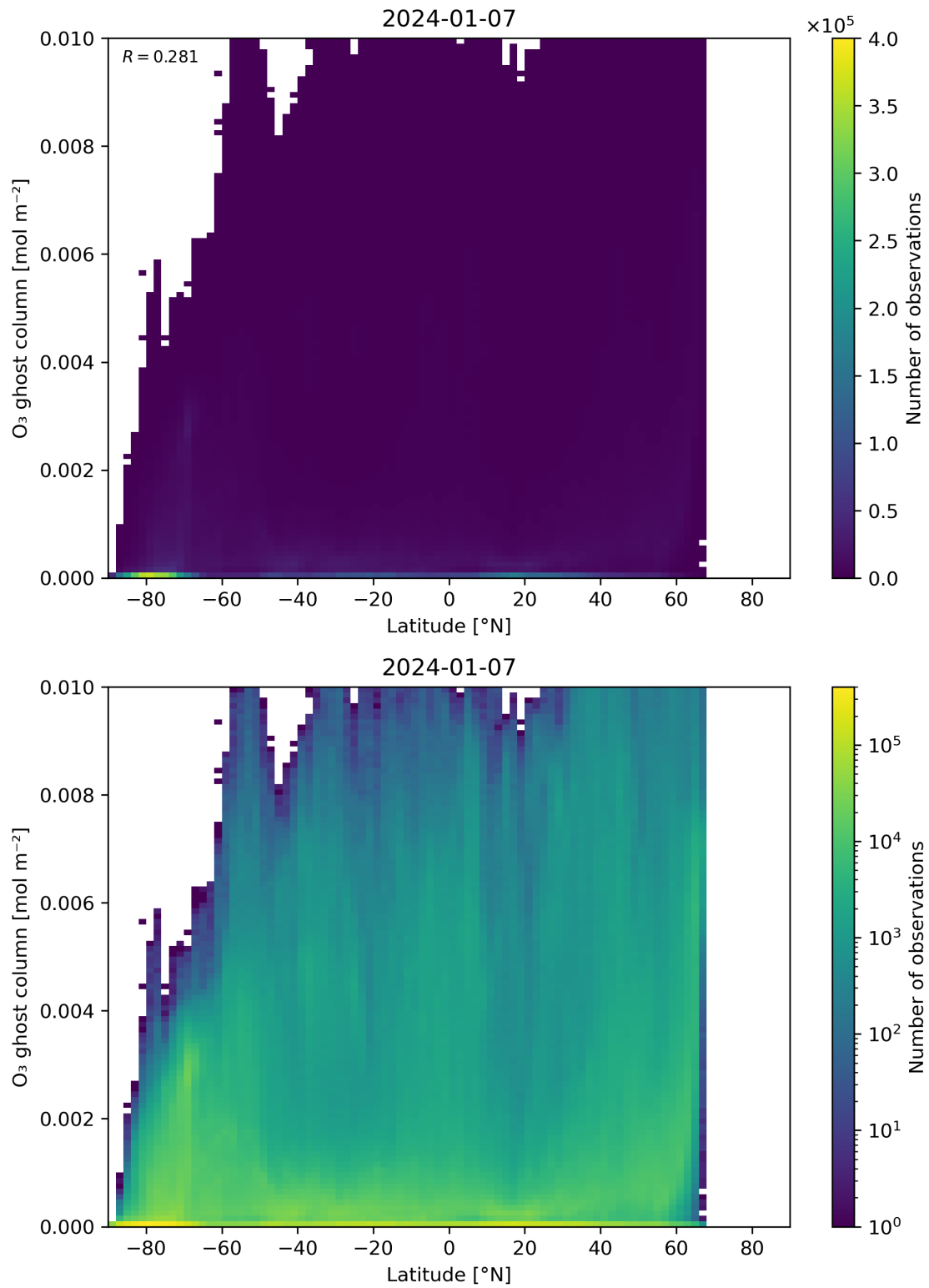
Figure 35: Scatter density plot of “Latitude” against “O 3 ghost column” for 2024-01-06 to 2024-01-08.
