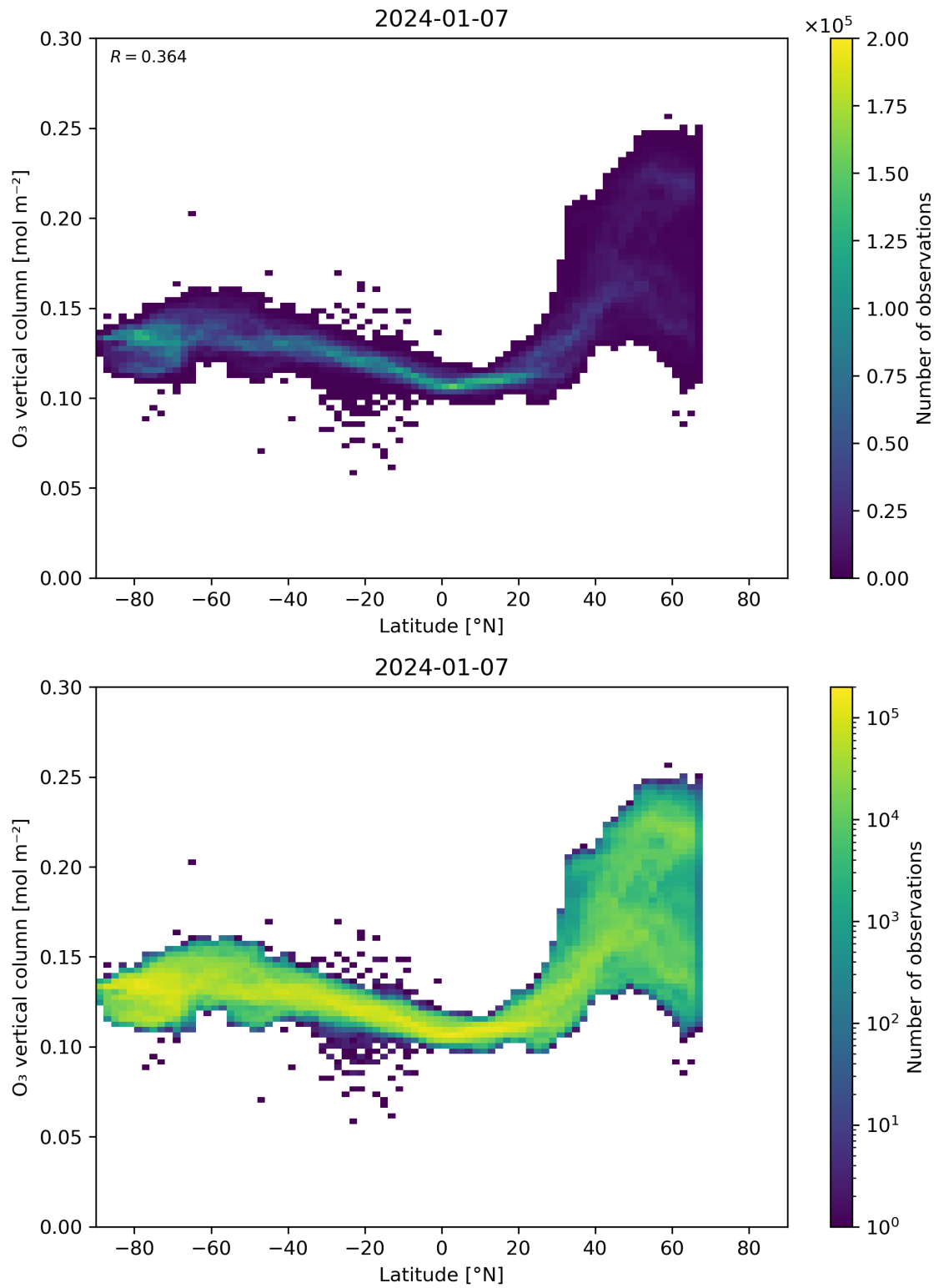
Figure 36: Scatter density plot of “Latitude” against “O 3 vertical column” for 2024-01-06 to 2024-01-08.
