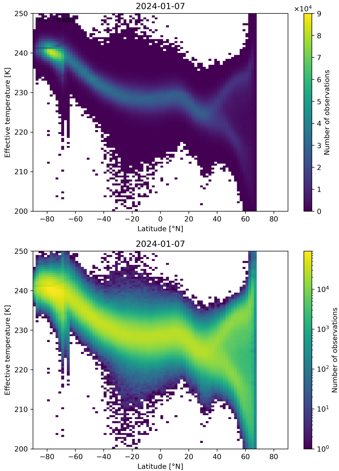
Figure 34: Scatter density plot of “Latitude” against “Effective temperature” for 2024-01-06 to 2024-01-08.
