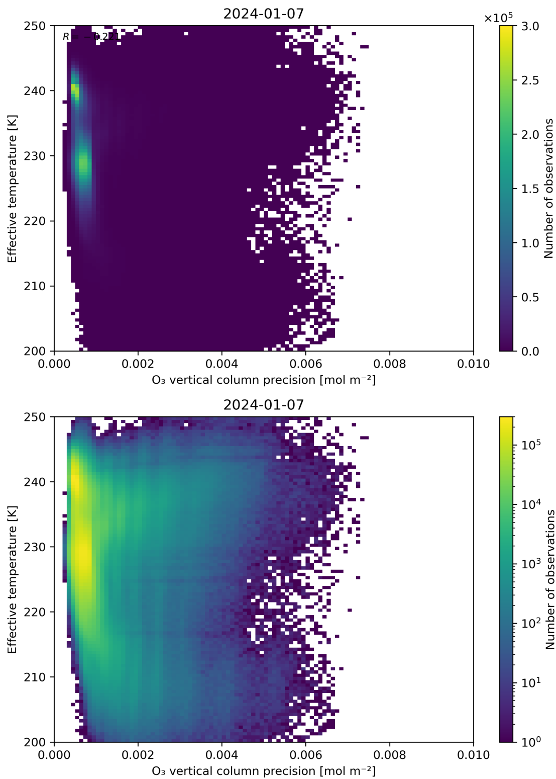
Figure 42: Scatter density plot of “O 3 vertical column precision” against “Effective temperature” for 2024-01-06 to 2024-01-08.
