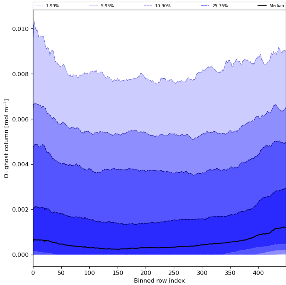
Figure 32: Along track statistics of “O 3 ghost column” for 2024-01-07 to 2024-01-09
