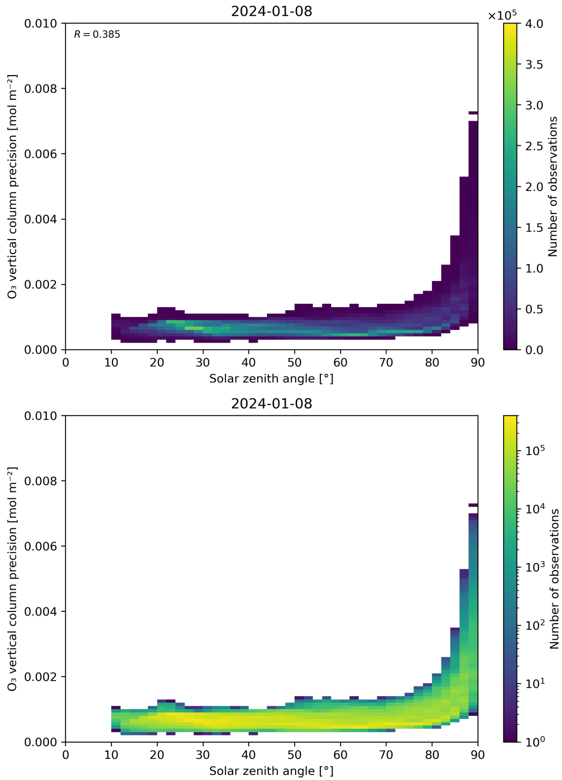
Figure 48: Scatter density plot of “Solar zenith angle” against “O 3 vertical column precision” for 2024-01-07 to 2024-01-09.
