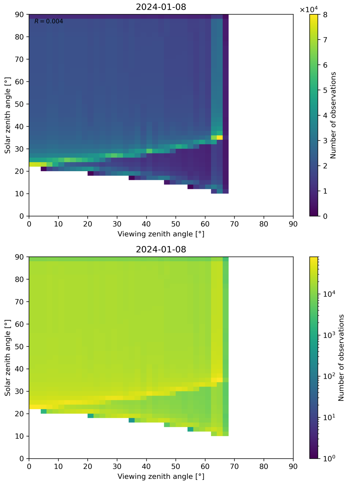
Figure 54: Scatter density plot of “Viewing zenith angle” against “Solar zenith angle” for 2024-01-07 to 2024-01-09.
