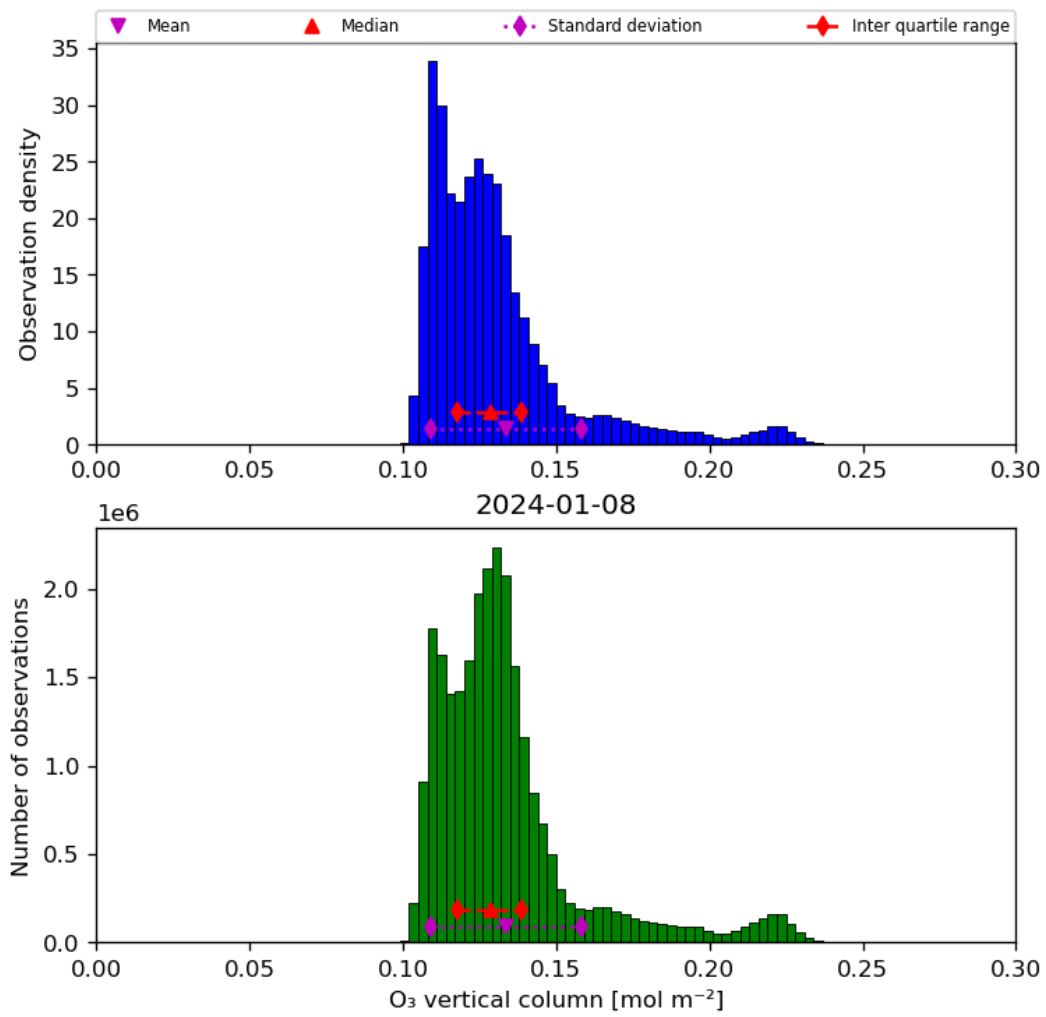
Figure 21: Histogram of “O 3 vertical column” for 2024-01-07 to 2024-01-09
