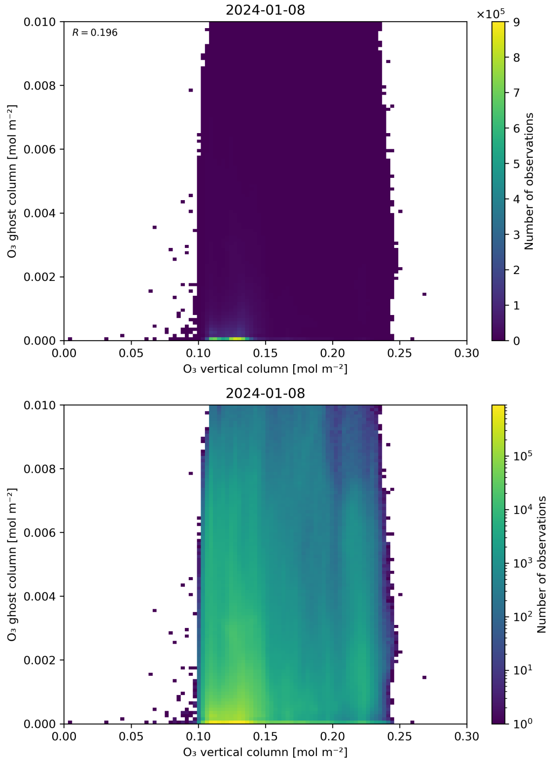
Figure 40: Scatter density plot of “O 3 vertical column” against “O 3 ghost column” for 2024-01-07 to 2024-01-09.
