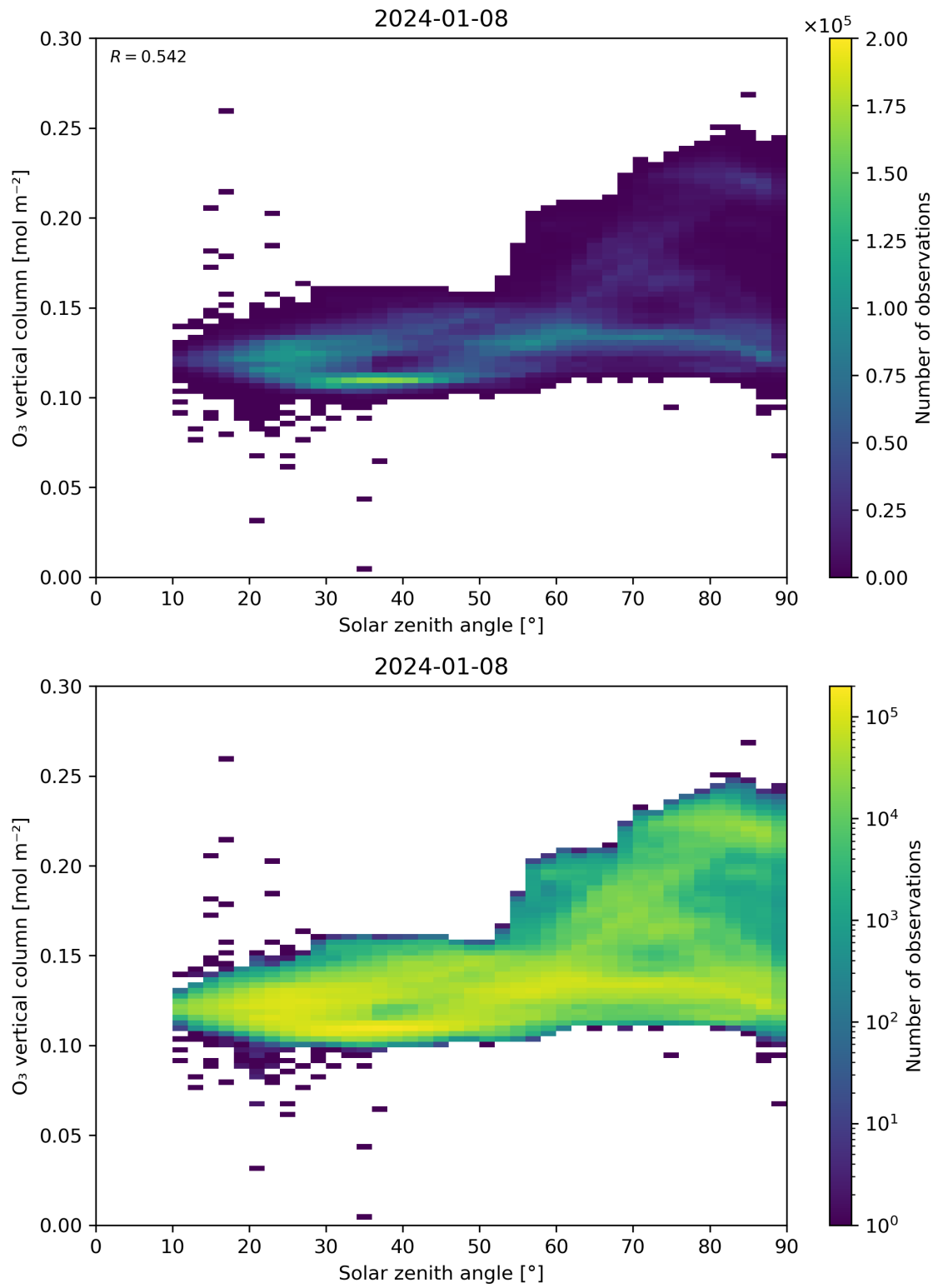
Figure 47: Scatter density plot of “Solar zenith angle” against “O 3 vertical column” for 2024-01-07 to 2024-01-09.
