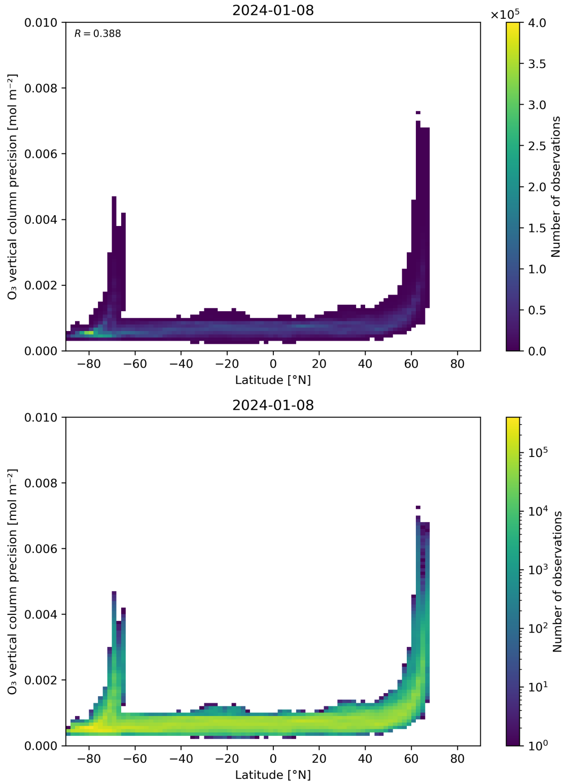
Figure 37: Scatter density plot of “Latitude” against “O 3 vertical column precision” for 2024-01-07 to 2024-01-09.
