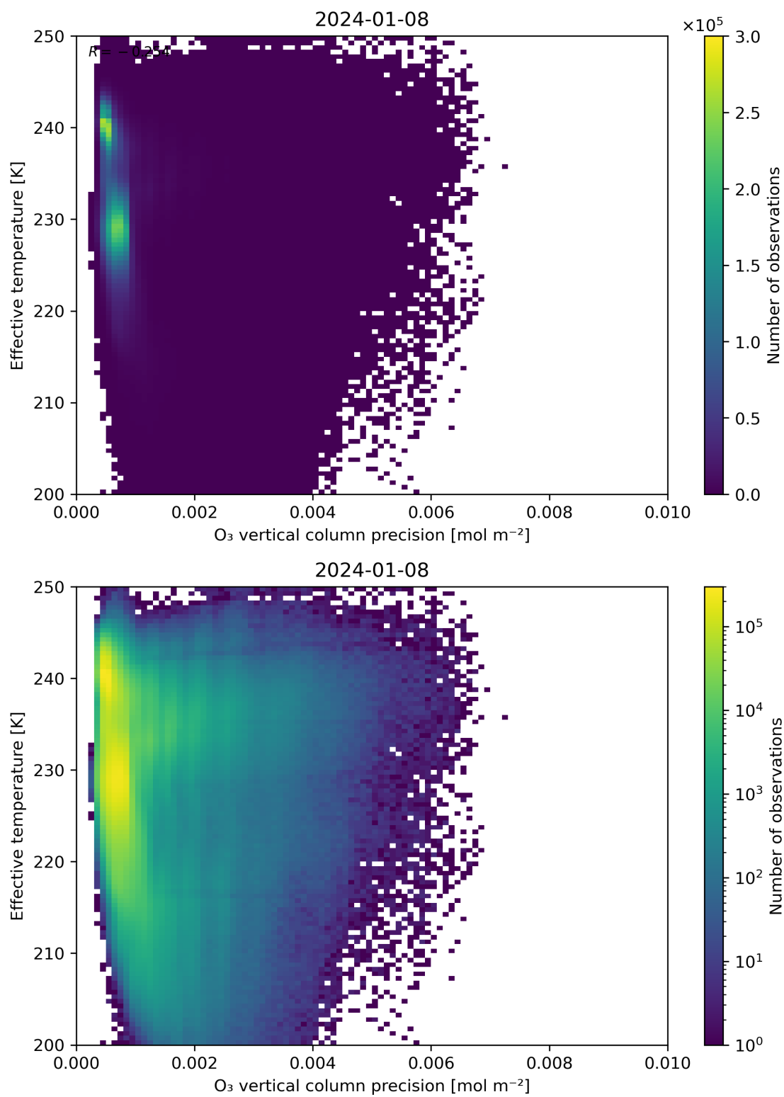
Figure 42: Scatter density plot of “ O_3 vertical column precision” against “Effective temperature” for 2024-01-07 to 2024-01-09.
