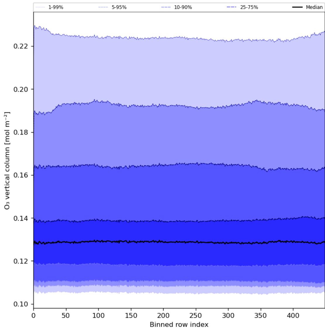
Figure 28: Along track statistics of “O 3 vertical column” for 2024-01-07 to 2024-01-09
