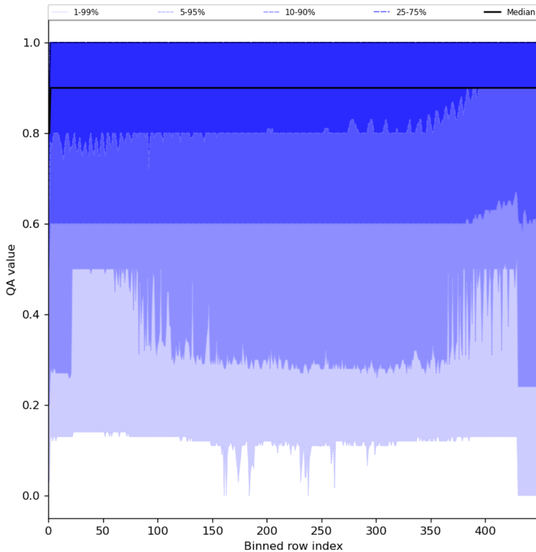
Figure 27: Along track statistics of “QA value” for 2024-01-07 to 2024-01-09
