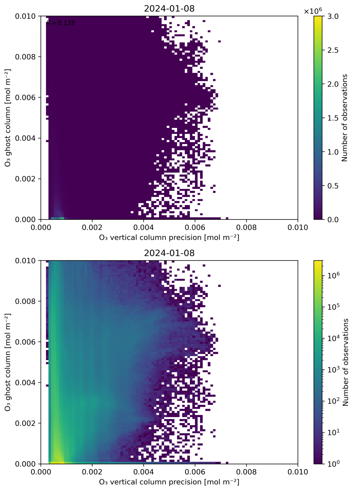
Figure 43: Scatter density plot of “ \text{O}_3 vertical column precision” against “ \text{O}_3 ghost column” for 2024-01-07 to 2024-01-09.
