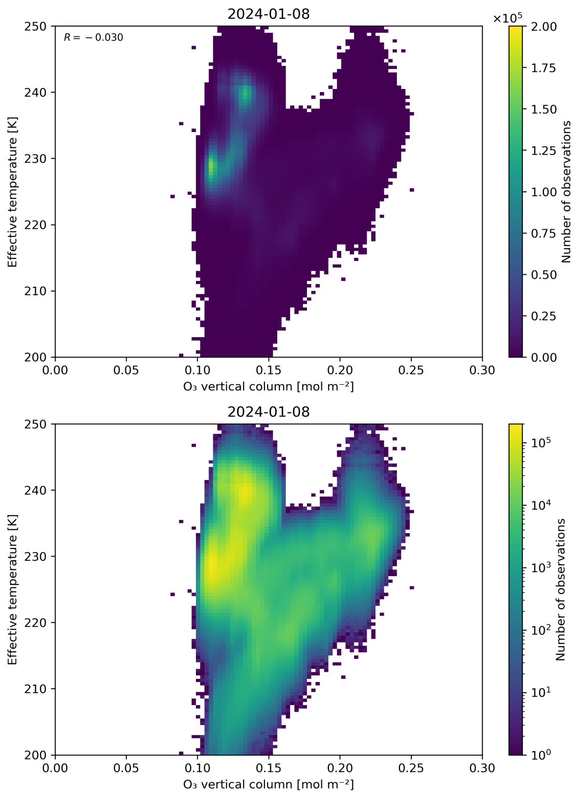
Figure 39: Scatter density plot of “O 3 vertical column” against “Effective temperature” for 2024-01-07 to 2024-01-09.
