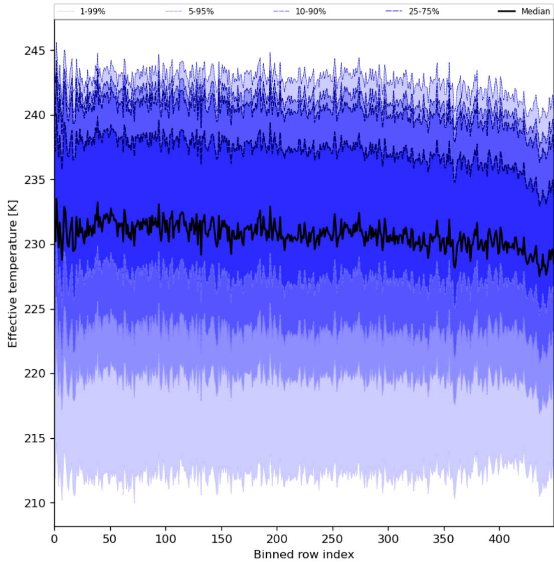
Figure 31: Along track statistics of “Effective temperature” for 2024-01-07 to 2024-01-09
