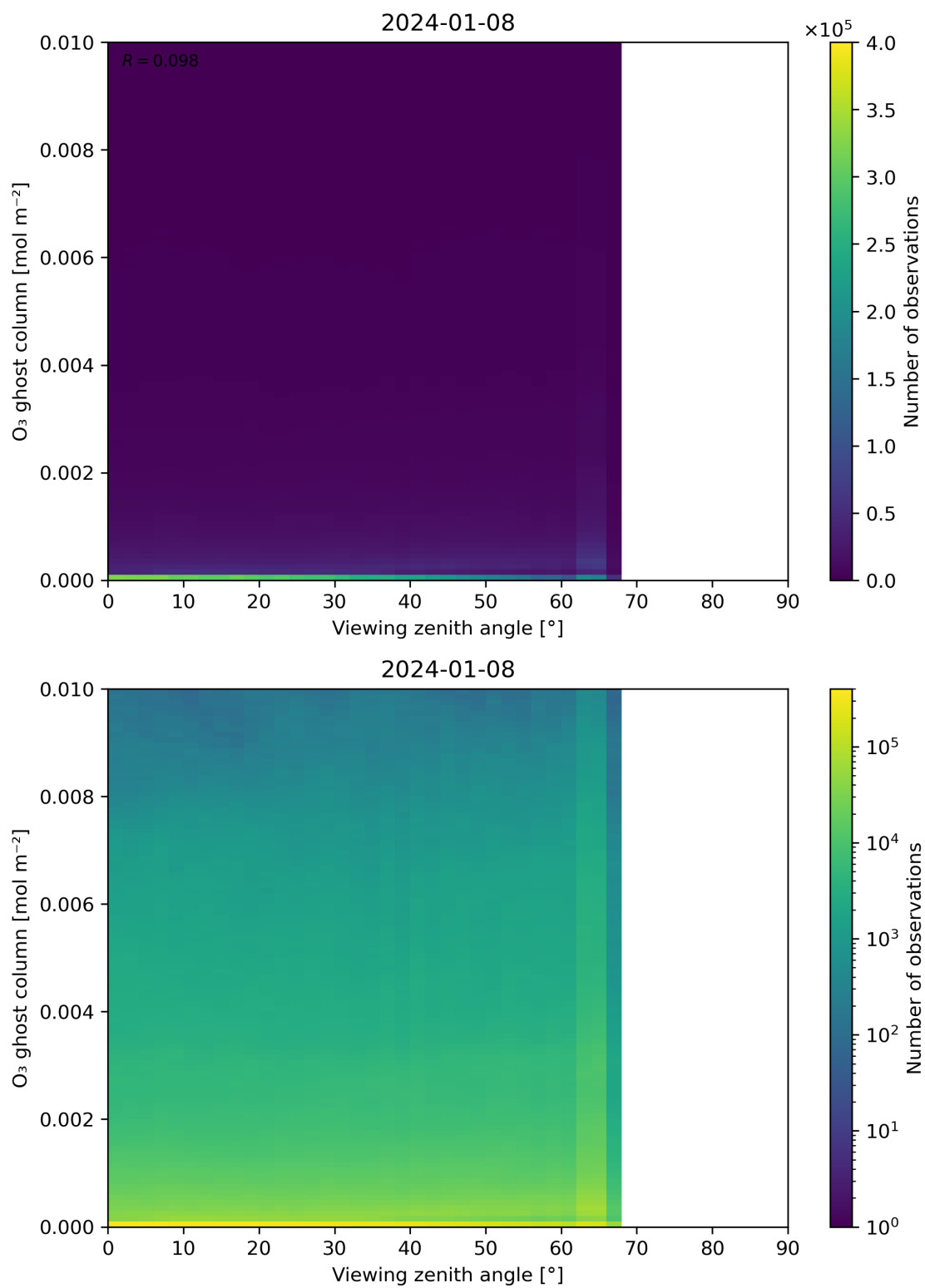
Figure 51: Scatter density plot of “Viewing zenith angle” against “O 3 ghost column” for 2024-01-07 to 2024-01-09.
