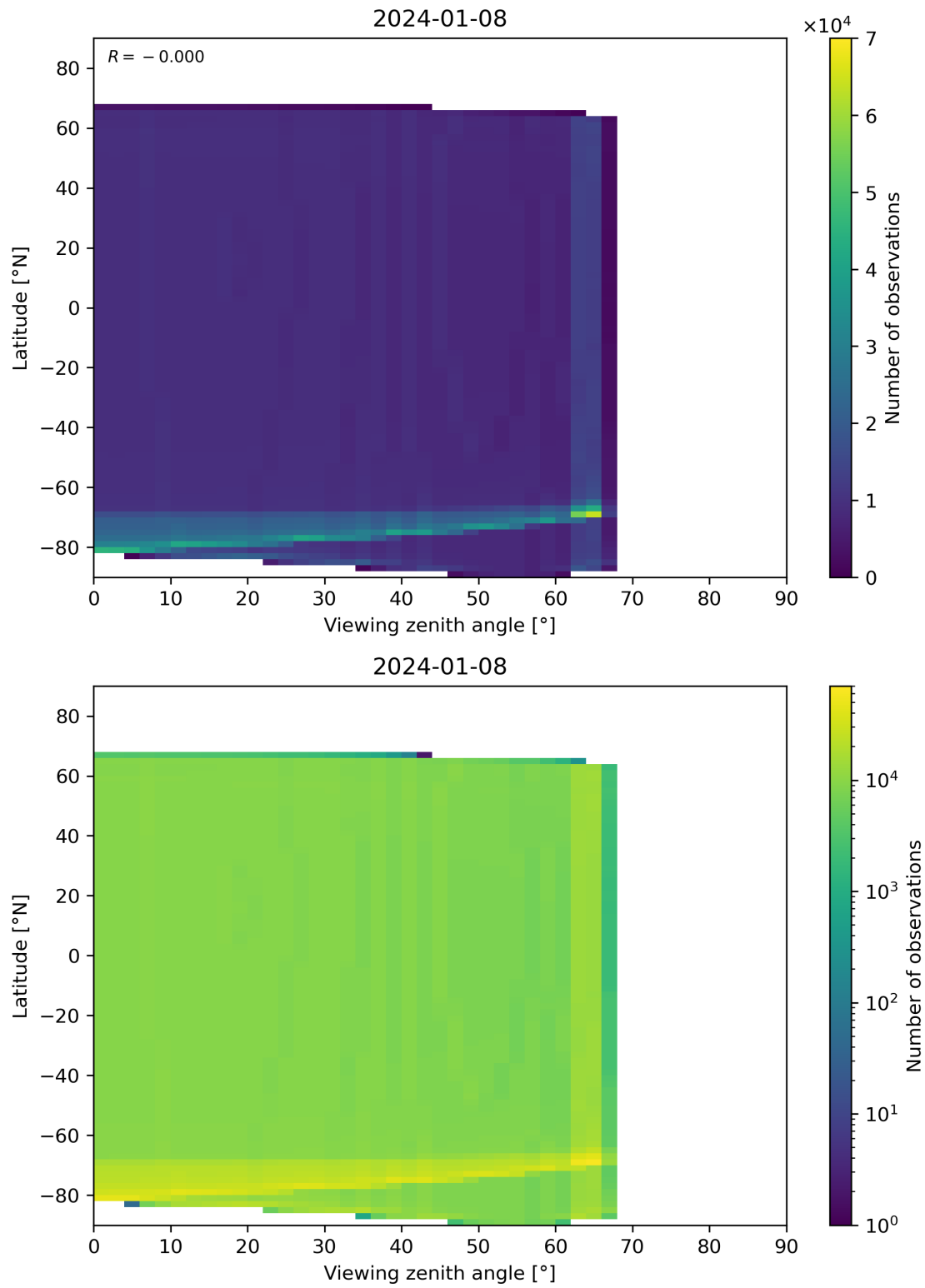
Figure 49: Scatter density plot of “Viewing zenith angle” against “Latitude” for 2024-01-07 to 2024-01-09.
