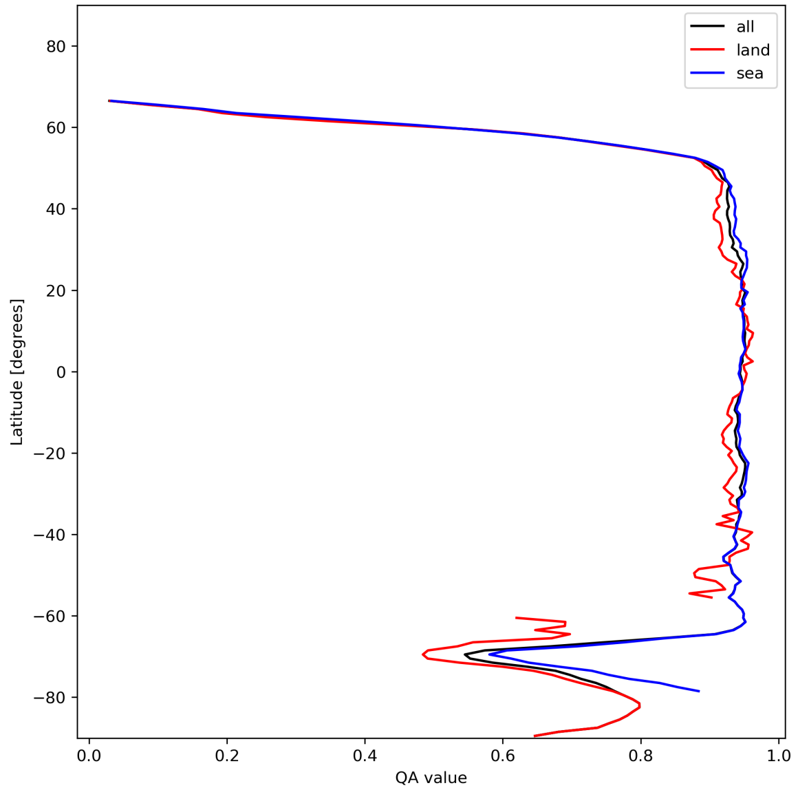
Figure 13: Zonal average of “QA value” for 2024-01-07 to 2024-01-09.
