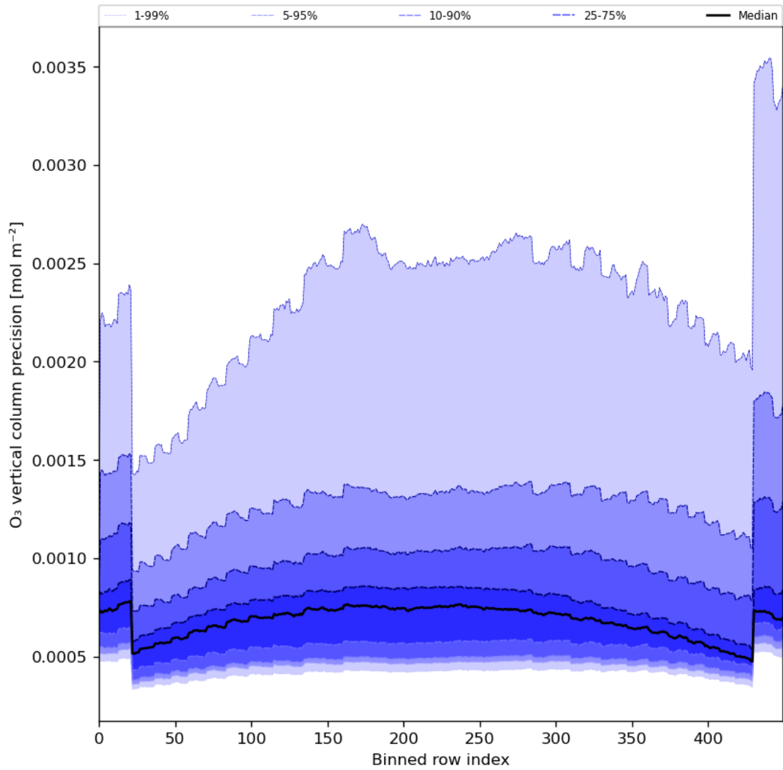
Figure 29: Along track statistics of “O 3 vertical column precision” for 2024-01-07 to 2024-01-09
