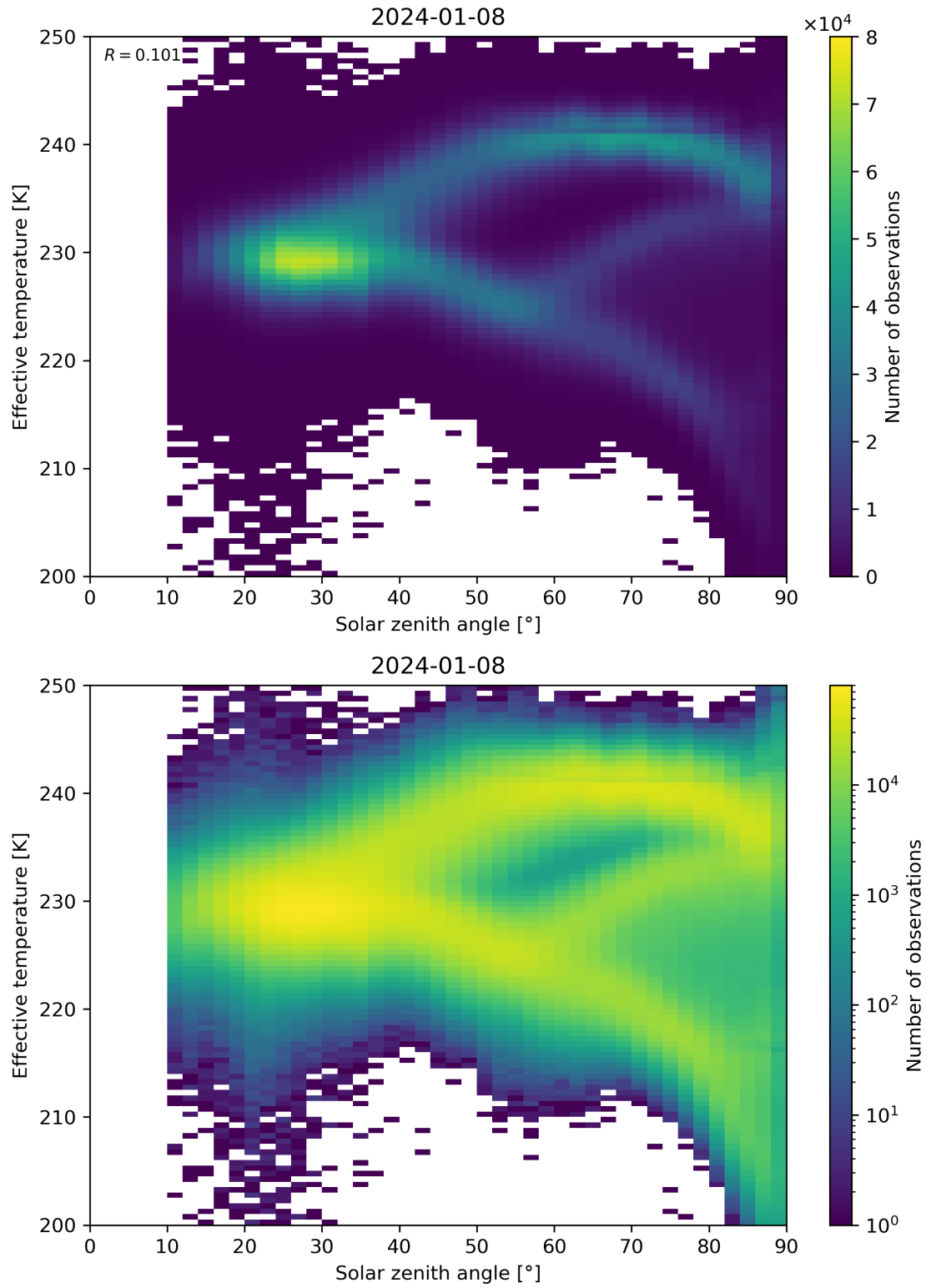
Figure 45: Scatter density plot of “Solar zenith angle” against “Effective temperature” for 2024-01-07 to 2024-01-09.
