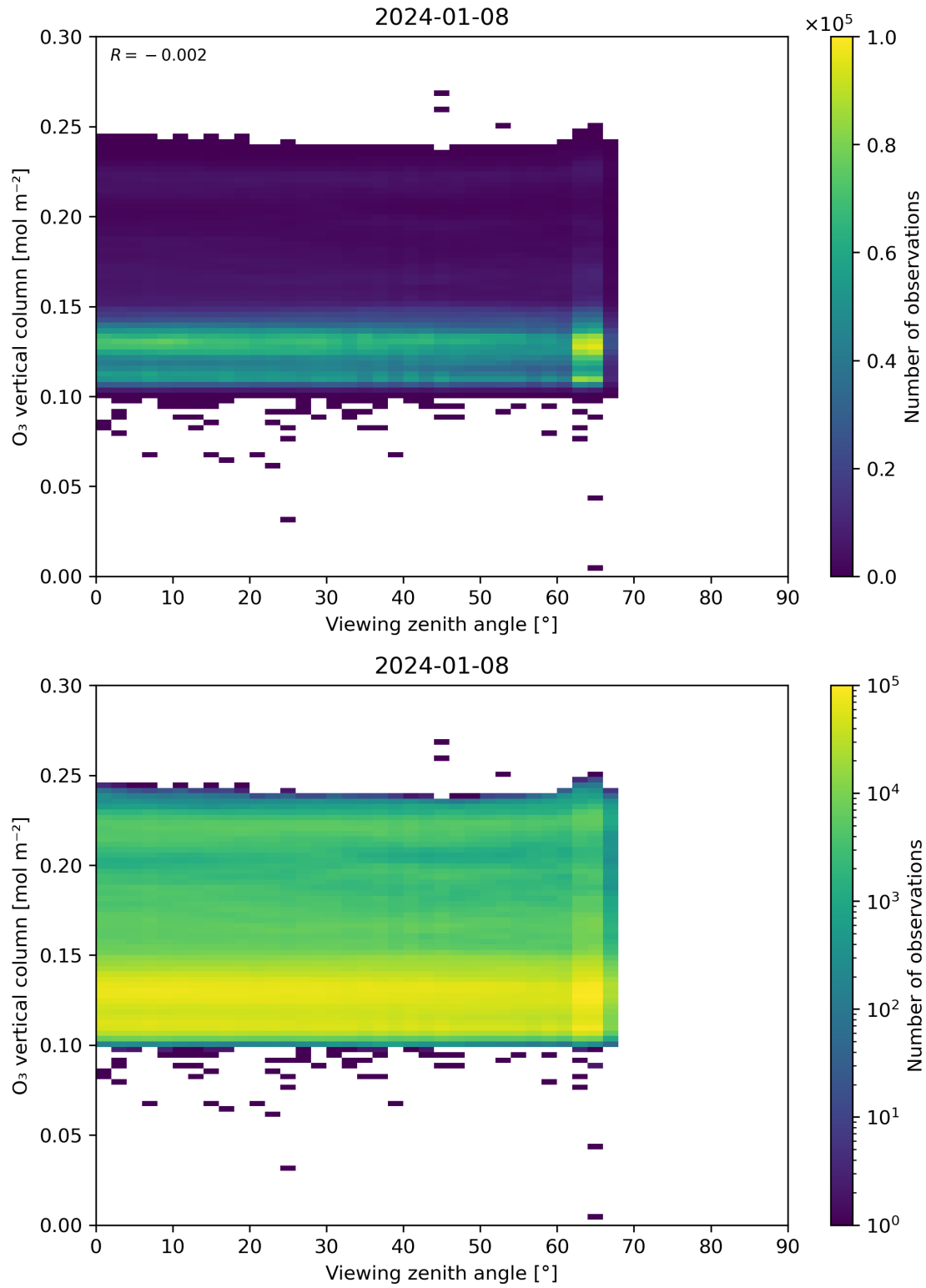
Figure 52: Scatter density plot of “Viewing zenith angle” against “O 3 vertical column” for 2024-01-07 to 2024-01-09.
