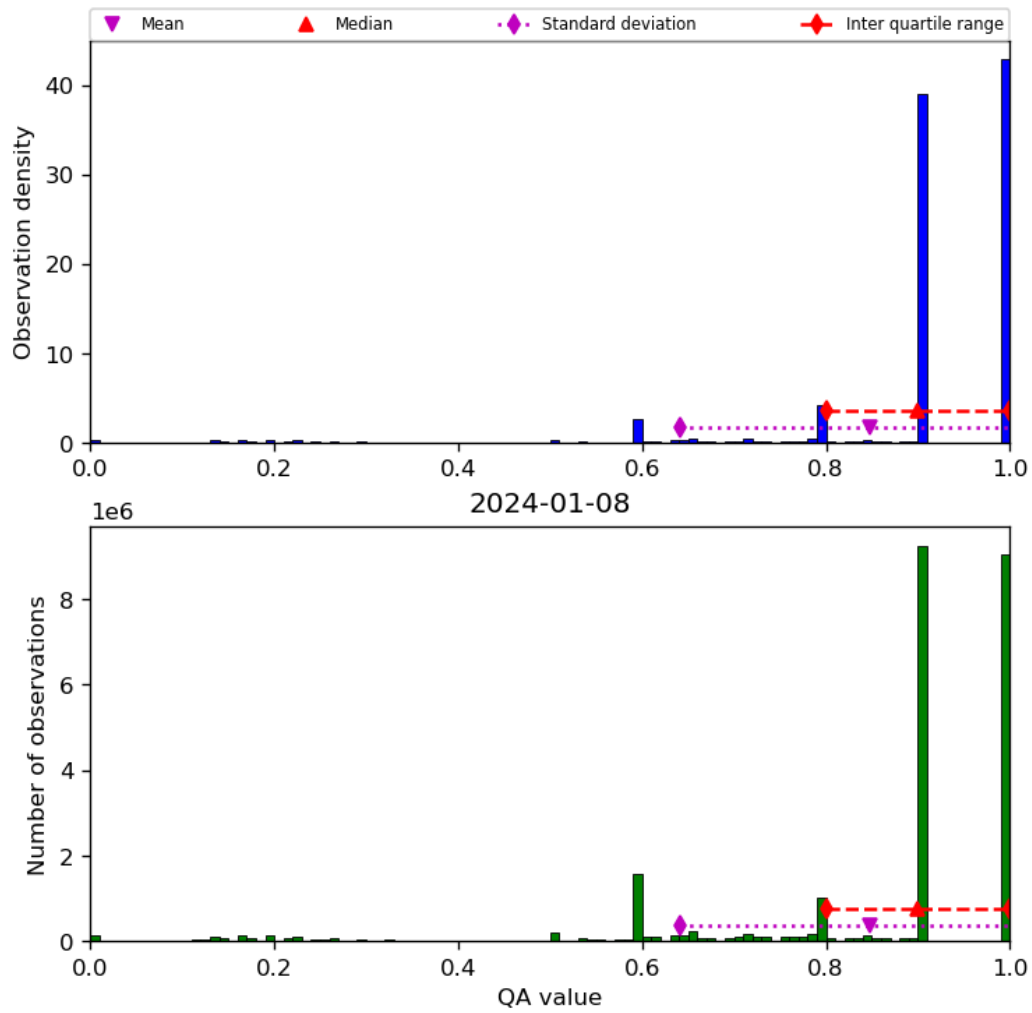
Figure 20: Histogram of “QA value” for 2024-01-07 to 2024-01-09
