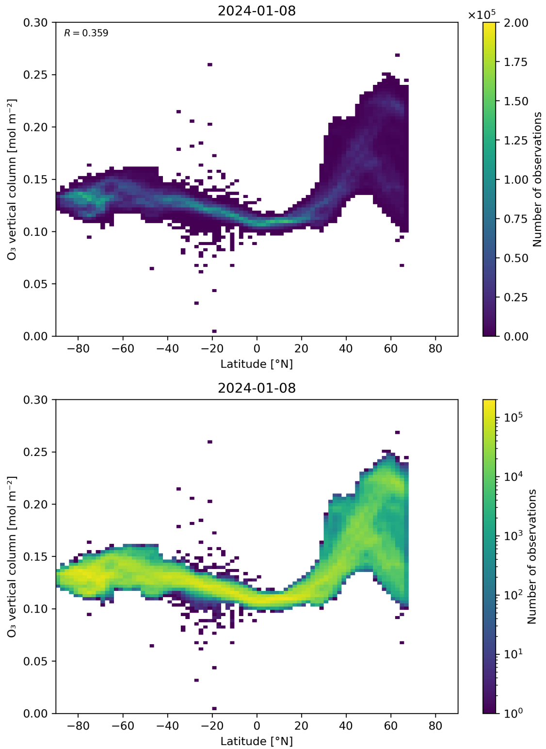
Figure 36: Scatter density plot of “Latitude” against “O 3 vertical column” for 2024-01-07 to 2024-01-09.
