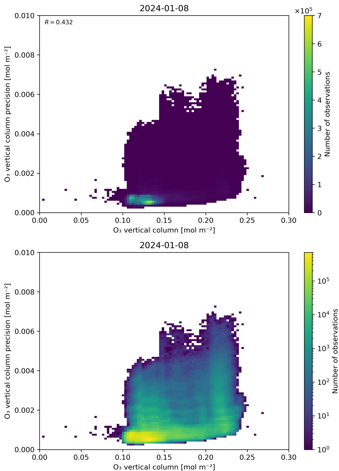
Figure 41: Scatter density plot of “O 3 vertical column” against “O 3 vertical column precision” for 2024-01-07 to 2024-01-09.
