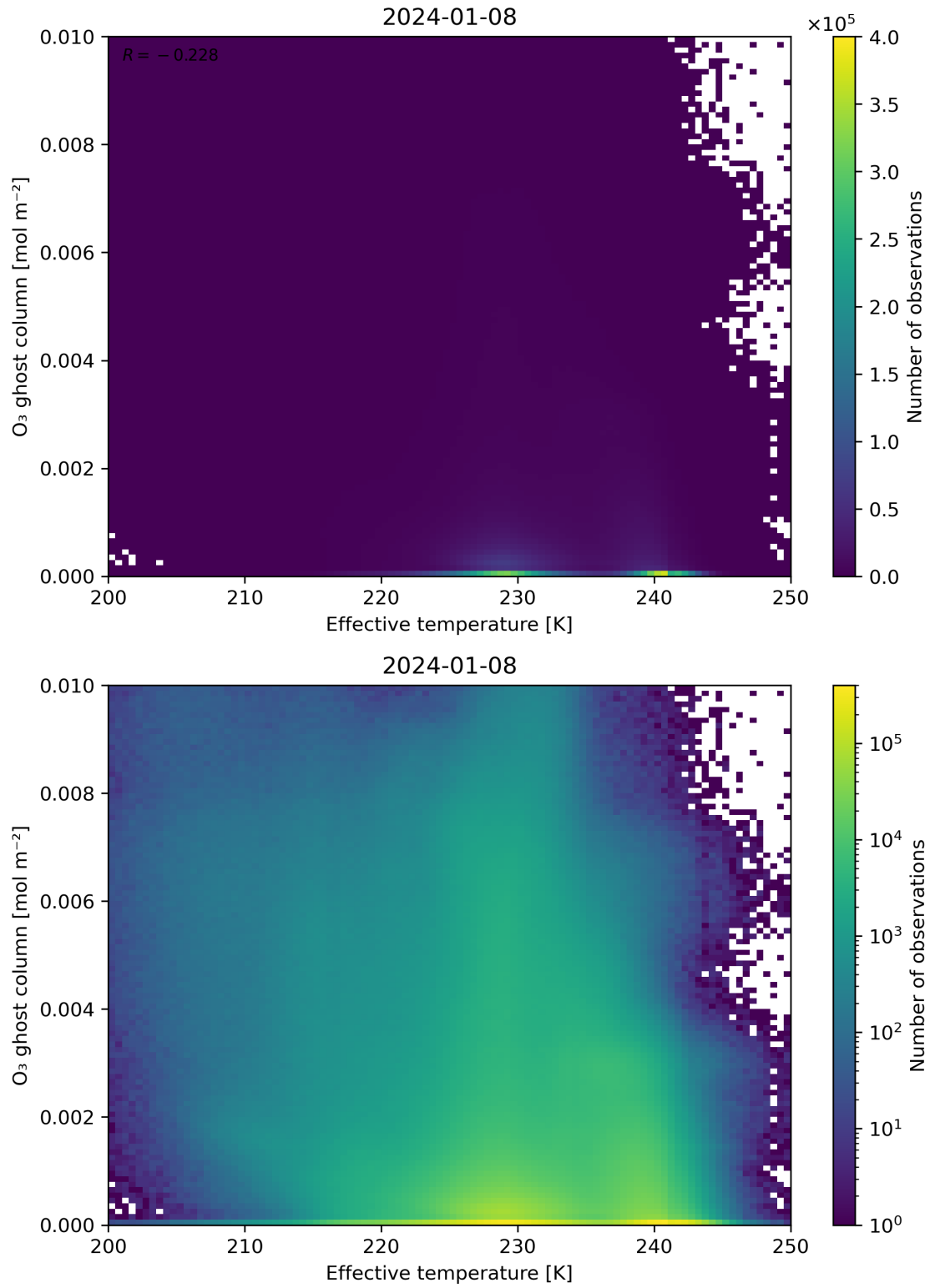
Figure 38: Scatter density plot of “Effective temperature” against “O 3 ghost column” for 2024-01-07 to 2024-01-09.
