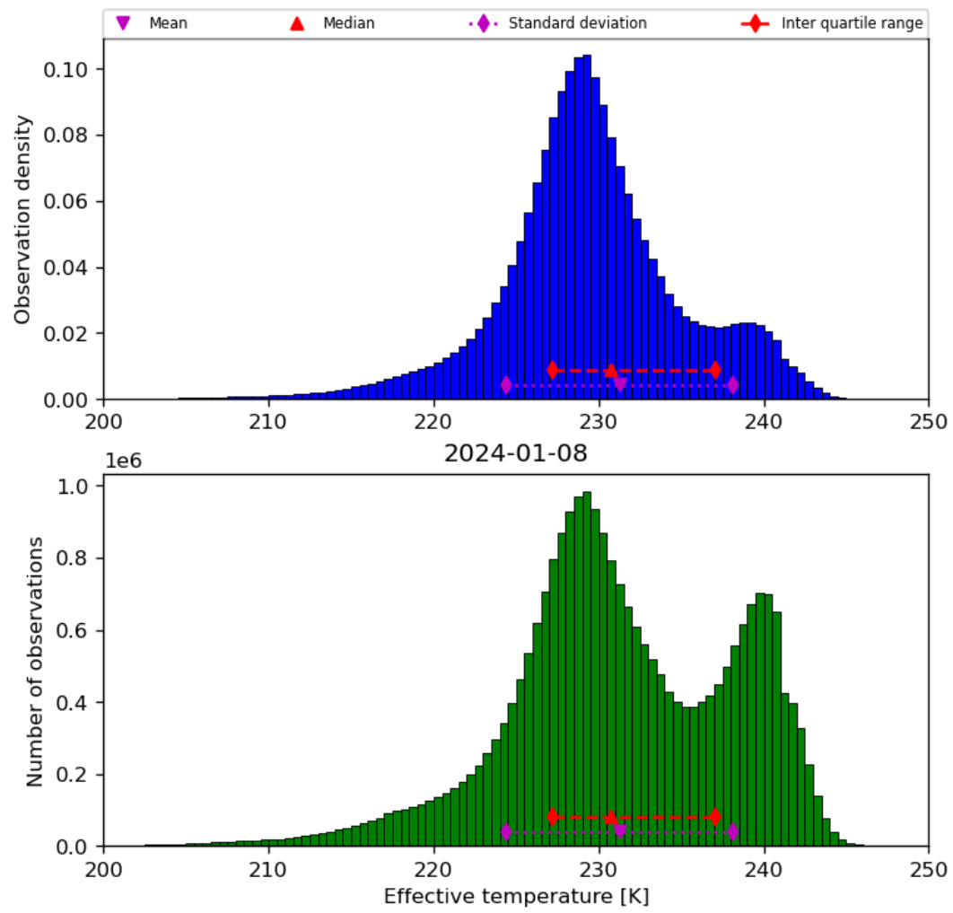
Figure 24: Histogram of “Effective temperature” for 2024-01-07 to 2024-01-09
