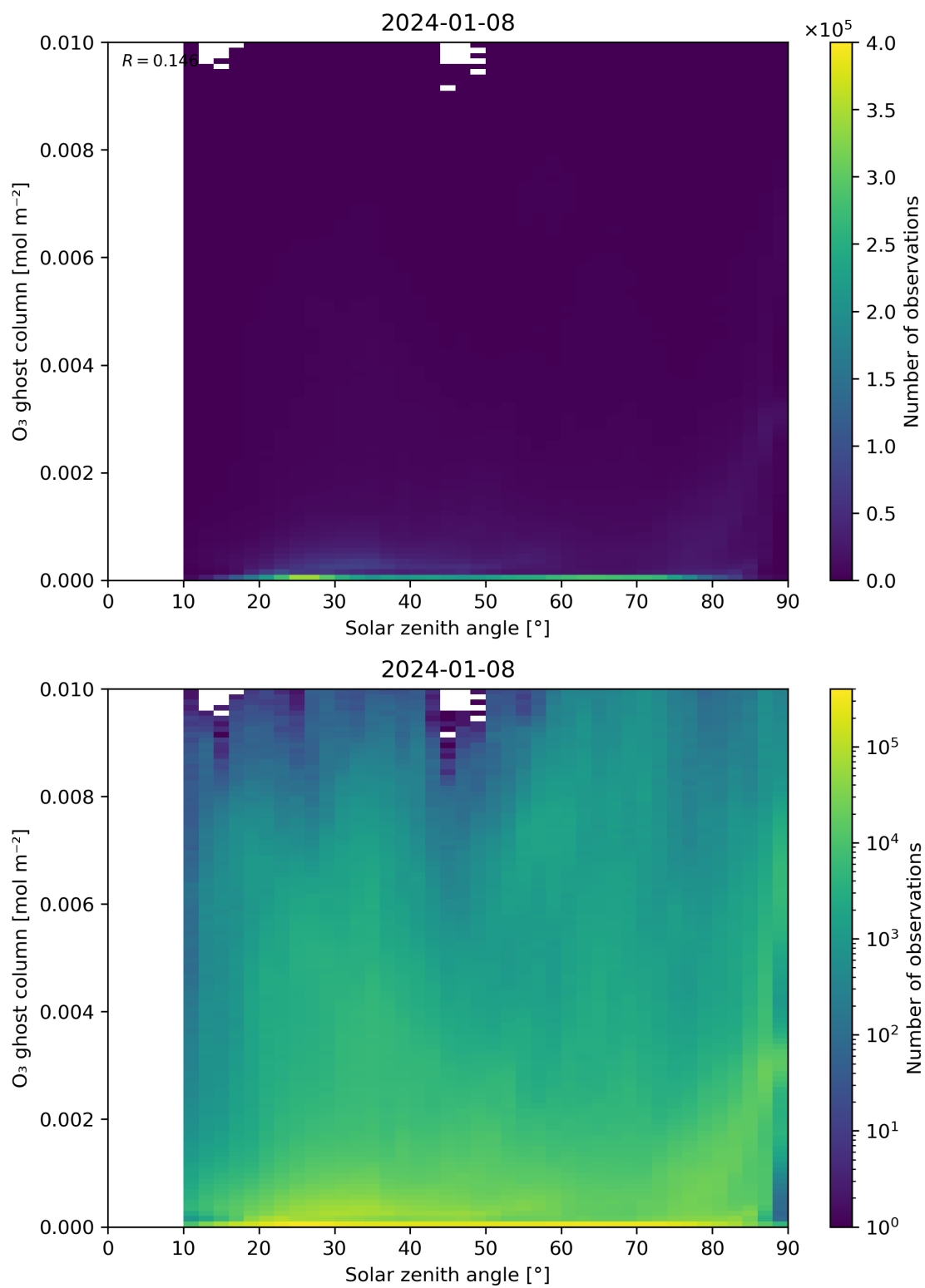
Figure 46: Scatter density plot of “Solar zenith angle” against “O 3 ghost column” for 2024-01-07 to 2024-01-09.
