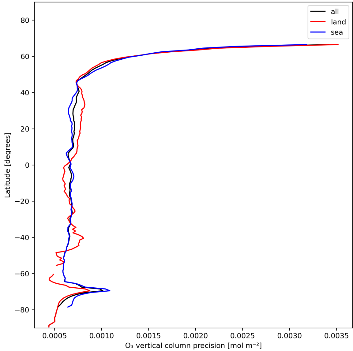
Figure 15: Zonal average of “O 3 vertical column precision” for 2024-01-07 to 2024-01-09.
