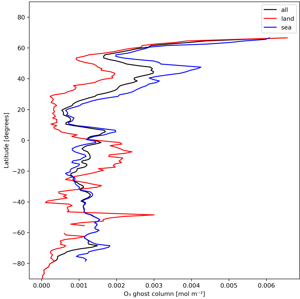
Figure 18: Zonal average of “O 3 ghost column” for 2024-01-07 to 2024-01-09.
