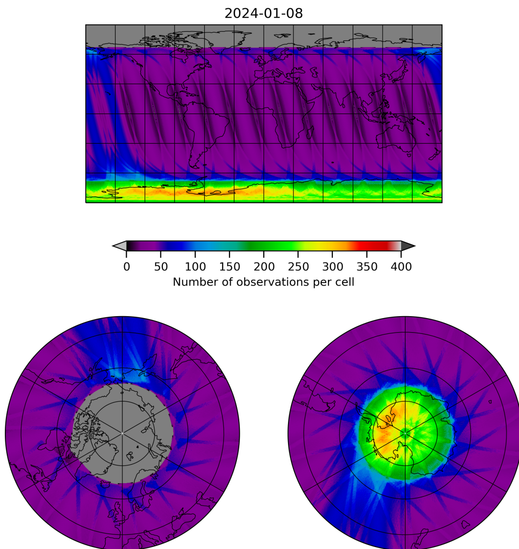
Figure 12: Map of the number of observations for 2024-01-07 to 2024-01-09
