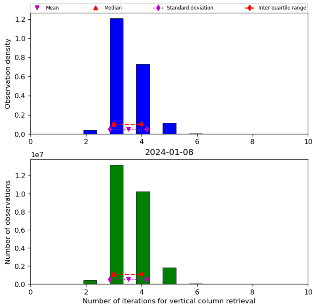
Figure 26: Histogram of “Number of iterations for vertical column retrieval” for 2024-01-07 to 2024-01-09
