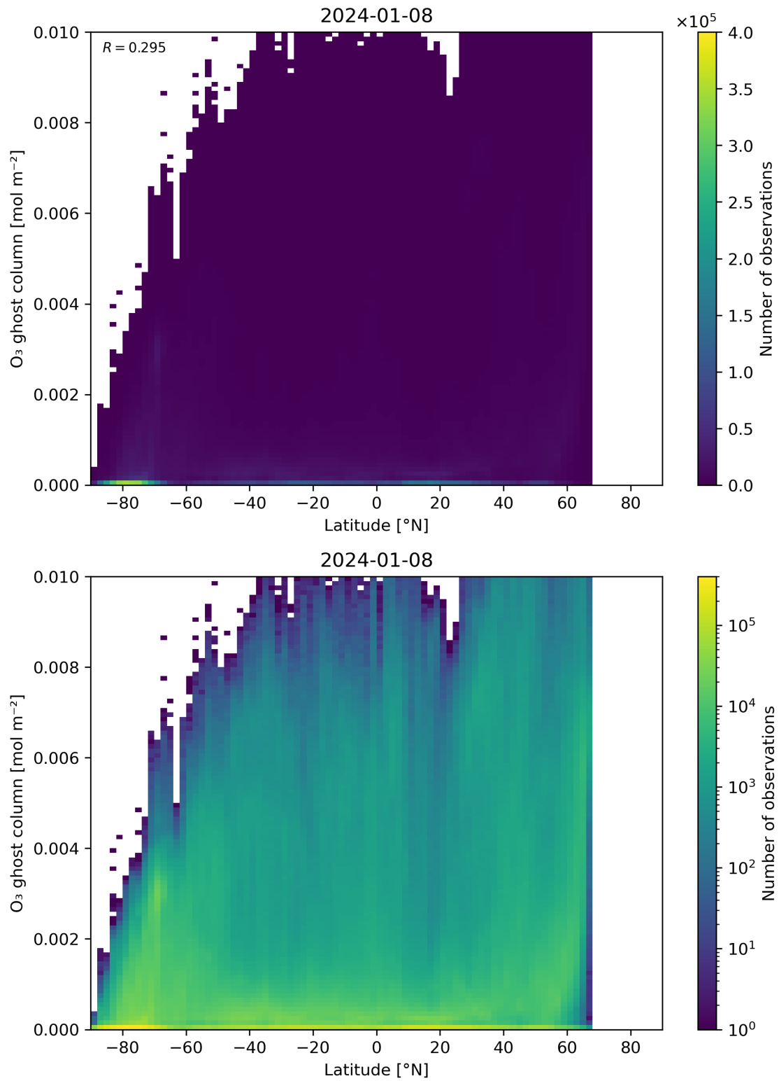
Figure 35: Scatter density plot of “Latitude” against “O 3 ghost column” for 2024-01-07 to 2024-01-09.
