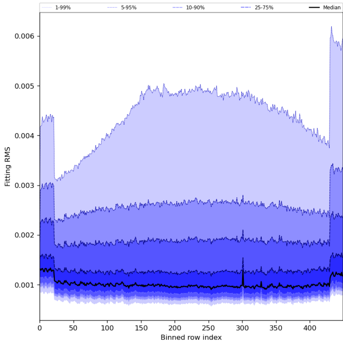
Figure 30: Along track statistics of “Fitting RMS” for 2024-01-07 to 2024-01-09
