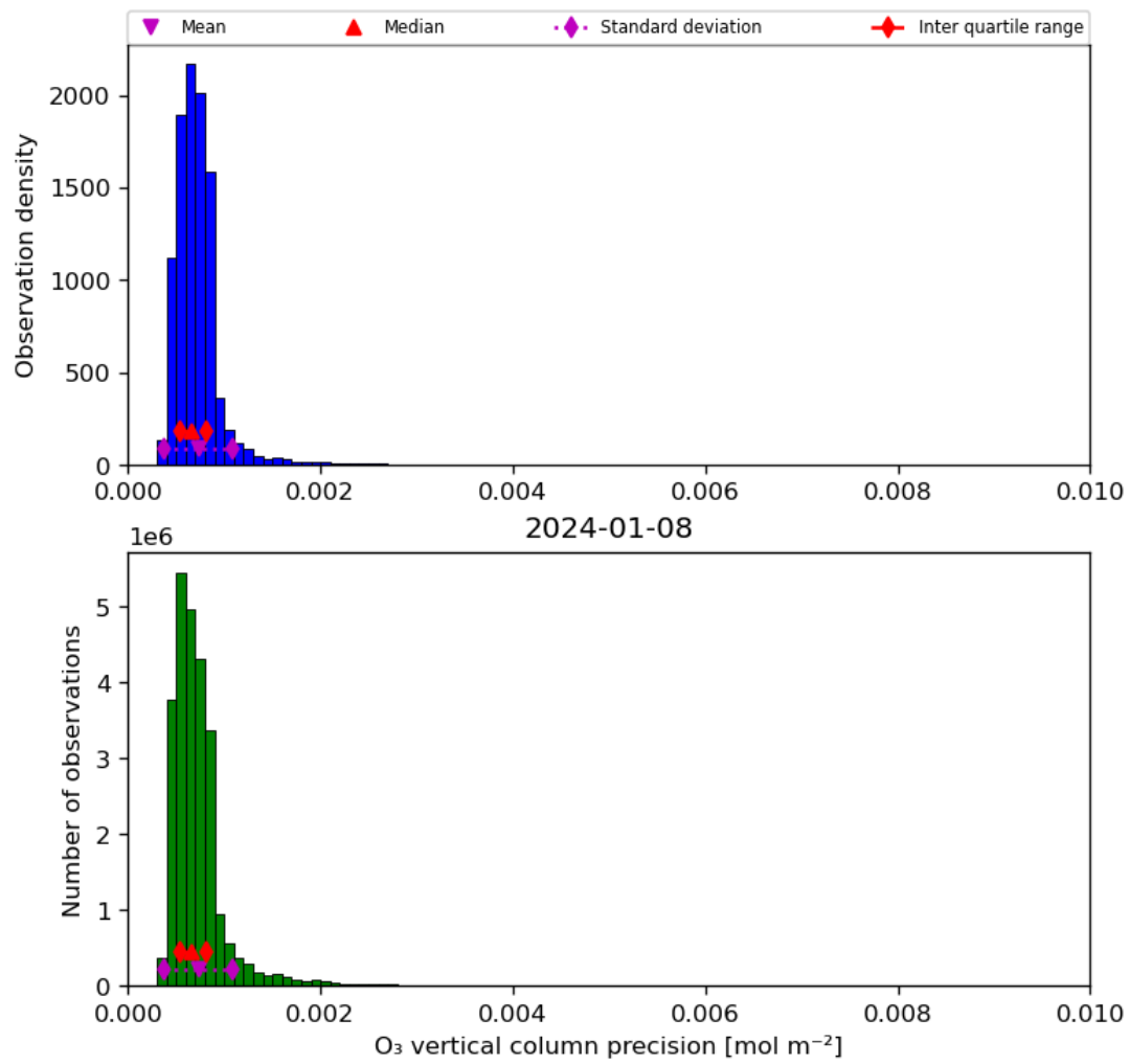
Figure 22: Histogram of “O 3 vertical column precision” for 2024-01-07 to 2024-01-09
