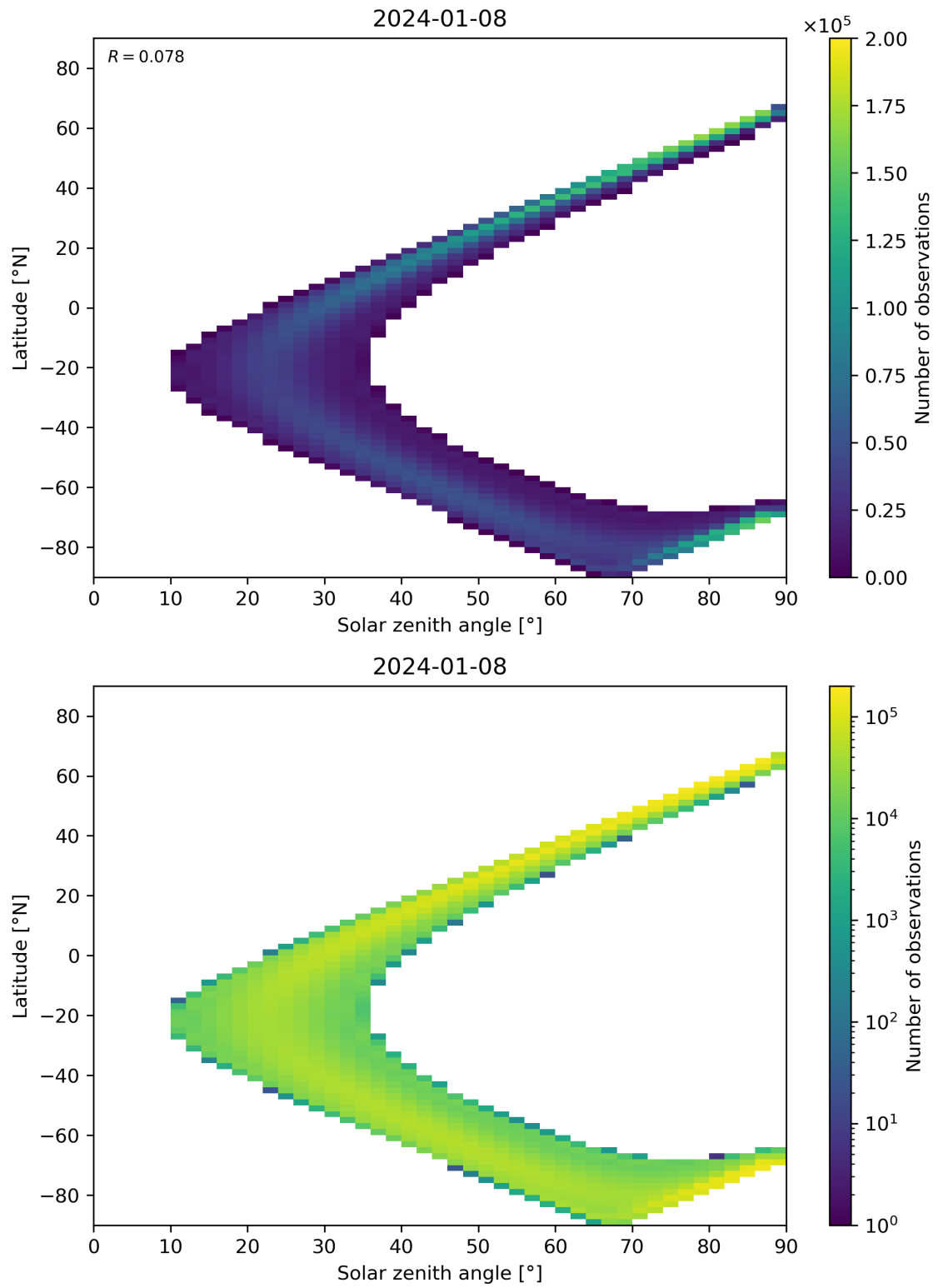
Figure 44: Scatter density plot of “Solar zenith angle” against “Latitude” for 2024-01-07 to 2024-01-09.
