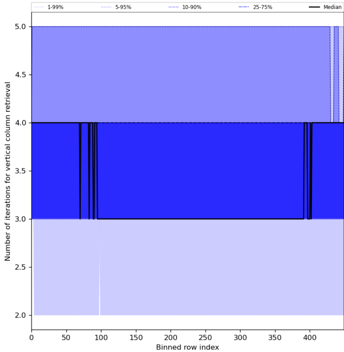
Figure 33: Along track statistics of “Number of iterations for vertical column retrieval” for 2024-01-07 to 2024-01-09
