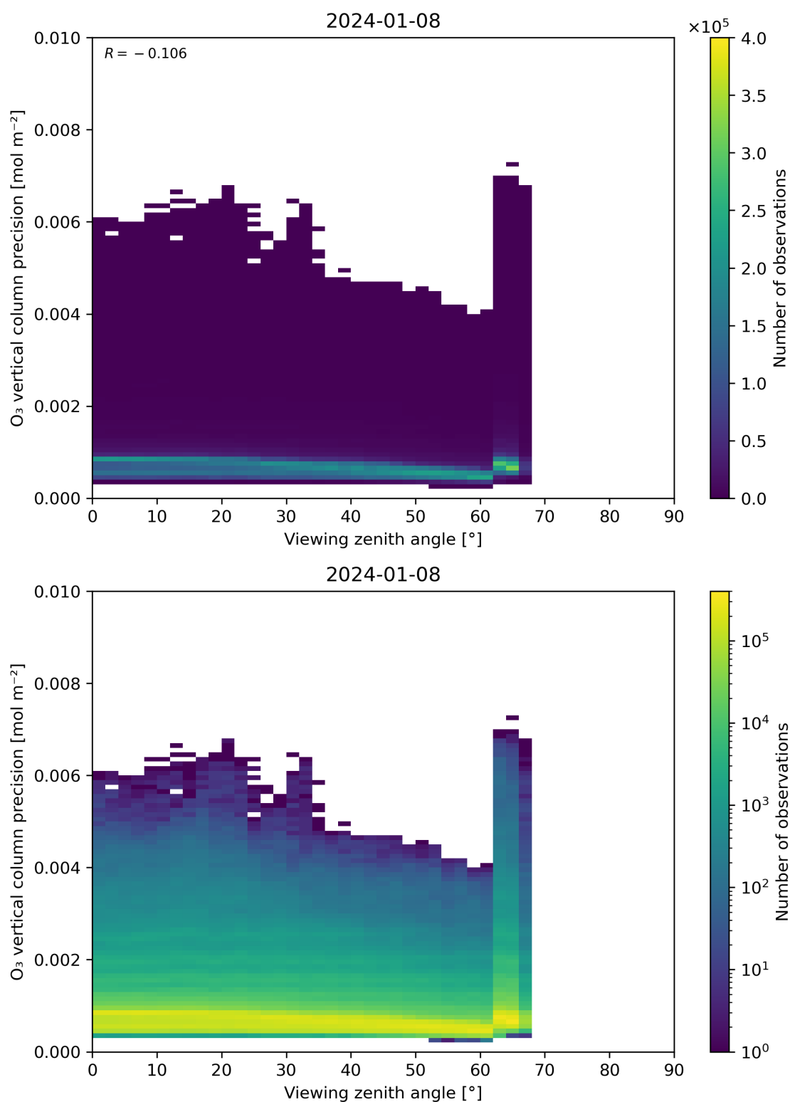
Figure 53: Scatter density plot of “Viewing zenith angle” against “O 3 vertical column precision” for 2024-01-07 to 2024-01-09.
