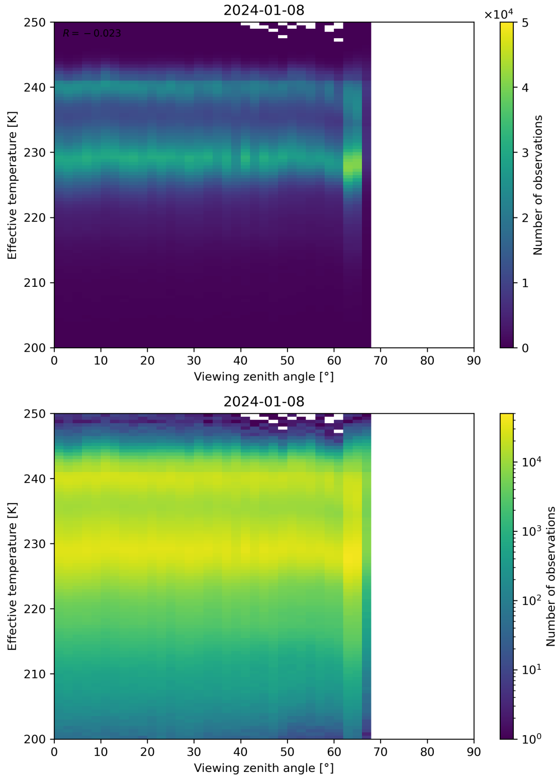
Figure 50: Scatter density plot of “Viewing zenith angle” against “Effective temperature” for 2024-01-07 to 2024-01-09.
