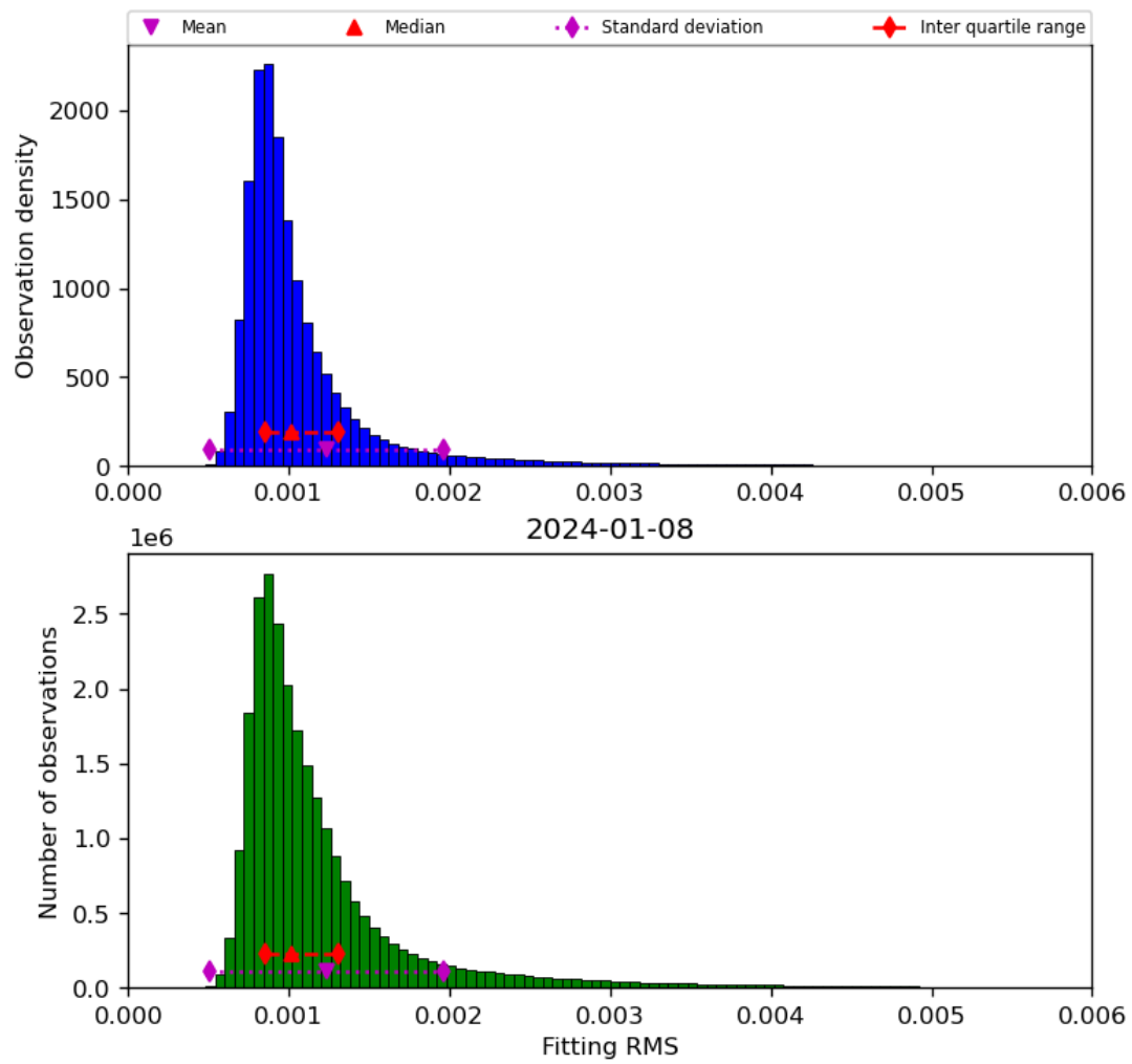
Figure 23: Histogram of “Fitting RMS” for 2024-01-07 to 2024-01-09
