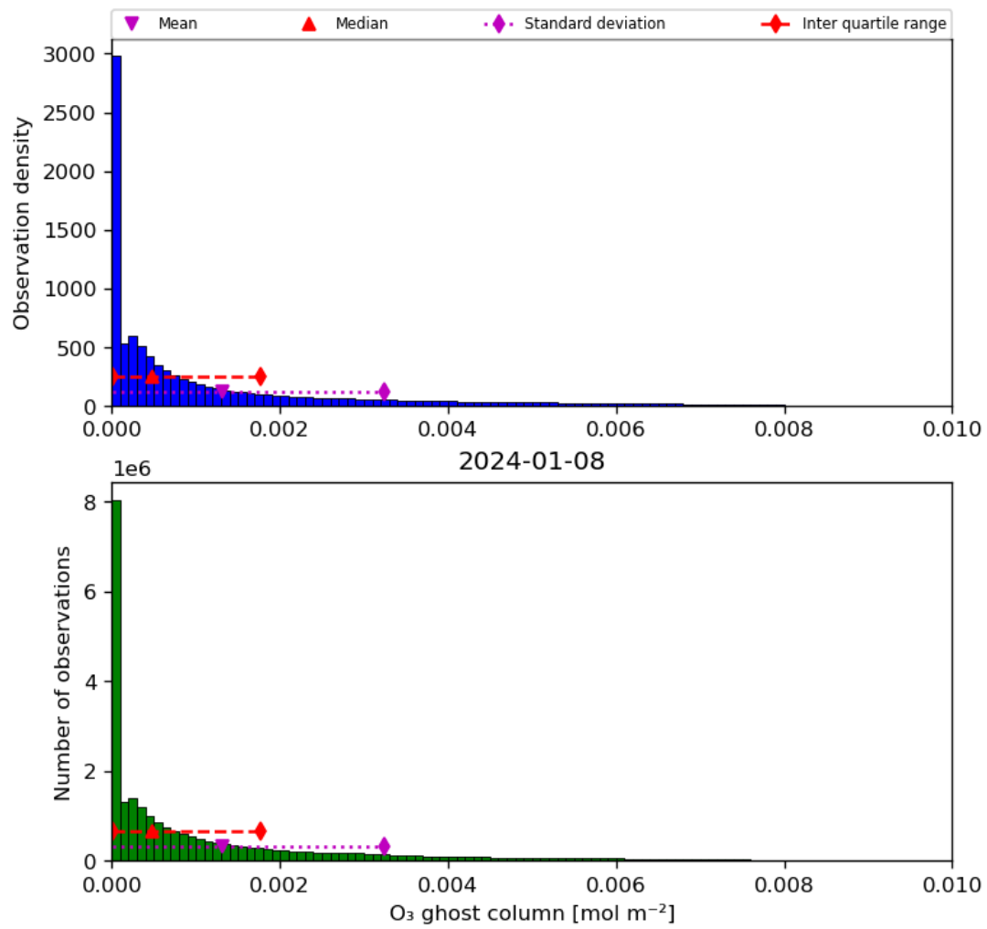
Figure 25: Histogram of “O 3 ghost column” for 2024-01-07 to 2024-01-09
