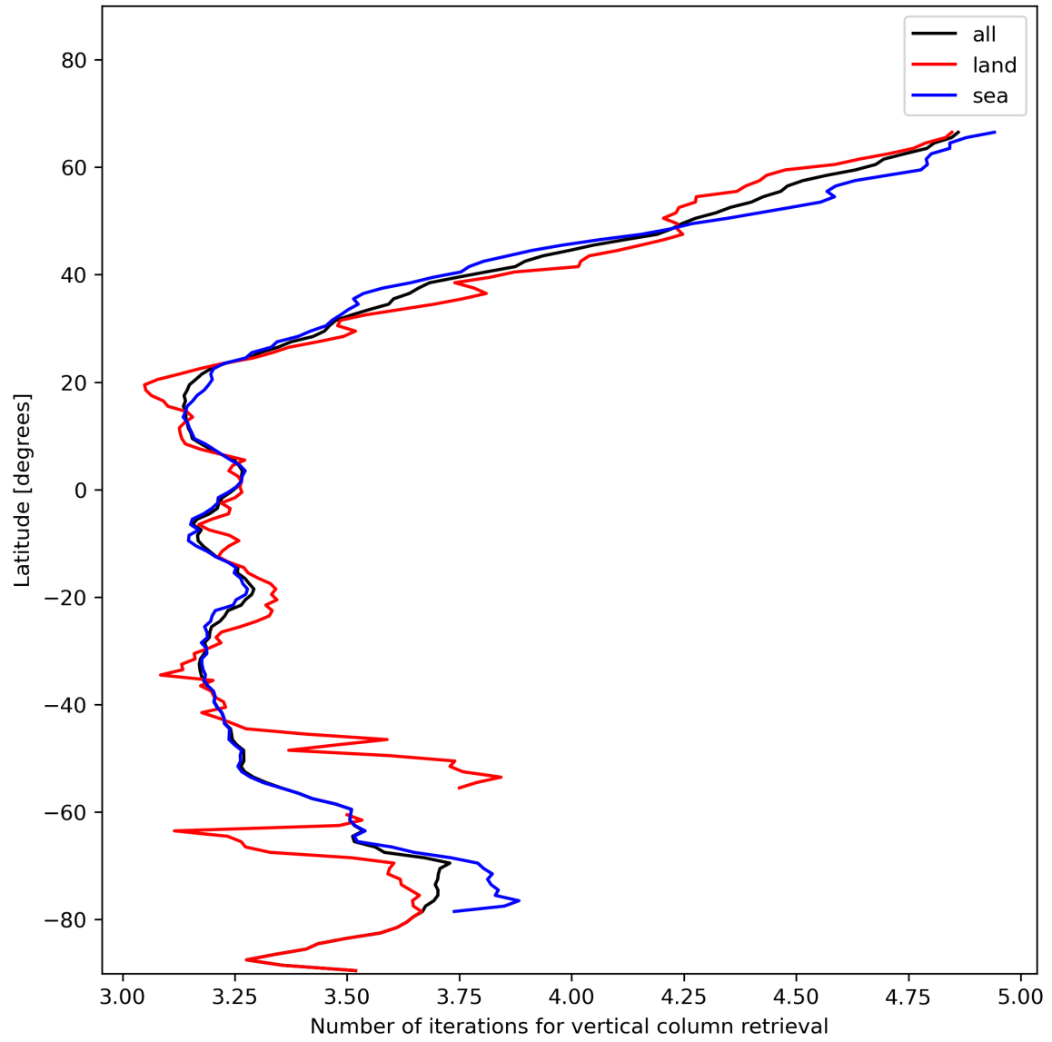
Figure 19: Zonal average of “Number of iterations for vertical column retrieval” for 2024-01-07 to 2024-01-09.
