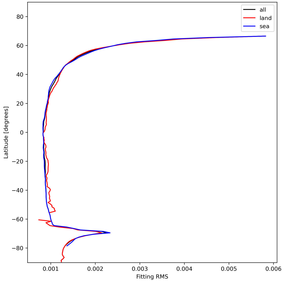
Figure 16: Zonal average of “Fitting RMS” for 2024-01-07 to 2024-01-09.
