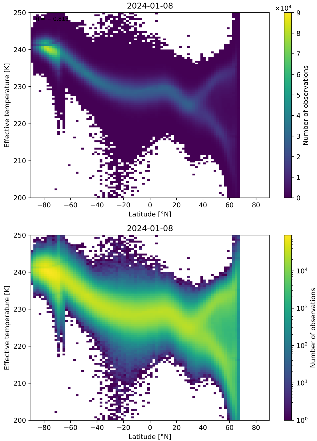
Figure 34: Scatter density plot of “Latitude” against “Effective temperature” for 2024-01-07 to 2024-01-09.
