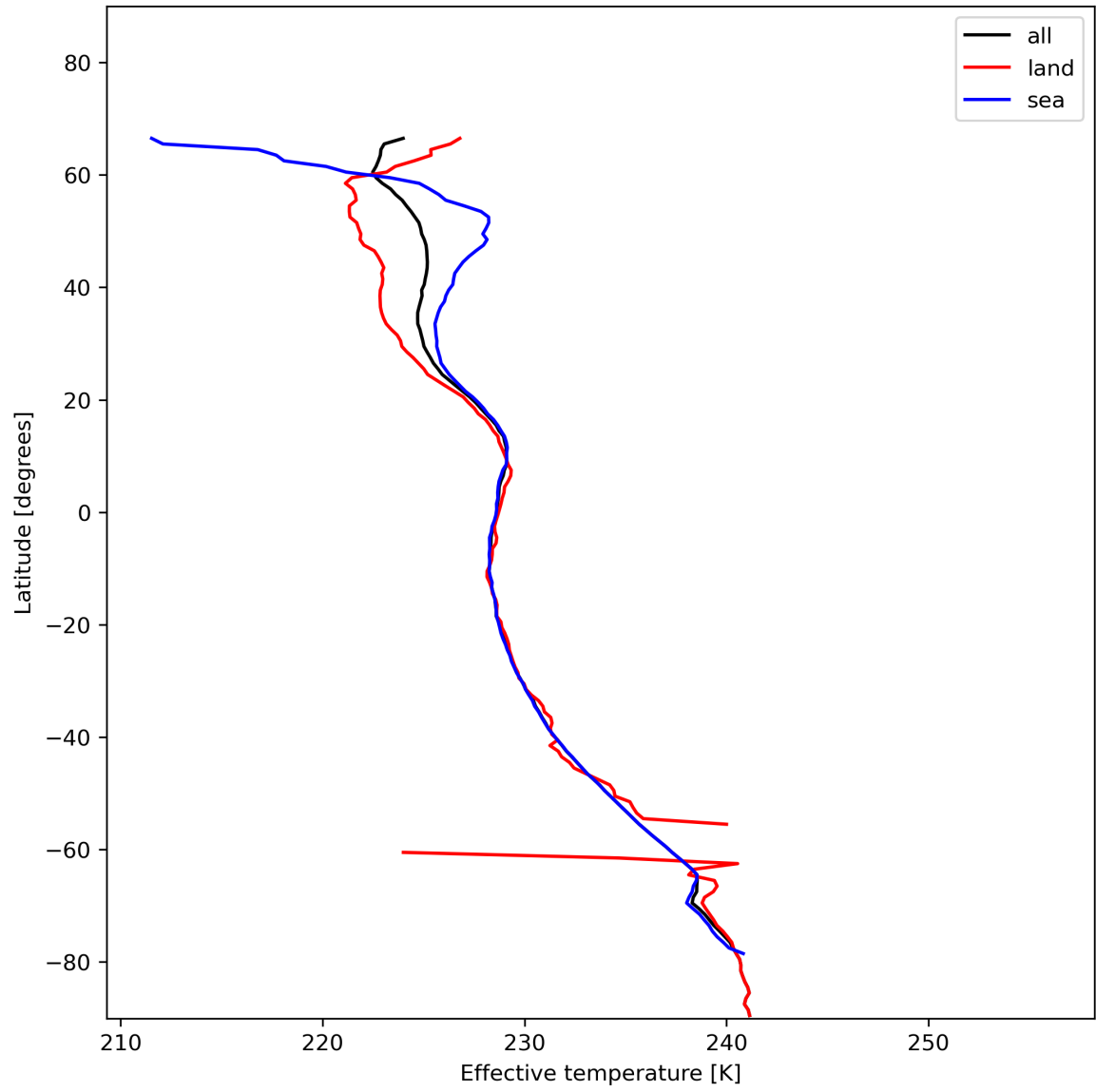
Figure 17: Zonal average of “Effective temperature” for 2024-01-07 to 2024-01-09.
