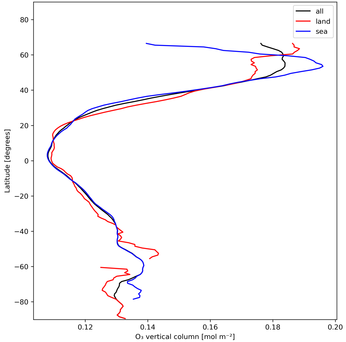
Figure 14: Zonal average of “O 3 vertical column” for 2024-01-07 to 2024-01-09.
