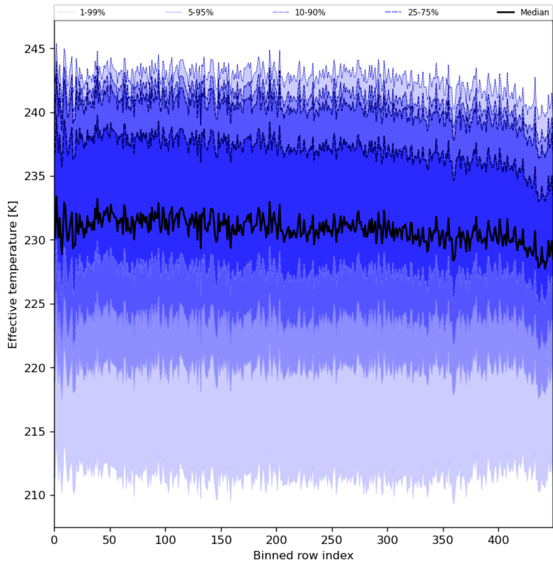
Figure 31: Along track statistics of “Effective temperature” for 2024-01-08 to 2024-01-10
