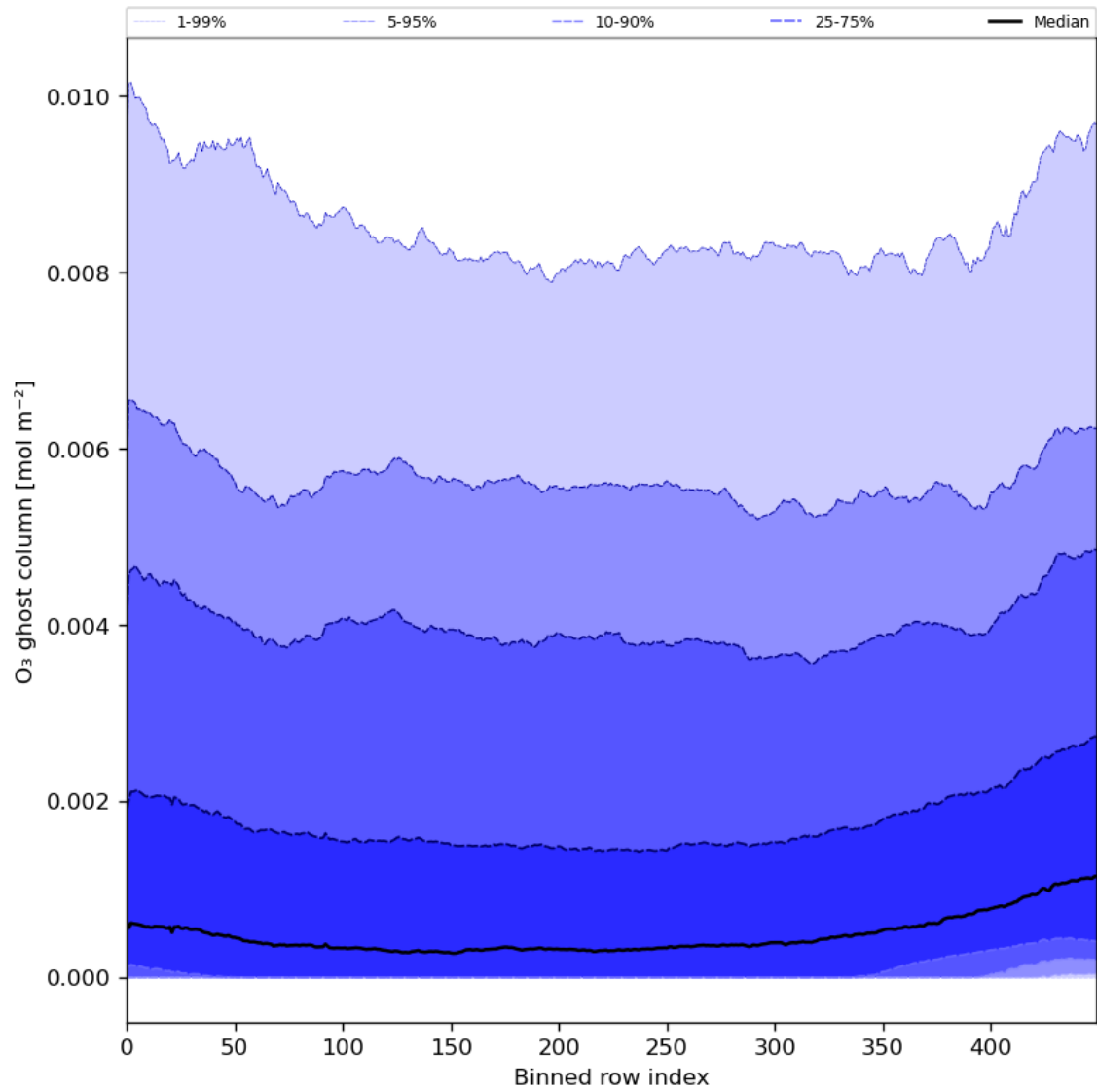
Figure 32: Along track statistics of “O 3 ghost column” for 2024-01-08 to 2024-01-10
