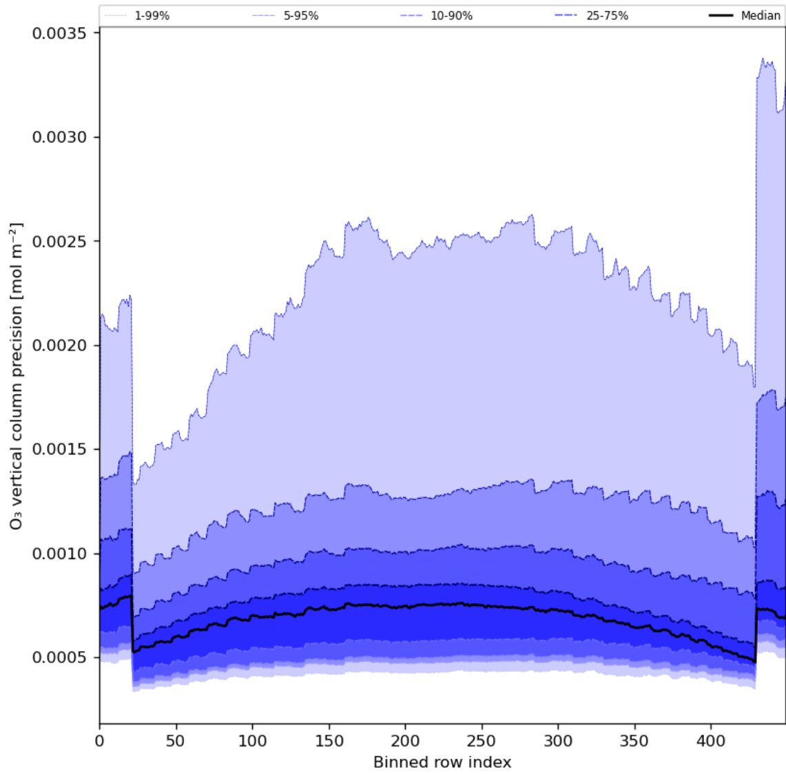
Figure 29: Along track statistics of “O 3 vertical column precision” for 2024-01-08 to 2024-01-10
