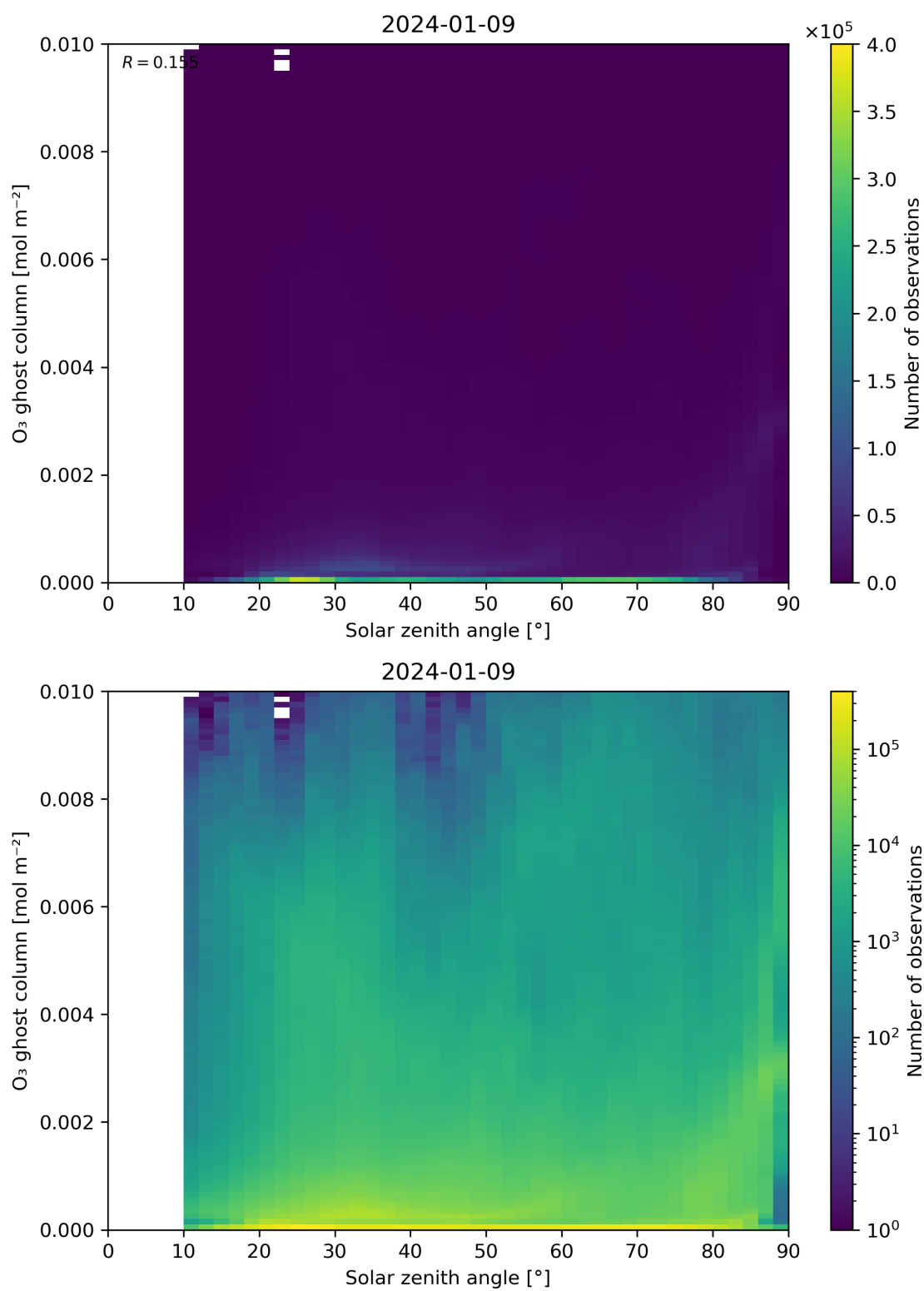
Figure 46: Scatter density plot of “Solar zenith angle” against “O 3 ghost column” for 2024-01-08 to 2024-01-10.
