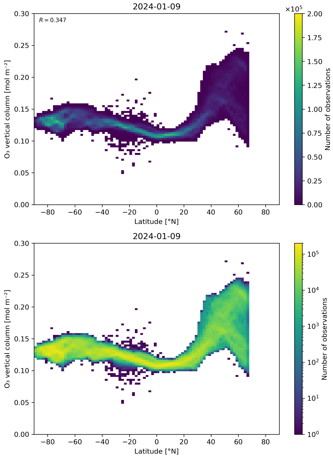
Figure 36: Scatter density plot of “Latitude” against “O 3 vertical column” for 2024-01-08 to 2024-01-10.
