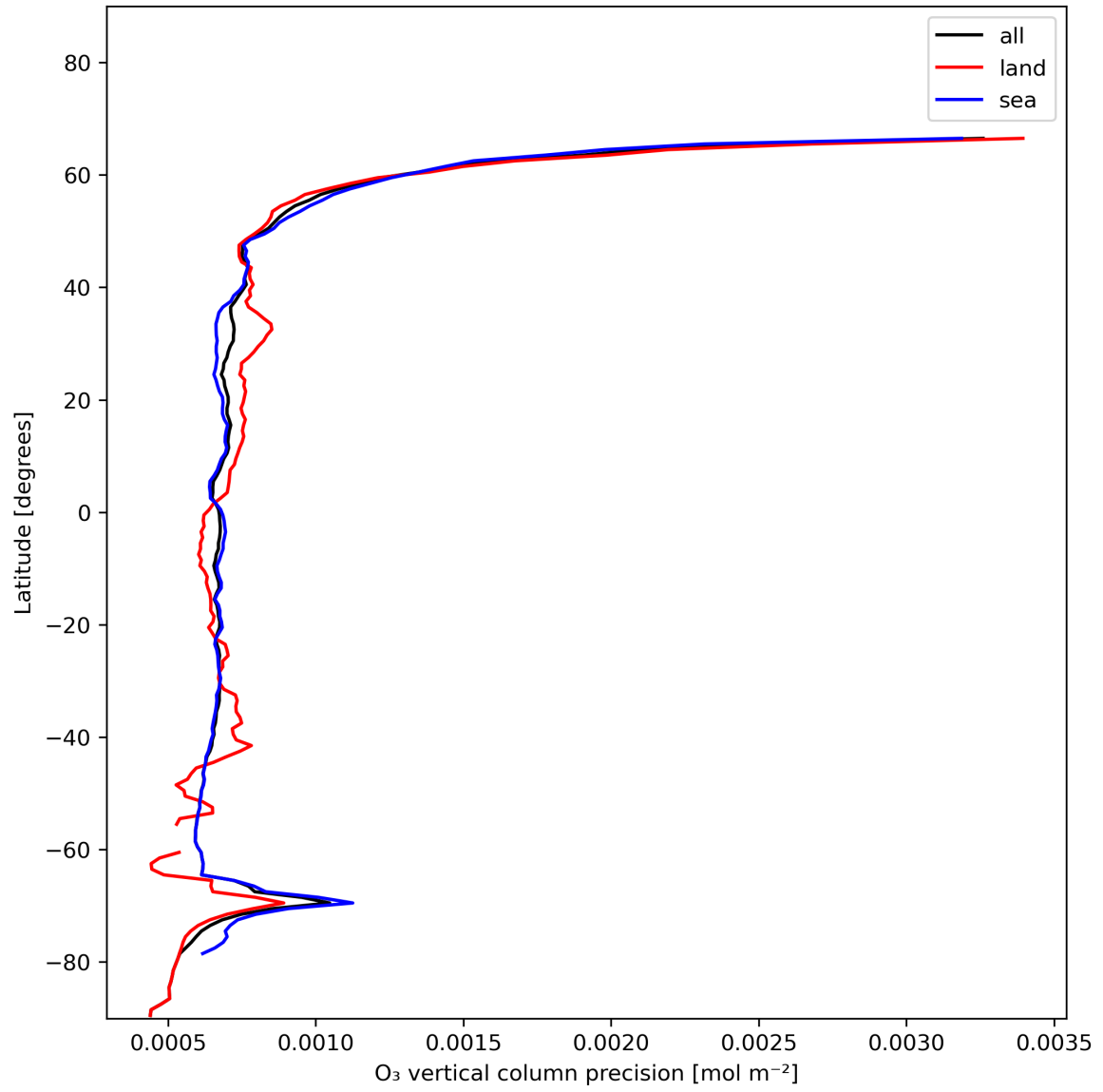
Figure 15: Zonal average of “O 3 vertical column precision” for 2024-01-08 to 2024-01-10.
