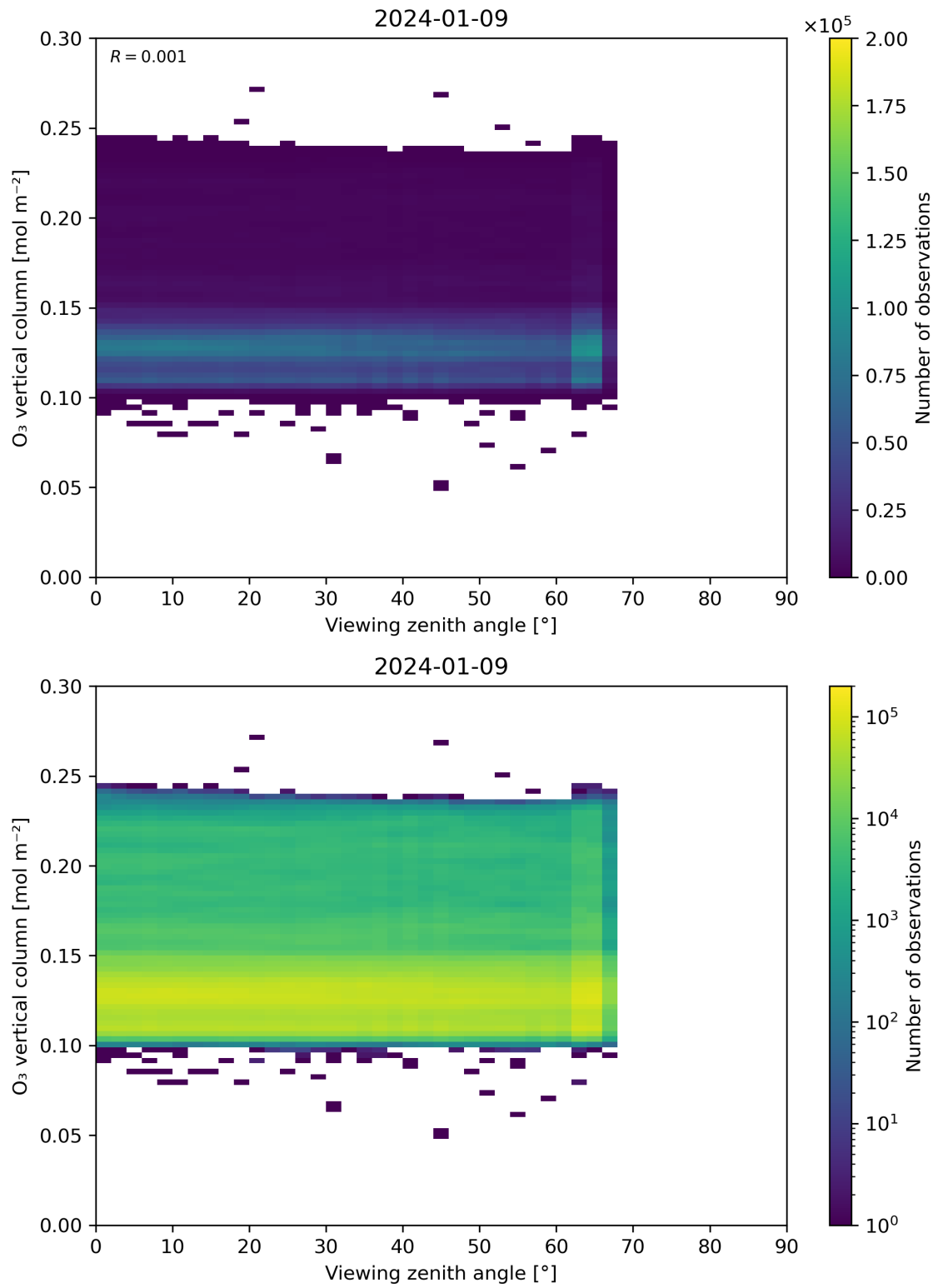
Figure 52: Scatter density plot of “Viewing zenith angle” against “O 3 vertical column” for 2024-01-08 to 2024-01-10.
