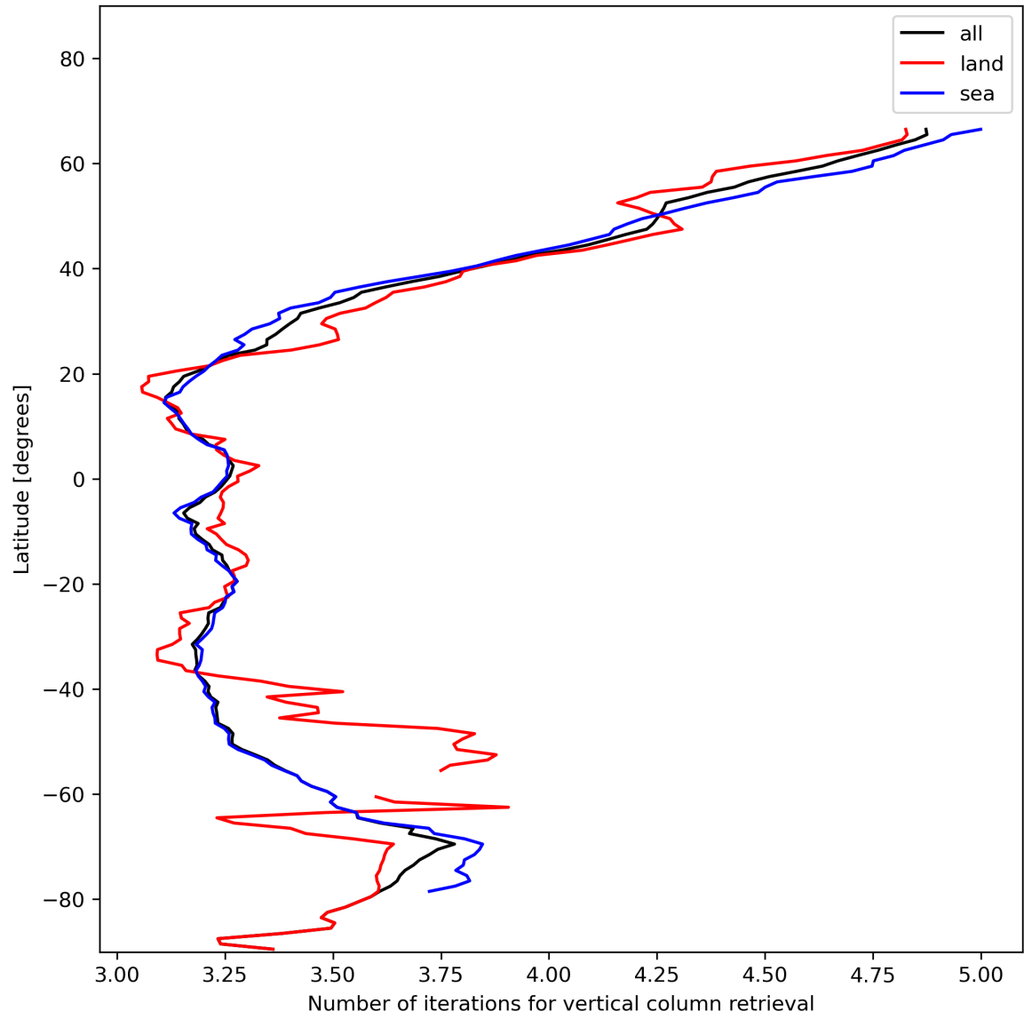
Figure 19: Zonal average of “Number of iterations for vertical column retrieval” for 2024-01-08 to 2024-01-10.
