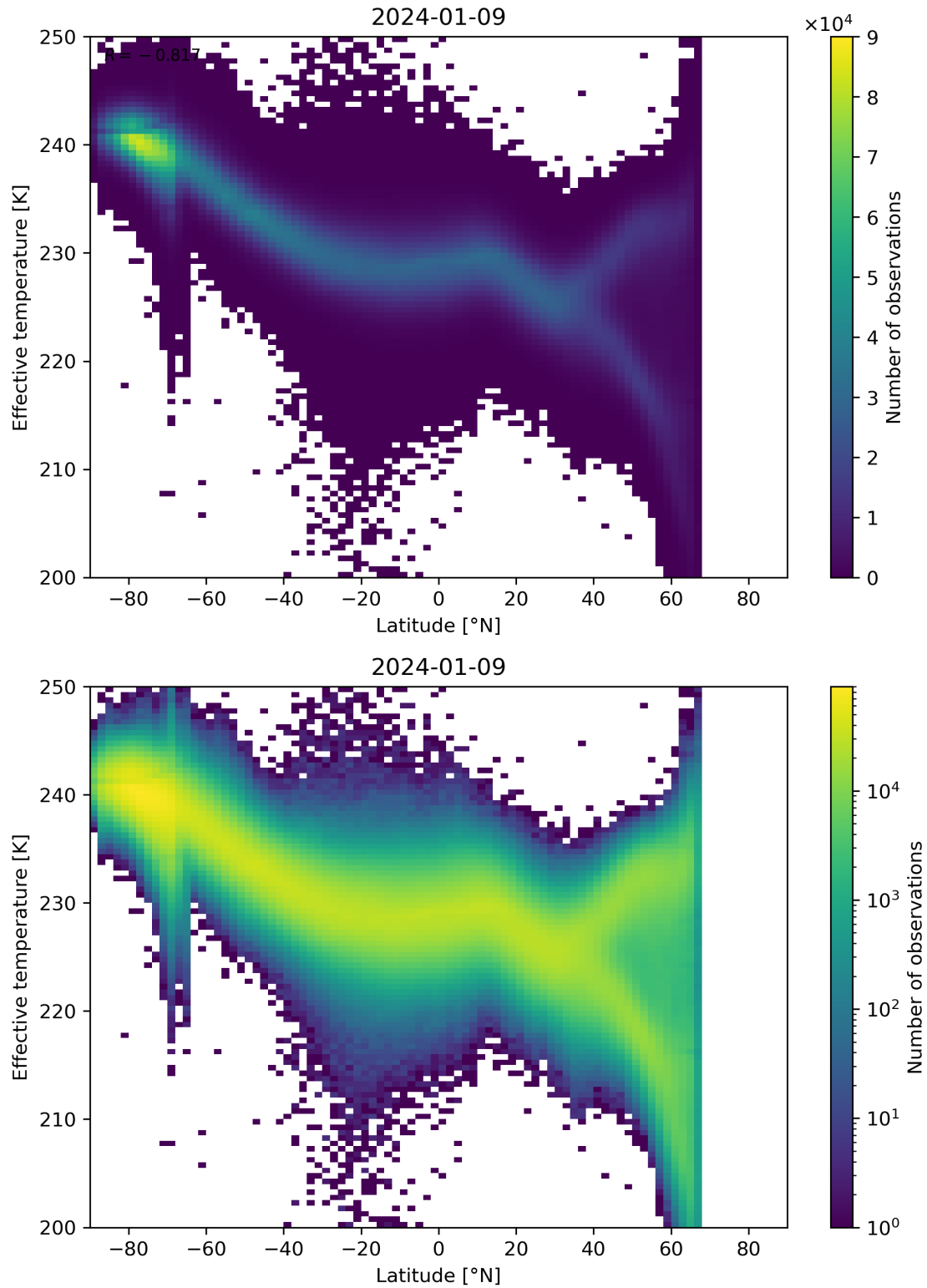
Figure 34: Scatter density plot of “Latitude” against “Effective temperature” for 2024-01-08 to 2024-01-10.
