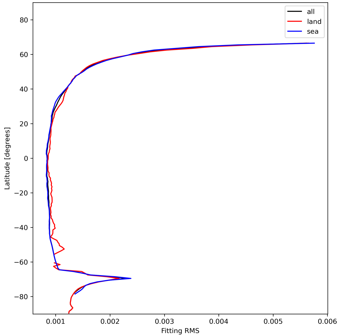
Figure 16: Zonal average of “Fitting RMS” for 2024-01-08 to 2024-01-10.
