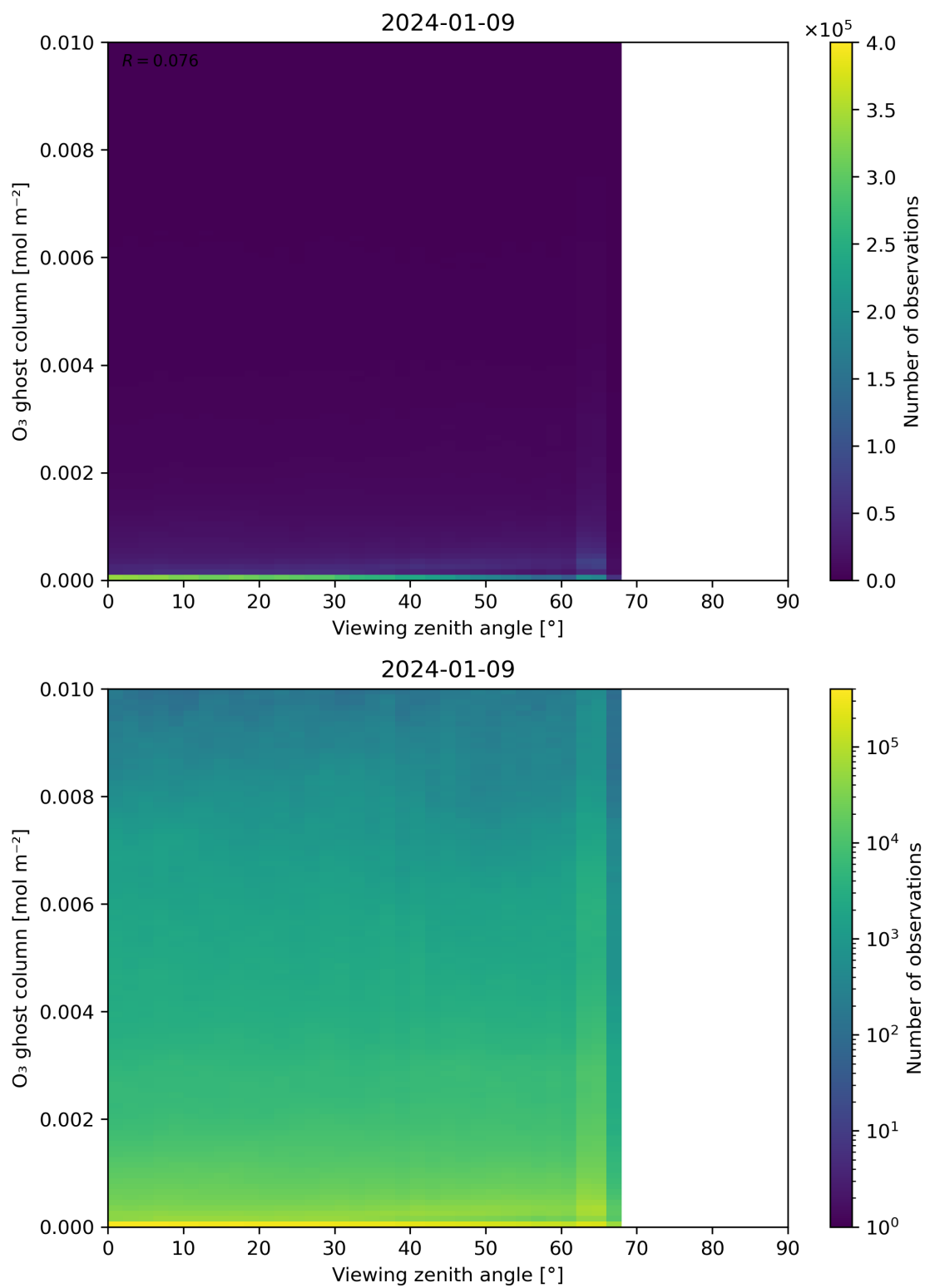
Figure 51: Scatter density plot of “Viewing zenith angle” against “O 3 ghost column” for 2024-01-08 to 2024-01-10.
