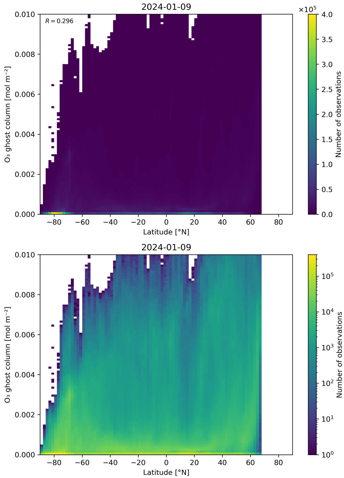
Figure 35: Scatter density plot of “Latitude” against “O 3 ghost column” for 2024-01-08 to 2024-01-10.
