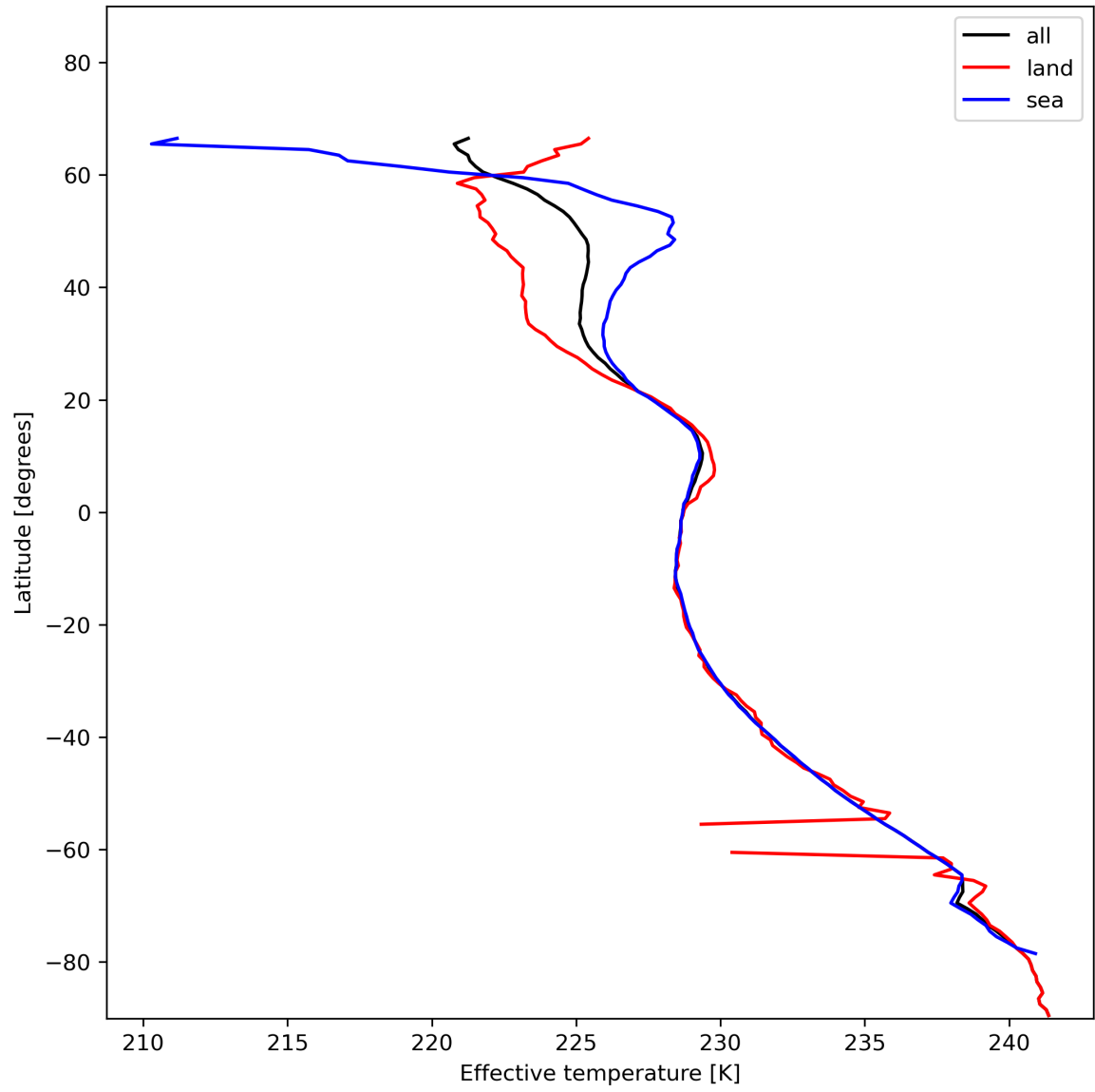
Figure 17: Zonal average of "Effective temperature" for 2024-01-08 to 2024-01-10.
