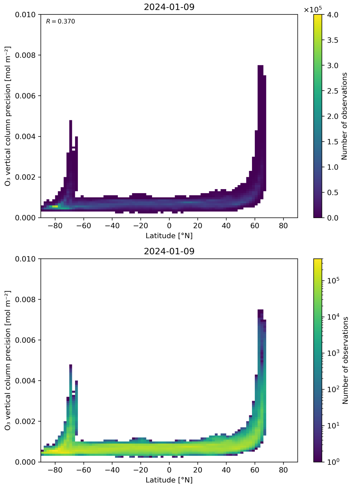
Figure 37: Scatter density plot of “Latitude” against “O 3 vertical column precision” for 2024-01-08 to 2024-01-10.
