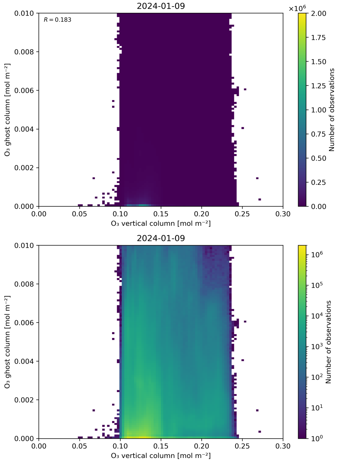
Figure 40: Scatter density plot of “O 3 vertical column” against “O 3 ghost column” for 2024-01-08 to 2024-01-10.
