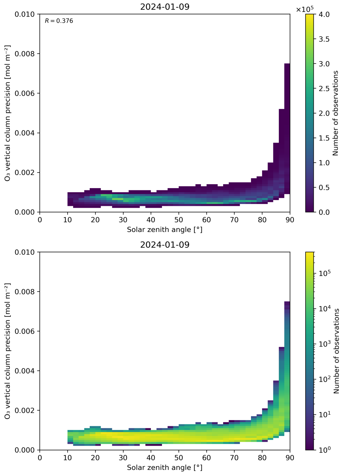
Figure 48: Scatter density plot of “Solar zenith angle” against “O 3 vertical column precision” for 2024-01-08 to 2024-01-10.
