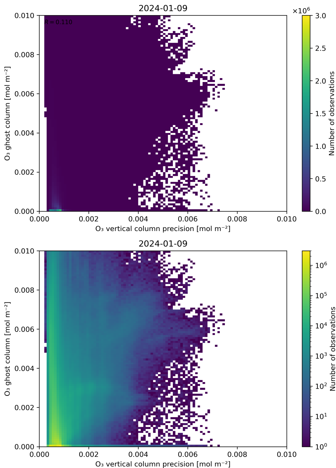
Figure 43: Scatter density plot of “O 3 vertical column precision” against “O 3 ghost column” for 2024-01-08 to 2024-01-10.
