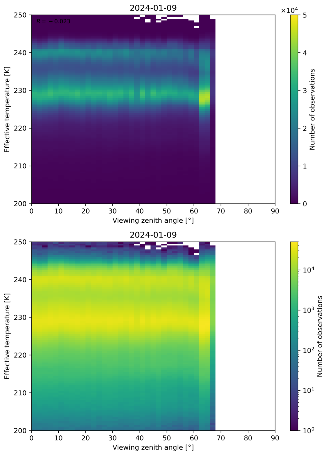
Figure 50: Scatter density plot of “Viewing zenith angle” against “Effective temperature” for 2024-01-08 to 2024-01-10.
