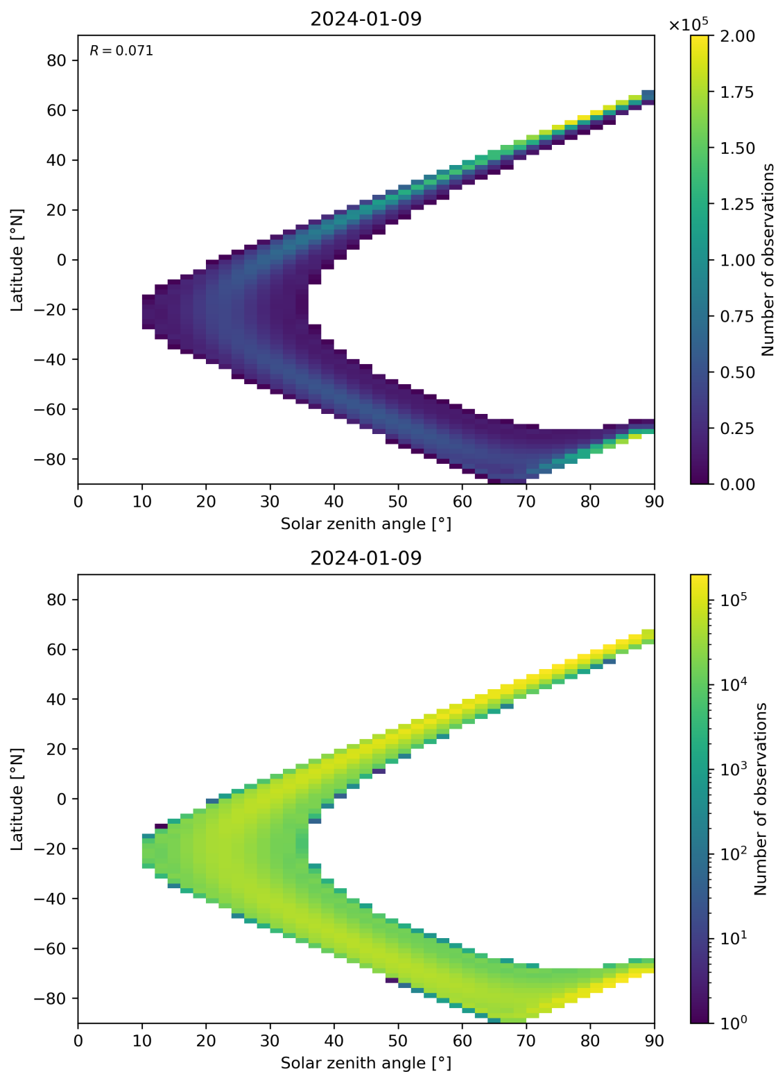
Figure 44: Scatter density plot of “Solar zenith angle” against “Latitude” for 2024-01-08 to 2024-01-10.
