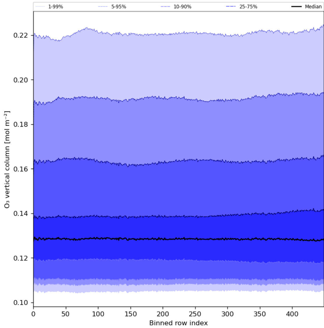
Figure 28: Along track statistics of “O 3 vertical column” for 2024-01-08 to 2024-01-10
