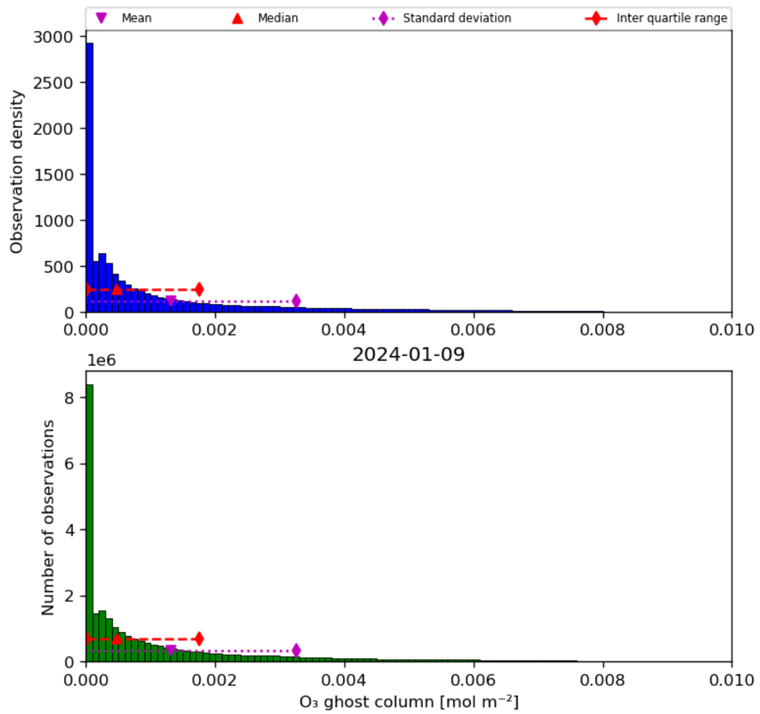
Figure 25: Histogram of “O 3 ghost column” for 2024-01-08 to 2024-01-10
