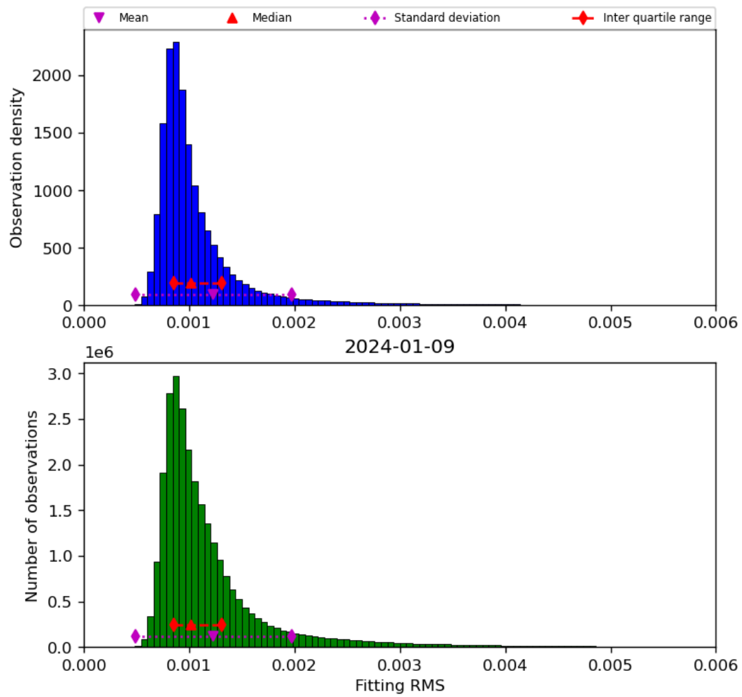
Figure 23: Histogram of “Fitting RMS” for 2024-01-08 to 2024-01-10
