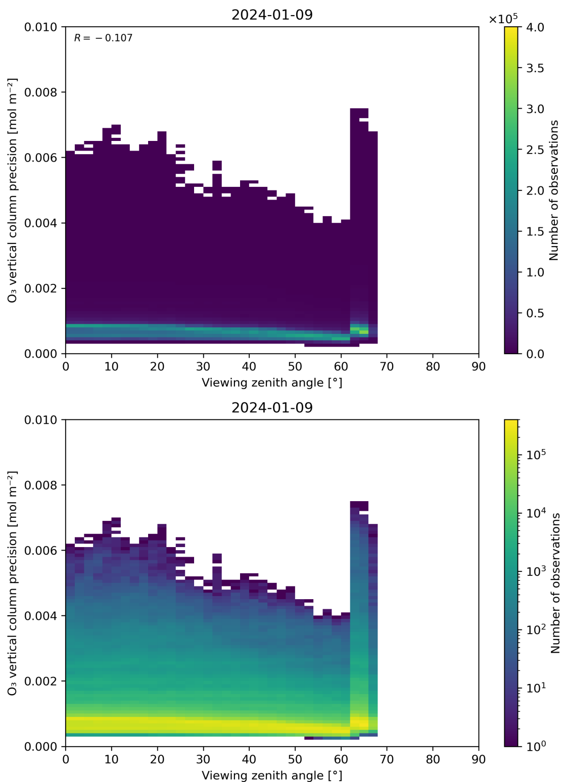
Figure 53: Scatter density plot of “Viewing zenith angle” against “O 3 vertical column precision” for 2024-01-08 to 2024-01-10.
