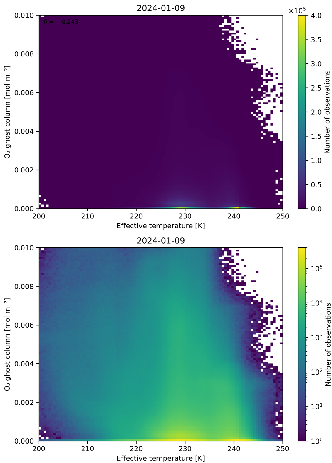
Figure 38: Scatter density plot of “Effective temperature” against “O 3 ghost column” for 2024-01-08 to 2024-01-10.
