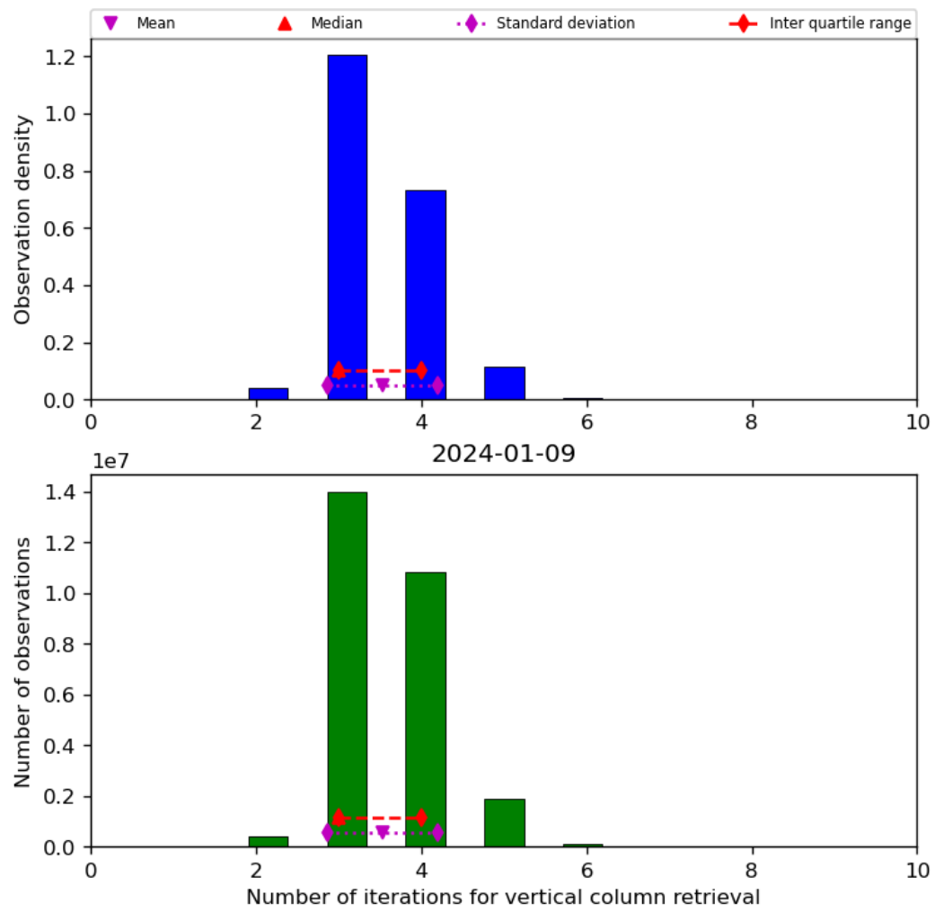
Figure 26: Histogram of “Number of iterations for vertical column retrieval” for 2024-01-08 to 2024-01-10
