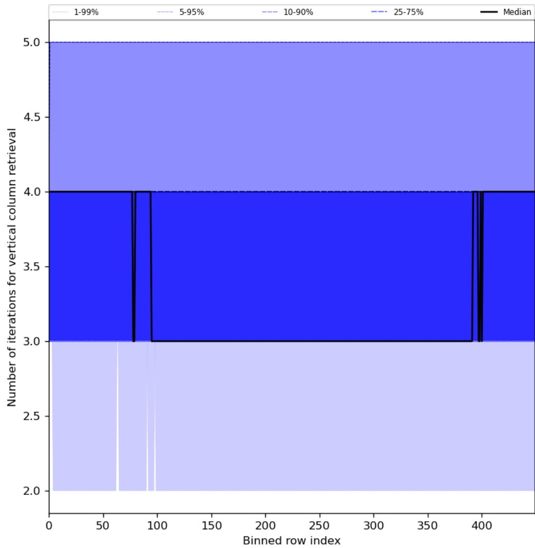
Figure 33: Along track statistics of “Number of iterations for vertical column retrieval” for 2024-01-08 to 2024-01-10
