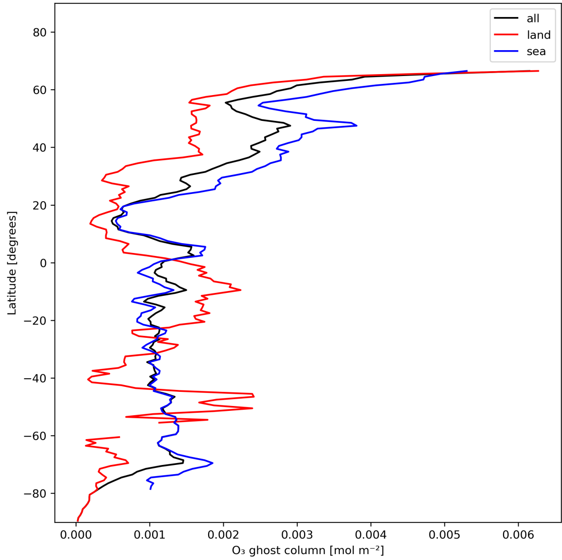
Figure 18: Zonal average of “O 3 ghost column” for 2024-01-08 to 2024-01-10.
