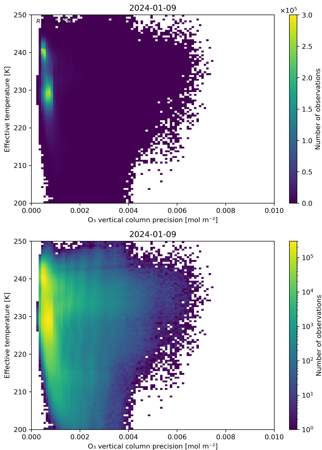
Figure 42: Scatter density plot of “O 3 vertical column precision” against “Effective temperature” for 2024-01-08 to 2024-01-10.
