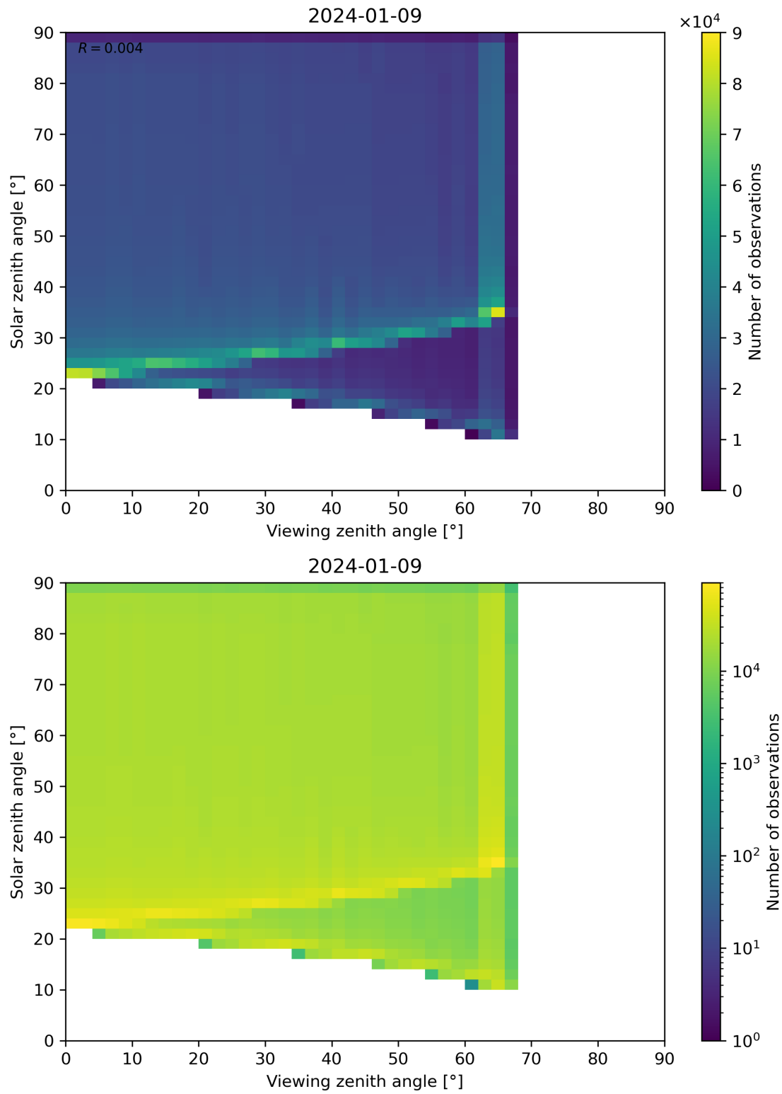
Figure 54: Scatter density plot of “Viewing zenith angle” against “Solar zenith angle” for 2024-01-08 to 2024-01-10.
