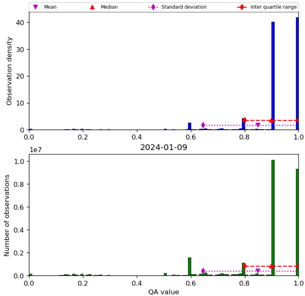
Figure 20: Histogram of “QA value” for 2024-01-08 to 2024-01-10
