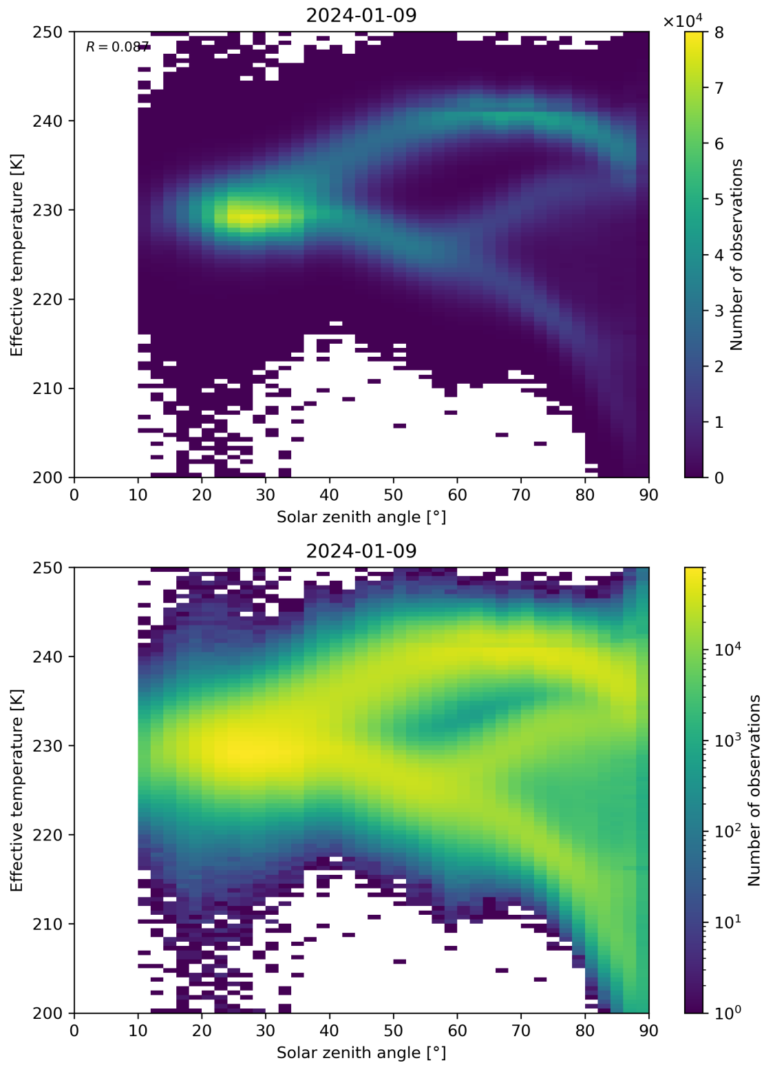
Figure 45: Scatter density plot of “Solar zenith angle” against “Effective temperature” for 2024-01-08 to 2024-01-10.
