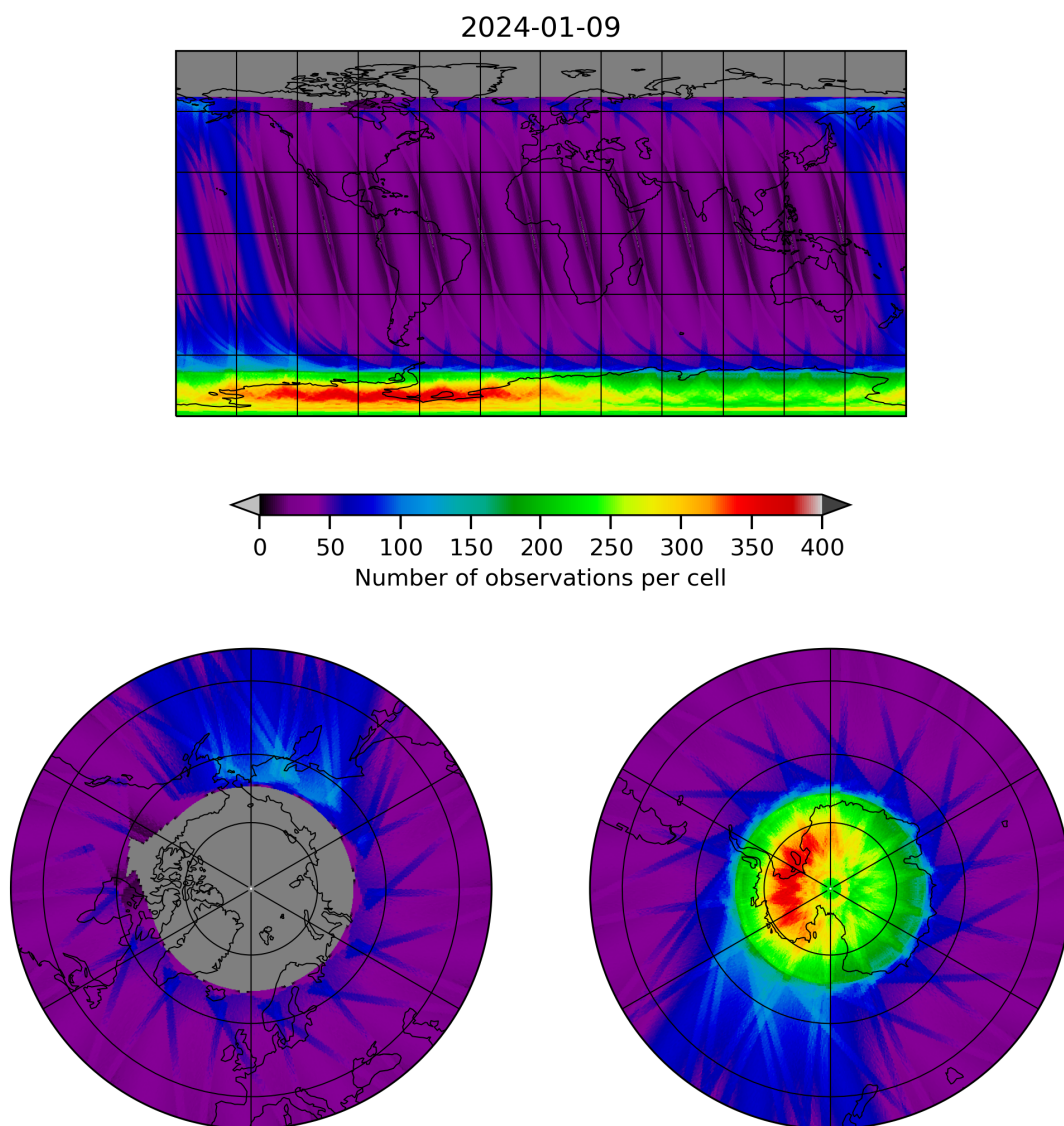
Figure 12: Map of the number of observations for 2024-01-08 to 2024-01-10
