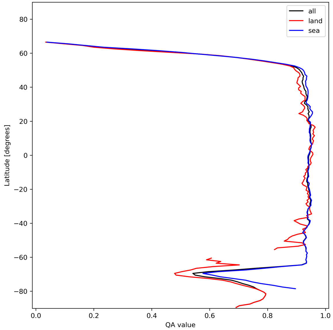
Figure 13: Zonal average of “QA value” for 2024-01-08 to 2024-01-10.
