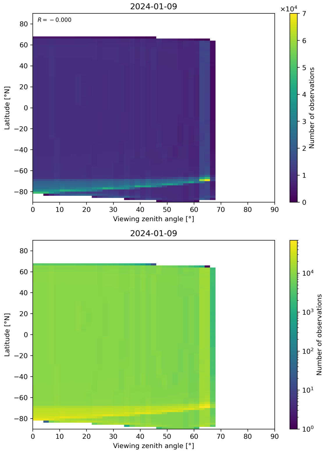
Figure 49: Scatter density plot of “Viewing zenith angle” against “Latitude” for 2024-01-08 to 2024-01-10.
