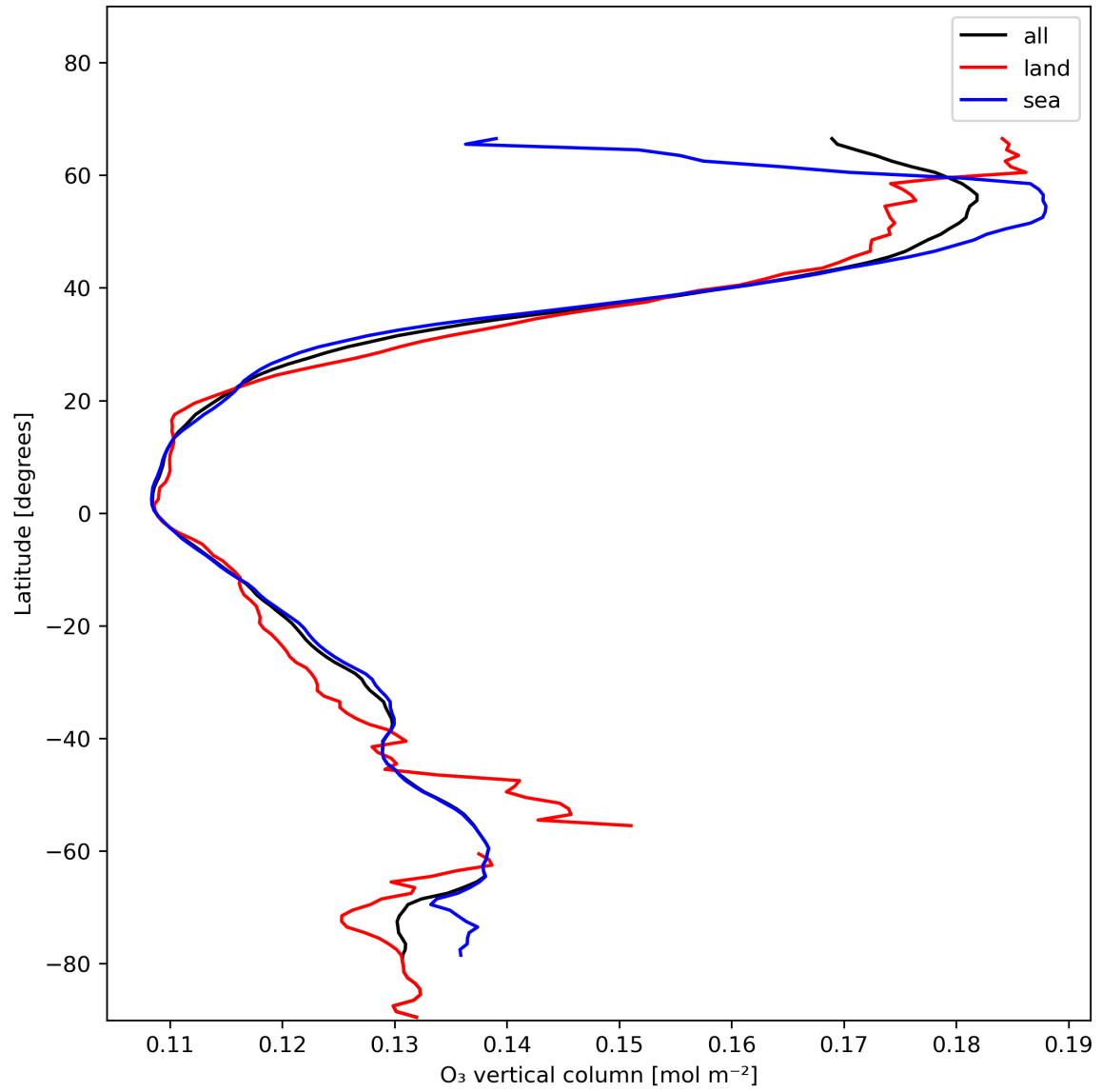
Figure 14: Zonal average of “O 3 vertical column” for 2024-01-08 to 2024-01-10.
