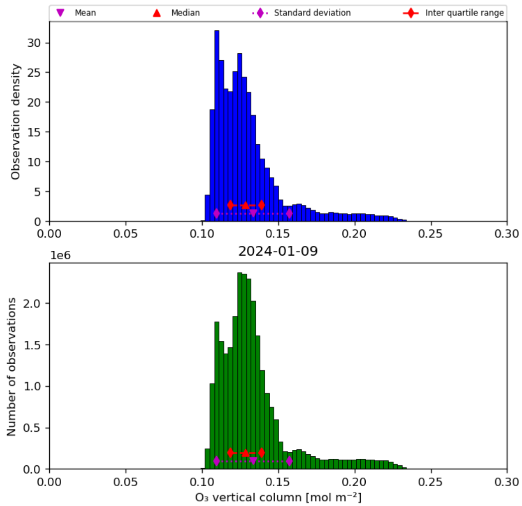
Figure 21: Histogram of “O 3 vertical column” for 2024-01-08 to 2024-01-10
