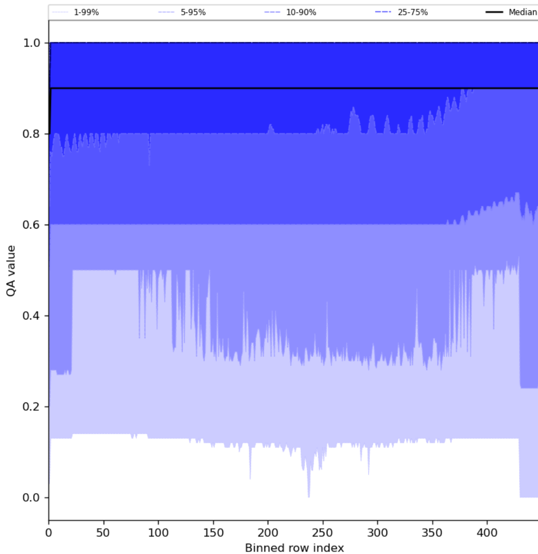
Figure 27: Along track statistics of “QA value” for 2024-01-08 to 2024-01-10
