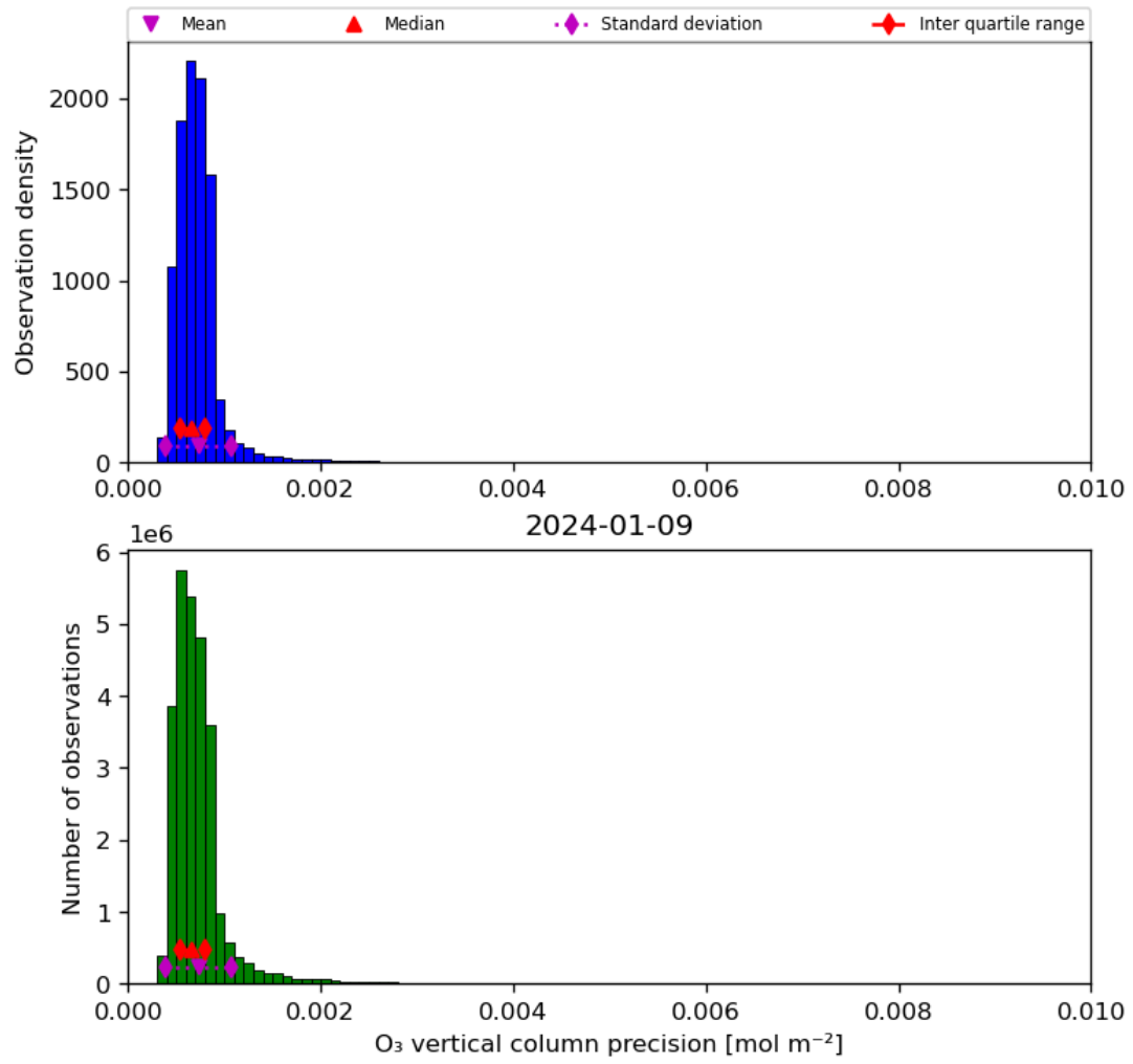
Figure 22: Histogram of “O 3 vertical column precision” for 2024-01-08 to 2024-01-10
