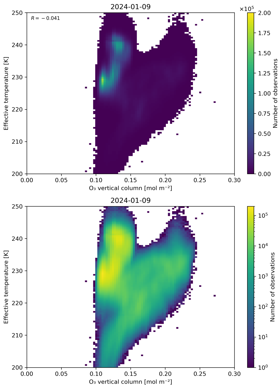
Figure 39: Scatter density plot of “O 3 vertical column” against “Effective temperature” for 2024-01-08 to 2024-01-10.
