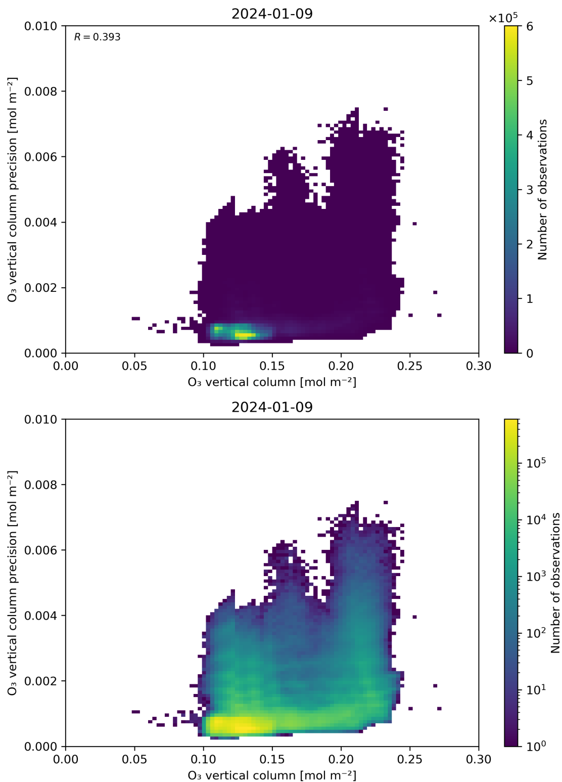
Figure 41: Scatter density plot of “O 3 vertical column” against “O 3 vertical column precision” for 2024-01-08 to 2024-01-10.
