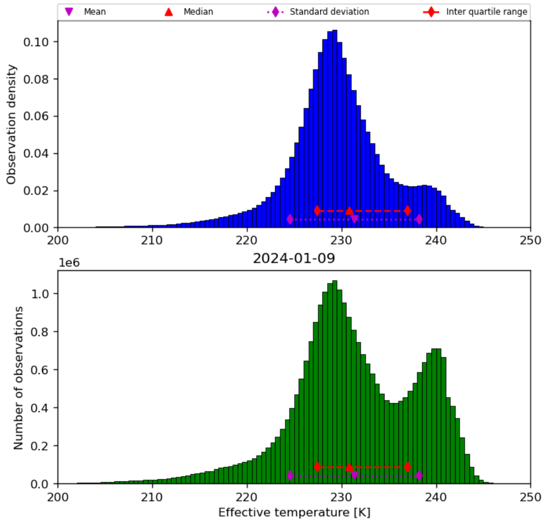
Figure 24: Histogram of “Effective temperature” for 2024-01-08 to 2024-01-10
