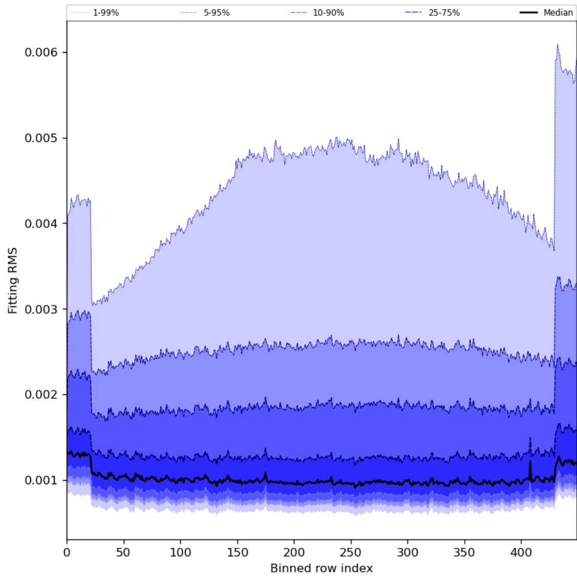
Figure 30: Along track statistics of “Fitting RMS” for 2024-01-08 to 2024-01-10
