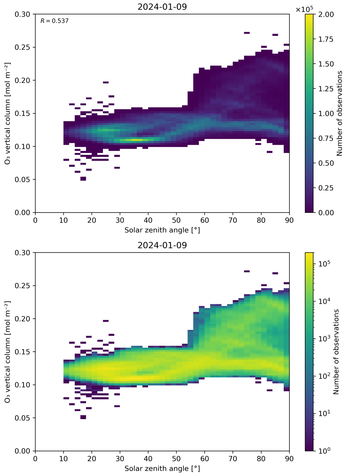
Figure 47: Scatter density plot of “Solar zenith angle” against “O 3 vertical column” for 2024-01-08 to 2024-01-10.
