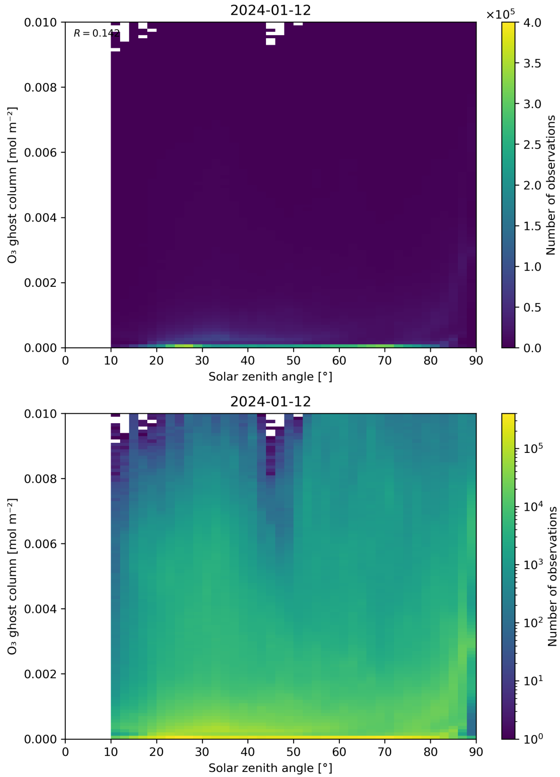
Figure 46: Scatter density plot of “Solar zenith angle” against “O 3 ghost column” for 2024-01-11 to 2024-01-13.
