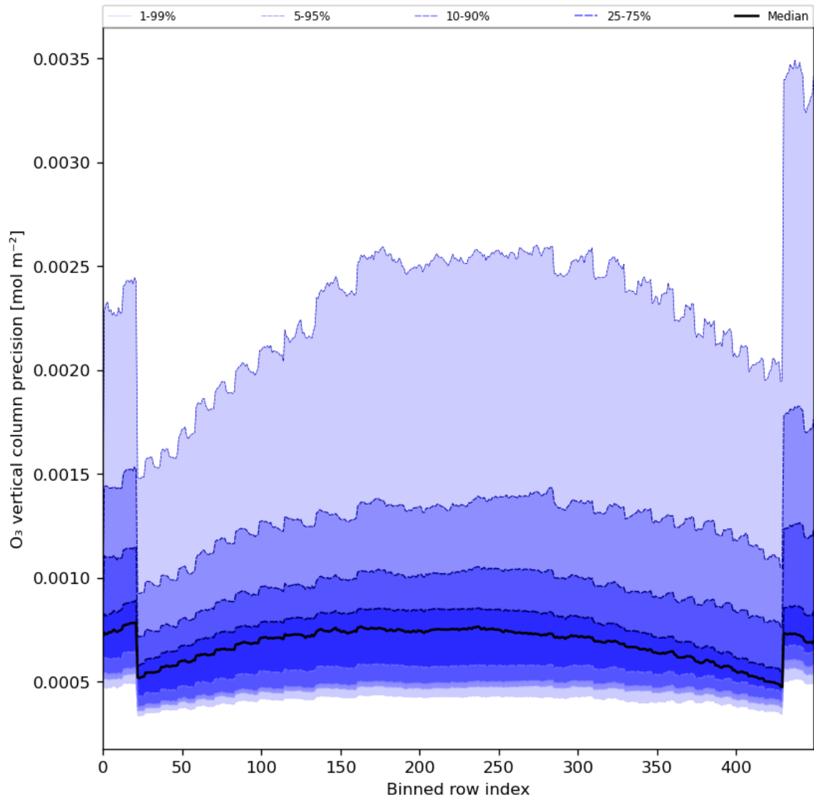
Figure 29: Along track statistics of “O 3 vertical column precision” for 2024-01-11 to 2024-01-13
