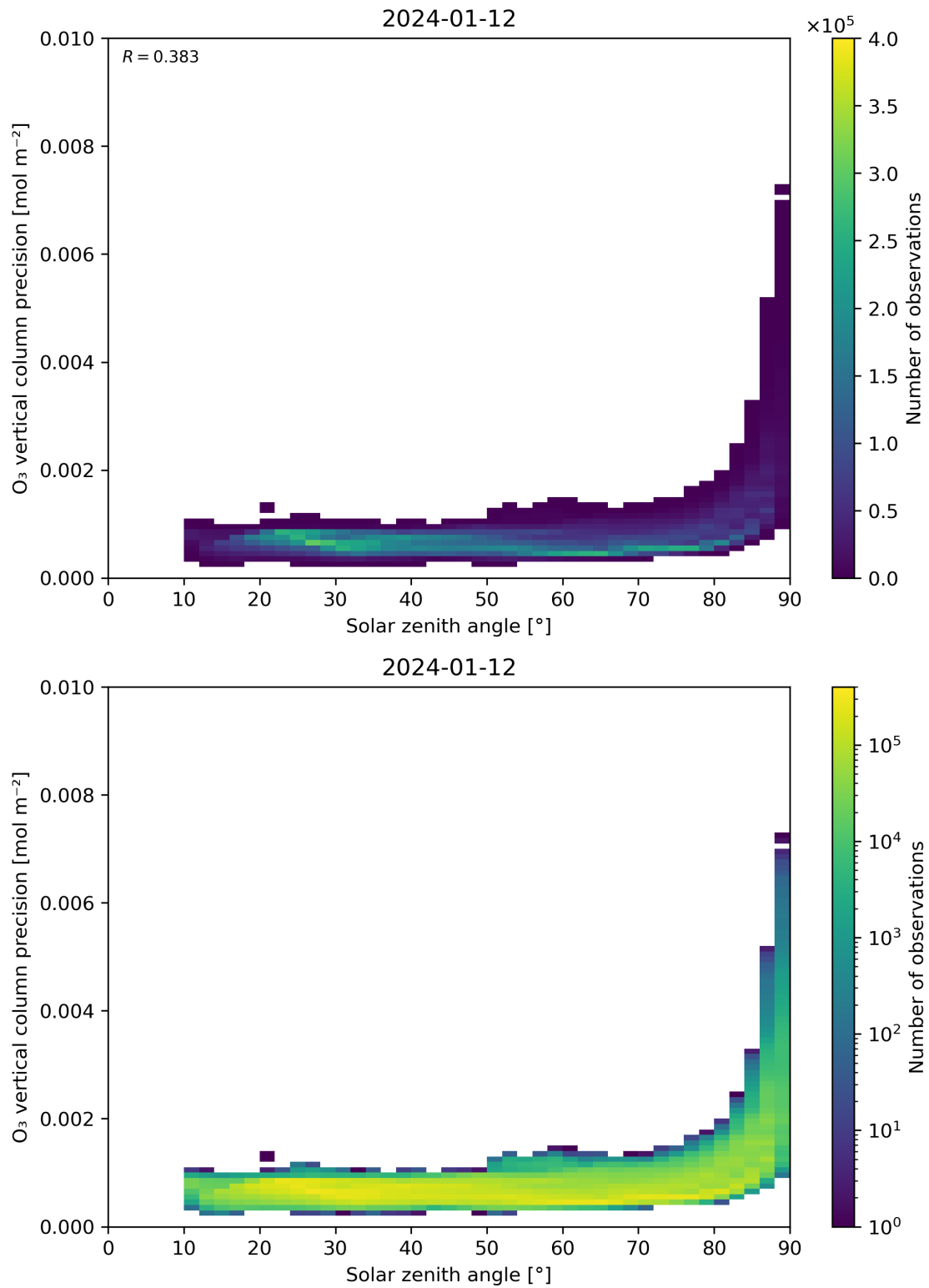
Figure 48: Scatter density plot of “Solar zenith angle” against “O 3 vertical column precision” for 2024-01-11 to 2024-01-13.
