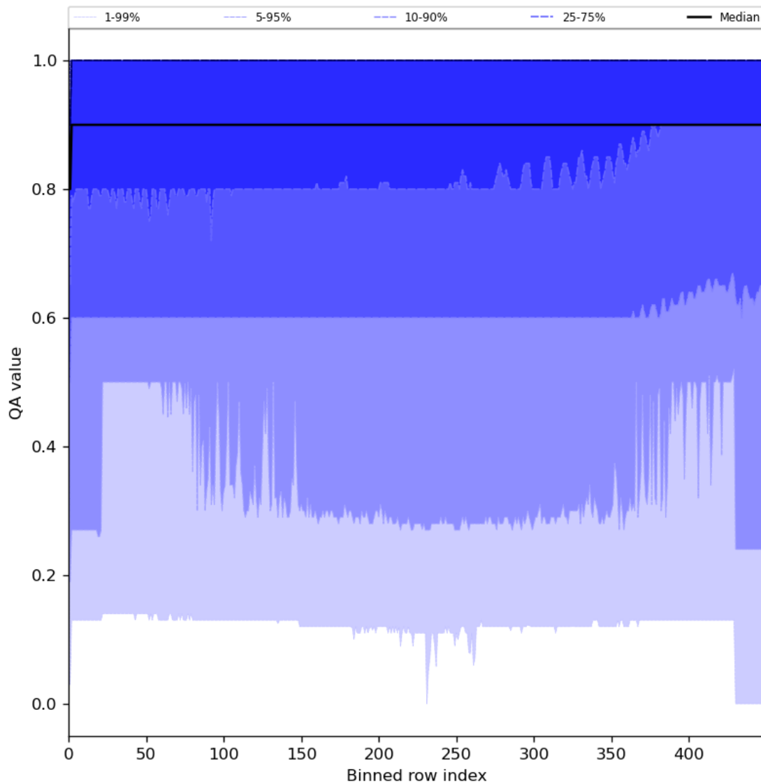
Figure 27: Along track statistics of “QA value” for 2024-01-11 to 2024-01-13
