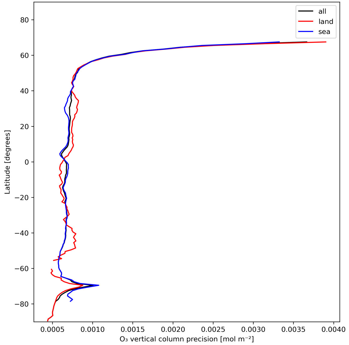
Figure 15: Zonal average of “O 3 vertical column precision” for 2024-01-11 to 2024-01-13.
