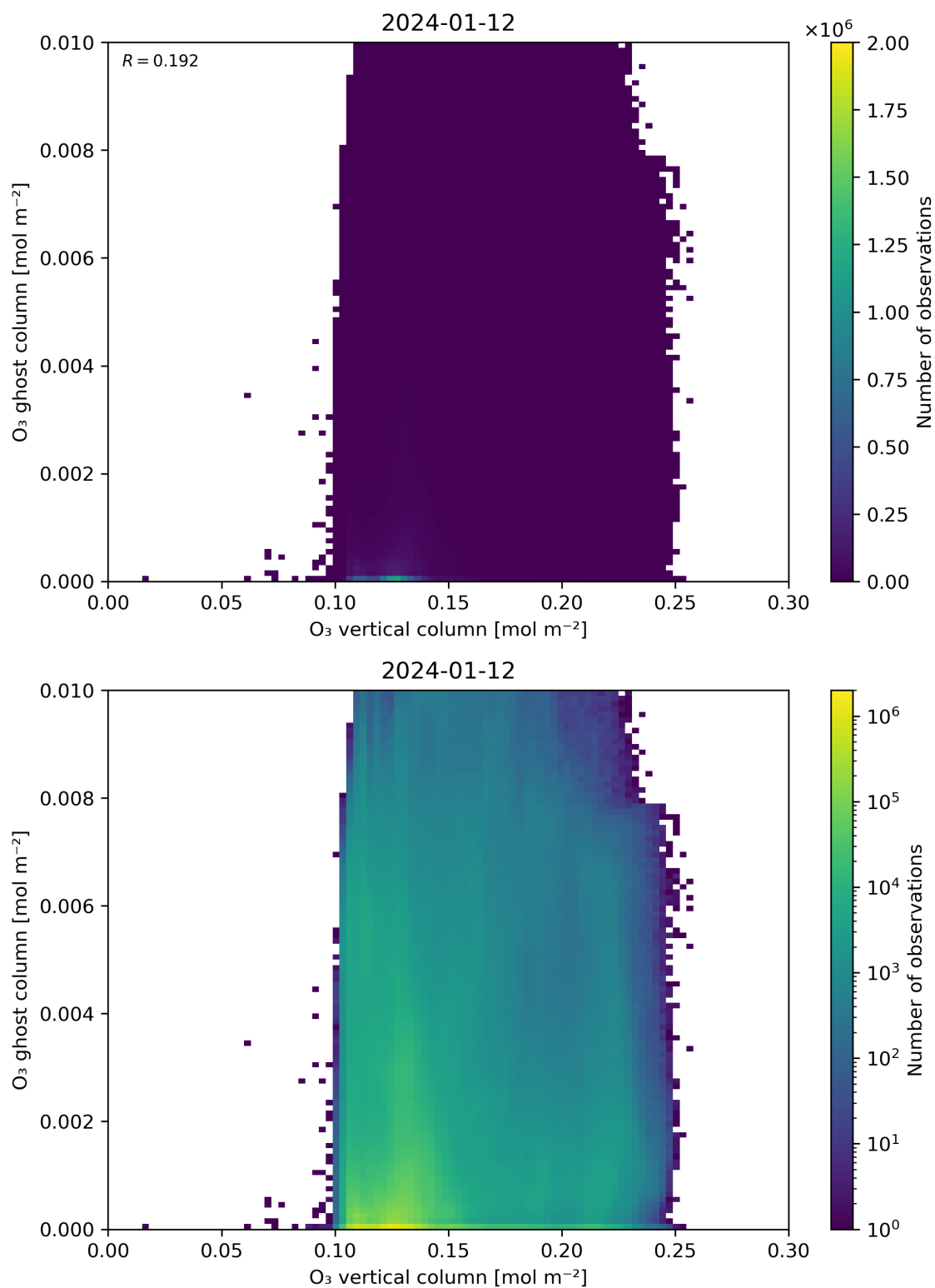
Figure 40: Scatter density plot of “O 3 vertical column” against “O 3 ghost column” for 2024-01-11 to 2024-01-13.
