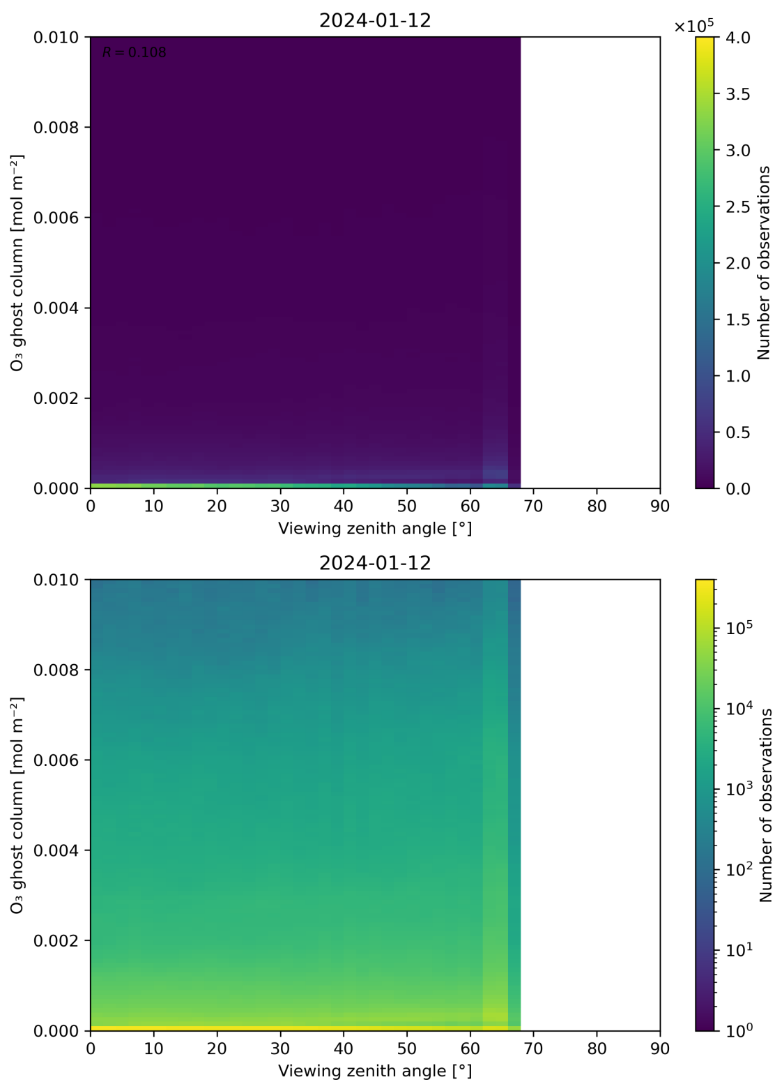
Figure 51: Scatter density plot of “Viewing zenith angle” against “O 3 ghost column” for 2024-01-11 to 2024-01-13.
