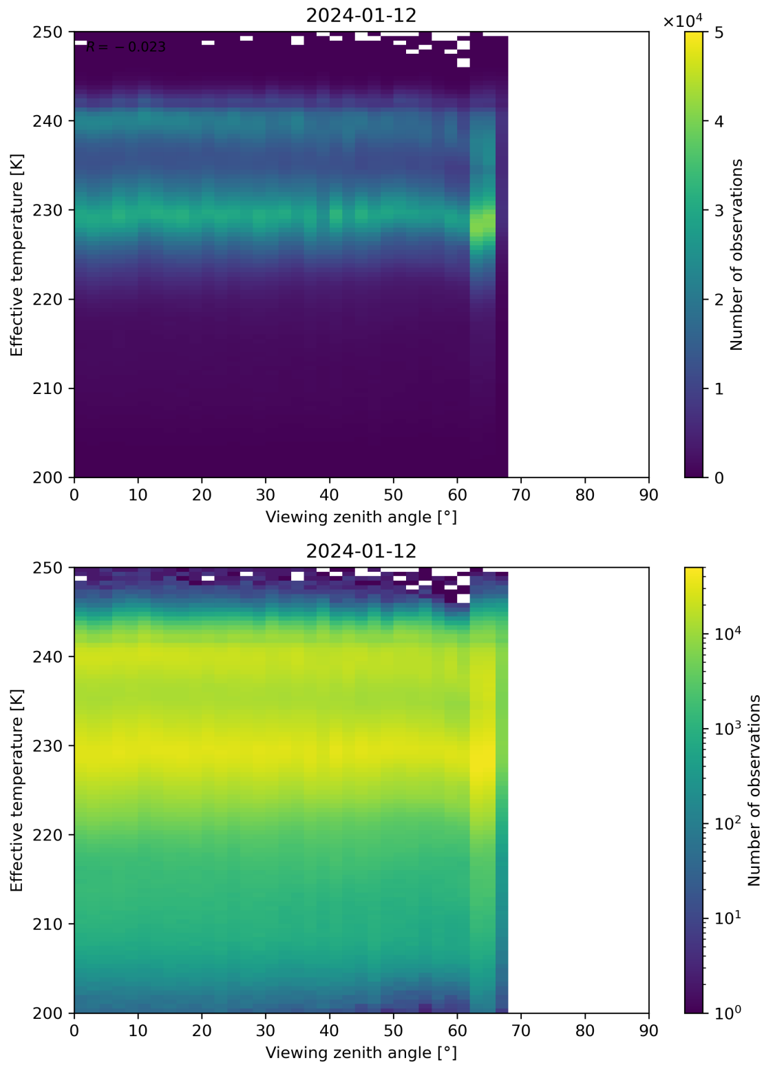
Figure 50: Scatter density plot of “Viewing zenith angle” against “Effective temperature” for 2024-01-11 to 2024-01-13.
