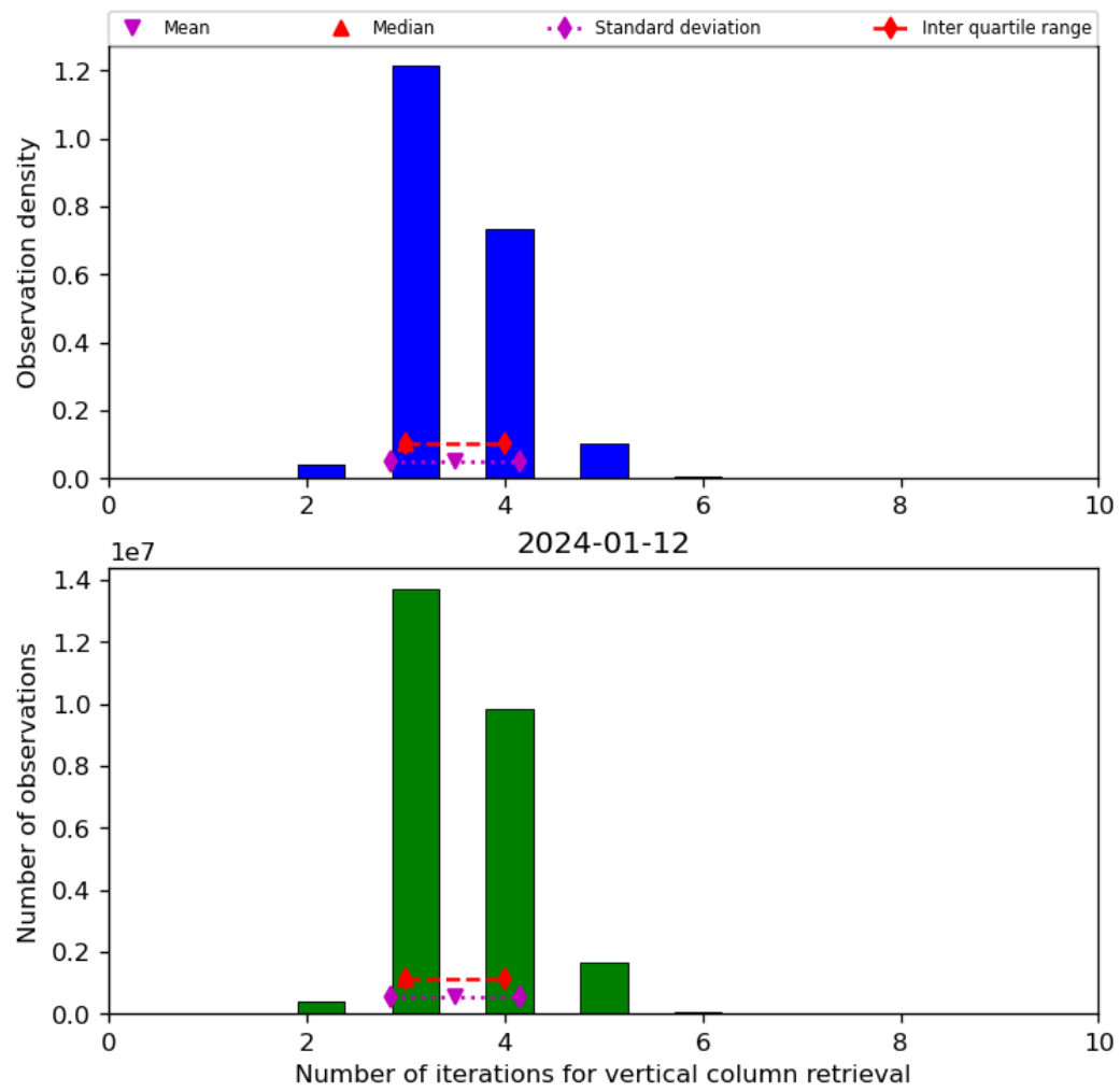
Figure 26: Histogram of “Number of iterations for vertical column retrieval” for 2024-01-11 to 2024-01-13
