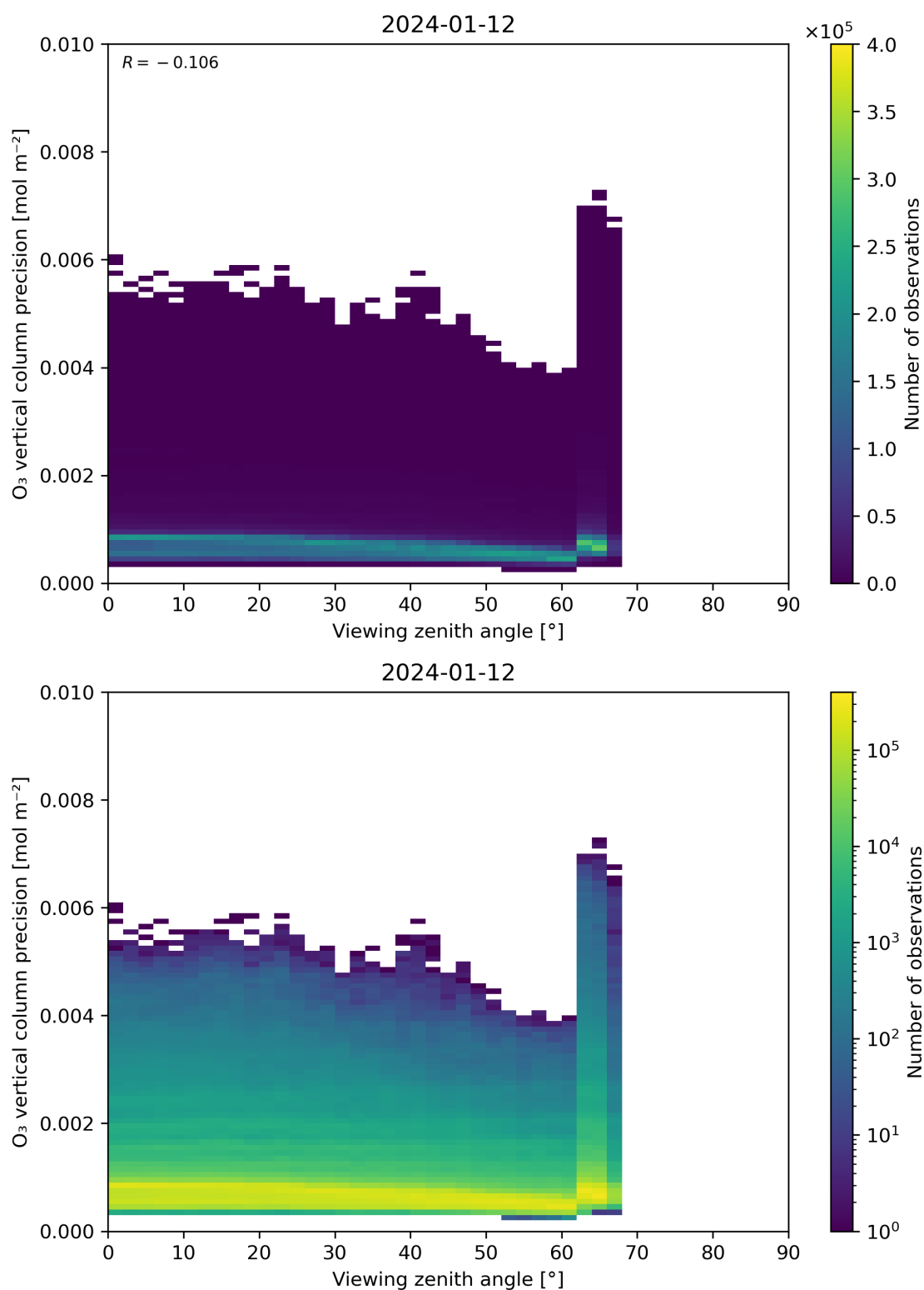
Figure 53: Scatter density plot of “Viewing zenith angle” against “O 3 vertical column precision” for 2024-01-11 to 2024-01-13.
