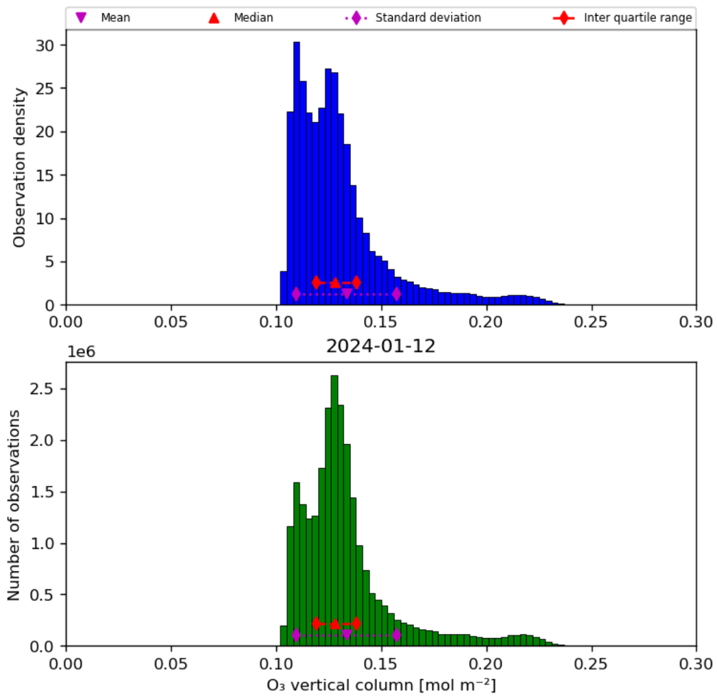
Figure 21: Histogram of “O 3 vertical column” for 2024-01-11 to 2024-01-13
