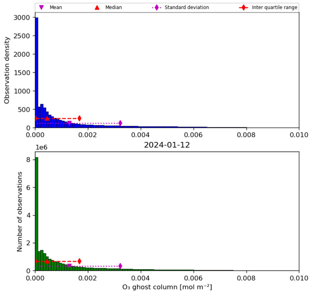
Figure 25: Histogram of “O 3 ghost column” for 2024-01-11 to 2024-01-13
