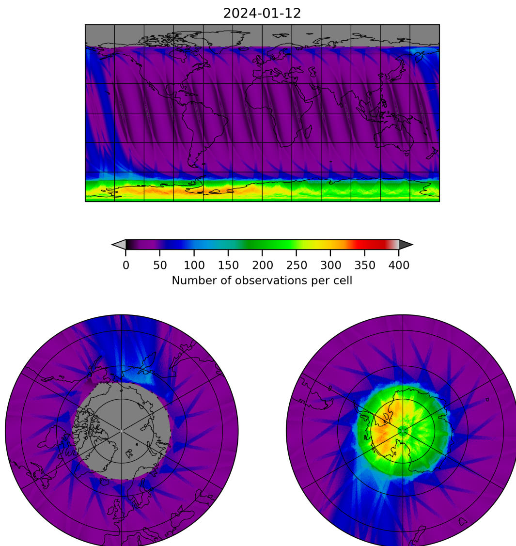
Figure 12: Map of the number of observations for 2024-01-11 to 2024-01-13
