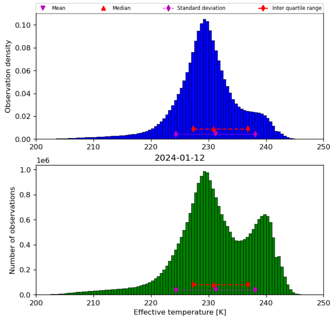
Figure 24: Histogram of “Effective temperature” for 2024-01-11 to 2024-01-13
