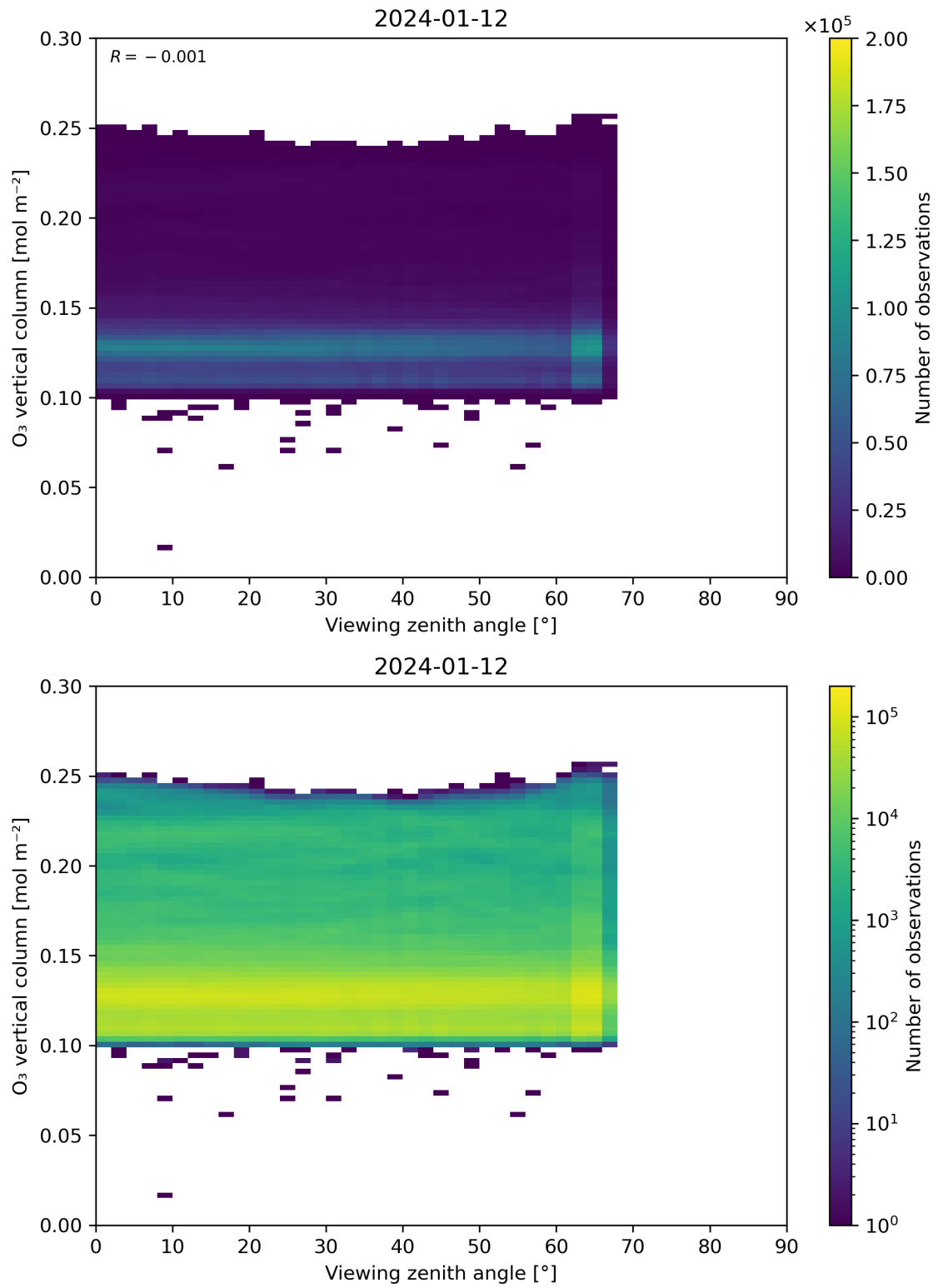
Figure 52: Scatter density plot of “Viewing zenith angle” against “O 3 vertical column” for 2024-01-11 to 2024-01-13.
