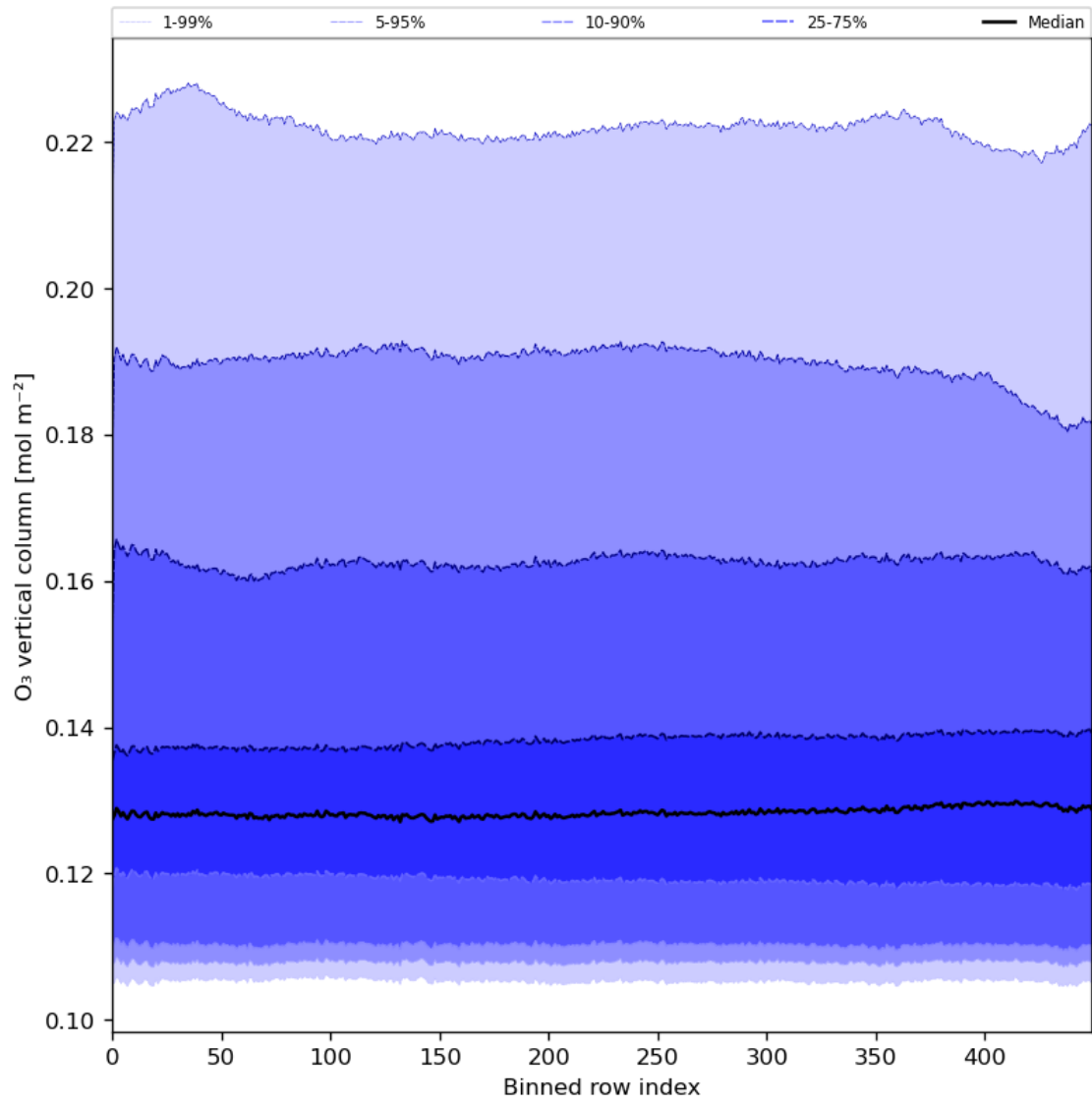
Figure 28: Along track statistics of “O 3 vertical column” for 2024-01-11 to 2024-01-13
