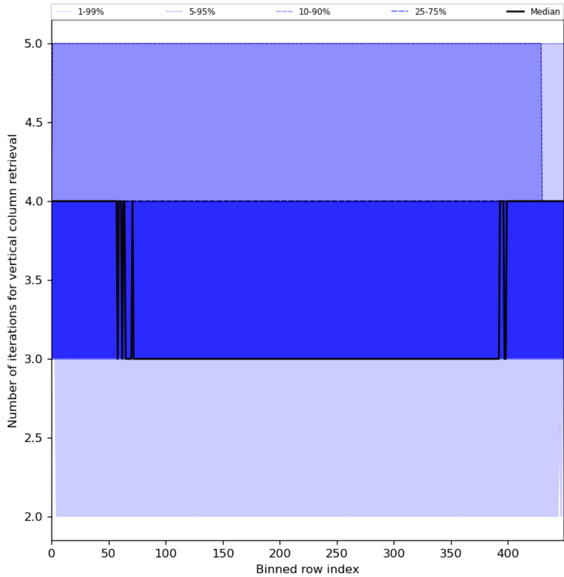
Figure 33: Along track statistics of “Number of iterations for vertical column retrieval” for 2024-01-11 to 2024-01-13
