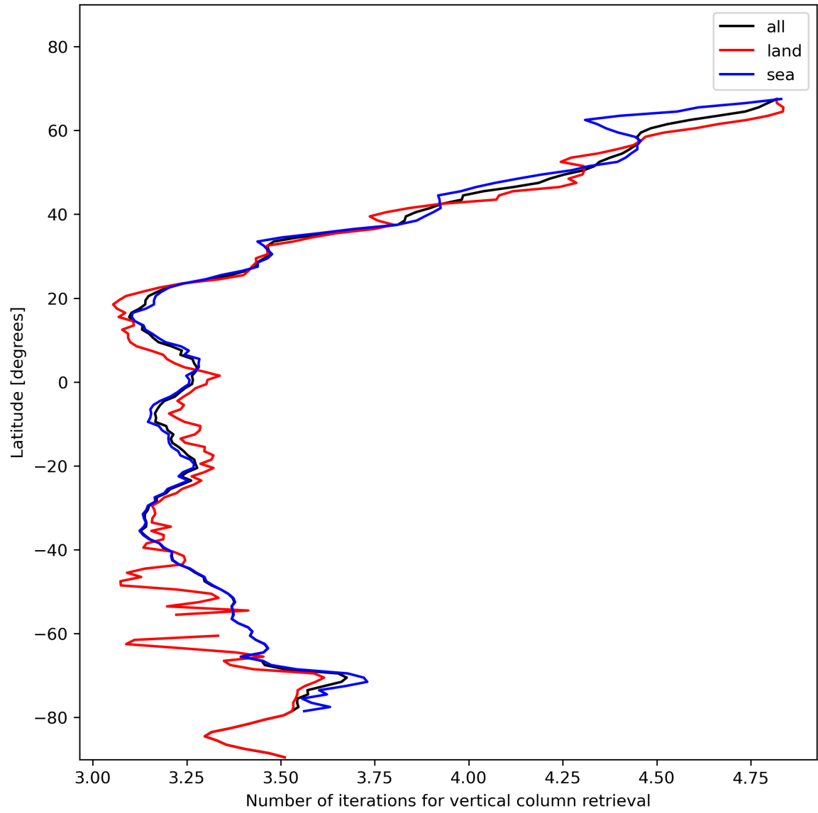
Figure 19: Zonal average of “Number of iterations for vertical column retrieval” for 2024-01-11 to 2024-01-13.
