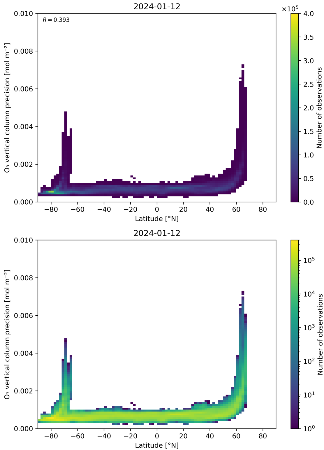
Figure 37: Scatter density plot of “Latitude” against “O 3 vertical column precision” for 2024-01-11 to 2024-01-13.
