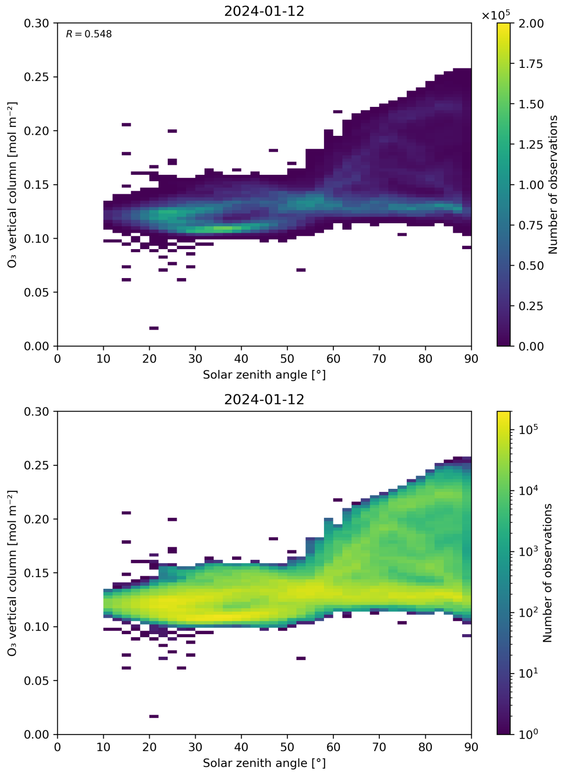
Figure 47: Scatter density plot of “Solar zenith angle” against “O 3 vertical column” for 2024-01-11 to 2024-01-13.
