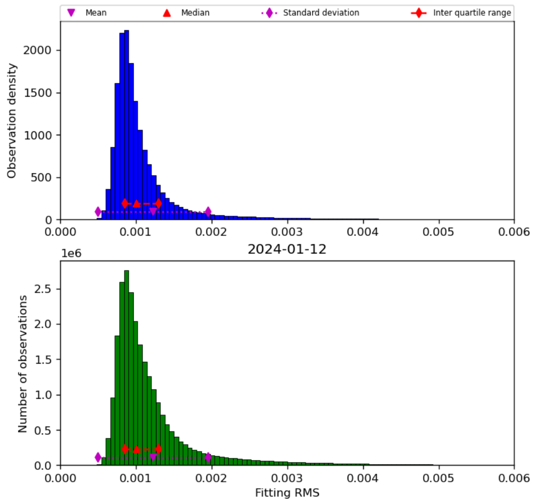
Figure 23: Histogram of “Fitting RMS” for 2024-01-11 to 2024-01-13
