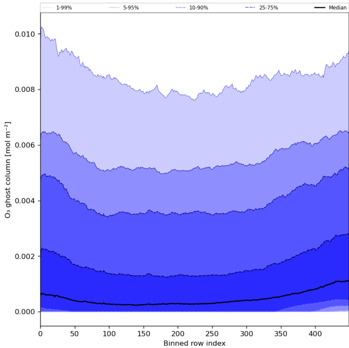
Figure 32: Along track statistics of “O 3 ghost column” for 2024-01-11 to 2024-01-13
