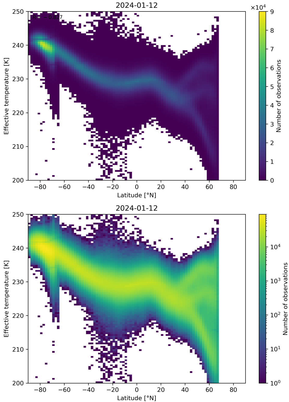
Figure 34: Scatter density plot of “Latitude” against “Effective temperature” for 2024-01-11 to 2024-01-13.
