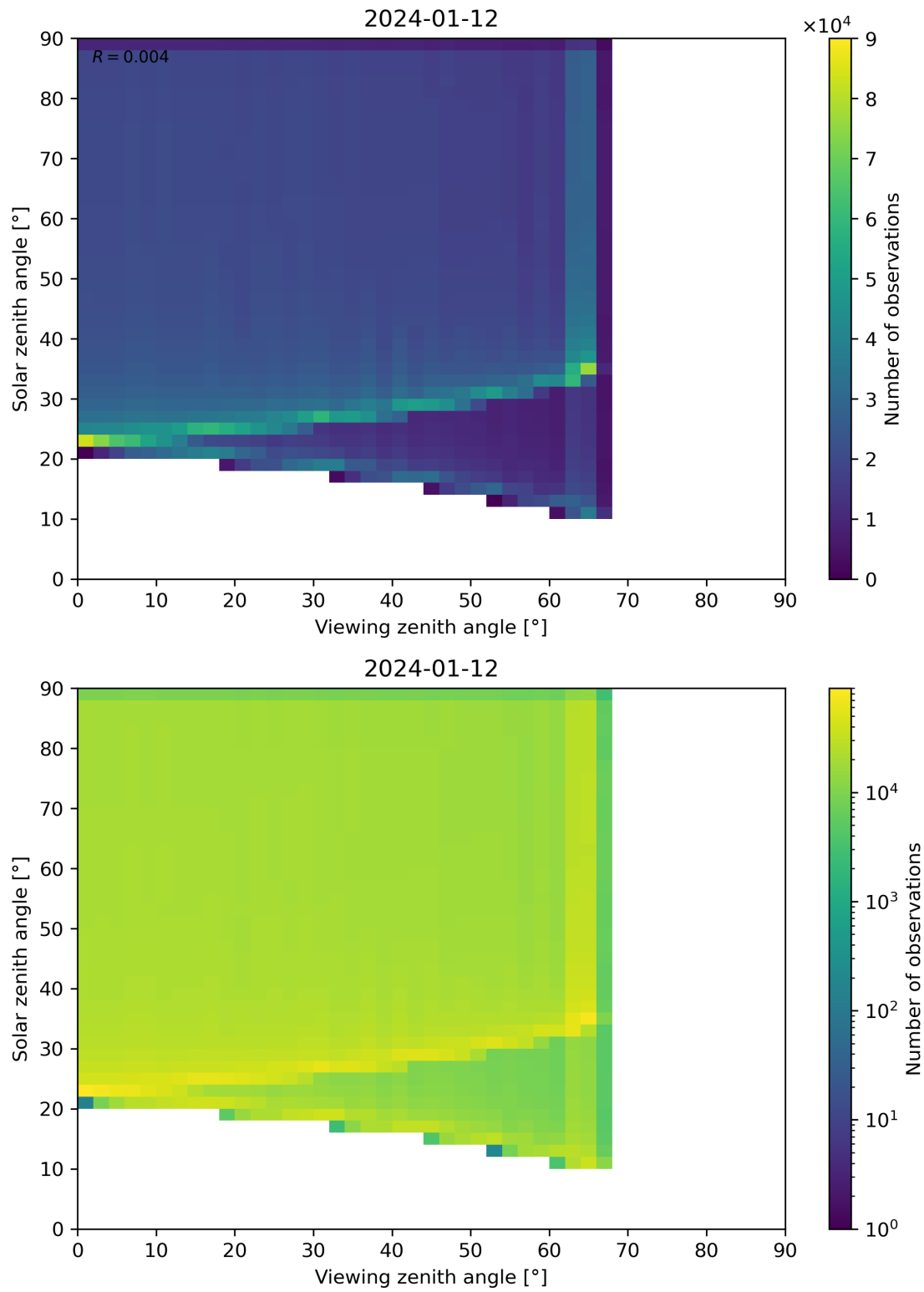
Figure 54: Scatter density plot of “Viewing zenith angle” against “Solar zenith angle” for 2024-01-11 to 2024-01-13.
