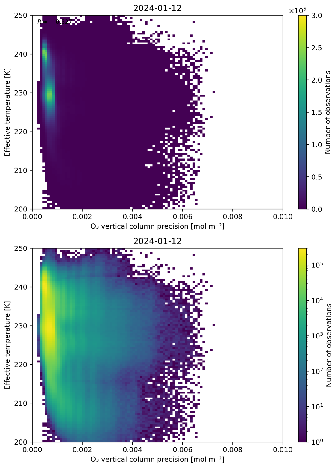
Figure 42: Scatter density plot of “O 3 vertical column precision” against “Effective temperature” for 2024-01-11 to 2024-01-13.
