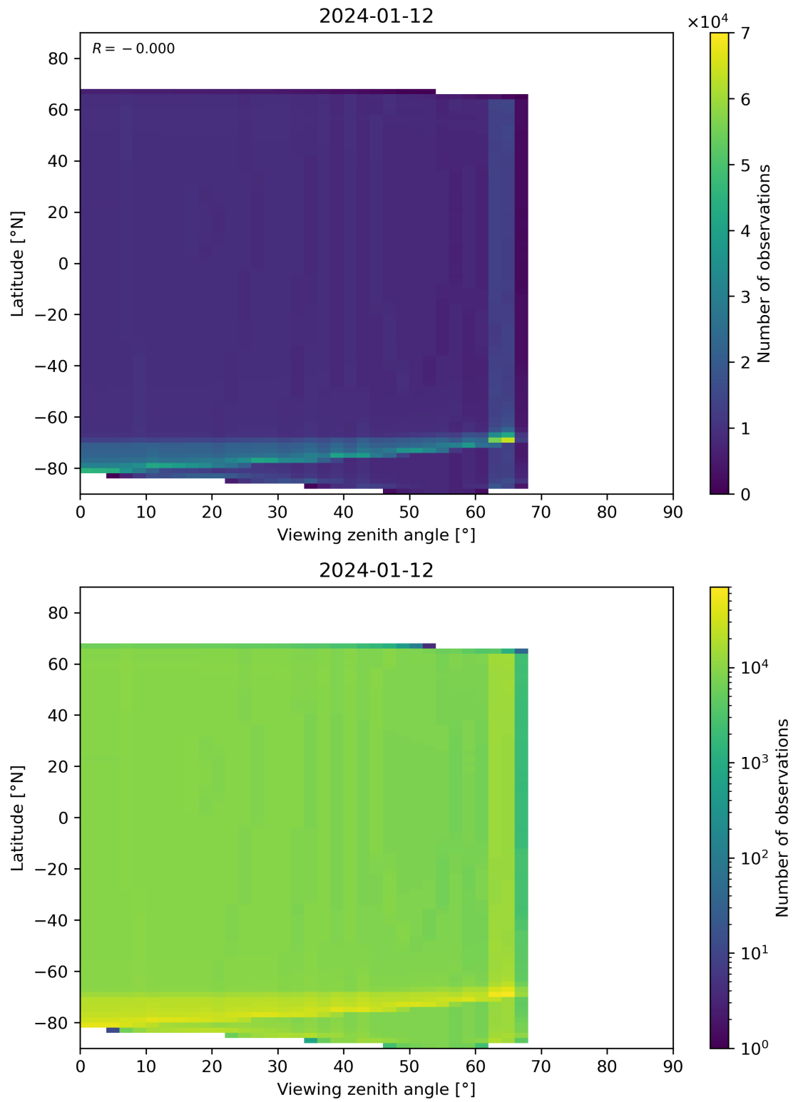
Figure 49: Scatter density plot of “Viewing zenith angle” against “Latitude” for 2024-01-11 to 2024-01-13.
