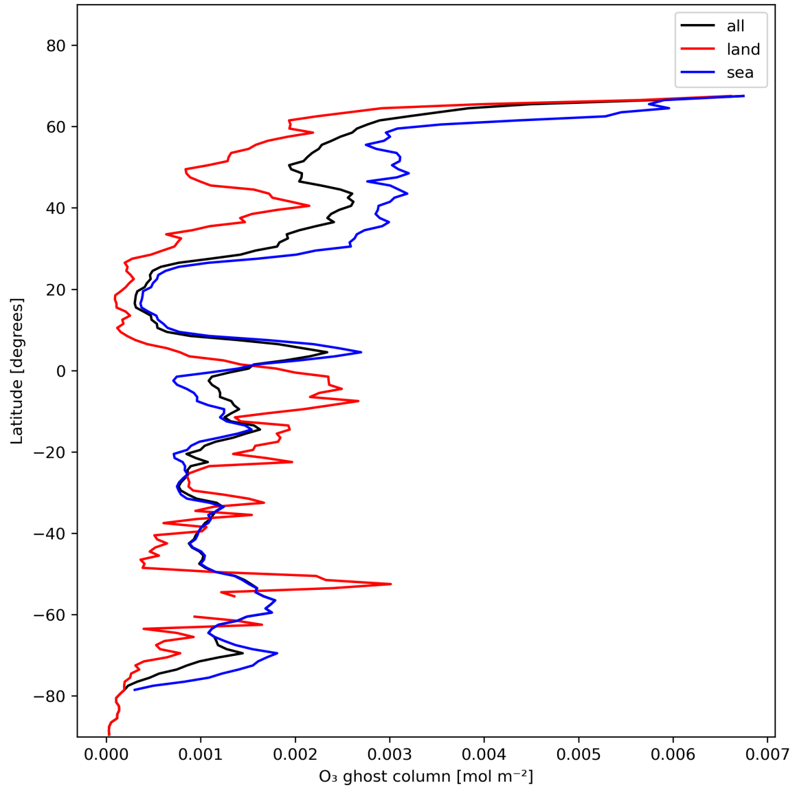
Figure 18: Zonal average of "O 3 ghost column" for 2024-01-11 to 2024-01-13.
