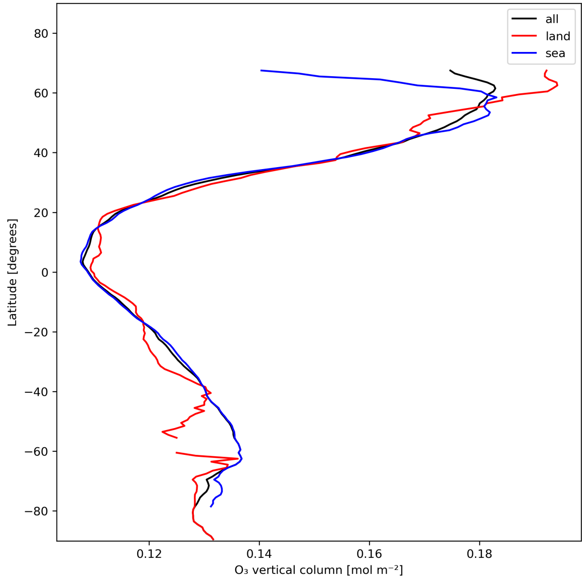
Figure 14: Zonal average of “O 3 vertical column” for 2024-01-11 to 2024-01-13.
