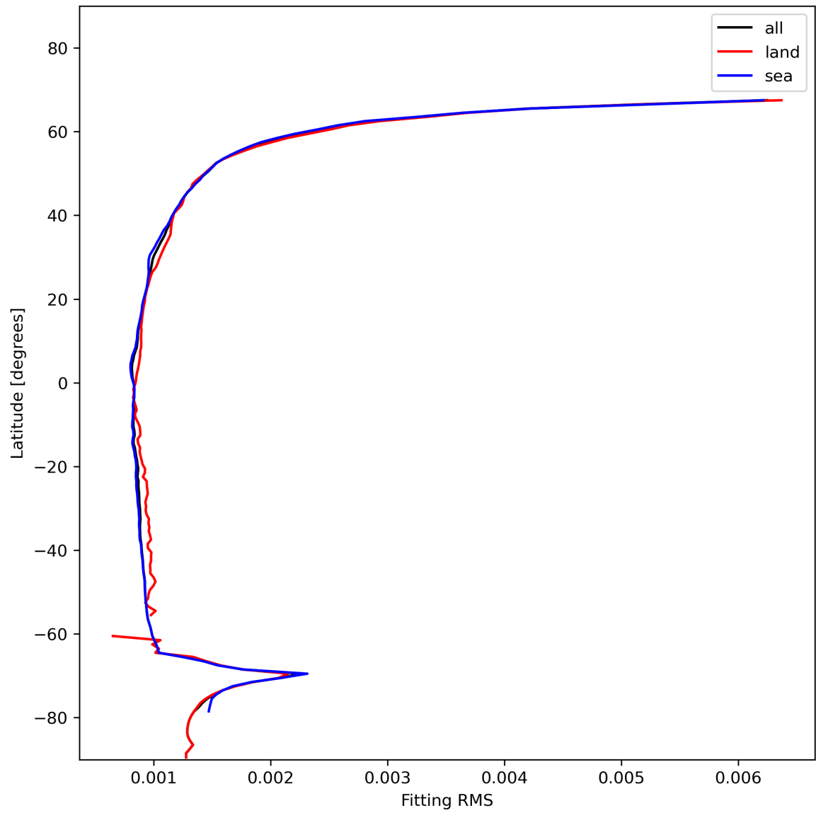
Figure 16: Zonal average of “Fitting RMS” for 2024-01-11 to 2024-01-13.
