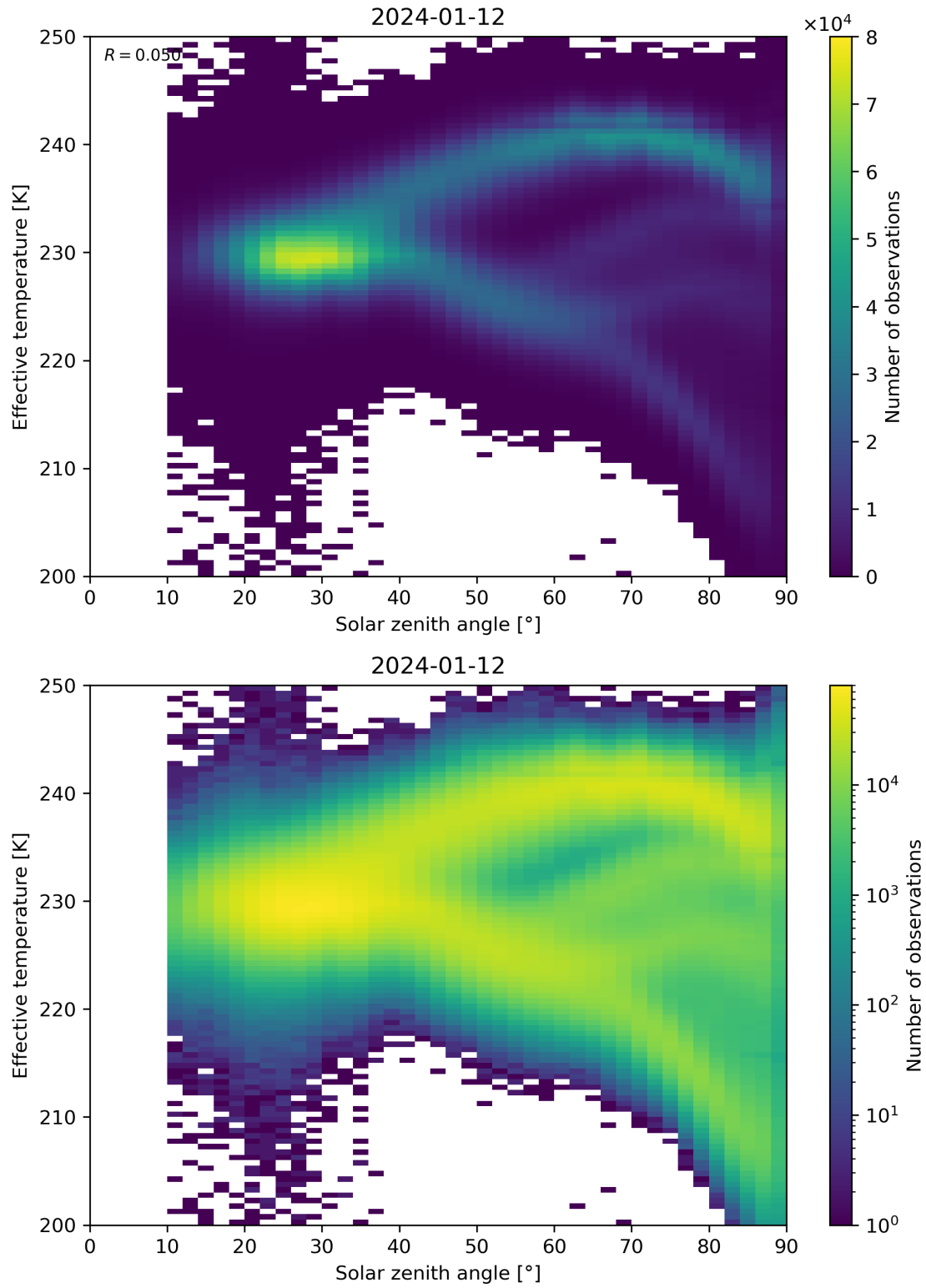
Figure 45: Scatter density plot of “Solar zenith angle” against “Effective temperature” for 2024-01-11 to 2024-01-13.
