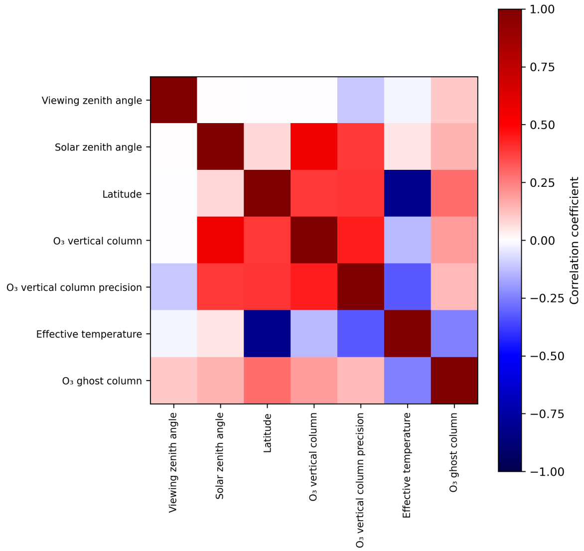
Figure 2: Map of correlation matrix for 2024-01-11 to 2024-01-13.
