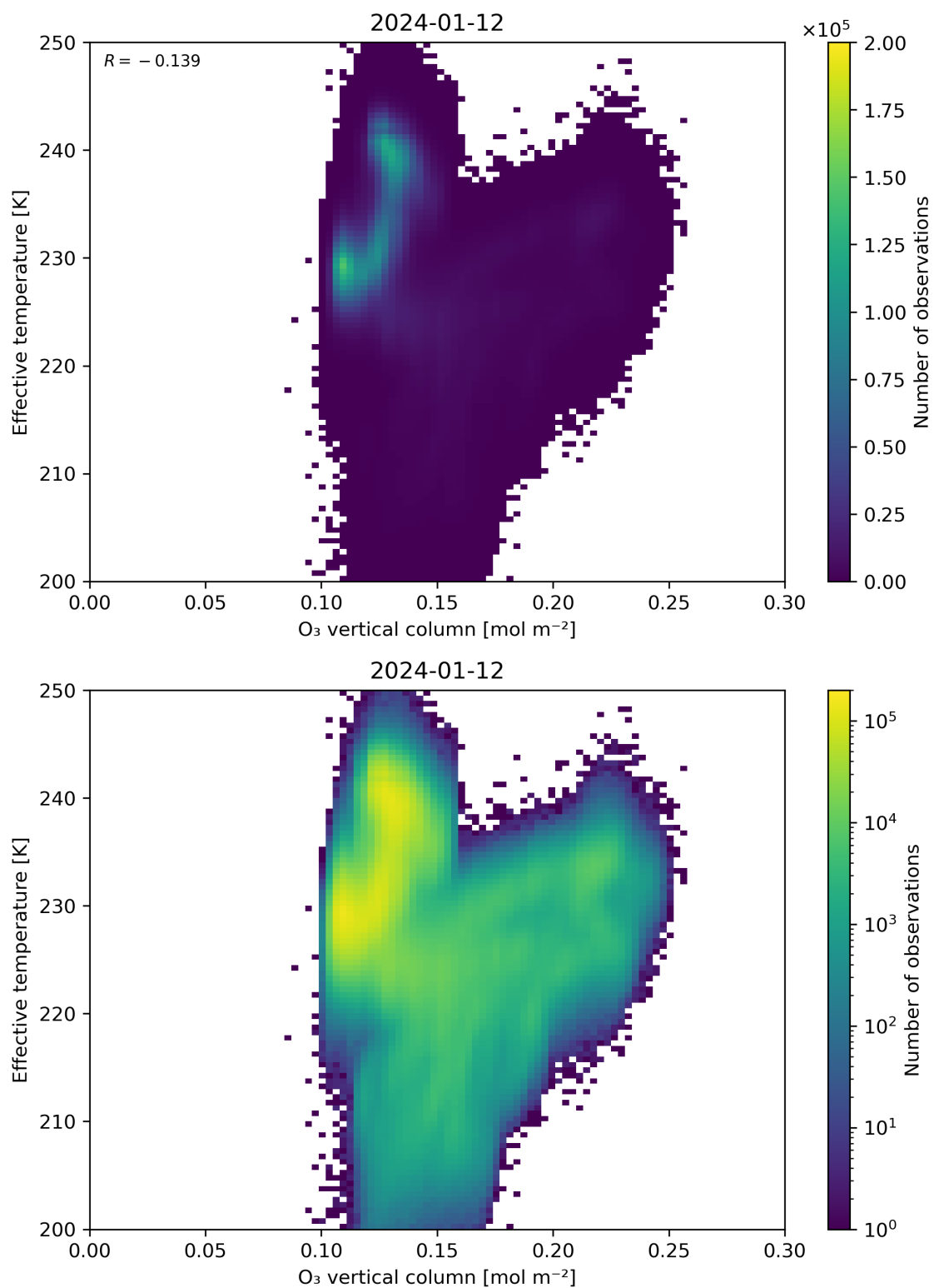
Figure 39: Scatter density plot of “O 3 vertical column” against “Effective temperature” for 2024-01-11 to 2024-01-13.
