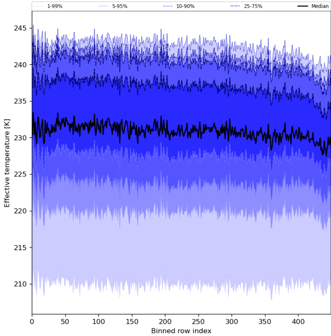
Figure 31: Along track statistics of “Effective temperature” for 2024-01-11 to 2024-01-13
