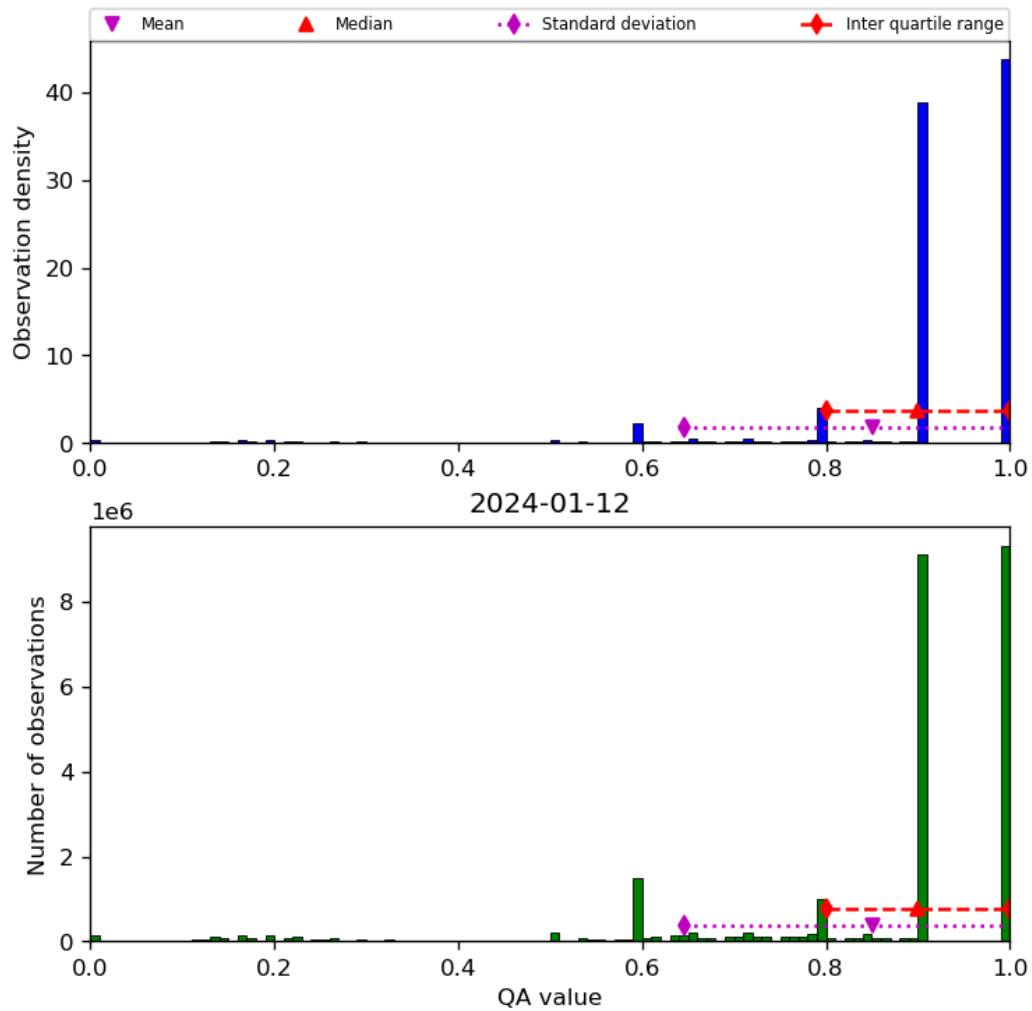
Figure 20: Histogram of “QA value” for 2024-01-11 to 2024-01-13
