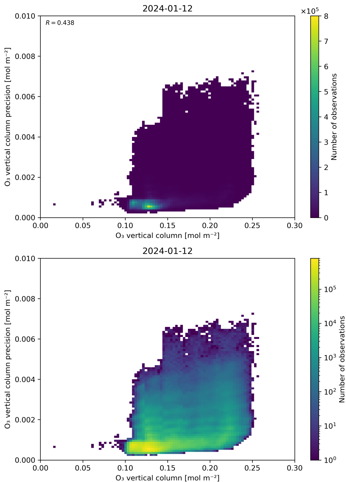
Figure 41: Scatter density plot of “O 3 vertical column” against “O 3 vertical column precision” for 2024-01-11 to 2024-01-13.
