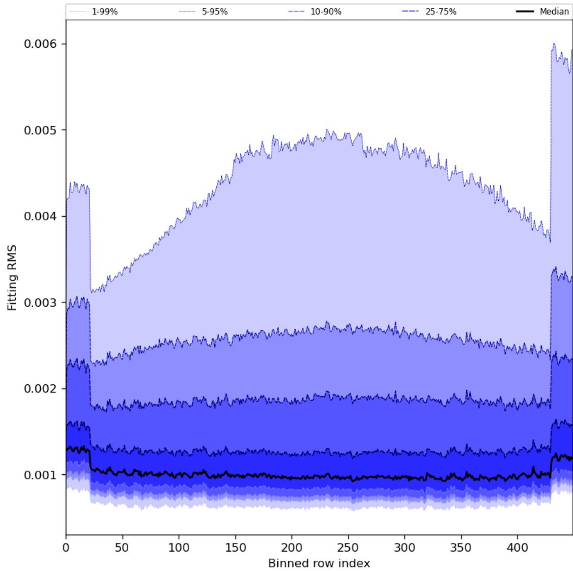
Figure 30: Along track statistics of “Fitting RMS” for 2024-01-11 to 2024-01-13
