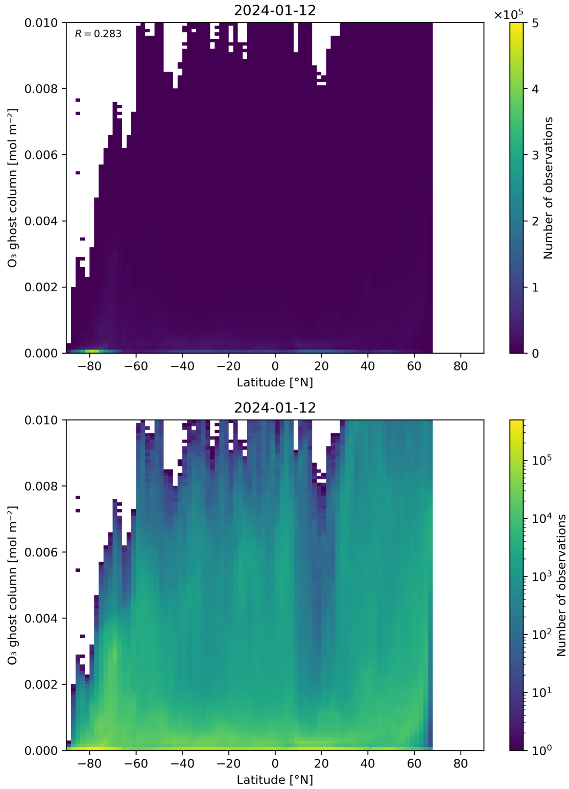
Figure 35: Scatter density plot of “Latitude” against “O 3 ghost column” for 2024-01-11 to 2024-01-13.
