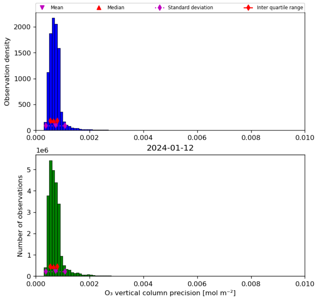
Figure 22: Histogram of “O 3 vertical column precision” for 2024-01-11 to 2024-01-13
