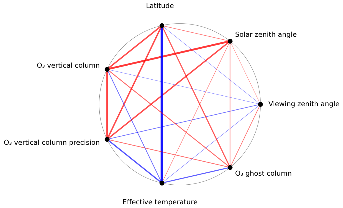
Figure 1: Map of correlation graph for 2024-01-11 to 2024-01-13.
