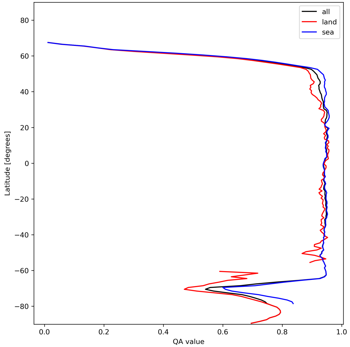
Figure 13: Zonal average of “QA value” for 2024-01-11 to 2024-01-13.
