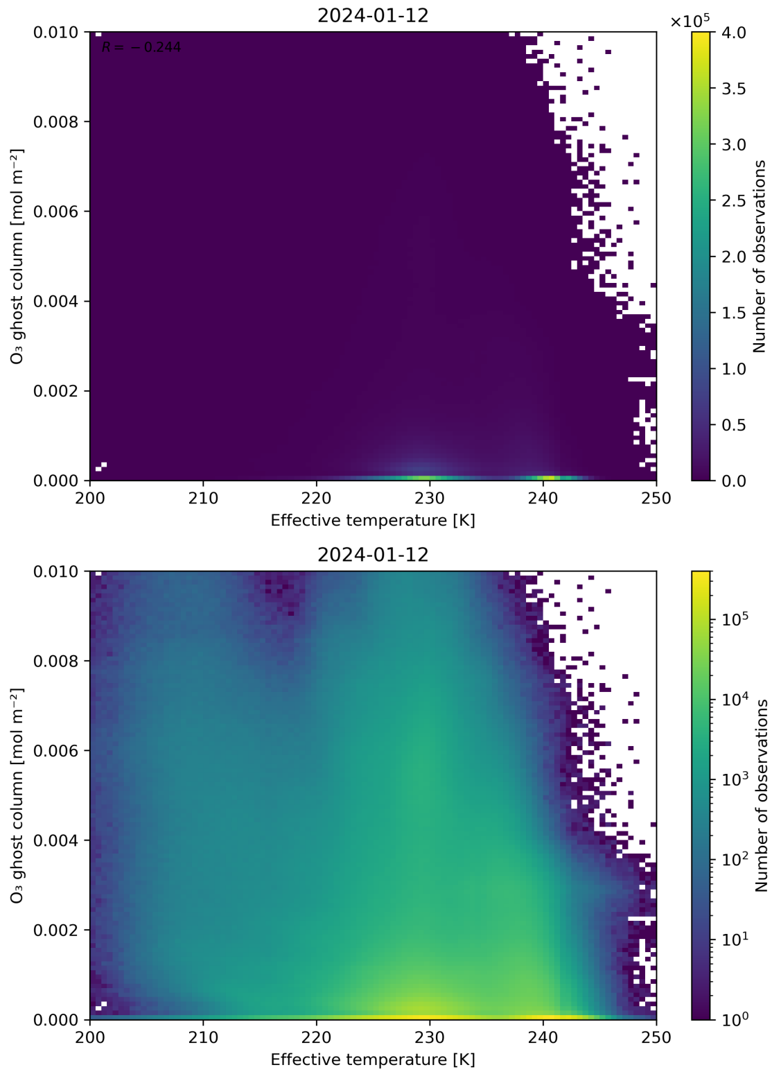
Figure 38: Scatter density plot of “Effective temperature” against “O 3 ghost column” for 2024-01-11 to 2024-01-13.
