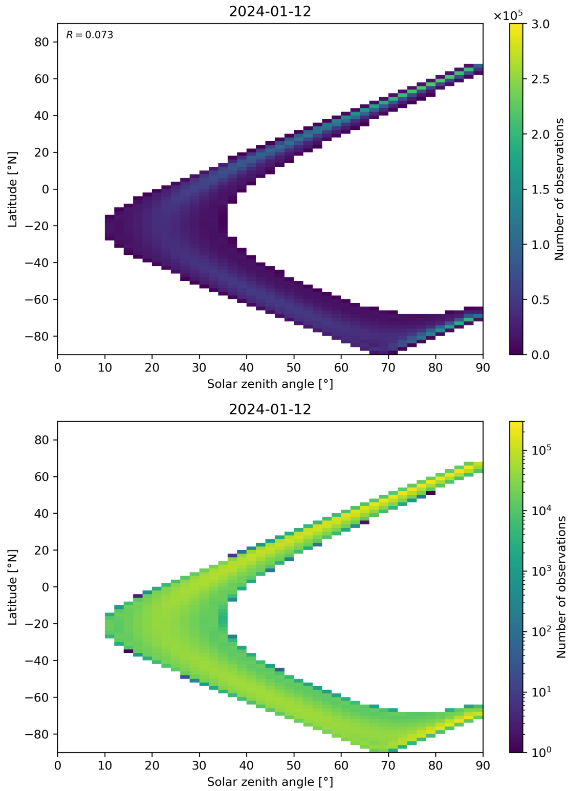
Figure 44: Scatter density plot of “Solar zenith angle” against “Latitude” for 2024-01-11 to 2024-01-13.
