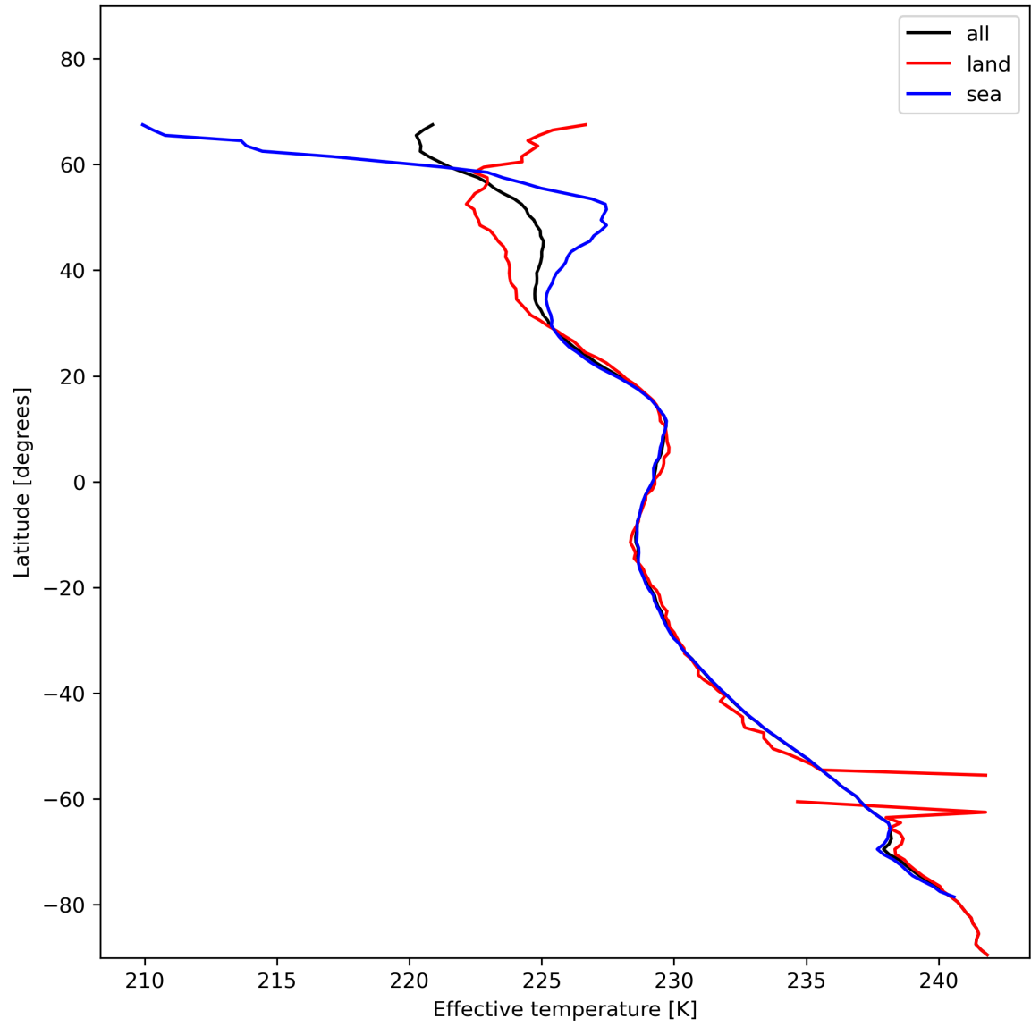
Figure 17: Zonal average of “Effective temperature” for 2024-01-11 to 2024-01-13.
