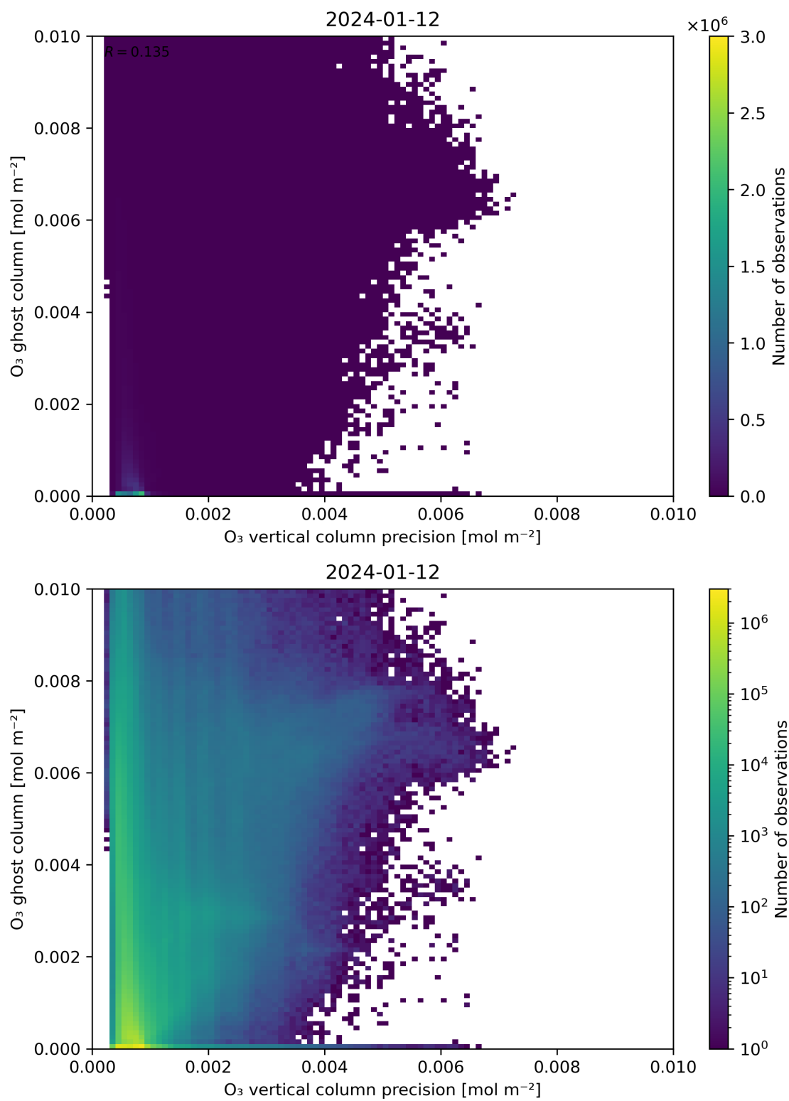
Figure 43: Scatter density plot of “ \text{O}_3 vertical column precision” against “ \text{O}_3 ghost column” for 2024-01-11 to 2024-01-13.
