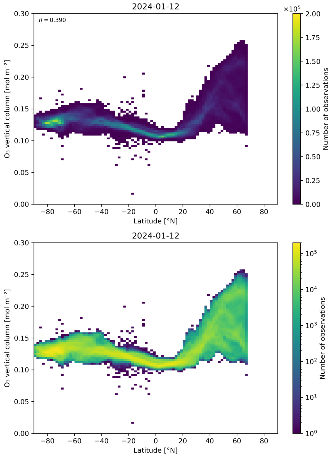
Figure 36: Scatter density plot of “Latitude” against “O 3 vertical column” for 2024-01-11 to 2024-01-13.
