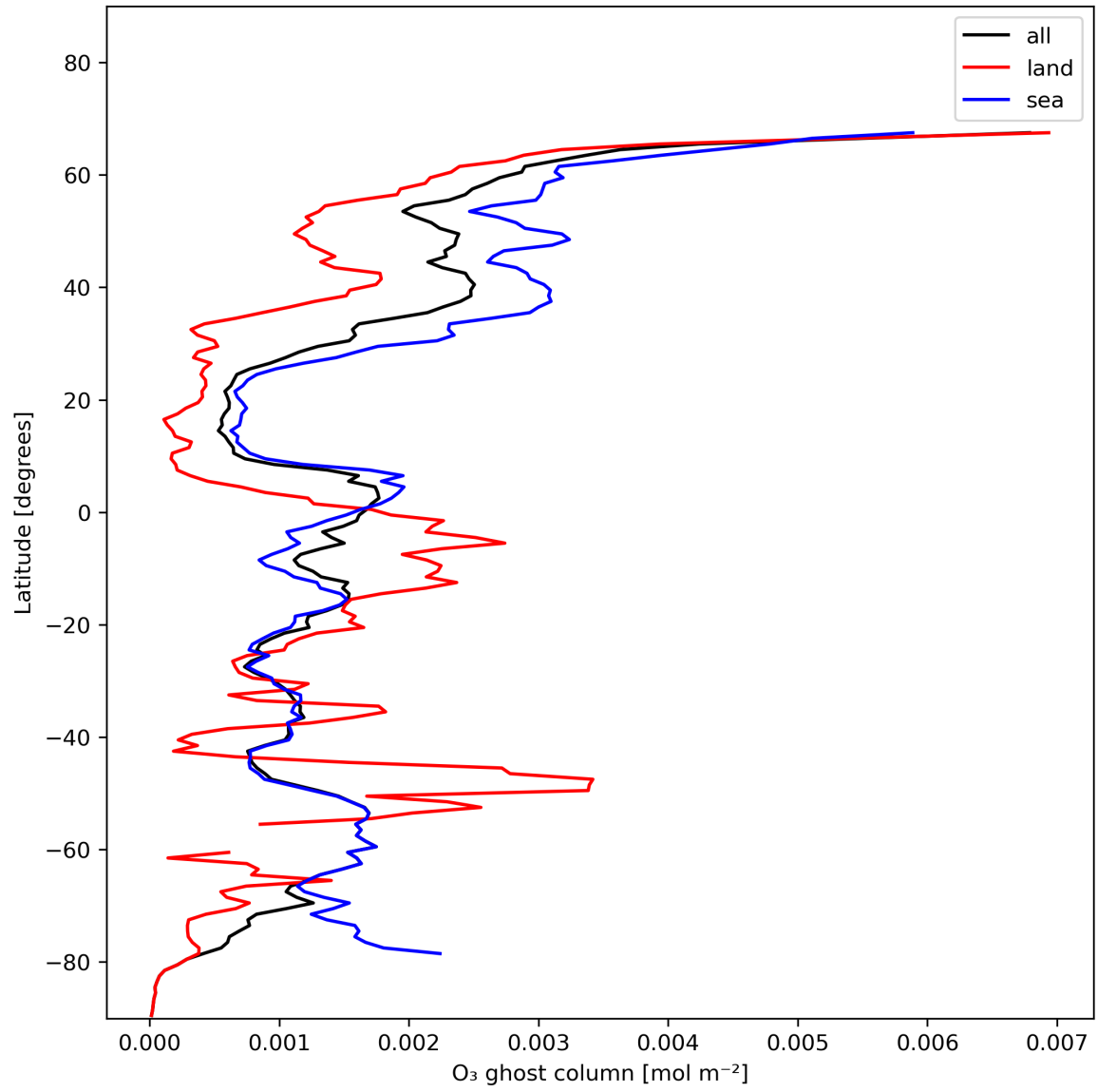
Figure 18: Zonal average of “O 3 ghost column” for 2024-01-12 to 2024-01-14.
