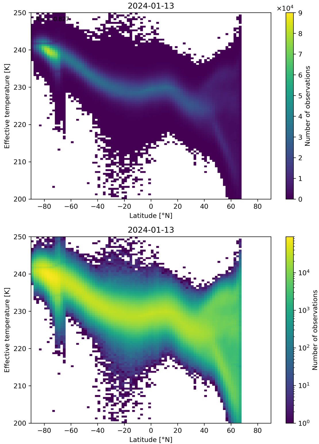
Figure 34: Scatter density plot of “Latitude” against “Effective temperature” for 2024-01-12 to 2024-01-14.
