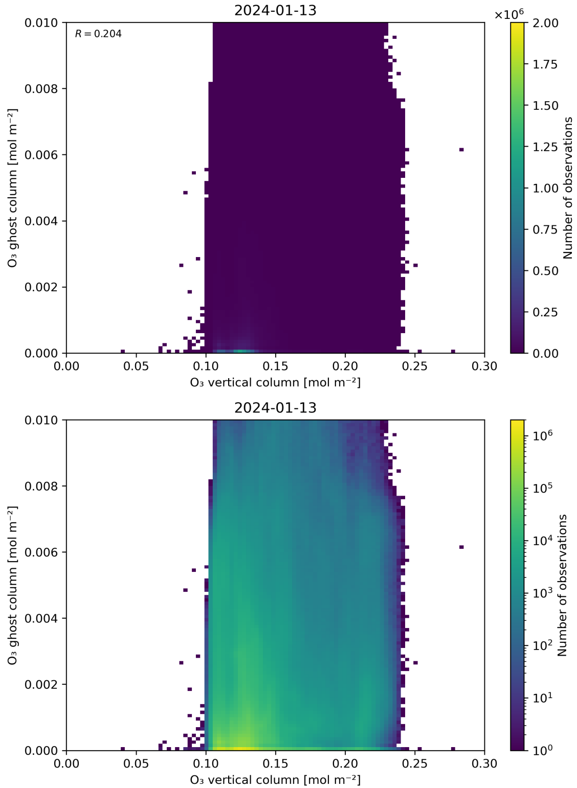
Figure 40: Scatter density plot of “O 3 vertical column” against “O 3 ghost column” for 2024-01-12 to 2024-01-14.
