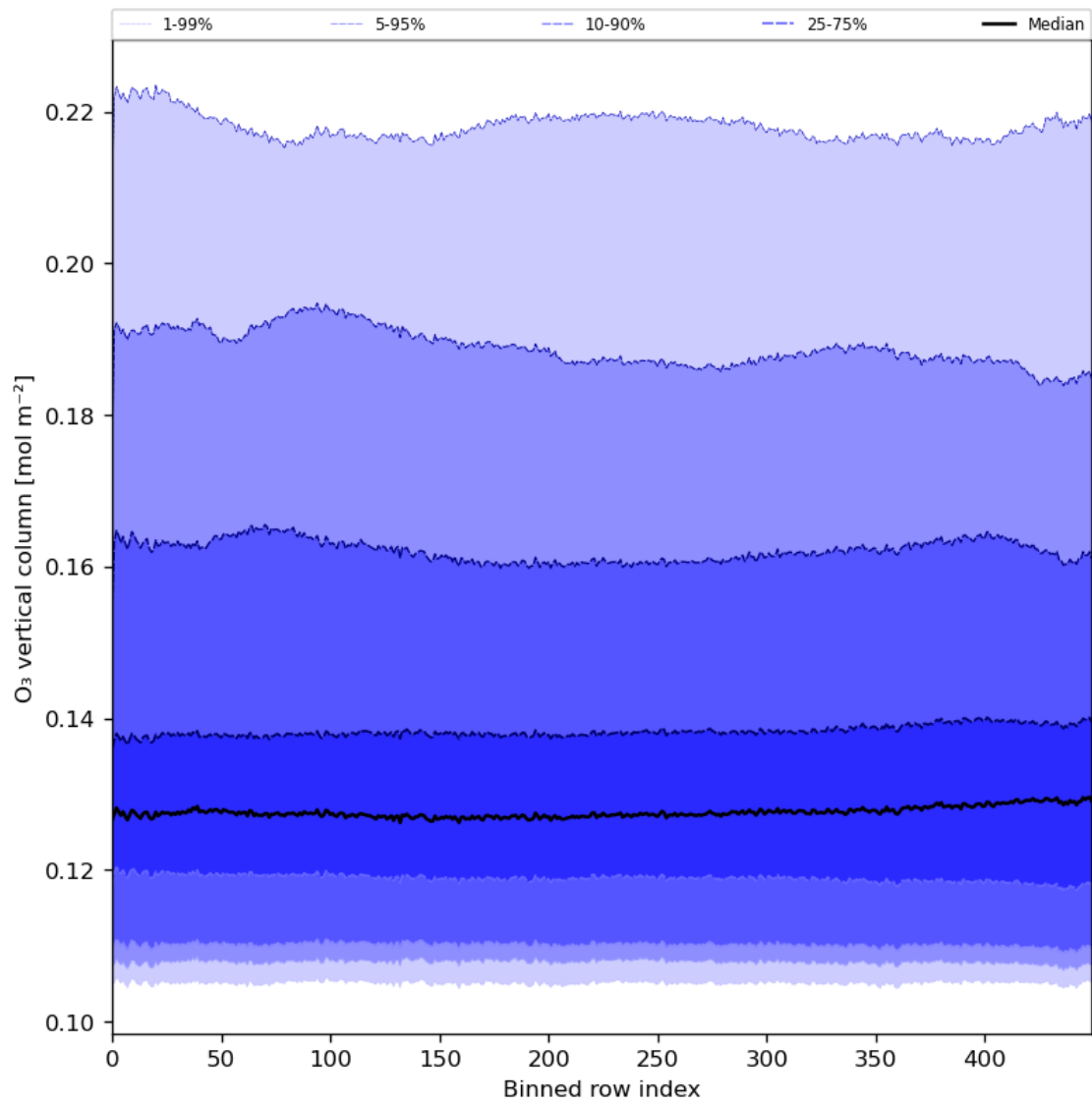
Figure 28: Along track statistics of “O 3 vertical column” for 2024-01-12 to 2024-01-14
