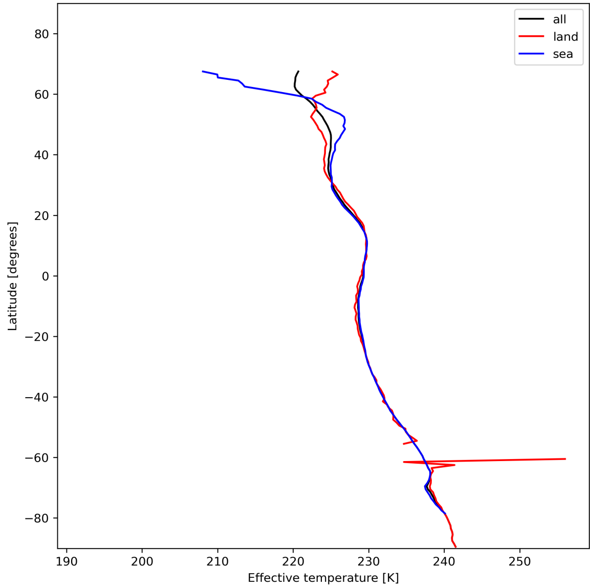
Figure 17: Zonal average of “Effective temperature” for 2024-01-12 to 2024-01-14.
