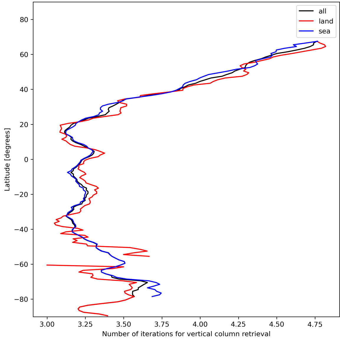
Figure 19: Zonal average of “Number of iterations for vertical column retrieval” for 2024-01-12 to 2024-01-14.
