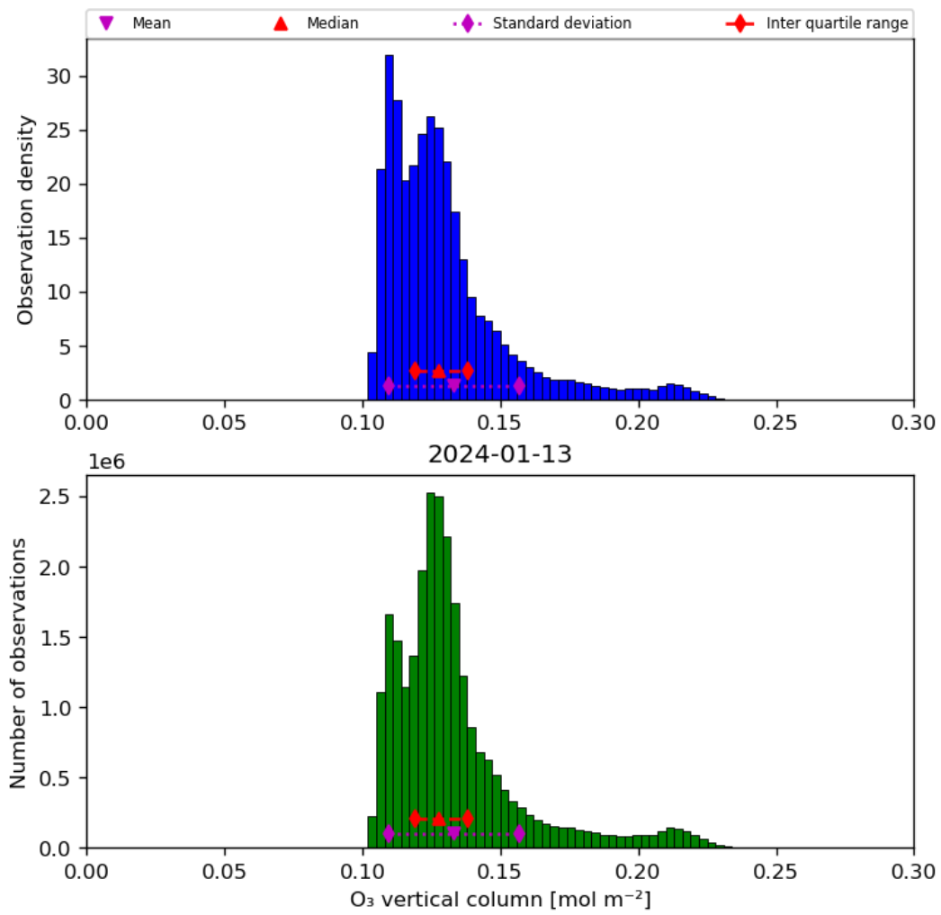
Figure 21: Histogram of “O 3 vertical column” for 2024-01-12 to 2024-01-14
