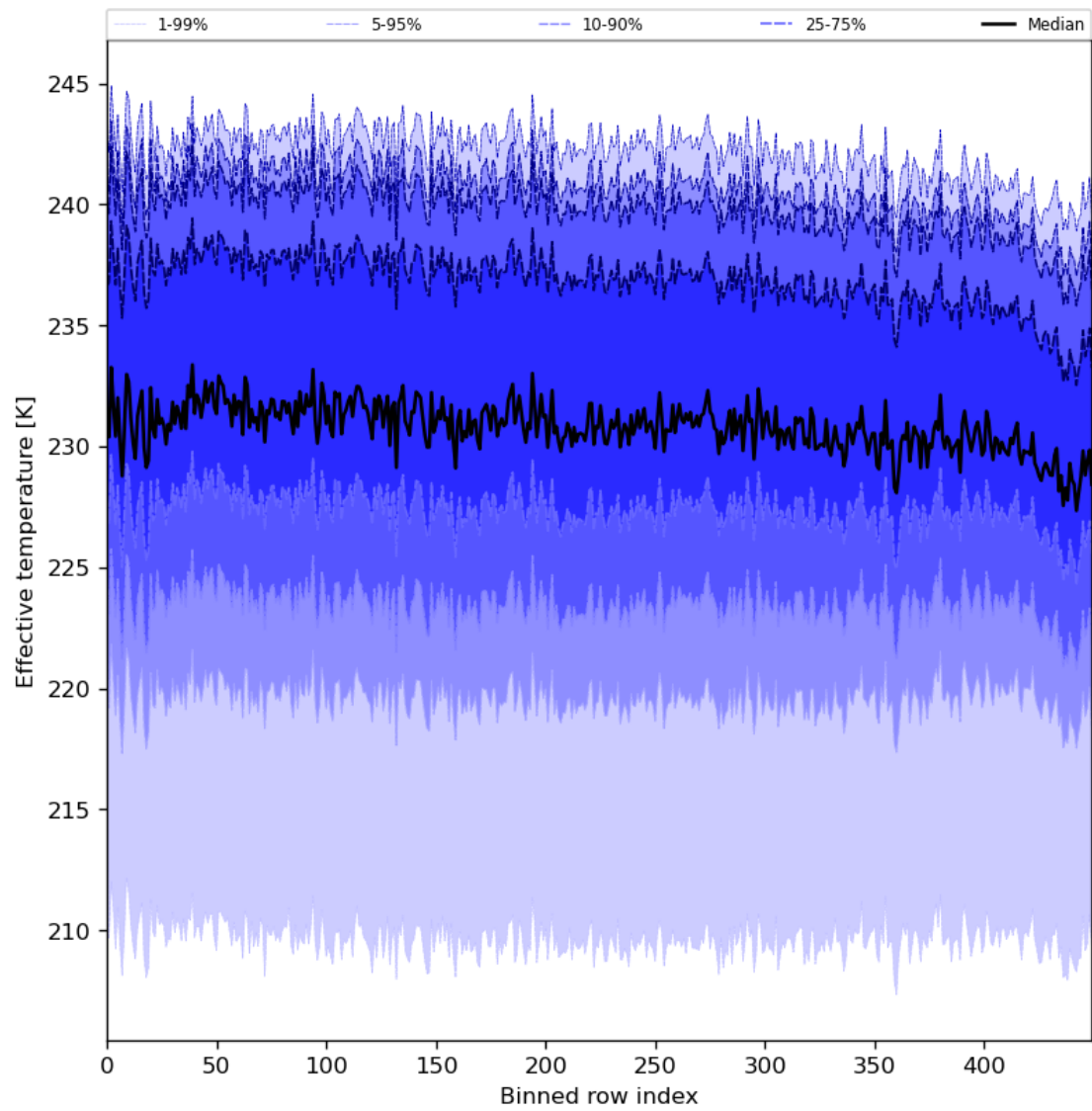
Figure 31: Along track statistics of “Effective temperature” for 2024-01-12 to 2024-01-14
