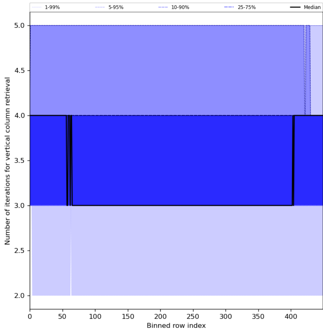
Figure 33: Along track statistics of “Number of iterations for vertical column retrieval” for 2024-01-12 to 2024-01-14
