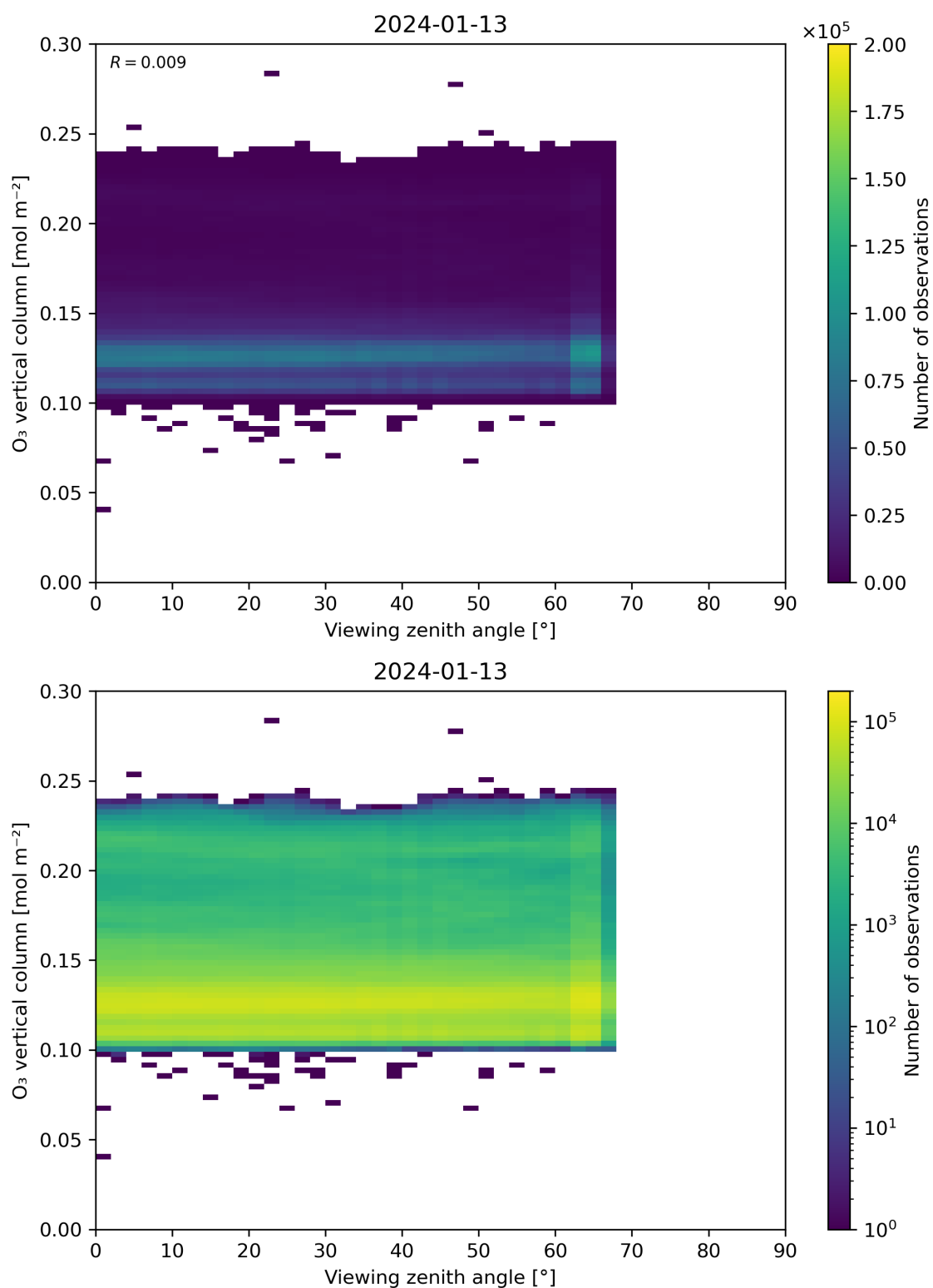
Figure 52: Scatter density plot of “Viewing zenith angle” against “O 3 vertical column” for 2024-01-12 to 2024-01-14.
