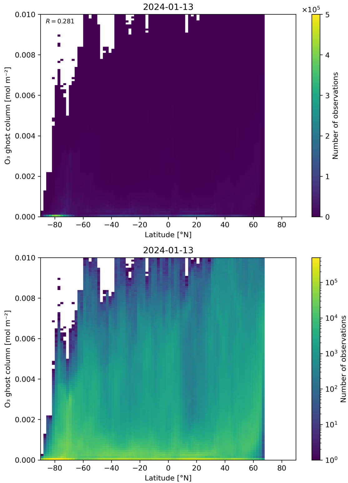
Figure 35: Scatter density plot of “Latitude” against “O 3 ghost column” for 2024-01-12 to 2024-01-14.
