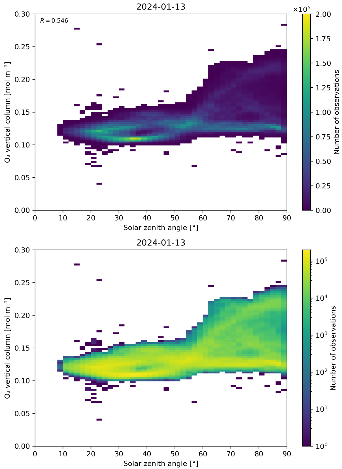
Figure 47: Scatter density plot of “Solar zenith angle” against “O 3 vertical column” for 2024-01-12 to 2024-01-14.
