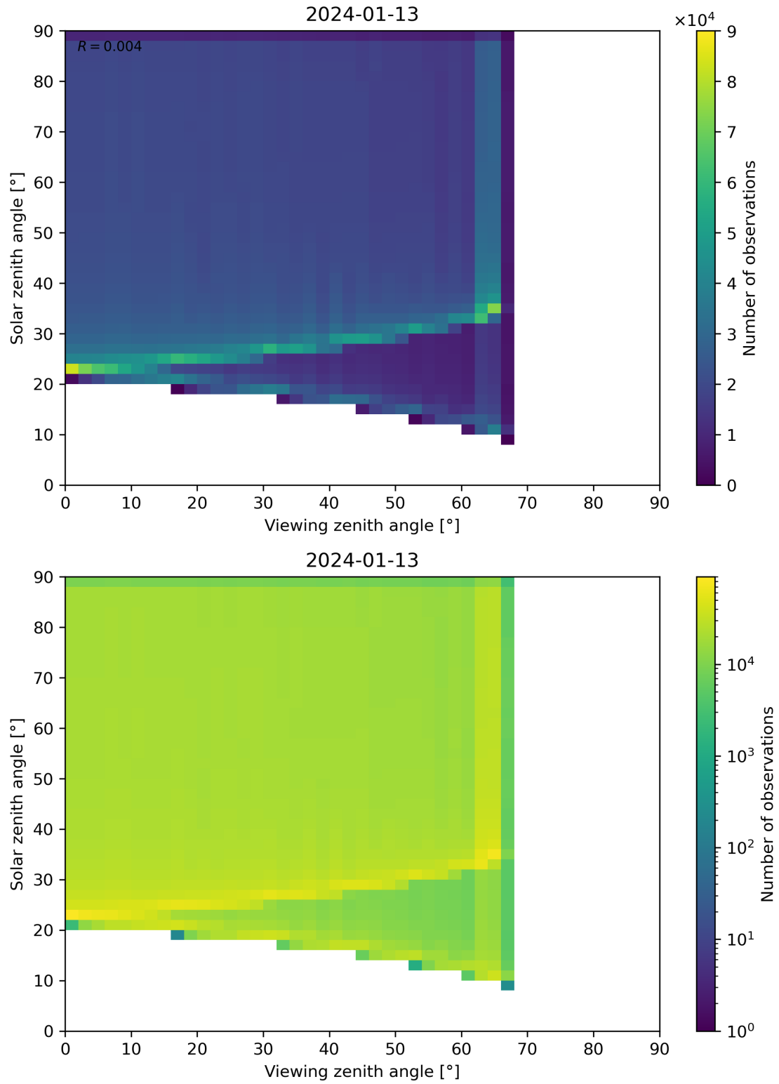
Figure 54: Scatter density plot of “Viewing zenith angle” against “Solar zenith angle” for 2024-01-12 to 2024-01-14.
