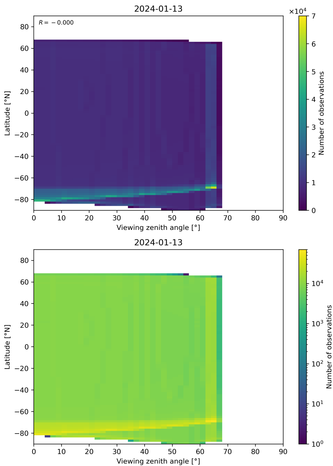
Figure 49: Scatter density plot of “Viewing zenith angle” against “Latitude” for 2024-01-12 to 2024-01-14.
