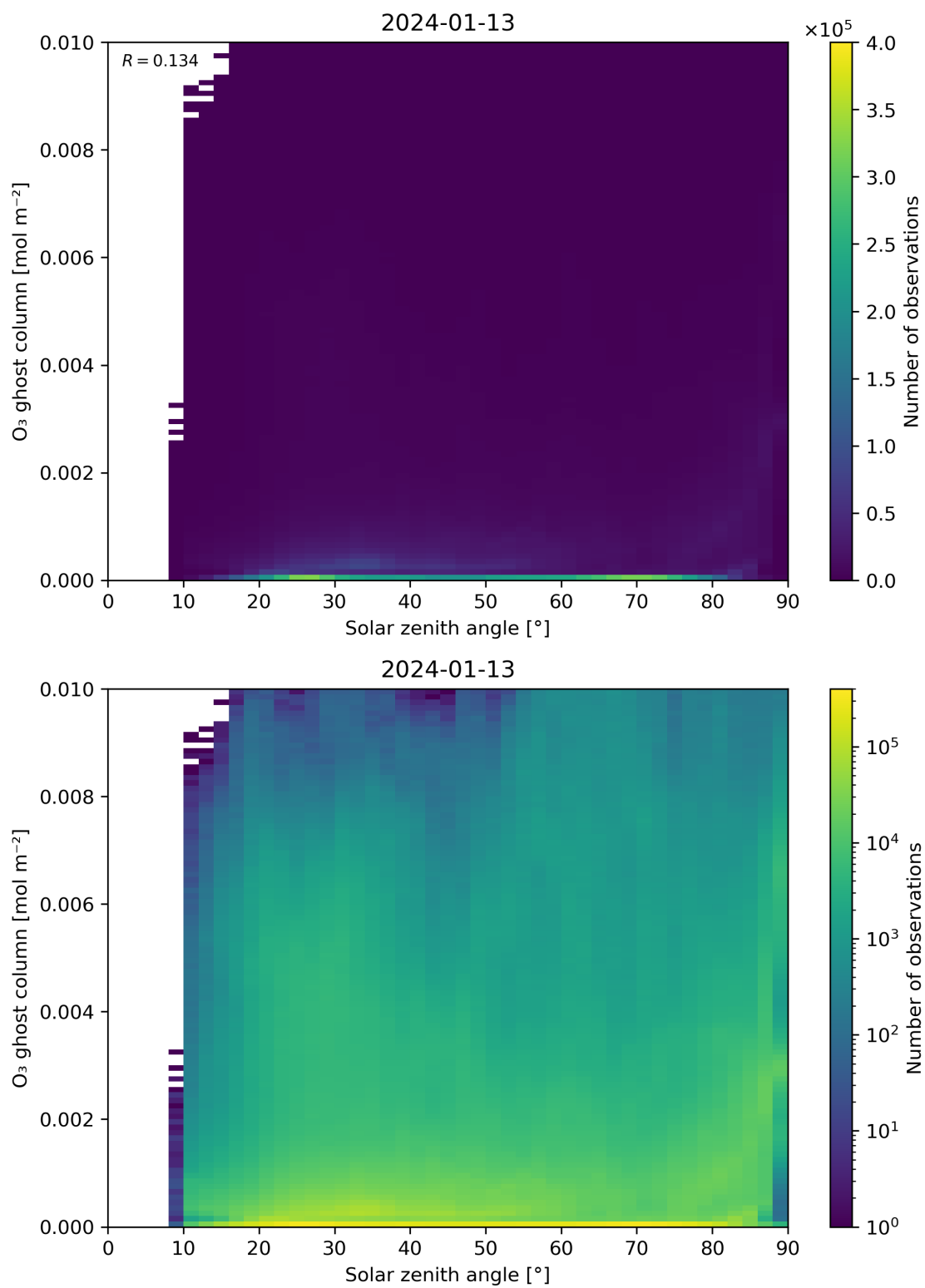
Figure 46: Scatter density plot of “Solar zenith angle” against “O 3 ghost column” for 2024-01-12 to 2024-01-14.
