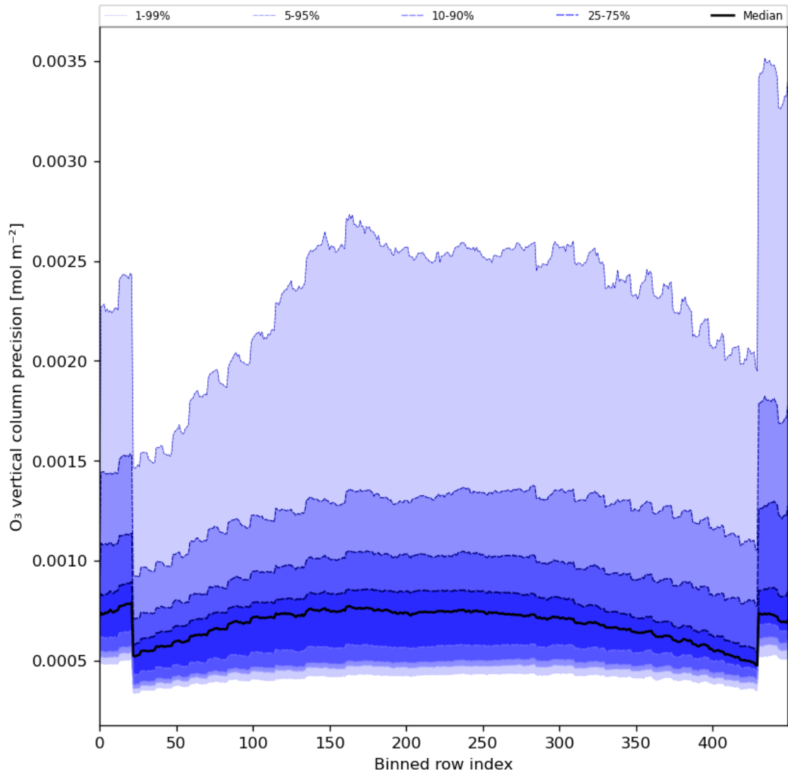
Figure 29: Along track statistics of “O 3 vertical column precision” for 2024-01-12 to 2024-01-14
