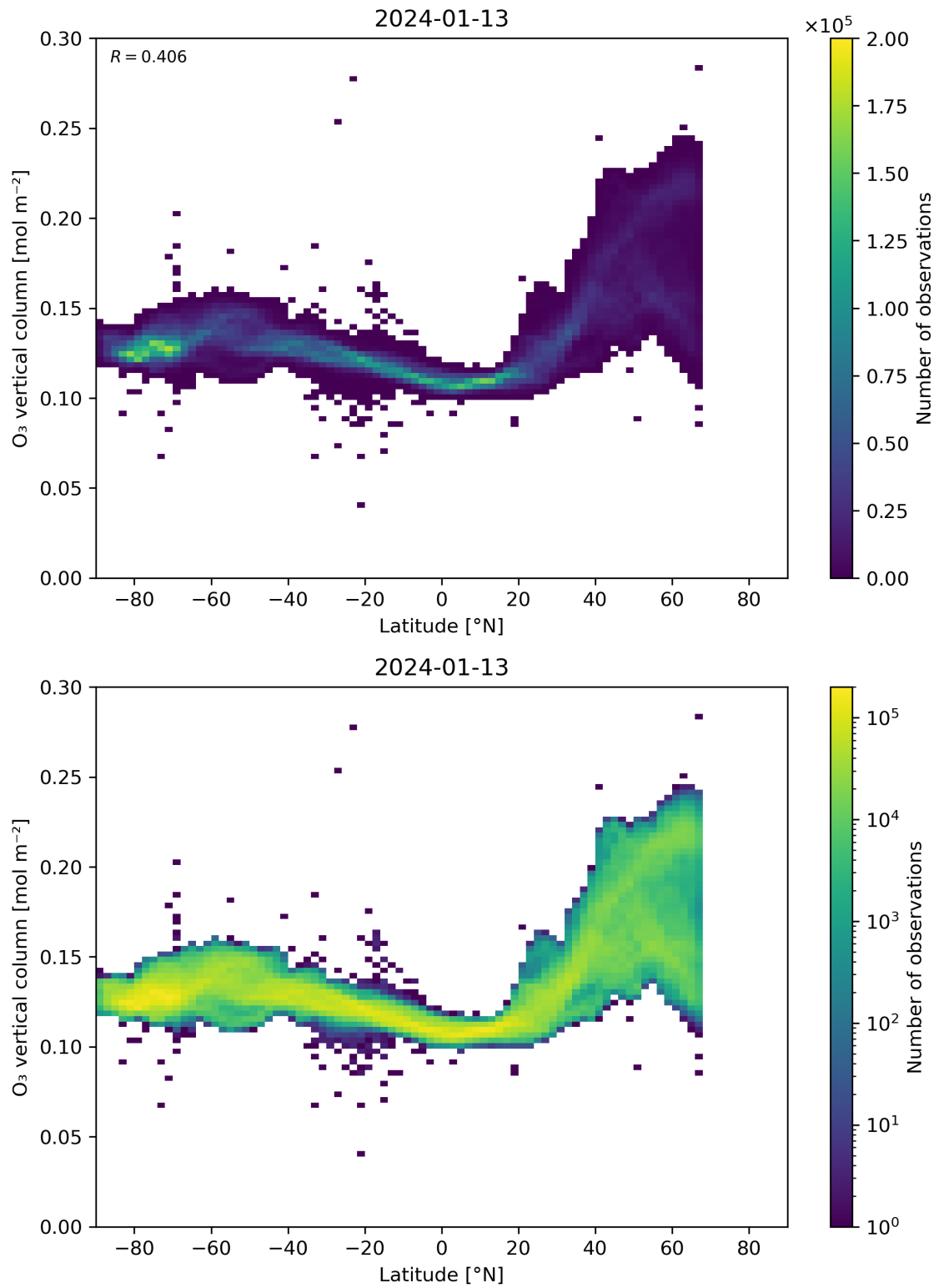
Figure 36: Scatter density plot of “Latitude” against “O 3 vertical column” for 2024-01-12 to 2024-01-14.
