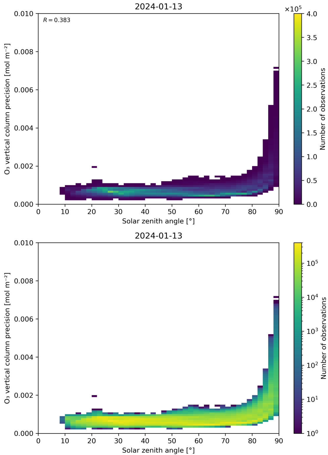
Figure 48: Scatter density plot of “Solar zenith angle” against “O 3 vertical column precision” for 2024-01-12 to 2024-01-14.
