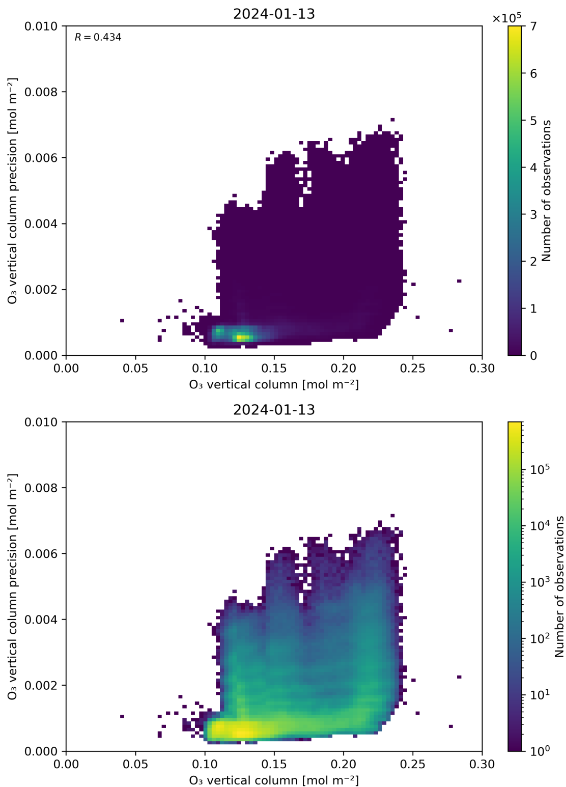
Figure 41: Scatter density plot of “O 3 vertical column” against “O 3 vertical column precision” for 2024-01-12 to 2024-01-14.
