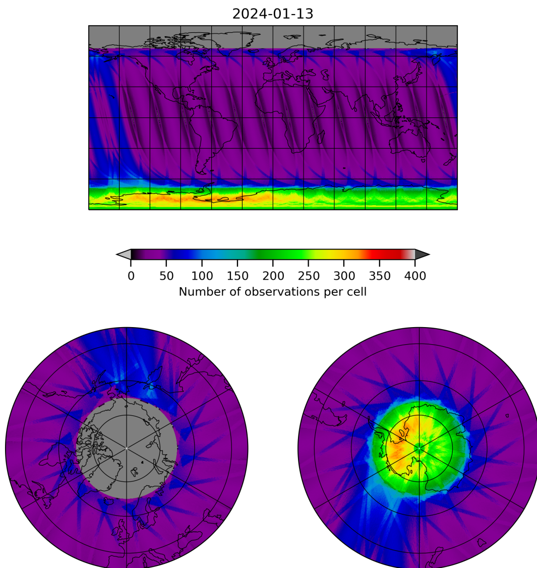
Figure 12: Map of the number of observations for 2024-01-12 to 2024-01-14
