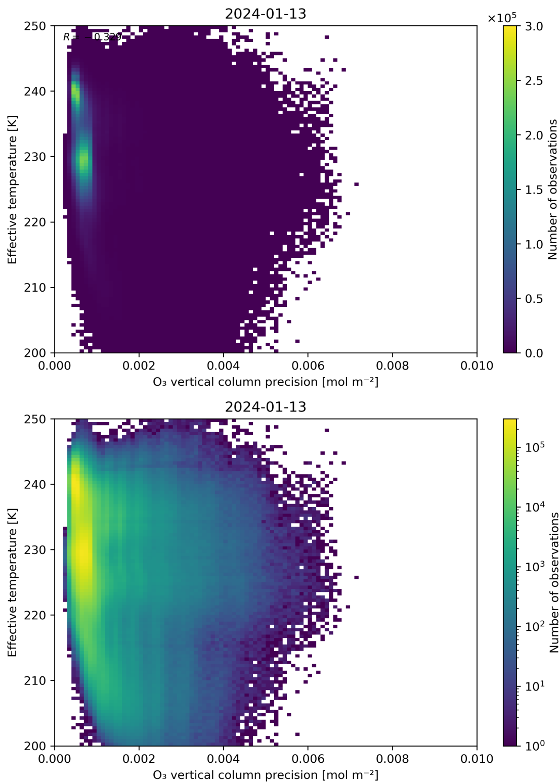
Figure 42: Scatter density plot of “O 3 vertical column precision” against “Effective temperature” for 2024-01-12 to 2024-01-14.
