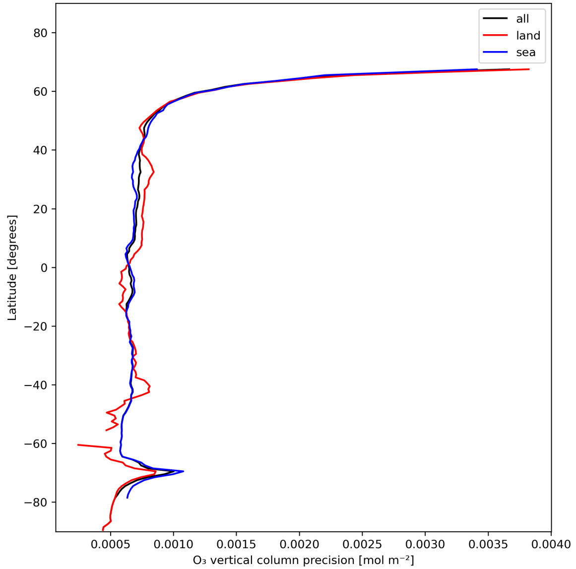
Figure 15: Zonal average of “O 3 vertical column precision” for 2024-01-12 to 2024-01-14.
