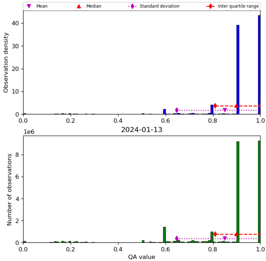
Figure 20: Histogram of “QA value” for 2024-01-12 to 2024-01-14
