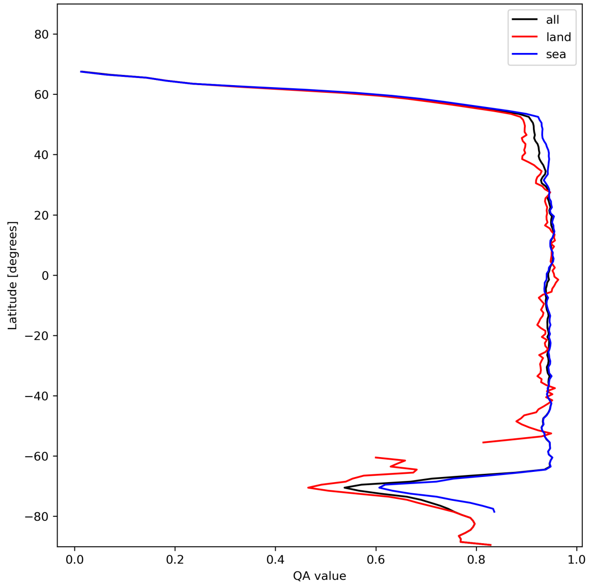
Figure 13: Zonal average of “QA value” for 2024-01-12 to 2024-01-14.
