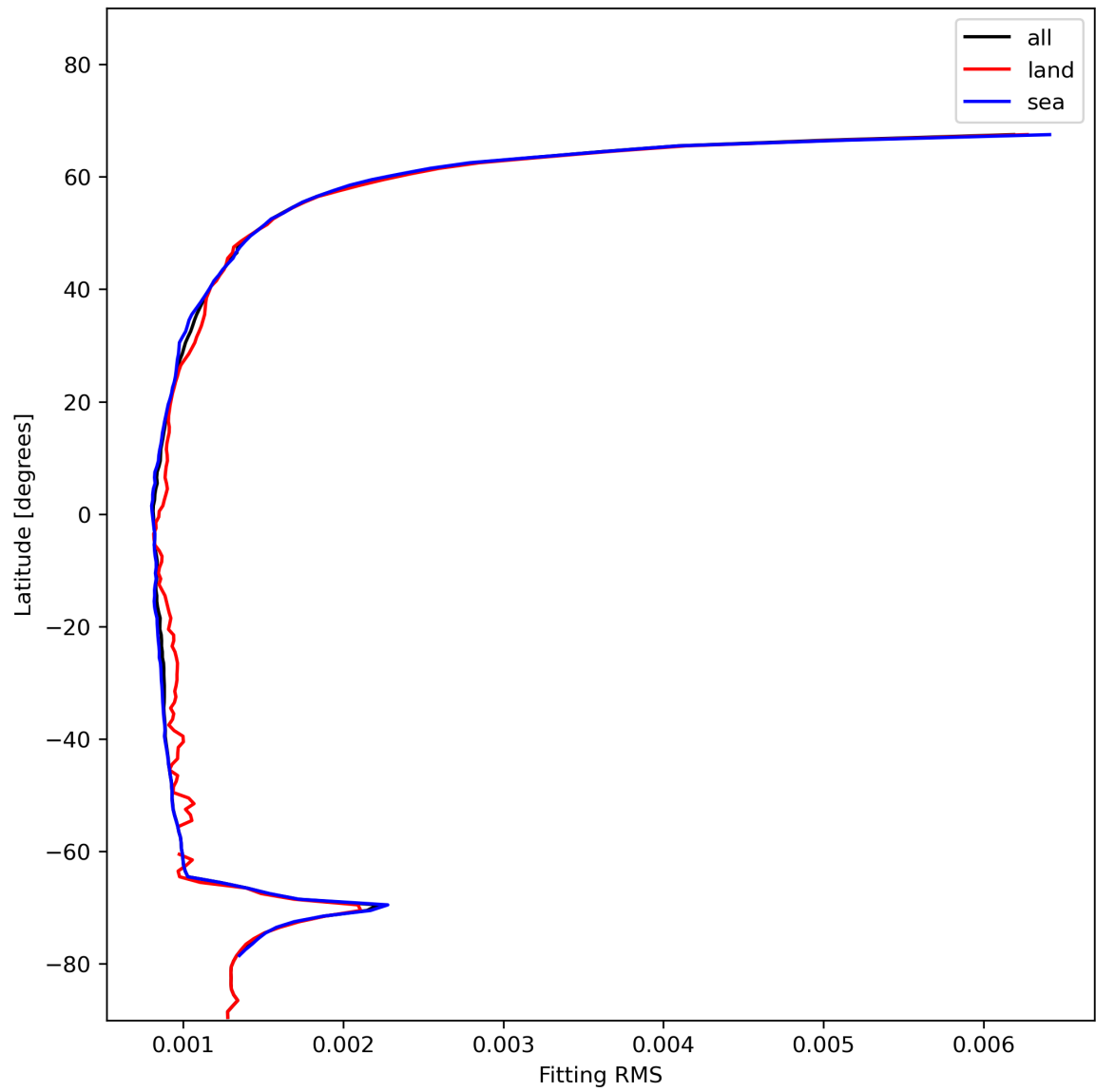
Figure 16: Zonal average of “Fitting RMS” for 2024-01-12 to 2024-01-14.
