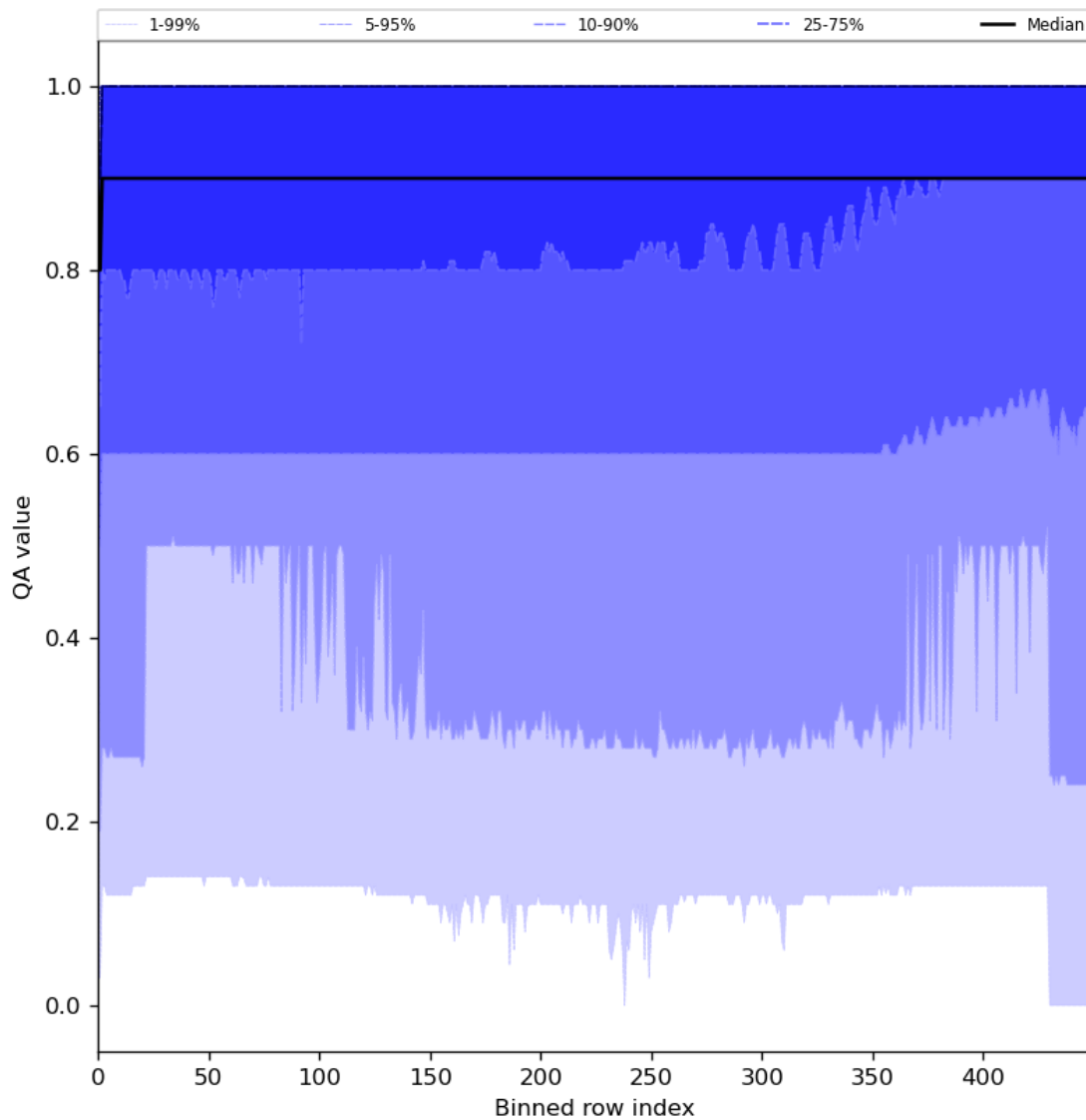
Figure 27: Along track statistics of “QA value” for 2024-01-12 to 2024-01-14
