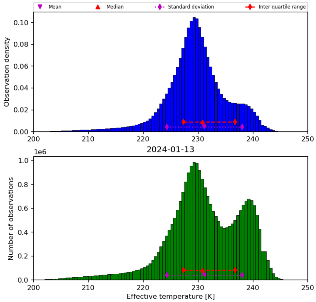
Figure 24: Histogram of “Effective temperature” for 2024-01-12 to 2024-01-14
