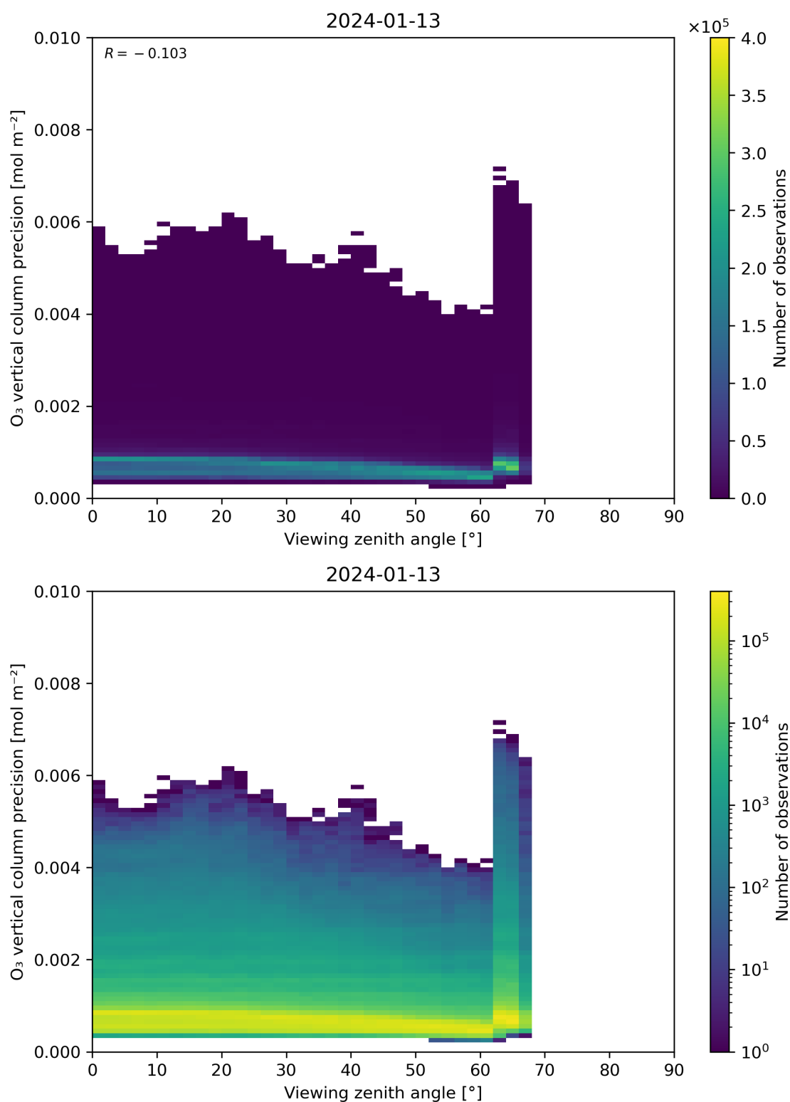
Figure 53: Scatter density plot of “Viewing zenith angle” against “O 3 vertical column precision” for 2024-01-12 to 2024-01-14.
