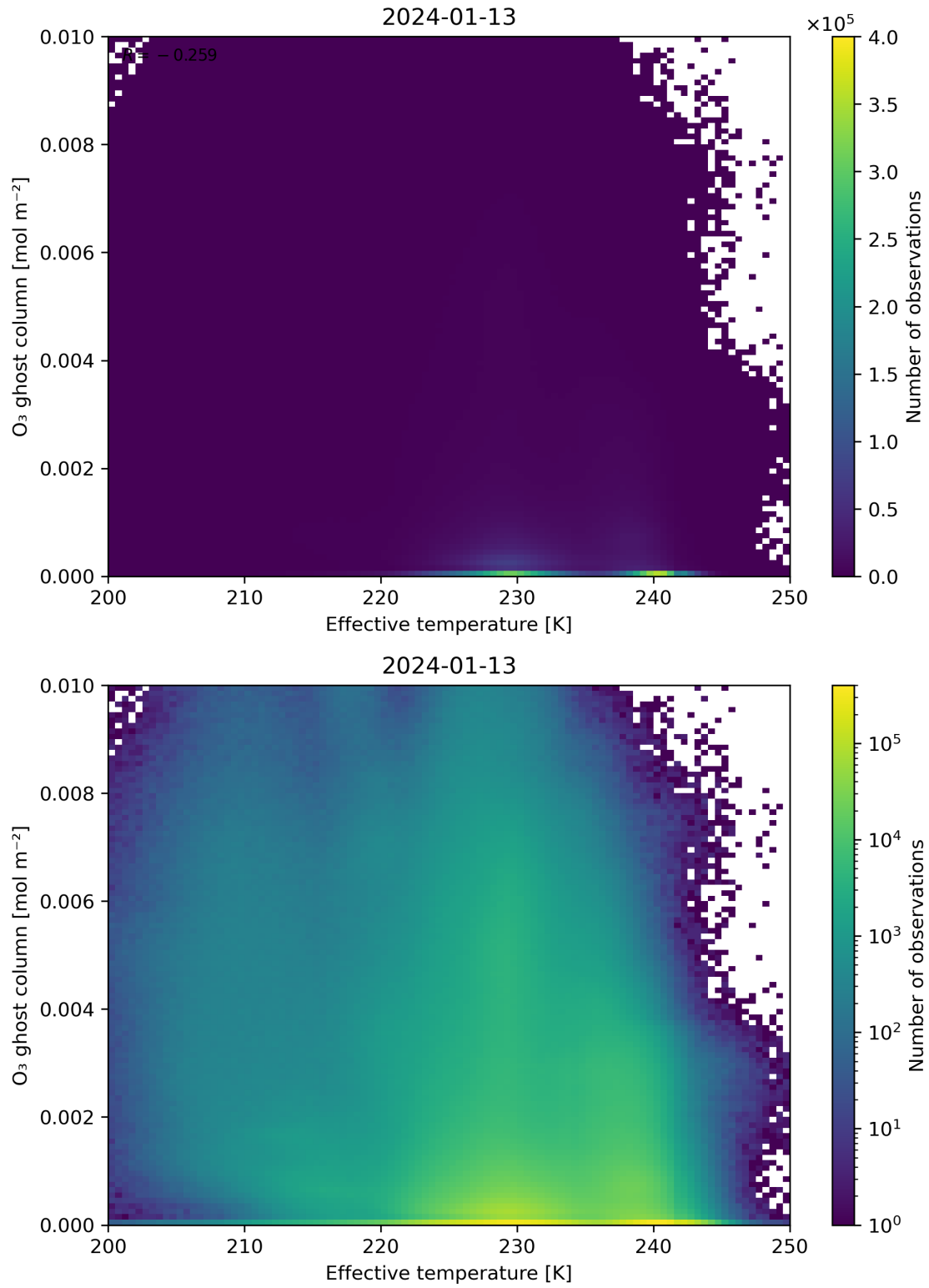
Figure 38: Scatter density plot of “Effective temperature” against “O 3 ghost column” for 2024-01-12 to 2024-01-14.
