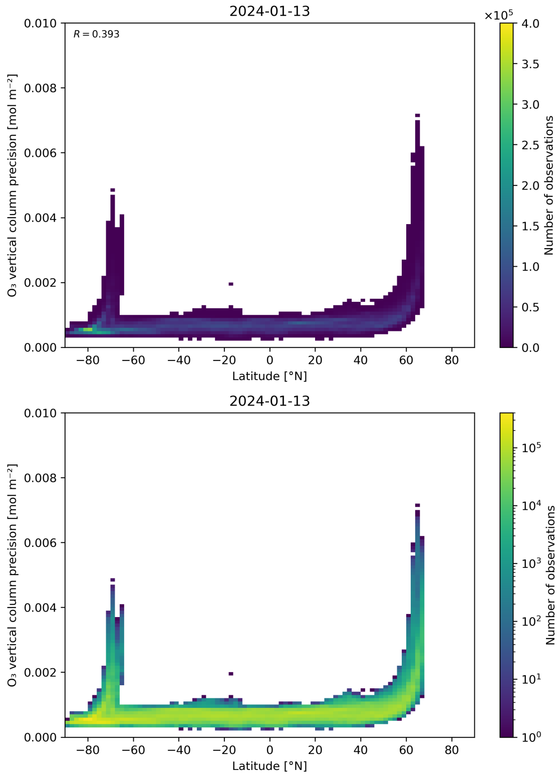
Figure 37: Scatter density plot of “Latitude” against “O 3 vertical column precision” for 2024-01-12 to 2024-01-14.
