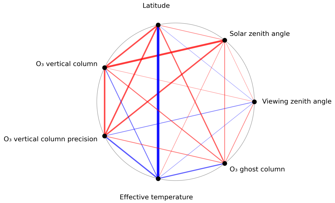
Figure 1: Map of correlation graph for 2024-01-12 to 2024-01-14.
