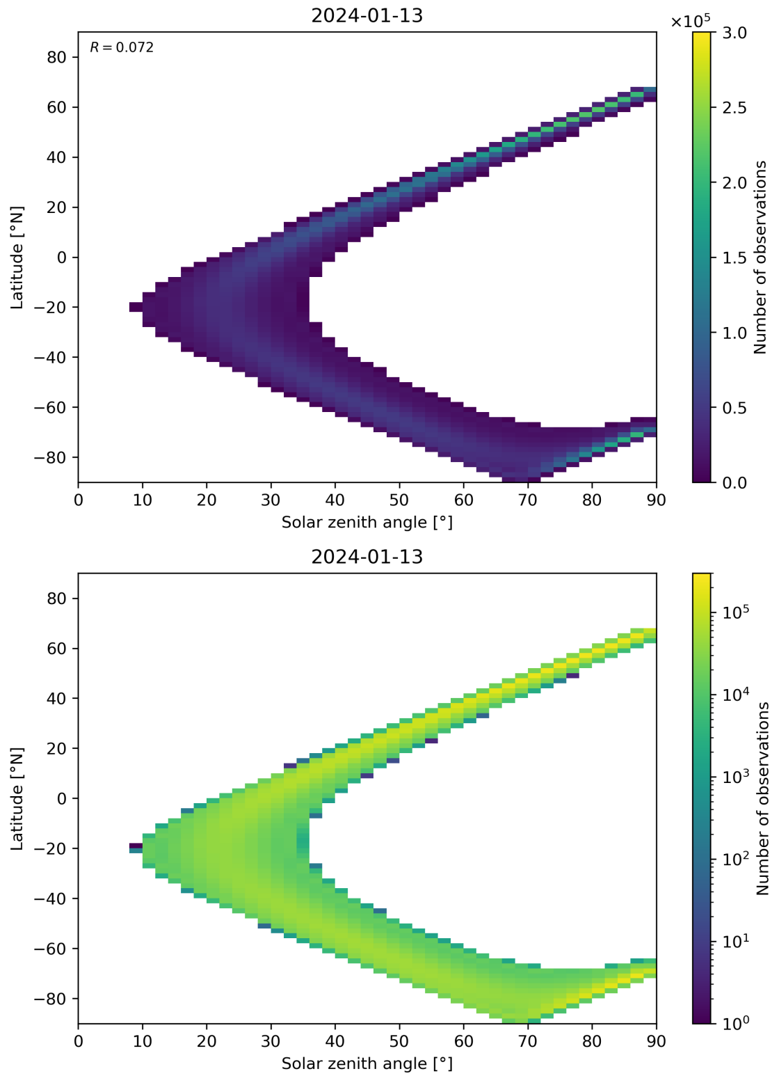
Figure 44: Scatter density plot of “Solar zenith angle” against “Latitude” for 2024-01-12 to 2024-01-14.
