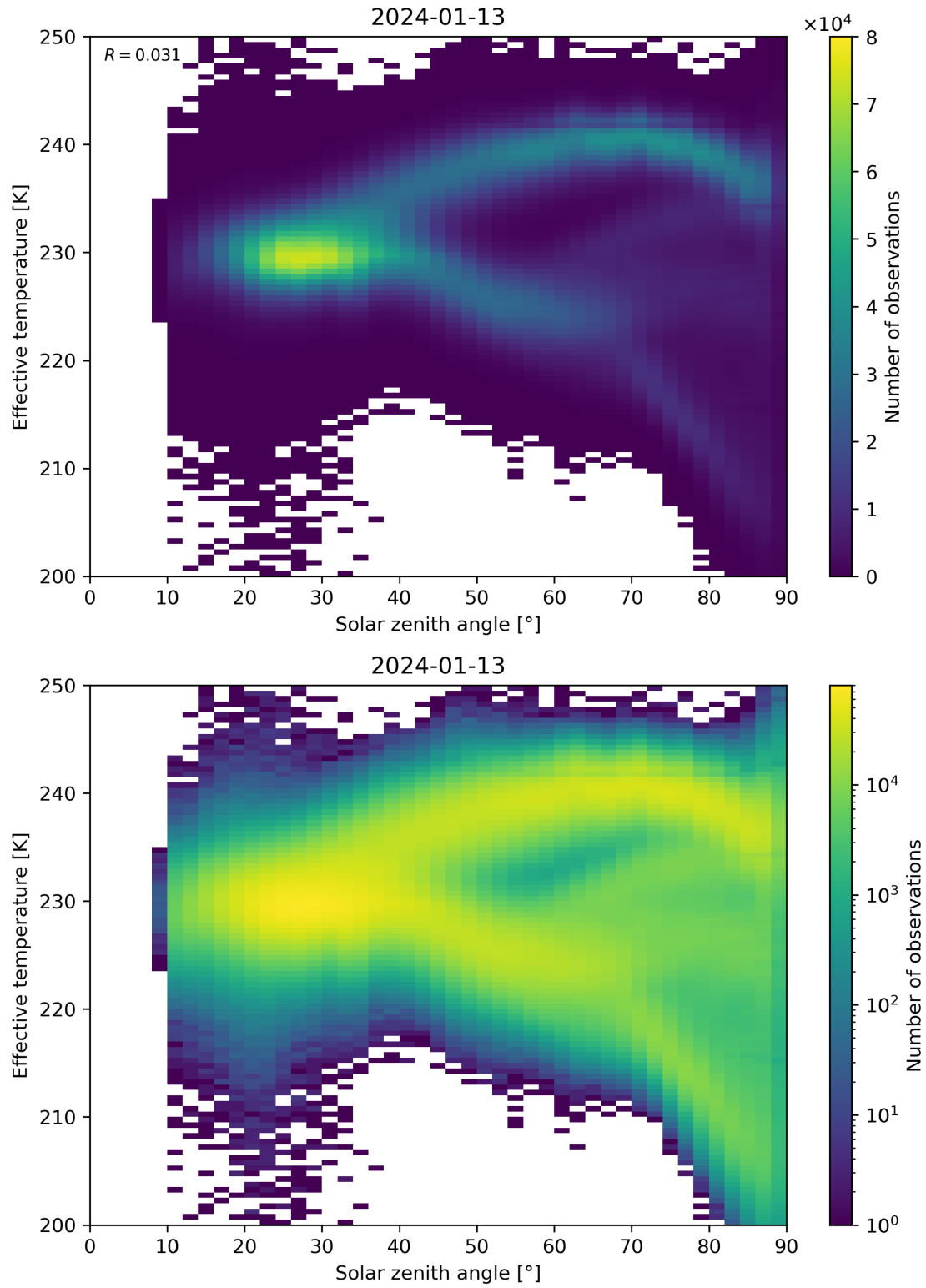
Figure 45: Scatter density plot of “Solar zenith angle” against “Effective temperature” for 2024-01-12 to 2024-01-14.
