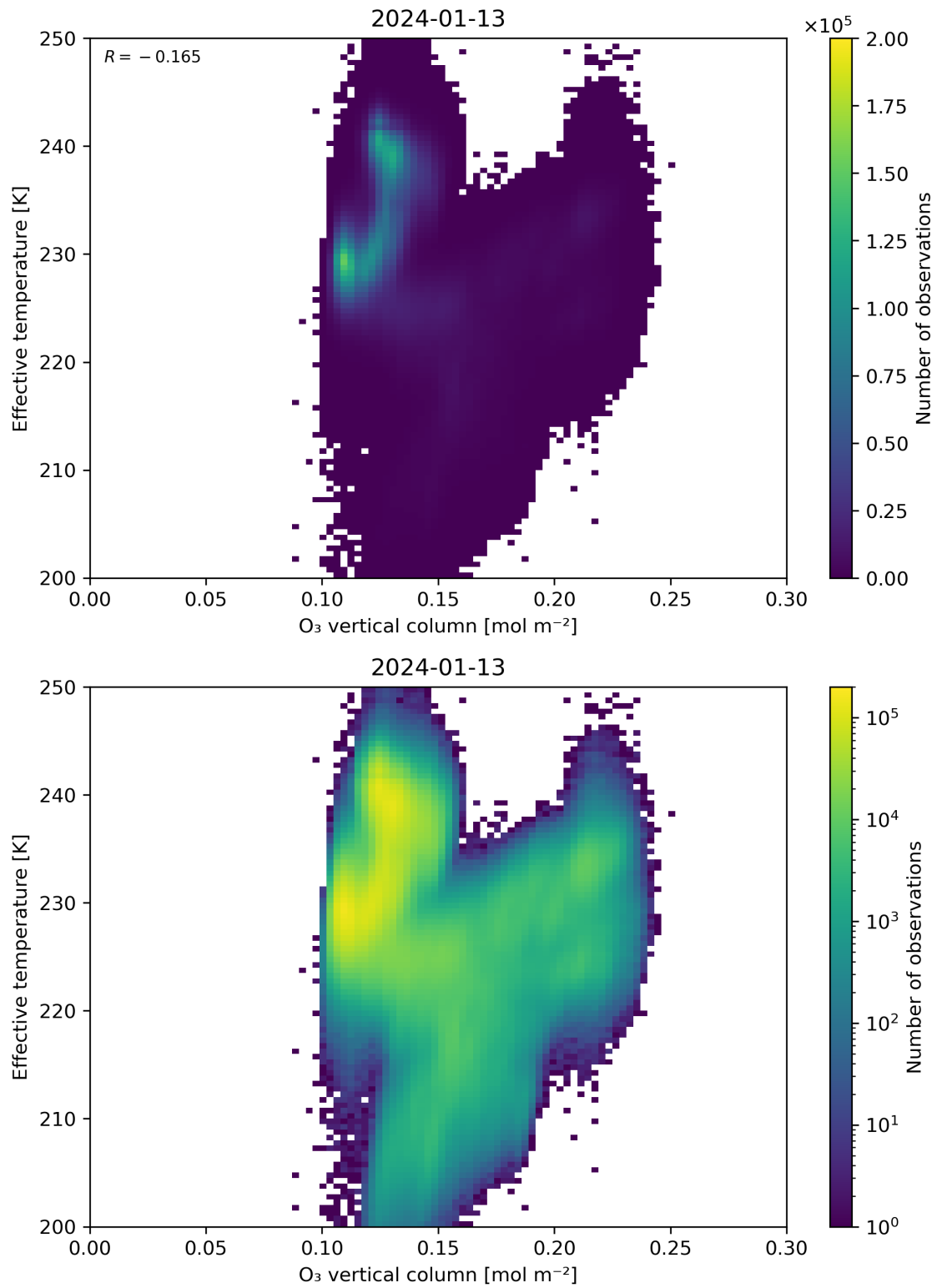
Figure 39: Scatter density plot of “O 3 vertical column” against “Effective temperature” for 2024-01-12 to 2024-01-14.
