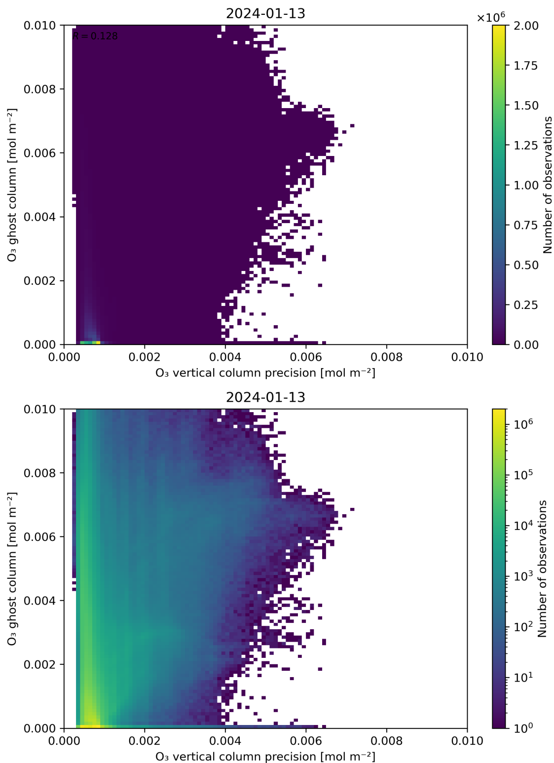
Figure 43: Scatter density plot of “O 3 vertical column precision” against “O 3 ghost column” for 2024-01-12 to 2024-01-14.
