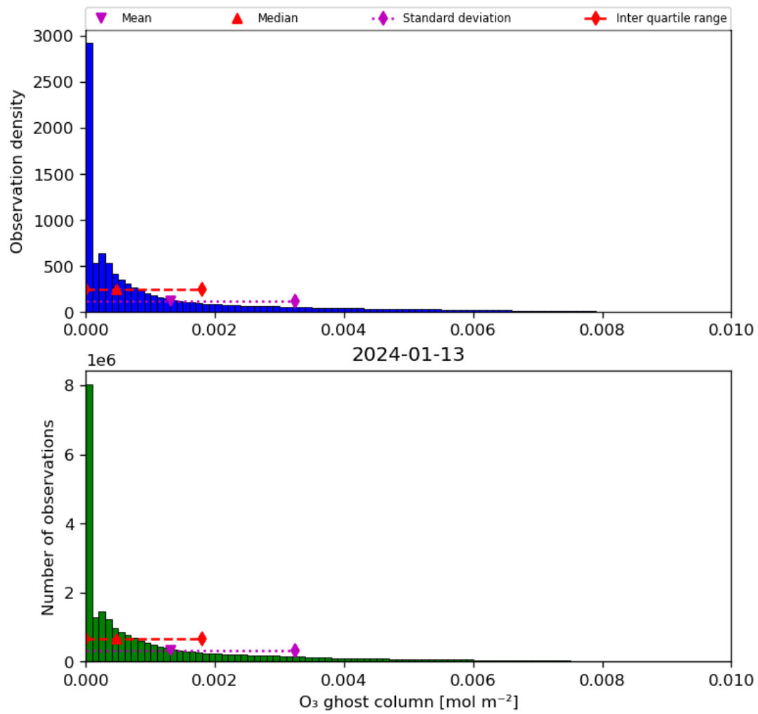
Figure 25: Histogram of “O 3 ghost column” for 2024-01-12 to 2024-01-14
