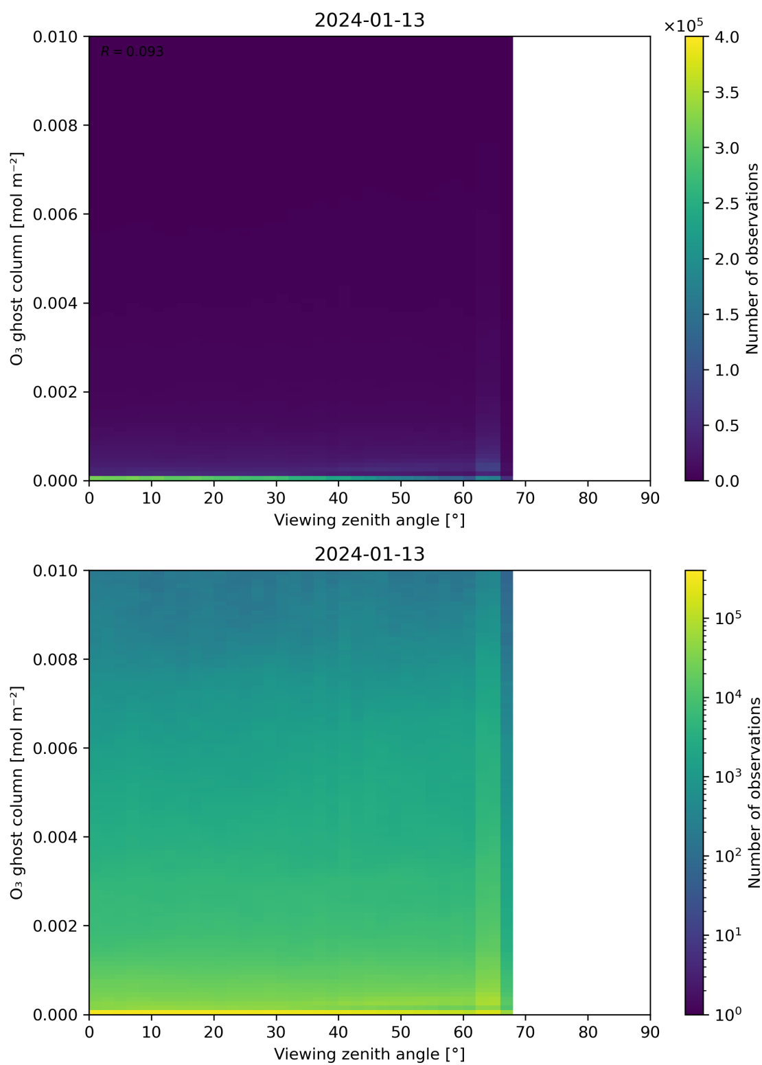
Figure 51: Scatter density plot of “Viewing zenith angle” against “O 3 ghost column” for 2024-01-12 to 2024-01-14.
