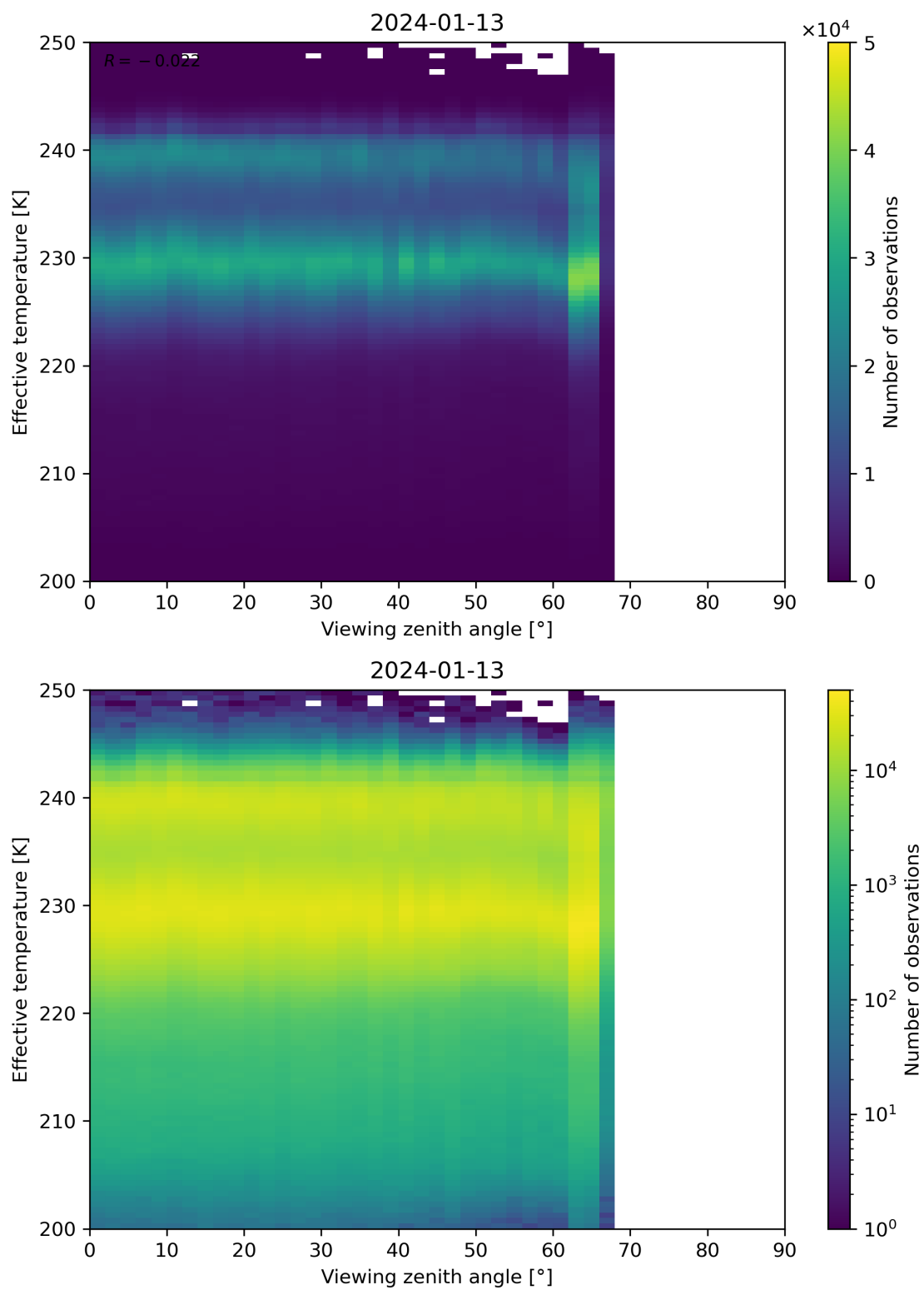
Figure 50: Scatter density plot of “Viewing zenith angle” against “Effective temperature” for 2024-01-12 to 2024-01-14.
