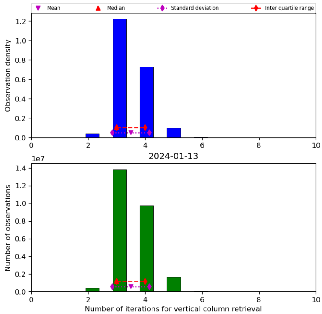
Figure 26: Histogram of “Number of iterations for vertical column retrieval” for 2024-01-12 to 2024-01-14
