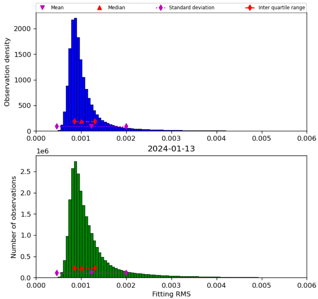
Figure 23: Histogram of “Fitting RMS” for 2024-01-12 to 2024-01-14
