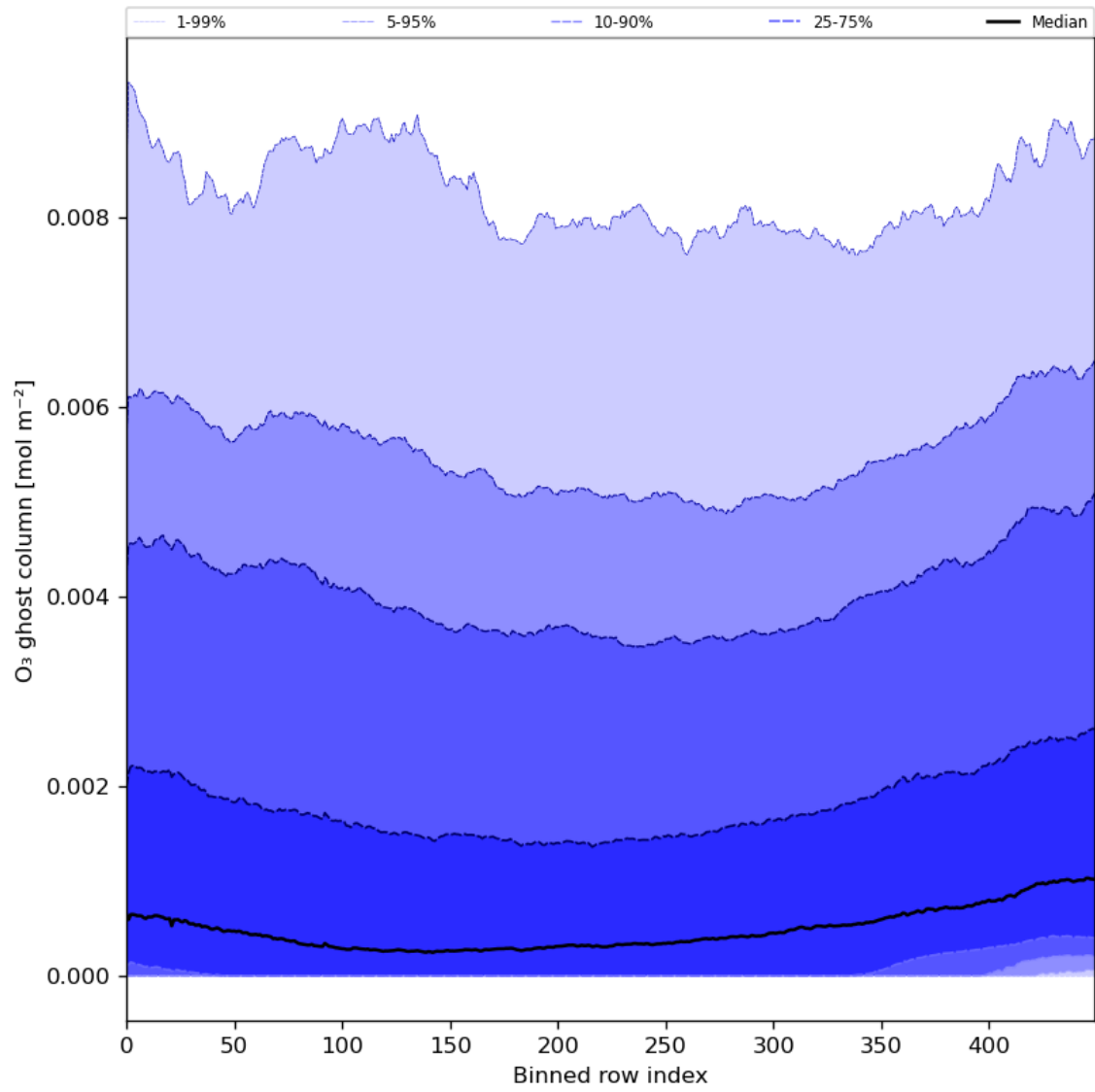
Figure 32: Along track statistics of “O 3 ghost column” for 2024-01-12 to 2024-01-14
