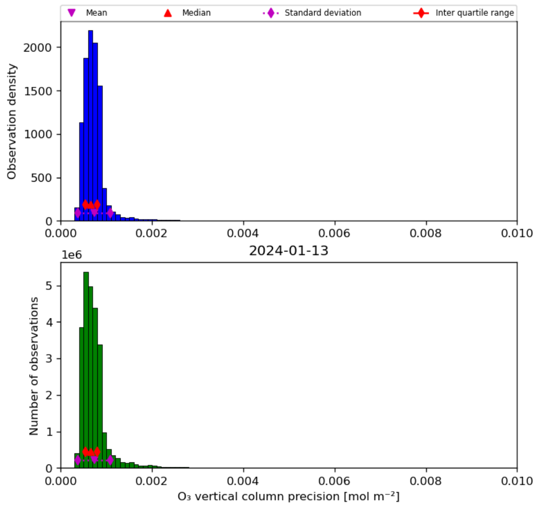
Figure 22: Histogram of “O 3 vertical column precision” for 2024-01-12 to 2024-01-14
