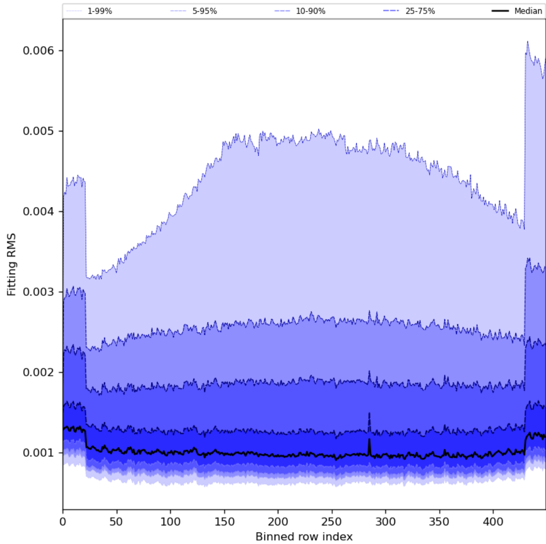
Figure 30: Along track statistics of “Fitting RMS” for 2024-01-12 to 2024-01-14
