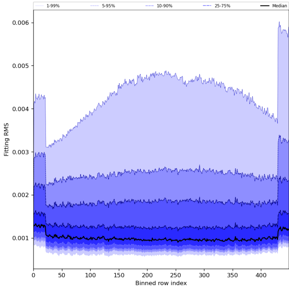
Figure 30: Along track statistics of “Fitting RMS” for 2024-01-15 to 2024-01-16
