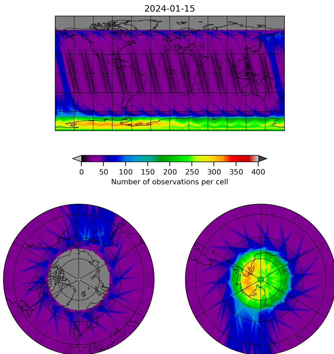
Figure 12: Map of the number of observations for 2024-01-15 to 2024-01-16
