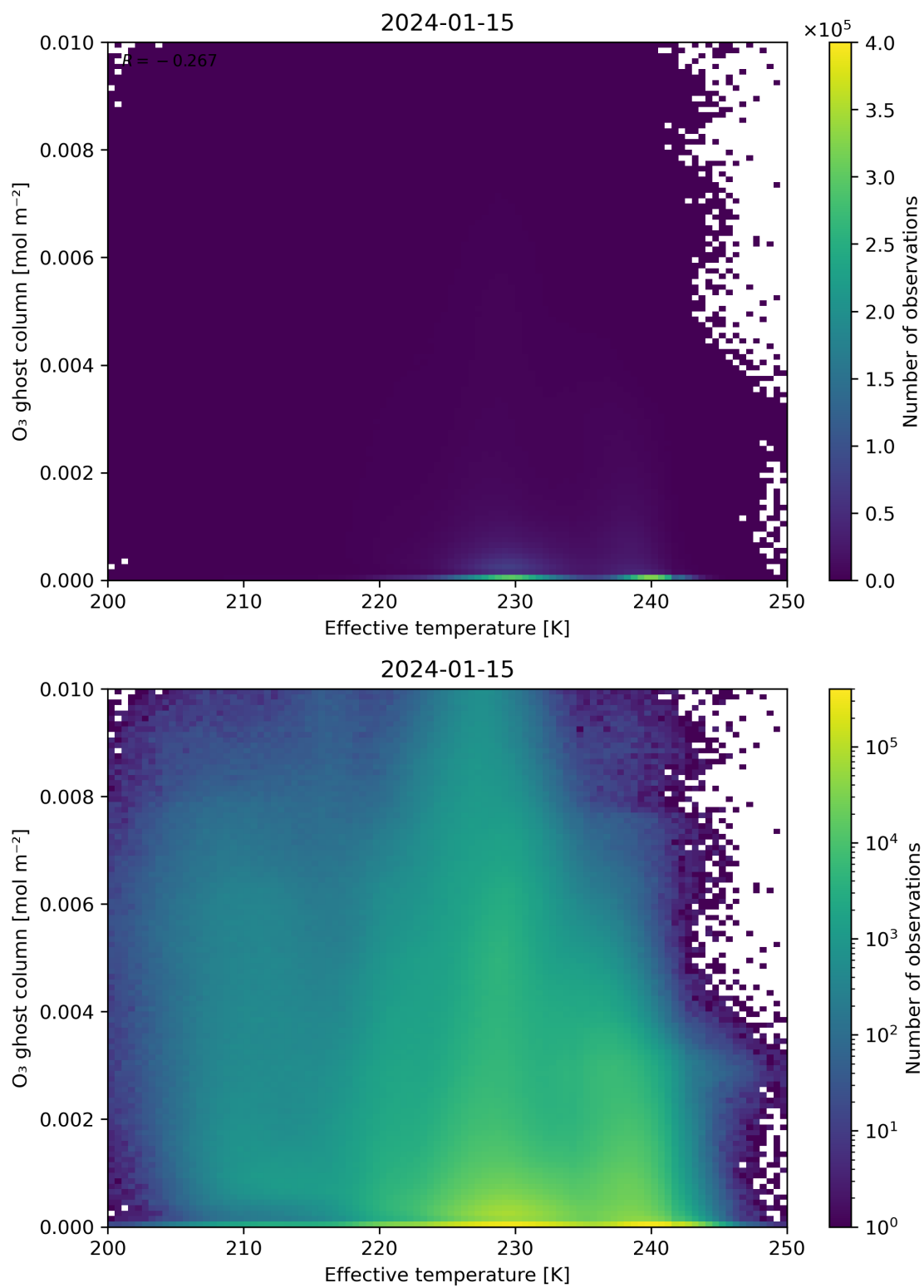
Figure 38: Scatter density plot of “Effective temperature” against “O 3 ghost column” for 2024-01-15 to 2024-01-16.
