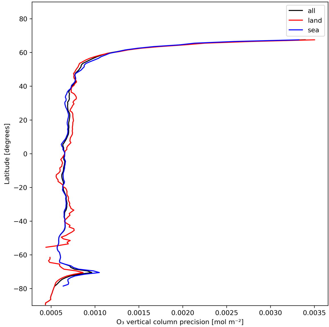
Figure 15: Zonal average of “O 3 vertical column precision” for 2024-01-15 to 2024-01-16.
