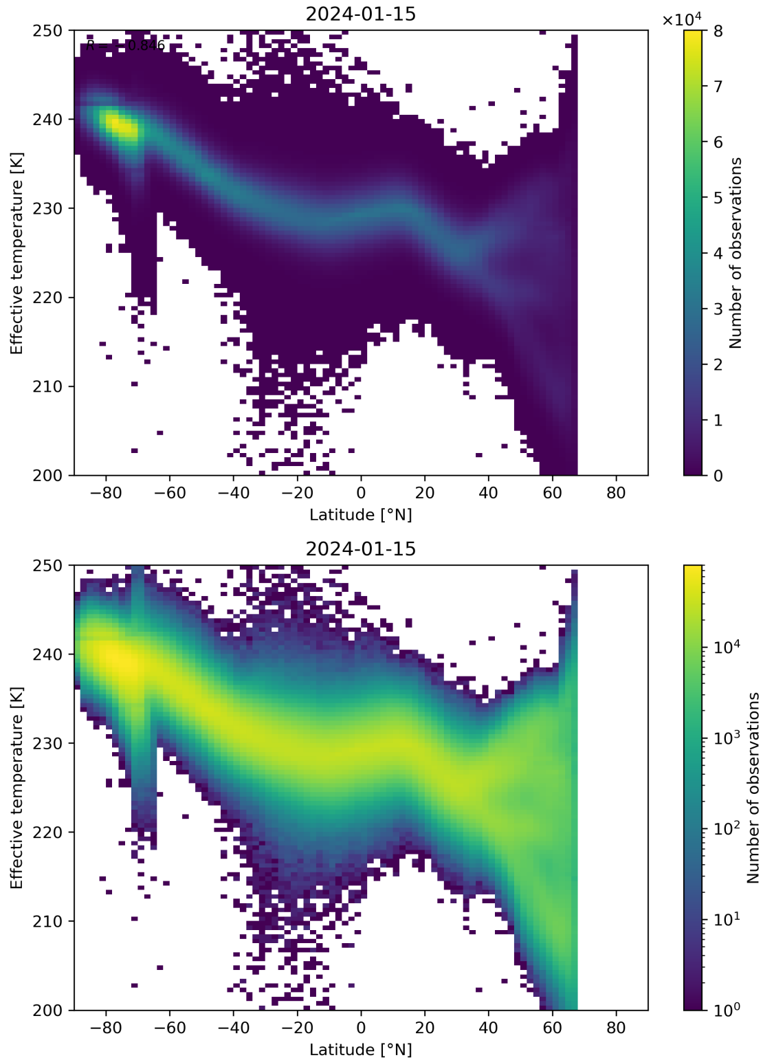
Figure 34: Scatter density plot of “Latitude” against “Effective temperature” for 2024-01-15 to 2024-01-16.
