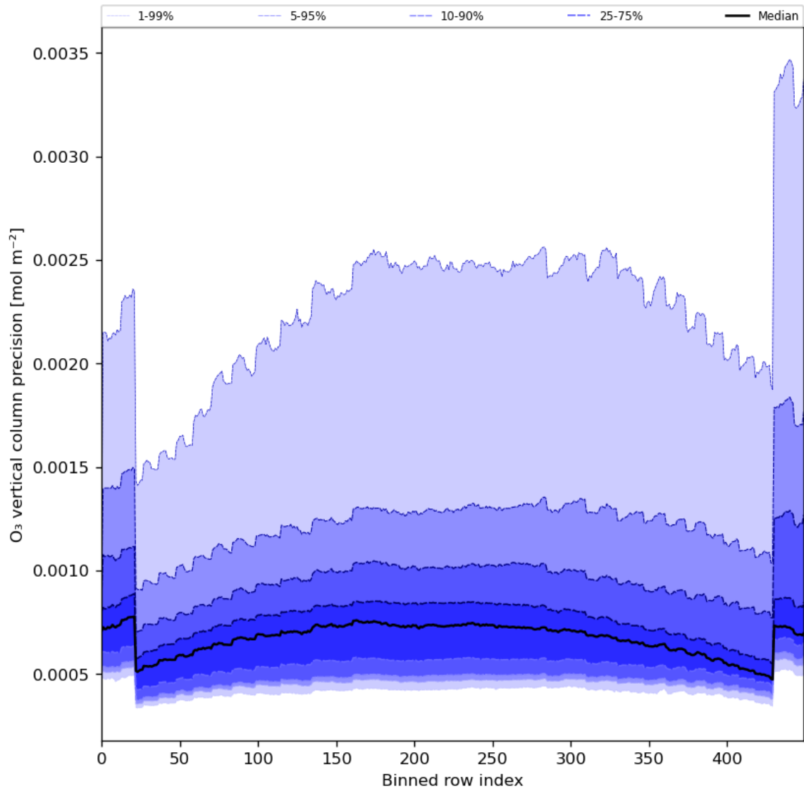
Figure 29: Along track statistics of “O 3 vertical column precision” for 2024-01-15 to 2024-01-16
