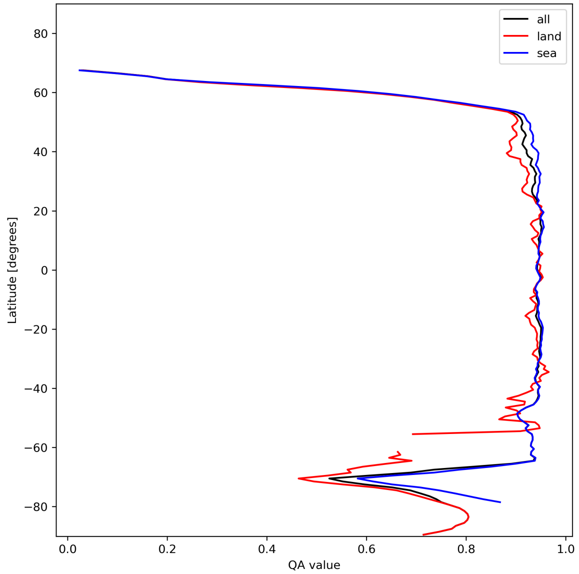
Figure 13: Zonal average of “QA value” for 2024-01-15 to 2024-01-16.
