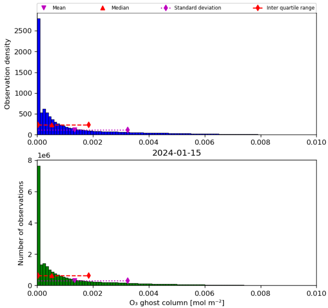
Figure 25: Histogram of “O 3 ghost column” for 2024-01-15 to 2024-01-16
