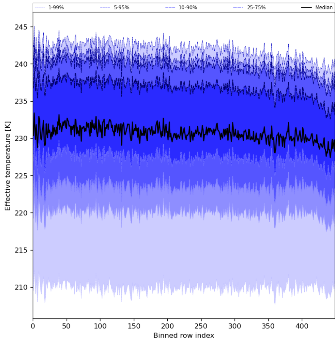
Figure 31: Along track statistics of “Effective temperature” for 2024-01-15 to 2024-01-16
