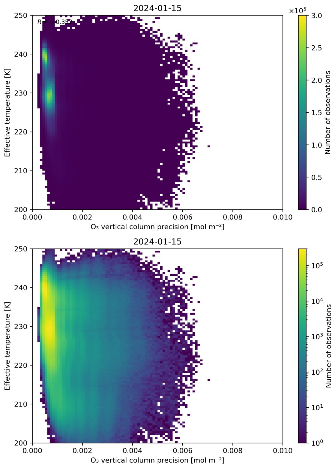
Figure 42: Scatter density plot of “O 3 vertical column precision” against “Effective temperature” for 2024-01-15 to 2024-01-16.
