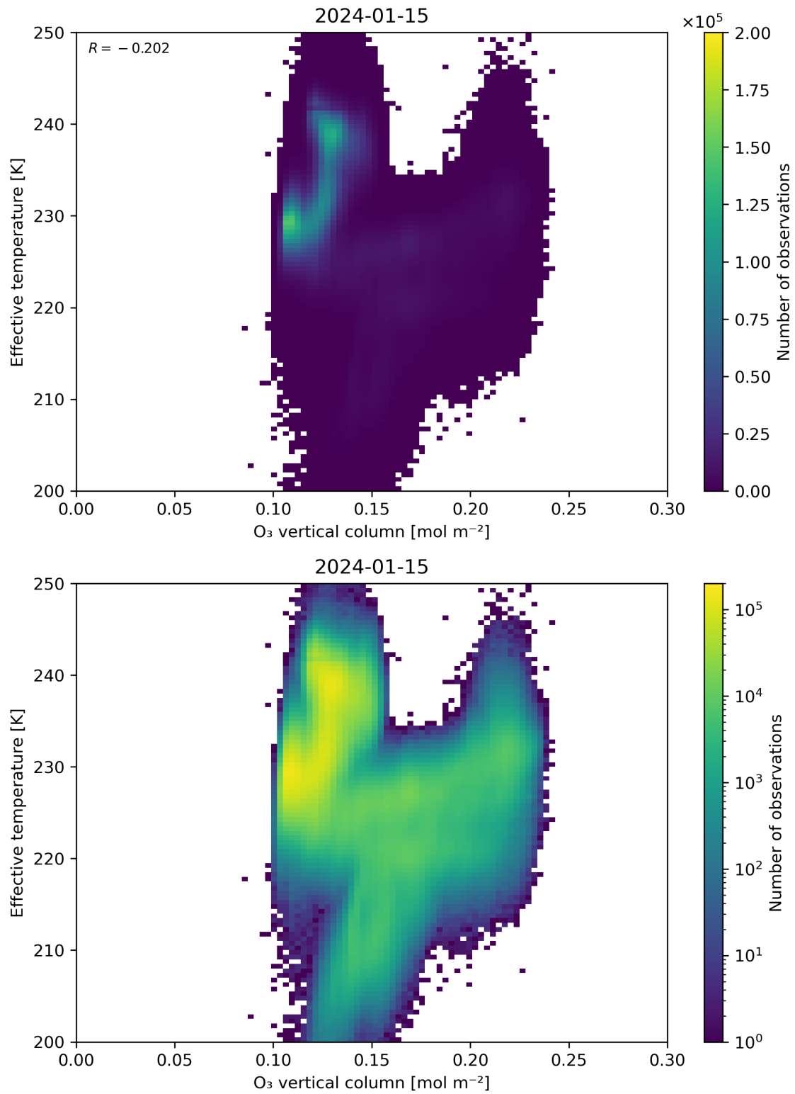
Figure 39: Scatter density plot of “O 3 vertical column” against “Effective temperature” for 2024-01-15 to 2024-01-16.
