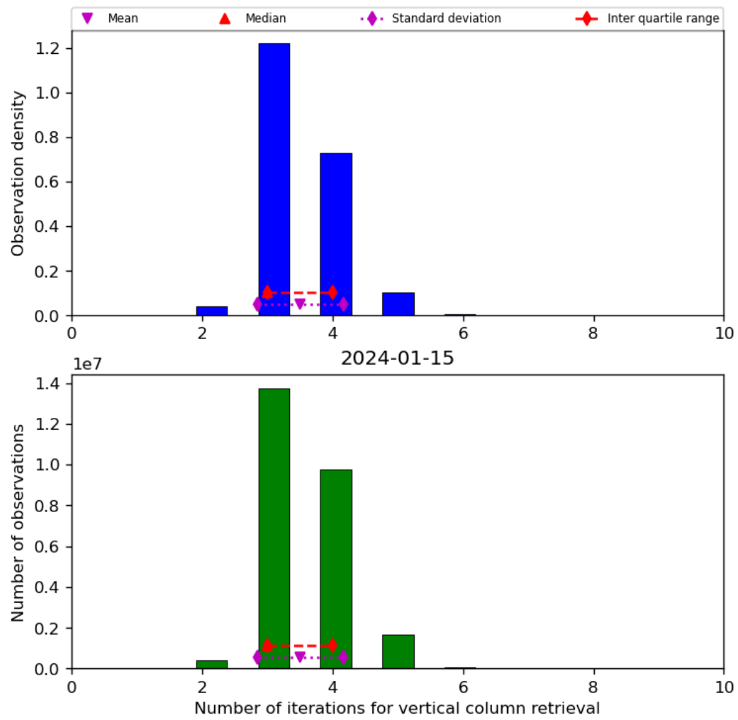
Figure 26: Histogram of “Number of iterations for vertical column retrieval” for 2024-01-15 to 2024-01-16
