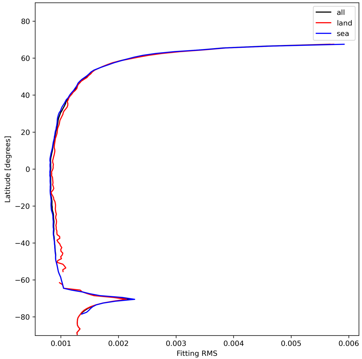
Figure 16: Zonal average of “Fitting RMS” for 2024-01-15 to 2024-01-16.
