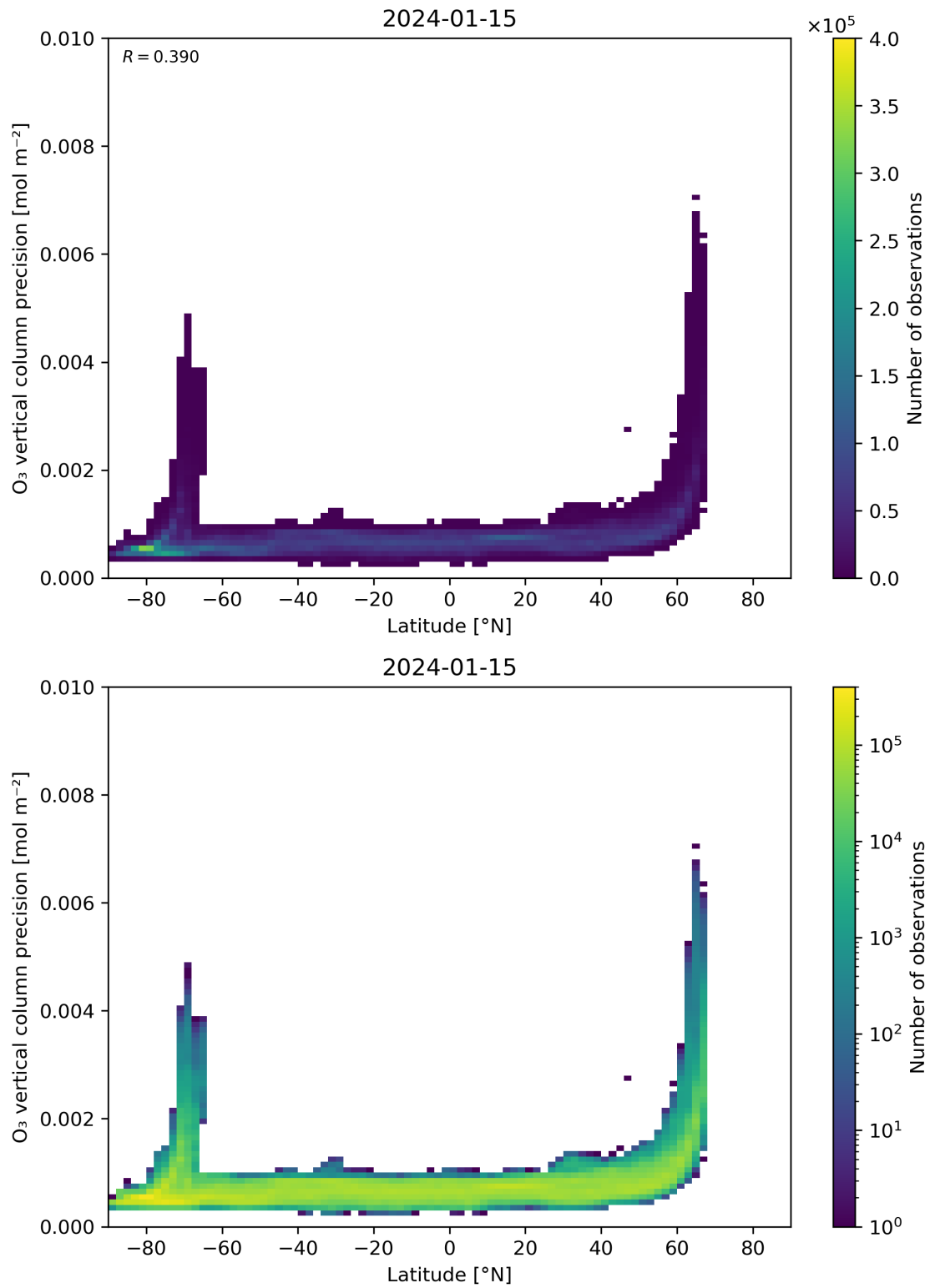
Figure 37: Scatter density plot of “Latitude” against “O 3 vertical column precision” for 2024-01-15 to 2024-01-16.
