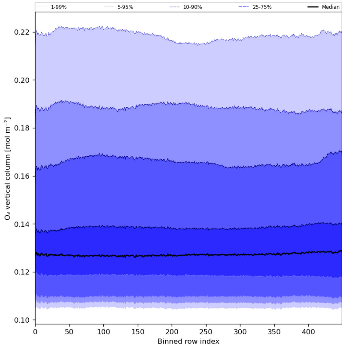
Figure 28: Along track statistics of “O 3 vertical column” for 2024-01-15 to 2024-01-16
