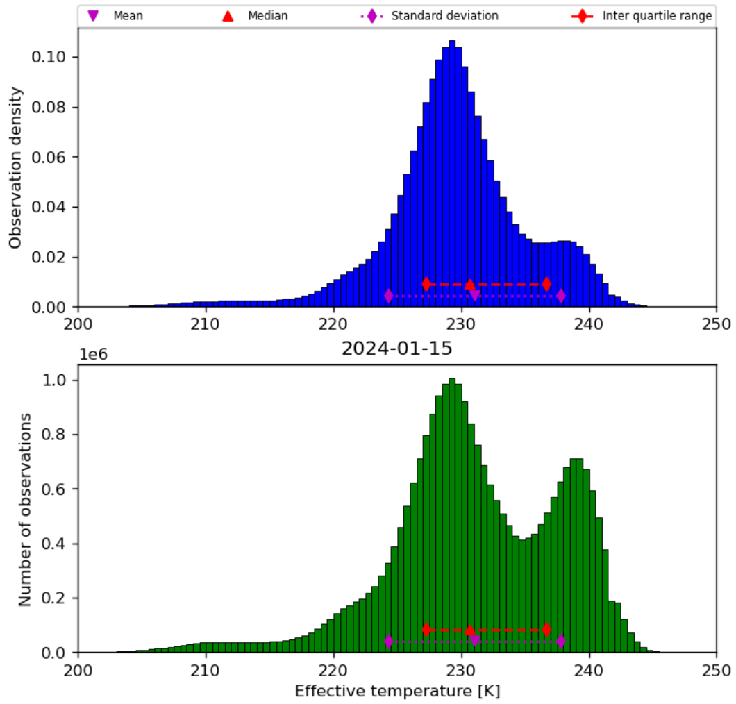
Figure 24: Histogram of “Effective temperature” for 2024-01-15 to 2024-01-16
