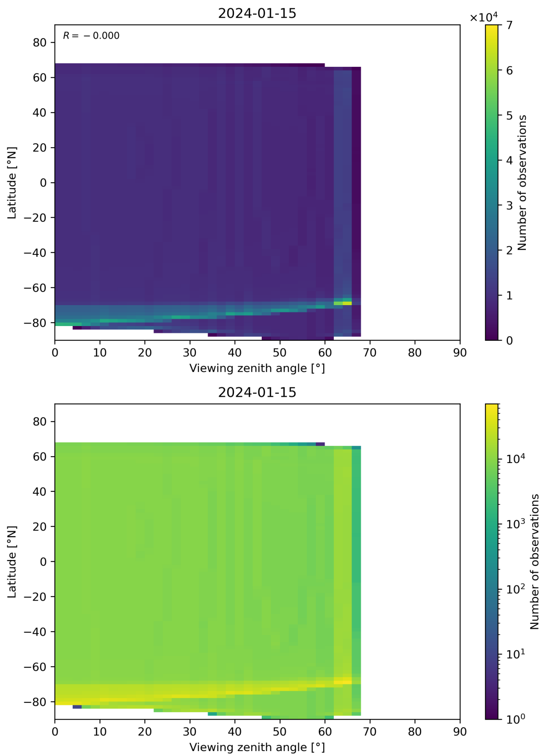
Figure 49: Scatter density plot of “Viewing zenith angle” against “Latitude” for 2024-01-15 to 2024-01-16.
