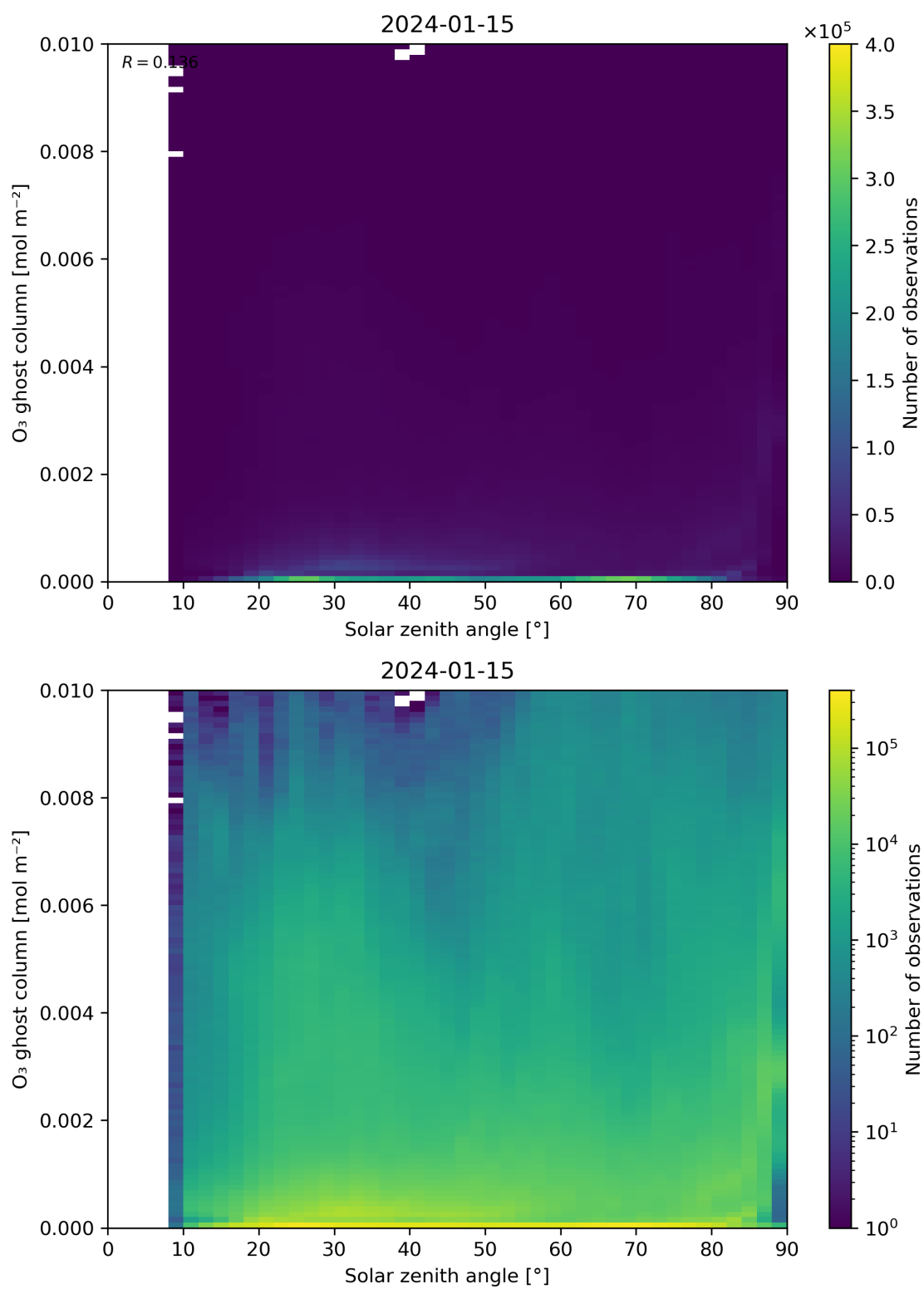
Figure 46: Scatter density plot of “Solar zenith angle” against “O 3 ghost column” for 2024-01-15 to 2024-01-16.
