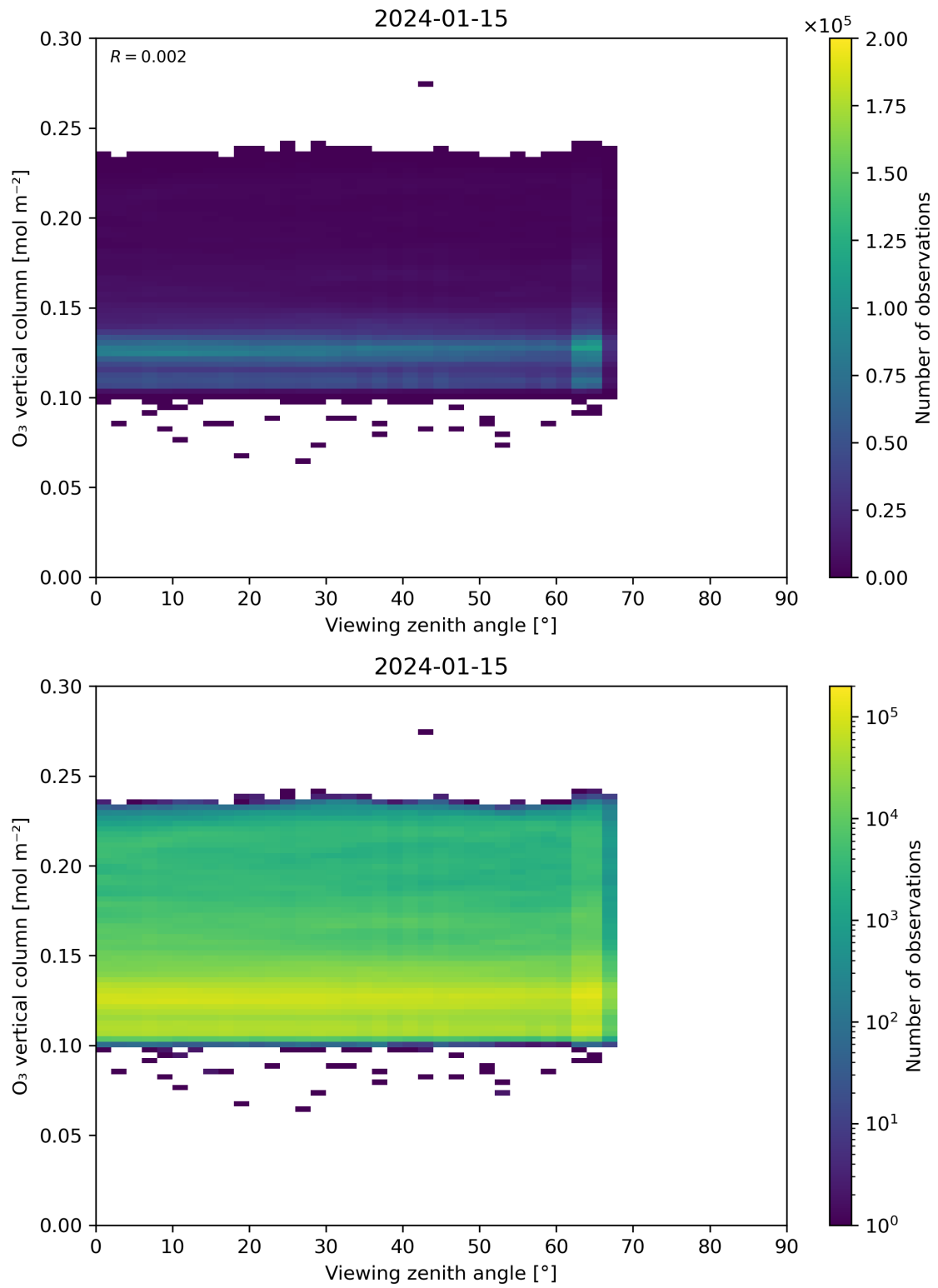
Figure 52: Scatter density plot of “Viewing zenith angle” against “O 3 vertical column” for 2024-01-15 to 2024-01-16.
