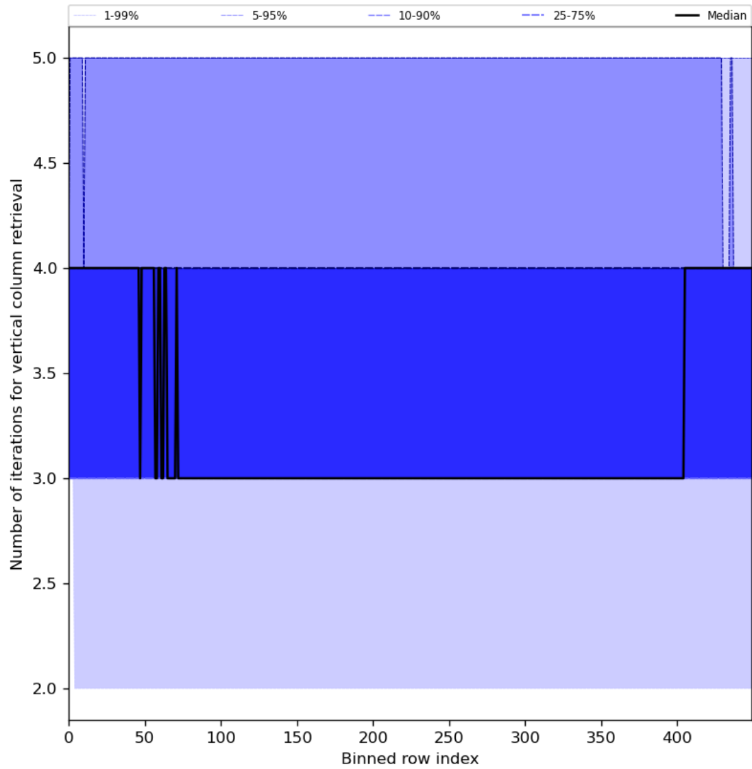
Figure 33: Along track statistics of “Number of iterations for vertical column retrieval” for 2024-01-15 to 2024-01-16
