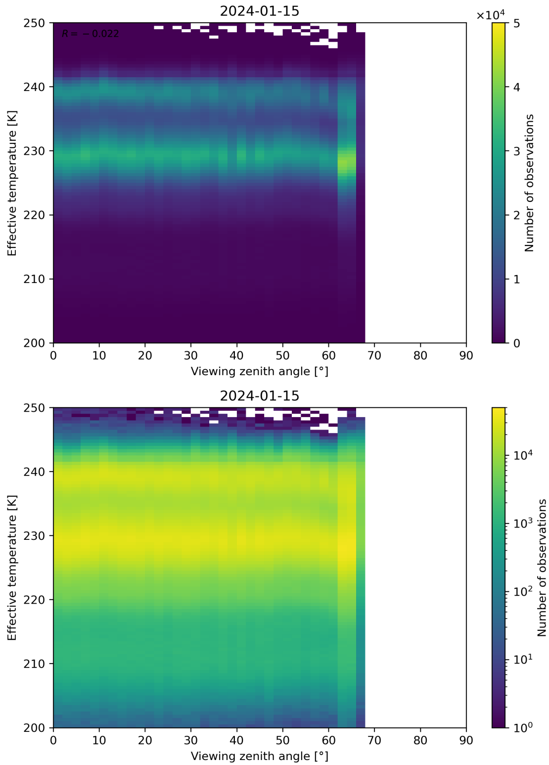
Figure 50: Scatter density plot of “Viewing zenith angle” against “Effective temperature” for 2024-01-15 to 2024-01-16.
