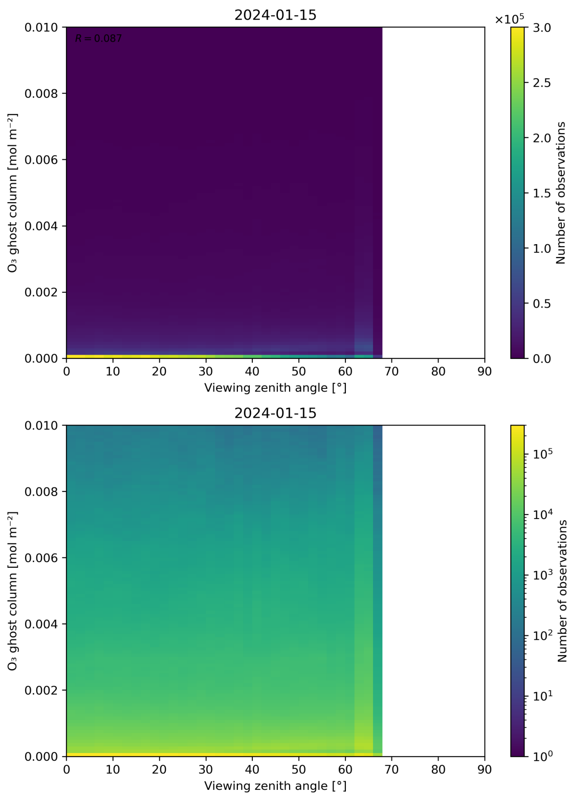
Figure 51: Scatter density plot of “Viewing zenith angle” against “O 3 ghost column” for 2024-01-15 to 2024-01-16.
