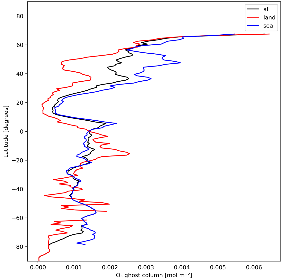
Figure 18: Zonal average of “O 3 ghost column” for 2024-01-15 to 2024-01-16.
