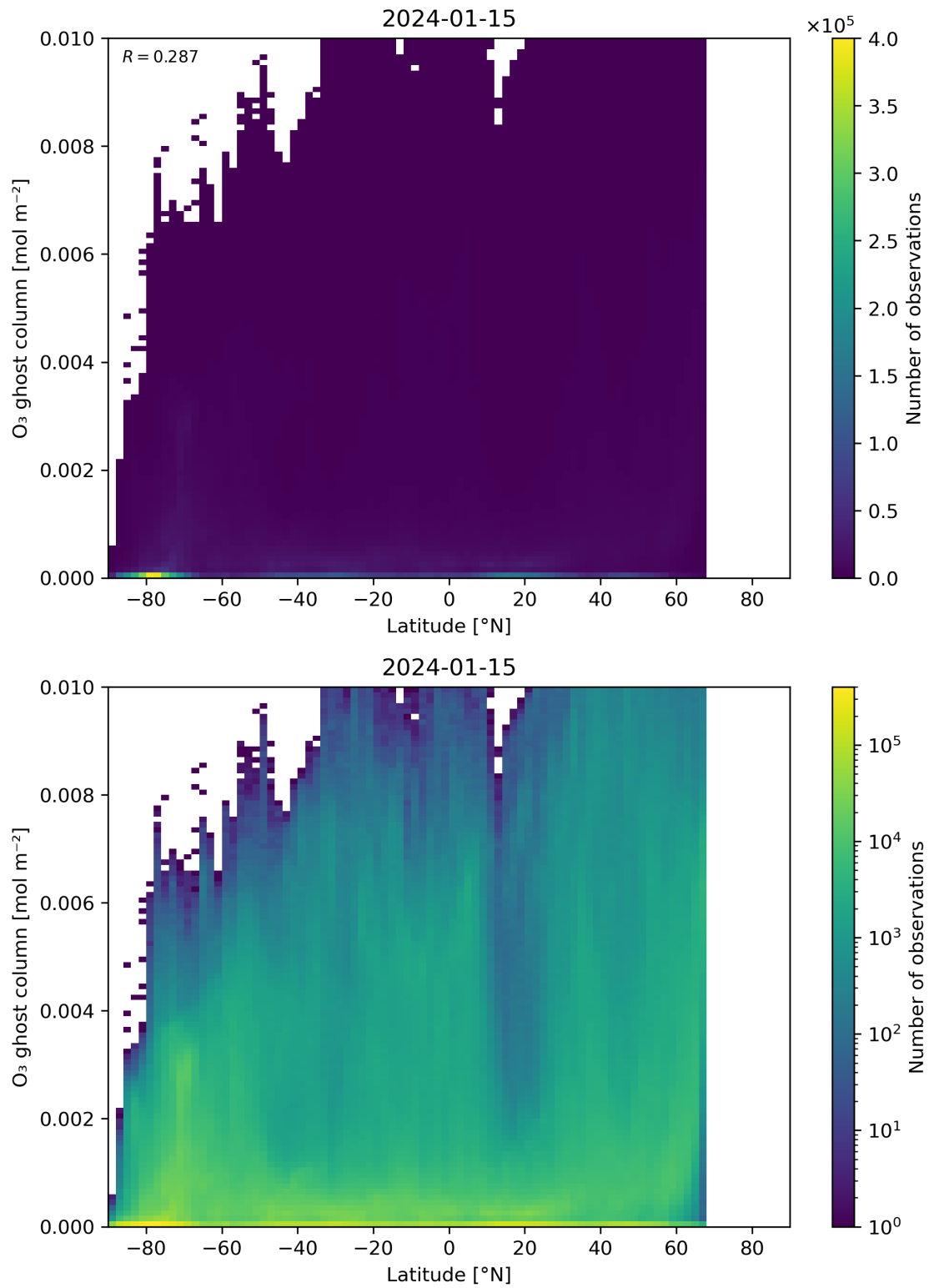
Figure 35: Scatter density plot of “Latitude” against “O 3 ghost column” for 2024-01-15 to 2024-01-16.
