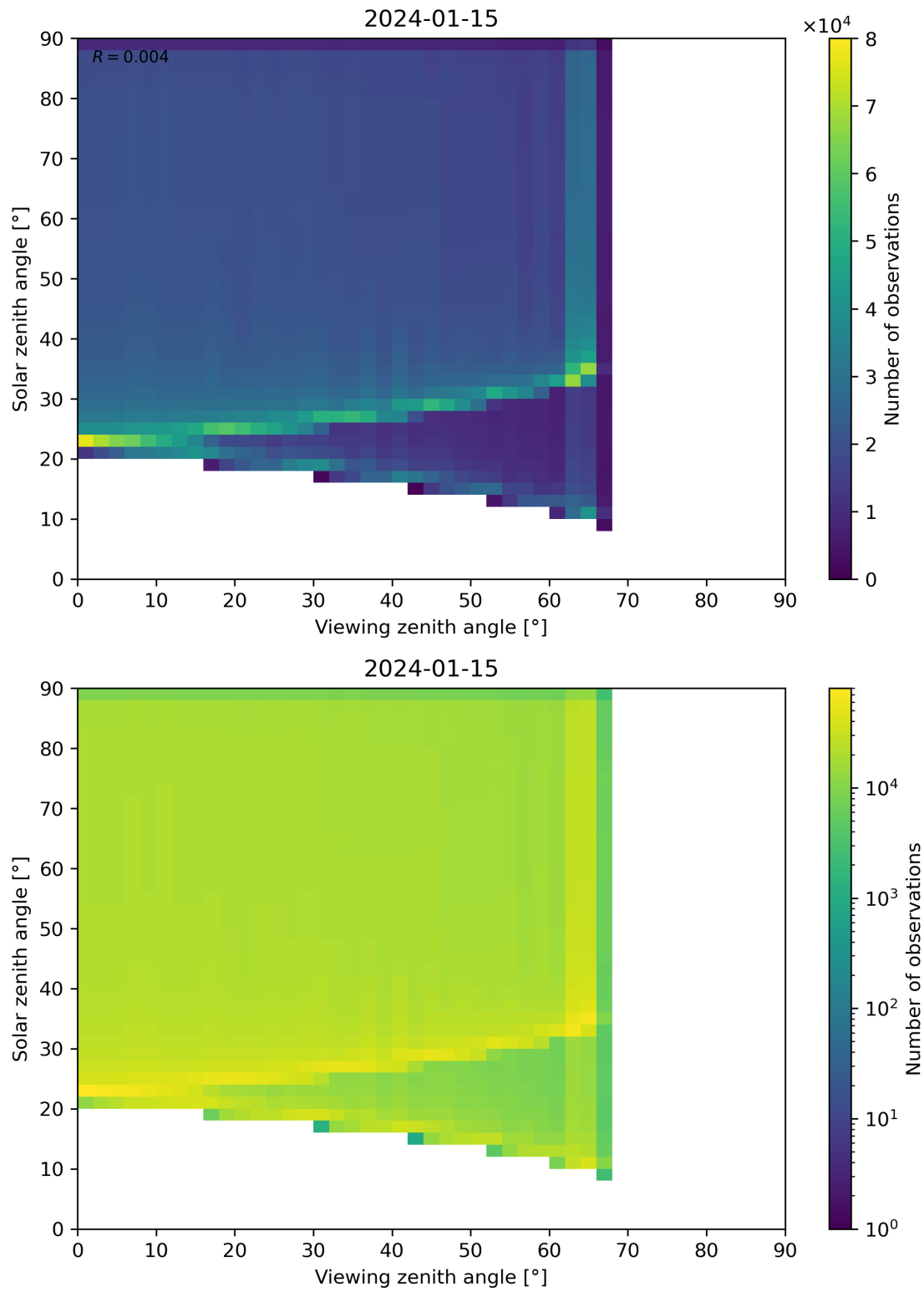
Figure 54: Scatter density plot of “Viewing zenith angle” against “Solar zenith angle” for 2024-01-15 to 2024-01-16.
