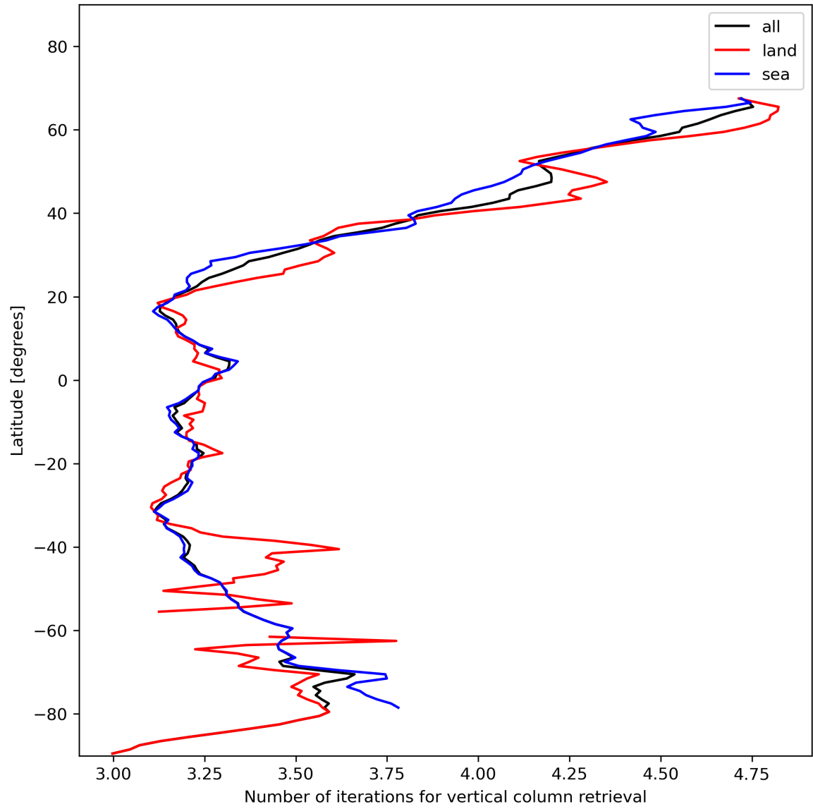
Figure 19: Zonal average of “Number of iterations for vertical column retrieval” for 2024-01-15 to 2024-01-16.
