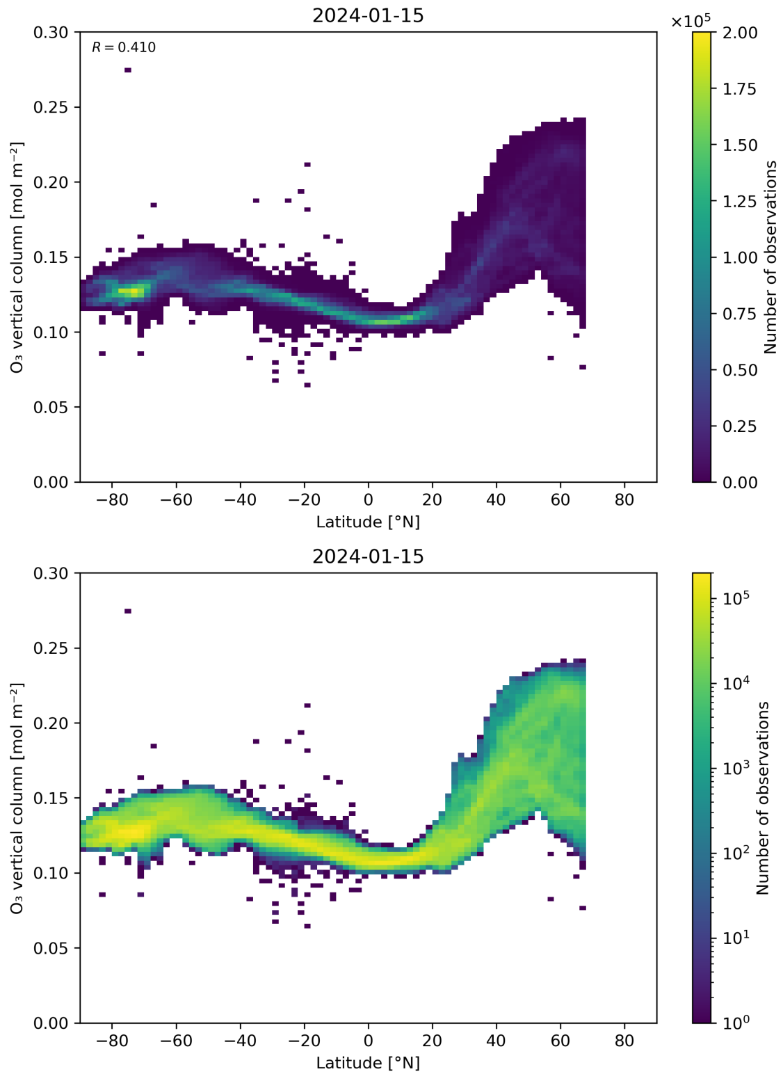
Figure 36: Scatter density plot of “Latitude” against “O 3 vertical column” for 2024-01-15 to 2024-01-16.
