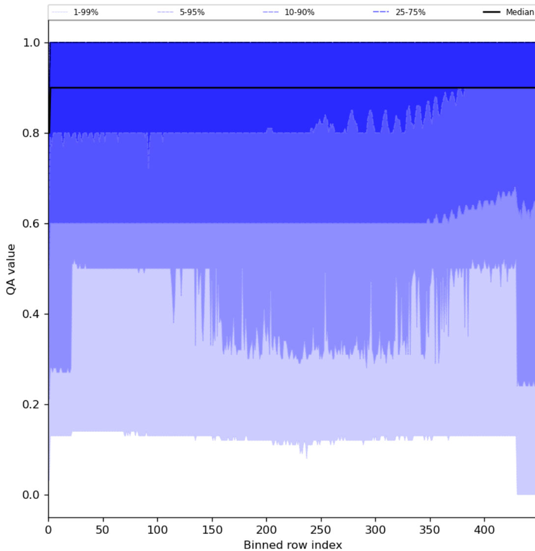
Figure 27: Along track statistics of “QA value” for 2024-01-15 to 2024-01-16
