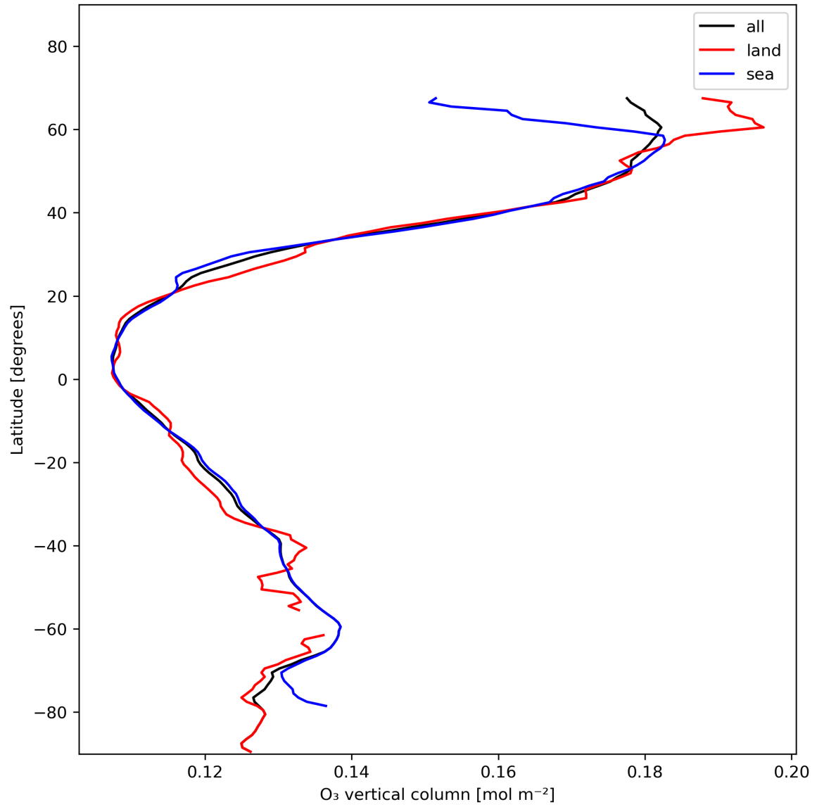
Figure 14: Zonal average of “O 3 vertical column” for 2024-01-15 to 2024-01-16.
