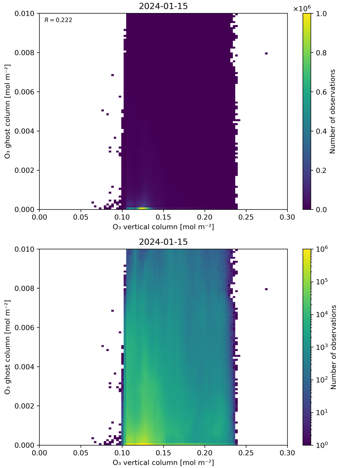
Figure 40: Scatter density plot of “O 3 vertical column” against “O 3 ghost column” for 2024-01-15 to 2024-01-16.
