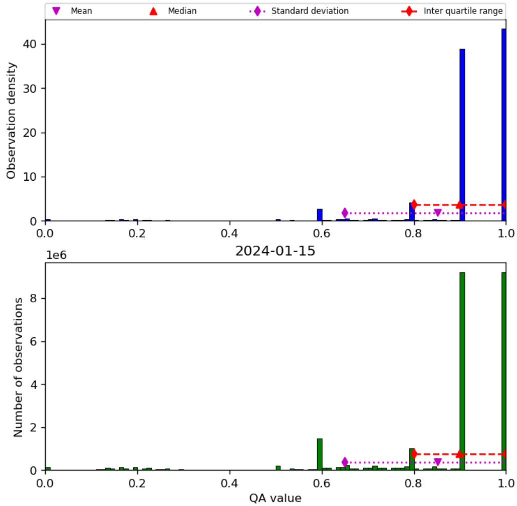
Figure 20: Histogram of “QA value” for 2024-01-15 to 2024-01-16
