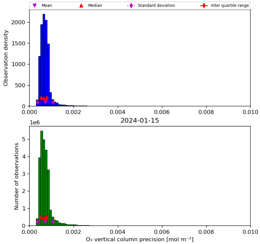
Figure 22: Histogram of “O 3 vertical column precision” for 2024-01-15 to 2024-01-16
