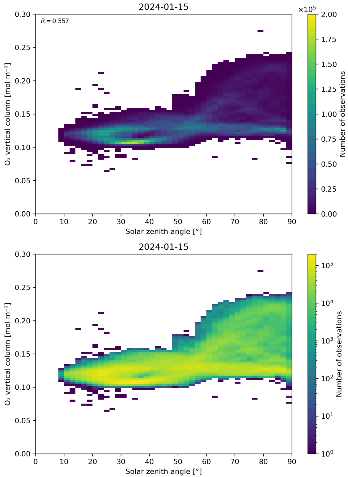
Figure 47: Scatter density plot of “Solar zenith angle” against “O 3 vertical column” for 2024-01-15 to 2024-01-16.
