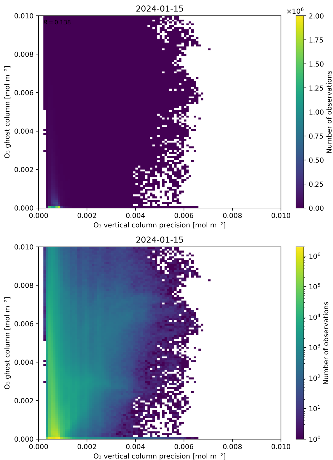
Figure 43: Scatter density plot of “ \text{O}_3 vertical column precision” against “ \text{O}_3 ghost column” for 2024-01-15 to 2024-01-16.
