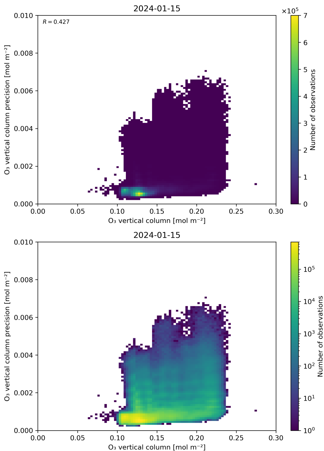
Figure 41: Scatter density plot of “O 3 vertical column” against “O 3 vertical column precision” for 2024-01-15 to 2024-01-16.
