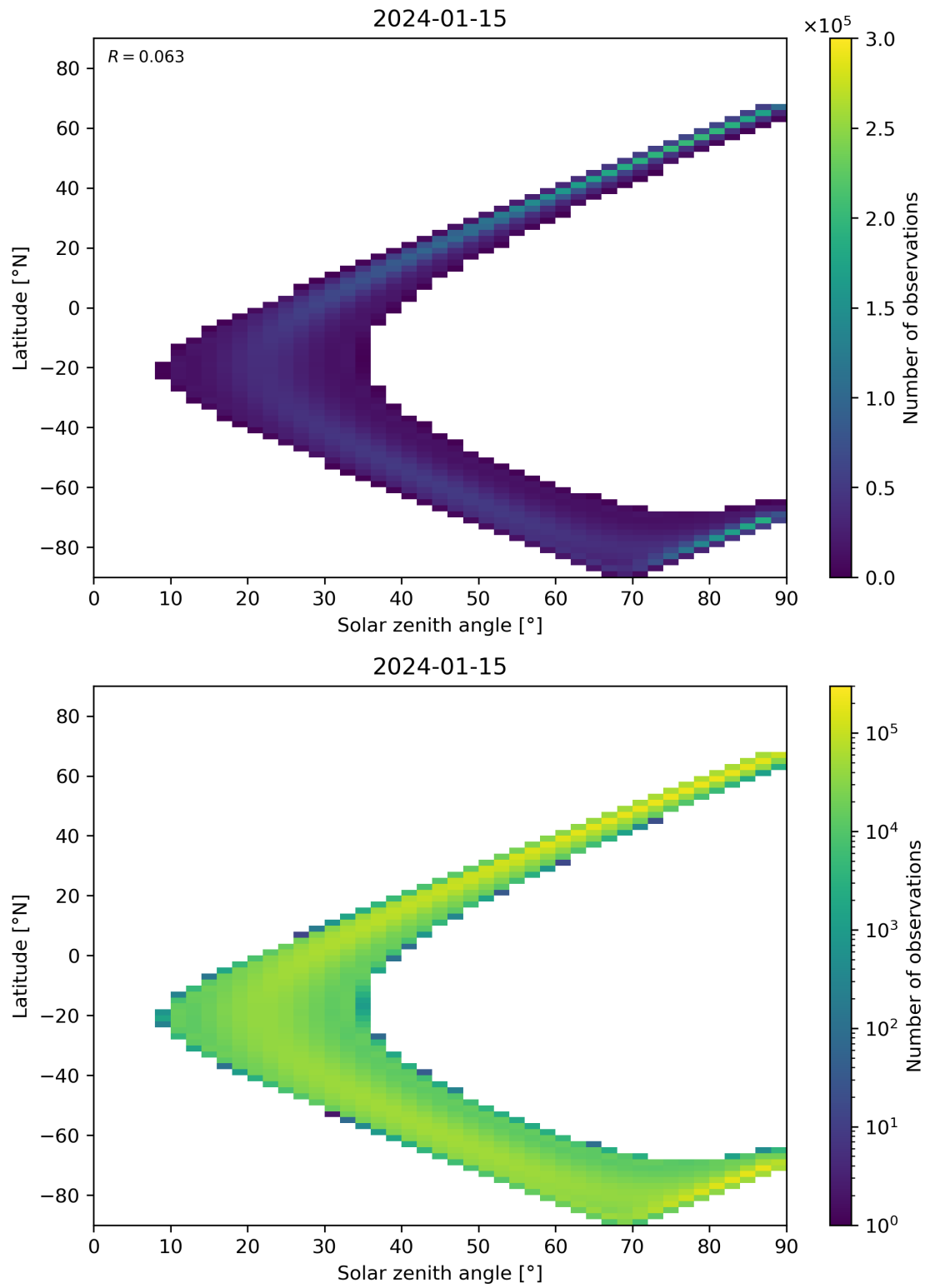
Figure 44: Scatter density plot of “Solar zenith angle” against “Latitude” for 2024-01-15 to 2024-01-16.
