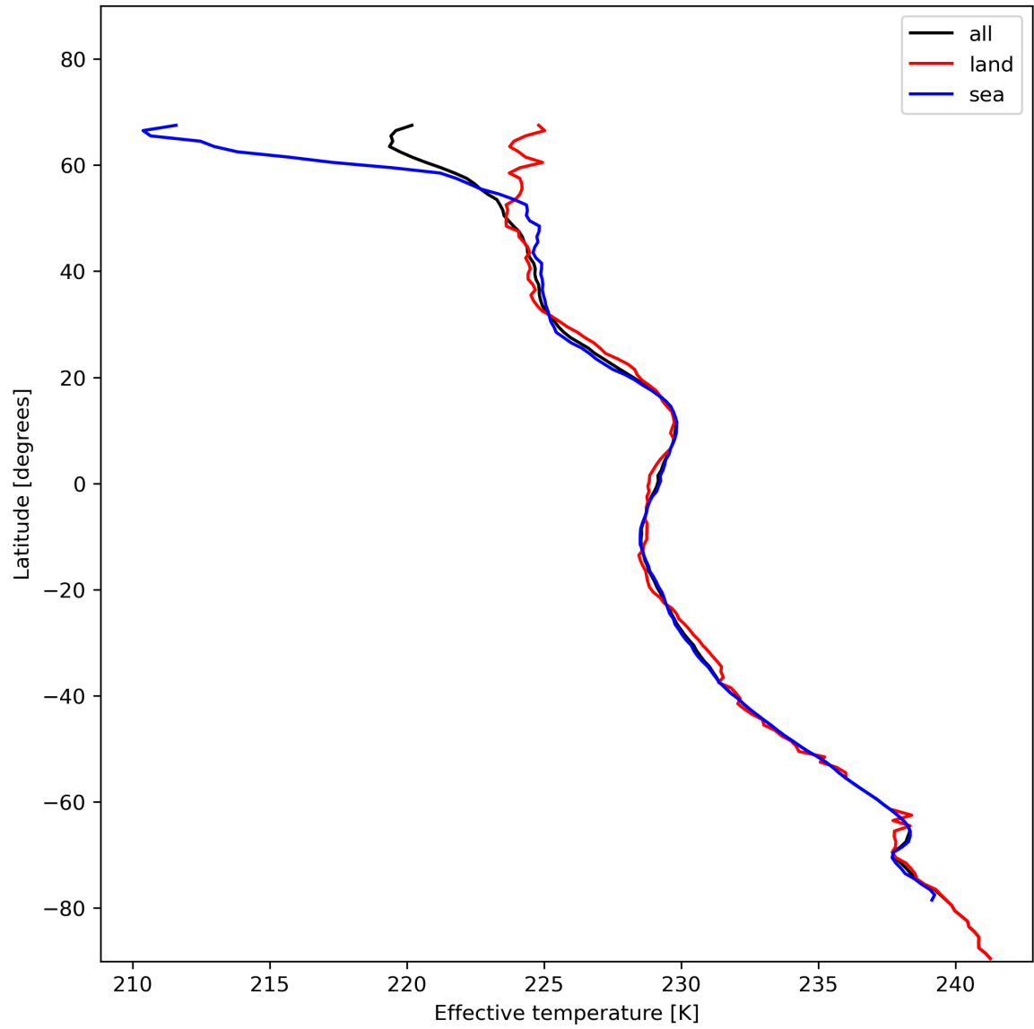
Figure 17: Zonal average of "Effective temperature" for 2024-01-15 to 2024-01-16.
