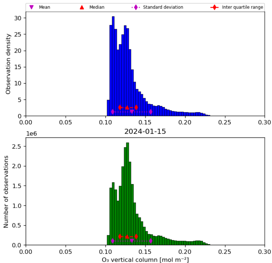
Figure 21: Histogram of “O 3 vertical column” for 2024-01-15 to 2024-01-16
