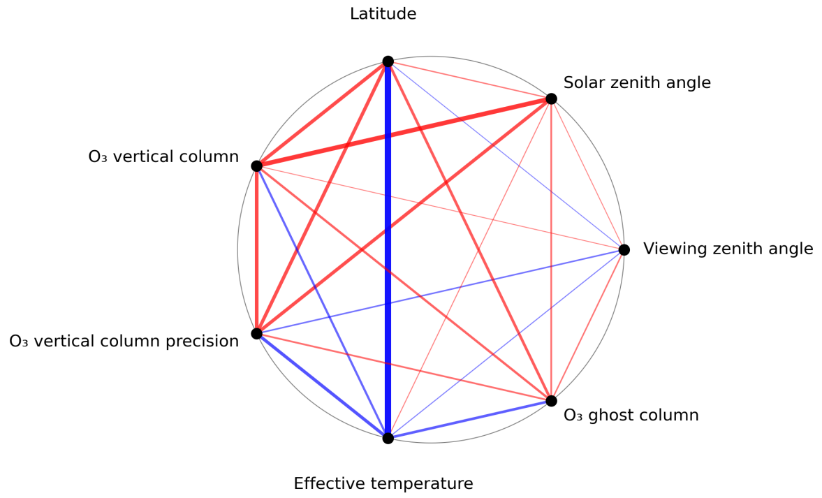
Figure 1: Map of correlation graph for 2024-01-15 to 2024-01-16.
