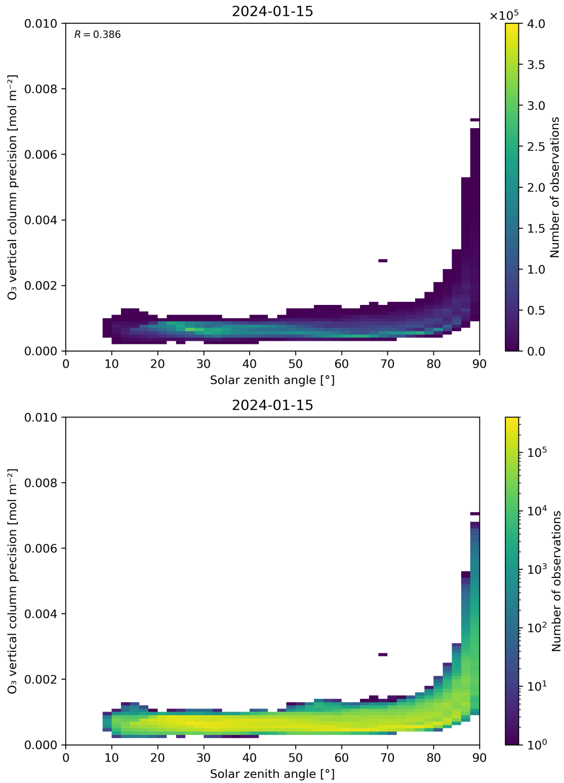
Figure 48: Scatter density plot of “Solar zenith angle” against “O 3 vertical column precision” for 2024-01-15 to 2024-01-16.
