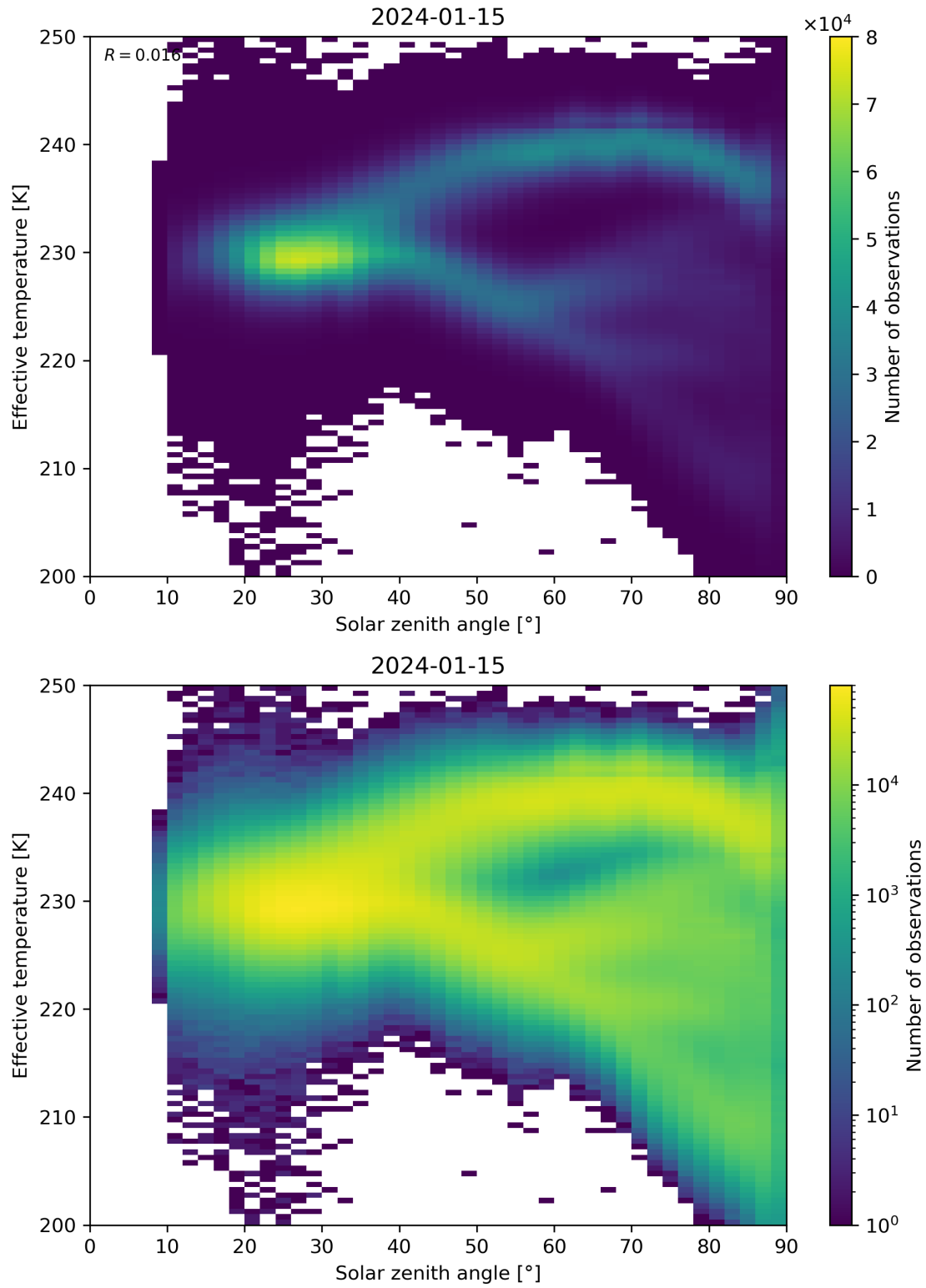
Figure 45: Scatter density plot of “Solar zenith angle” against “Effective temperature” for 2024-01-15 to 2024-01-16.
