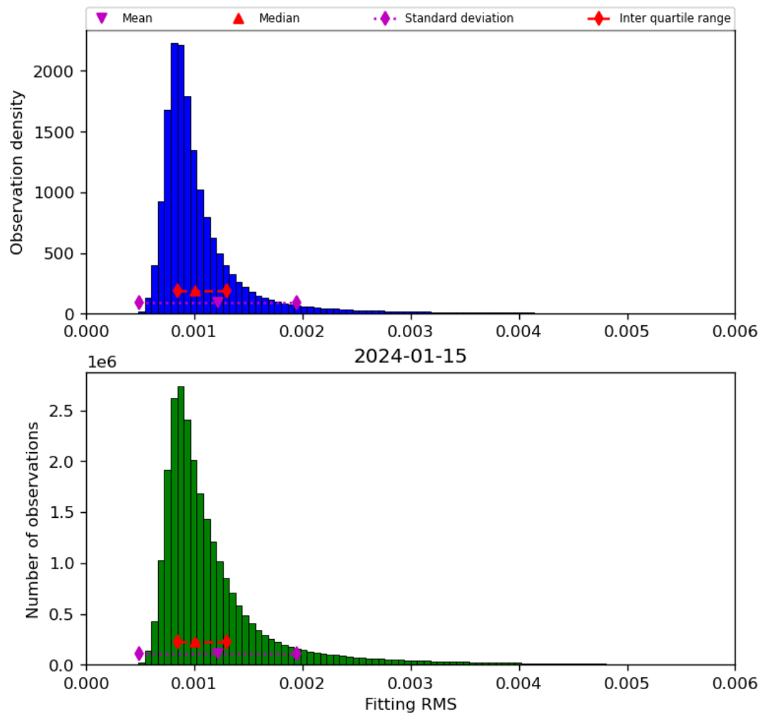
Figure 23: Histogram of “Fitting RMS” for 2024-01-15 to 2024-01-16
