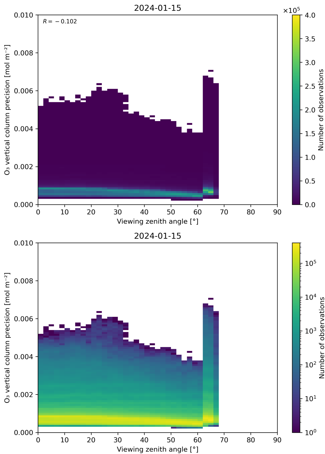
Figure 53: Scatter density plot of “Viewing zenith angle” against “O 3 vertical column precision” for 2024-01-15 to 2024-01-16.
