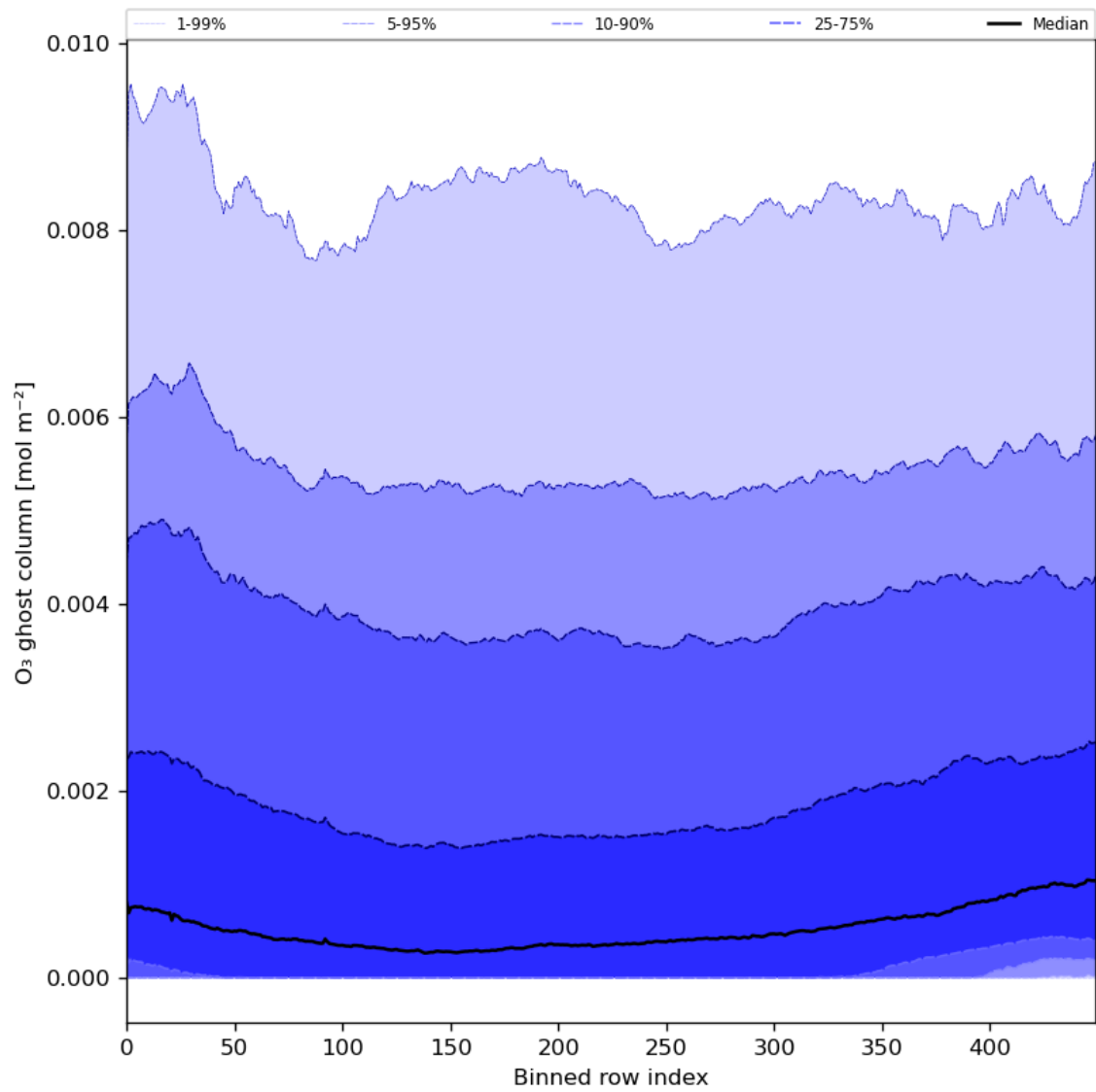
Figure 32: Along track statistics of “O 3 ghost column” for 2024-01-15 to 2024-01-16
