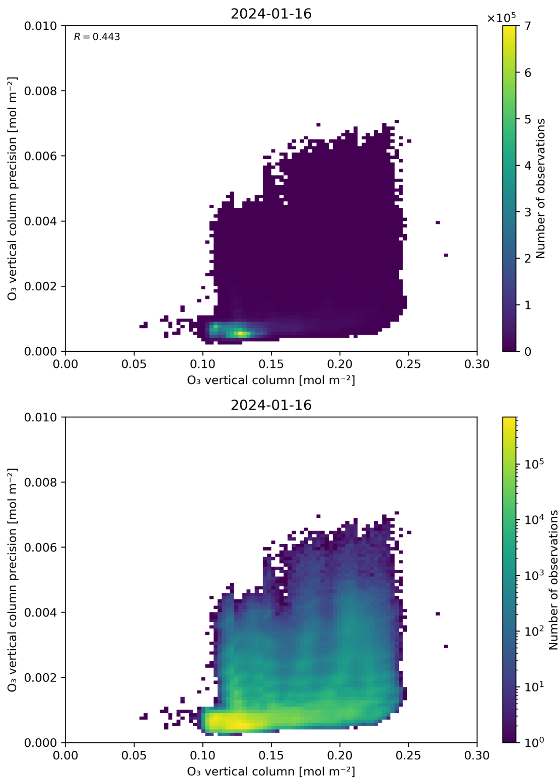
Figure 41: Scatter density plot of “O 3 vertical column” against “O 3 vertical column precision” for 2024-01-15 to 2024-01-17.
