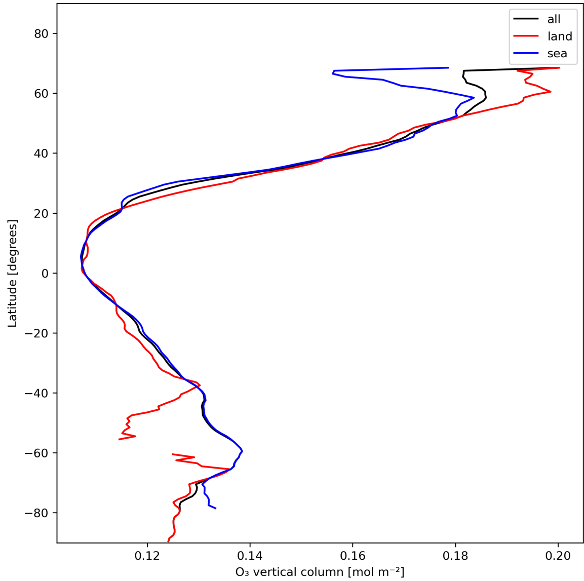
Figure 14: Zonal average of “O 3 vertical column” for 2024-01-15 to 2024-01-17.
