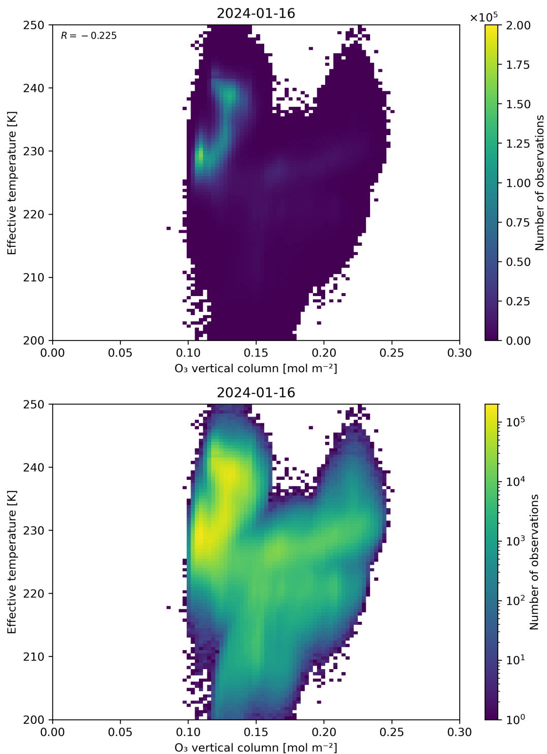
Figure 39: Scatter density plot of “O 3 vertical column” against “Effective temperature” for 2024-01-15 to 2024-01-17.
