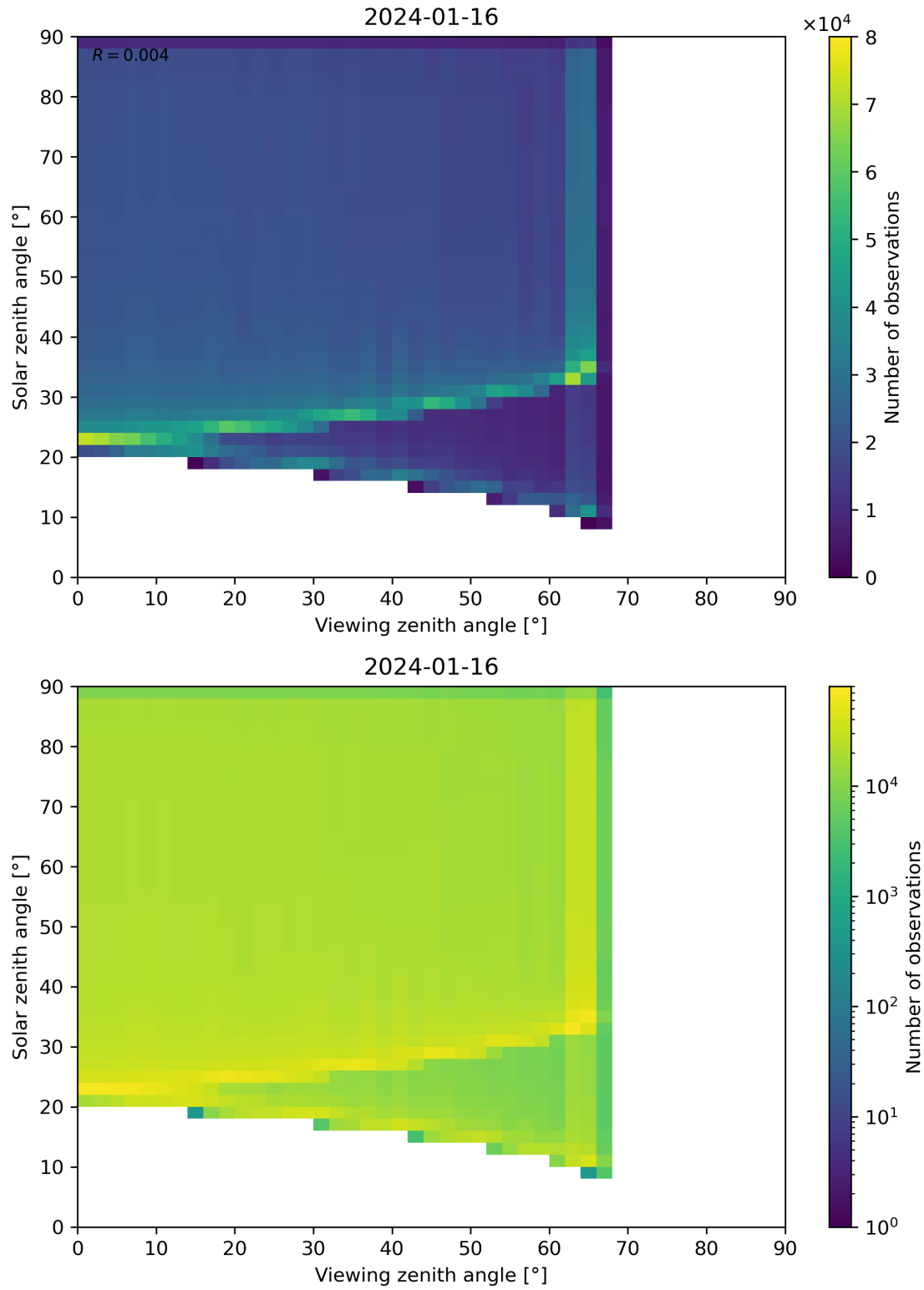
Figure 54: Scatter density plot of “Viewing zenith angle” against “Solar zenith angle” for 2024-01-15 to 2024-01-17.
