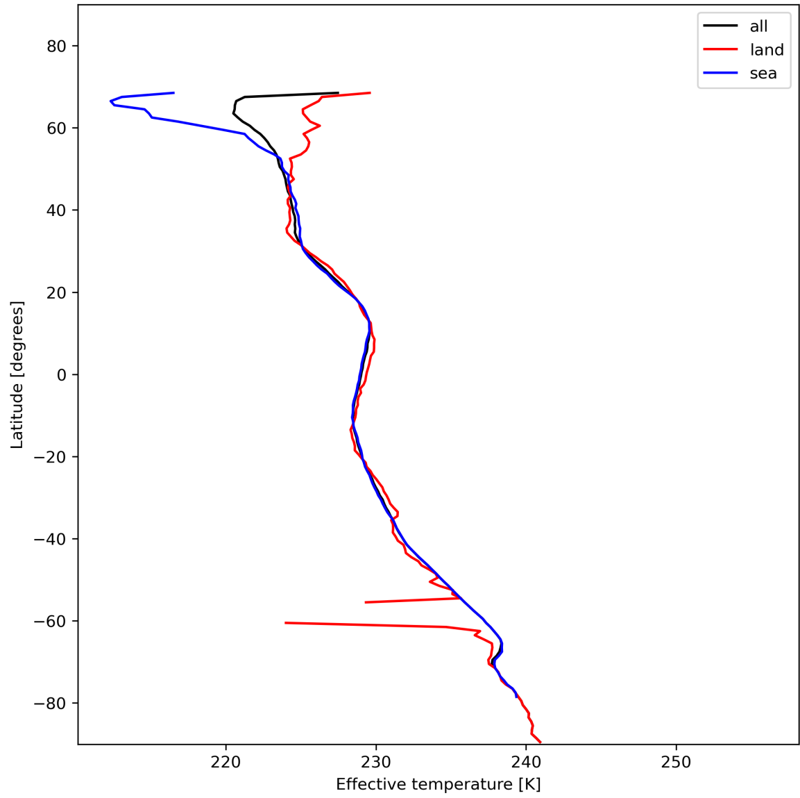
Figure 17: Zonal average of “Effective temperature” for 2024-01-15 to 2024-01-17.
