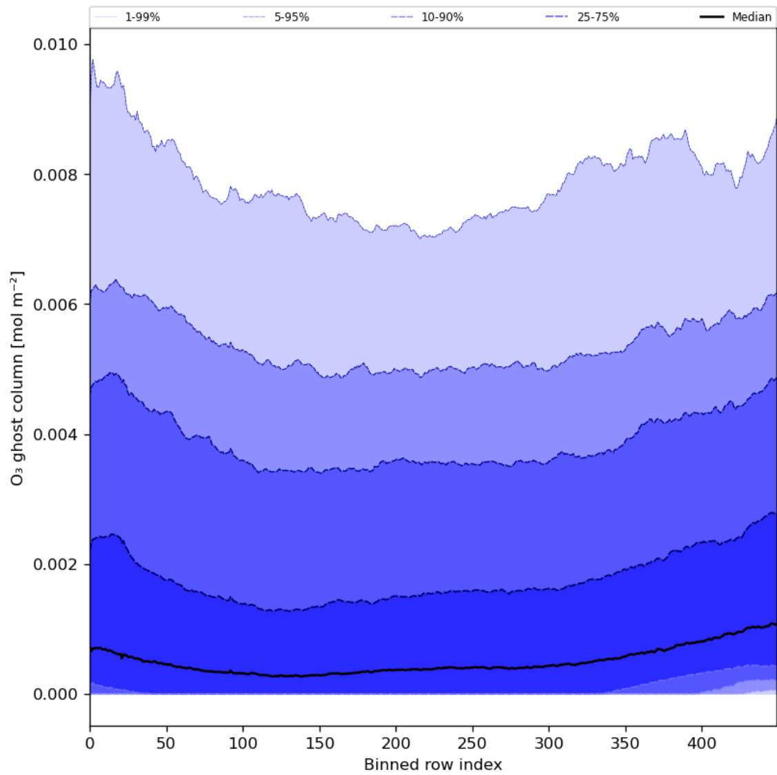
Figure 32: Along track statistics of “O 3 ghost column” for 2024-01-15 to 2024-01-17
