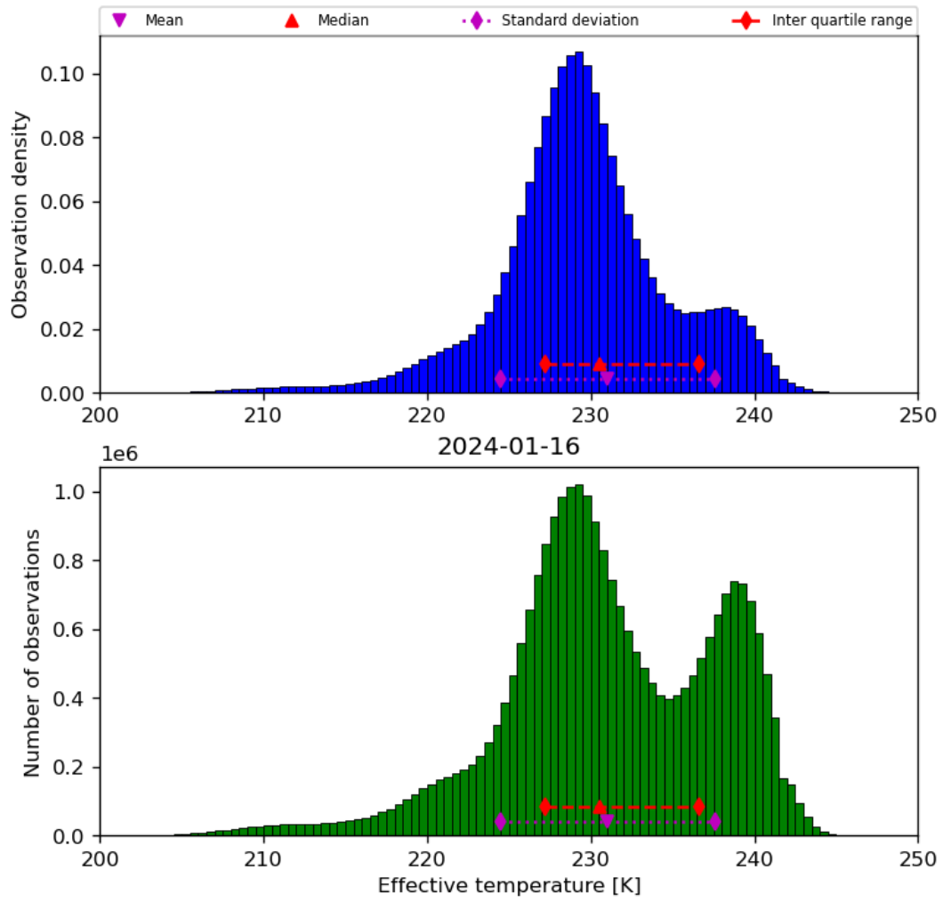
Figure 24: Histogram of “Effective temperature” for 2024-01-15 to 2024-01-17
