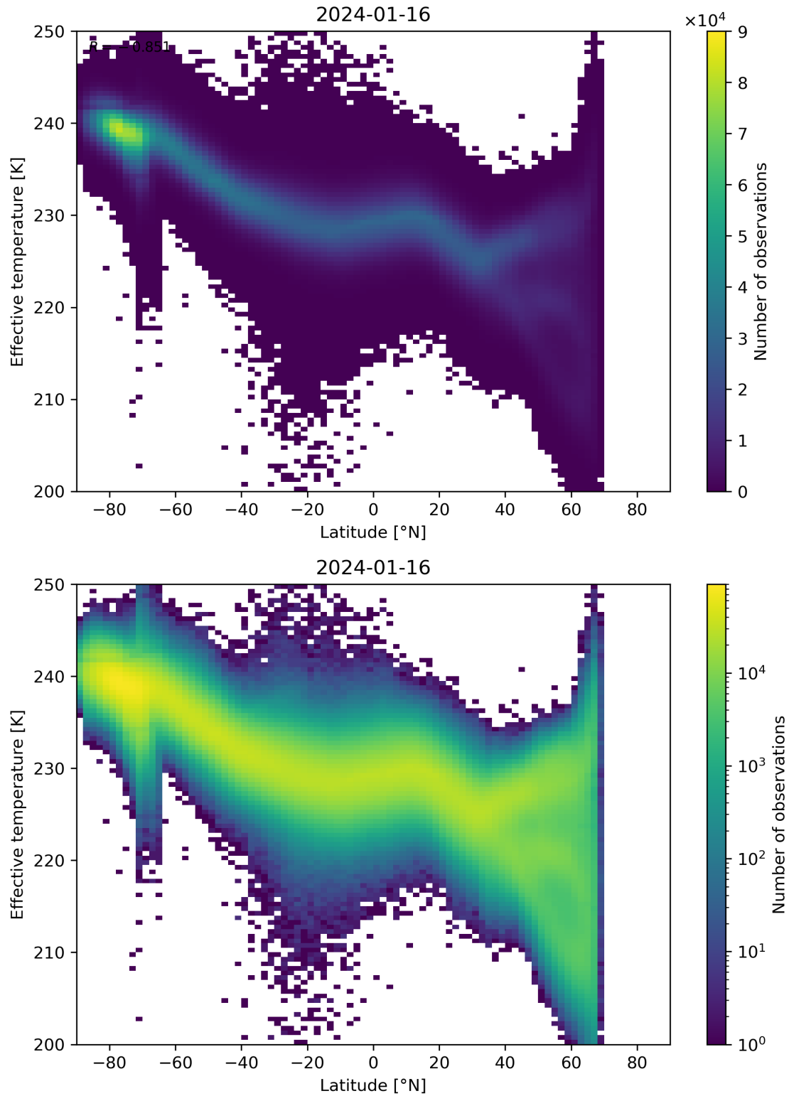
Figure 34: Scatter density plot of “Latitude” against “Effective temperature” for 2024-01-15 to 2024-01-17.
