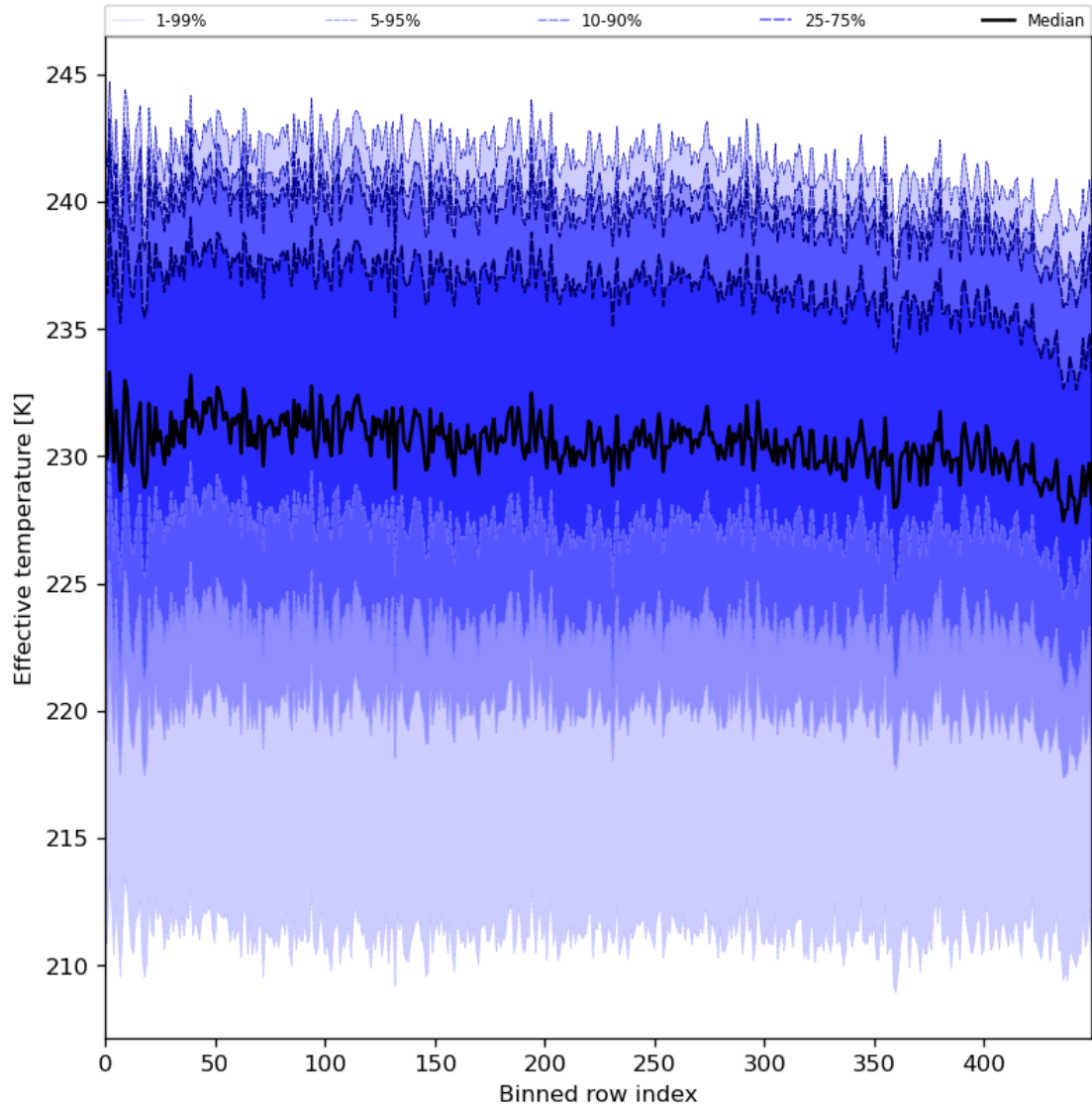
Figure 31: Along track statistics of “Effective temperature” for 2024-01-15 to 2024-01-17
