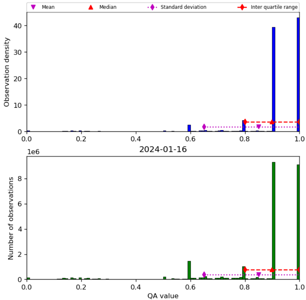
Figure 20: Histogram of “QA value” for 2024-01-15 to 2024-01-17
