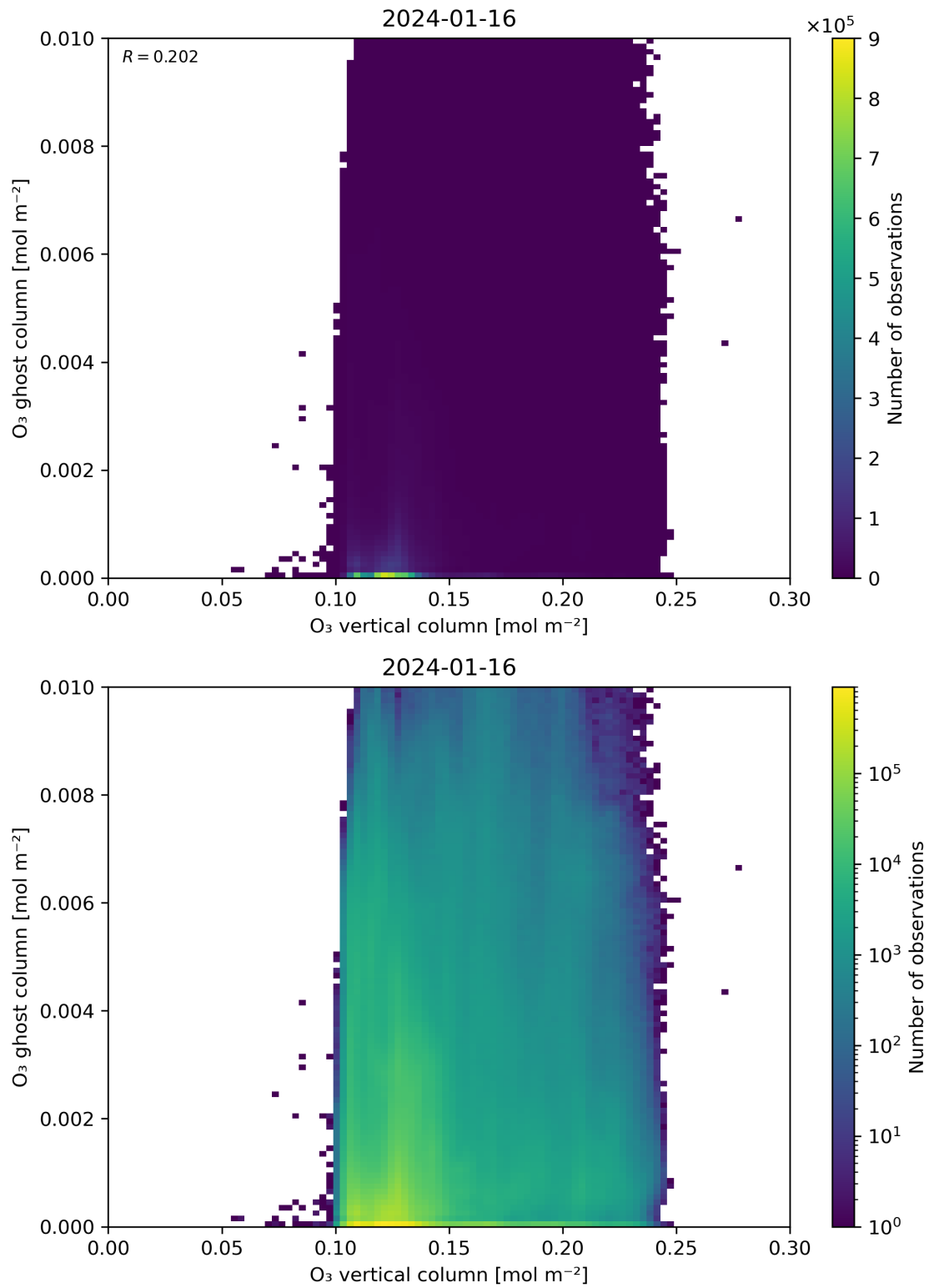
Figure 40: Scatter density plot of “O 3 vertical column” against “O 3 ghost column” for 2024-01-15 to 2024-01-17.
