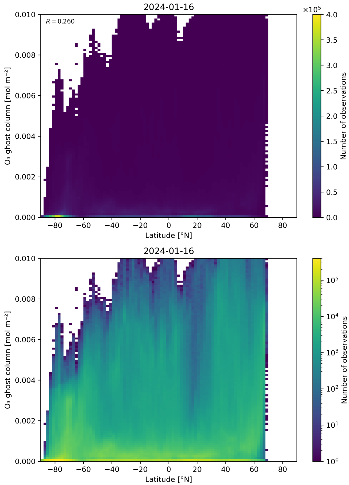
Figure 35: Scatter density plot of “Latitude” against “O 3 ghost column” for 2024-01-15 to 2024-01-17.
