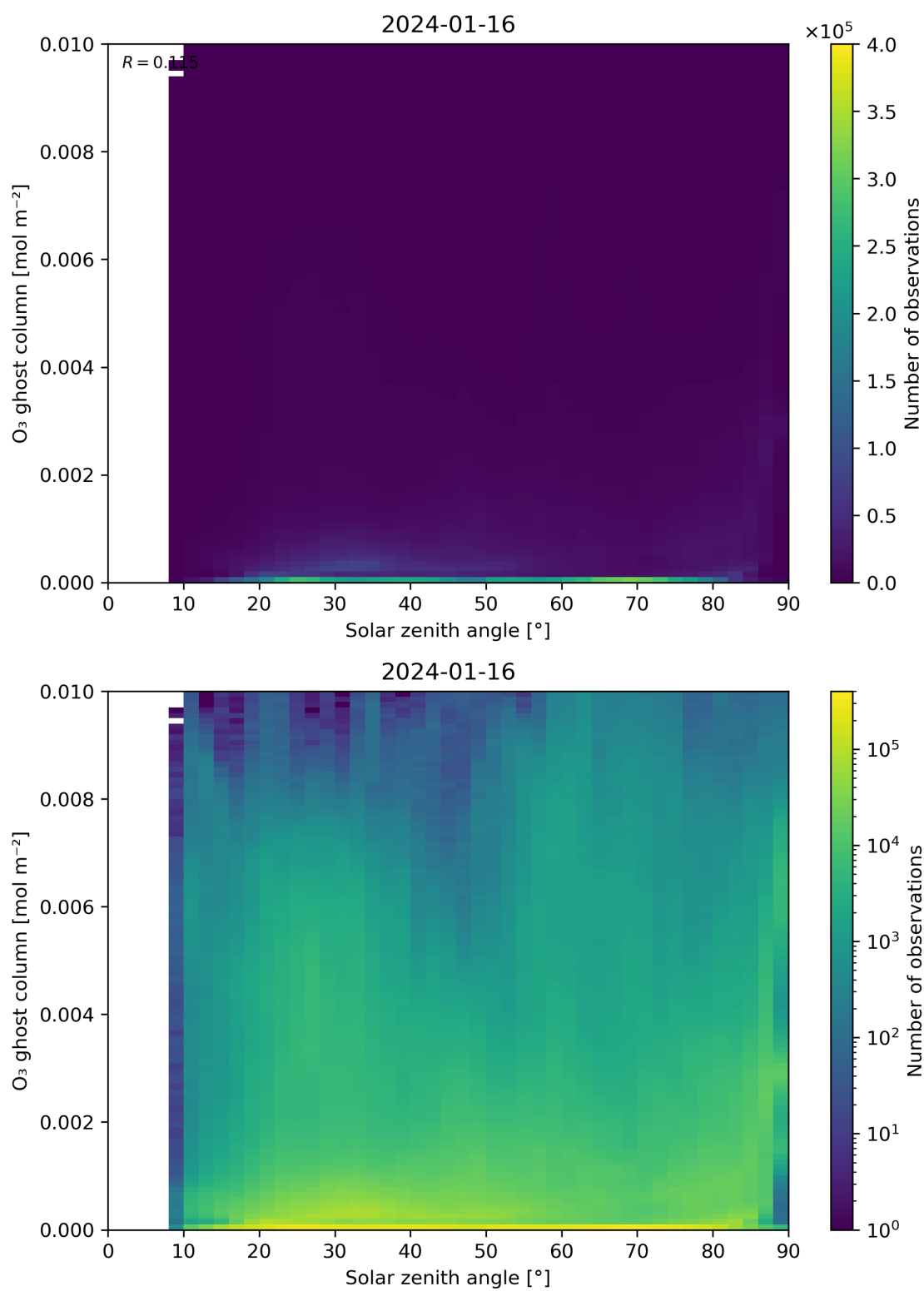
Figure 46: Scatter density plot of “Solar zenith angle” against “O 3 ghost column” for 2024-01-15 to 2024-01-17.
