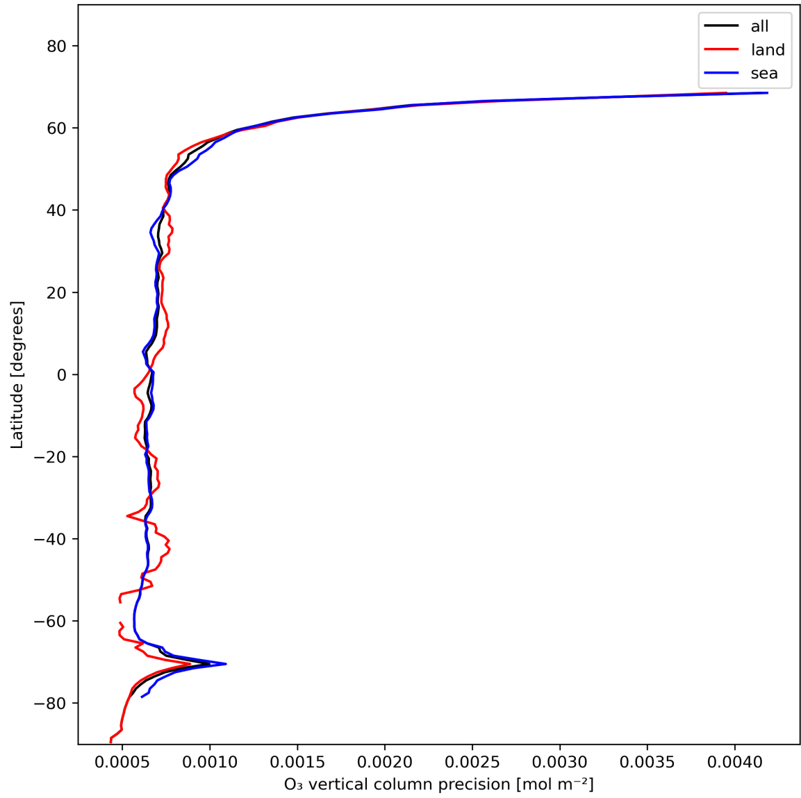
Figure 15: Zonal average of “O 3 vertical column precision” for 2024-01-15 to 2024-01-17.
