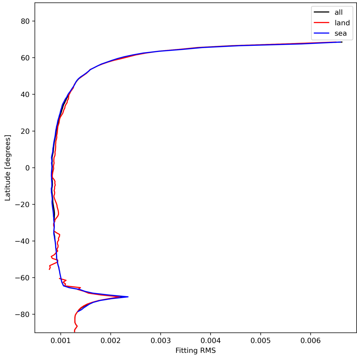
Figure 16: Zonal average of “Fitting RMS” for 2024-01-15 to 2024-01-17.
