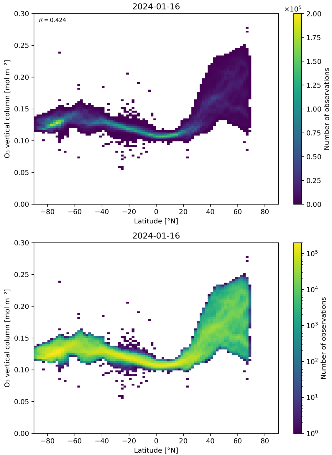
Figure 36: Scatter density plot of “Latitude” against “O 3 vertical column” for 2024-01-15 to 2024-01-17.
