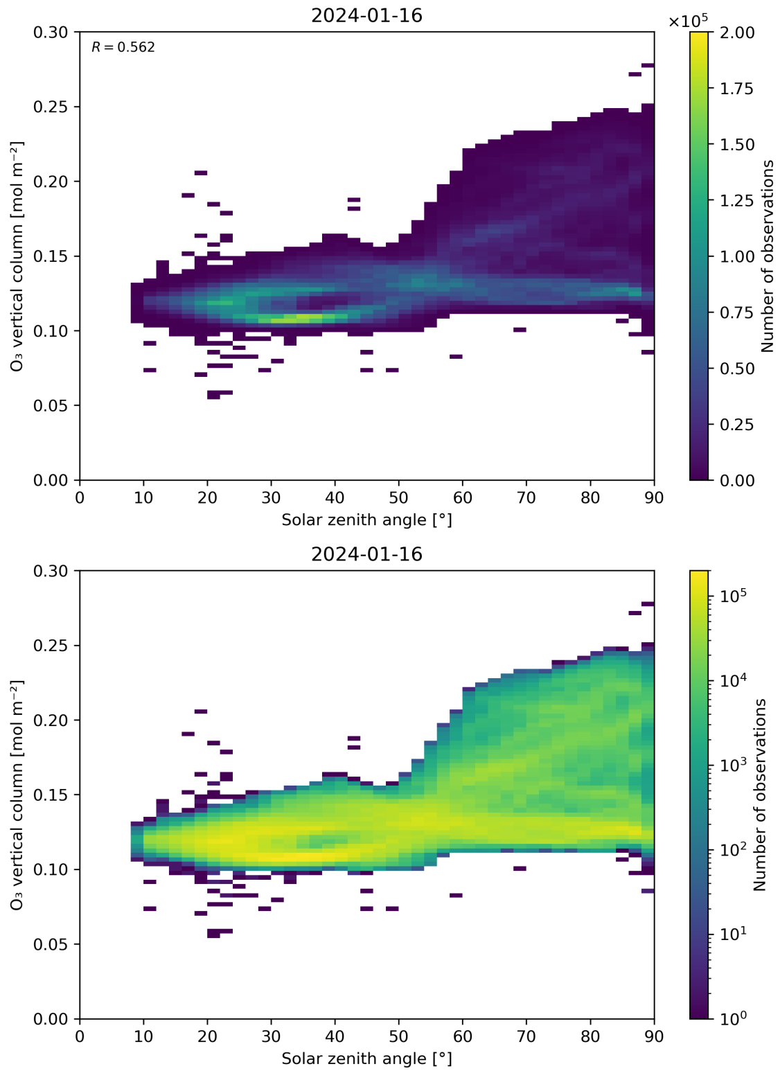
Figure 47: Scatter density plot of “Solar zenith angle” against “O 3 vertical column” for 2024-01-15 to 2024-01-17.
