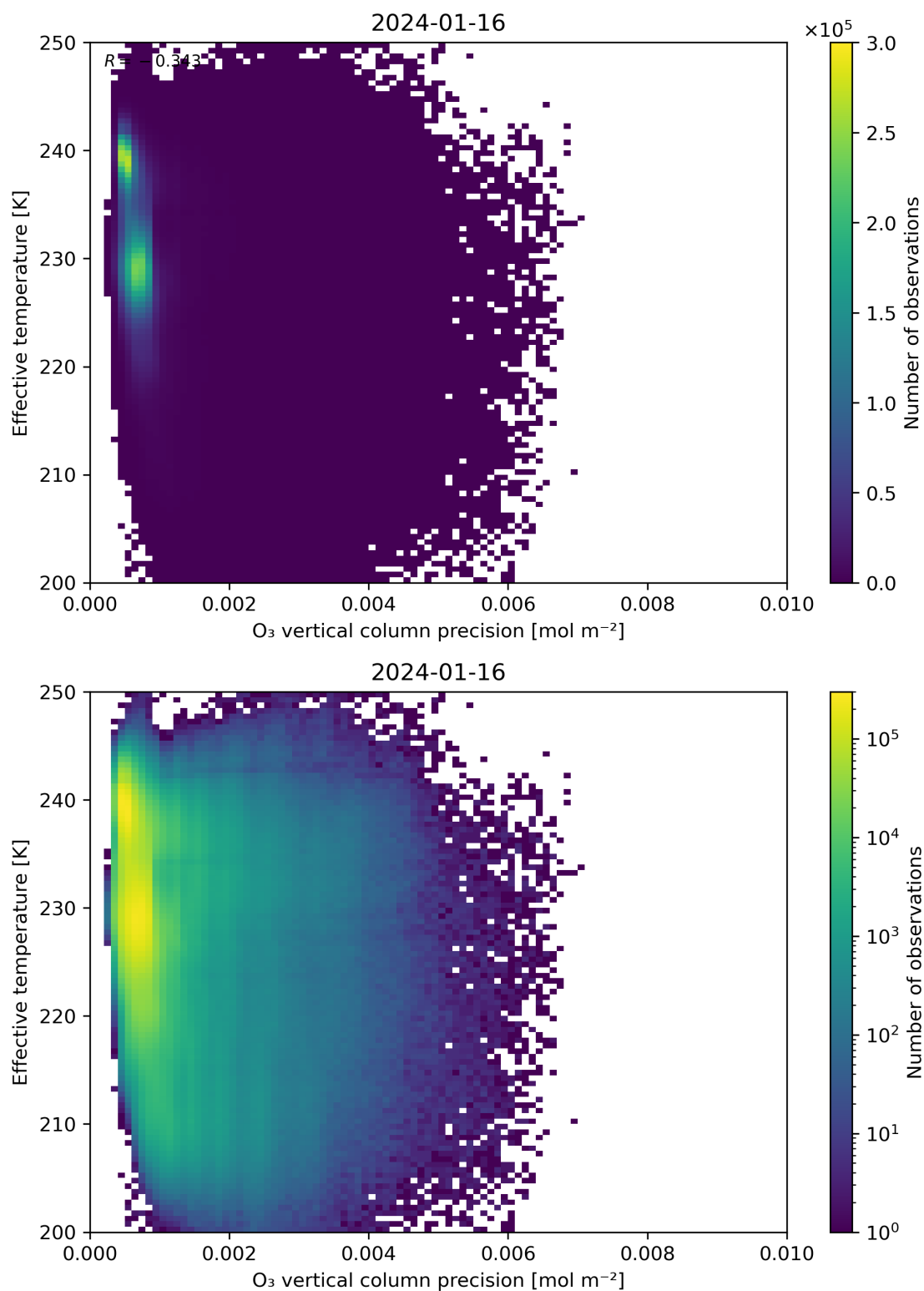
Figure 42: Scatter density plot of “O 3 vertical column precision” against “Effective temperature” for 2024-01-15 to 2024-01-17.
