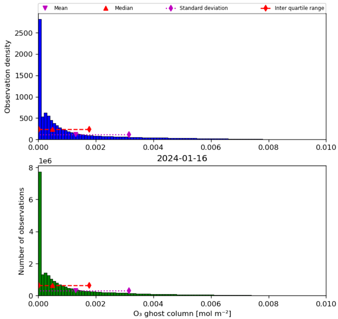
Figure 25: Histogram of “O 3 ghost column” for 2024-01-15 to 2024-01-17
