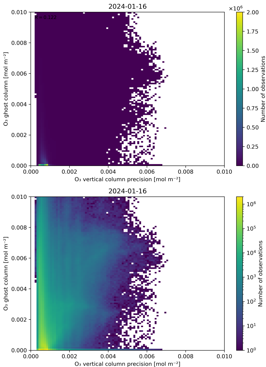
Figure 43: Scatter density plot of “ \text{O}_3 vertical column precision” against “ \text{O}_3 ghost column” for 2024-01-15 to 2024-01-17.
