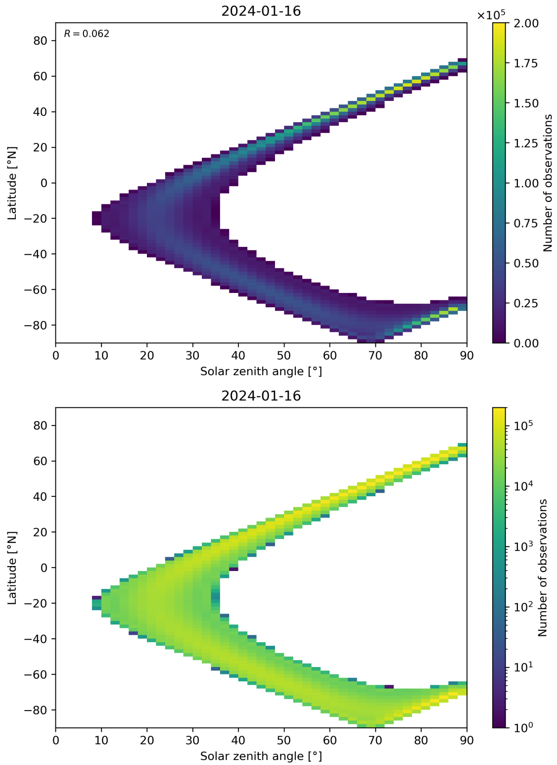
Figure 44: Scatter density plot of “Solar zenith angle” against “Latitude” for 2024-01-15 to 2024-01-17.
