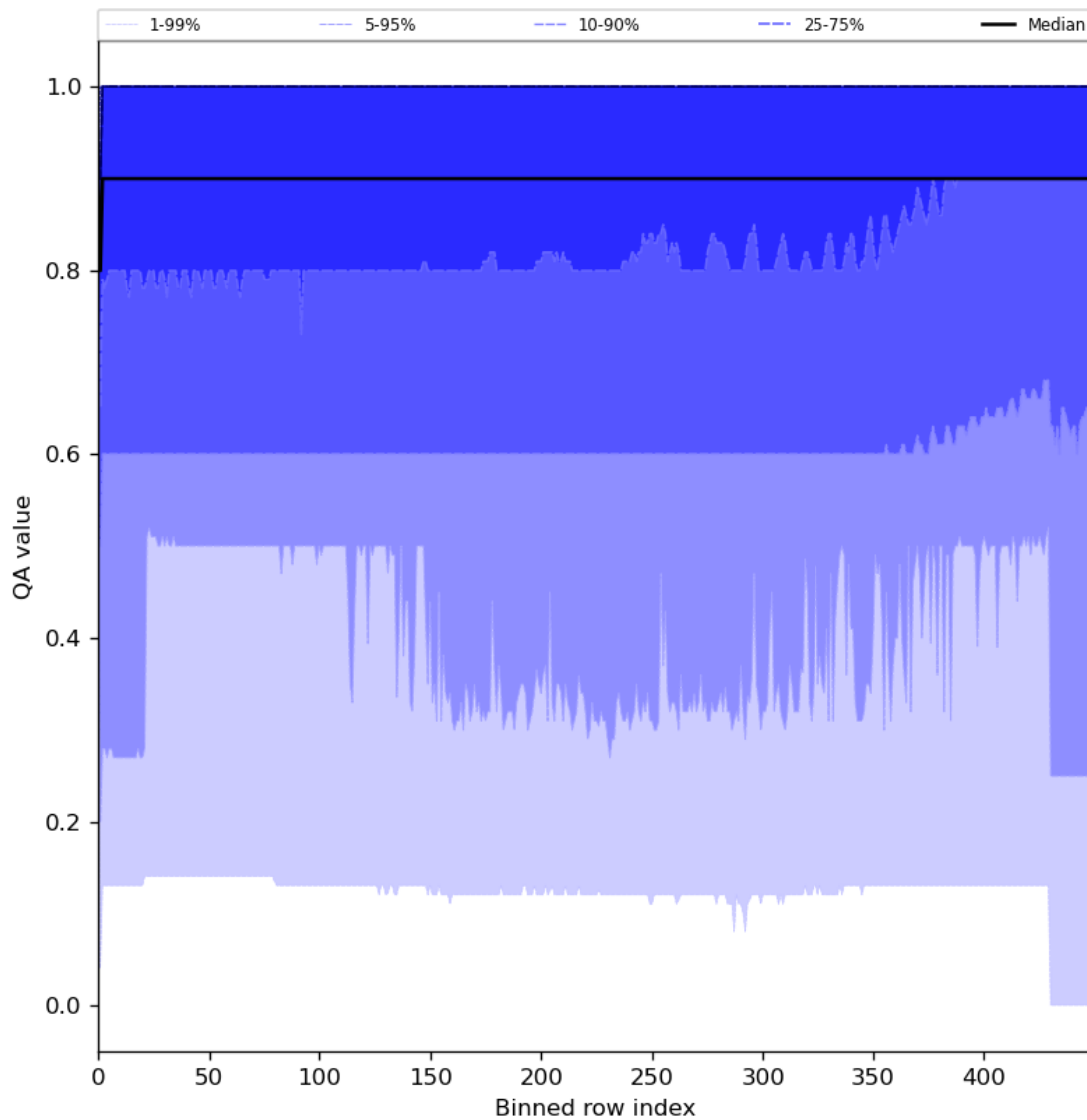
Figure 27: Along track statistics of “QA value” for 2024-01-15 to 2024-01-17
