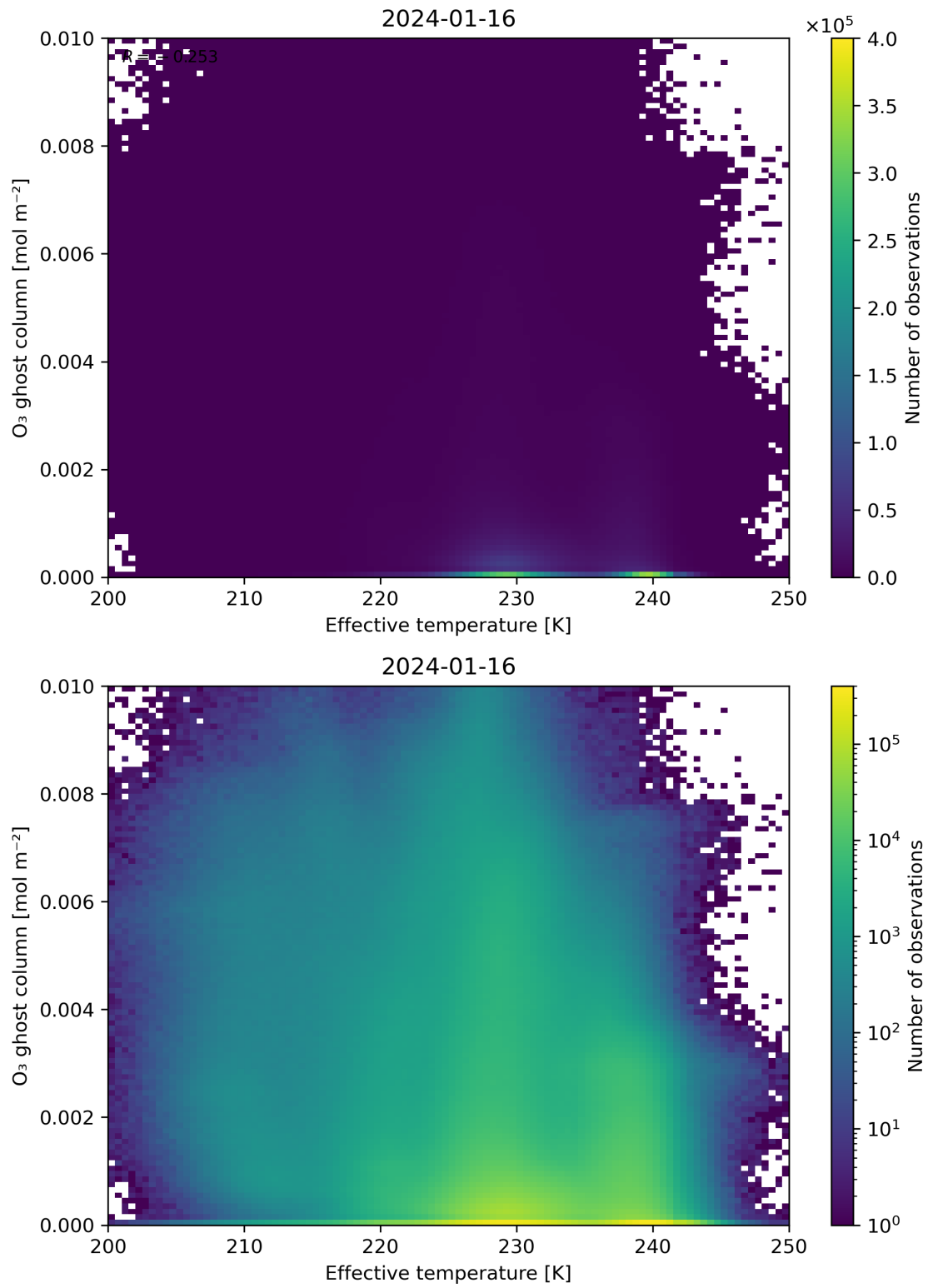
Figure 38: Scatter density plot of “Effective temperature” against “O 3 ghost column” for 2024-01-15 to 2024-01-17.
