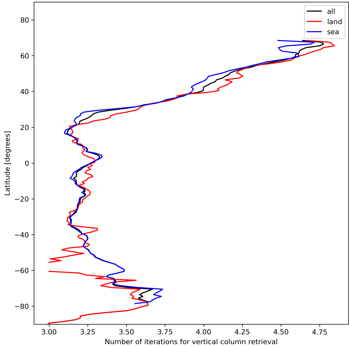
Figure 19: Zonal average of “Number of iterations for vertical column retrieval” for 2024-01-15 to 2024-01-17.
