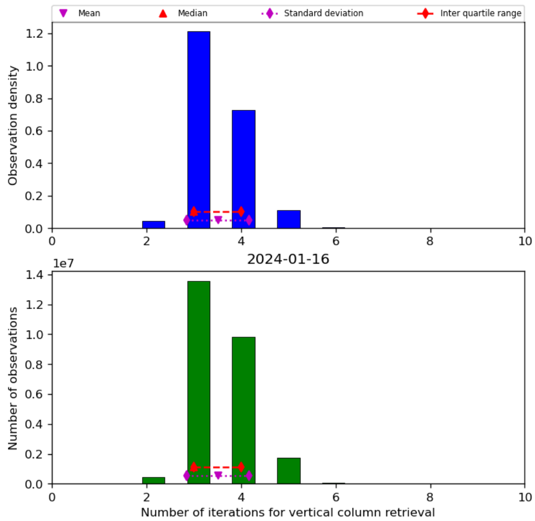
Figure 26: Histogram of “Number of iterations for vertical column retrieval” for 2024-01-15 to 2024-01-17
