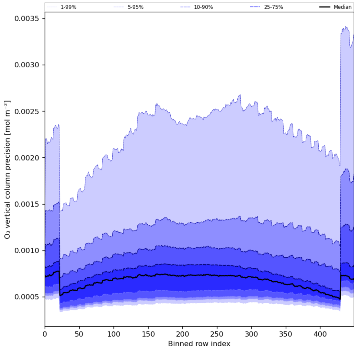
Figure 29: Along track statistics of “O 3 vertical column precision” for 2024-01-15 to 2024-01-17
