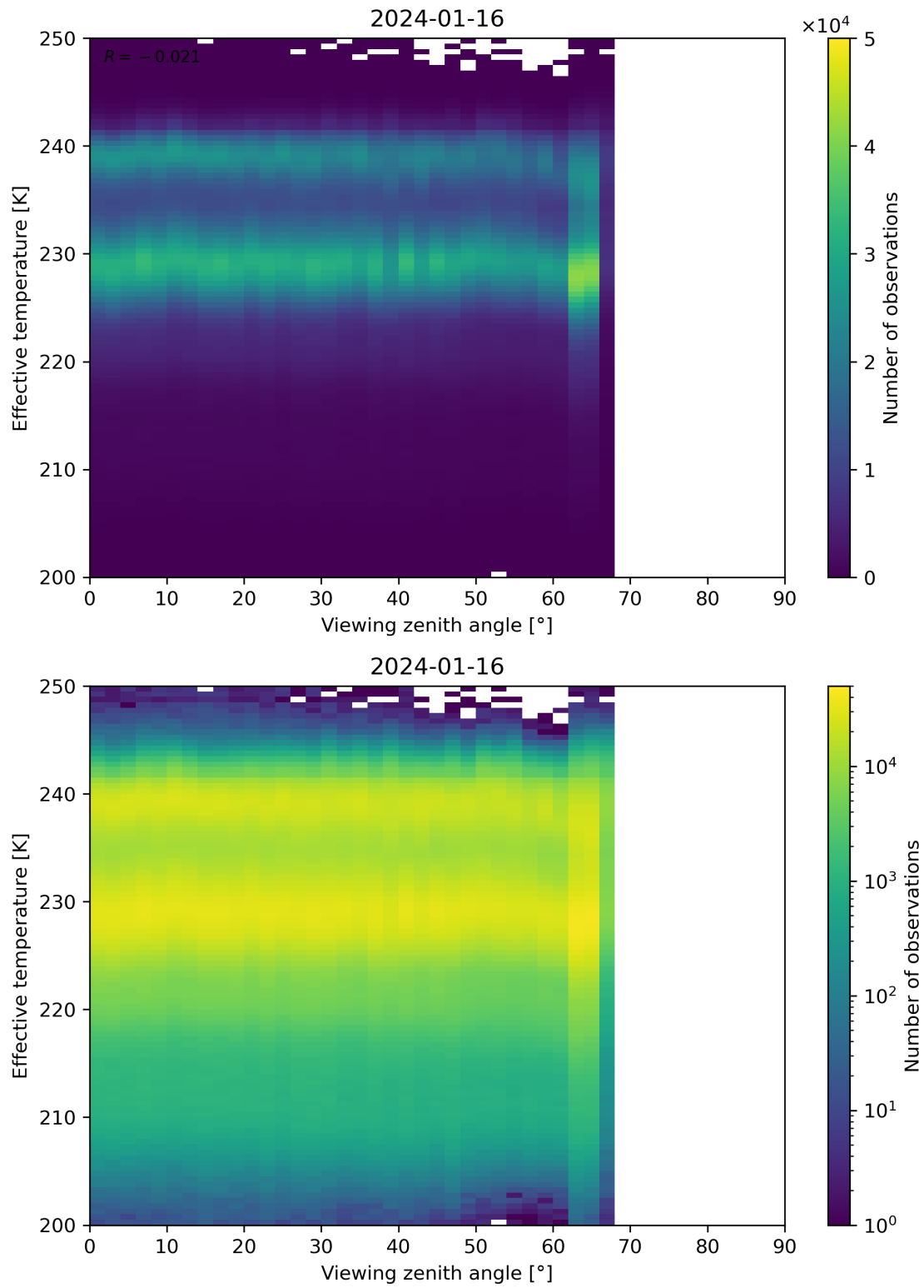
Figure 50: Scatter density plot of “Viewing zenith angle” against “Effective temperature” for 2024-01-15 to 2024-01-17.
