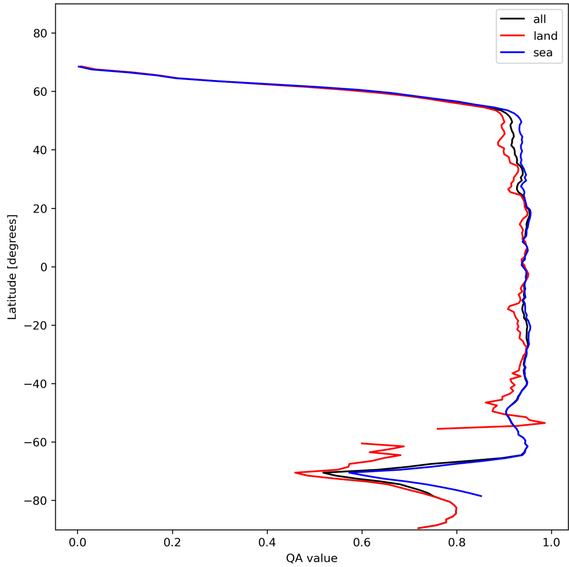
Figure 13: Zonal average of “QA value” for 2024-01-15 to 2024-01-17.
