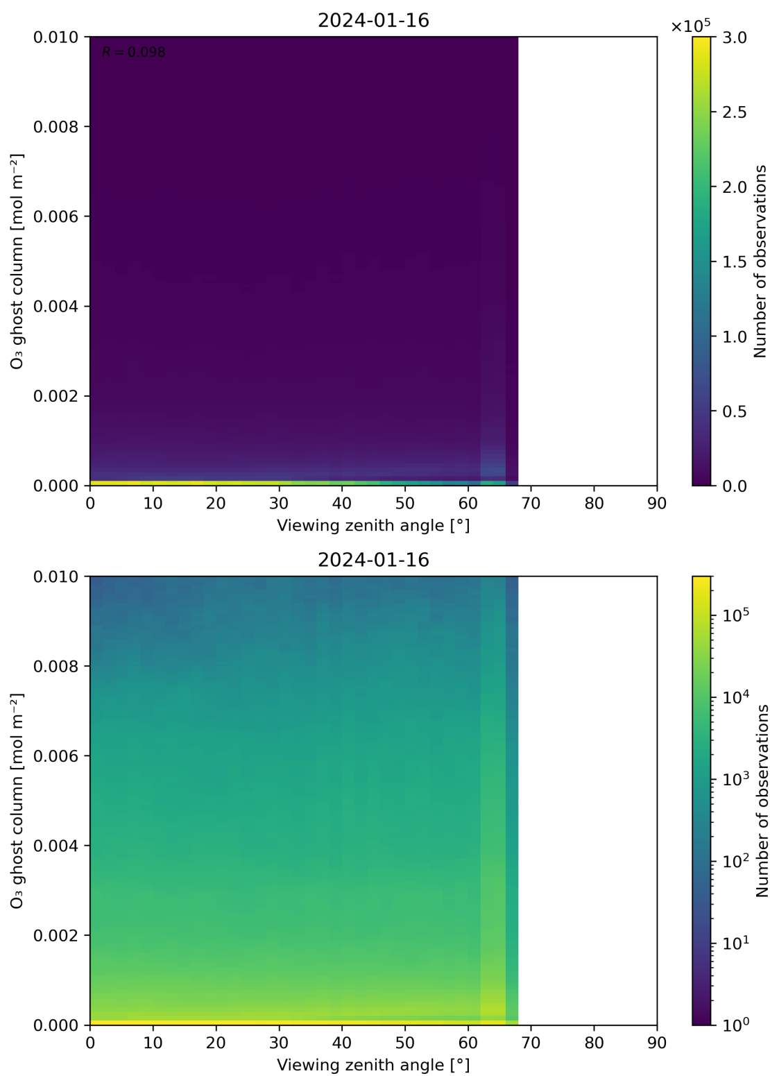
Figure 51: Scatter density plot of “Viewing zenith angle” against “O 3 ghost column” for 2024-01-15 to 2024-01-17.
