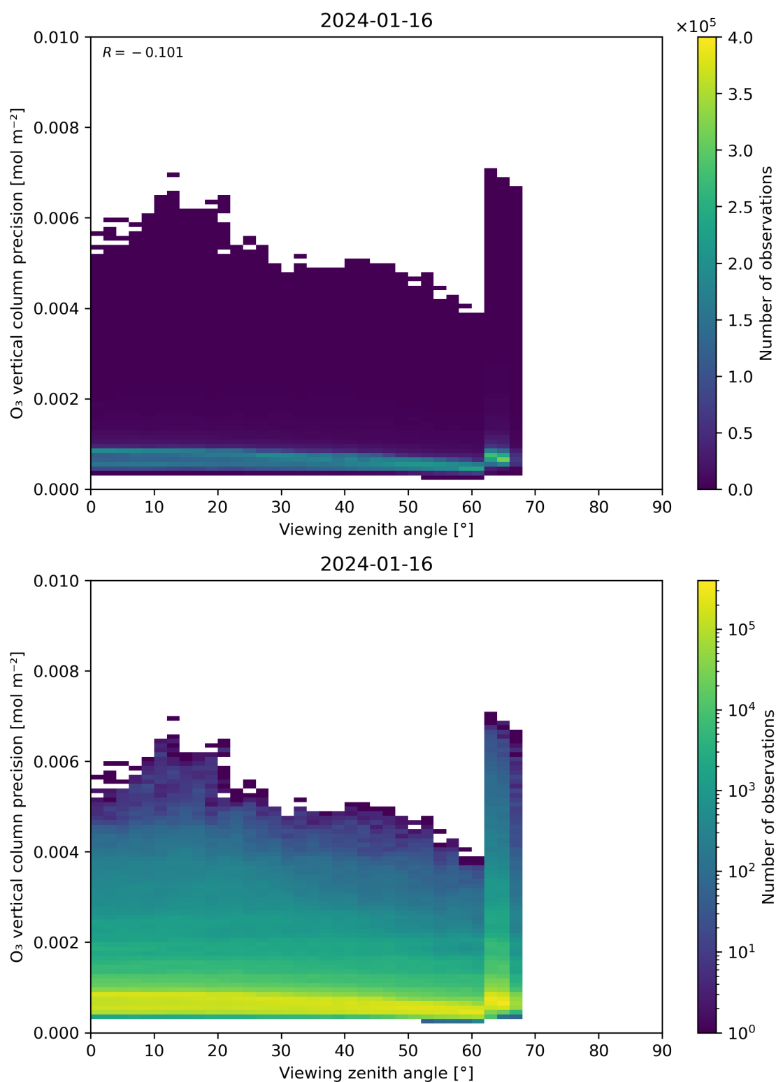
Figure 53: Scatter density plot of “Viewing zenith angle” against “O 3 vertical column precision” for 2024-01-15 to 2024-01-17.
