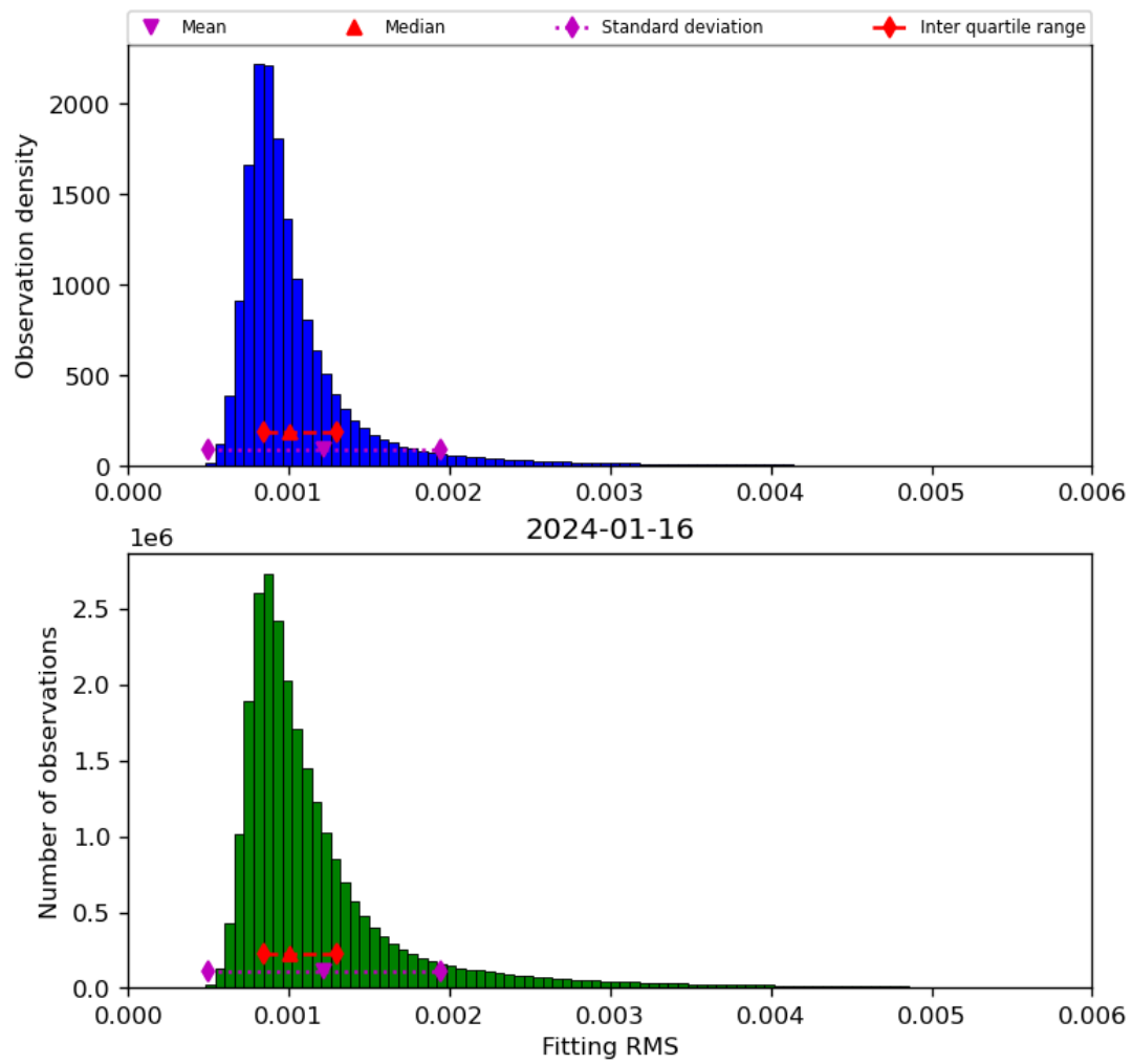
Figure 23: Histogram of “Fitting RMS” for 2024-01-15 to 2024-01-17
