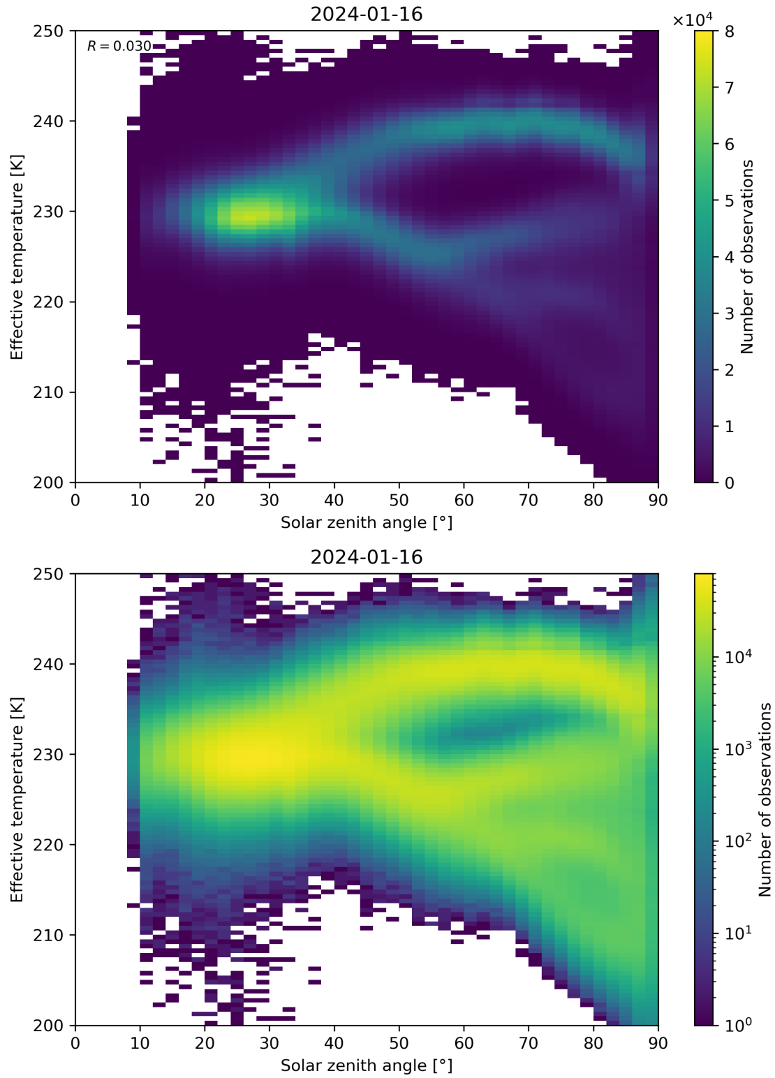
Figure 45: Scatter density plot of “Solar zenith angle” against “Effective temperature” for 2024-01-15 to 2024-01-17.
