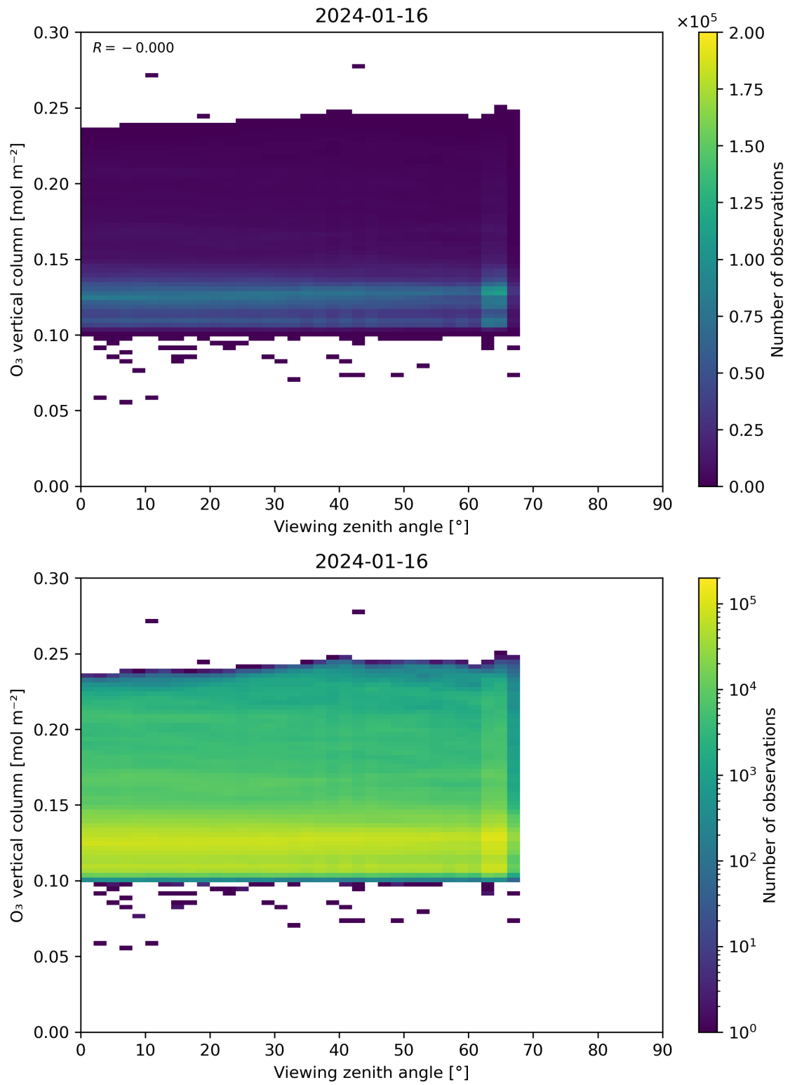
Figure 52: Scatter density plot of “Viewing zenith angle” against “O 3 vertical column” for 2024-01-15 to 2024-01-17.
