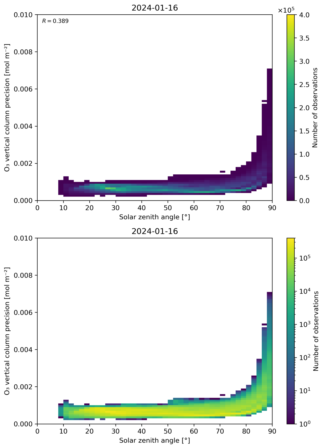
Figure 48: Scatter density plot of “Solar zenith angle” against “O 3 vertical column precision” for 2024-01-15 to 2024-01-17.
