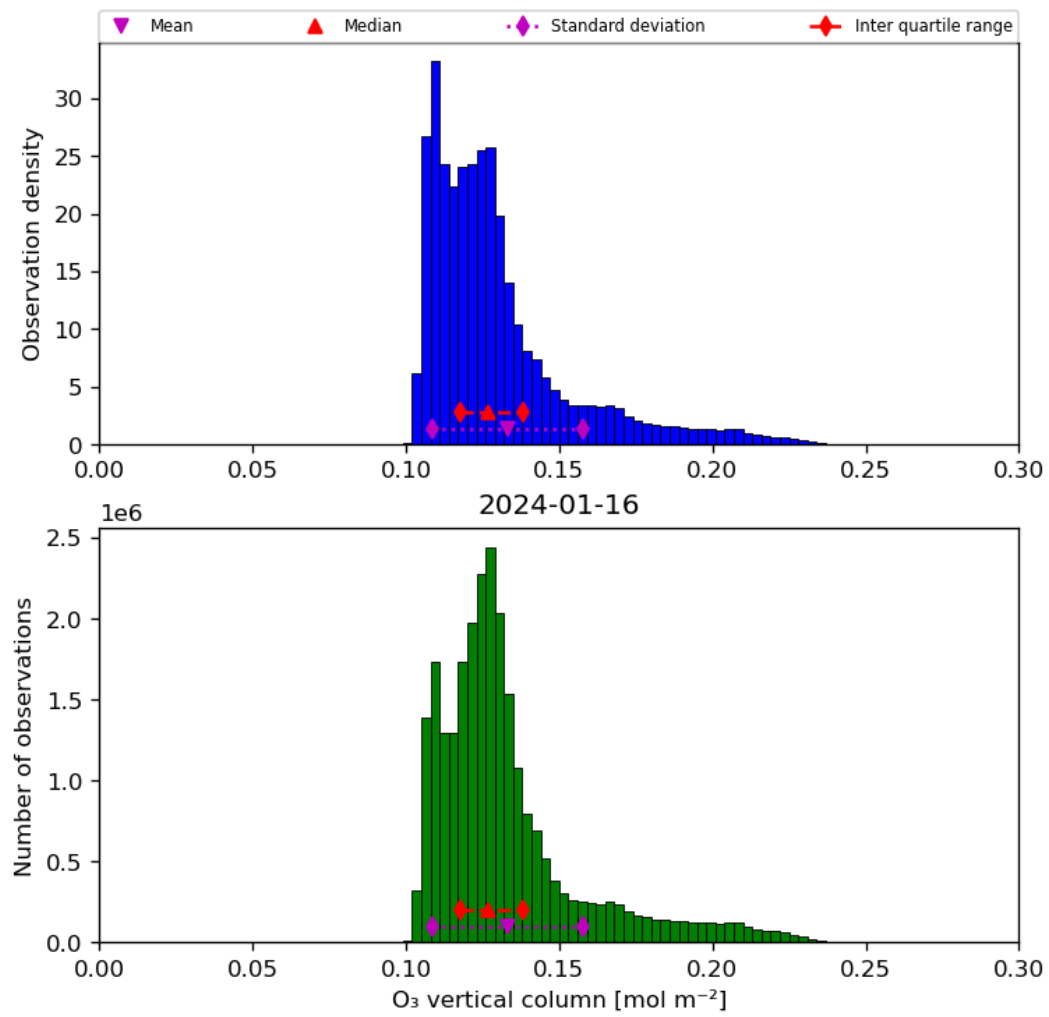
Figure 21: Histogram of “O 3 vertical column” for 2024-01-15 to 2024-01-17
