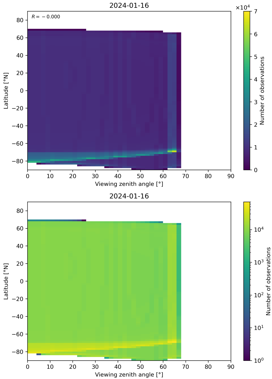
Figure 49: Scatter density plot of “Viewing zenith angle” against “Latitude” for 2024-01-15 to 2024-01-17.
