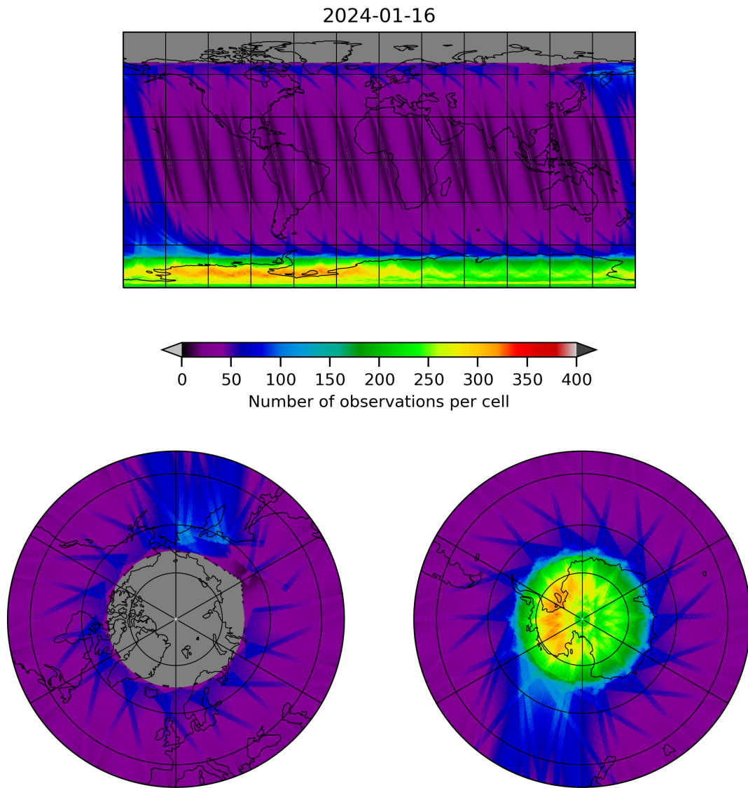
Figure 12: Map of the number of observations for 2024-01-15 to 2024-01-17
