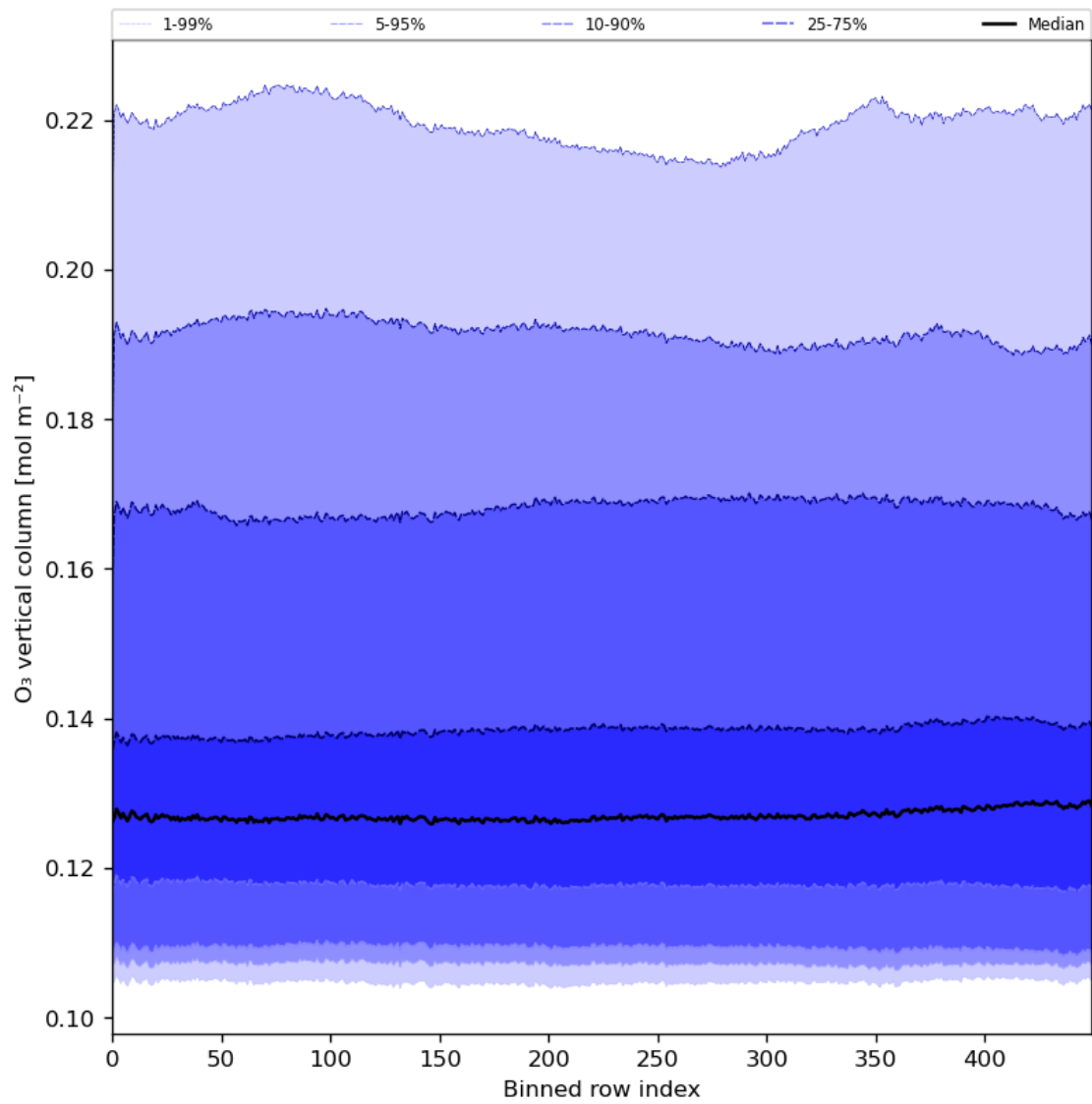
Figure 28: Along track statistics of “O 3 vertical column” for 2024-01-15 to 2024-01-17
