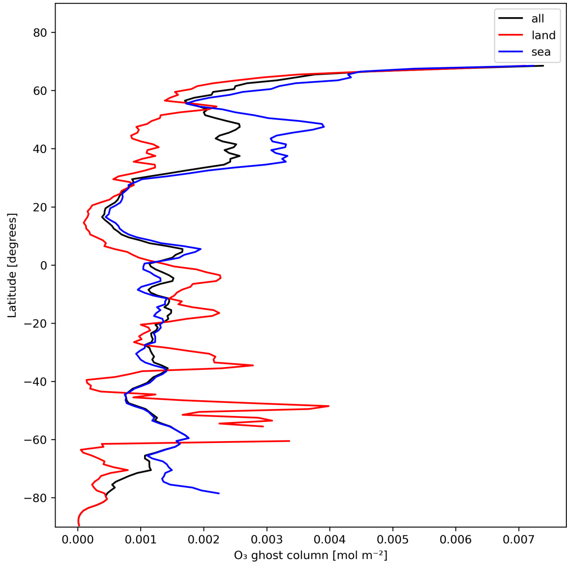
Figure 18: Zonal average of “O 3 ghost column” for 2024-01-15 to 2024-01-17.
