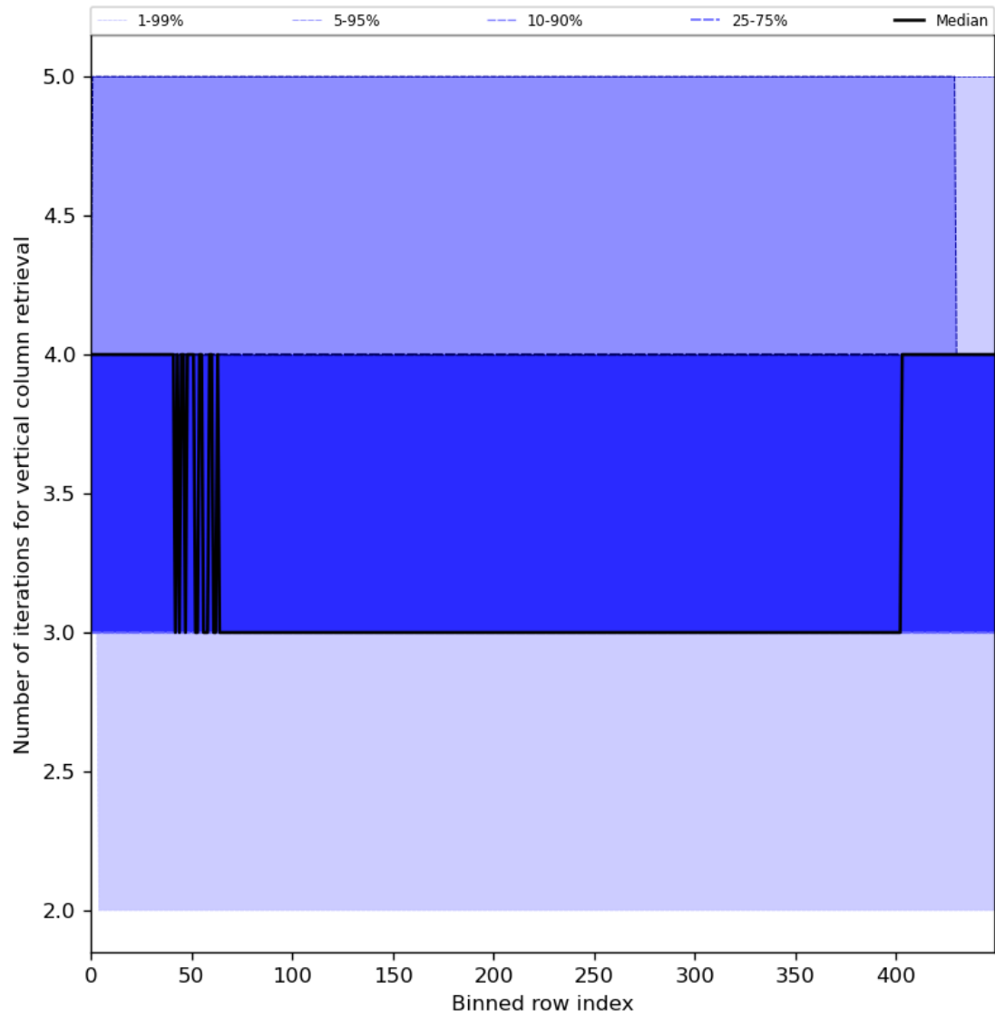
Figure 33: Along track statistics of “Number of iterations for vertical column retrieval” for 2024-01-15 to 2024-01-17
