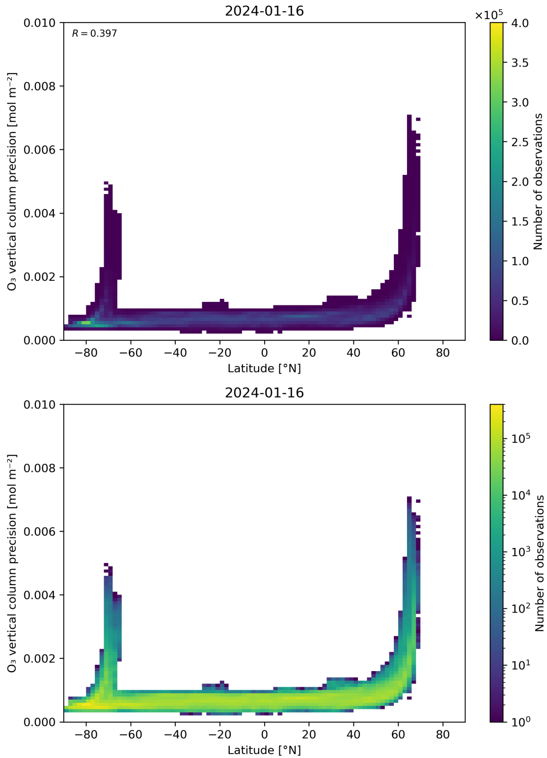
Figure 37: Scatter density plot of “Latitude” against “O 3 vertical column precision” for 2024-01-15 to 2024-01-17.
