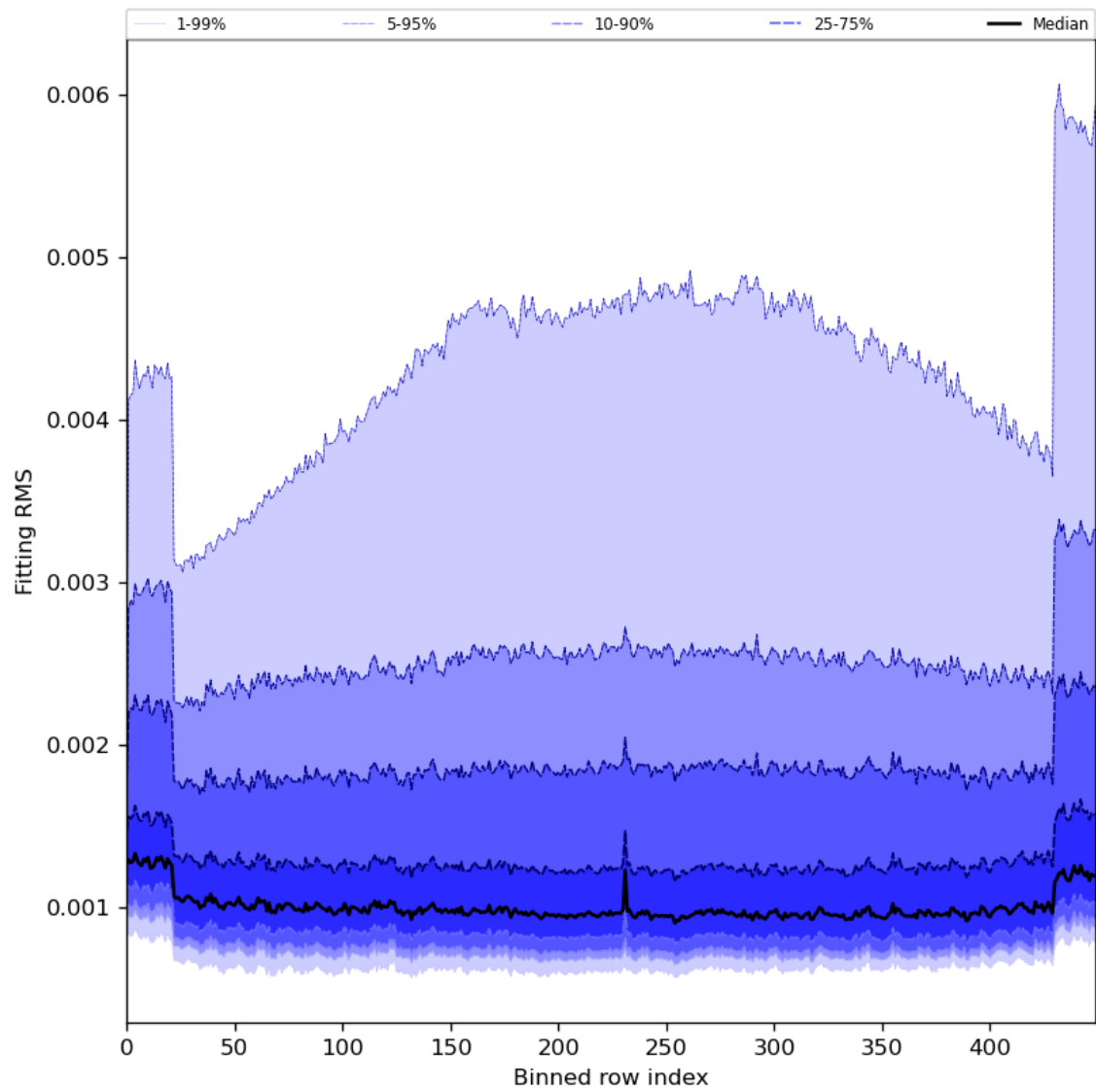
Figure 30: Along track statistics of “Fitting RMS” for 2024-01-15 to 2024-01-17
