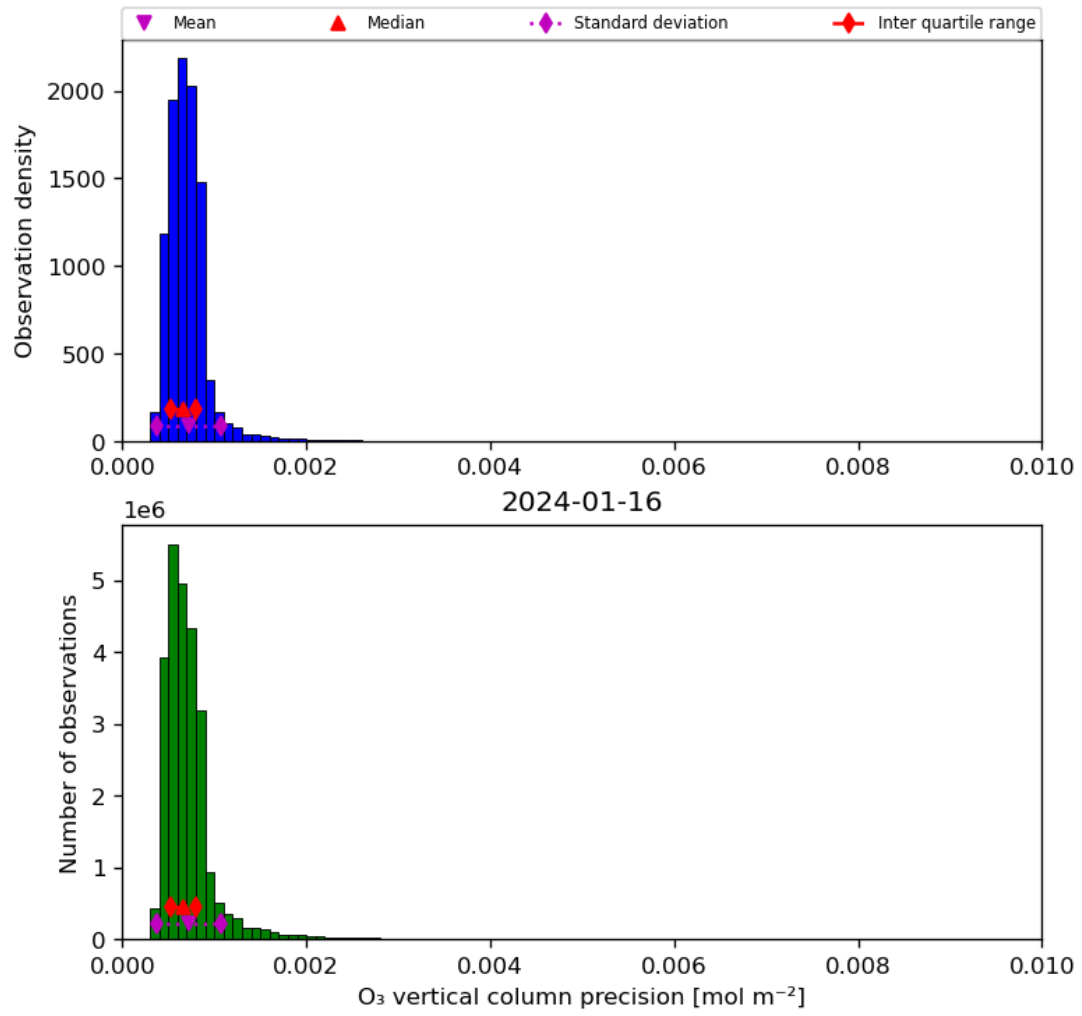
Figure 22: Histogram of “O 3 vertical column precision” for 2024-01-15 to 2024-01-17
