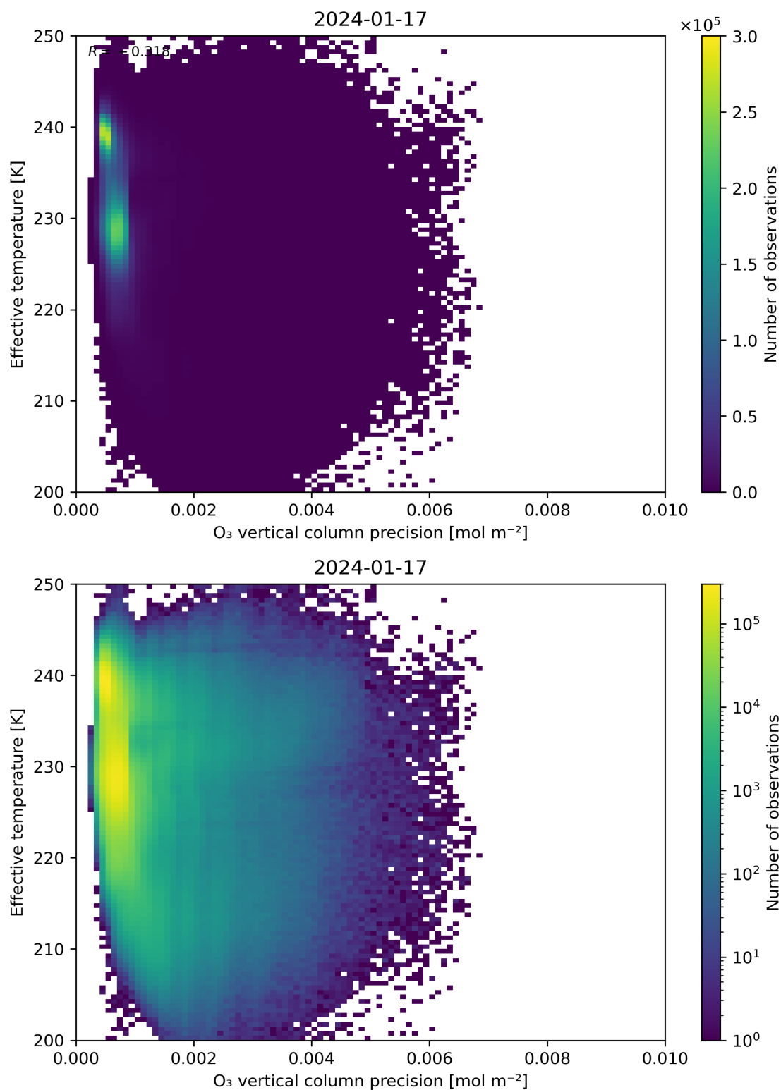
Figure 42: Scatter density plot of “O 3 vertical column precision” against “Effective temperature” for 2024-01-16 to 2024-01-18.
