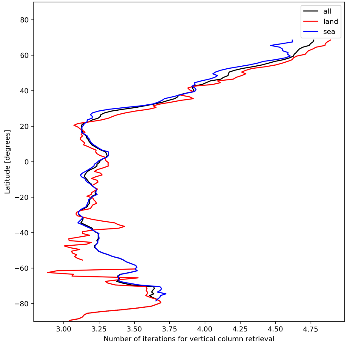
Figure 19: Zonal average of “Number of iterations for vertical column retrieval” for 2024-01-16 to 2024-01-18.
