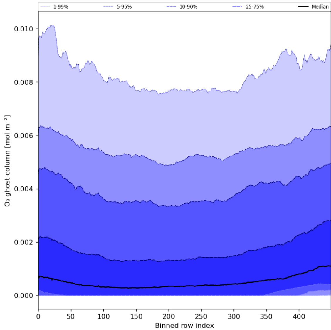
Figure 32: Along track statistics of “O 3 ghost column” for 2024-01-16 to 2024-01-18
