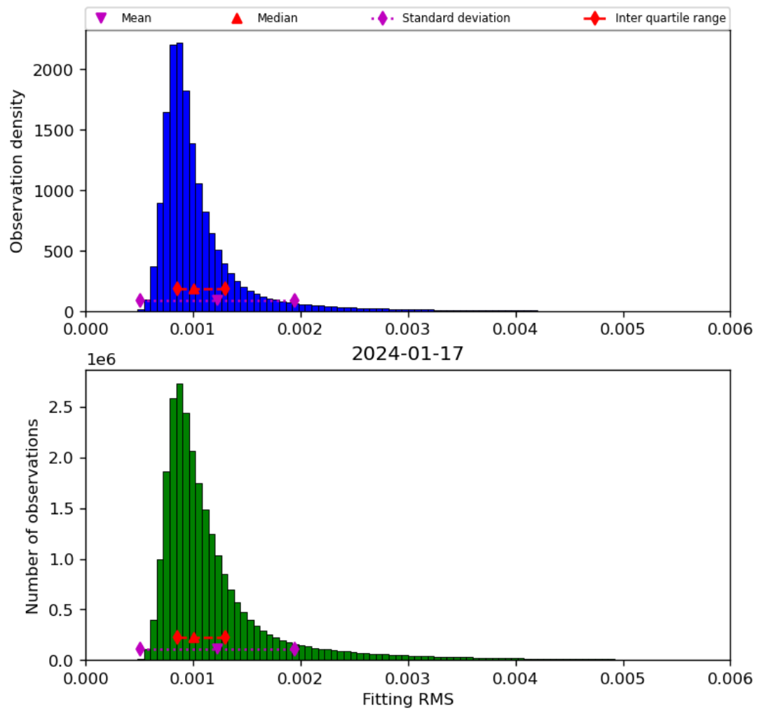
Figure 23: Histogram of “Fitting RMS” for 2024-01-16 to 2024-01-18
