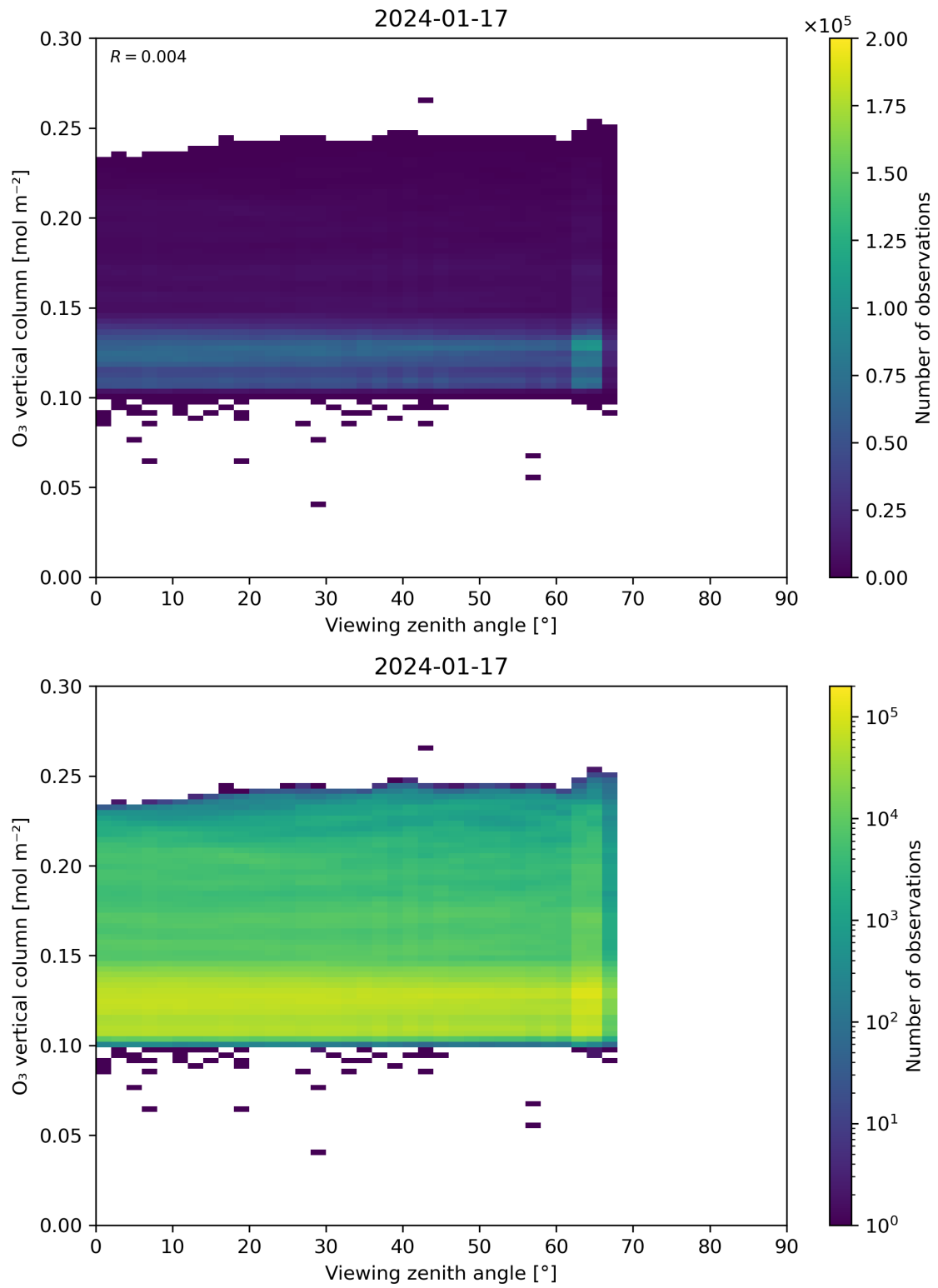
Figure 52: Scatter density plot of “Viewing zenith angle” against “O 3 vertical column” for 2024-01-16 to 2024-01-18.
