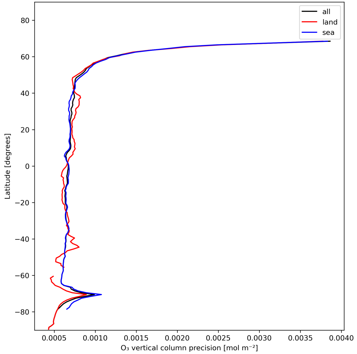
Figure 15: Zonal average of “O 3 vertical column precision” for 2024-01-16 to 2024-01-18.
