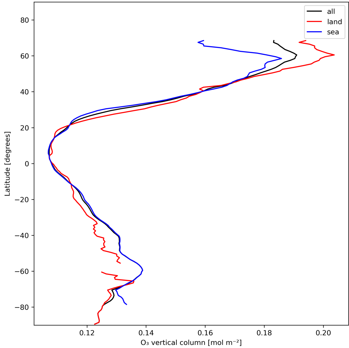
Figure 14: Zonal average of “O 3 vertical column” for 2024-01-16 to 2024-01-18.
