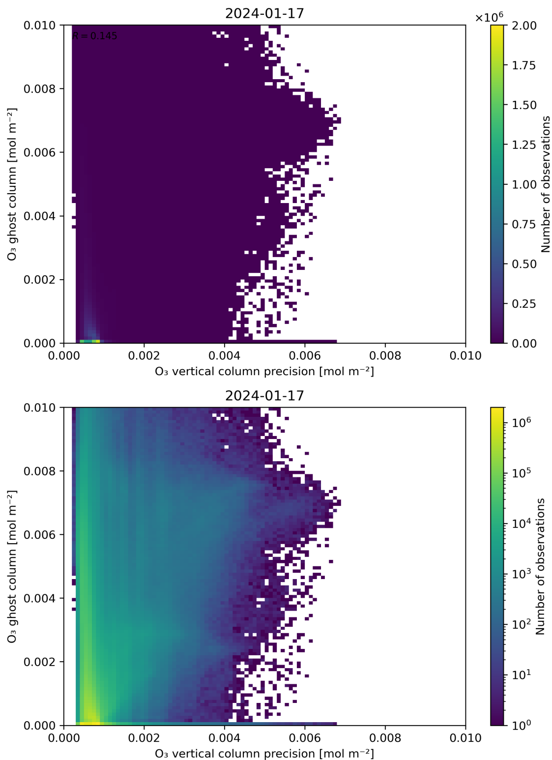
Figure 43: Scatter density plot of “ \text{O}_3 vertical column precision” against “ \text{O}_3 ghost column” for 2024-01-16 to 2024-01-18.
