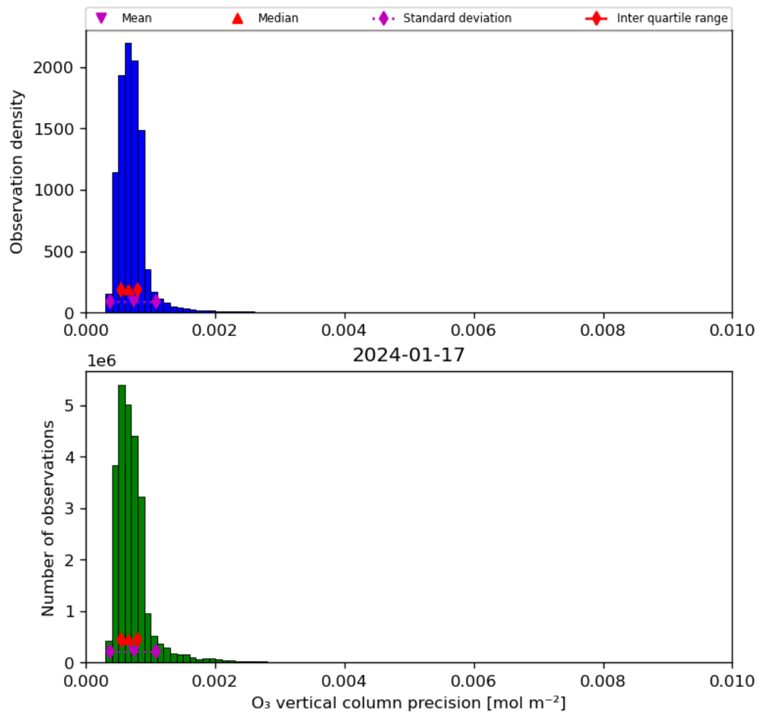
Figure 22: Histogram of “O 3 vertical column precision” for 2024-01-16 to 2024-01-18
