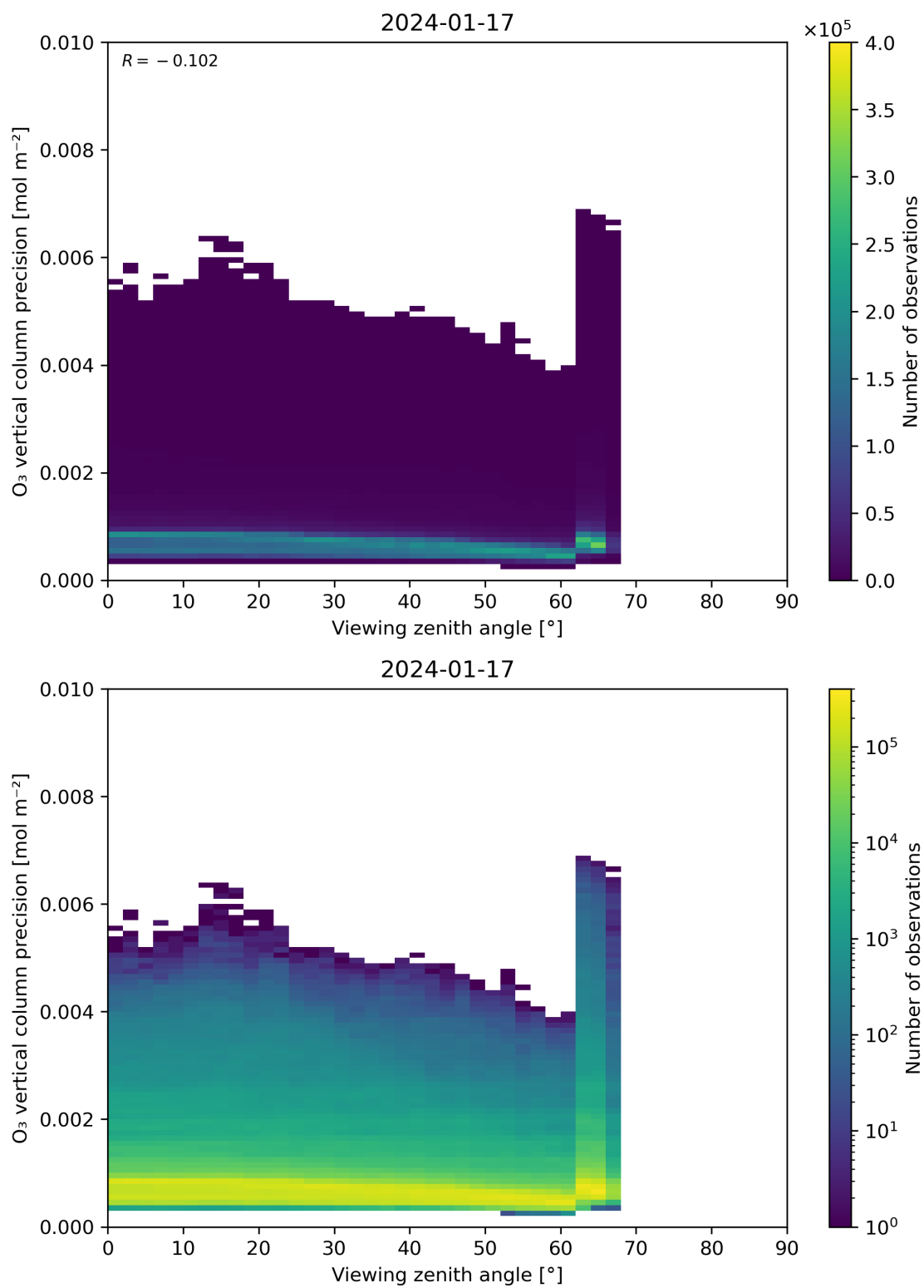
Figure 53: Scatter density plot of “Viewing zenith angle” against “O 3 vertical column precision” for 2024-01-16 to 2024-01-18.
