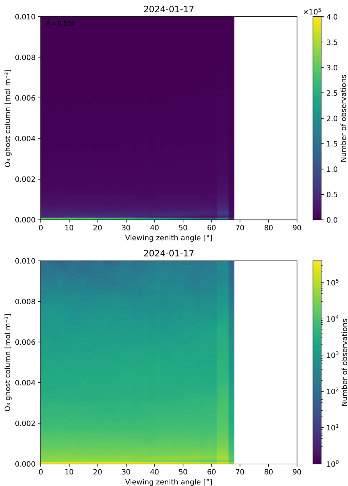
Figure 51: Scatter density plot of “Viewing zenith angle” against “O 3 ghost column” for 2024-01-16 to 2024-01-18.
