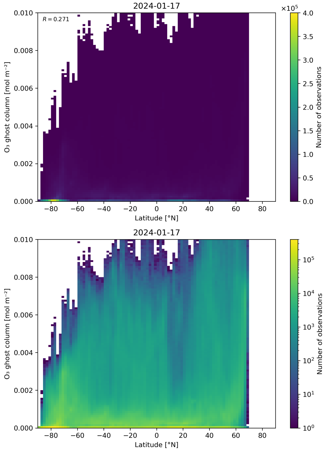
Figure 35: Scatter density plot of “Latitude” against “O 3 ghost column” for 2024-01-16 to 2024-01-18.
