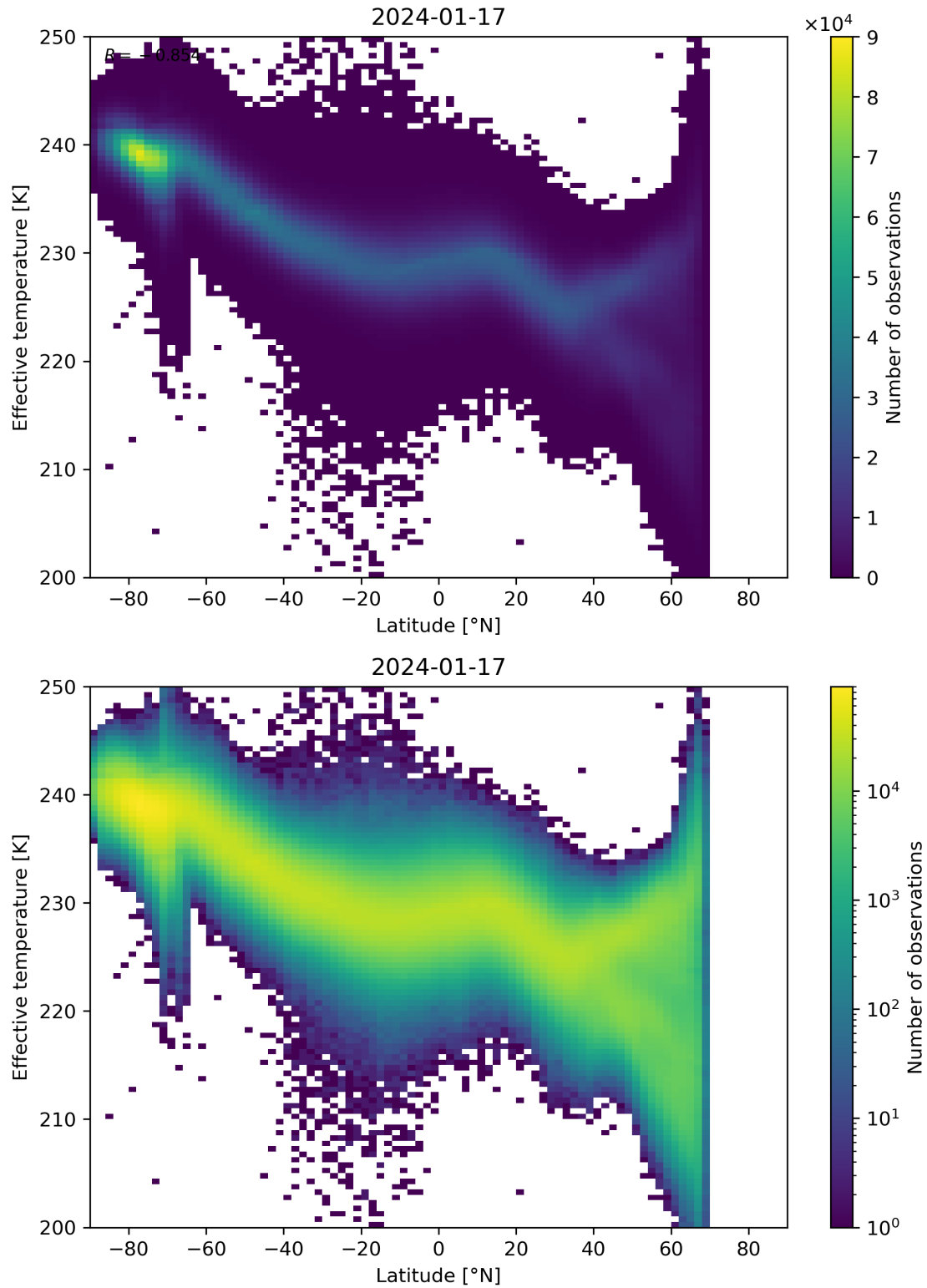
Figure 34: Scatter density plot of “Latitude” against “Effective temperature” for 2024-01-16 to 2024-01-18.
