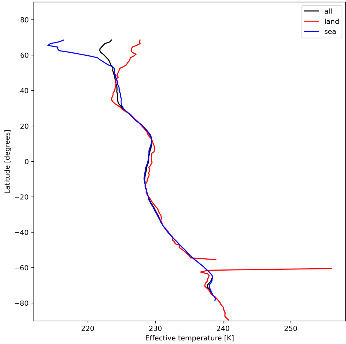
Figure 17: Zonal average of "Effective temperature" for 2024-01-16 to 2024-01-18.
