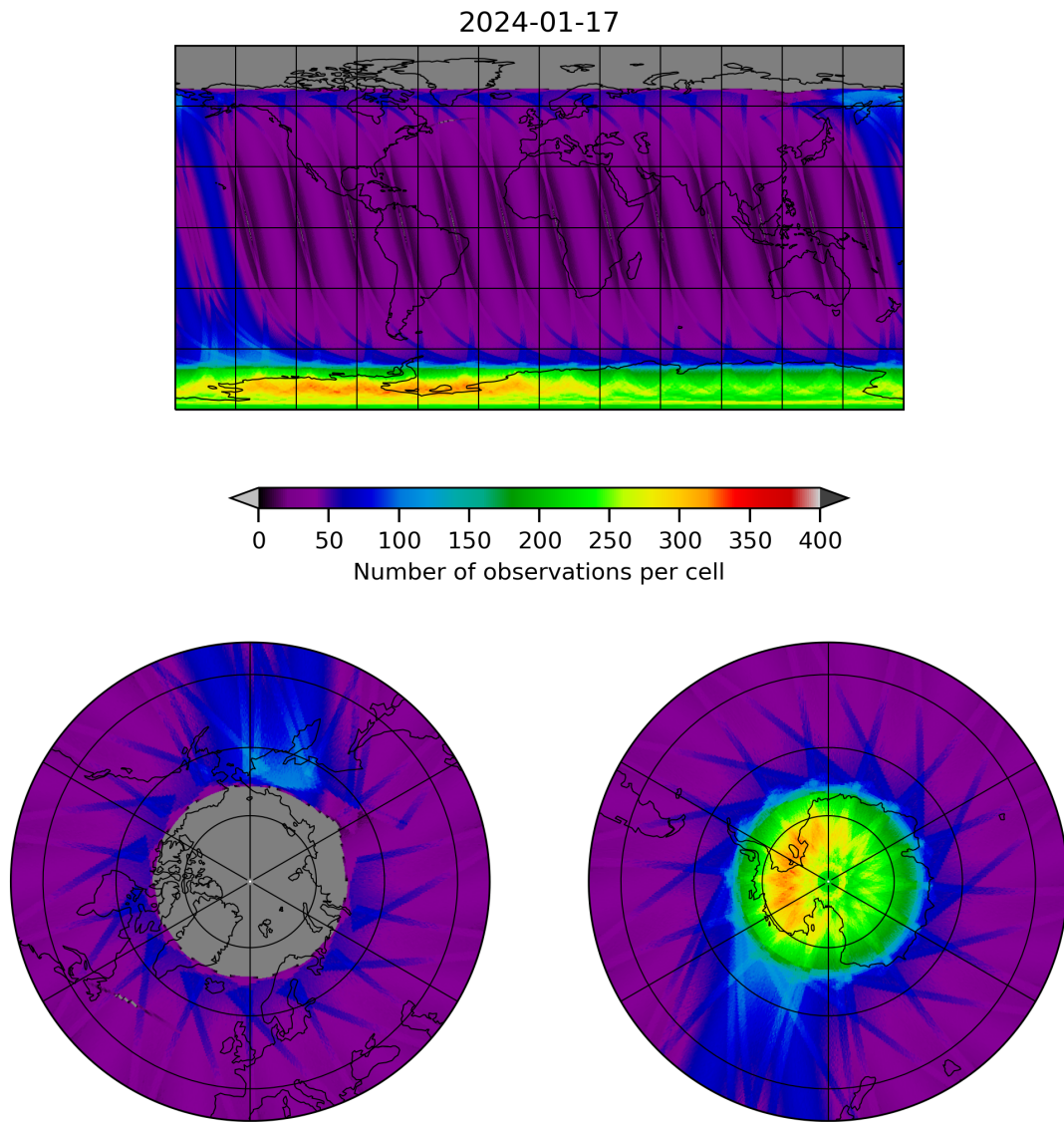
Figure 12: Map of the number of observations for 2024-01-16 to 2024-01-18
