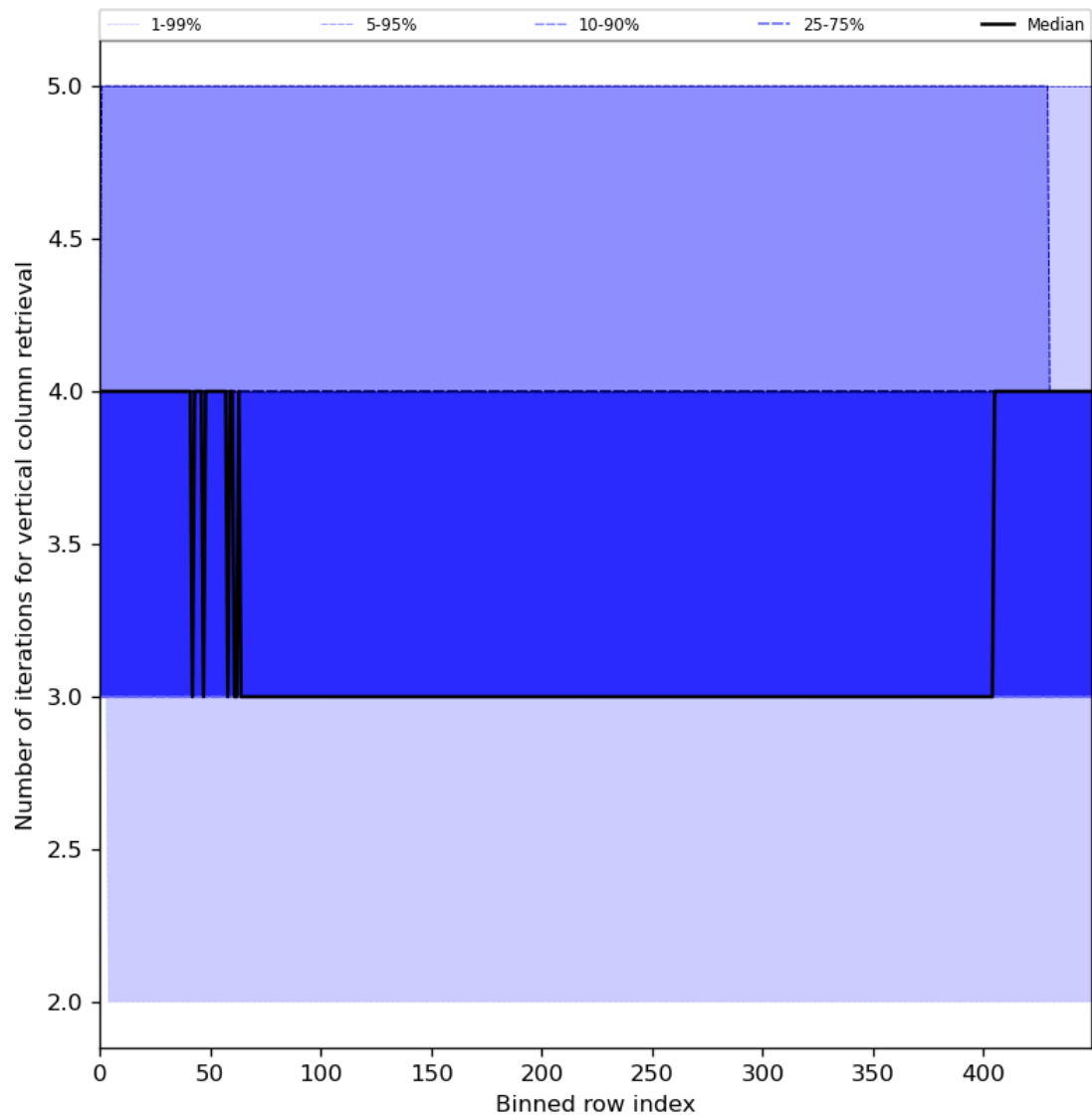
Figure 33: Along track statistics of “Number of iterations for vertical column retrieval” for 2024-01-16 to 2024-01-18
