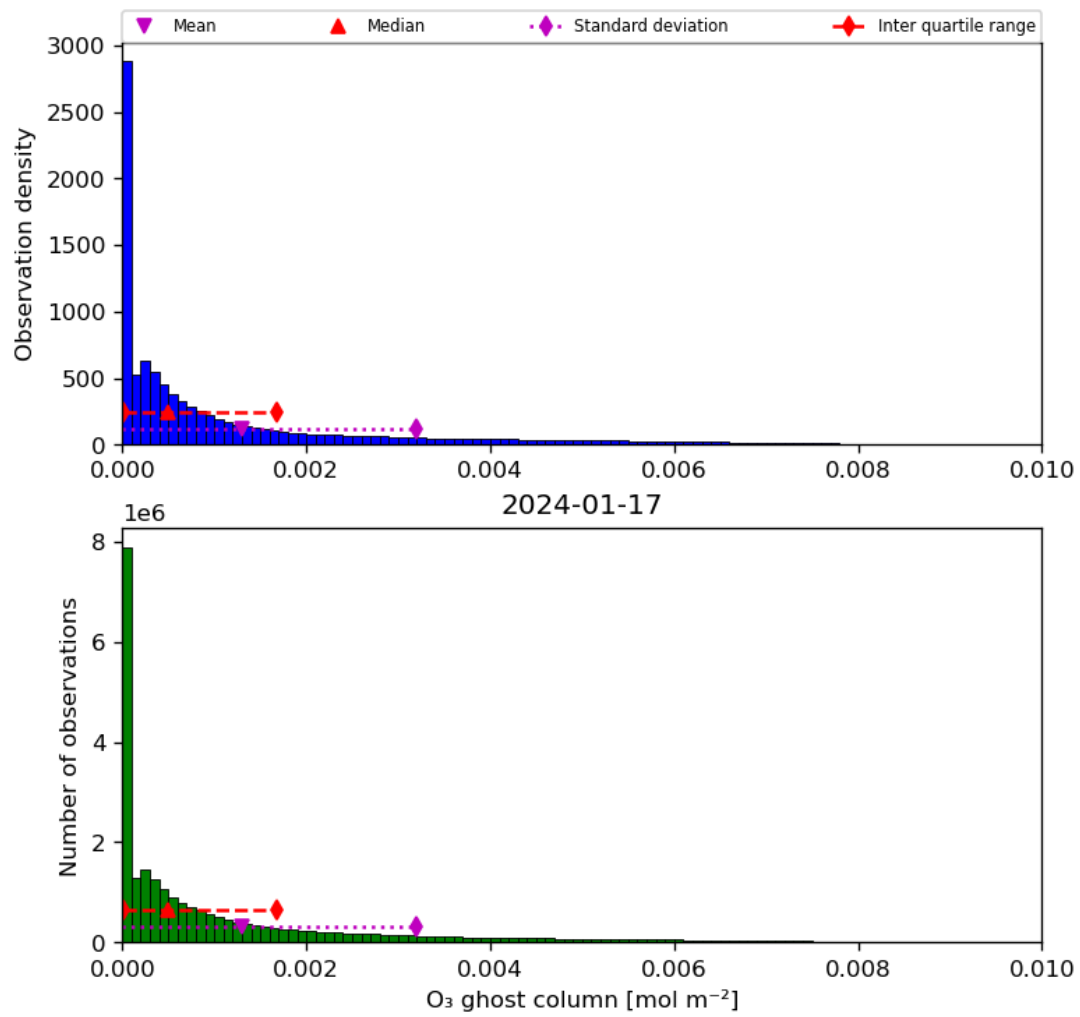
Figure 25: Histogram of “O 3 ghost column” for 2024-01-16 to 2024-01-18
