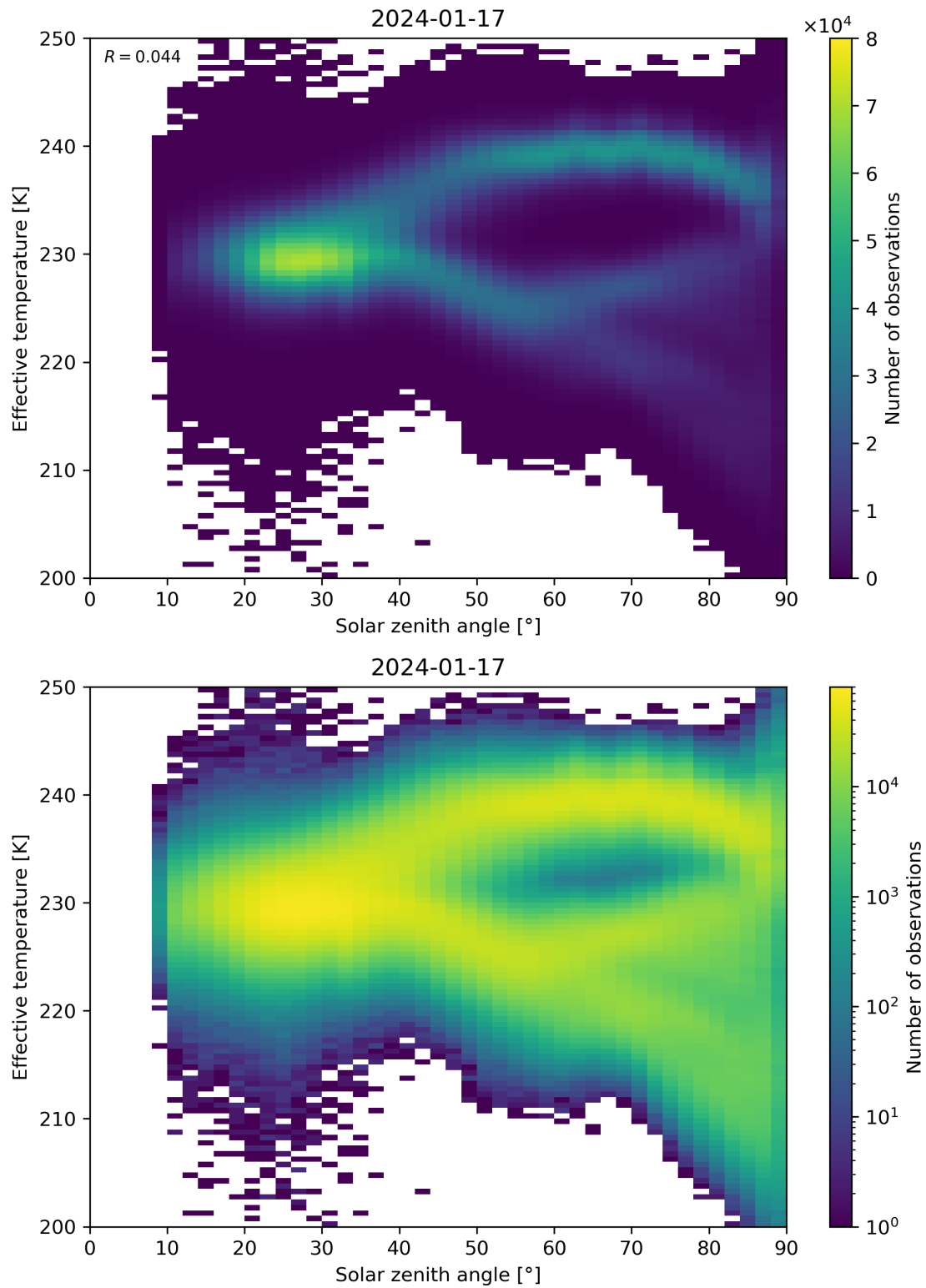
Figure 45: Scatter density plot of “Solar zenith angle” against “Effective temperature” for 2024-01-16 to 2024-01-18.
