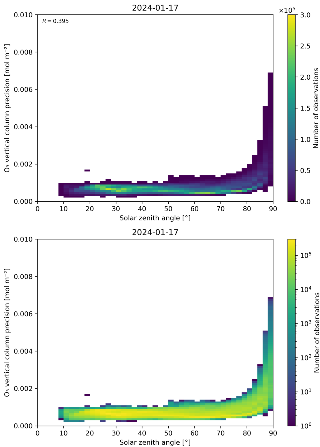
Figure 48: Scatter density plot of “Solar zenith angle” against “O 3 vertical column precision” for 2024-01-16 to 2024-01-18.
