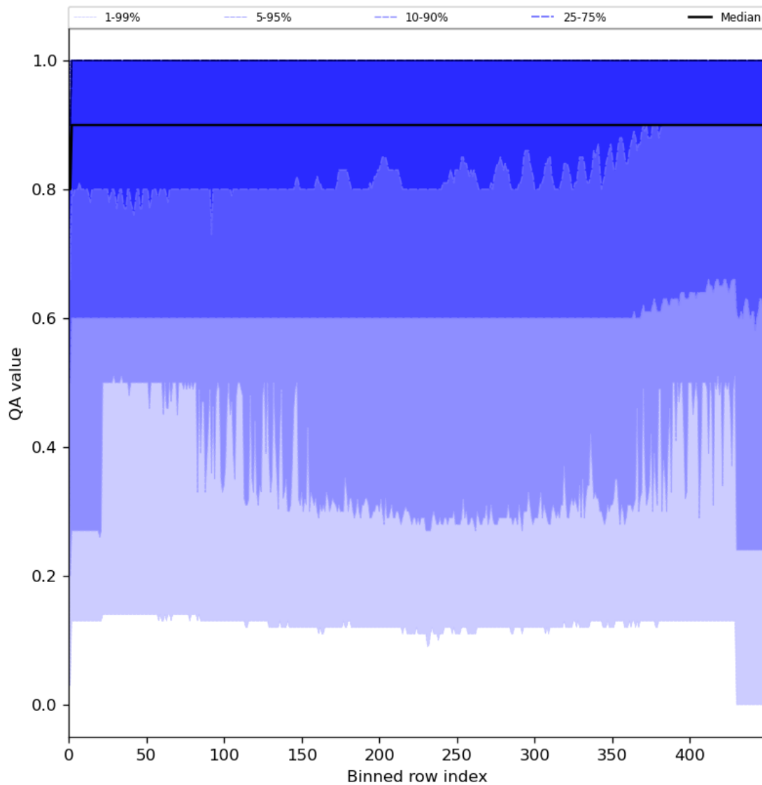
Figure 27: Along track statistics of “QA value” for 2024-01-16 to 2024-01-18
