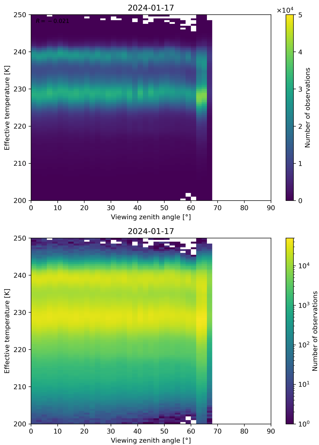
Figure 50: Scatter density plot of “Viewing zenith angle” against “Effective temperature” for 2024-01-16 to 2024-01-18.
