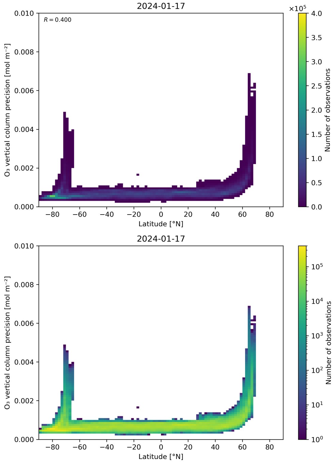
Figure 37: Scatter density plot of “Latitude” against “O 3 vertical column precision” for 2024-01-16 to 2024-01-18.
