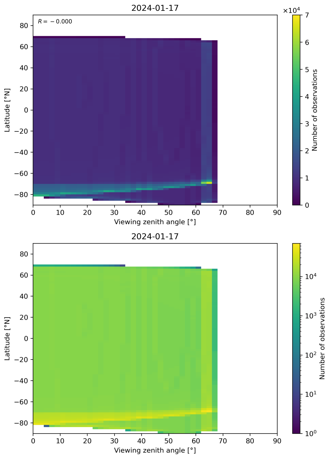
Figure 49: Scatter density plot of “Viewing zenith angle” against “Latitude” for 2024-01-16 to 2024-01-18.
