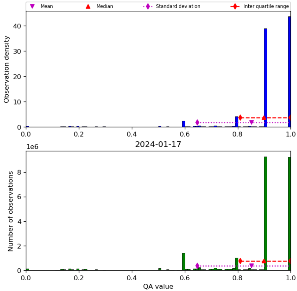
Figure 20: Histogram of “QA value” for 2024-01-16 to 2024-01-18
