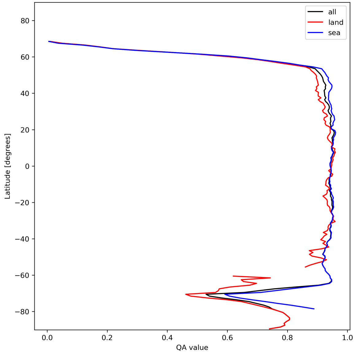
Figure 13: Zonal average of “QA value” for 2024-01-16 to 2024-01-18.
