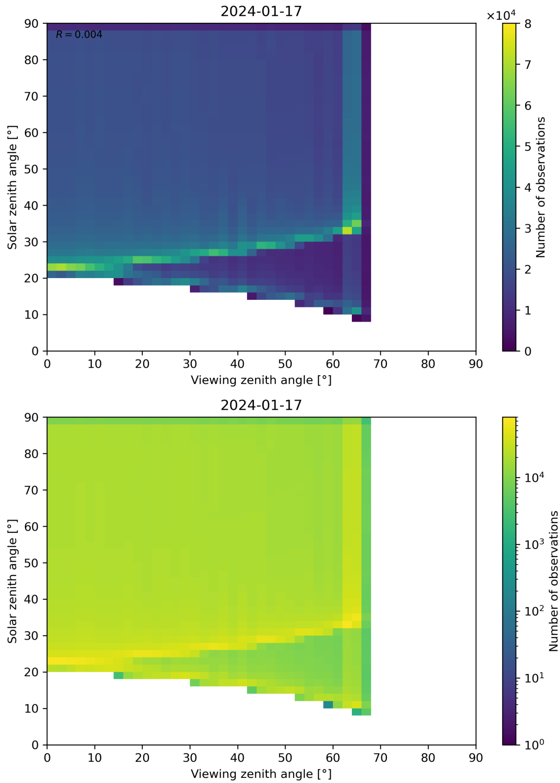
Figure 54: Scatter density plot of “Viewing zenith angle” against “Solar zenith angle” for 2024-01-16 to 2024-01-18.
