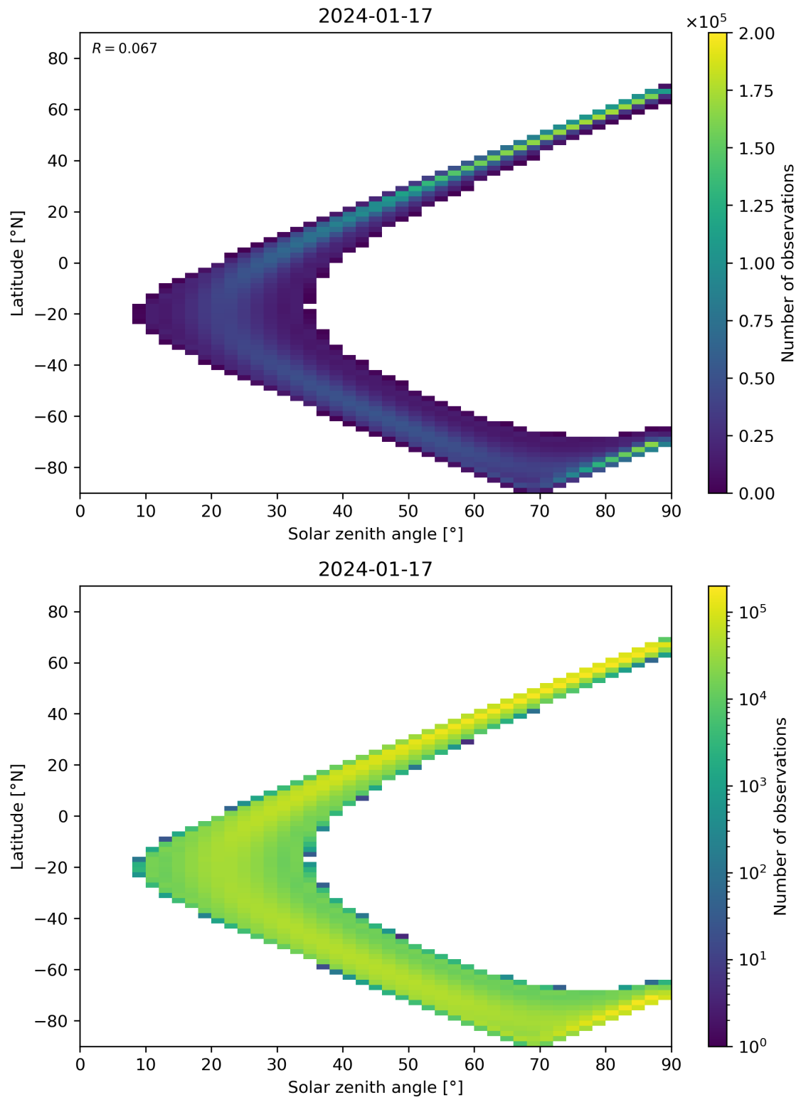
Figure 44: Scatter density plot of “Solar zenith angle” against “Latitude” for 2024-01-16 to 2024-01-18.
