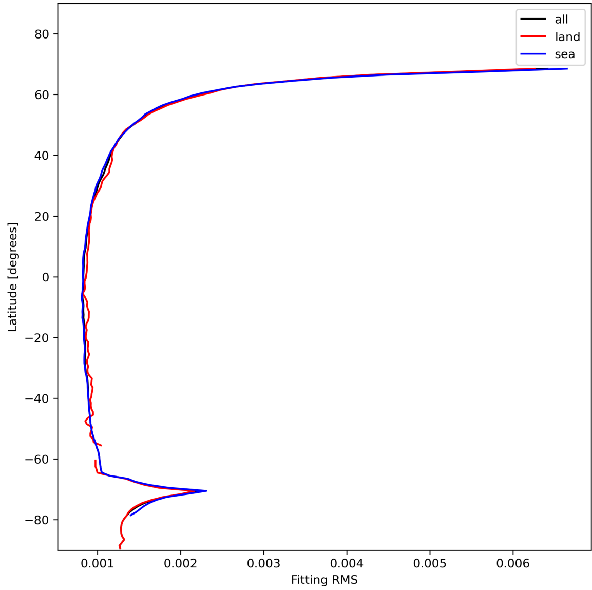
Figure 16: Zonal average of “Fitting RMS” for 2024-01-16 to 2024-01-18.
