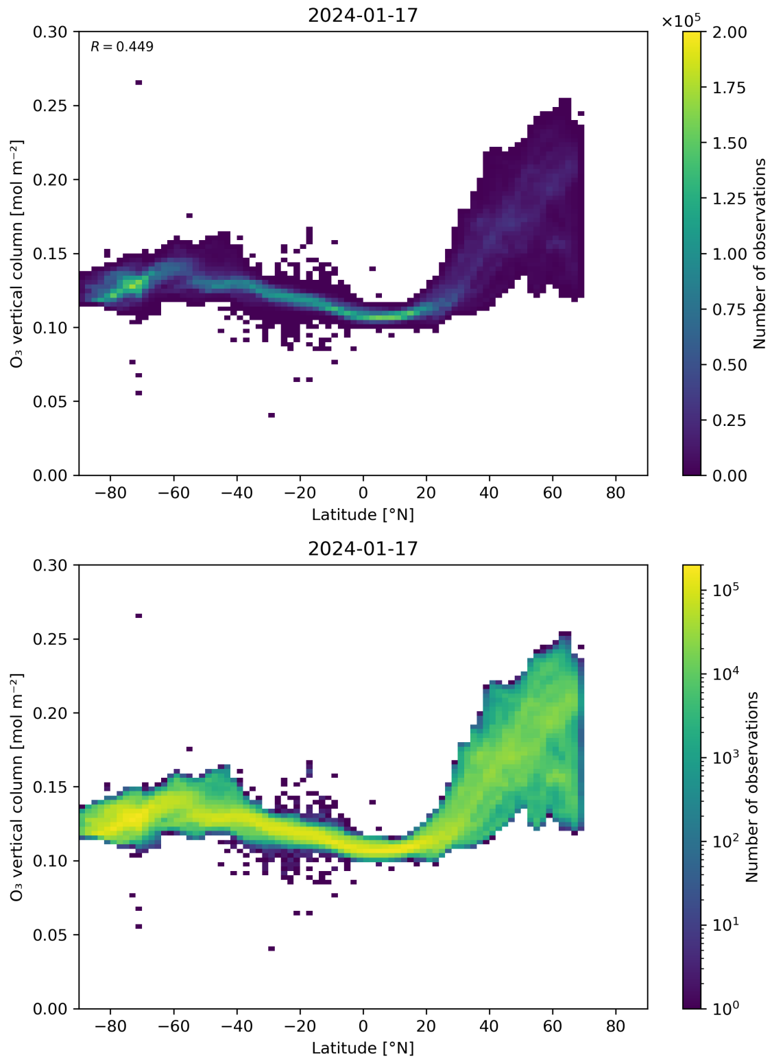
Figure 36: Scatter density plot of “Latitude” against “O 3 vertical column” for 2024-01-16 to 2024-01-18.
