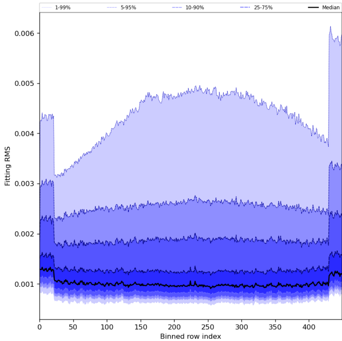
Figure 30: Along track statistics of “Fitting RMS” for 2024-01-16 to 2024-01-18
