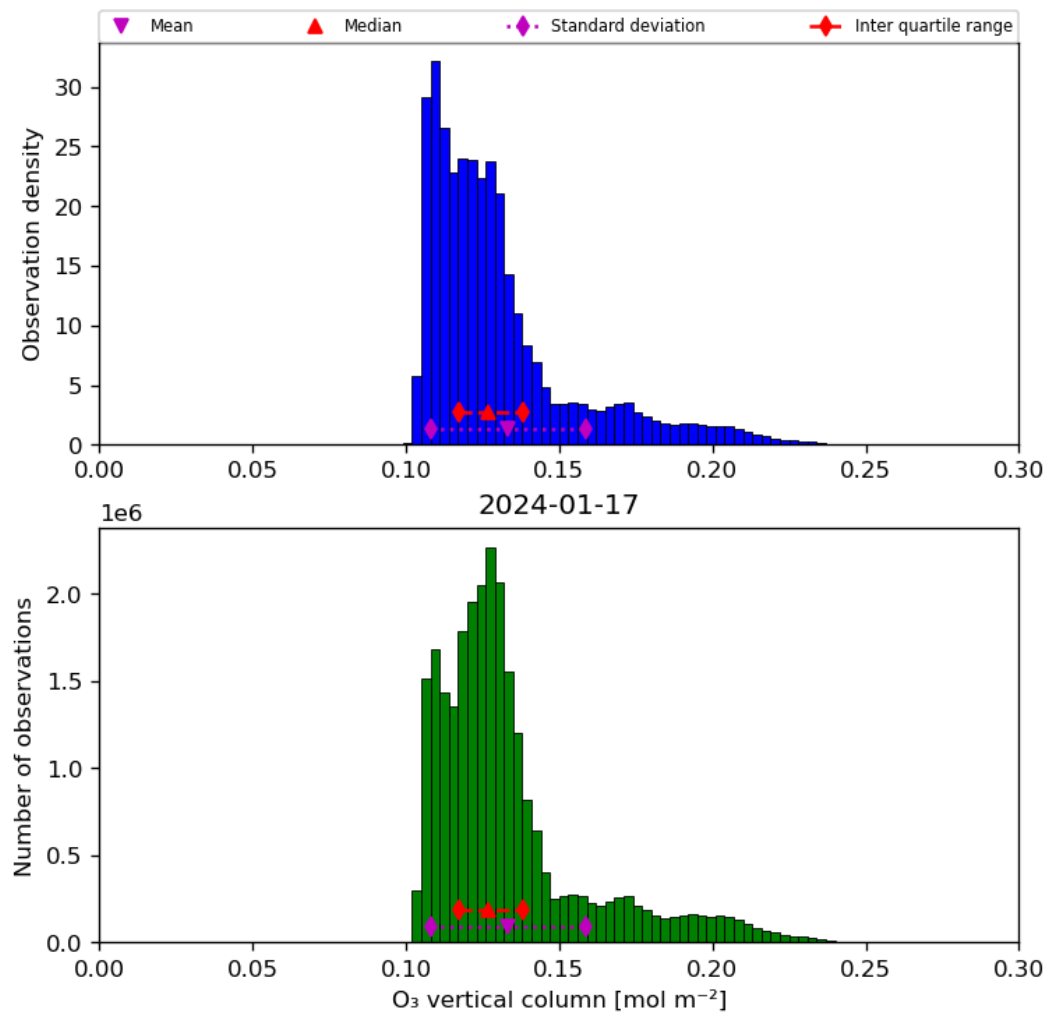
Figure 21: Histogram of “O 3 vertical column” for 2024-01-16 to 2024-01-18
