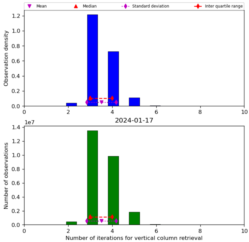
Figure 26: Histogram of “Number of iterations for vertical column retrieval” for 2024-01-16 to 2024-01-18
