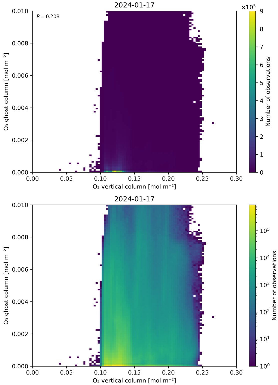
Figure 40: Scatter density plot of “O 3 vertical column” against “O 3 ghost column” for 2024-01-16 to 2024-01-18.
