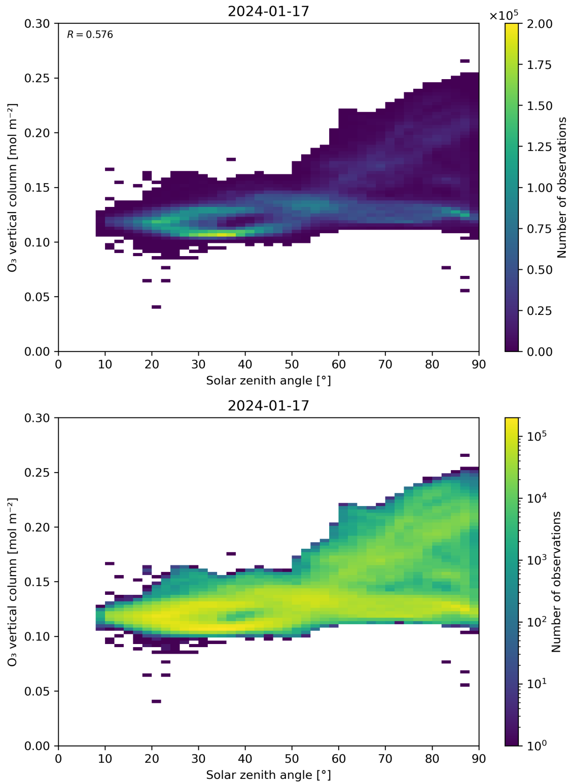
Figure 47: Scatter density plot of “Solar zenith angle” against “O 3 vertical column” for 2024-01-16 to 2024-01-18.
