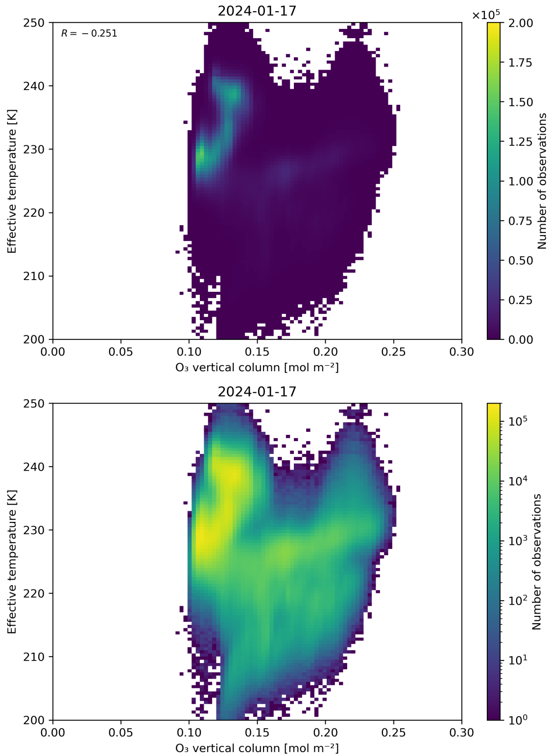
Figure 39: Scatter density plot of “O 3 vertical column” against “Effective temperature” for 2024-01-16 to 2024-01-18.
