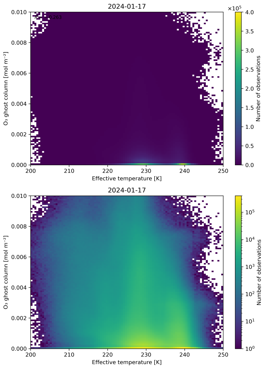
Figure 38: Scatter density plot of “Effective temperature” against “O 3 ghost column” for 2024-01-16 to 2024-01-18.
