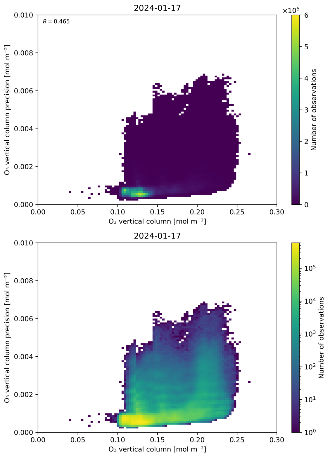
Figure 41: Scatter density plot of “O 3 vertical column” against “O 3 vertical column precision” for 2024-01-16 to 2024-01-18.
