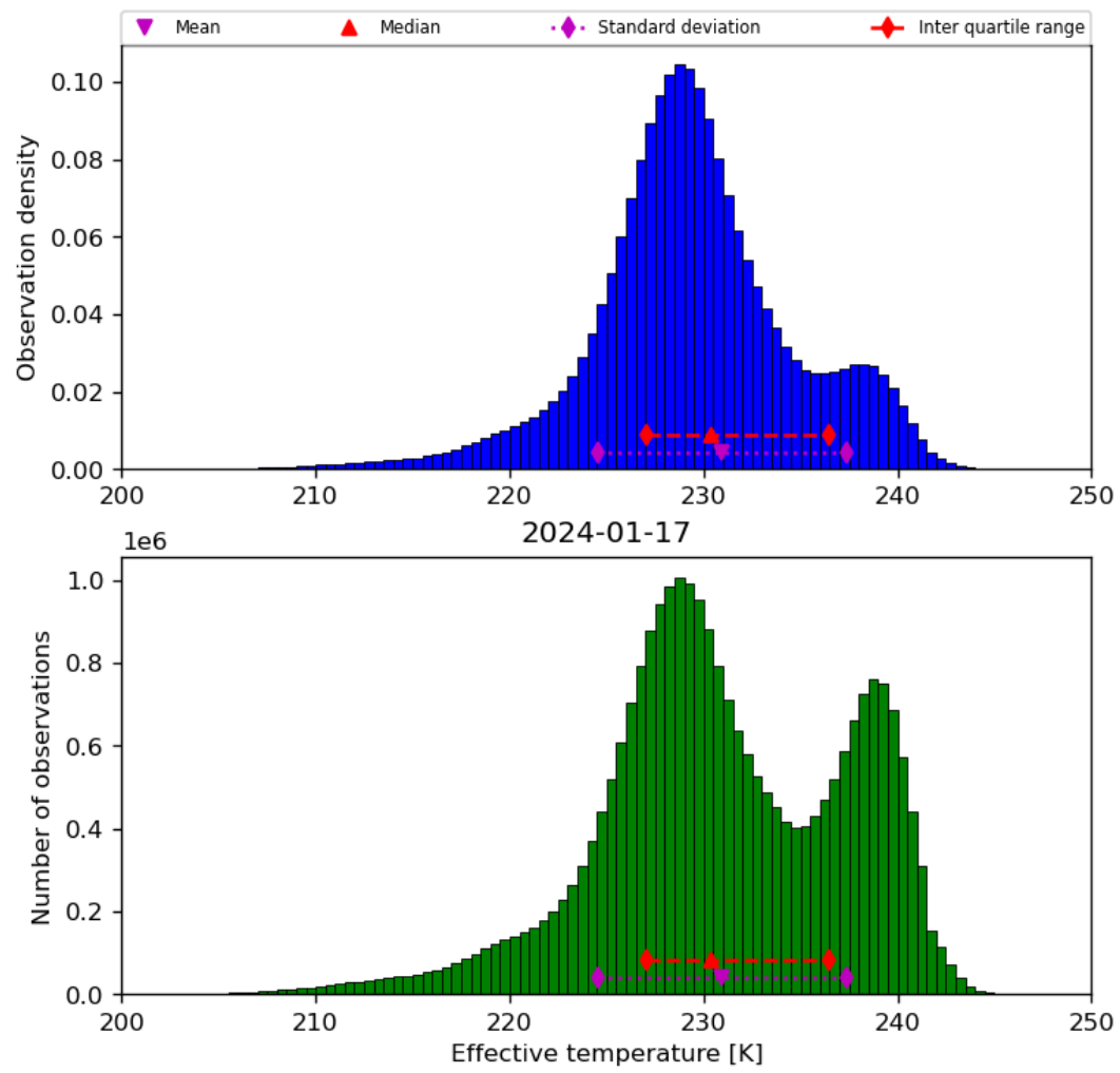
Figure 24: Histogram of “Effective temperature” for 2024-01-16 to 2024-01-18
