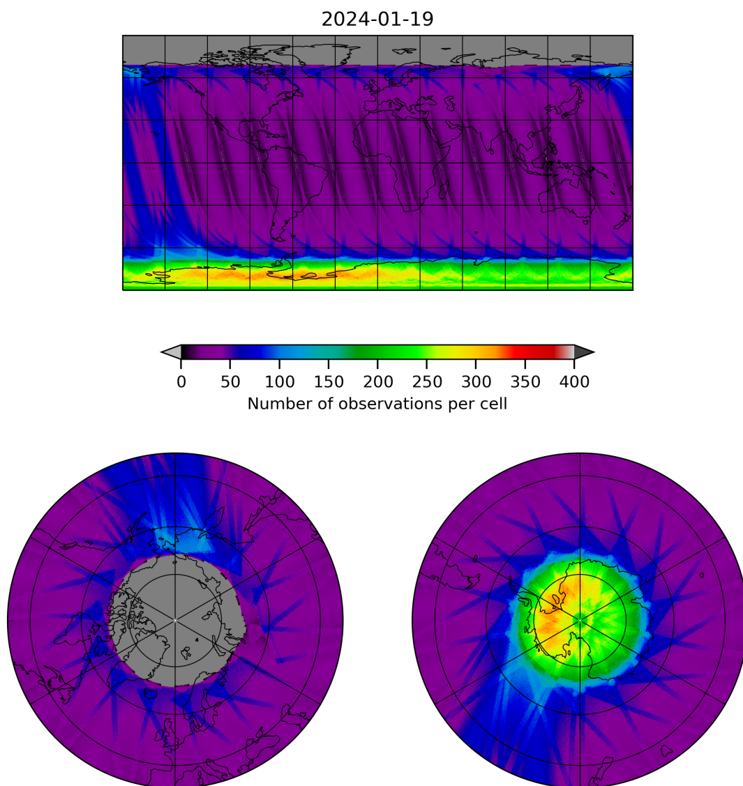
Figure 12: Map of the number of observations for 2024-01-18 to 2024-01-20
