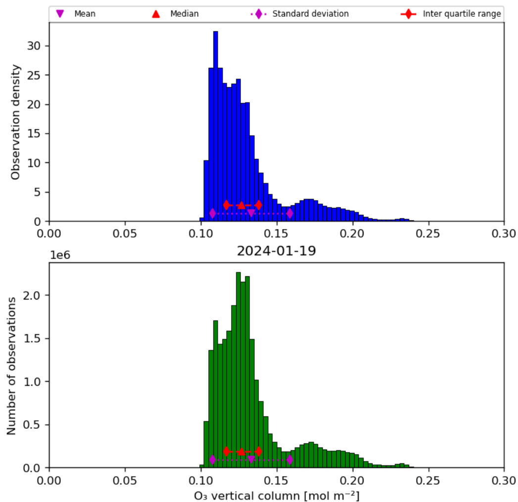
Figure 21: Histogram of “O 3 vertical column” for 2024-01-18 to 2024-01-20
