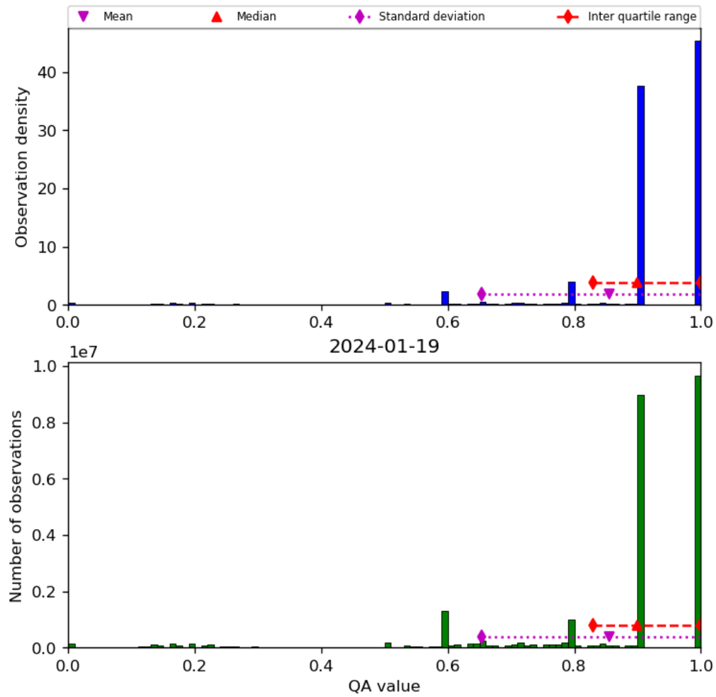
Figure 20: Histogram of “QA value” for 2024-01-18 to 2024-01-20
