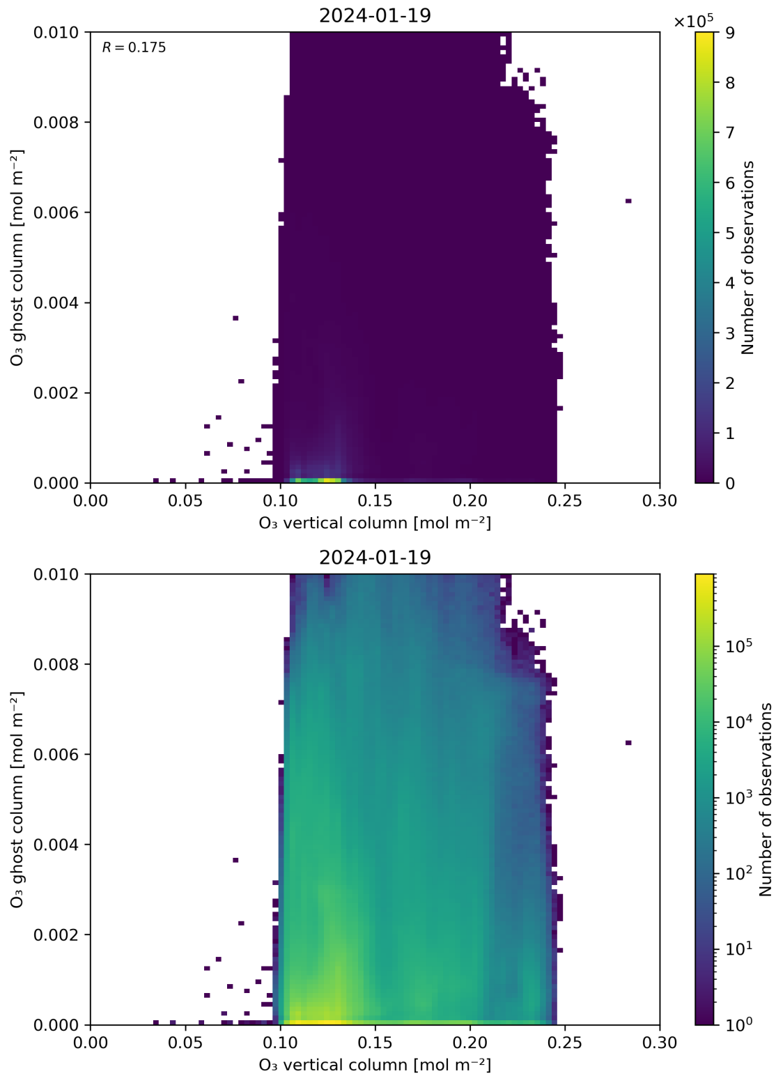
Figure 40: Scatter density plot of “O 3 vertical column” against “O 3 ghost column” for 2024-01-18 to 2024-01-20.
