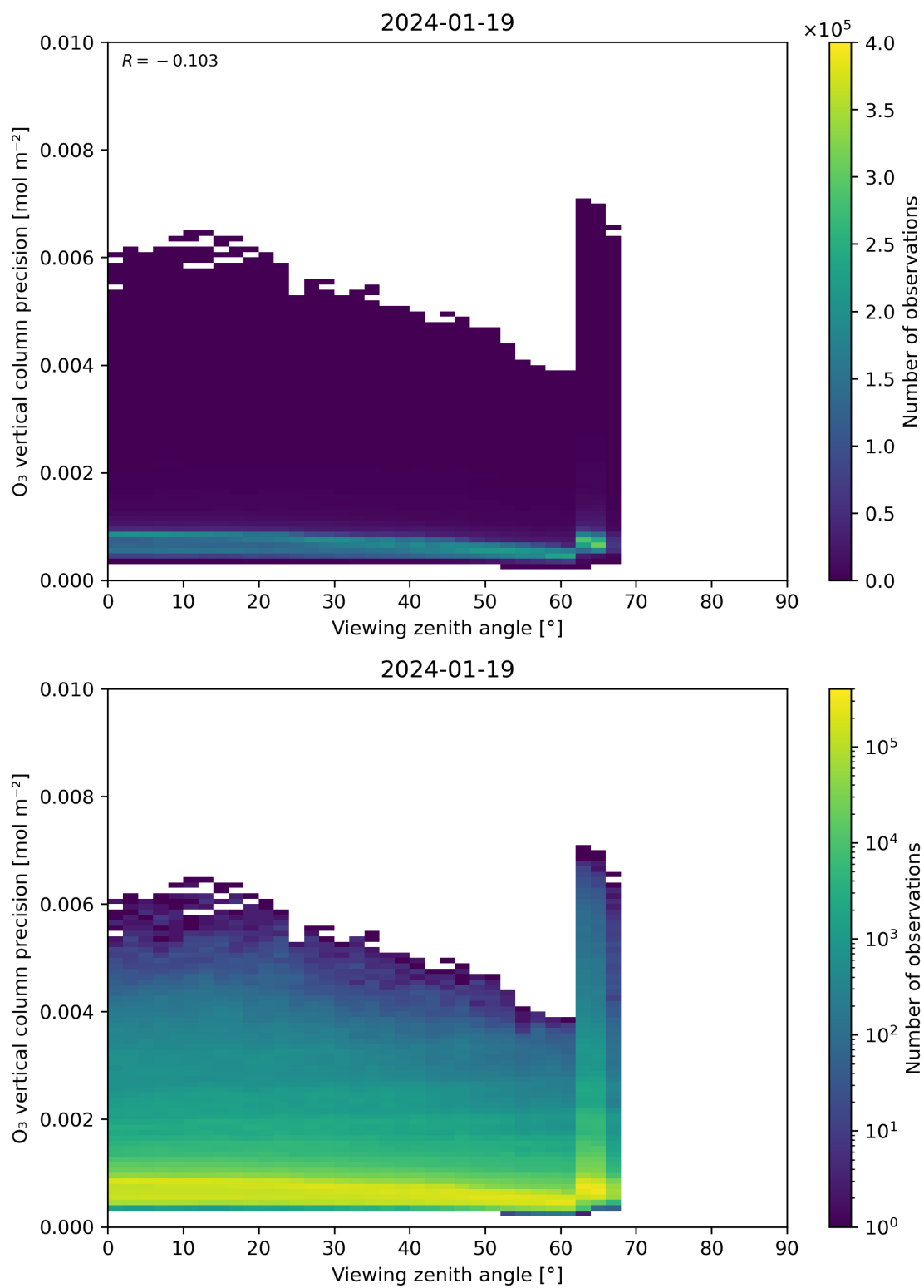
Figure 53: Scatter density plot of “Viewing zenith angle” against “O 3 vertical column precision” for 2024-01-18 to 2024-01-20.
