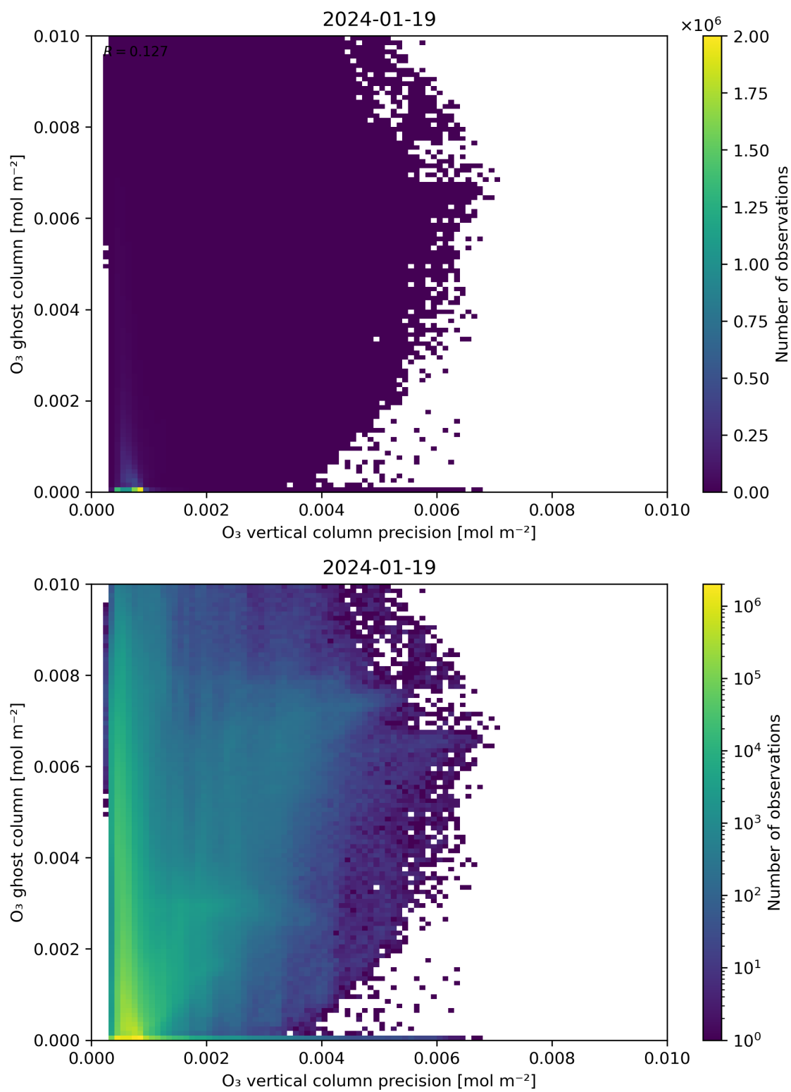
Figure 43: Scatter density plot of “ \text{O}_3 vertical column precision” against “ \text{O}_3 ghost column” for 2024-01-18 to 2024-01-20.
