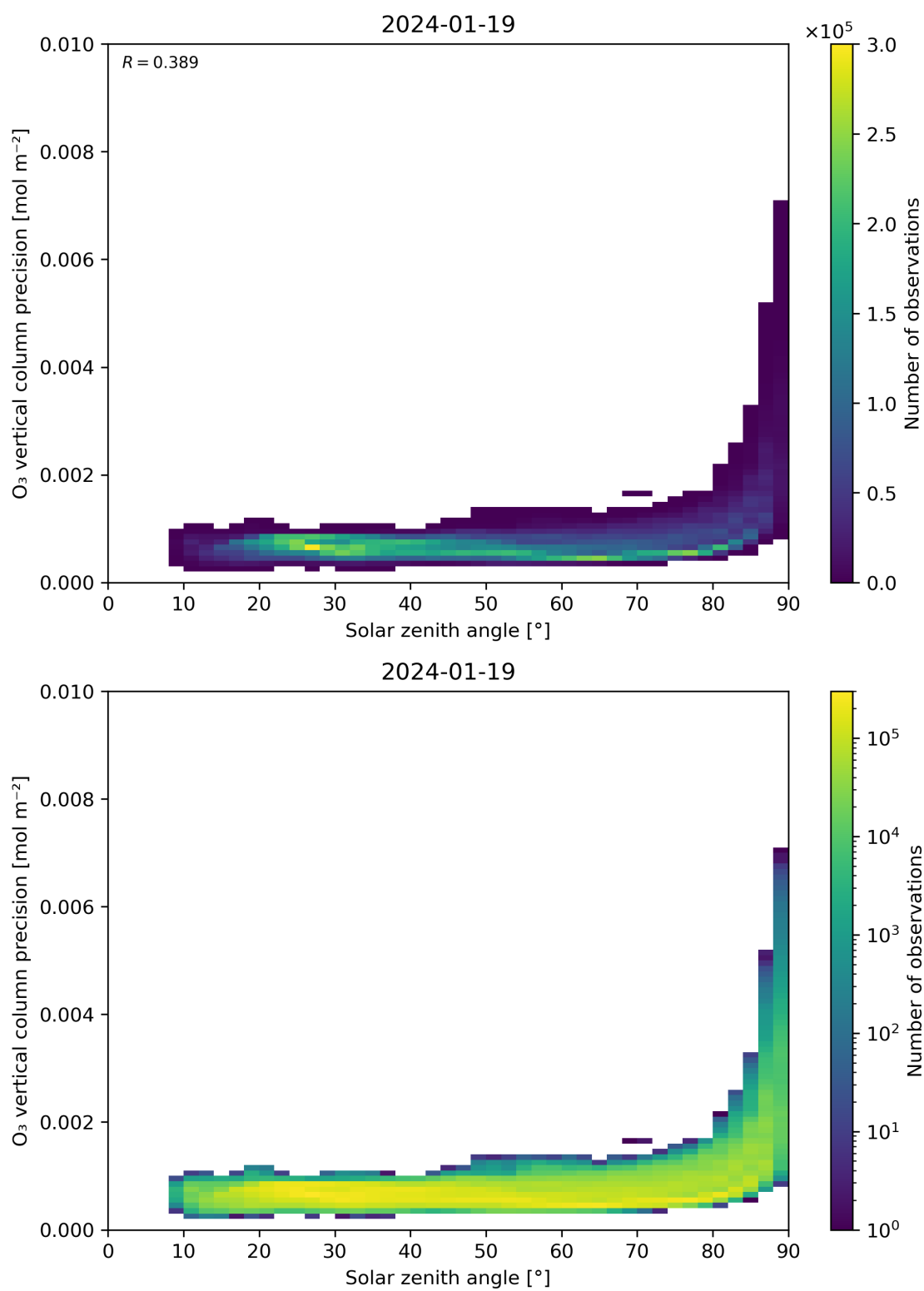
Figure 48: Scatter density plot of “Solar zenith angle” against “O 3 vertical column precision” for 2024-01-18 to 2024-01-20.
