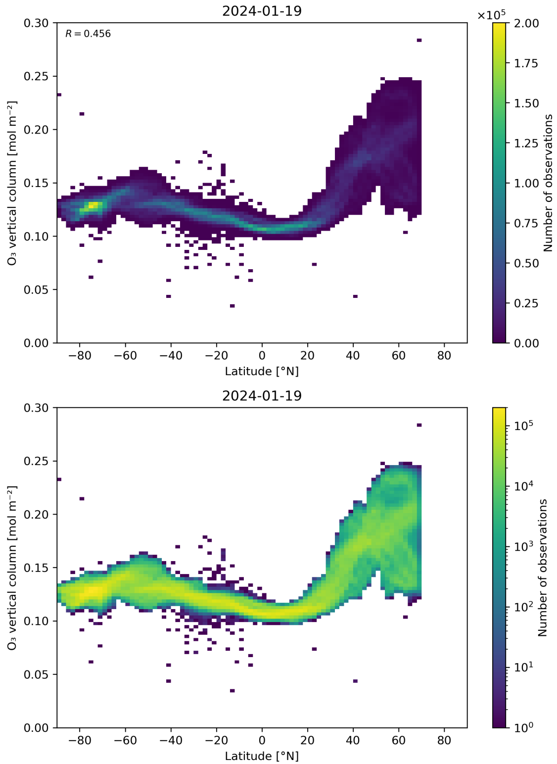
Figure 36: Scatter density plot of “Latitude” against “O 3 vertical column” for 2024-01-18 to 2024-01-20.
