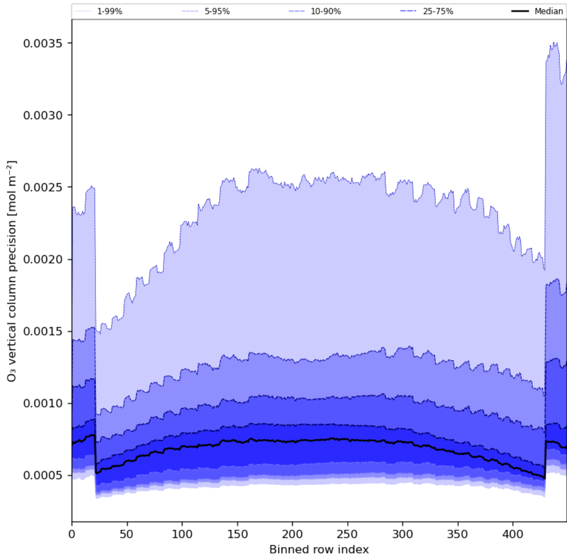
Figure 29: Along track statistics of “O 3 vertical column precision” for 2024-01-18 to 2024-01-20
