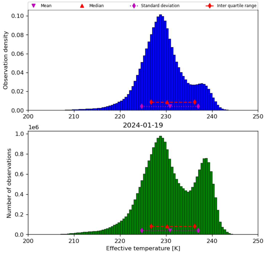
Figure 24: Histogram of “Effective temperature” for 2024-01-18 to 2024-01-20
