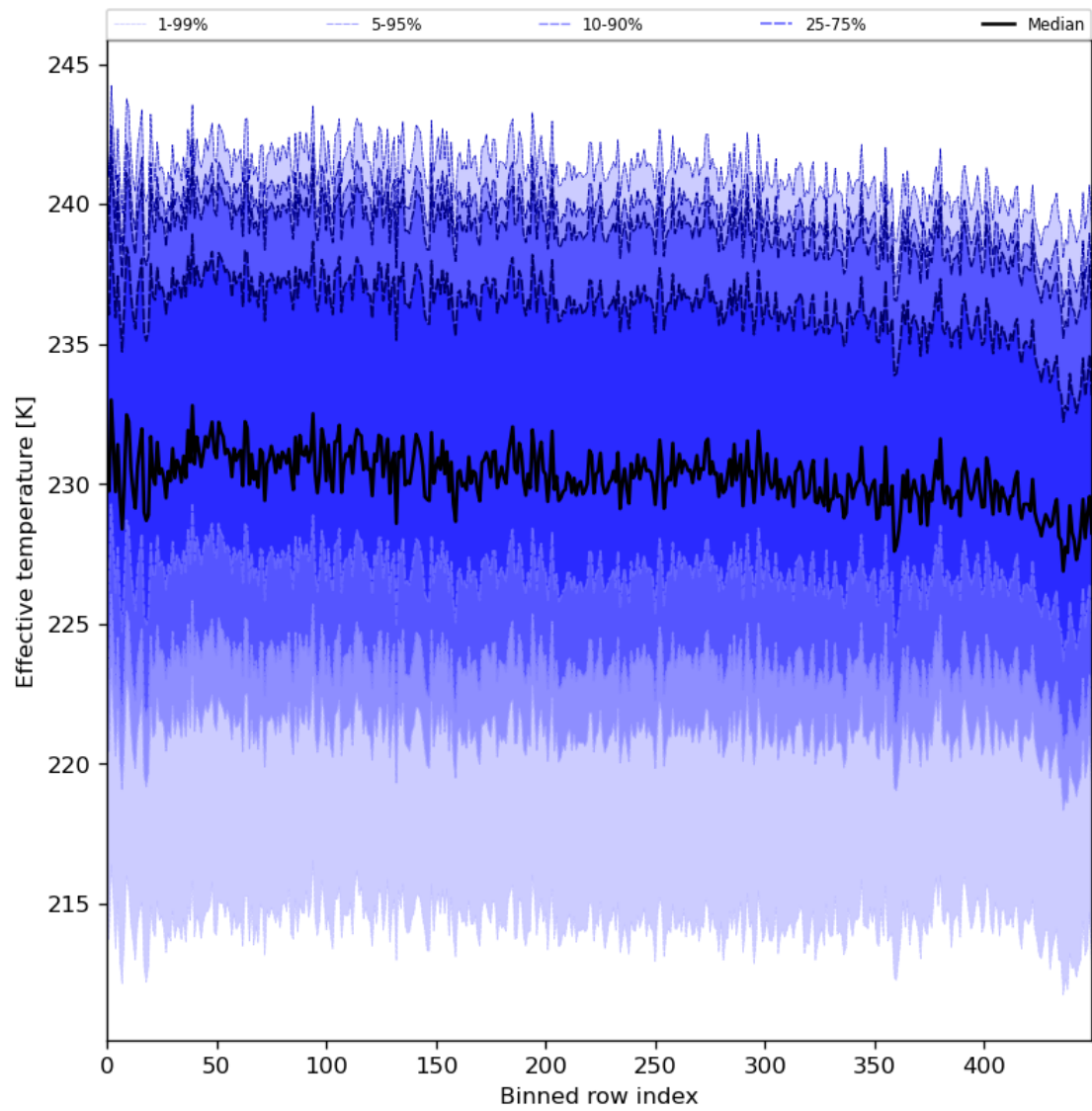
Figure 31: Along track statistics of “Effective temperature” for 2024-01-18 to 2024-01-20
