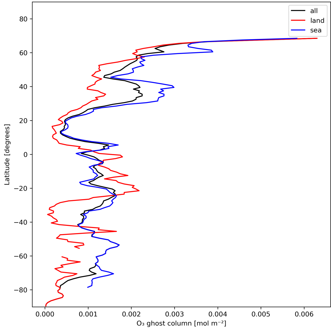
Figure 18: Zonal average of “O 3 ghost column” for 2024-01-18 to 2024-01-20.
