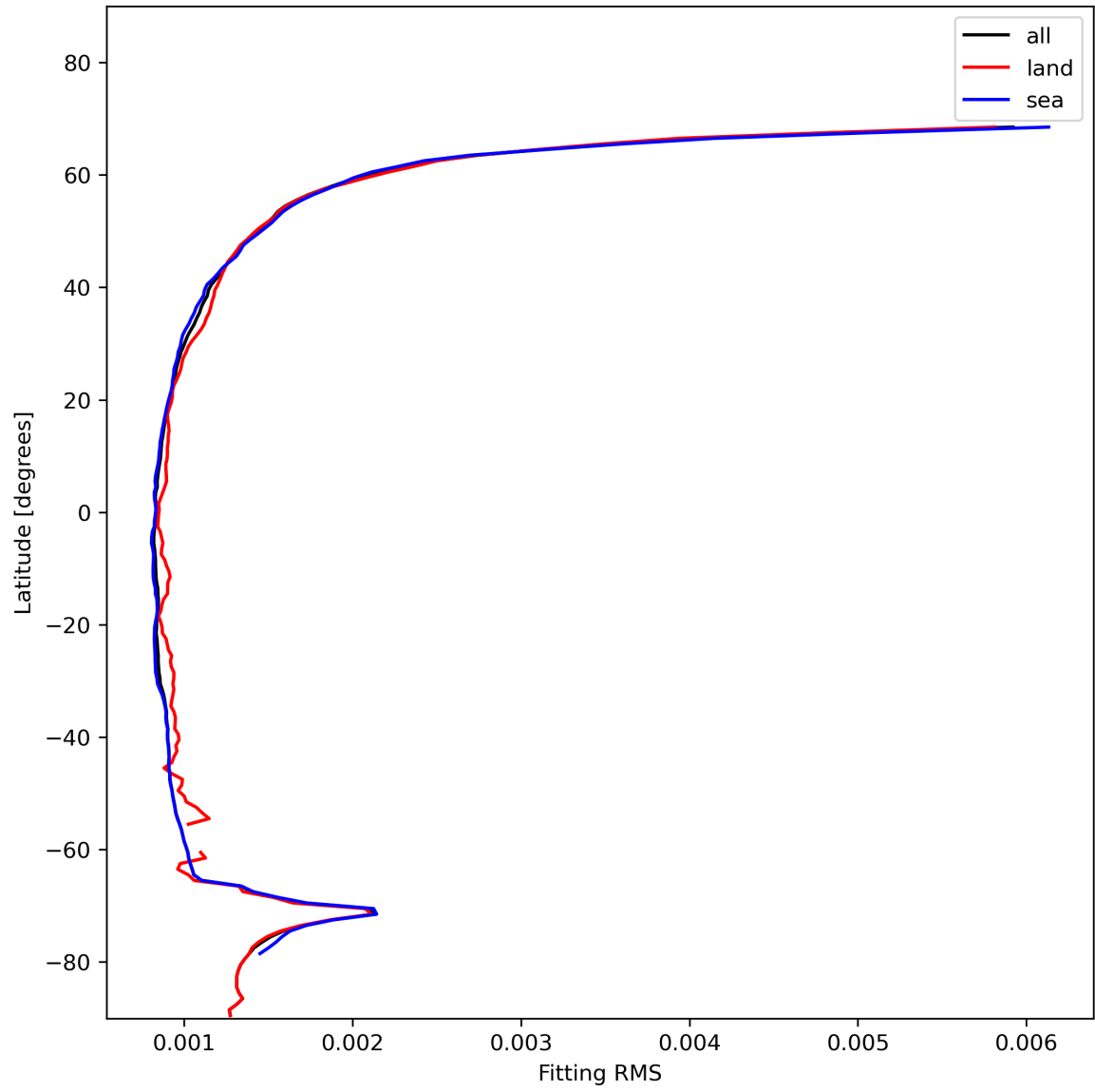
Figure 16: Zonal average of “Fitting RMS” for 2024-01-18 to 2024-01-20.
