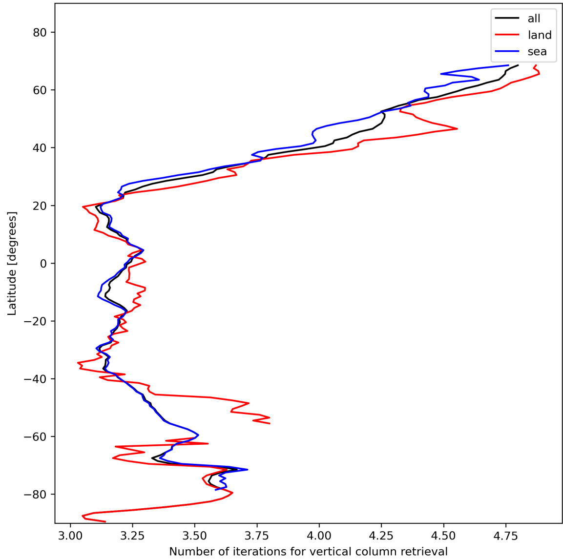
Figure 19: Zonal average of “Number of iterations for vertical column retrieval” for 2024-01-18 to 2024-01-20.
