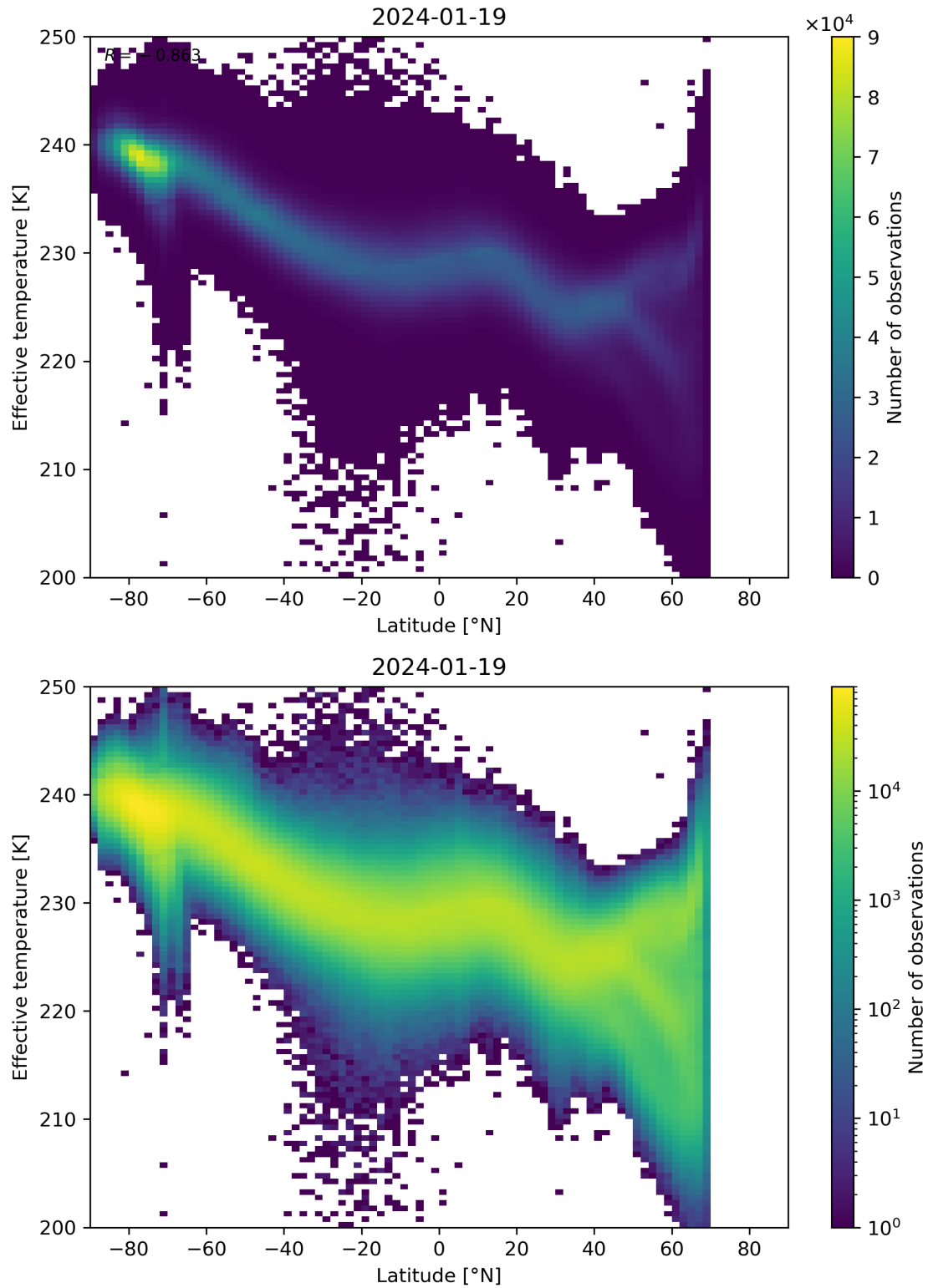
Figure 34: Scatter density plot of “Latitude” against “Effective temperature” for 2024-01-18 to 2024-01-20.
