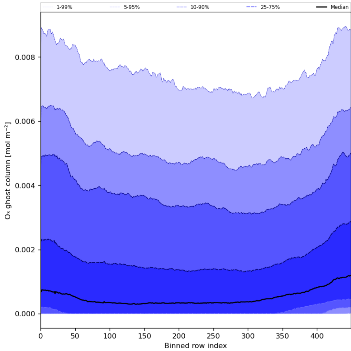
Figure 32: Along track statistics of “O 3 ghost column” for 2024-01-18 to 2024-01-20
