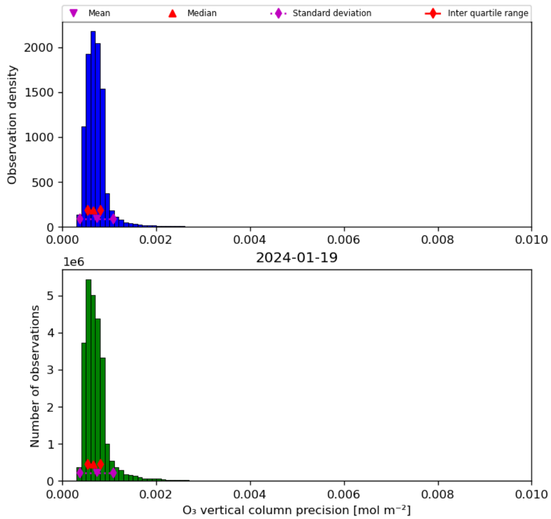
Figure 22: Histogram of “O 3 vertical column precision” for 2024-01-18 to 2024-01-20
