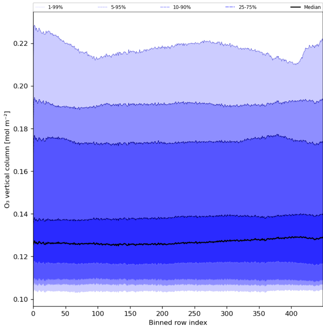
Figure 28: Along track statistics of “O 3 vertical column” for 2024-01-18 to 2024-01-20
