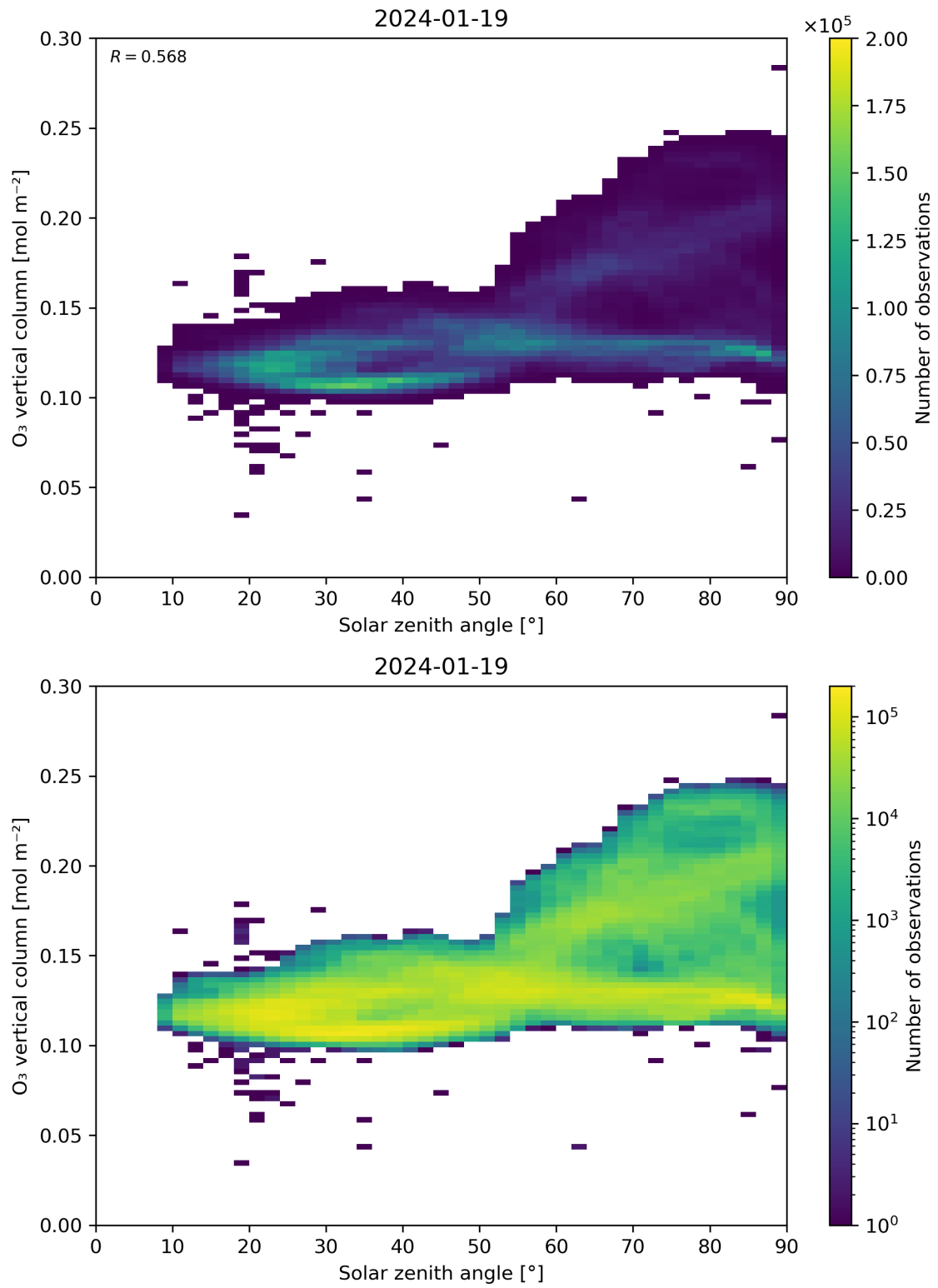
Figure 47: Scatter density plot of “Solar zenith angle” against “O 3 vertical column” for 2024-01-18 to 2024-01-20.
