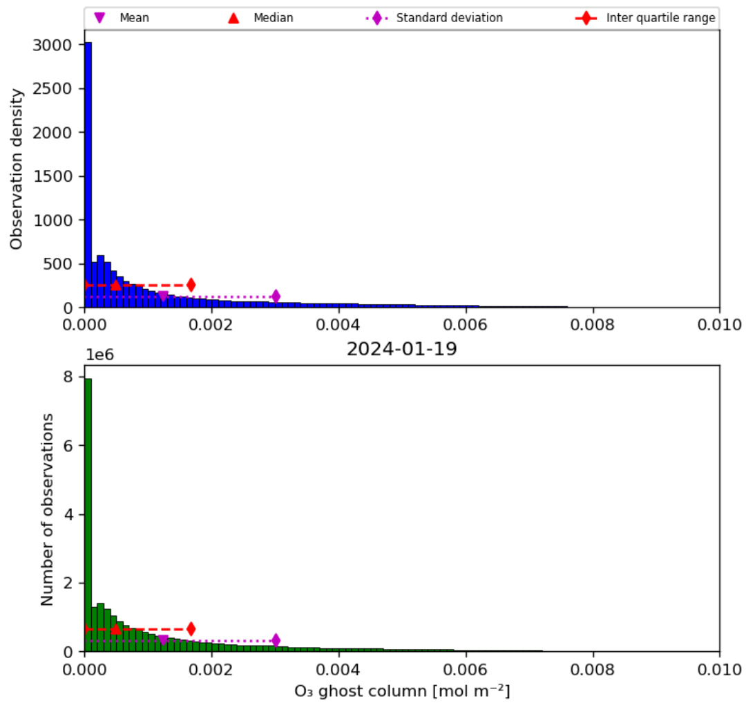
Figure 25: Histogram of “O 3 ghost column” for 2024-01-18 to 2024-01-20
