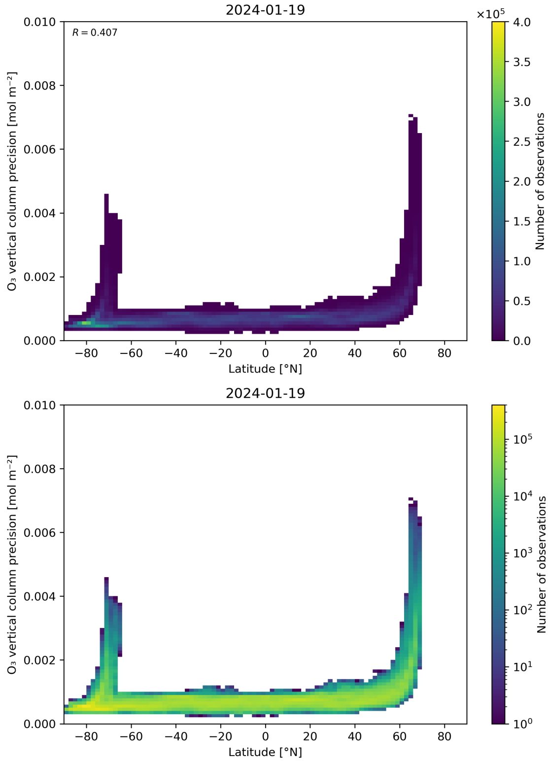
Figure 37: Scatter density plot of “Latitude” against “O 3 vertical column precision” for 2024-01-18 to 2024-01-20.
