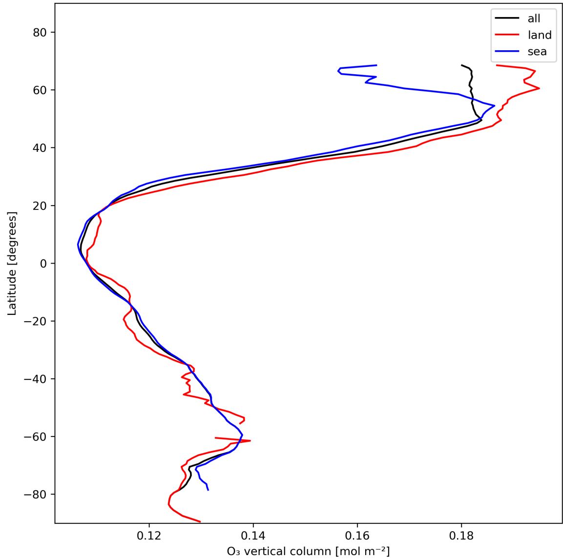
Figure 14: Zonal average of “O 3 vertical column” for 2024-01-18 to 2024-01-20.
