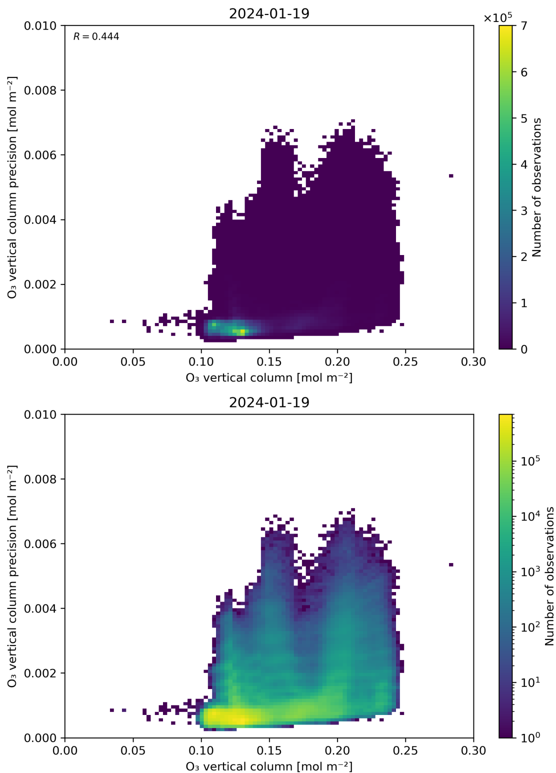
Figure 41: Scatter density plot of “O 3 vertical column” against “O 3 vertical column precision” for 2024-01-18 to 2024-01-20.
