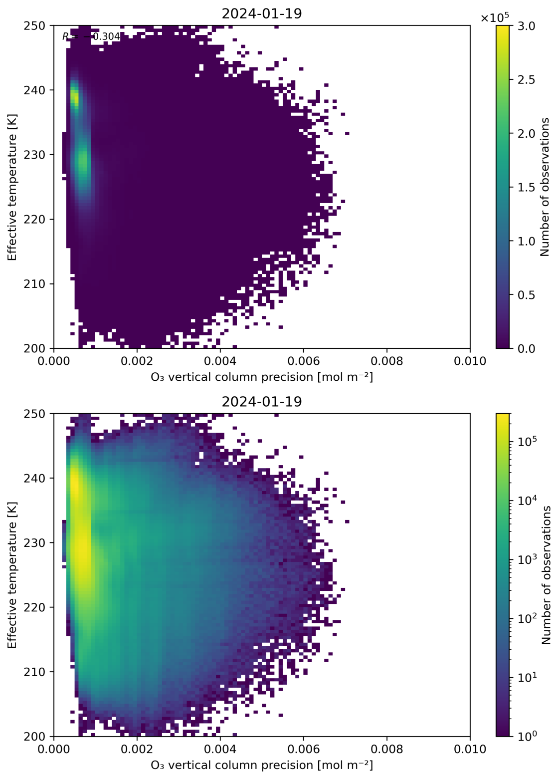
Figure 42: Scatter density plot of “O 3 vertical column precision” against “Effective temperature” for 2024-01-18 to 2024-01-20.
