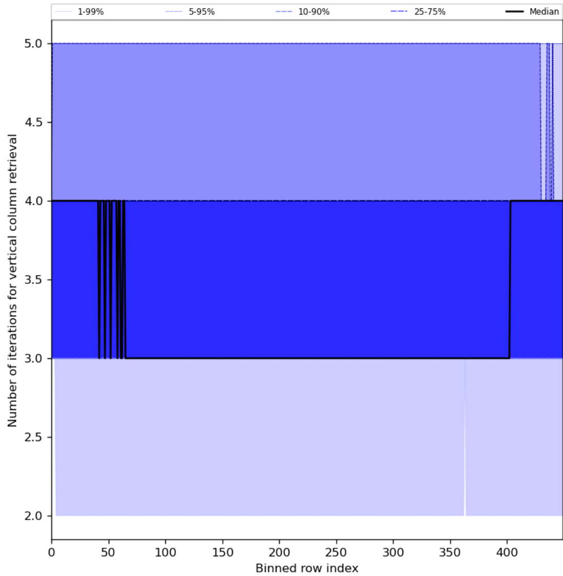
Figure 33: Along track statistics of “Number of iterations for vertical column retrieval” for 2024-01-18 to 2024-01-20
