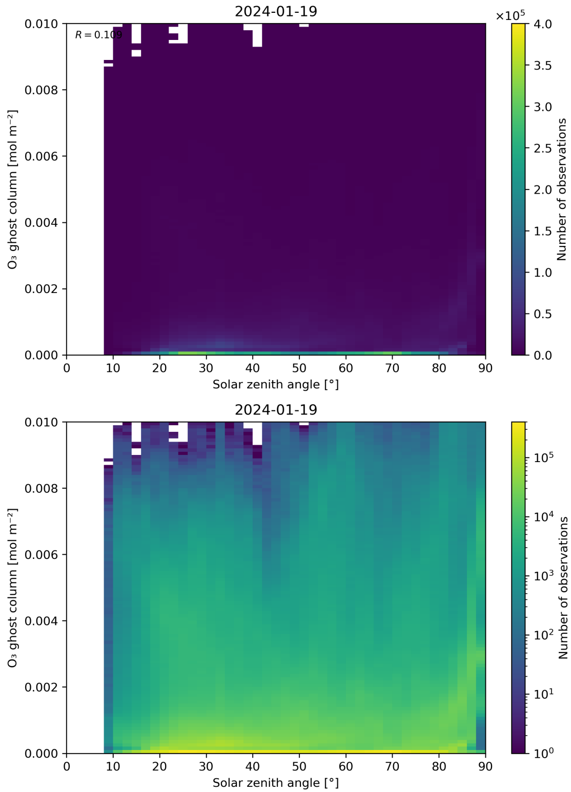
Figure 46: Scatter density plot of “Solar zenith angle” against “O 3 ghost column” for 2024-01-18 to 2024-01-20.
