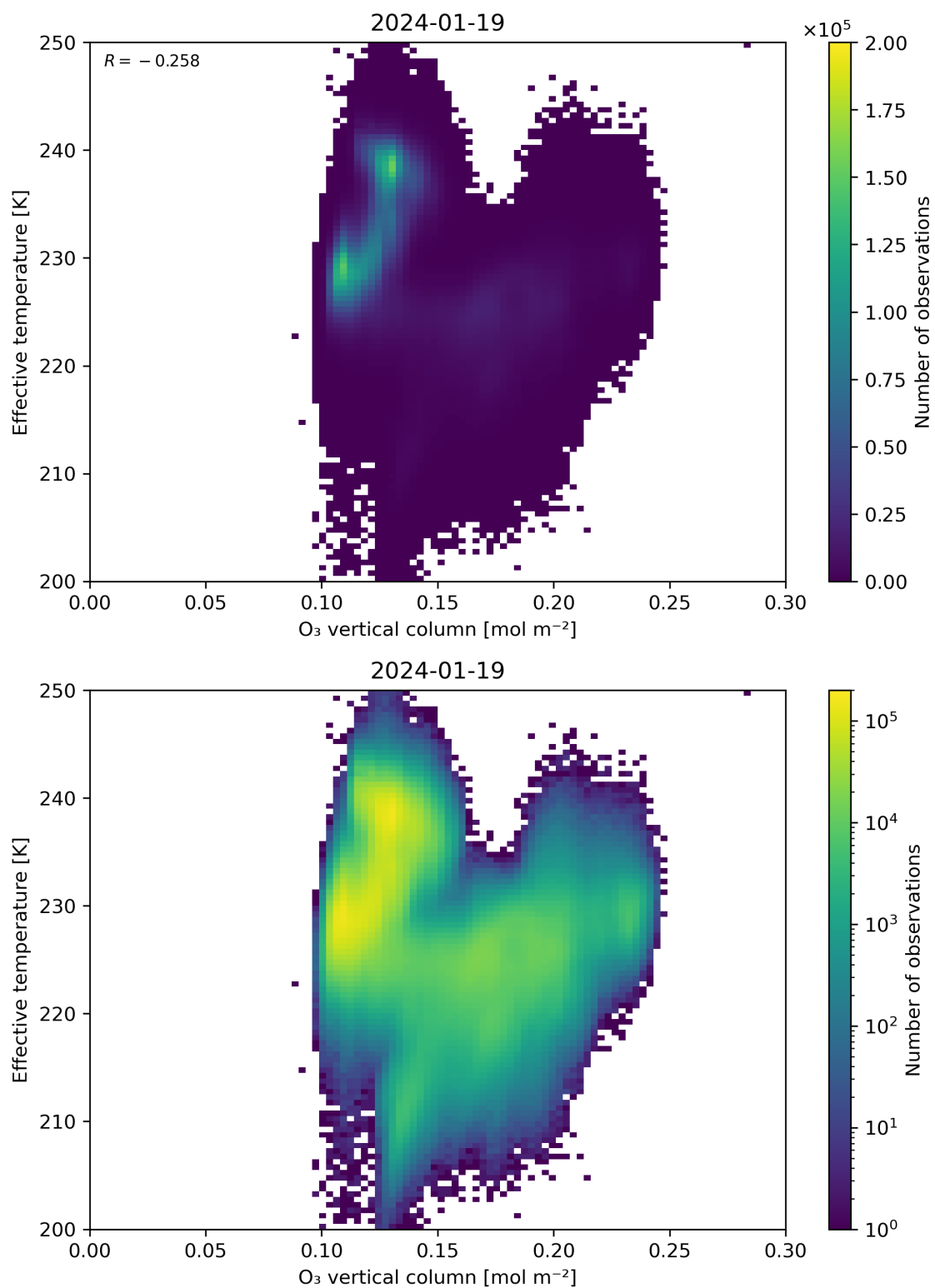
Figure 39: Scatter density plot of “O 3 vertical column” against “Effective temperature” for 2024-01-18 to 2024-01-20.
