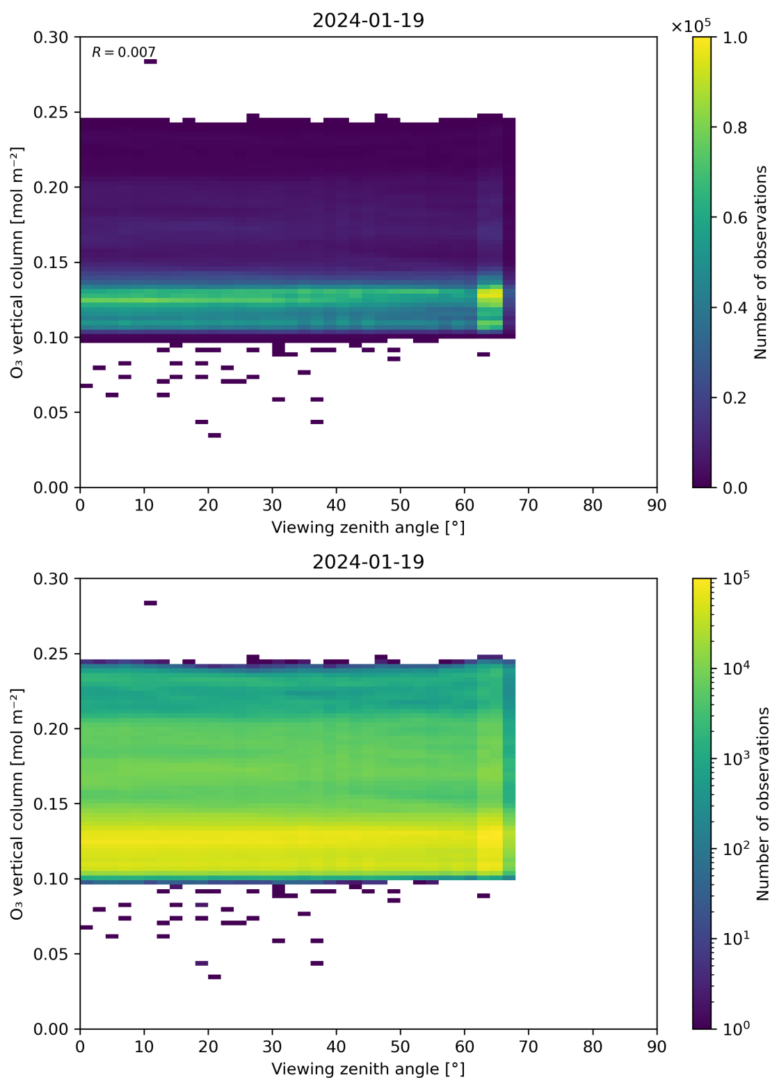
Figure 52: Scatter density plot of “Viewing zenith angle” against “O 3 vertical column” for 2024-01-18 to 2024-01-20.
