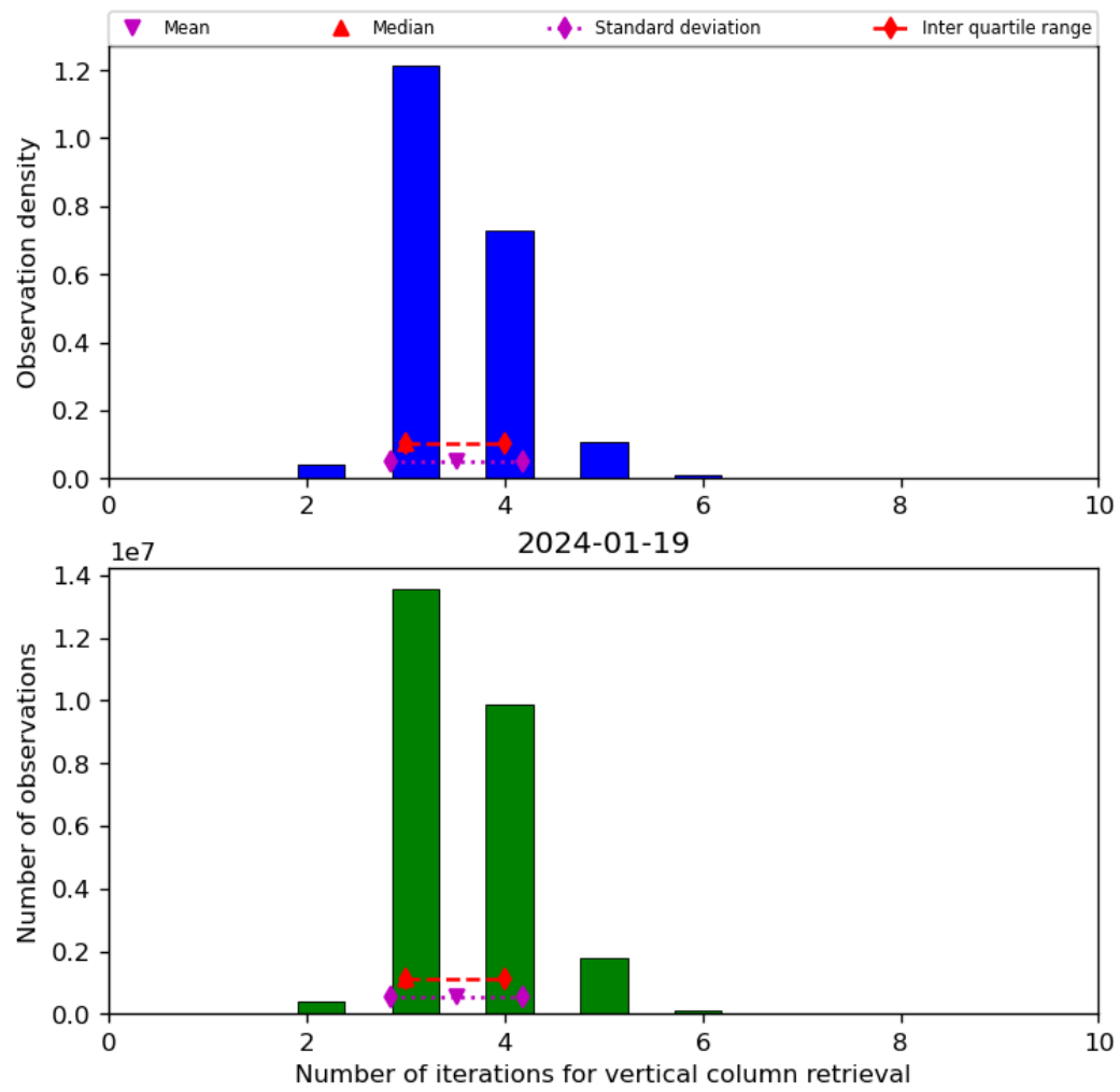
Figure 26: Histogram of “Number of iterations for vertical column retrieval” for 2024-01-18 to 2024-01-20
