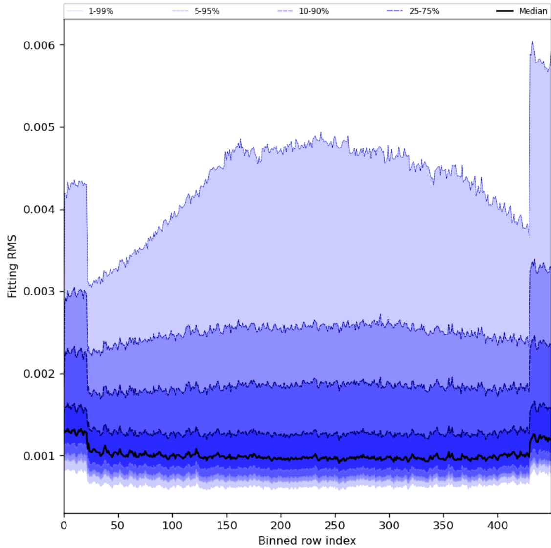
Figure 30: Along track statistics of “Fitting RMS” for 2024-01-18 to 2024-01-20
