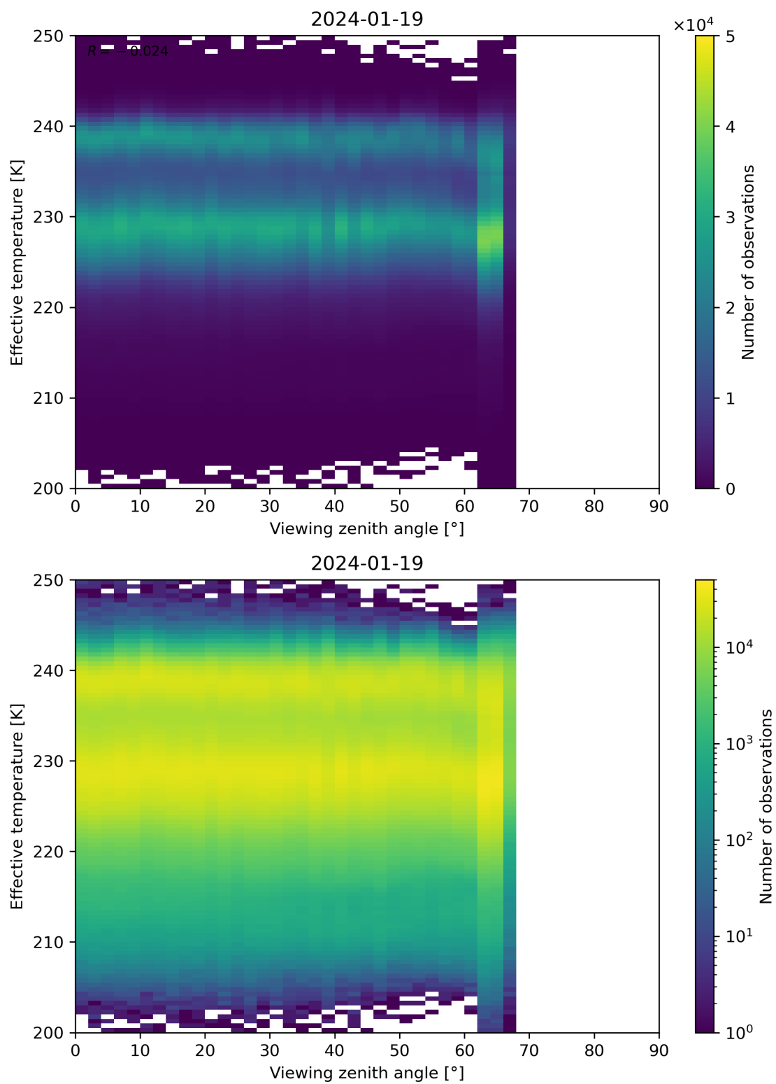
Figure 50: Scatter density plot of “Viewing zenith angle” against “Effective temperature” for 2024-01-18 to 2024-01-20.
