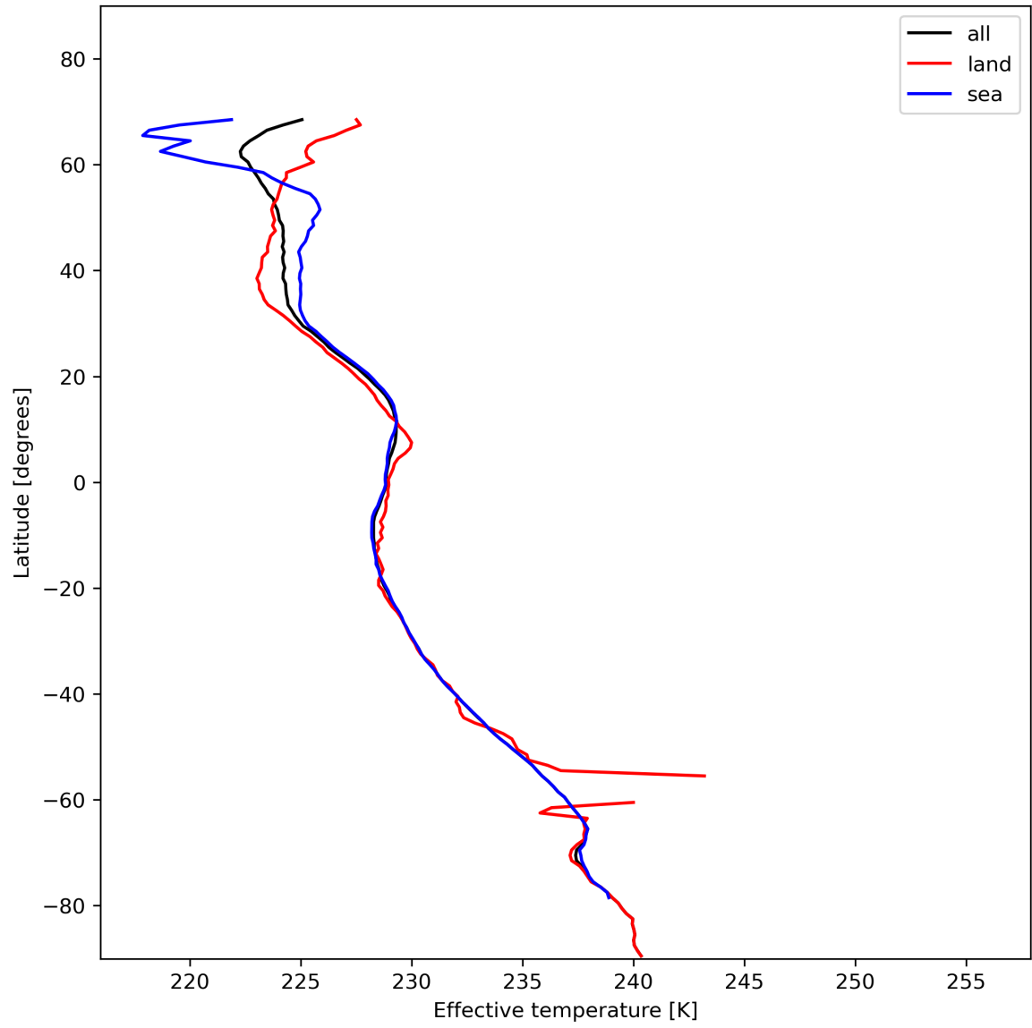
Figure 17: Zonal average of "Effective temperature" for 2024-01-18 to 2024-01-20.
