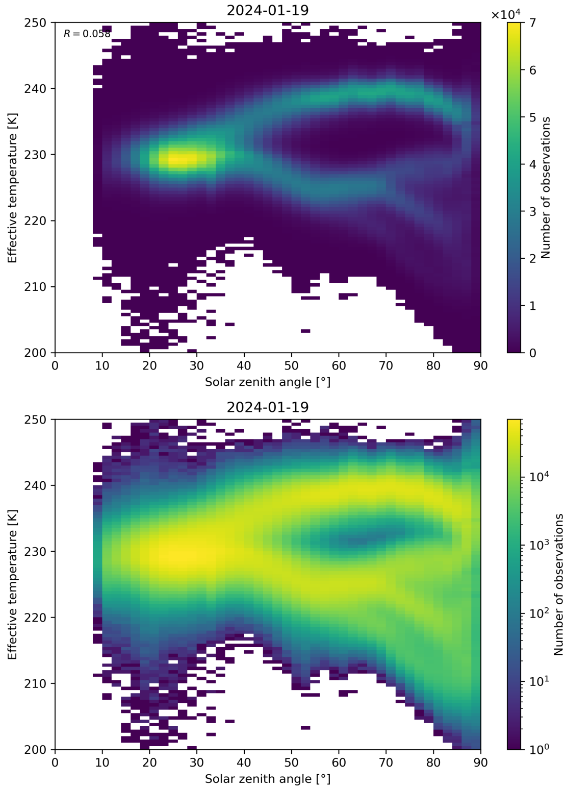
Figure 45: Scatter density plot of “Solar zenith angle” against “Effective temperature” for 2024-01-18 to 2024-01-20.
