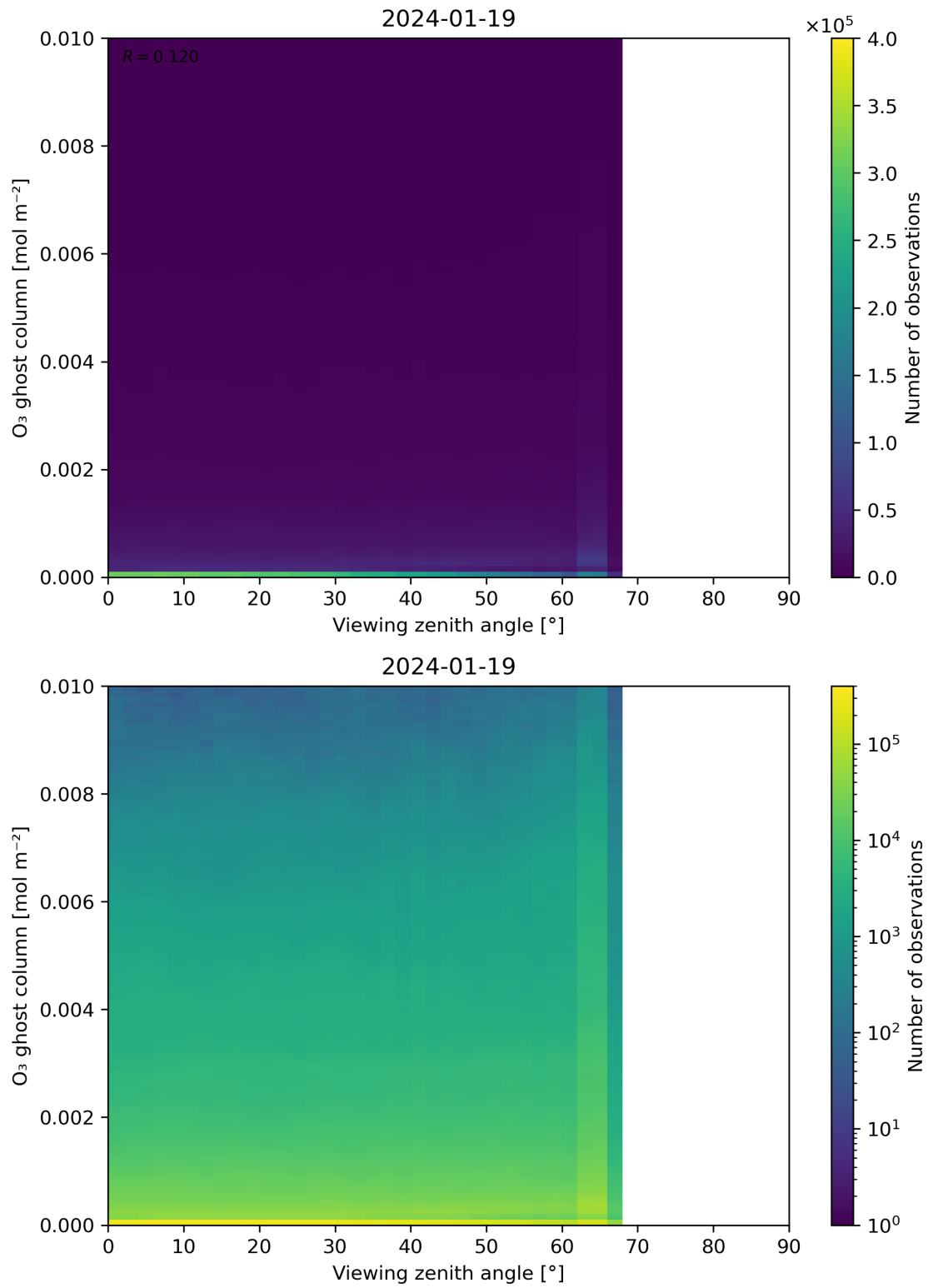
Figure 51: Scatter density plot of “Viewing zenith angle” against “O 3 ghost column” for 2024-01-18 to 2024-01-20.
