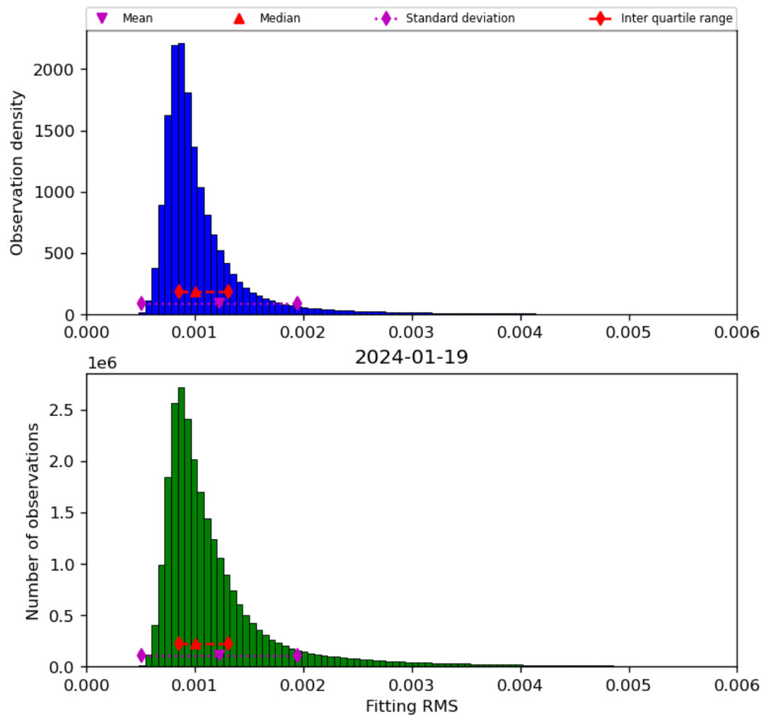
Figure 23: Histogram of “Fitting RMS” for 2024-01-18 to 2024-01-20
