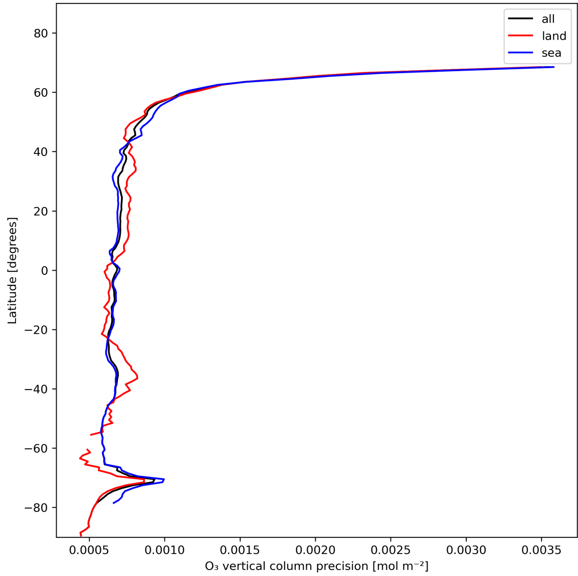
Figure 15: Zonal average of “O 3 vertical column precision” for 2024-01-18 to 2024-01-20.
