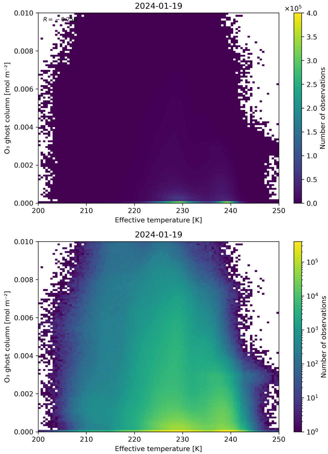
Figure 38: Scatter density plot of “Effective temperature” against “O 3 ghost column” for 2024-01-18 to 2024-01-20.
