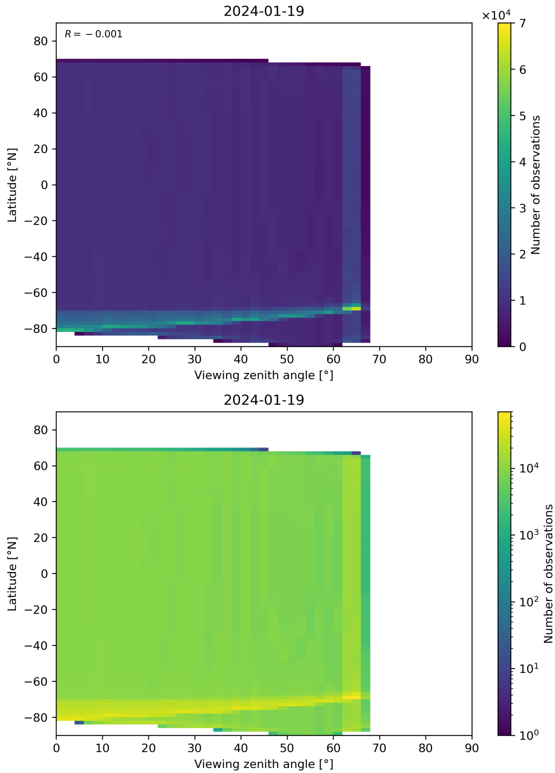
Figure 49: Scatter density plot of “Viewing zenith angle” against “Latitude” for 2024-01-18 to 2024-01-20.
