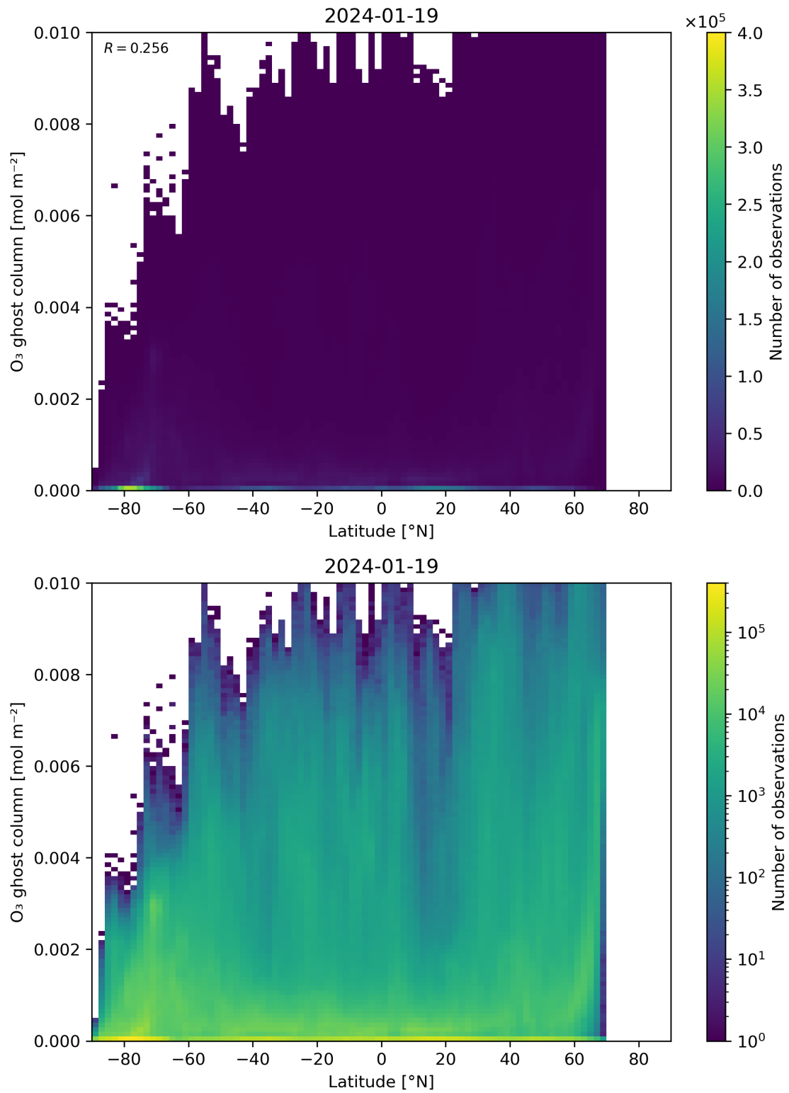
Figure 35: Scatter density plot of “Latitude” against “O 3 ghost column” for 2024-01-18 to 2024-01-20.
