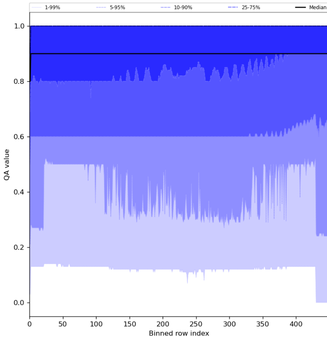
Figure 27: Along track statistics of “QA value” for 2024-01-18 to 2024-01-20
