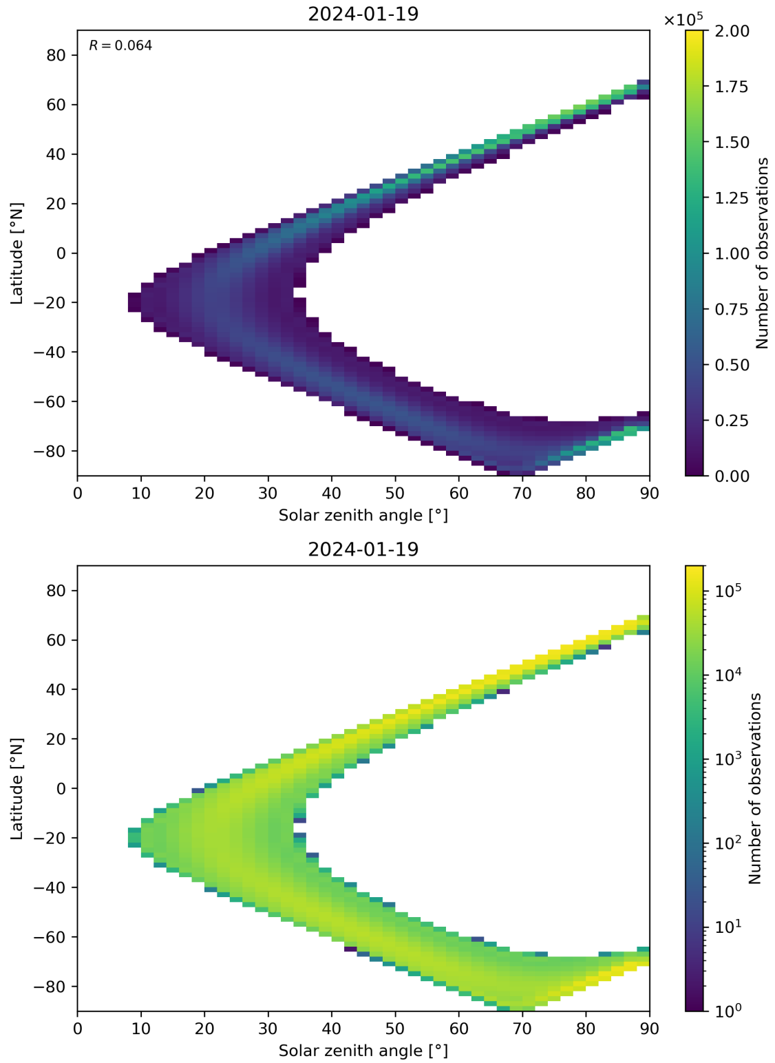
Figure 44: Scatter density plot of “Solar zenith angle” against “Latitude” for 2024-01-18 to 2024-01-20.
