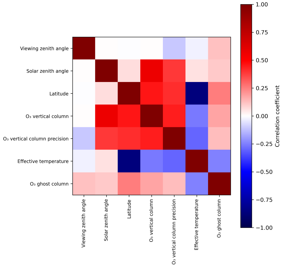
Figure 2: Map of correlation matrix for 2024-01-18 to 2024-01-20.
