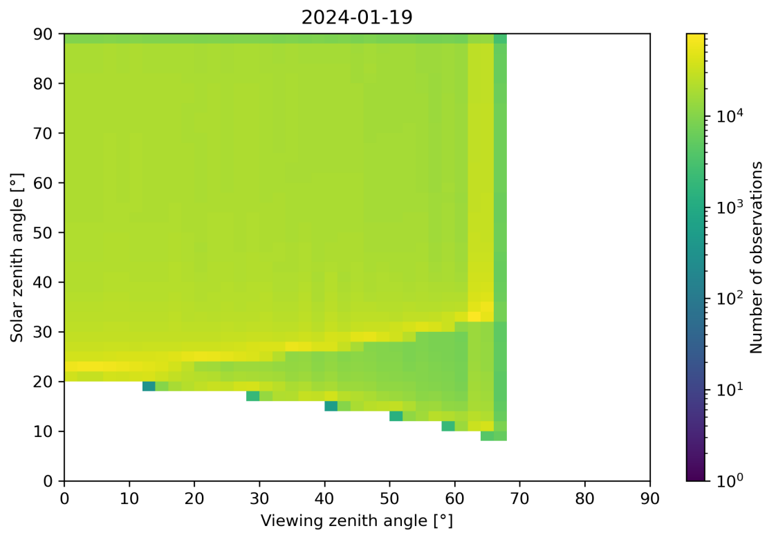
Figure 54: Scatter density plot of “Viewing zenith angle” against “Solar zenith angle” for 2024-01-18 to 2024-01-20.
