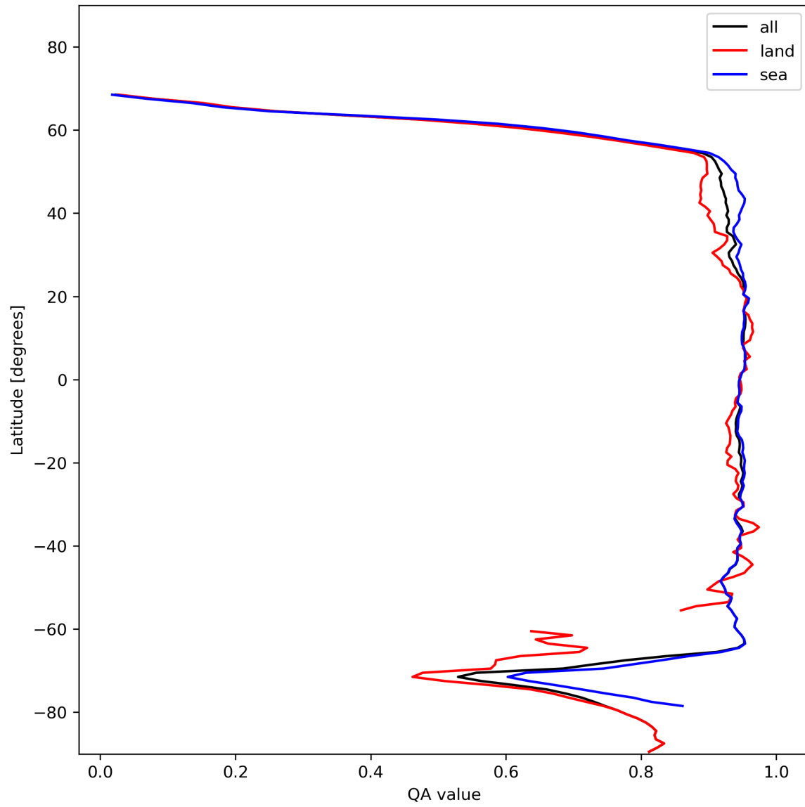
Figure 13: Zonal average of “QA value” for 2024-01-18 to 2024-01-20.
