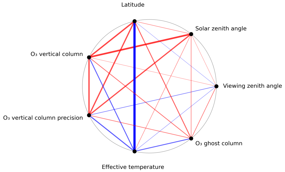
Figure 1: Map of correlation graph for 2024-01-18 to 2024-01-20.
