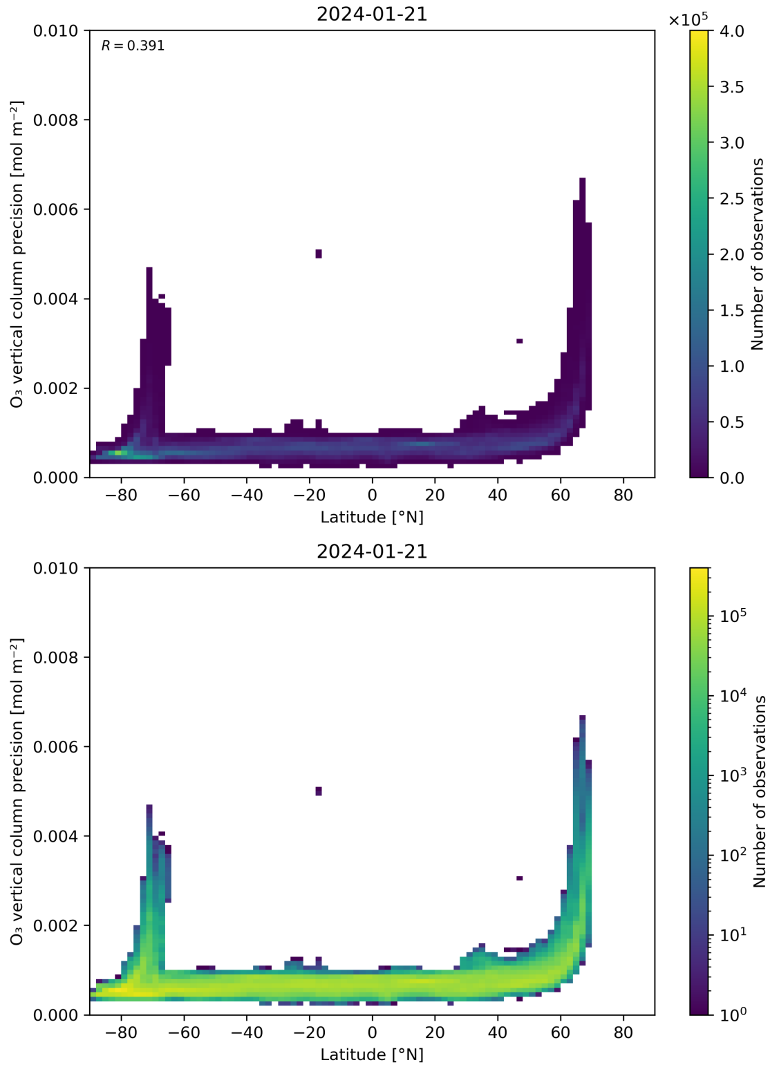
Figure 37: Scatter density plot of “Latitude” against “O 3 vertical column precision” for 2024-01-21 to 2024-01-22.
