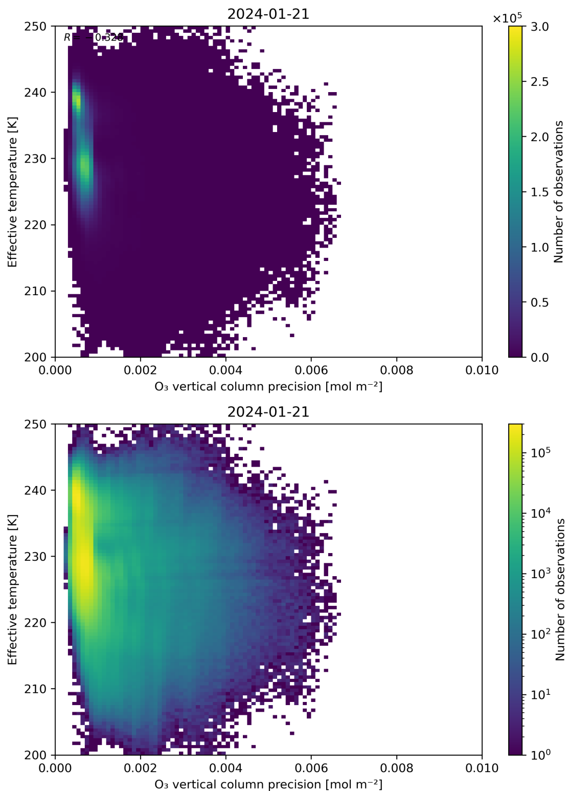
Figure 42: Scatter density plot of “ \text{O}_3 vertical column precision” against “Effective temperature” for 2024-01-21 to 2024-01-22.
