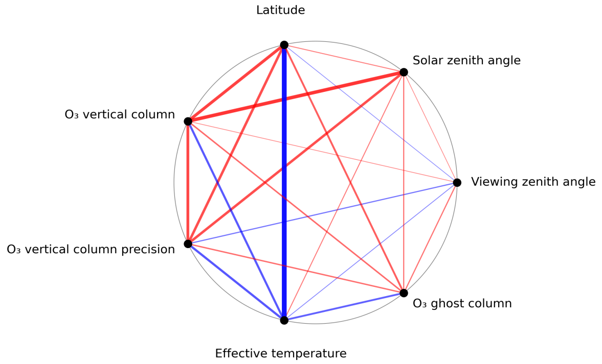
Figure 1: Map of correlation graph for 2024-01-21 to 2024-01-22.
