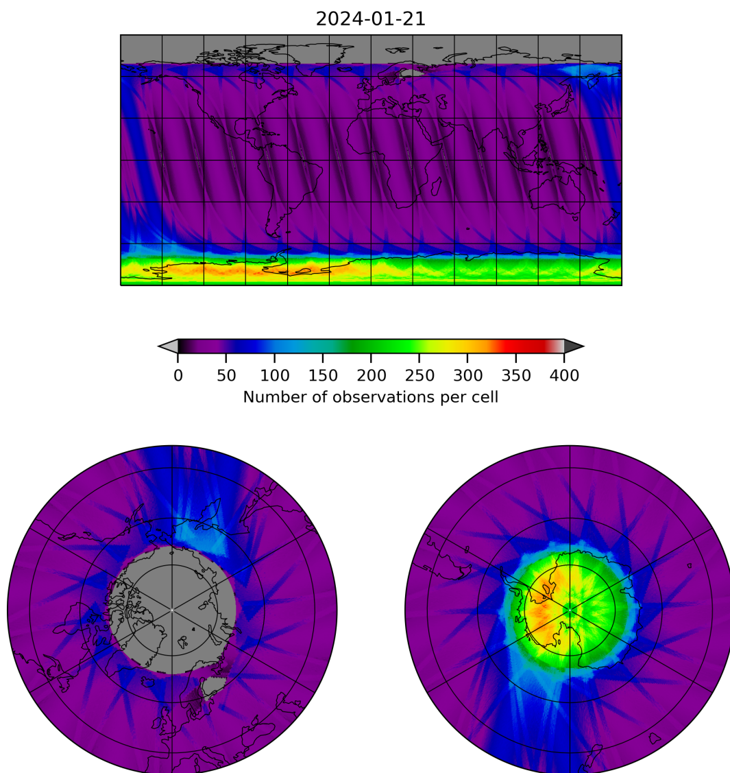
Figure 12: Map of the number of observations for 2024-01-21 to 2024-01-22
