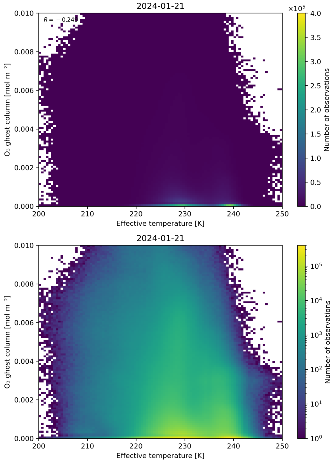
Figure 38: Scatter density plot of “Effective temperature” against “O 3 ghost column” for 2024-01-21 to 2024-01-22.
