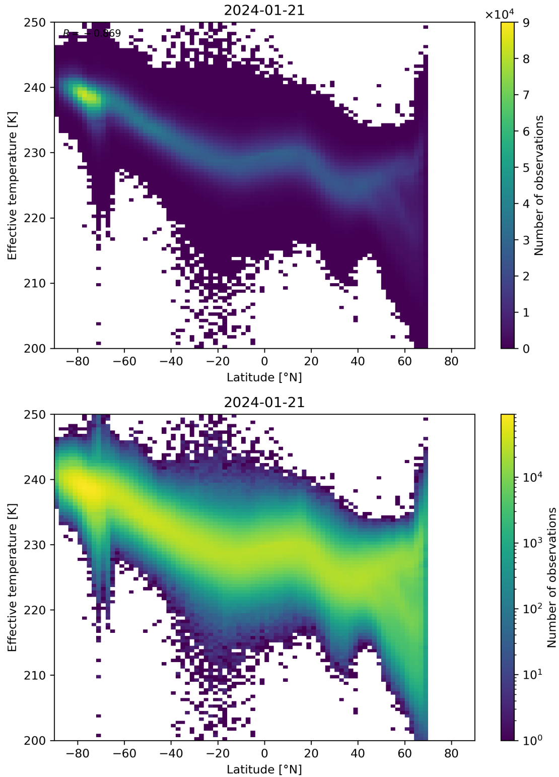
Figure 34: Scatter density plot of “Latitude” against “Effective temperature” for 2024-01-21 to 2024-01-22.
