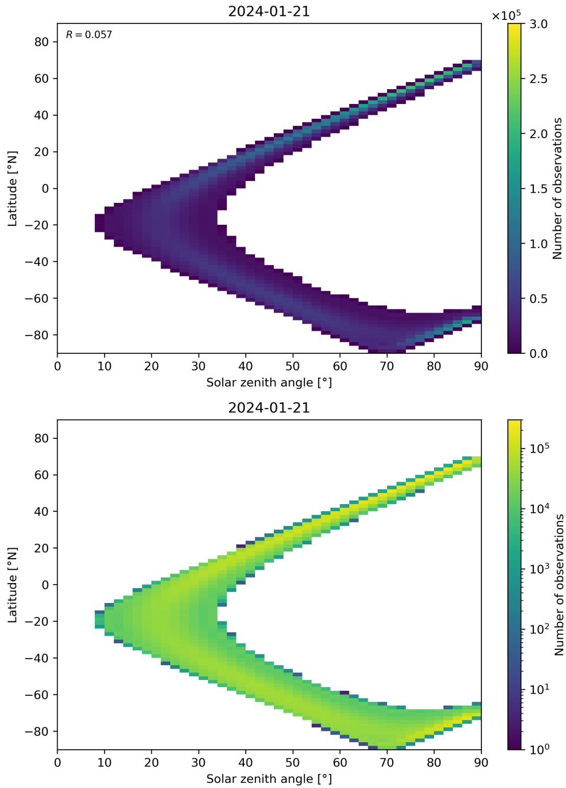
Figure 44: Scatter density plot of “Solar zenith angle” against “Latitude” for 2024-01-21 to 2024-01-22.
