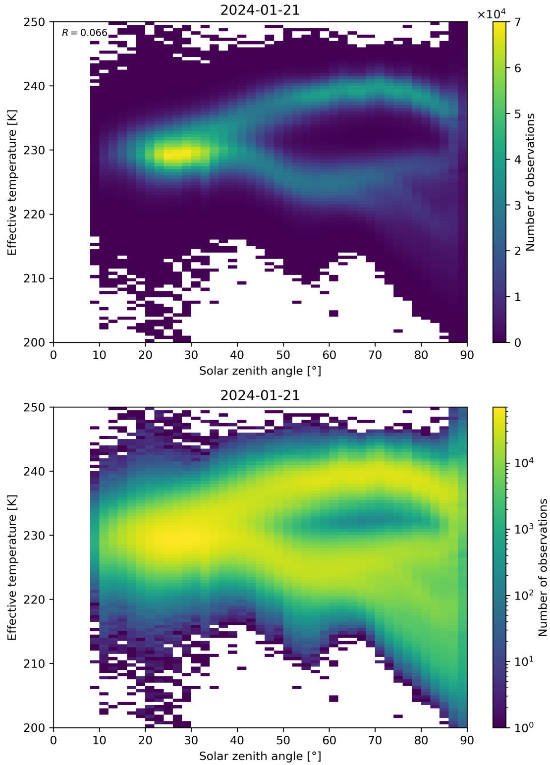
Figure 45: Scatter density plot of “Solar zenith angle” against “Effective temperature” for 2024-01-21 to 2024-01-22.
