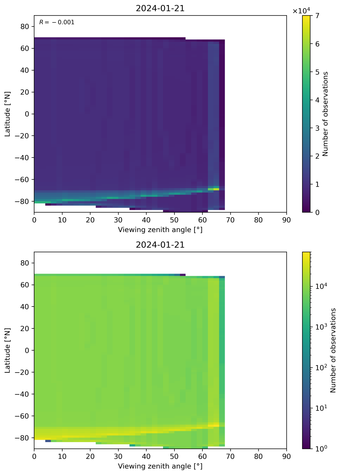
Figure 49: Scatter density plot of “Viewing zenith angle” against “Latitude” for 2024-01-21 to 2024-01-22.
