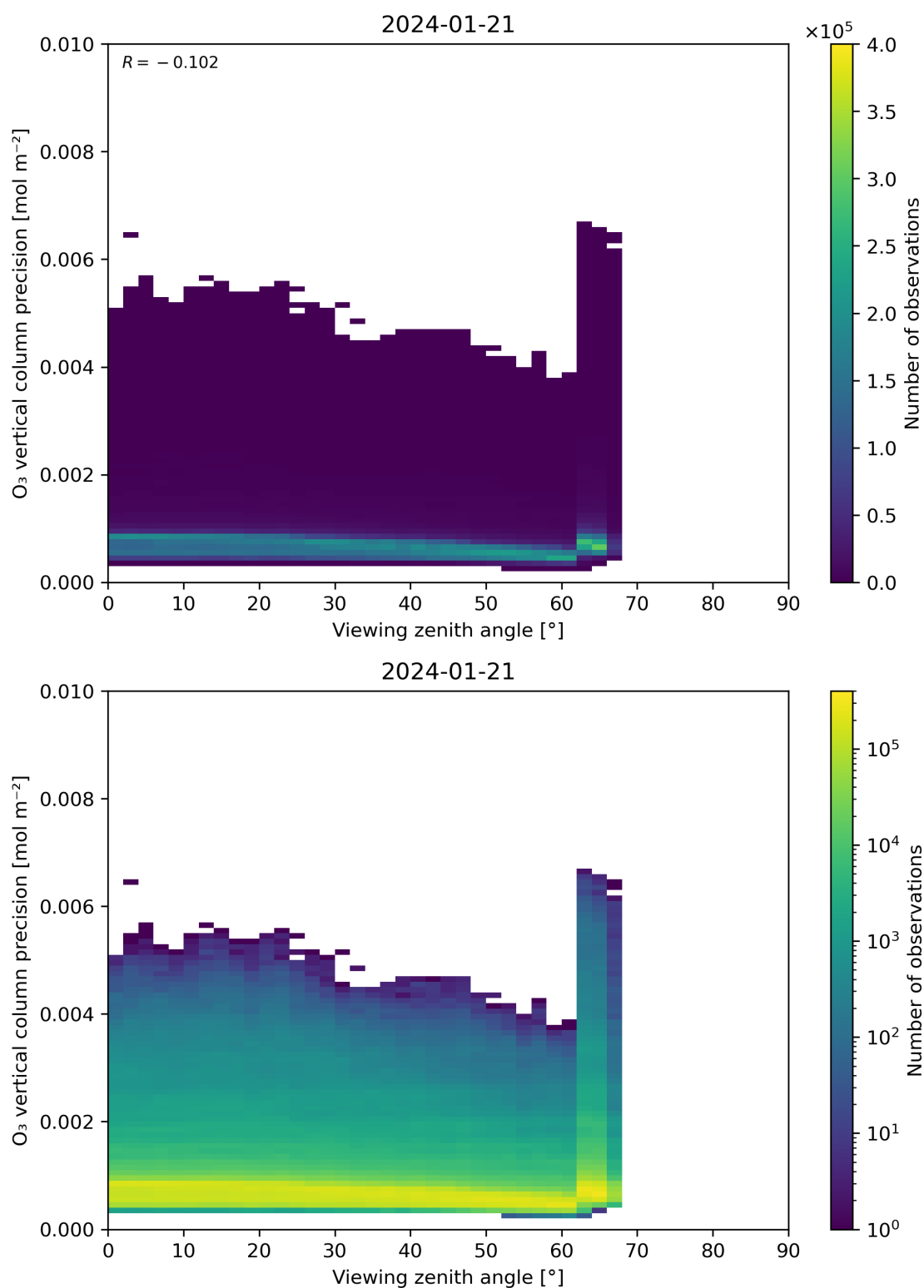
Figure 53: Scatter density plot of “Viewing zenith angle” against “O 3 vertical column precision” for 2024-01-21 to 2024-01-22.
