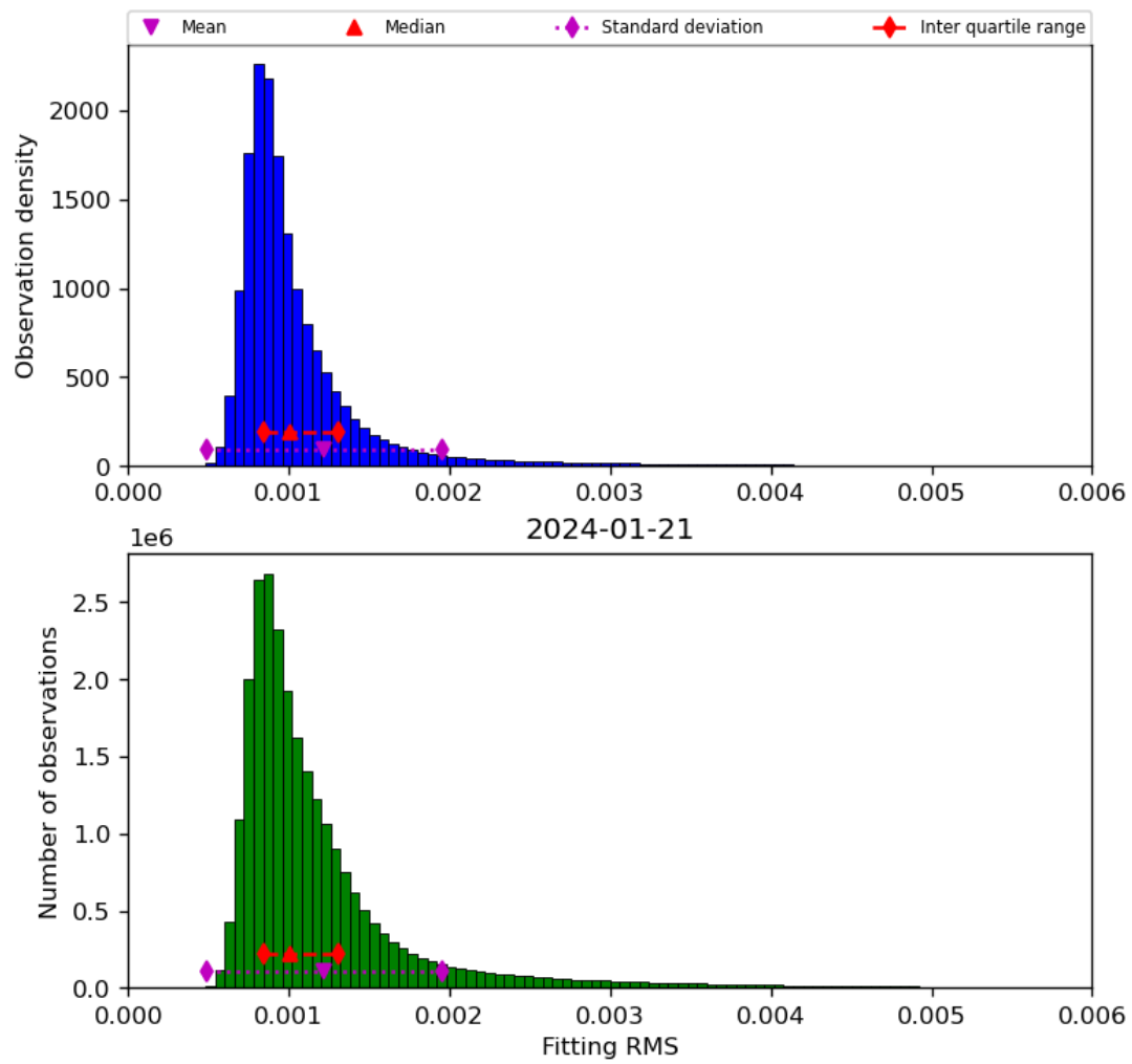
Figure 23: Histogram of “Fitting RMS” for 2024-01-21 to 2024-01-22
