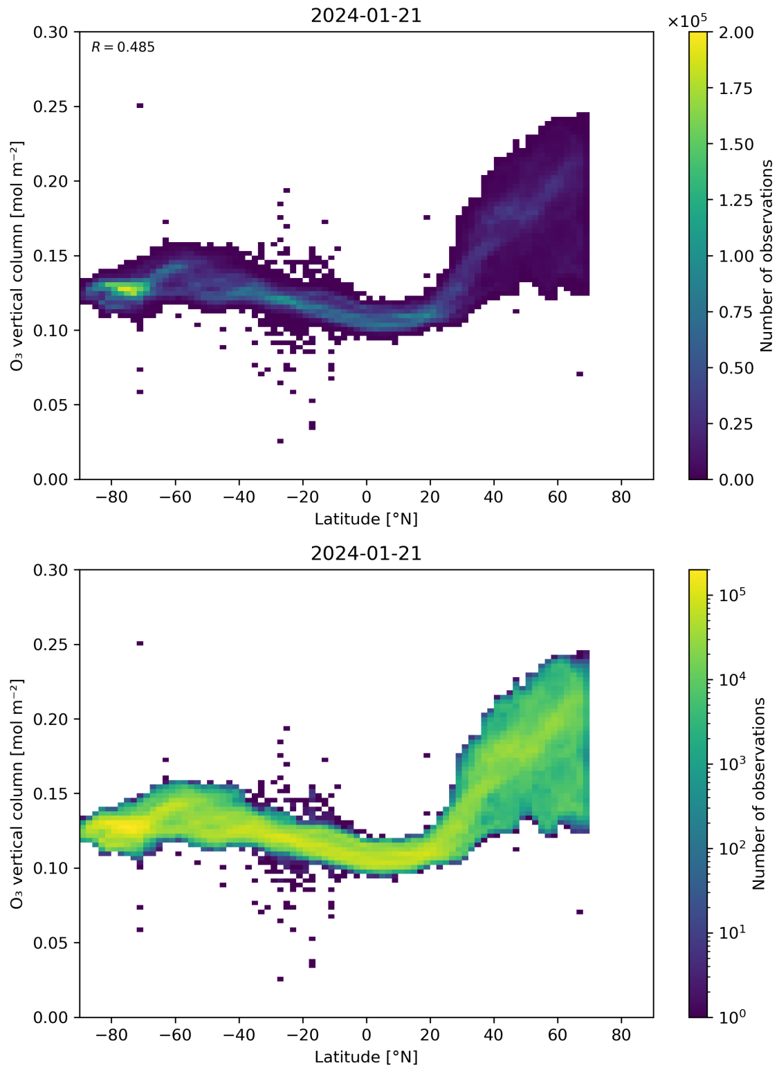
Figure 36: Scatter density plot of “Latitude” against “O 3 vertical column” for 2024-01-21 to 2024-01-22.
