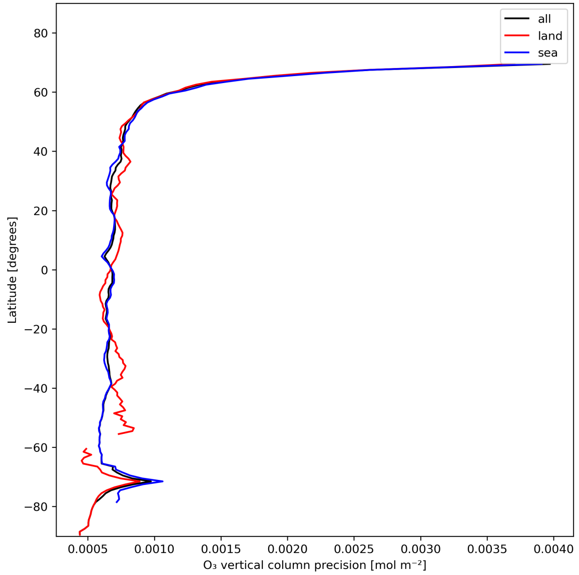
Figure 15: Zonal average of “O 3 vertical column precision” for 2024-01-21 to 2024-01-22.
