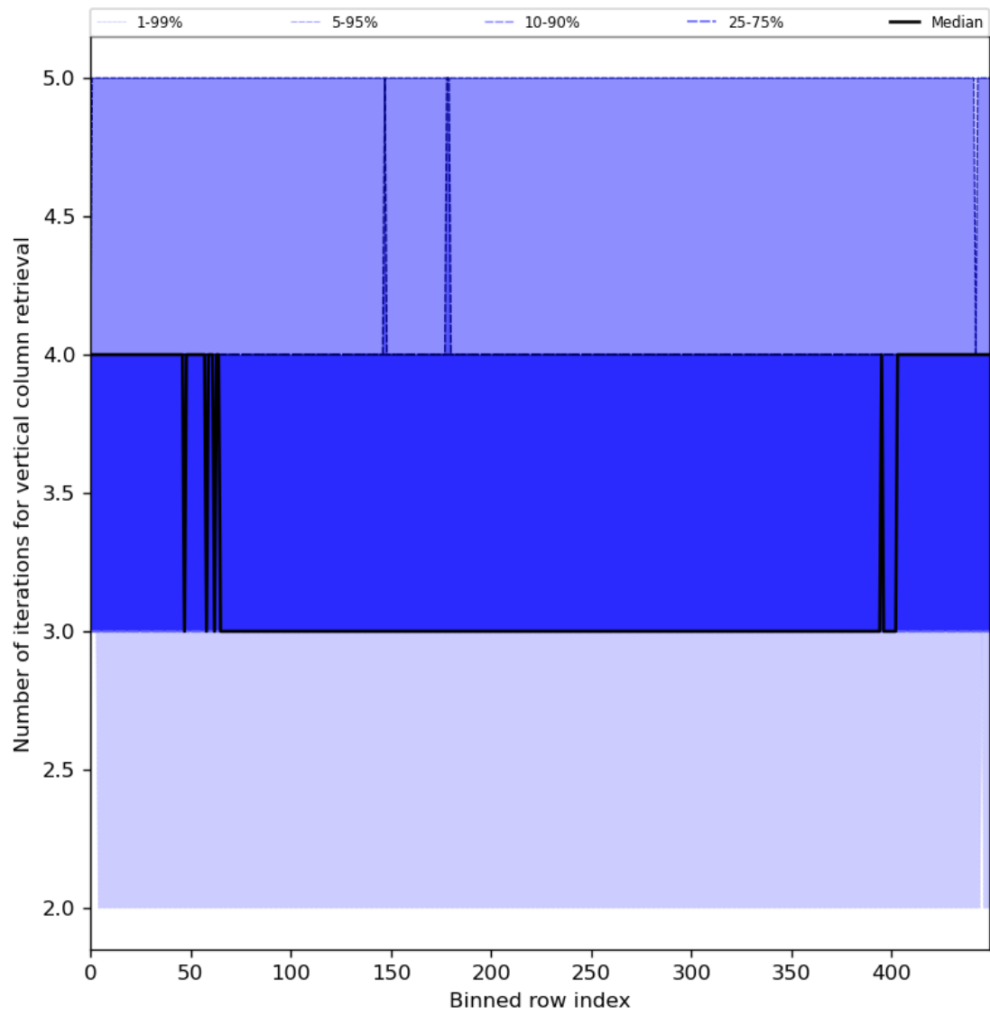
Figure 33: Along track statistics of “Number of iterations for vertical column retrieval” for 2024-01-21 to 2024-01-22
