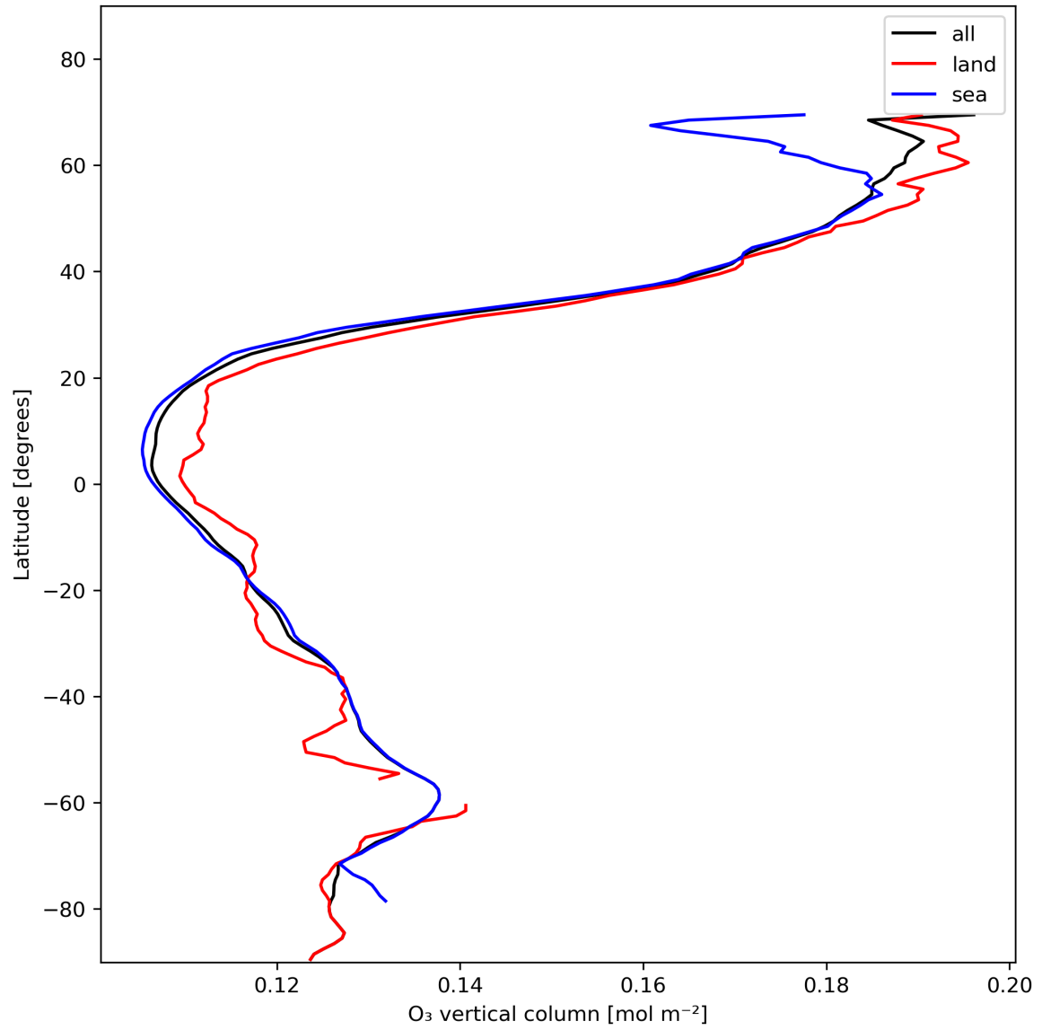
Figure 14: Zonal average of “O 3 vertical column” for 2024-01-21 to 2024-01-22.
