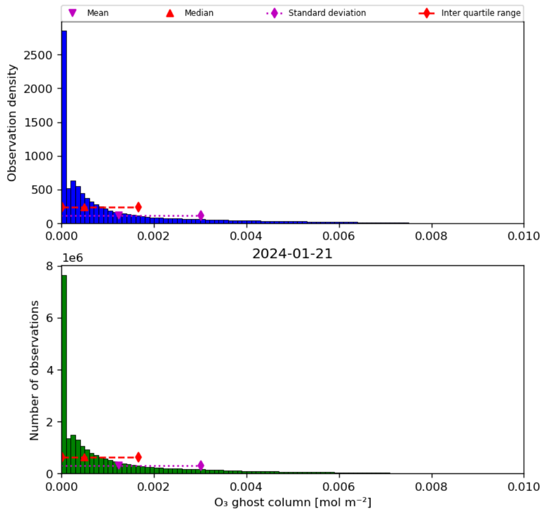
Figure 25: Histogram of “O 3 ghost column” for 2024-01-21 to 2024-01-22
