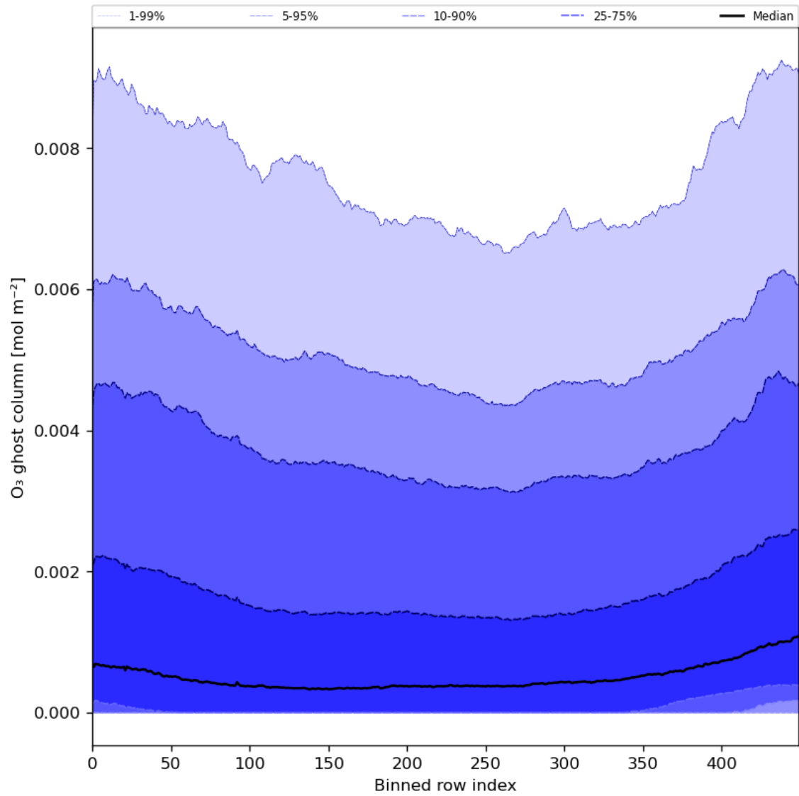
Figure 32: Along track statistics of “O 3 ghost column” for 2024-01-21 to 2024-01-22
