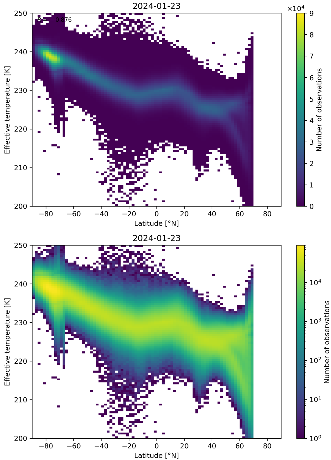
Figure 34: Scatter density plot of “Latitude” against “Effective temperature” for 2024-01-22 to 2024-01-24.
