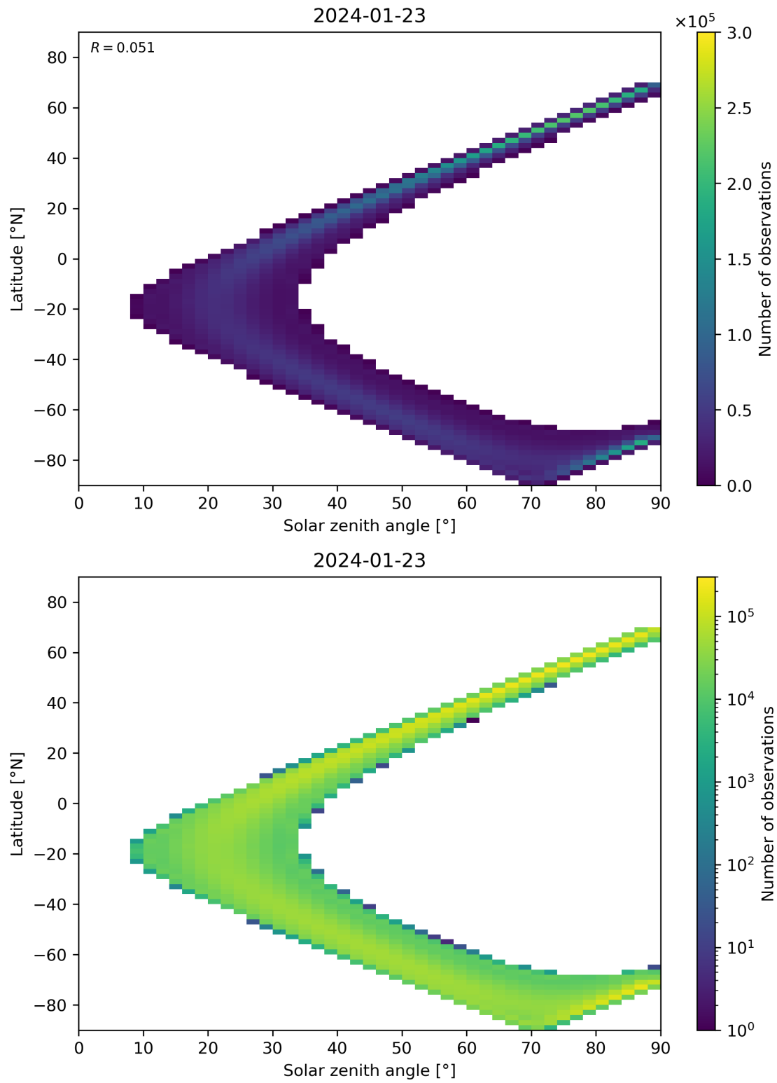
Figure 44: Scatter density plot of “Solar zenith angle” against “Latitude” for 2024-01-22 to 2024-01-24.
