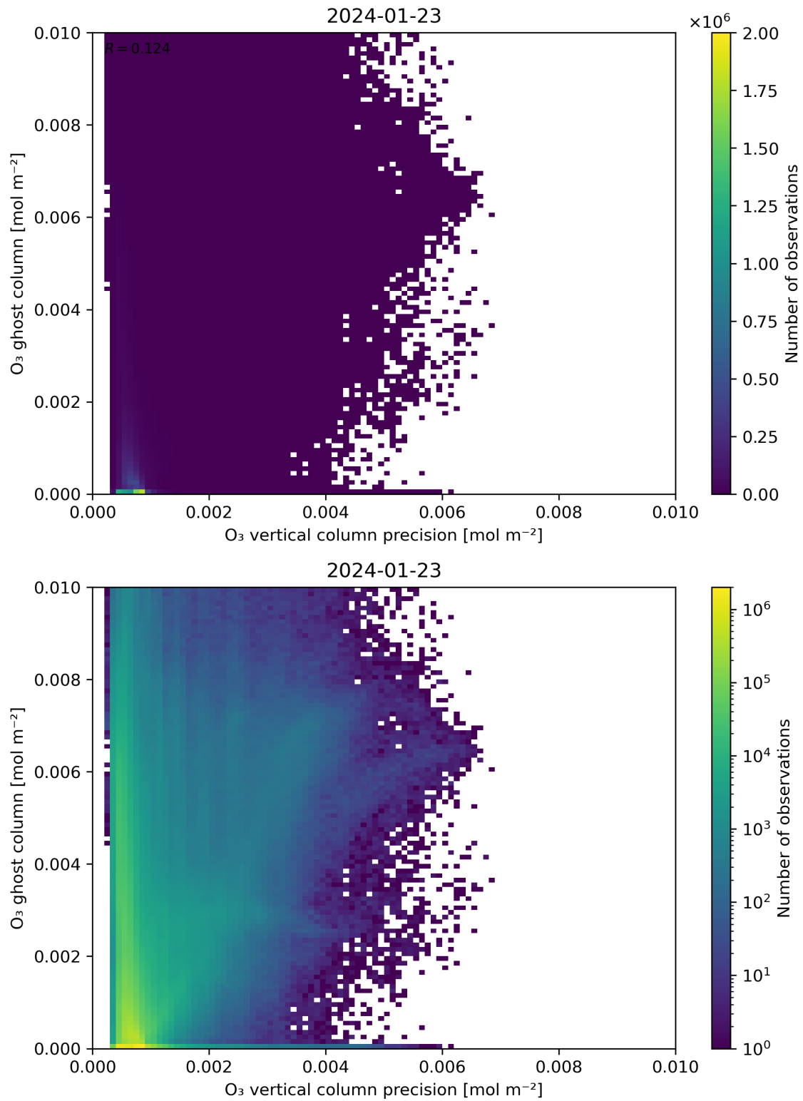
Figure 43: Scatter density plot of “ \text{O}_3 vertical column precision” against “ \text{O}_3 ghost column” for 2024-01-22 to 2024-01-24.
