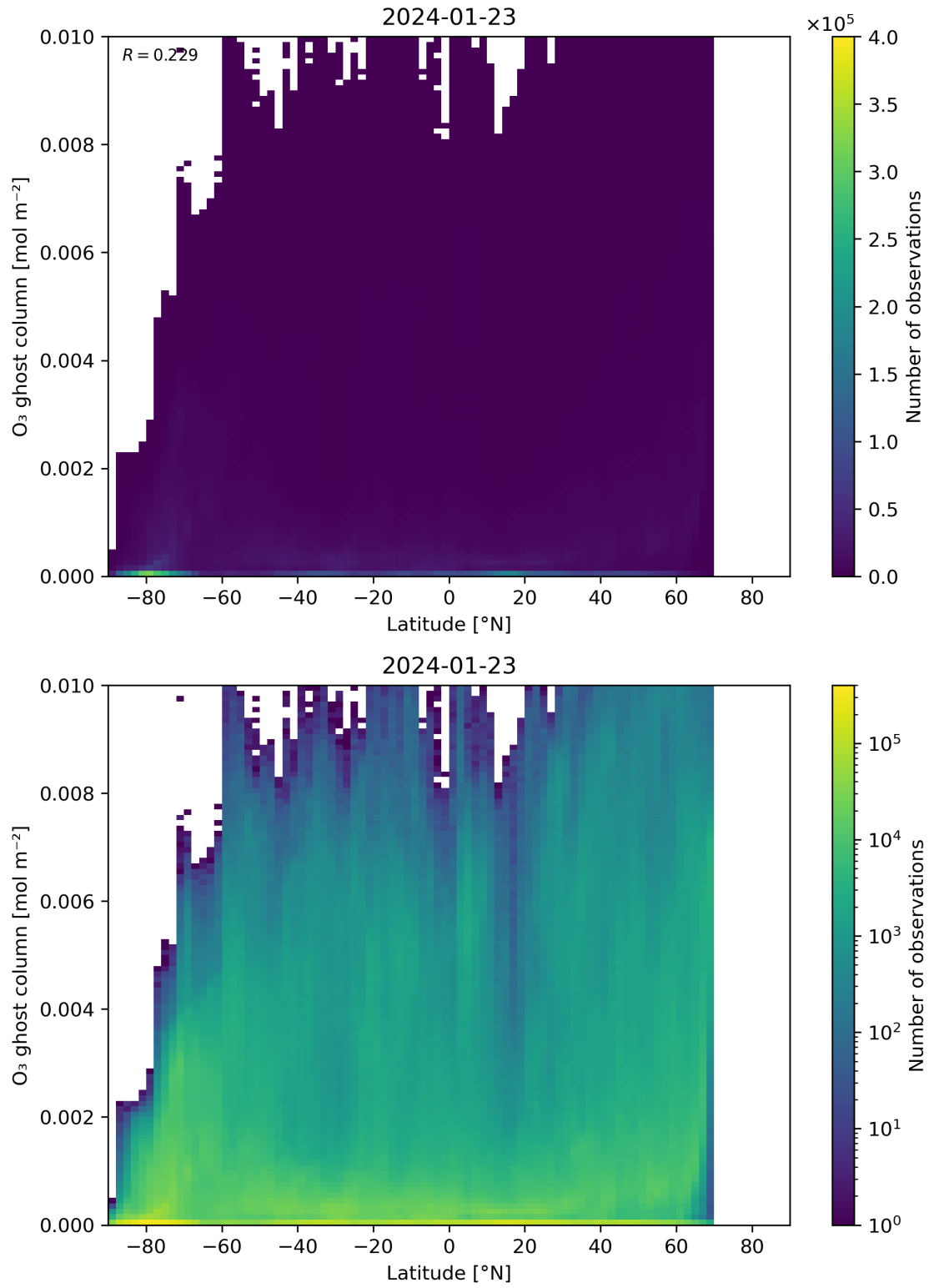
Figure 35: Scatter density plot of “Latitude” against “O 3 ghost column” for 2024-01-22 to 2024-01-24.
