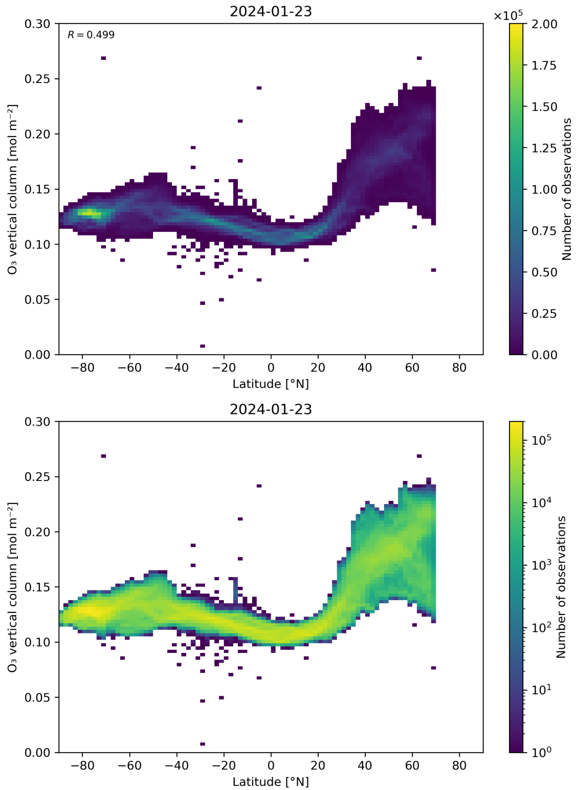
Figure 36: Scatter density plot of “Latitude” against “O 3 vertical column” for 2024-01-22 to 2024-01-24.
