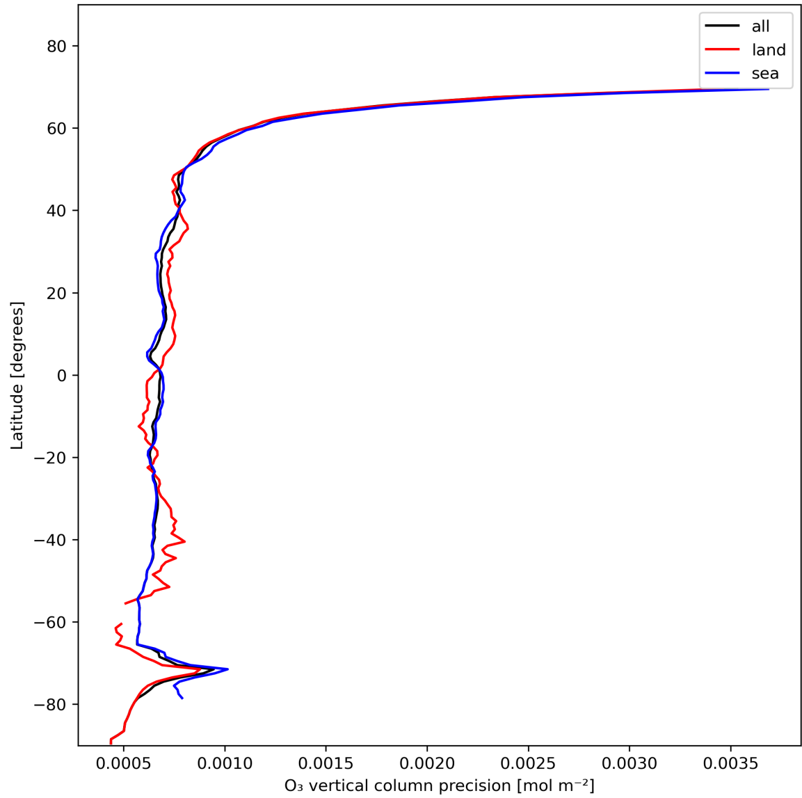
Figure 15: Zonal average of “O 3 vertical column precision” for 2024-01-22 to 2024-01-24.
