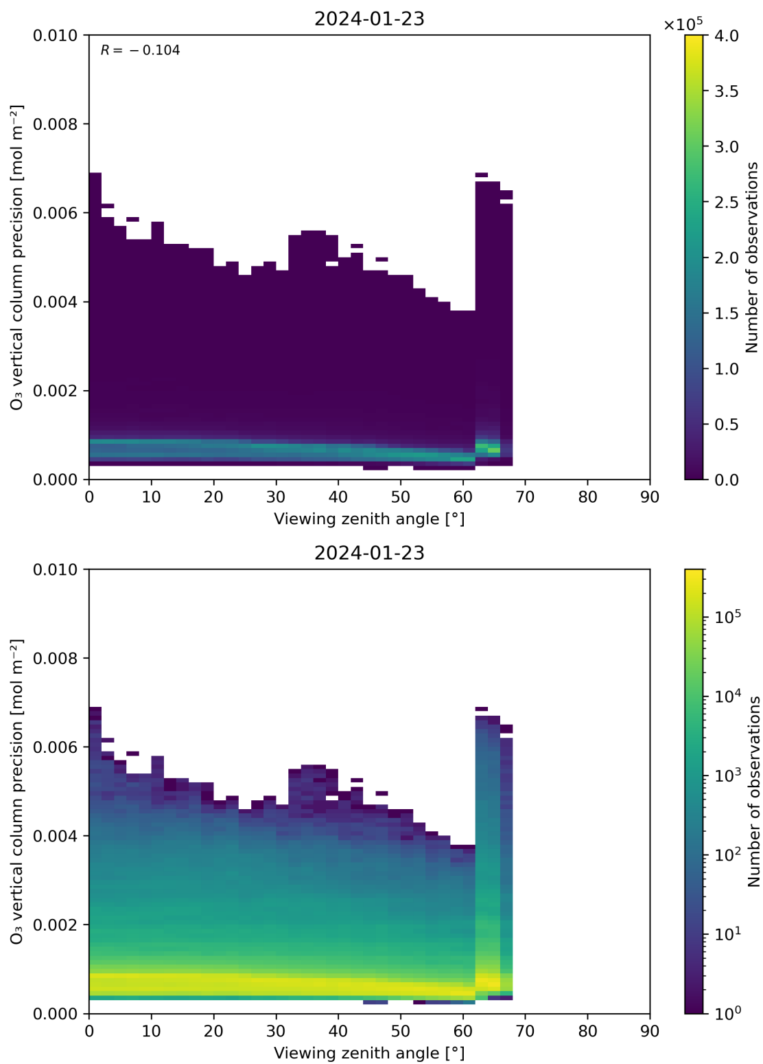
Figure 53: Scatter density plot of “Viewing zenith angle” against “O 3 vertical column precision” for 2024-01-22 to 2024-01-24.
