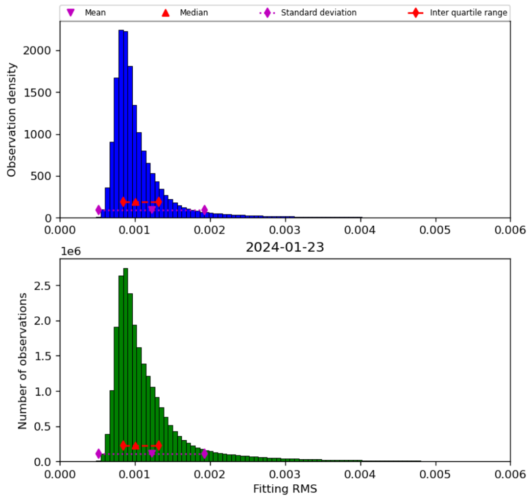
Figure 23: Histogram of “Fitting RMS” for 2024-01-22 to 2024-01-24
