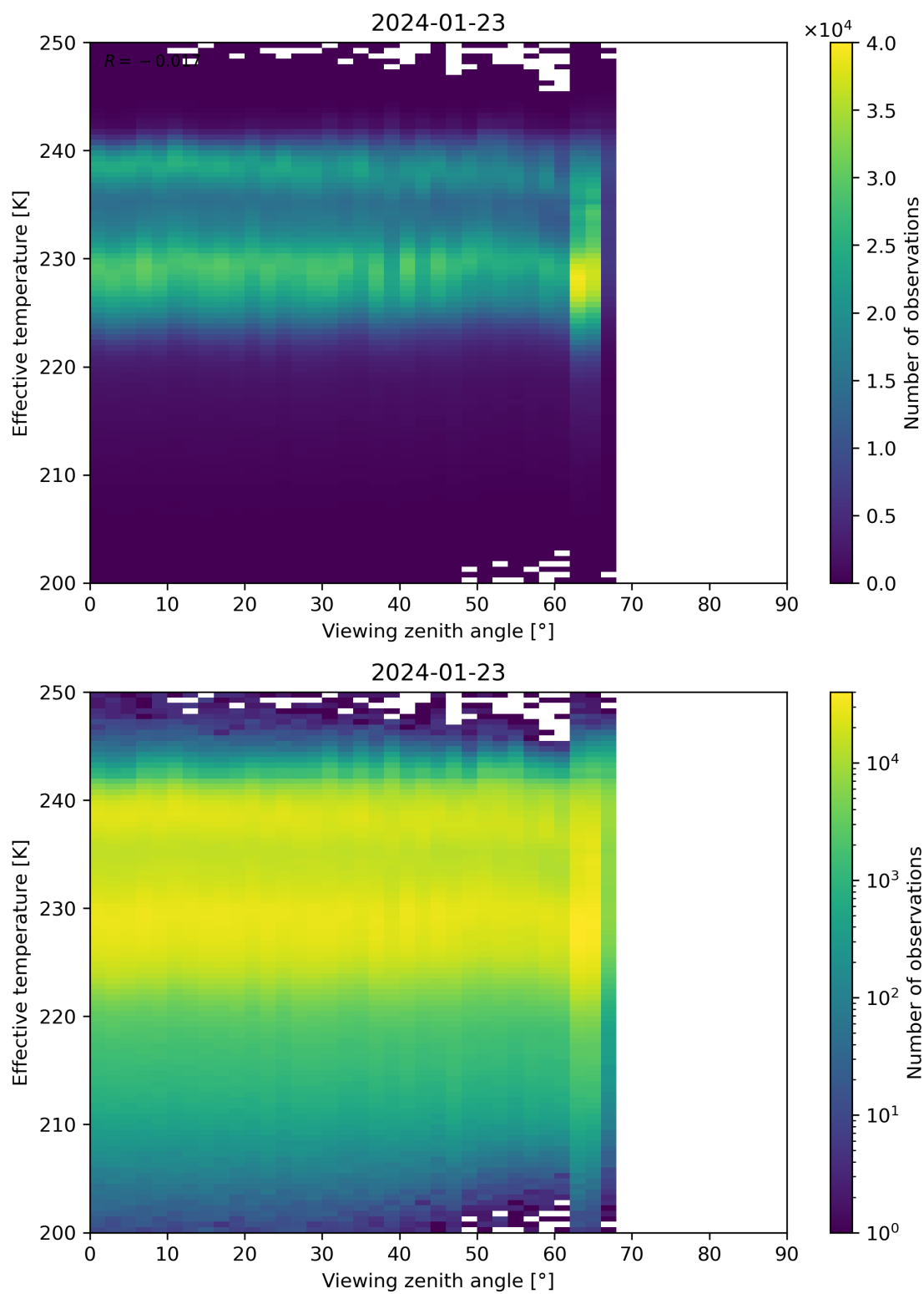
Figure 50: Scatter density plot of “Viewing zenith angle” against “Effective temperature” for 2024-01-22 to 2024-01-24.
