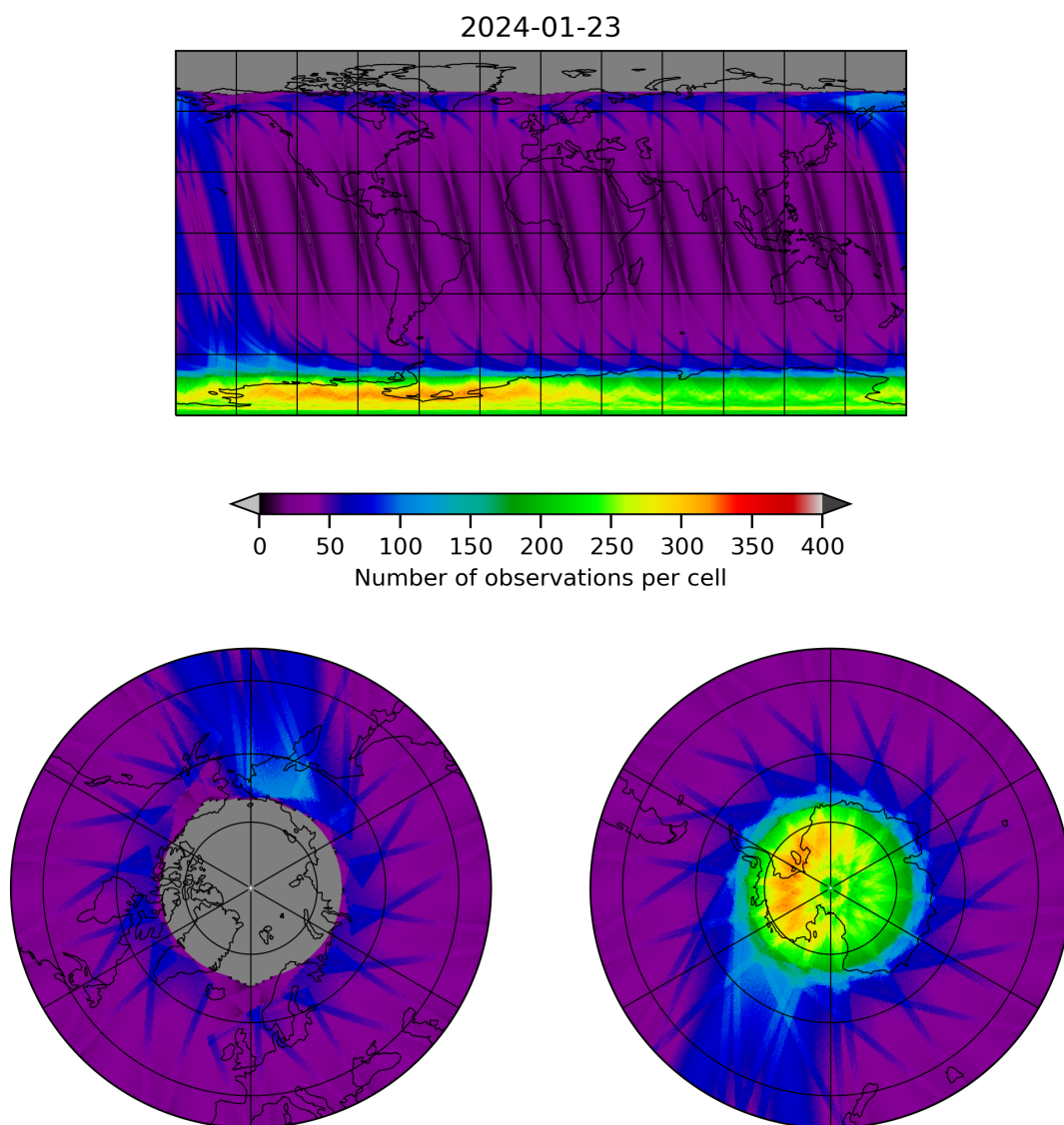
Figure 12: Map of the number of observations for 2024-01-22 to 2024-01-24
