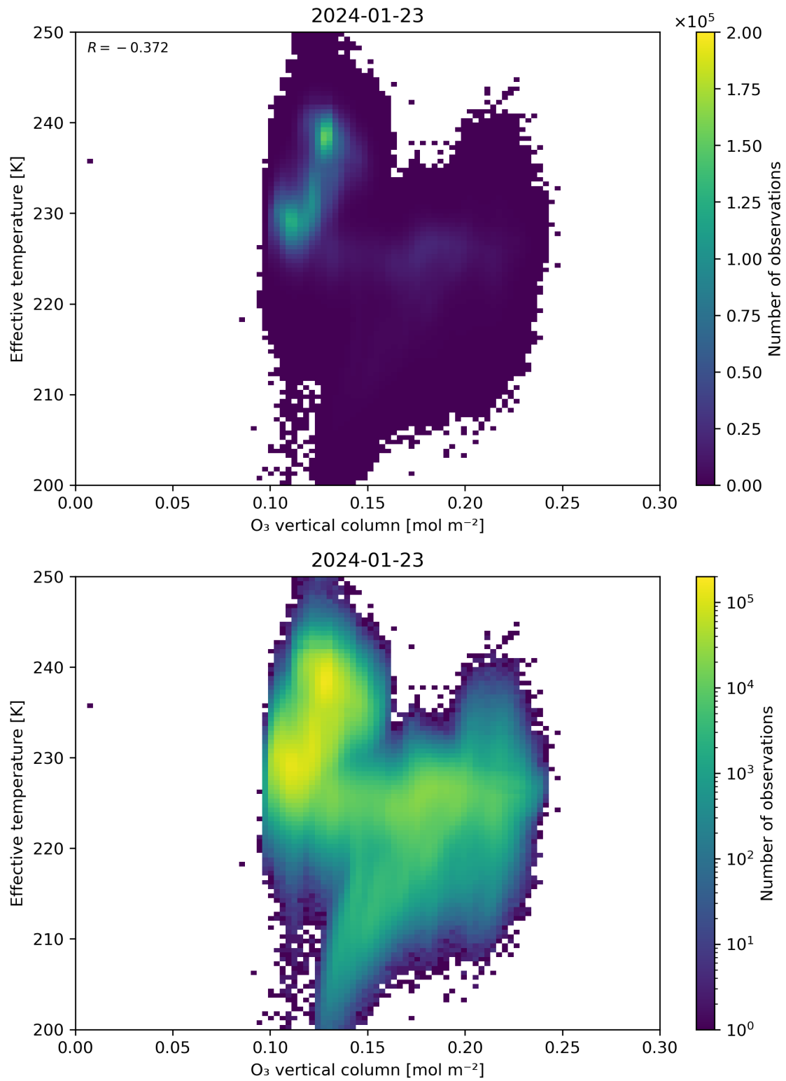
Figure 39: Scatter density plot of “O 3 vertical column” against “Effective temperature” for 2024-01-22 to 2024-01-24.
