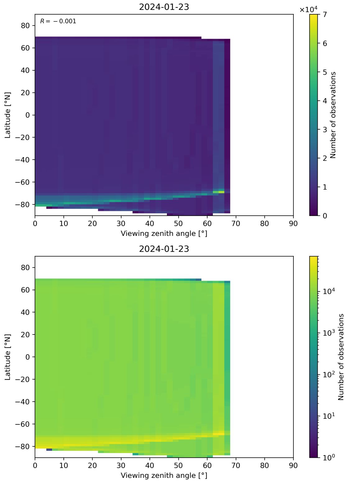
Figure 49: Scatter density plot of “Viewing zenith angle” against “Latitude” for 2024-01-22 to 2024-01-24.
