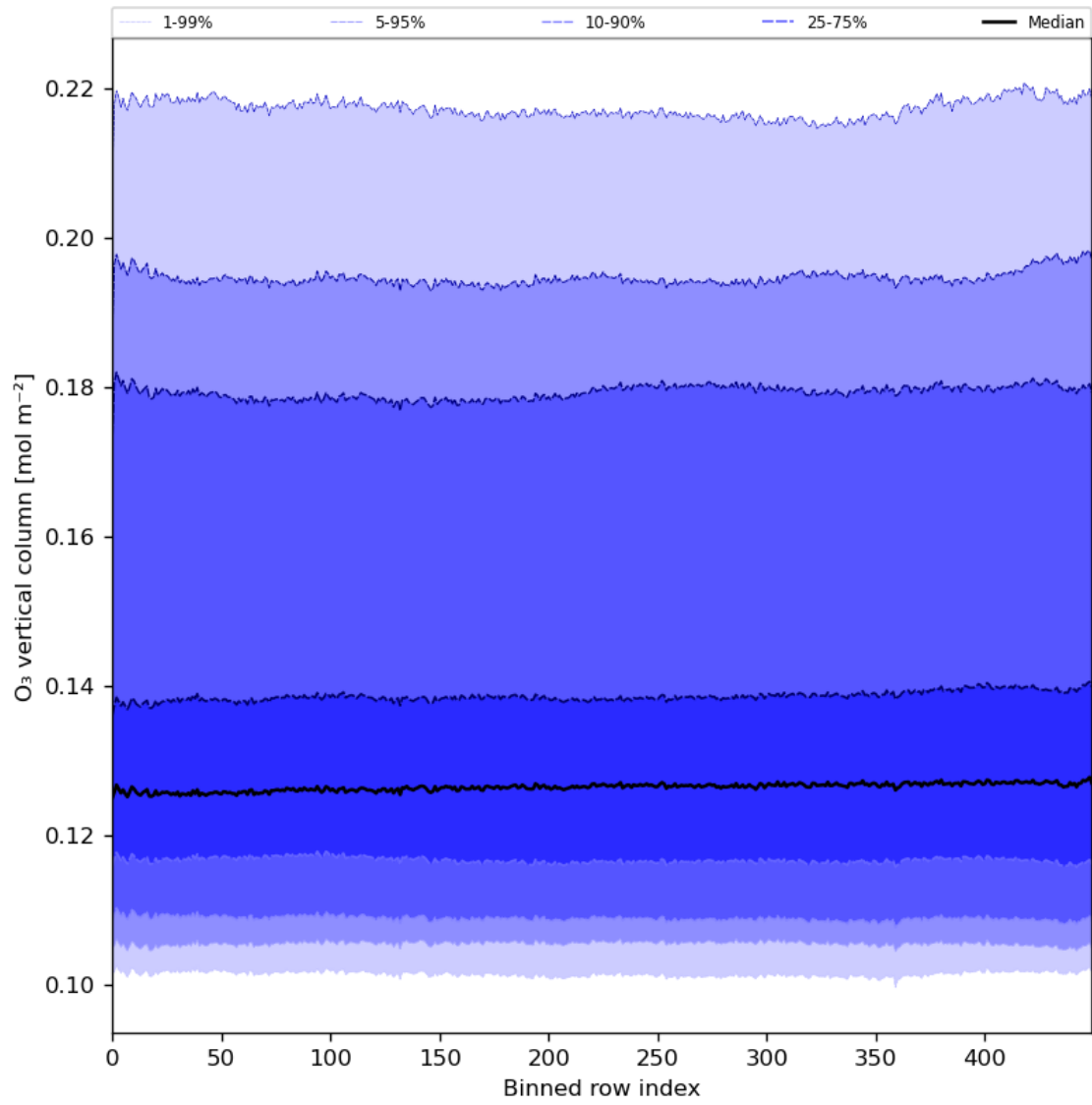
Figure 28: Along track statistics of “ \text{O}_3 vertical column” for 2024-01-22 to 2024-01-24
