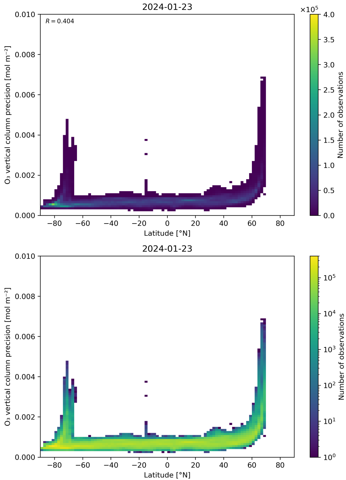
Figure 37: Scatter density plot of “Latitude” against “O 3 vertical column precision” for 2024-01-22 to 2024-01-24.
