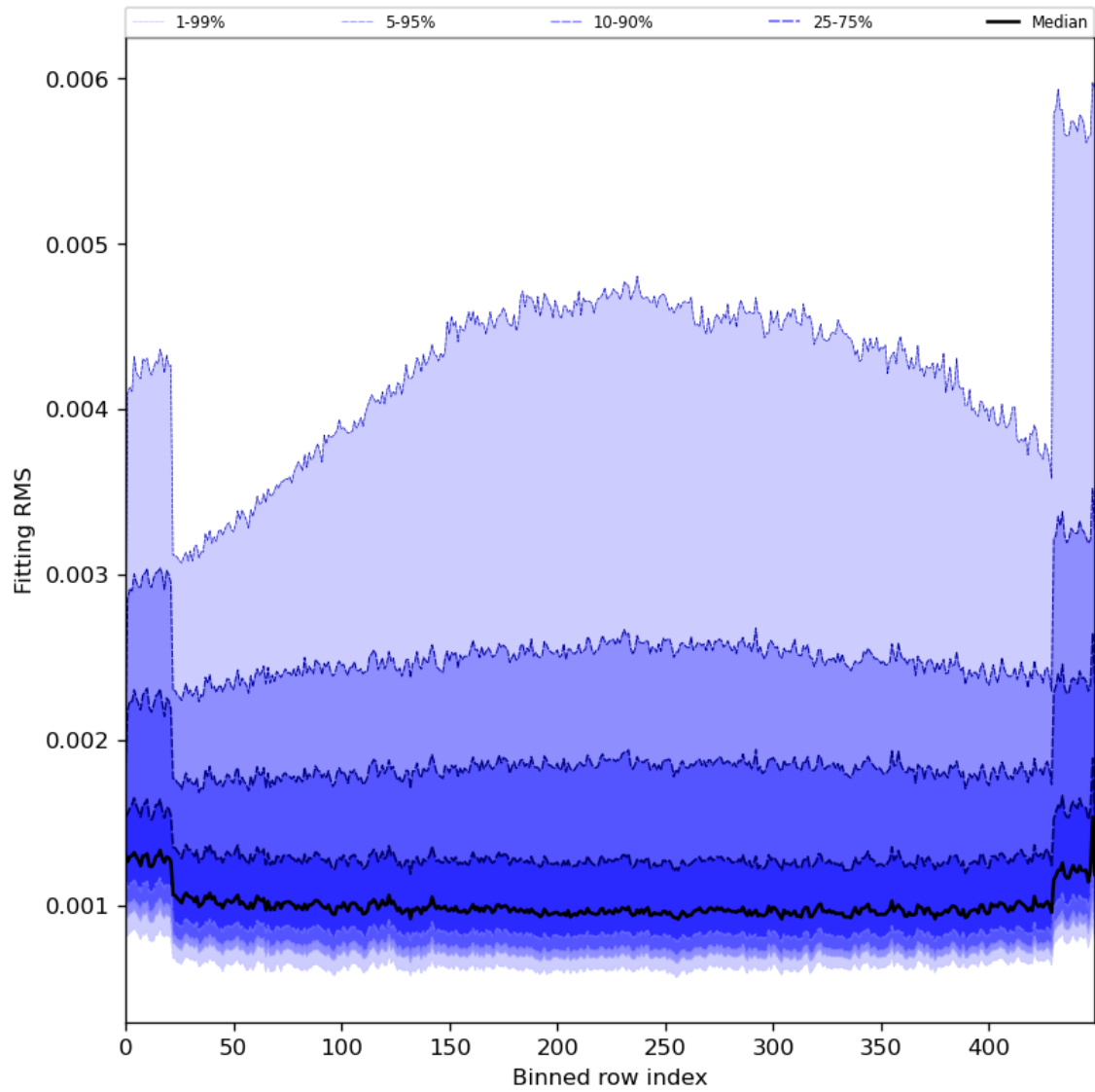
Figure 30: Along track statistics of “Fitting RMS” for 2024-01-22 to 2024-01-24
