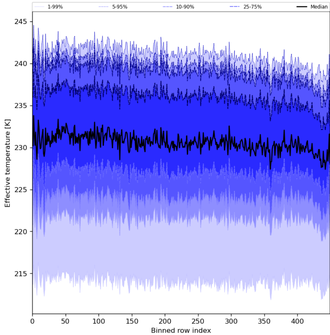
Figure 31: Along track statistics of “Effective temperature” for 2024-01-22 to 2024-01-24
