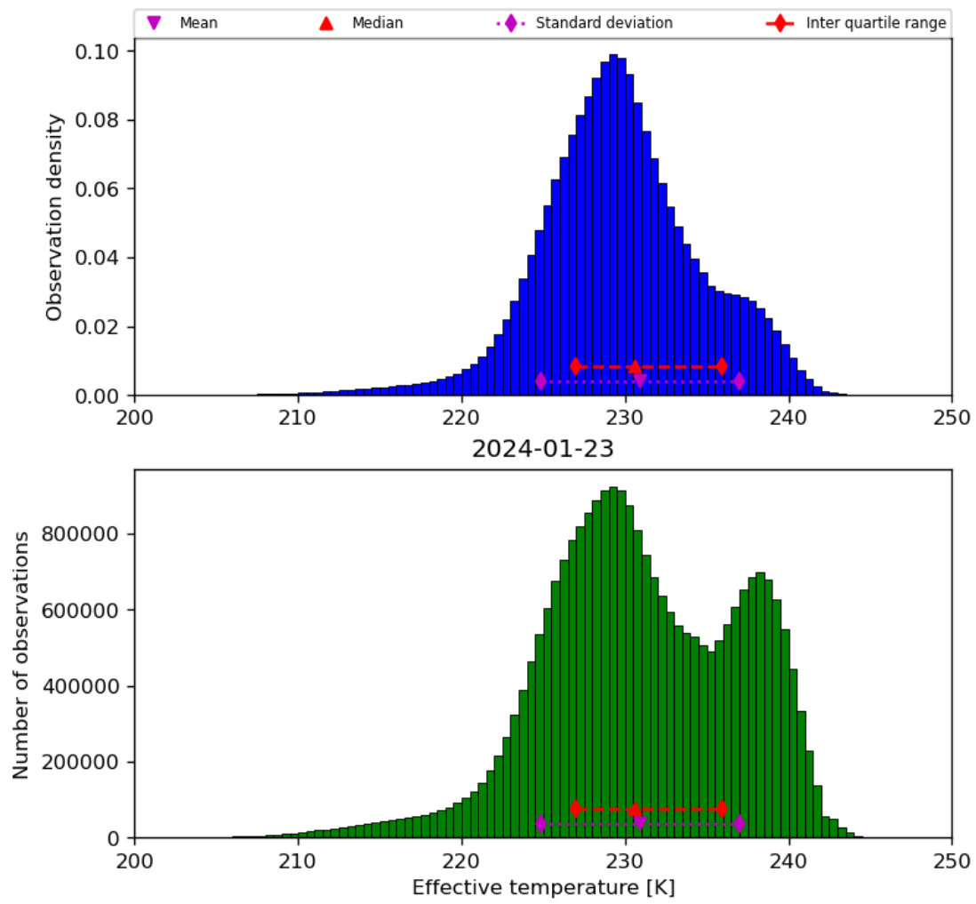
Figure 24: Histogram of “Effective temperature” for 2024-01-22 to 2024-01-24
