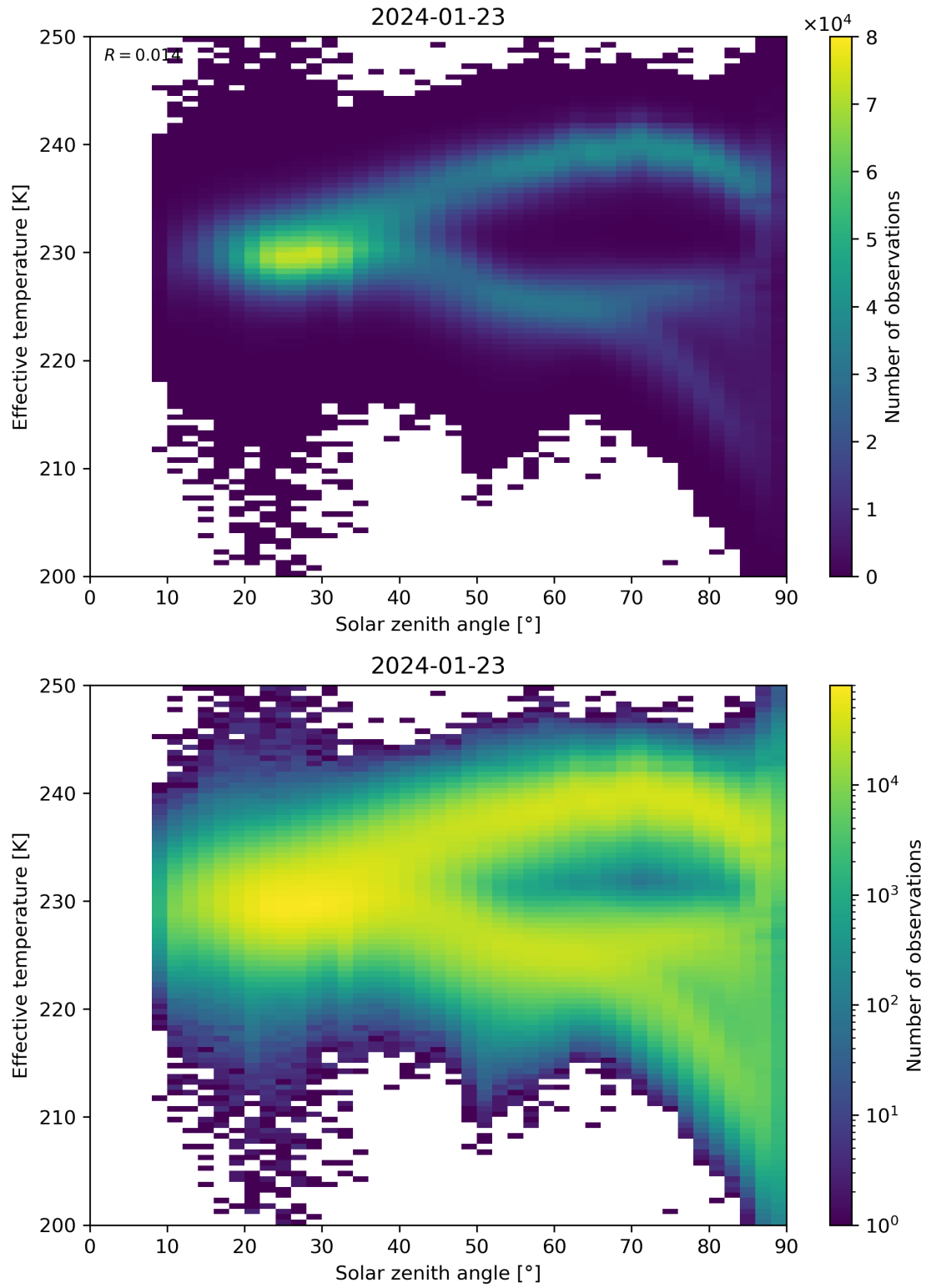
Figure 45: Scatter density plot of “Solar zenith angle” against “Effective temperature” for 2024-01-22 to 2024-01-24.
