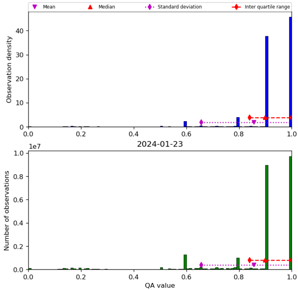
Figure 20: Histogram of “QA value” for 2024-01-22 to 2024-01-24
