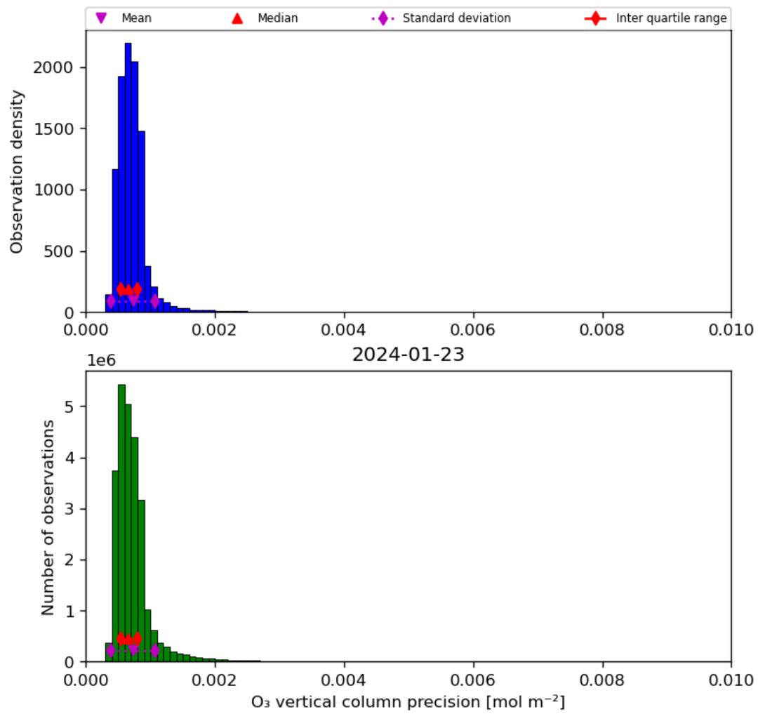
Figure 22: Histogram of “O 3 vertical column precision” for 2024-01-22 to 2024-01-24
