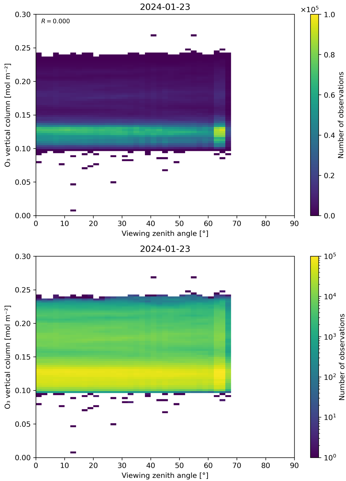
Figure 52: Scatter density plot of “Viewing zenith angle” against “O 3 vertical column” for 2024-01-22 to 2024-01-24.
