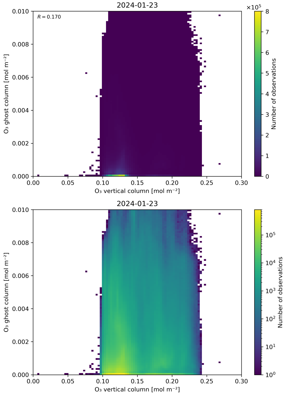
Figure 40: Scatter density plot of “O 3 vertical column” against “O 3 ghost column” for 2024-01-22 to 2024-01-24.
