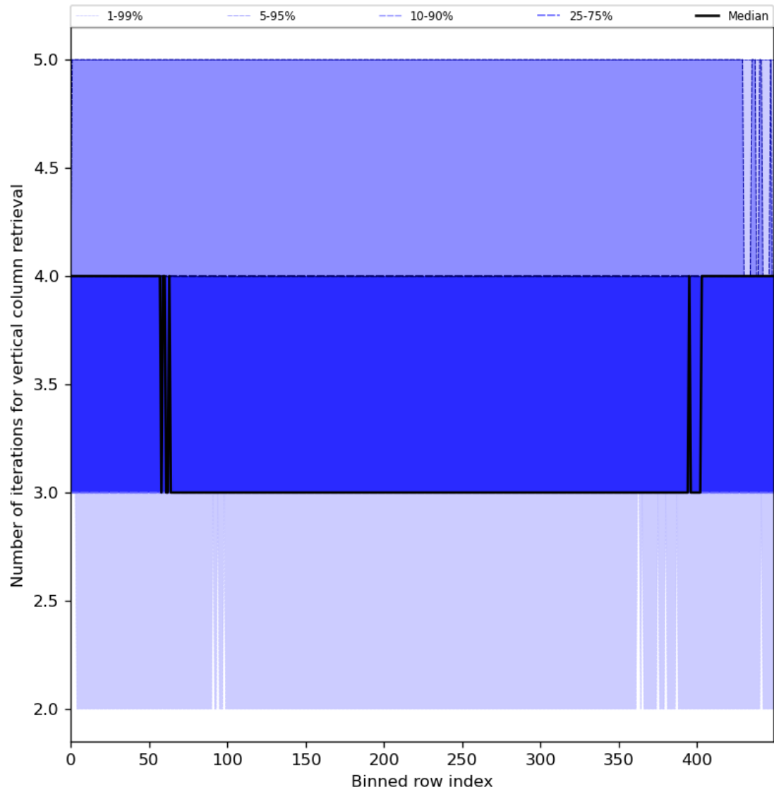
Figure 33: Along track statistics of “Number of iterations for vertical column retrieval” for 2024-01-22 to 2024-01-24
