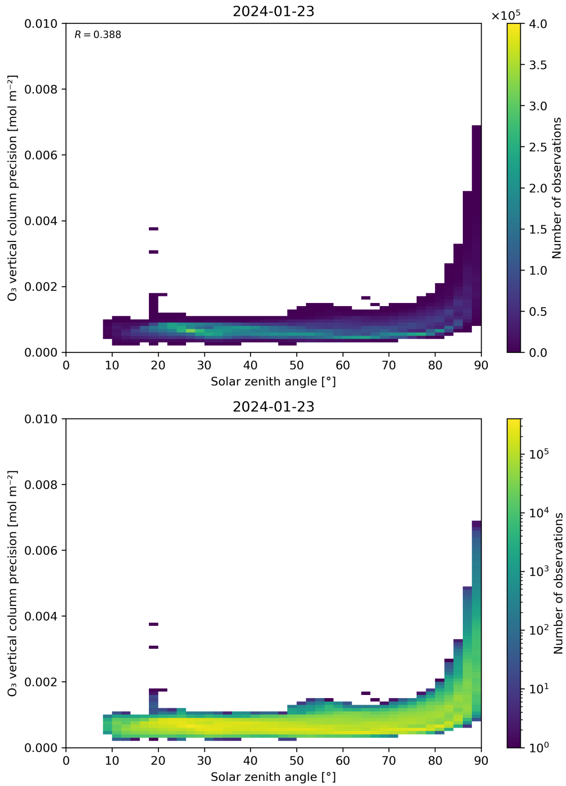
Figure 48: Scatter density plot of “Solar zenith angle” against “O 3 vertical column precision” for 2024-01-22 to 2024-01-24.
