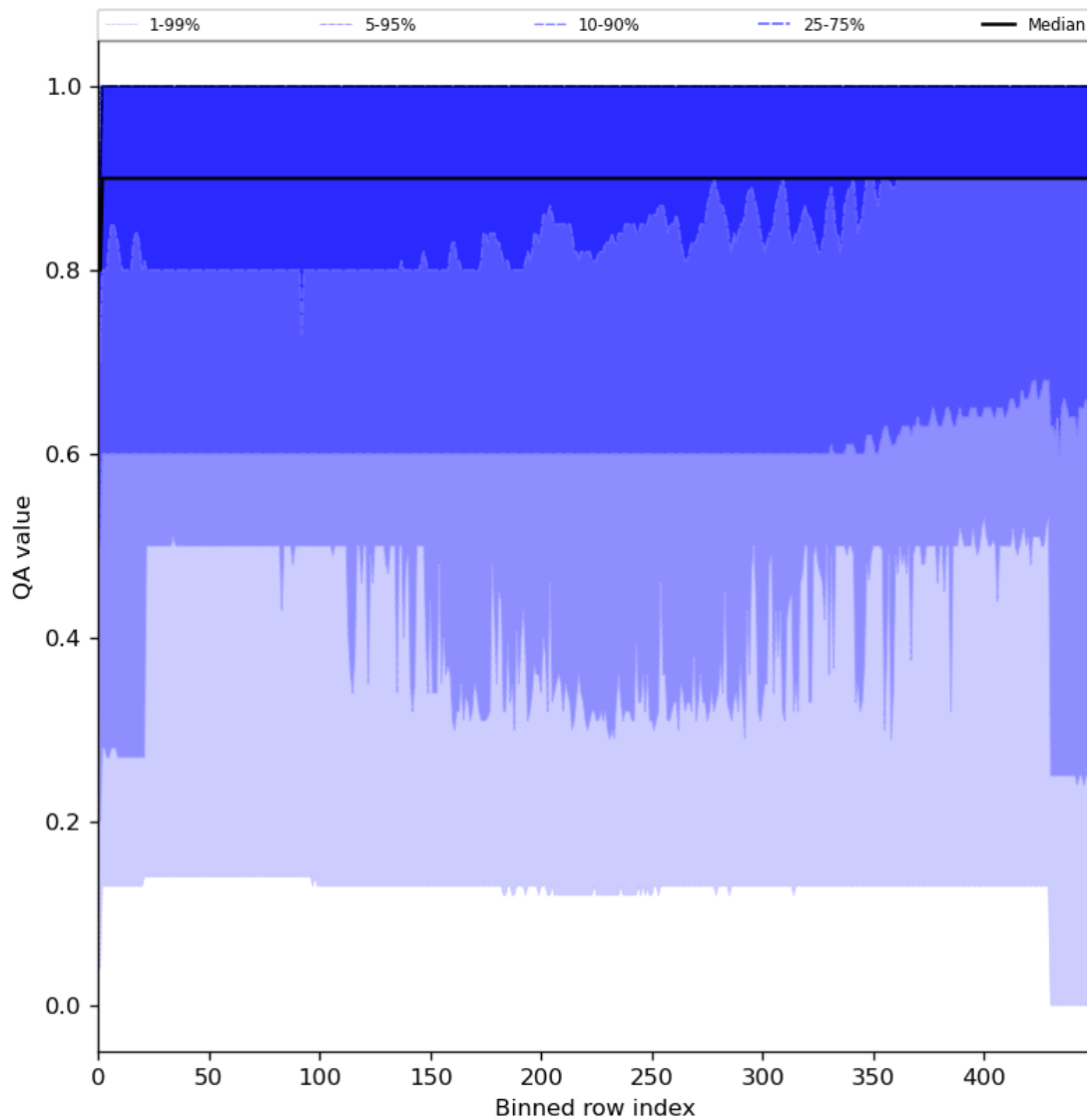
Figure 27: Along track statistics of “QA value” for 2024-01-22 to 2024-01-24
