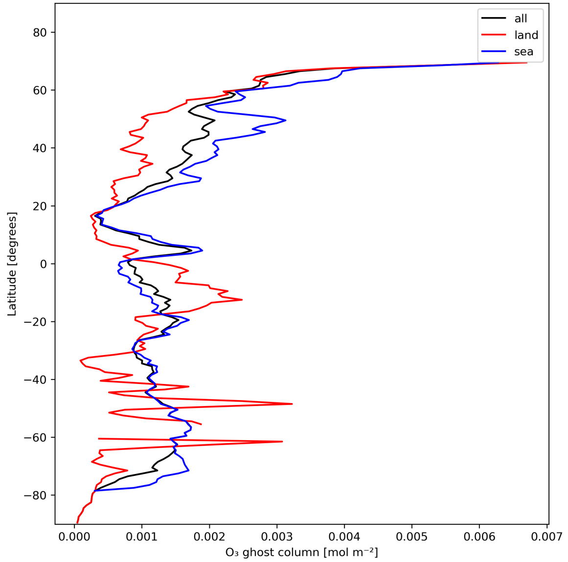
Figure 18: Zonal average of "O 3 ghost column" for 2024-01-22 to 2024-01-24.
