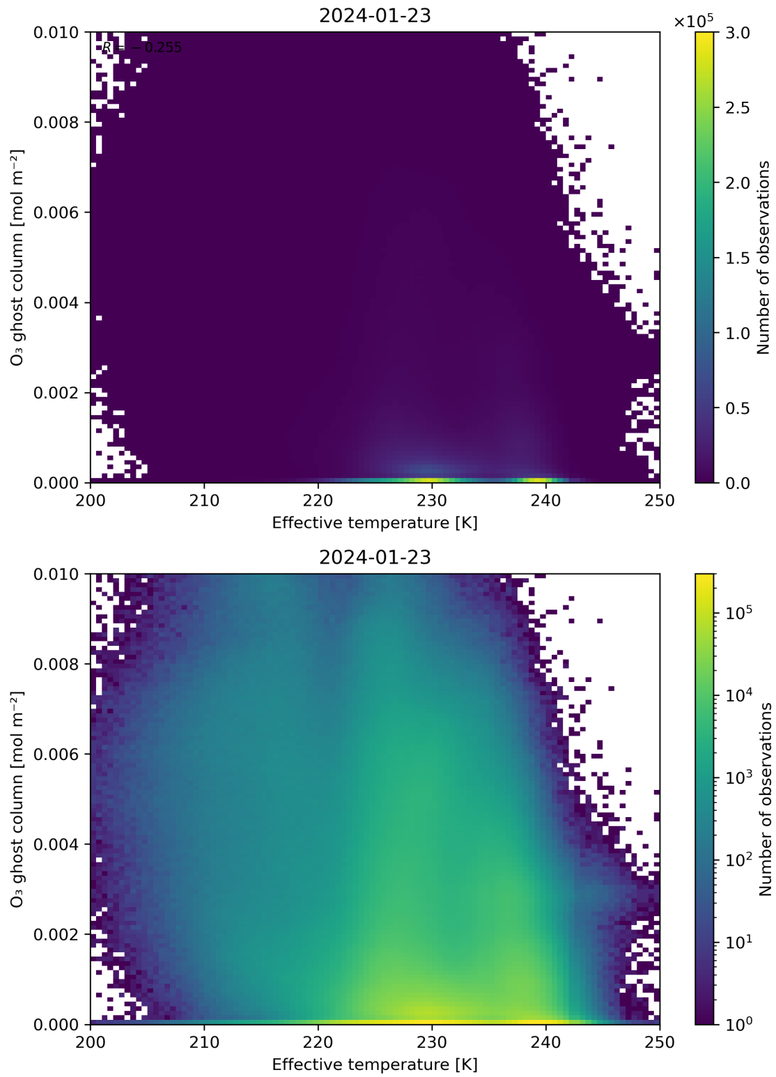
Figure 38: Scatter density plot of “Effective temperature” against “O 3 ghost column” for 2024-01-22 to 2024-01-24.
