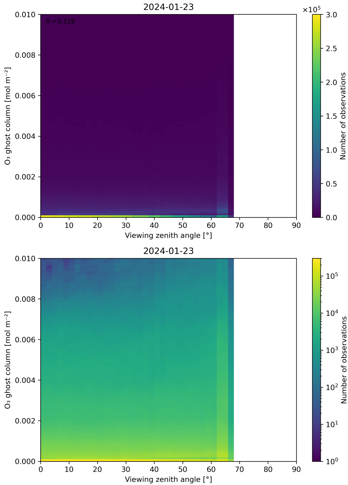
Figure 51: Scatter density plot of “Viewing zenith angle” against “O 3 ghost column” for 2024-01-22 to 2024-01-24.
