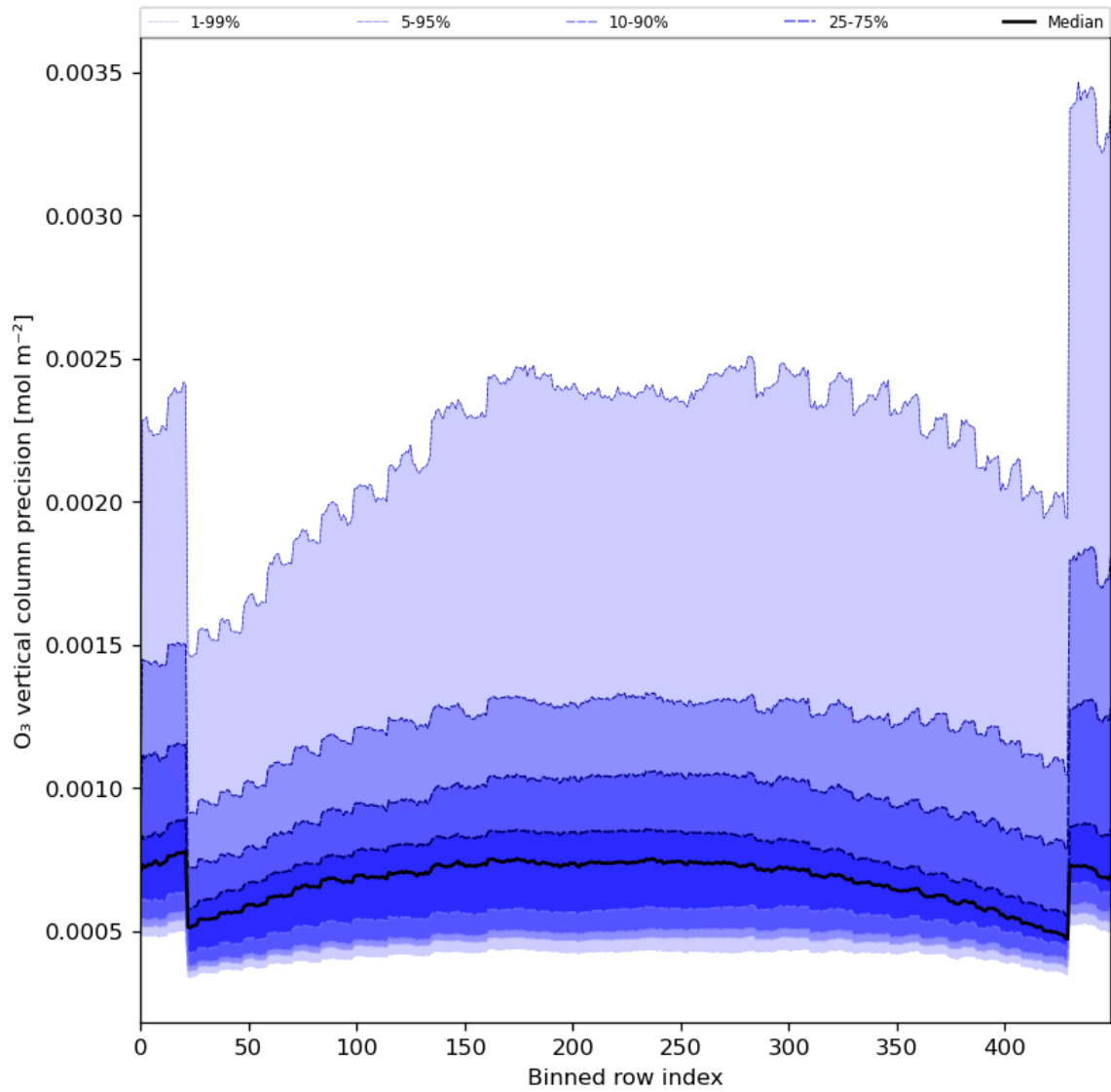
Figure 29: Along track statistics of “O 3 vertical column precision” for 2024-01-22 to 2024-01-24
