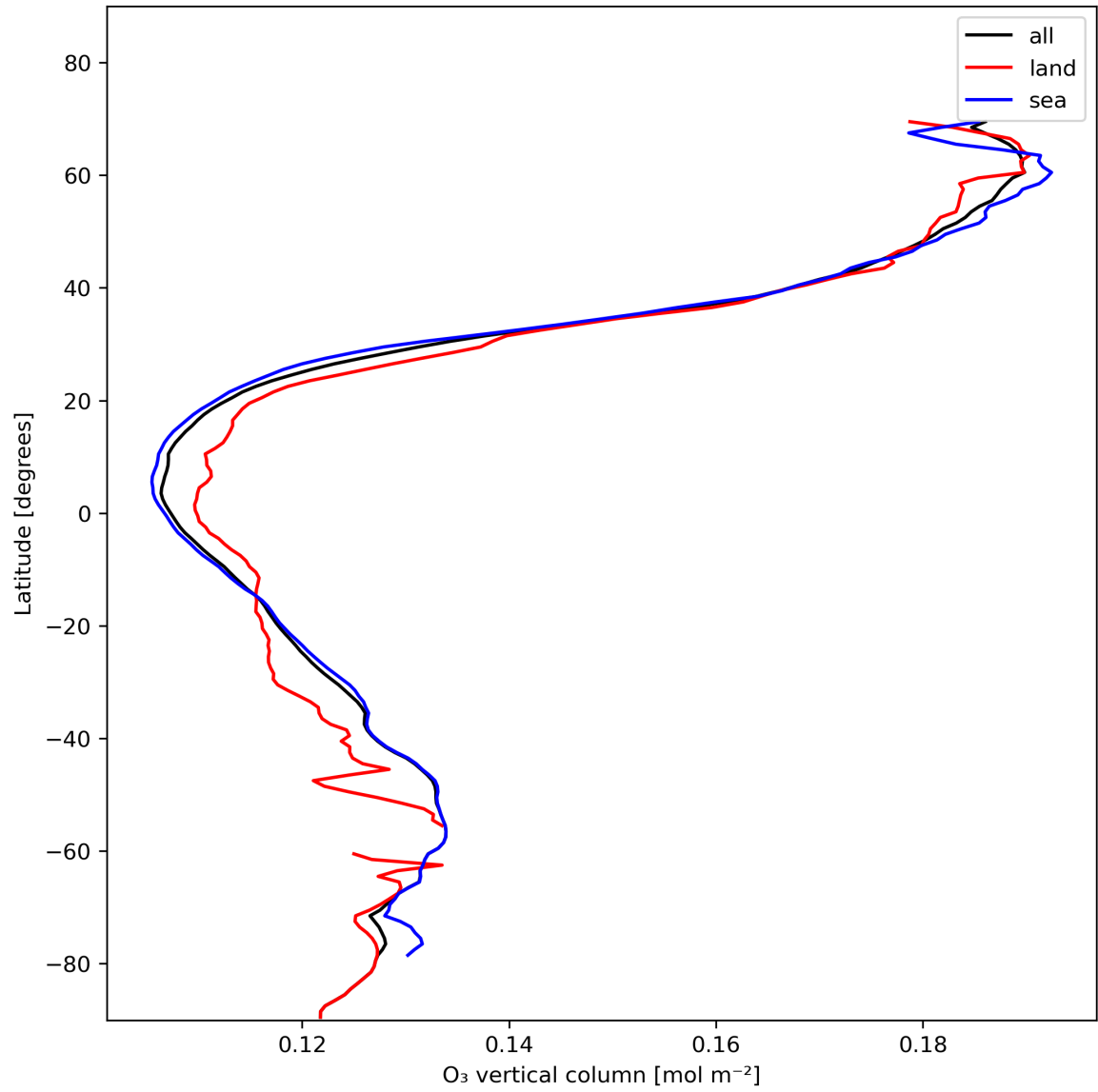
Figure 14: Zonal average of “O 3 vertical column” for 2024-01-22 to 2024-01-24.
