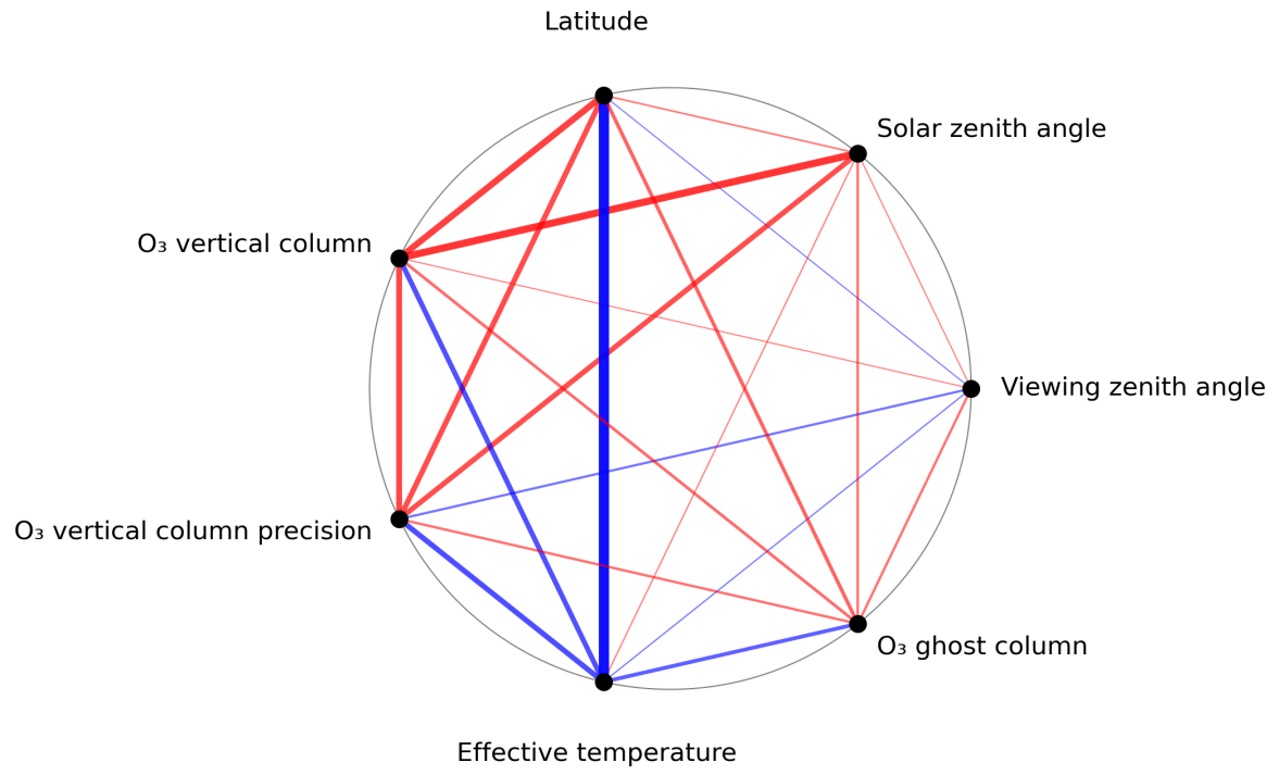
Figure 1: Map of correlation graph for 2024-01-22 to 2024-01-24.
