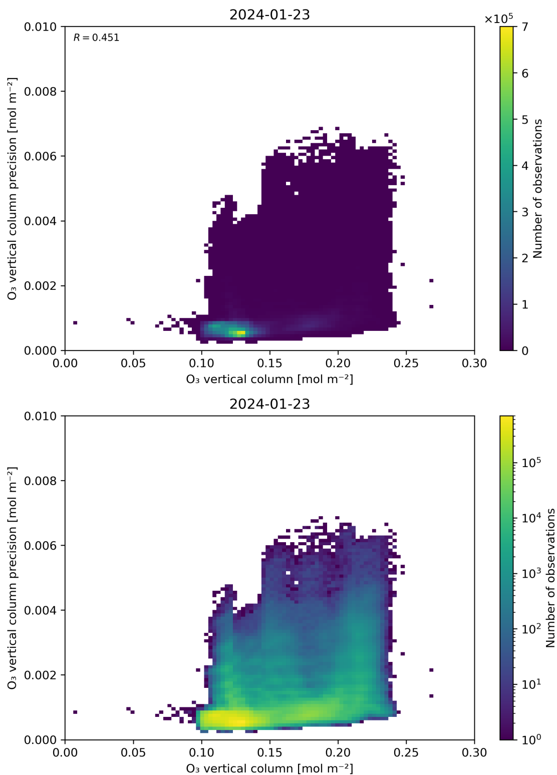
Figure 41: Scatter density plot of “O 3 vertical column” against “O 3 vertical column precision” for 2024-01-22 to 2024-01-24.
