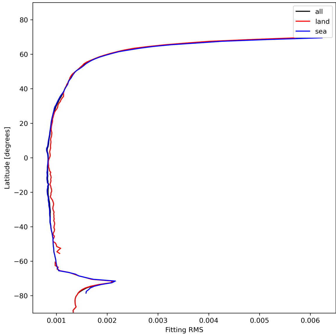
Figure 16: Zonal average of “Fitting RMS” for 2024-01-22 to 2024-01-24.
