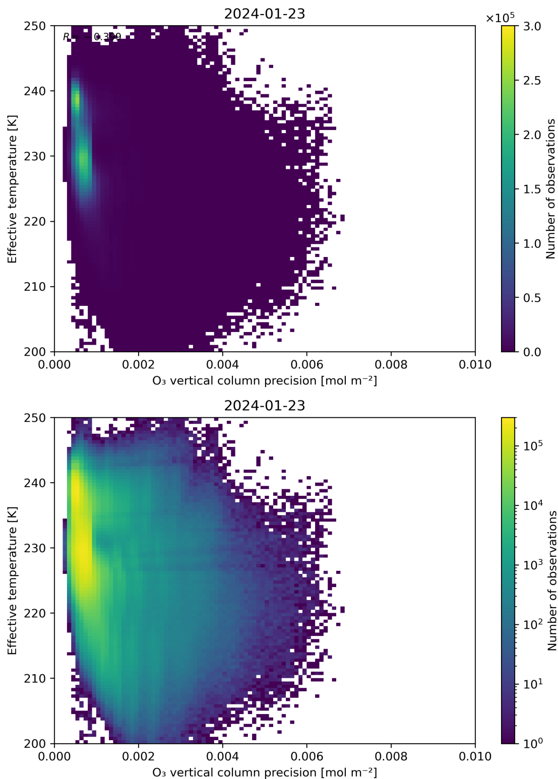
Figure 42: Scatter density plot of “O 3 vertical column precision” against “Effective temperature” for 2024-01-22 to 2024-01-24.
