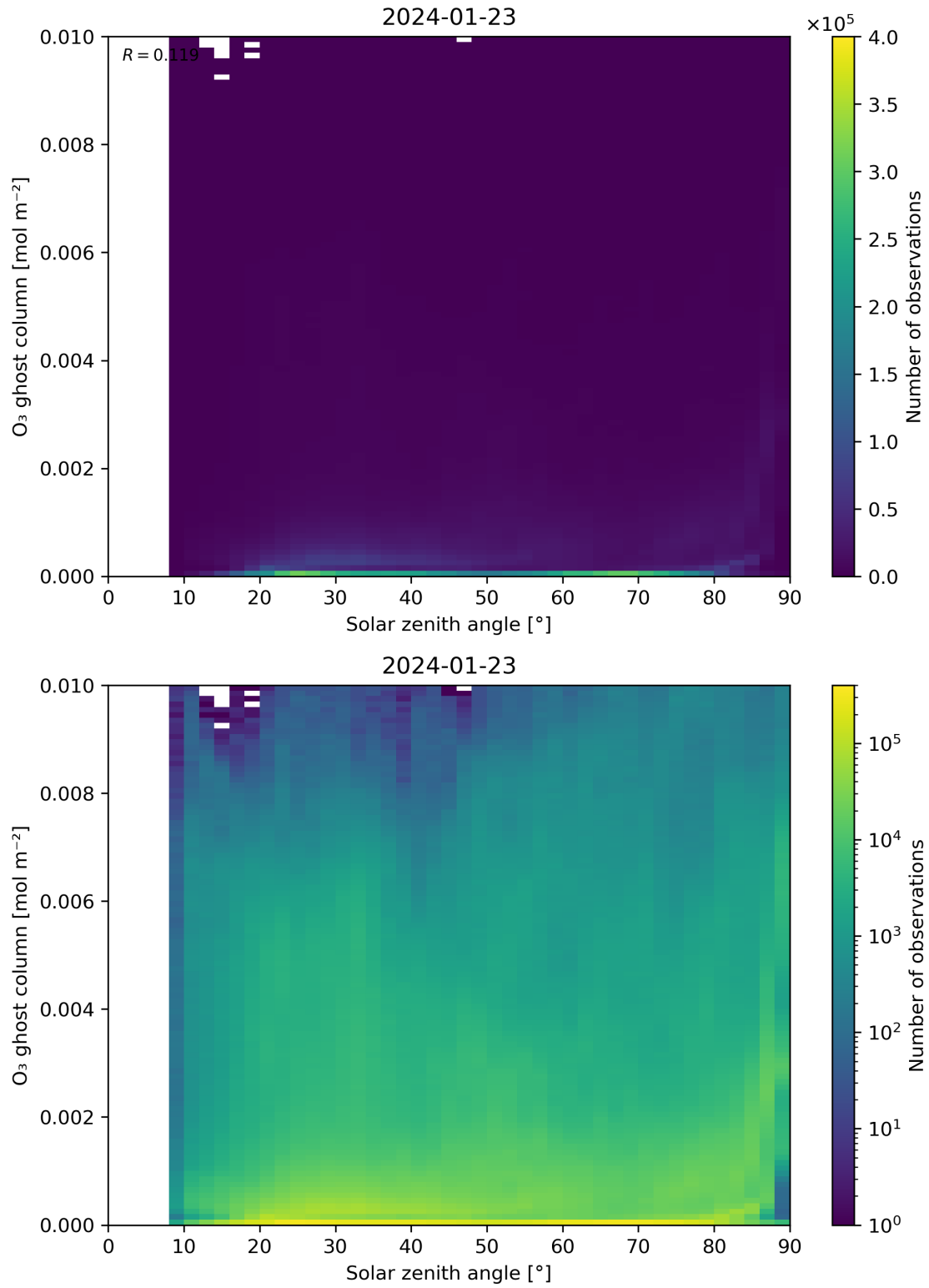
Figure 46: Scatter density plot of “Solar zenith angle” against “O 3 ghost column” for 2024-01-22 to 2024-01-24.
