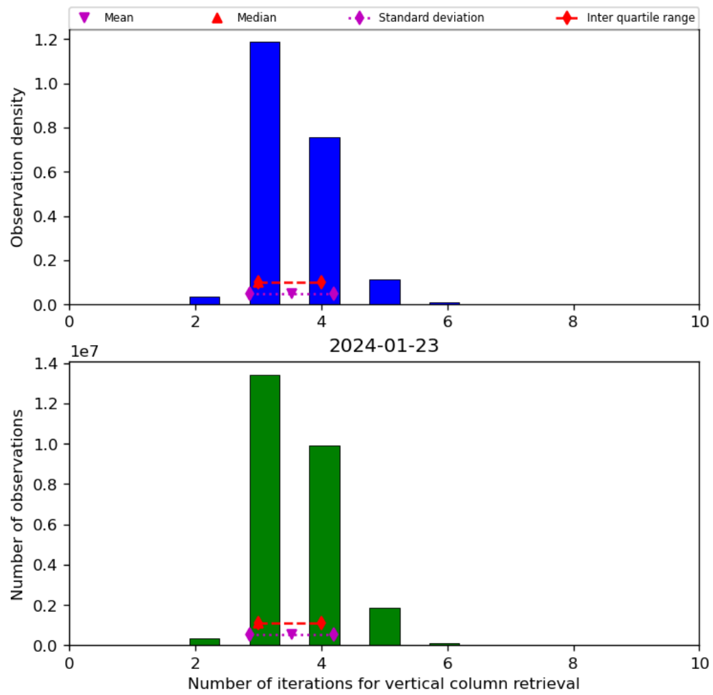
Figure 26: Histogram of “Number of iterations for vertical column retrieval” for 2024-01-22 to 2024-01-24
