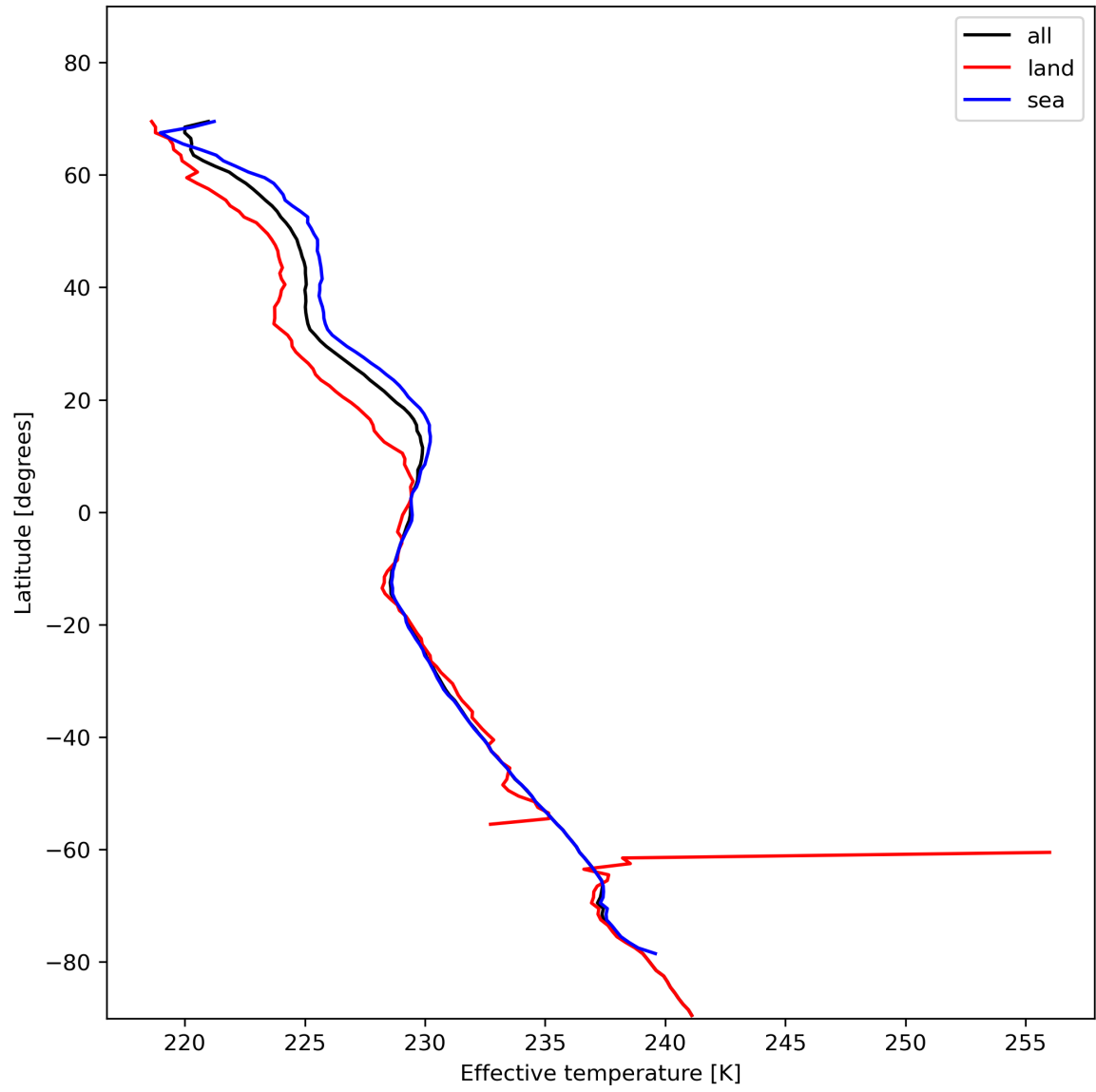
Figure 17: Zonal average of “Effective temperature” for 2024-01-22 to 2024-01-24.
