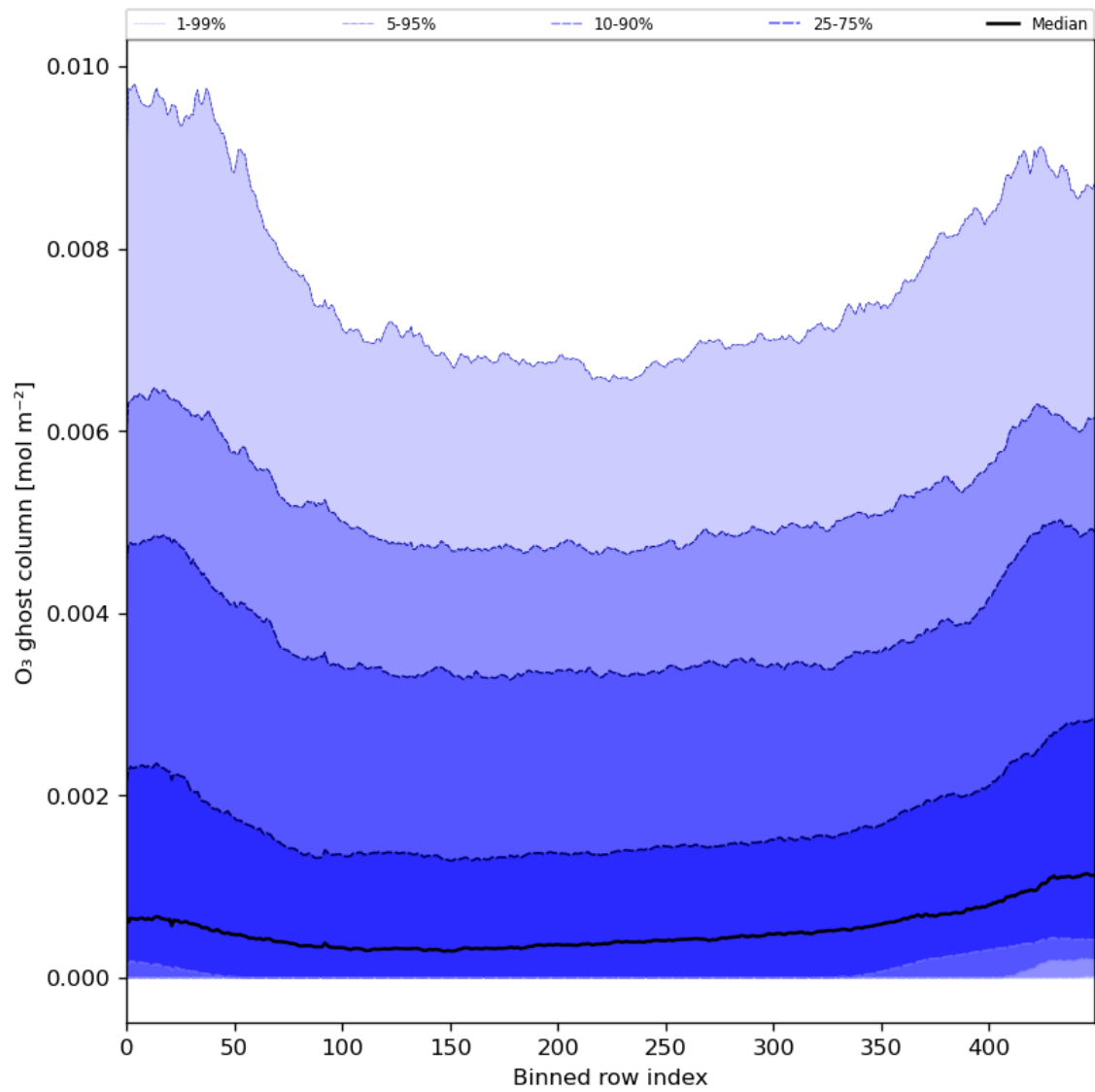
Figure 32: Along track statistics of “O 3 ghost column” for 2024-01-22 to 2024-01-24
