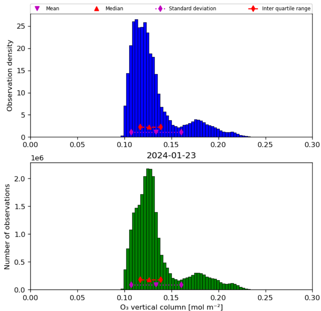
Figure 21: Histogram of “O 3 vertical column” for 2024-01-22 to 2024-01-24
