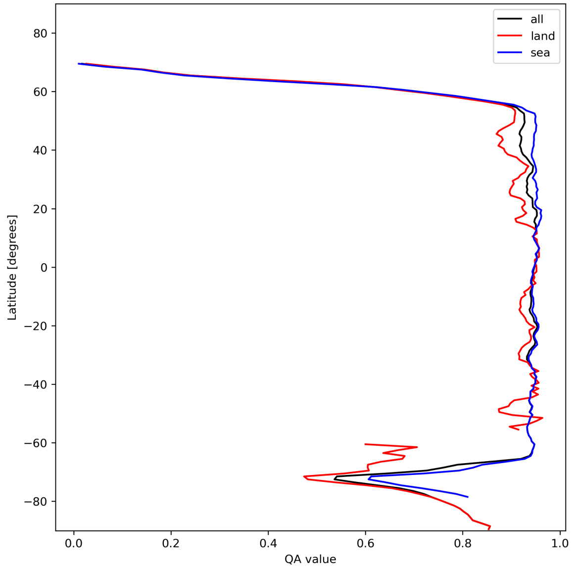
Figure 13: Zonal average of “QA value” for 2024-01-22 to 2024-01-24.
