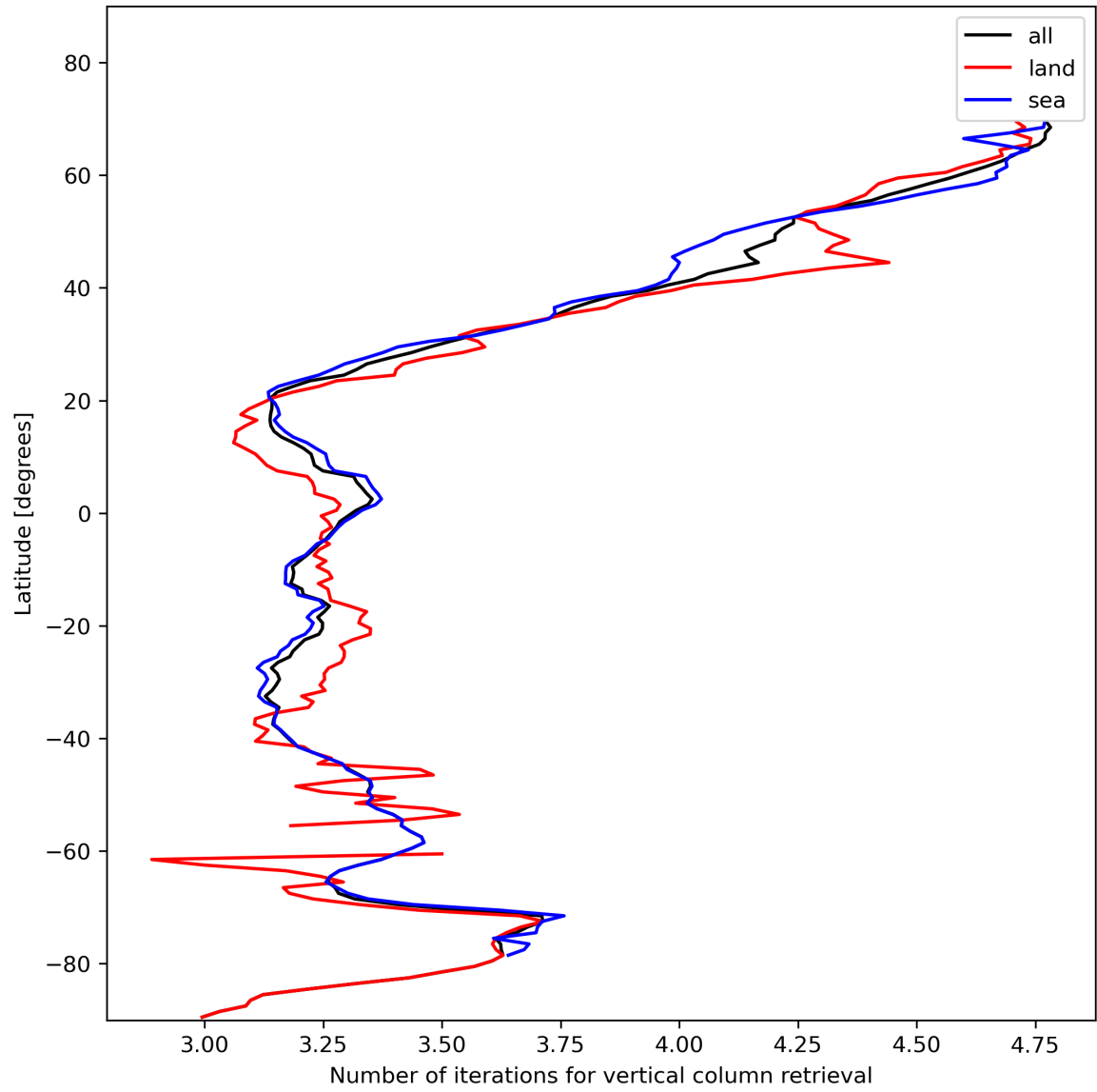
Figure 19: Zonal average of “Number of iterations for vertical column retrieval” for 2024-01-22 to 2024-01-24.
