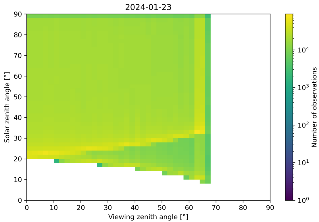
Figure 54: Scatter density plot of “Viewing zenith angle” against “Solar zenith angle” for 2024-01-22 to 2024-01-24.
