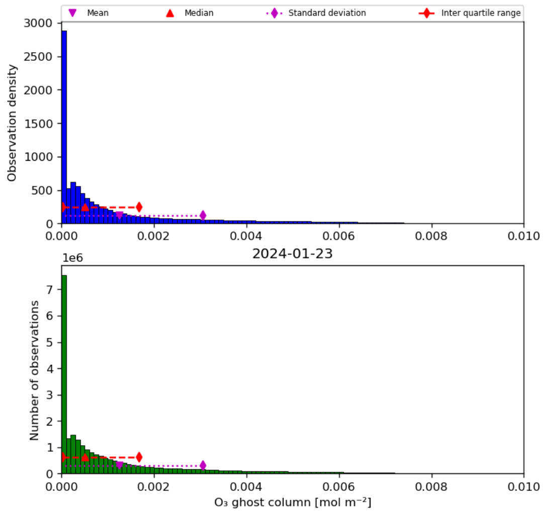
Figure 25: Histogram of “O 3 ghost column” for 2024-01-22 to 2024-01-24
