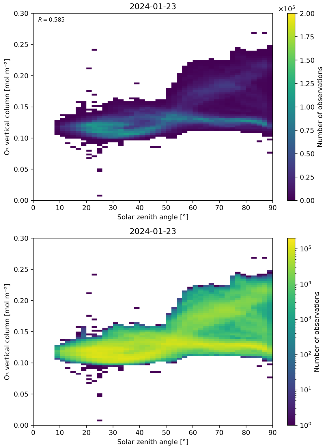
Figure 47: Scatter density plot of “Solar zenith angle” against “O 3 vertical column” for 2024-01-22 to 2024-01-24.
