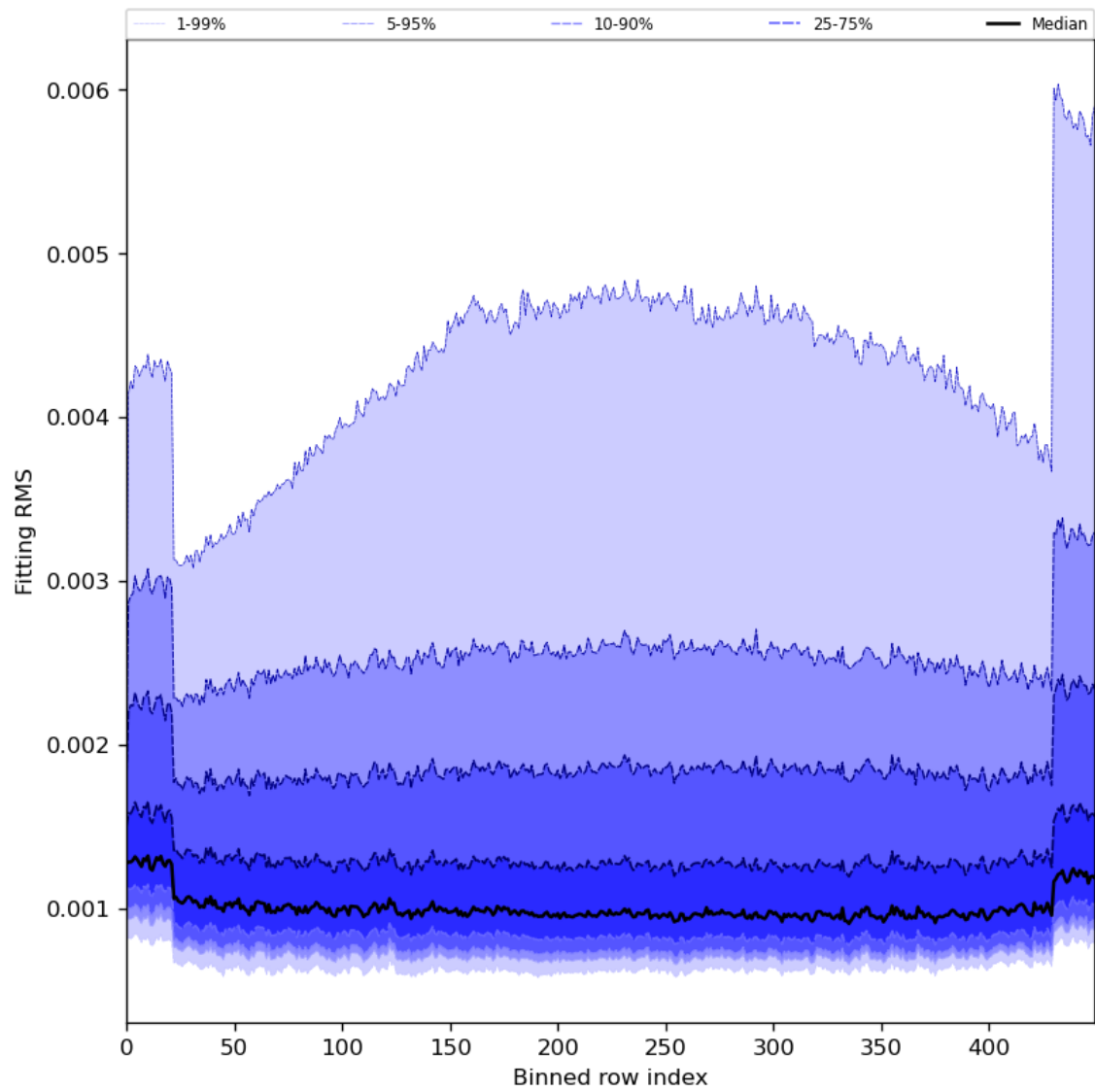
Figure 30: Along track statistics of “Fitting RMS” for 2024-01-23 to 2024-01-25
