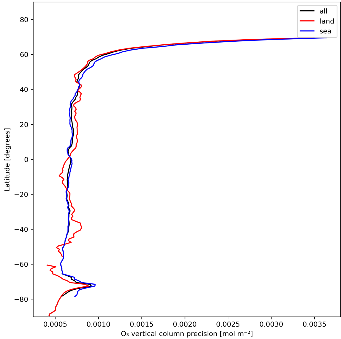
Figure 15: Zonal average of “O 3 vertical column precision” for 2024-01-23 to 2024-01-25.
