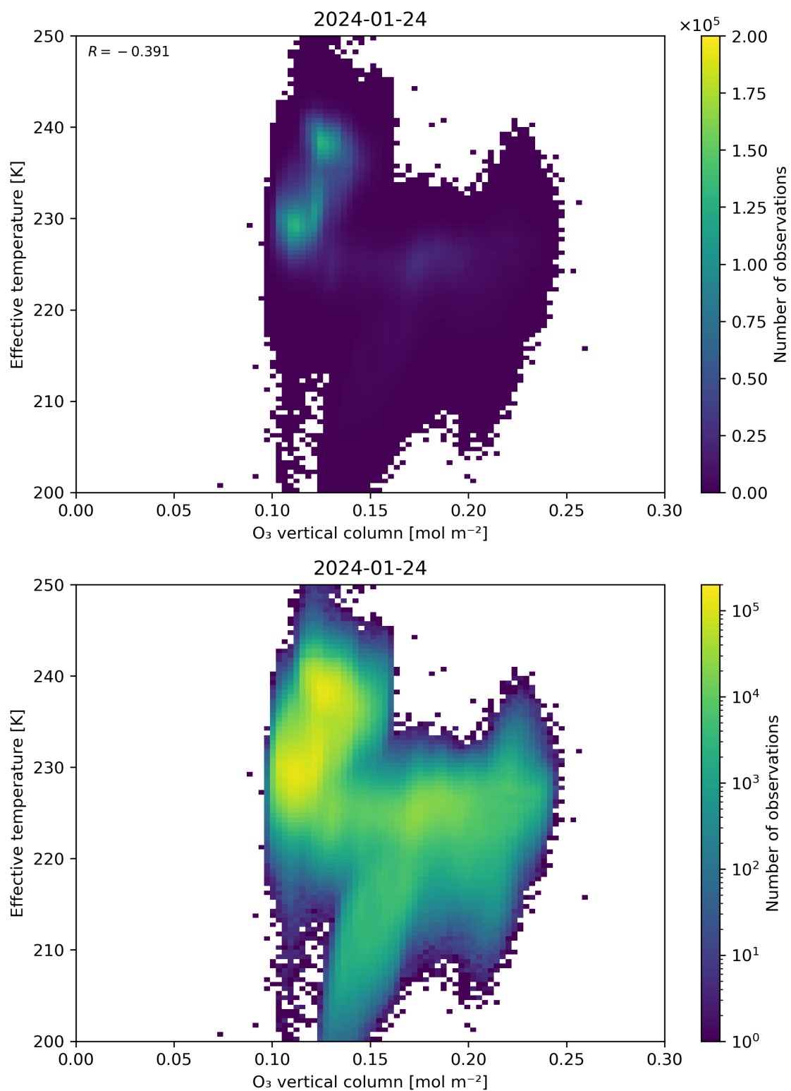
Figure 39: Scatter density plot of “O 3 vertical column” against “Effective temperature” for 2024-01-23 to 2024-01-25.
