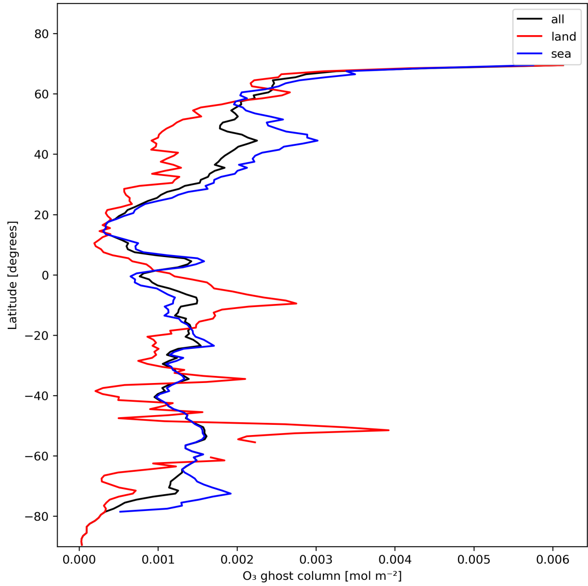
Figure 18: Zonal average of “O 3 ghost column” for 2024-01-23 to 2024-01-25.
