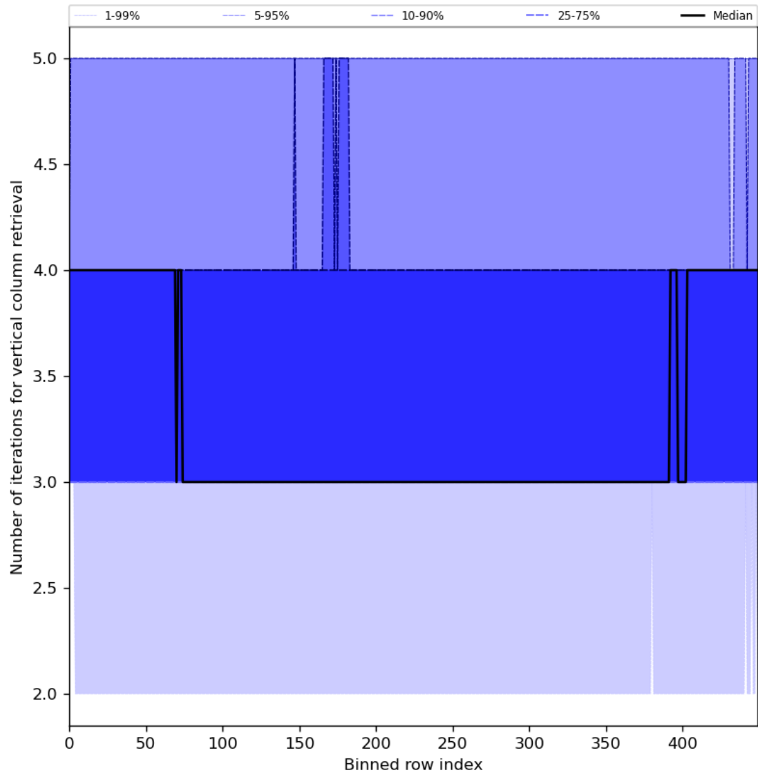
Figure 33: Along track statistics of “Number of iterations for vertical column retrieval” for 2024-01-23 to 2024-01-25
