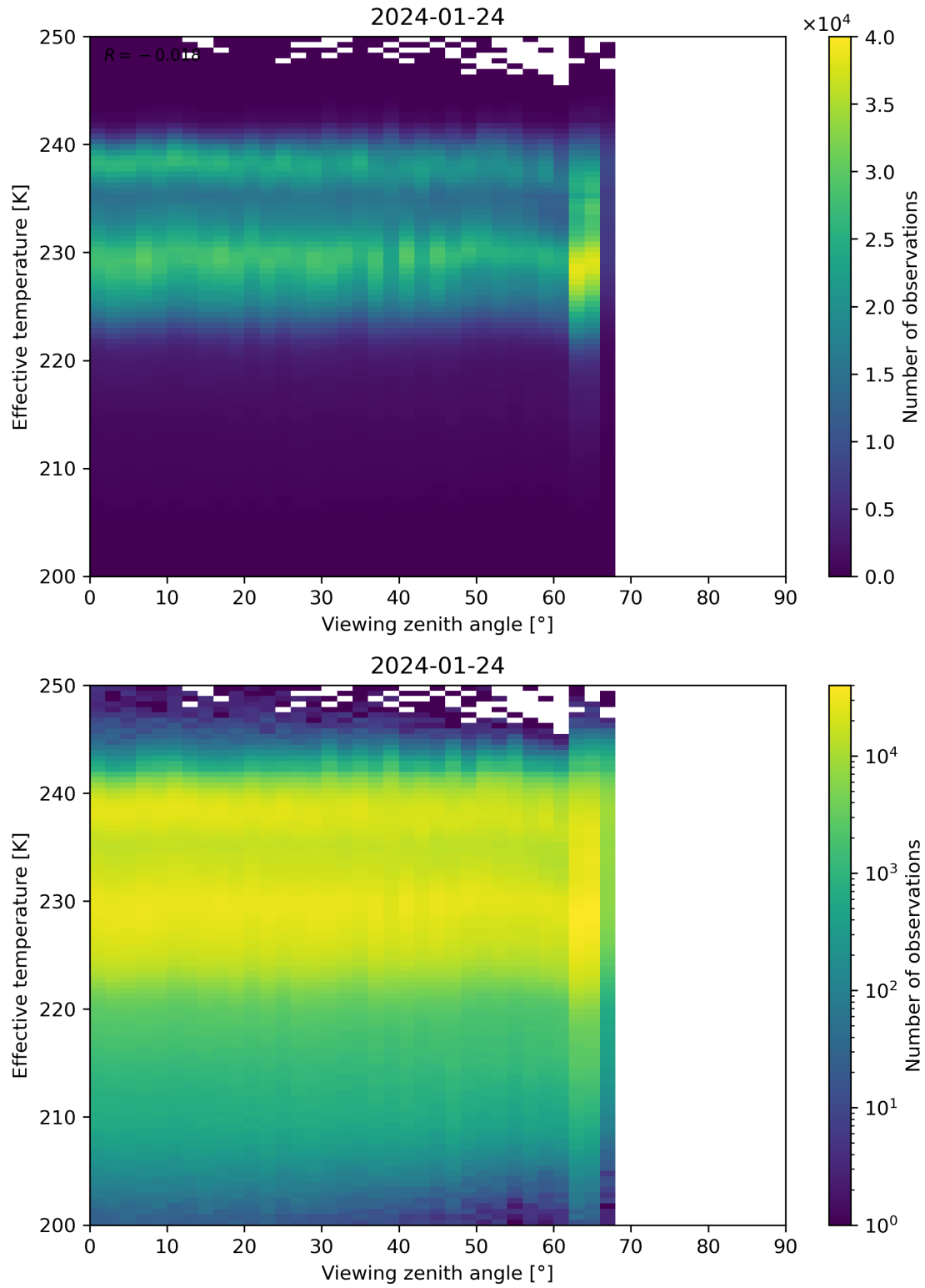
Figure 50: Scatter density plot of “Viewing zenith angle” against “Effective temperature” for 2024-01-23 to 2024-01-25.
