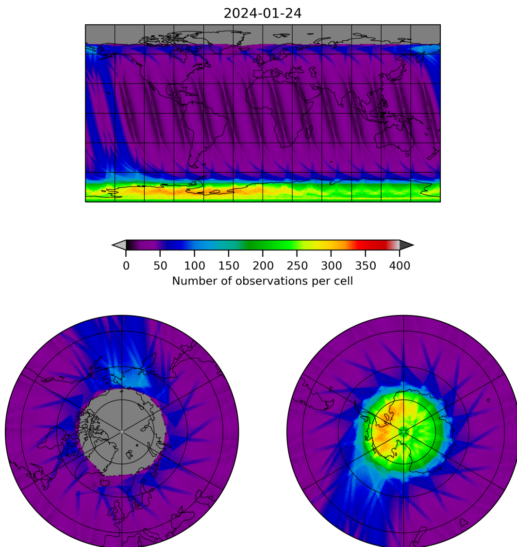
Figure 12: Map of the number of observations for 2024-01-23 to 2024-01-25
