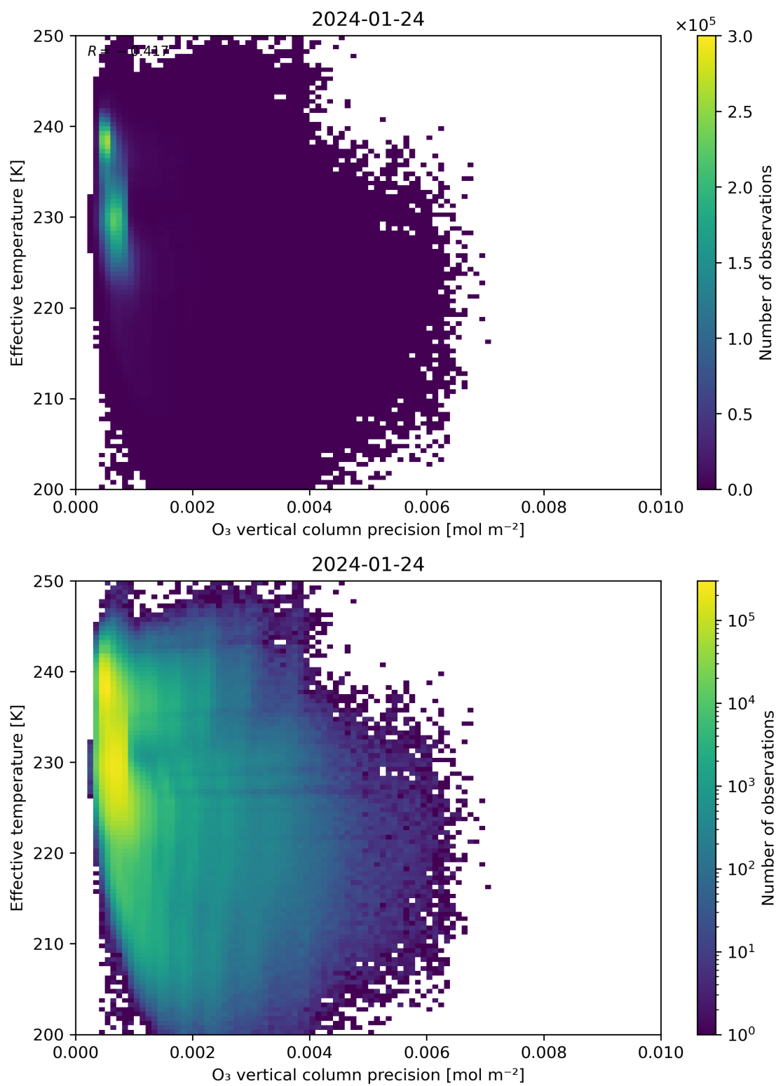
Figure 42: Scatter density plot of “O 3 vertical column precision” against “Effective temperature” for 2024-01-23 to 2024-01-25.
