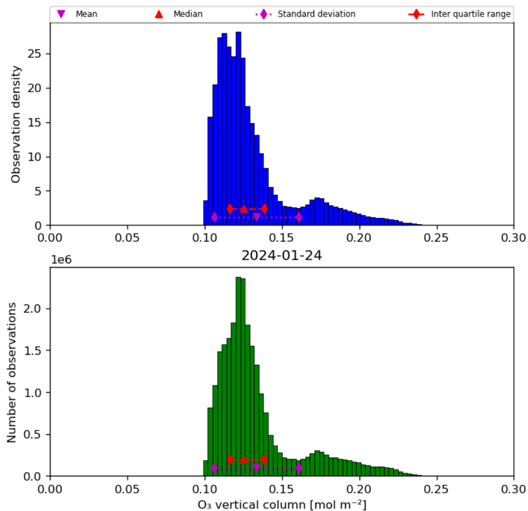
Figure 21: Histogram of “O 3 vertical column” for 2024-01-23 to 2024-01-25
