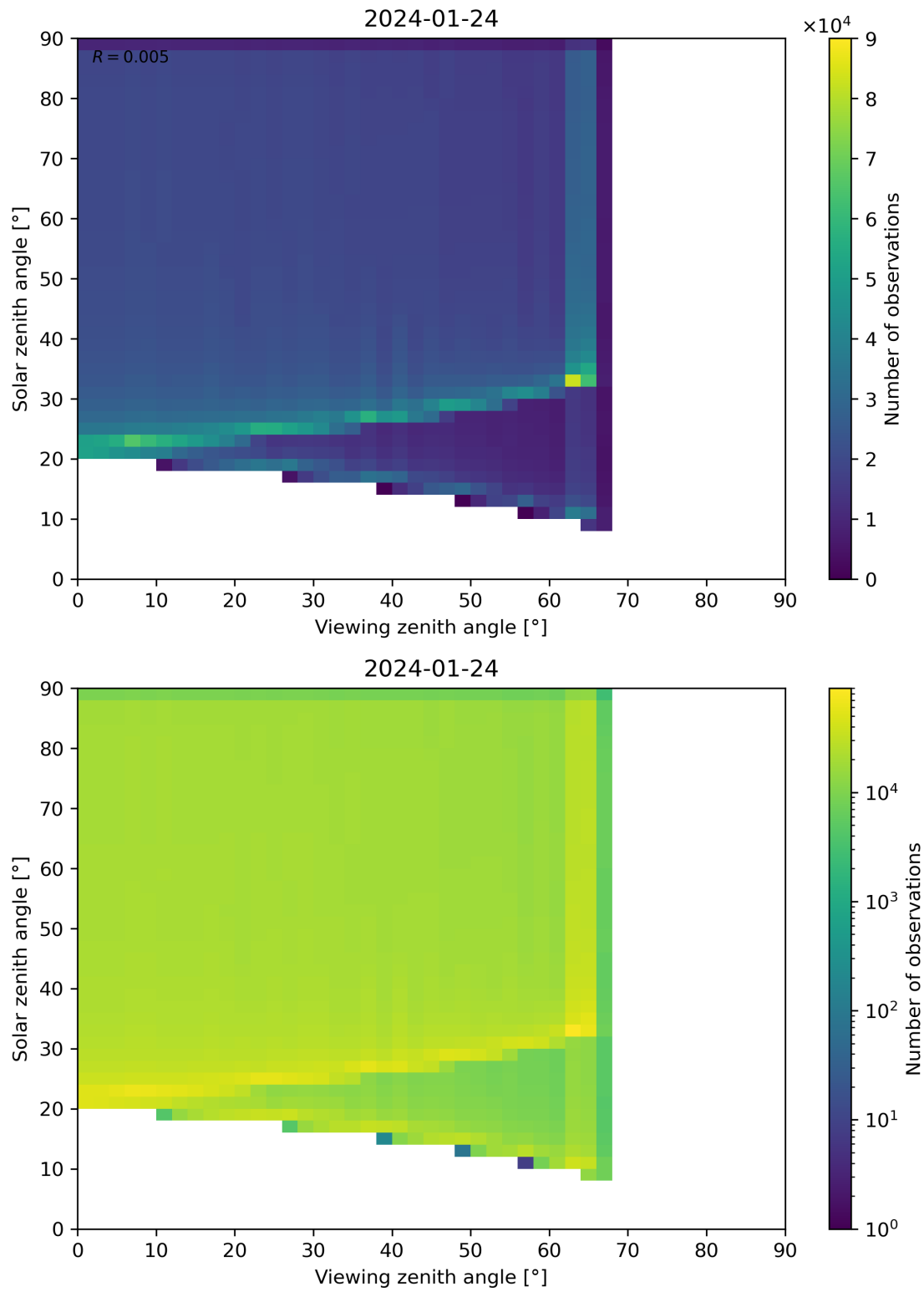
Figure 54: Scatter density plot of “Viewing zenith angle” against “Solar zenith angle” for 2024-01-23 to 2024-01-25.
