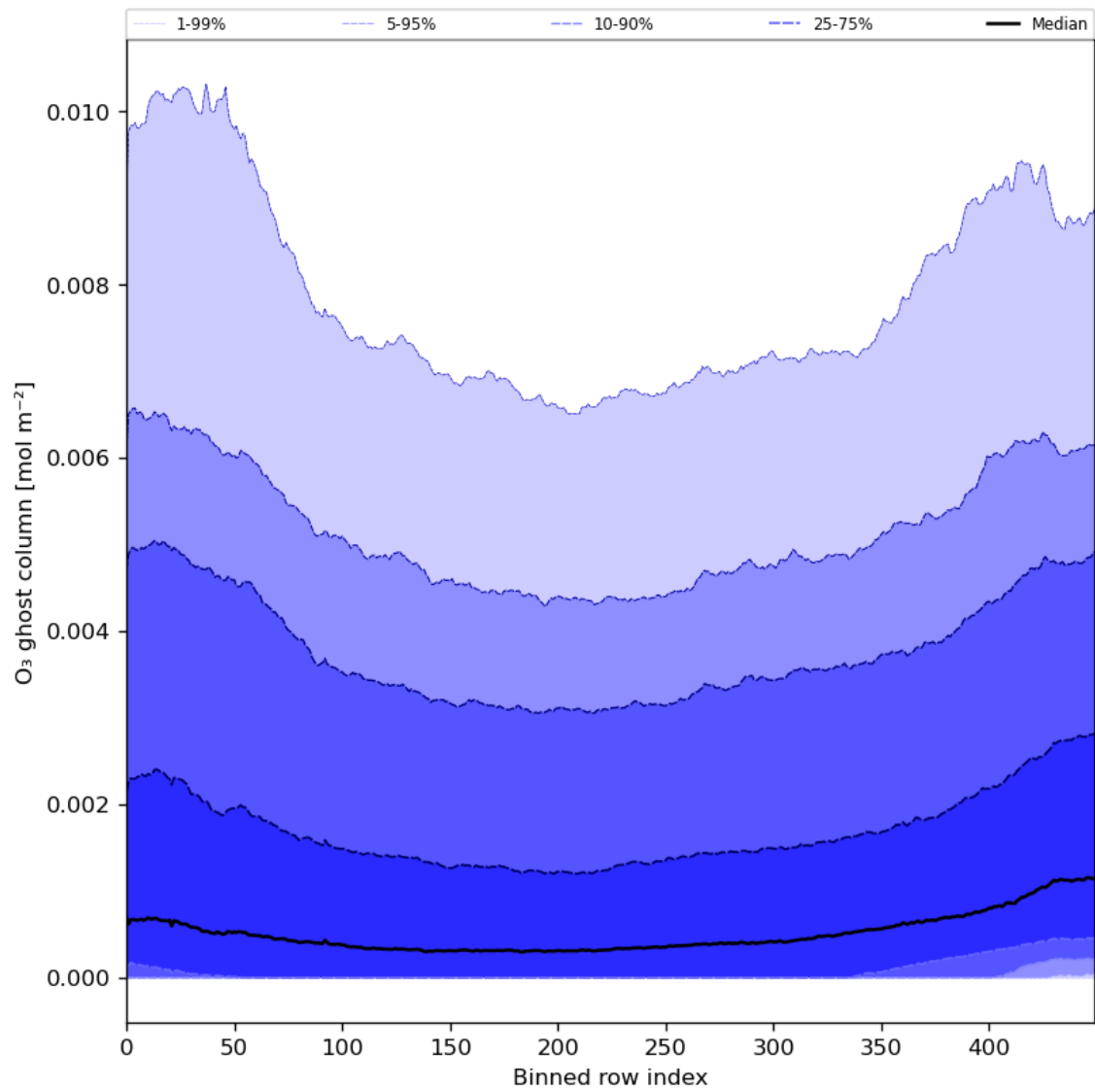
Figure 32: Along track statistics of “O 3 ghost column” for 2024-01-23 to 2024-01-25
