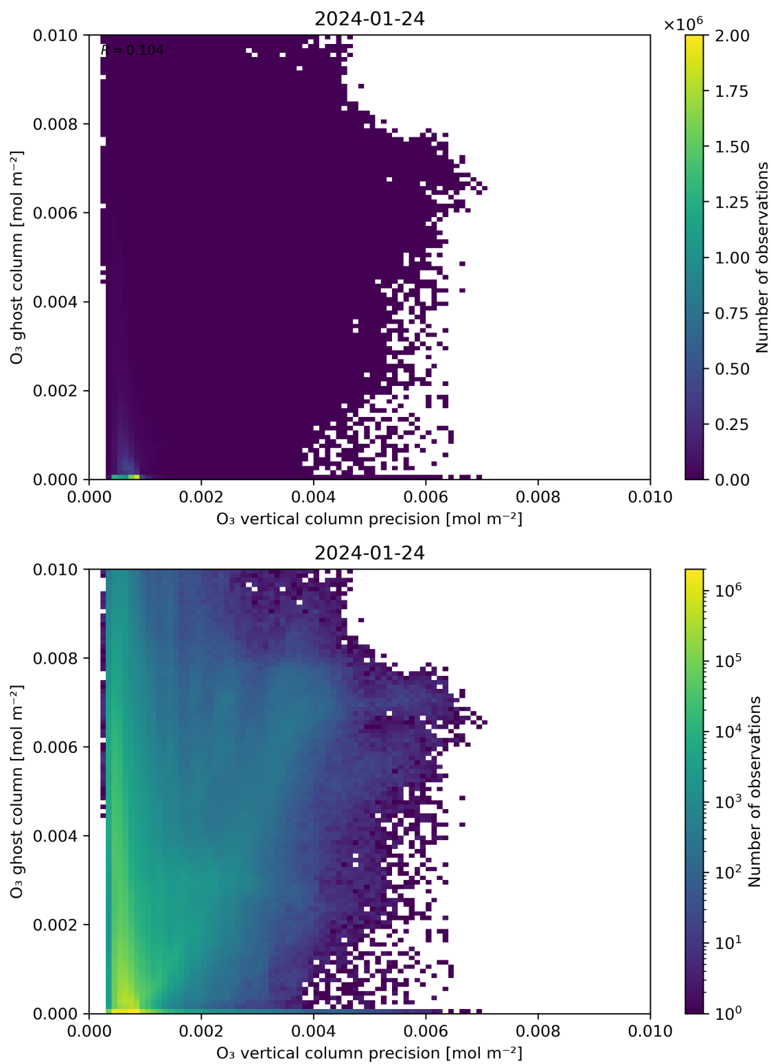
Figure 43: Scatter density plot of “O 3 vertical column precision” against “O 3 ghost column” for 2024-01-23 to 2024-01-25.
