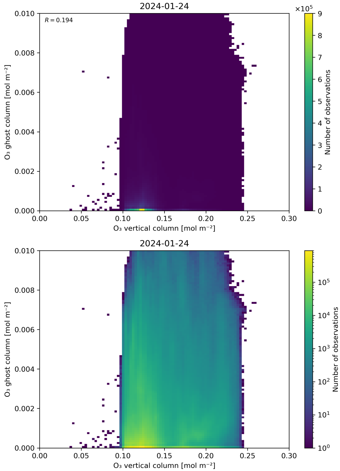
Figure 40: Scatter density plot of “O 3 vertical column” against “O 3 ghost column” for 2024-01-23 to 2024-01-25.
