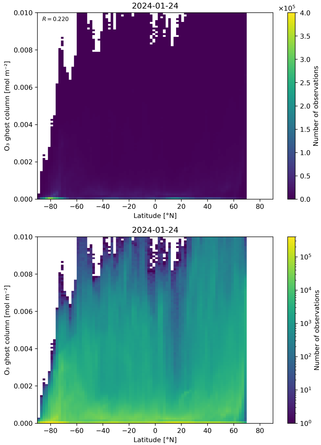
Figure 35: Scatter density plot of “Latitude” against “O 3 ghost column” for 2024-01-23 to 2024-01-25.
