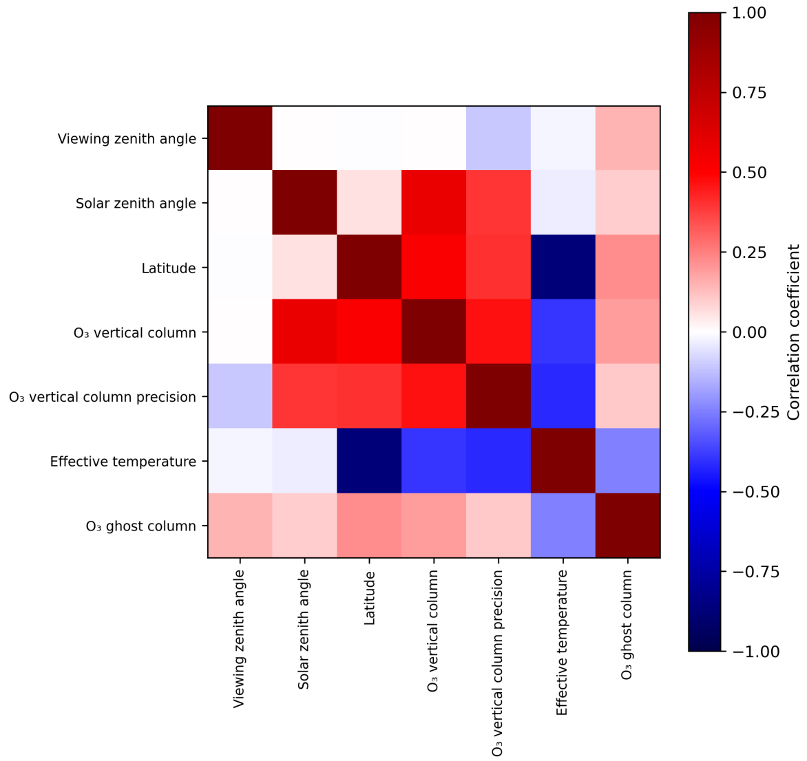
Figure 2: Map of correlation matrix for 2024-01-23 to 2024-01-25.
