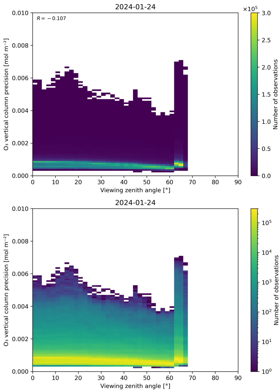
Figure 53: Scatter density plot of “Viewing zenith angle” against “O 3 vertical column precision” for 2024-01-23 to 2024-01-25.
