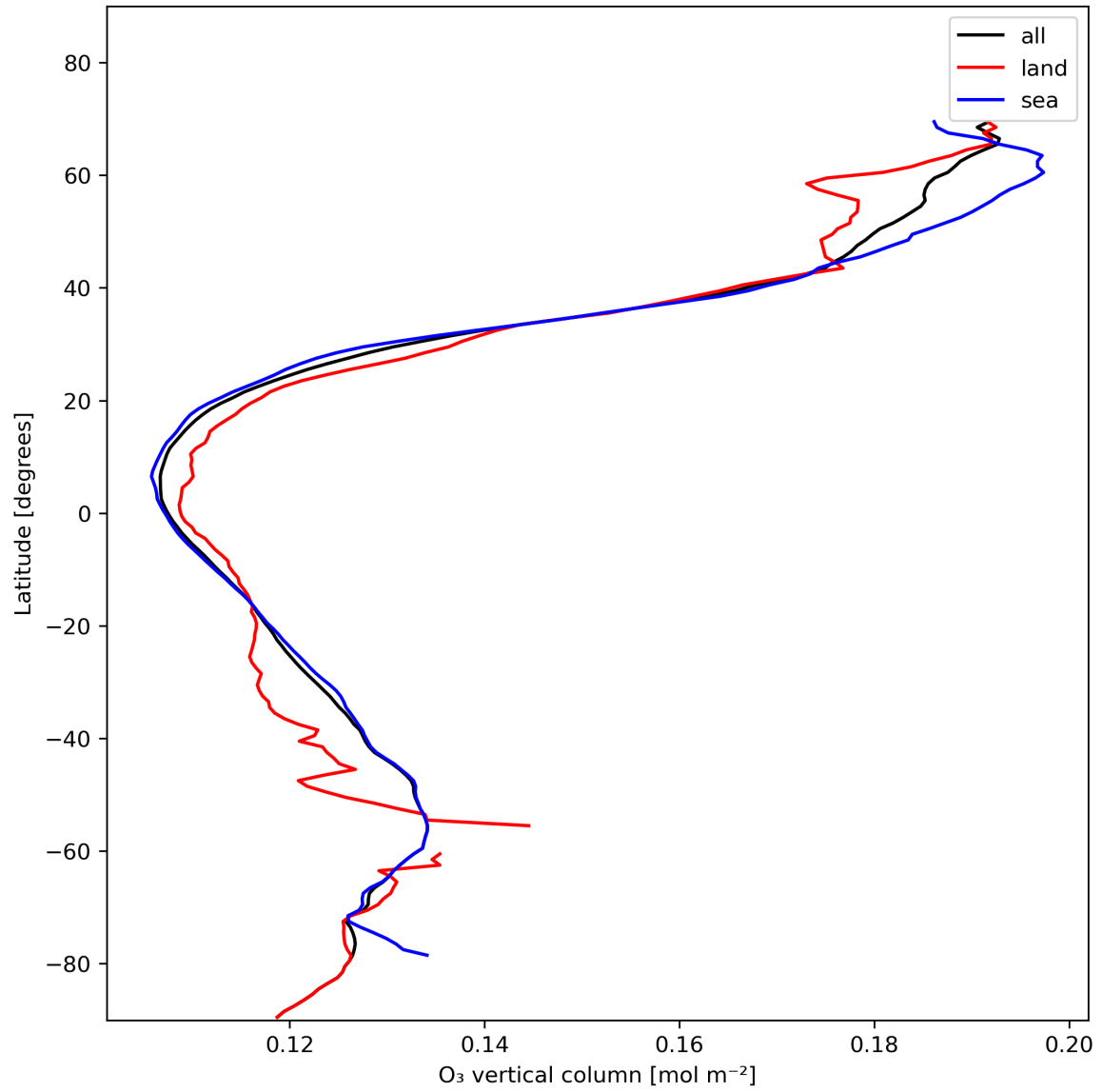
Figure 14: Zonal average of “O 3 vertical column” for 2024-01-23 to 2024-01-25.
