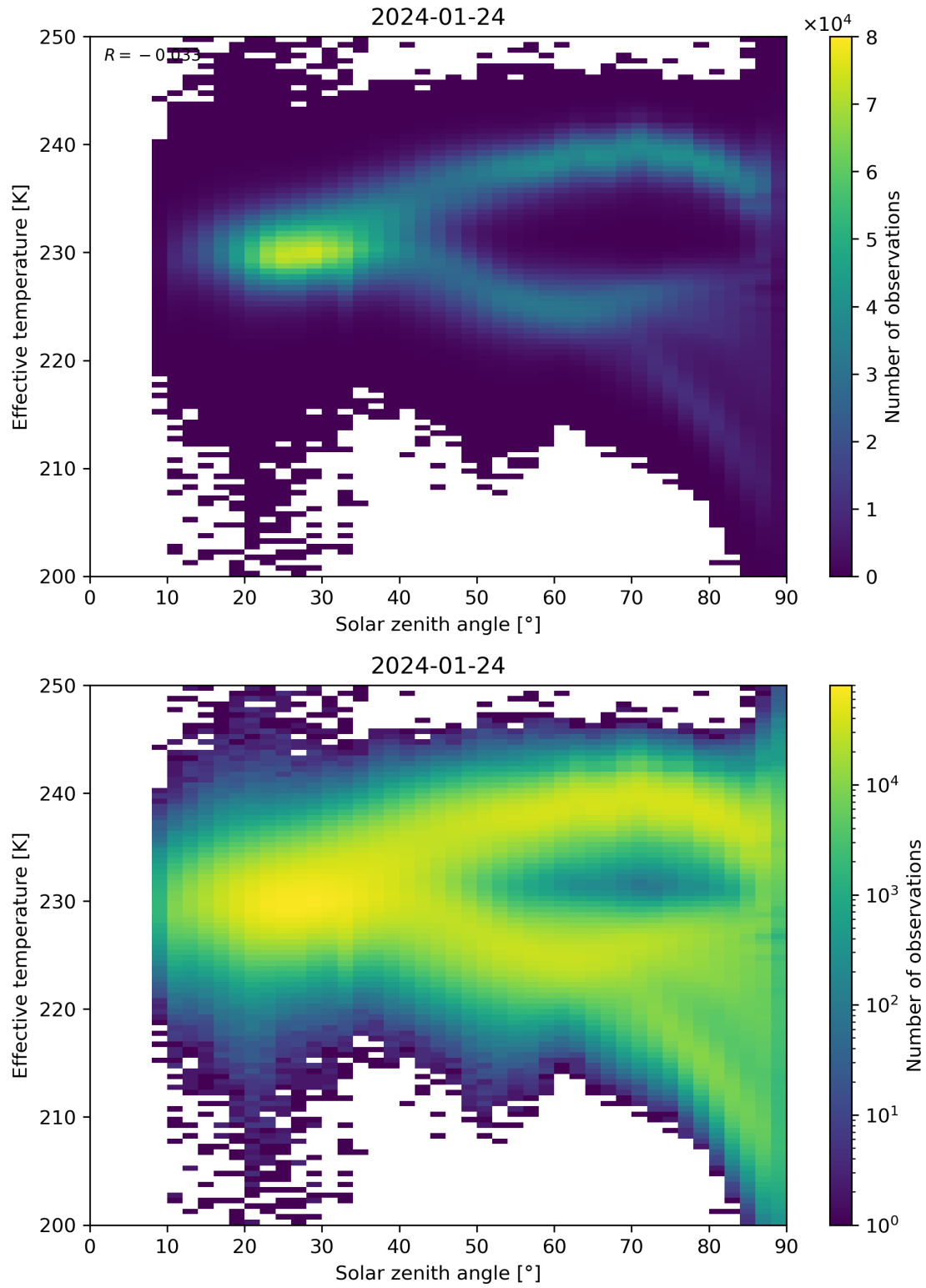
Figure 45: Scatter density plot of “Solar zenith angle” against “Effective temperature” for 2024-01-23 to 2024-01-25.
