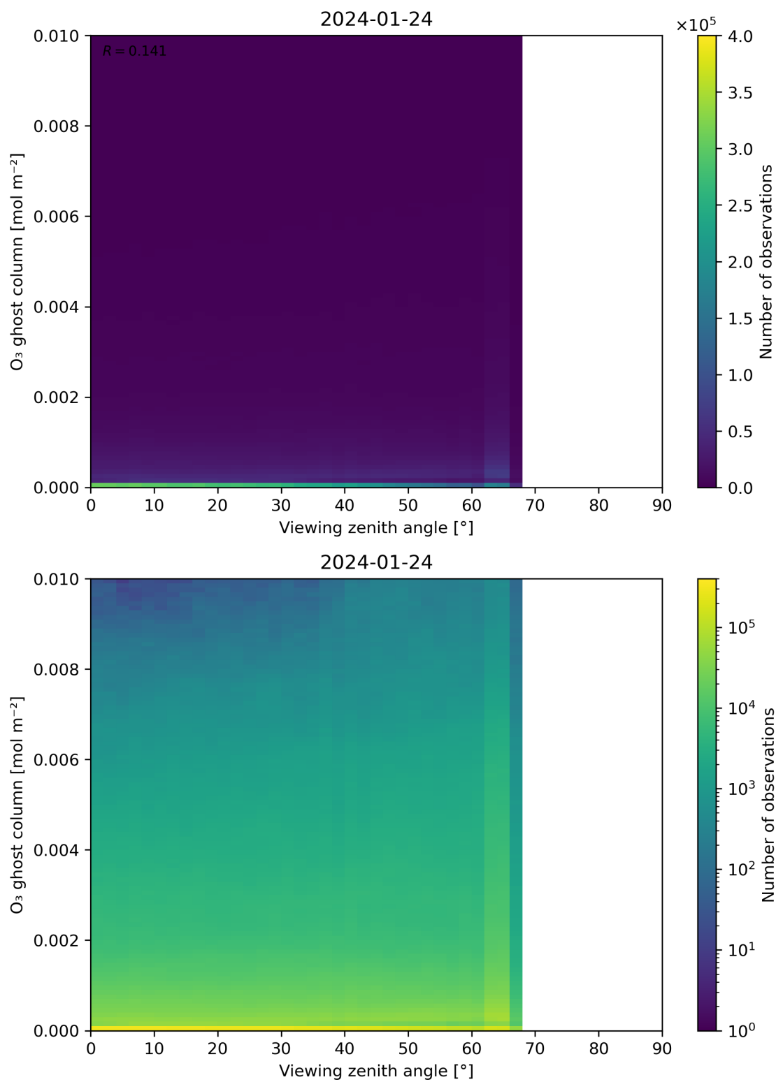
Figure 51: Scatter density plot of “Viewing zenith angle” against “O 3 ghost column” for 2024-01-23 to 2024-01-25.
