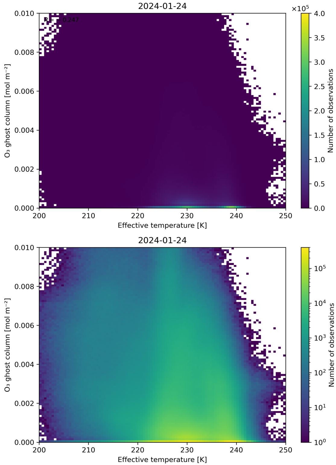
Figure 38: Scatter density plot of “Effective temperature” against “O 3 ghost column” for 2024-01-23 to 2024-01-25.
