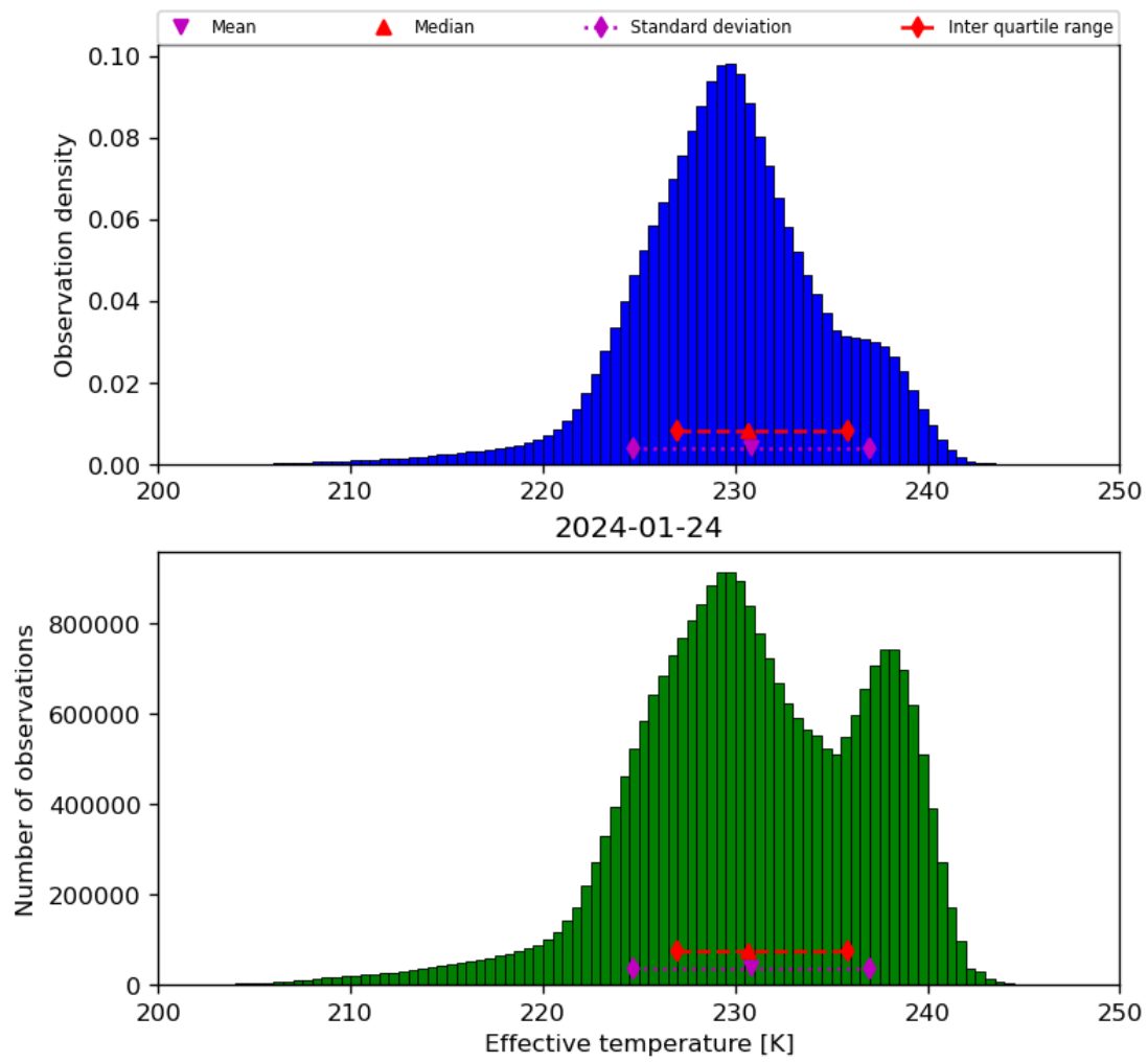
Figure 24: Histogram of “Effective temperature” for 2024-01-23 to 2024-01-25
