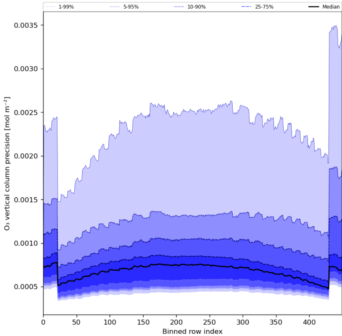
Figure 29: Along track statistics of “O 3 vertical column precision” for 2024-01-23 to 2024-01-25
