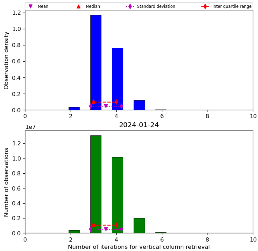
Figure 26: Histogram of “Number of iterations for vertical column retrieval” for 2024-01-23 to 2024-01-25
