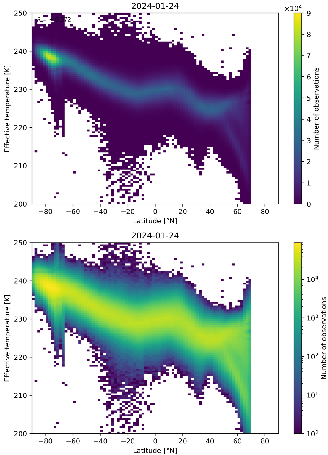
Figure 34: Scatter density plot of “Latitude” against “Effective temperature” for 2024-01-23 to 2024-01-25.
