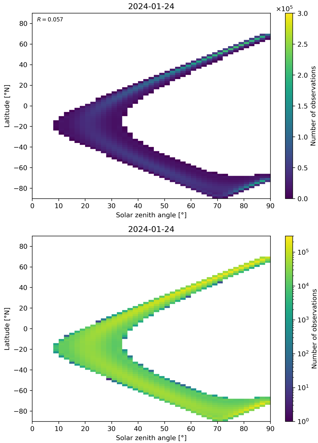
Figure 44: Scatter density plot of “Solar zenith angle” against “Latitude” for 2024-01-23 to 2024-01-25.
