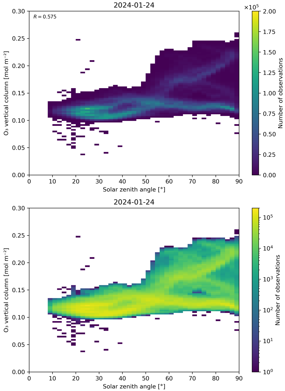
Figure 47: Scatter density plot of “Solar zenith angle” against “O 3 vertical column” for 2024-01-23 to 2024-01-25.
