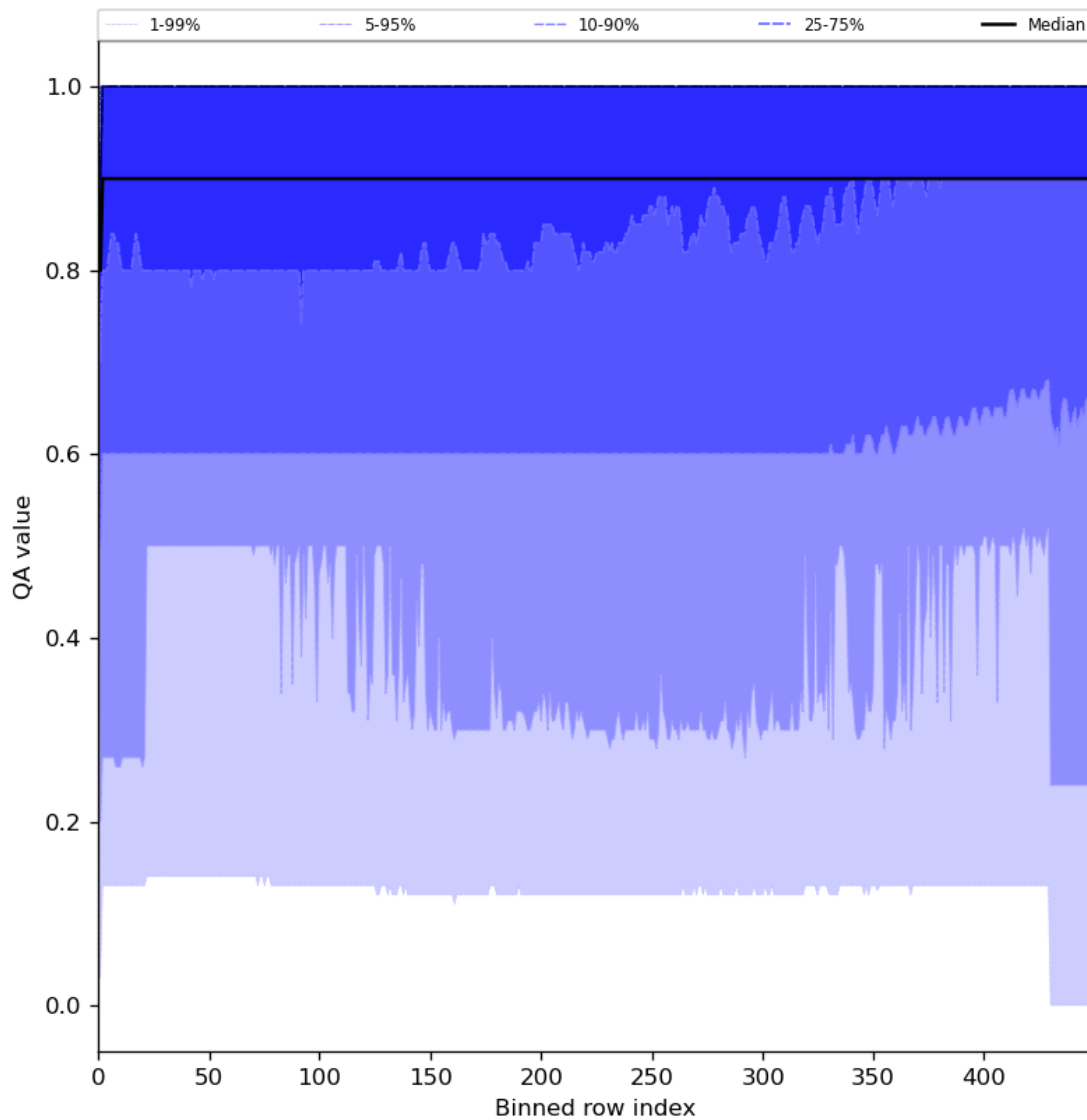
Figure 27: Along track statistics of “QA value” for 2024-01-23 to 2024-01-25
