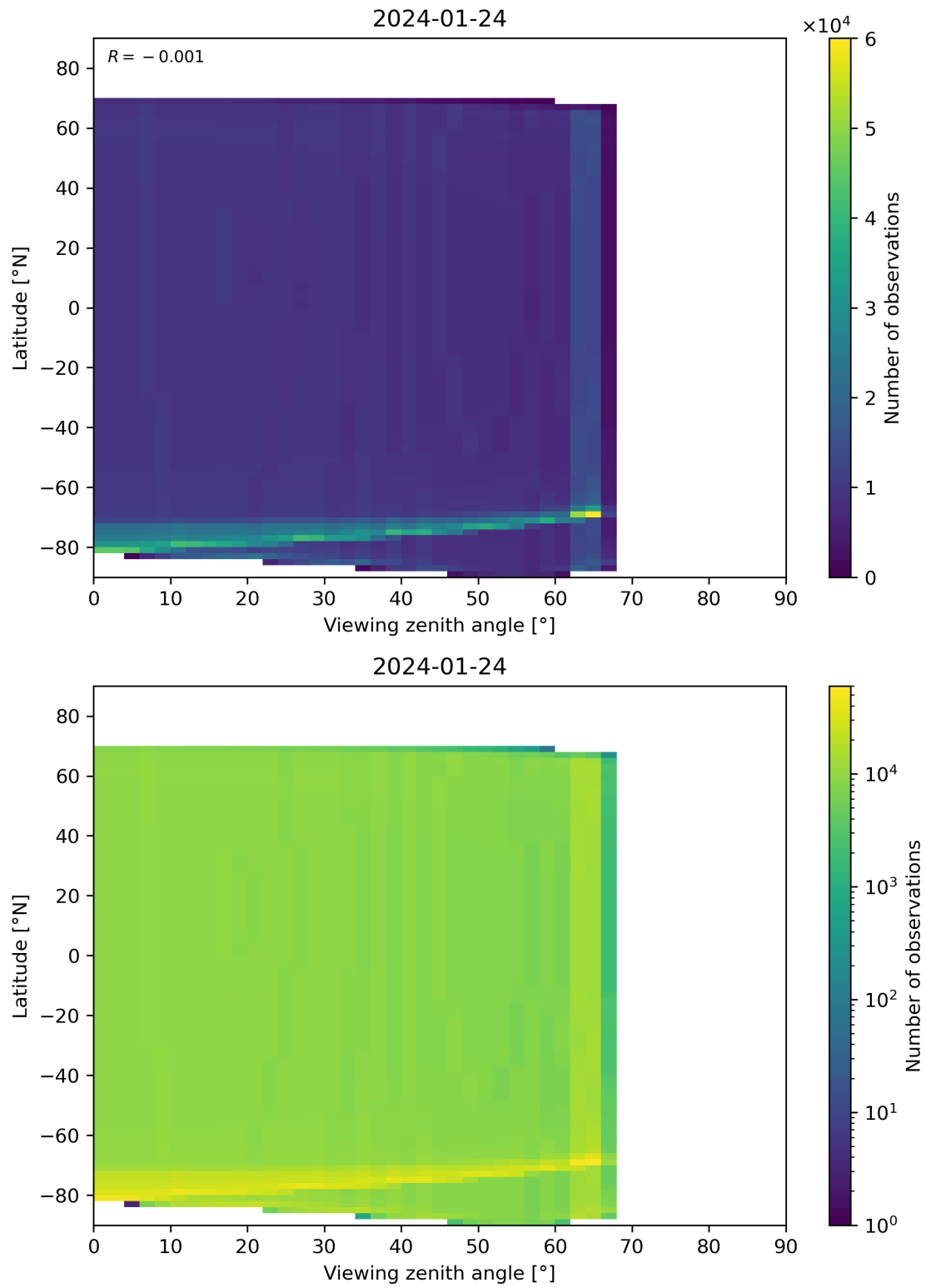
Figure 49: Scatter density plot of “Viewing zenith angle” against “Latitude” for 2024-01-23 to 2024-01-25.
