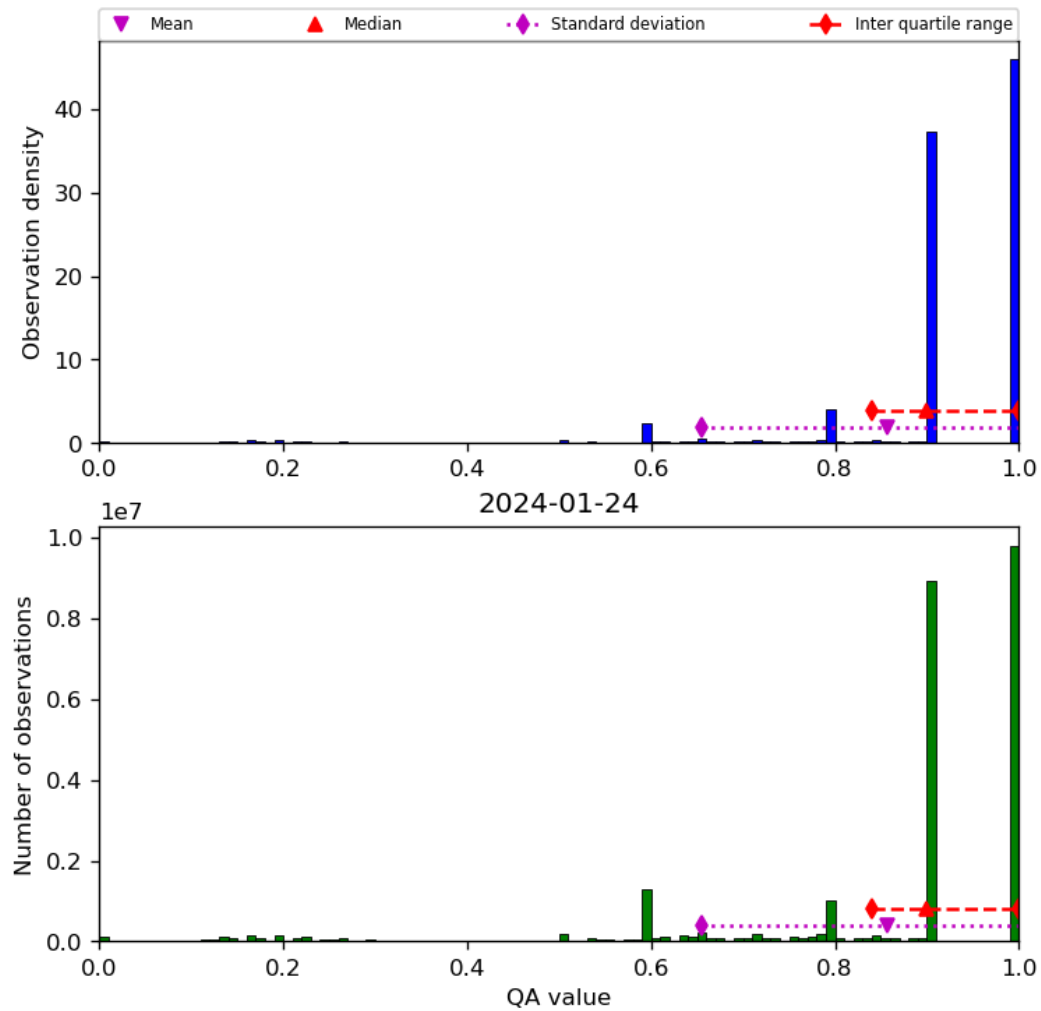
Figure 20: Histogram of “QA value” for 2024-01-23 to 2024-01-25
