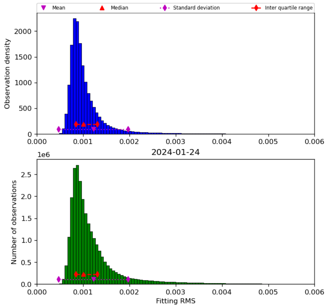
Figure 23: Histogram of “Fitting RMS” for 2024-01-23 to 2024-01-25
