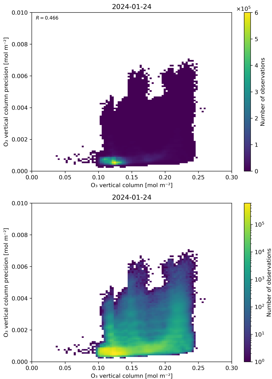
Figure 41: Scatter density plot of “O 3 vertical column” against “O 3 vertical column precision” for 2024-01-23 to 2024-01-25.
