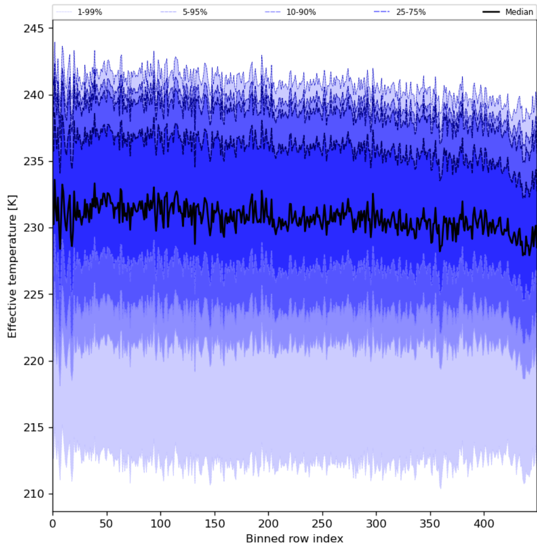
Figure 31: Along track statistics of “Effective temperature” for 2024-01-23 to 2024-01-25
