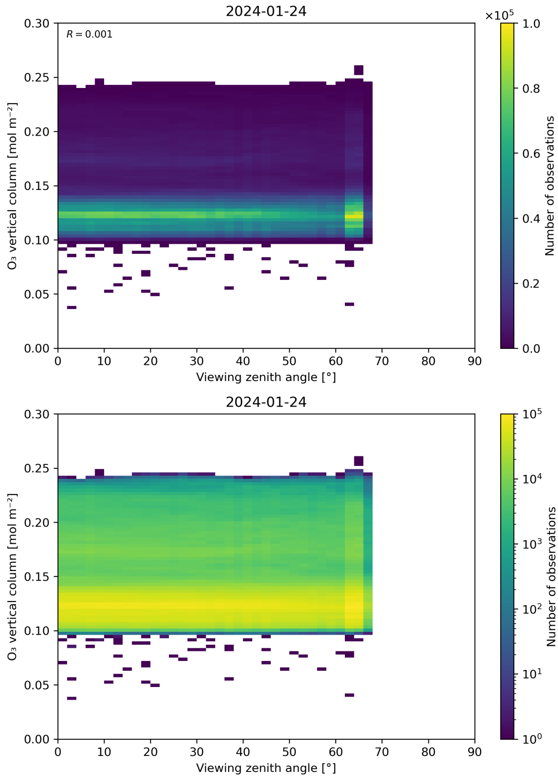
Figure 52: Scatter density plot of “Viewing zenith angle” against “O 3 vertical column” for 2024-01-23 to 2024-01-25.
