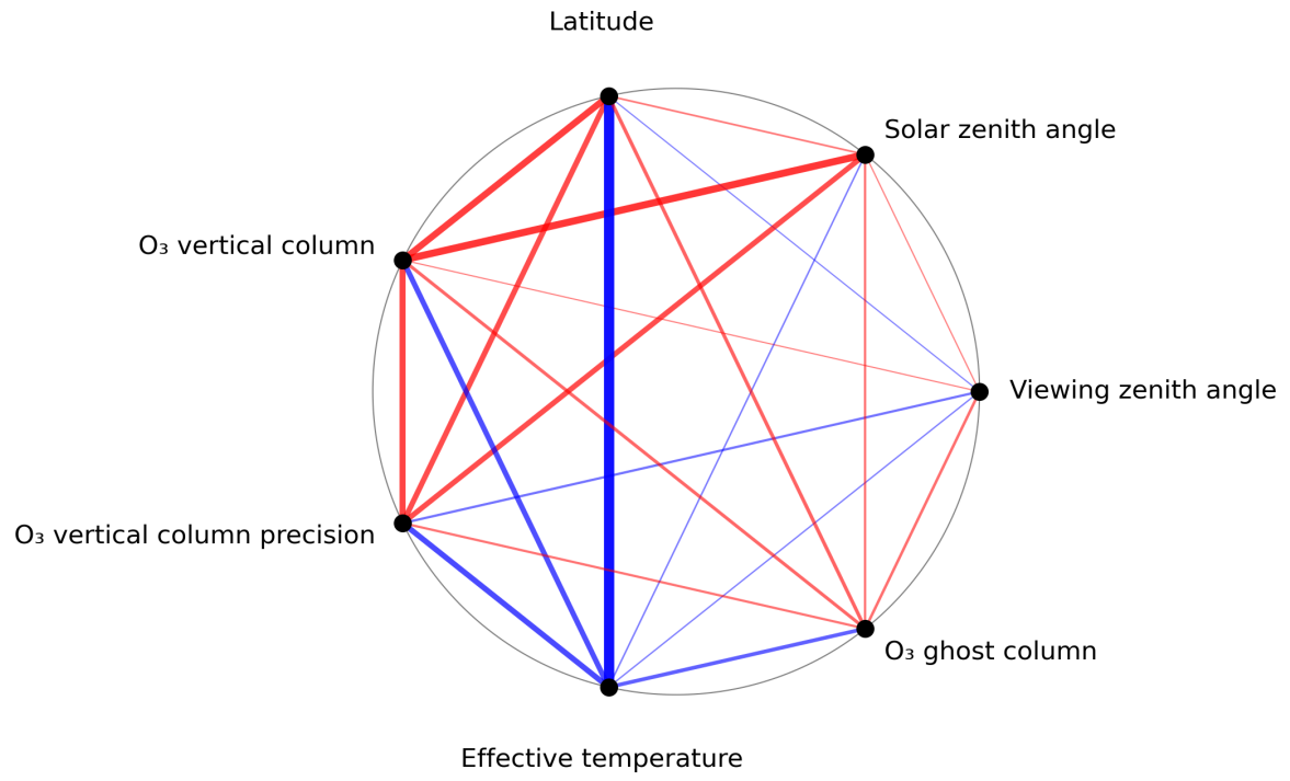
Figure 1: Map of correlation graph for 2024-01-23 to 2024-01-25.
