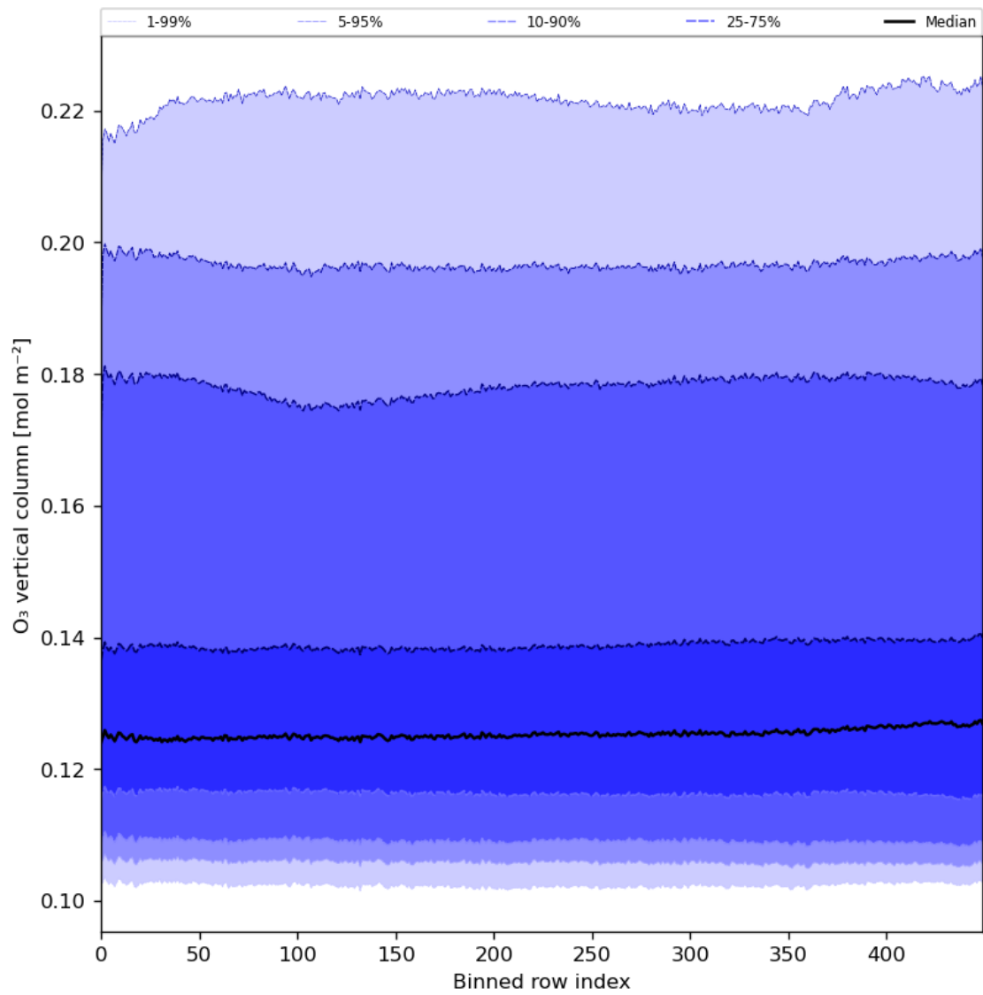
Figure 28: Along track statistics of “O 3 vertical column” for 2024-01-23 to 2024-01-25
