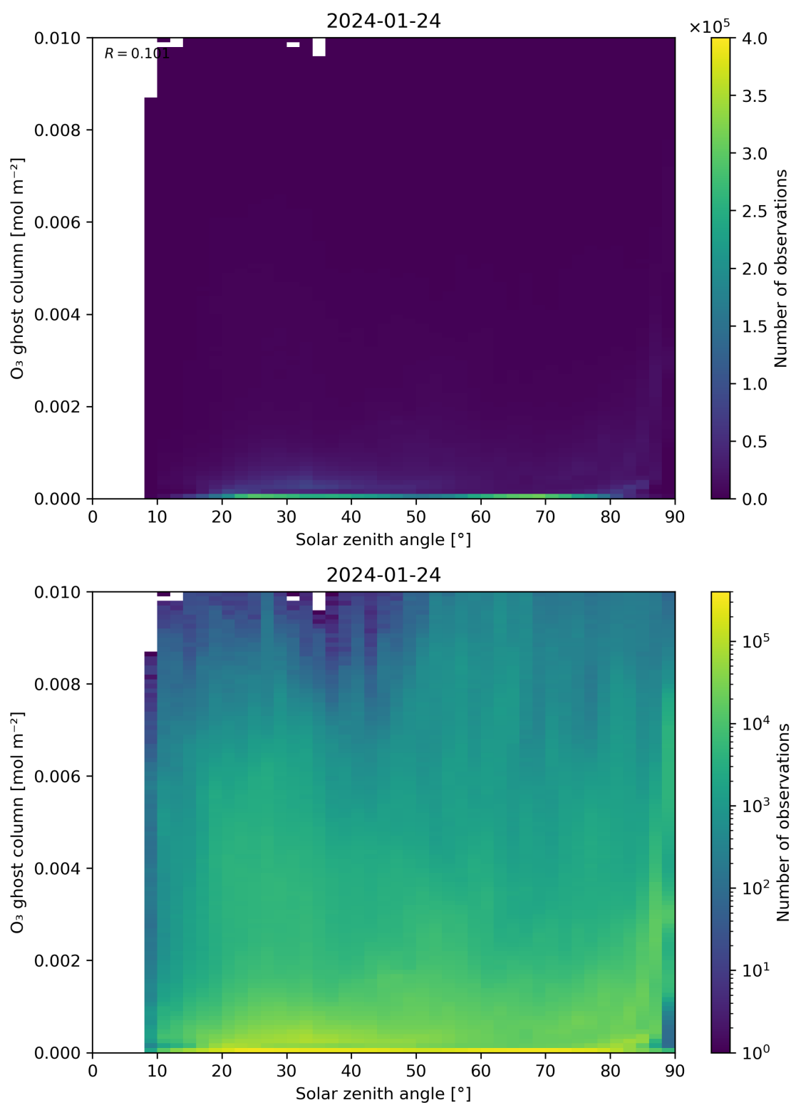
Figure 46: Scatter density plot of “Solar zenith angle” against “O 3 ghost column” for 2024-01-23 to 2024-01-25.
