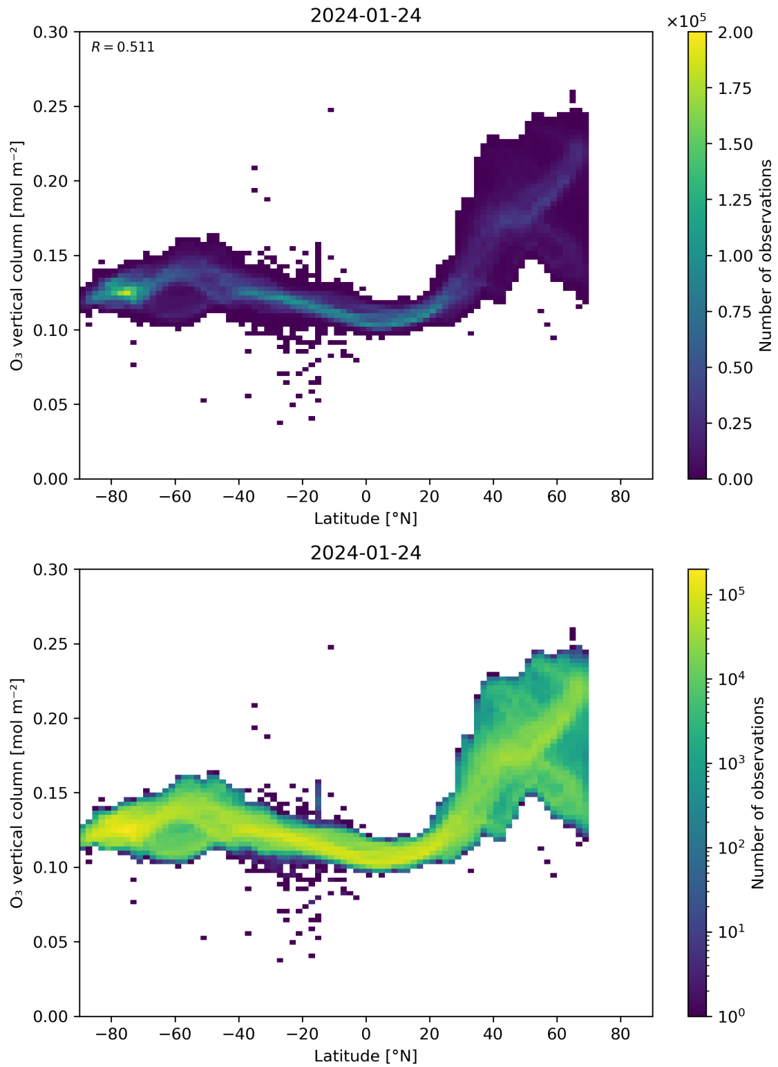
Figure 36: Scatter density plot of “Latitude” against “O 3 vertical column” for 2024-01-23 to 2024-01-25.
