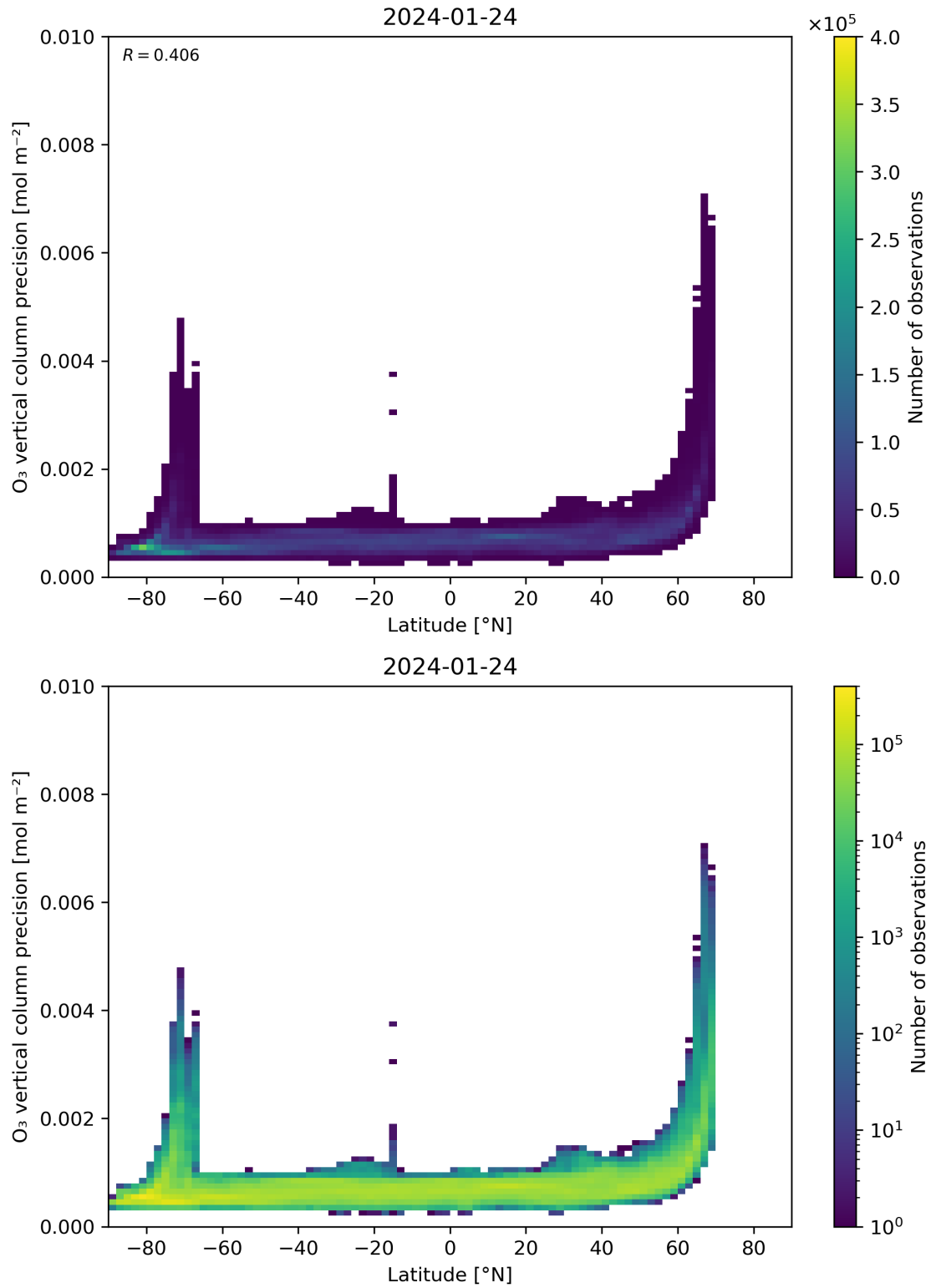
Figure 37: Scatter density plot of “Latitude” against “O 3 vertical column precision” for 2024-01-23 to 2024-01-25.
