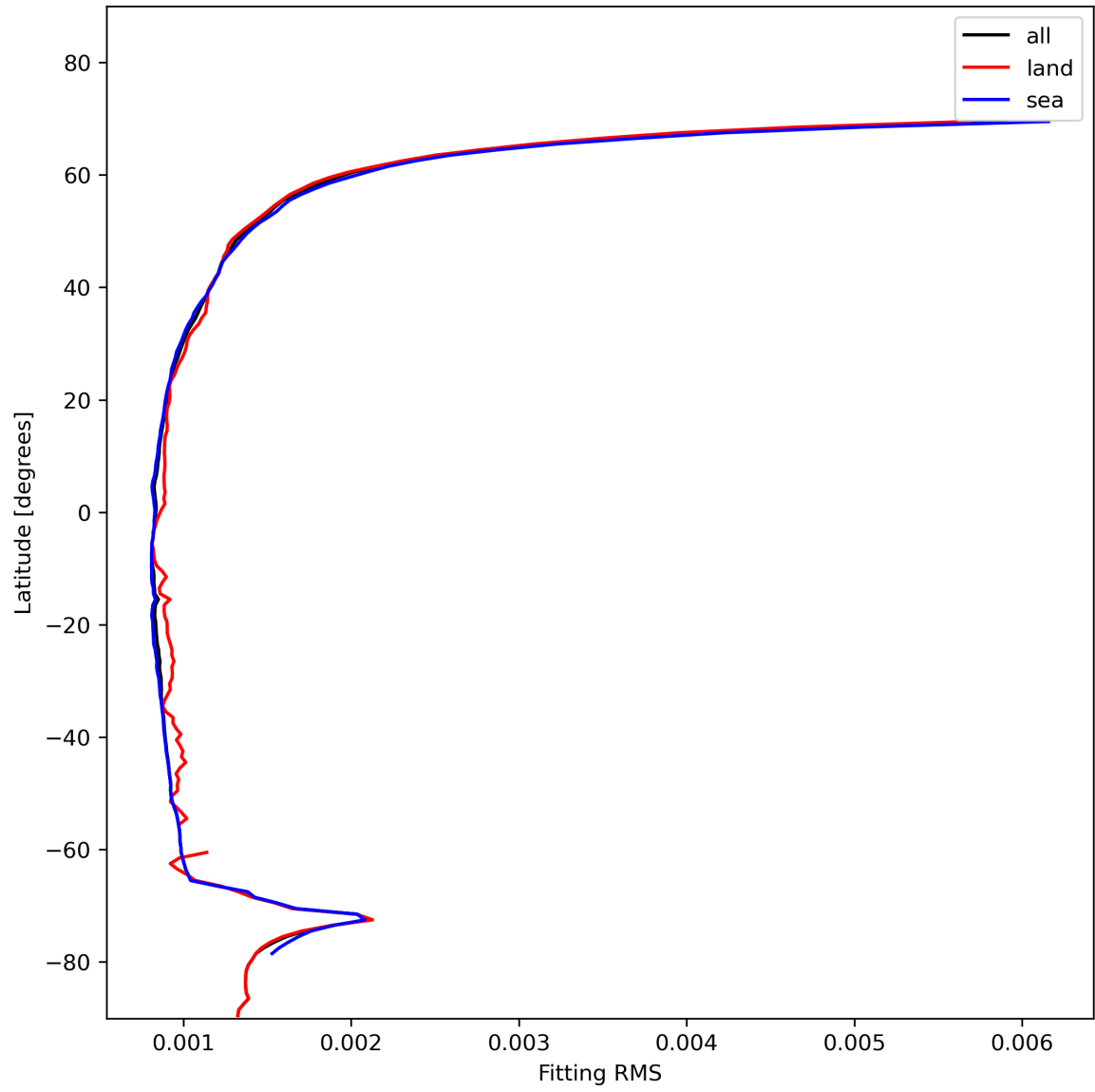
Figure 16: Zonal average of “Fitting RMS” for 2024-01-23 to 2024-01-25.
