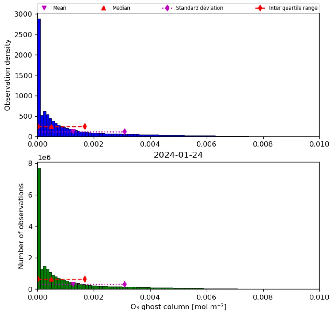
Figure 25: Histogram of “O 3 ghost column” for 2024-01-23 to 2024-01-25
