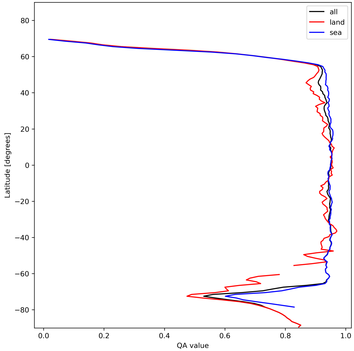
Figure 13: Zonal average of “QA value” for 2024-01-23 to 2024-01-25.
