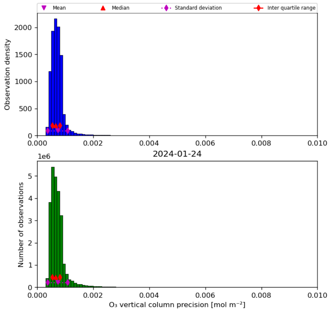
Figure 22: Histogram of “O 3 vertical column precision” for 2024-01-23 to 2024-01-25
