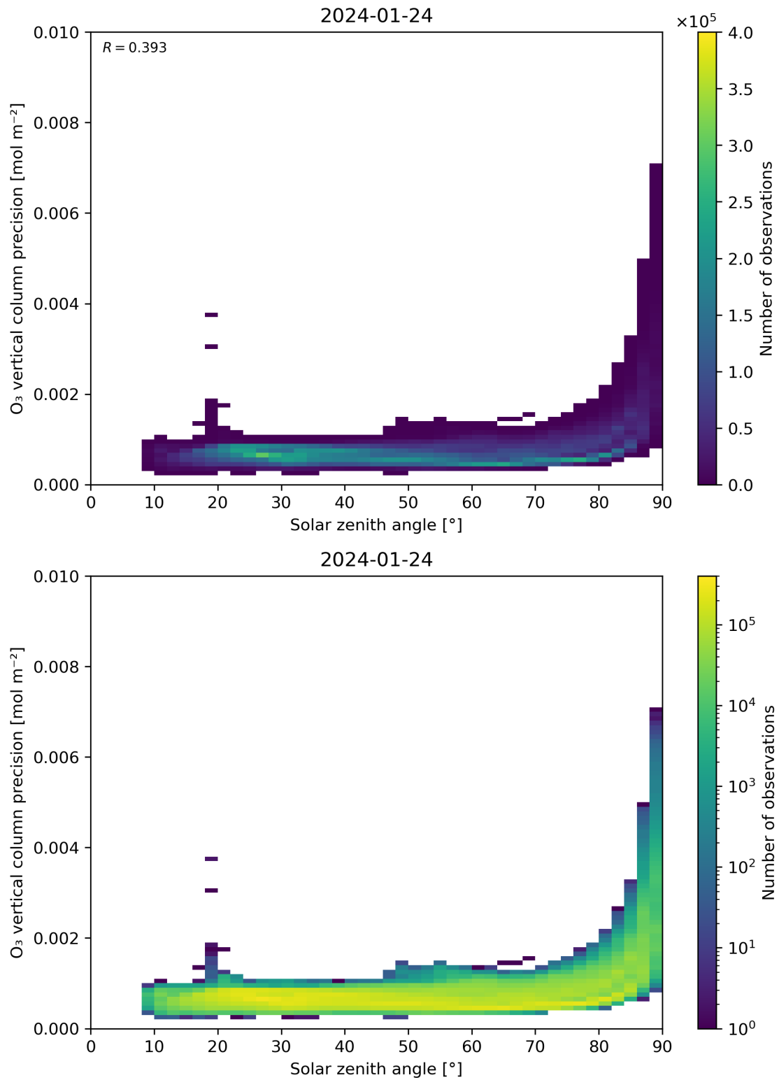
Figure 48: Scatter density plot of “Solar zenith angle” against “O 3 vertical column precision” for 2024-01-23 to 2024-01-25.
