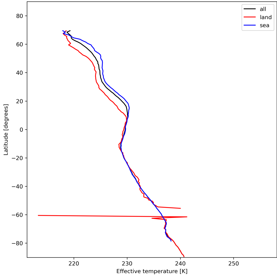
Figure 17: Zonal average of “Effective temperature” for 2024-01-23 to 2024-01-25.
