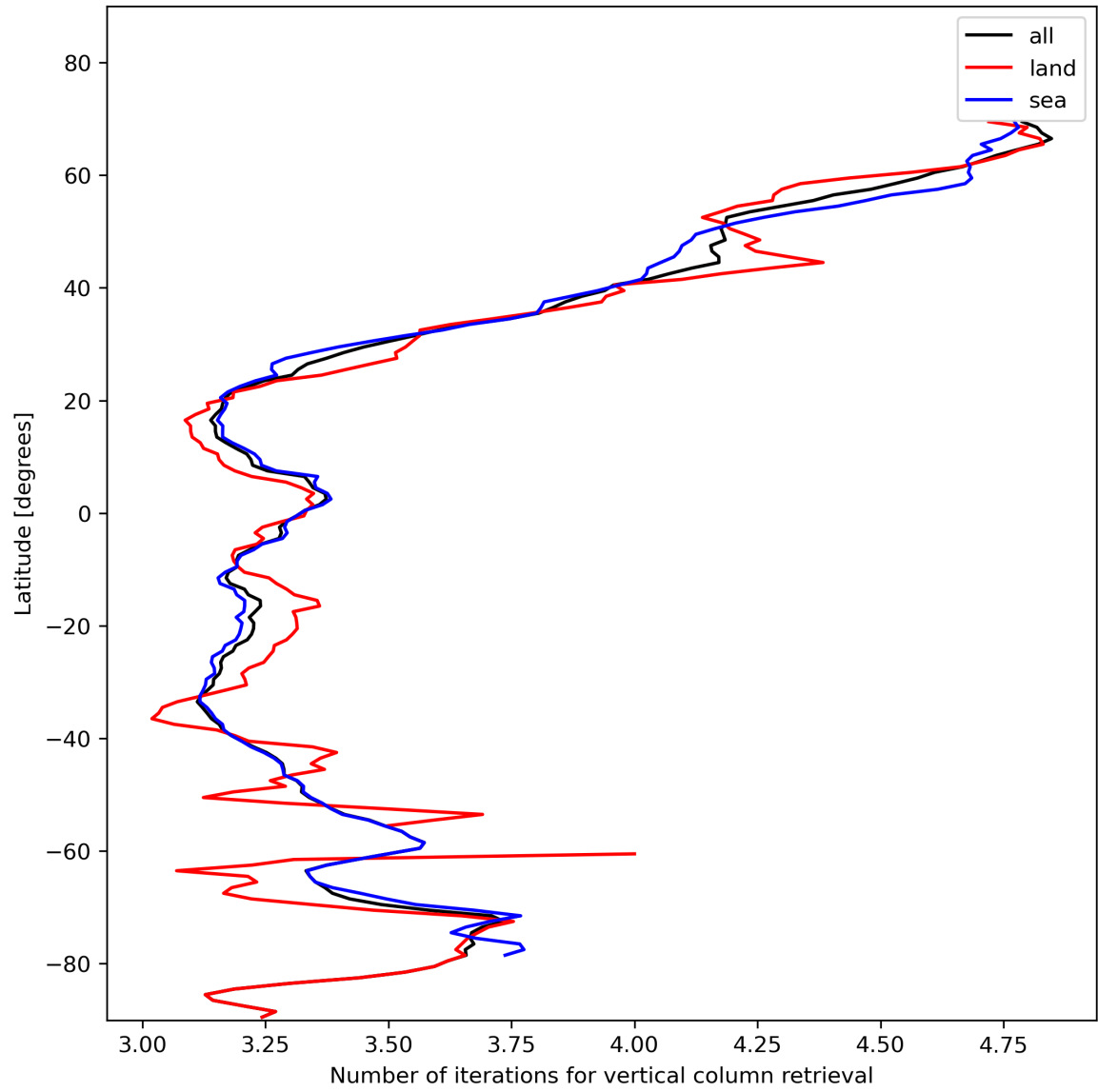
Figure 19: Zonal average of “Number of iterations for vertical column retrieval” for 2024-01-23 to 2024-01-25.
