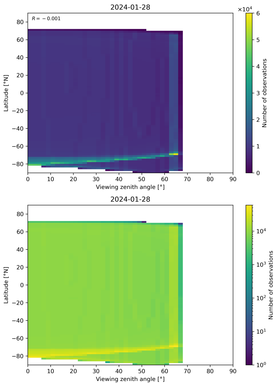
Figure 49: Scatter density plot of “Viewing zenith angle” against “Latitude” for 2024-01-27 to 2024-01-29.
