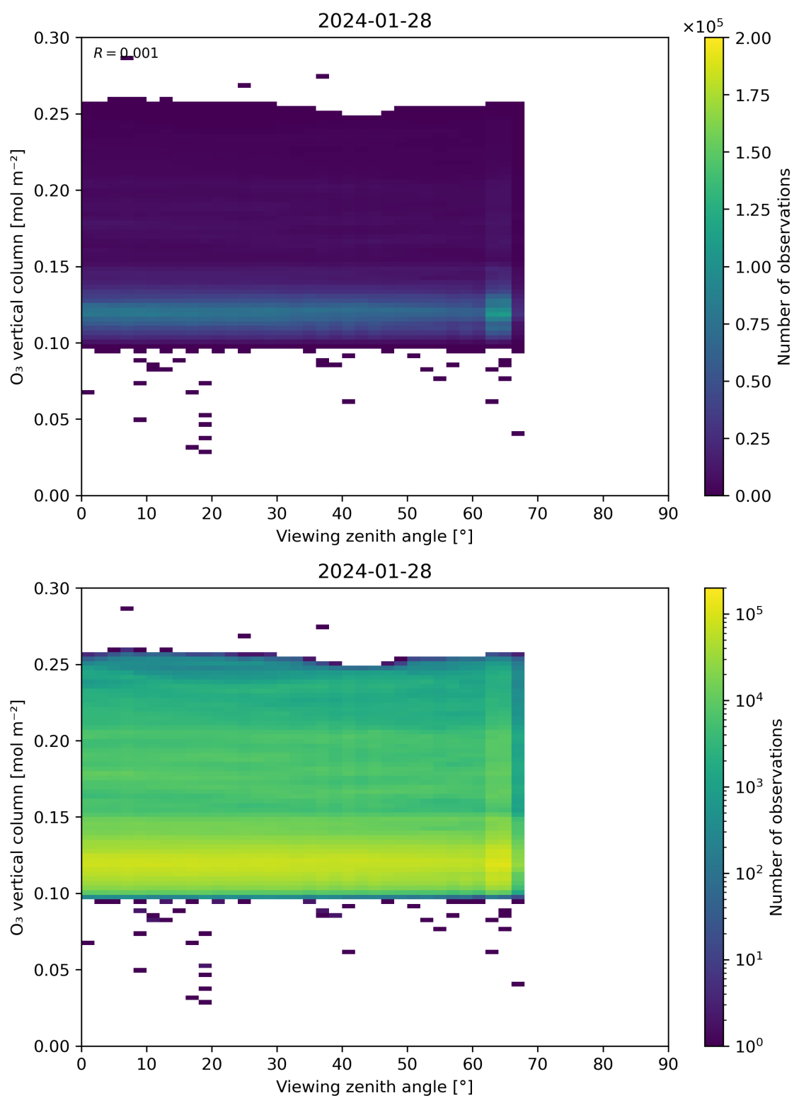
Figure 52: Scatter density plot of “Viewing zenith angle” against “O 3 vertical column” for 2024-01-27 to 2024-01-29.
