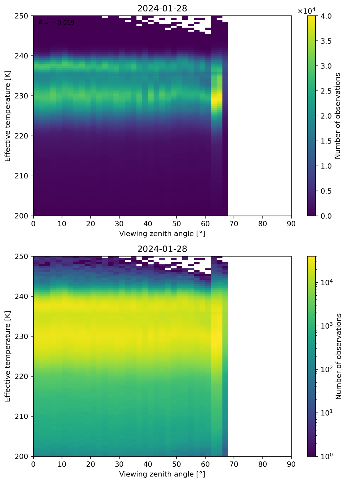
Figure 50: Scatter density plot of “Viewing zenith angle” against “Effective temperature” for 2024-01-27 to 2024-01-29.
