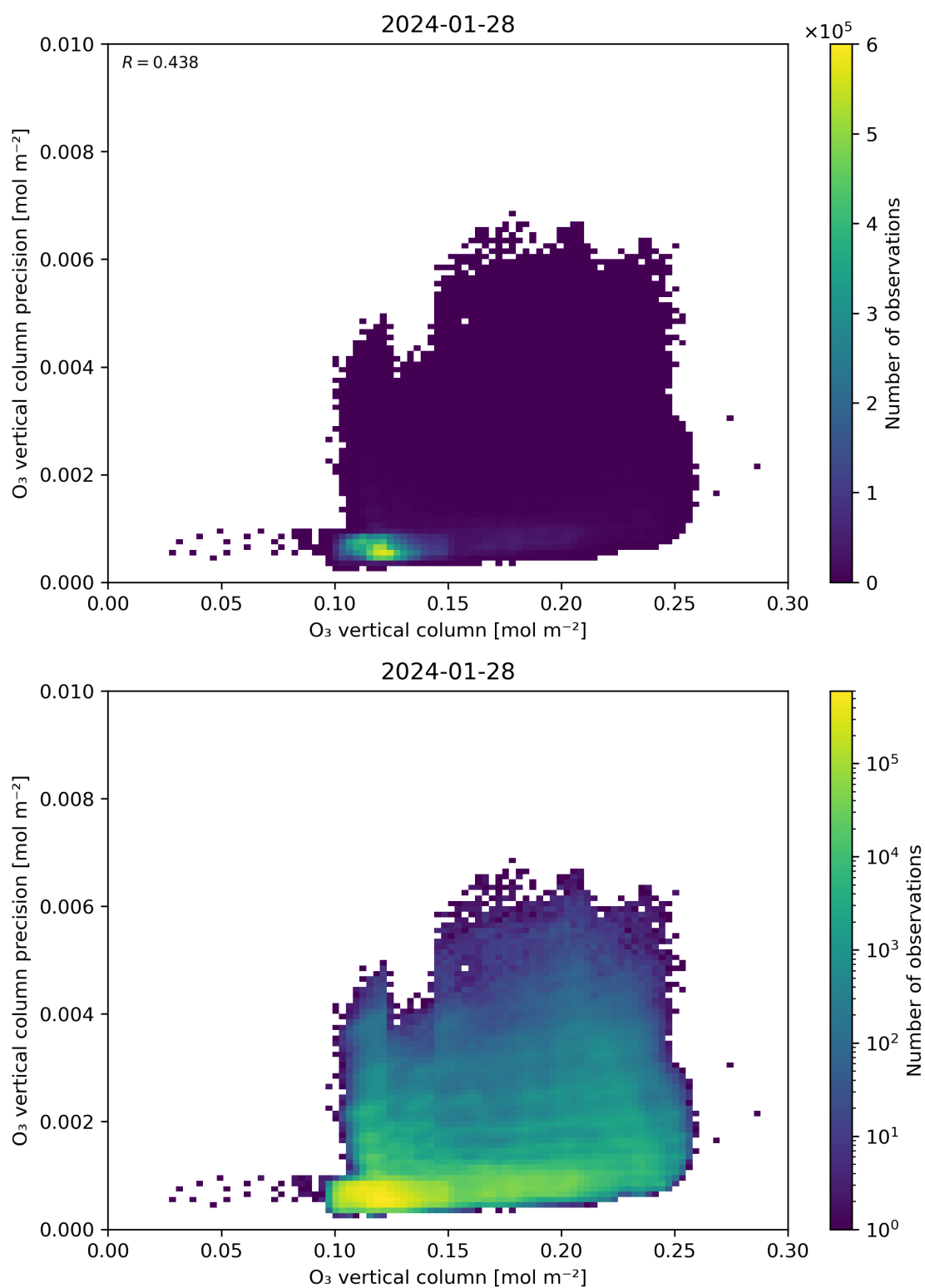
Figure 41: Scatter density plot of “O 3 vertical column” against “O 3 vertical column precision” for 2024-01-27 to 2024-01-29.
