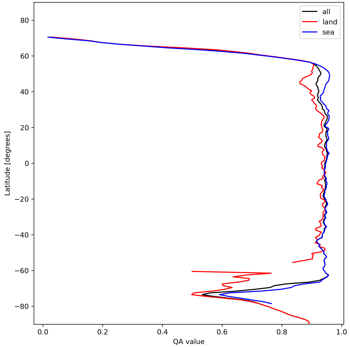
Figure 13: Zonal average of “QA value” for 2024-01-27 to 2024-01-29.
