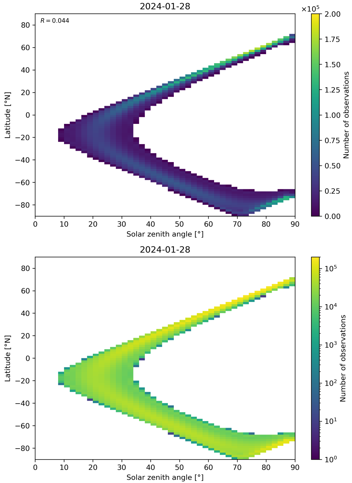
Figure 44: Scatter density plot of “Solar zenith angle” against “Latitude” for 2024-01-27 to 2024-01-29.
