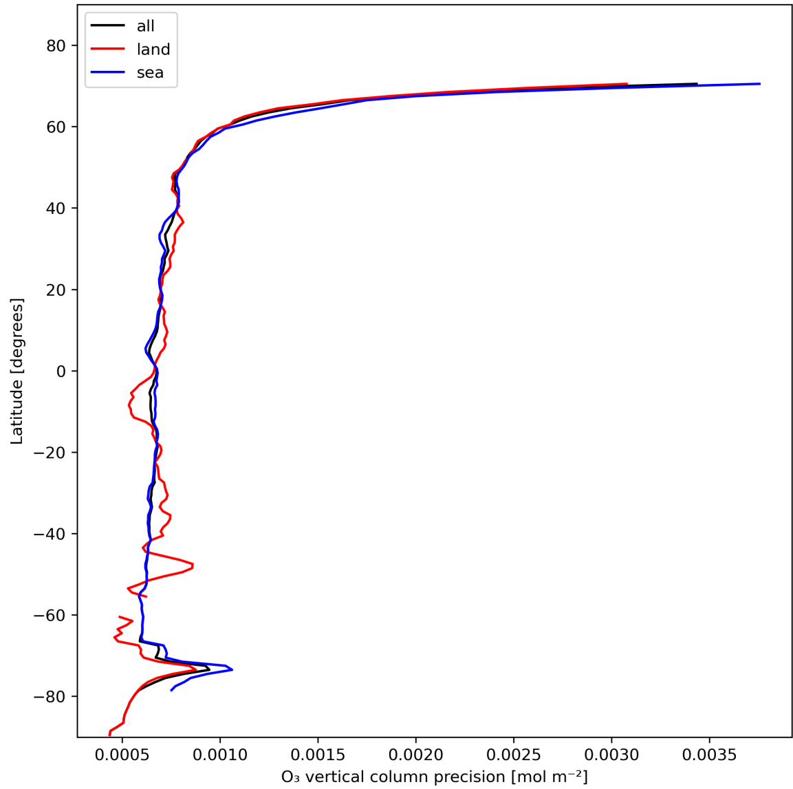
Figure 15: Zonal average of “O 3 vertical column precision” for 2024-01-27 to 2024-01-29.
