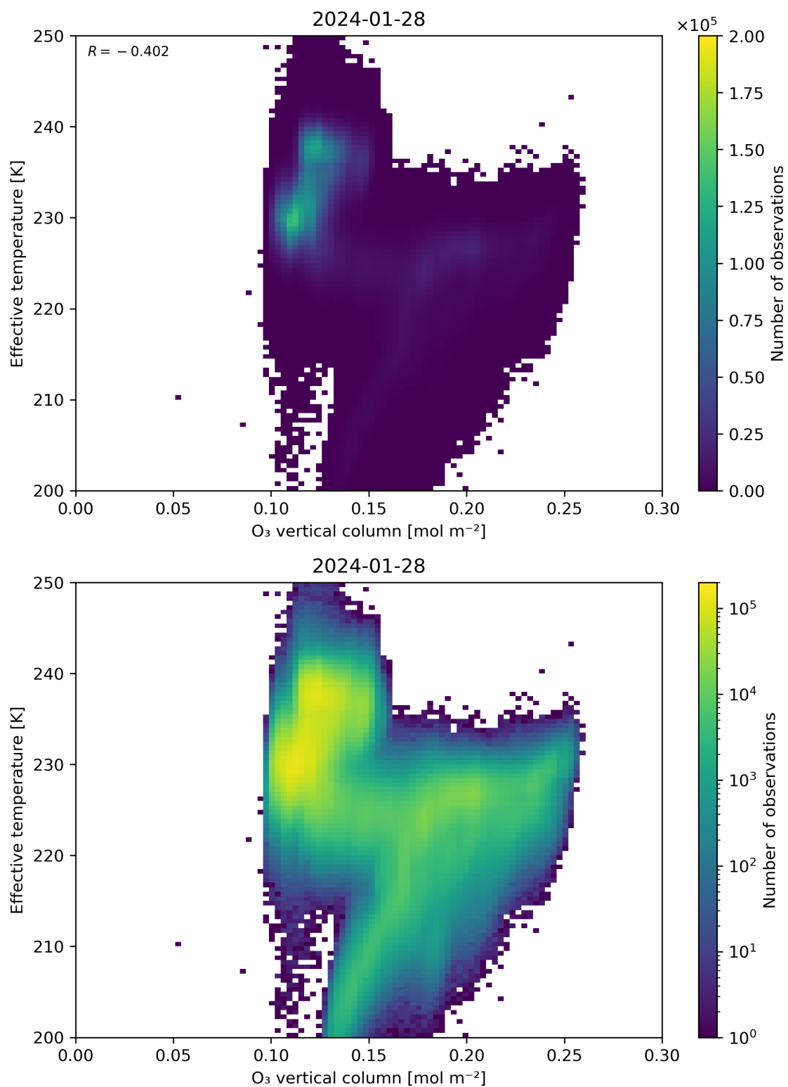
Figure 39: Scatter density plot of “O 3 vertical column” against “Effective temperature” for 2024-01-27 to 2024-01-29.
