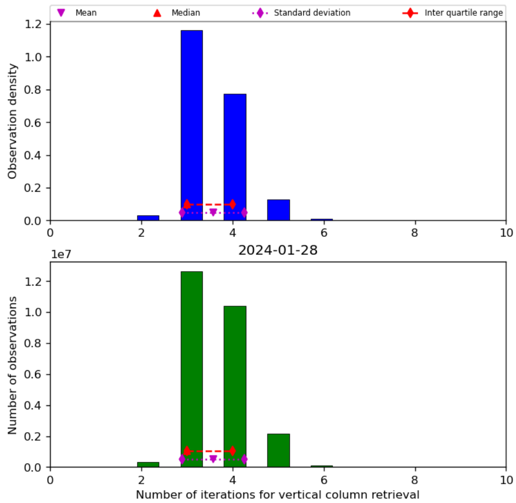
Figure 26: Histogram of “Number of iterations for vertical column retrieval” for 2024-01-27 to 2024-01-29
