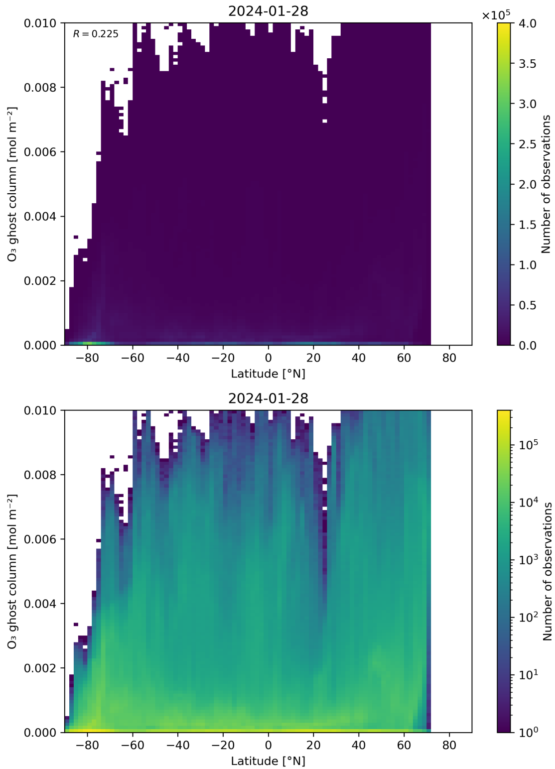
Figure 35: Scatter density plot of “Latitude” against “O 3 ghost column” for 2024-01-27 to 2024-01-29.
