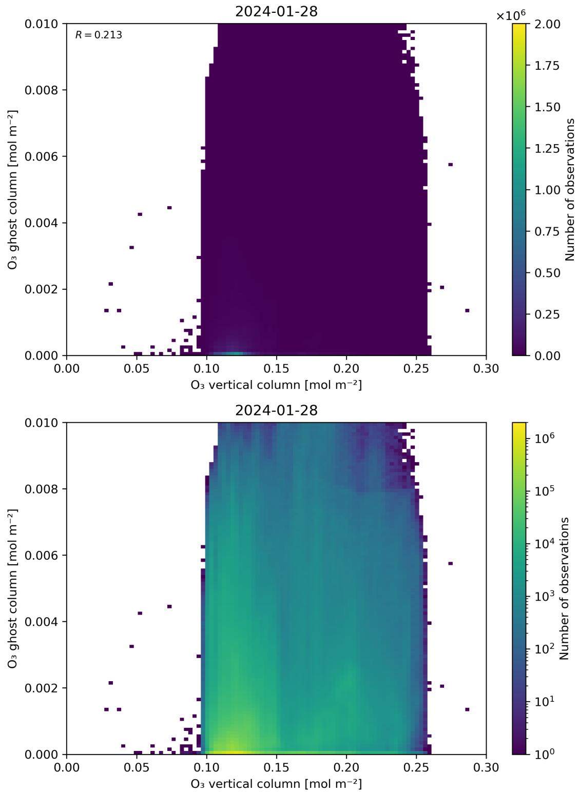
Figure 40: Scatter density plot of “O 3 vertical column” against “O 3 ghost column” for 2024-01-27 to 2024-01-29.
