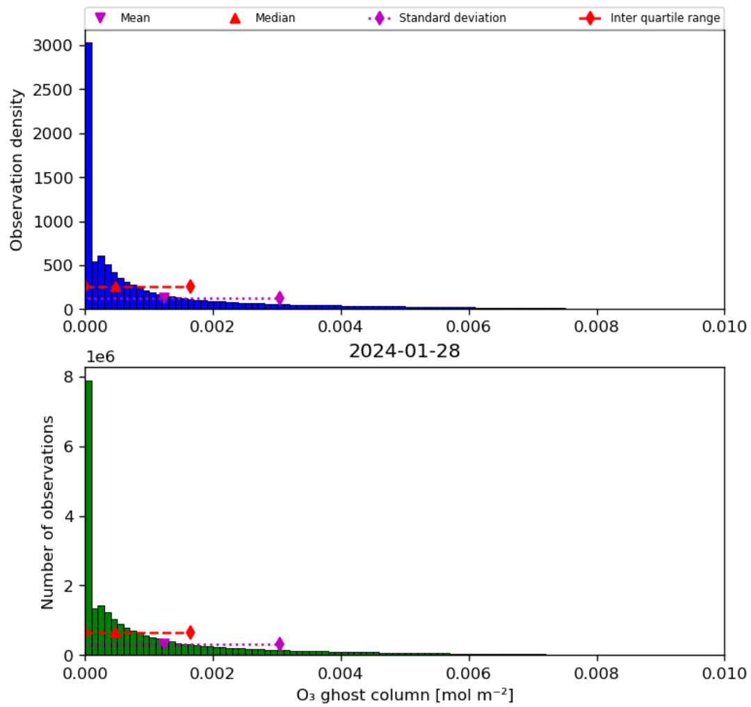
Figure 25: Histogram of “O 3 ghost column” for 2024-01-27 to 2024-01-29
