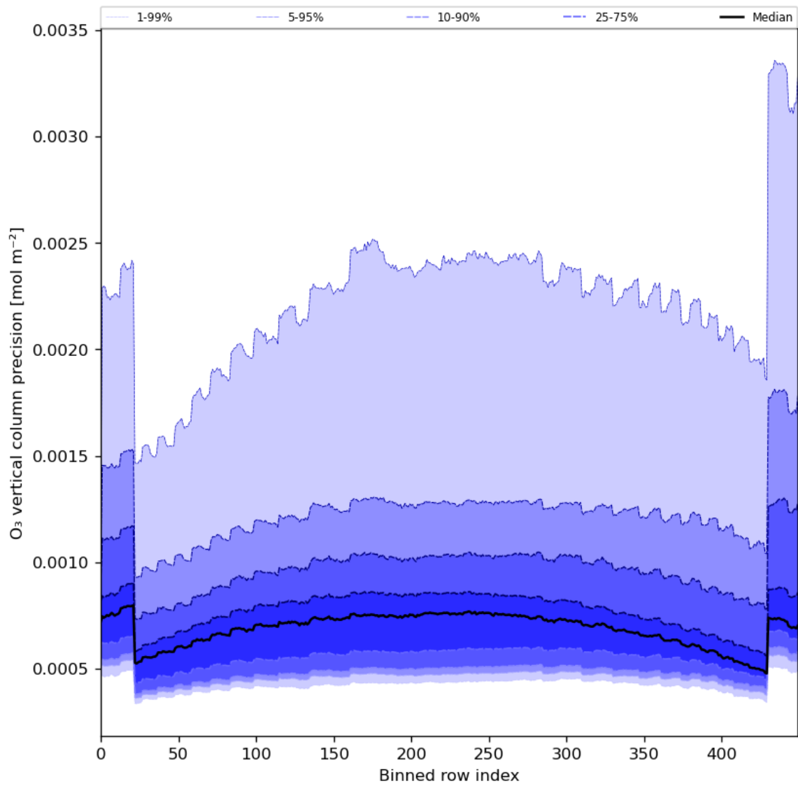
Figure 29: Along track statistics of “O 3 vertical column precision” for 2024-01-27 to 2024-01-29
