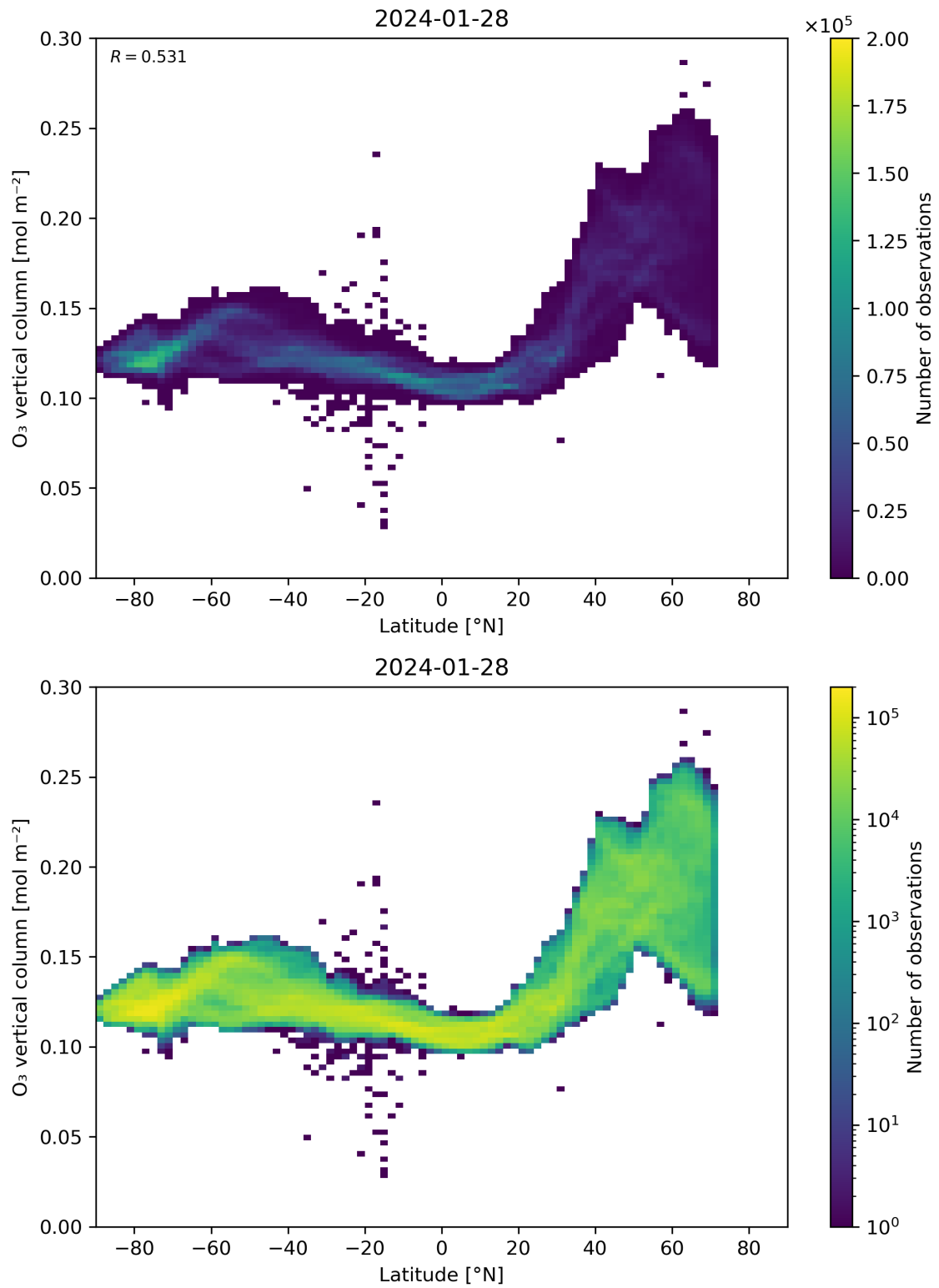
Figure 36: Scatter density plot of “Latitude” against “O 3 vertical column” for 2024-01-27 to 2024-01-29.
