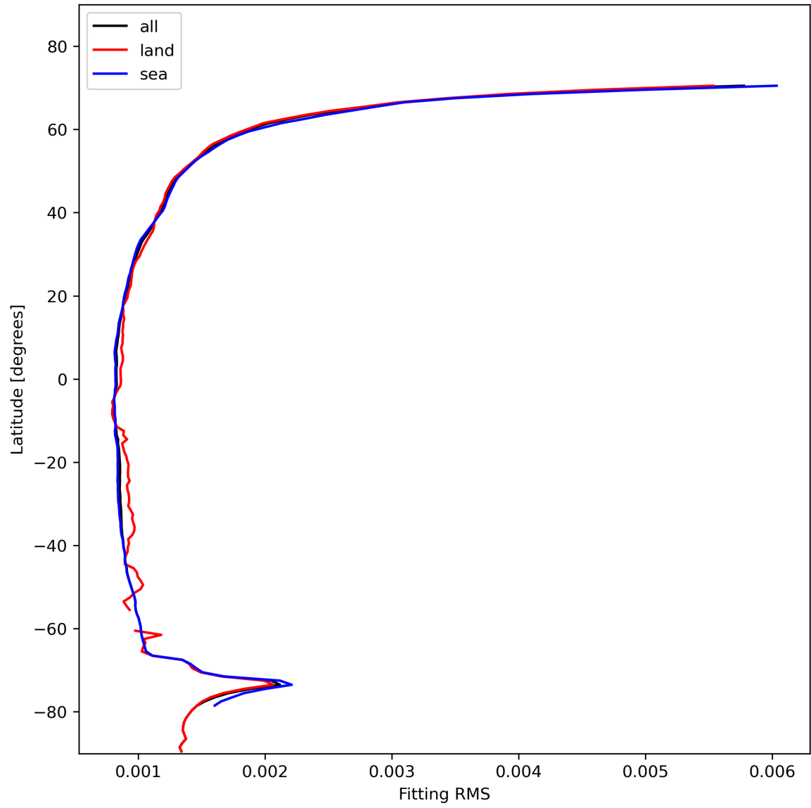
Figure 16: Zonal average of “Fitting RMS” for 2024-01-27 to 2024-01-29.
