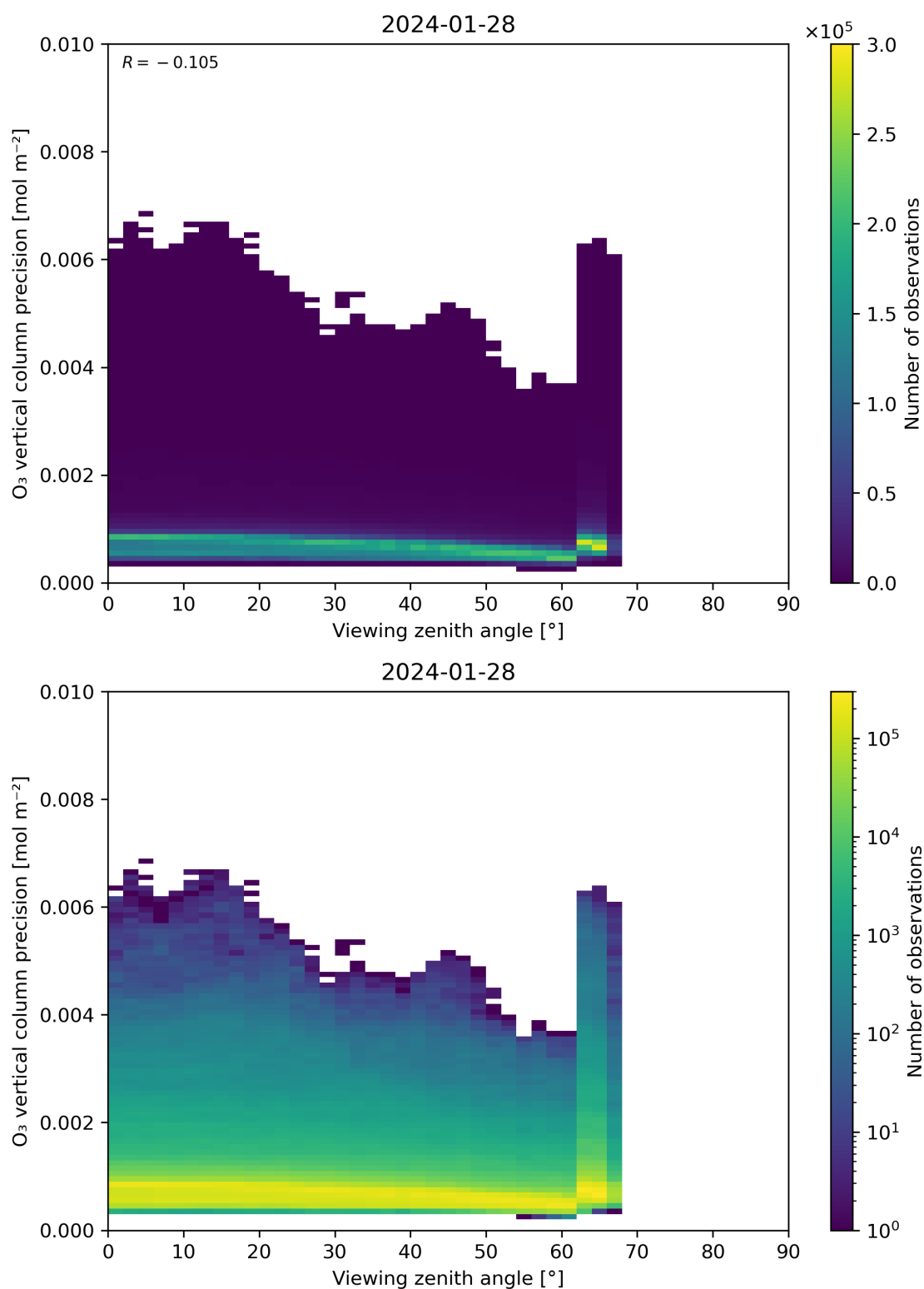
Figure 53: Scatter density plot of “Viewing zenith angle” against “O 3 vertical column precision” for 2024-01-27 to 2024-01-29.
