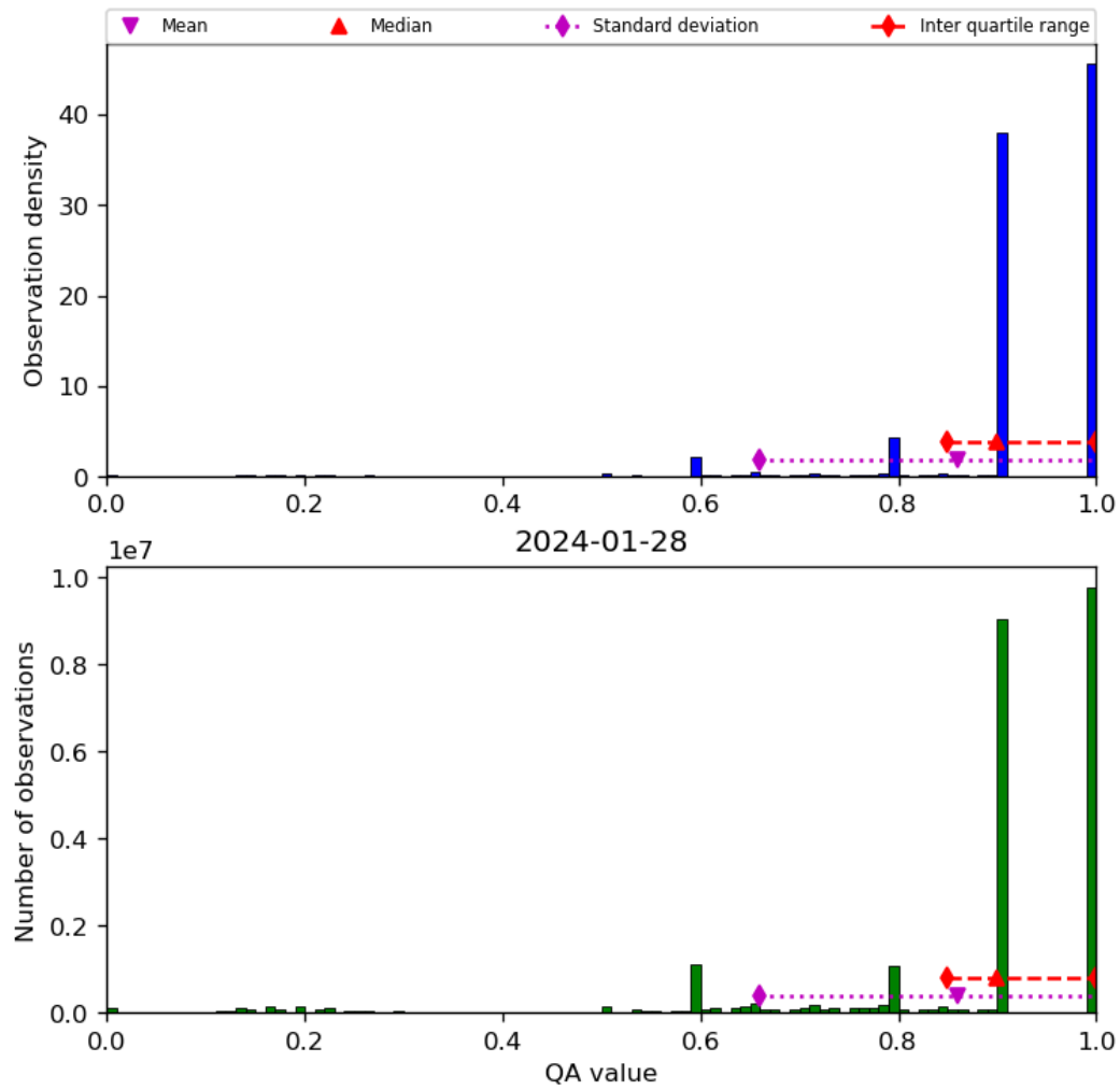
Figure 20: Histogram of “QA value” for 2024-01-27 to 2024-01-29
