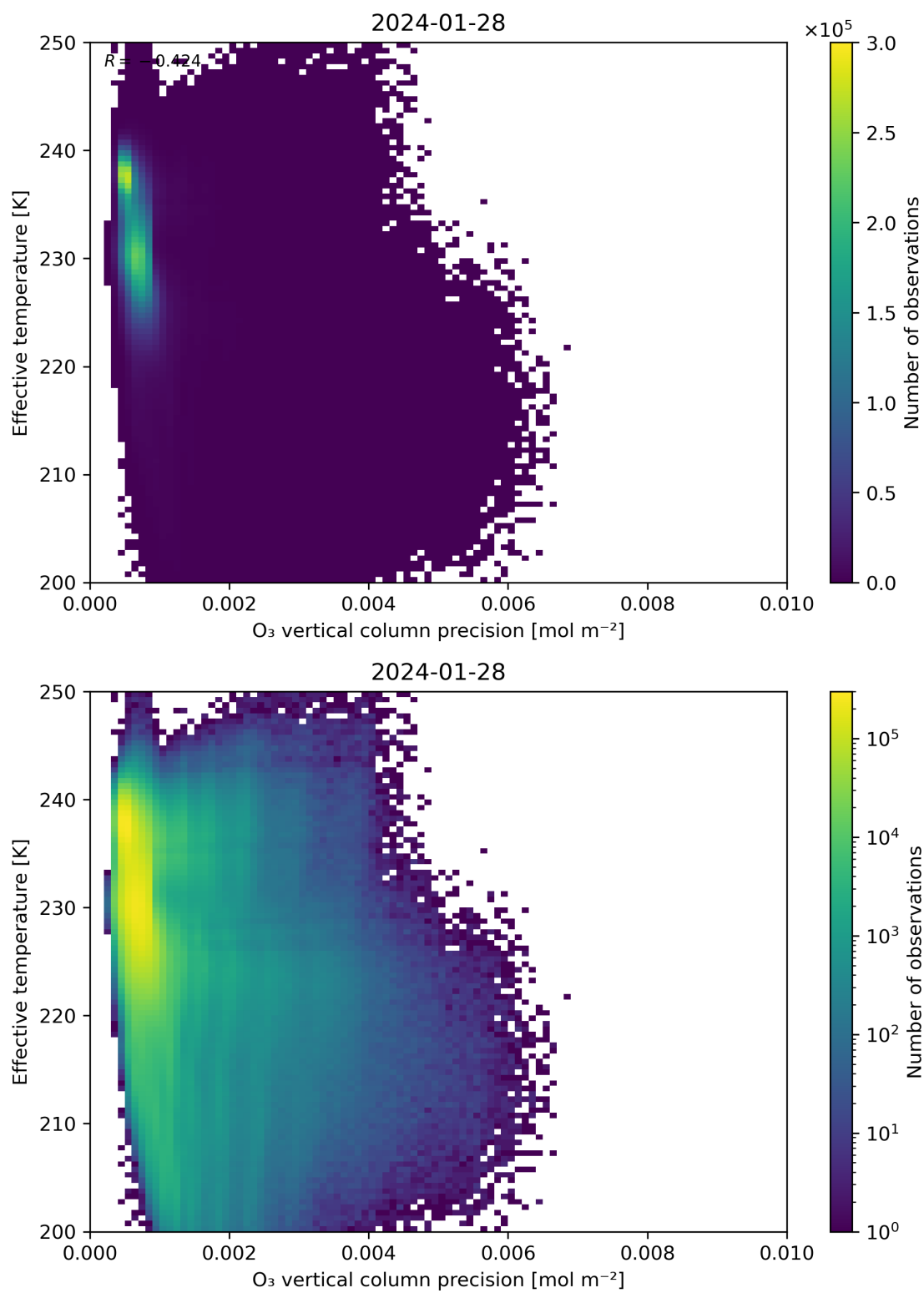
Figure 42: Scatter density plot of “O 3 vertical column precision” against “Effective temperature” for 2024-01-27 to 2024-01-29.
