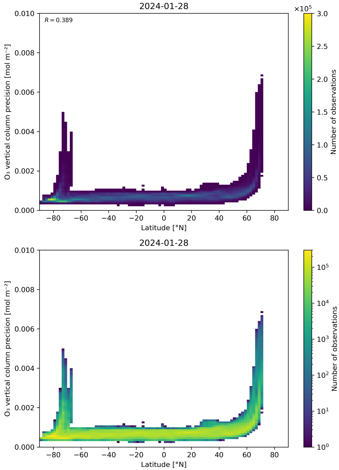
Figure 37: Scatter density plot of “Latitude” against “O 3 vertical column precision” for 2024-01-27 to 2024-01-29.
