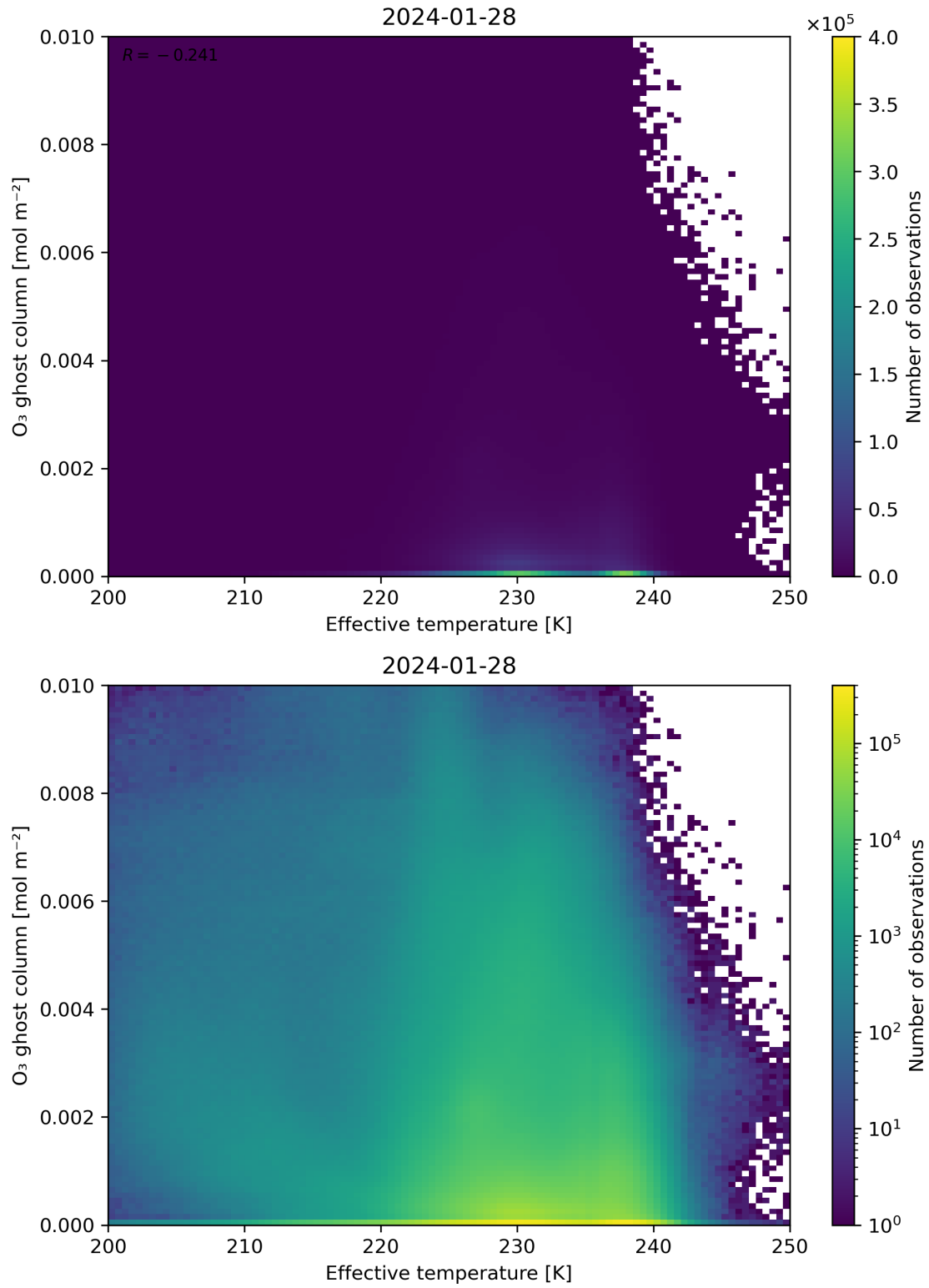
Figure 38: Scatter density plot of “Effective temperature” against “O 3 ghost column” for 2024-01-27 to 2024-01-29.
