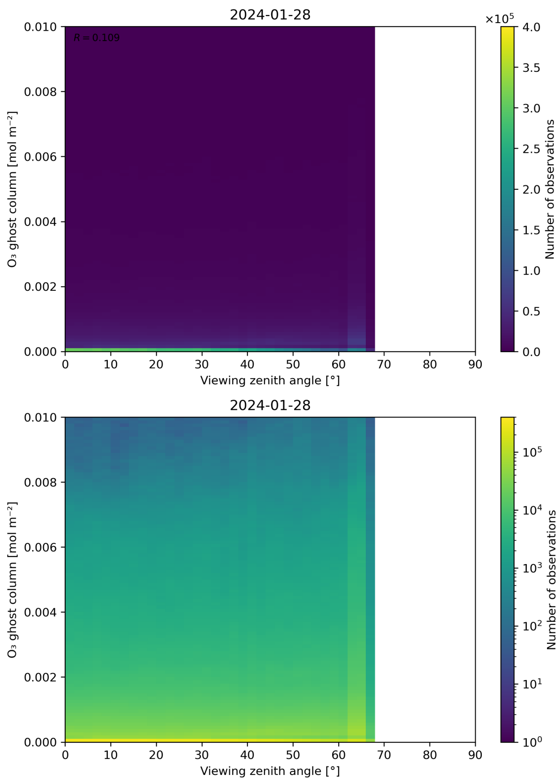
Figure 51: Scatter density plot of “Viewing zenith angle” against “O 3 ghost column” for 2024-01-27 to 2024-01-29.
