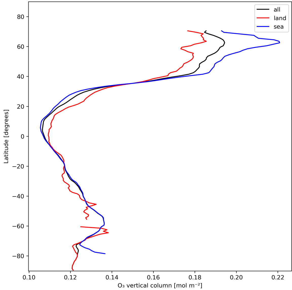
Figure 14: Zonal average of “O 3 vertical column” for 2024-01-27 to 2024-01-29.
