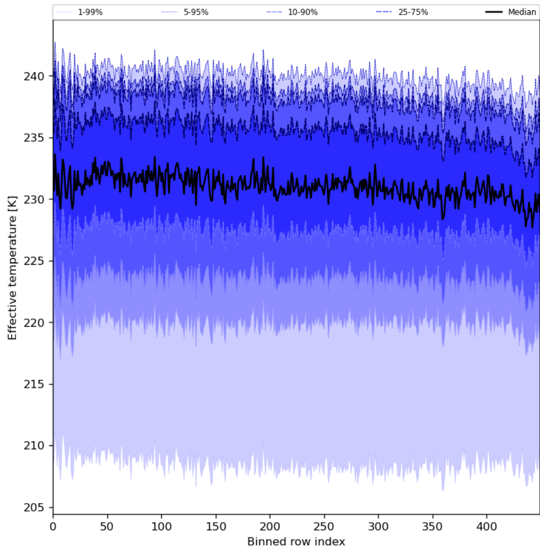
Figure 31: Along track statistics of “Effective temperature” for 2024-01-27 to 2024-01-29
