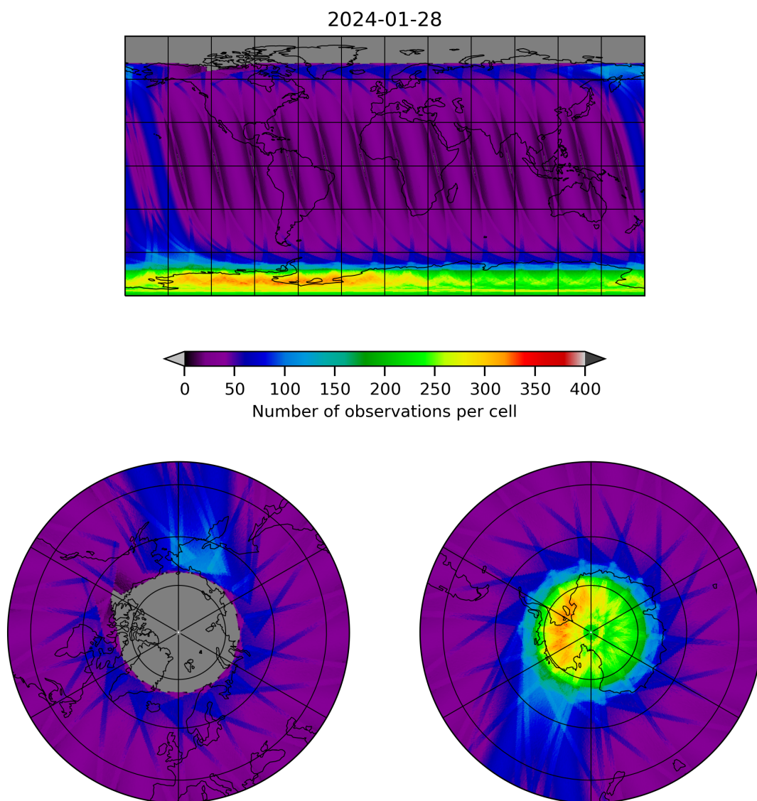
Figure 12: Map of the number of observations for 2024-01-27 to 2024-01-29
