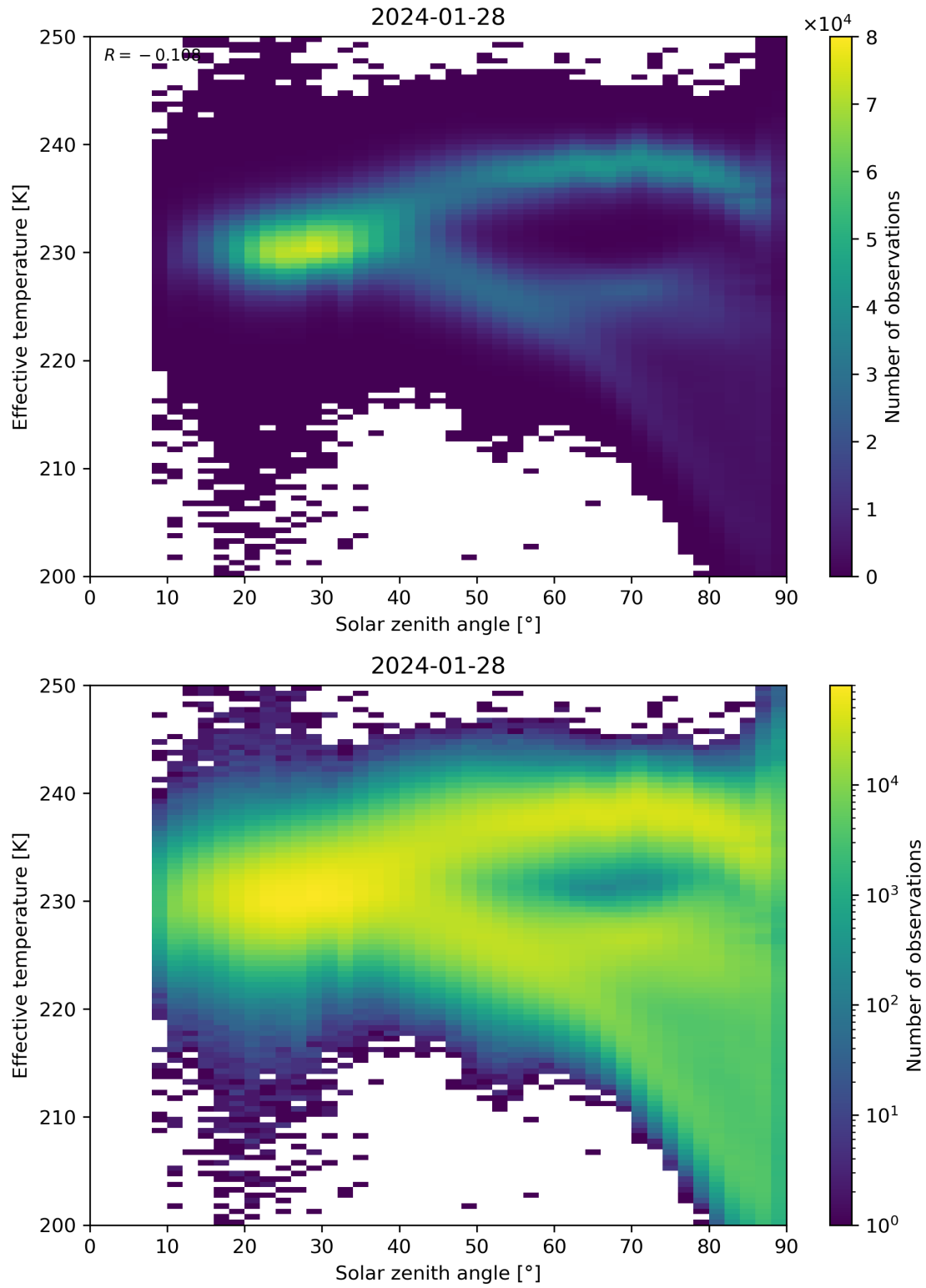
Figure 45: Scatter density plot of “Solar zenith angle” against “Effective temperature” for 2024-01-27 to 2024-01-29.
