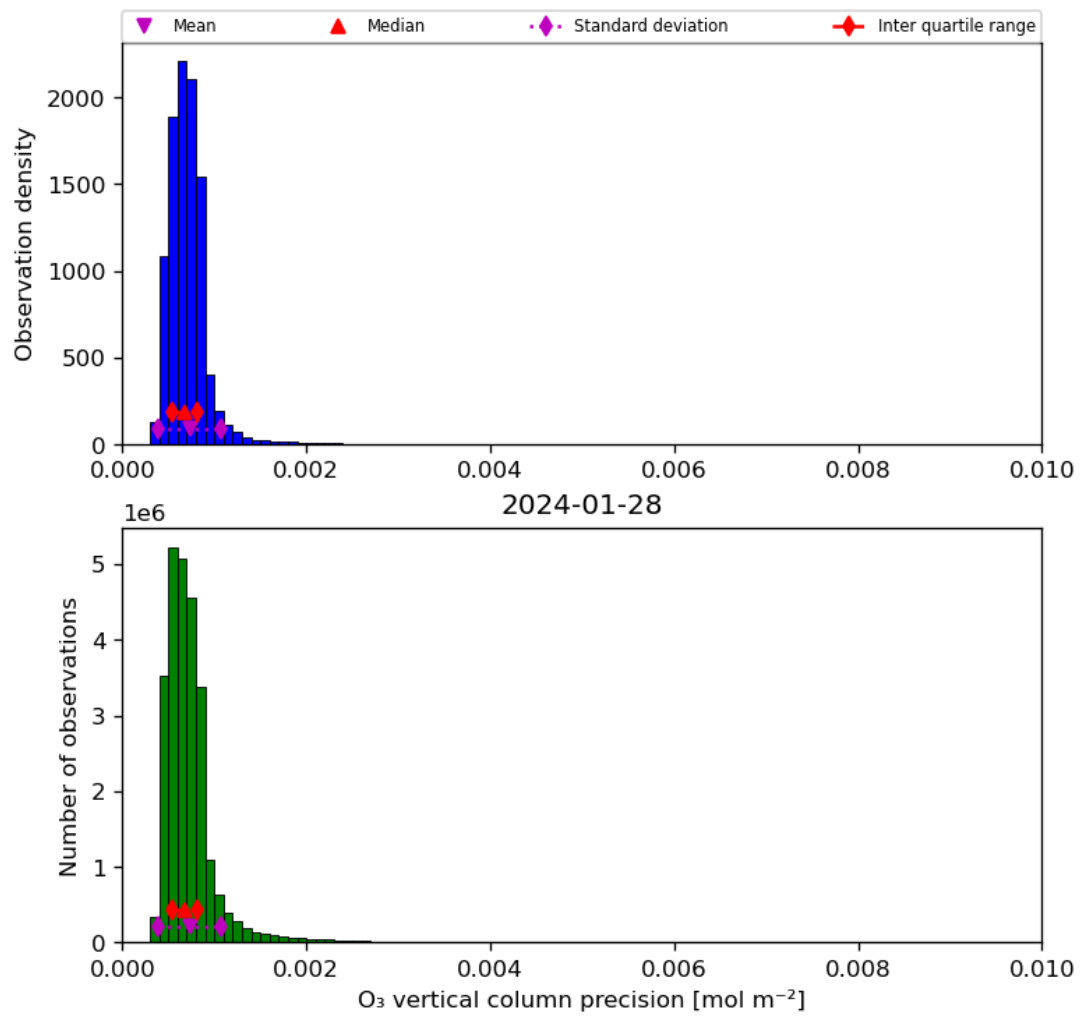
Figure 22: Histogram of “O 3 vertical column precision” for 2024-01-27 to 2024-01-29
