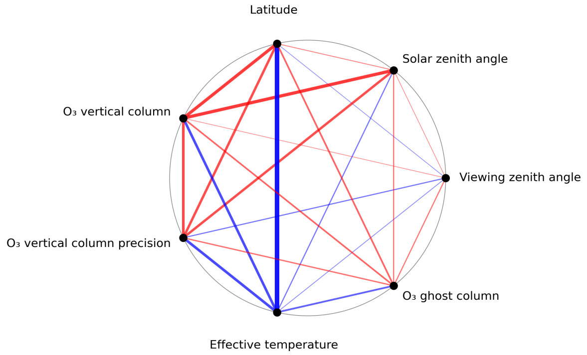
Figure 1: Map of correlation graph for 2024-01-27 to 2024-01-29.
