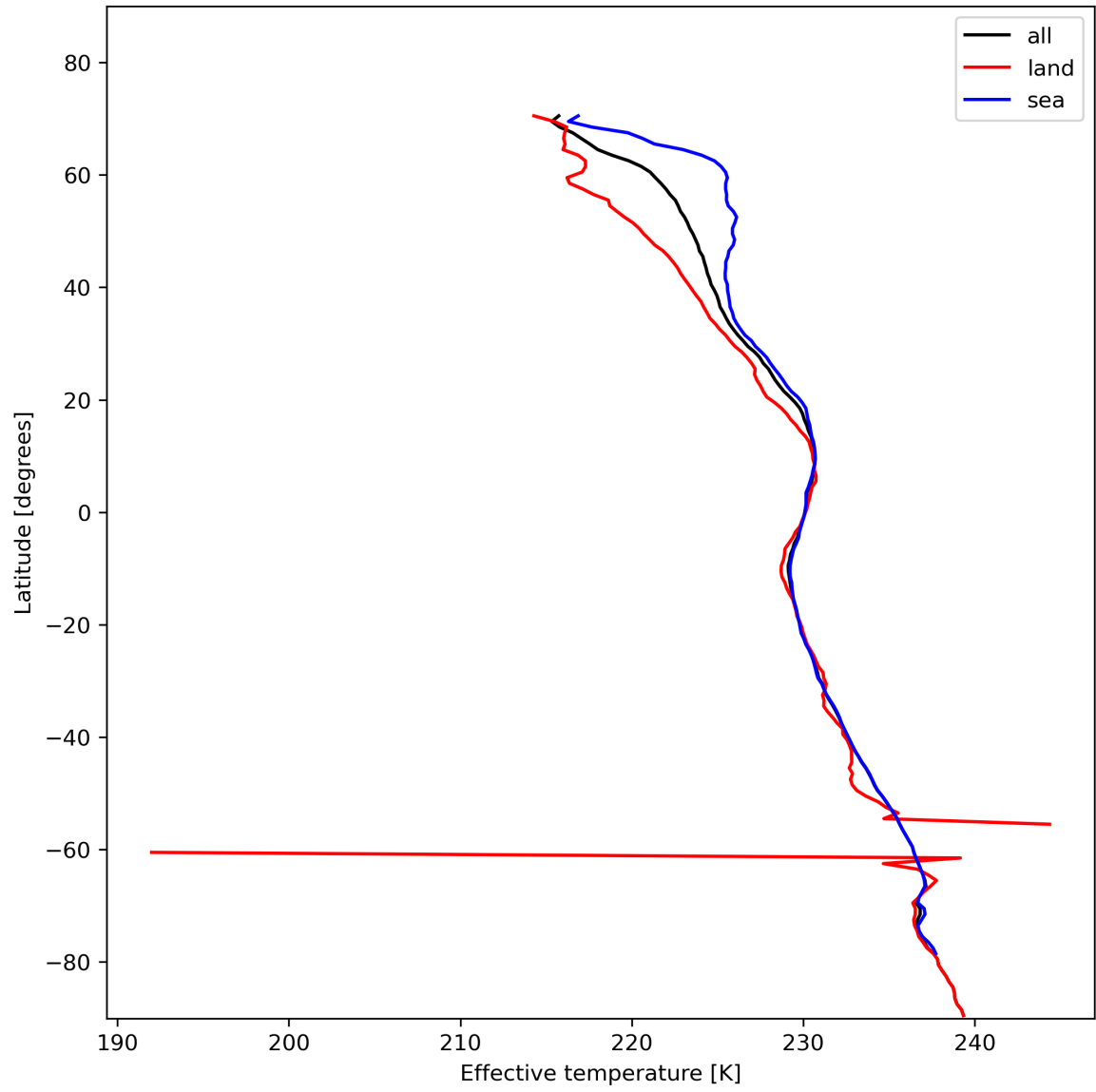
Figure 17: Zonal average of “Effective temperature” for 2024-01-27 to 2024-01-29.
