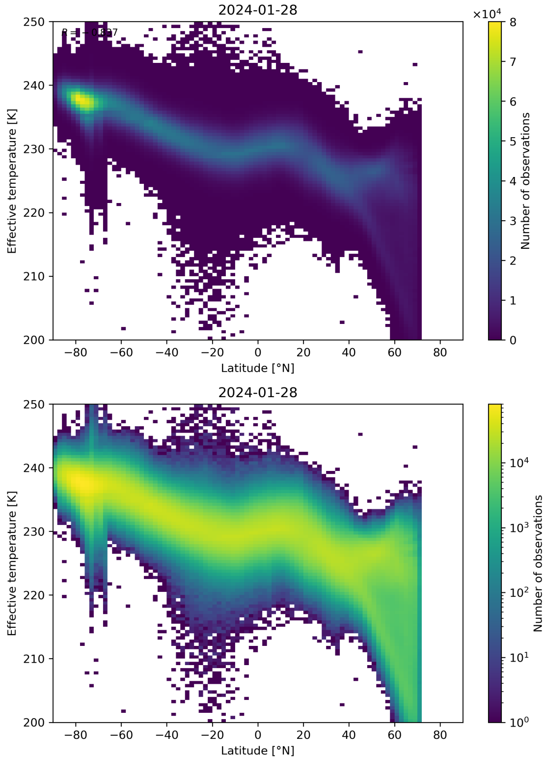
Figure 34: Scatter density plot of “Latitude” against “Effective temperature” for 2024-01-27 to 2024-01-29.
