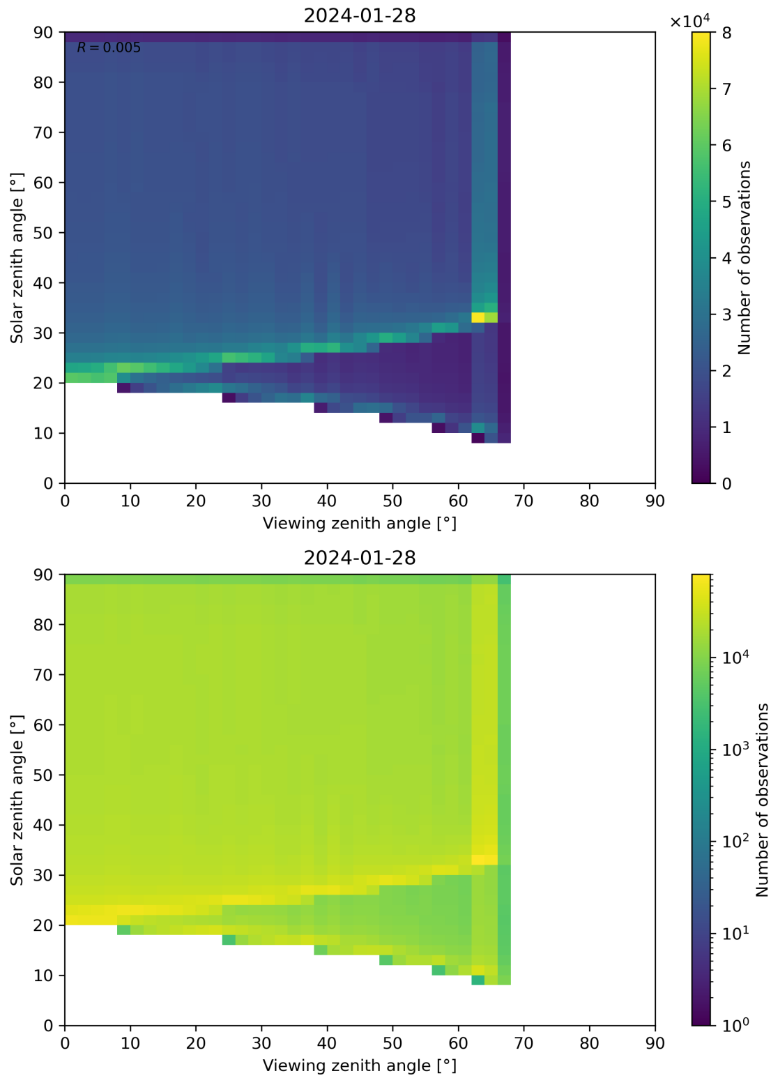
Figure 54: Scatter density plot of “Viewing zenith angle” against “Solar zenith angle” for 2024-01-27 to 2024-01-29.
