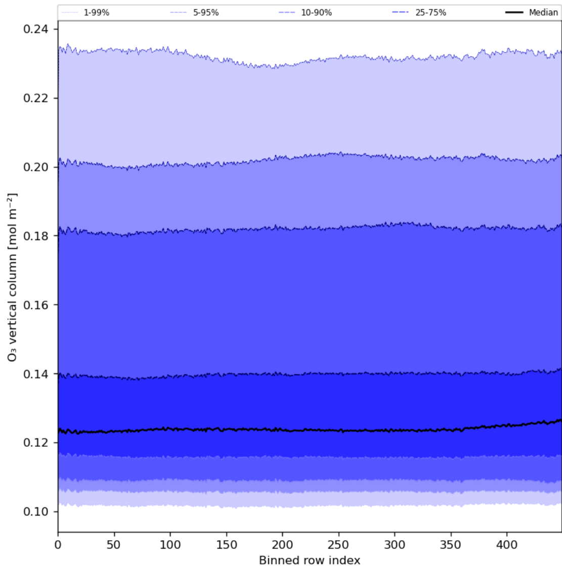
Figure 28: Along track statistics of “O 3 vertical column” for 2024-01-27 to 2024-01-29
