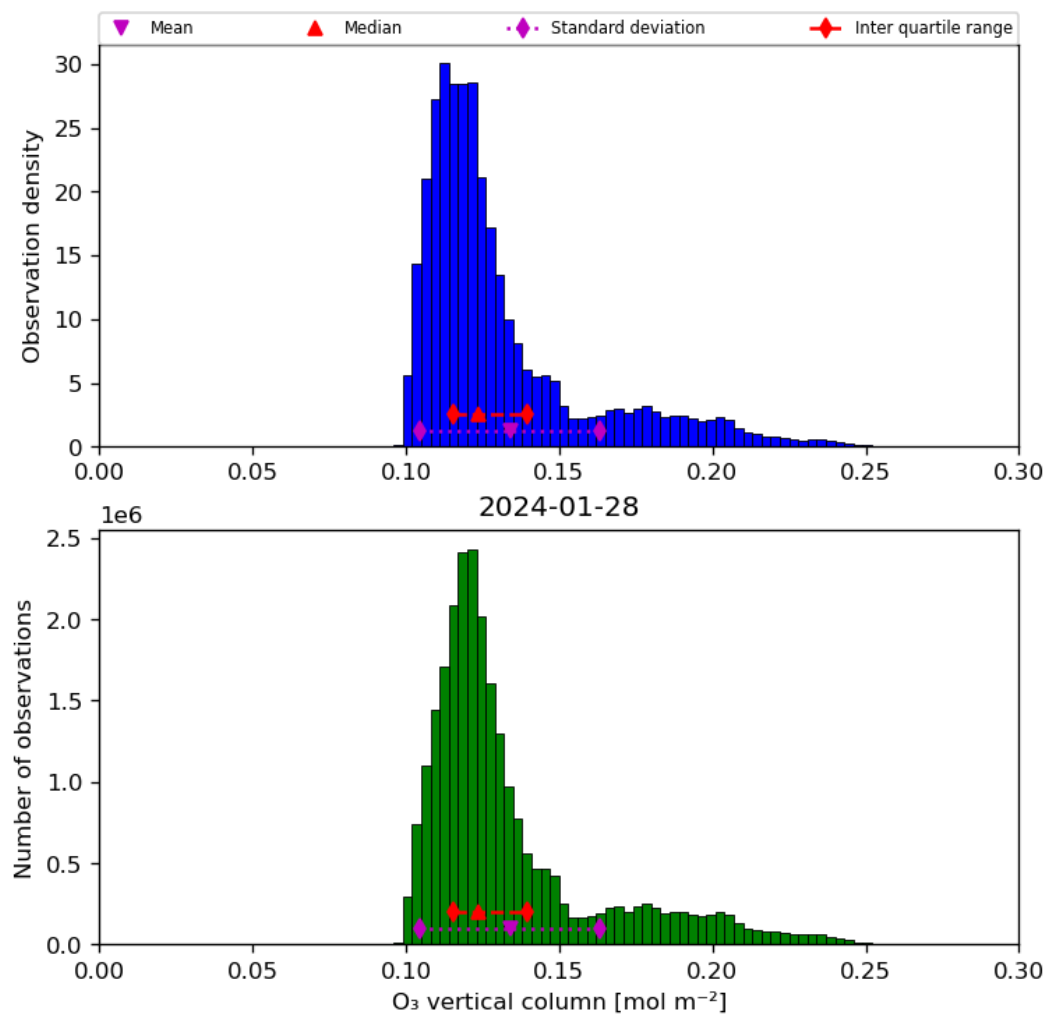
Figure 21: Histogram of “O 3 vertical column” for 2024-01-27 to 2024-01-29
