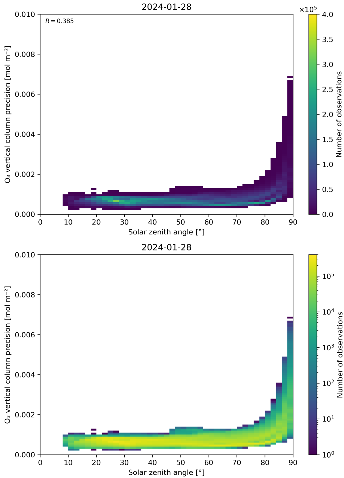
Figure 48: Scatter density plot of “Solar zenith angle” against “O 3 vertical column precision” for 2024-01-27 to 2024-01-29.
