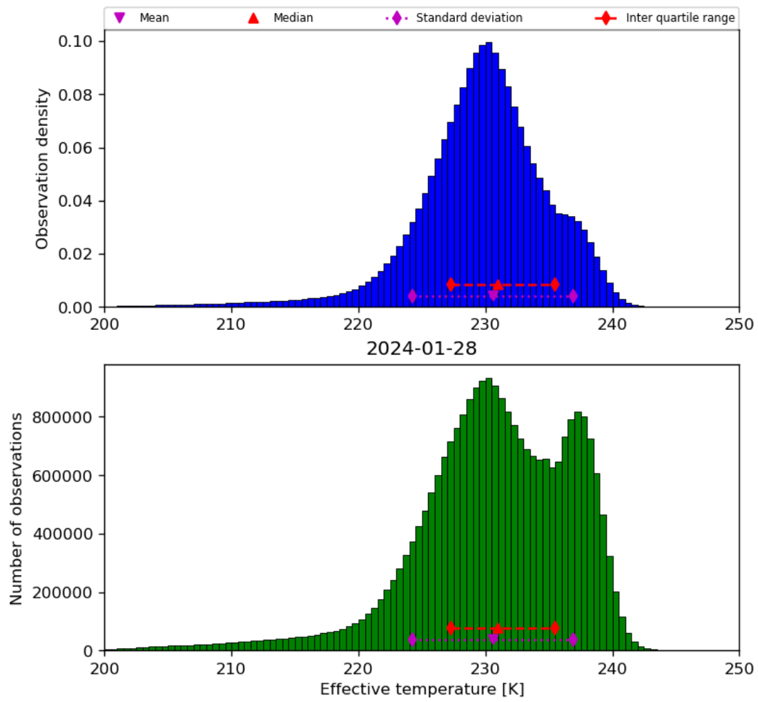
Figure 24: Histogram of “Effective temperature” for 2024-01-27 to 2024-01-29
