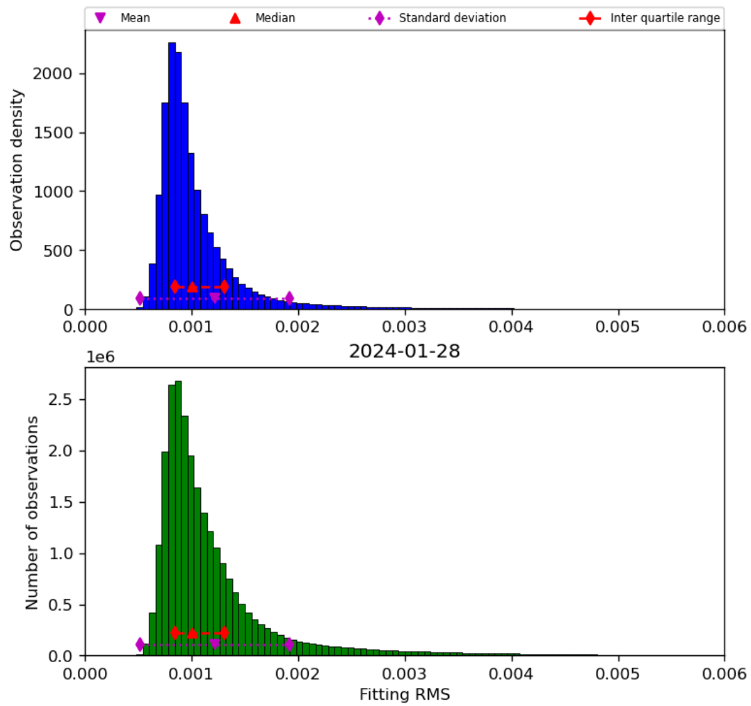
Figure 23: Histogram of “Fitting RMS” for 2024-01-27 to 2024-01-29
