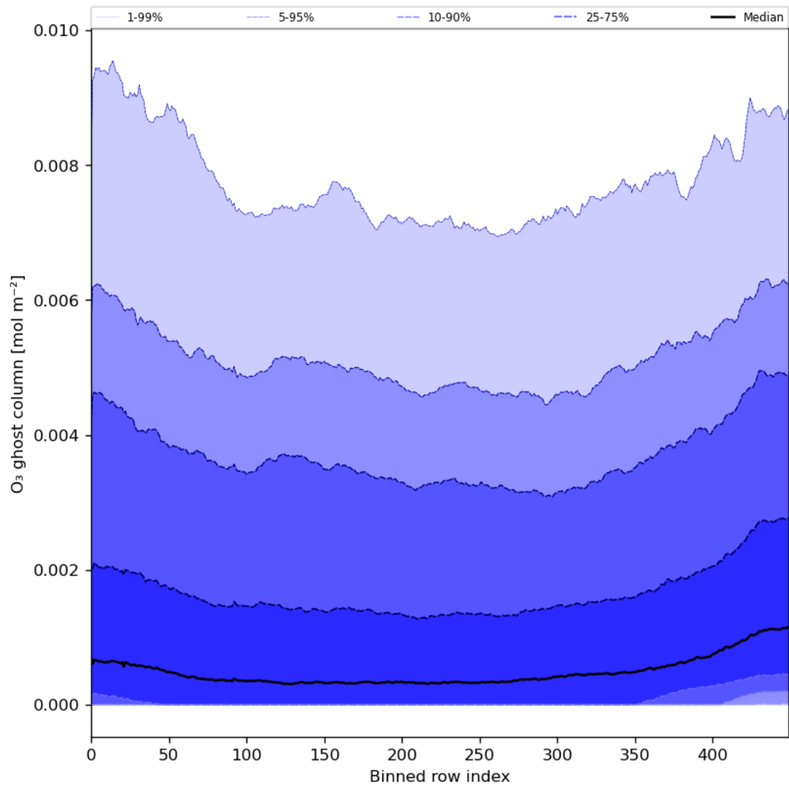
Figure 32: Along track statistics of “O 3 ghost column” for 2024-01-27 to 2024-01-29
