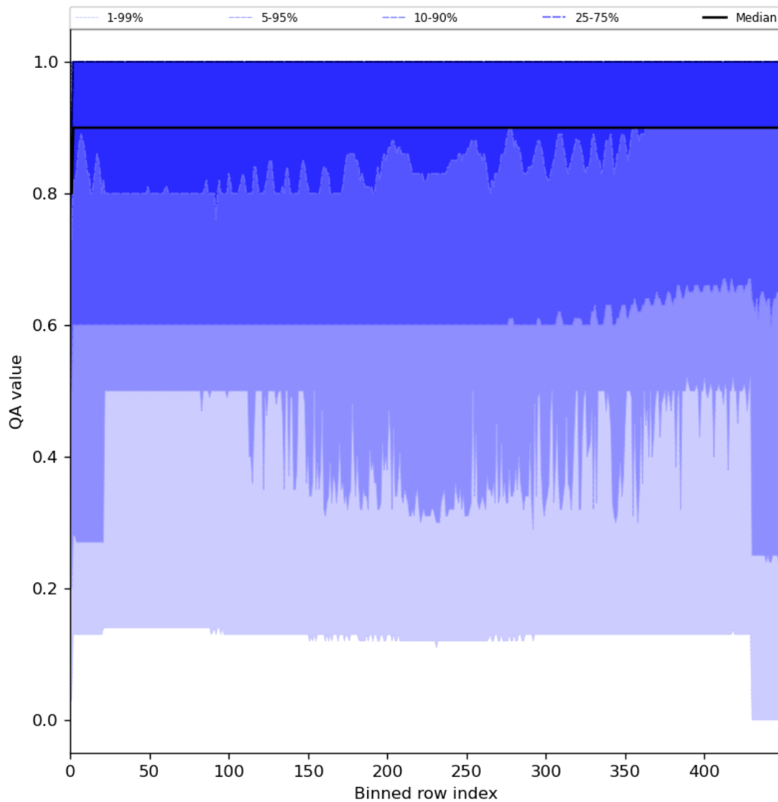
Figure 27: Along track statistics of “QA value” for 2024-01-27 to 2024-01-29
