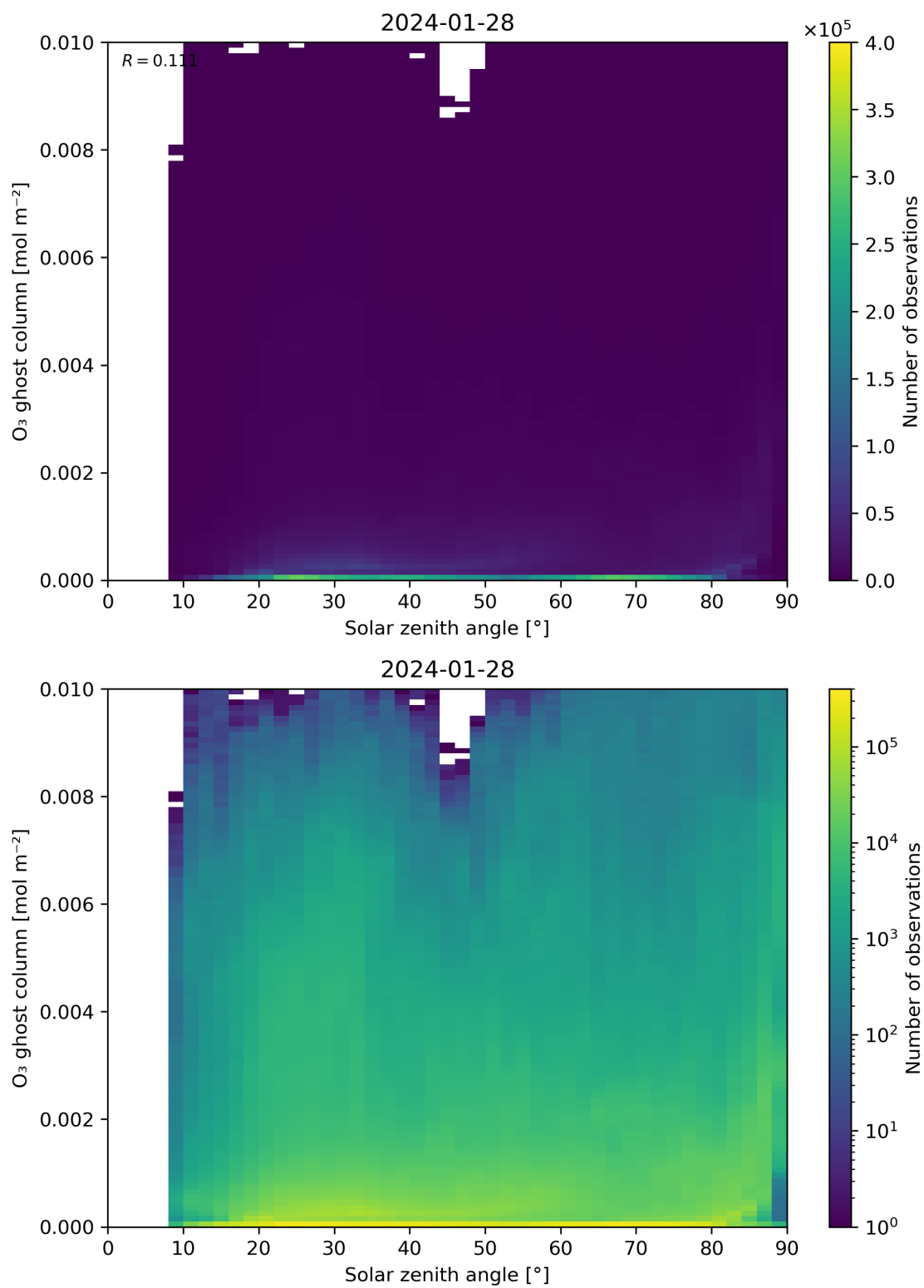
Figure 46: Scatter density plot of “Solar zenith angle” against “O 3 ghost column” for 2024-01-27 to 2024-01-29.
