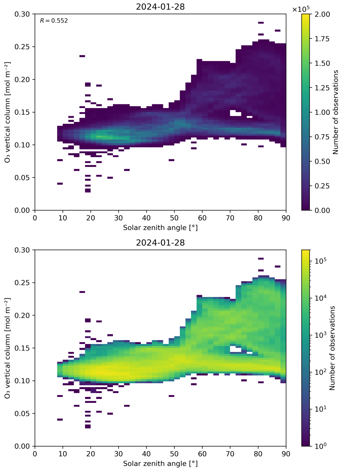
Figure 47: Scatter density plot of “Solar zenith angle” against “O 3 vertical column” for 2024-01-27 to 2024-01-29.
