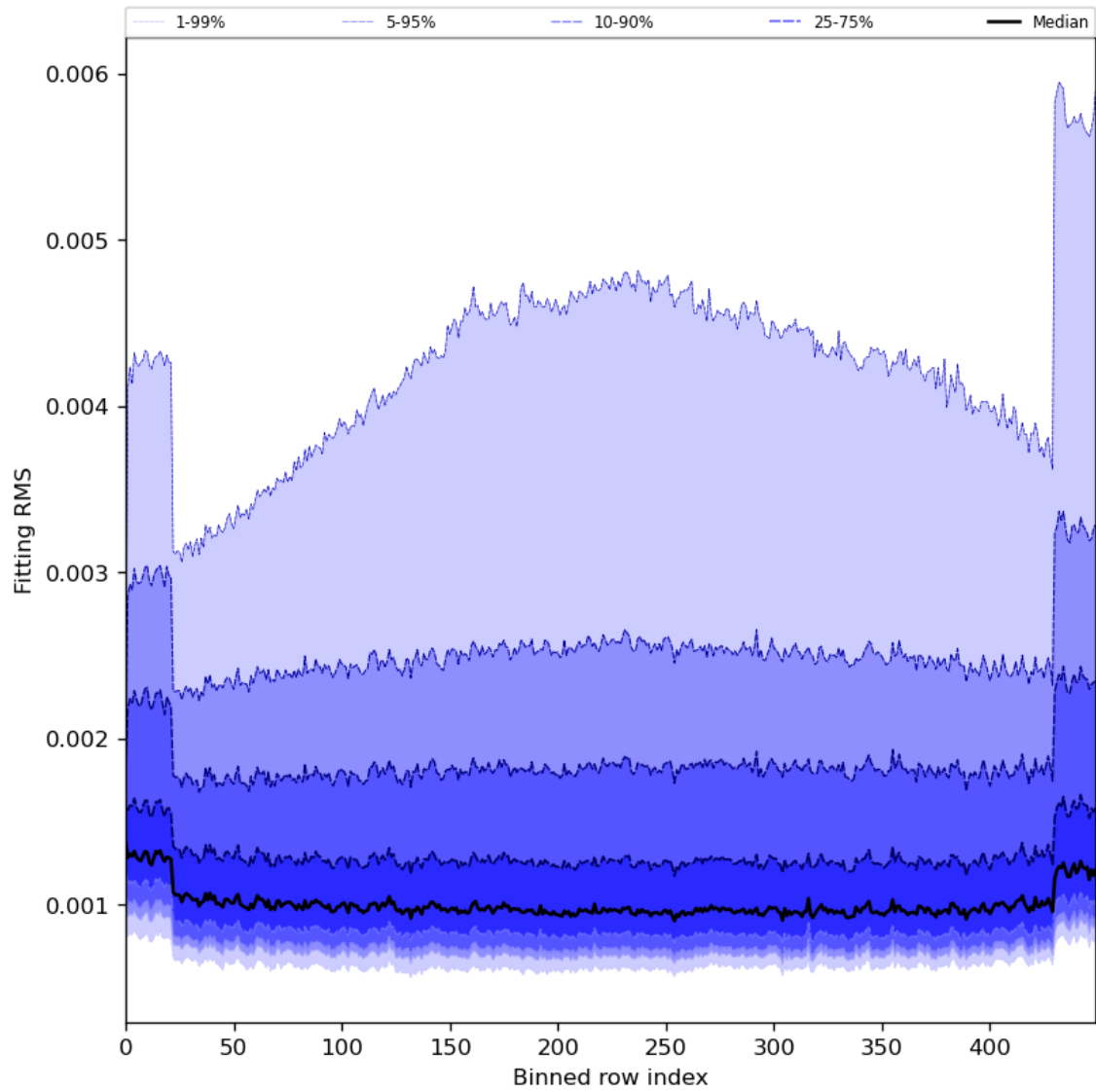
Figure 30: Along track statistics of “Fitting RMS” for 2024-01-27 to 2024-01-29
