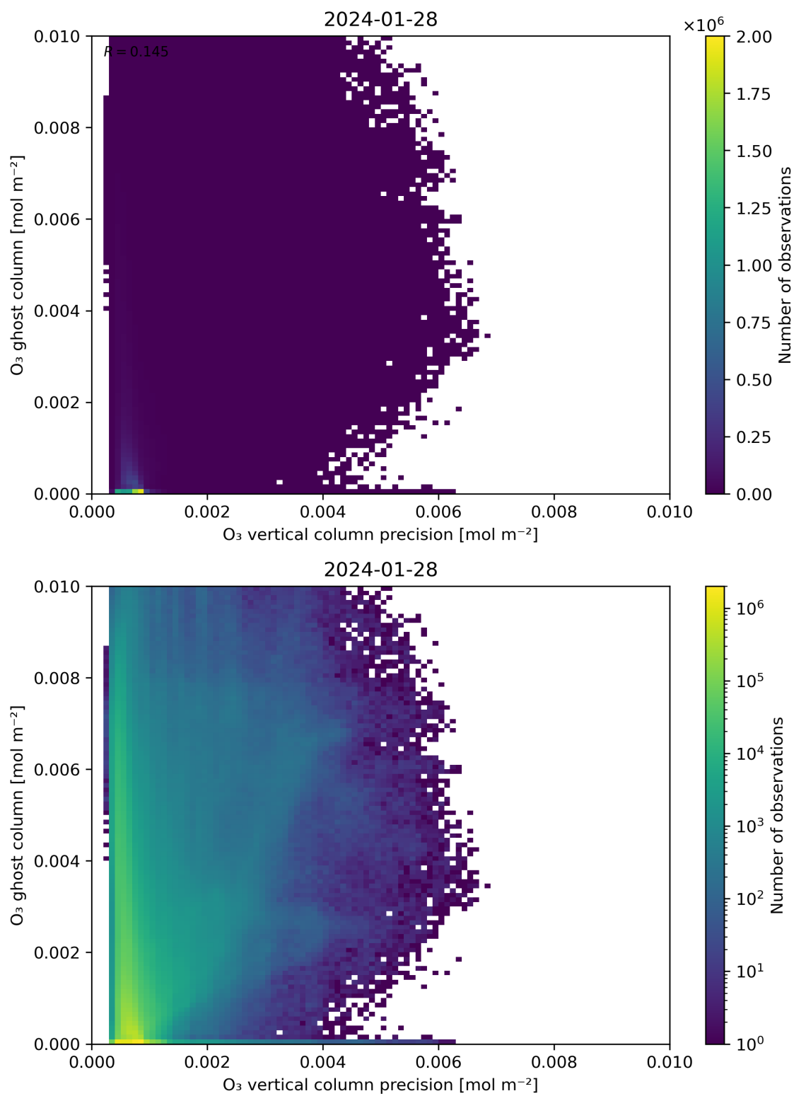
Figure 43: Scatter density plot of “O 3 vertical column precision” against “O 3 ghost column” for 2024-01-27 to 2024-01-29.
