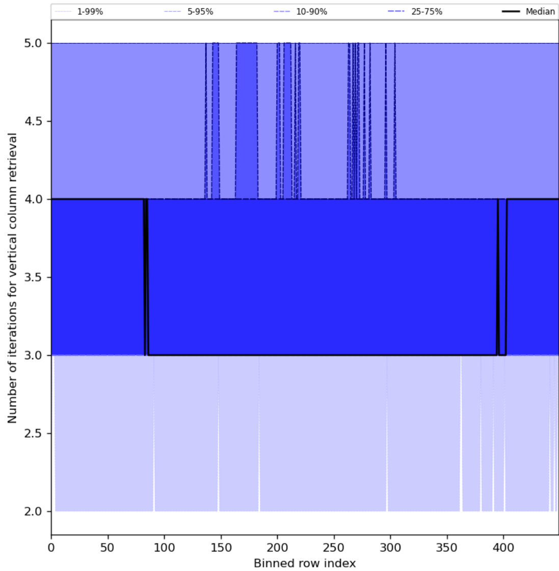
Figure 33: Along track statistics of “Number of iterations for vertical column retrieval” for 2024-01-27 to 2024-01-29
