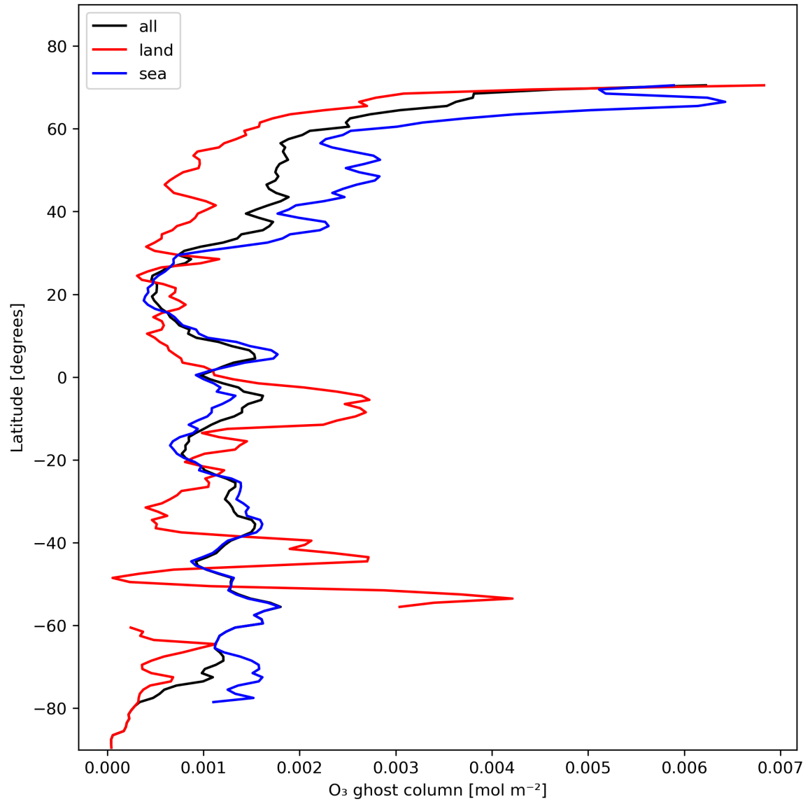
Figure 18: Zonal average of “O 3 ghost column” for 2024-01-27 to 2024-01-29.
