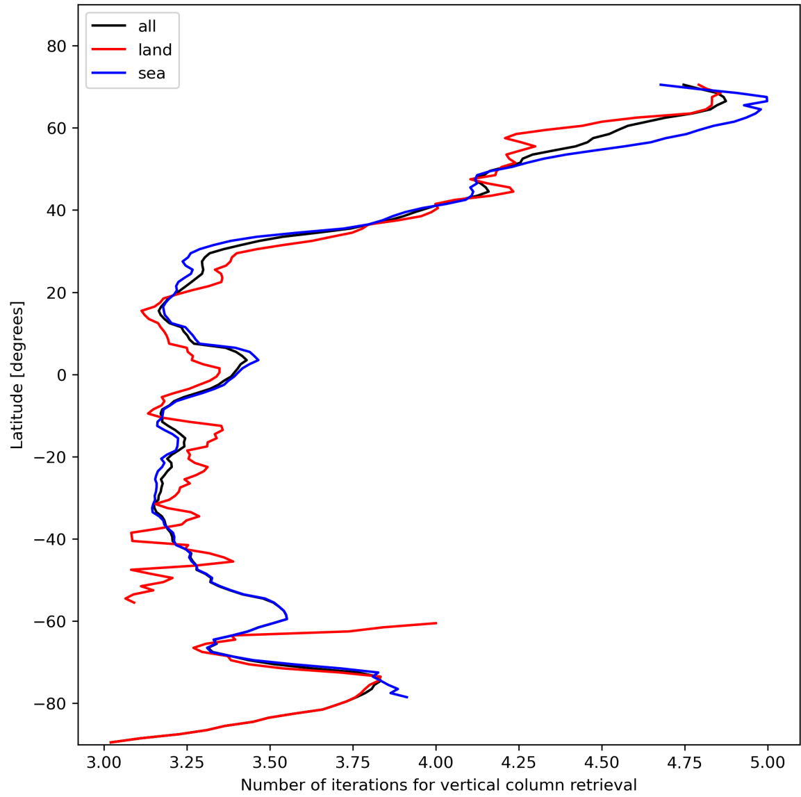
Figure 19: Zonal average of “Number of iterations for vertical column retrieval” for 2024-01-27 to 2024-01-29.
