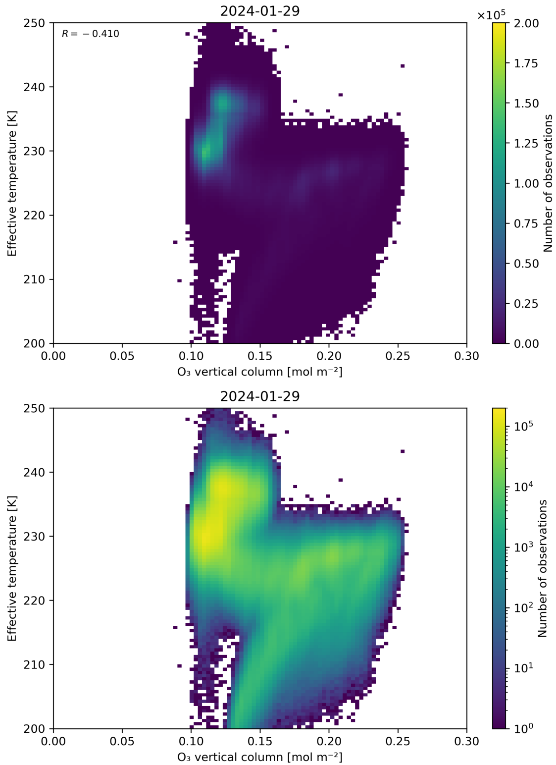
Figure 39: Scatter density plot of “O 3 vertical column” against “Effective temperature” for 2024-01-28 to 2024-01-30.
