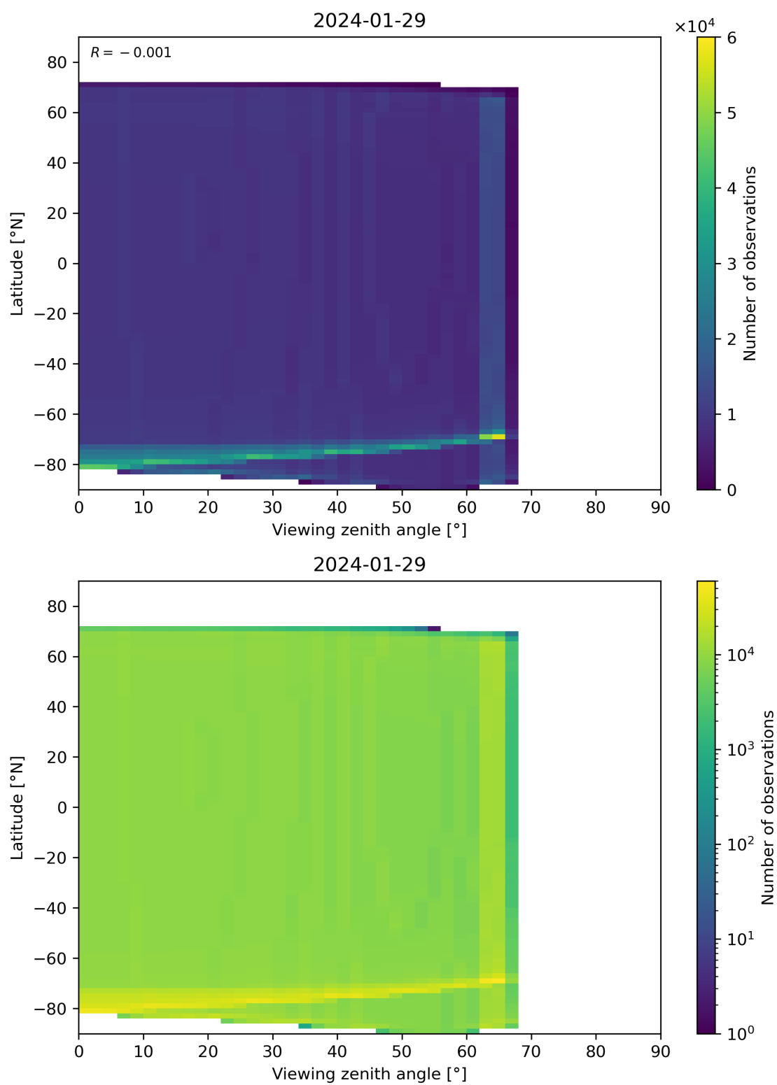
Figure 49: Scatter density plot of “Viewing zenith angle” against “Latitude” for 2024-01-28 to 2024-01-30.
