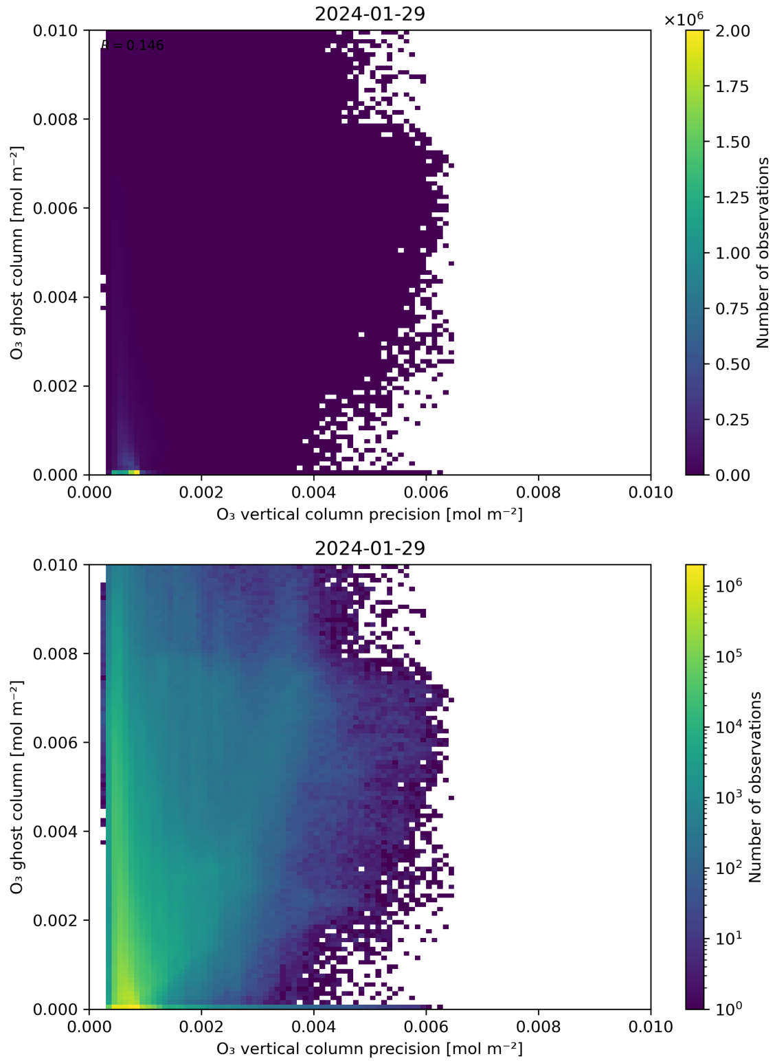
Figure 43: Scatter density plot of “O 3 vertical column precision” against “O 3 ghost column” for 2024-01-28 to 2024-01-30.
