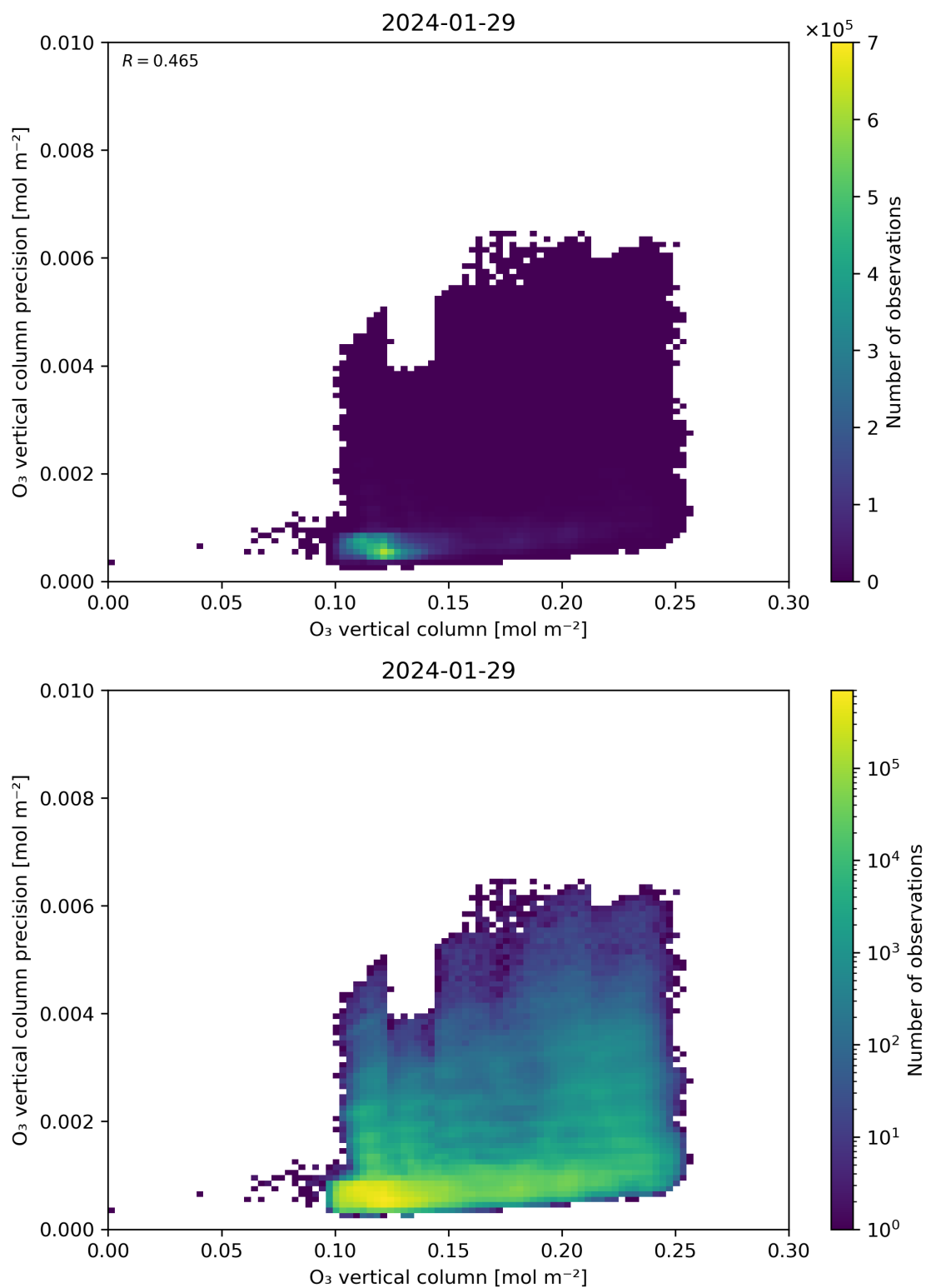
Figure 41: Scatter density plot of “O 3 vertical column” against “O 3 vertical column precision” for 2024-01-28 to 2024-01-30.
