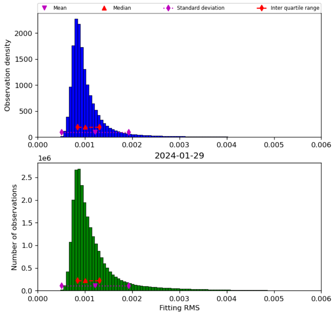
Figure 23: Histogram of “Fitting RMS” for 2024-01-28 to 2024-01-30
