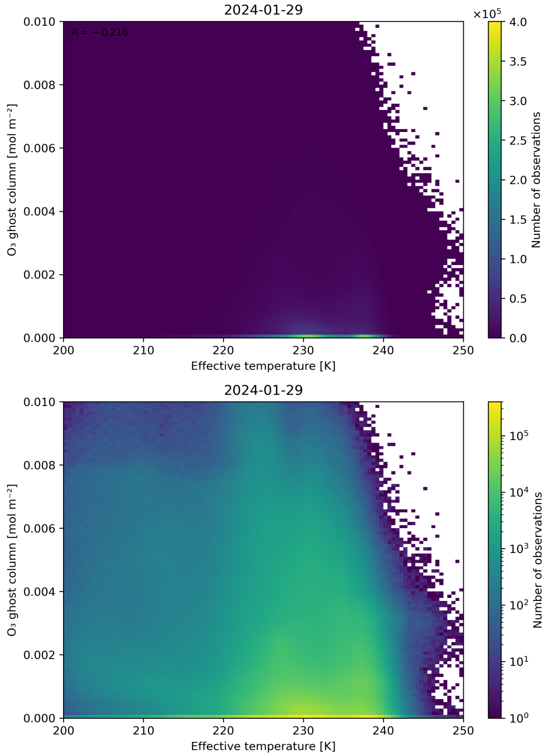
Figure 38: Scatter density plot of “Effective temperature” against “O 3 ghost column” for 2024-01-28 to 2024-01-30.
