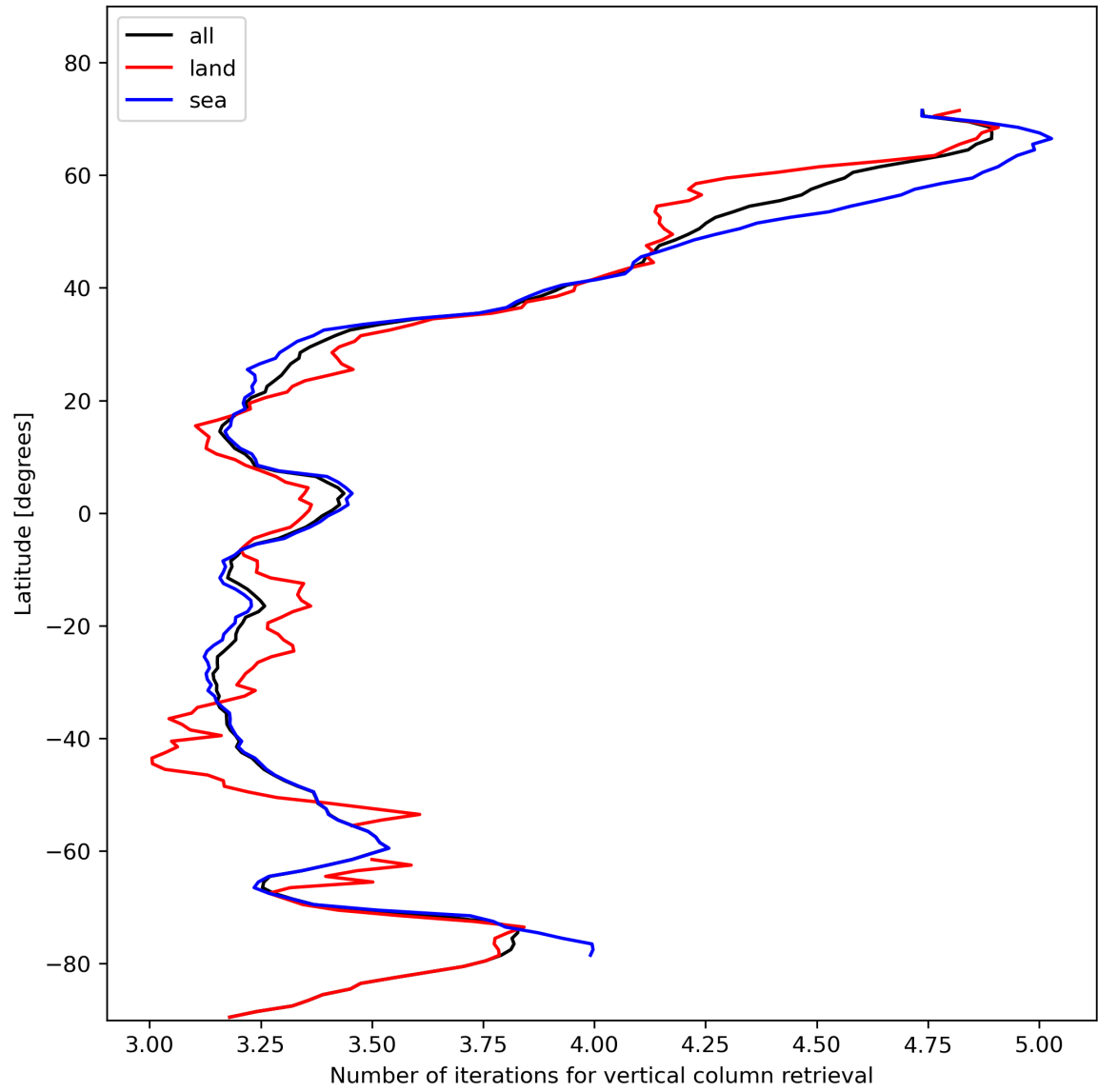
Figure 19: Zonal average of “Number of iterations for vertical column retrieval” for 2024-01-28 to 2024-01-30.
