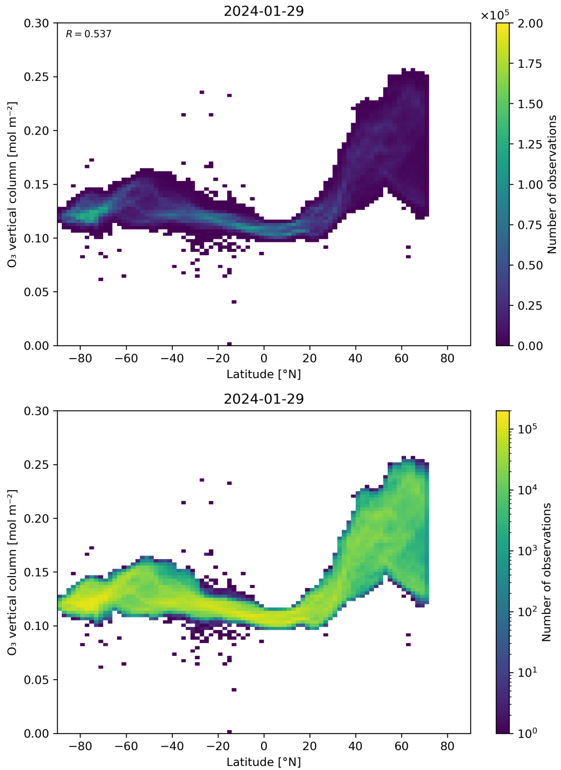
Figure 36: Scatter density plot of “Latitude” against “O 3 vertical column” for 2024-01-28 to 2024-01-30.
