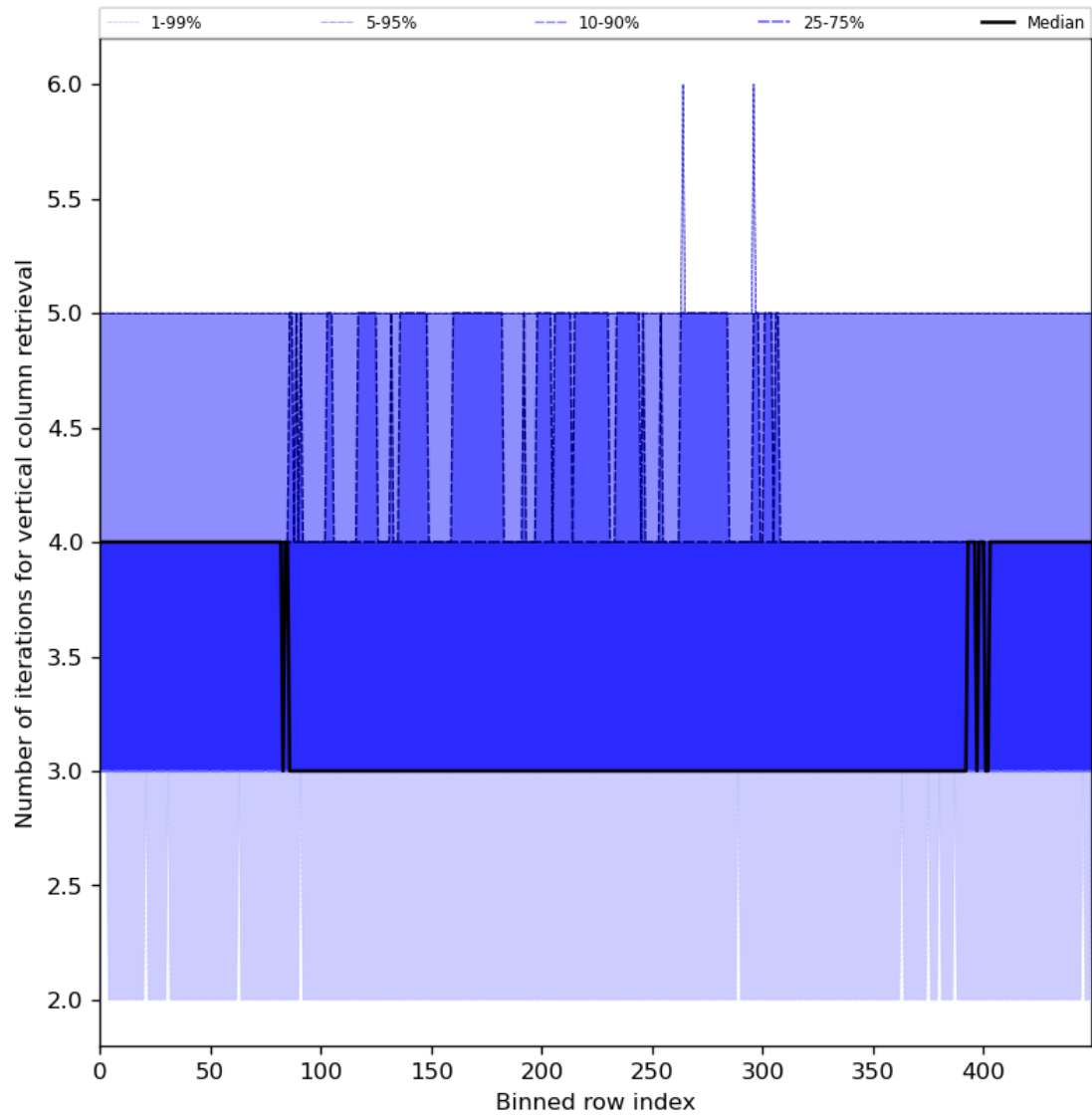
Figure 33: Along track statistics of “Number of iterations for vertical column retrieval” for 2024-01-28 to 2024-01-30
