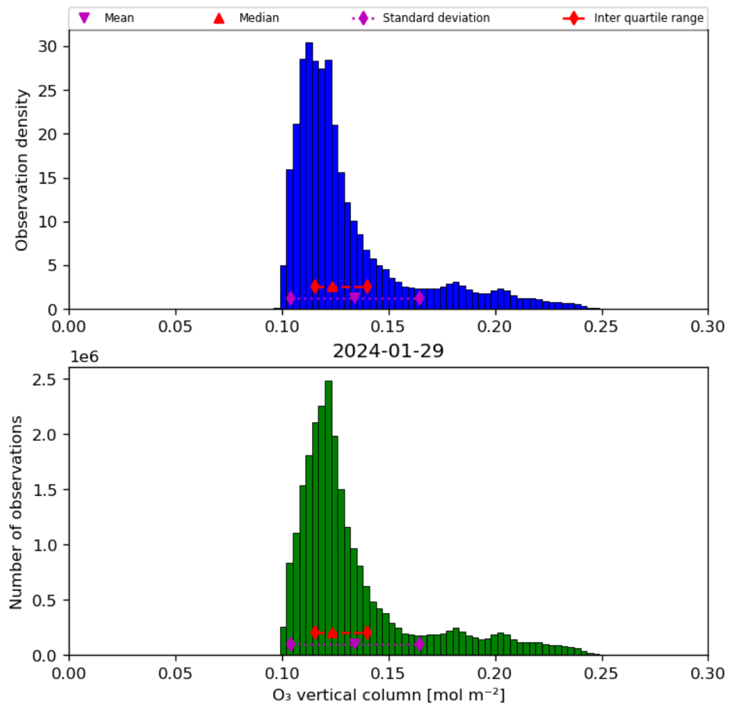
Figure 21: Histogram of “O 3 vertical column” for 2024-01-28 to 2024-01-30
