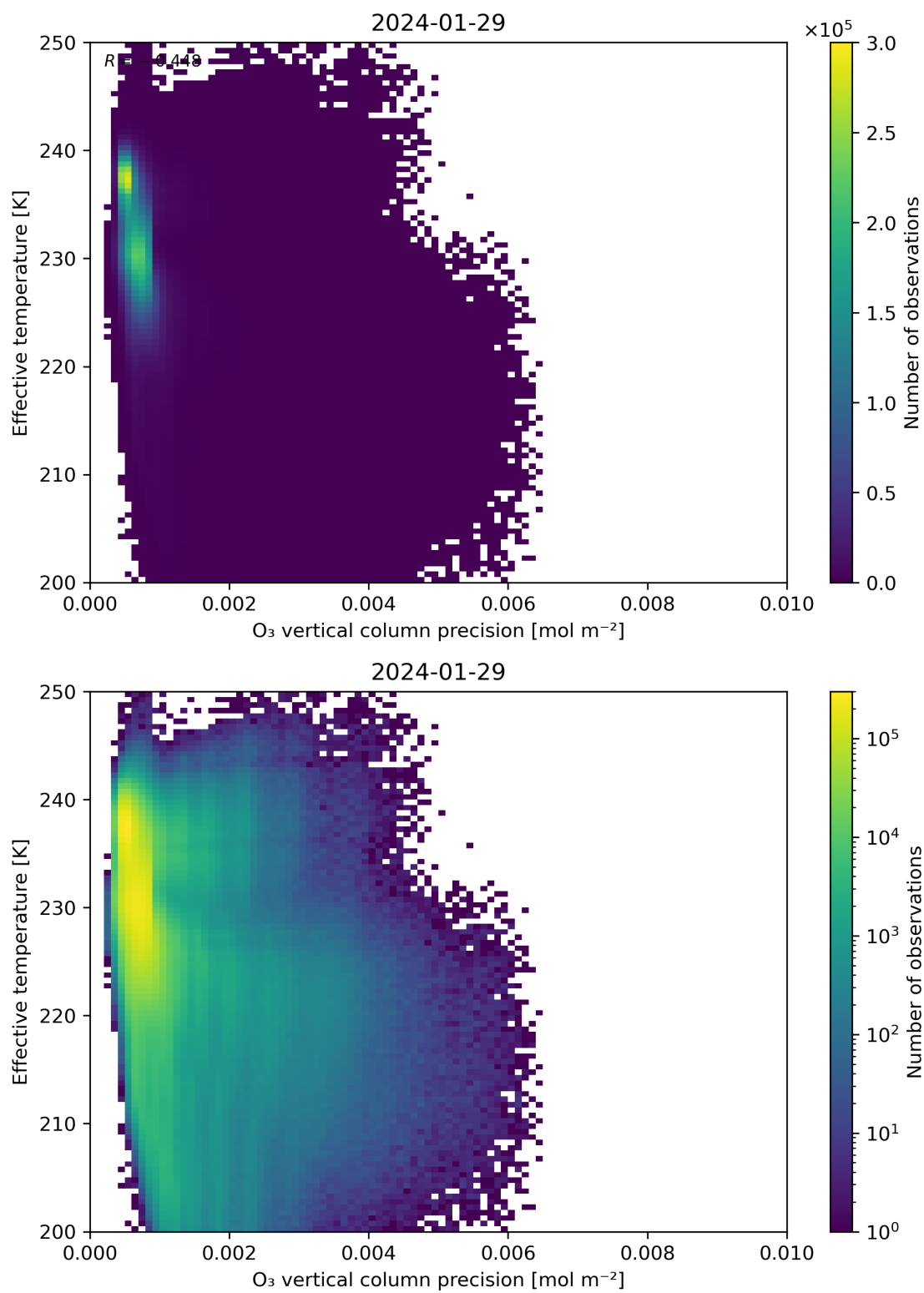
Figure 42: Scatter density plot of “O 3 vertical column precision” against “Effective temperature” for 2024-01-28 to 2024-01-30.
