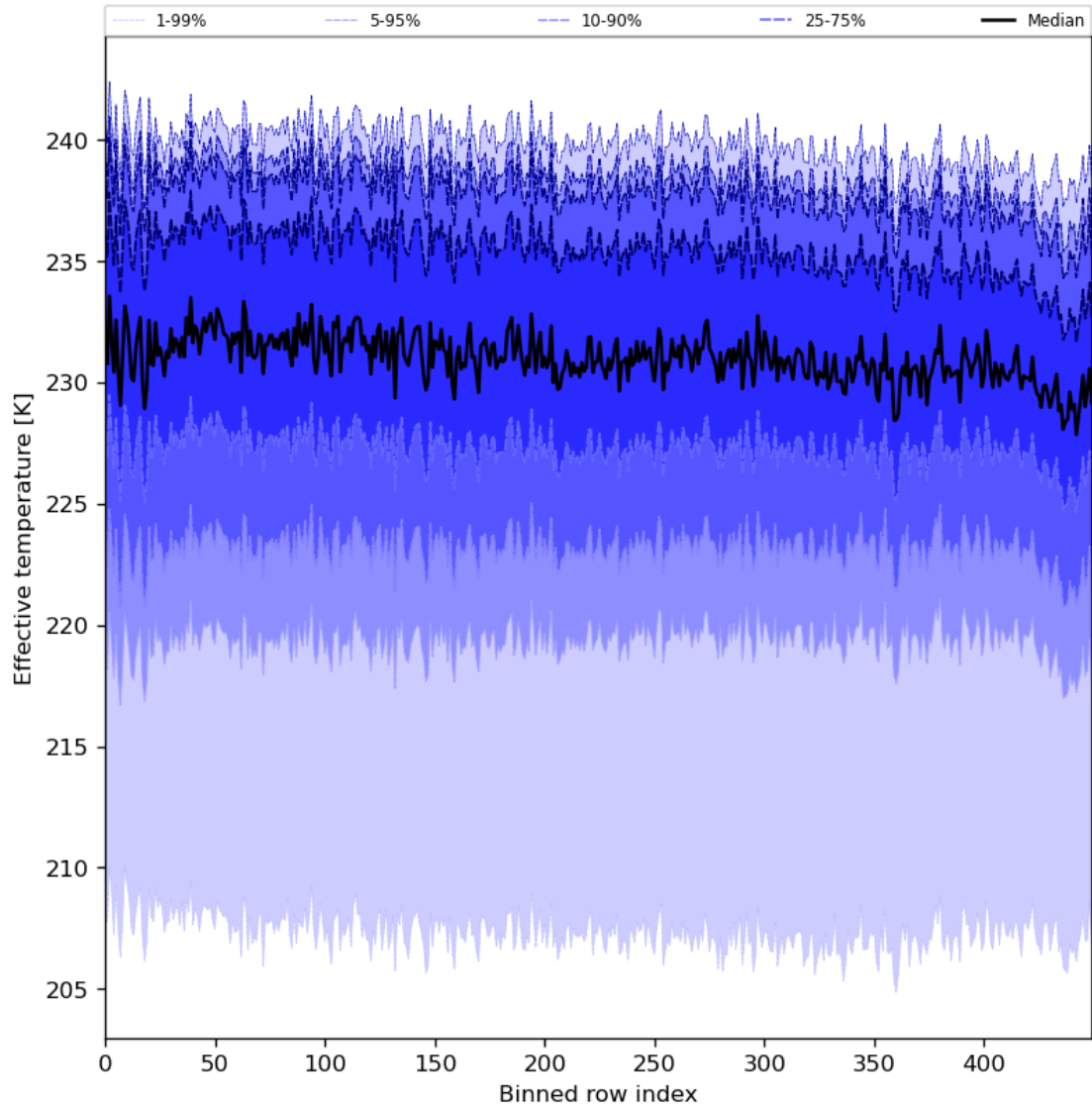
Figure 31: Along track statistics of “Effective temperature” for 2024-01-28 to 2024-01-30
