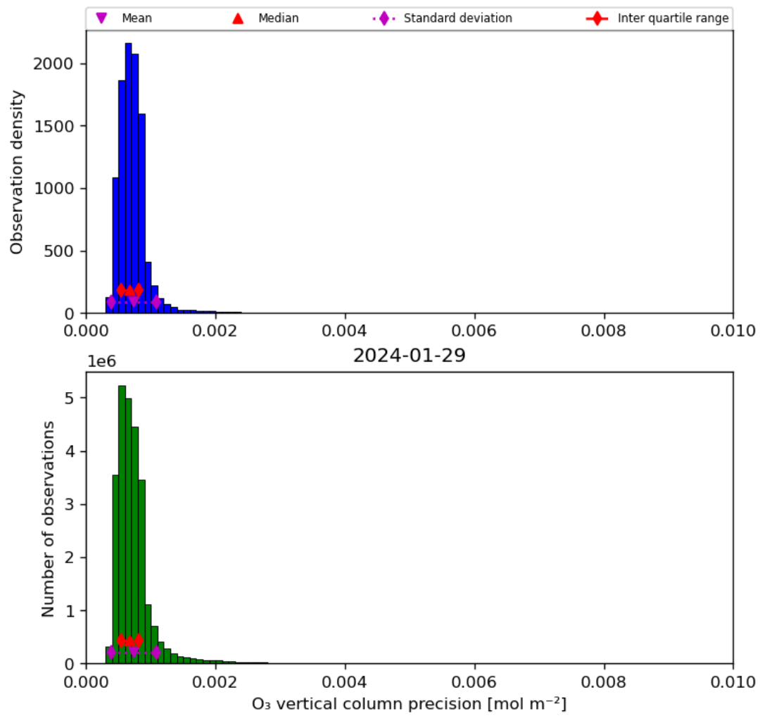
Figure 22: Histogram of “O 3 vertical column precision” for 2024-01-28 to 2024-01-30
