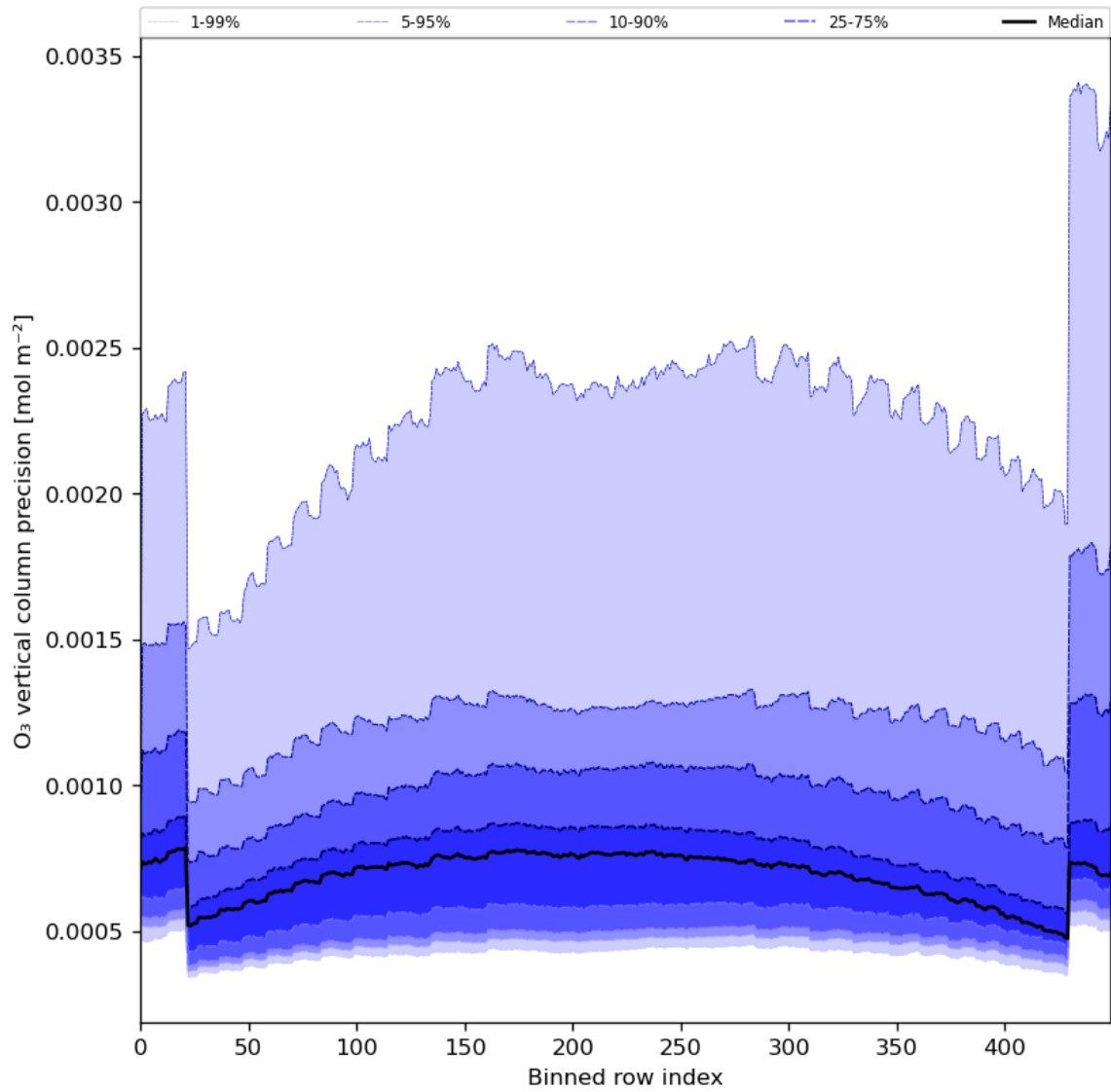
Figure 29: Along track statistics of “O 3 vertical column precision” for 2024-01-28 to 2024-01-30
