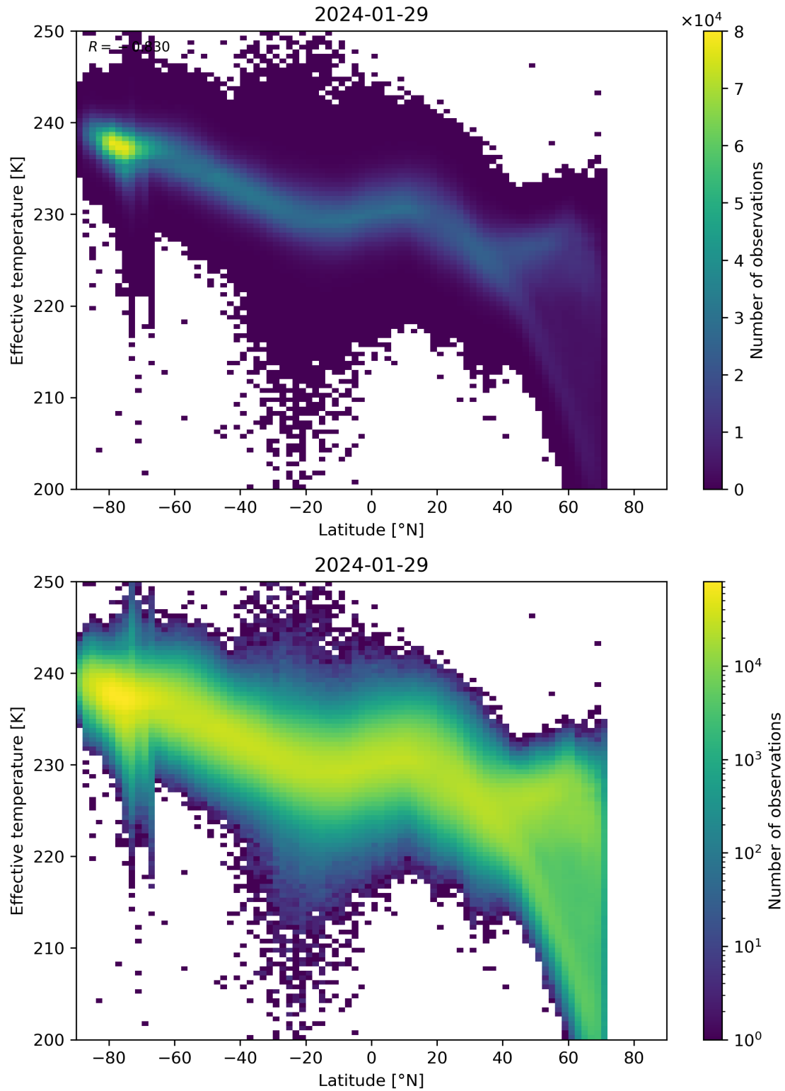
Figure 34: Scatter density plot of “Latitude” against “Effective temperature” for 2024-01-28 to 2024-01-30.
