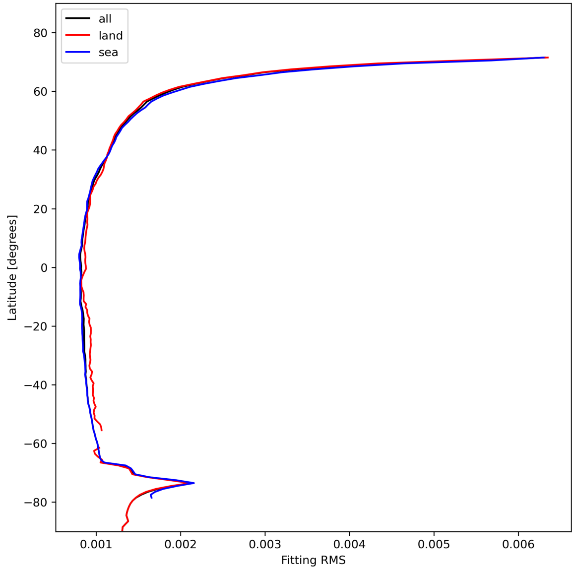
Figure 16: Zonal average of “Fitting RMS” for 2024-01-28 to 2024-01-30.
