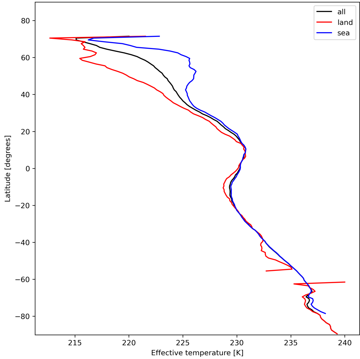
Figure 17: Zonal average of "Effective temperature" for 2024-01-28 to 2024-01-30.
