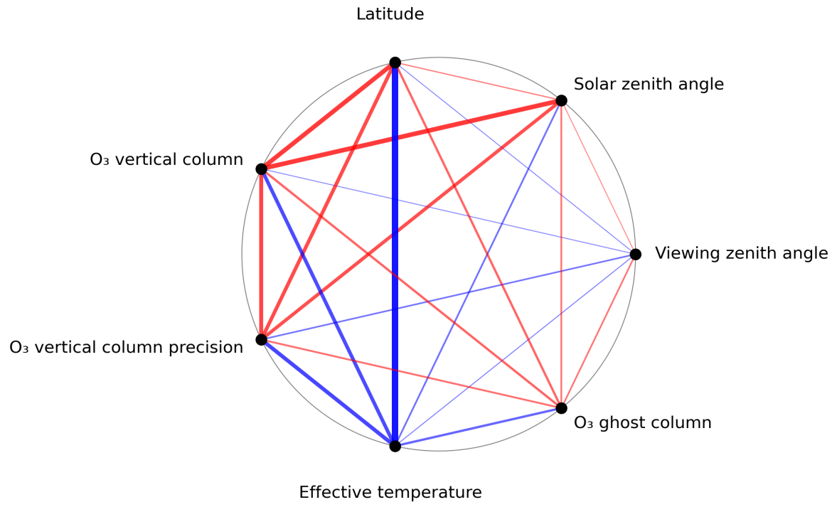
Figure 1: Map of correlation graph for 2024-01-28 to 2024-01-30.
