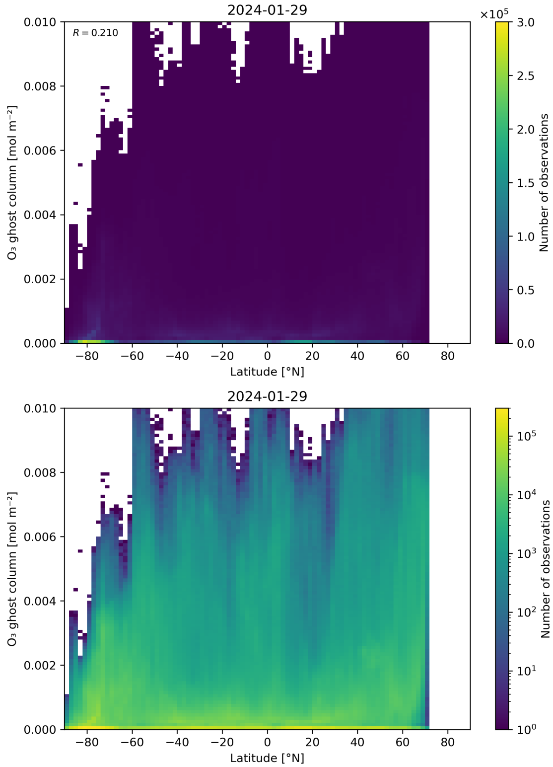
Figure 35: Scatter density plot of “Latitude” against “O 3 ghost column” for 2024-01-28 to 2024-01-30.
