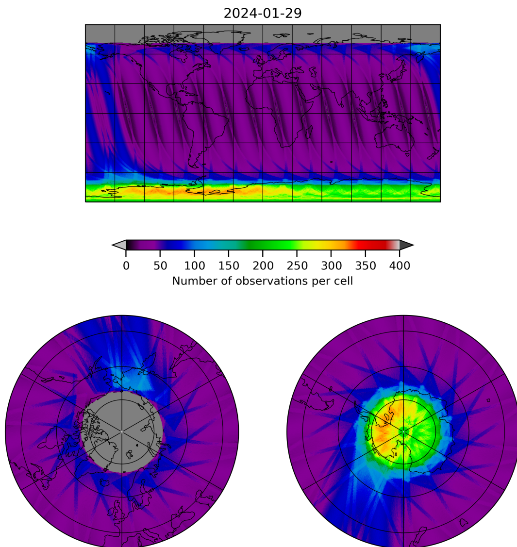
Figure 12: Map of the number of observations for 2024-01-28 to 2024-01-30
