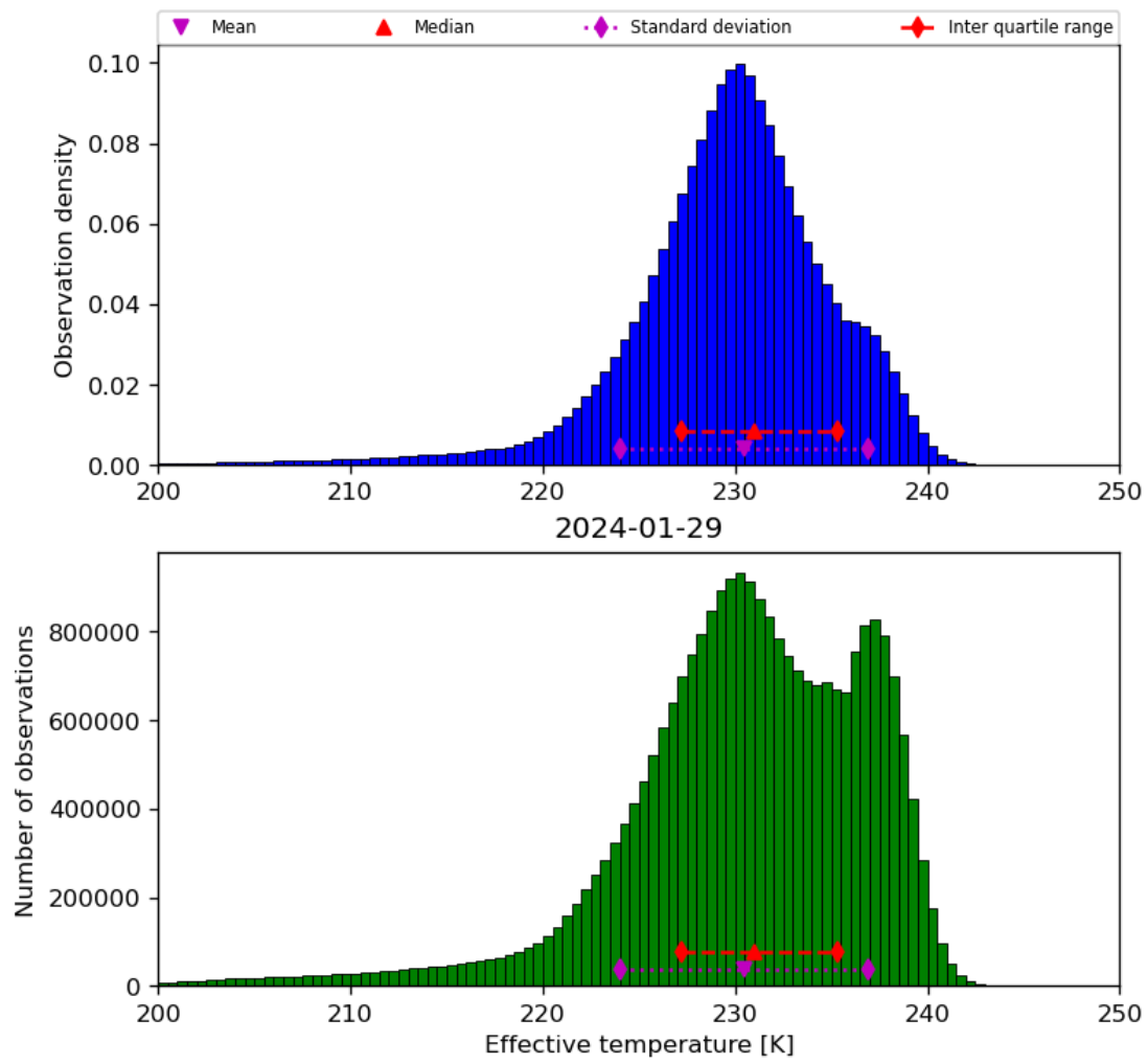
Figure 24: Histogram of “Effective temperature” for 2024-01-28 to 2024-01-30
