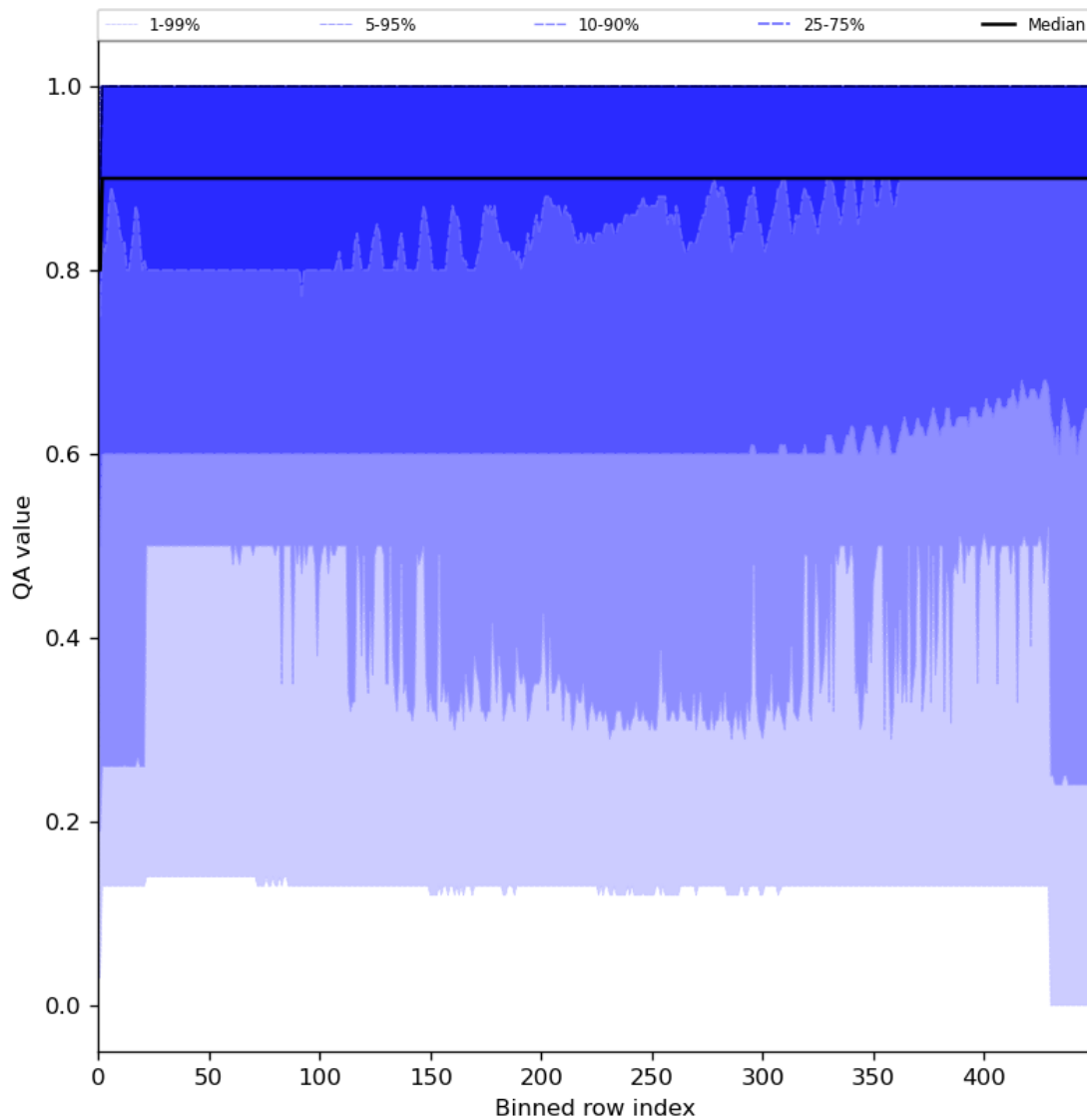
Figure 27: Along track statistics of “QA value” for 2024-01-28 to 2024-01-30
