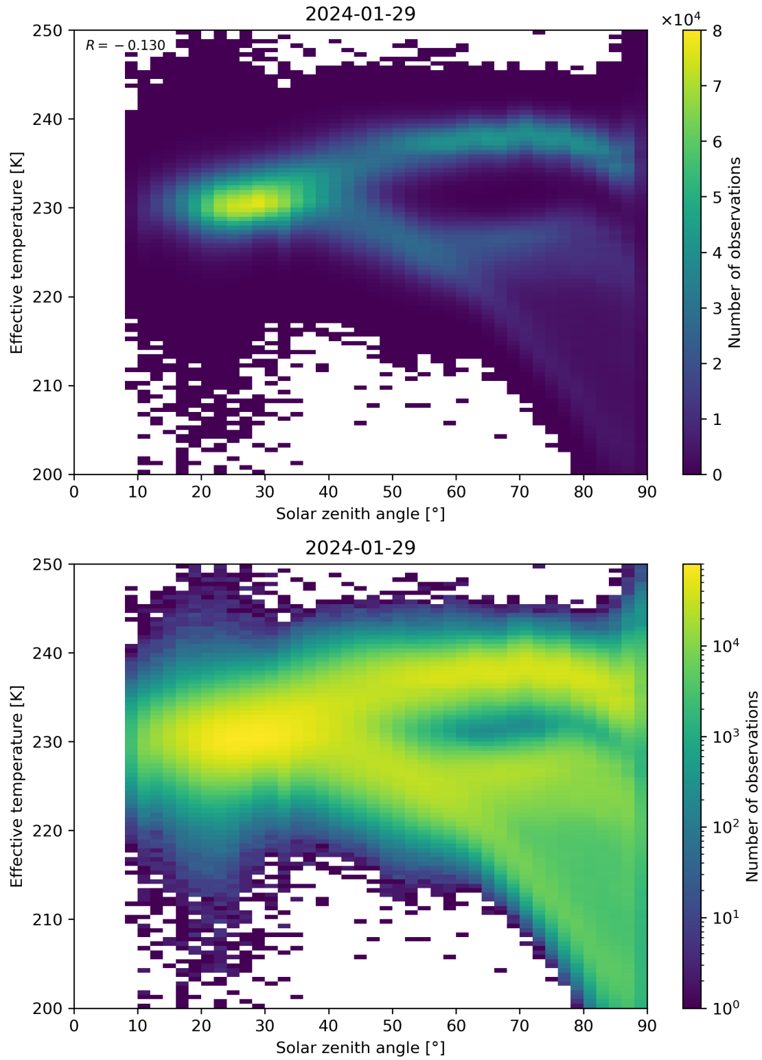
Figure 45: Scatter density plot of “Solar zenith angle” against “Effective temperature” for 2024-01-28 to 2024-01-30.
