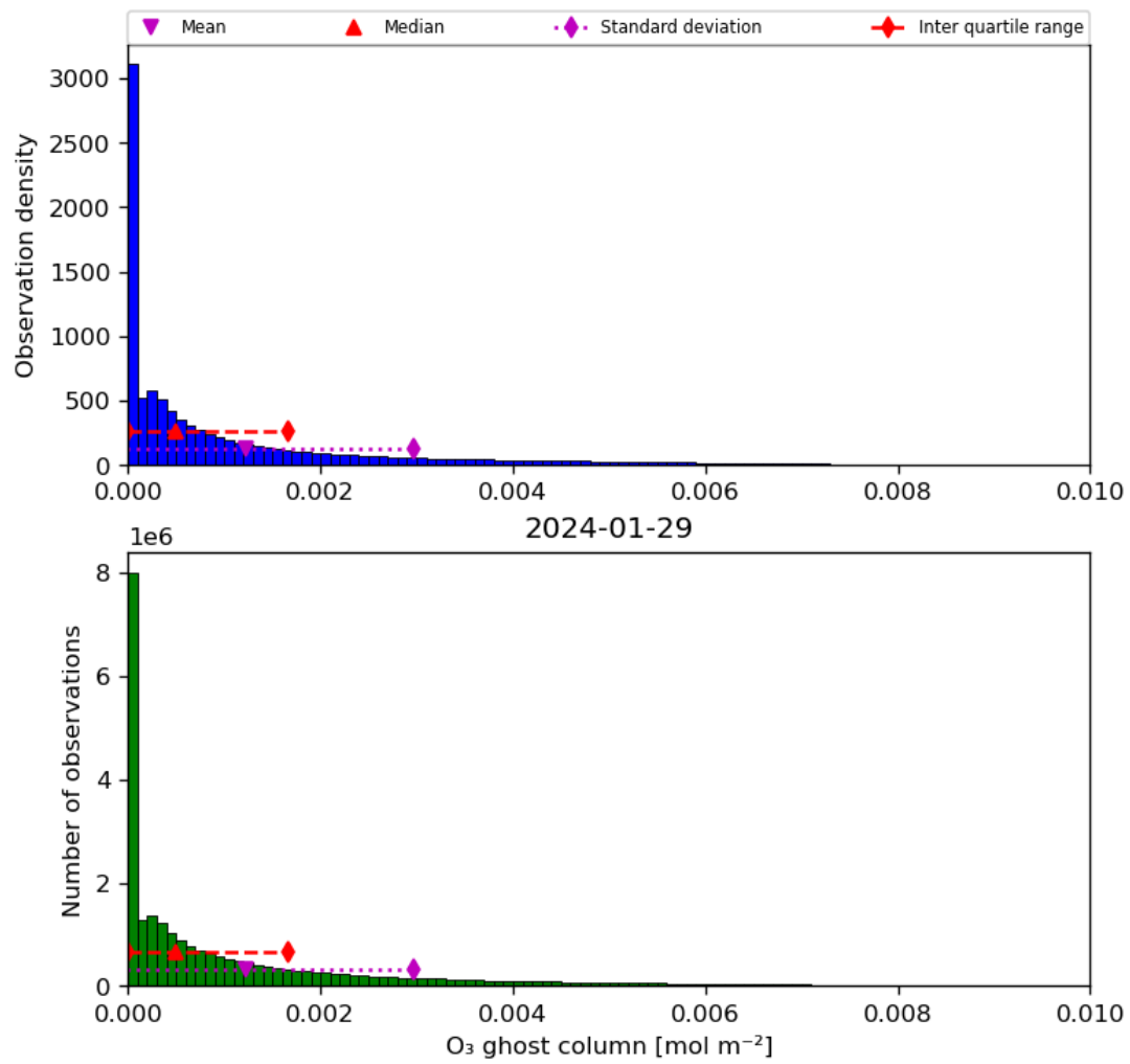
Figure 25: Histogram of “O 3 ghost column” for 2024-01-28 to 2024-01-30
