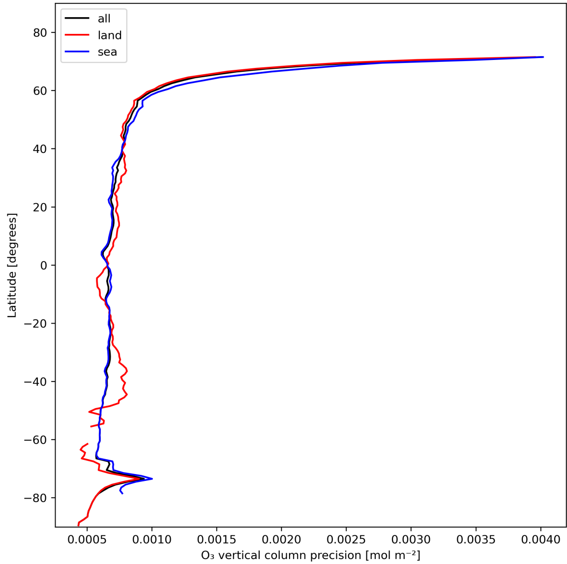
Figure 15: Zonal average of “O 3 vertical column precision” for 2024-01-28 to 2024-01-30.
