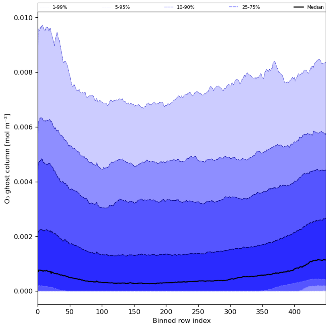
Figure 32: Along track statistics of “O 3 ghost column” for 2024-01-28 to 2024-01-30
