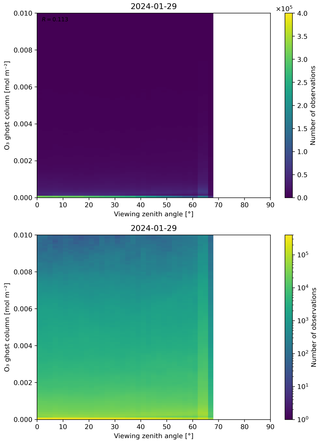
Figure 51: Scatter density plot of “Viewing zenith angle” against “O 3 ghost column” for 2024-01-28 to 2024-01-30.
