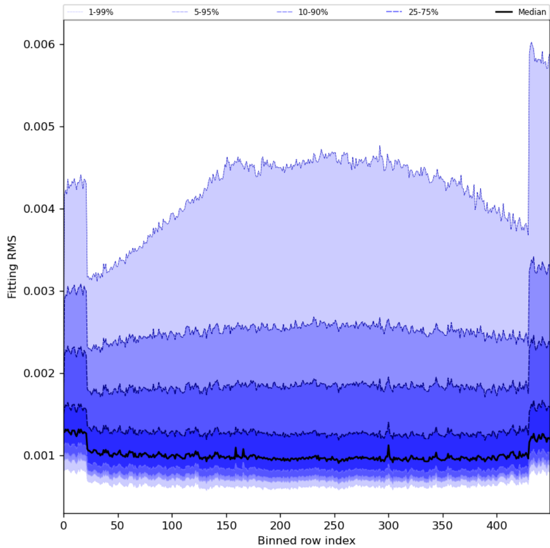
Figure 30: Along track statistics of “Fitting RMS” for 2024-01-28 to 2024-01-30
