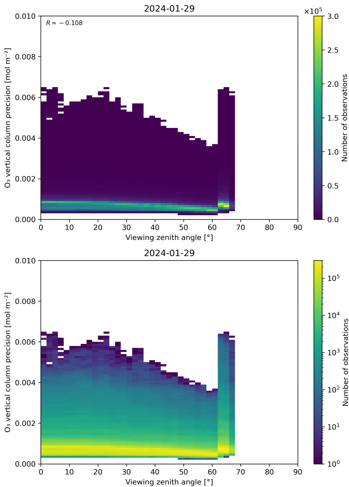
Figure 53: Scatter density plot of “Viewing zenith angle” against “O 3 vertical column precision” for 2024-01-28 to 2024-01-30.
