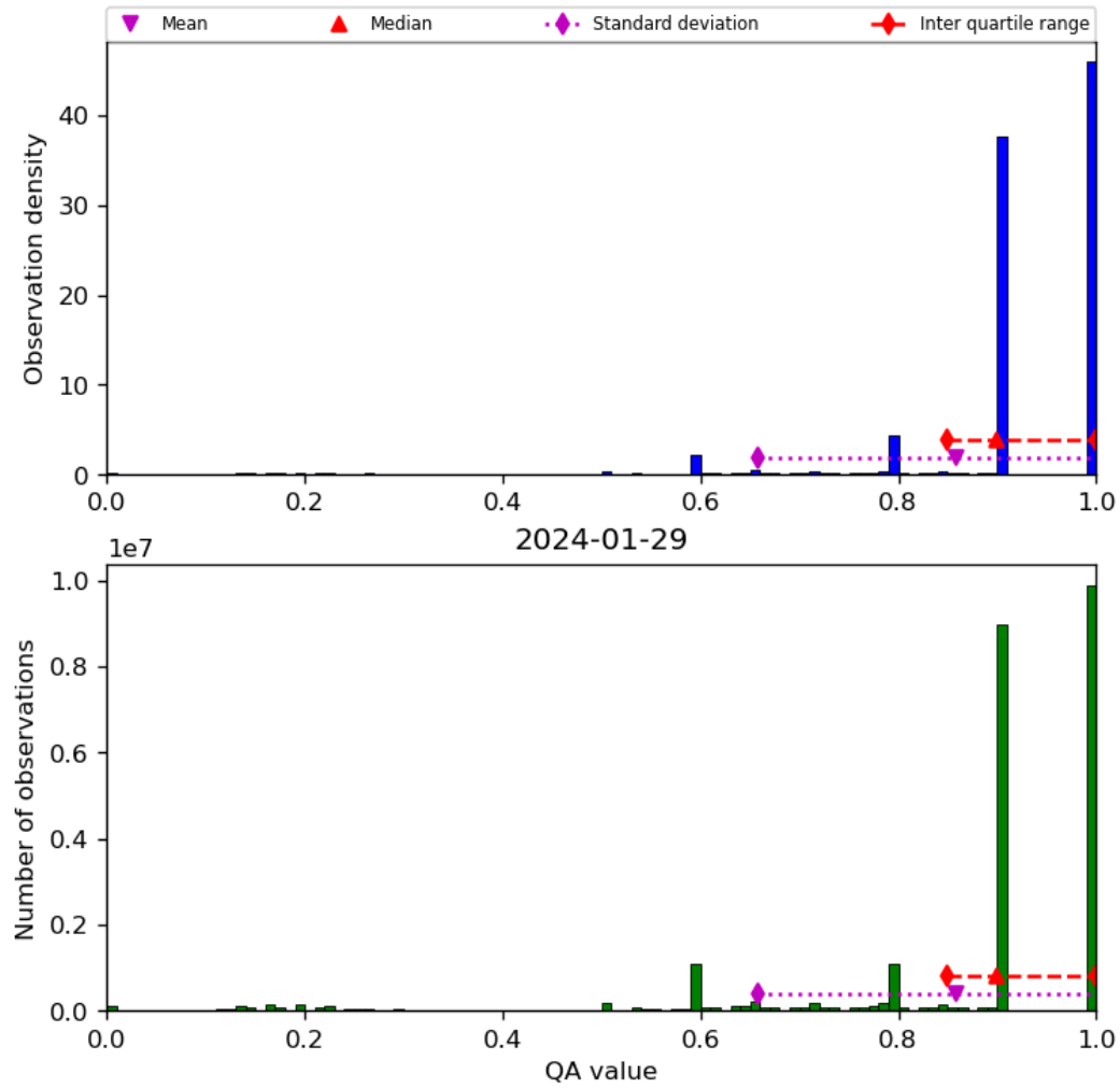
Figure 20: Histogram of “QA value” for 2024-01-28 to 2024-01-30
