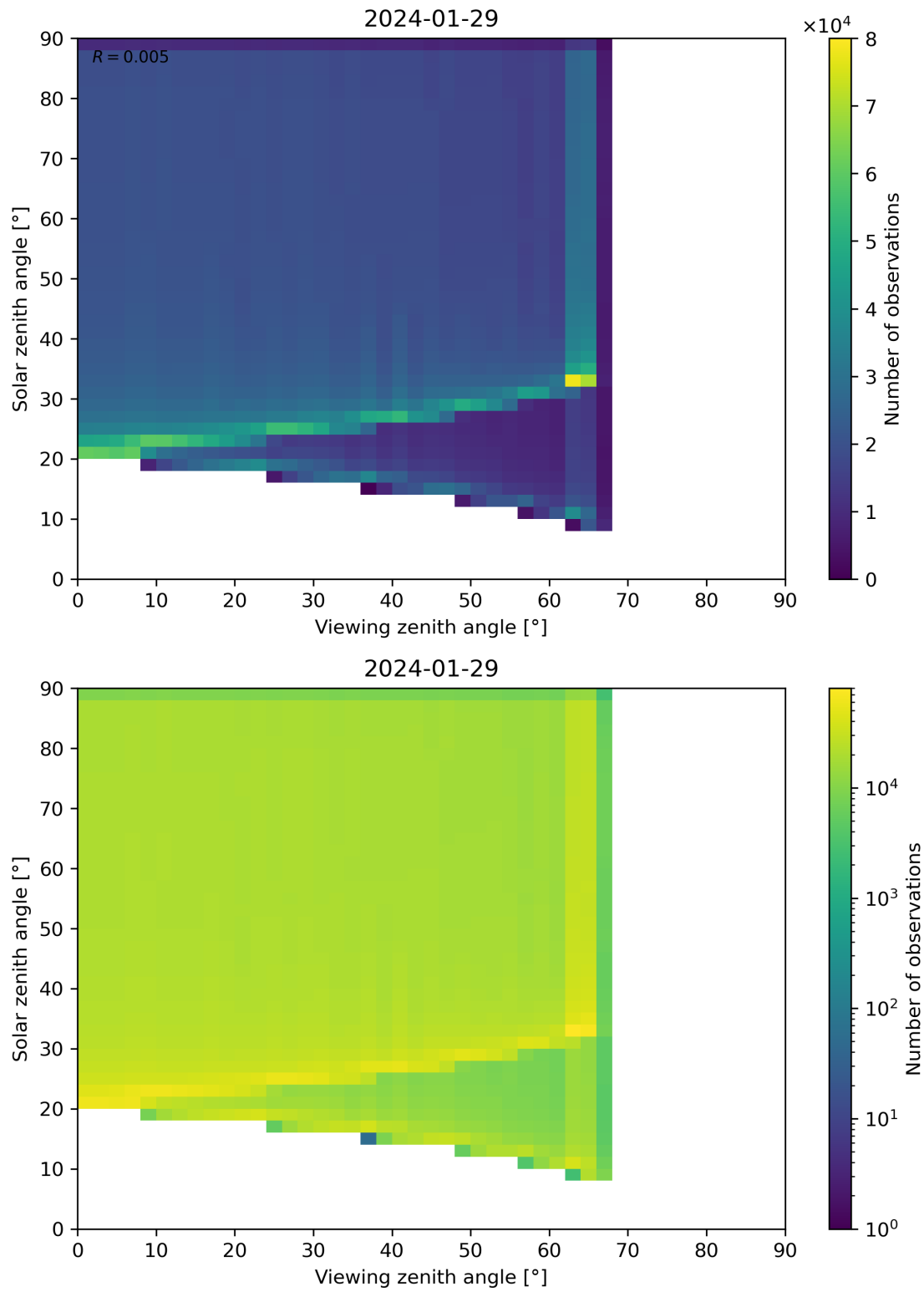
Figure 54: Scatter density plot of “Viewing zenith angle” against “Solar zenith angle” for 2024-01-28 to 2024-01-30.
