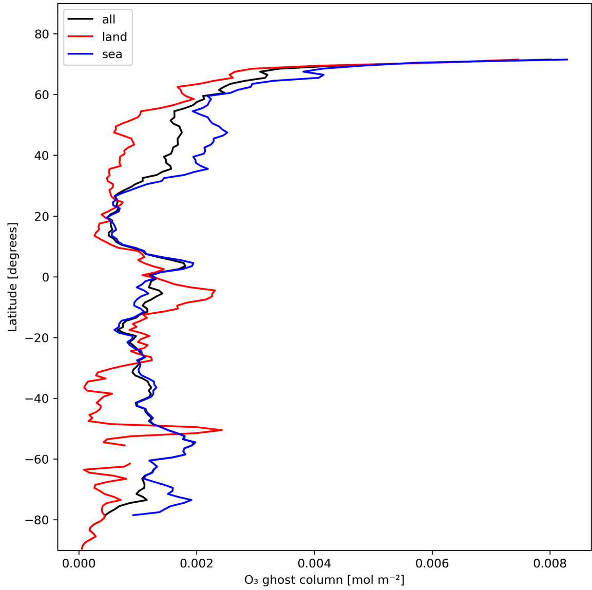
Figure 18: Zonal average of "O 3 ghost column" for 2024-01-28 to 2024-01-30.
