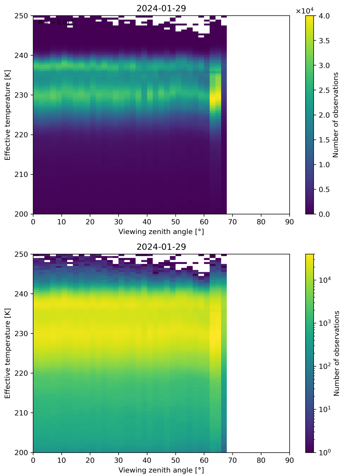
Figure 50: Scatter density plot of “Viewing zenith angle” against “Effective temperature” for 2024-01-28 to 2024-01-30.
