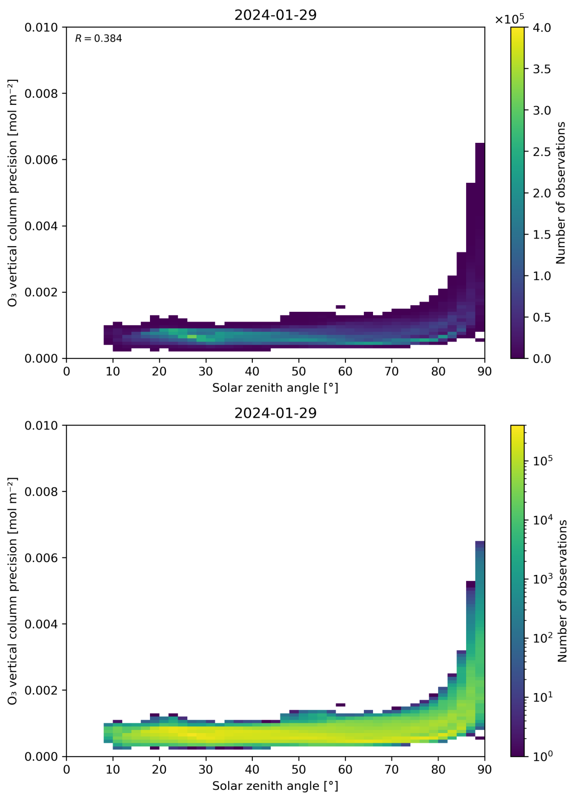
Figure 48: Scatter density plot of “Solar zenith angle” against “O 3 vertical column precision” for 2024-01-28 to 2024-01-30.
