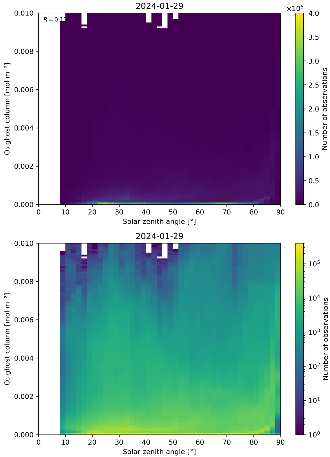
Figure 46: Scatter density plot of “Solar zenith angle” against “O 3 ghost column” for 2024-01-28 to 2024-01-30.
