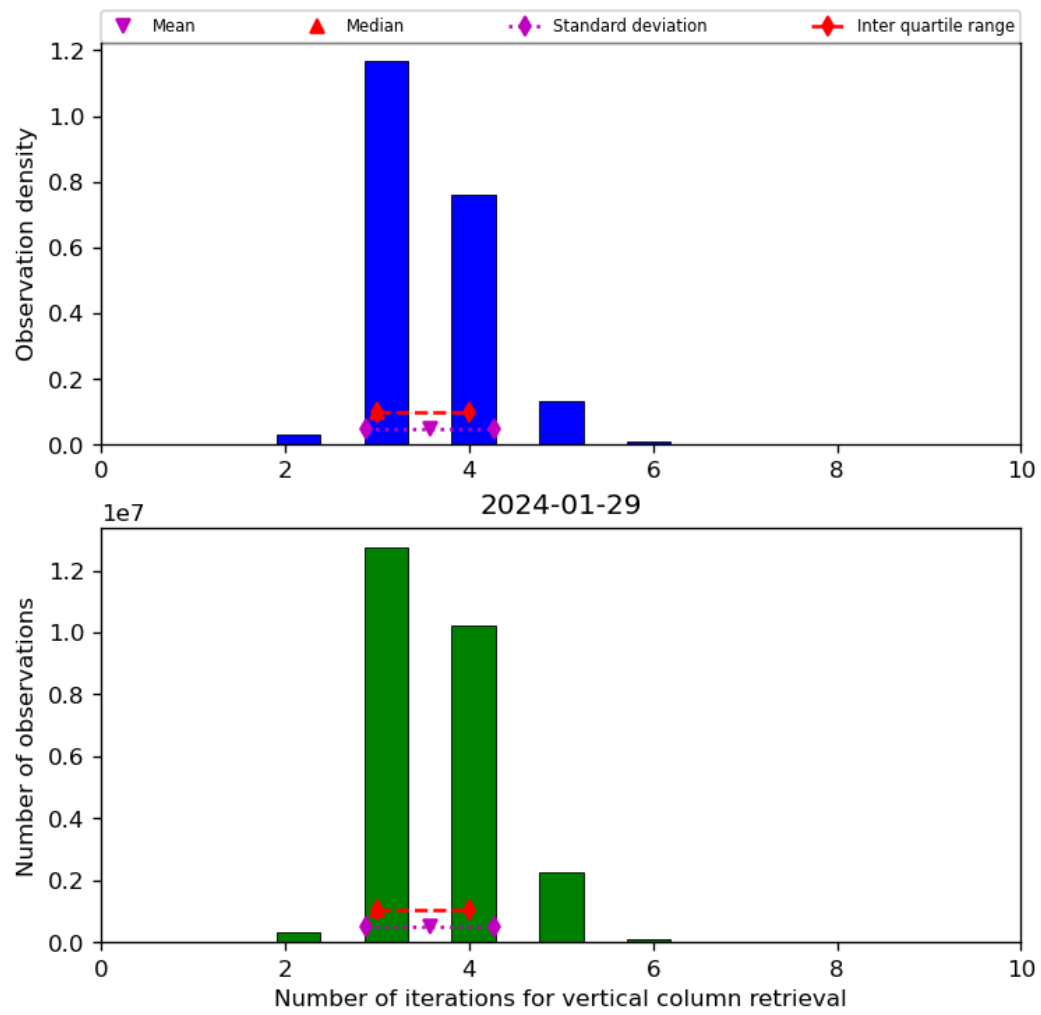
Figure 26: Histogram of “Number of iterations for vertical column retrieval” for 2024-01-28 to 2024-01-30
