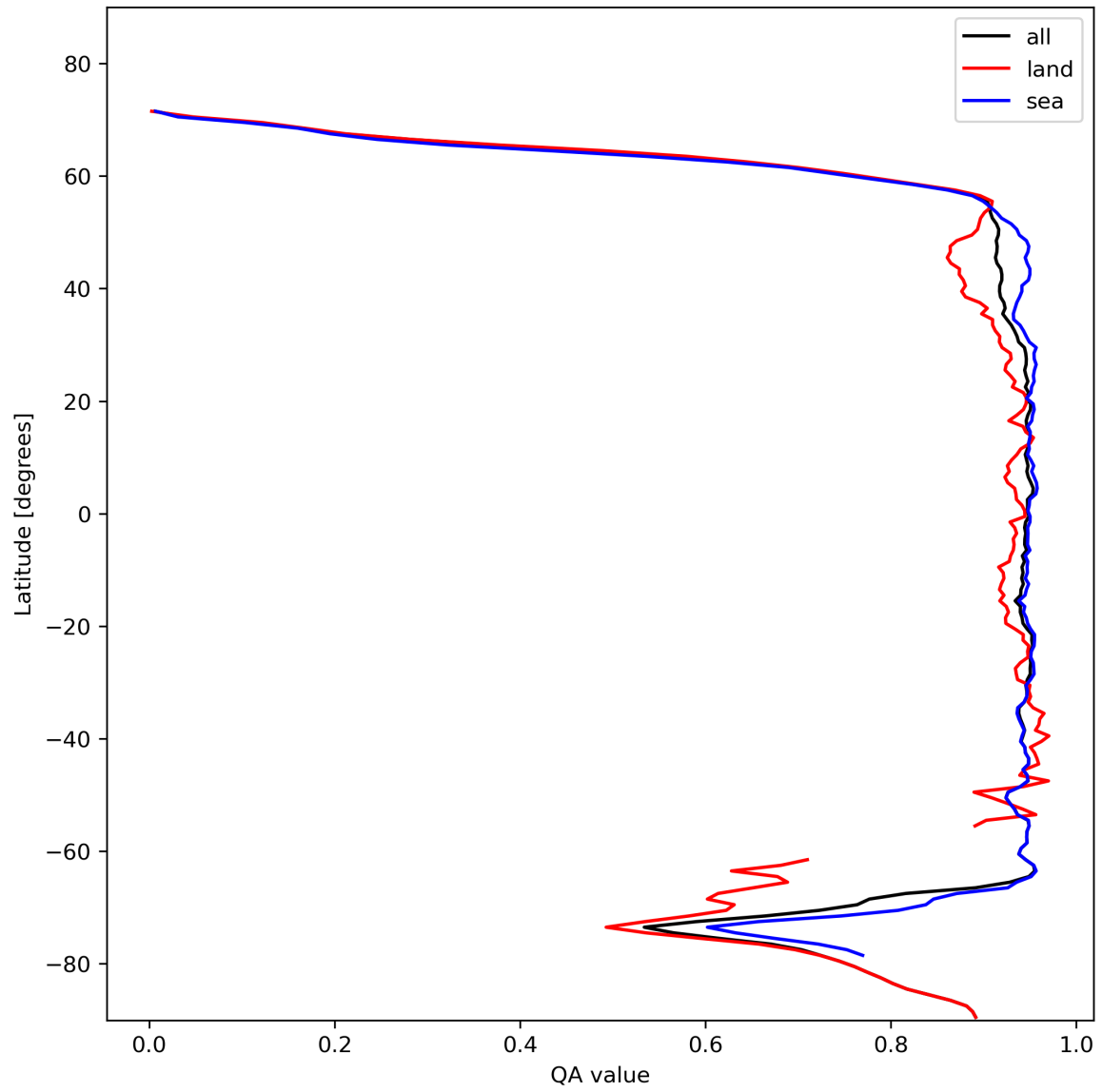
Figure 13: Zonal average of “QA value” for 2024-01-28 to 2024-01-30.
