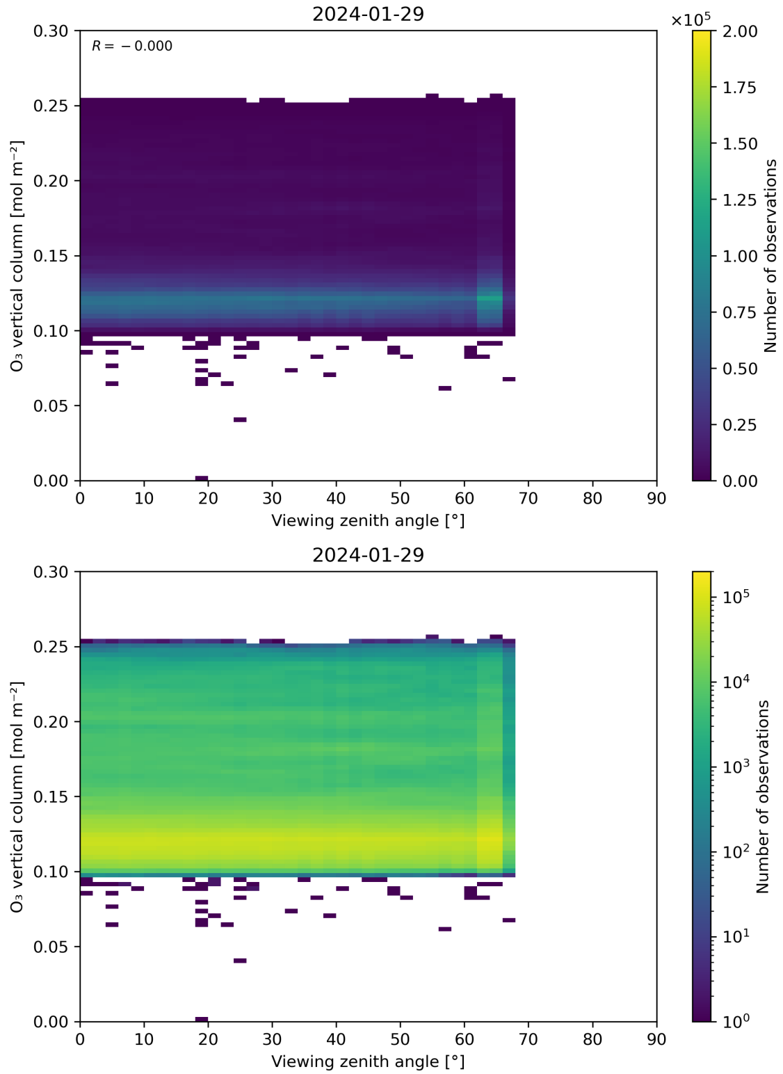
Figure 52: Scatter density plot of “Viewing zenith angle” against “O 3 vertical column” for 2024-01-28 to 2024-01-30.
