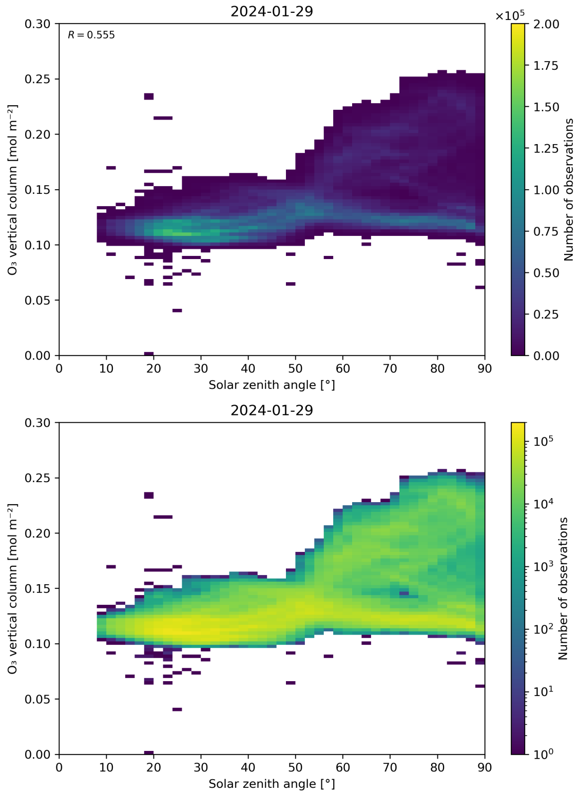
Figure 47: Scatter density plot of “Solar zenith angle” against “O 3 vertical column” for 2024-01-28 to 2024-01-30.
