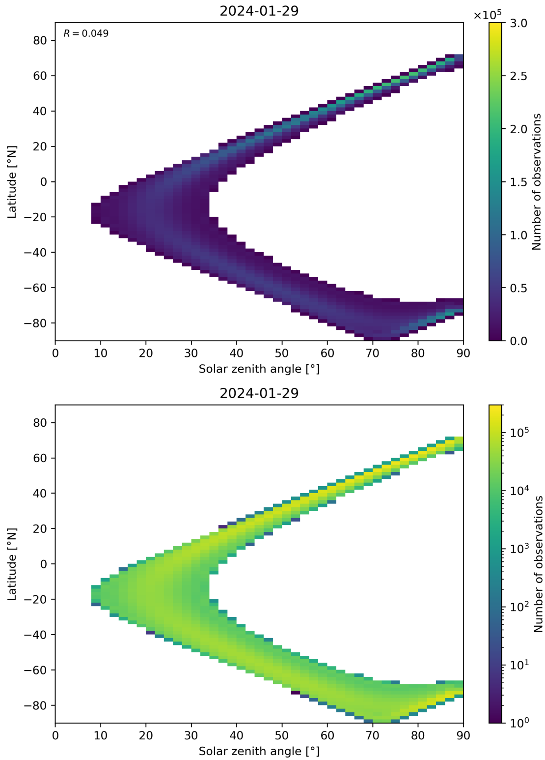
Figure 44: Scatter density plot of “Solar zenith angle” against “Latitude” for 2024-01-28 to 2024-01-30.
