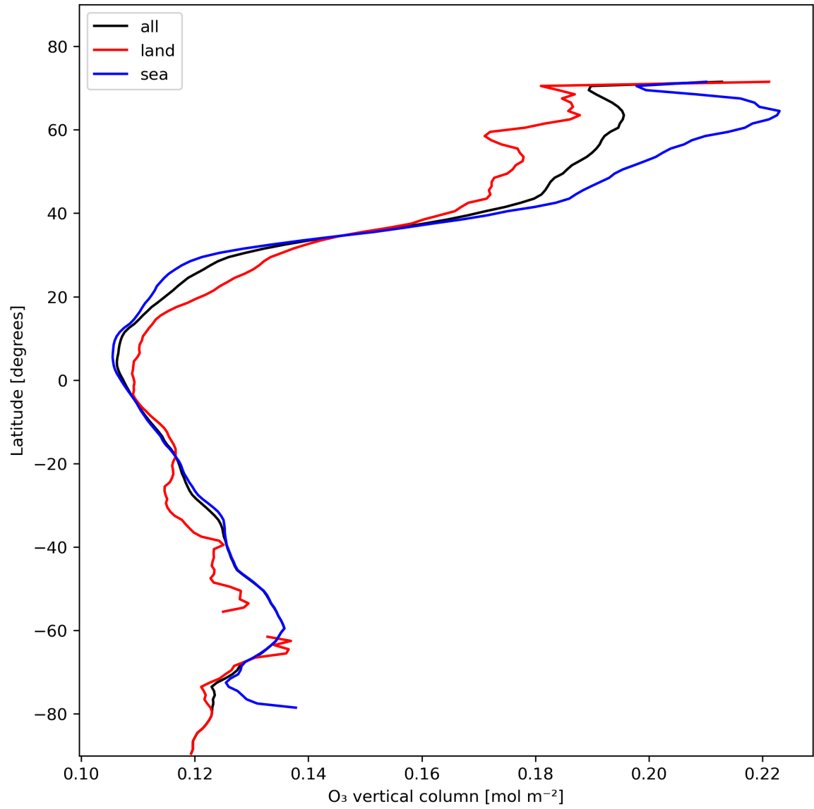
Figure 14: Zonal average of “O 3 vertical column” for 2024-01-28 to 2024-01-30.
