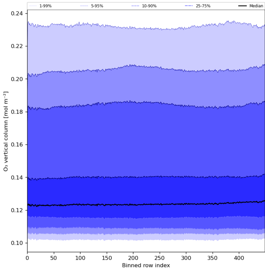
Figure 28: Along track statistics of “O 3 vertical column” for 2024-01-28 to 2024-01-30
