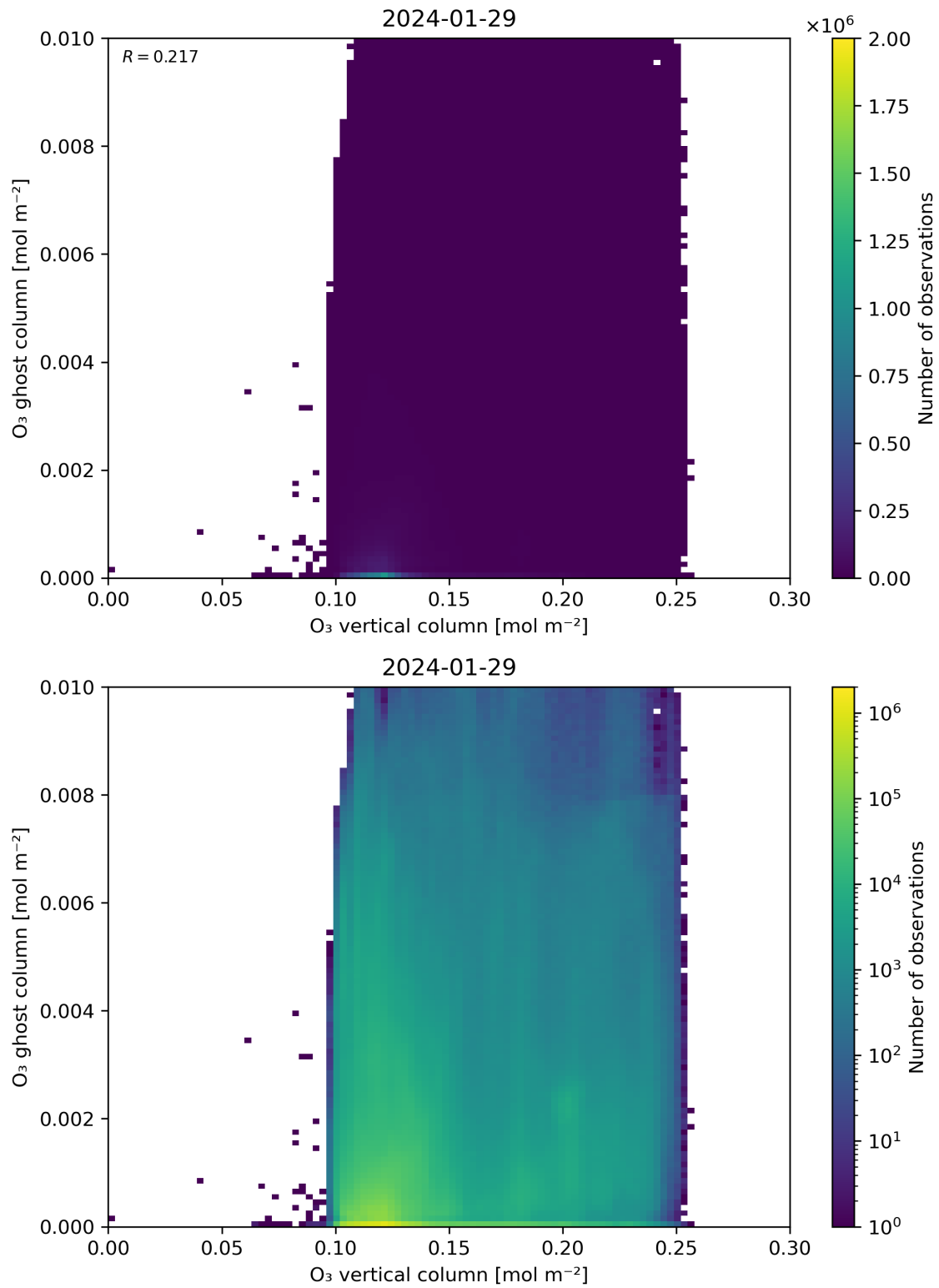
Figure 40: Scatter density plot of “O 3 vertical column” against “O 3 ghost column” for 2024-01-28 to 2024-01-30.
