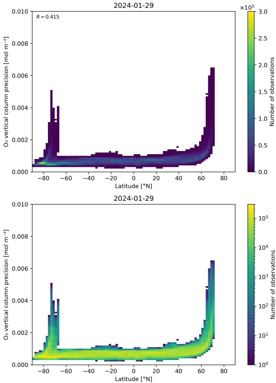
Figure 37: Scatter density plot of “Latitude” against “O 3 vertical column precision” for 2024-01-28 to 2024-01-30.
