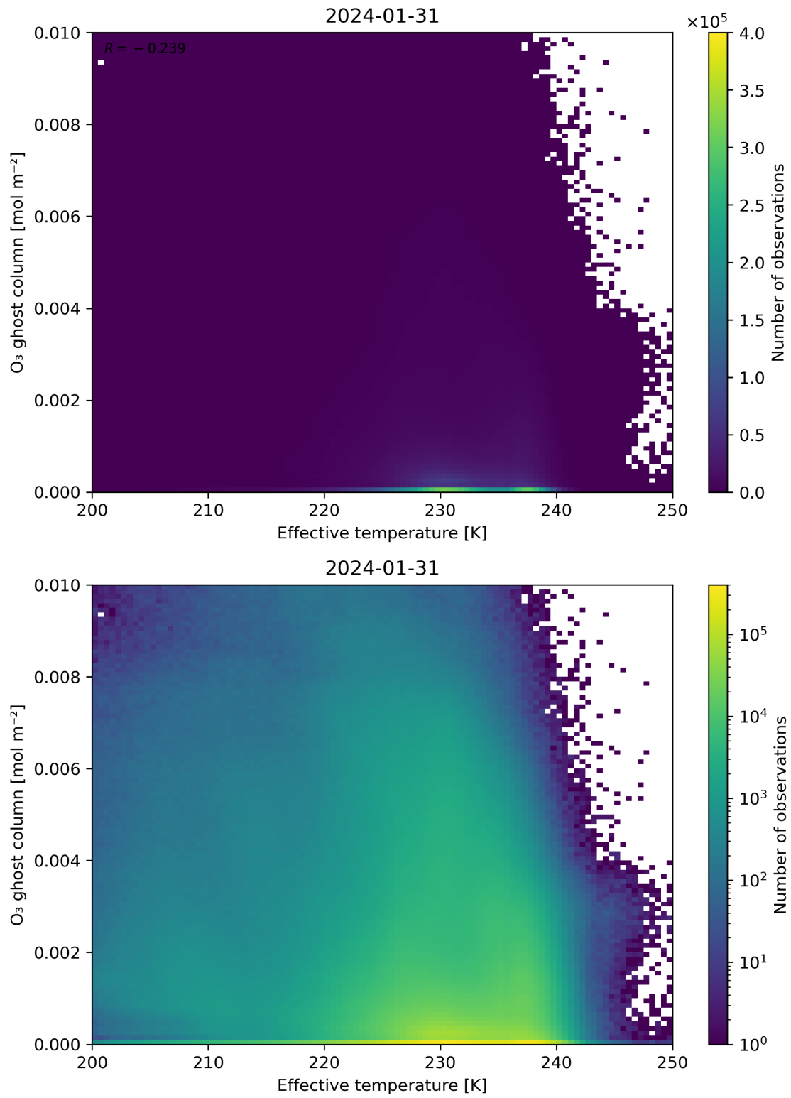
Figure 38: Scatter density plot of “Effective temperature” against “O 3 ghost column” for 2024-01-31 to 2024-02-01.
