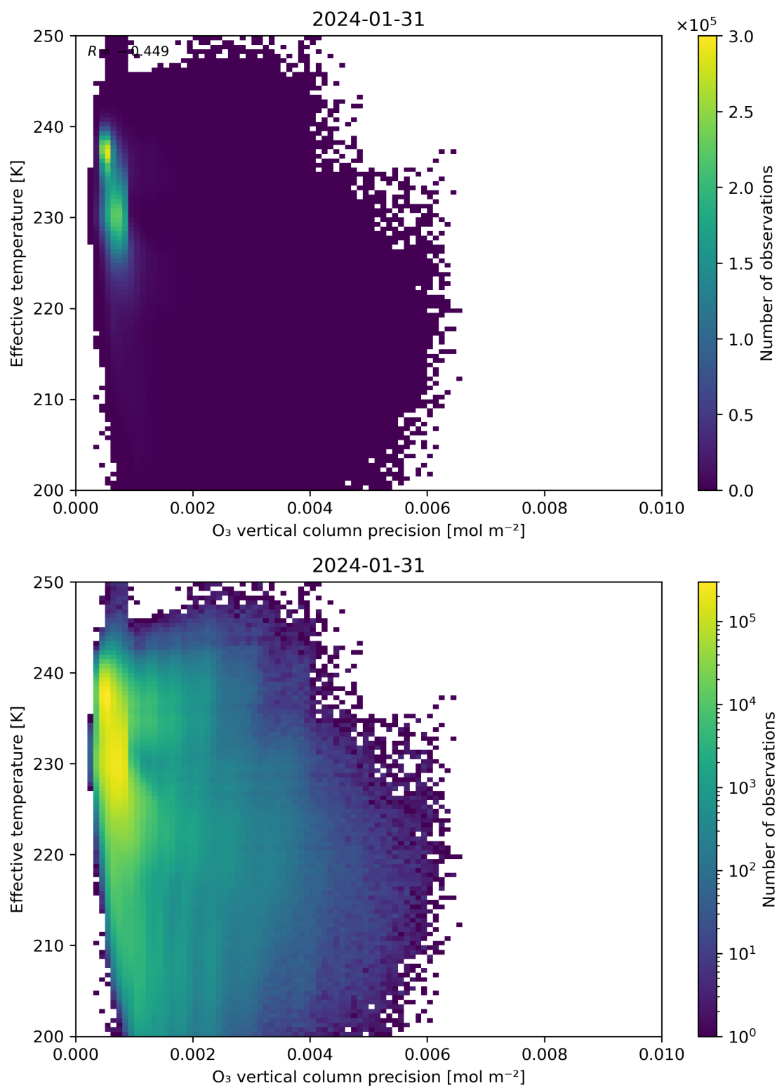
Figure 42: Scatter density plot of “O 3 vertical column precision” against “Effective temperature” for 2024-01-31 to 2024-02-01.
