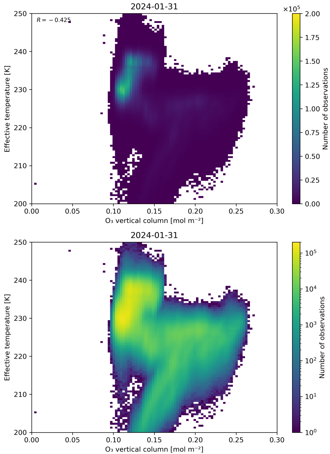
Figure 39: Scatter density plot of “O 3 vertical column” against “Effective temperature” for 2024-01-31 to 2024-02-01.
