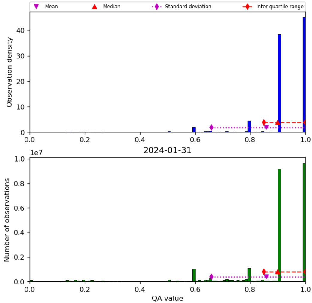
Figure 20: Histogram of “QA value” for 2024-01-31 to 2024-02-01
