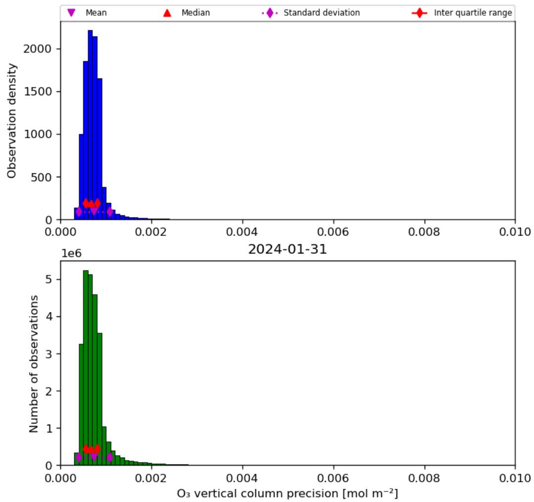
Figure 22: Histogram of “O 3 vertical column precision” for 2024-01-31 to 2024-02-01
