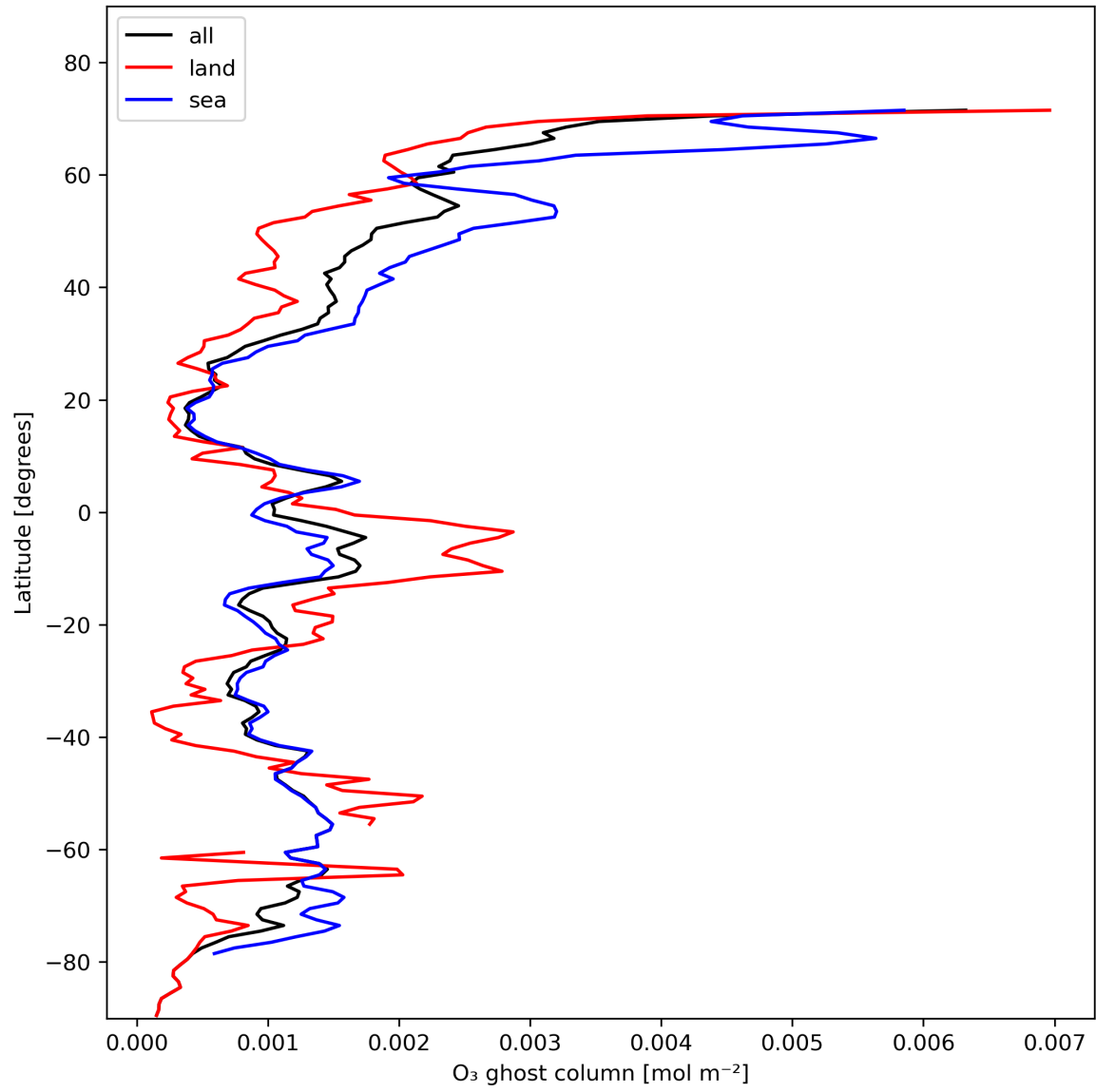
Figure 18: Zonal average of "O 3 ghost column" for 2024-01-31 to 2024-02-01.
