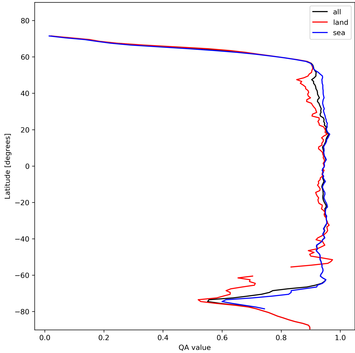
Figure 13: Zonal average of “QA value” for 2024-01-31 to 2024-02-01.
