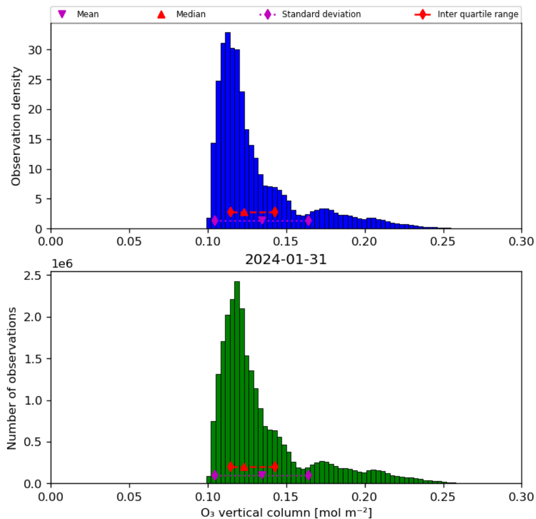
Figure 21: Histogram of “O 3 vertical column” for 2024-01-31 to 2024-02-01
