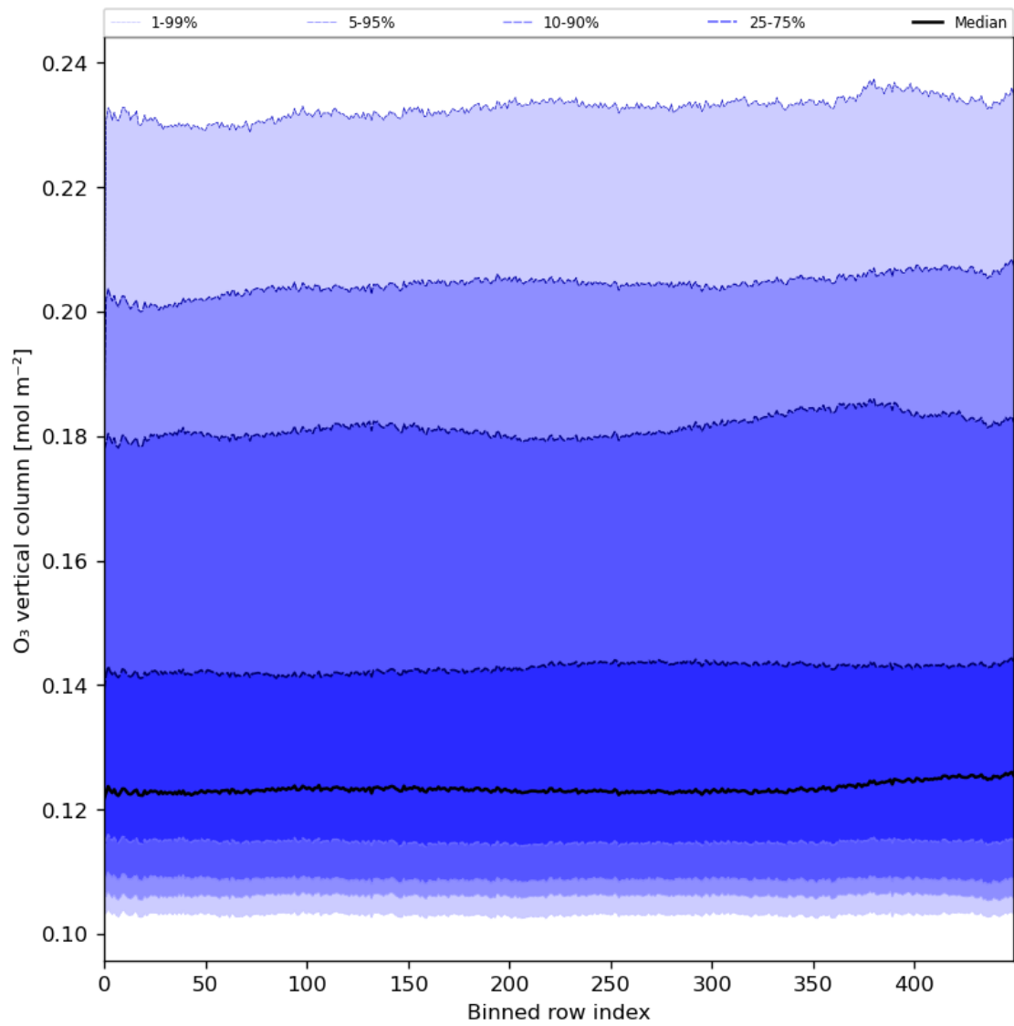
Figure 28: Along track statistics of “O 3 vertical column” for 2024-01-31 to 2024-02-01
