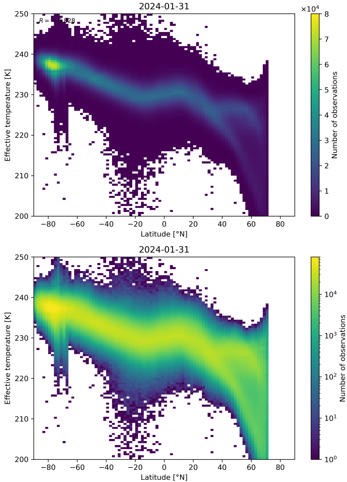
Figure 34: Scatter density plot of “Latitude” against “Effective temperature” for 2024-01-31 to 2024-02-01.
