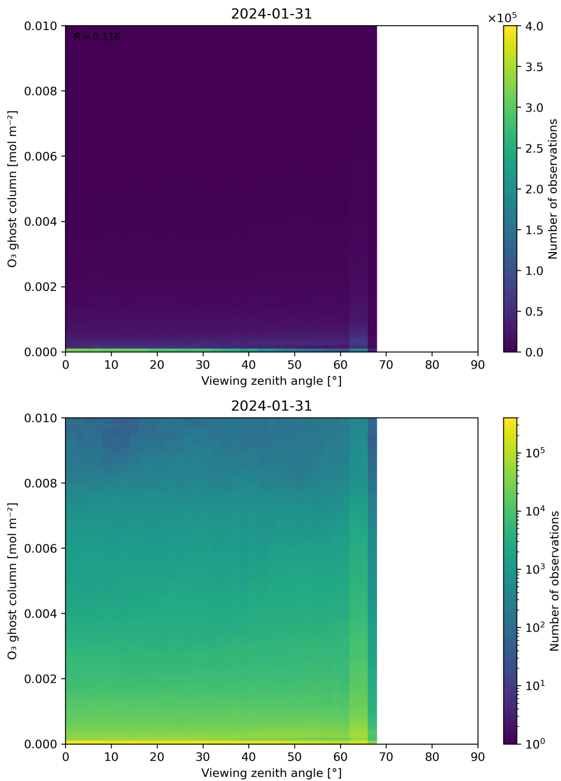
Figure 51: Scatter density plot of “Viewing zenith angle” against “O 3 ghost column” for 2024-01-31 to 2024-02-01.
