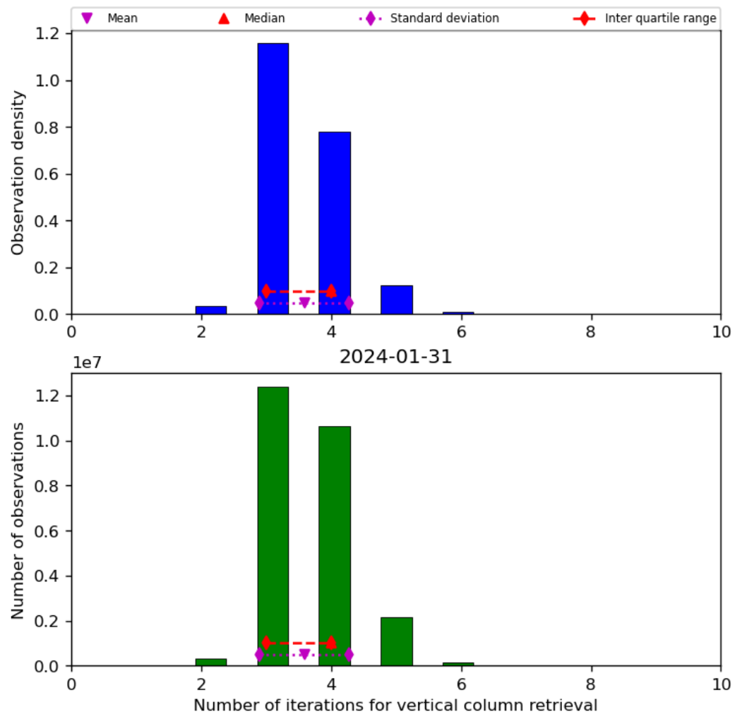
Figure 26: Histogram of “Number of iterations for vertical column retrieval” for 2024-01-31 to 2024-02-01
