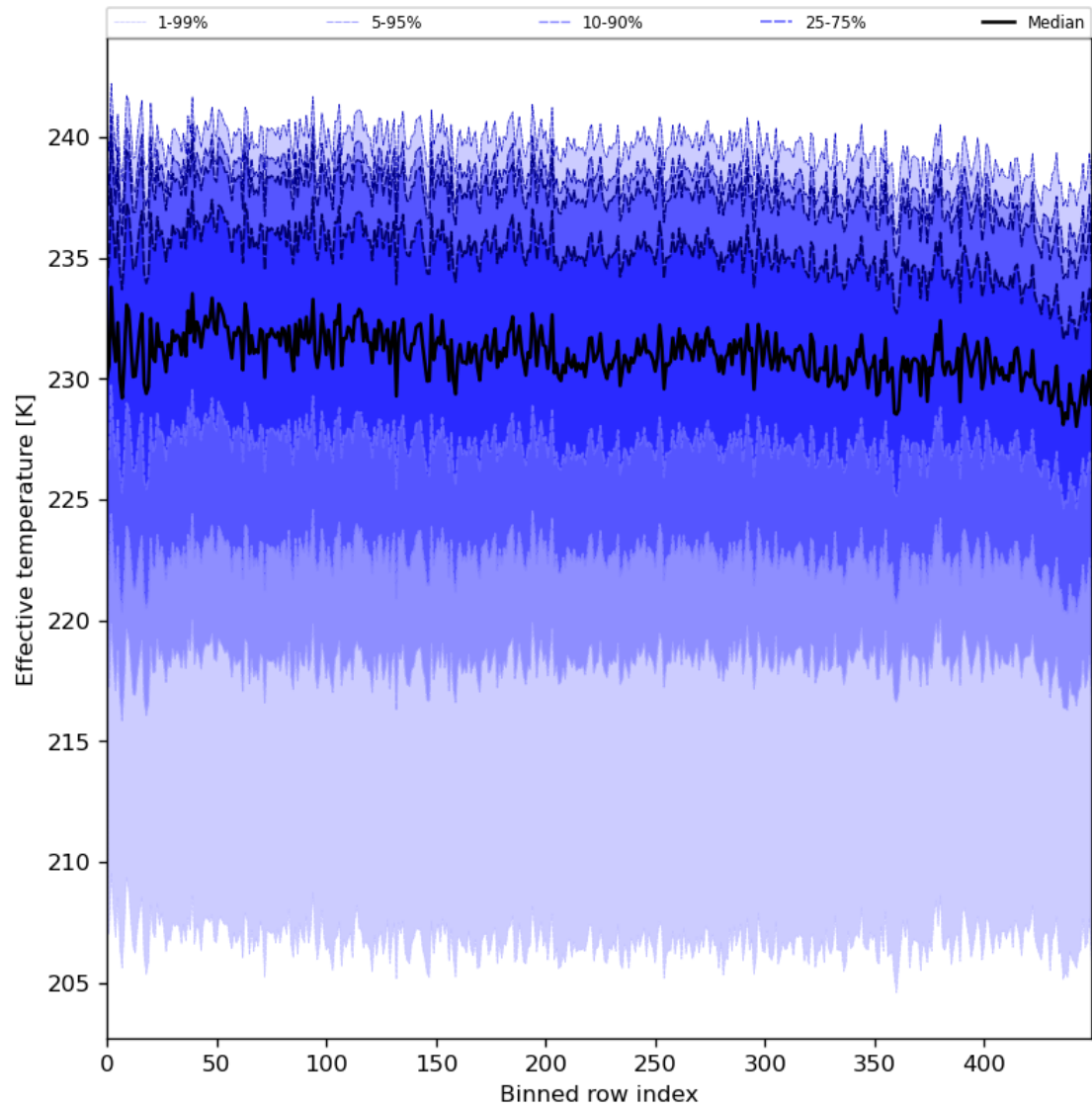
Figure 31: Along track statistics of “Effective temperature” for 2024-01-31 to 2024-02-01
