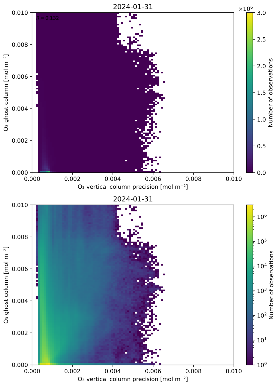
Figure 43: Scatter density plot of “O 3 vertical column precision” against “O 3 ghost column” for 2024-01-31 to 2024-02-01.
