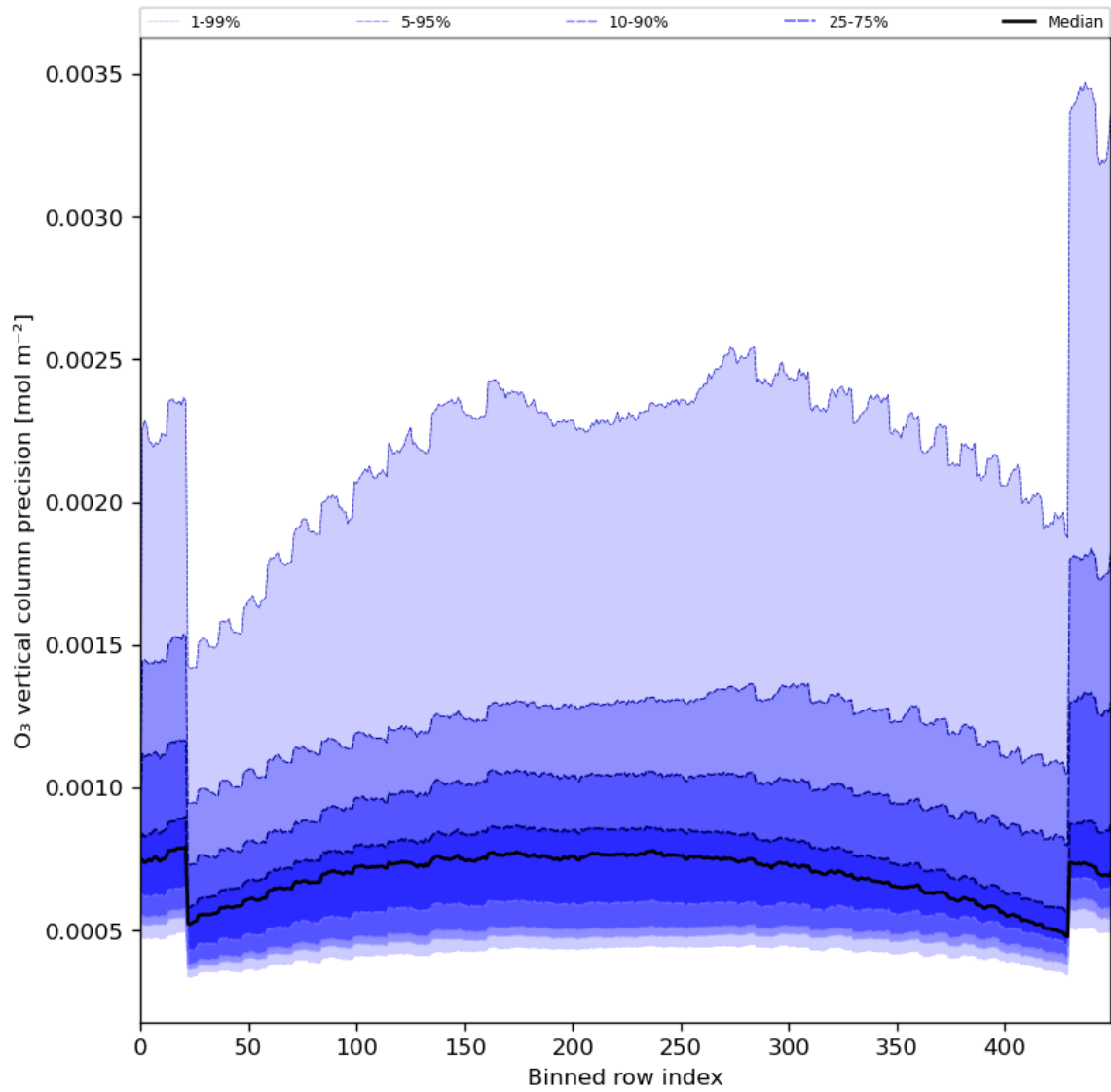
Figure 29: Along track statistics of “O 3 vertical column precision” for 2024-01-31 to 2024-02-01
