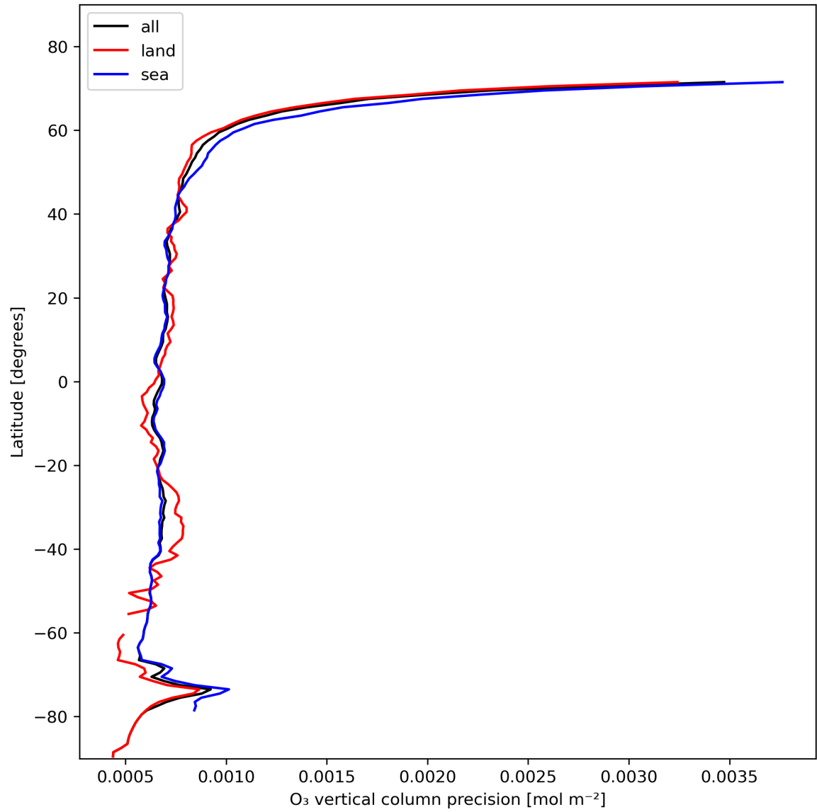
Figure 15: Zonal average of "O 3 vertical column precision" for 2024-01-31 to 2024-02-01.
