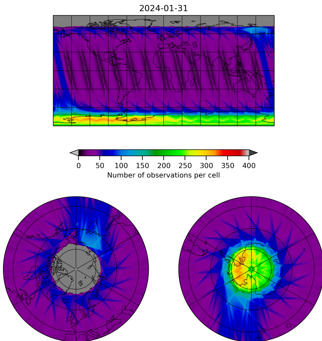
Figure 12: Map of the number of observations for 2024-01-31 to 2024-02-01
