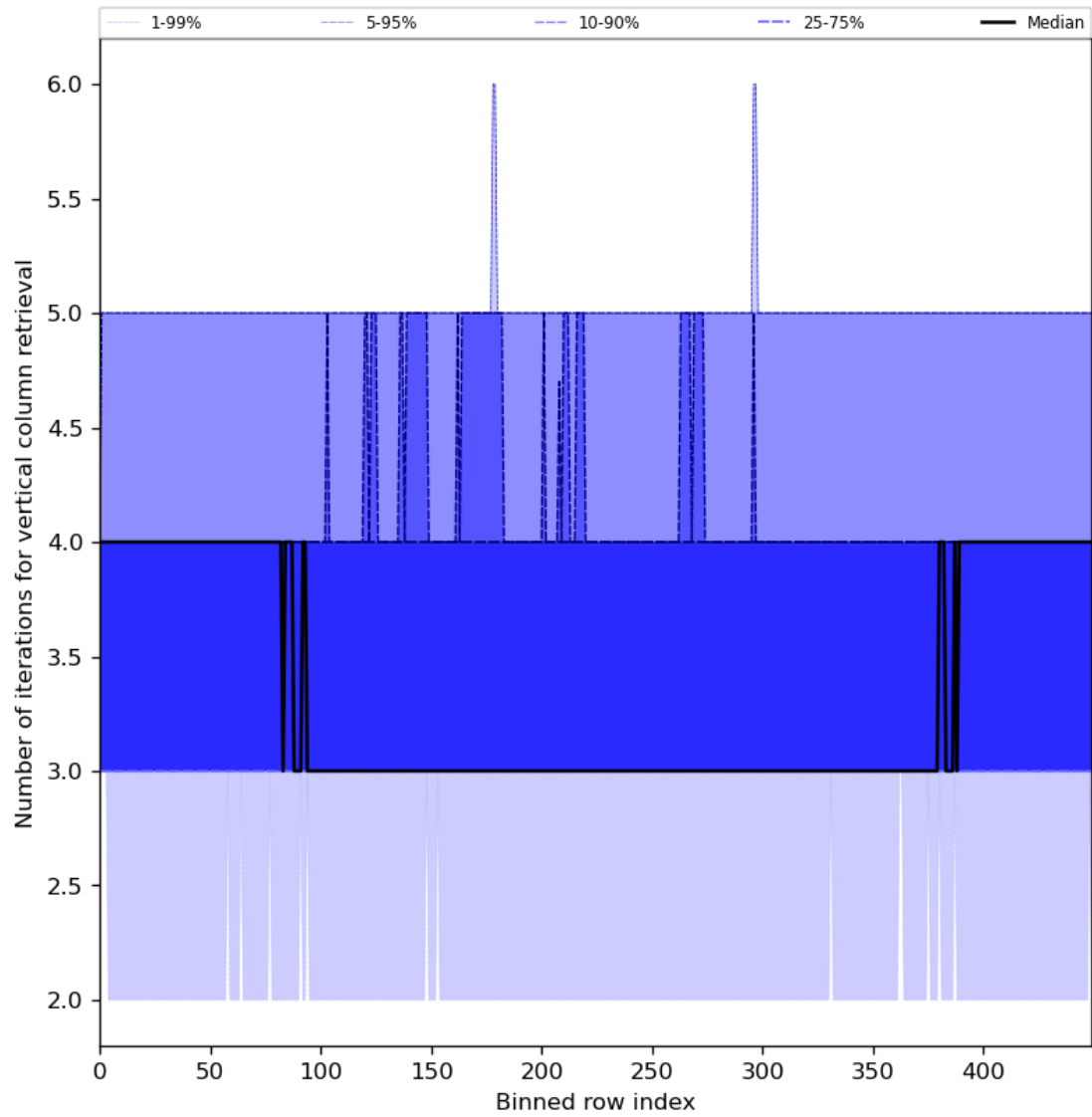
Figure 33: Along track statistics of “Number of iterations for vertical column retrieval” for 2024-01-31 to 2024-02-01
