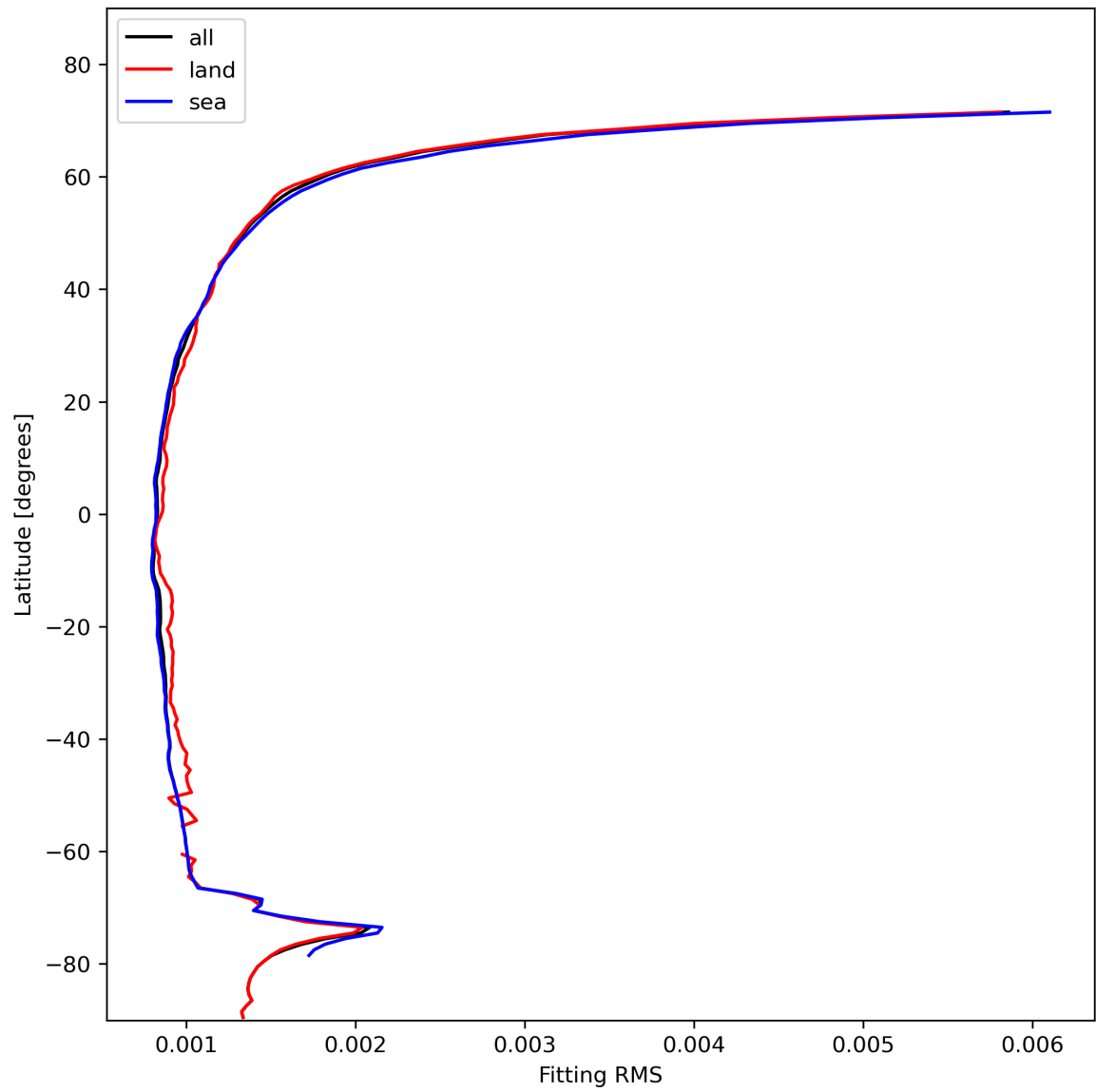
Figure 16: Zonal average of “Fitting RMS” for 2024-01-31 to 2024-02-01.
