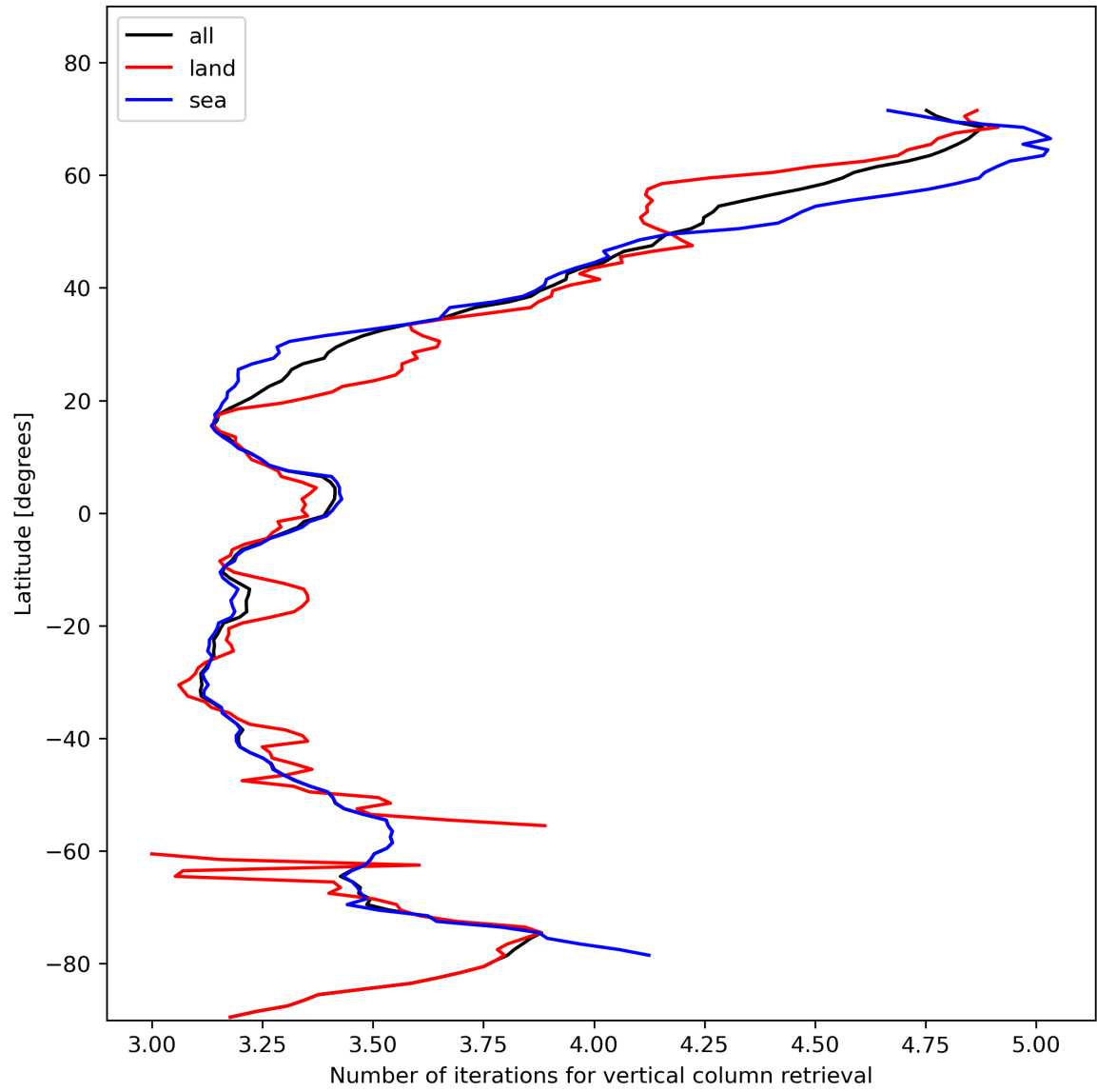
Figure 19: Zonal average of “Number of iterations for vertical column retrieval” for 2024-01-31 to 2024-02-01.
