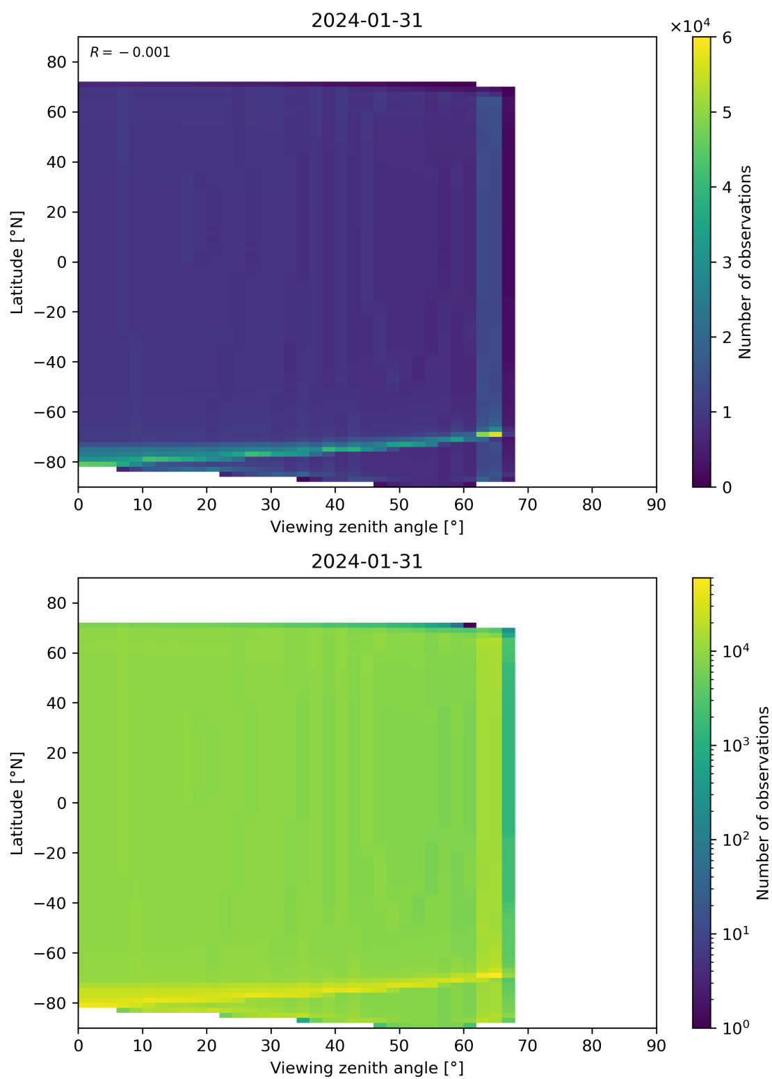
Figure 49: Scatter density plot of “Viewing zenith angle” against “Latitude” for 2024-01-31 to 2024-02-01.
