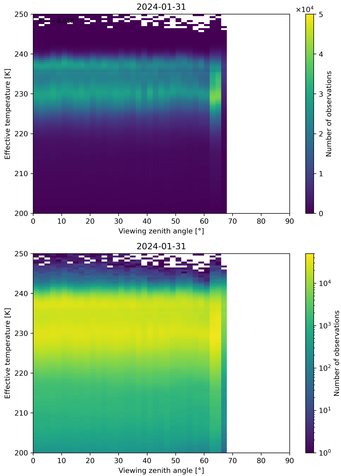
Figure 50: Scatter density plot of “Viewing zenith angle” against “Effective temperature” for 2024-01-31 to 2024-02-01.
