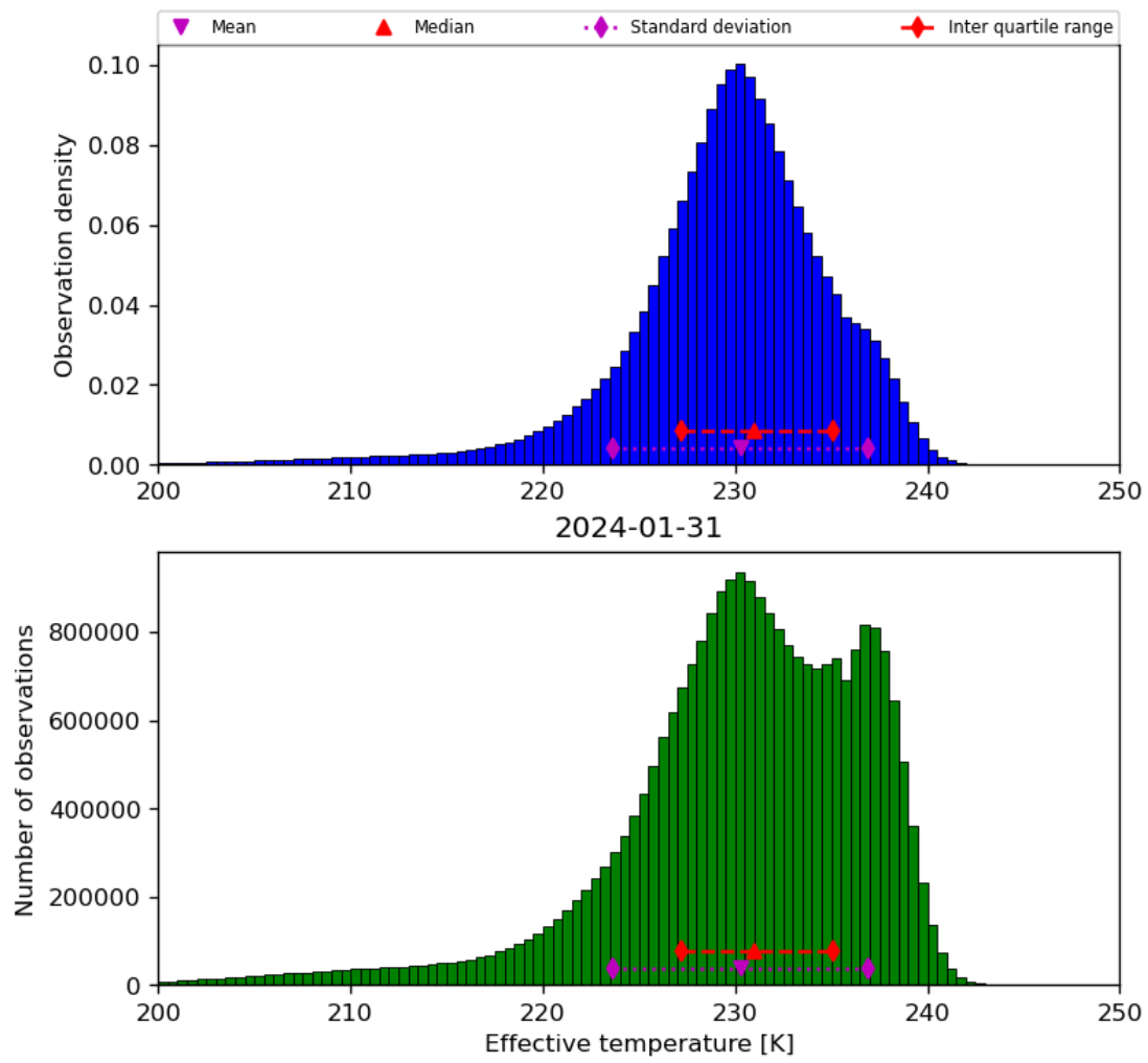
Figure 24: Histogram of “Effective temperature” for 2024-01-31 to 2024-02-01
