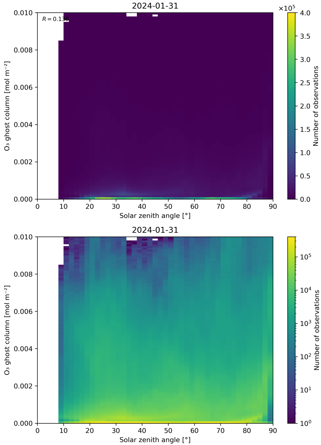
Figure 46: Scatter density plot of “Solar zenith angle” against “O 3 ghost column” for 2024-01-31 to 2024-02-01.
