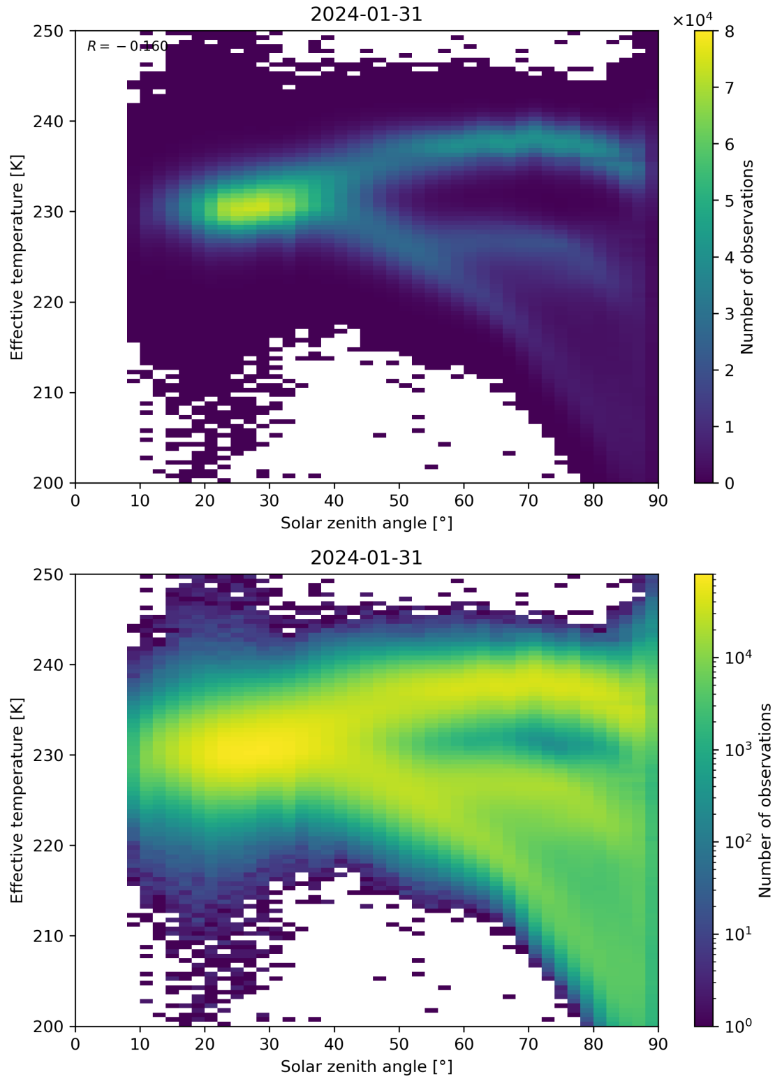
Figure 45: Scatter density plot of “Solar zenith angle” against “Effective temperature” for 2024-01-31 to 2024-02-01.
