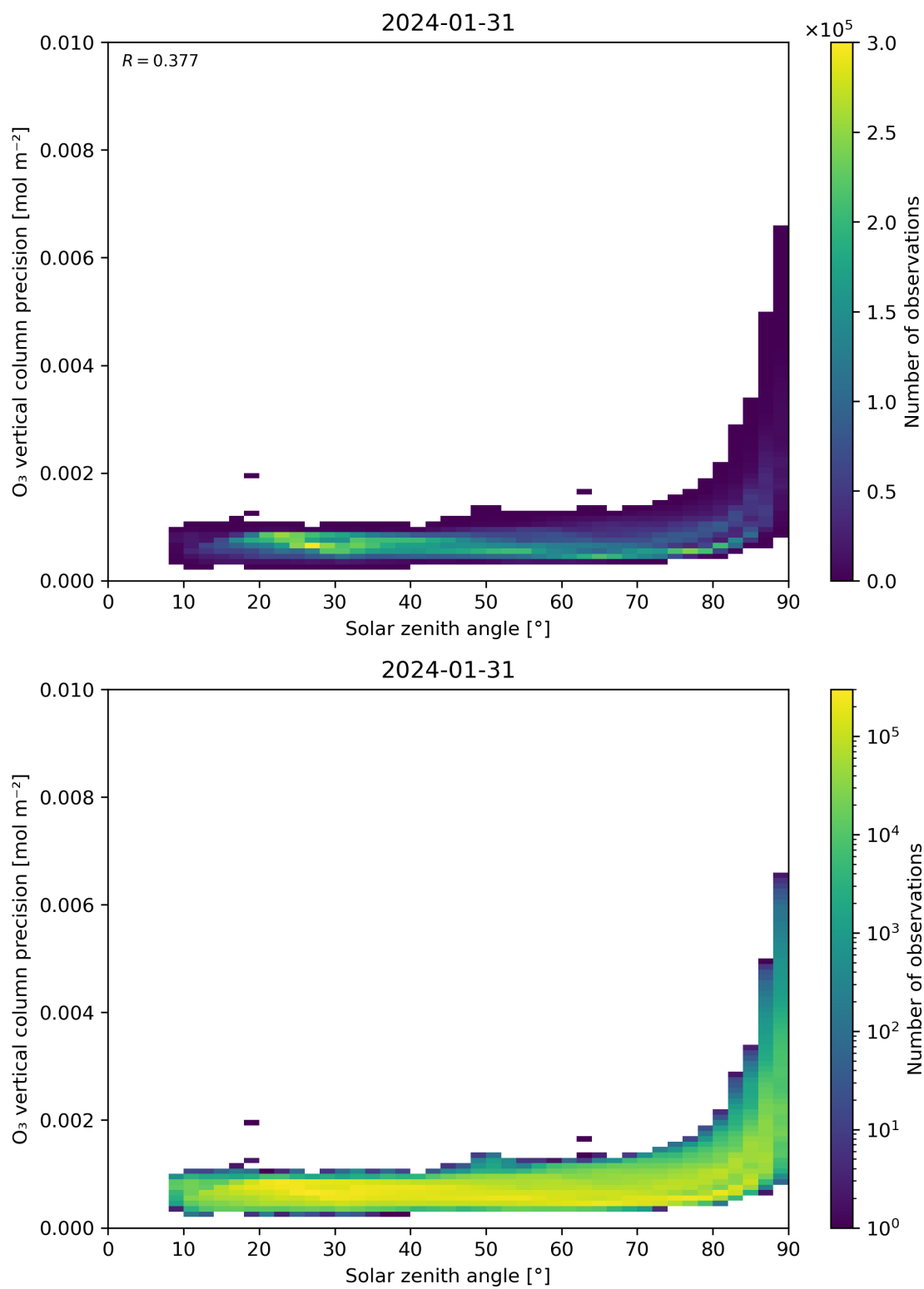
Figure 48: Scatter density plot of “Solar zenith angle” against “O 3 vertical column precision” for 2024-01-31 to 2024-02-01.
