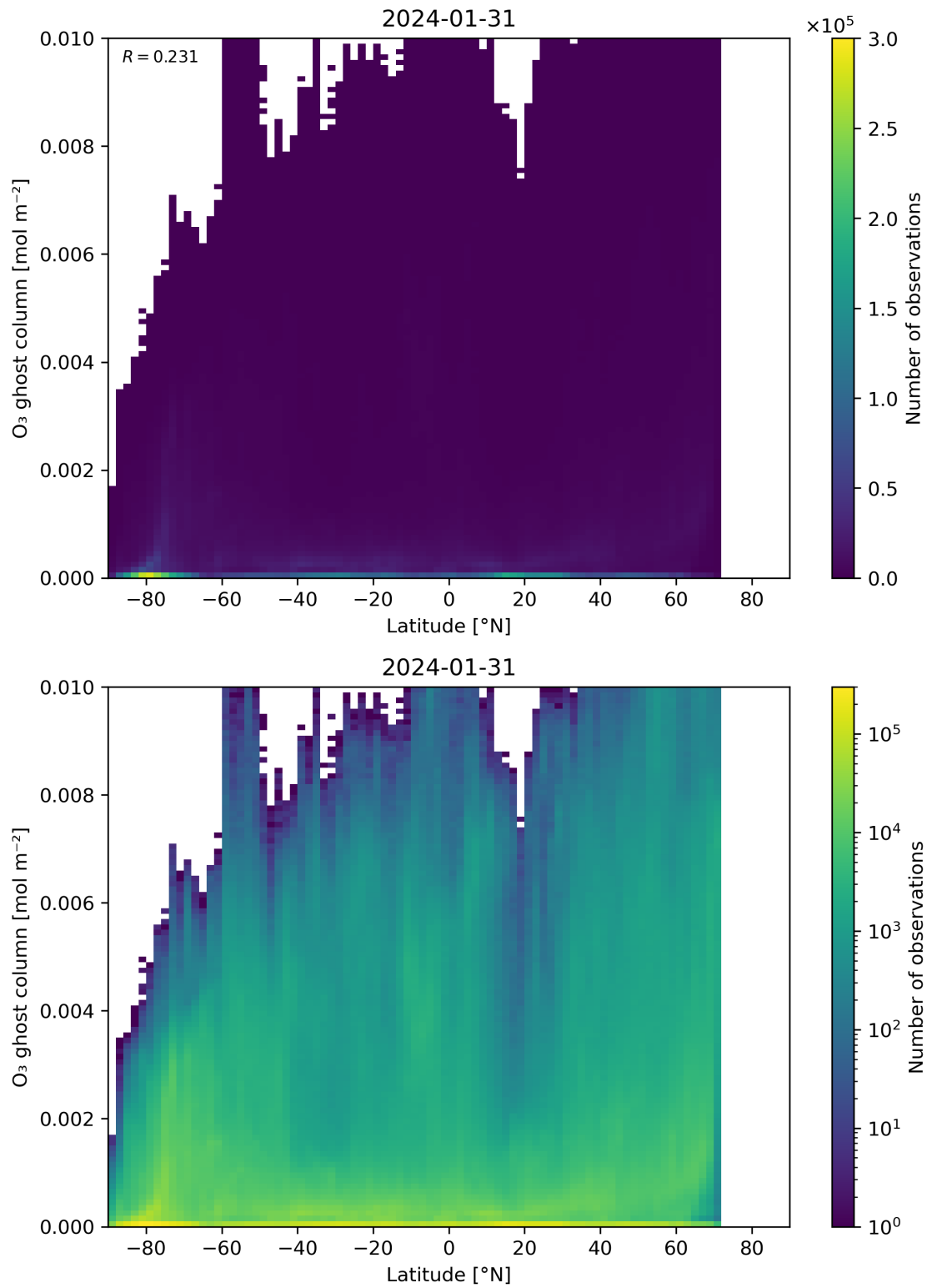
Figure 35: Scatter density plot of “Latitude” against “O 3 ghost column” for 2024-01-31 to 2024-02-01.
