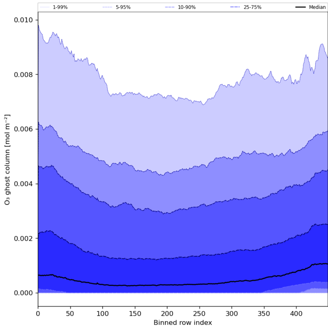
Figure 32: Along track statistics of “O 3 ghost column” for 2024-01-31 to 2024-02-01
