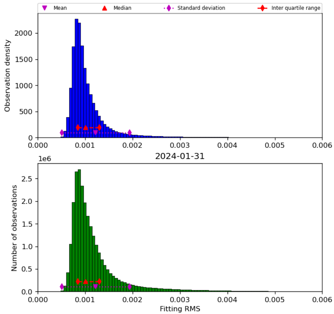
Figure 23: Histogram of “Fitting RMS” for 2024-01-31 to 2024-02-01
