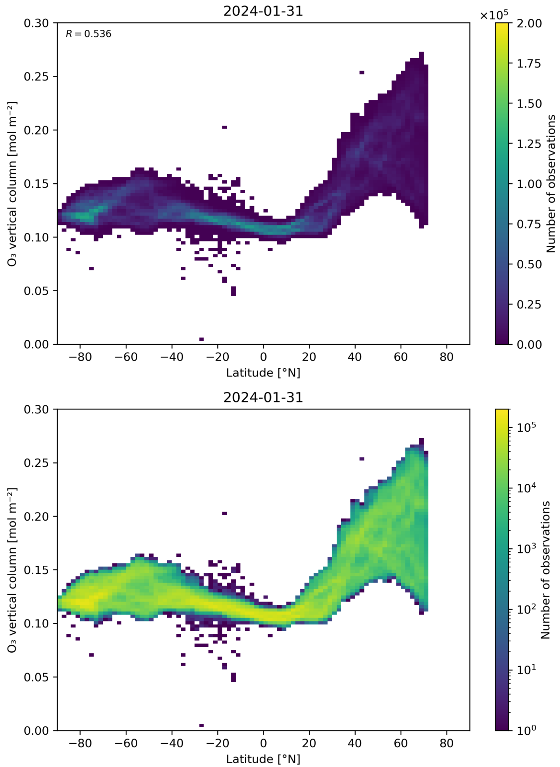
Figure 36: Scatter density plot of “Latitude” against “O 3 vertical column” for 2024-01-31 to 2024-02-01.
