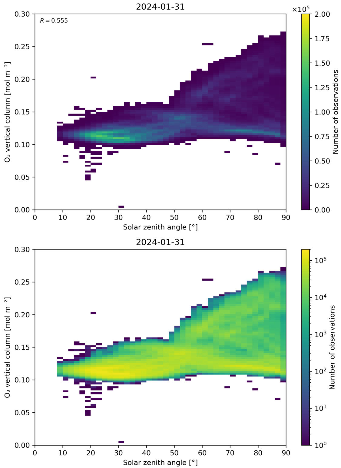
Figure 47: Scatter density plot of “Solar zenith angle” against “O 3 vertical column” for 2024-01-31 to 2024-02-01.
