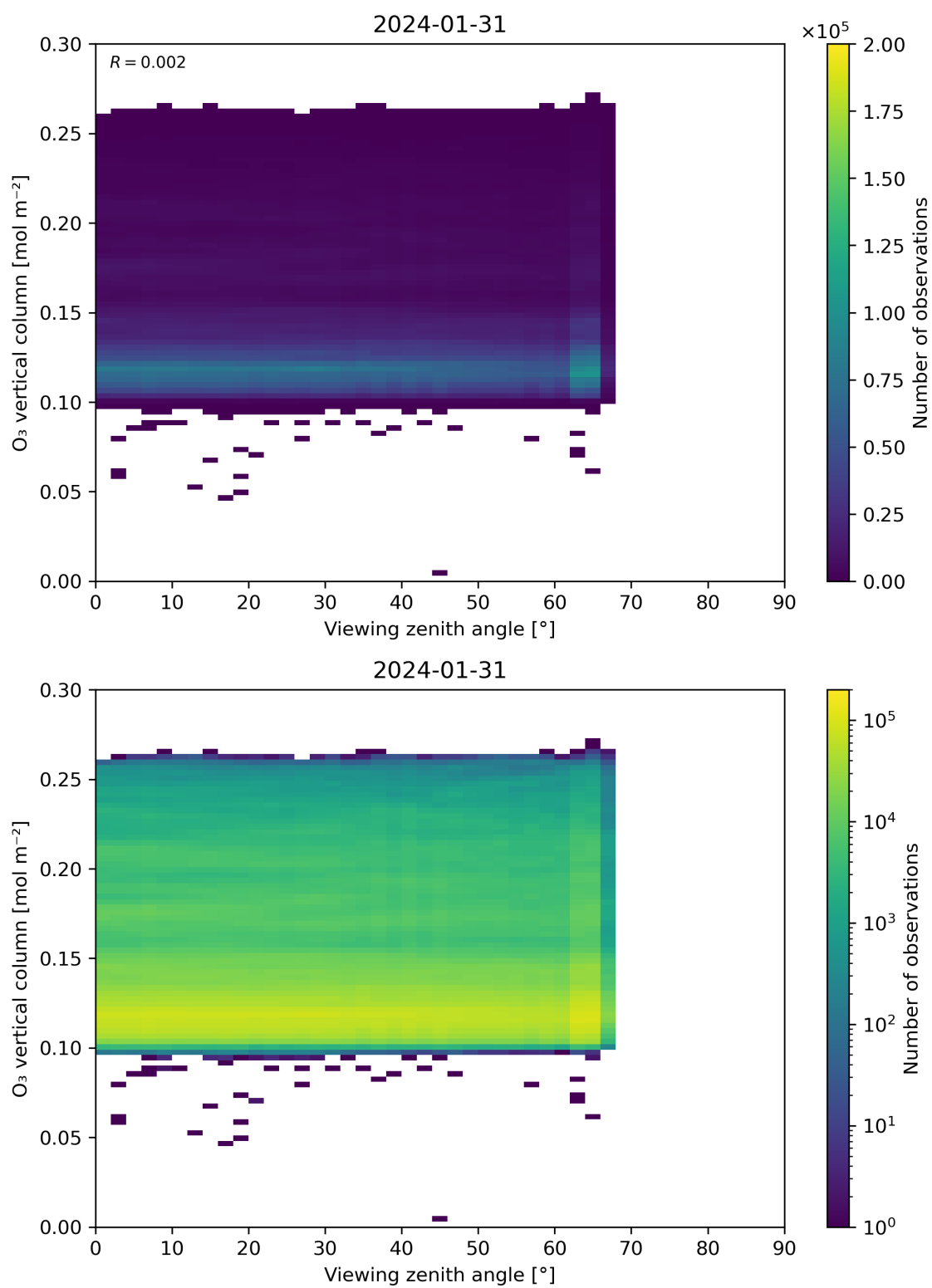
Figure 52: Scatter density plot of “Viewing zenith angle” against “O 3 vertical column” for 2024-01-31 to 2024-02-01.
