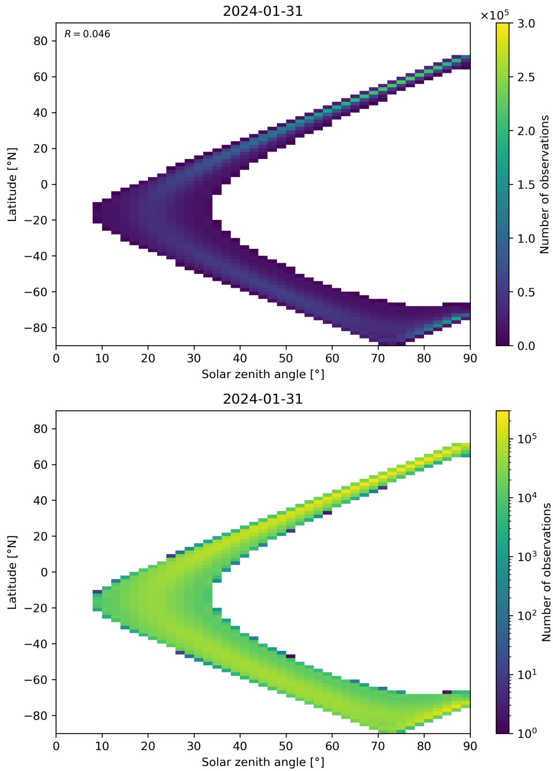
Figure 44: Scatter density plot of “Solar zenith angle” against “Latitude” for 2024-01-31 to 2024-02-01.
