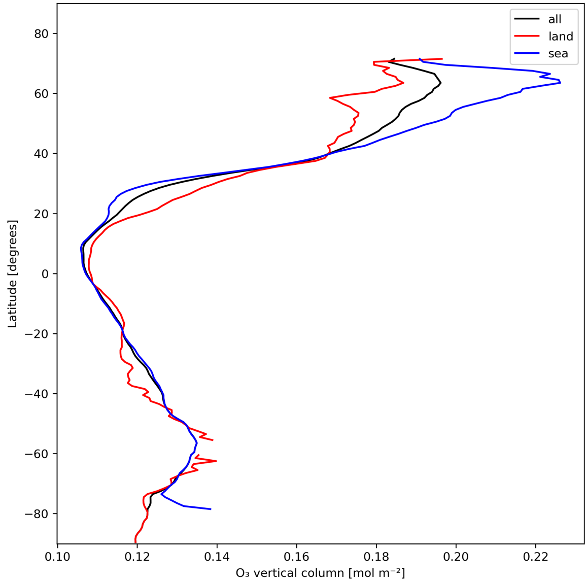
Figure 14: Zonal average of “O 3 vertical column” for 2024-01-31 to 2024-02-01.
