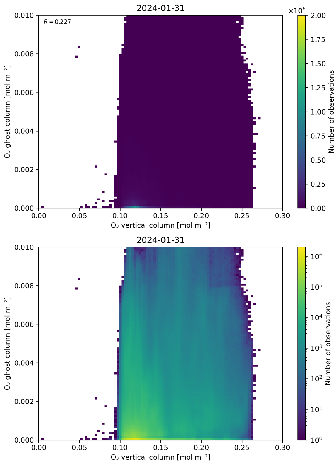
Figure 40: Scatter density plot of “O 3 vertical column” against “O 3 ghost column” for 2024-01-31 to 2024-02-01.
