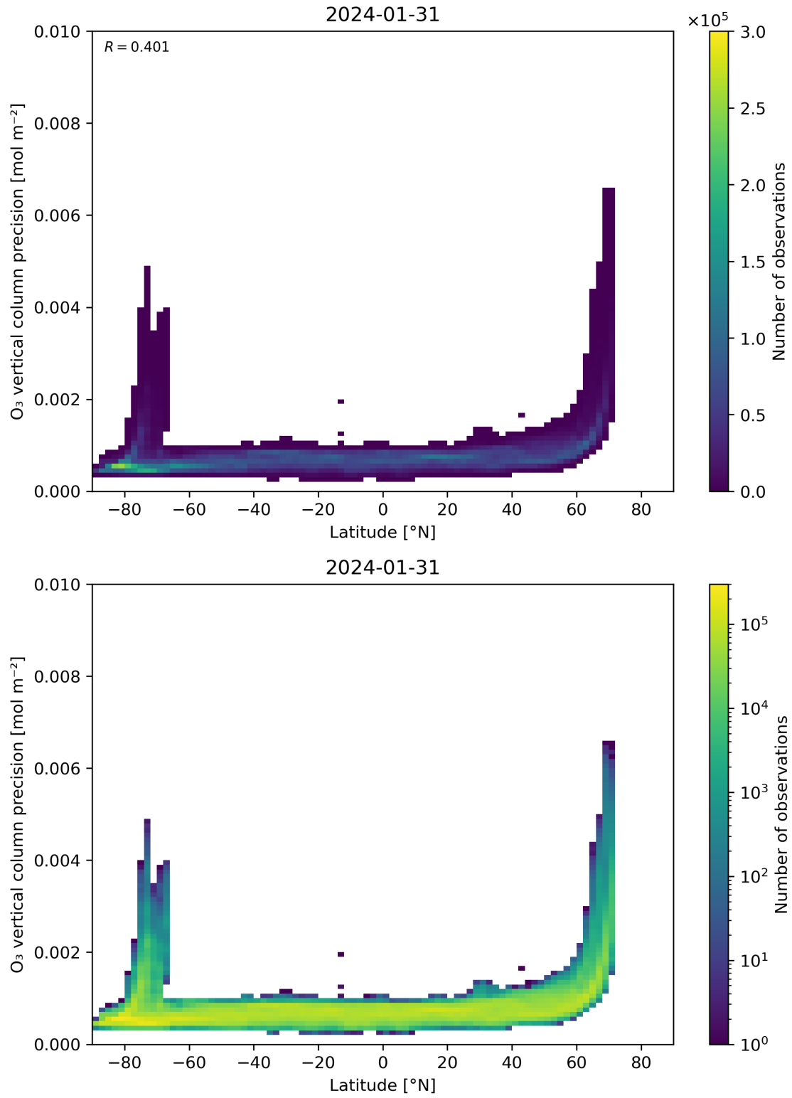
Figure 37: Scatter density plot of “Latitude” against “O 3 vertical column precision” for 2024-01-31 to 2024-02-01.
