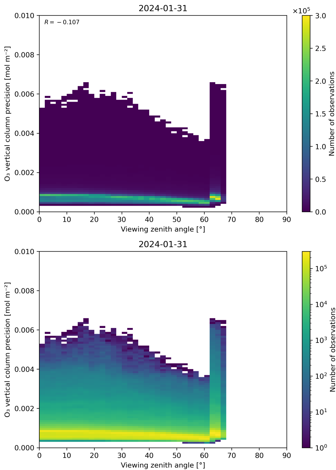
Figure 53: Scatter density plot of “Viewing zenith angle” against “O 3 vertical column precision” for 2024-01-31 to 2024-02-01.
