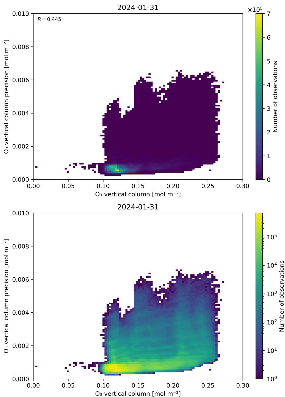
Figure 41: Scatter density plot of “O 3 vertical column” against “O 3 vertical column precision” for 2024-01-31 to 2024-02-01.
