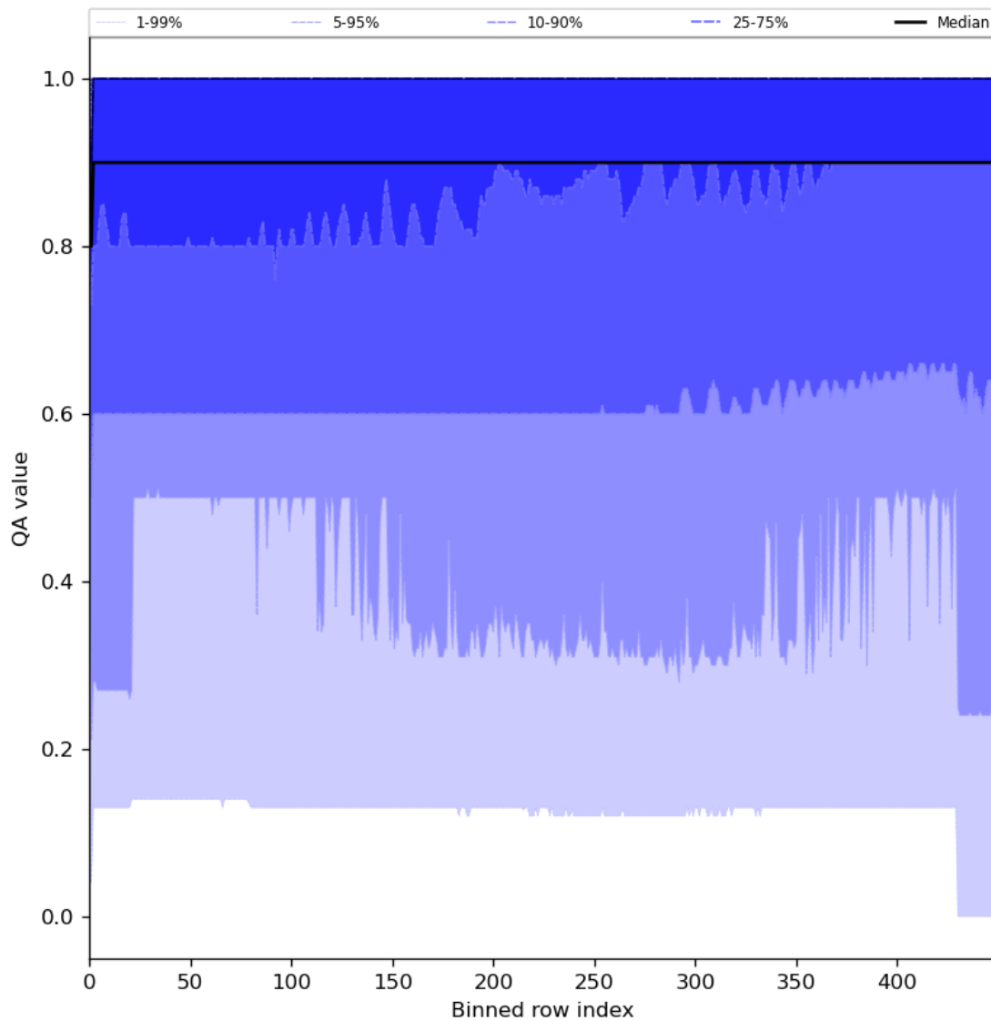
Figure 27: Along track statistics of “QA value” for 2024-01-31 to 2024-02-01
