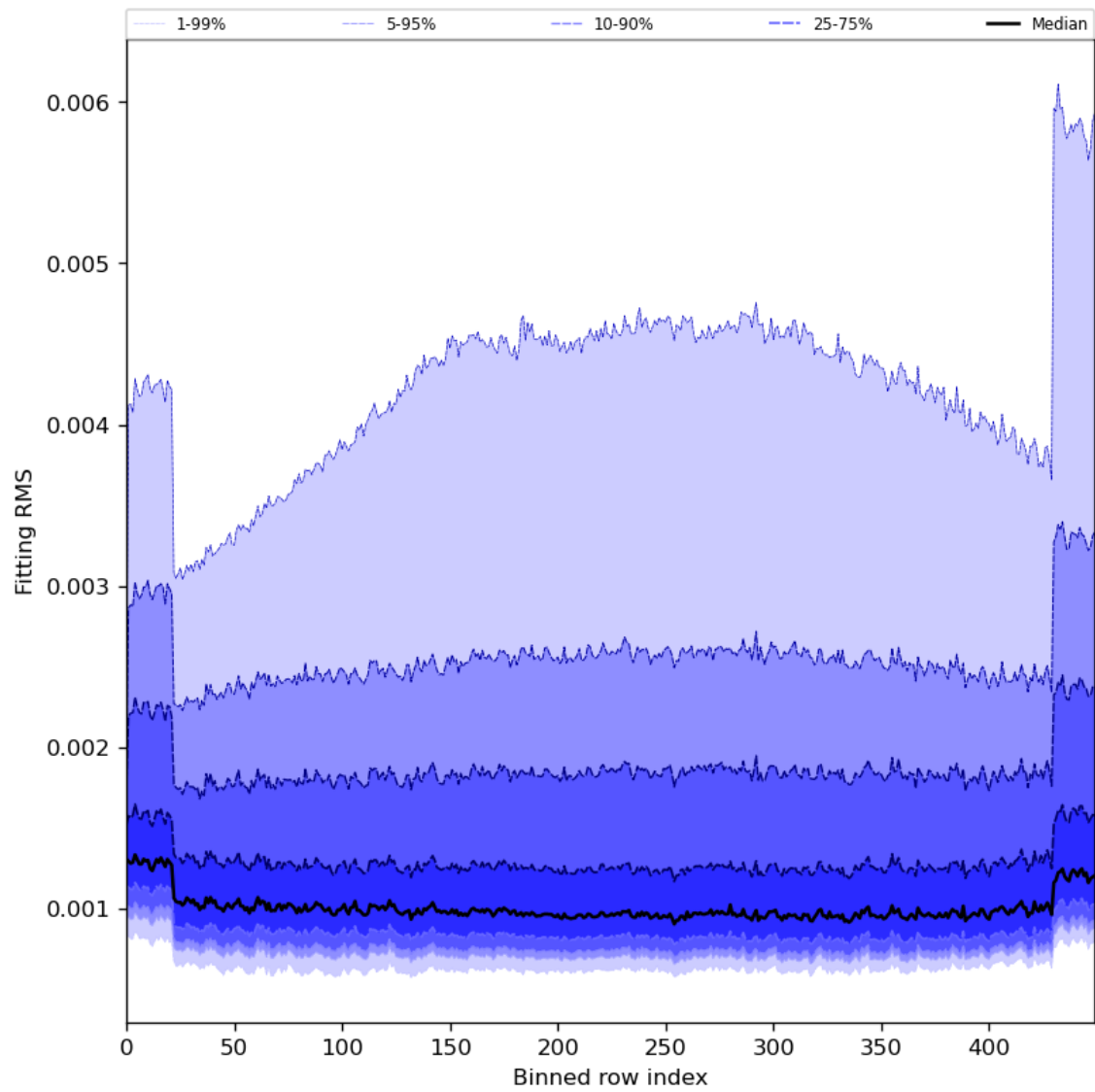
Figure 30: Along track statistics of “Fitting RMS” for 2024-01-31 to 2024-02-01
