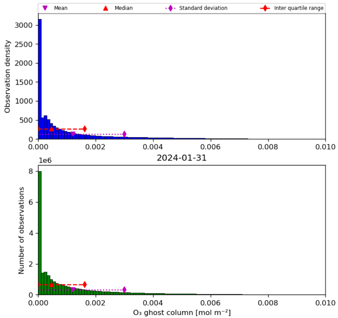
Figure 25: Histogram of “O 3 ghost column” for 2024-01-31 to 2024-02-01
