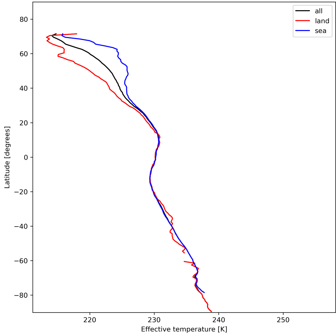
Figure 17: Zonal average of "Effective temperature" for 2024-01-31 to 2024-02-01.
