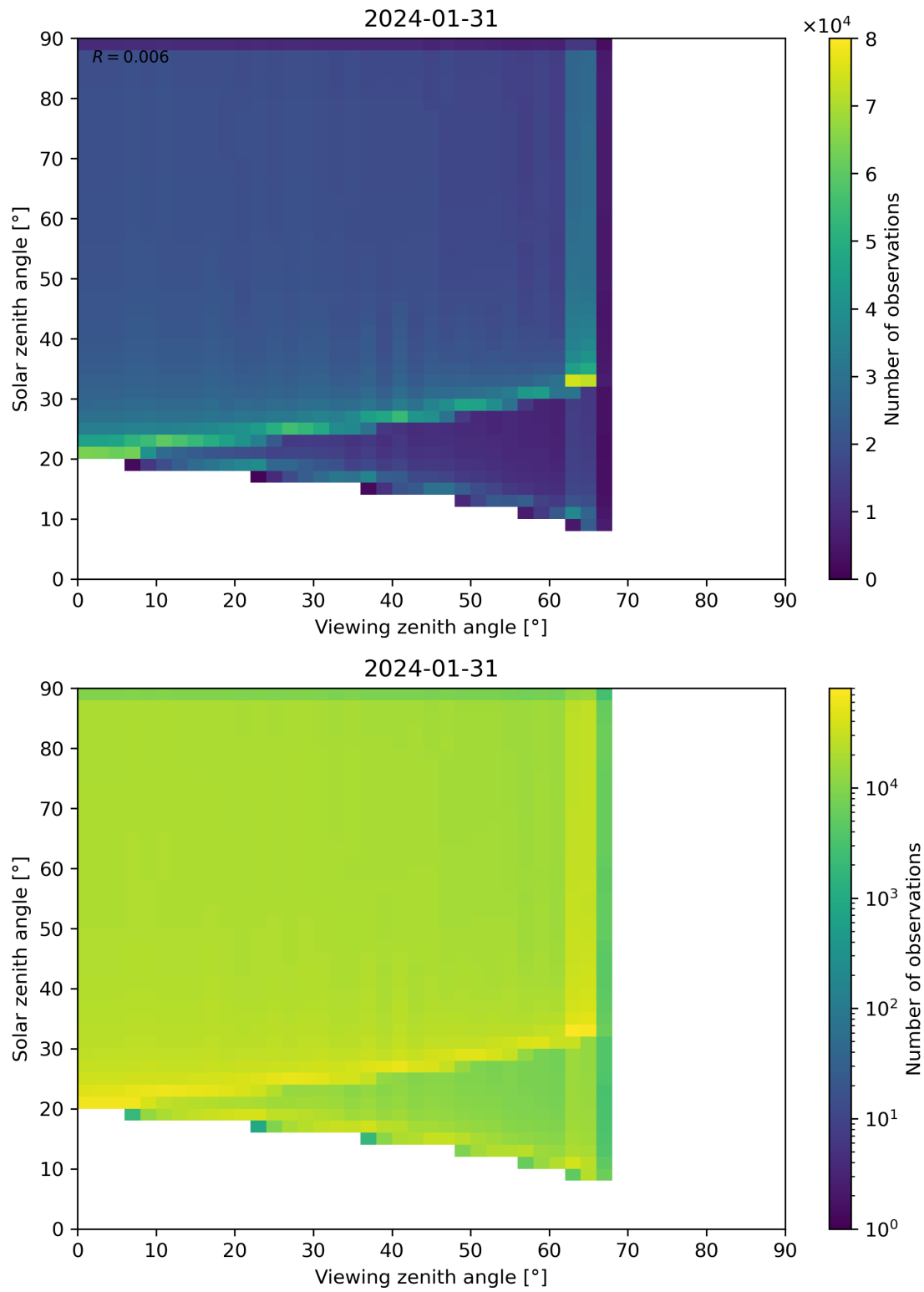
Figure 54: Scatter density plot of “Viewing zenith angle” against “Solar zenith angle” for 2024-01-31 to 2024-02-01.
