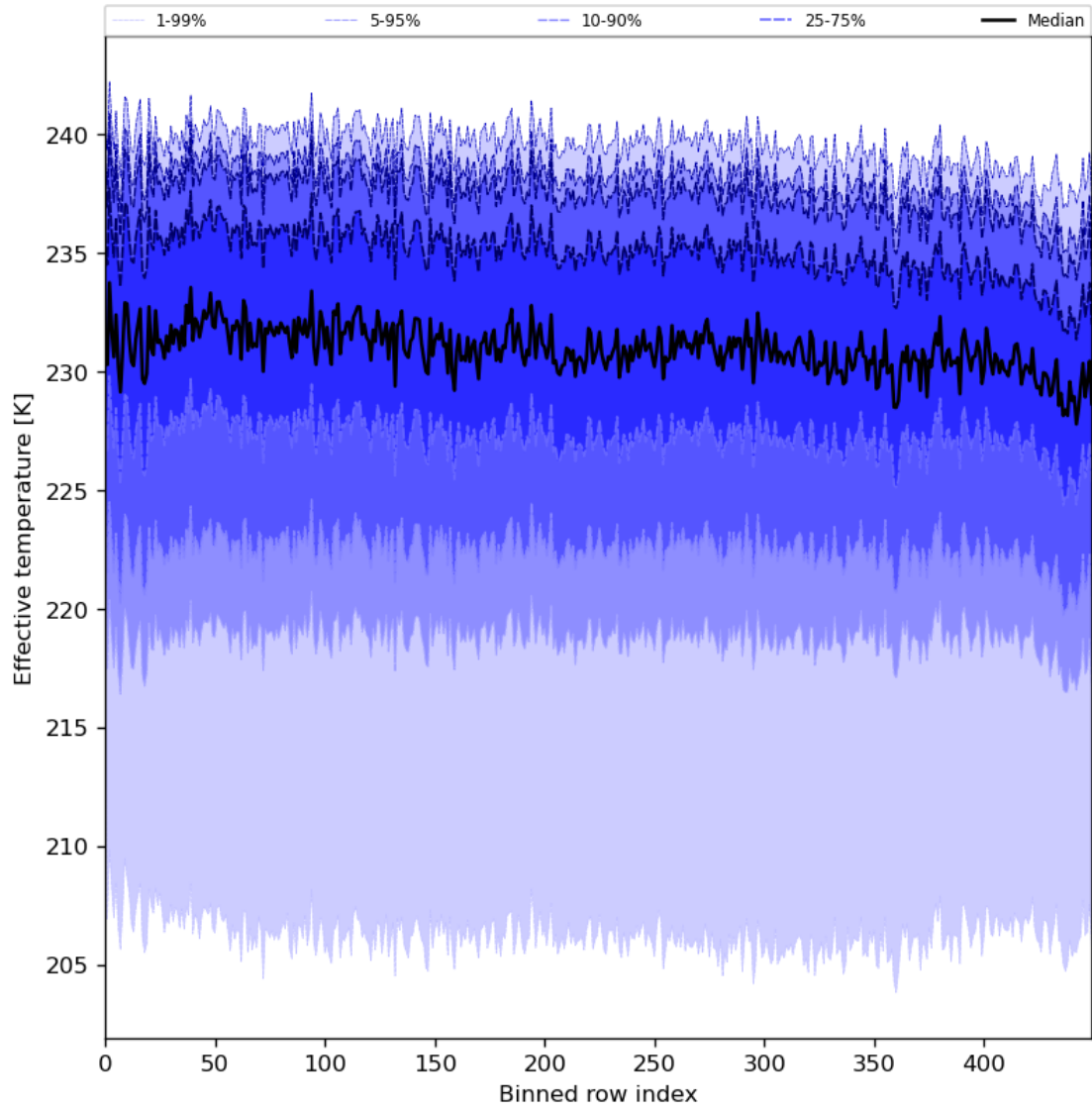
Figure 31: Along track statistics of “Effective temperature” for 2024-01-31 to 2024-02-02
