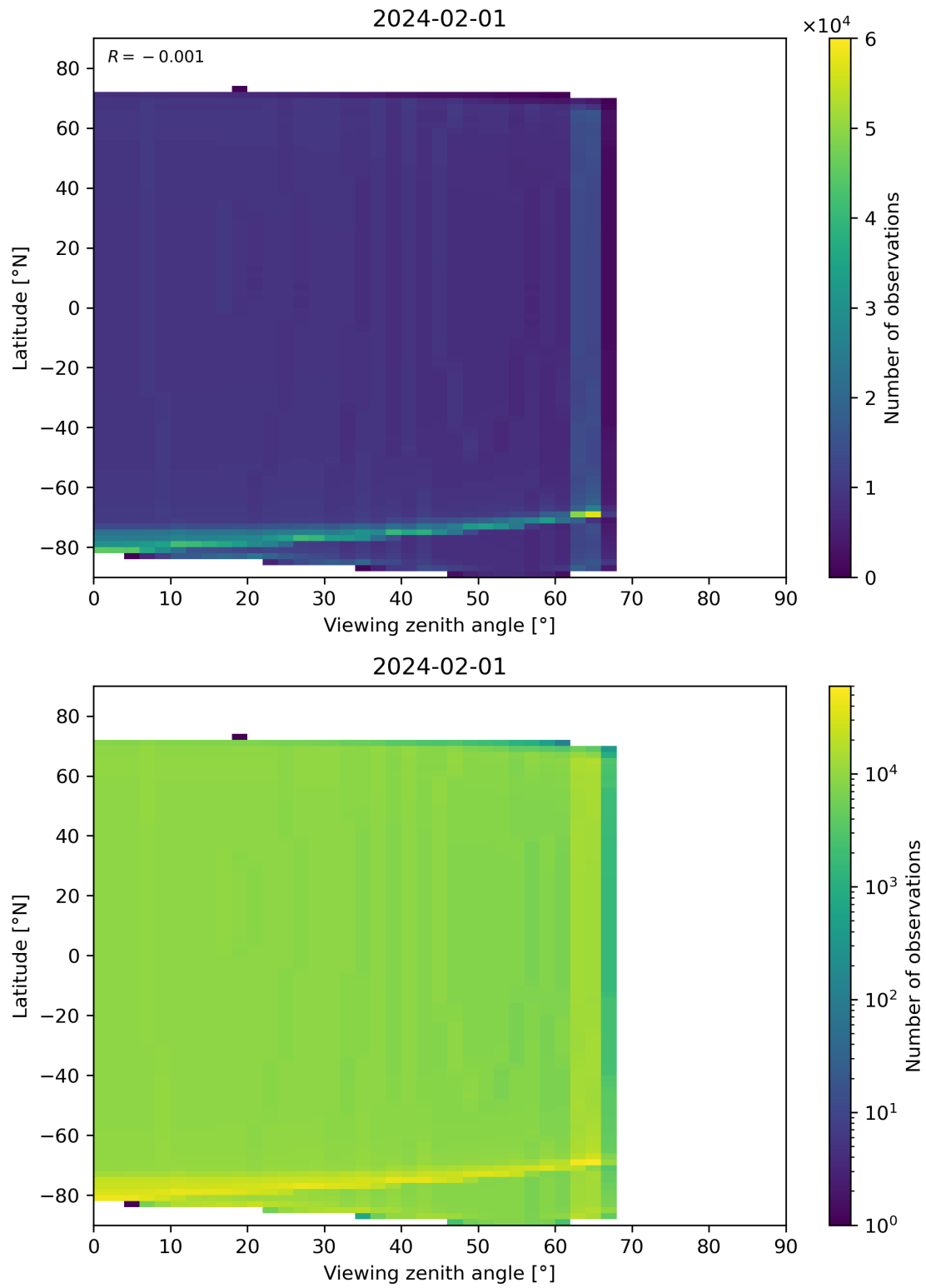
Figure 49: Scatter density plot of “Viewing zenith angle” against “Latitude” for 2024-01-31 to 2024-02-02.
