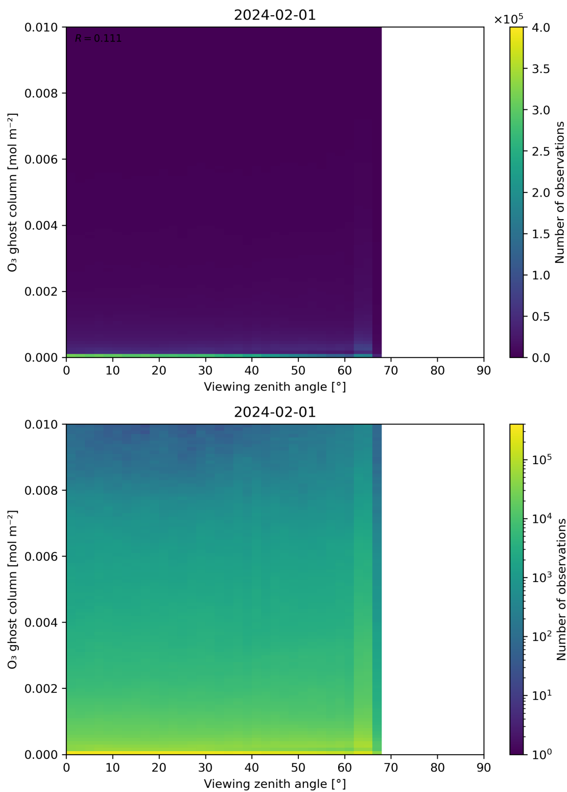
Figure 51: Scatter density plot of “Viewing zenith angle” against “O 3 ghost column” for 2024-01-31 to 2024-02-02.
