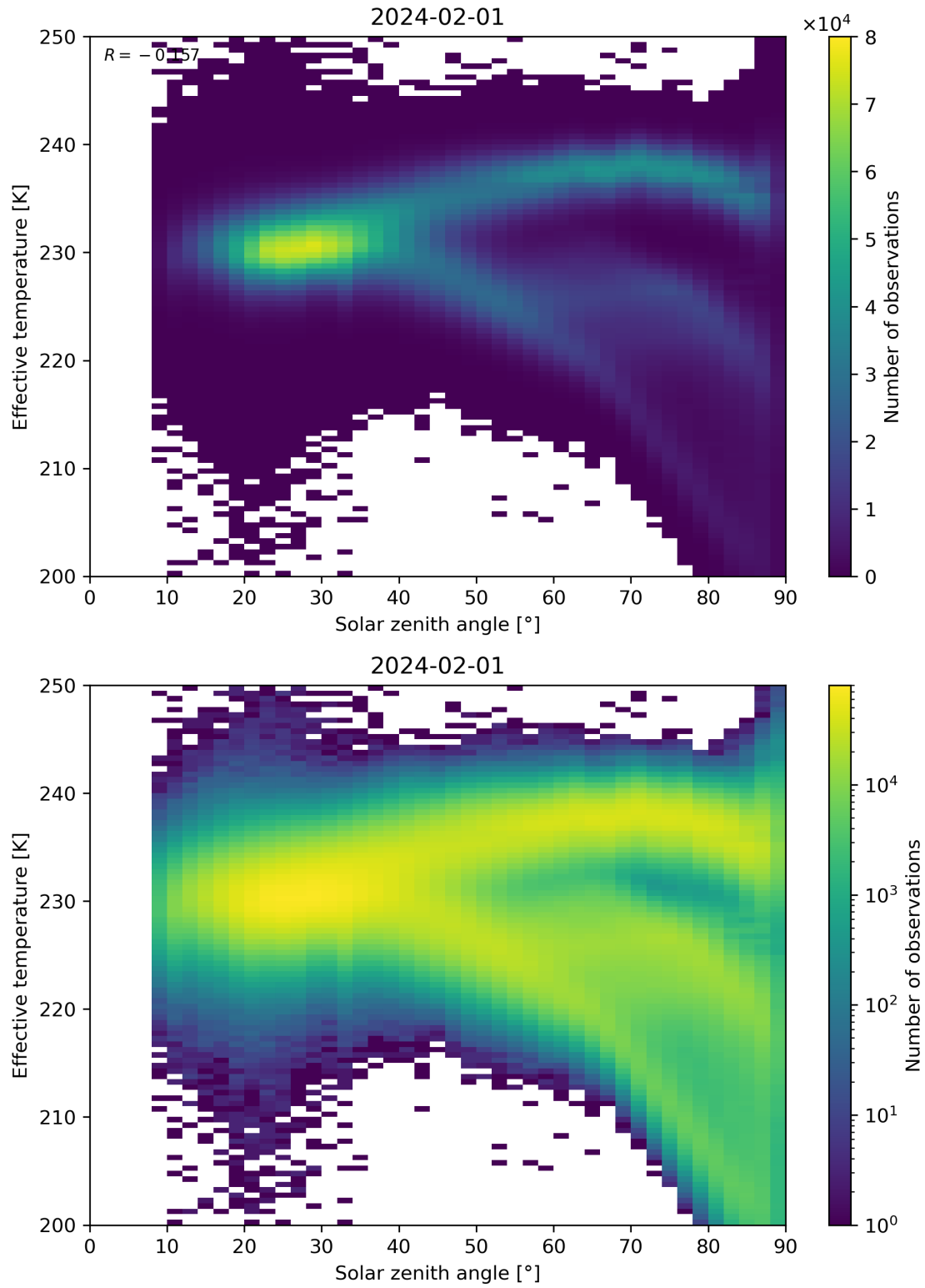
Figure 45: Scatter density plot of “Solar zenith angle” against “Effective temperature” for 2024-01-31 to 2024-02-02.
