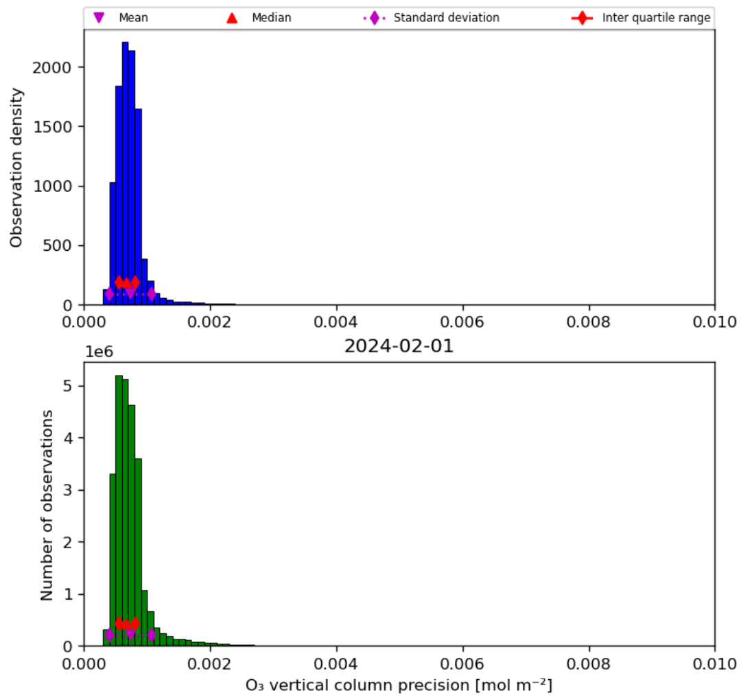
Figure 22: Histogram of “O 3 vertical column precision” for 2024-01-31 to 2024-02-02
