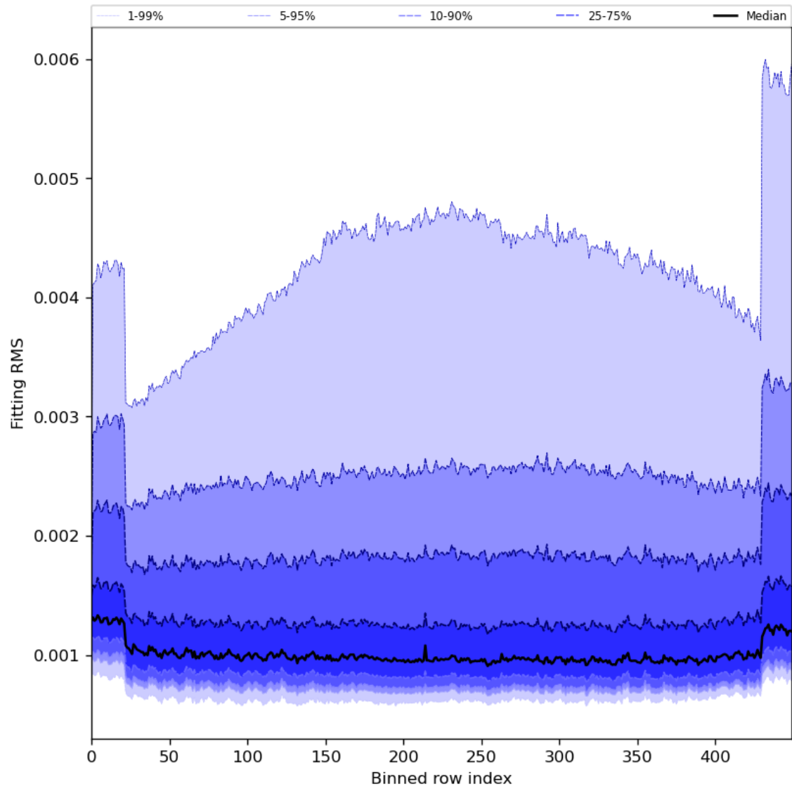
Figure 30: Along track statistics of “Fitting RMS” for 2024-01-31 to 2024-02-02
