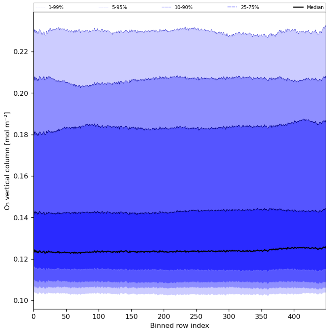
Figure 28: Along track statistics of “O 3 vertical column” for 2024-01-31 to 2024-02-02
