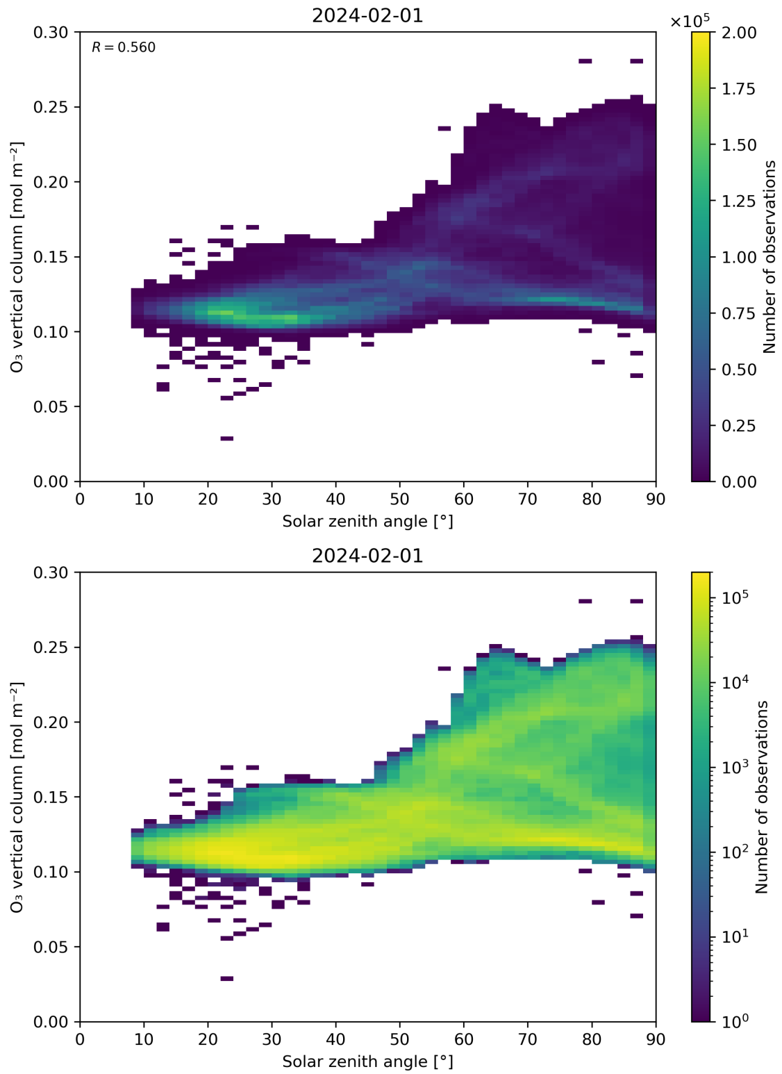
Figure 47: Scatter density plot of “Solar zenith angle” against “O 3 vertical column” for 2024-01-31 to 2024-02-02.
