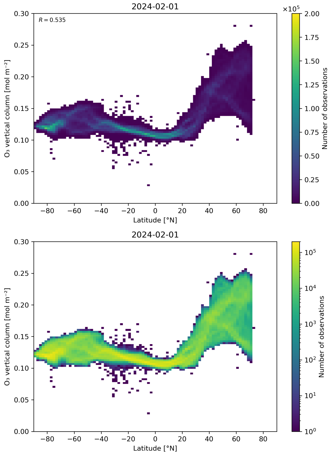
Figure 36: Scatter density plot of “Latitude” against “O 3 vertical column” for 2024-01-31 to 2024-02-02.
