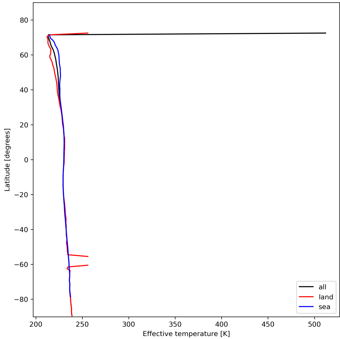
Figure 17: Zonal average of “Effective temperature” for 2024-01-31 to 2024-02-02.
