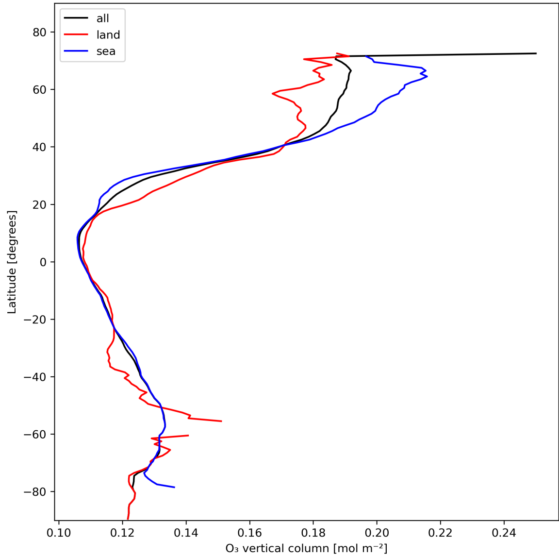
Figure 14: Zonal average of “O 3 vertical column” for 2024-01-31 to 2024-02-02.
