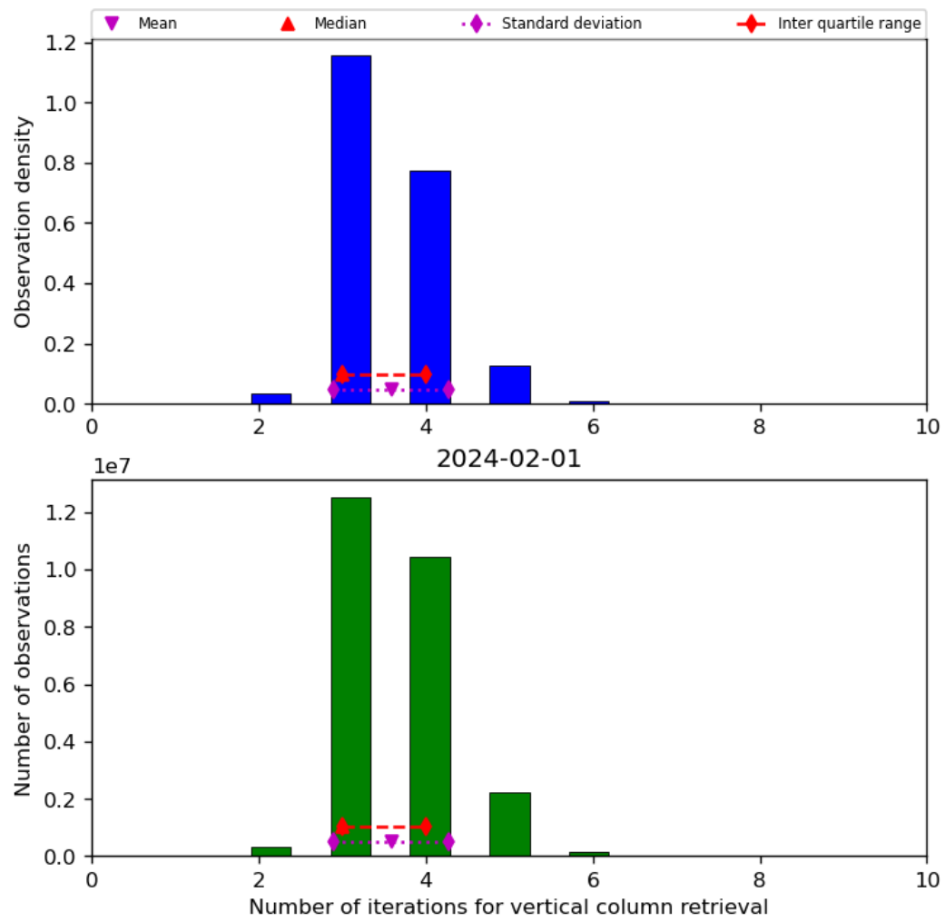
Figure 26: Histogram of “Number of iterations for vertical column retrieval” for 2024-01-31 to 2024-02-02
