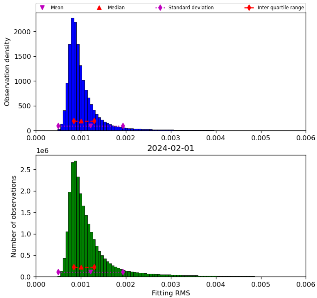
Figure 23: Histogram of “Fitting RMS” for 2024-01-31 to 2024-02-02
