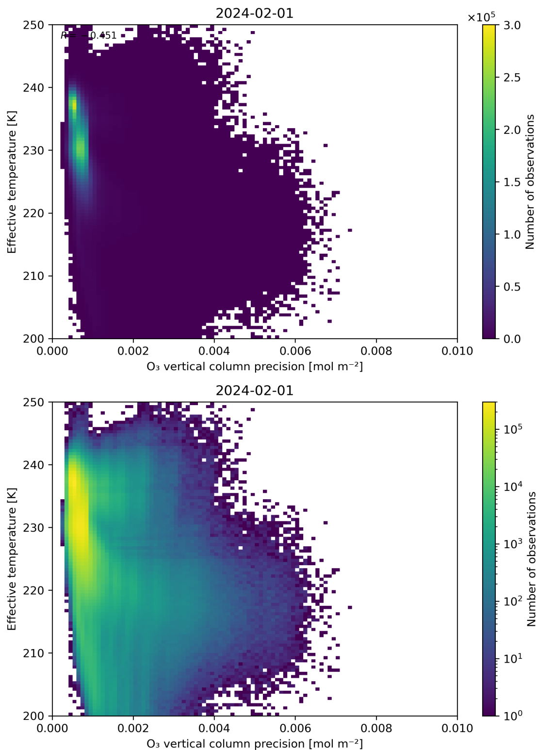
Figure 42: Scatter density plot of “O 3 vertical column precision” against “Effective temperature” for 2024-01-31 to 2024-02-02.
