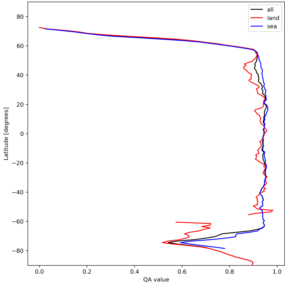
Figure 13: Zonal average of “QA value” for 2024-01-31 to 2024-02-02.
