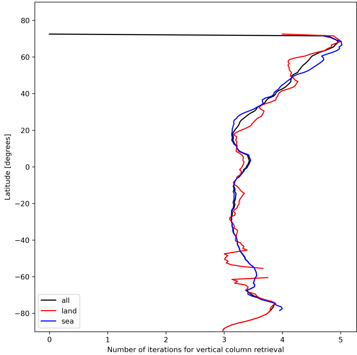
Figure 19: Zonal average of “Number of iterations for vertical column retrieval” for 2024-01-31 to 2024-02-02.
