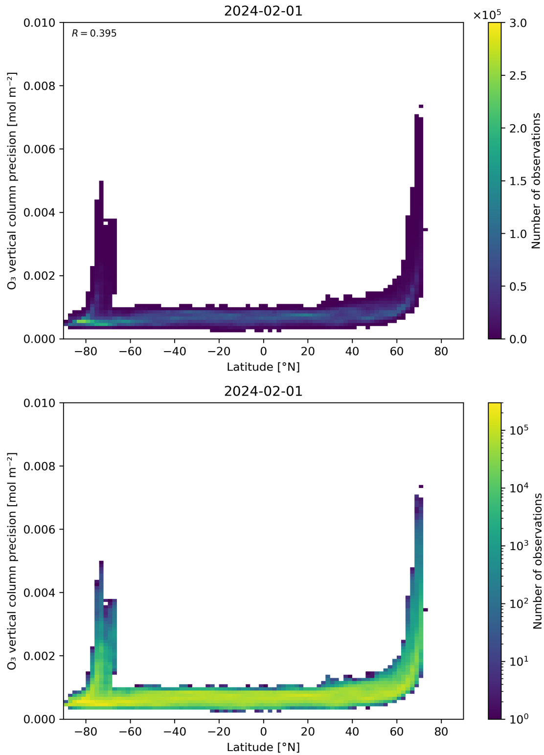
Figure 37: Scatter density plot of “Latitude” against “O 3 vertical column precision” for 2024-01-31 to 2024-02-02.
