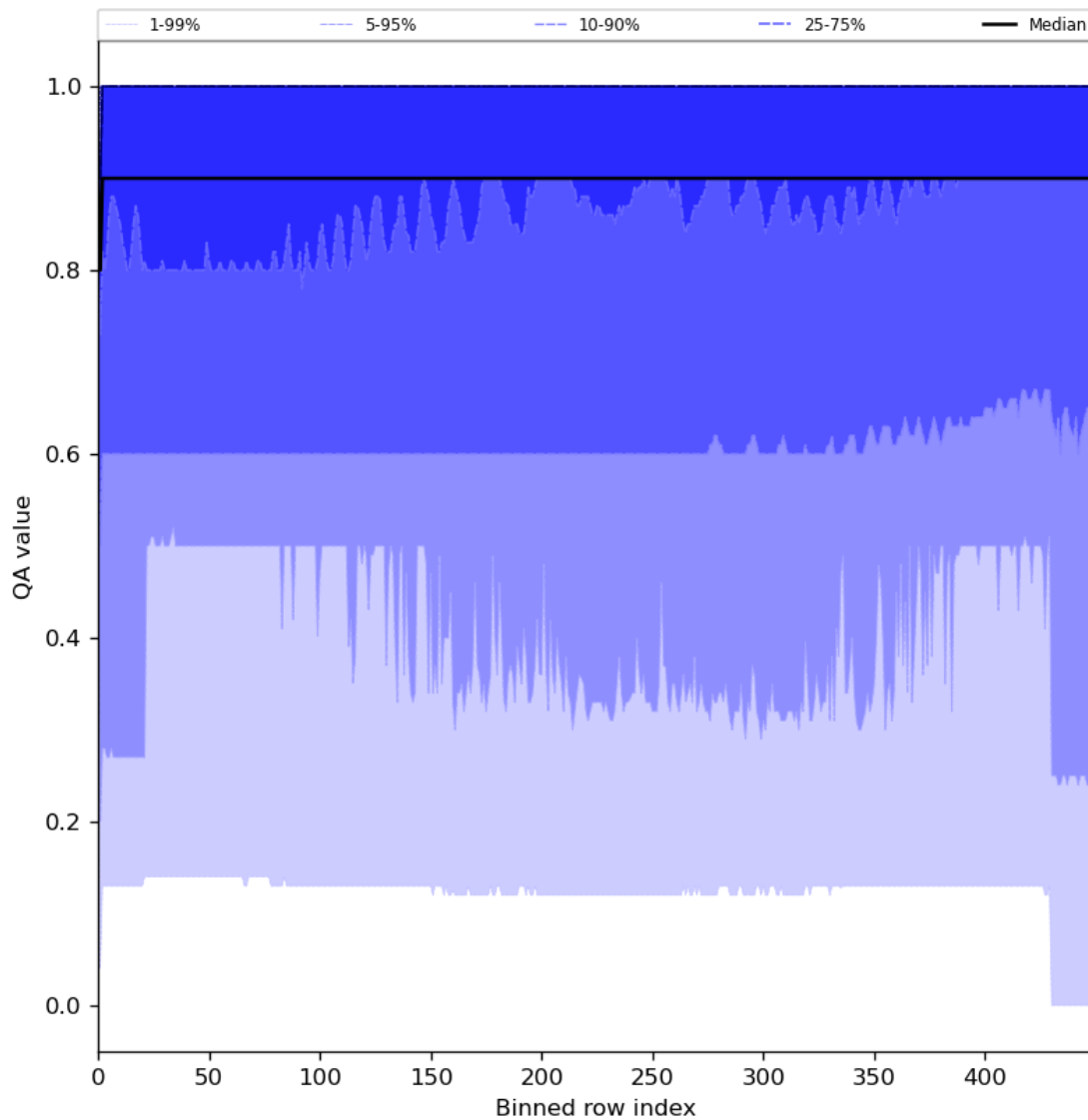
Figure 27: Along track statistics of “QA value” for 2024-01-31 to 2024-02-02
