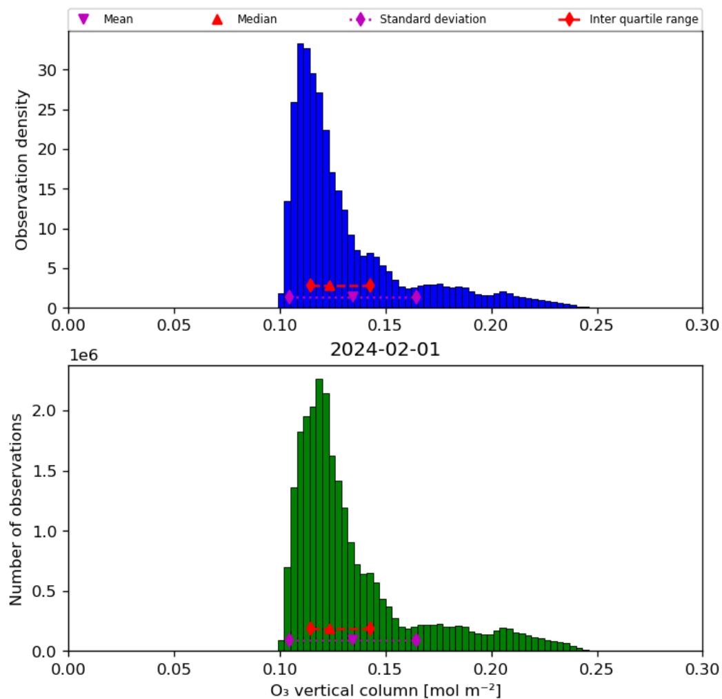
Figure 21: Histogram of “O 3 vertical column” for 2024-01-31 to 2024-02-02
