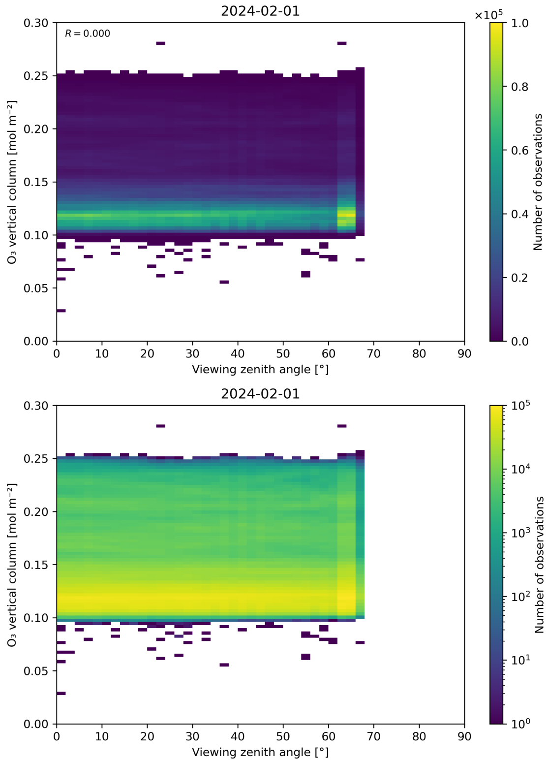
Figure 52: Scatter density plot of “Viewing zenith angle” against “O 3 vertical column” for 2024-01-31 to 2024-02-02.
