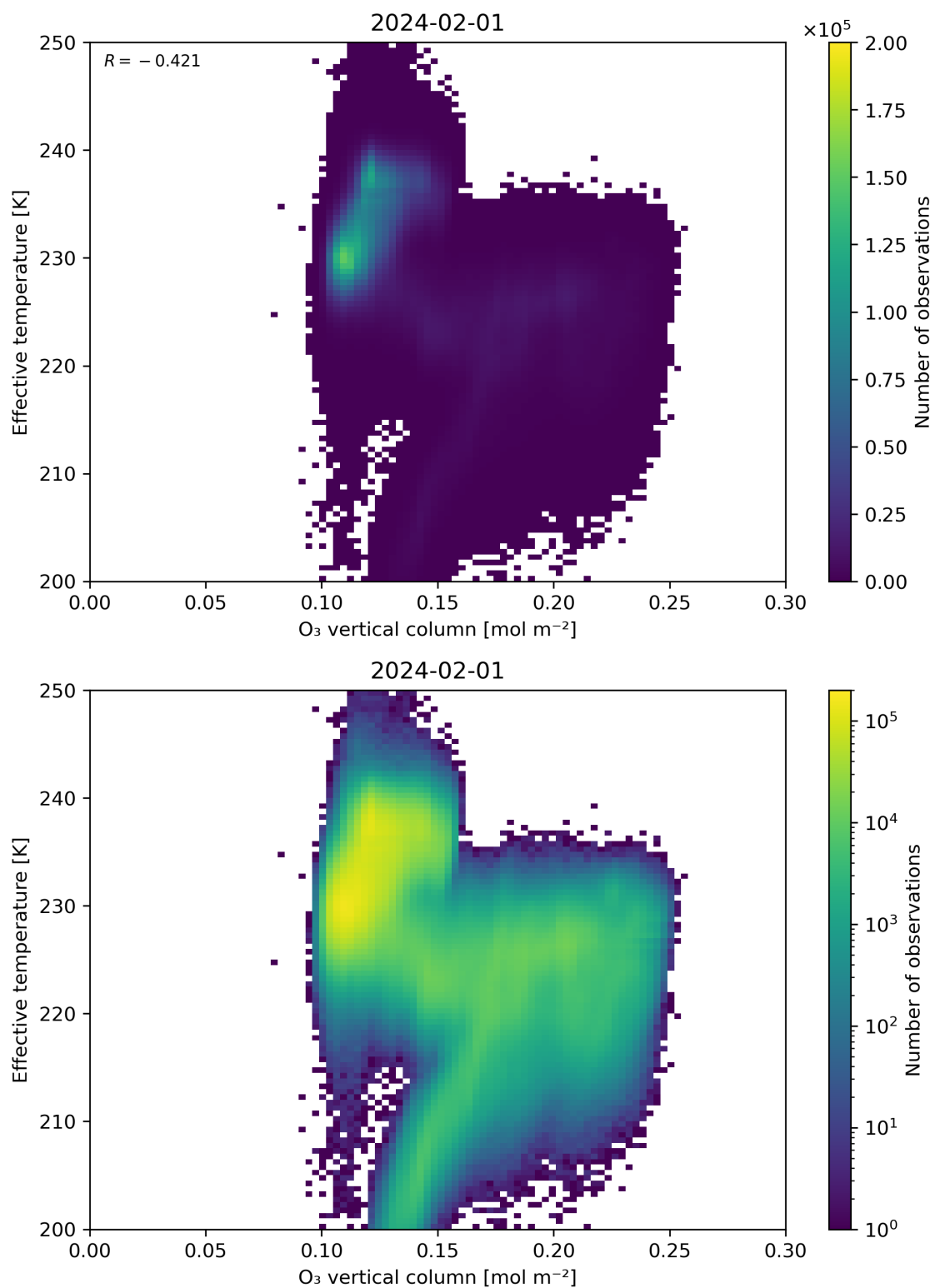
Figure 39: Scatter density plot of “O 3 vertical column” against “Effective temperature” for 2024-01-31 to 2024-02-02.
