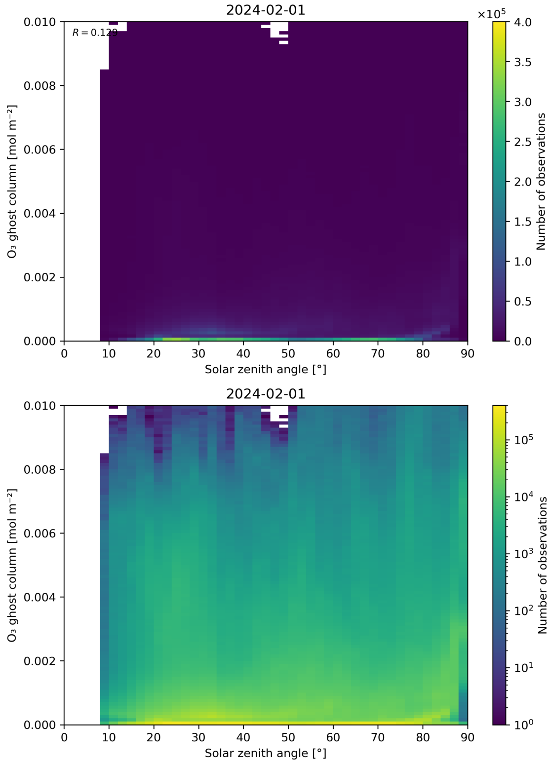
Figure 46: Scatter density plot of “Solar zenith angle” against “O 3 ghost column” for 2024-01-31 to 2024-02-02.
