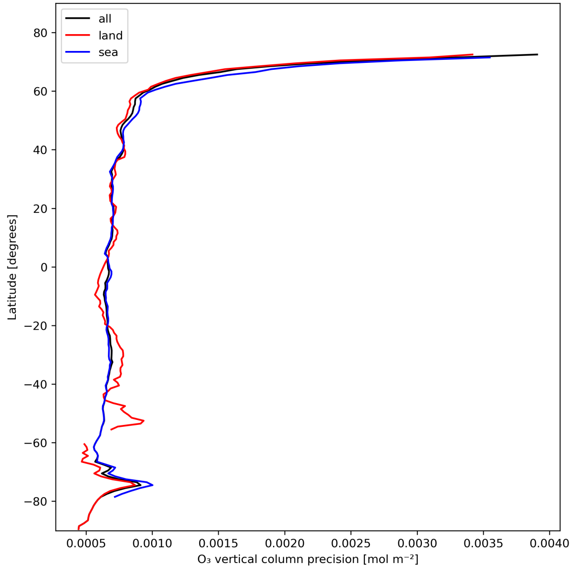
Figure 15: Zonal average of “O 3 vertical column precision” for 2024-01-31 to 2024-02-02.
