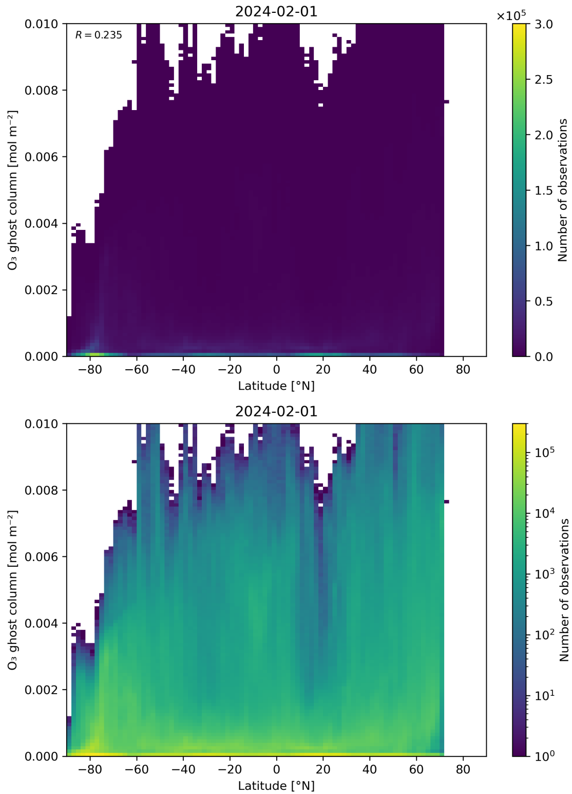
Figure 35: Scatter density plot of “Latitude” against “O 3 ghost column” for 2024-01-31 to 2024-02-02.
