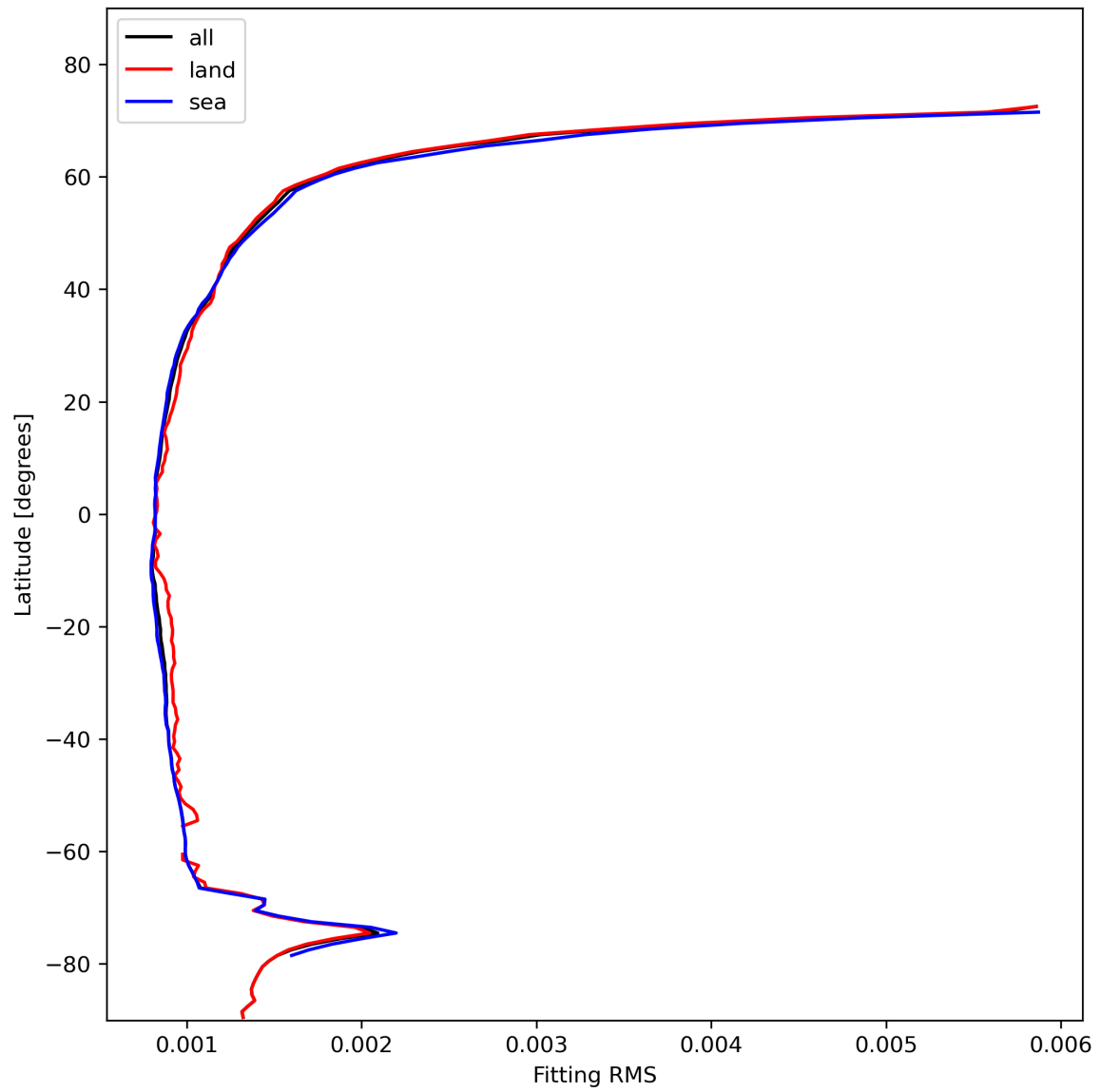
Figure 16: Zonal average of “Fitting RMS” for 2024-01-31 to 2024-02-02.
