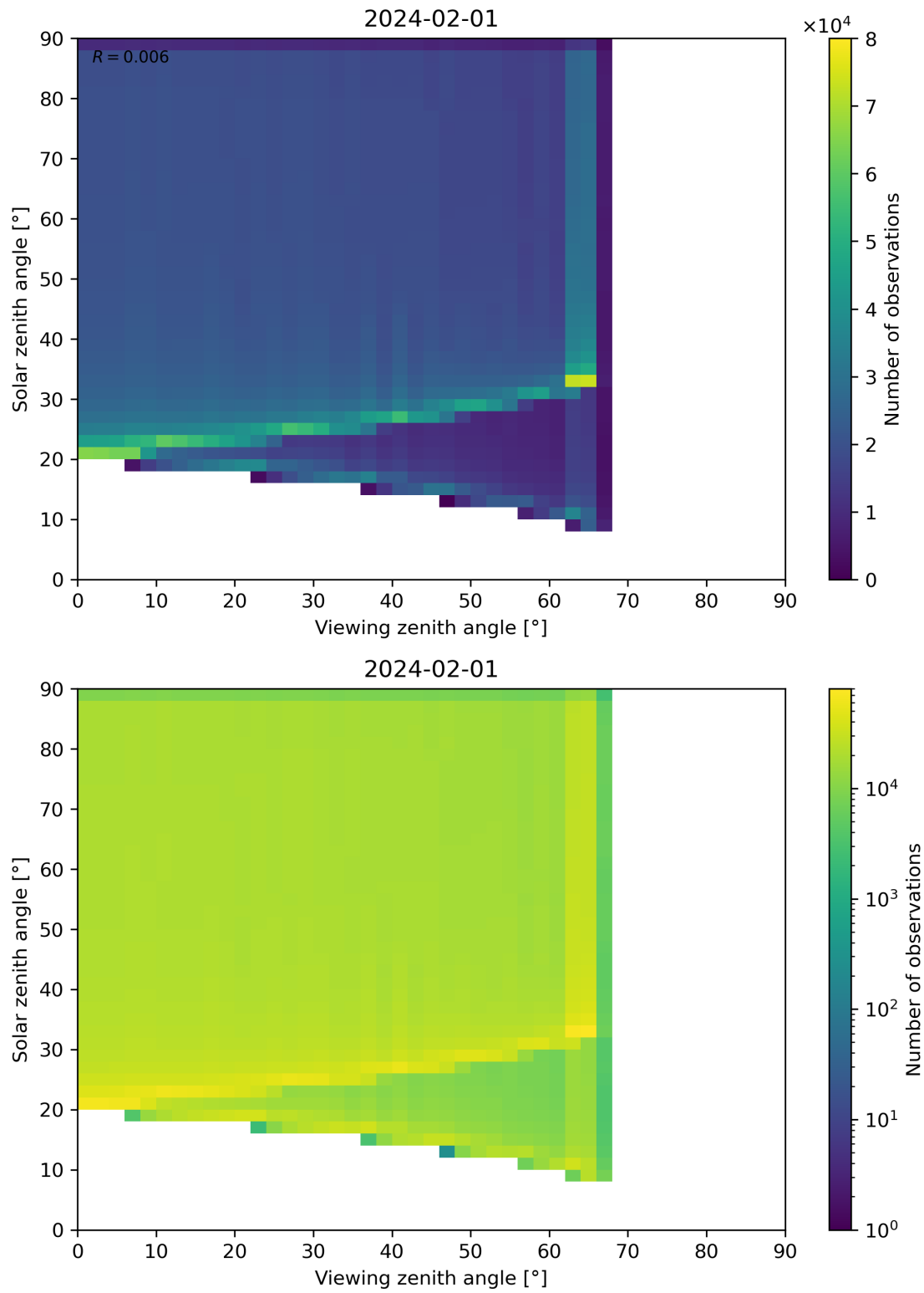
Figure 54: Scatter density plot of “Viewing zenith angle” against “Solar zenith angle” for 2024-01-31 to 2024-02-02.
