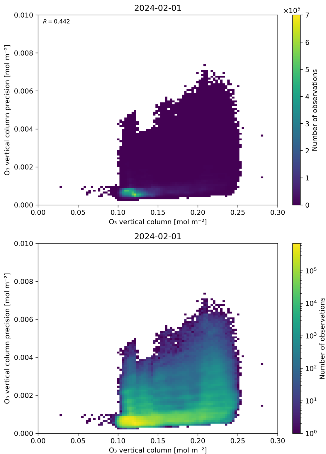
Figure 41: Scatter density plot of “O 3 vertical column” against “O 3 vertical column precision” for 2024-01-31 to 2024-02-02.
