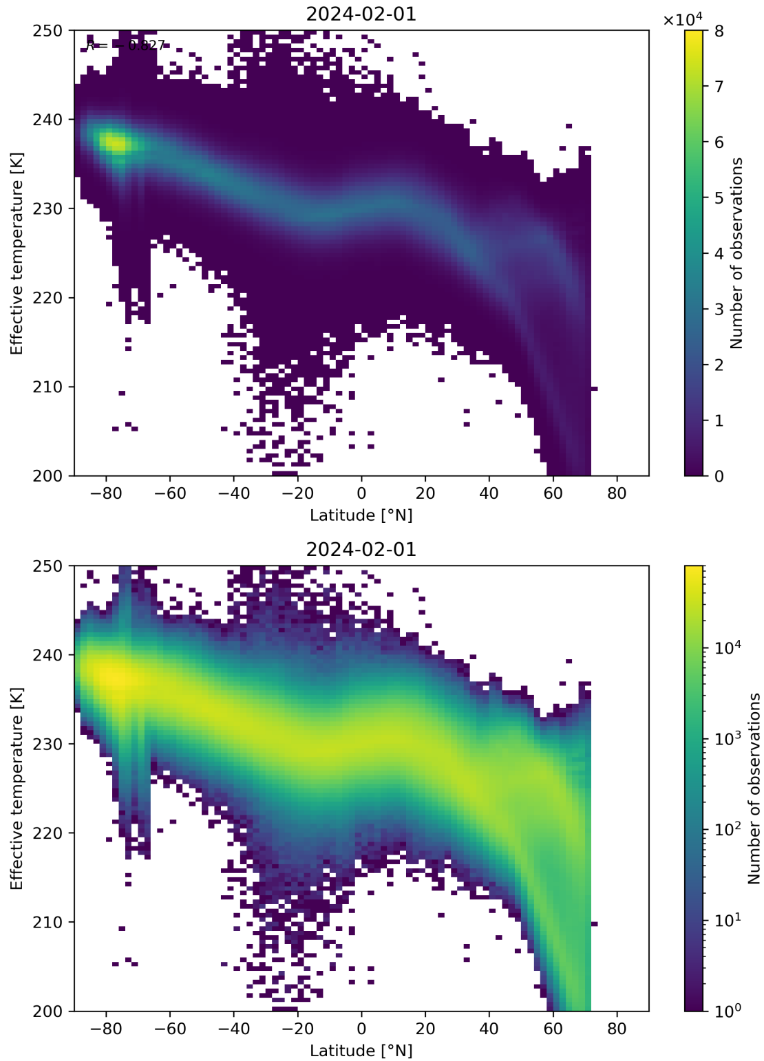
Figure 34: Scatter density plot of “Latitude” against “Effective temperature” for 2024-01-31 to 2024-02-02.
