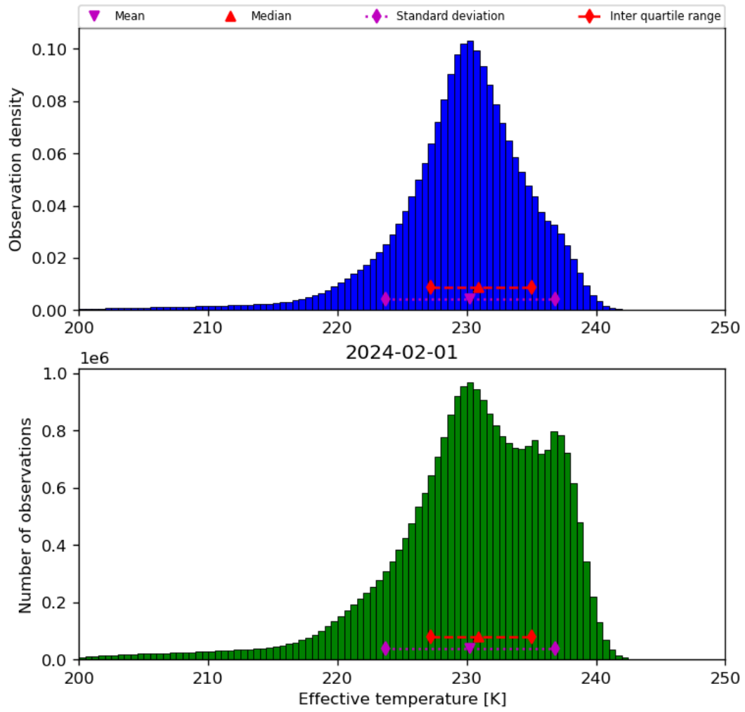
Figure 24: Histogram of “Effective temperature” for 2024-01-31 to 2024-02-02
