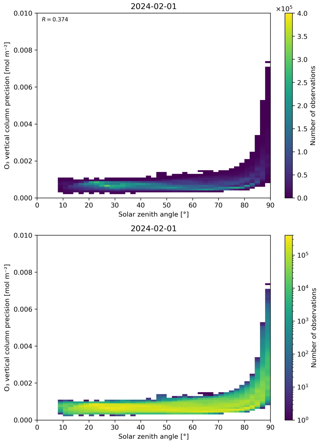
Figure 48: Scatter density plot of “Solar zenith angle” against “O 3 vertical column precision” for 2024-01-31 to 2024-02-02.
