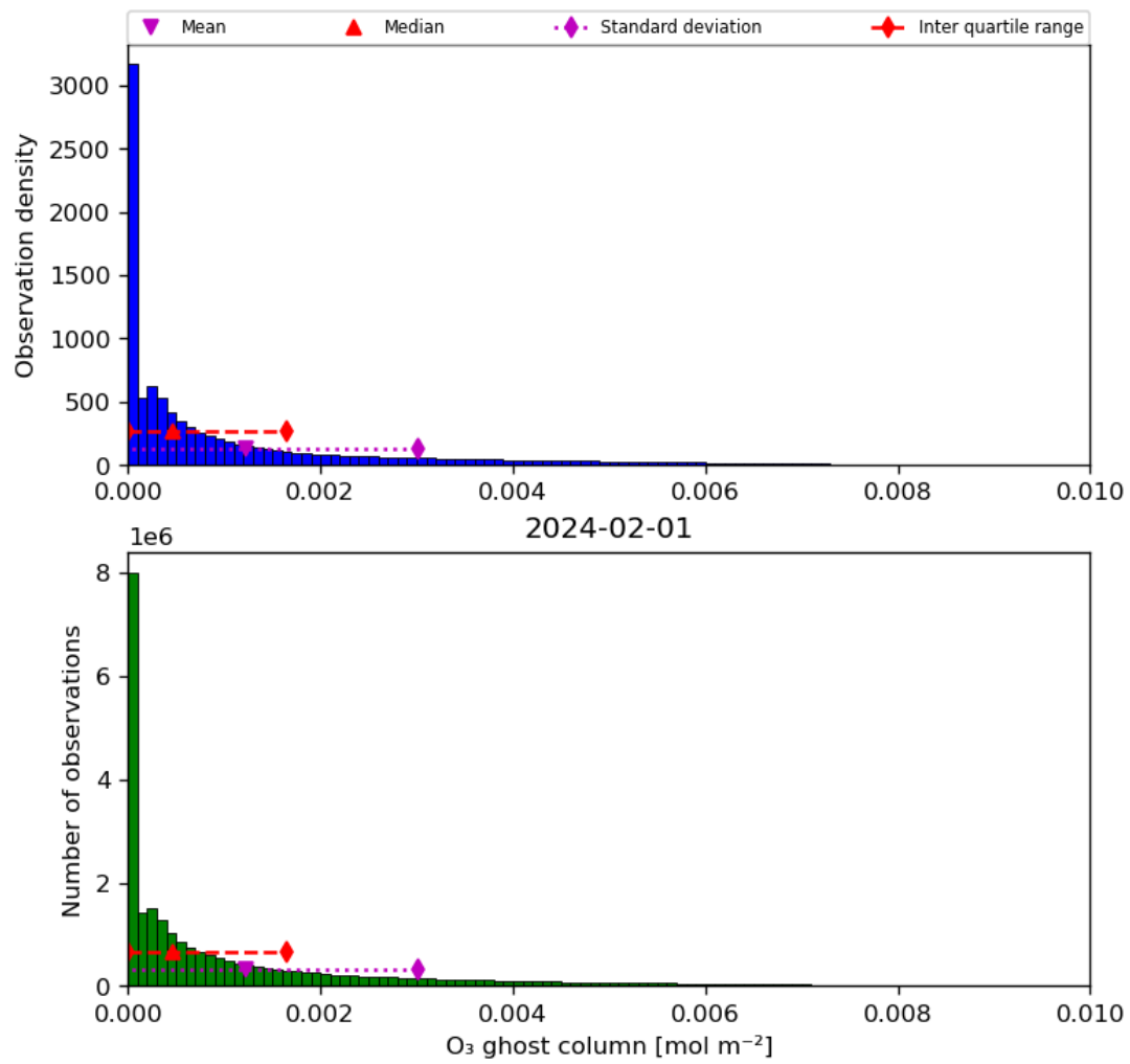
Figure 25: Histogram of “O 3 ghost column” for 2024-01-31 to 2024-02-02
