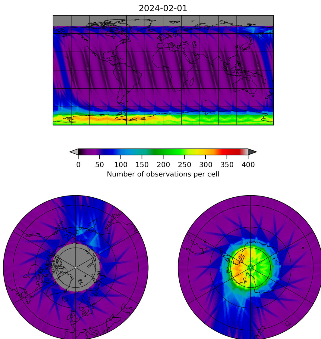
Figure 12: Map of the number of observations for 2024-01-31 to 2024-02-02
