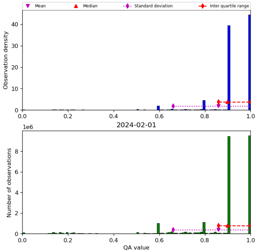
Figure 20: Histogram of “QA value” for 2024-01-31 to 2024-02-02
