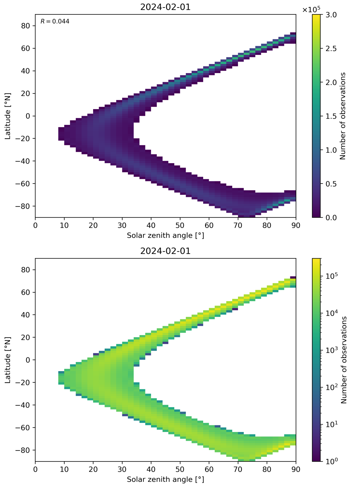
Figure 44: Scatter density plot of “Solar zenith angle” against “Latitude” for 2024-01-31 to 2024-02-02.
