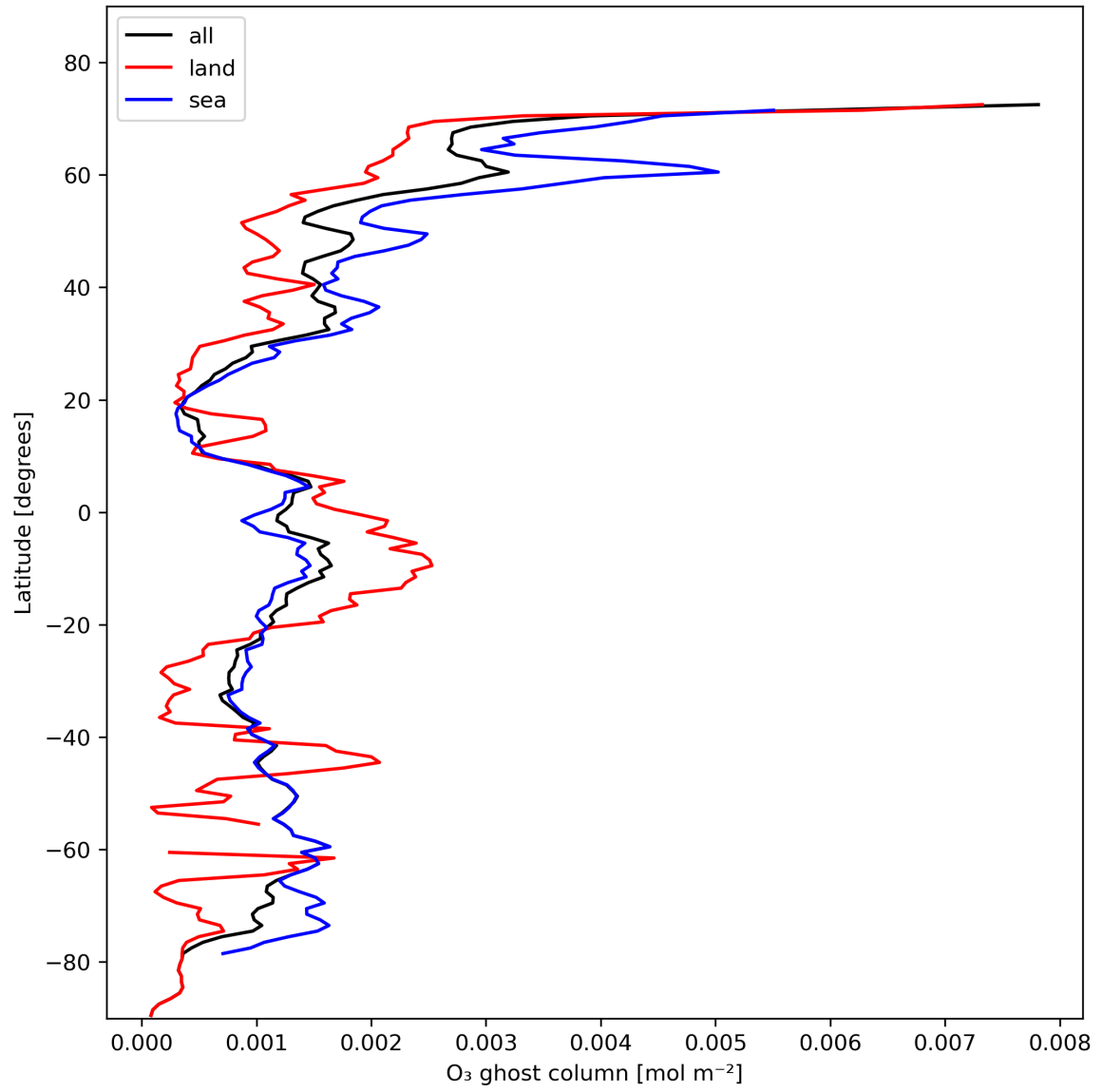
Figure 18: Zonal average of “O 3 ghost column” for 2024-01-31 to 2024-02-02.
