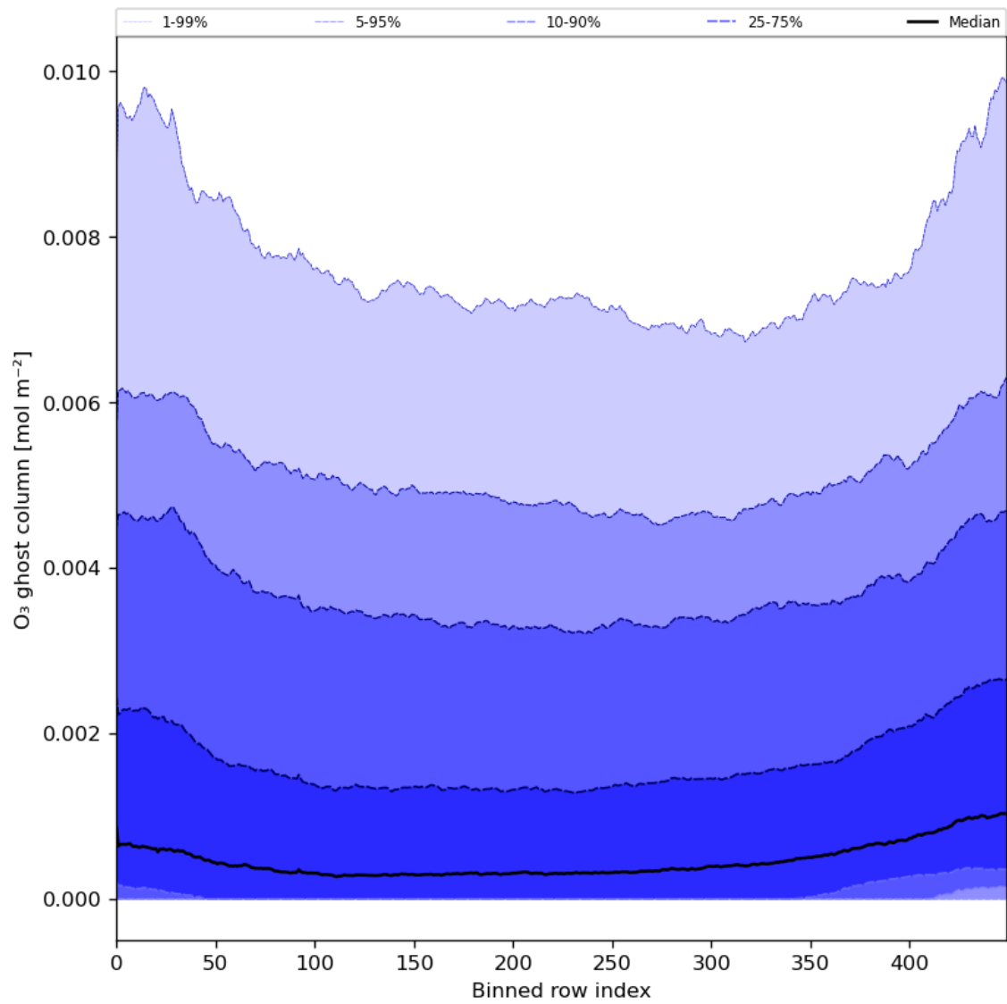
Figure 32: Along track statistics of "O 3 ghost column" for 2024-01-31 to 2024-02-02
