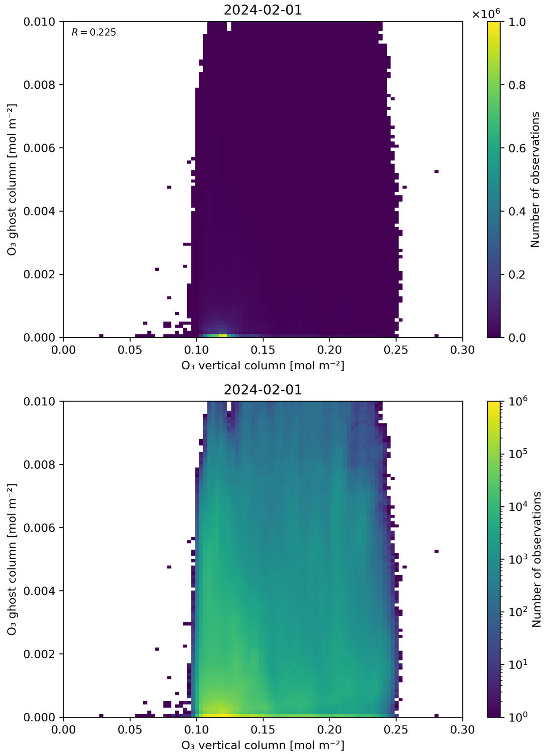
Figure 40: Scatter density plot of “O 3 vertical column” against “O 3 ghost column” for 2024-01-31 to 2024-02-02.
