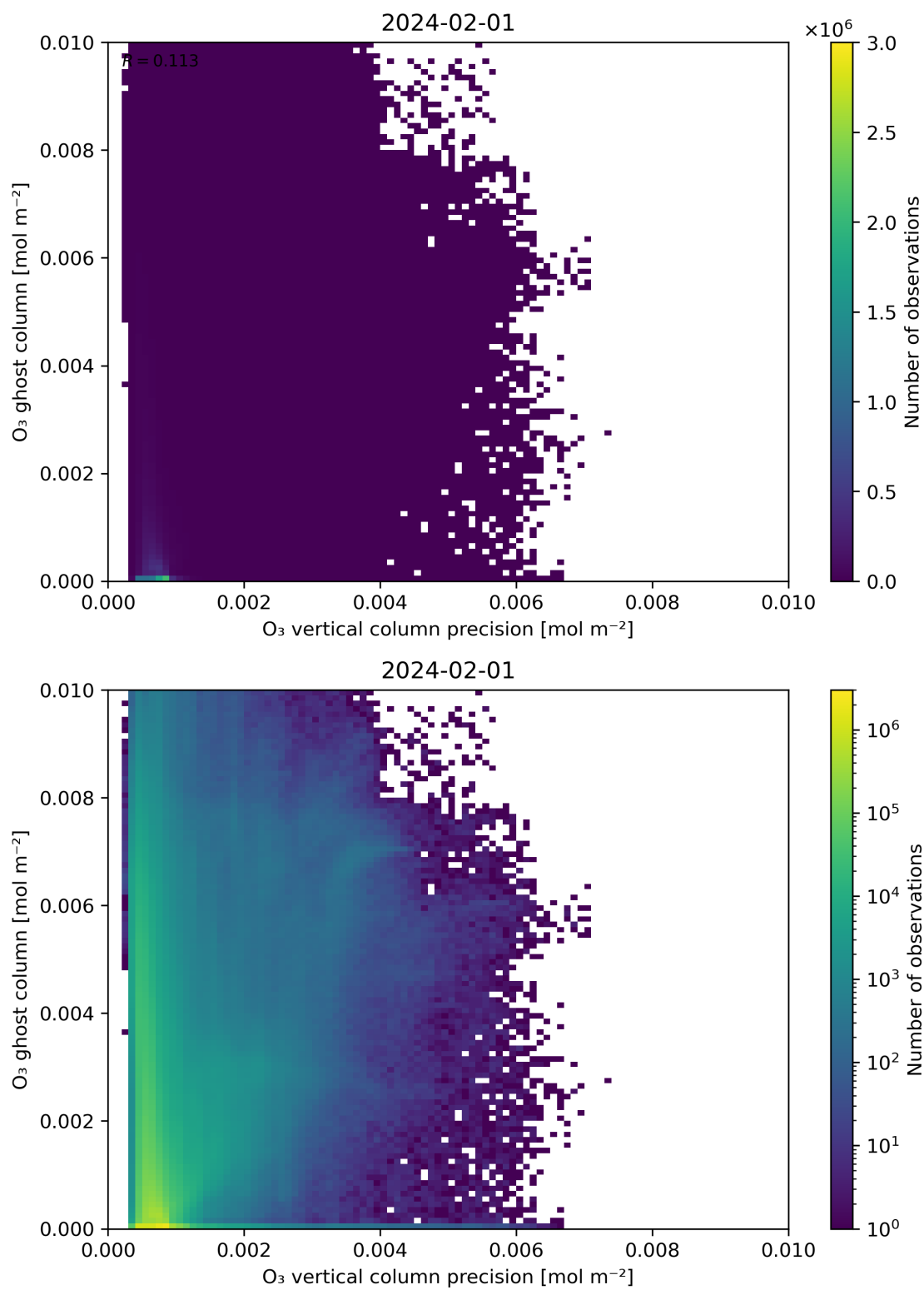
Figure 43: Scatter density plot of “O 3 vertical column precision” against “O 3 ghost column” for 2024-01-31 to 2024-02-02.
