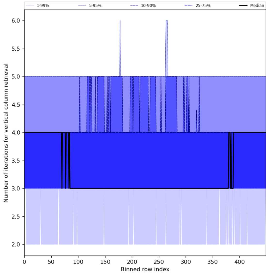
Figure 33: Along track statistics of “Number of iterations for vertical column retrieval” for 2024-01-31 to 2024-02-02
