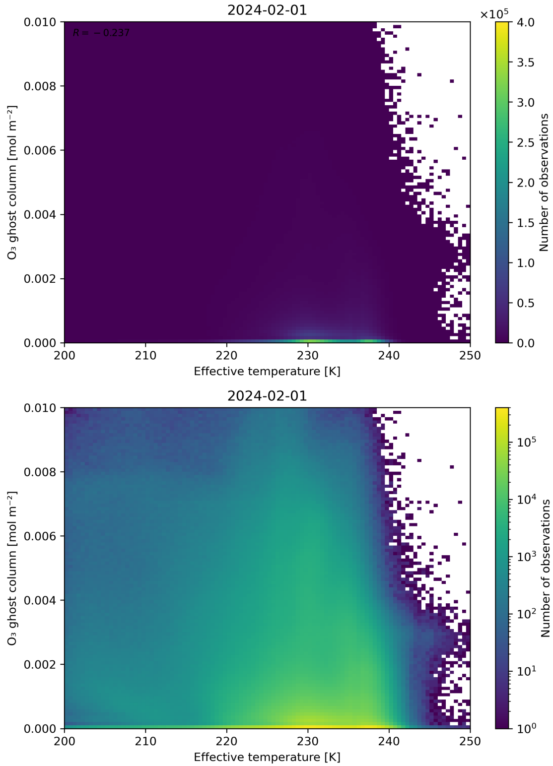
Figure 38: Scatter density plot of “Effective temperature” against “O 3 ghost column” for 2024-01-31 to 2024-02-02.
