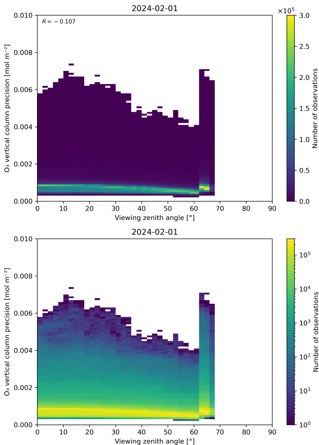
Figure 53: Scatter density plot of “Viewing zenith angle” against “O 3 vertical column precision” for 2024-01-31 to 2024-02-02.
