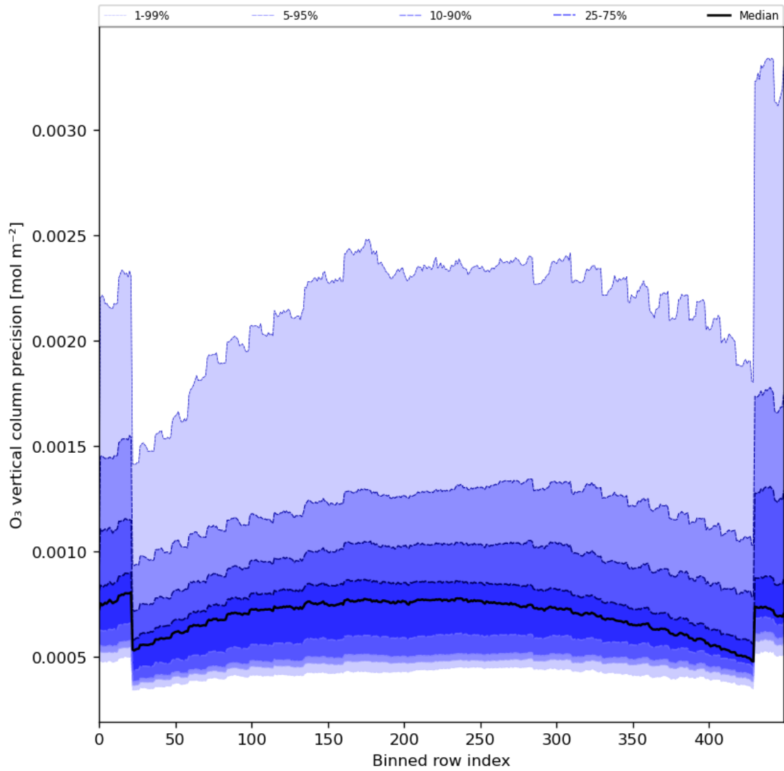
Figure 29: Along track statistics of “O 3 vertical column precision” for 2024-01-31 to 2024-02-02
