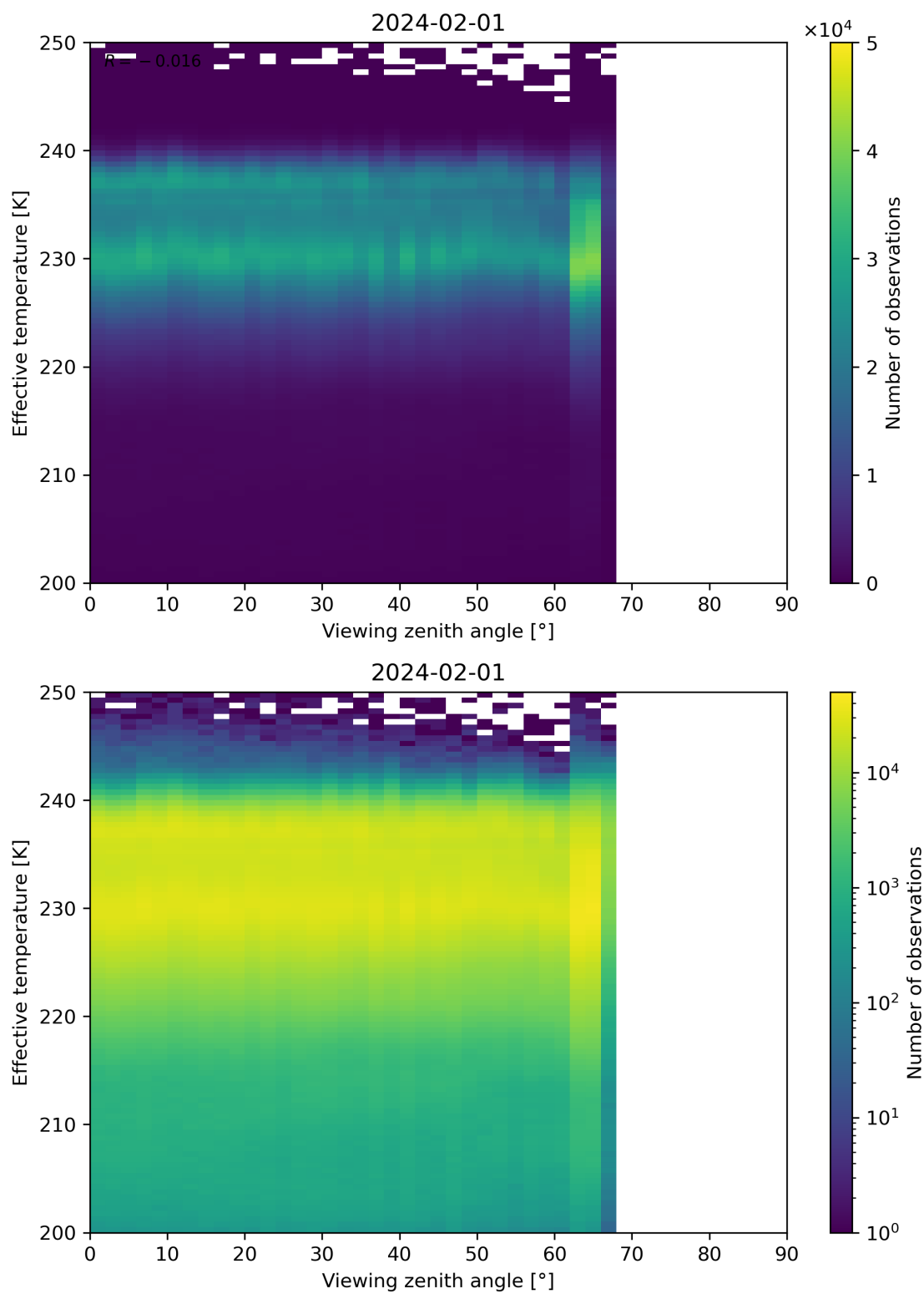
Figure 50: Scatter density plot of “Viewing zenith angle” against “Effective temperature” for 2024-01-31 to 2024-02-02.
