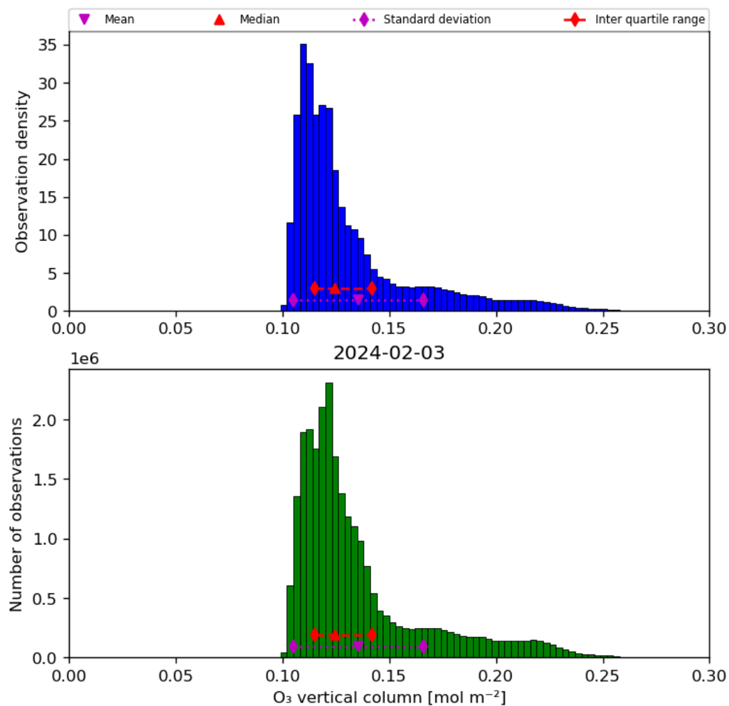
Figure 21: Histogram of “O 3 vertical column” for 2024-02-02 to 2024-02-04
