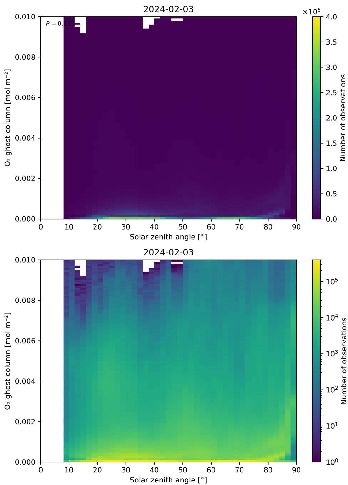
Figure 46: Scatter density plot of “Solar zenith angle” against “O 3 ghost column” for 2024-02-02 to 2024-02-04.
