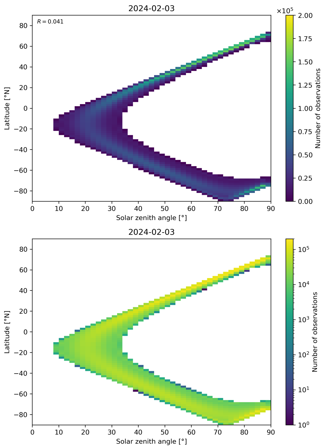
Figure 44: Scatter density plot of “Solar zenith angle” against “Latitude” for 2024-02-02 to 2024-02-04.
