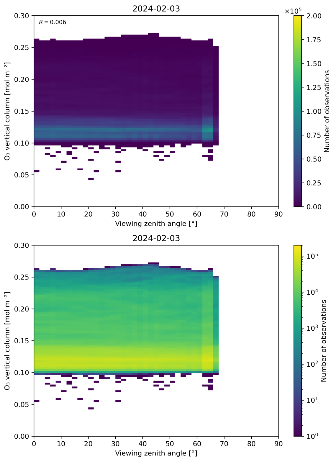
Figure 52: Scatter density plot of “Viewing zenith angle” against “O 3 vertical column” for 2024-02-02 to 2024-02-04.
