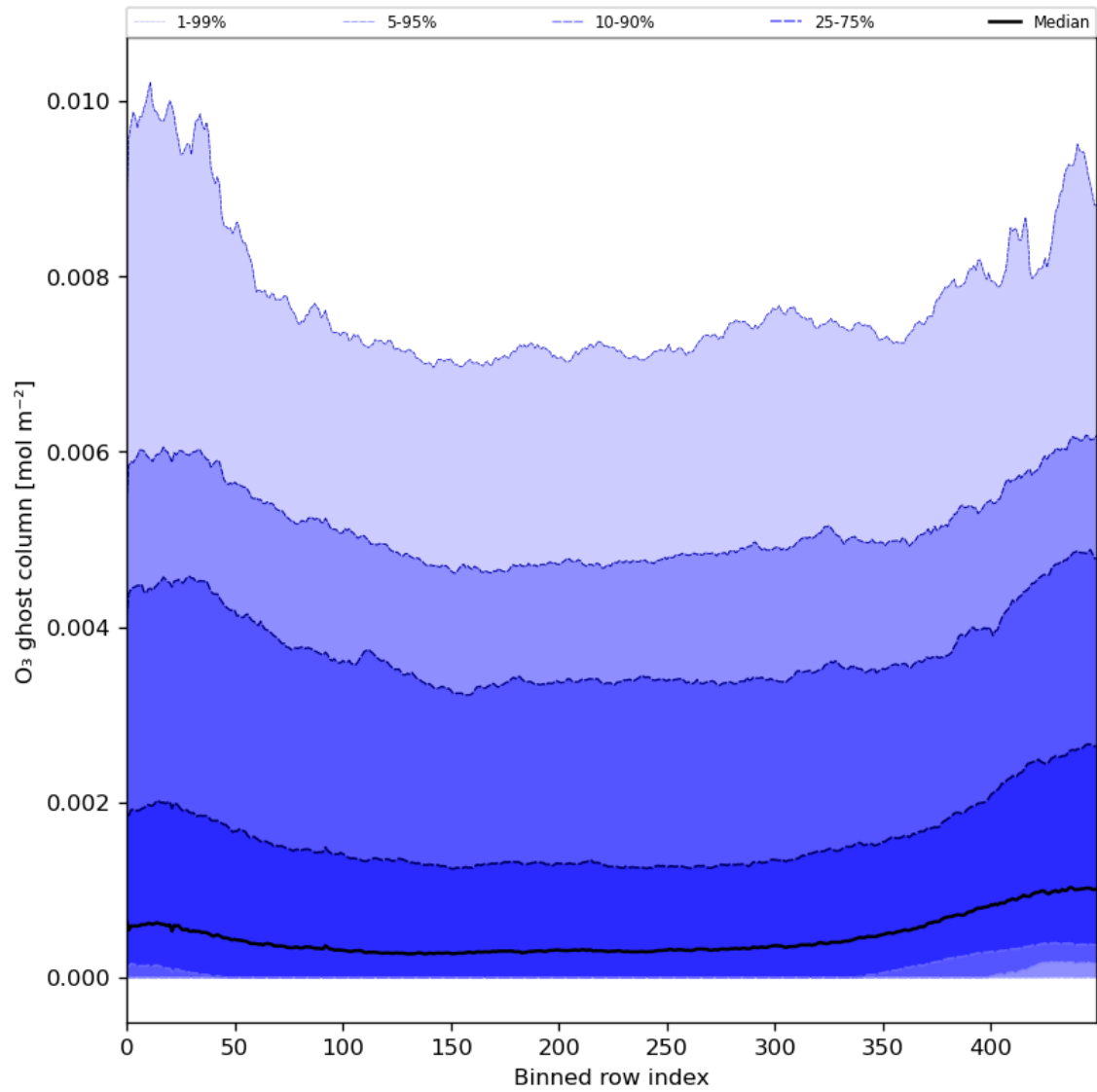
Figure 32: Along track statistics of “O 3 ghost column” for 2024-02-02 to 2024-02-04
