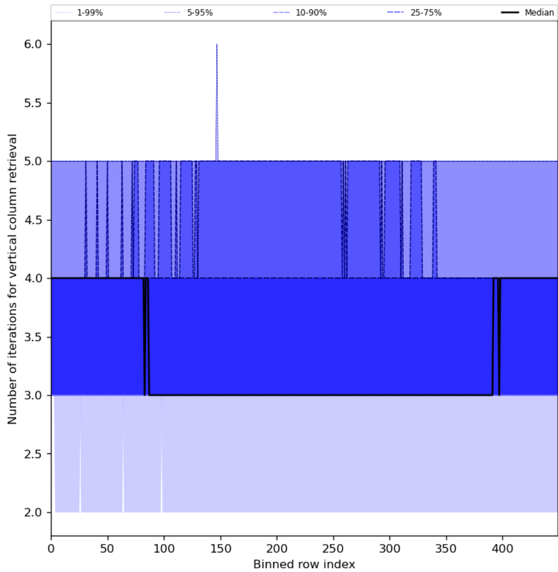
Figure 33: Along track statistics of “Number of iterations for vertical column retrieval” for 2024-02-02 to 2024-02-04
