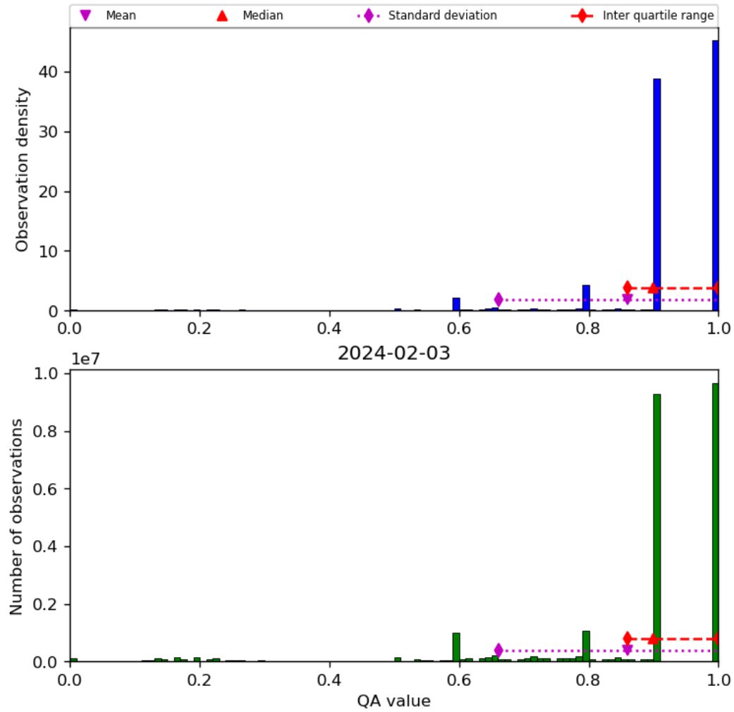
Figure 20: Histogram of “QA value” for 2024-02-02 to 2024-02-04
