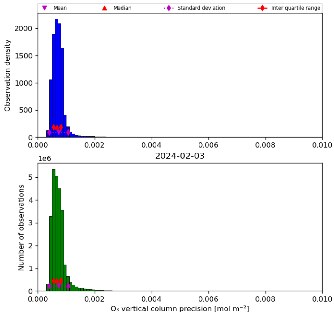
Figure 22: Histogram of “O 3 vertical column precision” for 2024-02-02 to 2024-02-04
