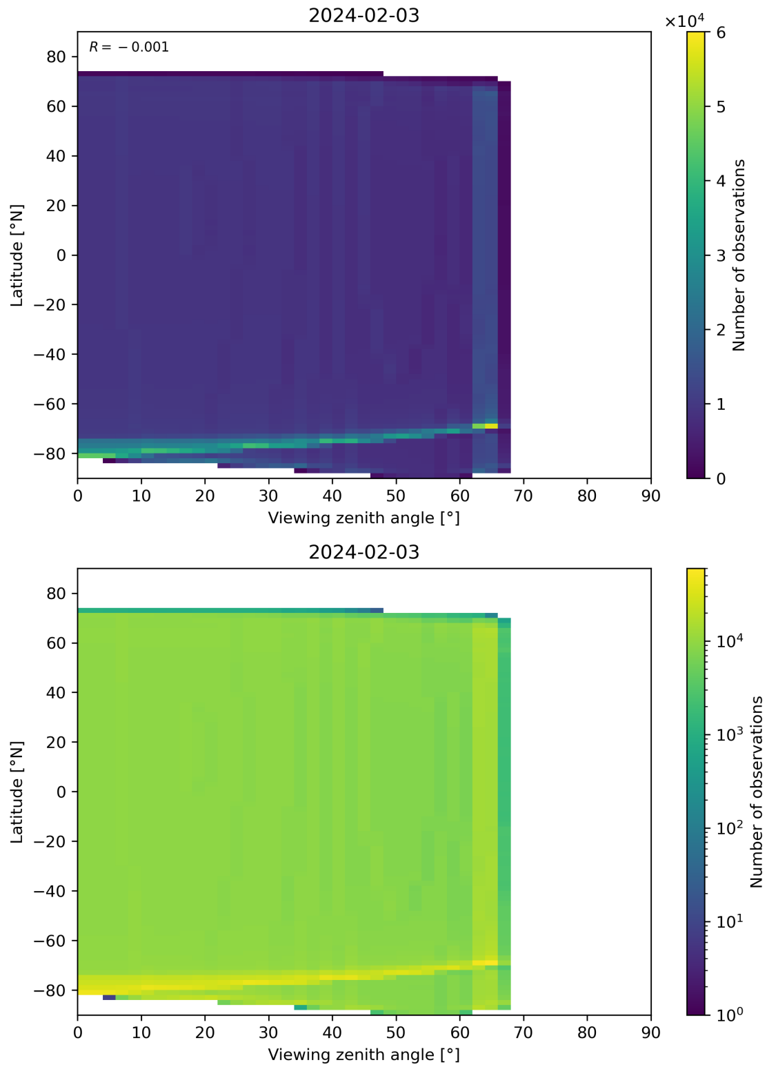
Figure 49: Scatter density plot of “Viewing zenith angle” against “Latitude” for 2024-02-02 to 2024-02-04.
