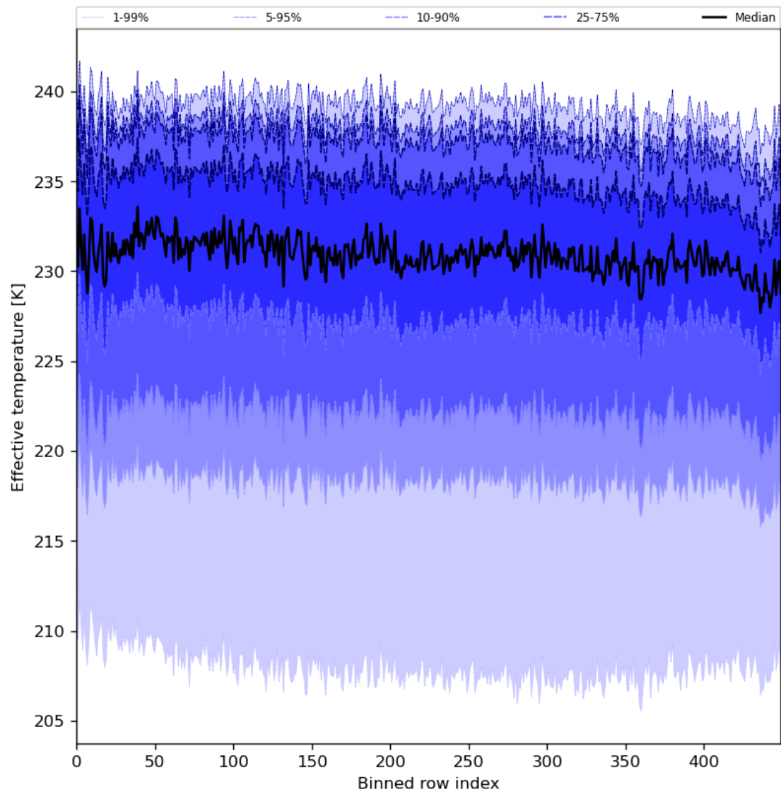
Figure 31: Along track statistics of “Effective temperature” for 2024-02-02 to 2024-02-04
