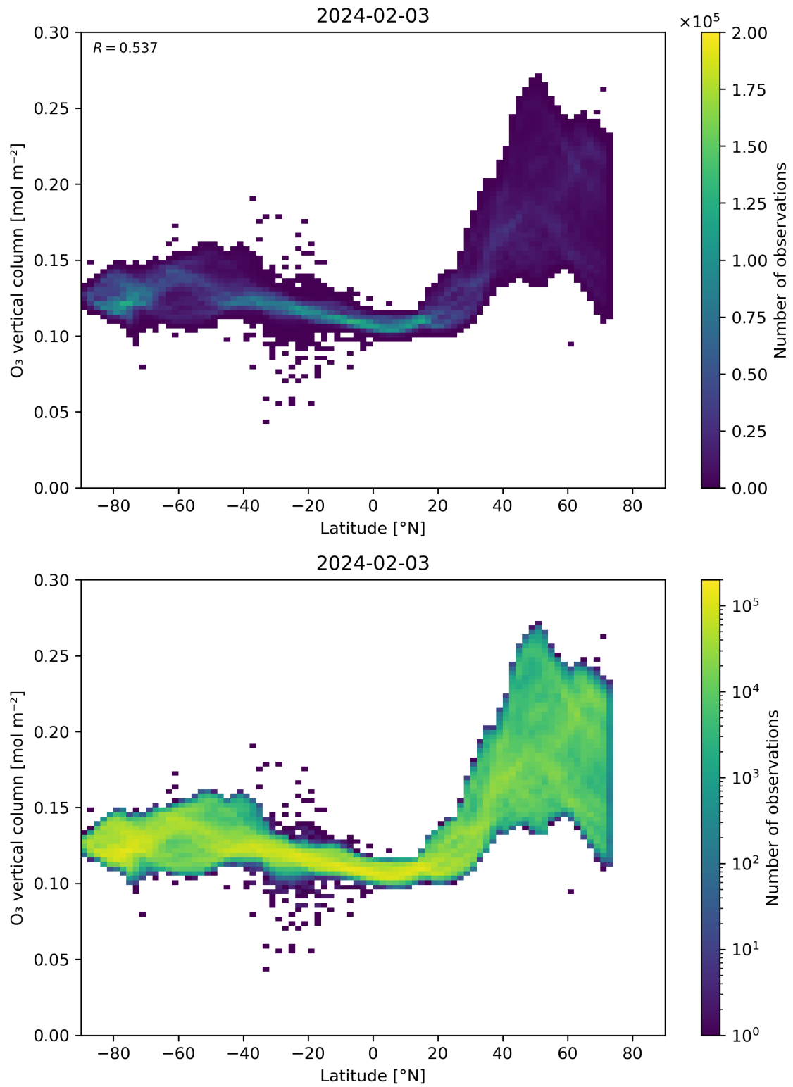
Figure 36: Scatter density plot of “Latitude” against “O 3 vertical column” for 2024-02-02 to 2024-02-04.
