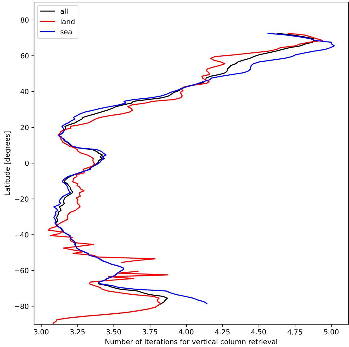
Figure 19: Zonal average of “Number of iterations for vertical column retrieval” for 2024-02-02 to 2024-02-04.
