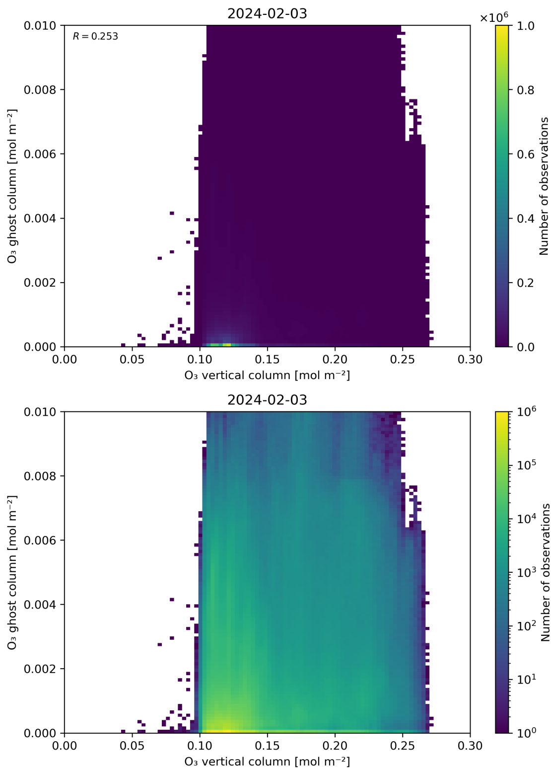
Figure 40: Scatter density plot of “O 3 vertical column” against “O 3 ghost column” for 2024-02-02 to 2024-02-04.
