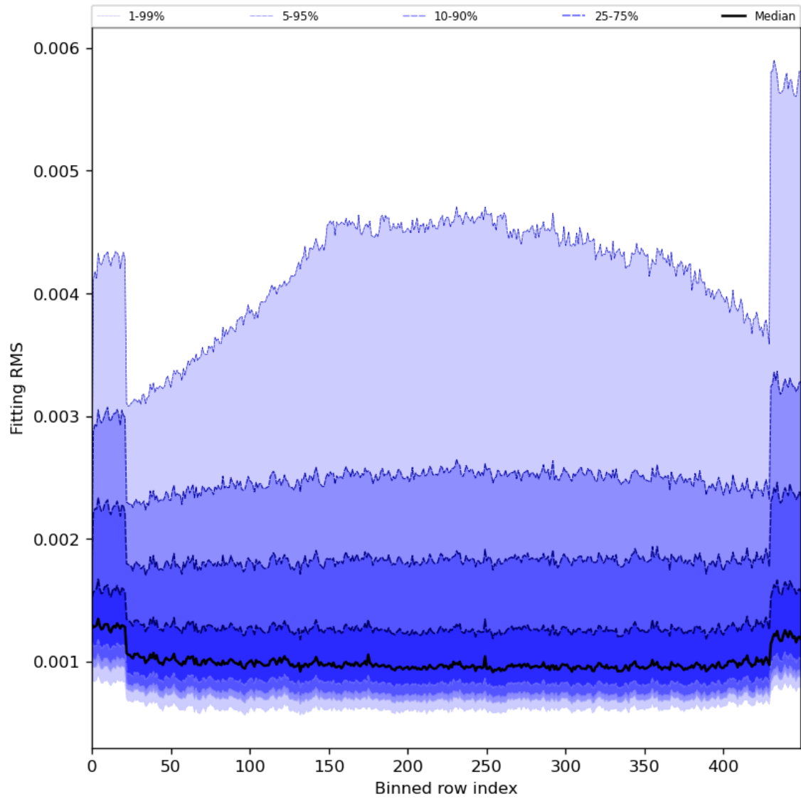
Figure 30: Along track statistics of “Fitting RMS” for 2024-02-02 to 2024-02-04
