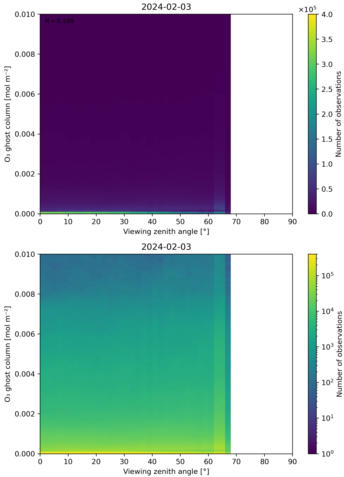
Figure 51: Scatter density plot of “Viewing zenith angle” against “O 3 ghost column” for 2024-02-02 to 2024-02-04.
