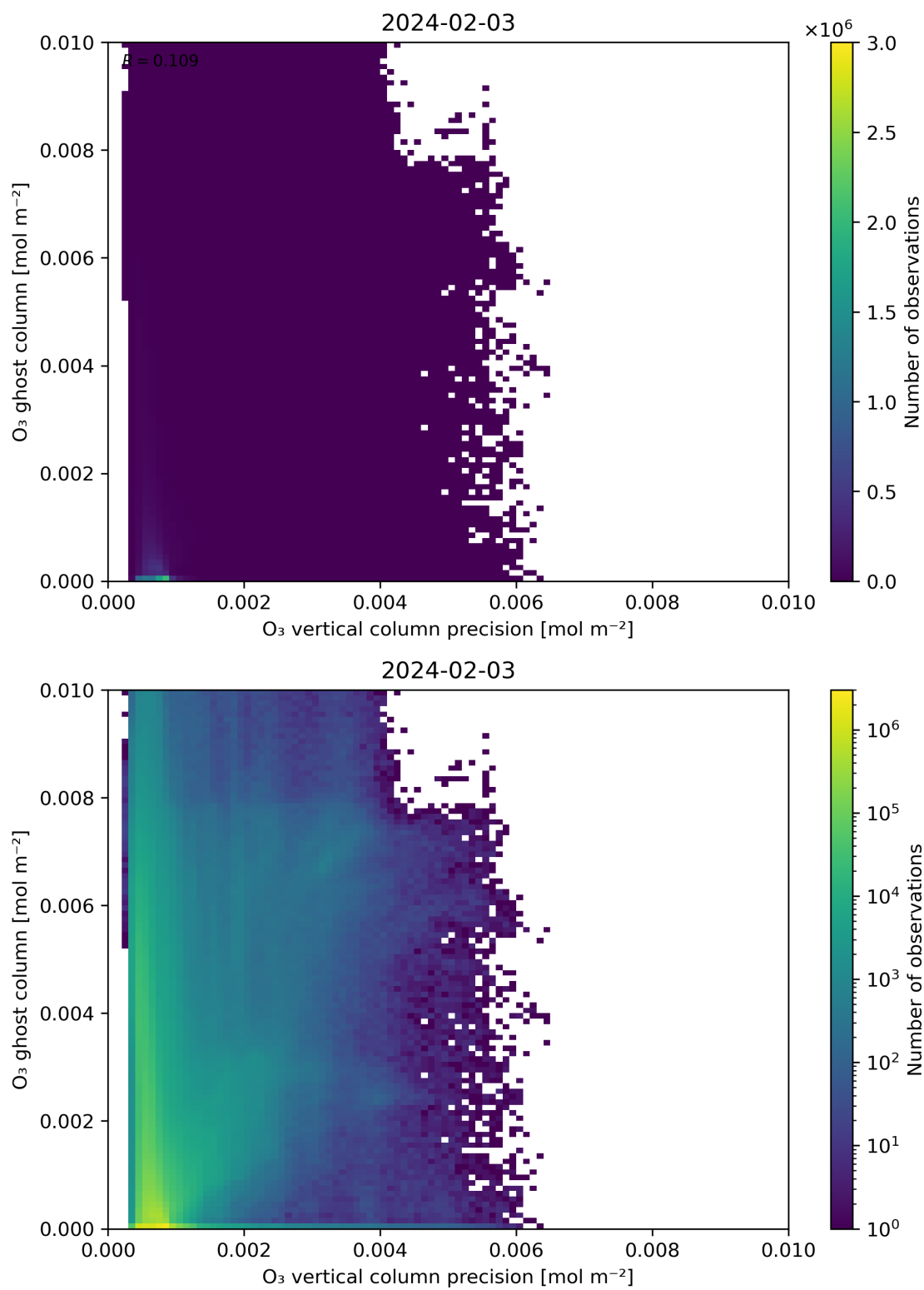
Figure 43: Scatter density plot of “O 3 vertical column precision” against “O 3 ghost column” for 2024-02-02 to 2024-02-04.
