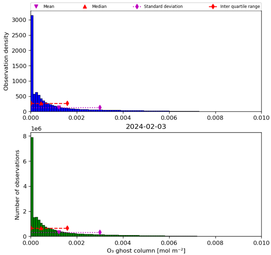
Figure 25: Histogram of “O 3 ghost column” for 2024-02-02 to 2024-02-04
