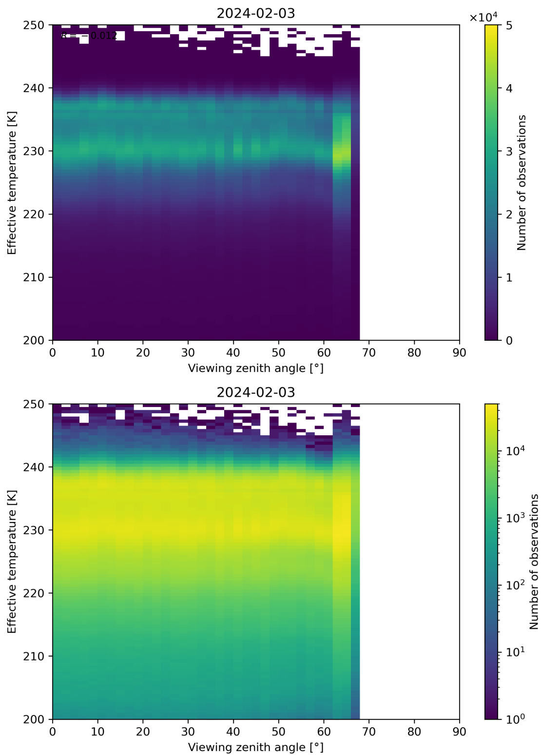
Figure 50: Scatter density plot of “Viewing zenith angle” against “Effective temperature” for 2024-02-02 to 2024-02-04.
