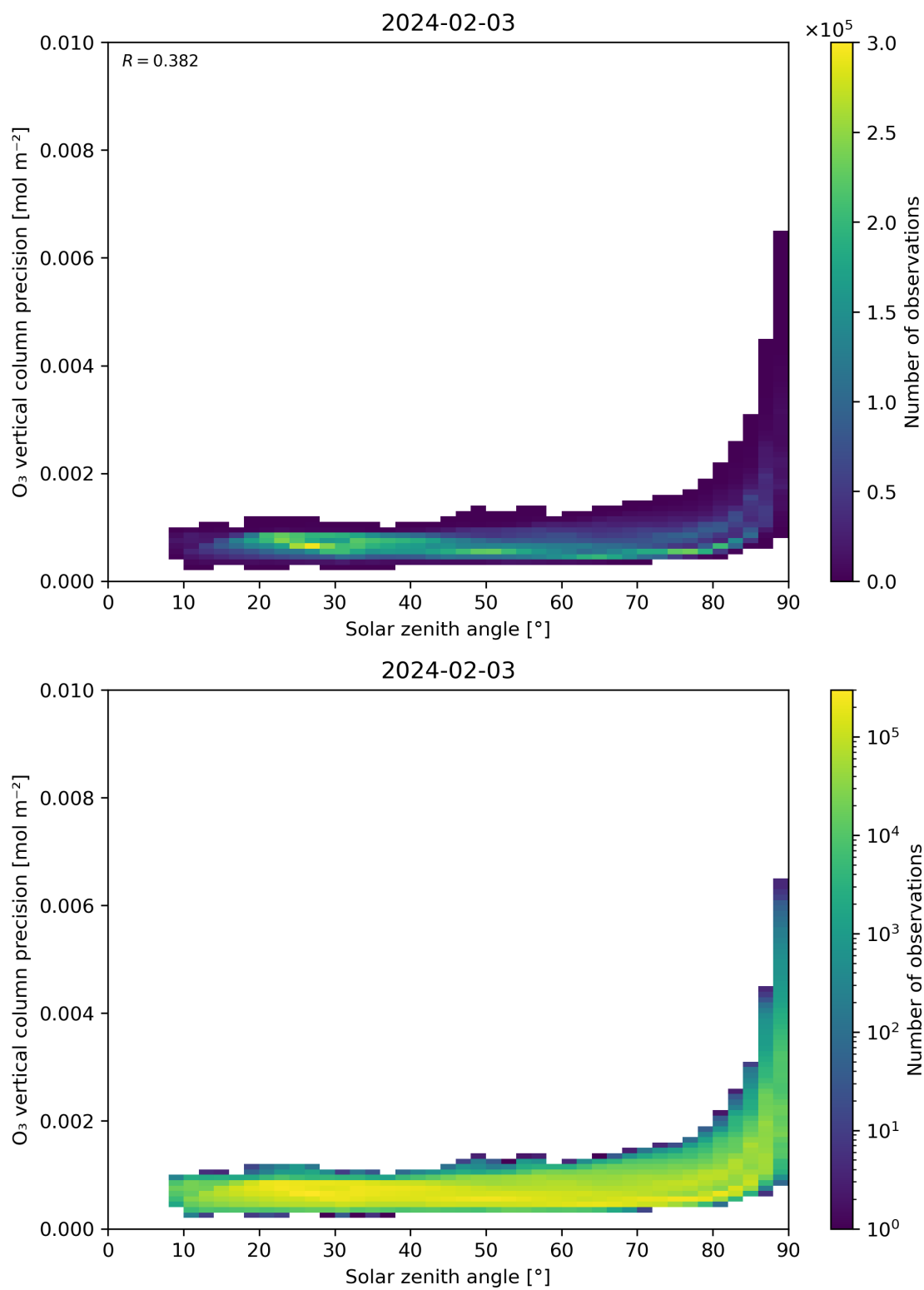
Figure 48: Scatter density plot of “Solar zenith angle” against “O 3 vertical column precision” for 2024-02-02 to 2024-02-04.
