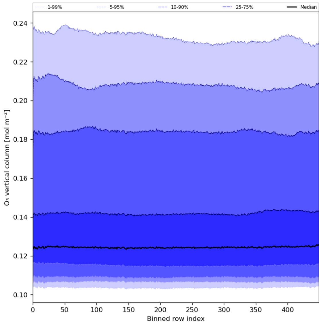
Figure 28: Along track statistics of “O 3 vertical column” for 2024-02-02 to 2024-02-04
