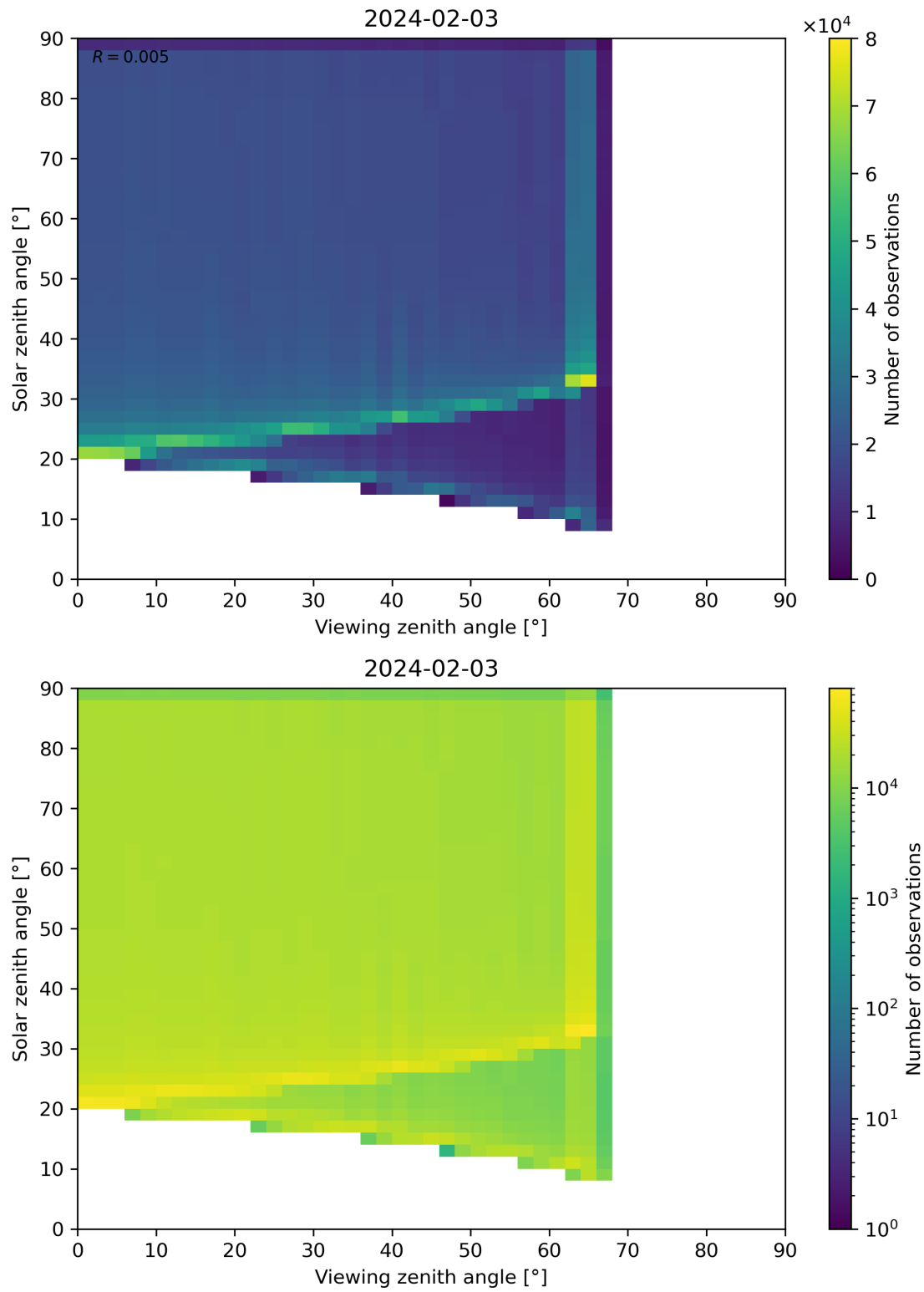
Figure 54: Scatter density plot of “Viewing zenith angle” against “Solar zenith angle” for 2024-02-02 to 2024-02-04.
