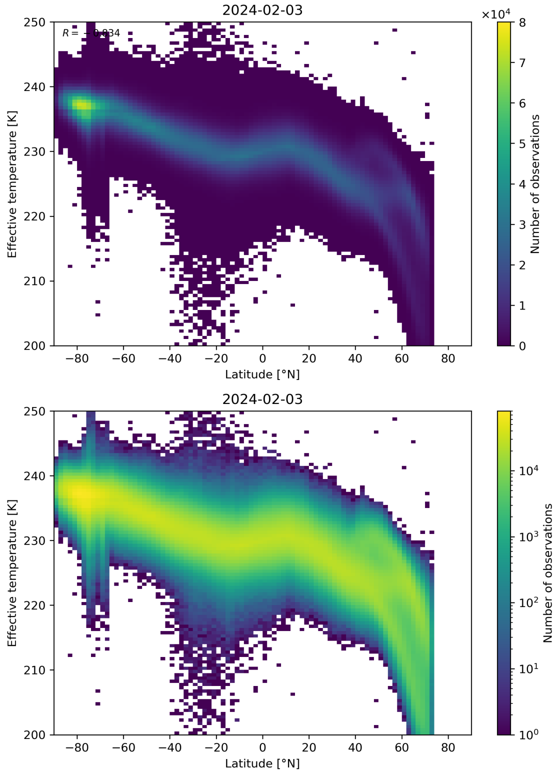
Figure 34: Scatter density plot of “Latitude” against “Effective temperature” for 2024-02-02 to 2024-02-04.
