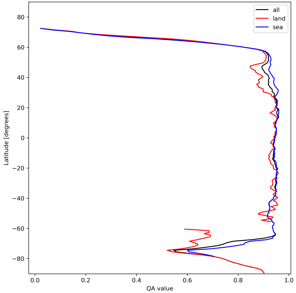
Figure 13: Zonal average of “QA value” for 2024-02-02 to 2024-02-04.
