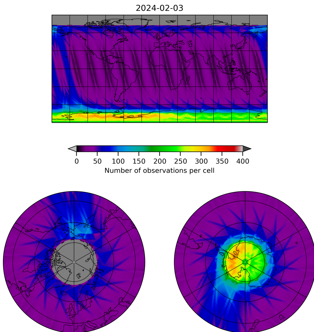
Figure 12: Map of the number of observations for 2024-02-02 to 2024-02-04
