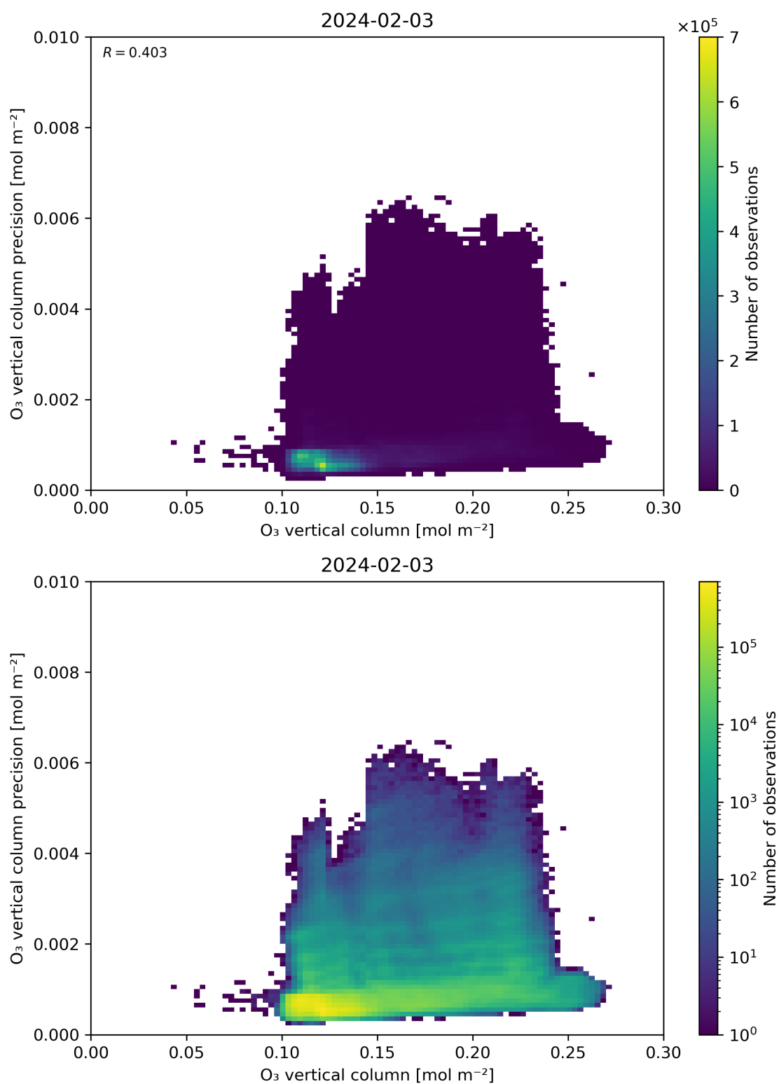
Figure 41: Scatter density plot of “O 3 vertical column” against “O 3 vertical column precision” for 2024-02-02 to 2024-02-04.
