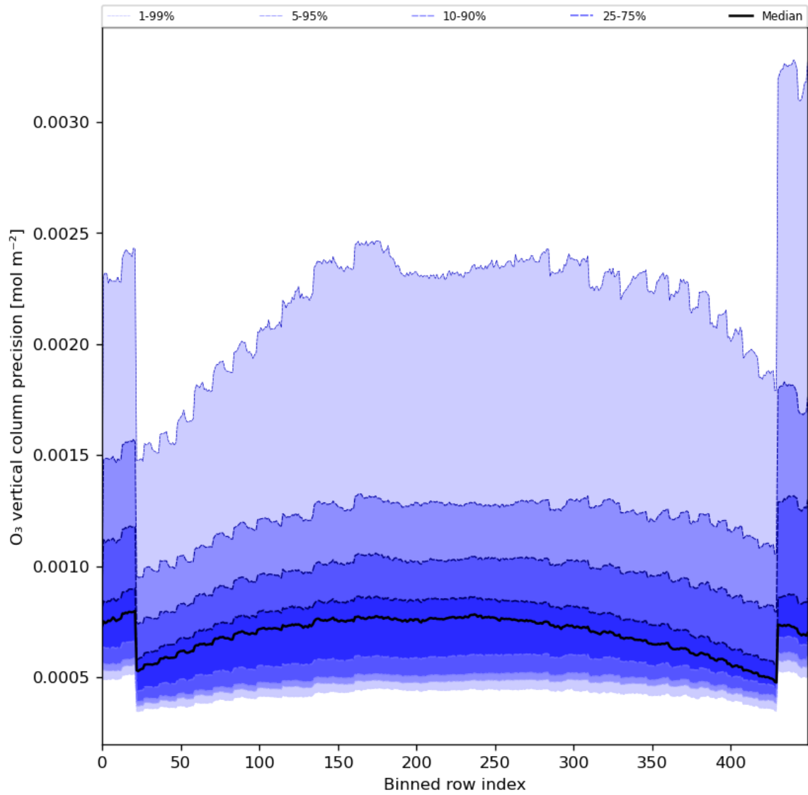
Figure 29: Along track statistics of “O 3 vertical column precision” for 2024-02-02 to 2024-02-04
