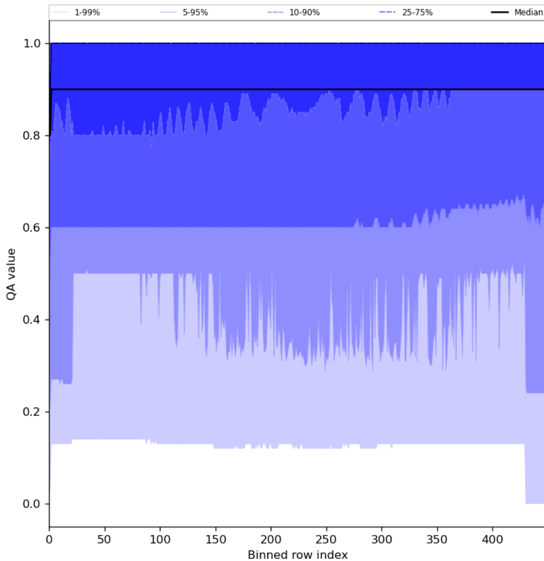
Figure 27: Along track statistics of “QA value” for 2024-02-02 to 2024-02-04
