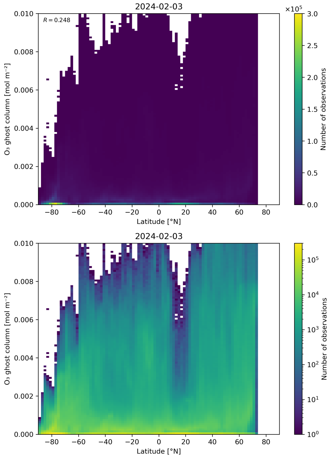
Figure 35: Scatter density plot of “Latitude” against “O 3 ghost column” for 2024-02-02 to 2024-02-04.
