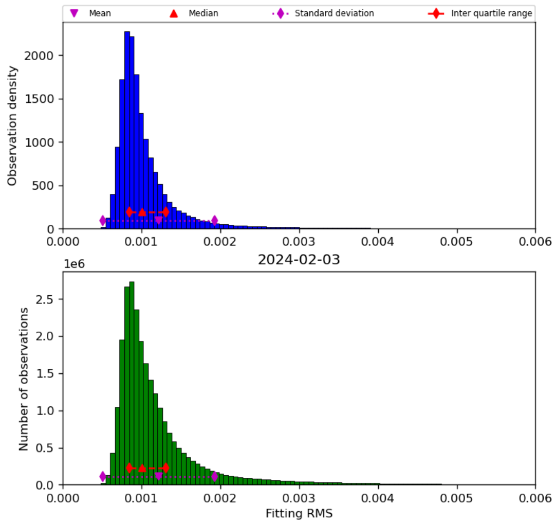
Figure 23: Histogram of “Fitting RMS” for 2024-02-02 to 2024-02-04
