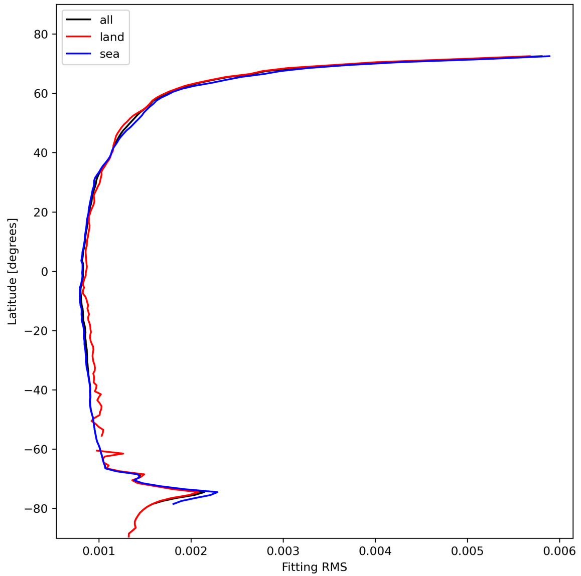
Figure 16: Zonal average of “Fitting RMS” for 2024-02-02 to 2024-02-04.
