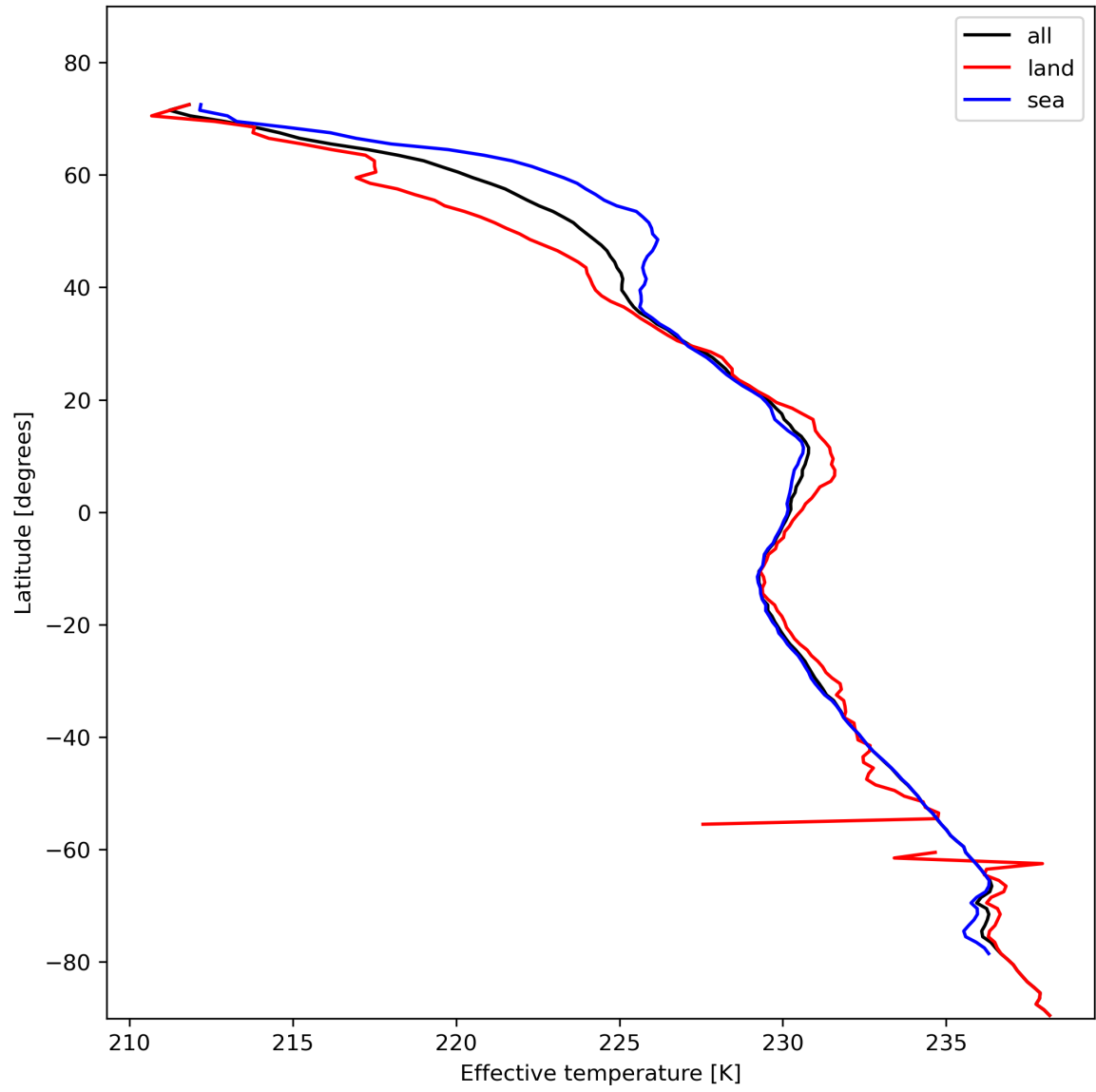
Figure 17: Zonal average of "Effective temperature" for 2024-02-02 to 2024-02-04.
