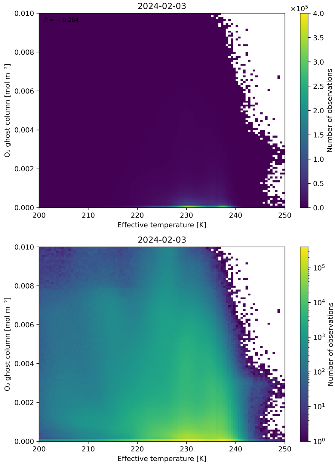
Figure 38: Scatter density plot of “Effective temperature” against “O 3 ghost column” for 2024-02-02 to 2024-02-04.
