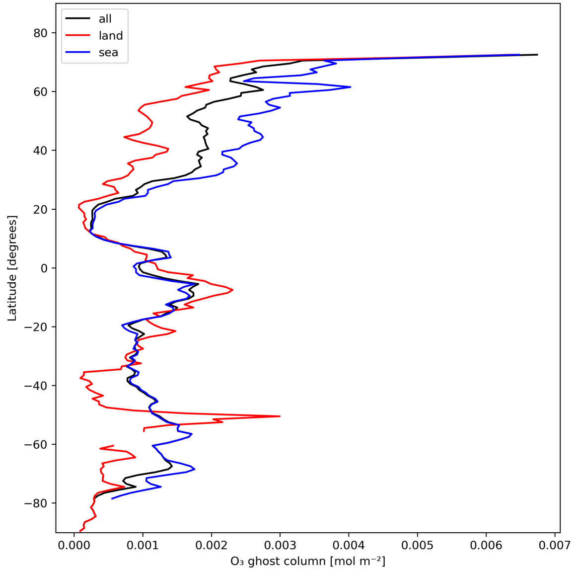
Figure 18: Zonal average of "O 3 ghost column" for 2024-02-02 to 2024-02-04.
