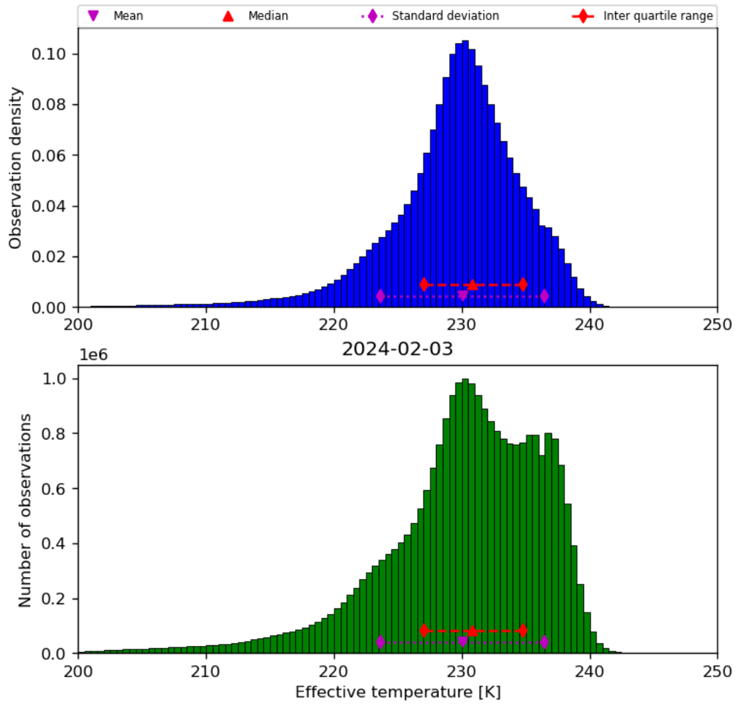
Figure 24: Histogram of “Effective temperature” for 2024-02-02 to 2024-02-04
