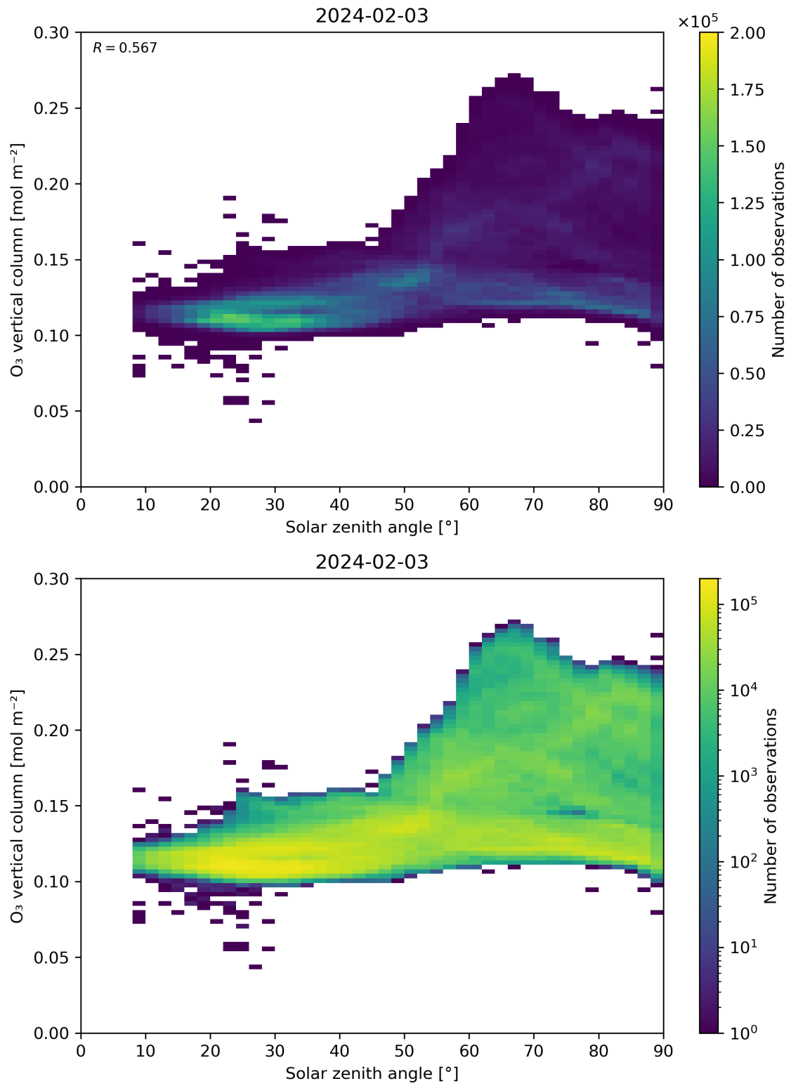
Figure 47: Scatter density plot of “Solar zenith angle” against “O 3 vertical column” for 2024-02-02 to 2024-02-04.
