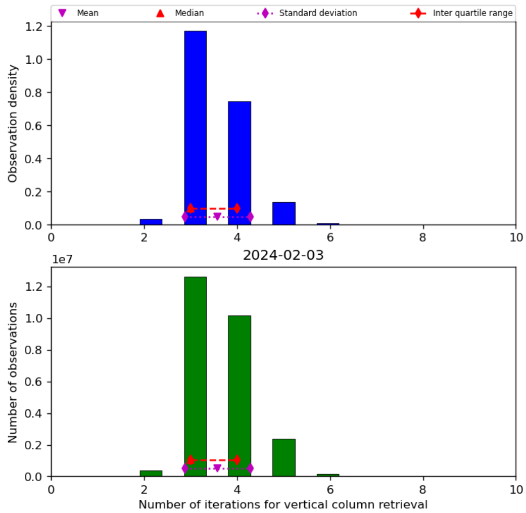
Figure 26: Histogram of “Number of iterations for vertical column retrieval” for 2024-02-02 to 2024-02-04
