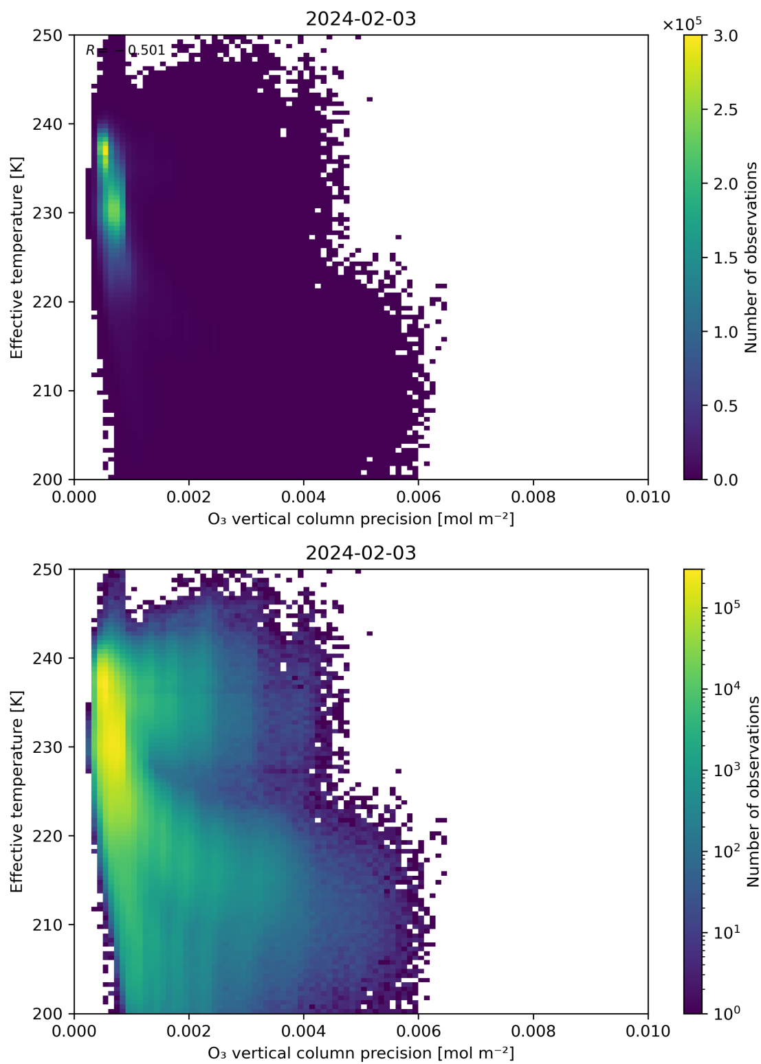
Figure 42: Scatter density plot of “ O_3 vertical column precision” against “Effective temperature” for 2024-02-02 to 2024-02-04.
