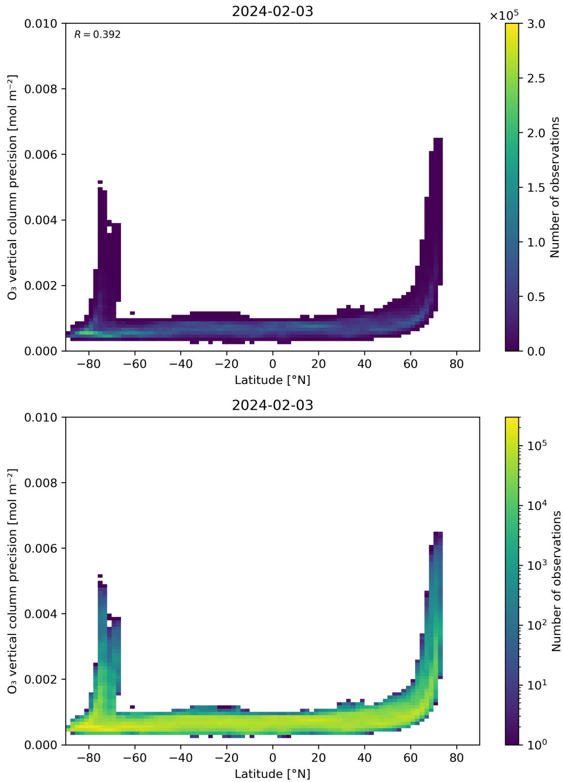
Figure 37: Scatter density plot of “Latitude” against “O 3 vertical column precision” for 2024-02-02 to 2024-02-04.
