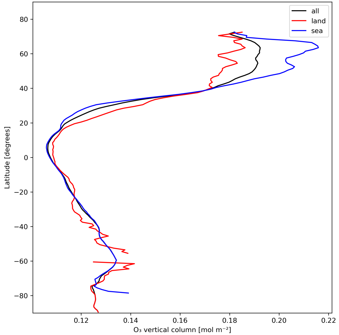
Figure 14: Zonal average of “O 3 vertical column” for 2024-02-02 to 2024-02-04.
