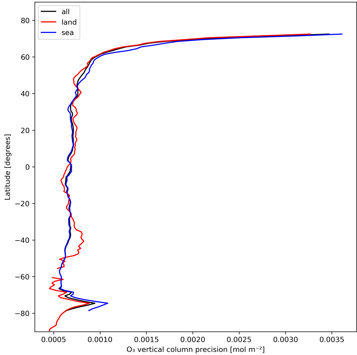
Figure 15: Zonal average of “O 3 vertical column precision” for 2024-02-02 to 2024-02-04.
