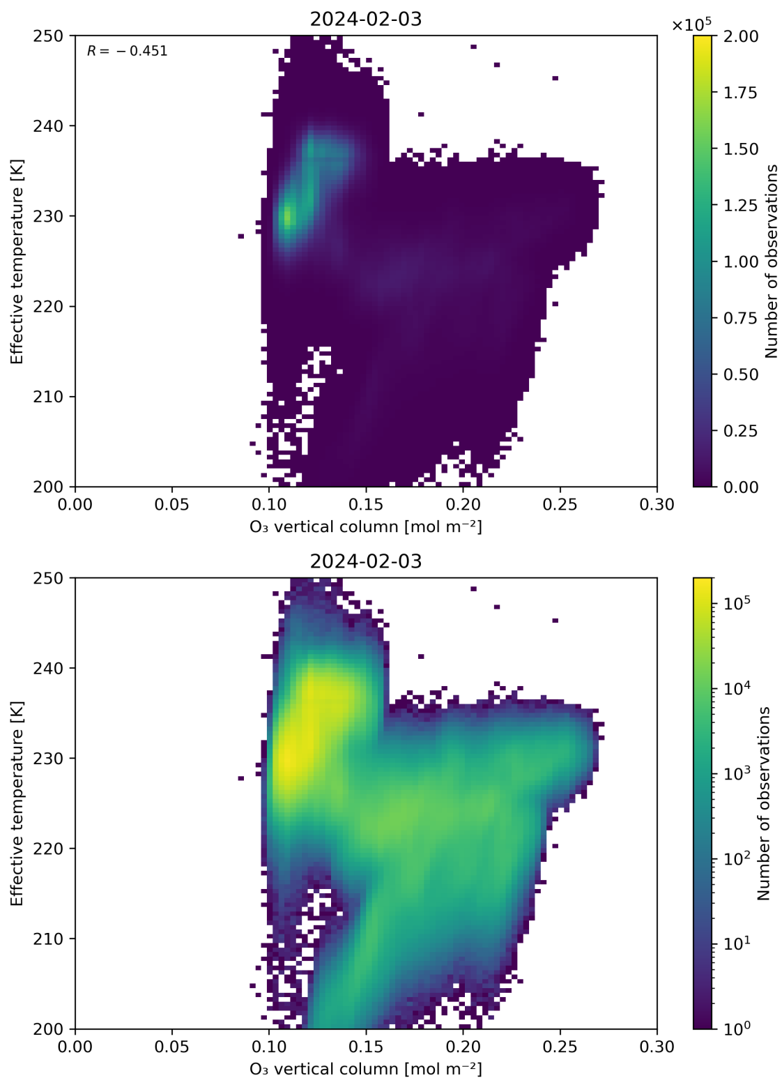
Figure 39: Scatter density plot of “O 3 vertical column” against “Effective temperature” for 2024-02-02 to 2024-02-04.
