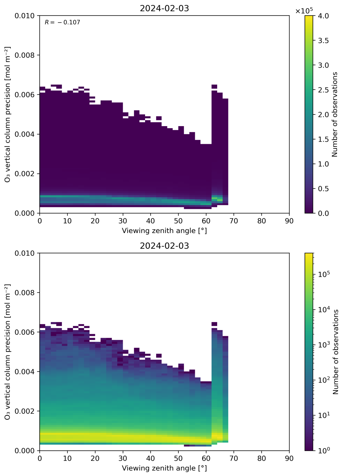
Figure 53: Scatter density plot of “Viewing zenith angle” against “O 3 vertical column precision” for 2024-02-02 to 2024-02-04.
