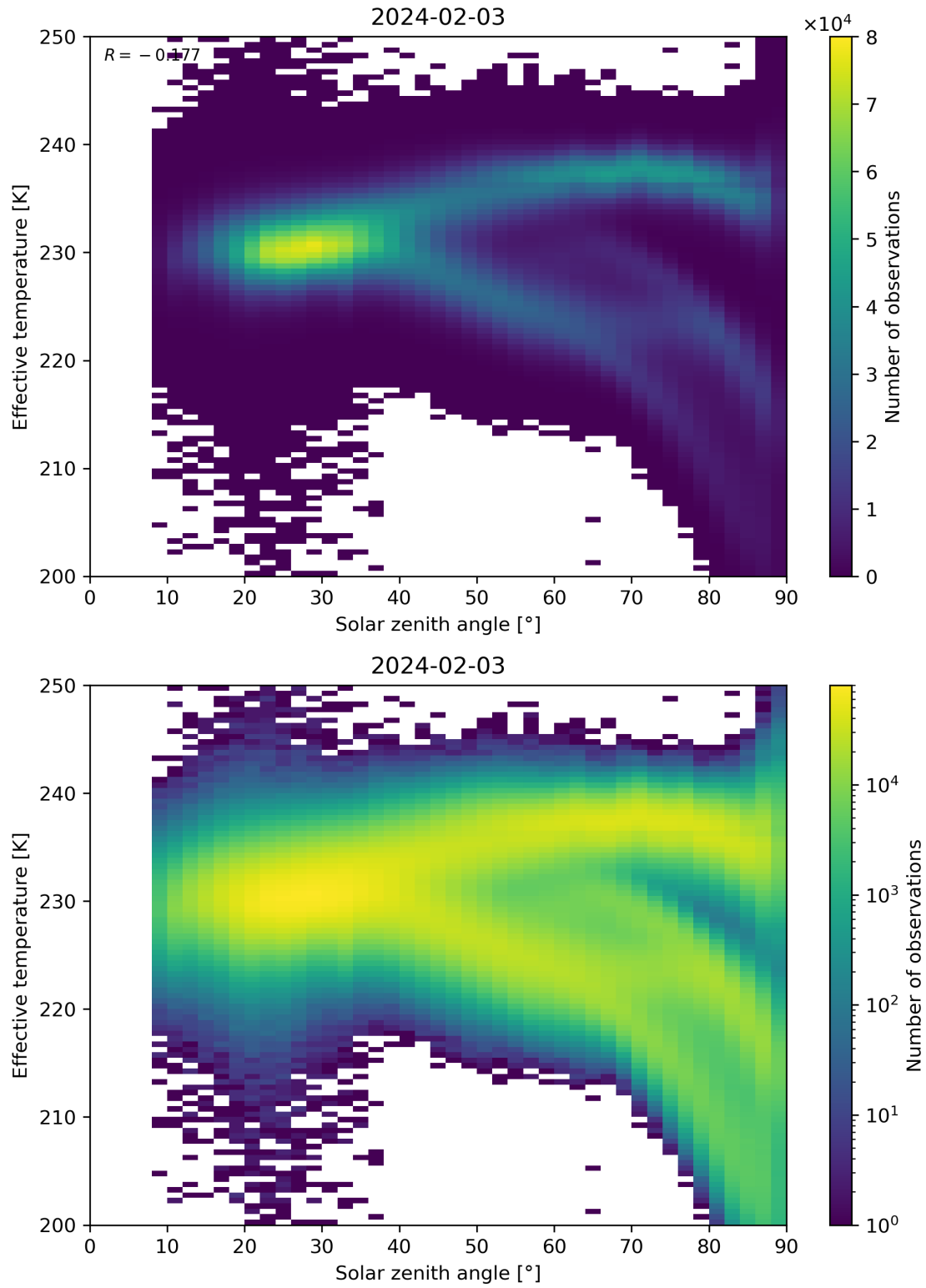
Figure 45: Scatter density plot of “Solar zenith angle” against “Effective temperature” for 2024-02-02 to 2024-02-04.
