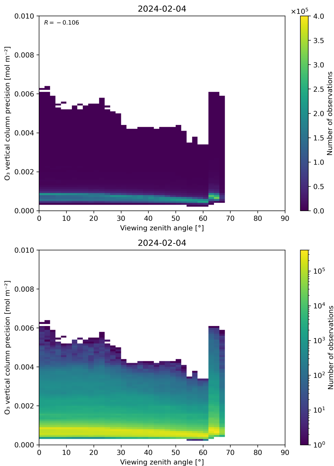
Figure 53: Scatter density plot of “Viewing zenith angle” against “O 3 vertical column precision” for 2024-02-03 to 2024-02-05.
