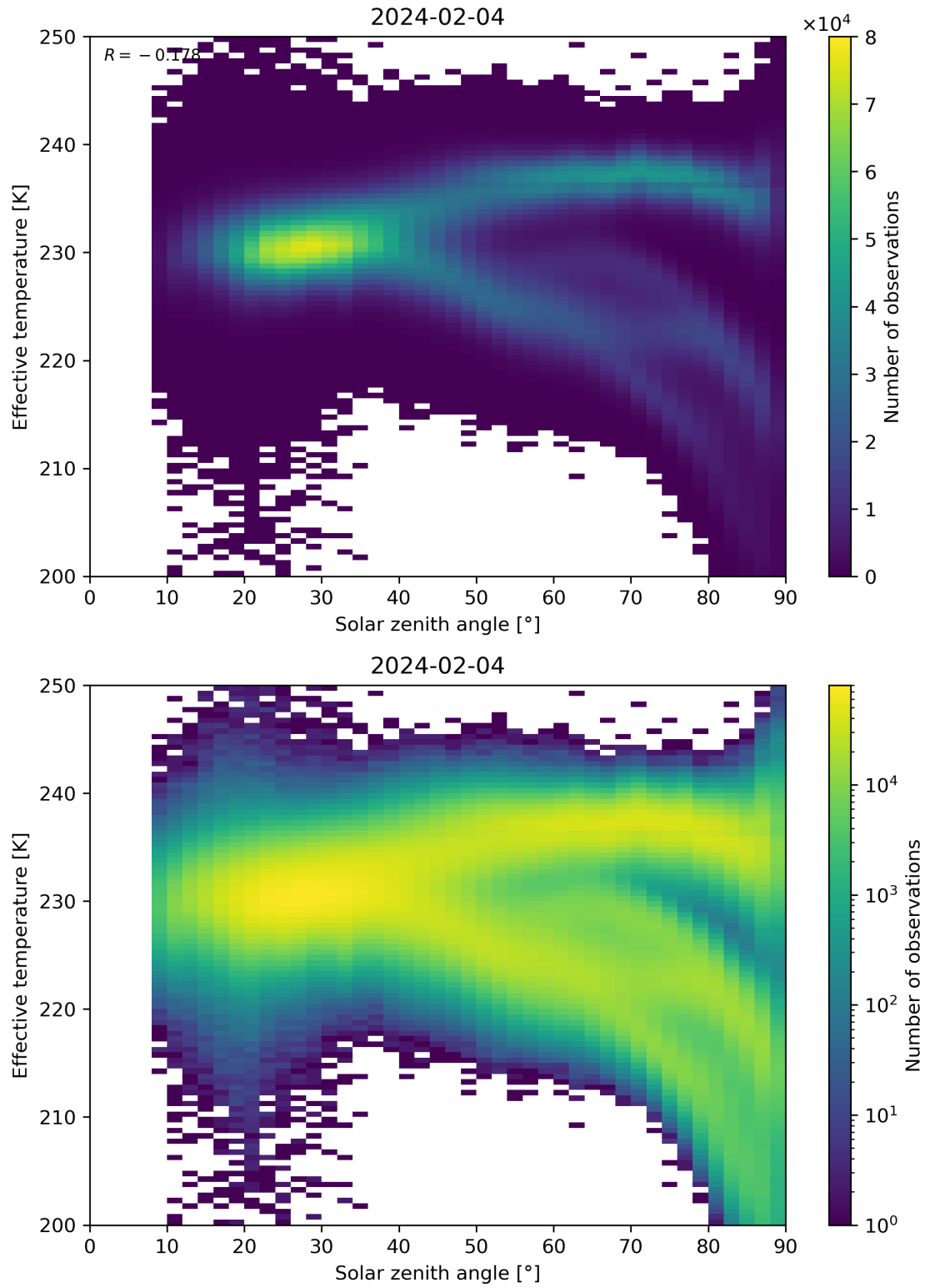
Figure 45: Scatter density plot of “Solar zenith angle” against “Effective temperature” for 2024-02-03 to 2024-02-05.
