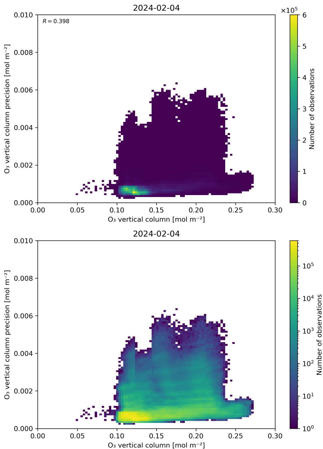
Figure 41: Scatter density plot of “O 3 vertical column” against “O 3 vertical column precision” for 2024-02-03 to 2024-02-05.
