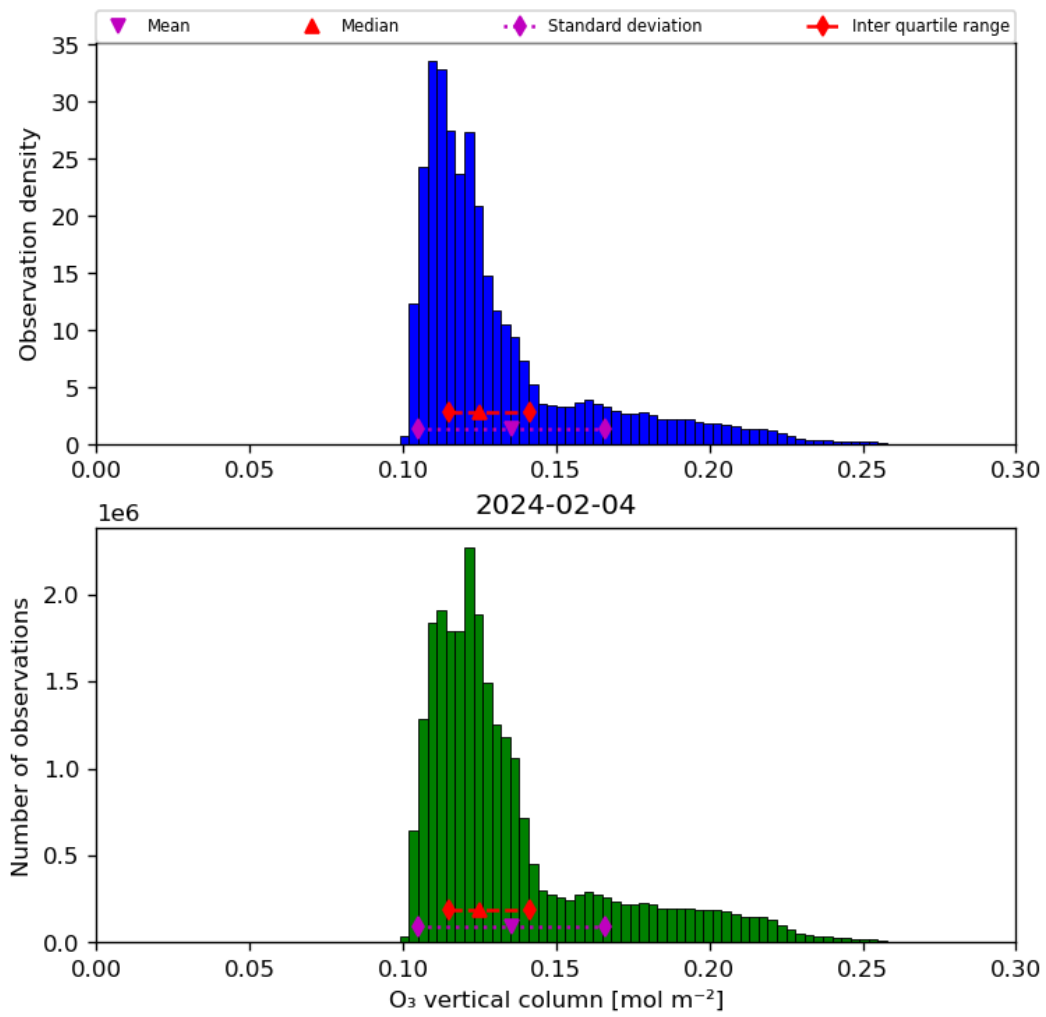
Figure 21: Histogram of “O 3 vertical column” for 2024-02-03 to 2024-02-05
