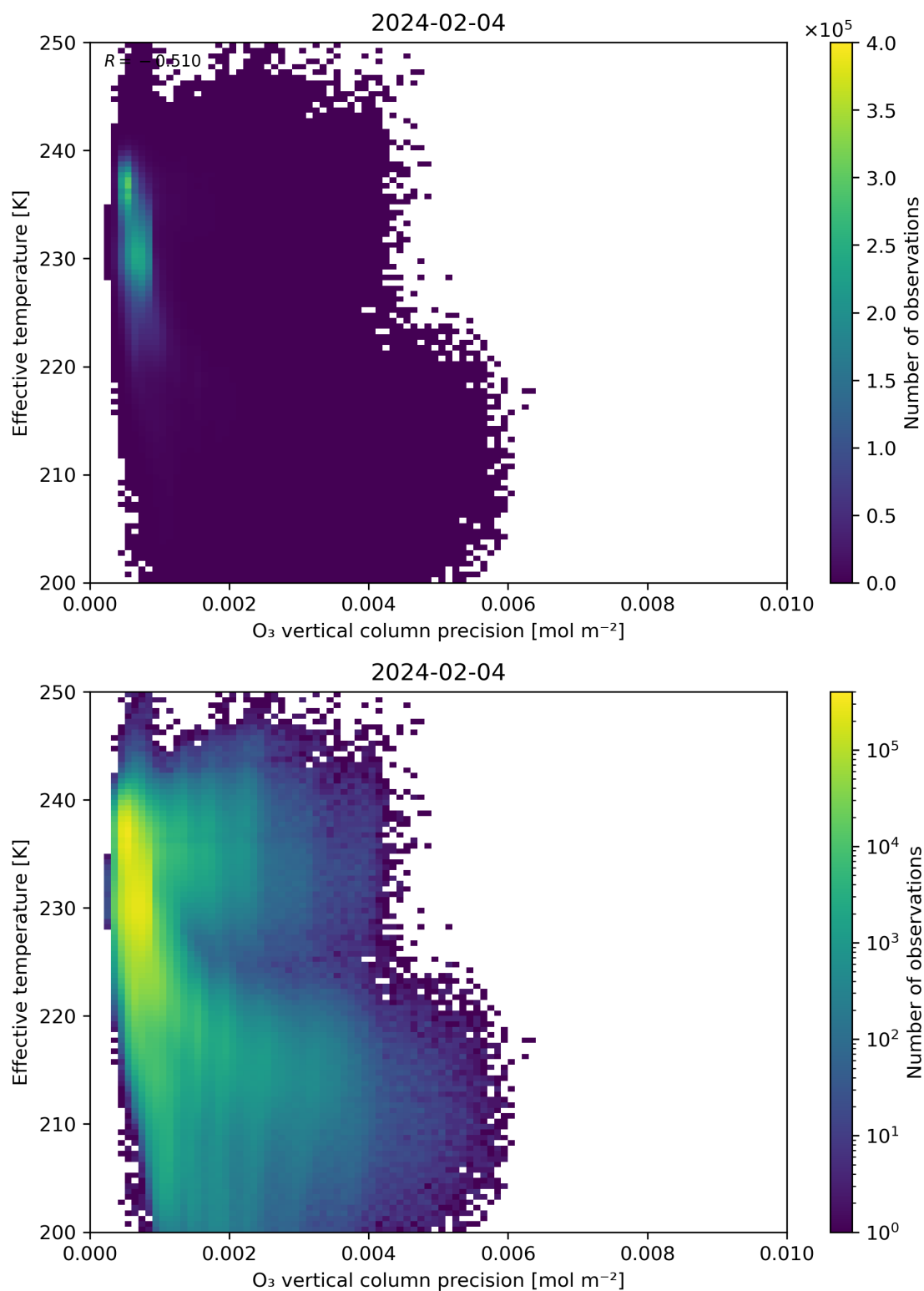
Figure 42: Scatter density plot of “O 3 vertical column precision” against “Effective temperature” for 2024-02-03 to 2024-02-05.
