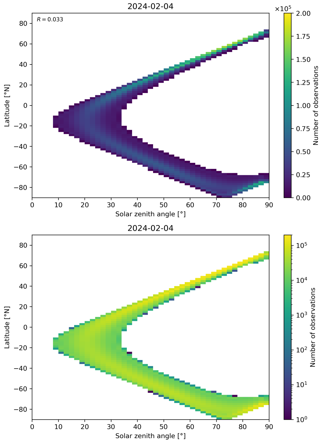
Figure 44: Scatter density plot of “Solar zenith angle” against “Latitude” for 2024-02-03 to 2024-02-05.
