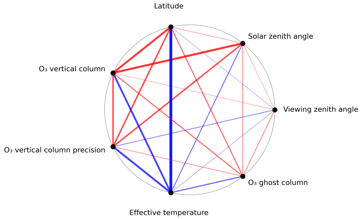
Figure 1: Map of correlation graph for 2024-02-03 to 2024-02-05.
