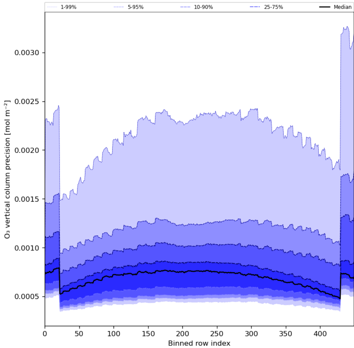
Figure 29: Along track statistics of “O 3 vertical column precision” for 2024-02-03 to 2024-02-05
