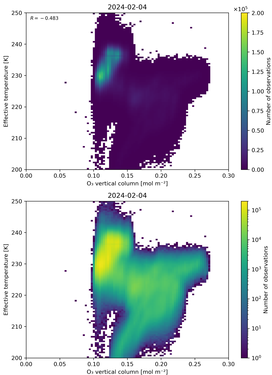
Figure 39: Scatter density plot of “O 3 vertical column” against “Effective temperature” for 2024-02-03 to 2024-02-05.
