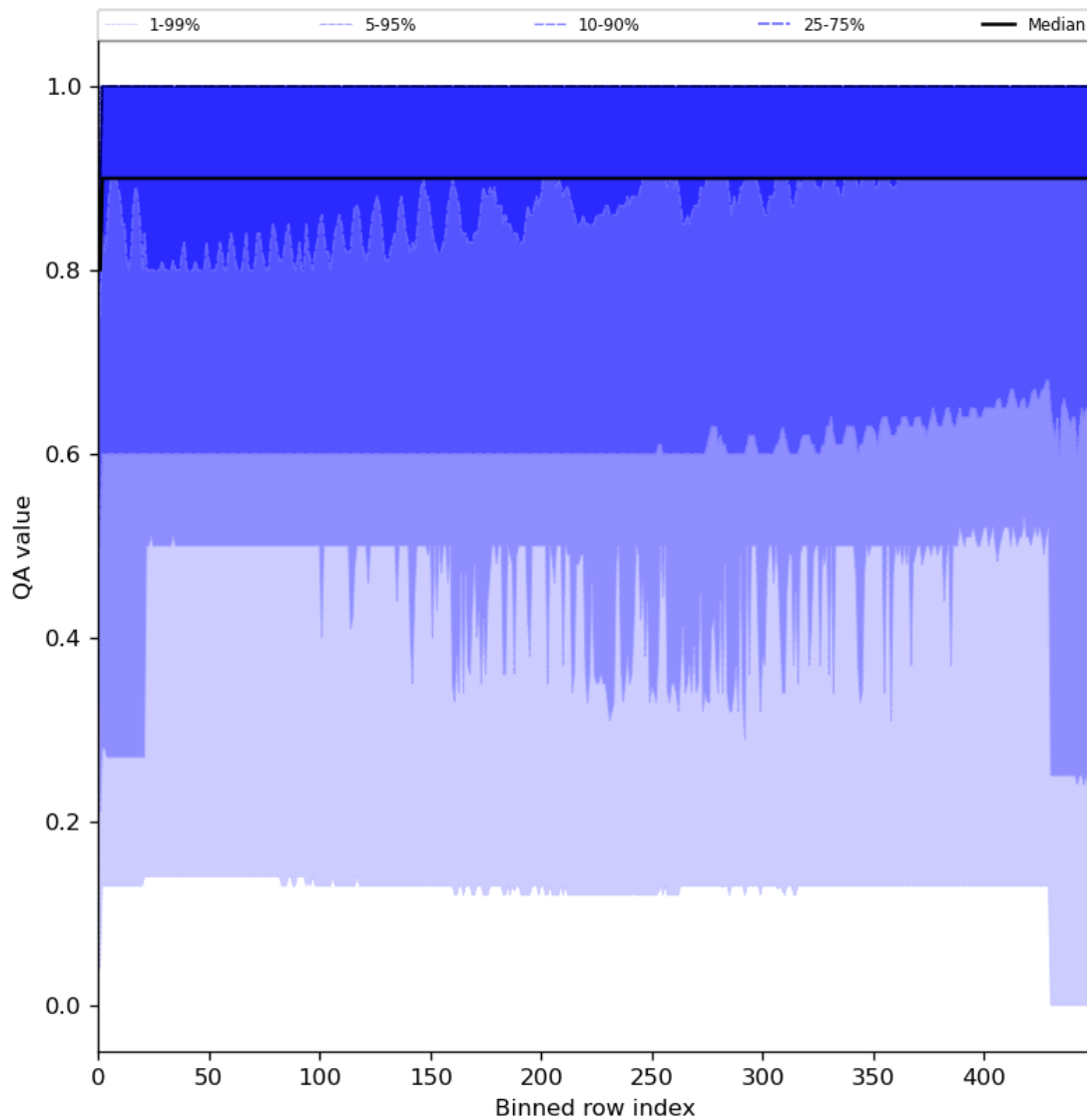
Figure 27: Along track statistics of “QA value” for 2024-02-03 to 2024-02-05
