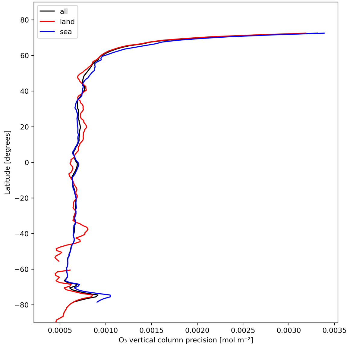
Figure 15: Zonal average of “O 3 vertical column precision” for 2024-02-03 to 2024-02-05.
