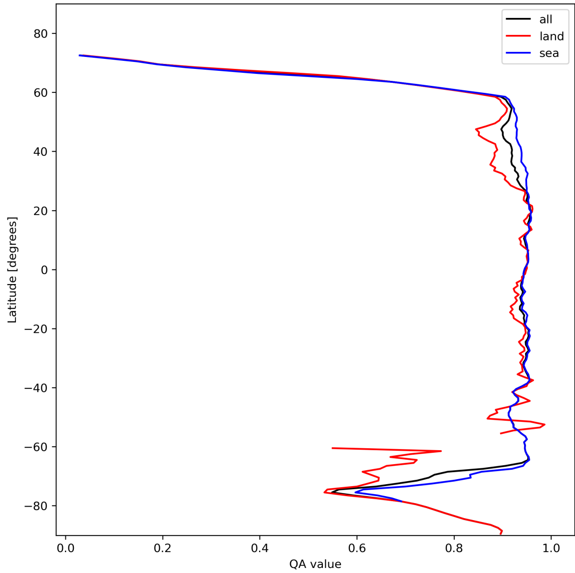
Figure 13: Zonal average of “QA value” for 2024-02-03 to 2024-02-05.
