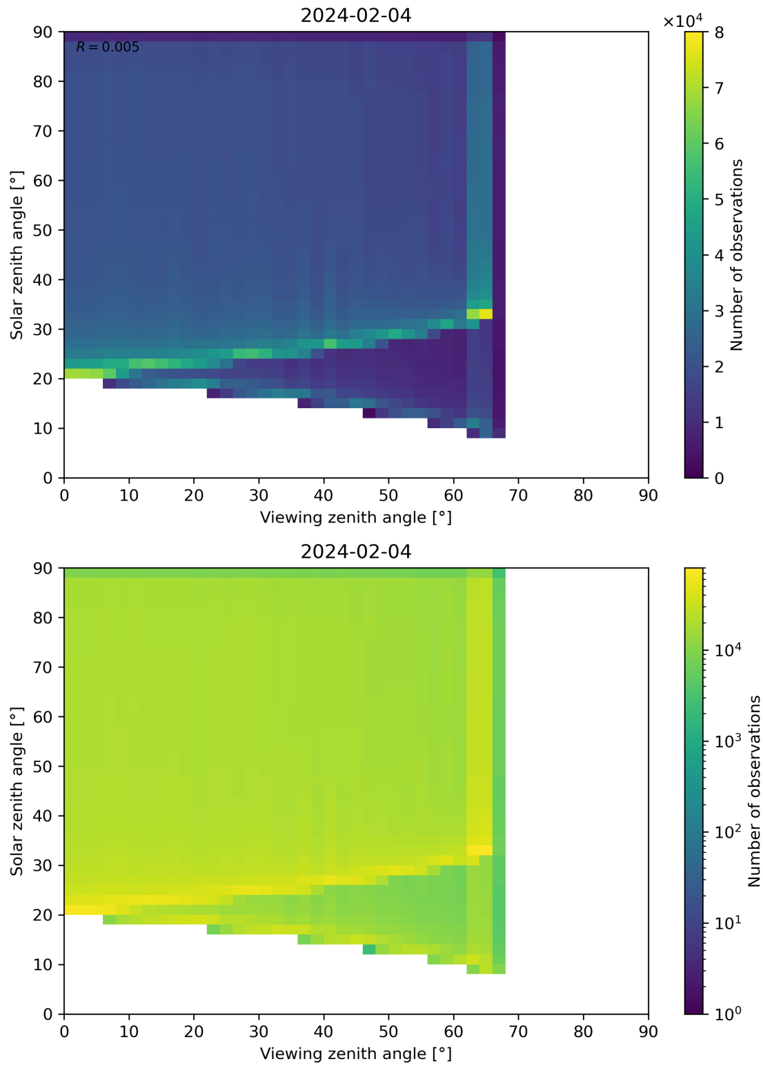
Figure 54: Scatter density plot of “Viewing zenith angle” against “Solar zenith angle” for 2024-02-03 to 2024-02-05.
