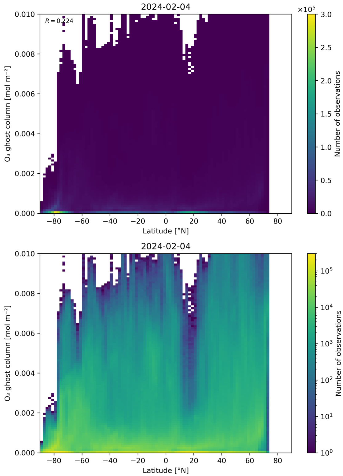
Figure 35: Scatter density plot of “Latitude” against “O 3 ghost column” for 2024-02-03 to 2024-02-05.
