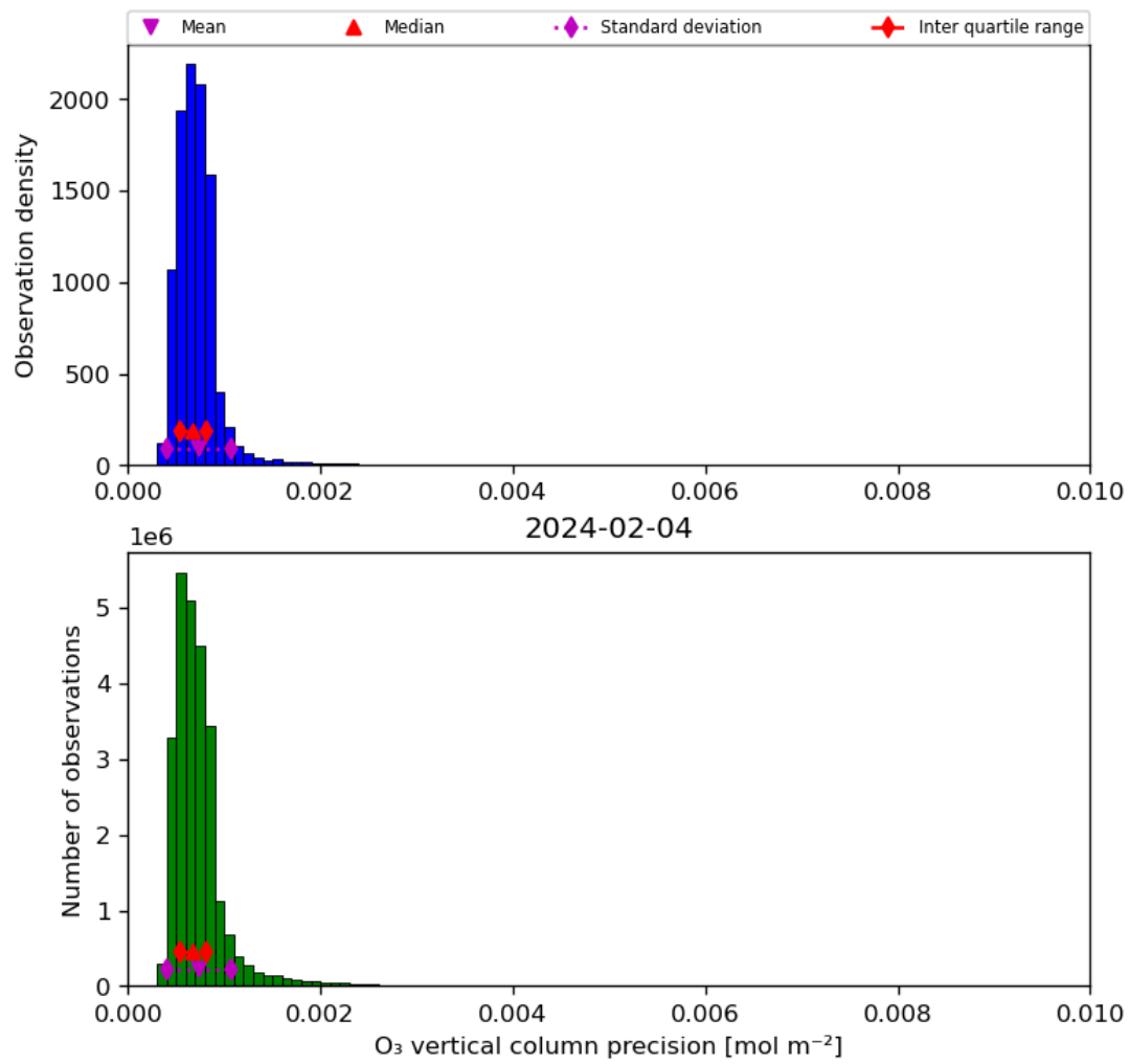
Figure 22: Histogram of “O 3 vertical column precision” for 2024-02-03 to 2024-02-05
