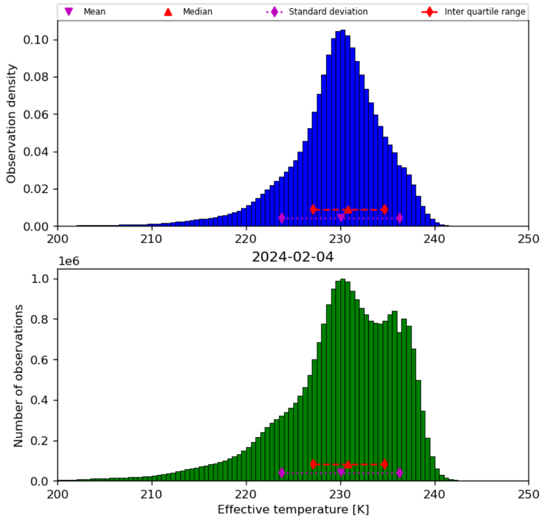
Figure 24: Histogram of “Effective temperature” for 2024-02-03 to 2024-02-05
