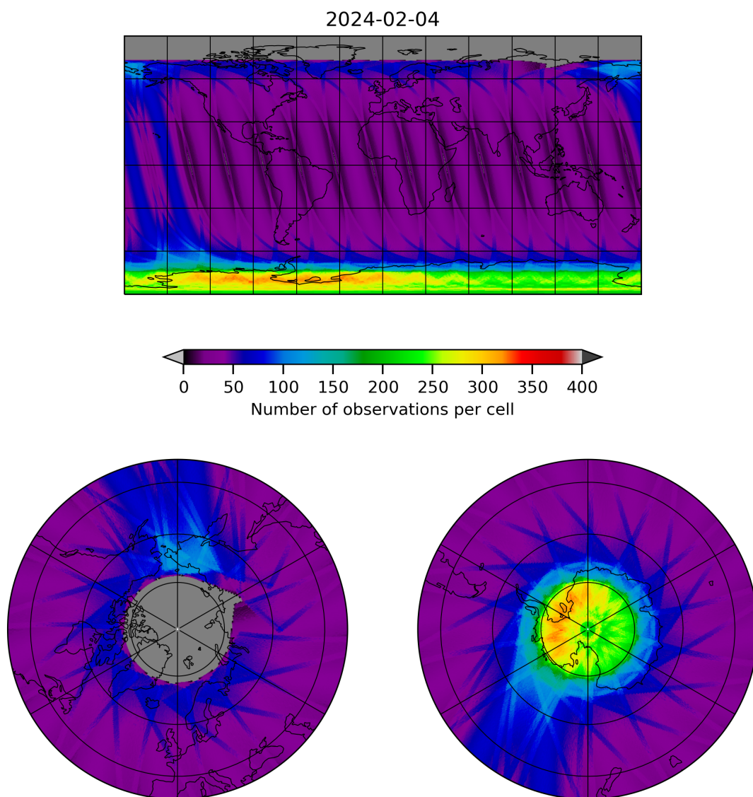
Figure 12: Map of the number of observations for 2024-02-03 to 2024-02-05
