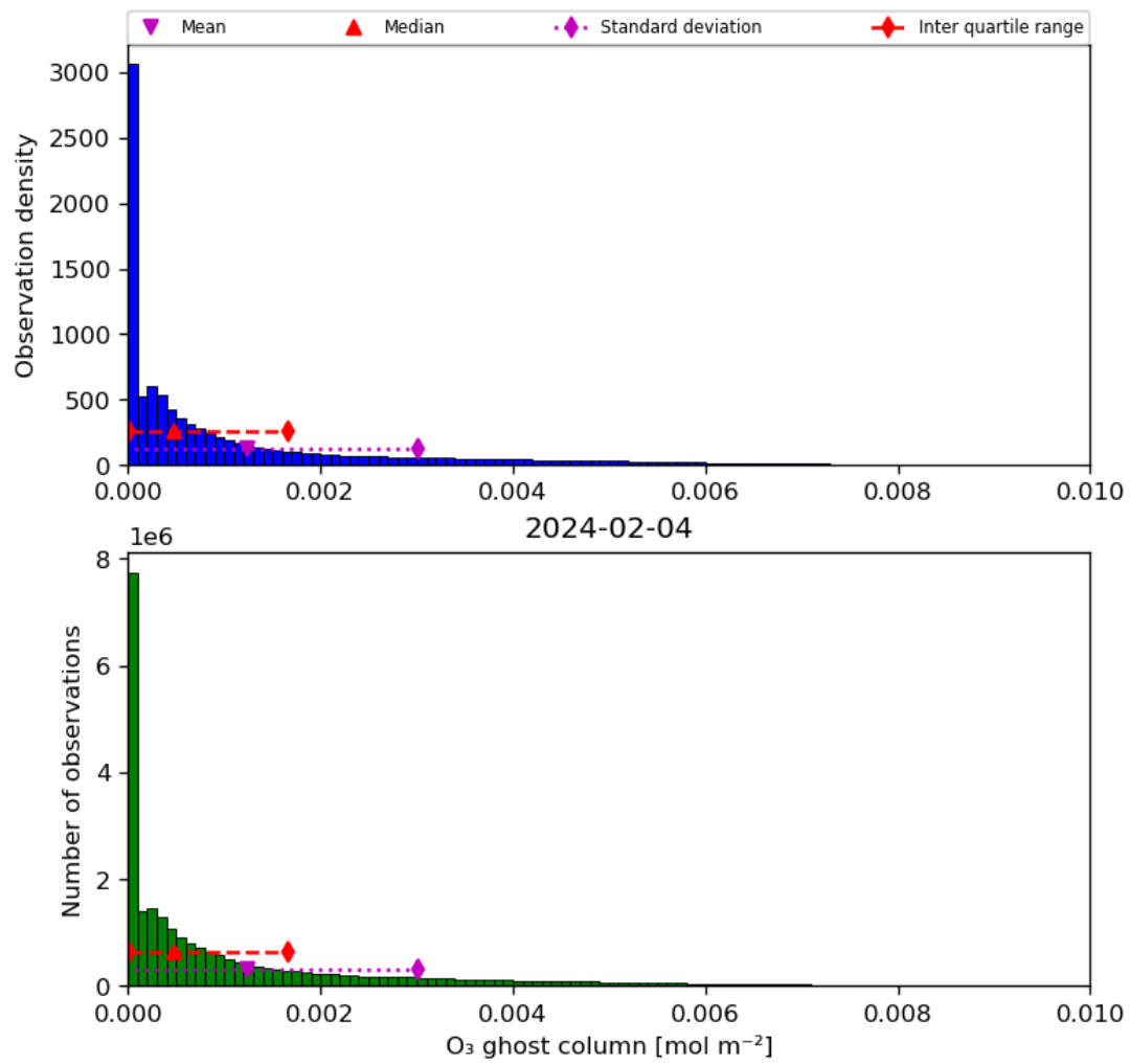
Figure 25: Histogram of “O 3 ghost column” for 2024-02-03 to 2024-02-05
