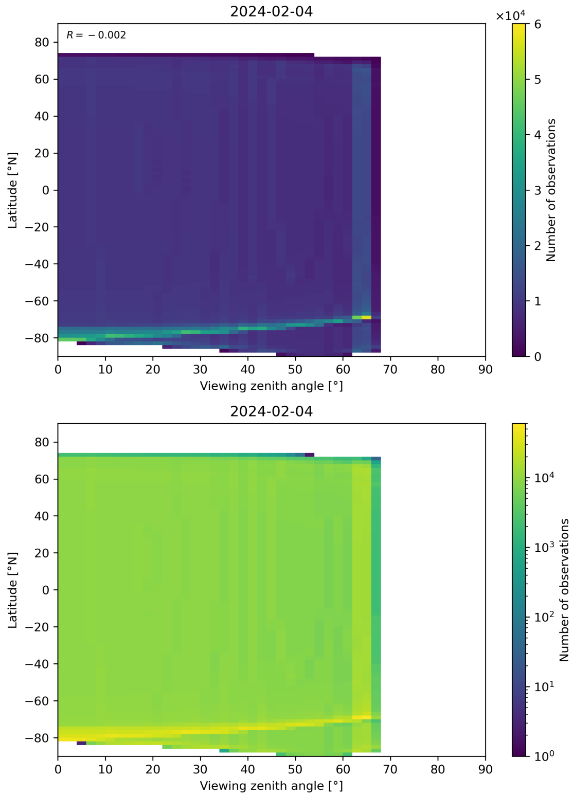
Figure 49: Scatter density plot of “Viewing zenith angle” against “Latitude” for 2024-02-03 to 2024-02-05.
