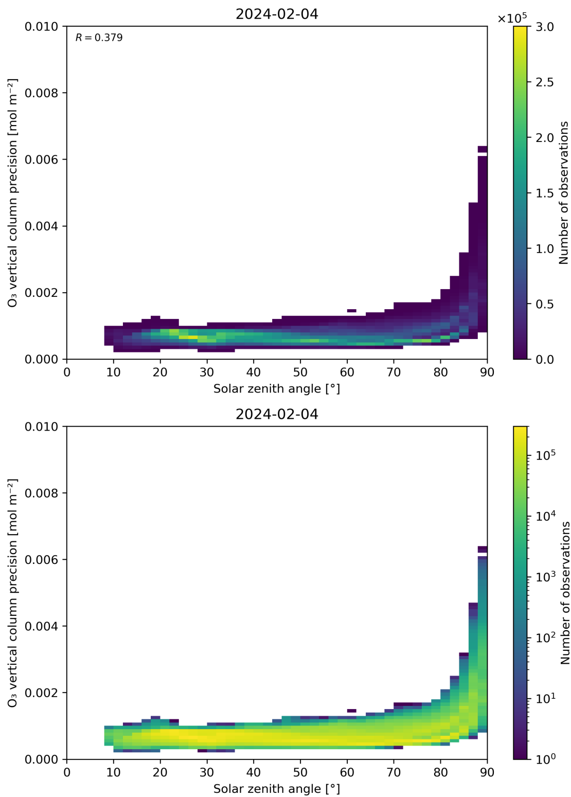
Figure 48: Scatter density plot of “Solar zenith angle” against “O 3 vertical column precision” for 2024-02-03 to 2024-02-05.
