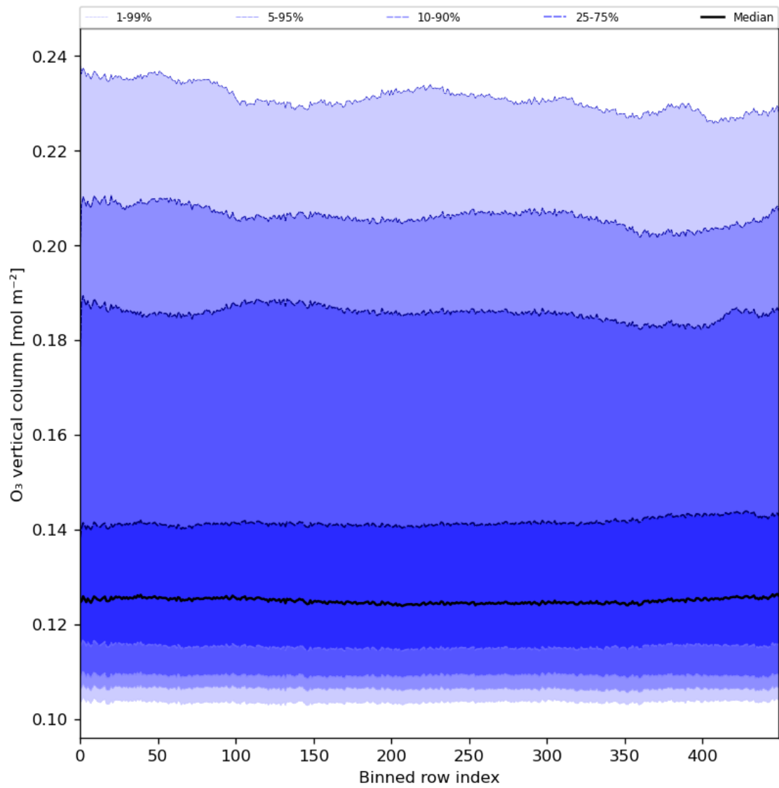
Figure 28: Along track statistics of “O 3 vertical column” for 2024-02-03 to 2024-02-05
