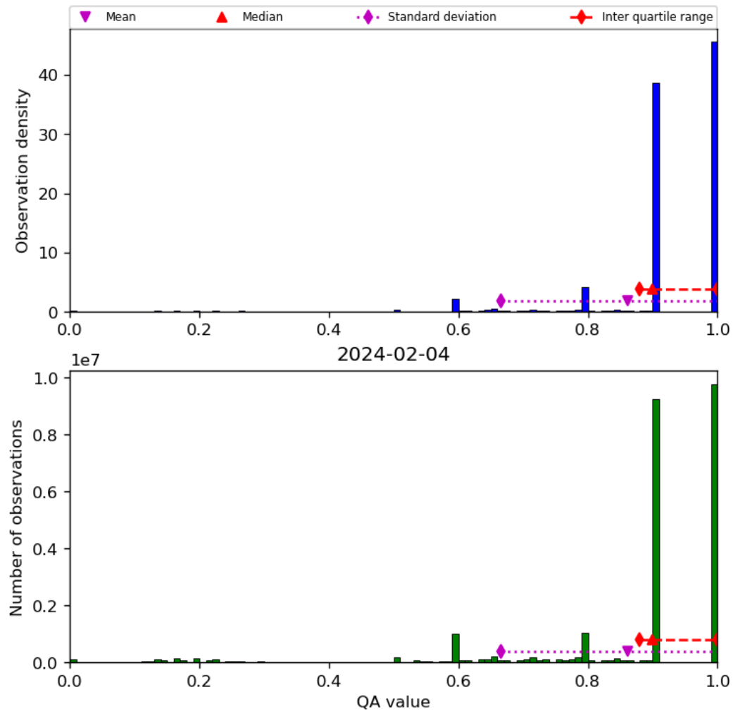
Figure 20: Histogram of “QA value” for 2024-02-03 to 2024-02-05
