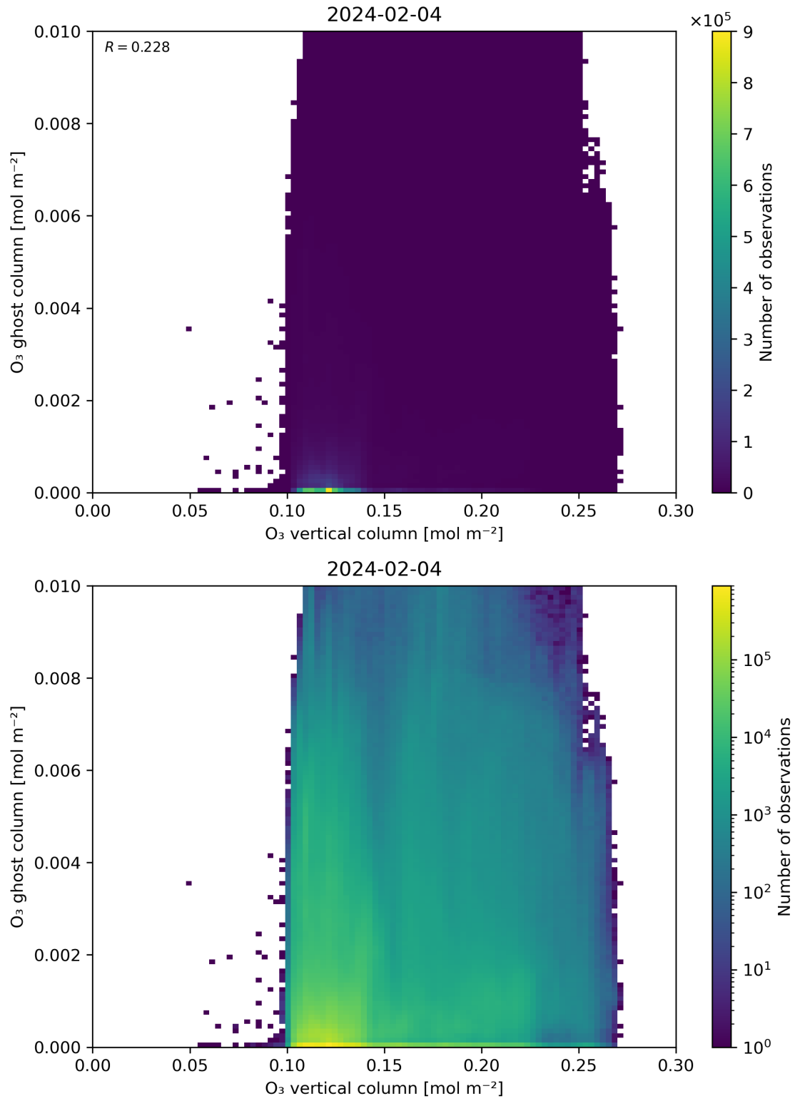
Figure 40: Scatter density plot of “O 3 vertical column” against “O 3 ghost column” for 2024-02-03 to 2024-02-05.
