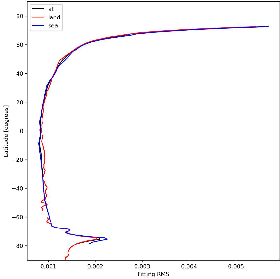
Figure 16: Zonal average of “Fitting RMS” for 2024-02-03 to 2024-02-05.
