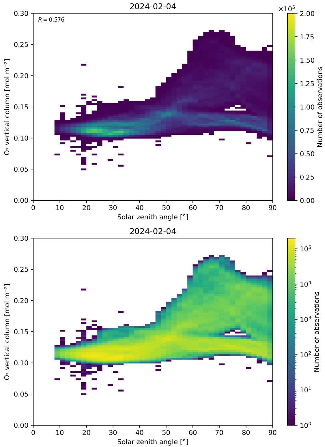
Figure 47: Scatter density plot of “Solar zenith angle” against “O 3 vertical column” for 2024-02-03 to 2024-02-05.
