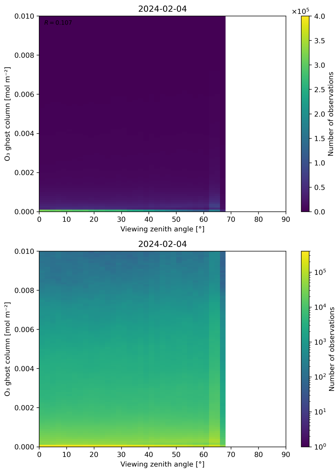
Figure 51: Scatter density plot of “Viewing zenith angle” against “O 3 ghost column” for 2024-02-03 to 2024-02-05.
