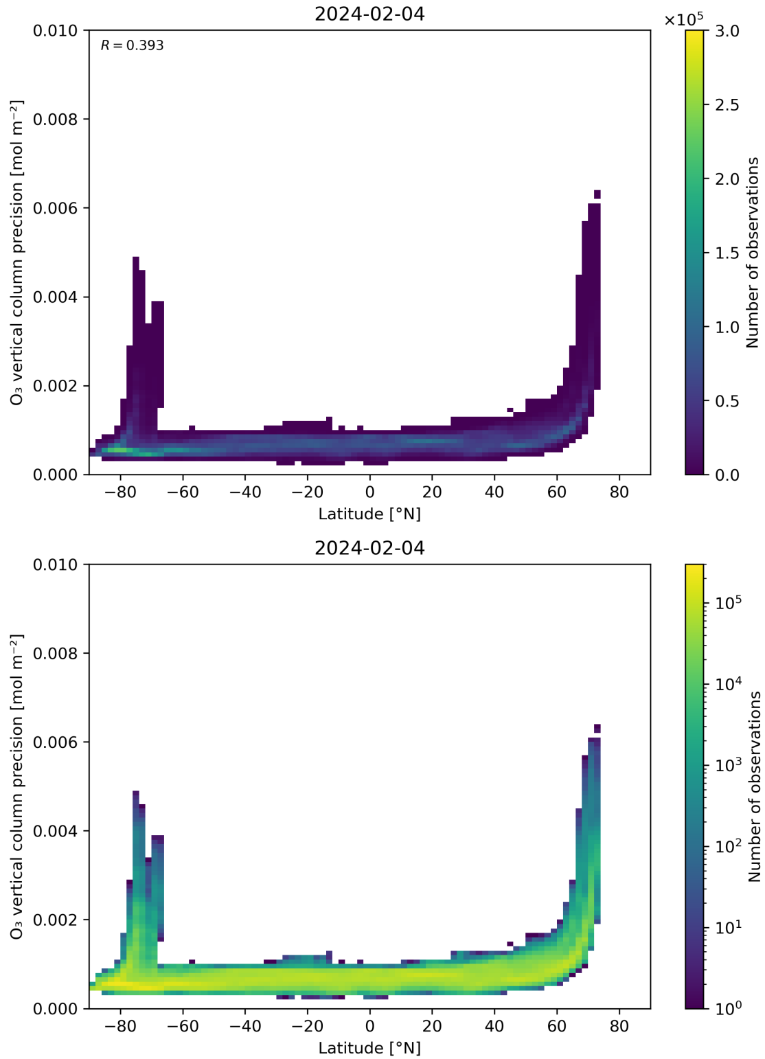
Figure 37: Scatter density plot of “Latitude” against “O 3 vertical column precision” for 2024-02-03 to 2024-02-05.
