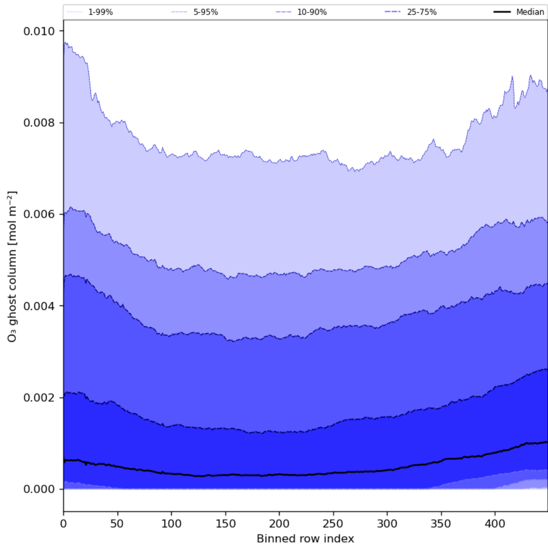
Figure 32: Along track statistics of “O 3 ghost column” for 2024-02-03 to 2024-02-05
