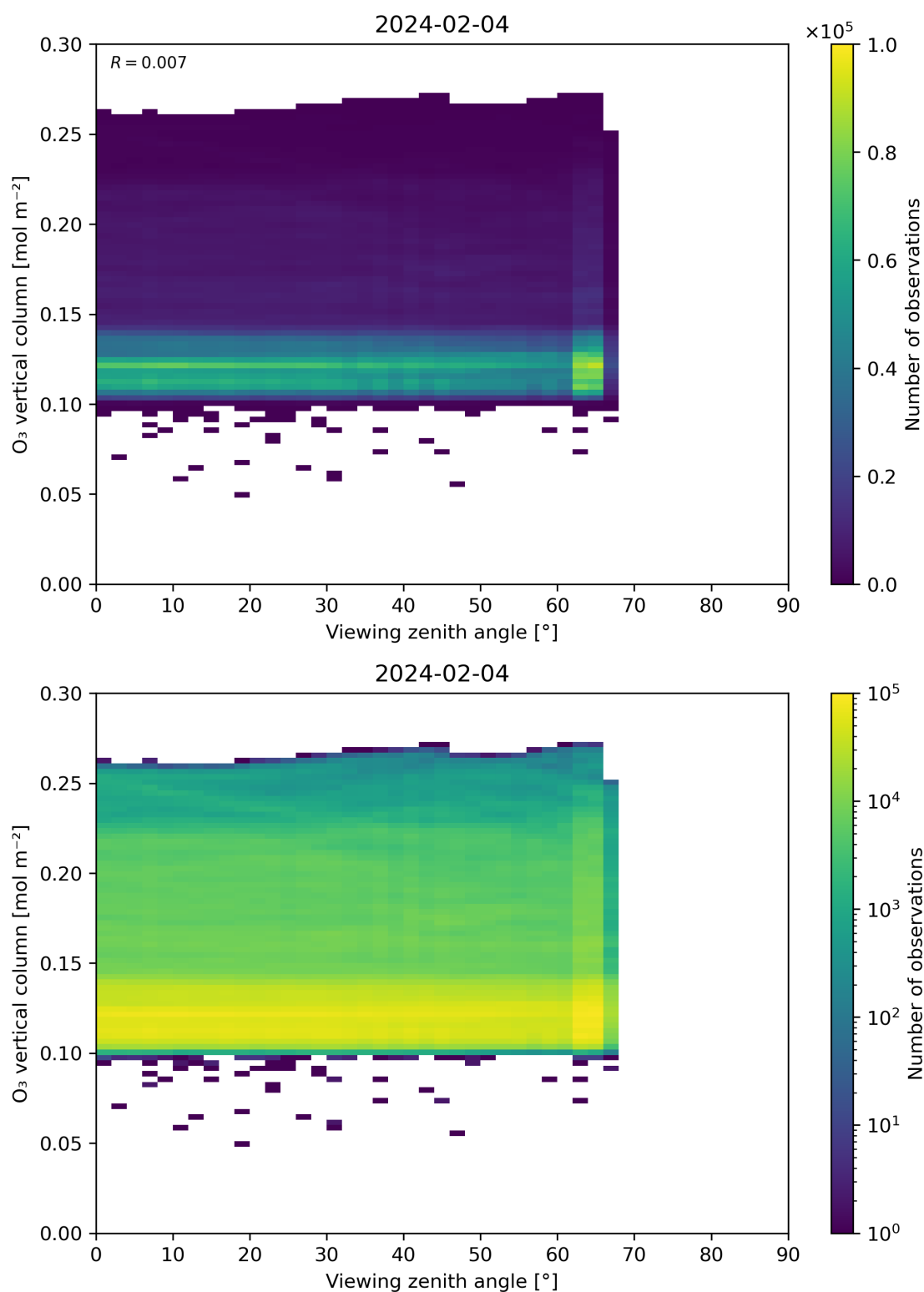
Figure 52: Scatter density plot of “Viewing zenith angle” against “O 3 vertical column” for 2024-02-03 to 2024-02-05.
