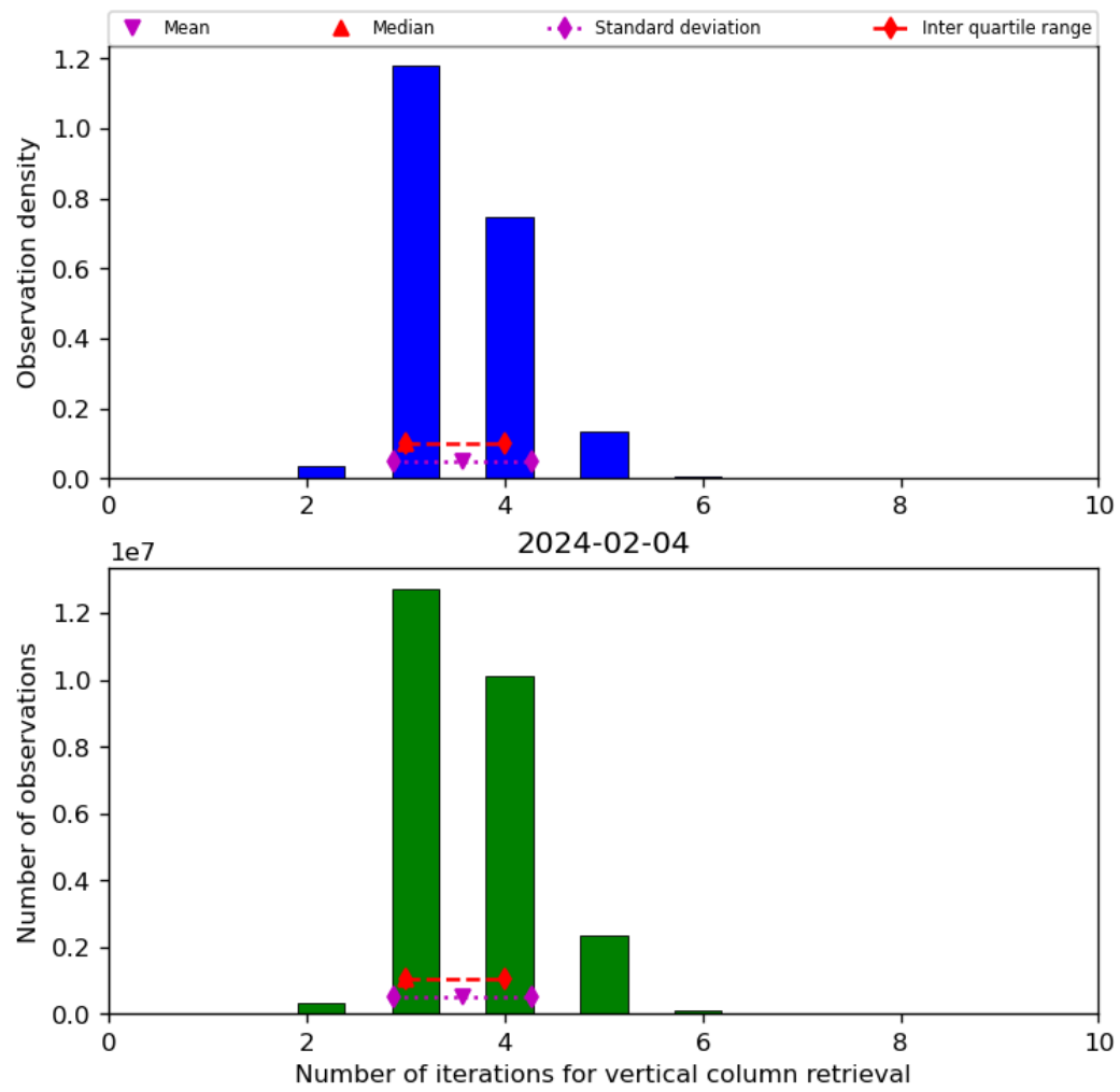
Figure 26: Histogram of “Number of iterations for vertical column retrieval” for 2024-02-03 to 2024-02-05
