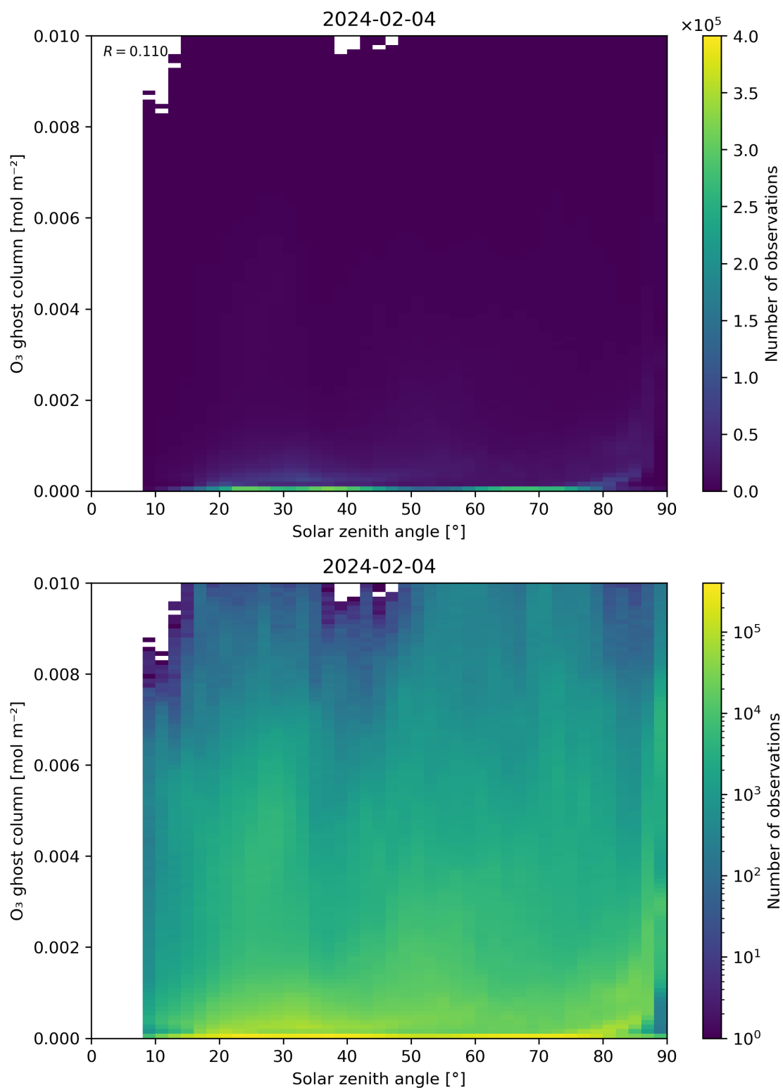
Figure 46: Scatter density plot of “Solar zenith angle” against “O 3 ghost column” for 2024-02-03 to 2024-02-05.
