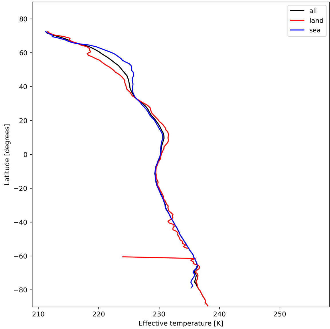
Figure 17: Zonal average of “Effective temperature” for 2024-02-03 to 2024-02-05.
