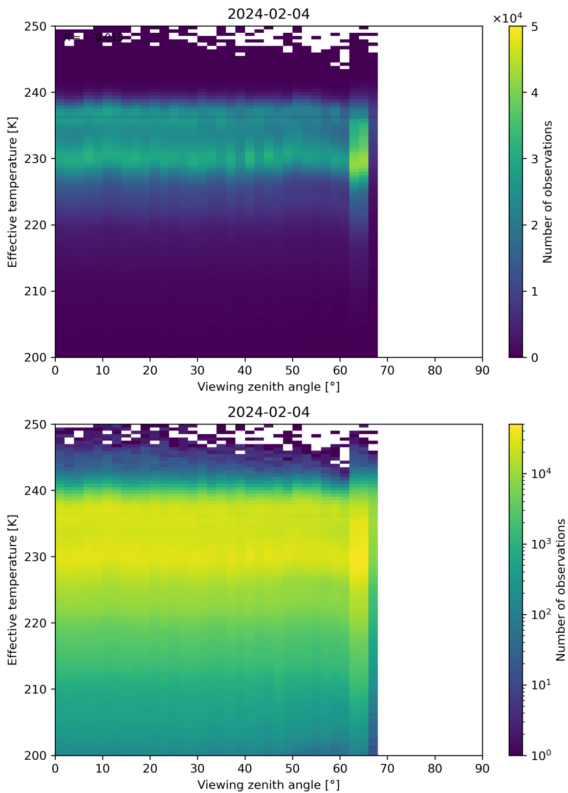
Figure 50: Scatter density plot of “Viewing zenith angle” against “Effective temperature” for 2024-02-03 to 2024-02-05.
