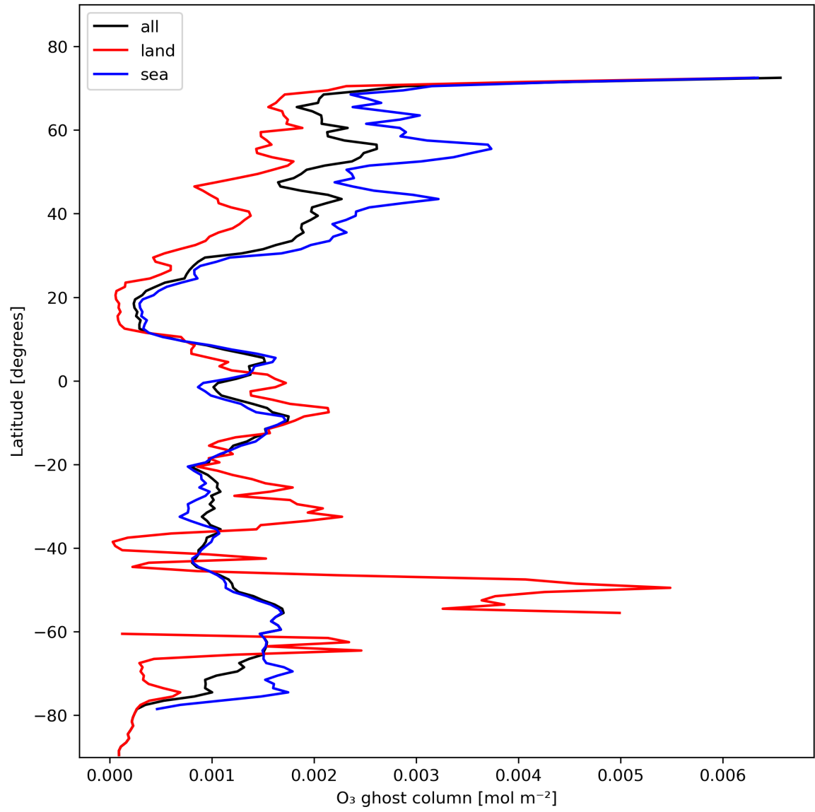
Figure 18: Zonal average of "O 3 ghost column" for 2024-02-03 to 2024-02-05.
