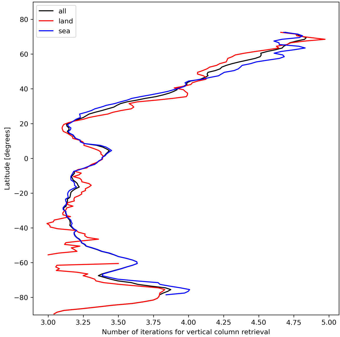
Figure 19: Zonal average of “Number of iterations for vertical column retrieval” for 2024-02-03 to 2024-02-05.
