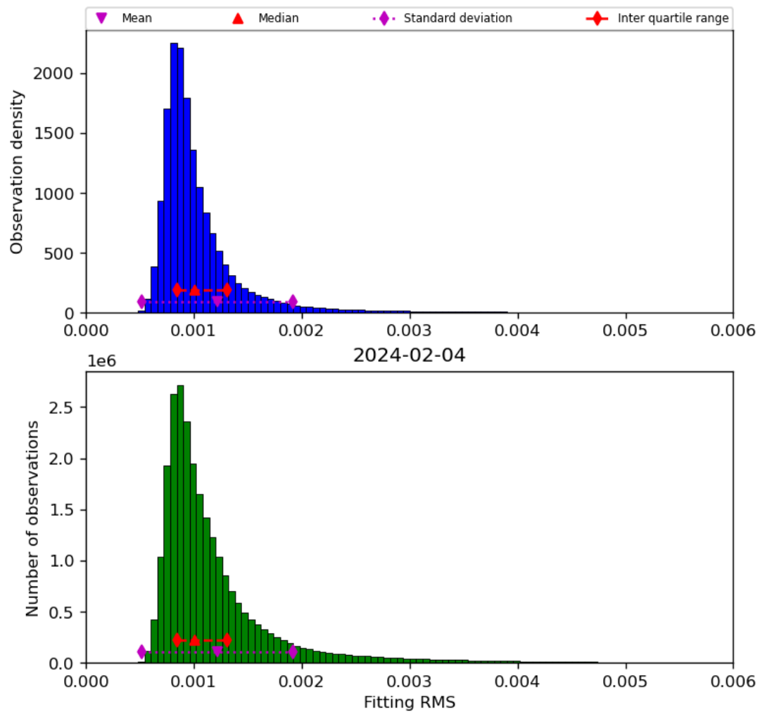
Figure 23: Histogram of “Fitting RMS” for 2024-02-03 to 2024-02-05
