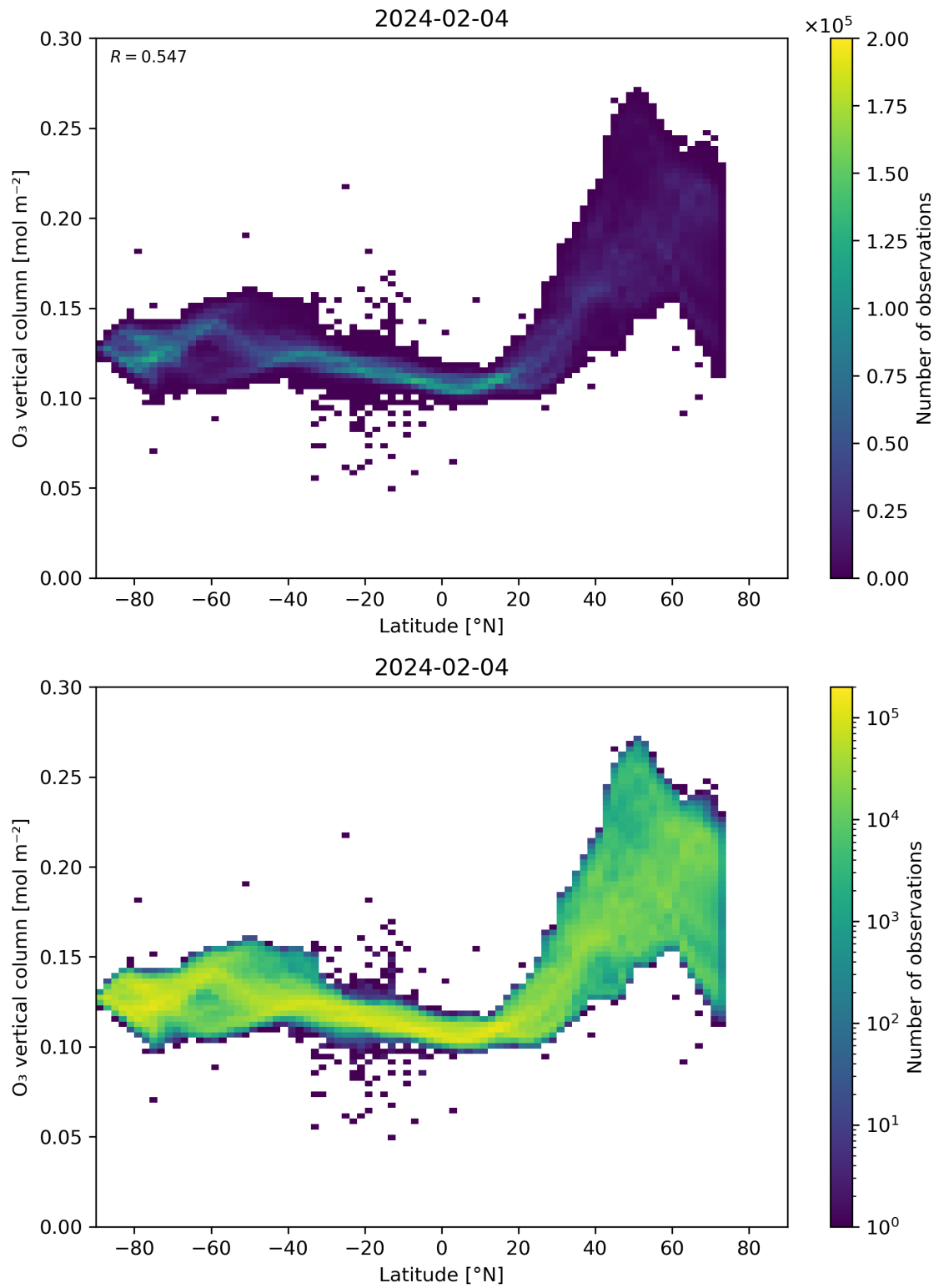
Figure 36: Scatter density plot of “Latitude” against “O 3 vertical column” for 2024-02-03 to 2024-02-05.
