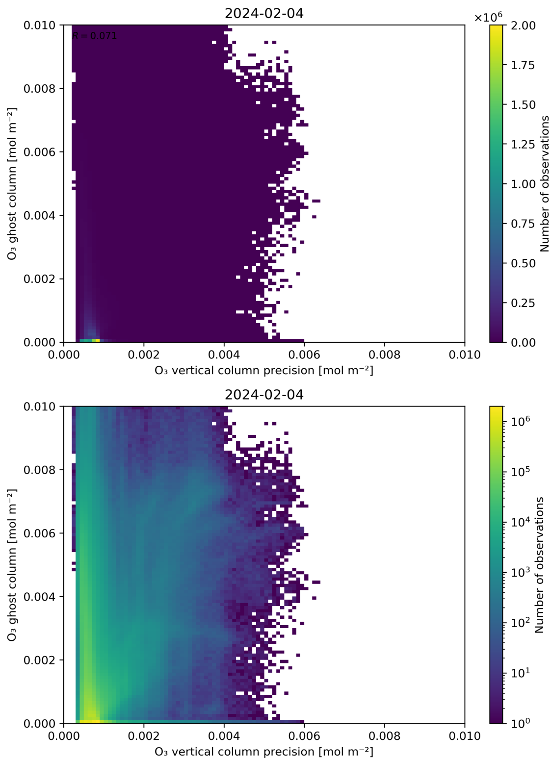
Figure 43: Scatter density plot of “ \text{O}_3 vertical column precision” against “ \text{O}_3 ghost column” for 2024-02-03 to 2024-02-05.
