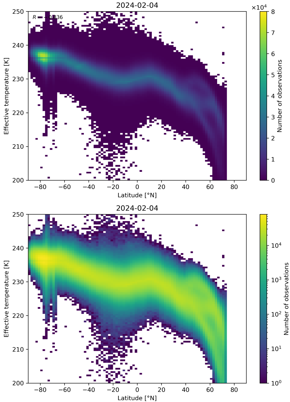
Figure 34: Scatter density plot of “Latitude” against “Effective temperature” for 2024-02-03 to 2024-02-05.
