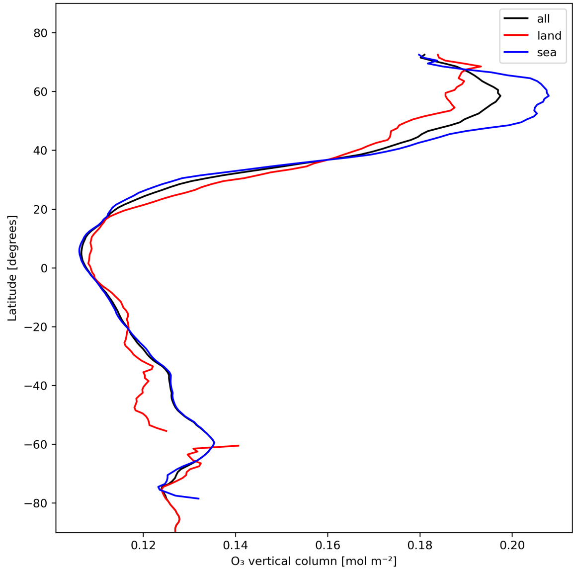
Figure 14: Zonal average of “O 3 vertical column” for 2024-02-03 to 2024-02-05.
