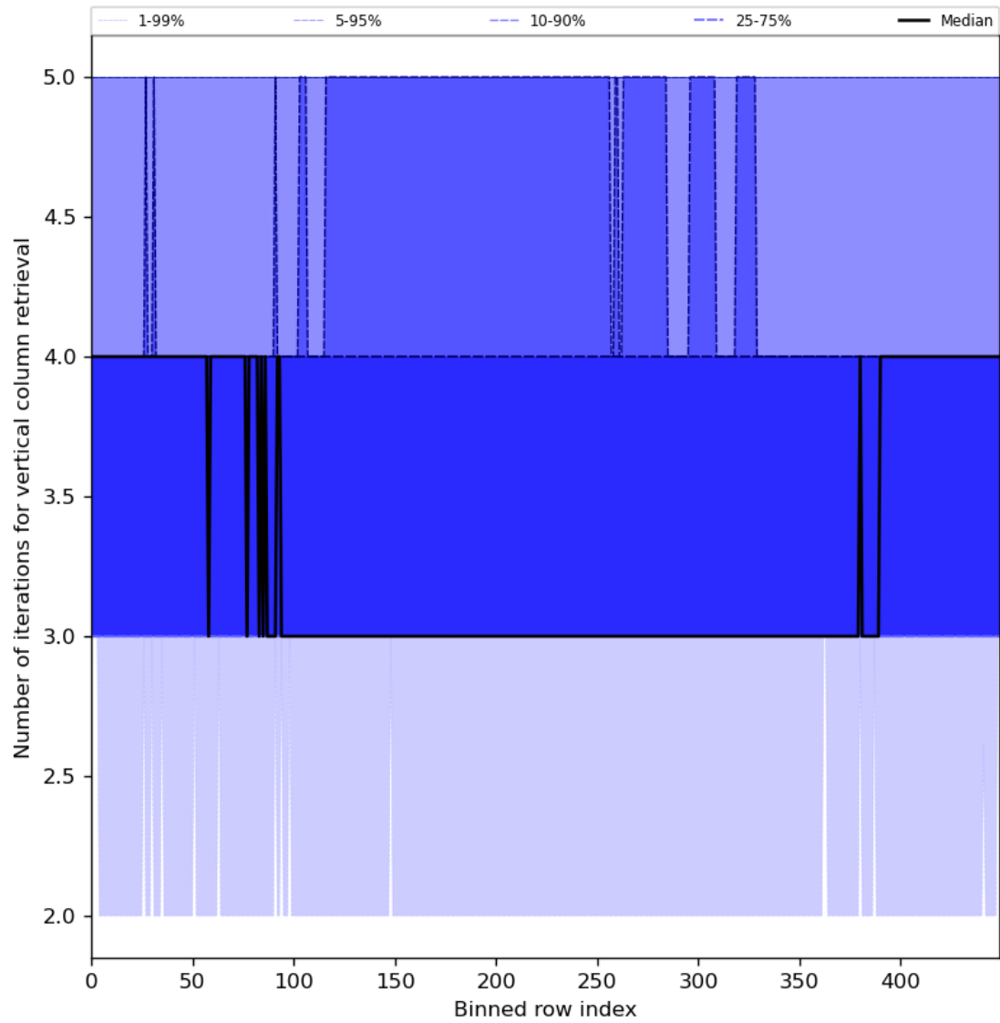
Figure 33: Along track statistics of “Number of iterations for vertical column retrieval” for 2024-02-03 to 2024-02-05
