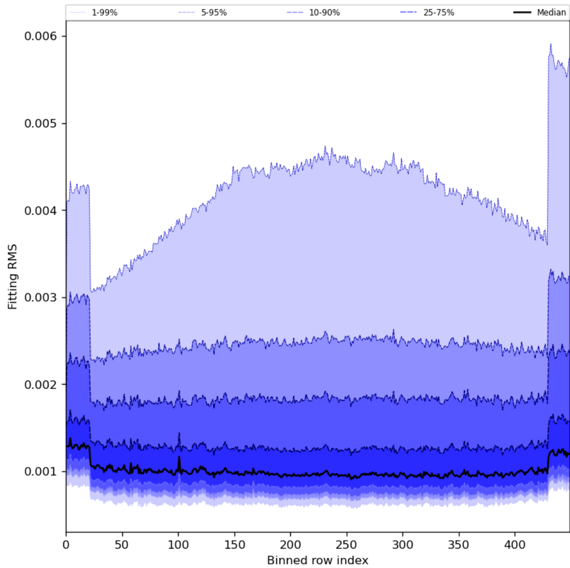
Figure 30: Along track statistics of “Fitting RMS” for 2024-02-03 to 2024-02-05
