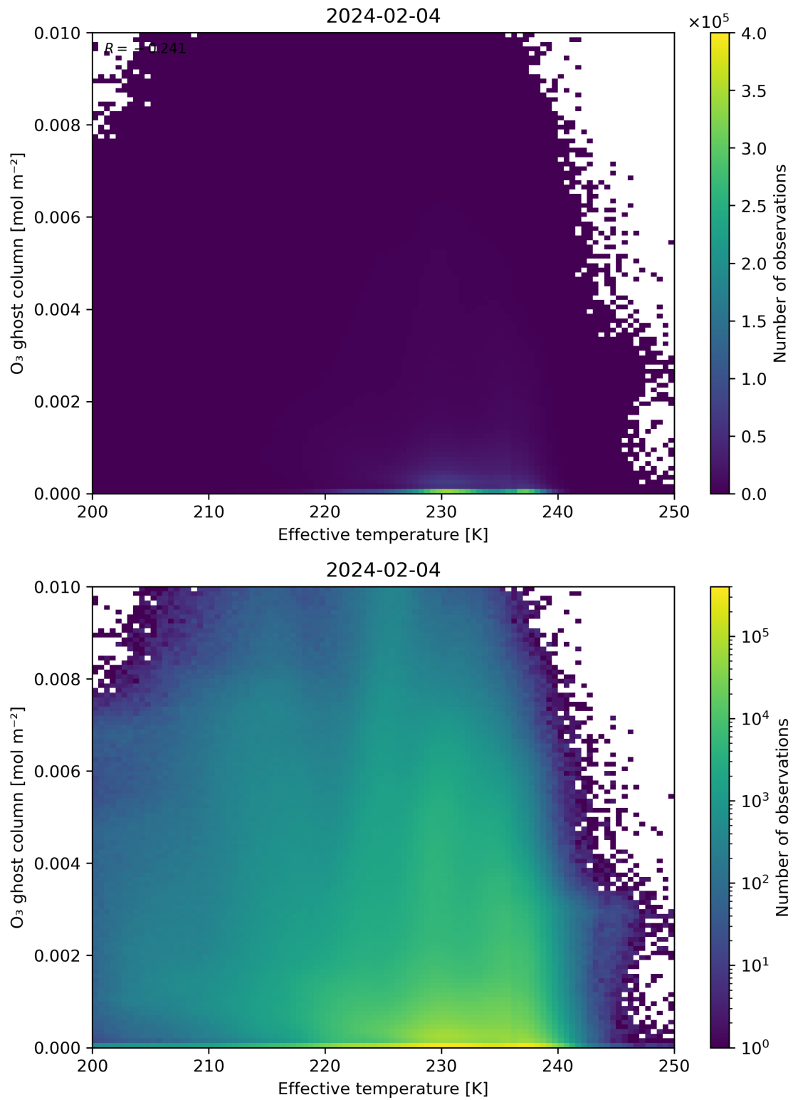
Figure 38: Scatter density plot of “Effective temperature” against “O 3 ghost column” for 2024-02-03 to 2024-02-05.
