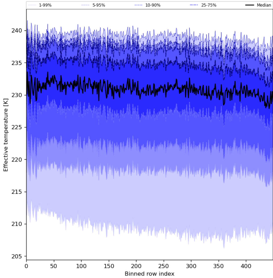
Figure 31: Along track statistics of "Effective temperature" for 2024-02-03 to 2024-02-05
