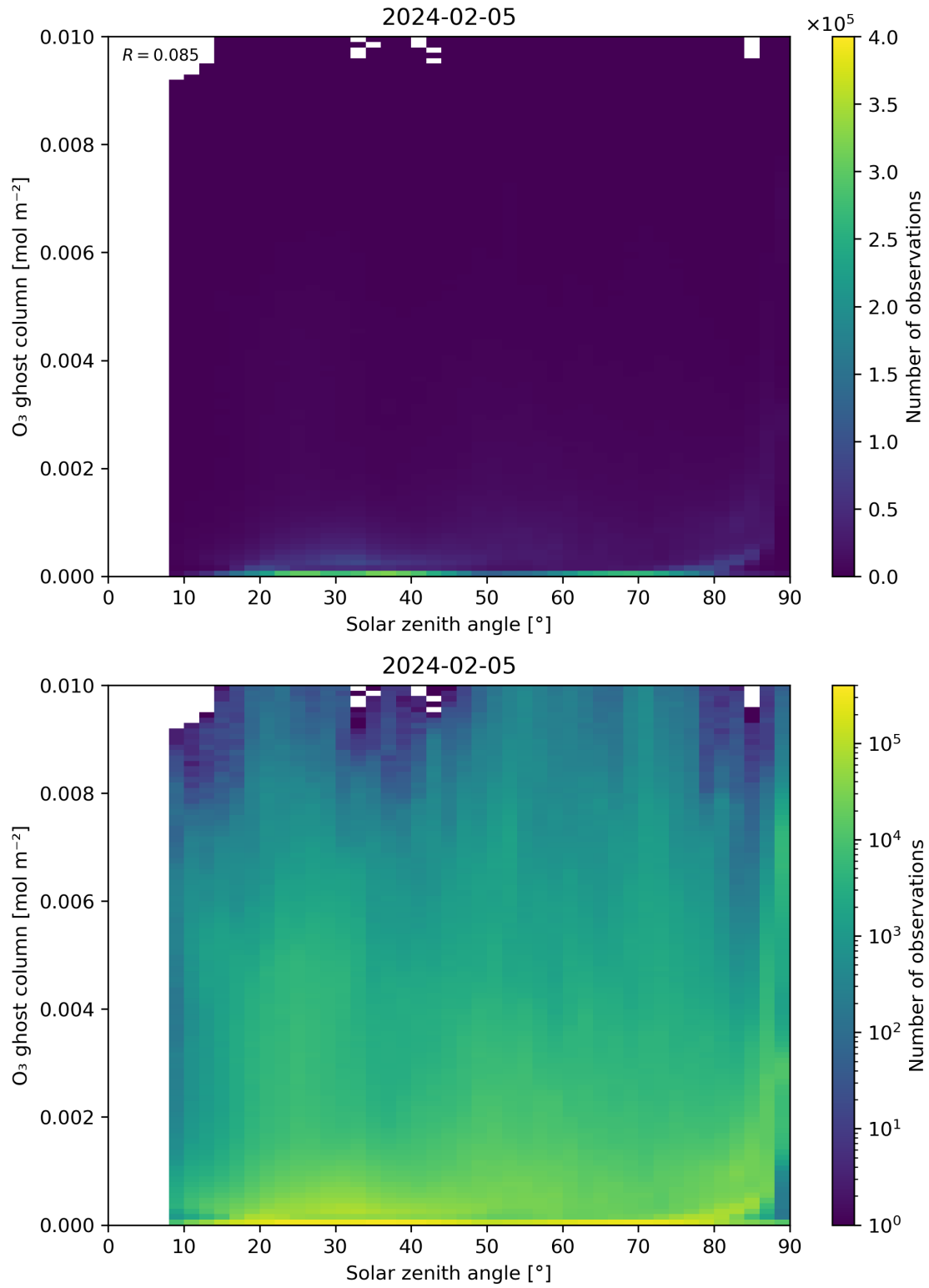
Figure 46: Scatter density plot of “Solar zenith angle” against “O 3 ghost column” for 2024-02-04 to 2024-02-06.
