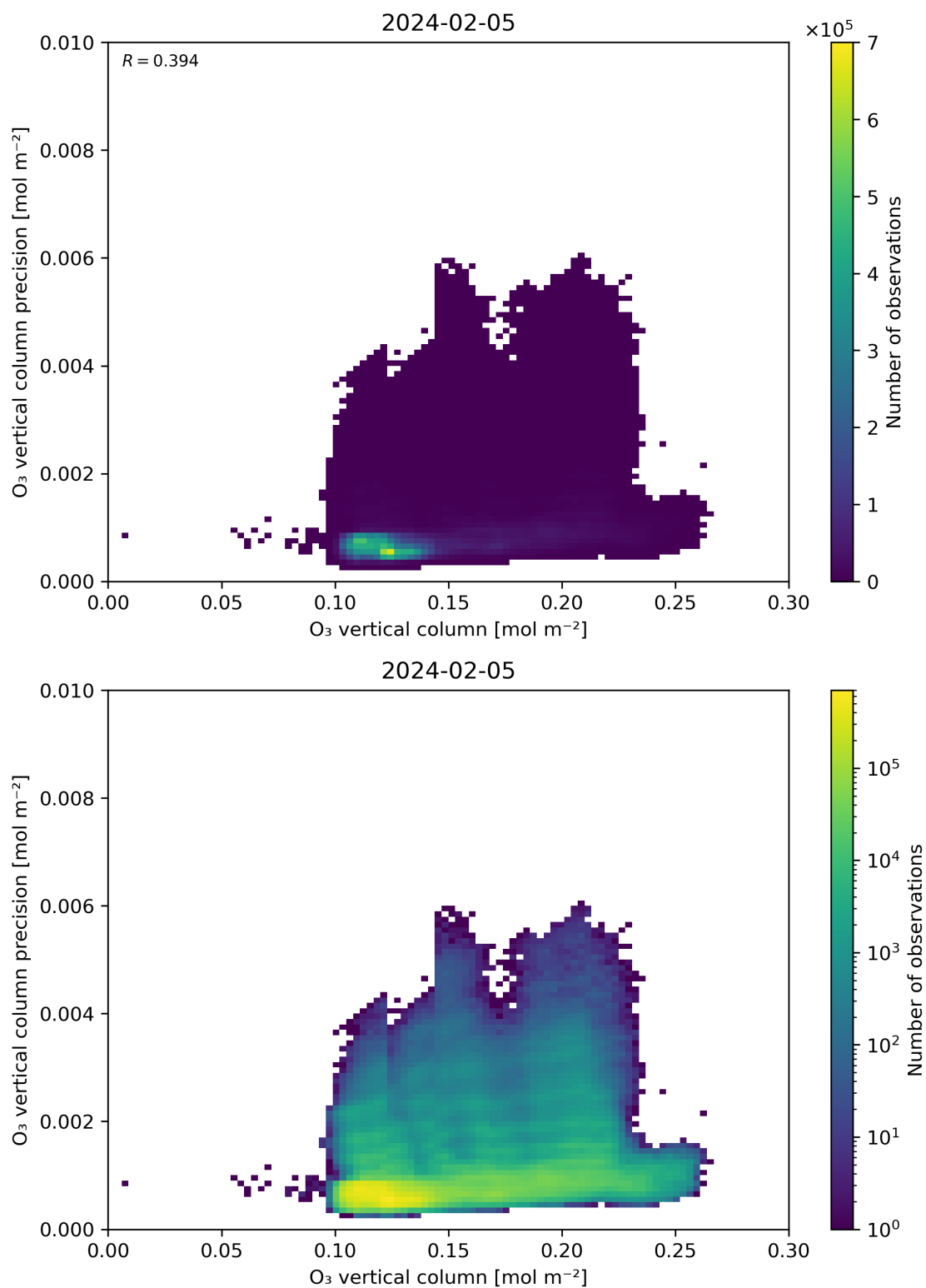
Figure 41: Scatter density plot of “O 3 vertical column” against “O 3 vertical column precision” for 2024-02-04 to 2024-02-06.
