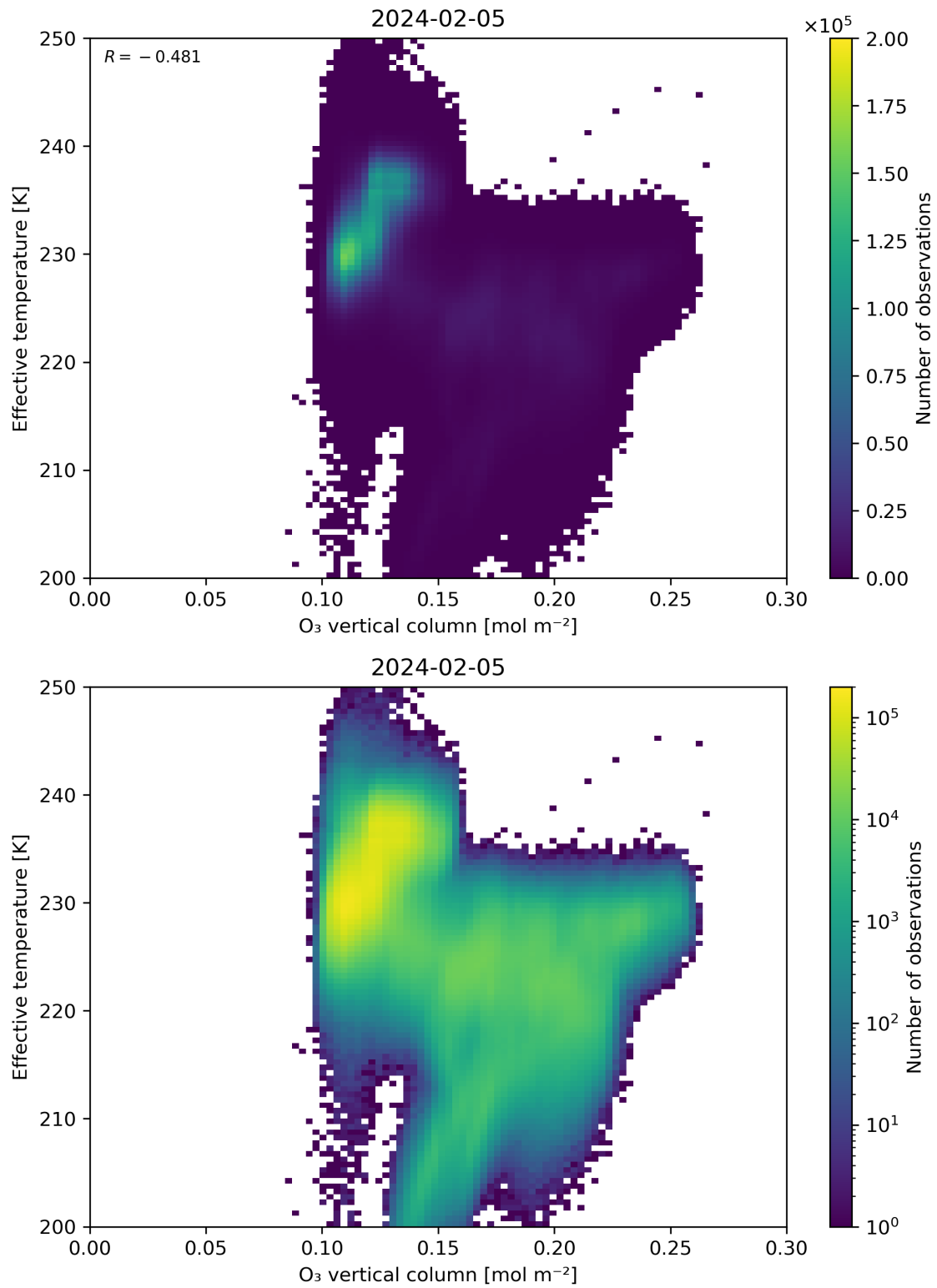
Figure 39: Scatter density plot of “O 3 vertical column” against “Effective temperature” for 2024-02-04 to 2024-02-06.
