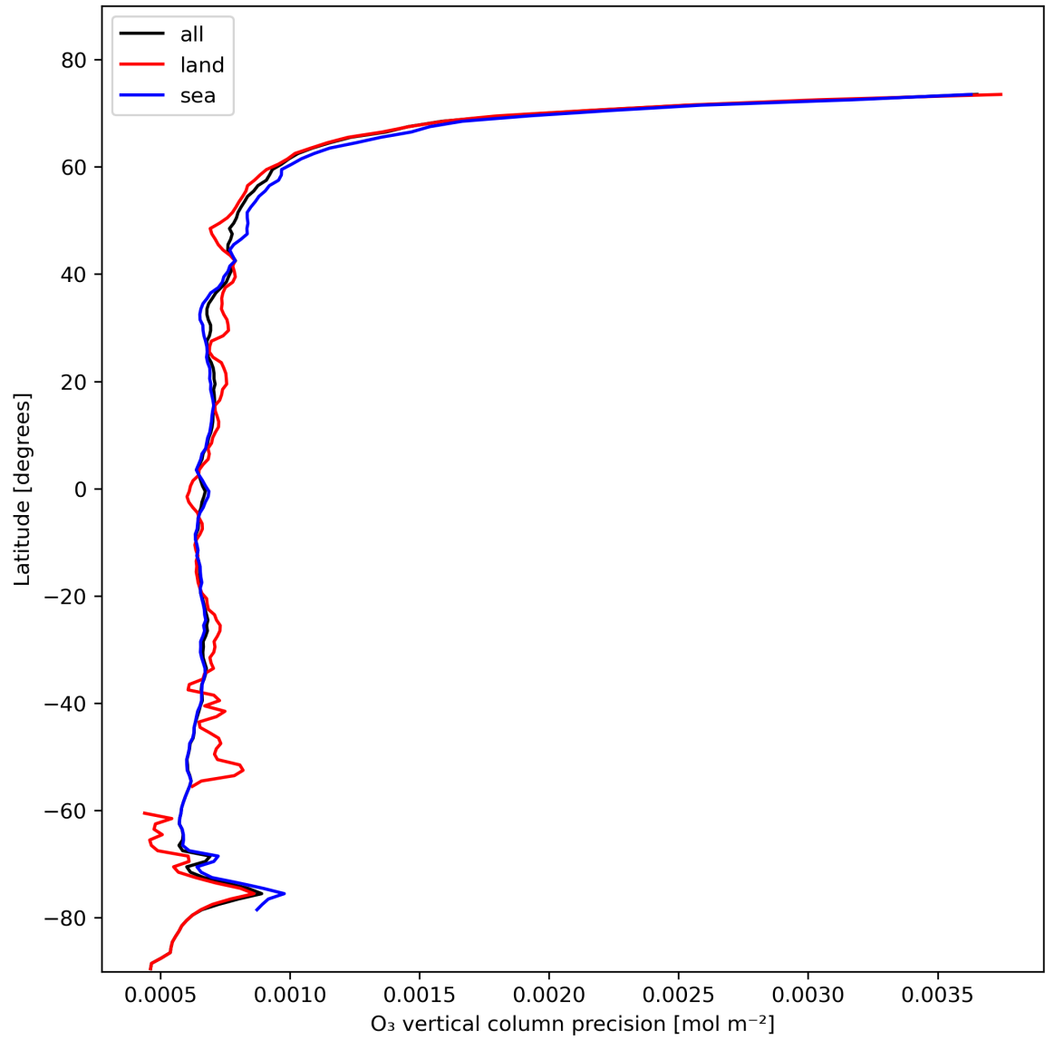
Figure 15: Zonal average of “O 3 vertical column precision” for 2024-02-04 to 2024-02-06.
