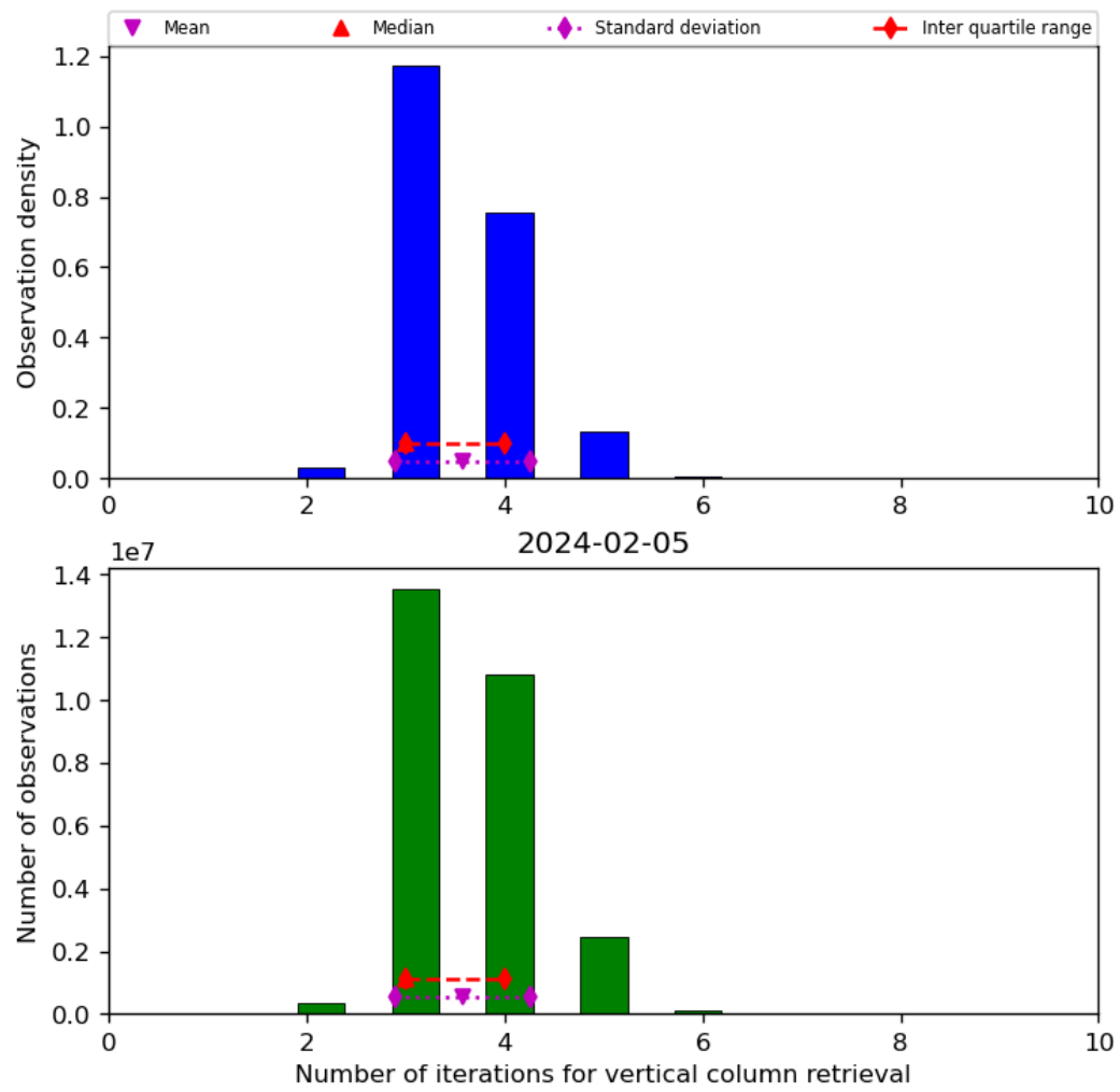
Figure 26: Histogram of “Number of iterations for vertical column retrieval” for 2024-02-04 to 2024-02-06
