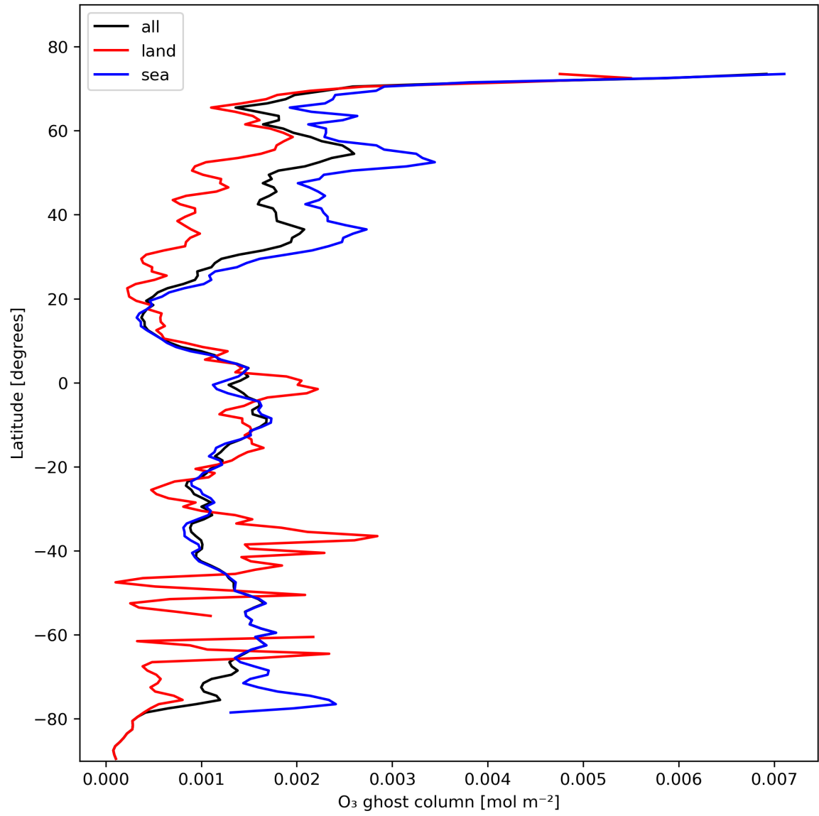
Figure 18: Zonal average of "O 3 ghost column" for 2024-02-04 to 2024-02-06.
