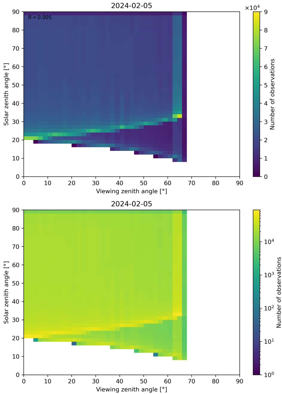
Figure 54: Scatter density plot of “Viewing zenith angle” against “Solar zenith angle” for 2024-02-04 to 2024-02-06.
