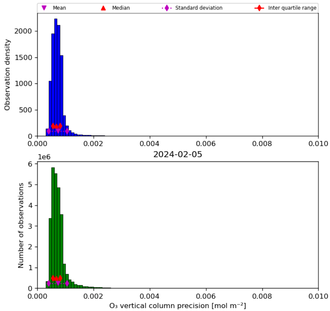
Figure 22: Histogram of “O 3 vertical column precision” for 2024-02-04 to 2024-02-06
