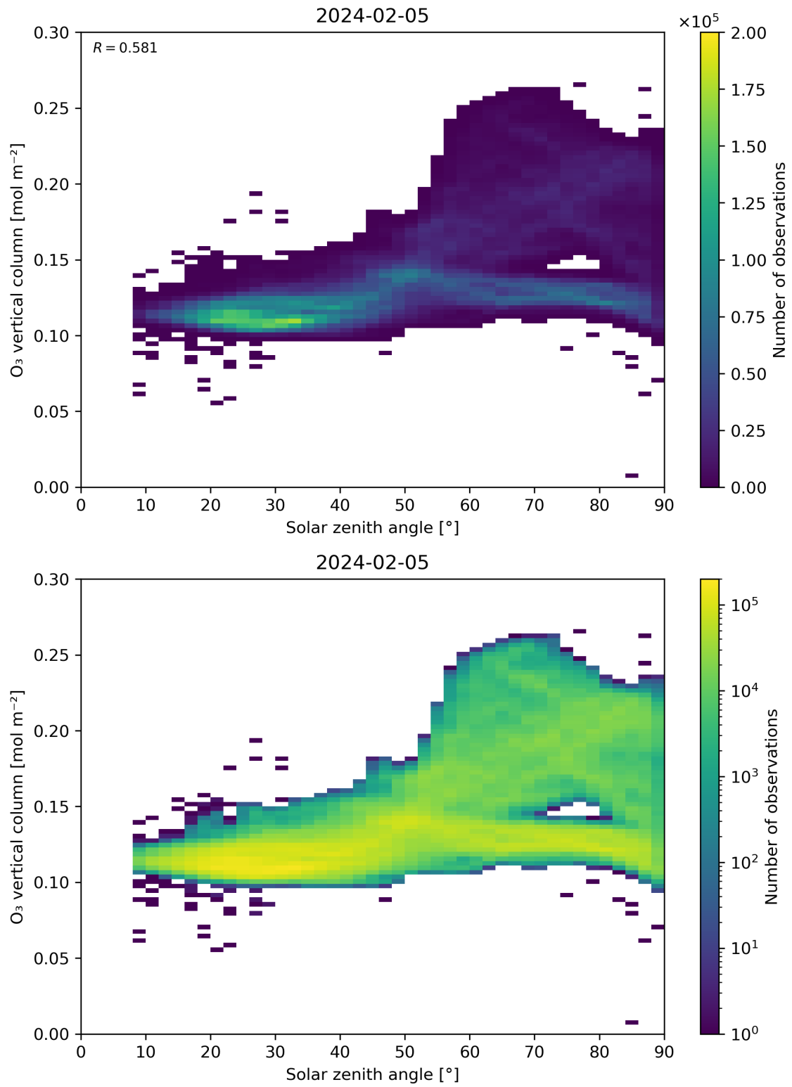
Figure 47: Scatter density plot of “Solar zenith angle” against “O 3 vertical column” for 2024-02-04 to 2024-02-06.
