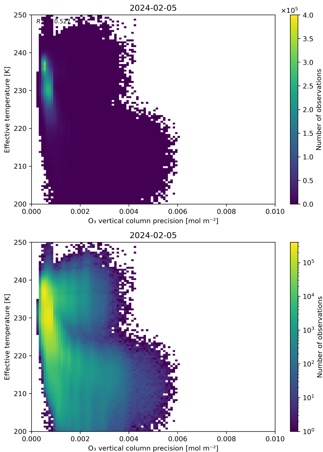
Figure 42: Scatter density plot of “O 3 vertical column precision” against “Effective temperature” for 2024-02-04 to 2024-02-06.
