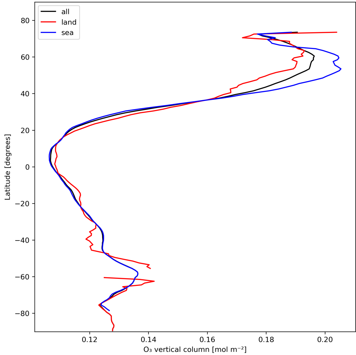
Figure 14: Zonal average of “O 3 vertical column” for 2024-02-04 to 2024-02-06.
