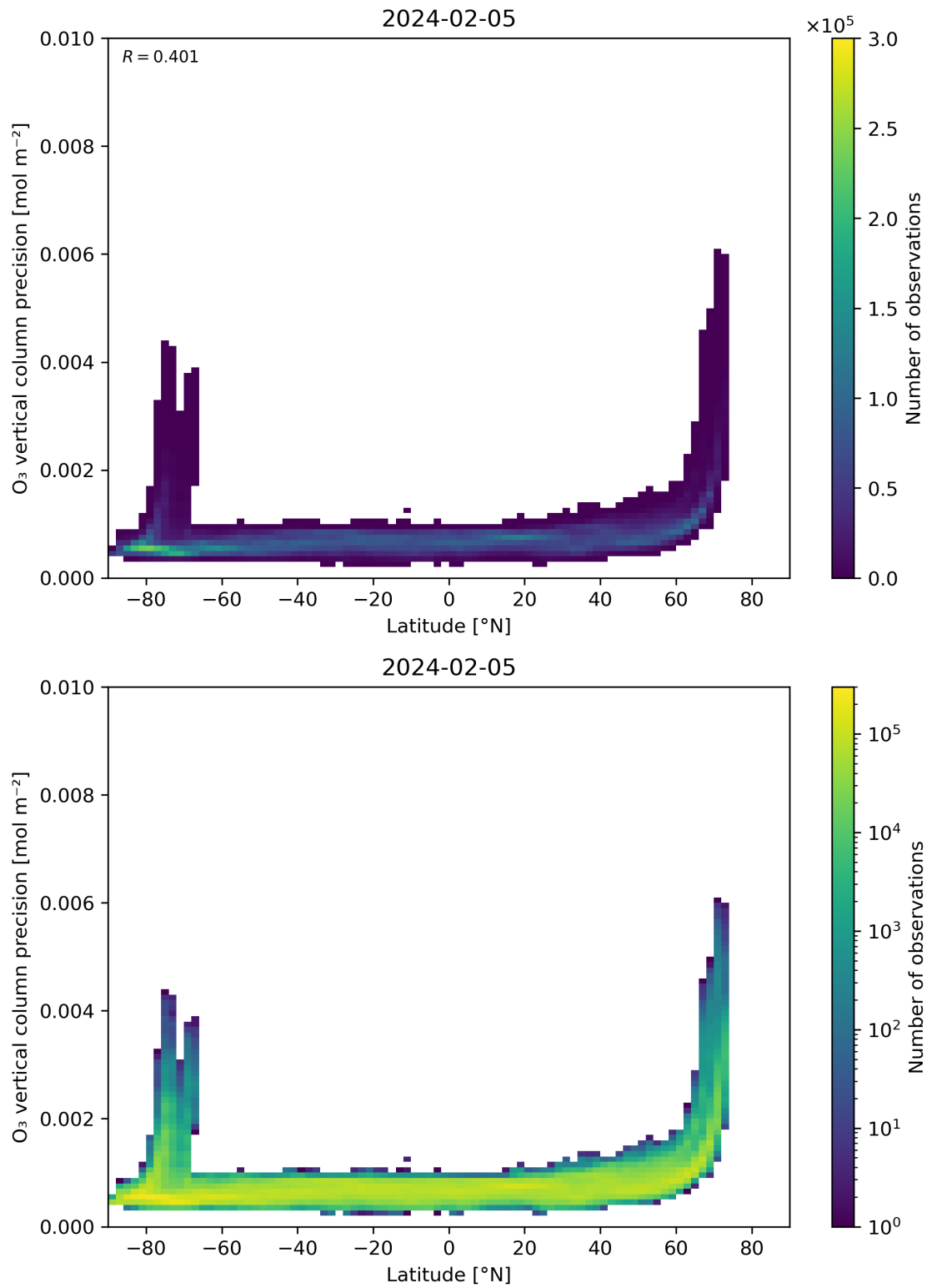
Figure 37: Scatter density plot of “Latitude” against “O 3 vertical column precision” for 2024-02-04 to 2024-02-06.
