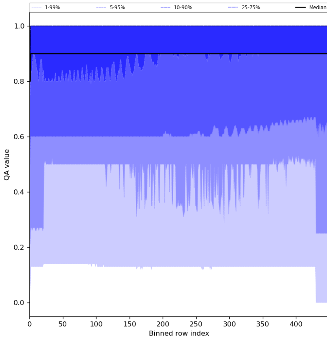
Figure 27: Along track statistics of “QA value” for 2024-02-04 to 2024-02-06
