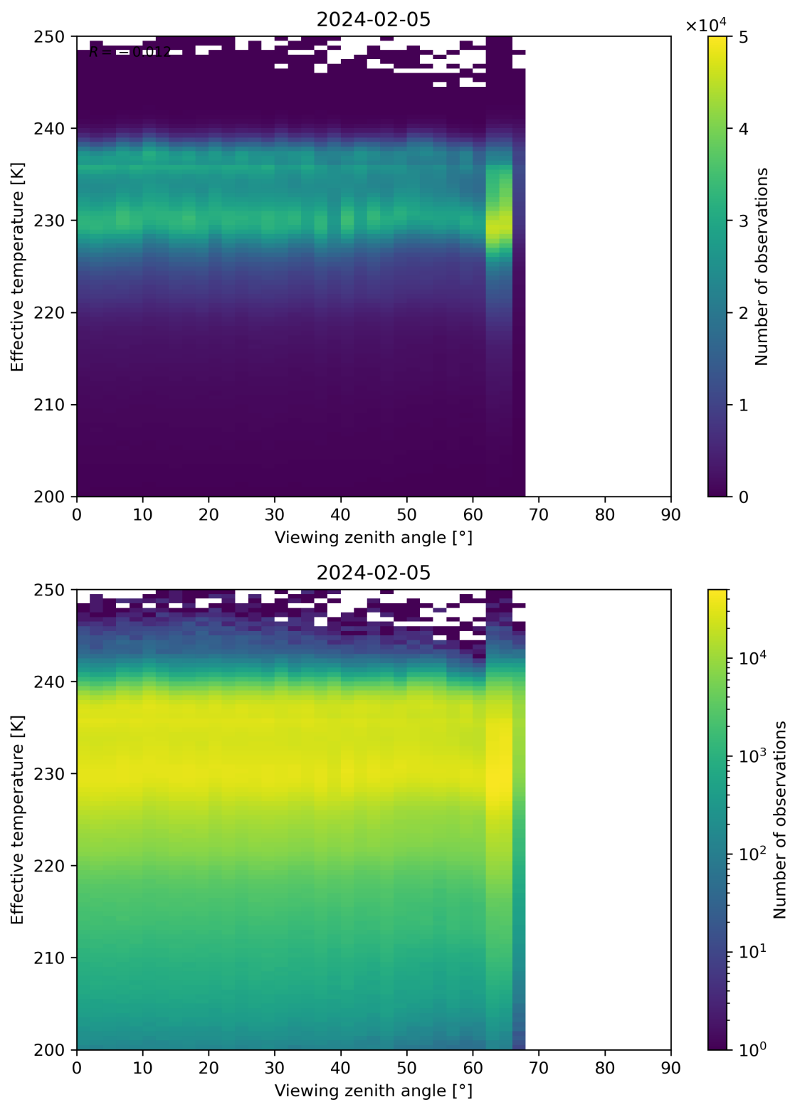
Figure 50: Scatter density plot of “Viewing zenith angle” against “Effective temperature” for 2024-02-04 to 2024-02-06.
