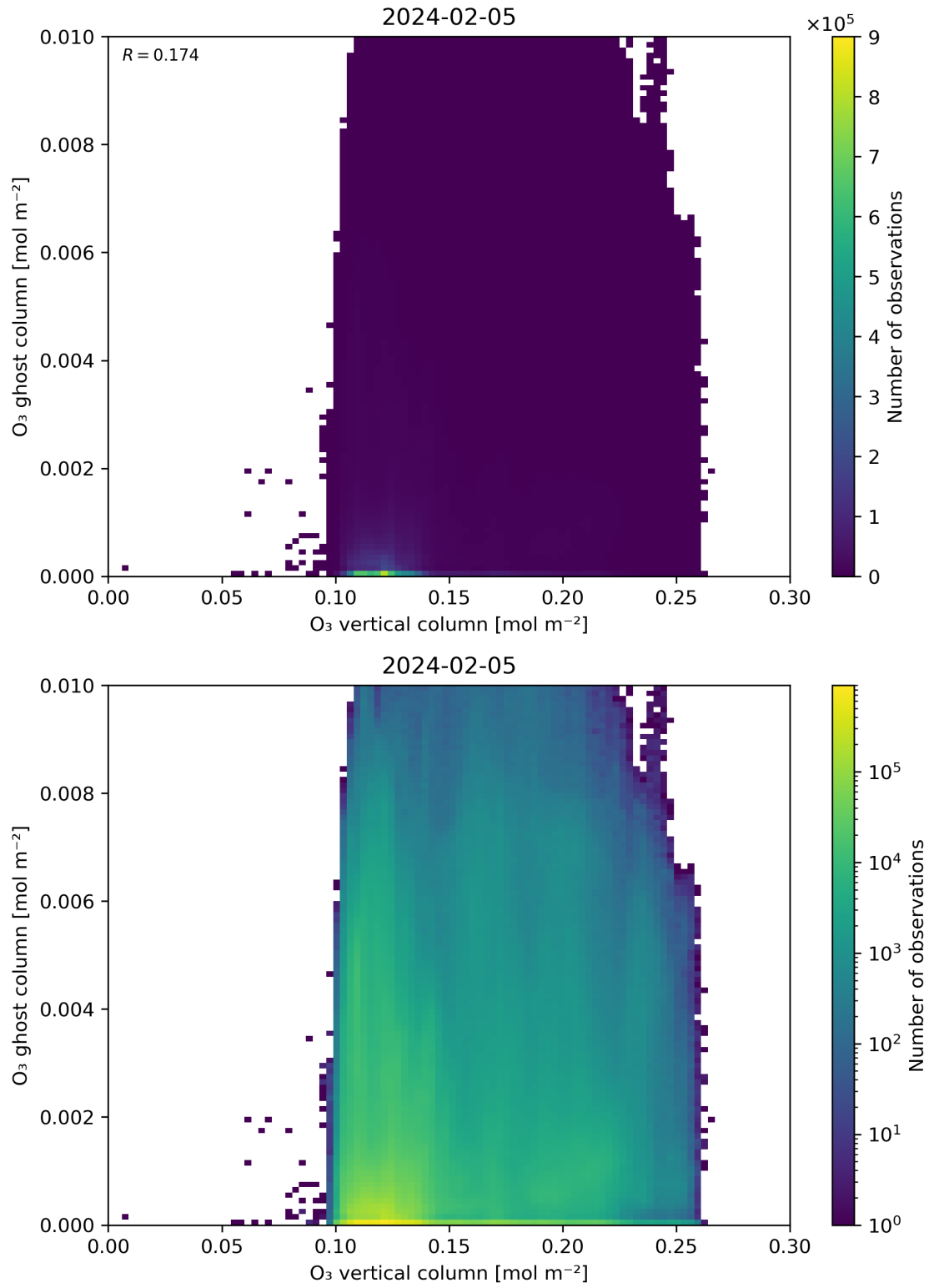
Figure 40: Scatter density plot of “O 3 vertical column” against “O 3 ghost column” for 2024-02-04 to 2024-02-06.
