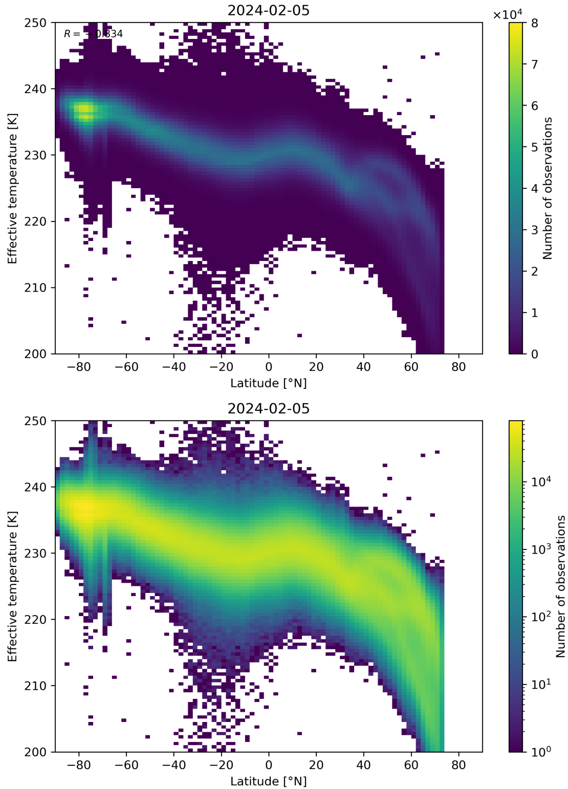
Figure 34: Scatter density plot of “Latitude” against “Effective temperature” for 2024-02-04 to 2024-02-06.
