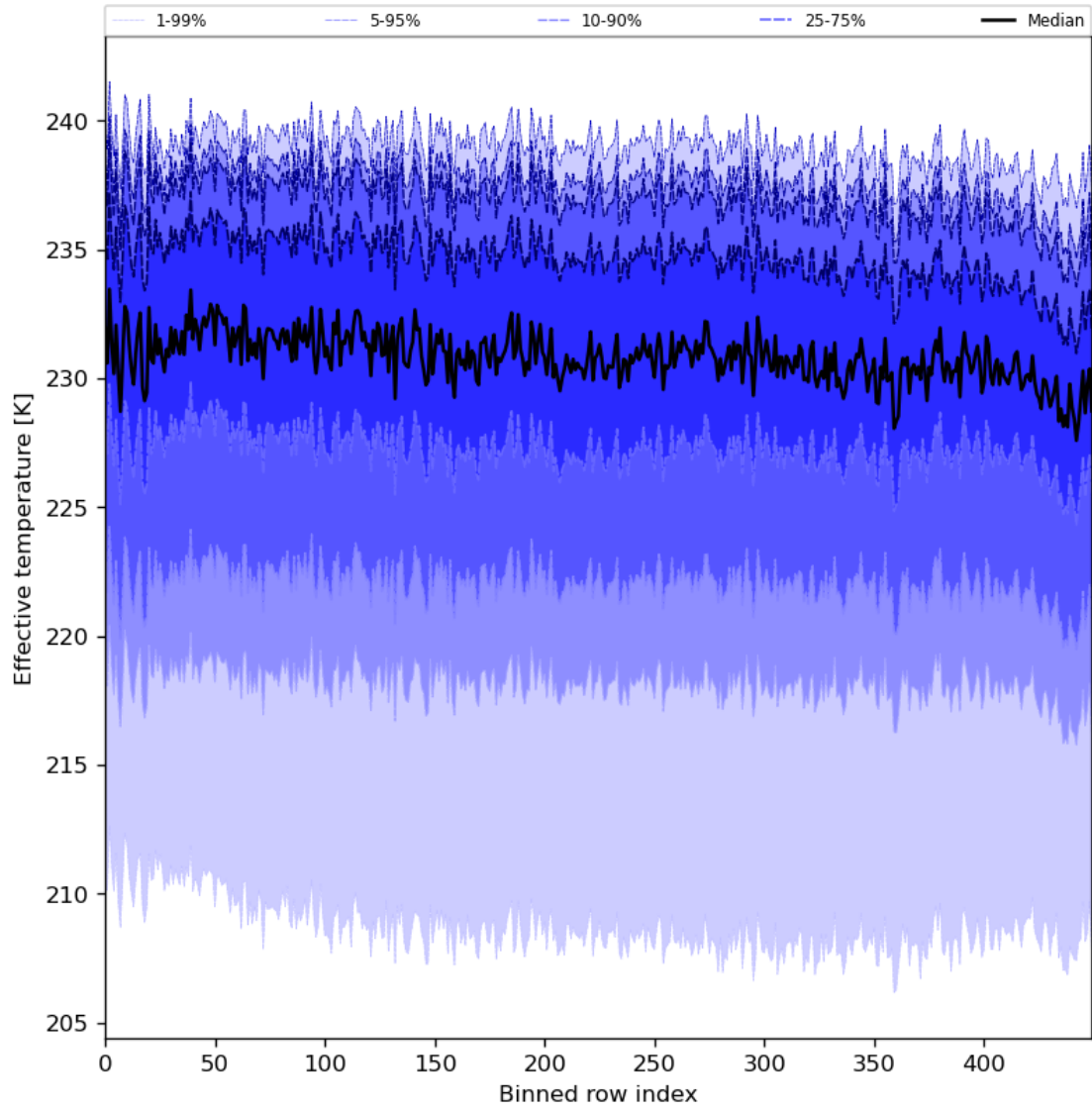
Figure 31: Along track statistics of “Effective temperature” for 2024-02-04 to 2024-02-06
