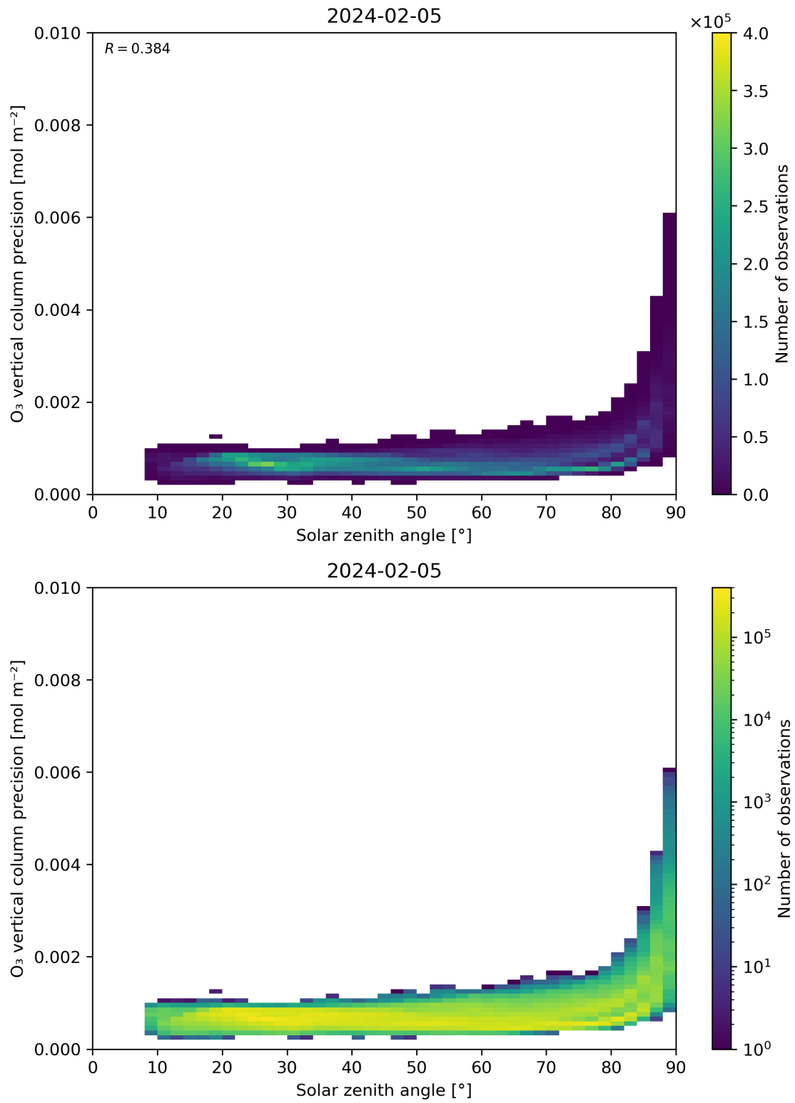
Figure 48: Scatter density plot of “Solar zenith angle” against “O 3 vertical column precision” for 2024-02-04 to 2024-02-06.
