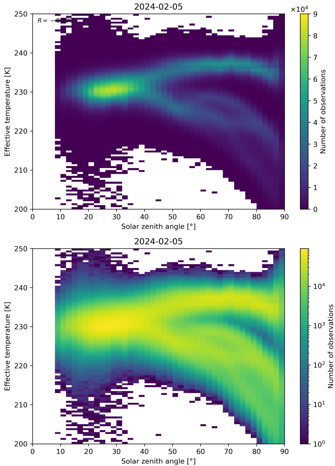
Figure 45: Scatter density plot of “Solar zenith angle” against “Effective temperature” for 2024-02-04 to 2024-02-06.
