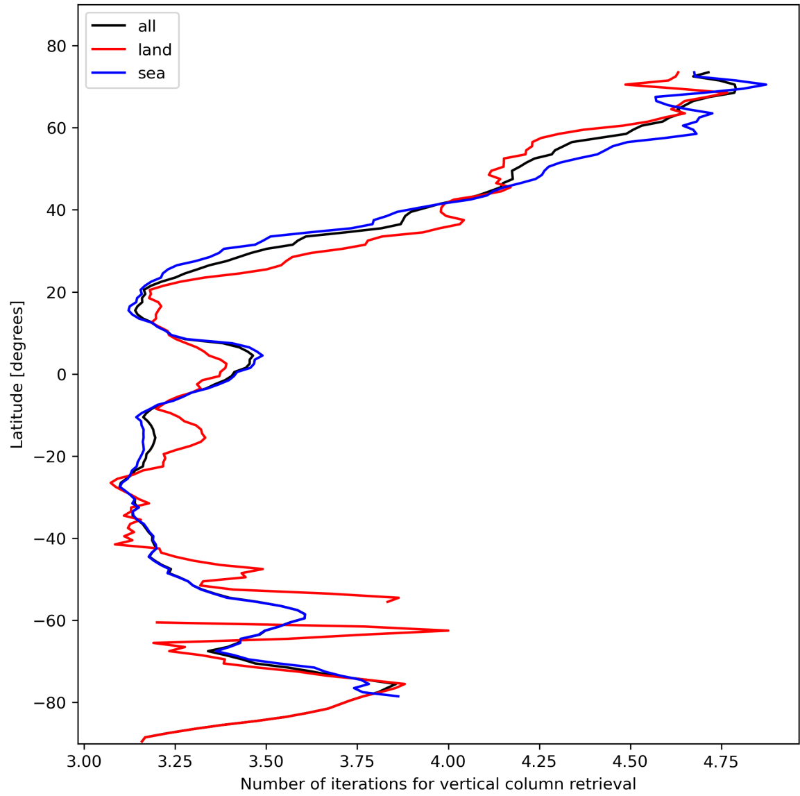
Figure 19: Zonal average of “Number of iterations for vertical column retrieval” for 2024-02-04 to 2024-02-06.
