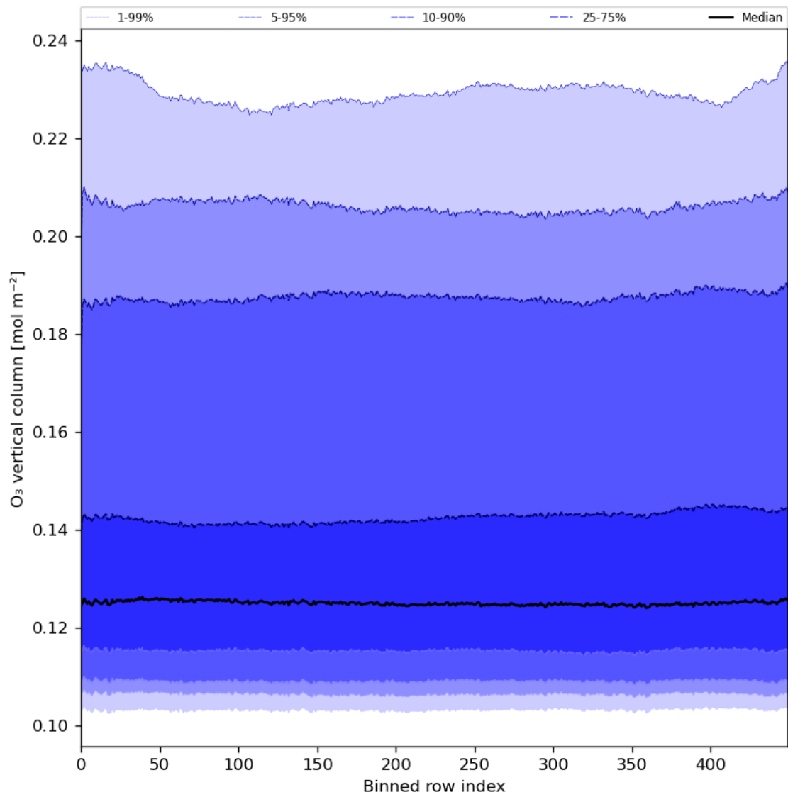
Figure 28: Along track statistics of “O 3 vertical column” for 2024-02-04 to 2024-02-06
