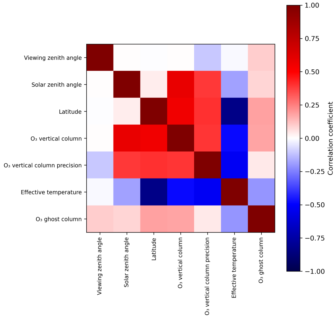
Figure 2: Map of correlation matrix for 2024-02-04 to 2024-02-06.
