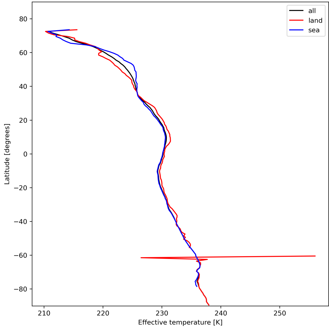
Figure 17: Zonal average of “Effective temperature” for 2024-02-04 to 2024-02-06.
