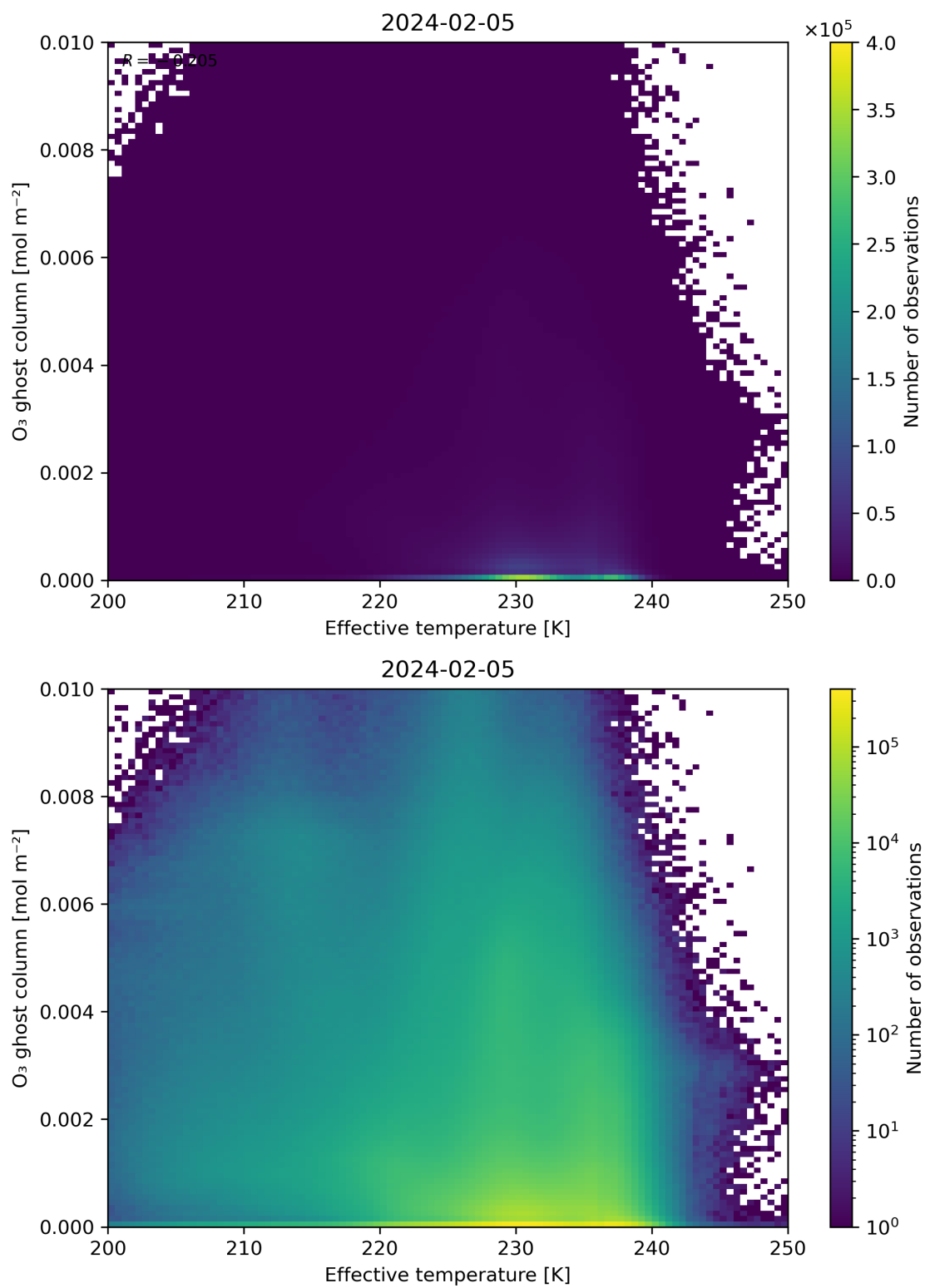
Figure 38: Scatter density plot of “Effective temperature” against “O 3 ghost column” for 2024-02-04 to 2024-02-06.
