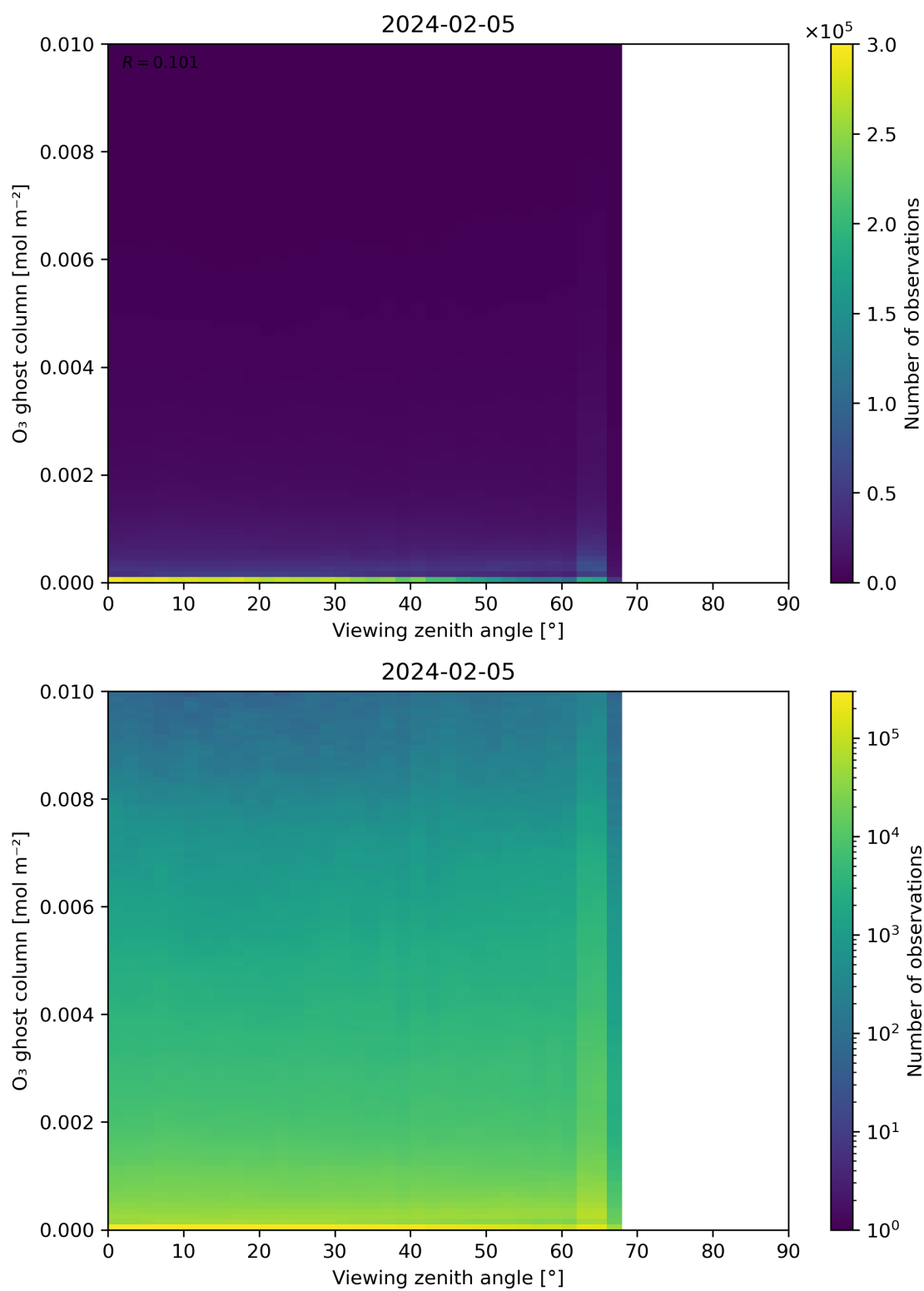
Figure 51: Scatter density plot of “Viewing zenith angle” against “O 3 ghost column” for 2024-02-04 to 2024-02-06.
