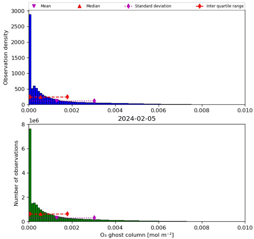
Figure 25: Histogram of “O 3 ghost column” for 2024-02-04 to 2024-02-06
