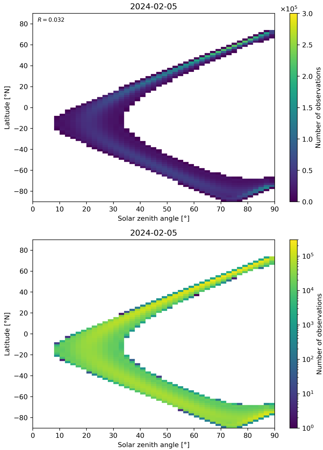
Figure 44: Scatter density plot of “Solar zenith angle” against “Latitude” for 2024-02-04 to 2024-02-06.
