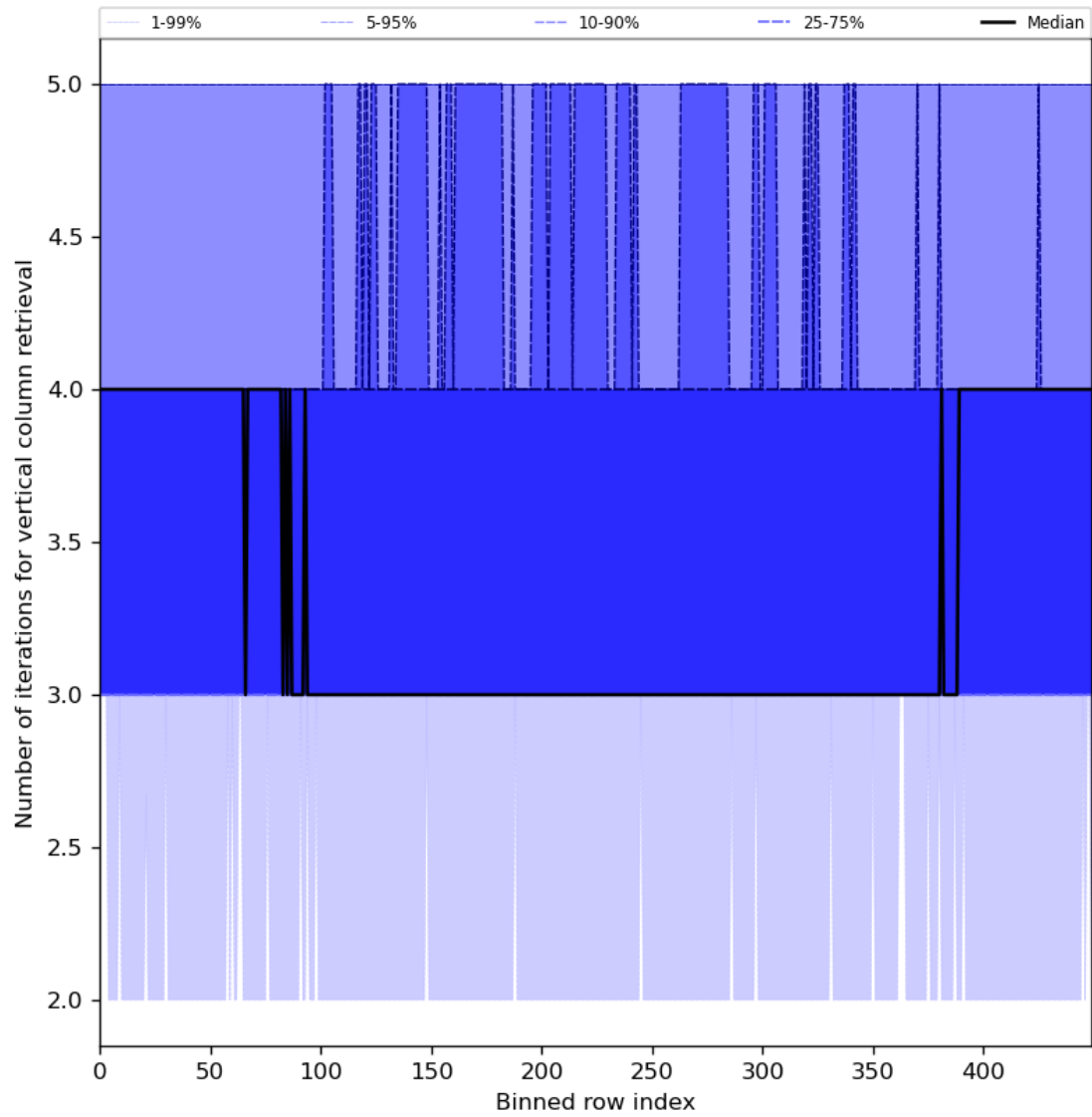
Figure 33: Along track statistics of “Number of iterations for vertical column retrieval” for 2024-02-04 to 2024-02-06
