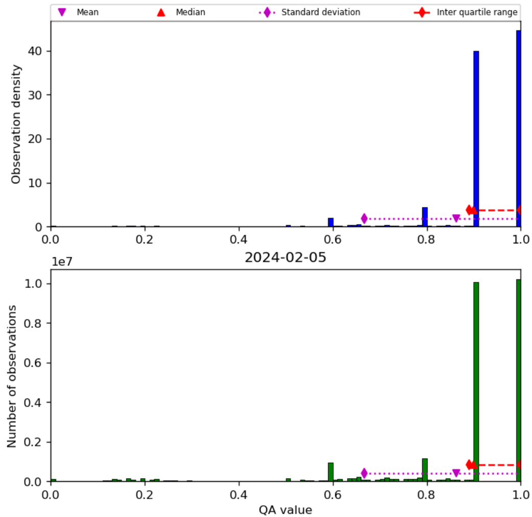
Figure 20: Histogram of “QA value” for 2024-02-04 to 2024-02-06
