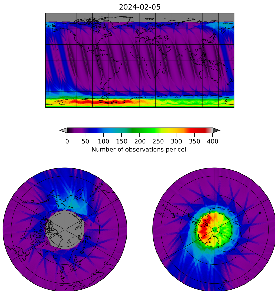
Figure 12: Map of the number of observations for 2024-02-04 to 2024-02-06
