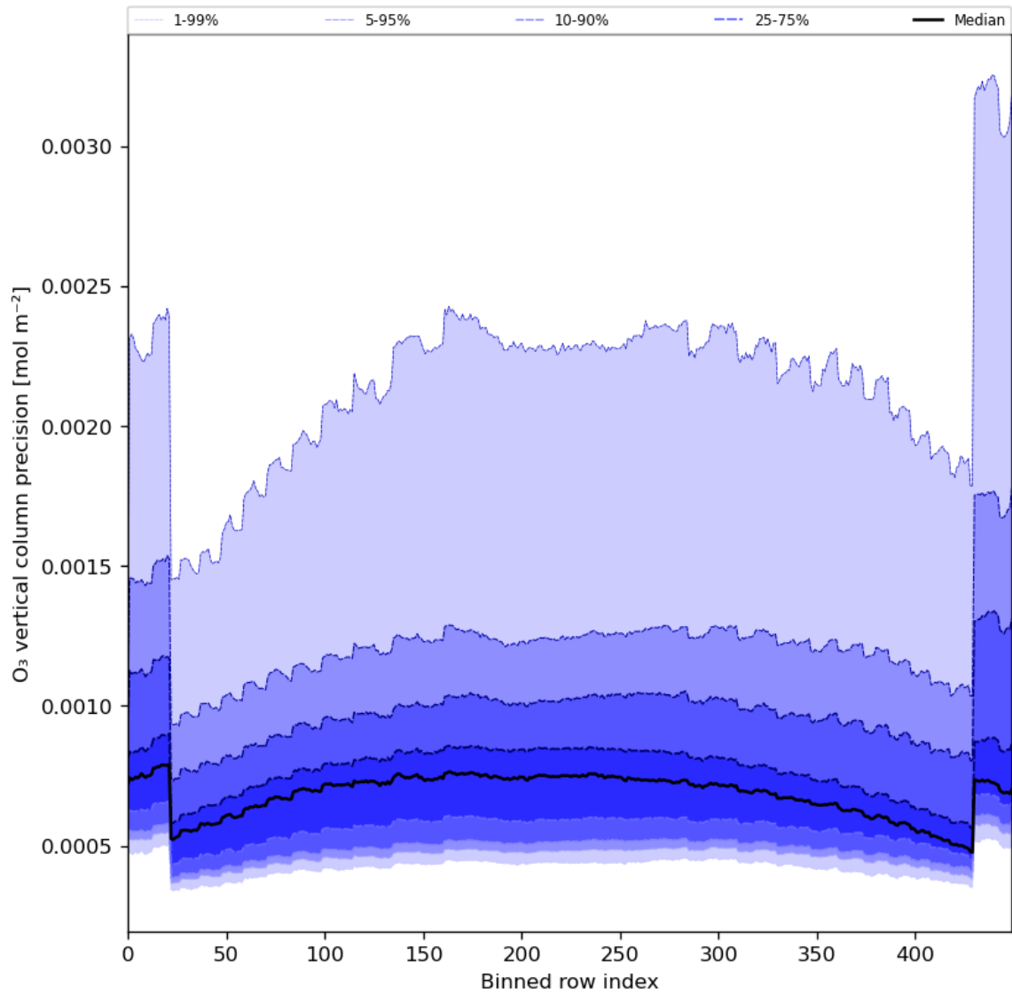
Figure 29: Along track statistics of “O 3 vertical column precision” for 2024-02-04 to 2024-02-06
