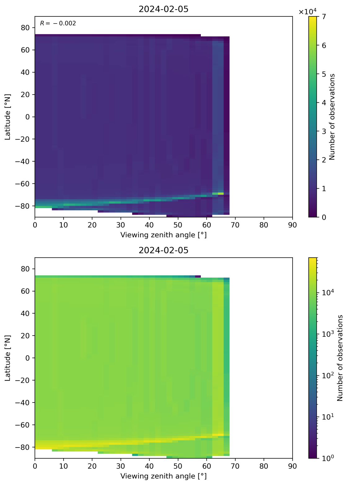
Figure 49: Scatter density plot of “Viewing zenith angle” against “Latitude” for 2024-02-04 to 2024-02-06.
