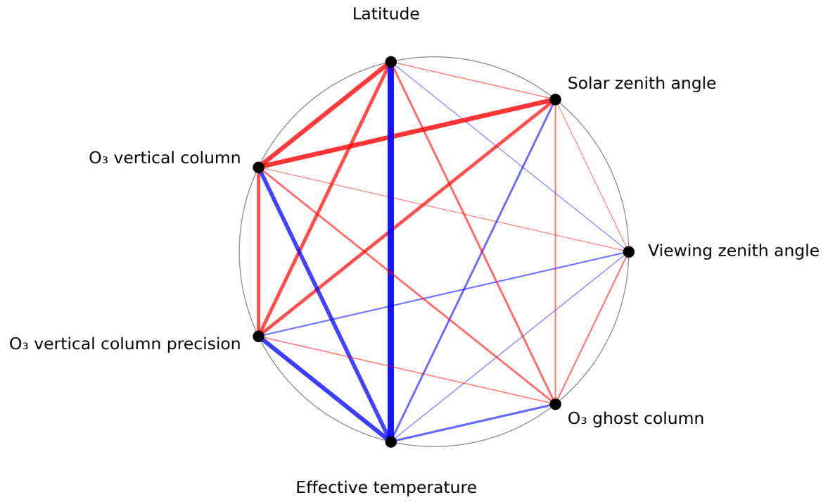
Figure 1: Map of correlation graph for 2024-02-04 to 2024-02-06.
