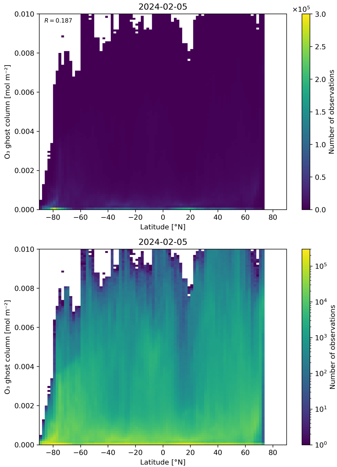
Figure 35: Scatter density plot of “Latitude” against “O 3 ghost column” for 2024-02-04 to 2024-02-06.
