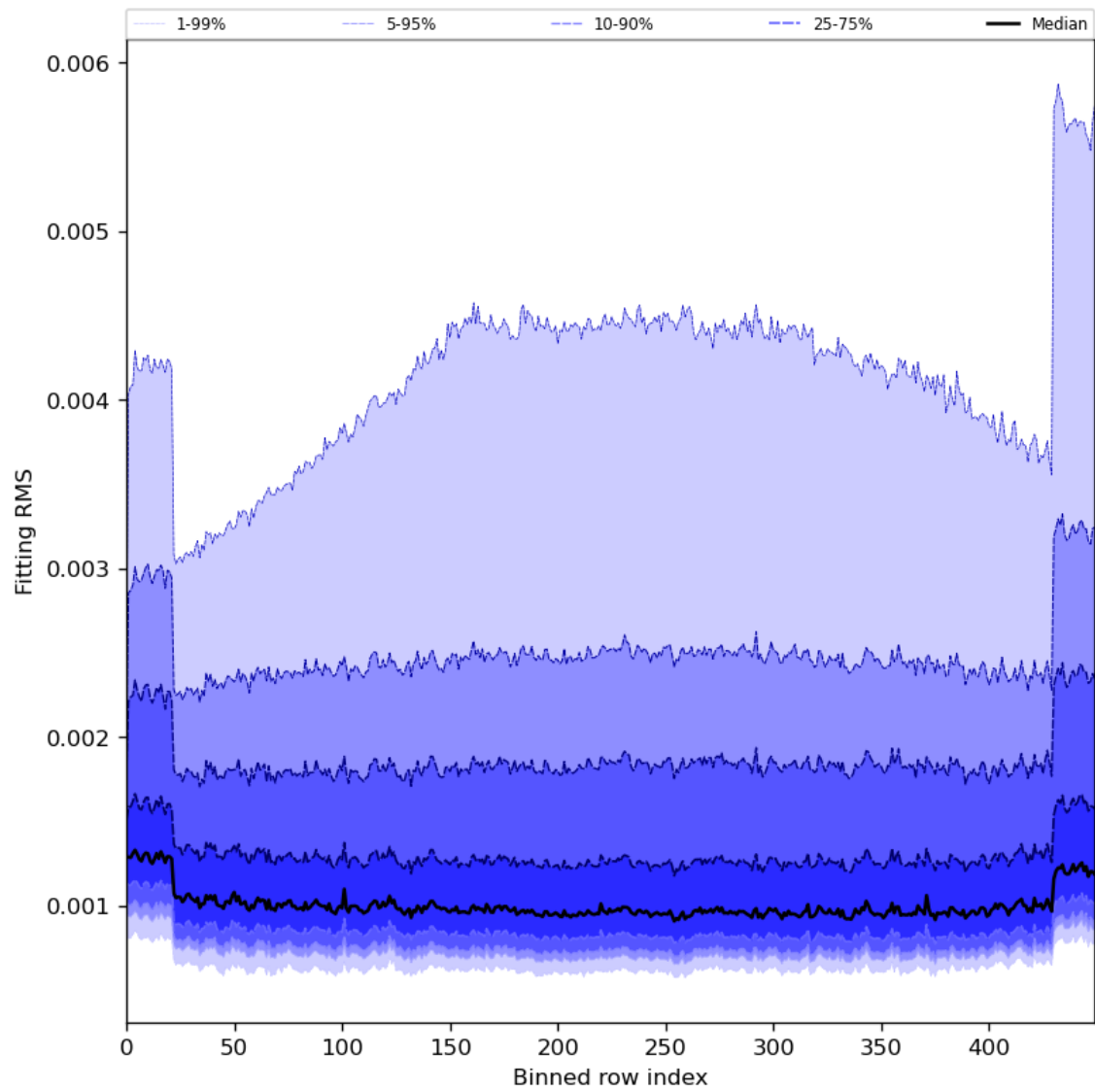
Figure 30: Along track statistics of “Fitting RMS” for 2024-02-04 to 2024-02-06
