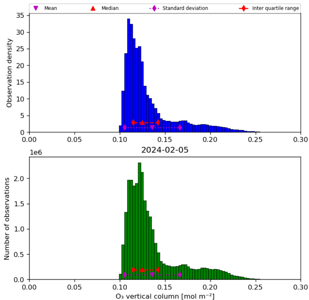
Figure 21: Histogram of “O 3 vertical column” for 2024-02-04 to 2024-02-06
