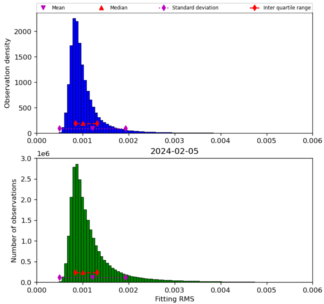
Figure 23: Histogram of “Fitting RMS” for 2024-02-04 to 2024-02-06
