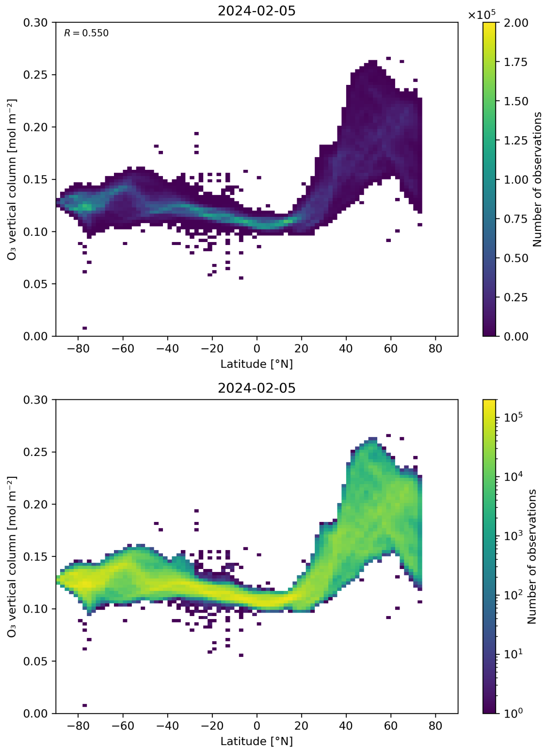
Figure 36: Scatter density plot of “Latitude” against “O 3 vertical column” for 2024-02-04 to 2024-02-06.
