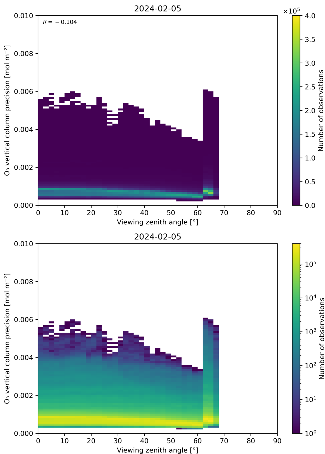
Figure 53: Scatter density plot of “Viewing zenith angle” against “O 3 vertical column precision” for 2024-02-04 to 2024-02-06.
