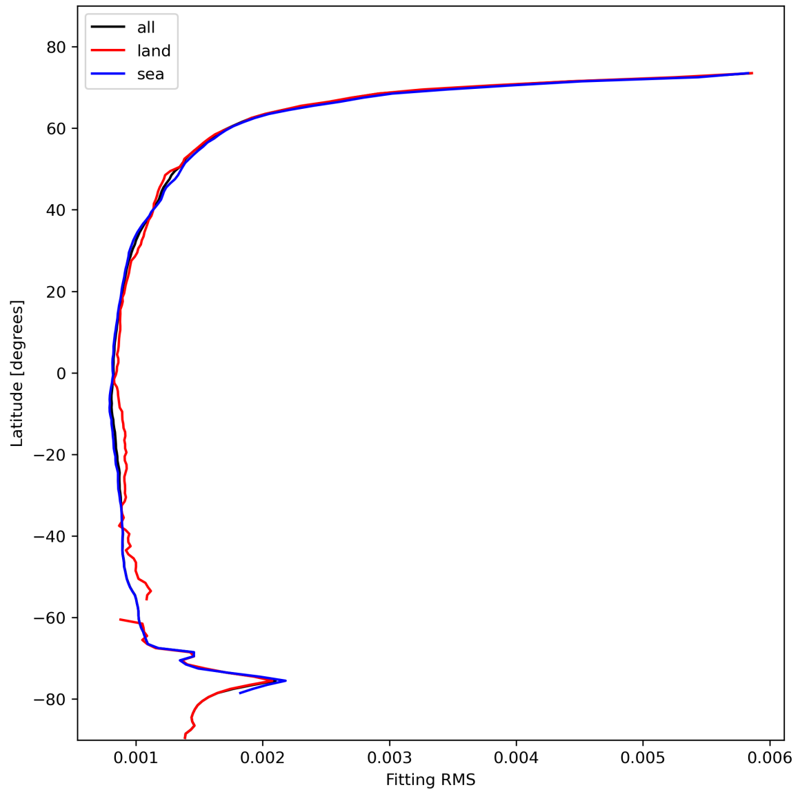
Figure 16: Zonal average of “Fitting RMS” for 2024-02-04 to 2024-02-06.
