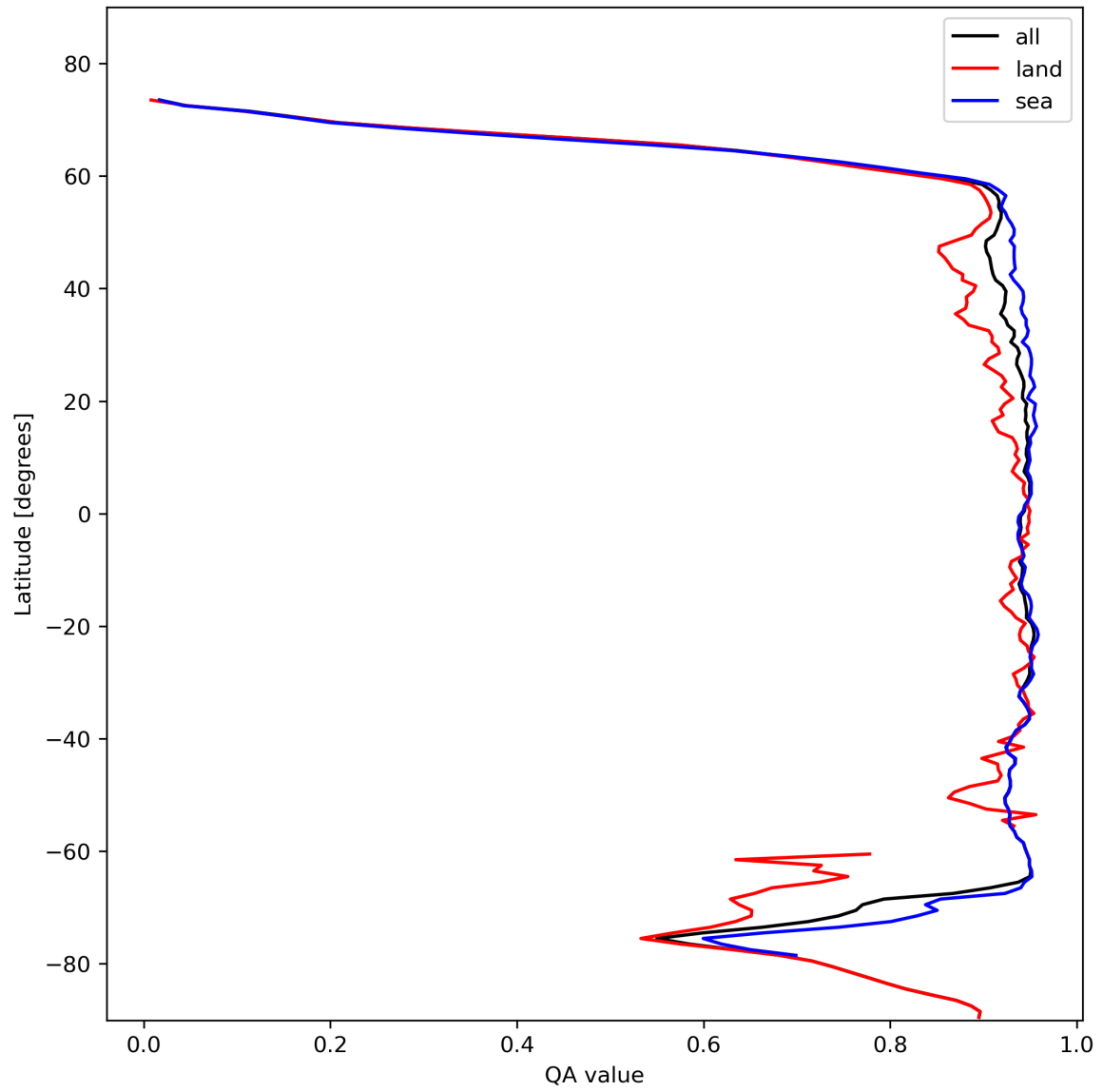
Figure 13: Zonal average of “QA value” for 2024-02-04 to 2024-02-06.
