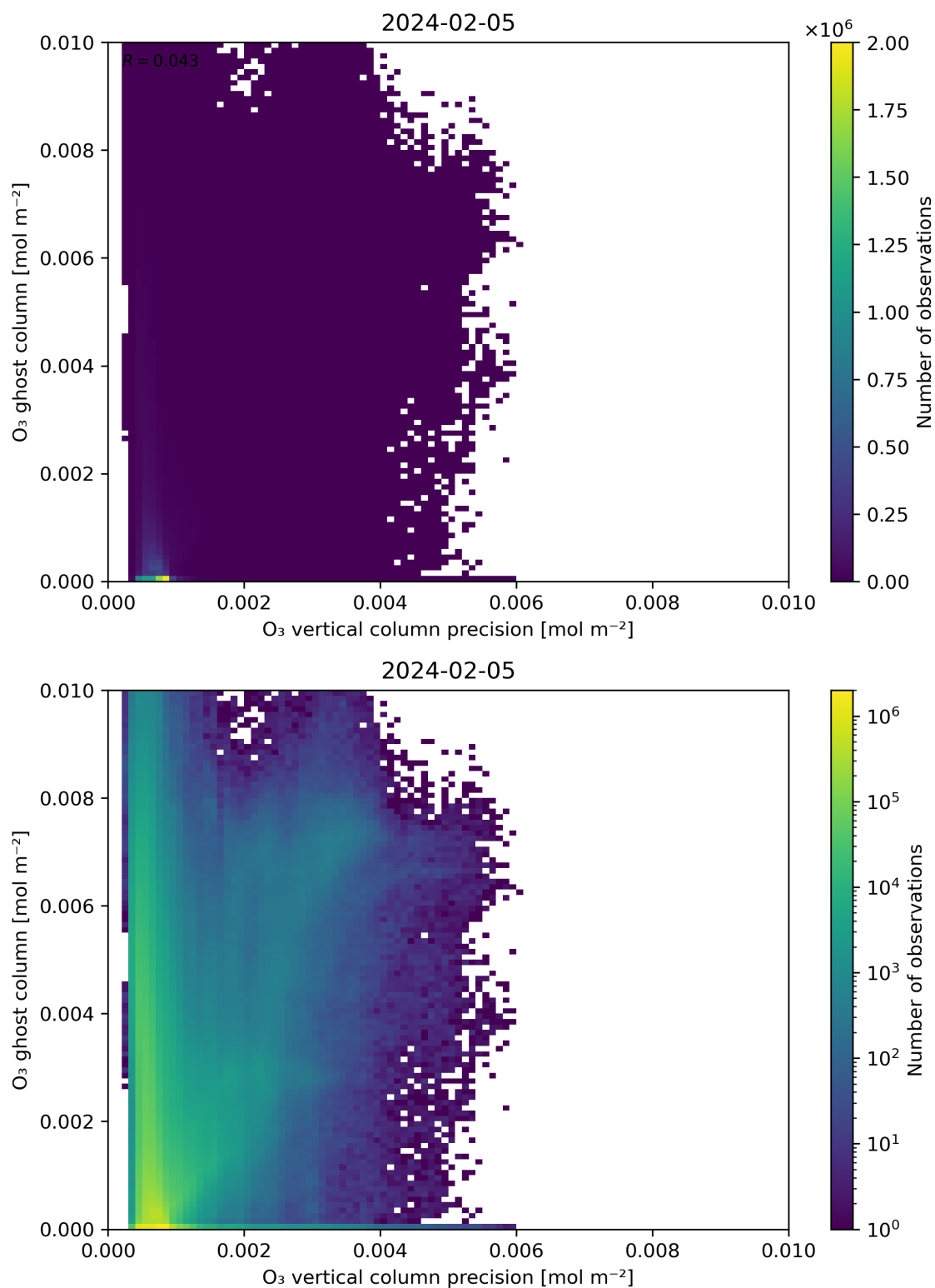
Figure 43: Scatter density plot of “ \text{O}_3 vertical column precision” against “ \text{O}_3 ghost column” for 2024-02-04 to 2024-02-06.
