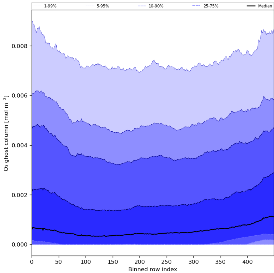
Figure 32: Along track statistics of “O 3 ghost column” for 2024-02-04 to 2024-02-06
