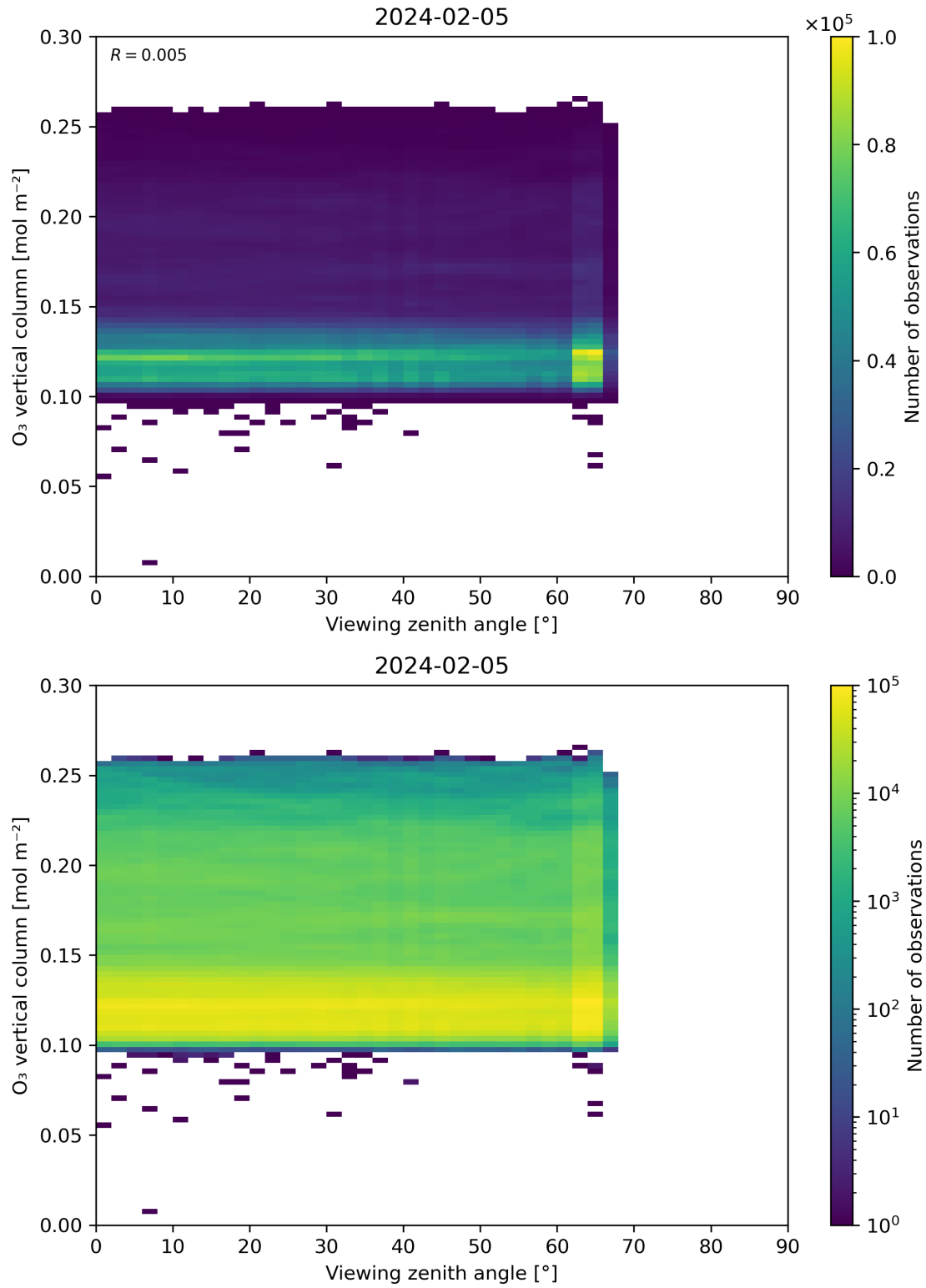
Figure 52: Scatter density plot of “Viewing zenith angle” against “O 3 vertical column” for 2024-02-04 to 2024-02-06.
