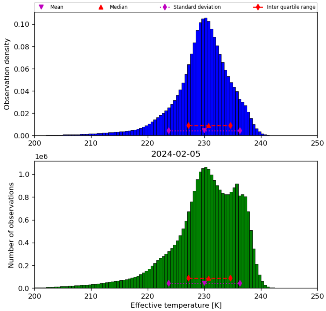
Figure 24: Histogram of “Effective temperature” for 2024-02-04 to 2024-02-06
