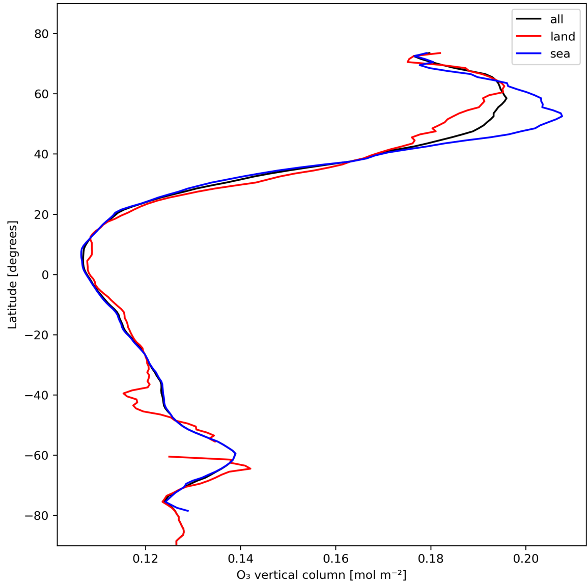
Figure 14: Zonal average of “O 3 vertical column” for 2024-02-06 to 2024-02-07.
