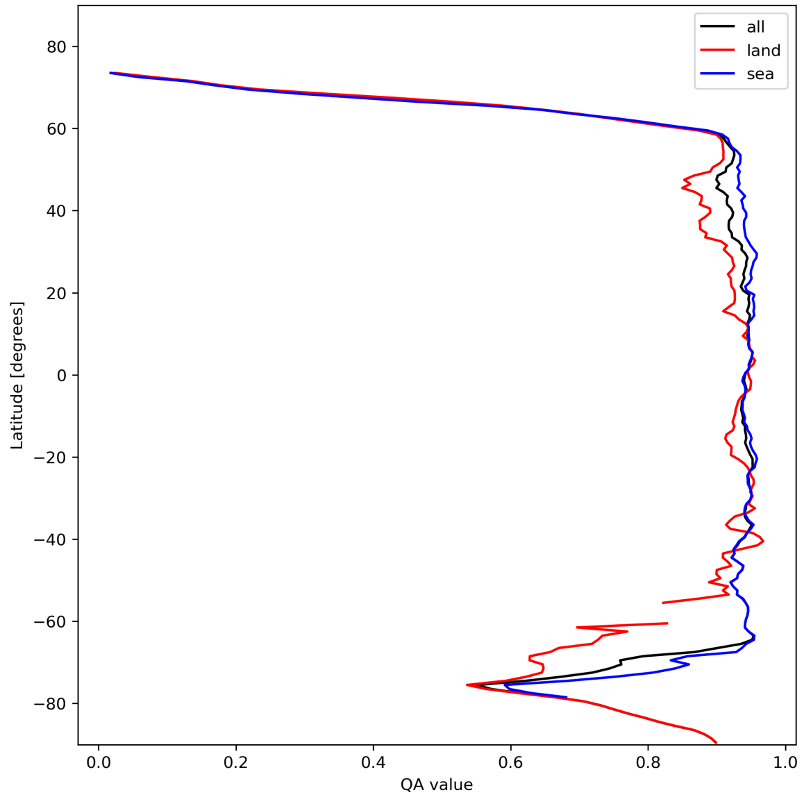
Figure 13: Zonal average of “QA value” for 2024-02-06 to 2024-02-07.
