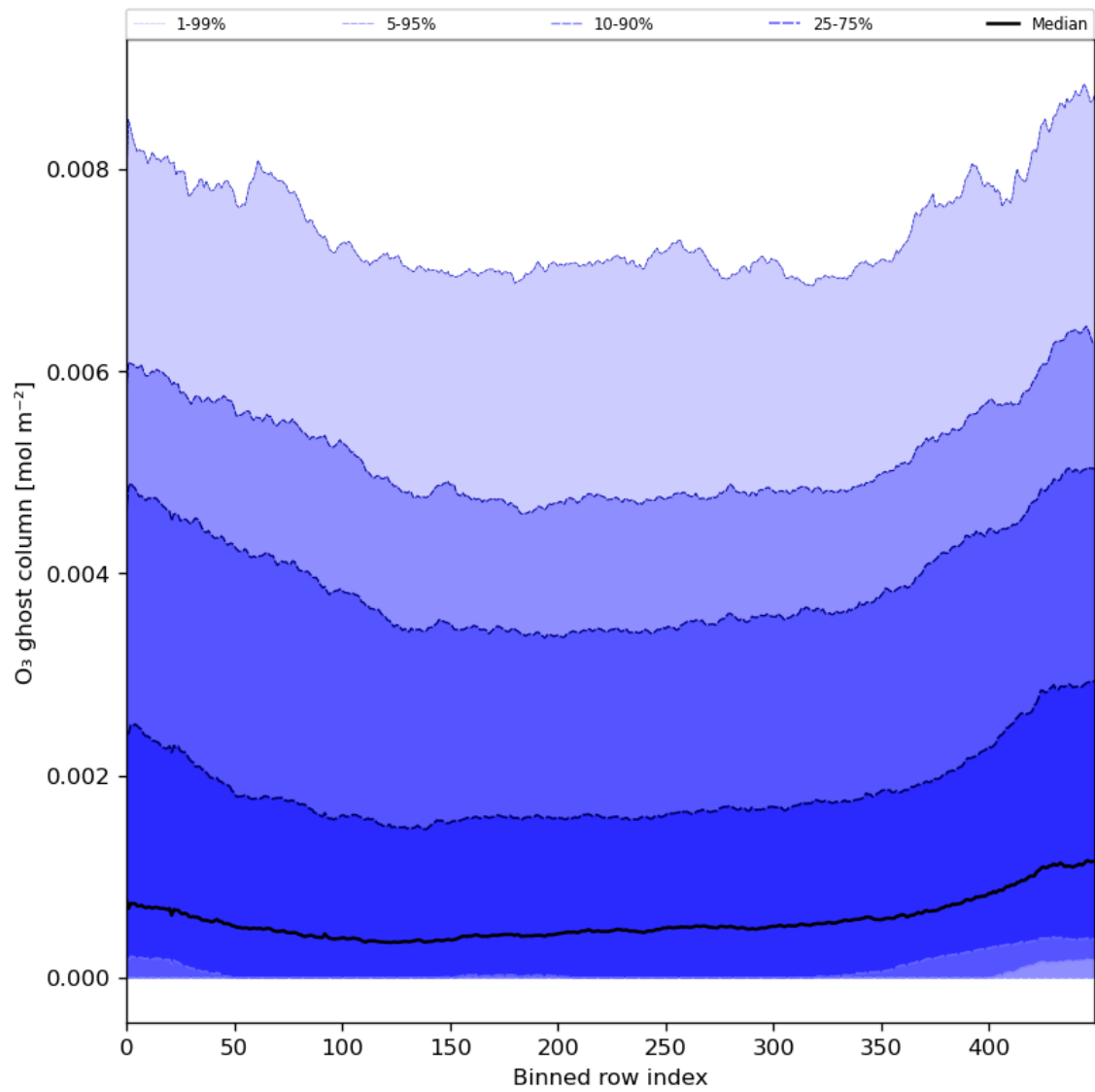
Figure 32: Along track statistics of “O 3 ghost column” for 2024-02-06 to 2024-02-07
