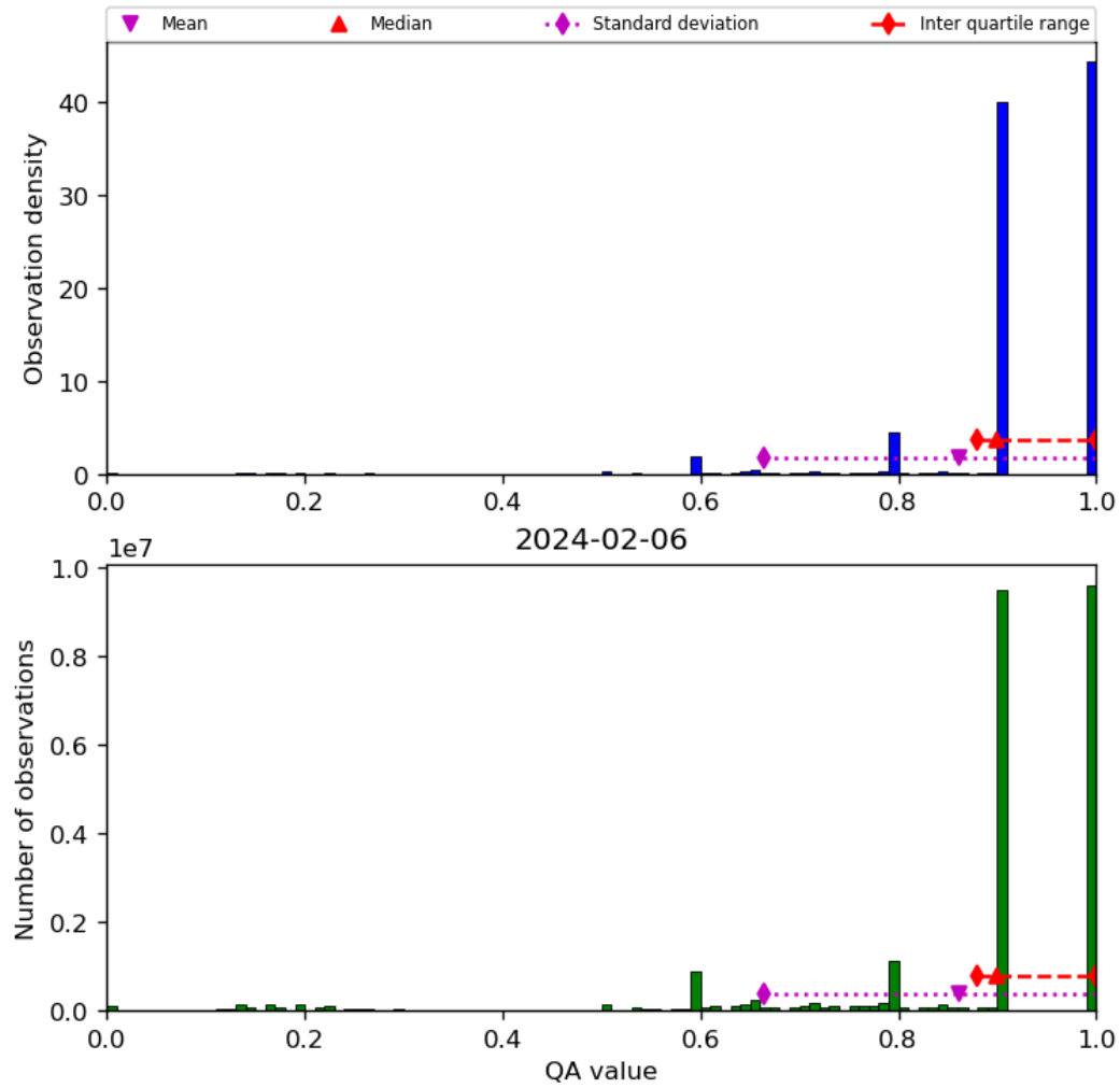
Figure 20: Histogram of “QA value” for 2024-02-06 to 2024-02-07
