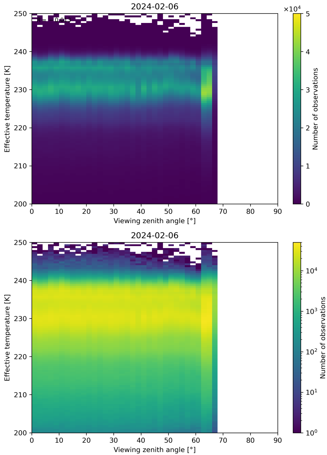
Figure 50: Scatter density plot of “Viewing zenith angle” against “Effective temperature” for 2024-02-06 to 2024-02-07.
