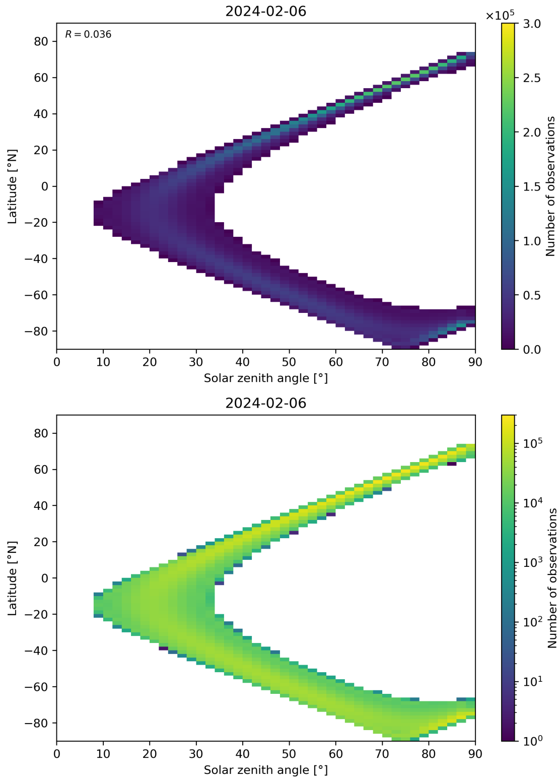
Figure 44: Scatter density plot of “Solar zenith angle” against “Latitude” for 2024-02-06 to 2024-02-07.
