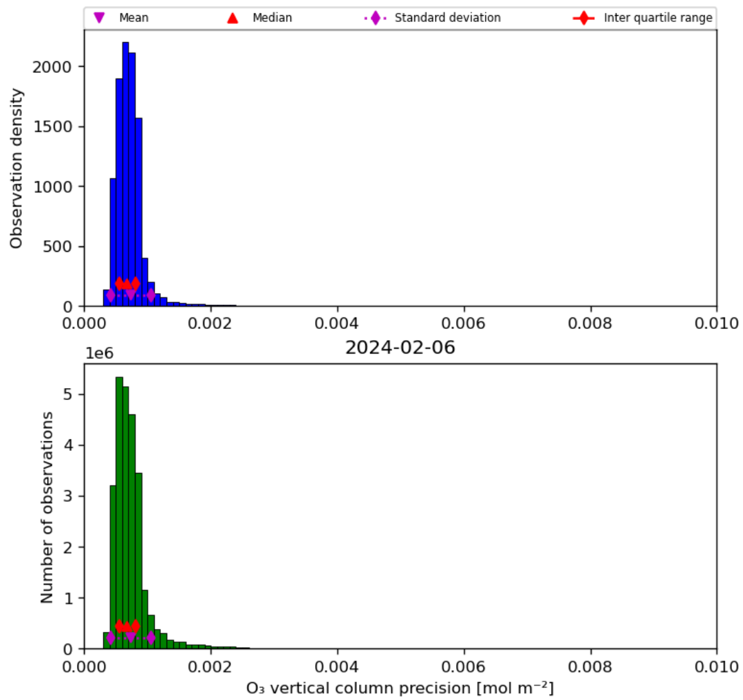
Figure 22: Histogram of “O 3 vertical column precision” for 2024-02-06 to 2024-02-07
