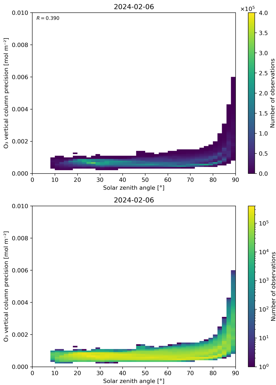
Figure 48: Scatter density plot of “Solar zenith angle” against “O 3 vertical column precision” for 2024-02-06 to 2024-02-07.
