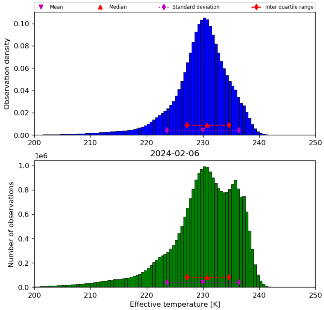
Figure 24: Histogram of “Effective temperature” for 2024-02-06 to 2024-02-07
