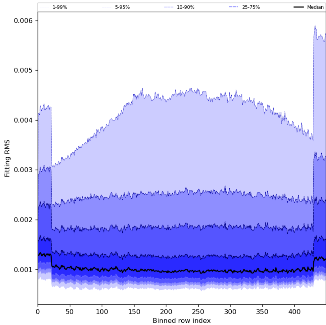
Figure 30: Along track statistics of “Fitting RMS” for 2024-02-06 to 2024-02-07
