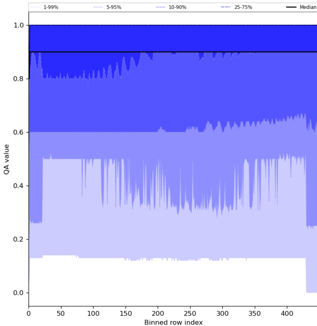
Figure 27: Along track statistics of “QA value” for 2024-02-06 to 2024-02-07
