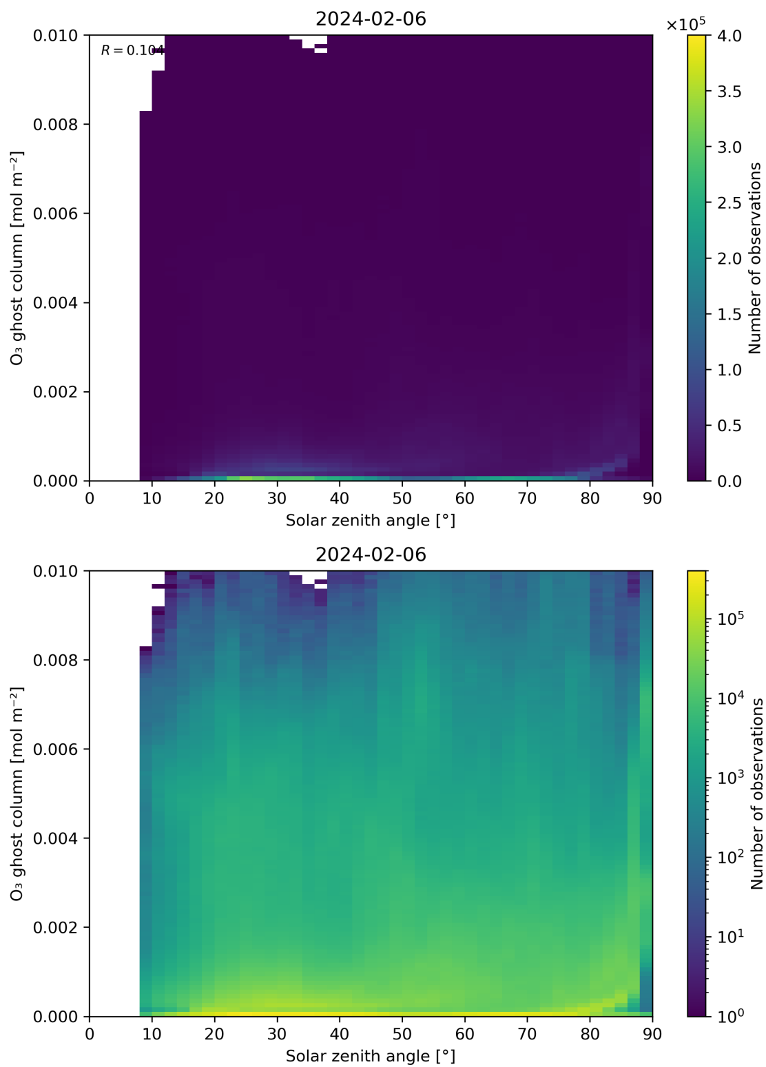
Figure 46: Scatter density plot of “Solar zenith angle” against “O 3 ghost column” for 2024-02-06 to 2024-02-07.
