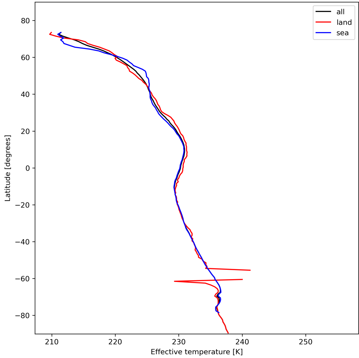
Figure 17: Zonal average of “Effective temperature” for 2024-02-06 to 2024-02-07.
