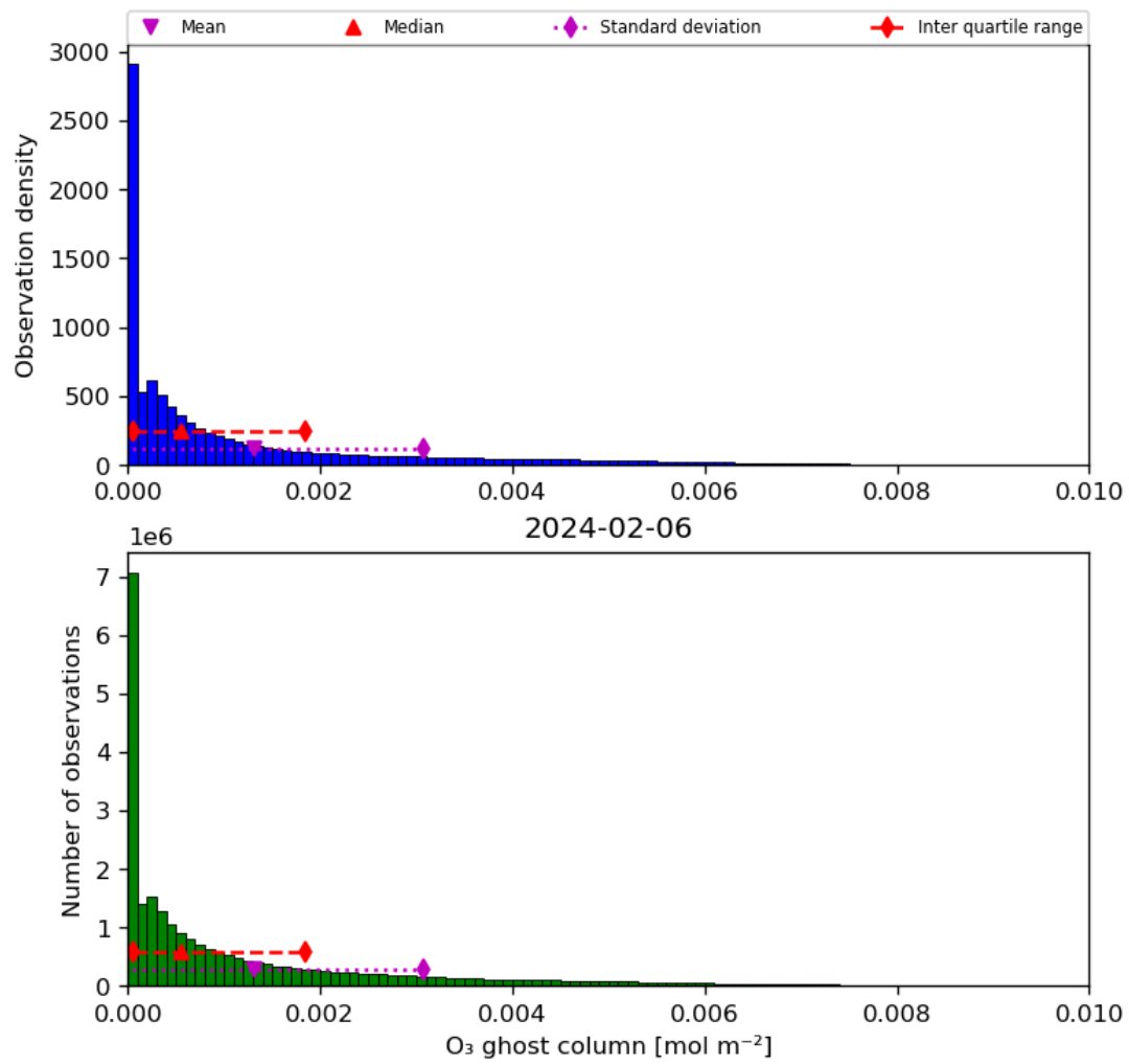
Figure 25: Histogram of “O 3 ghost column” for 2024-02-06 to 2024-02-07
