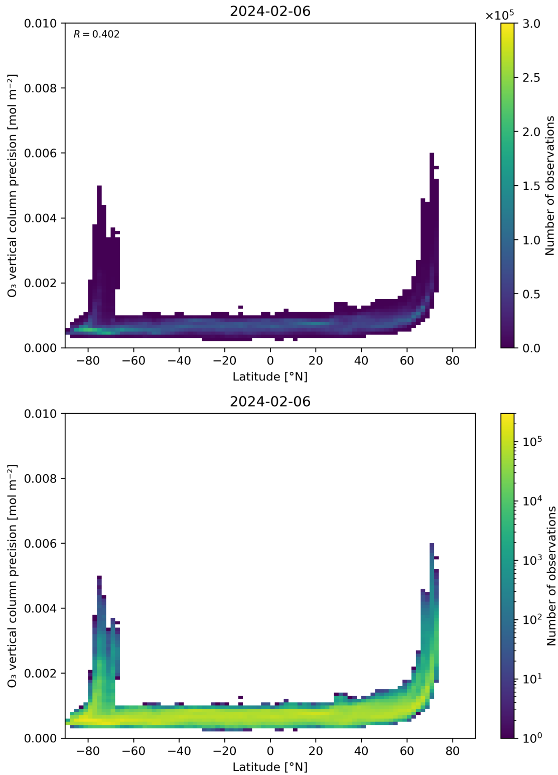
Figure 37: Scatter density plot of “Latitude” against “O 3 vertical column precision” for 2024-02-06 to 2024-02-07.
