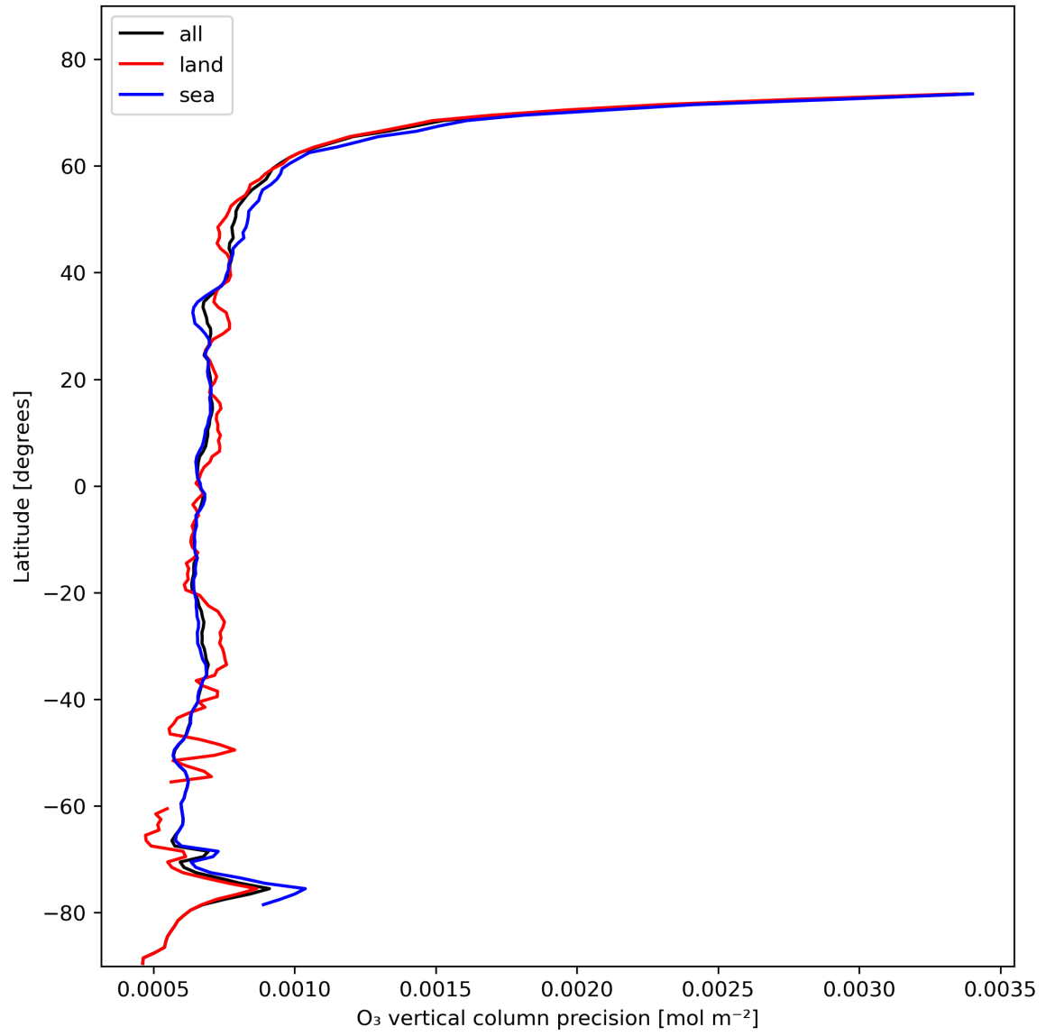
Figure 15: Zonal average of “O 3 vertical column precision” for 2024-02-06 to 2024-02-07.
