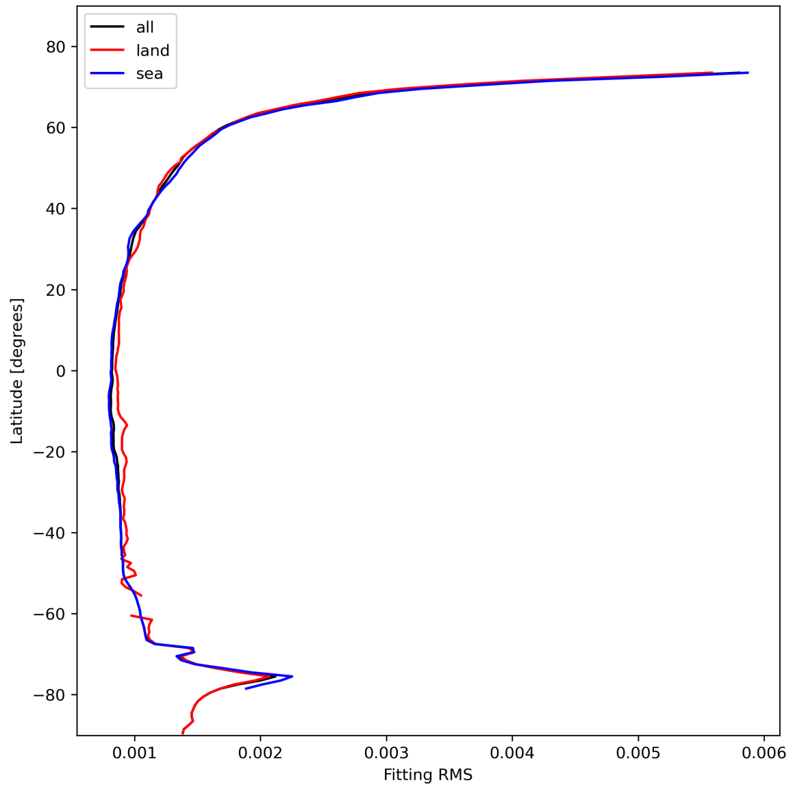
Figure 16: Zonal average of “Fitting RMS” for 2024-02-06 to 2024-02-07.
