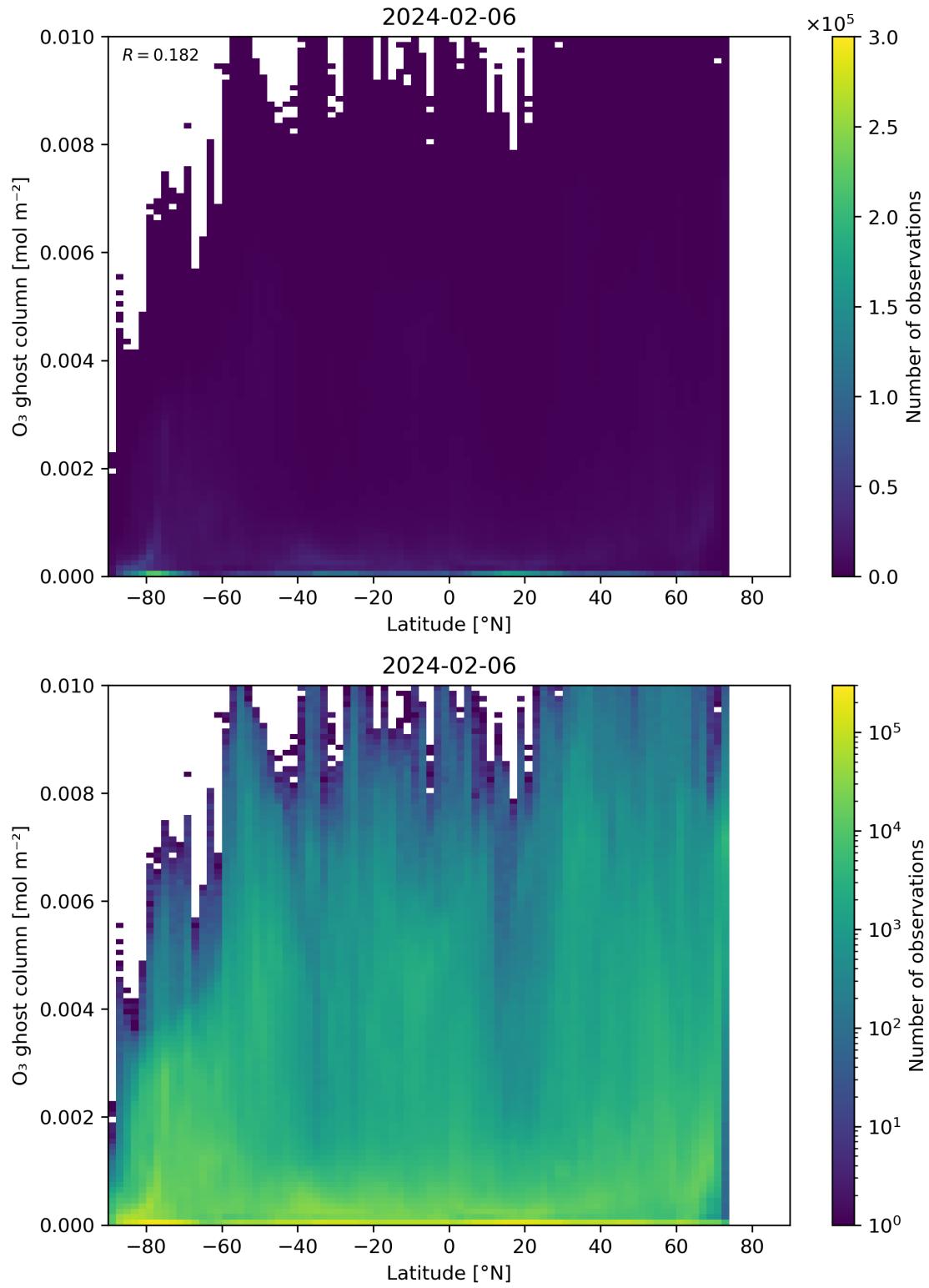
Figure 35: Scatter density plot of “Latitude” against “O 3 ghost column” for 2024-02-06 to 2024-02-07.
