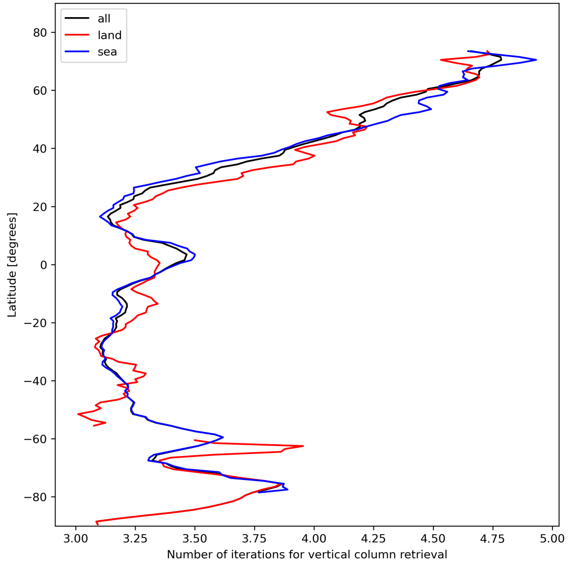
Figure 19: Zonal average of “Number of iterations for vertical column retrieval” for 2024-02-06 to 2024-02-07.
