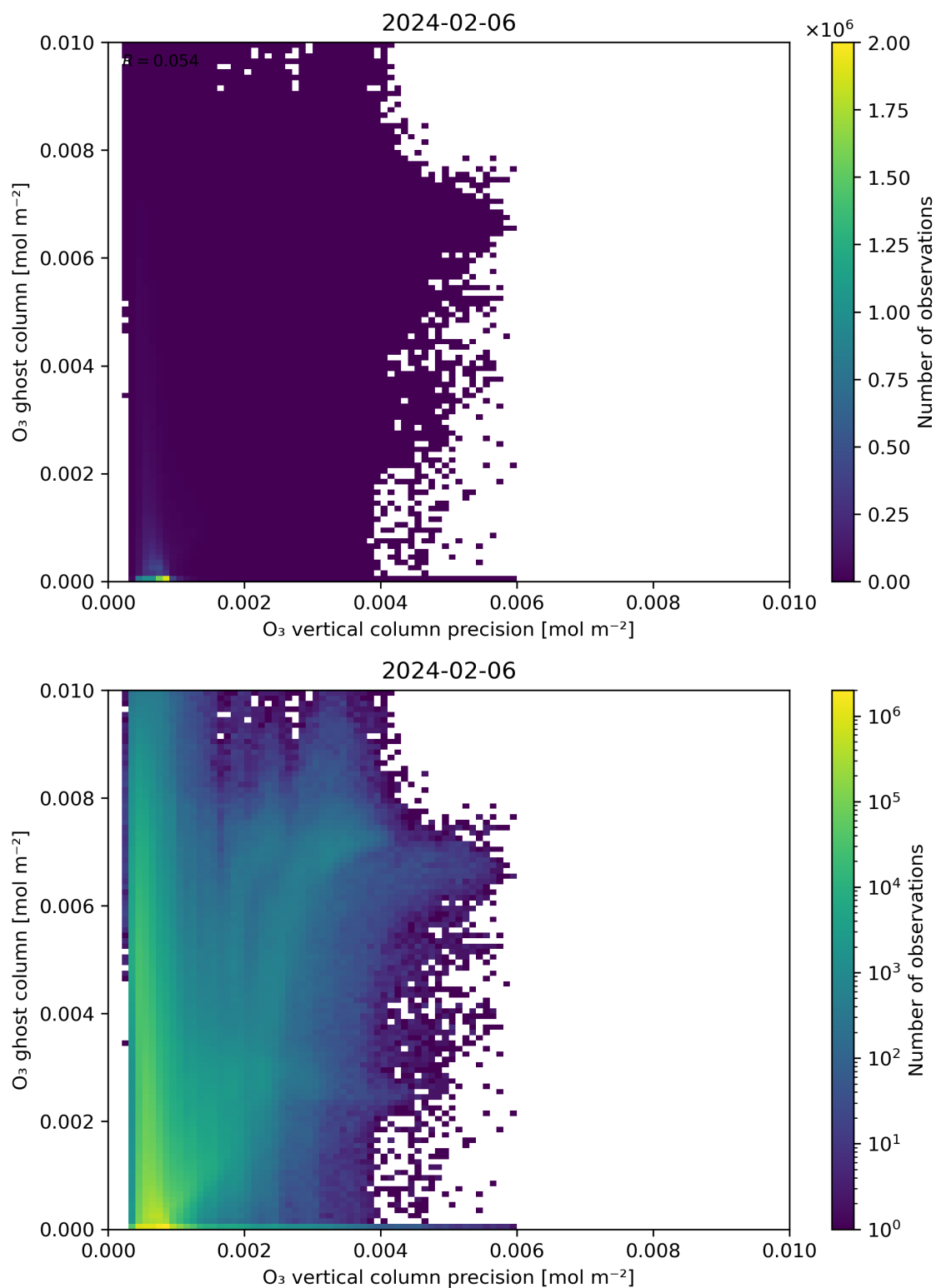
Figure 43: Scatter density plot of “O 3 vertical column precision” against “O 3 ghost column” for 2024-02-06 to 2024-02-07.
