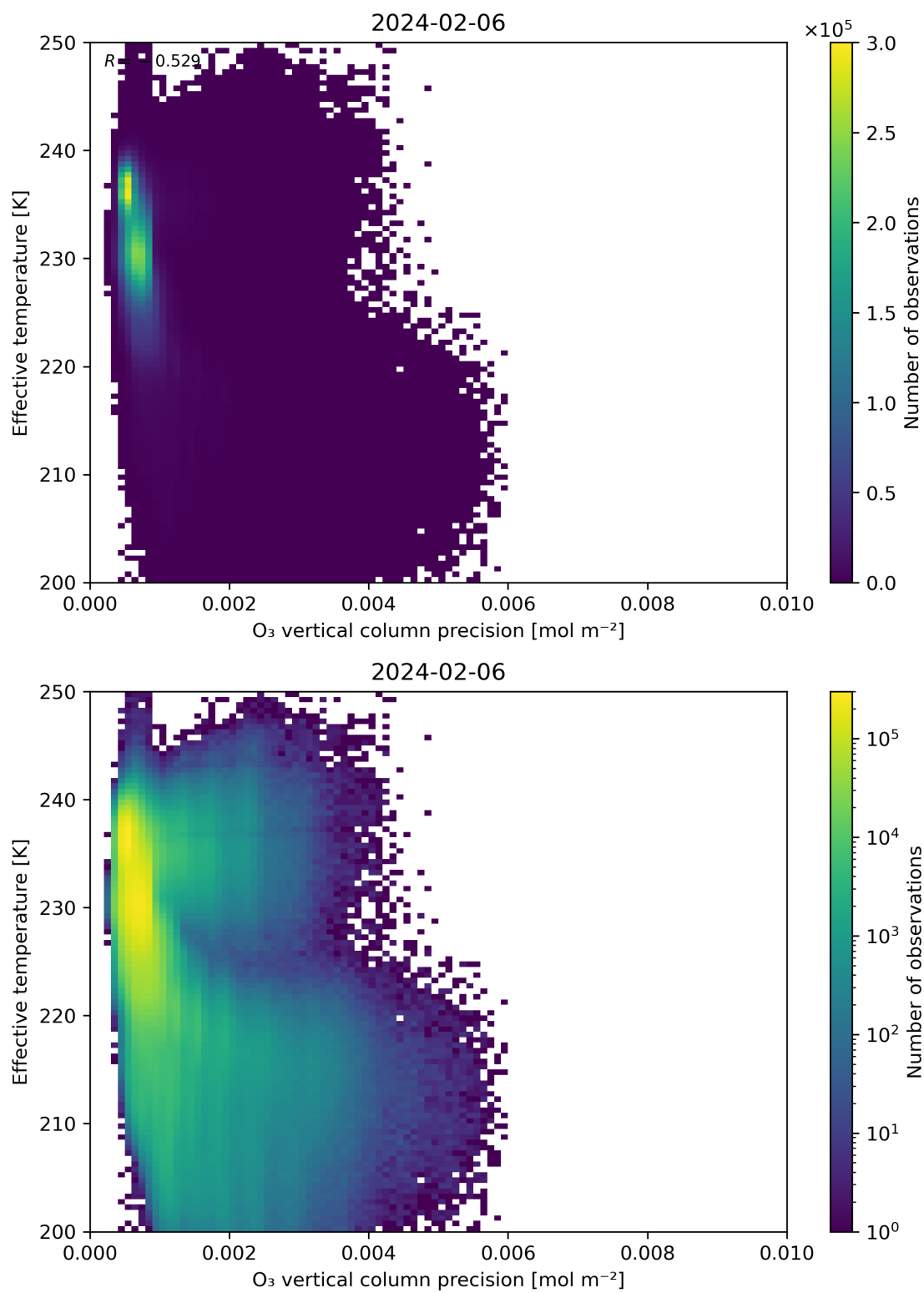
Figure 42: Scatter density plot of “O 3 vertical column precision” against “Effective temperature” for 2024-02-06 to 2024-02-07.
