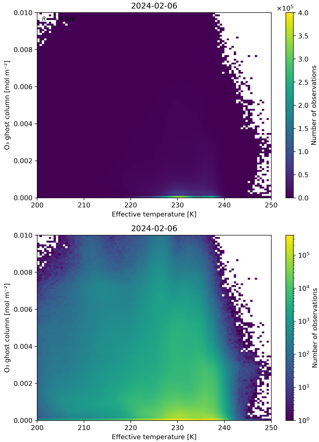
Figure 38: Scatter density plot of “Effective temperature” against “O 3 ghost column” for 2024-02-06 to 2024-02-07.
