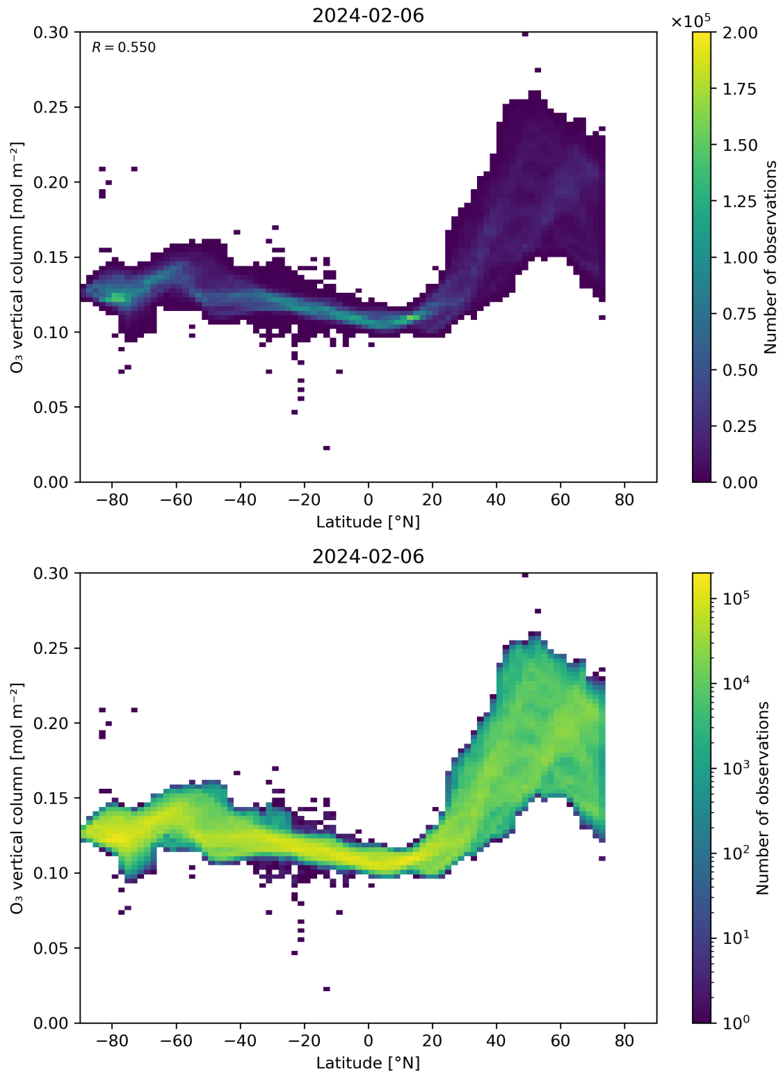
Figure 36: Scatter density plot of “Latitude” against “O 3 vertical column” for 2024-02-06 to 2024-02-07.
