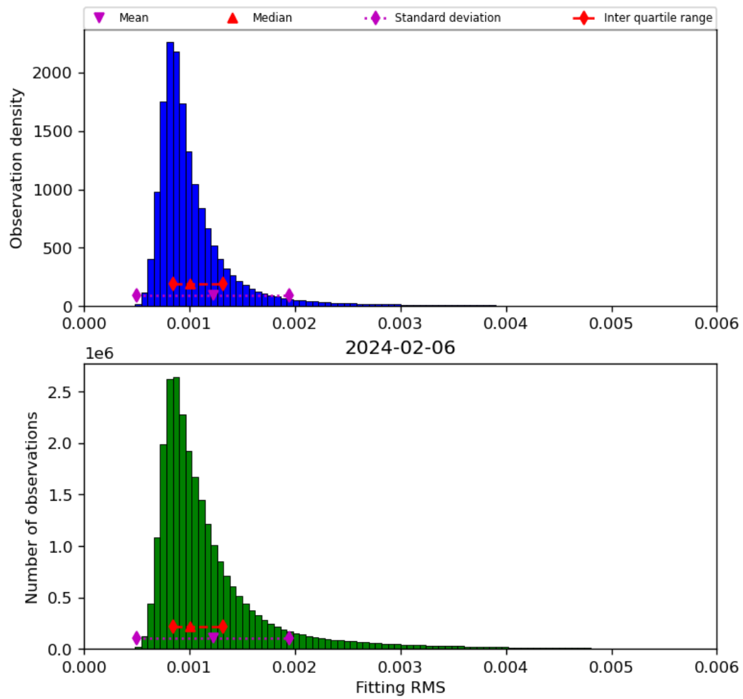
Figure 23: Histogram of “Fitting RMS” for 2024-02-06 to 2024-02-07
