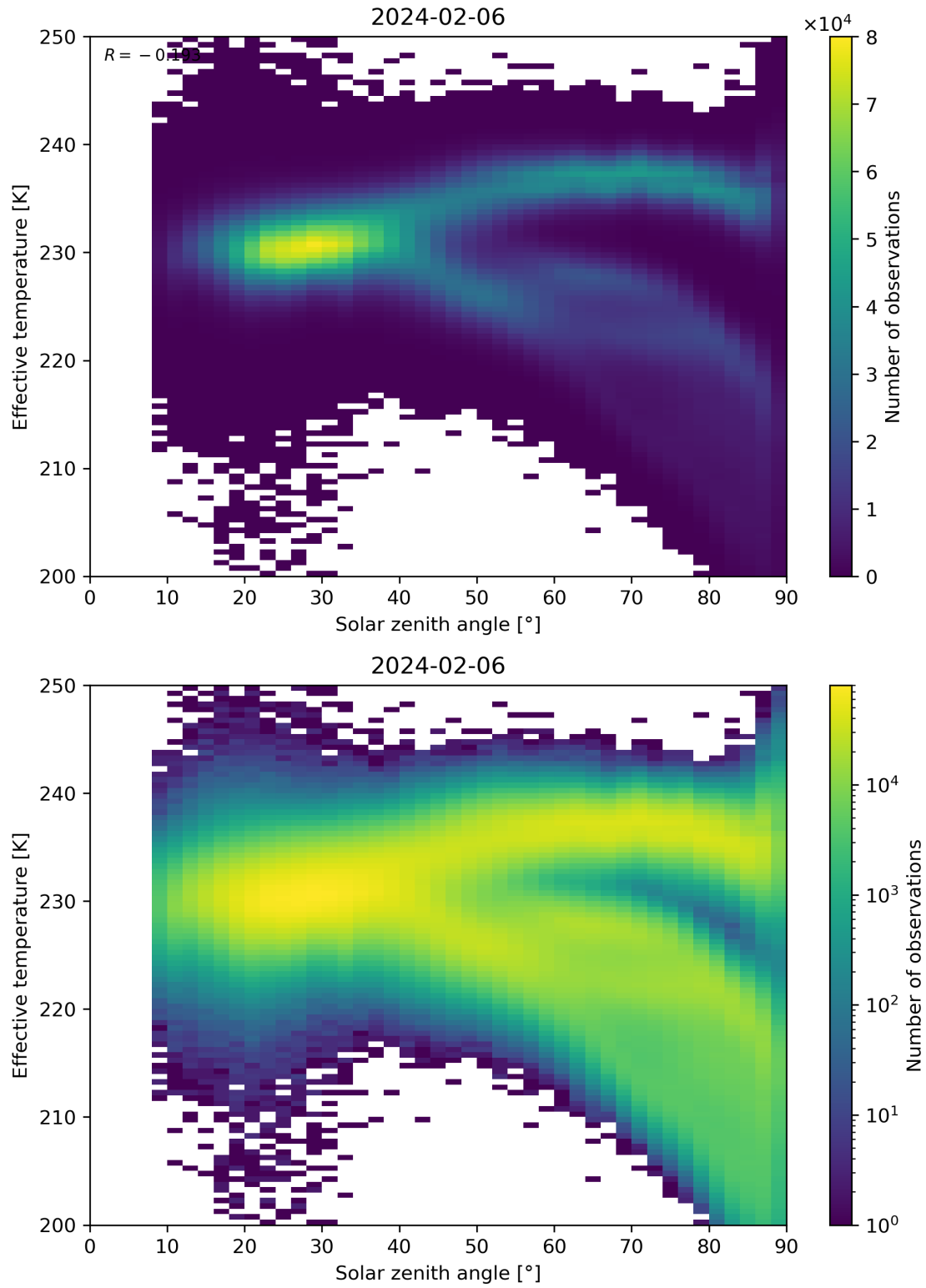
Figure 45: Scatter density plot of “Solar zenith angle” against “Effective temperature” for 2024-02-06 to 2024-02-07.
