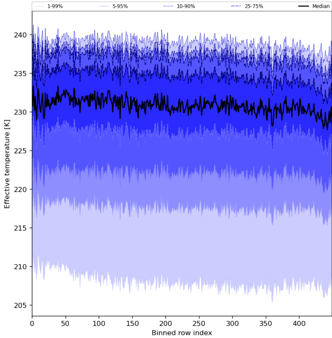
Figure 31: Along track statistics of “Effective temperature” for 2024-02-06 to 2024-02-07
