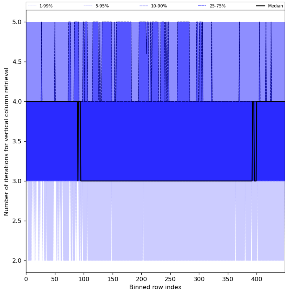
Figure 33: Along track statistics of “Number of iterations for vertical column retrieval” for 2024-02-06 to 2024-02-07
