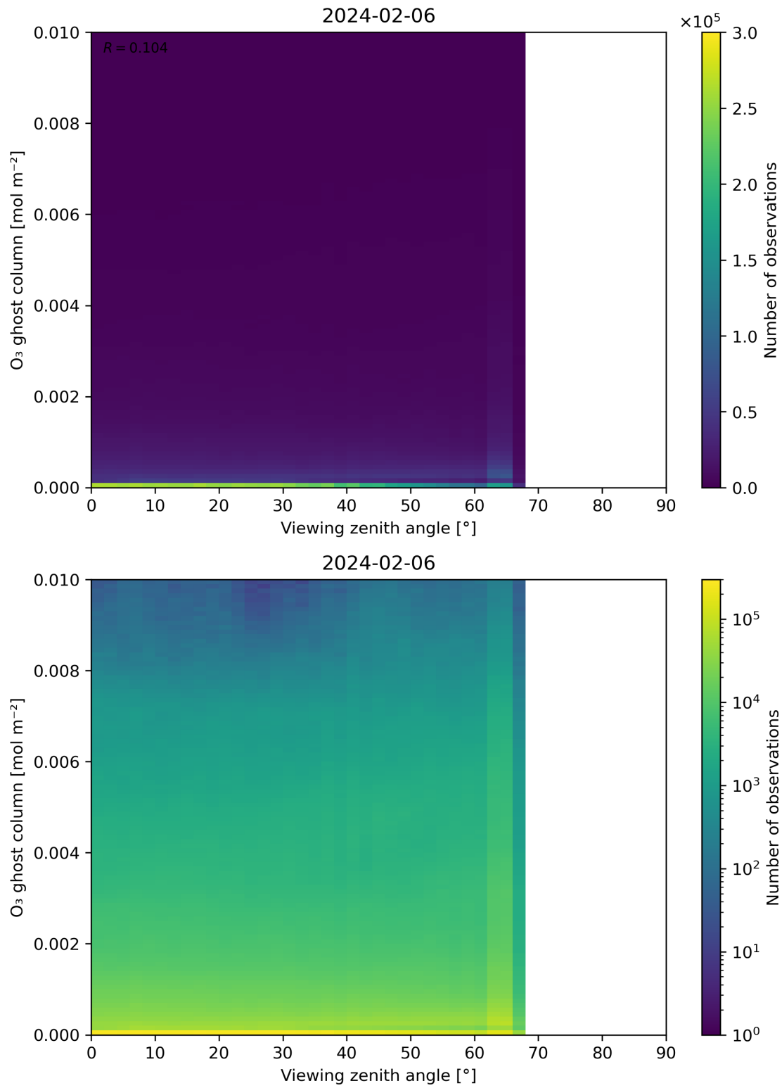
Figure 51: Scatter density plot of “Viewing zenith angle” against “O 3 ghost column” for 2024-02-06 to 2024-02-07.
