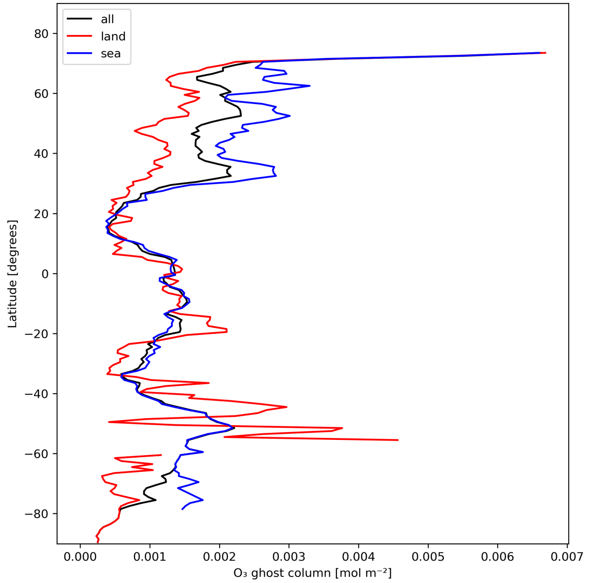
Figure 18: Zonal average of "O 3 ghost column" for 2024-02-06 to 2024-02-07.
