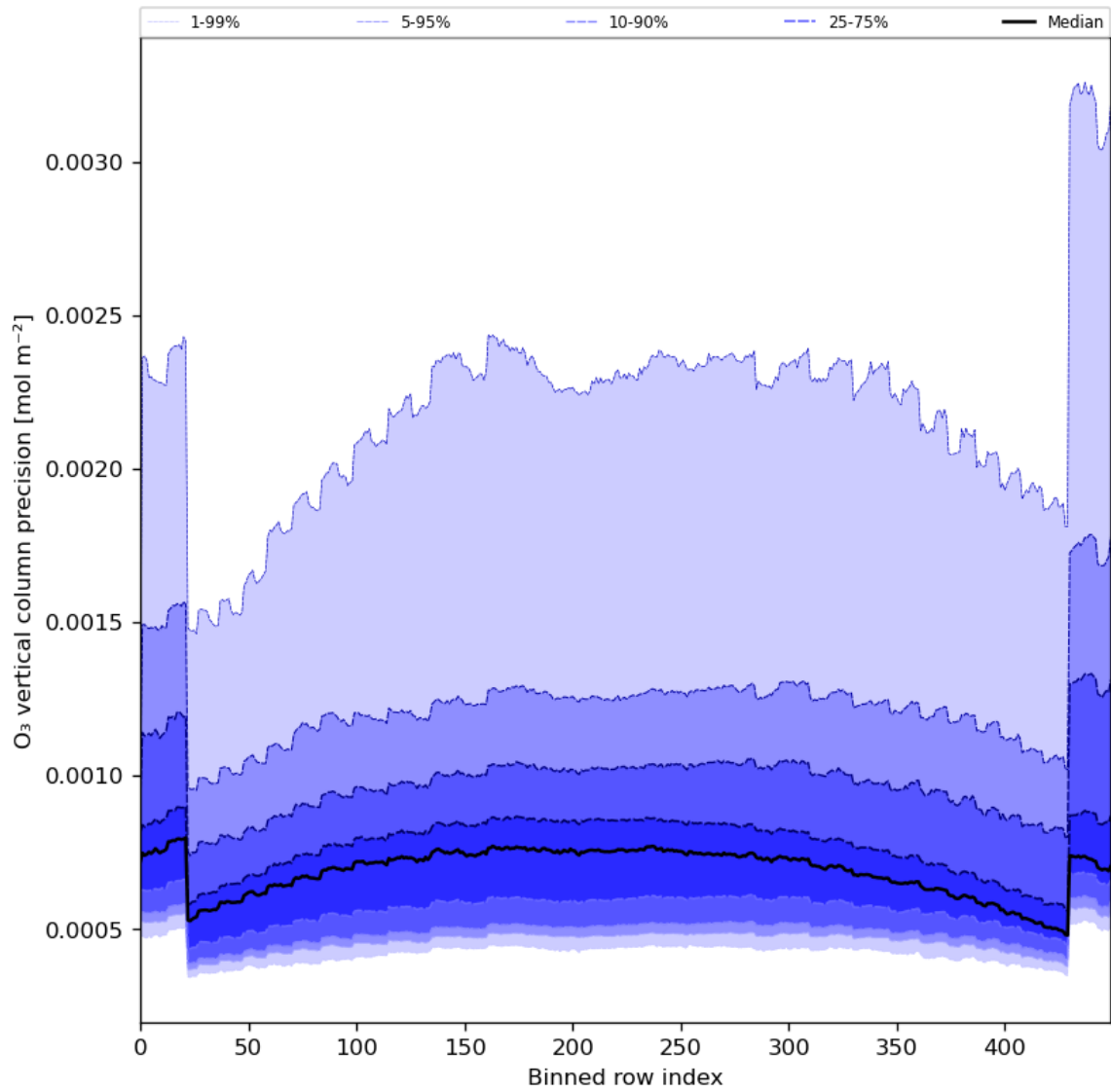
Figure 29: Along track statistics of “O 3 vertical column precision” for 2024-02-06 to 2024-02-07
