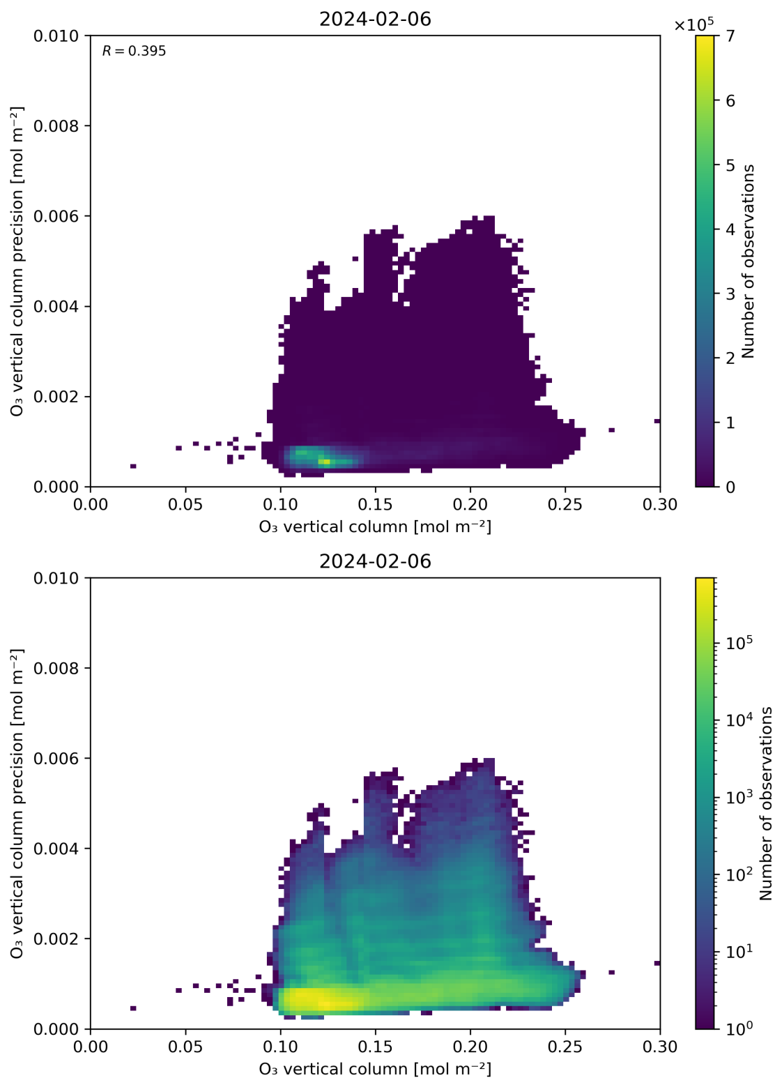
Figure 41: Scatter density plot of “O 3 vertical column” against “O 3 vertical column precision” for 2024-02-06 to 2024-02-07.
