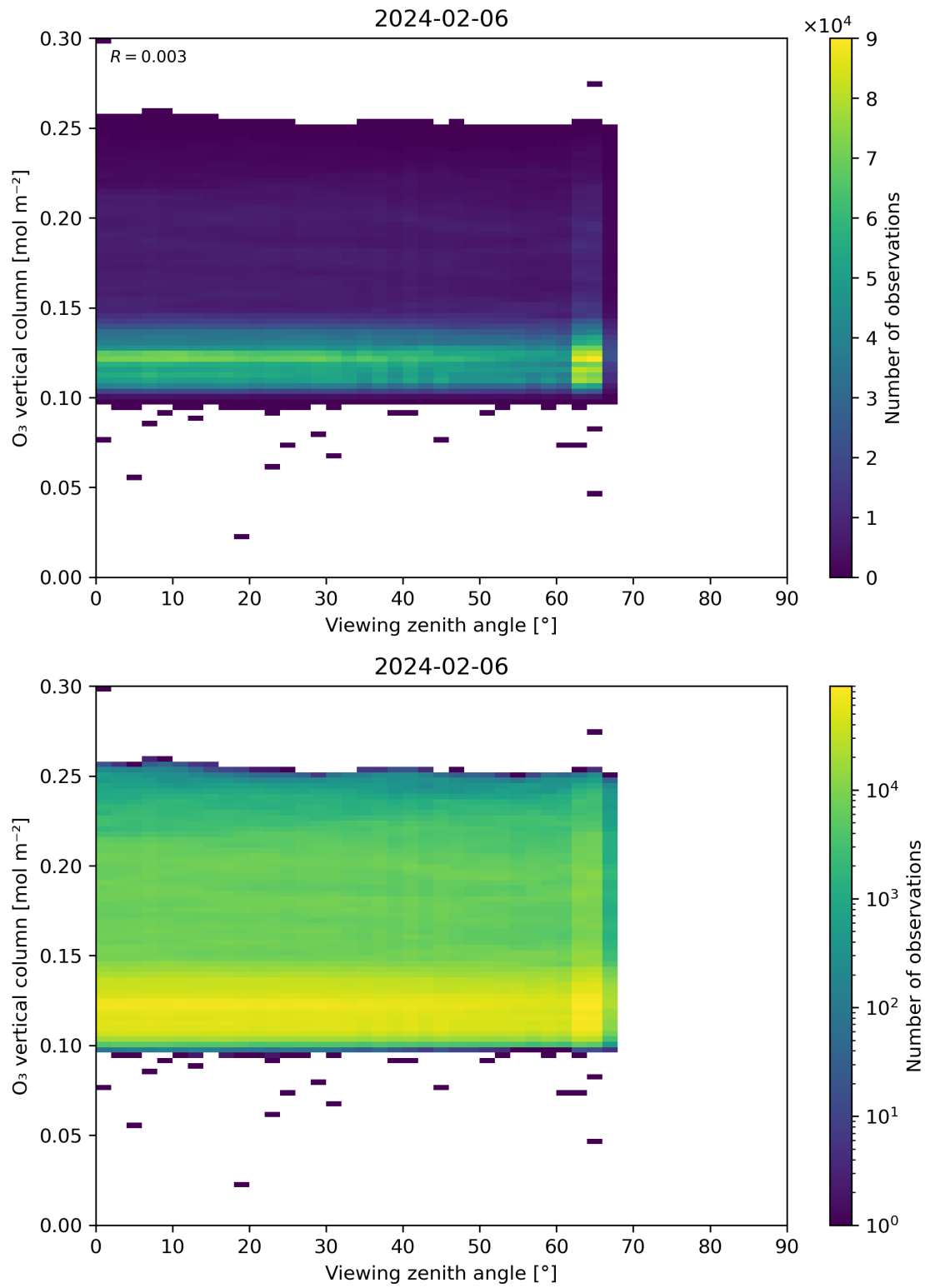
Figure 52: Scatter density plot of “Viewing zenith angle” against “O 3 vertical column” for 2024-02-06 to 2024-02-07.
