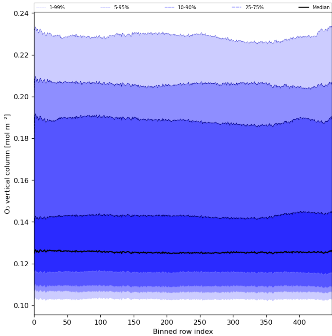
Figure 28: Along track statistics of “O 3 vertical column” for 2024-02-06 to 2024-02-07
