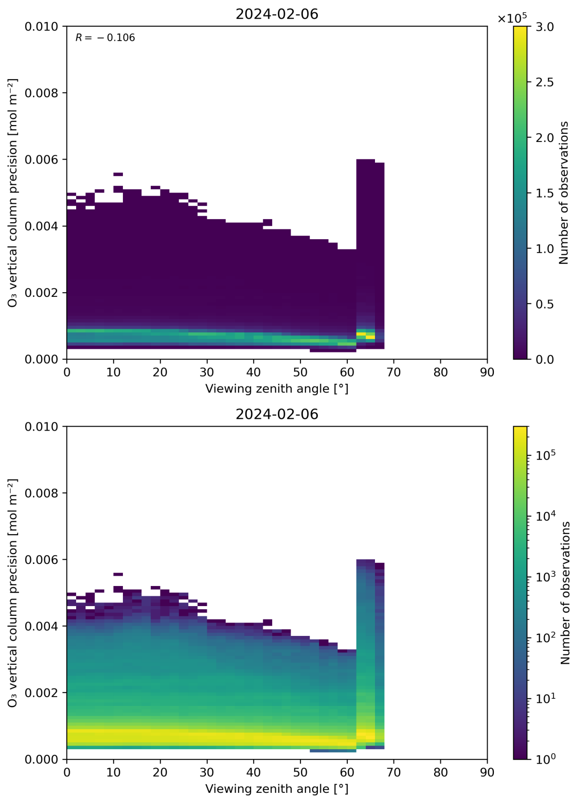
Figure 53: Scatter density plot of “Viewing zenith angle” against “O 3 vertical column precision” for 2024-02-06 to 2024-02-07.
