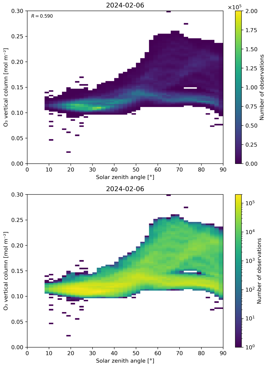
Figure 47: Scatter density plot of “Solar zenith angle” against “O 3 vertical column” for 2024-02-06 to 2024-02-07.
