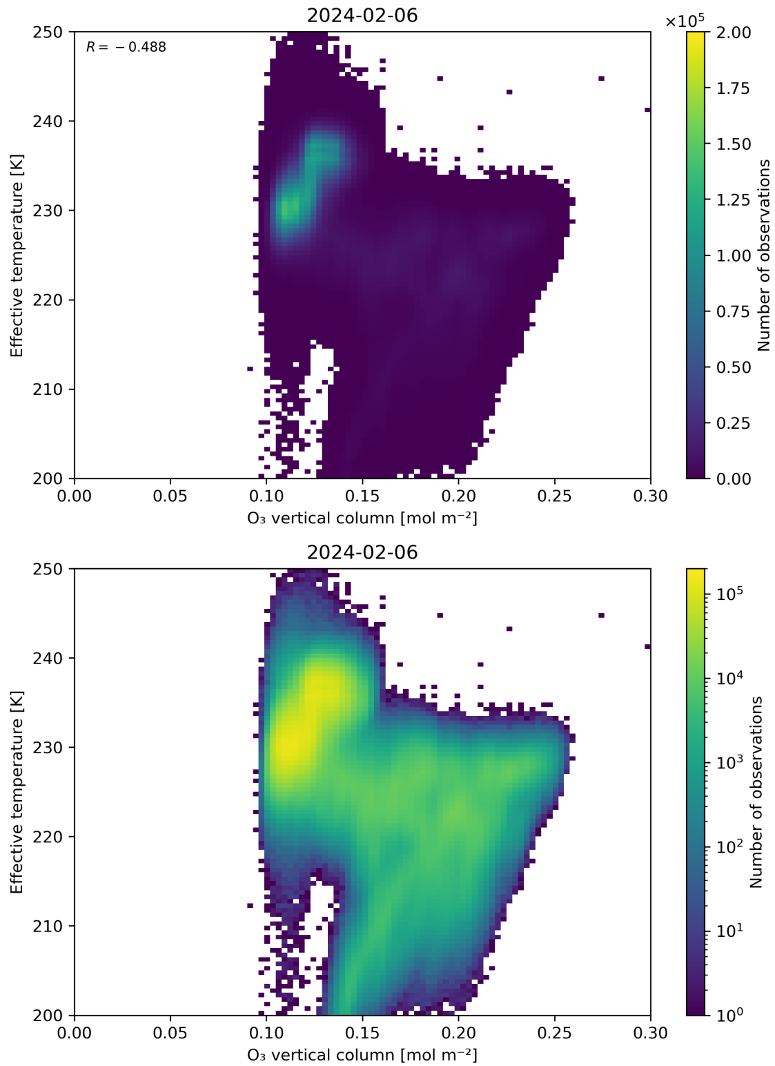
Figure 39: Scatter density plot of “O 3 vertical column” against “Effective temperature” for 2024-02-06 to 2024-02-07.
