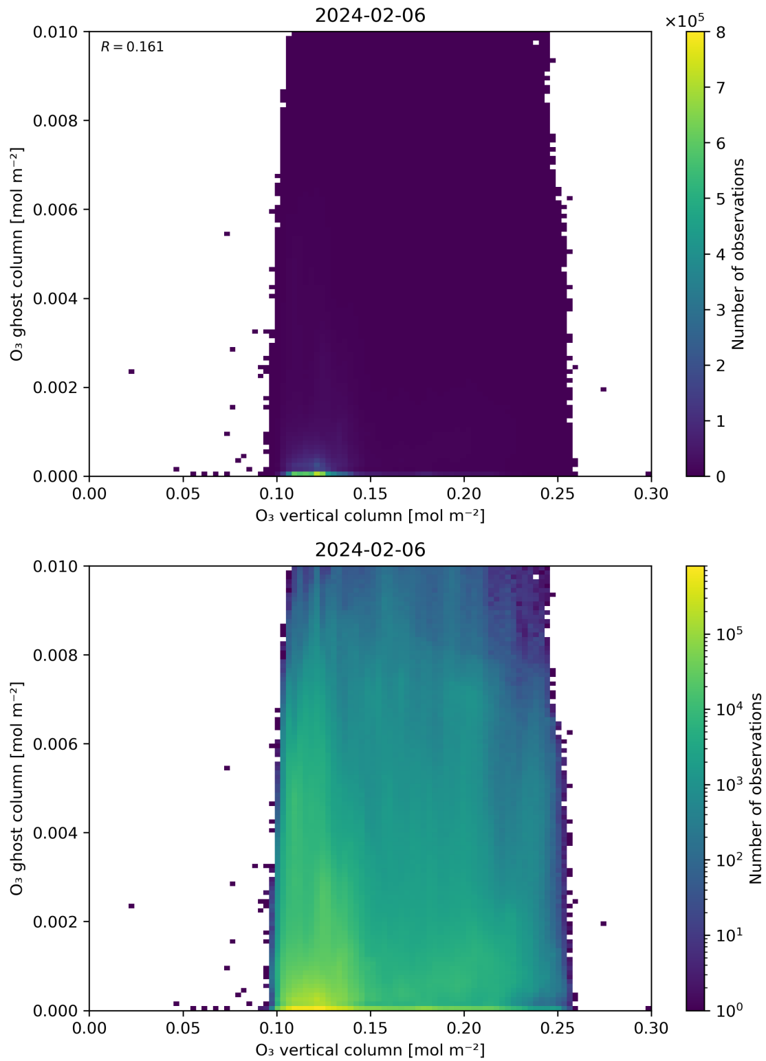
Figure 40: Scatter density plot of “O 3 vertical column” against “O 3 ghost column” for 2024-02-06 to 2024-02-07.
