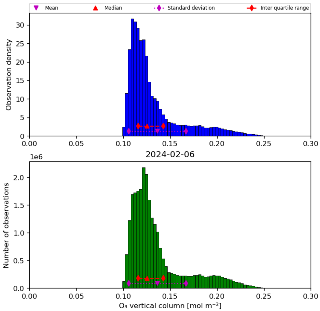
Figure 21: Histogram of “O 3 vertical column” for 2024-02-06 to 2024-02-07
