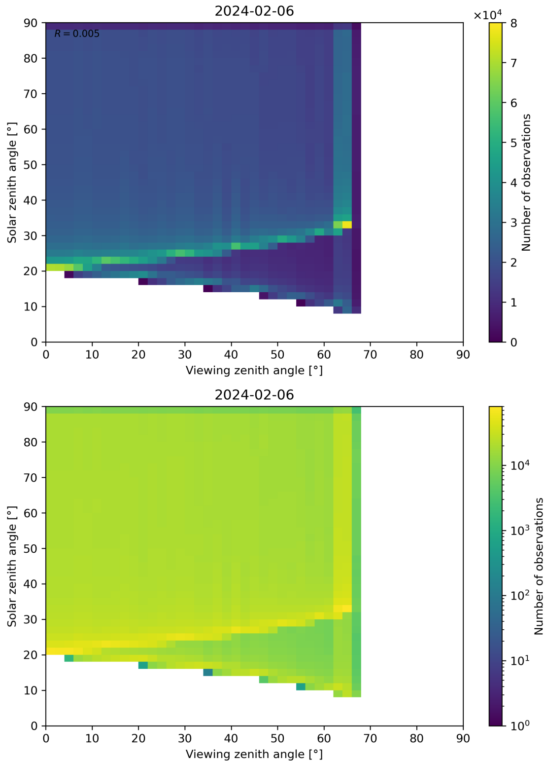
Figure 54: Scatter density plot of “Viewing zenith angle” against “Solar zenith angle” for 2024-02-06 to 2024-02-07.
