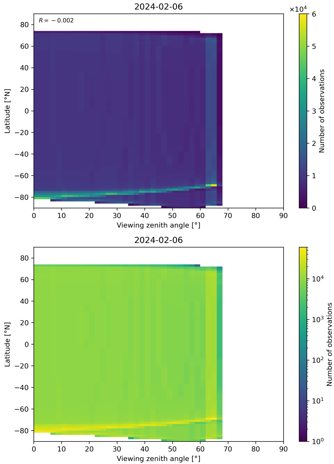
Figure 49: Scatter density plot of “Viewing zenith angle” against “Latitude” for 2024-02-06 to 2024-02-07.
