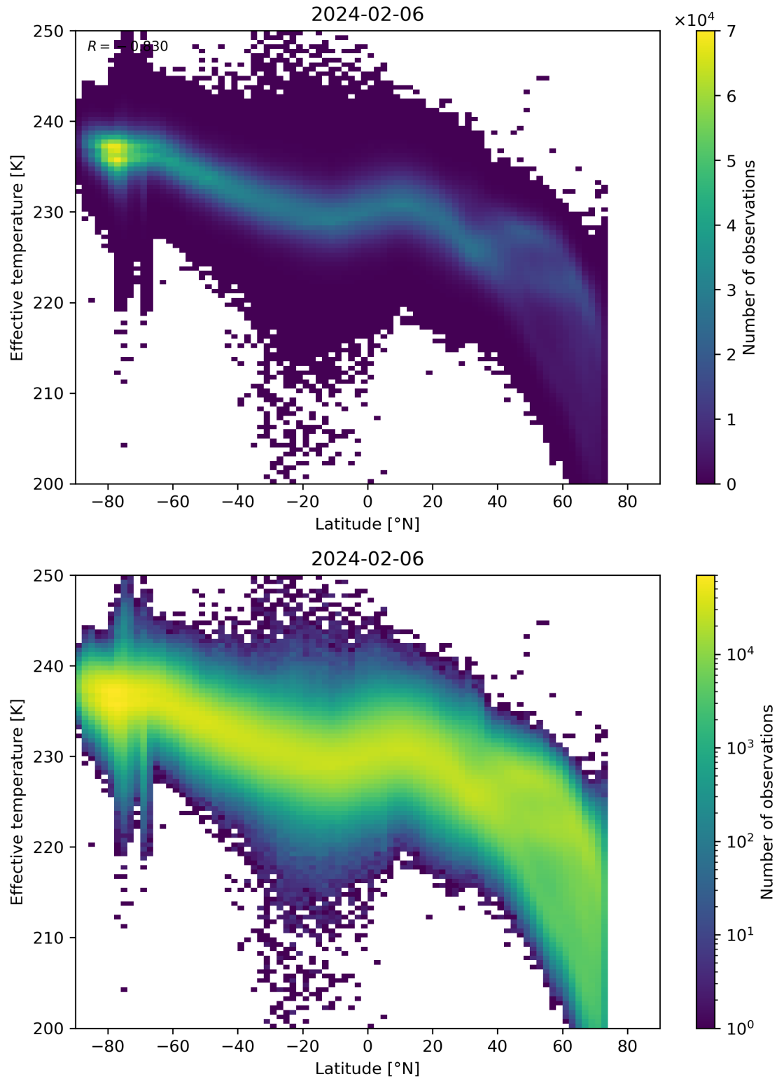
Figure 34: Scatter density plot of “Latitude” against “Effective temperature” for 2024-02-06 to 2024-02-07.
