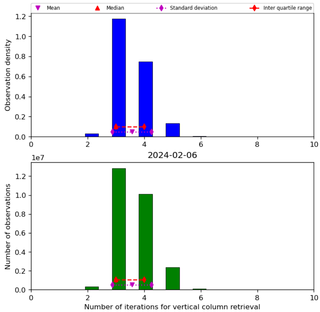
Figure 26: Histogram of “Number of iterations for vertical column retrieval” for 2024-02-06 to 2024-02-07
