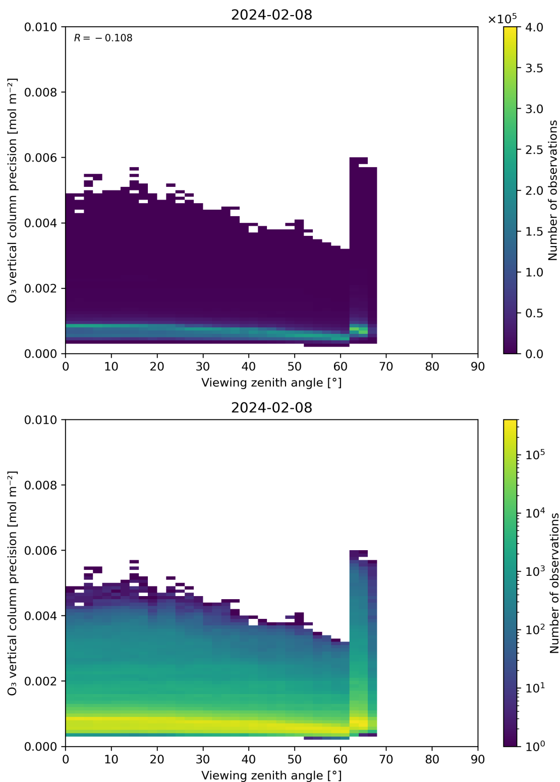
Figure 53: Scatter density plot of “Viewing zenith angle” against “O 3 vertical column precision” for 2024-02-07 to 2024-02-09.
