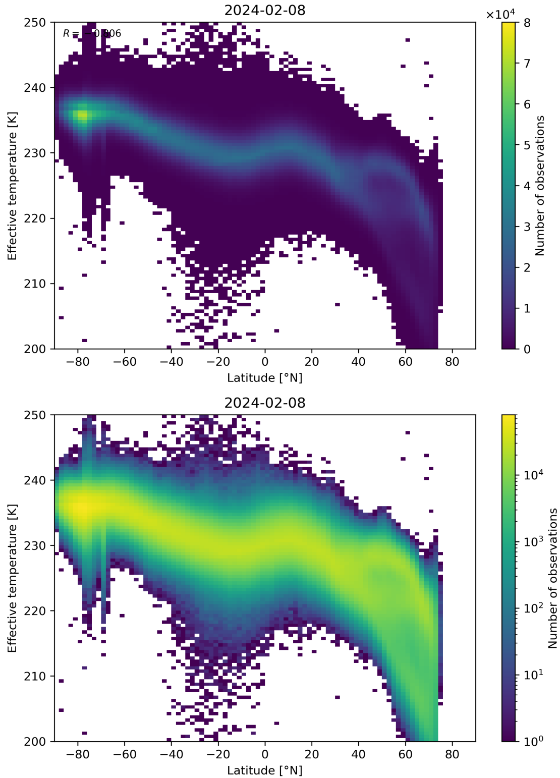
Figure 34: Scatter density plot of “Latitude” against “Effective temperature” for 2024-02-07 to 2024-02-09.
