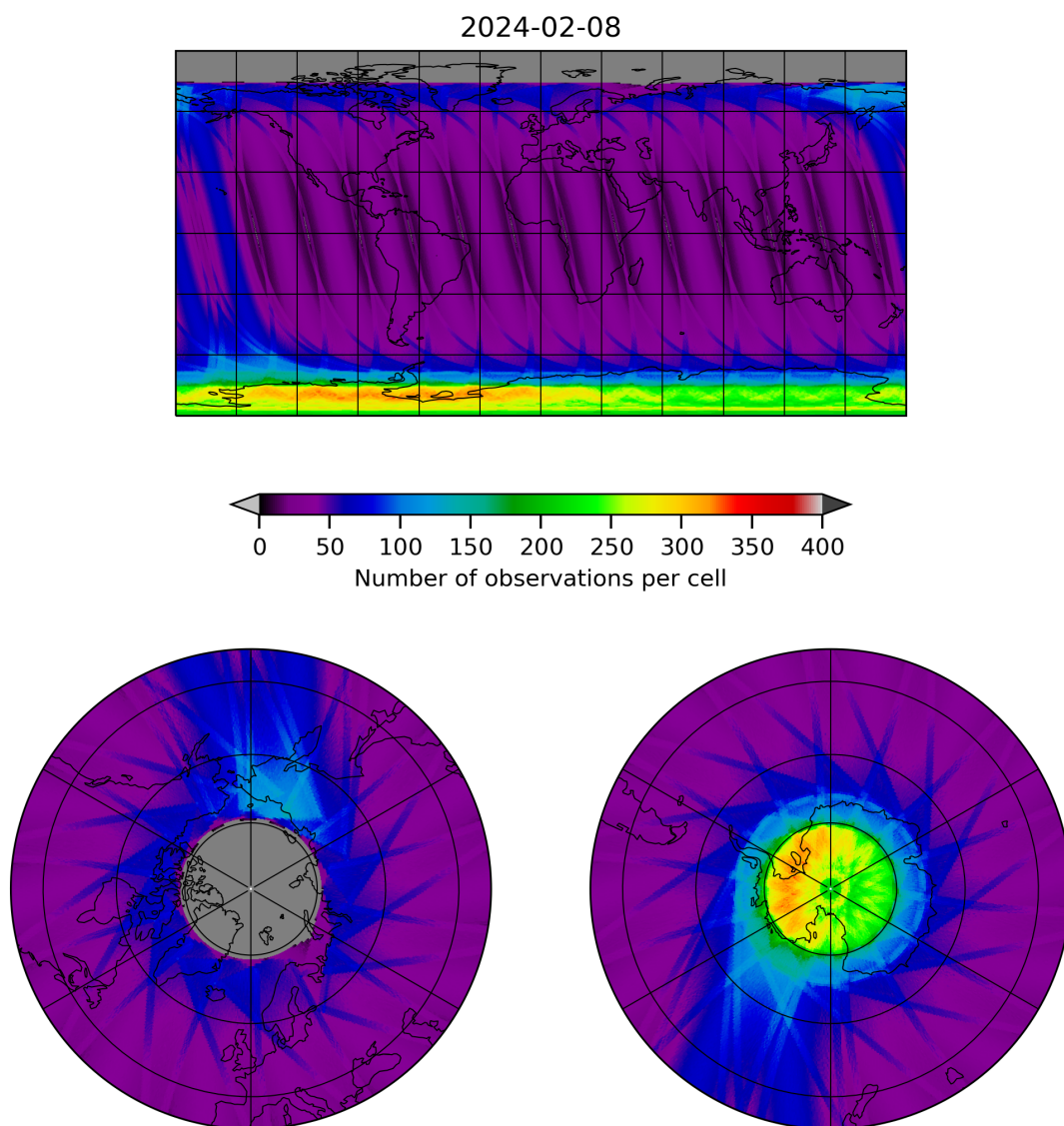
Figure 12: Map of the number of observations for 2024-02-07 to 2024-02-09
