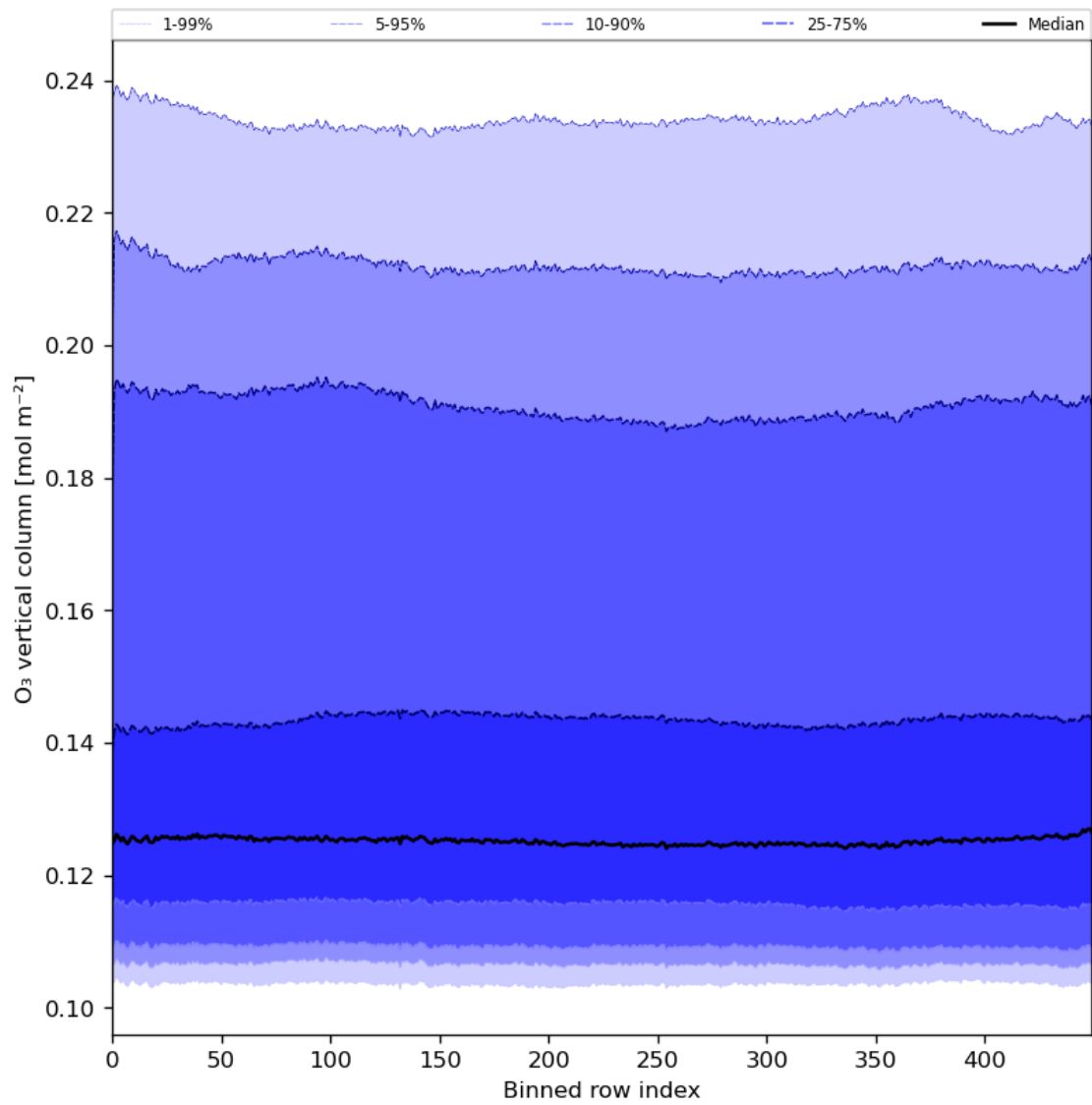
Figure 28: Along track statistics of “O 3 vertical column” for 2024-02-07 to 2024-02-09
