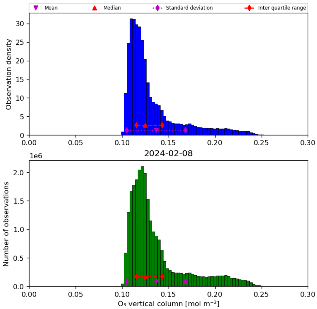
Figure 21: Histogram of “O 3 vertical column” for 2024-02-07 to 2024-02-09
