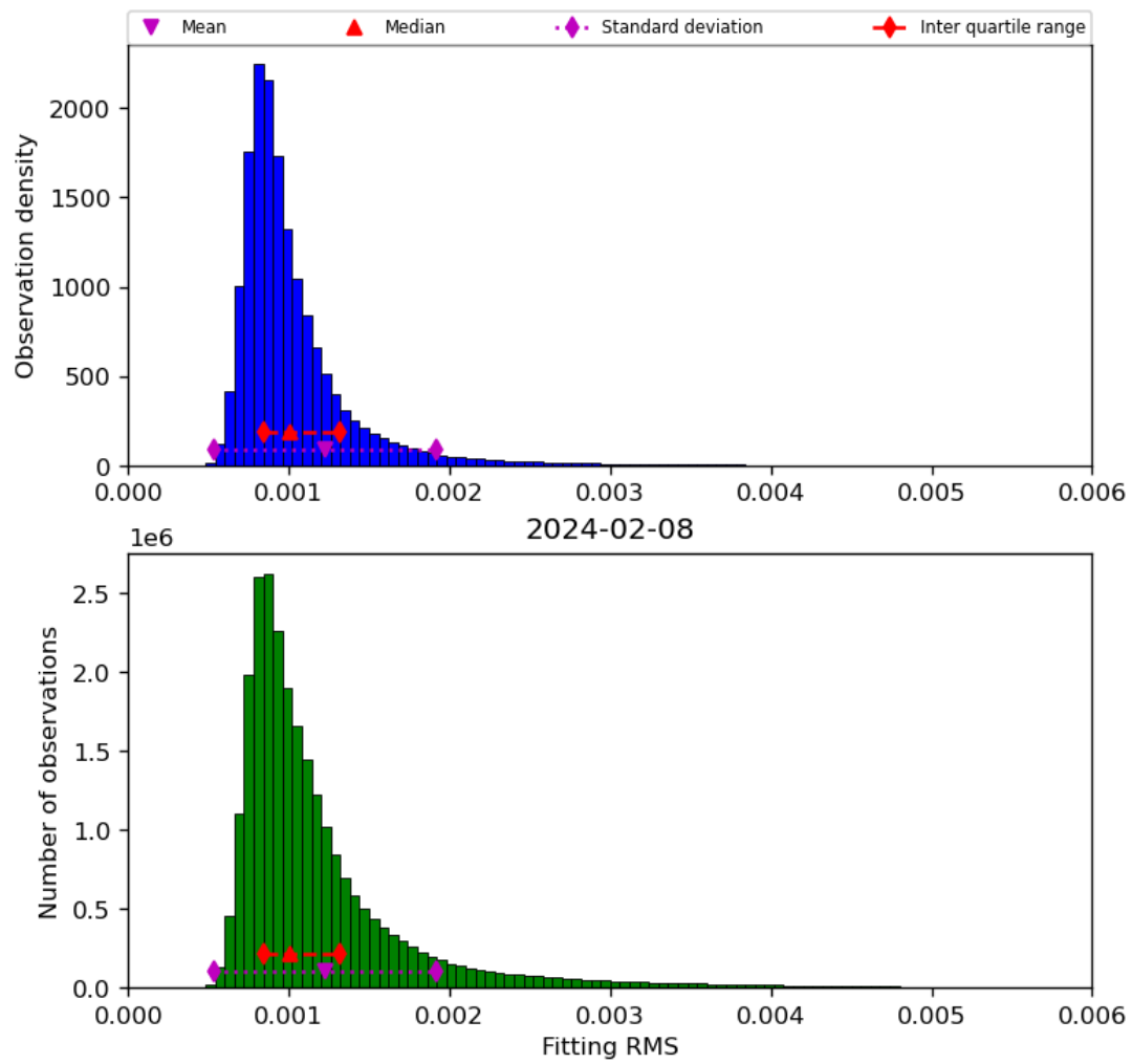
Figure 23: Histogram of “Fitting RMS” for 2024-02-07 to 2024-02-09
