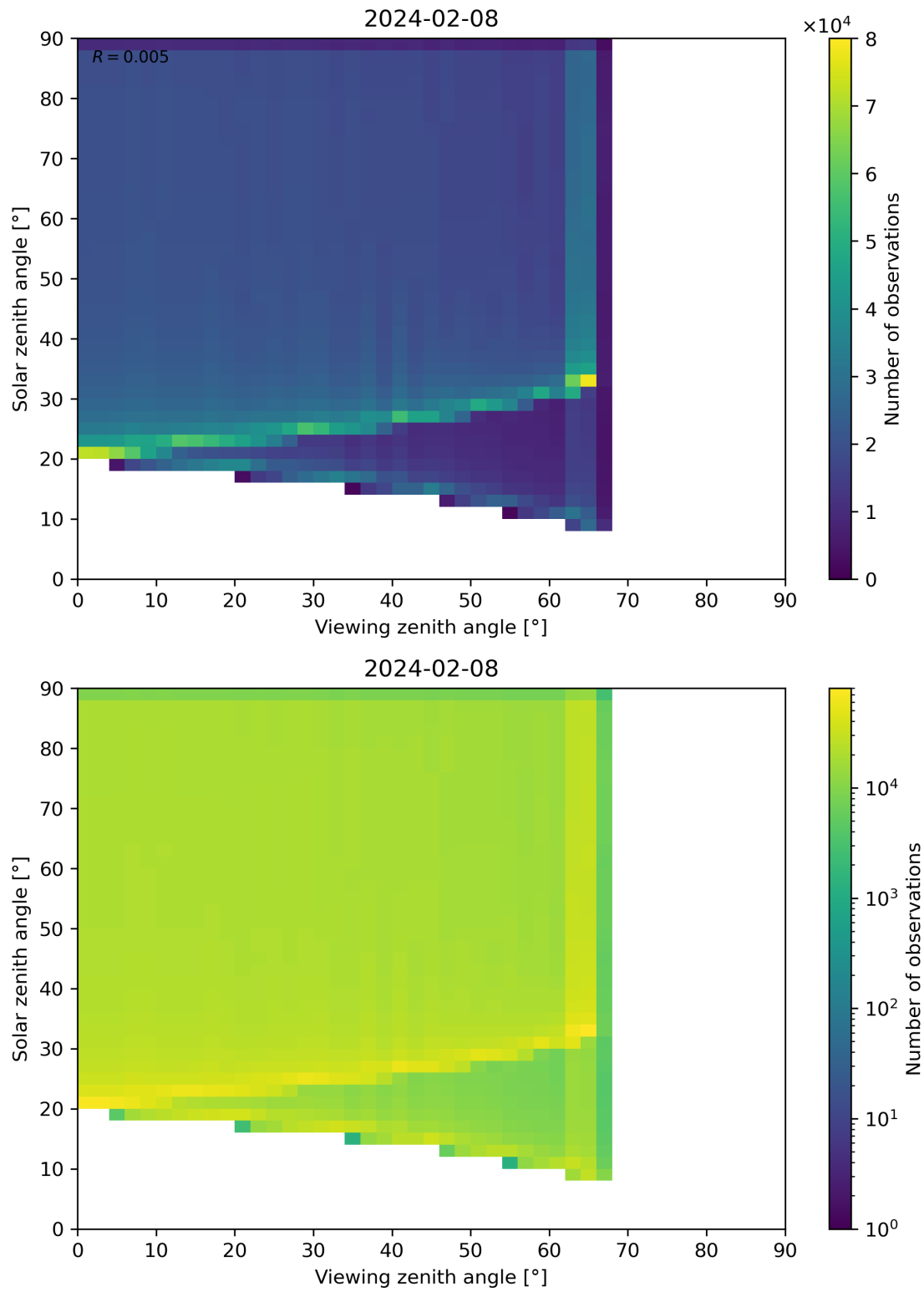
Figure 54: Scatter density plot of “Viewing zenith angle” against “Solar zenith angle” for 2024-02-07 to 2024-02-09.
