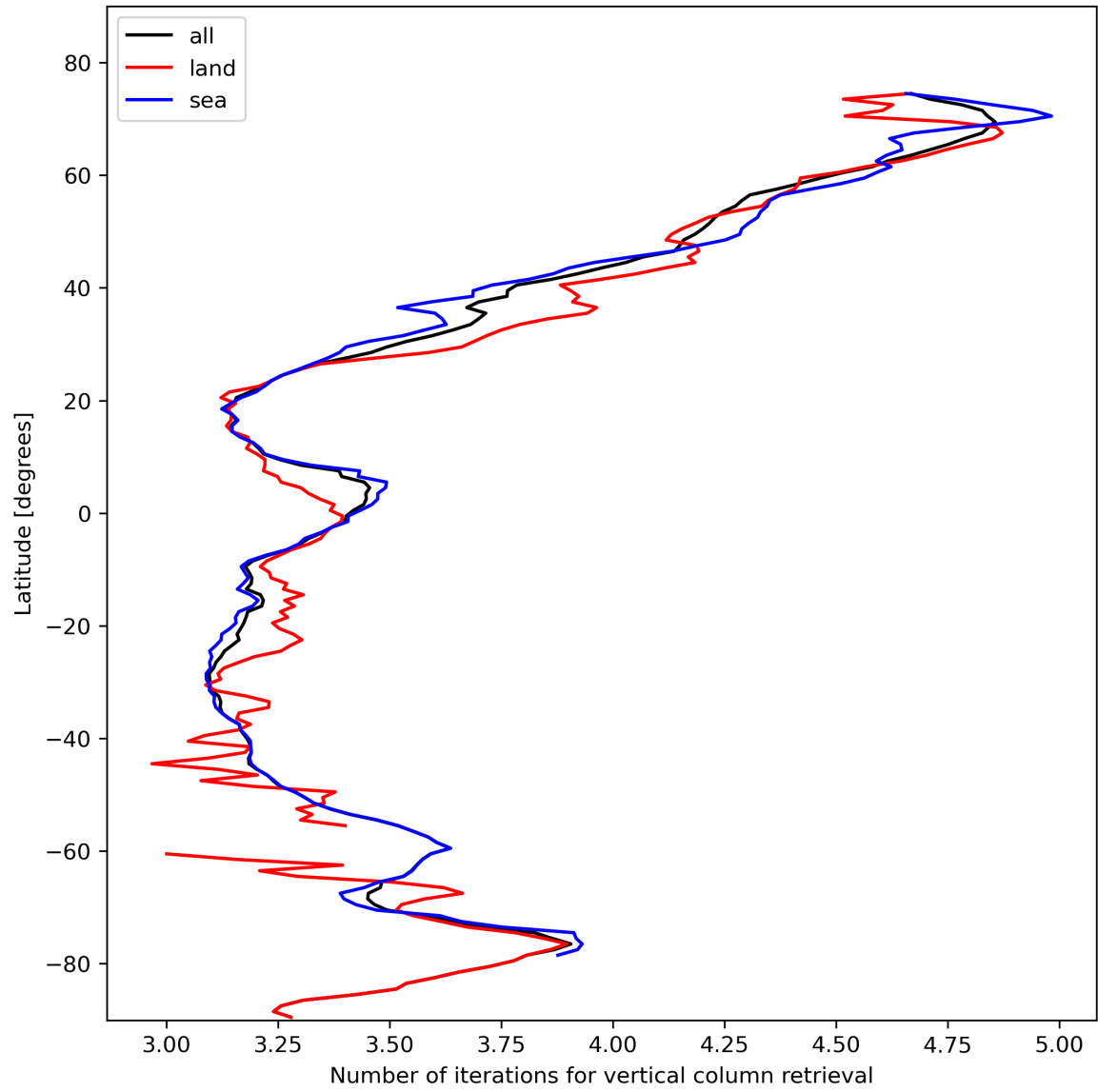
Figure 19: Zonal average of “Number of iterations for vertical column retrieval” for 2024-02-07 to 2024-02-09.
