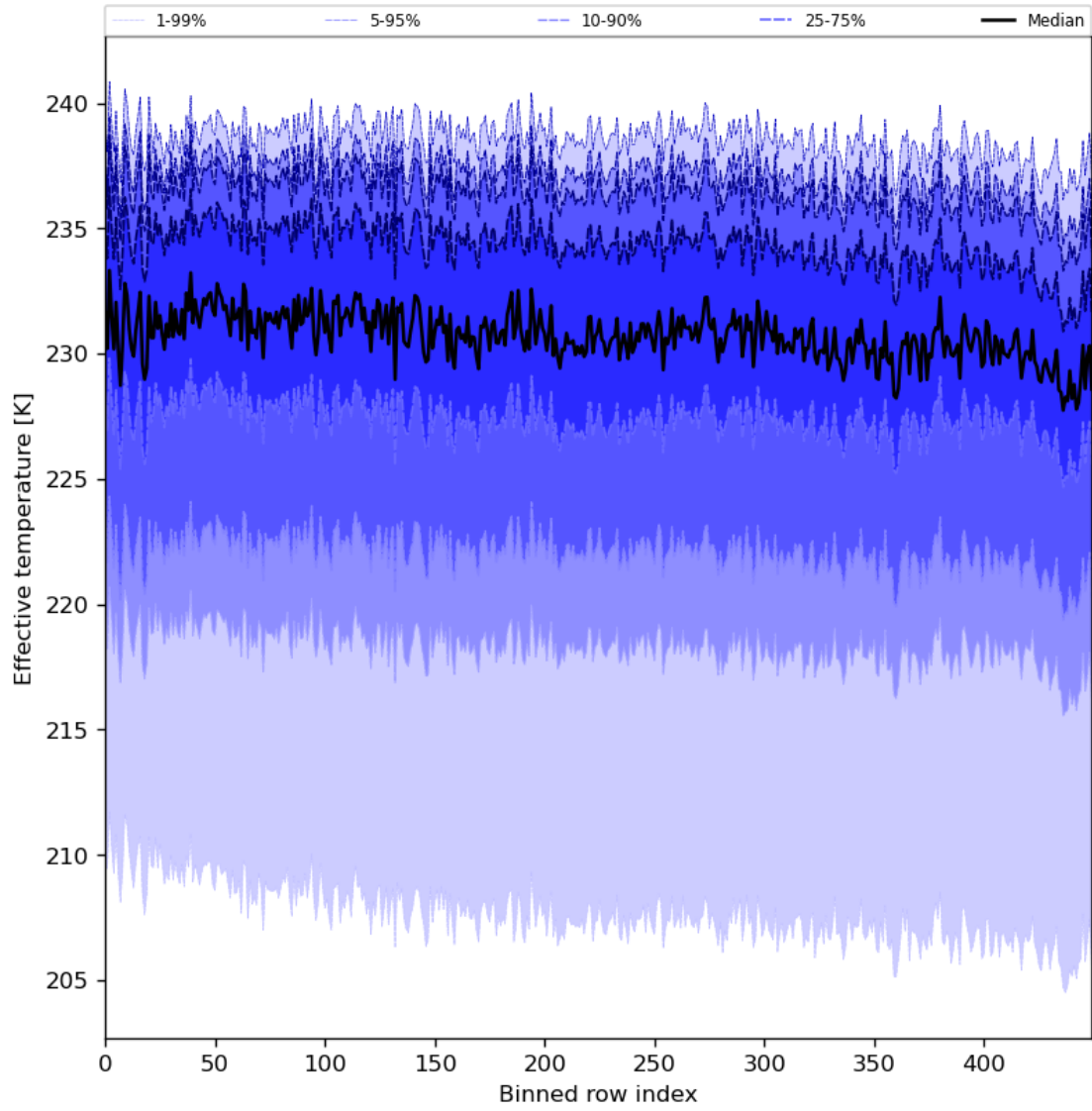
Figure 31: Along track statistics of “Effective temperature” for 2024-02-07 to 2024-02-09
