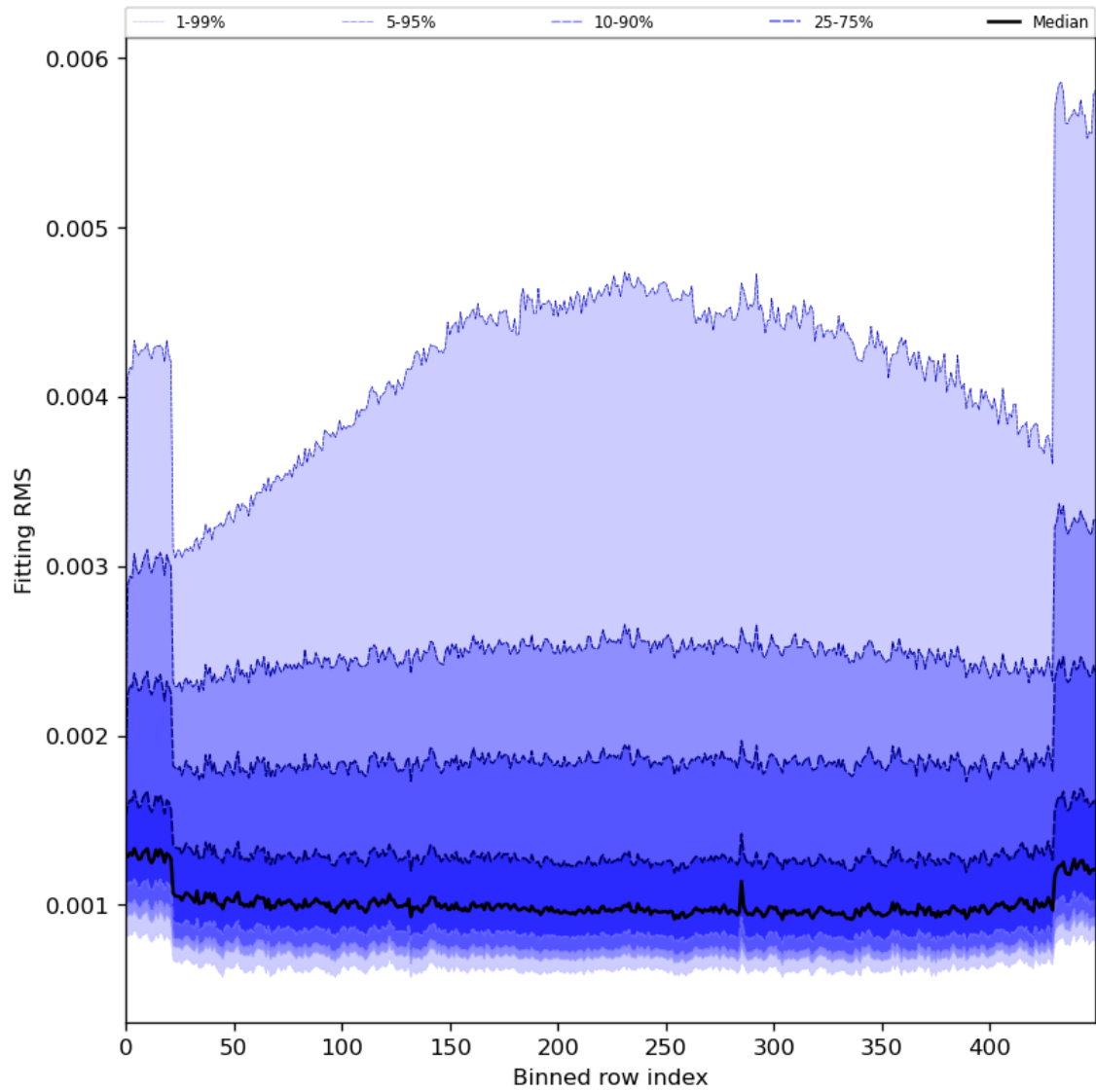
Figure 30: Along track statistics of “Fitting RMS” for 2024-02-07 to 2024-02-09
