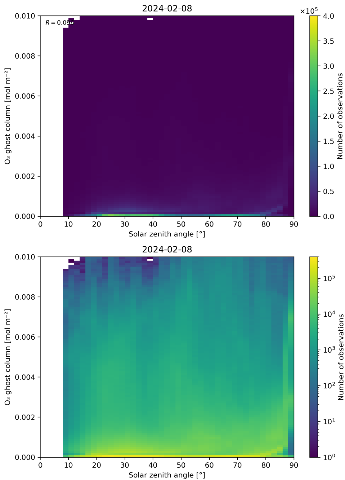
Figure 46: Scatter density plot of “Solar zenith angle” against “O 3 ghost column” for 2024-02-07 to 2024-02-09.
