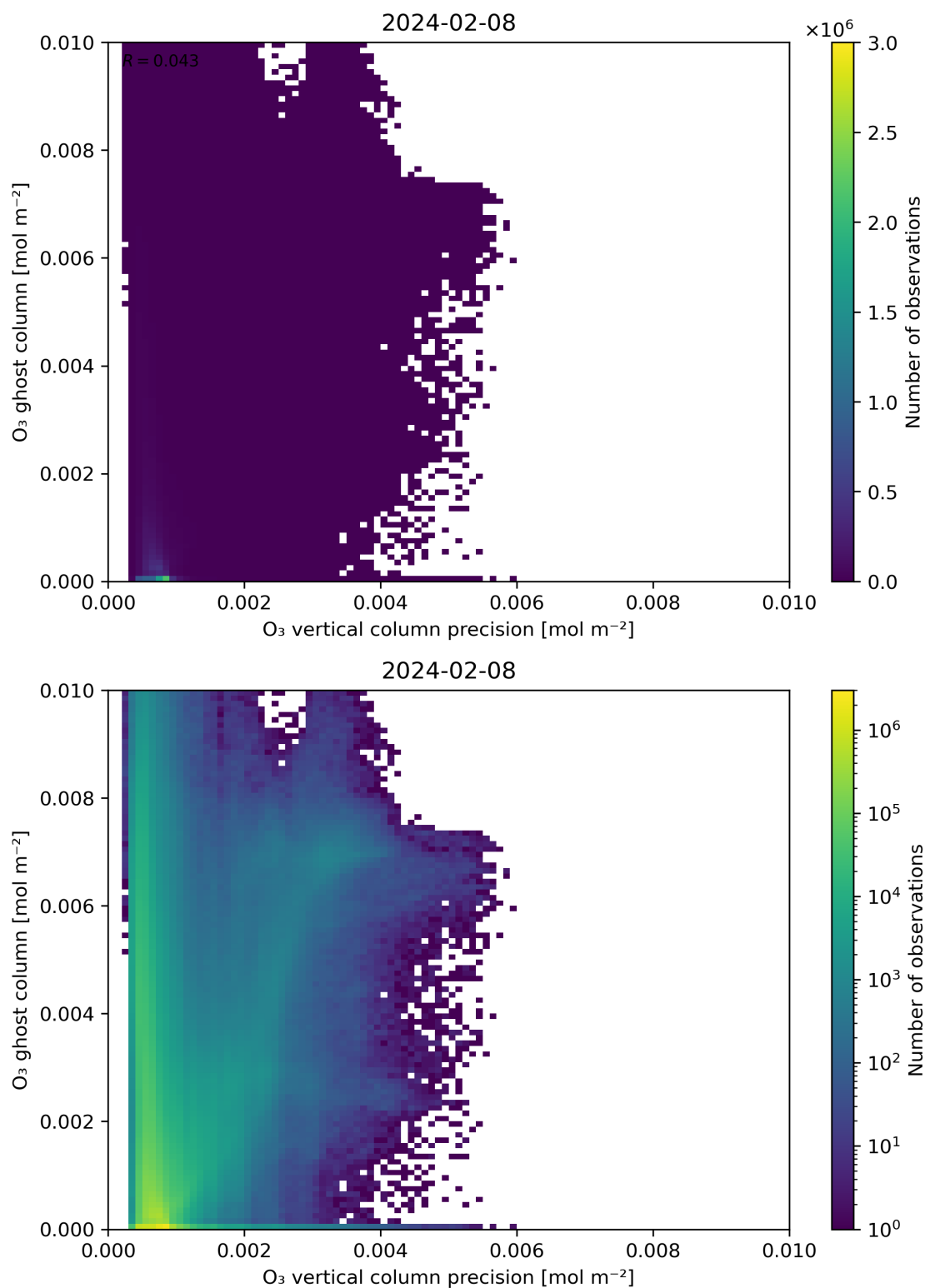
Figure 43: Scatter density plot of “ \text{O}_3 vertical column precision” against “ \text{O}_3 ghost column” for 2024-02-07 to 2024-02-09.
