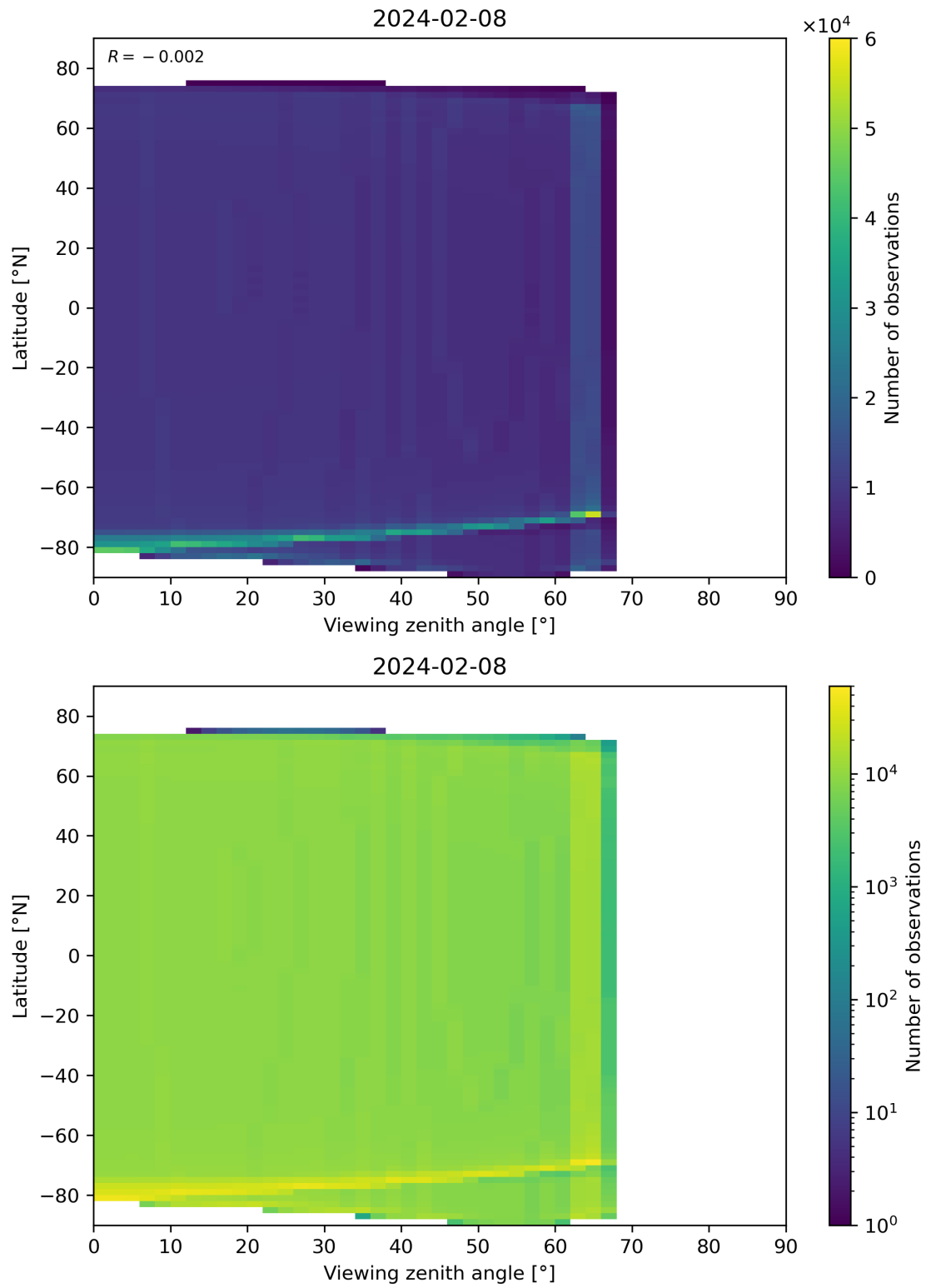
Figure 49: Scatter density plot of “Viewing zenith angle” against “Latitude” for 2024-02-07 to 2024-02-09.
