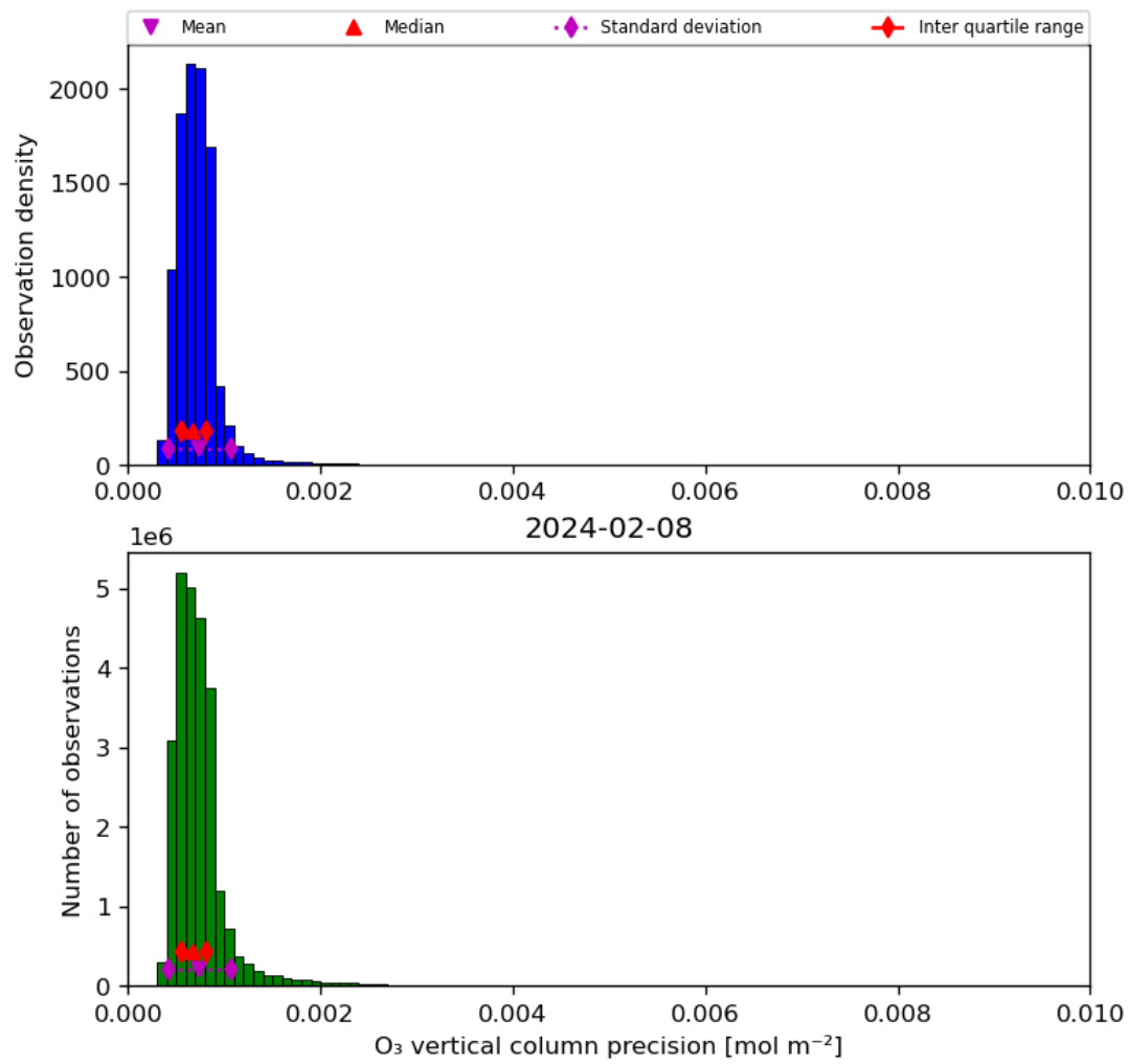
Figure 22: Histogram of “O 3 vertical column precision” for 2024-02-07 to 2024-02-09
