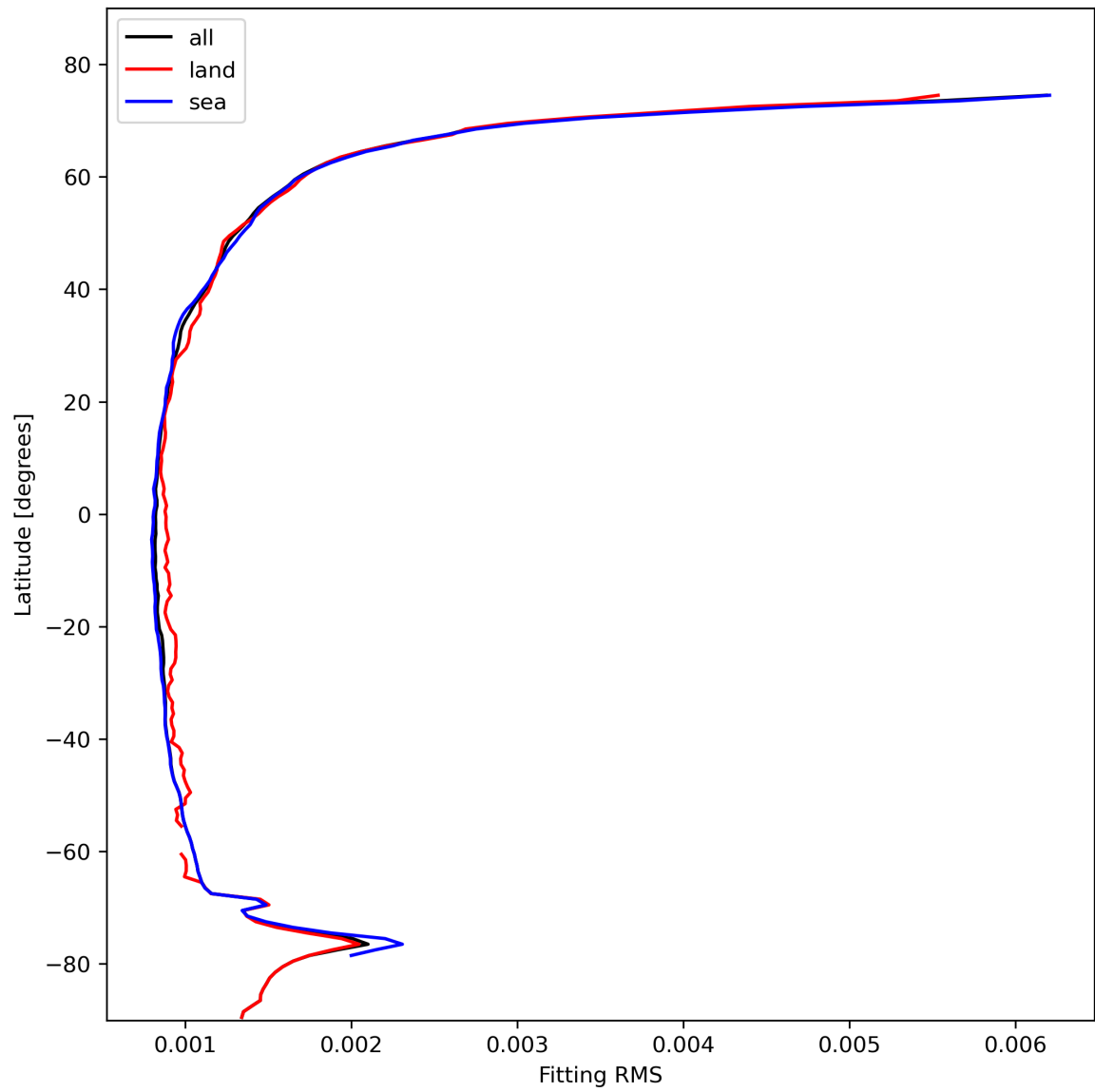
Figure 16: Zonal average of “Fitting RMS” for 2024-02-07 to 2024-02-09.
