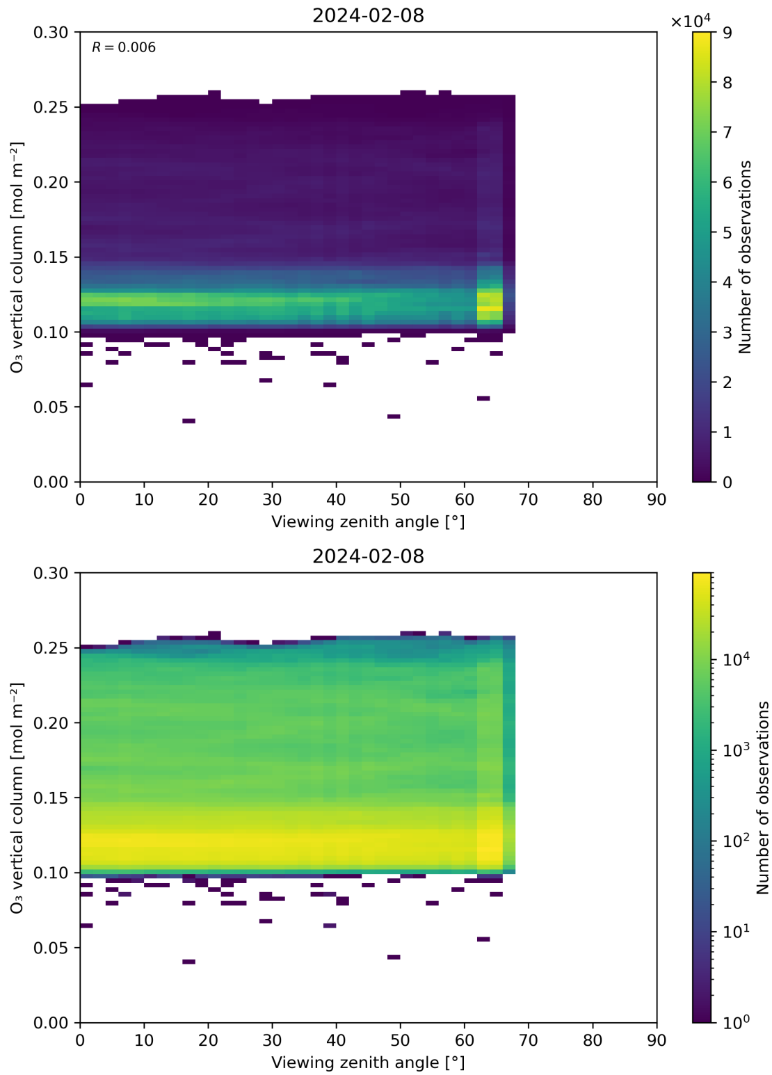
Figure 52: Scatter density plot of “Viewing zenith angle” against “O 3 vertical column” for 2024-02-07 to 2024-02-09.
