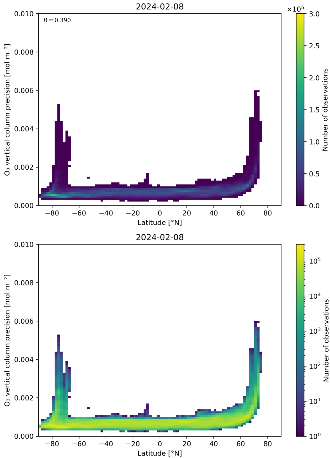
Figure 37: Scatter density plot of “Latitude” against “O 3 vertical column precision” for 2024-02-07 to 2024-02-09.
