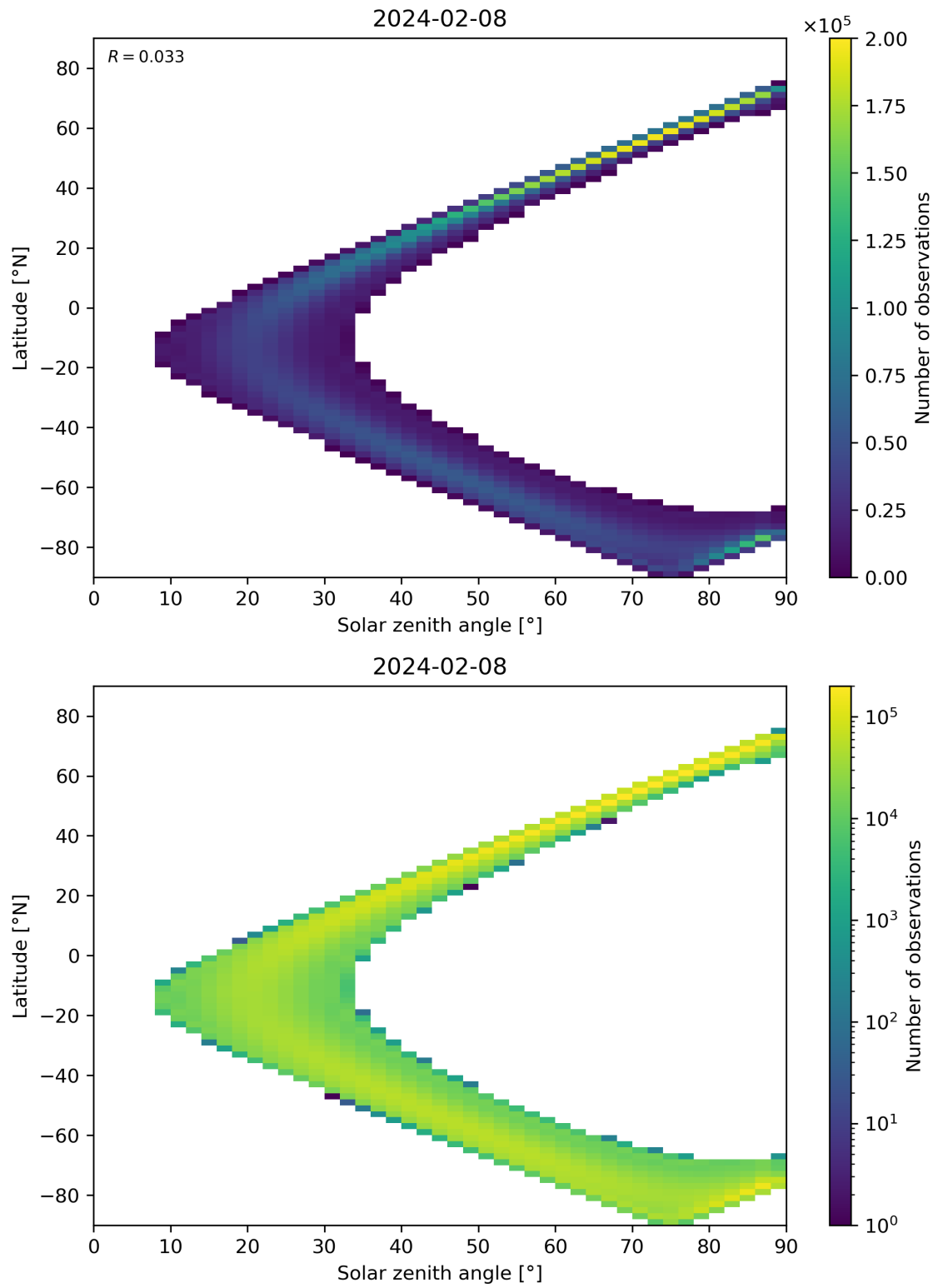
Figure 44: Scatter density plot of “Solar zenith angle” against “Latitude” for 2024-02-07 to 2024-02-09.
