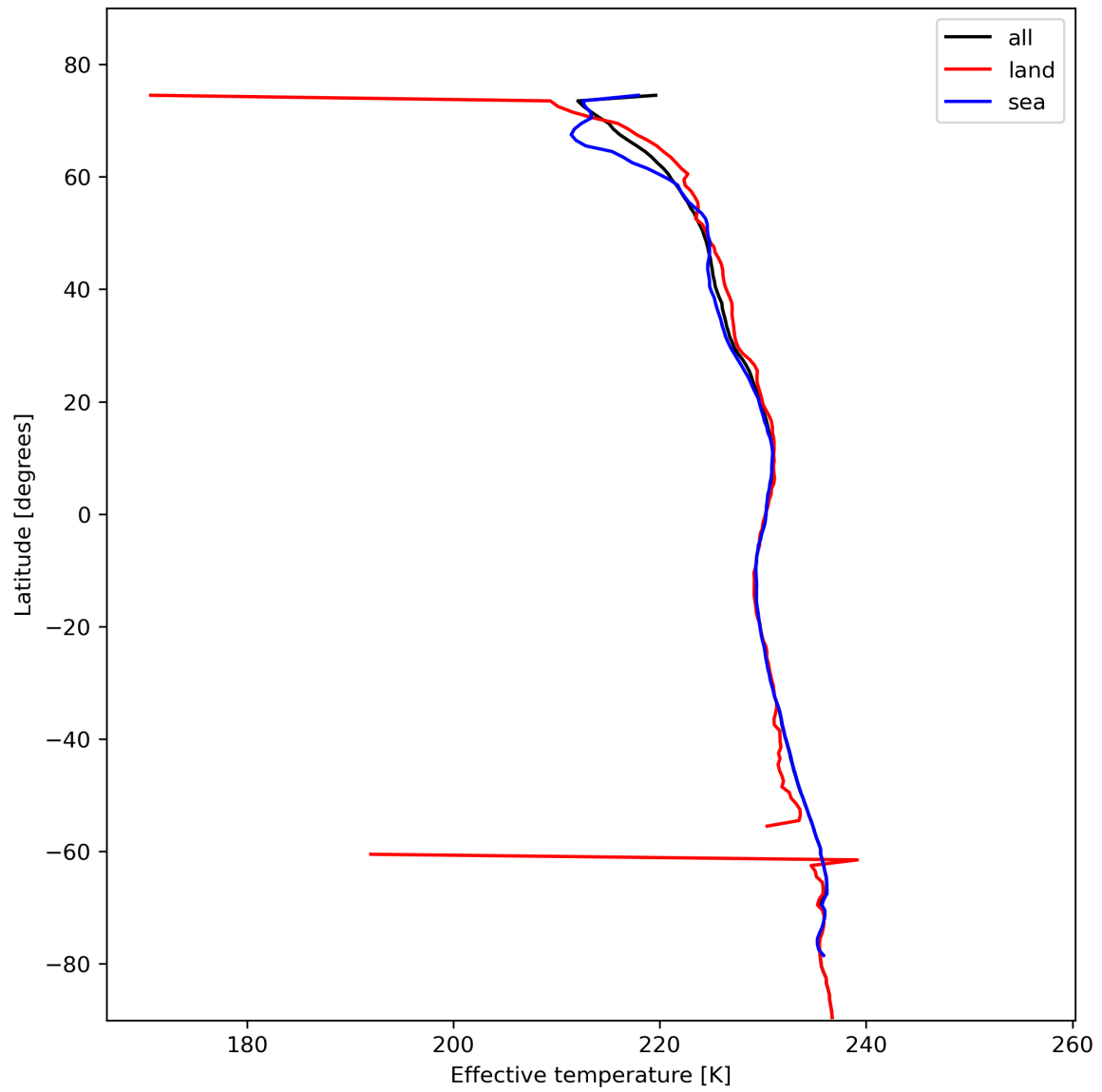
Figure 17: Zonal average of “Effective temperature” for 2024-02-07 to 2024-02-09.
