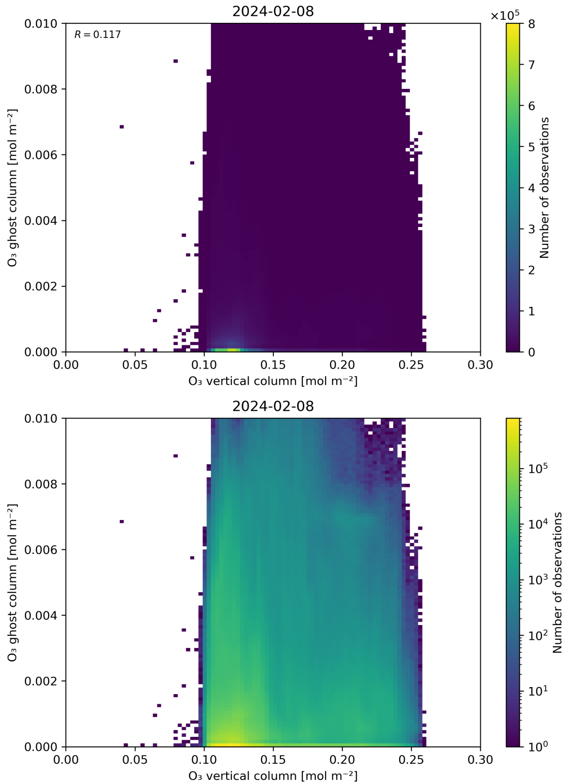
Figure 40: Scatter density plot of “O 3 vertical column” against “O 3 ghost column” for 2024-02-07 to 2024-02-09.
