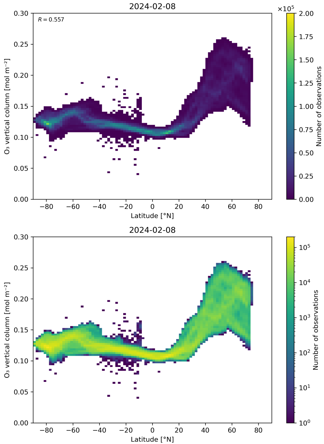
Figure 36: Scatter density plot of “Latitude” against “O 3 vertical column” for 2024-02-07 to 2024-02-09.
