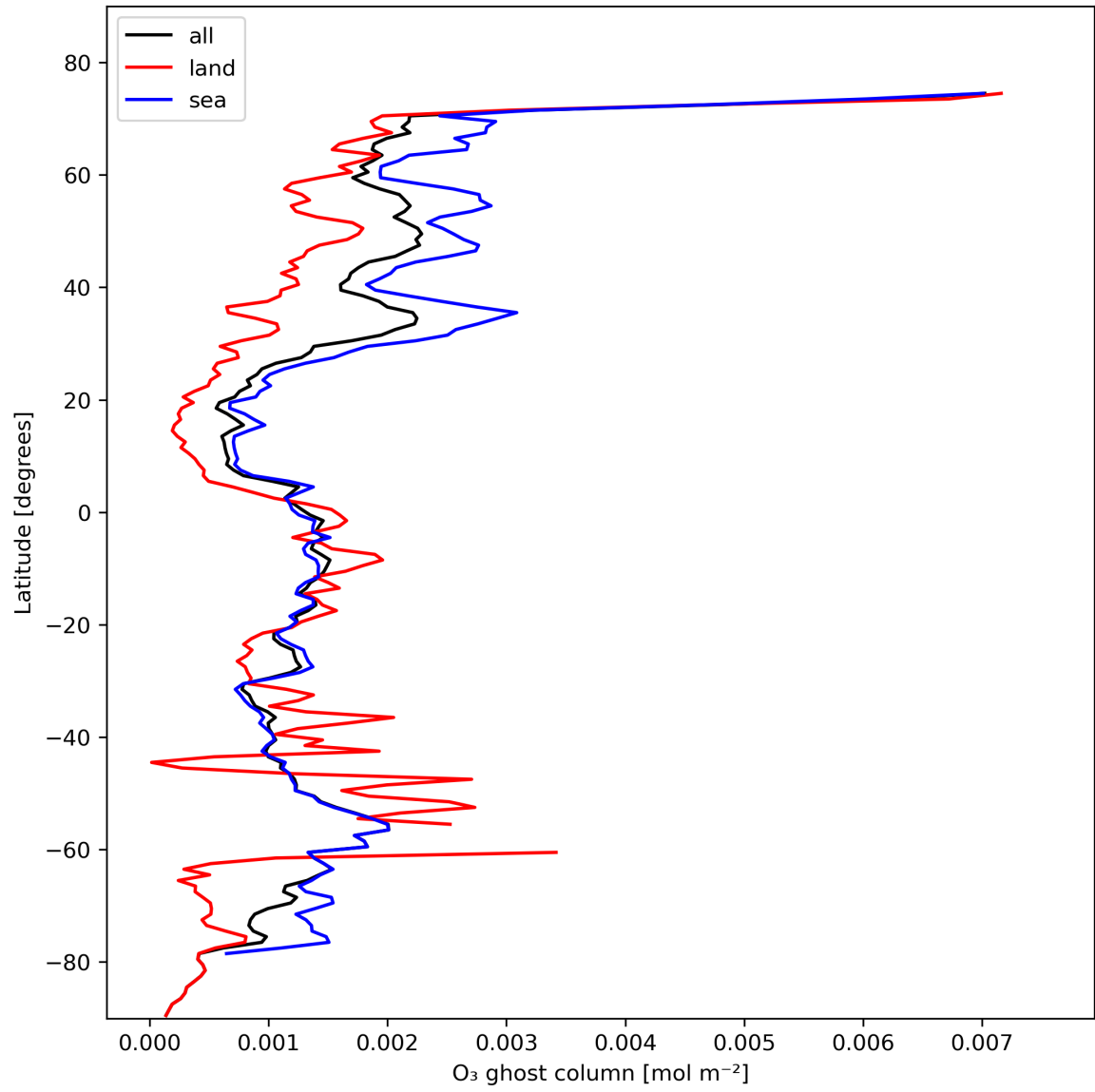
Figure 18: Zonal average of "O 3 ghost column" for 2024-02-07 to 2024-02-09.
