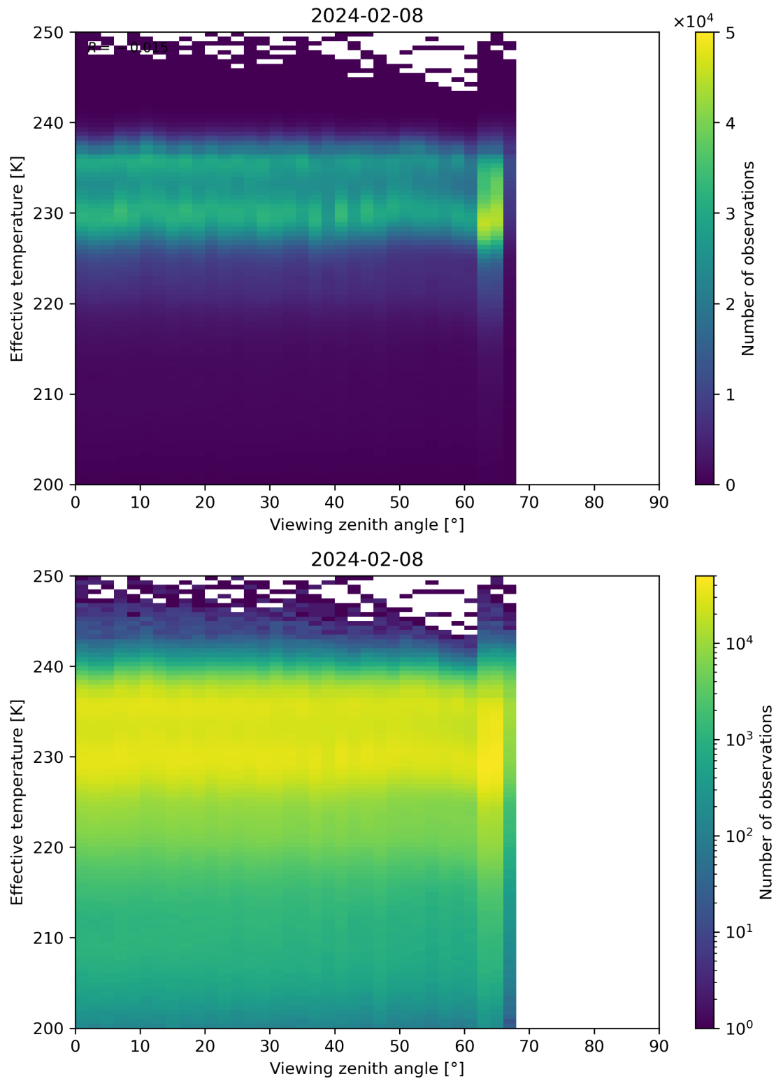
Figure 50: Scatter density plot of “Viewing zenith angle” against “Effective temperature” for 2024-02-07 to 2024-02-09.
