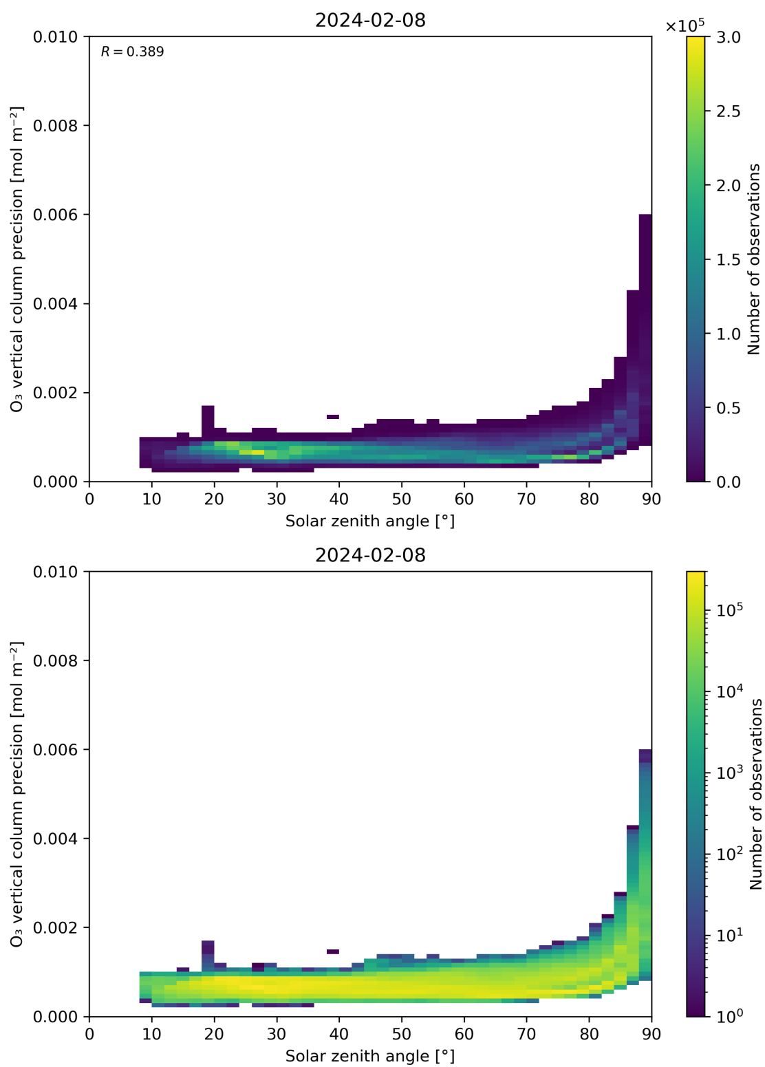
Figure 48: Scatter density plot of “Solar zenith angle” against “O 3 vertical column precision” for 2024-02-07 to 2024-02-09.
