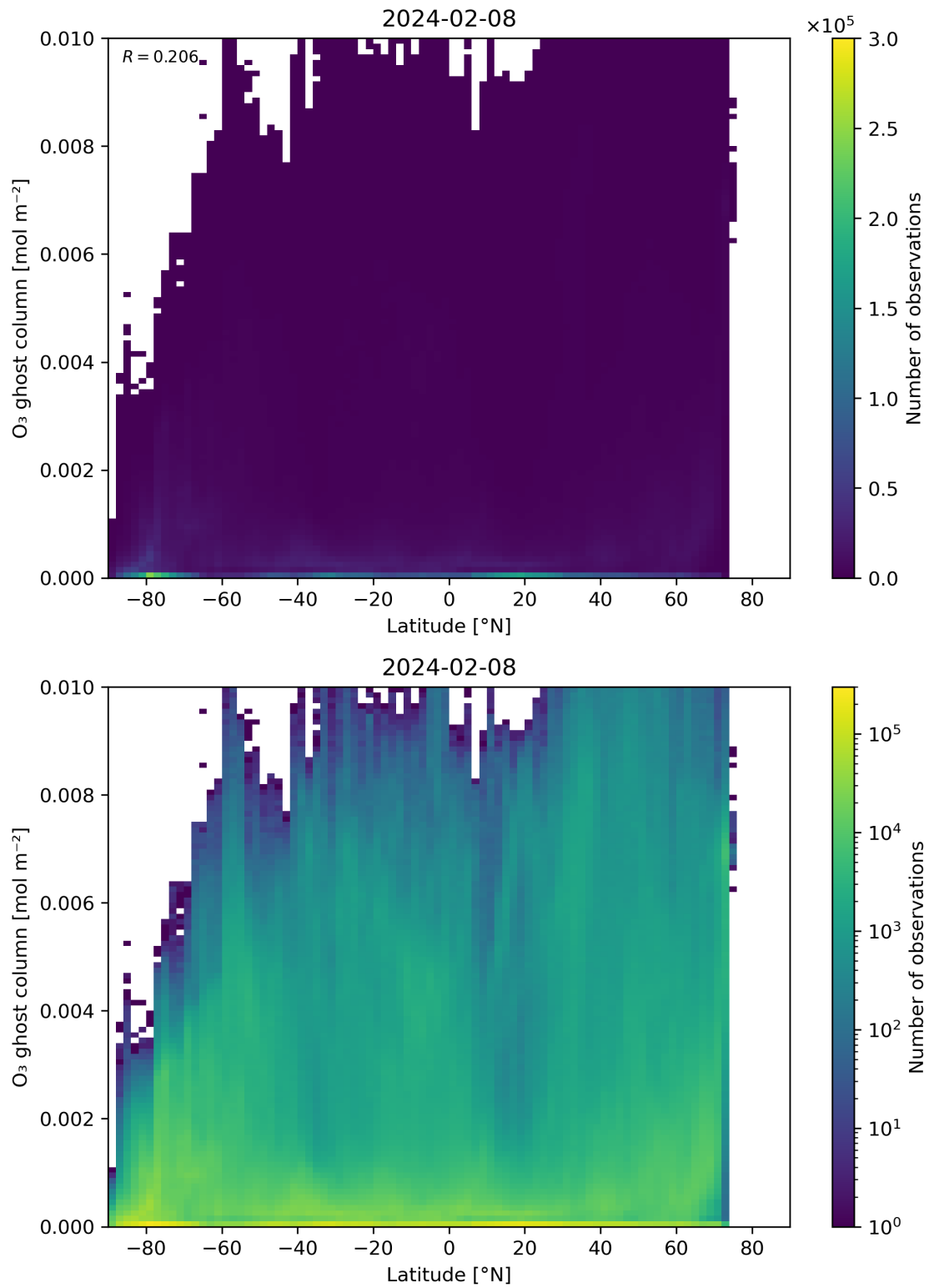
Figure 35: Scatter density plot of “Latitude” against “O 3 ghost column” for 2024-02-07 to 2024-02-09.
