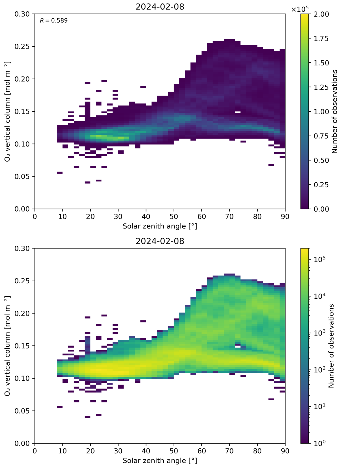
Figure 47: Scatter density plot of “Solar zenith angle” against “O 3 vertical column” for 2024-02-07 to 2024-02-09.
