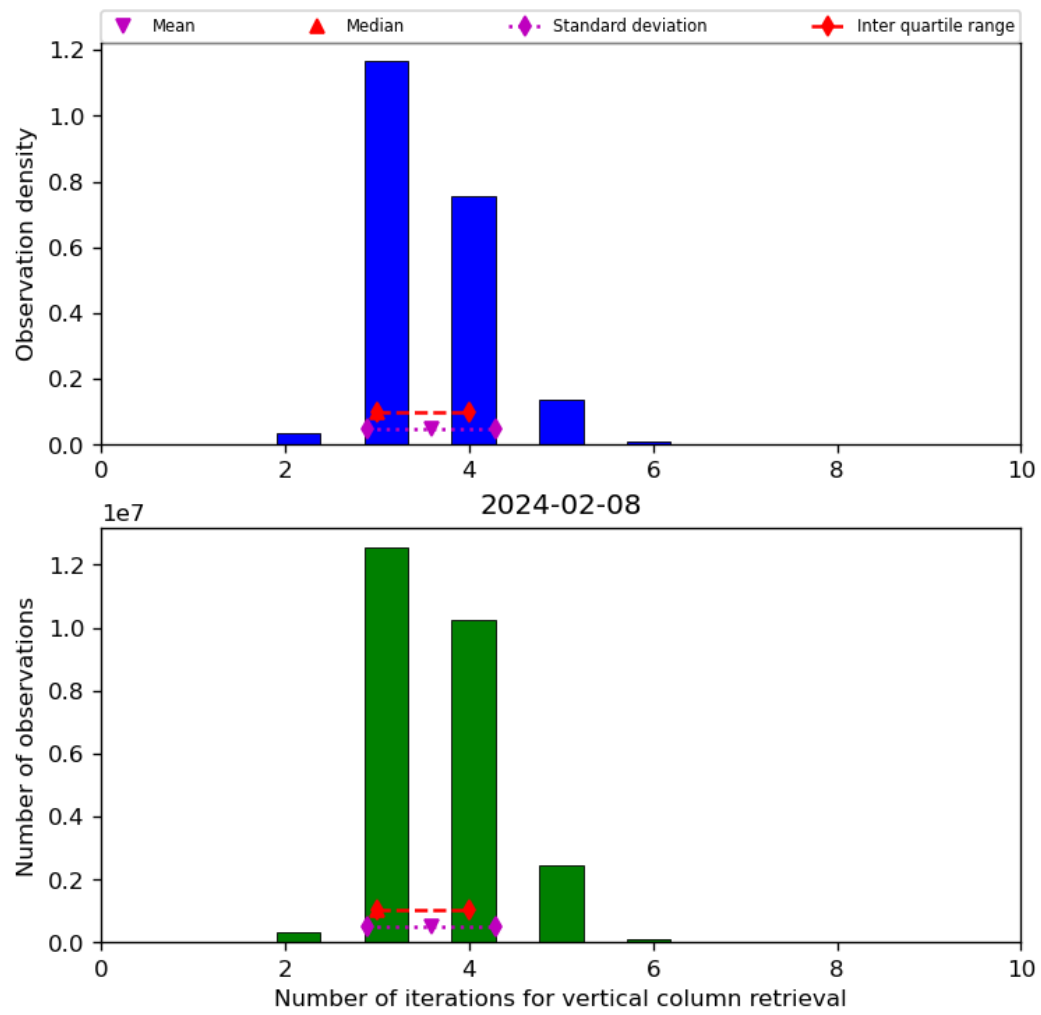
Figure 26: Histogram of “Number of iterations for vertical column retrieval” for 2024-02-07 to 2024-02-09
