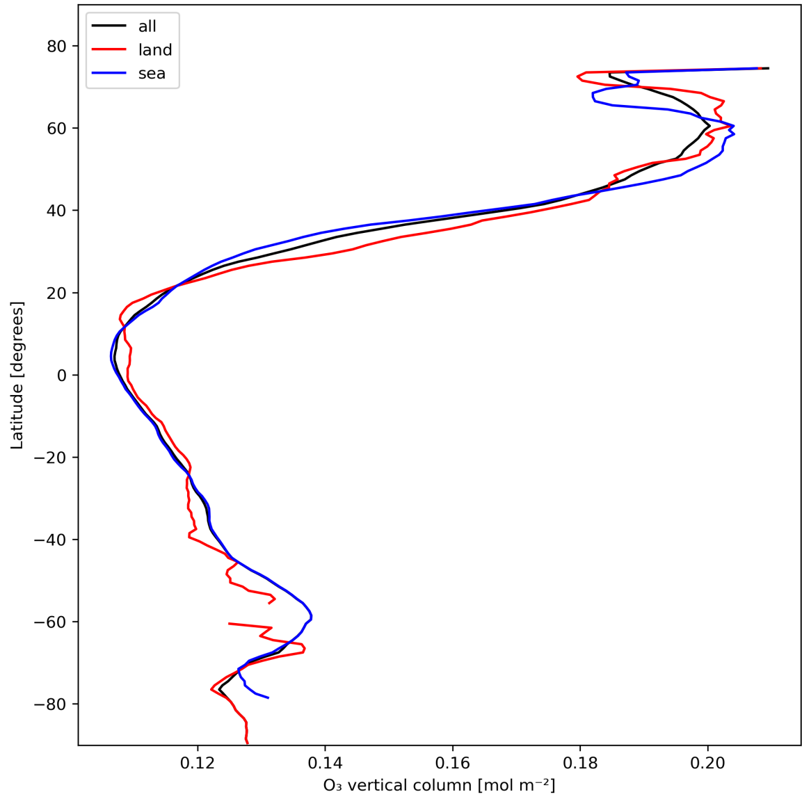
Figure 14: Zonal average of “O 3 vertical column” for 2024-02-07 to 2024-02-09.
