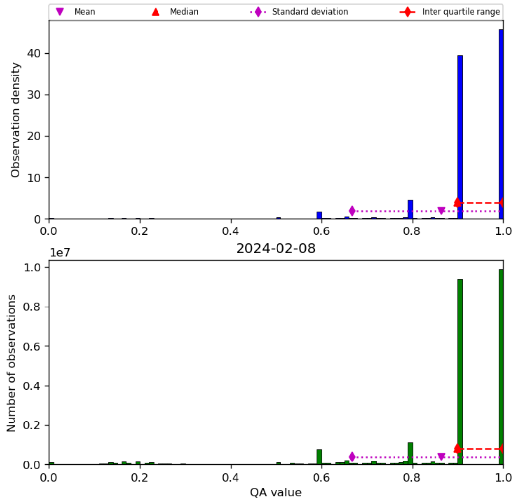
Figure 20: Histogram of “QA value” for 2024-02-07 to 2024-02-09
