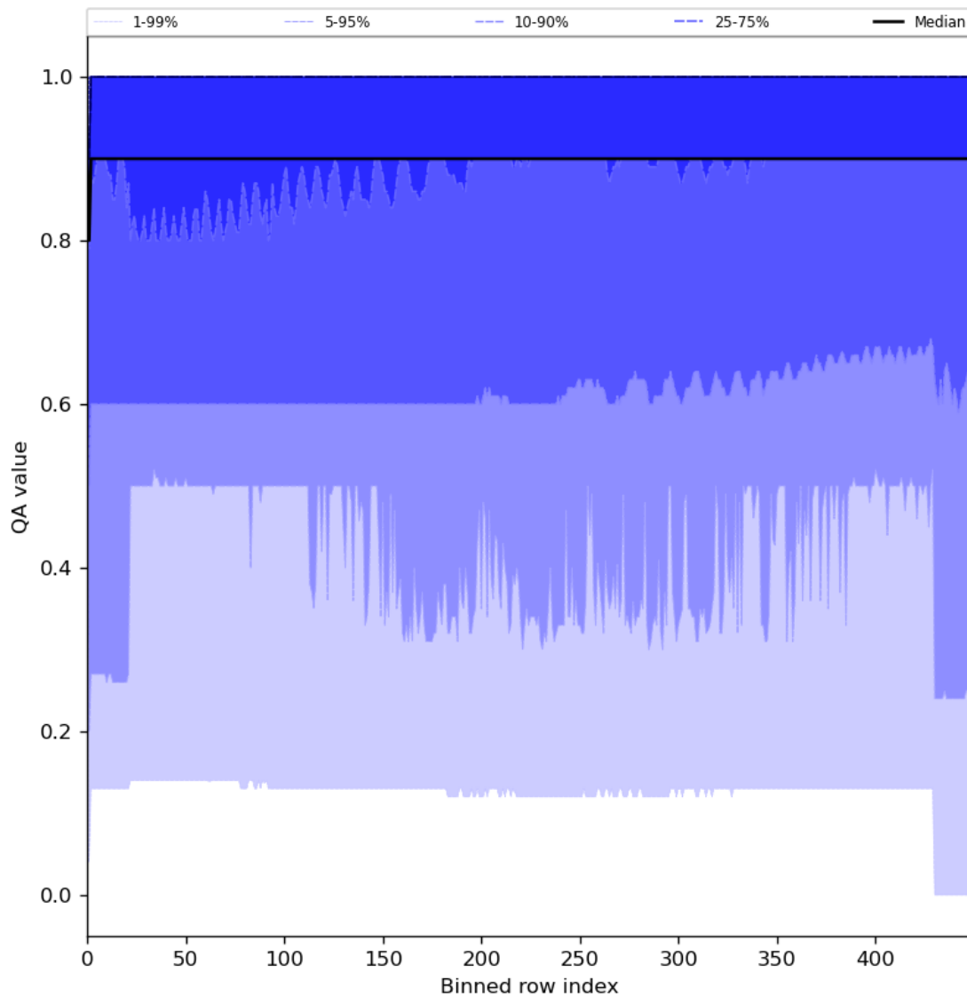
Figure 27: Along track statistics of “QA value” for 2024-02-07 to 2024-02-09
