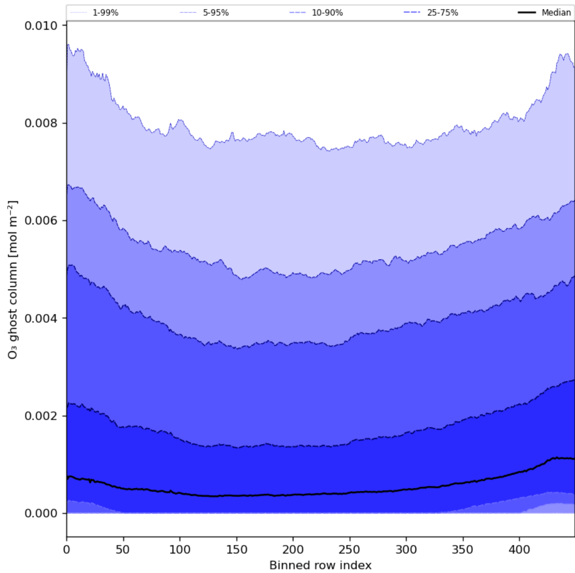
Figure 32: Along track statistics of “O 3 ghost column” for 2024-02-07 to 2024-02-09
