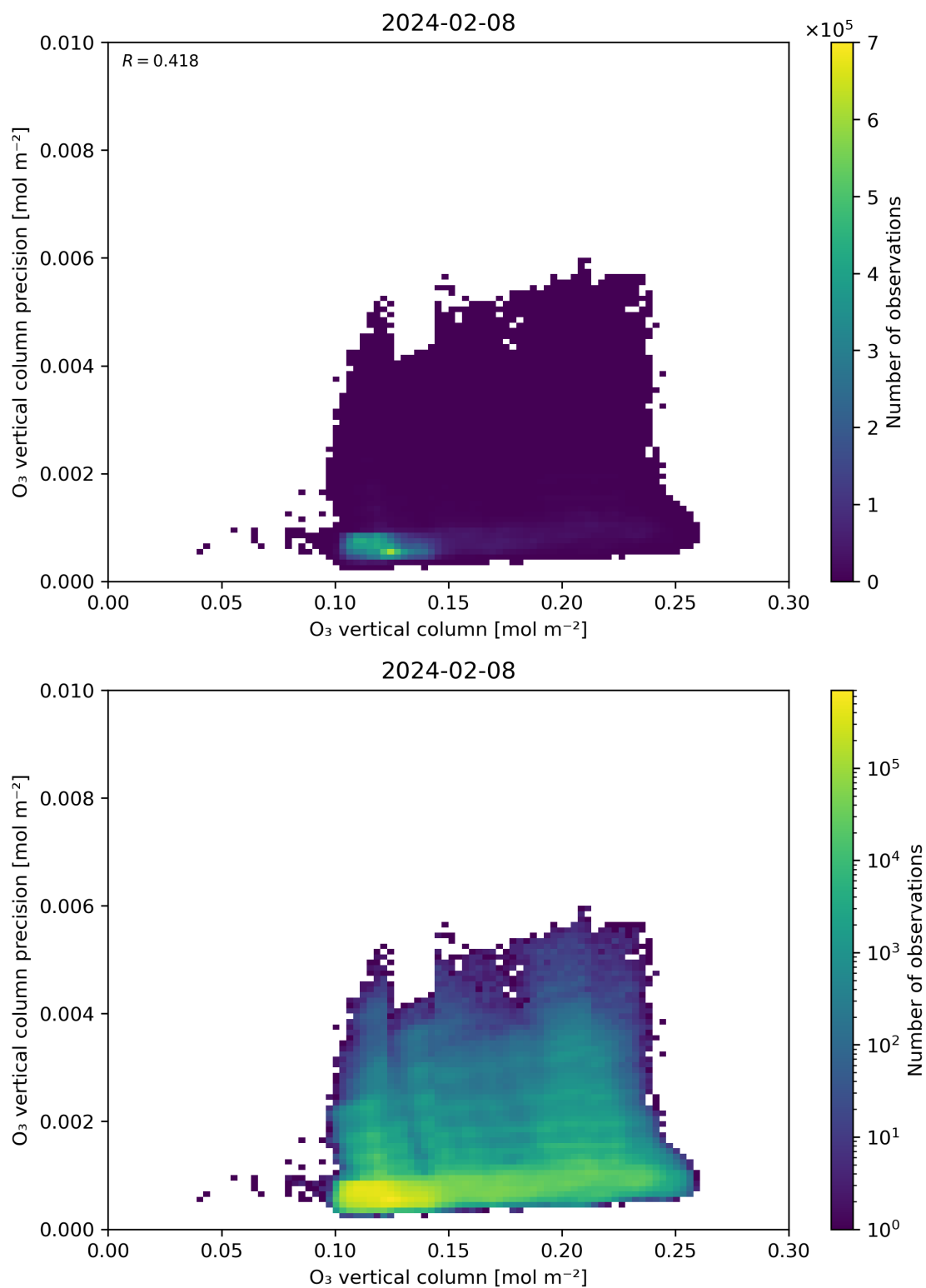
Figure 41: Scatter density plot of “O 3 vertical column” against “O 3 vertical column precision” for 2024-02-07 to 2024-02-09.
