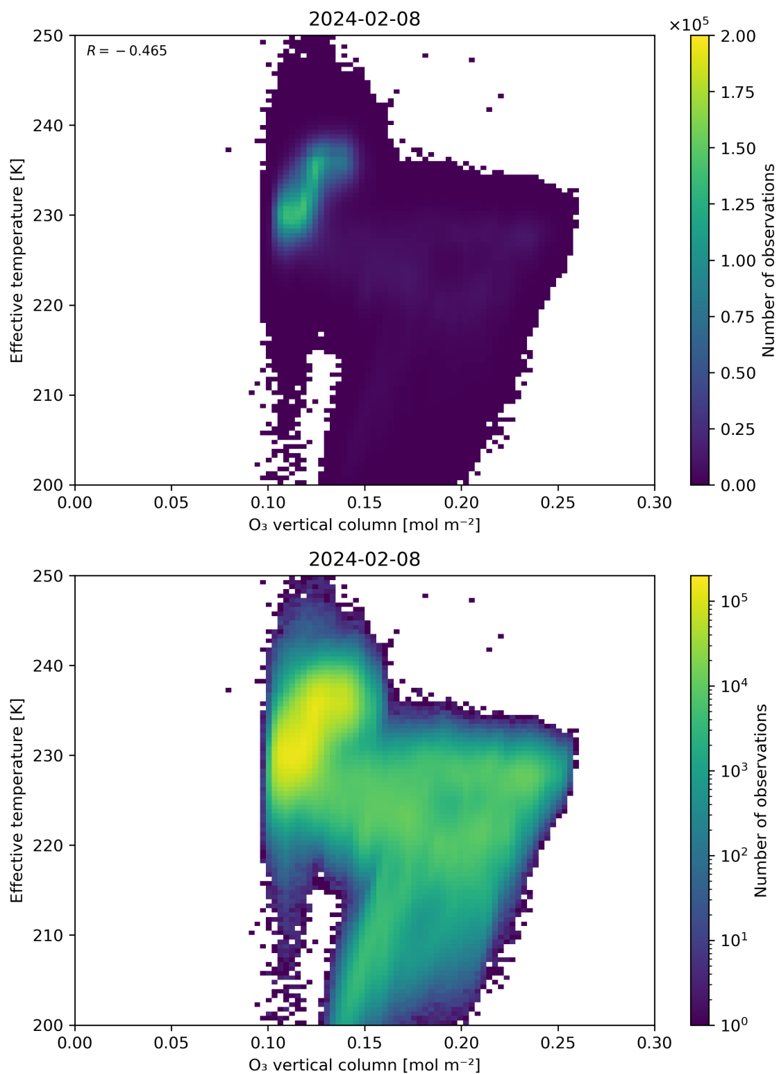
Figure 39: Scatter density plot of “O 3 vertical column” against “Effective temperature” for 2024-02-07 to 2024-02-09.
