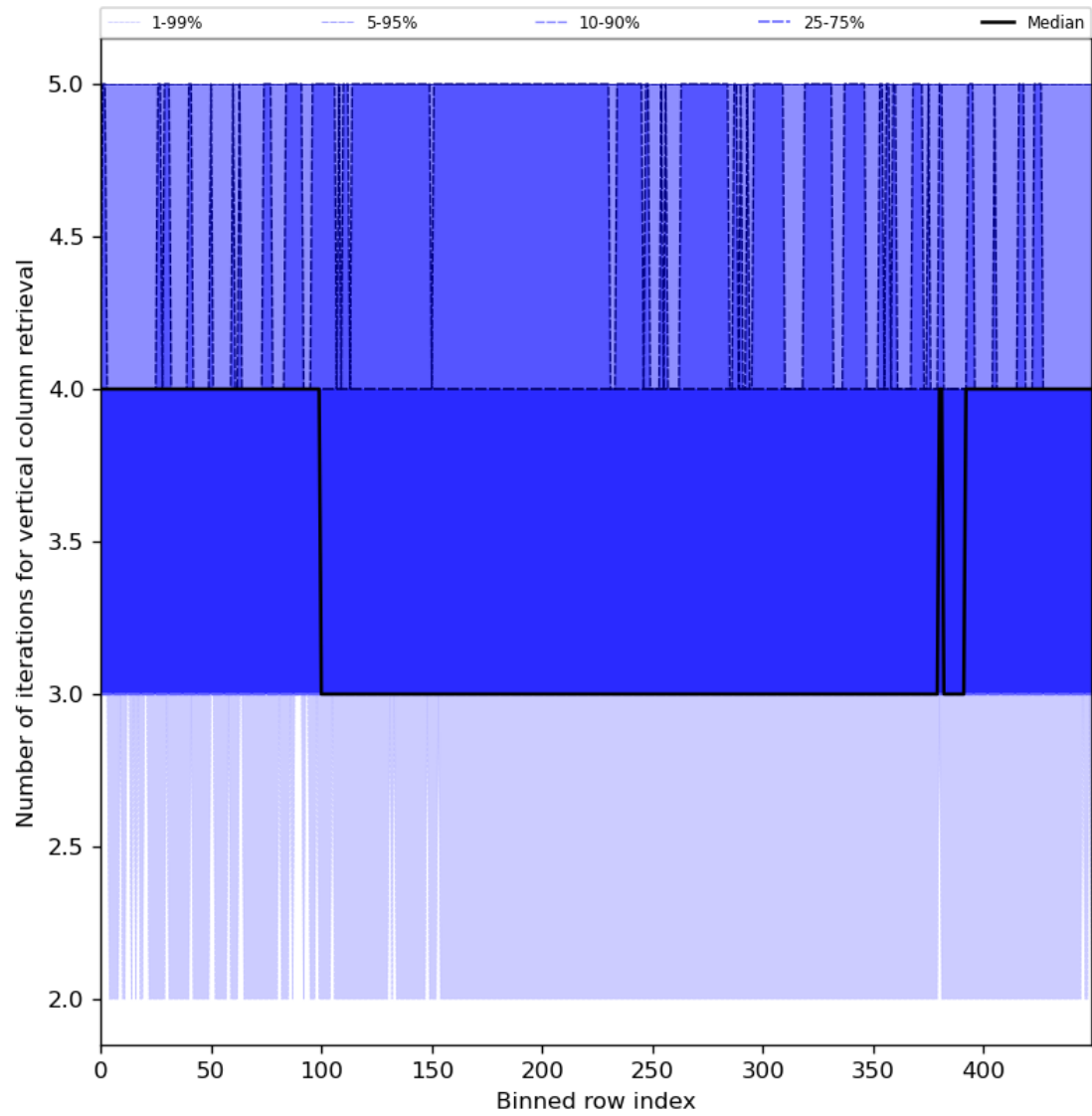
Figure 33: Along track statistics of “Number of iterations for vertical column retrieval” for 2024-02-07 to 2024-02-09
