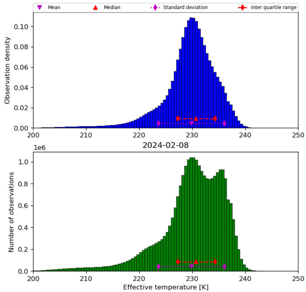
Figure 24: Histogram of “Effective temperature” for 2024-02-07 to 2024-02-09
