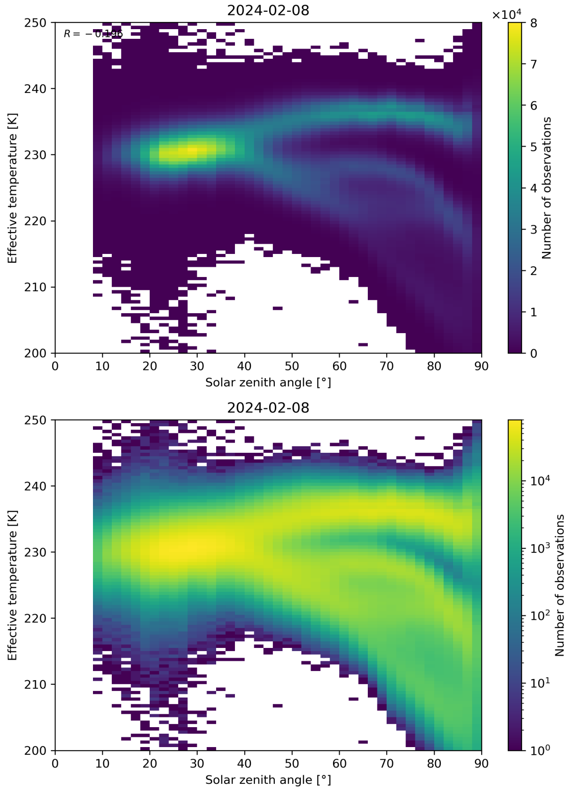
Figure 45: Scatter density plot of “Solar zenith angle” against “Effective temperature” for 2024-02-07 to 2024-02-09.
