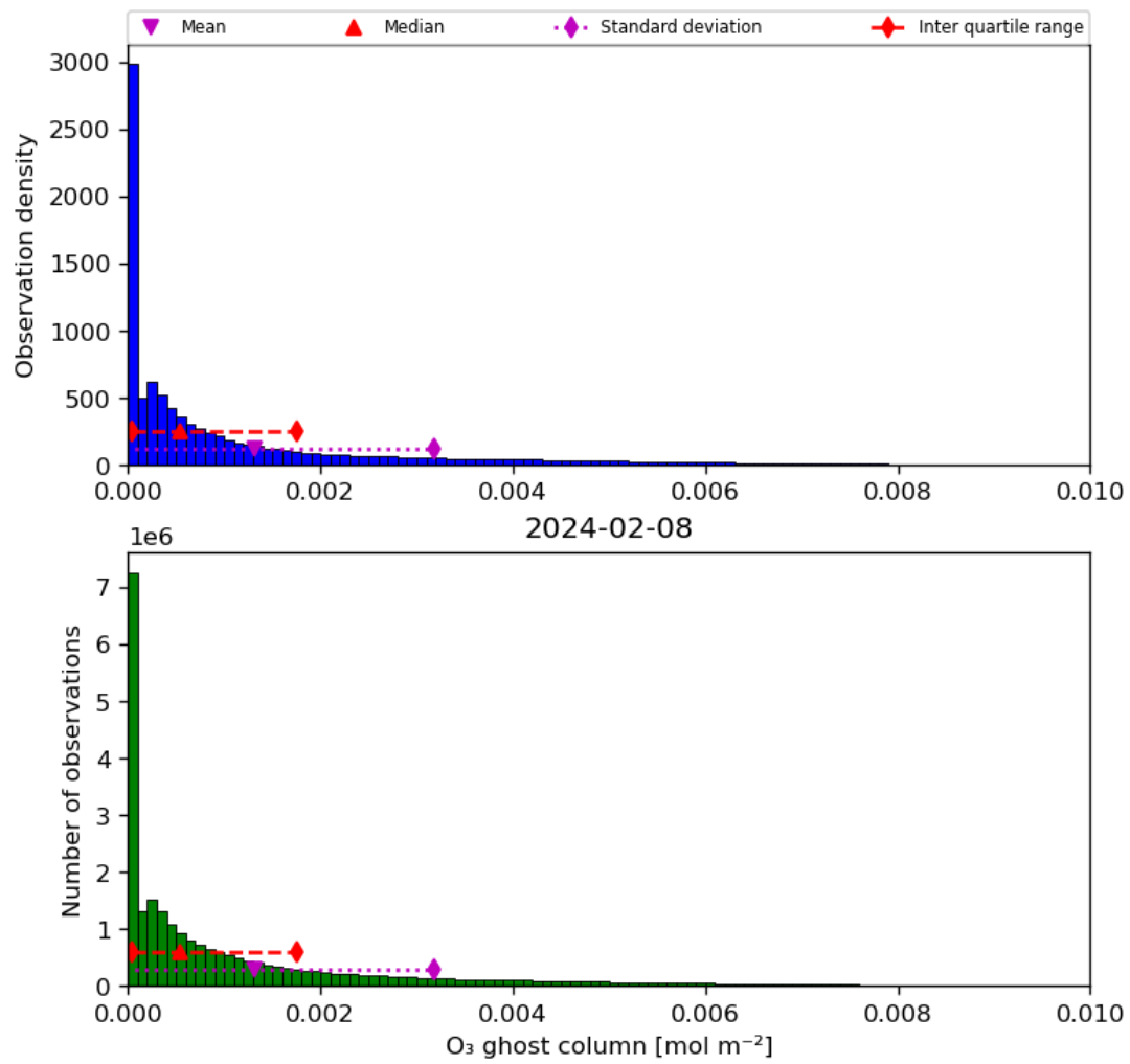
Figure 25: Histogram of “O 3 ghost column” for 2024-02-07 to 2024-02-09
