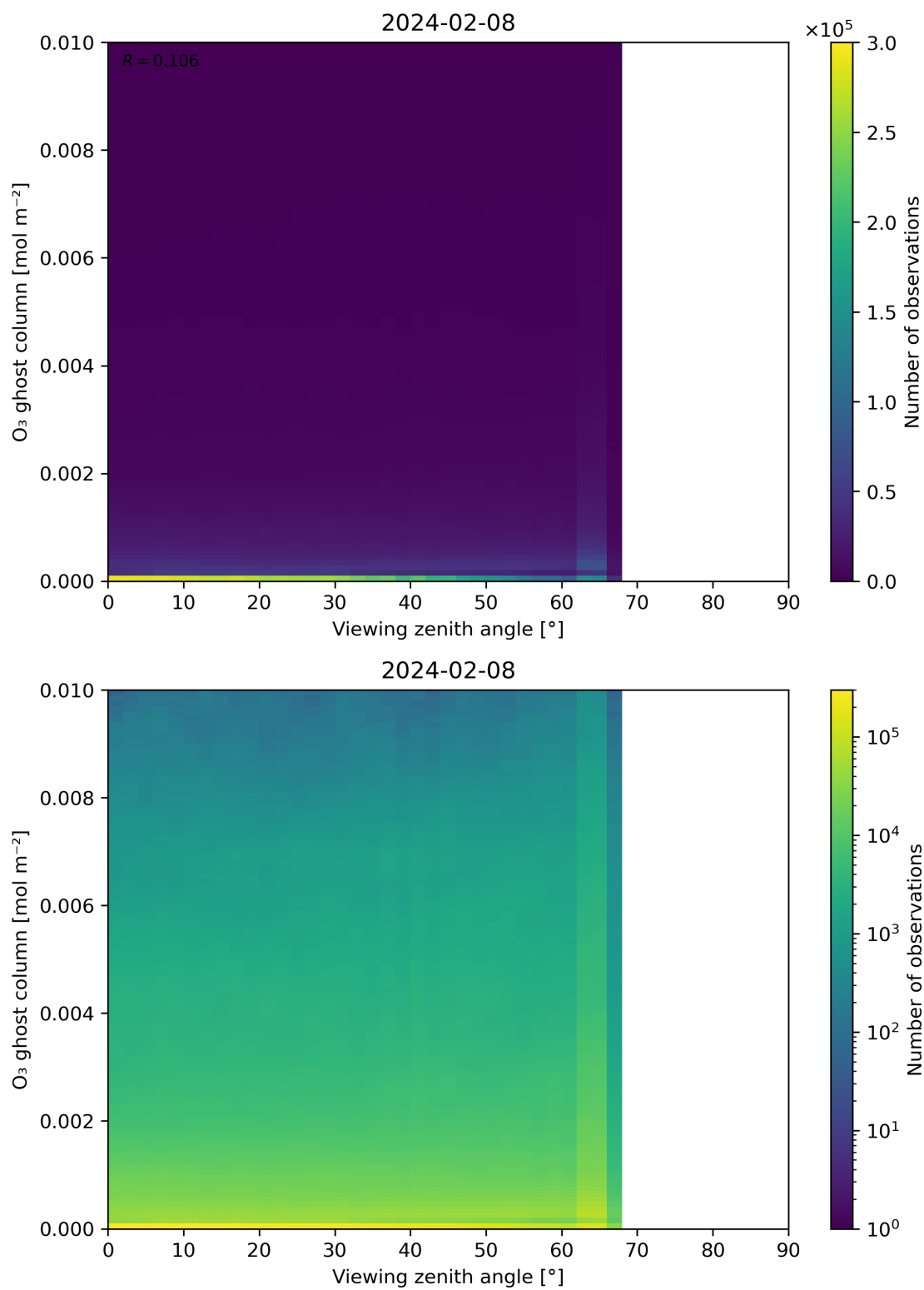
Figure 51: Scatter density plot of “Viewing zenith angle” against “O 3 ghost column” for 2024-02-07 to 2024-02-09.
