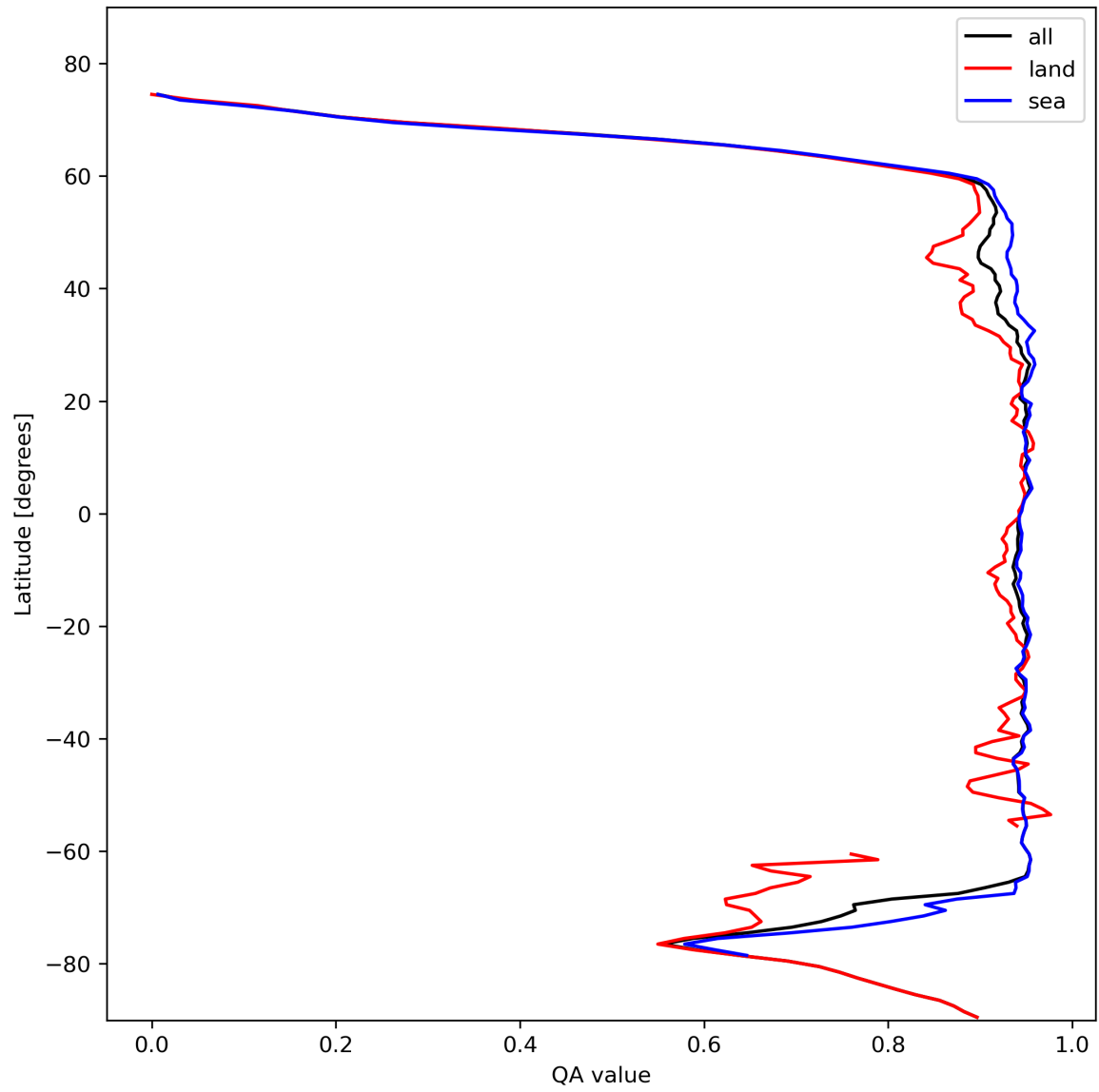
Figure 13: Zonal average of “QA value” for 2024-02-07 to 2024-02-09.
