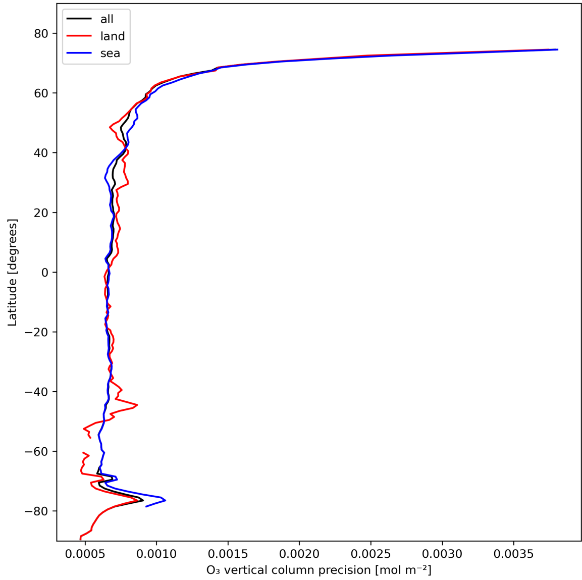
Figure 15: Zonal average of “O 3 vertical column precision” for 2024-02-07 to 2024-02-09.
