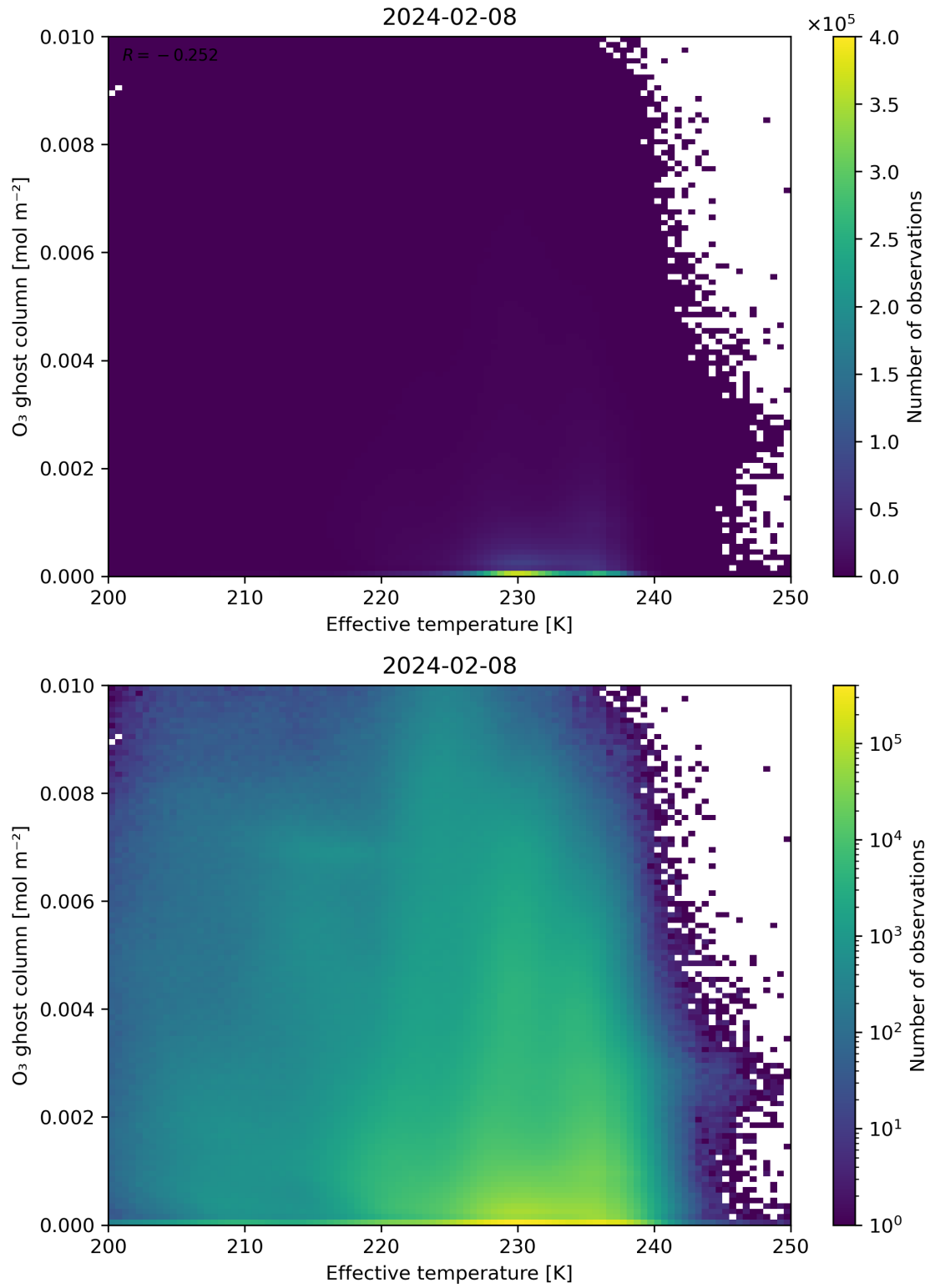
Figure 38: Scatter density plot of “Effective temperature” against “O 3 ghost column” for 2024-02-07 to 2024-02-09.
