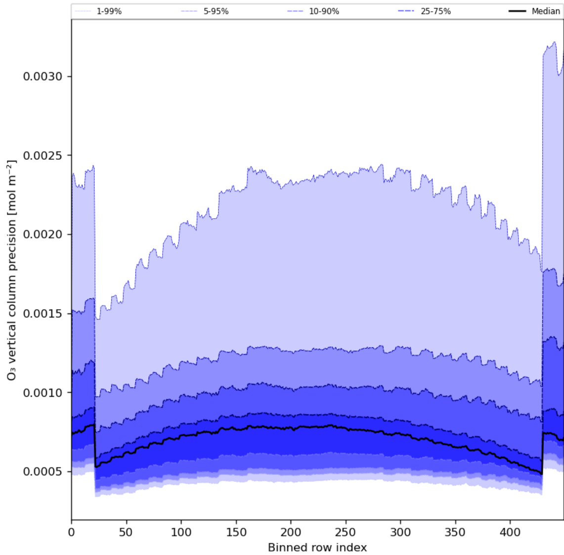
Figure 29: Along track statistics of “O 3 vertical column precision” for 2024-02-07 to 2024-02-09
