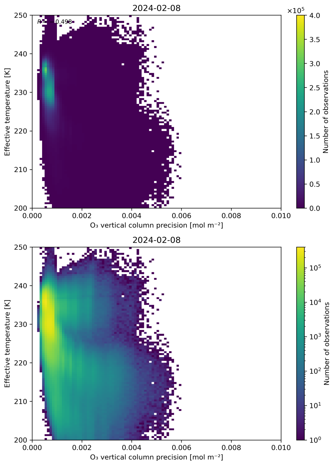
Figure 42: Scatter density plot of “ O_3 vertical column precision” against “Effective temperature” for 2024-02-07 to 2024-02-09.
