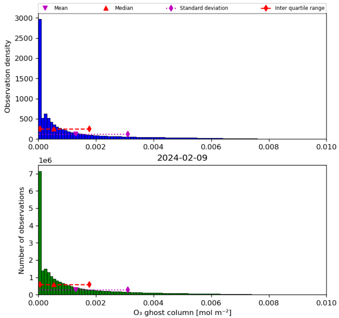
Figure 25: Histogram of “O 3 ghost column” for 2024-02-08 to 2024-02-10
