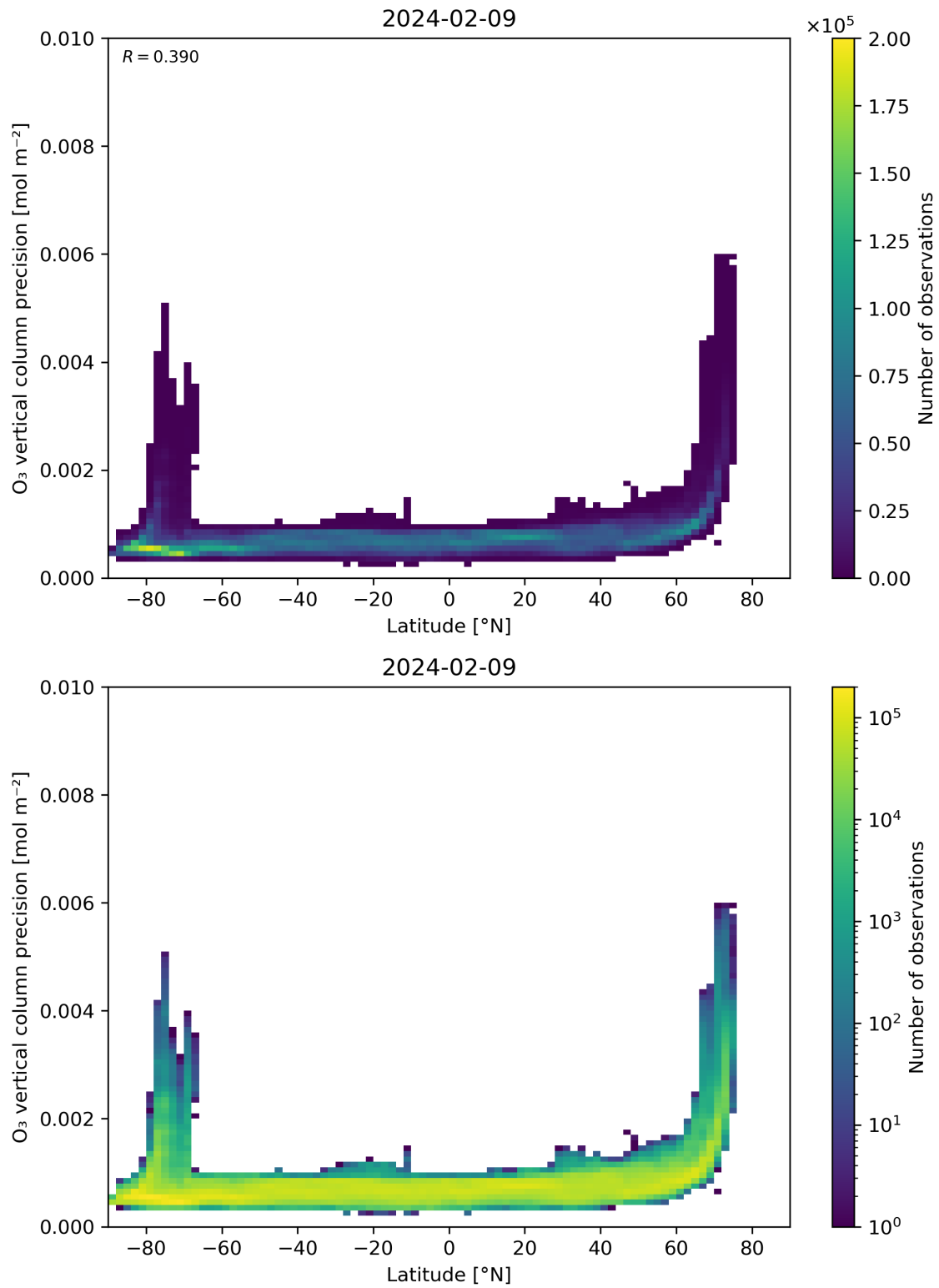
Figure 37: Scatter density plot of “Latitude” against “O 3 vertical column precision” for 2024-02-08 to 2024-02-10.
