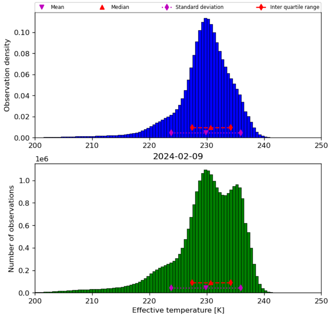
Figure 24: Histogram of “Effective temperature” for 2024-02-08 to 2024-02-10
