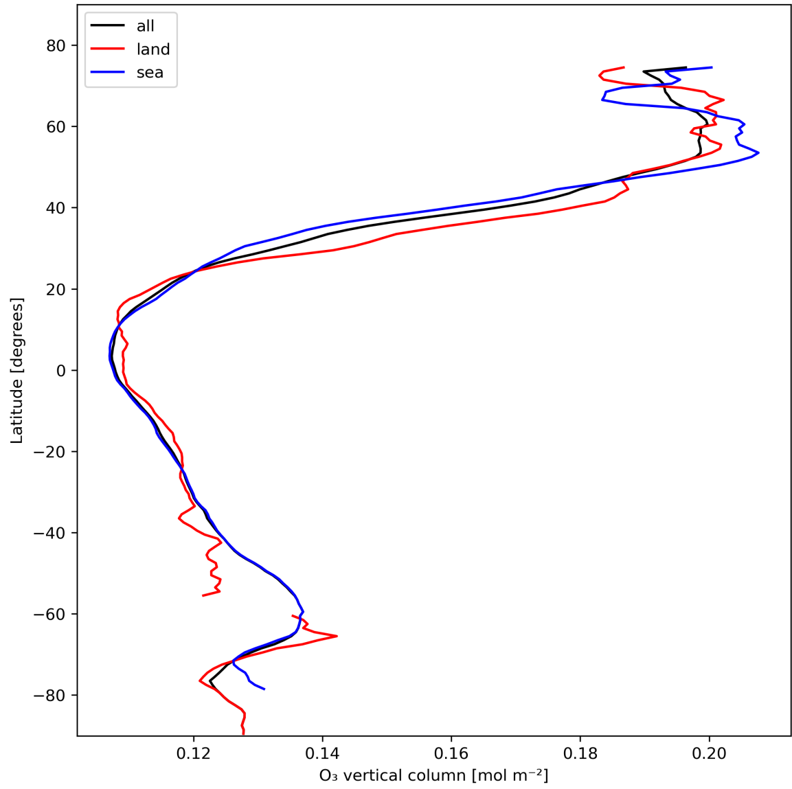
Figure 14: Zonal average of “O 3 vertical column” for 2024-02-08 to 2024-02-10.
