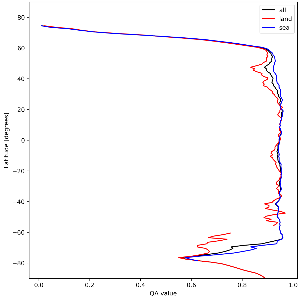
Figure 13: Zonal average of “QA value” for 2024-02-08 to 2024-02-10.
