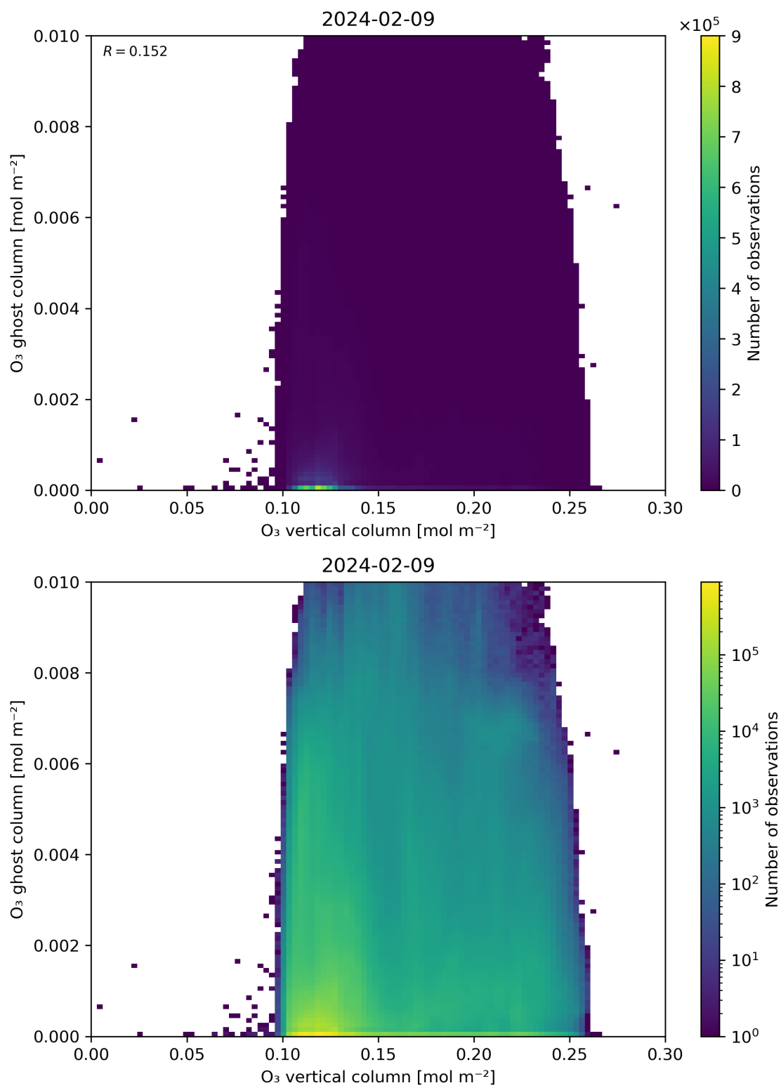
Figure 40: Scatter density plot of “O 3 vertical column” against “O 3 ghost column” for 2024-02-08 to 2024-02-10.
