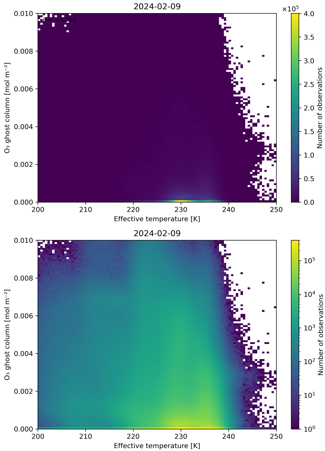
Figure 38: Scatter density plot of “Effective temperature” against “O 3 ghost column” for 2024-02-08 to 2024-02-10.
