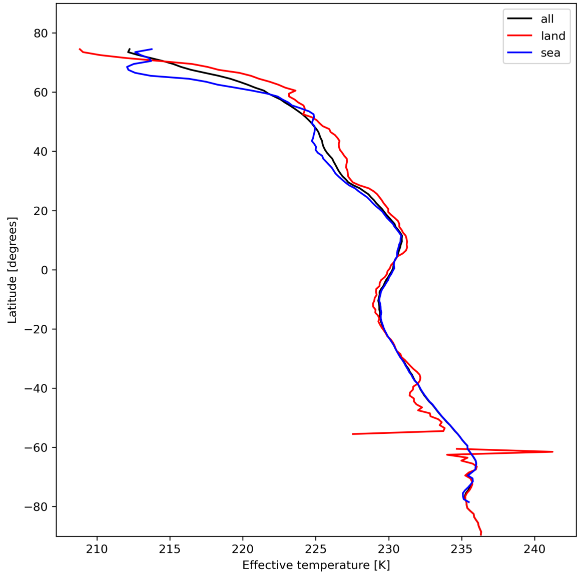
Figure 17: Zonal average of "Effective temperature" for 2024-02-08 to 2024-02-10.
