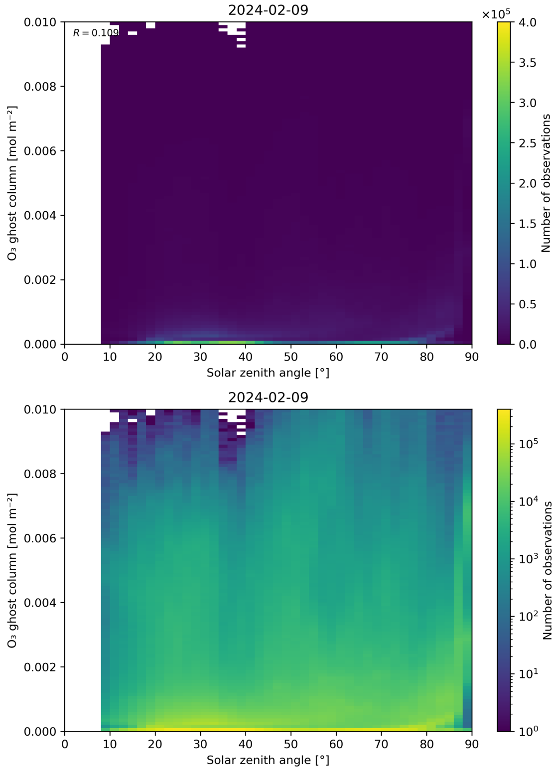
Figure 46: Scatter density plot of “Solar zenith angle” against “O 3 ghost column” for 2024-02-08 to 2024-02-10.
