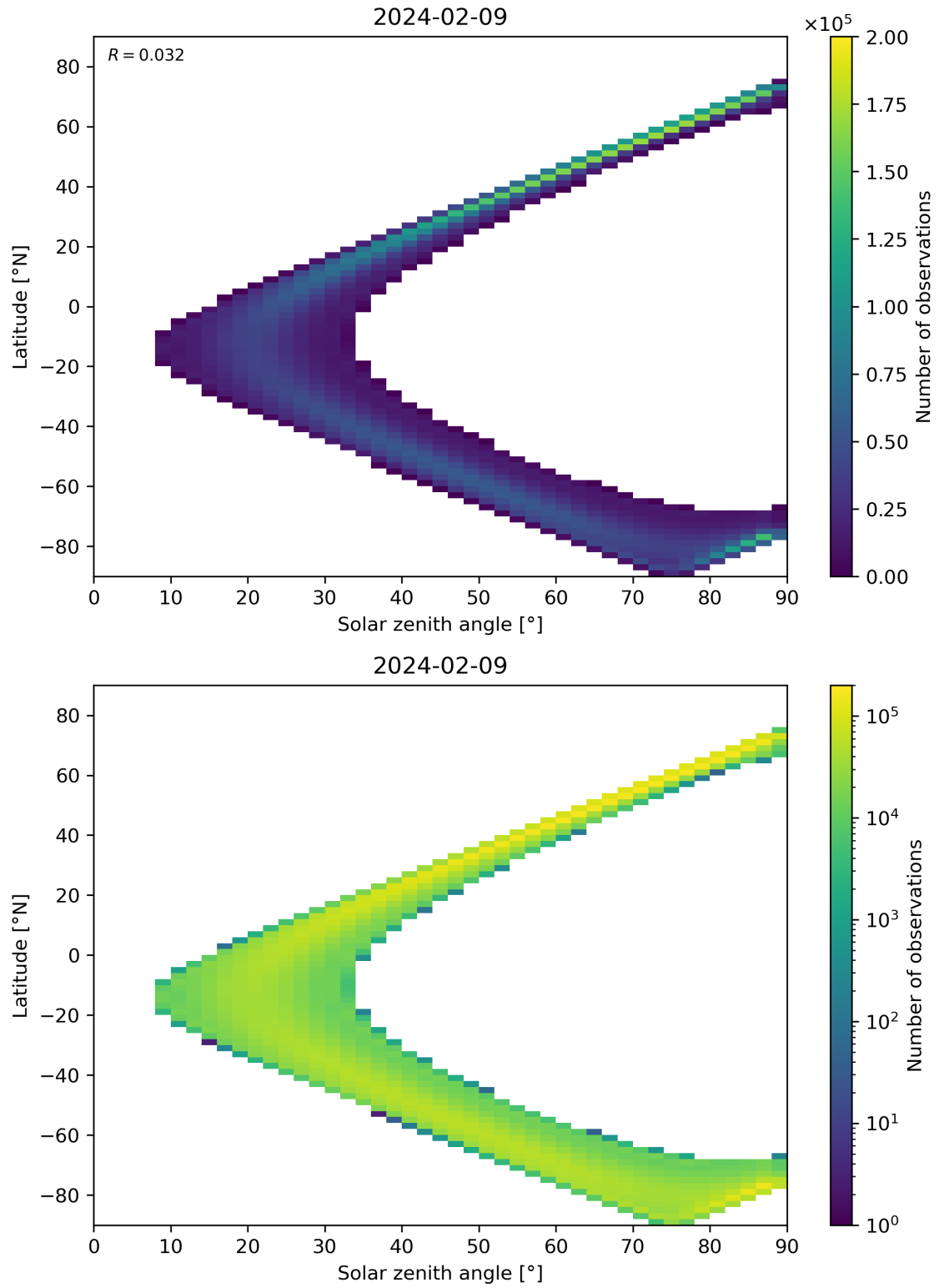
Figure 44: Scatter density plot of “Solar zenith angle” against “Latitude” for 2024-02-08 to 2024-02-10.
