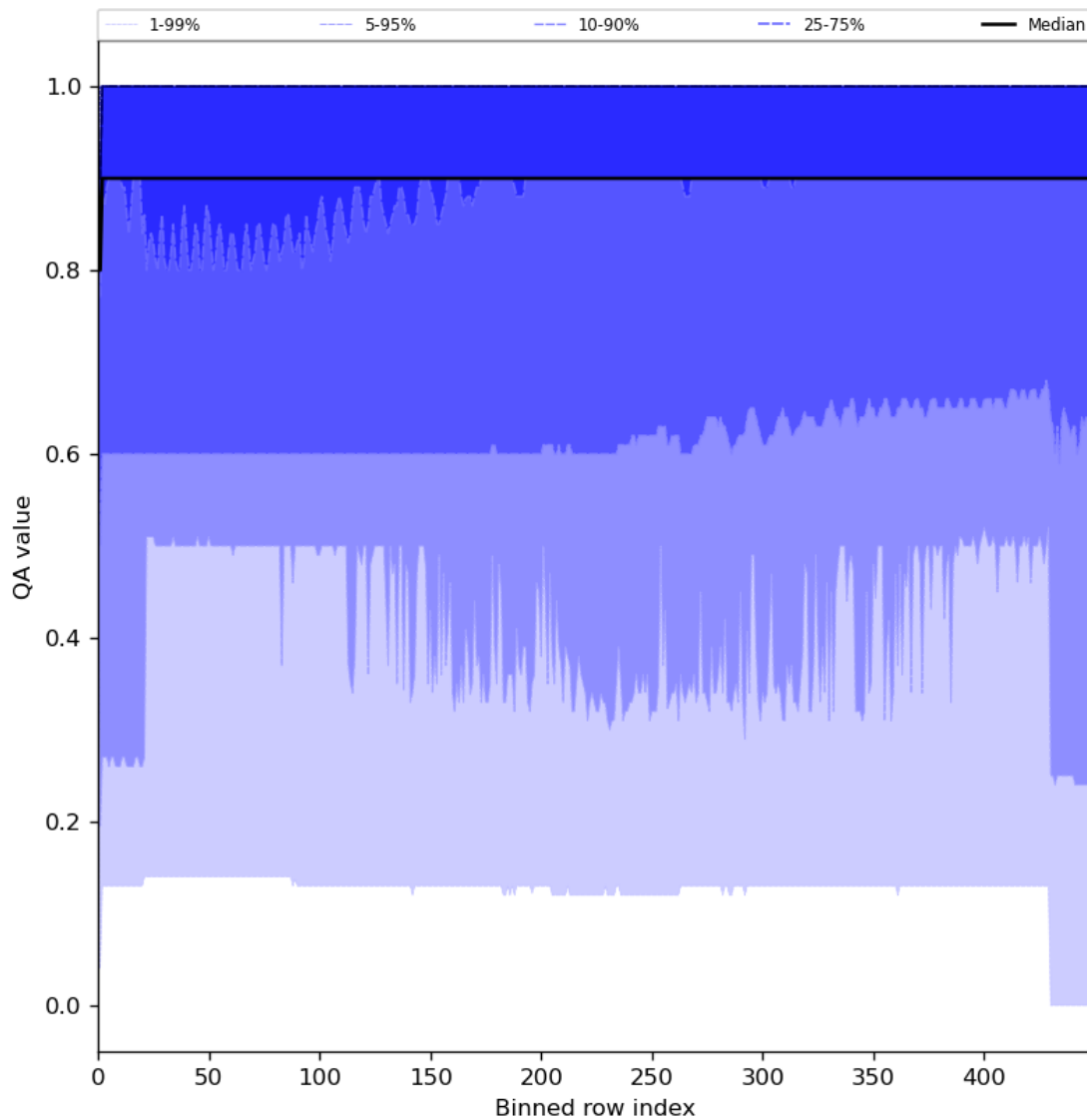
Figure 27: Along track statistics of “QA value” for 2024-02-08 to 2024-02-10
