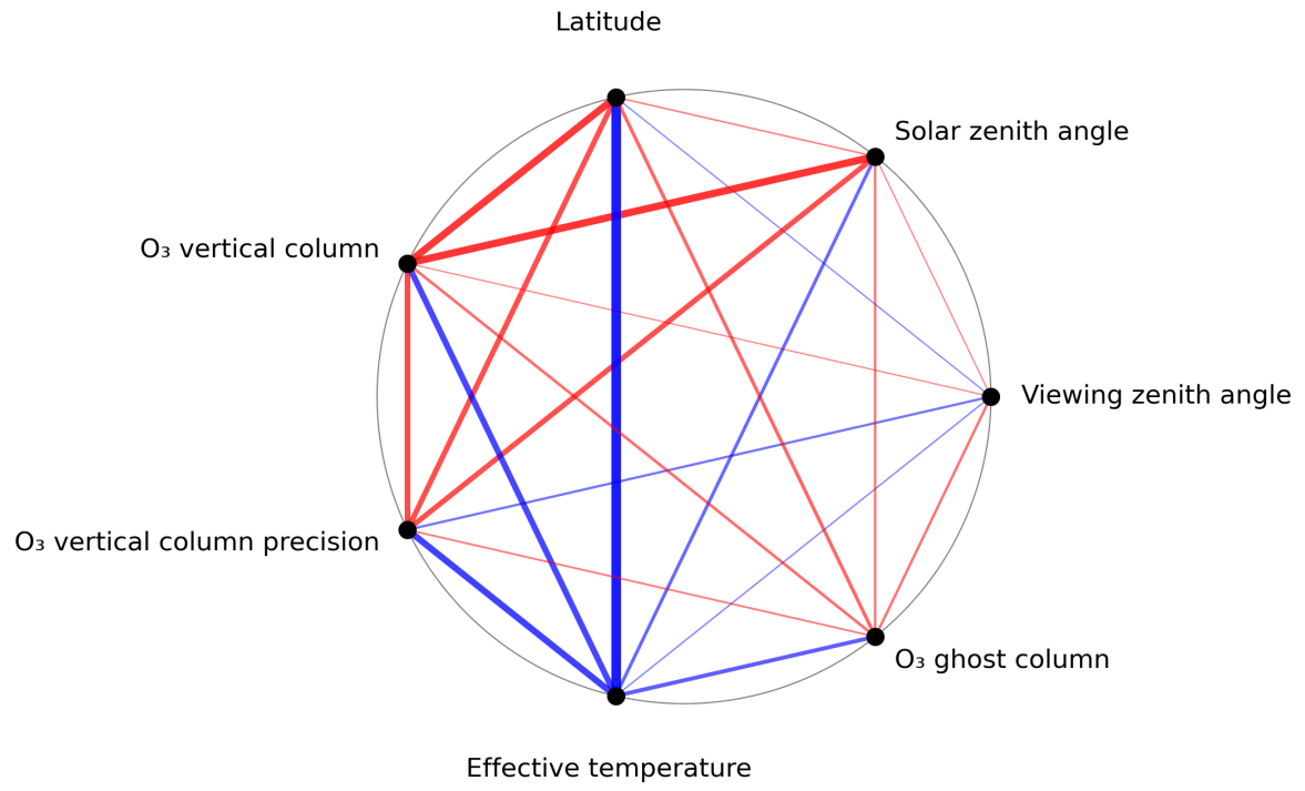
Figure 1: Map of correlation graph for 2024-02-08 to 2024-02-10.
