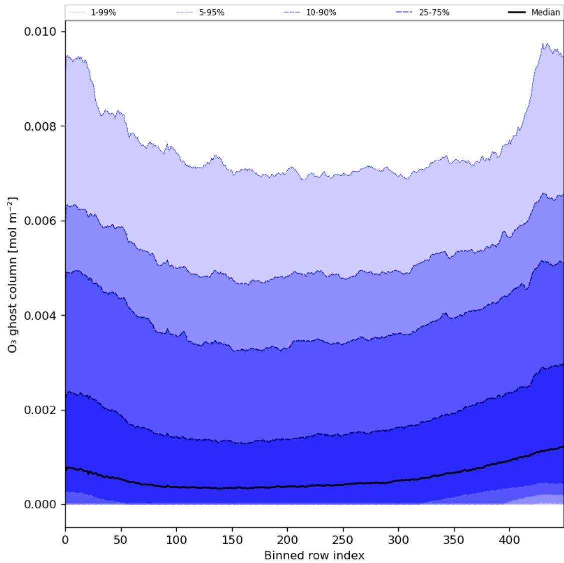
Figure 32: Along track statistics of “O 3 ghost column” for 2024-02-08 to 2024-02-10
