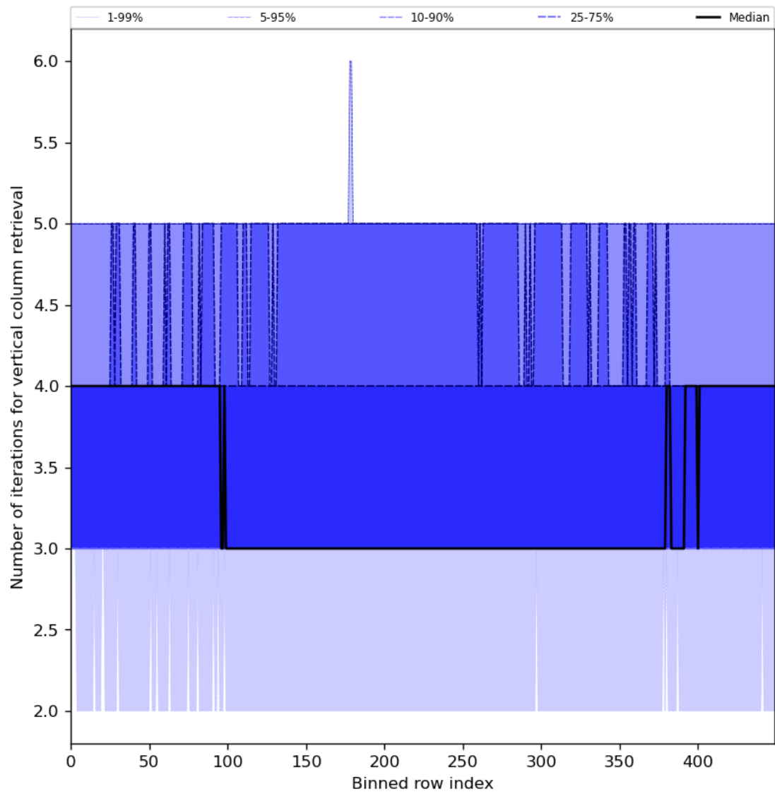
Figure 33: Along track statistics of “Number of iterations for vertical column retrieval” for 2024-02-08 to 2024-02-10
