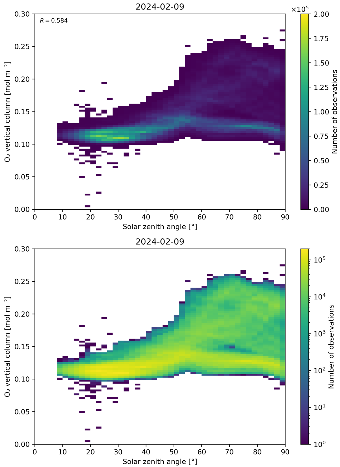
Figure 47: Scatter density plot of “Solar zenith angle” against “O 3 vertical column” for 2024-02-08 to 2024-02-10.
