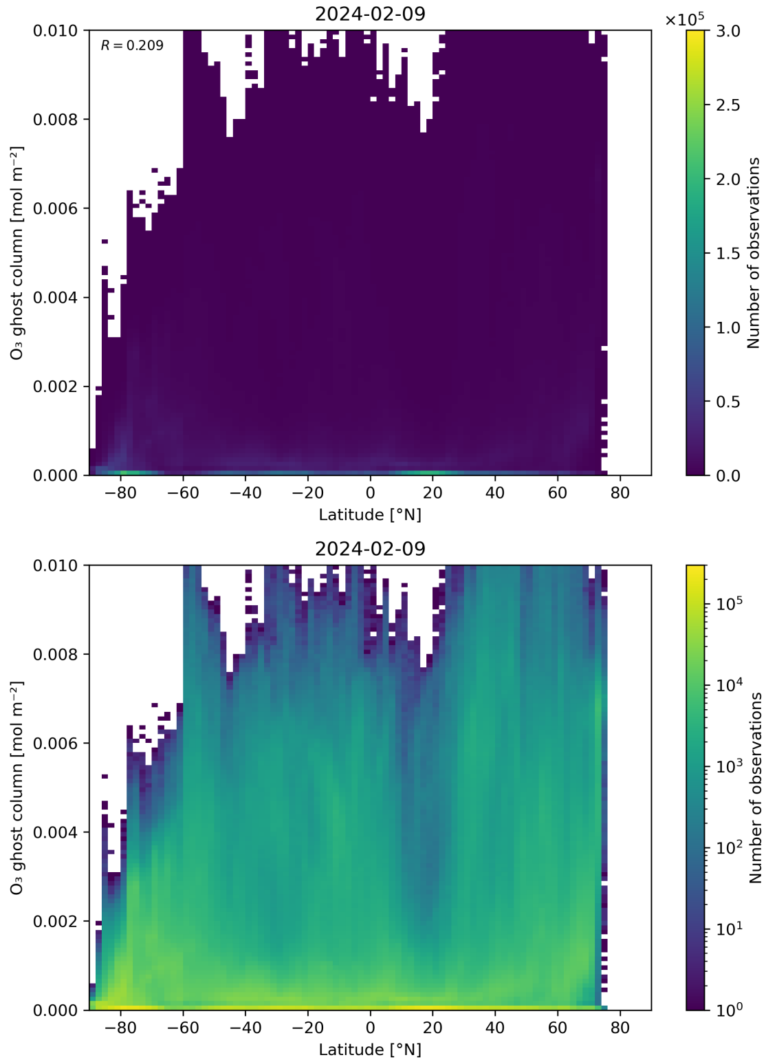
Figure 35: Scatter density plot of “Latitude” against “O 3 ghost column” for 2024-02-08 to 2024-02-10.
