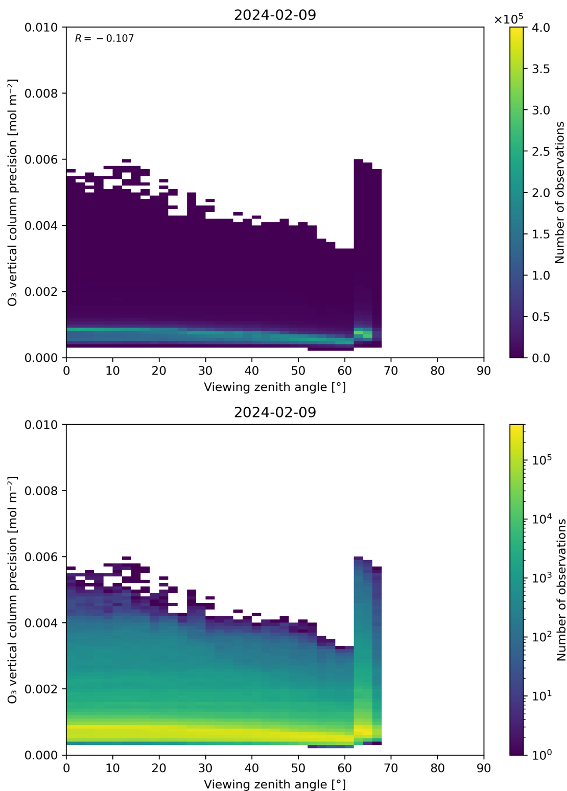
Figure 53: Scatter density plot of “Viewing zenith angle” against “O 3 vertical column precision” for 2024-02-08 to 2024-02-10.
