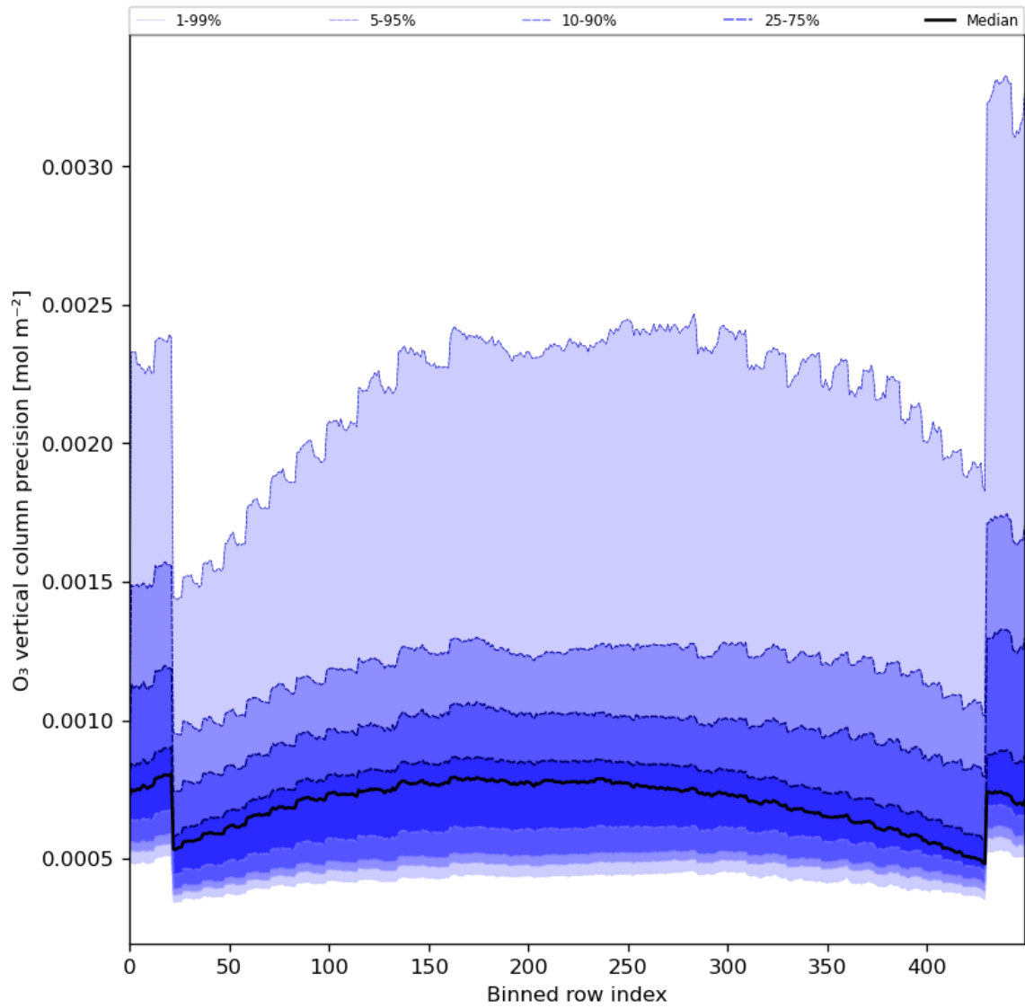
Figure 29: Along track statistics of “O 3 vertical column precision” for 2024-02-08 to 2024-02-10
