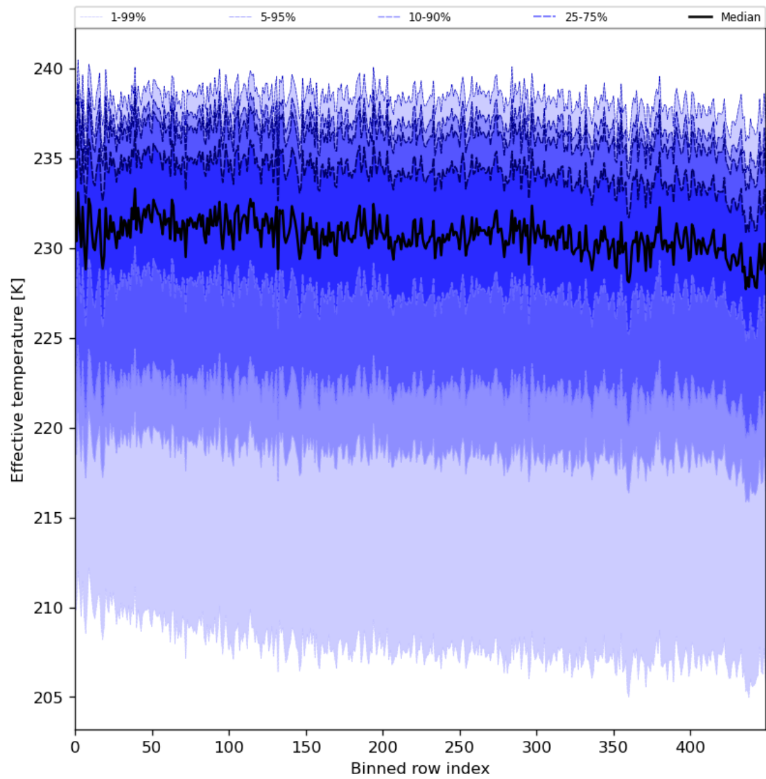
Figure 31: Along track statistics of “Effective temperature” for 2024-02-08 to 2024-02-10
