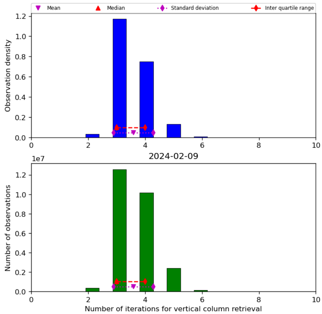
Figure 26: Histogram of “Number of iterations for vertical column retrieval” for 2024-02-08 to 2024-02-10
