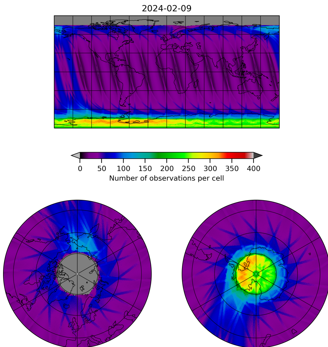
Figure 12: Map of the number of observations for 2024-02-08 to 2024-02-10
