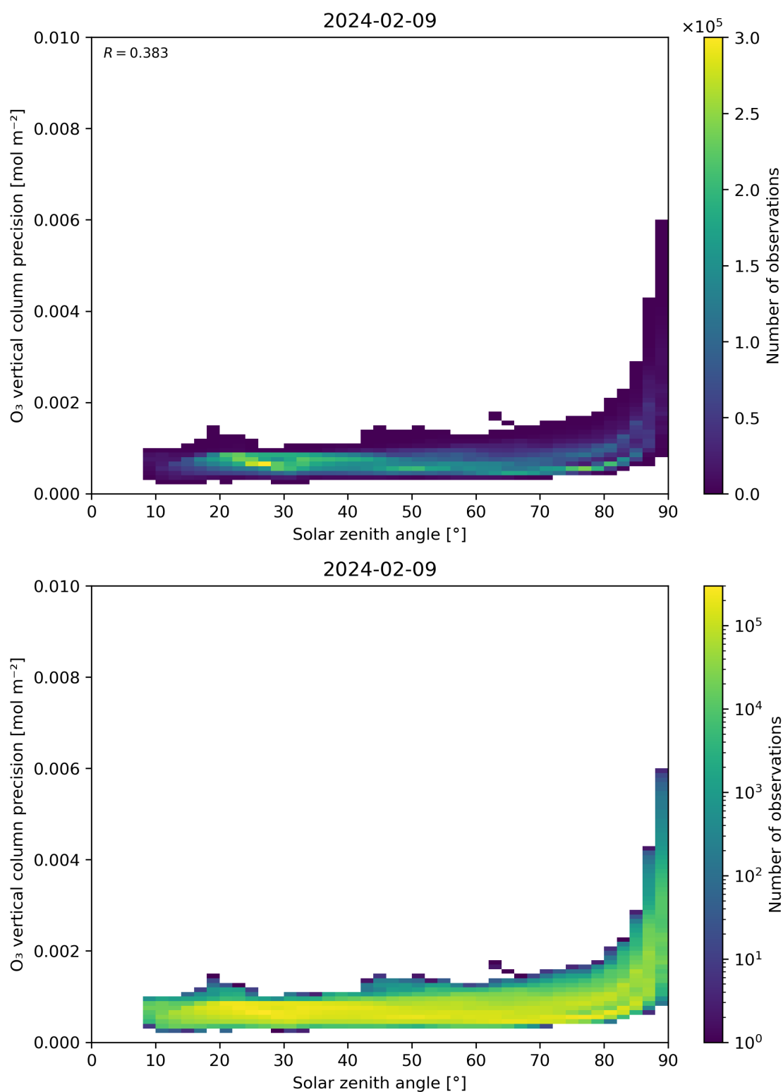
Figure 48: Scatter density plot of “Solar zenith angle” against “O 3 vertical column precision” for 2024-02-08 to 2024-02-10.
