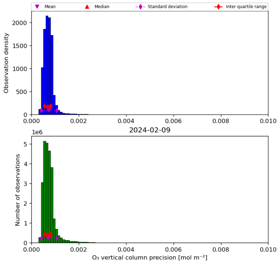
Figure 22: Histogram of “O 3 vertical column precision” for 2024-02-08 to 2024-02-10
