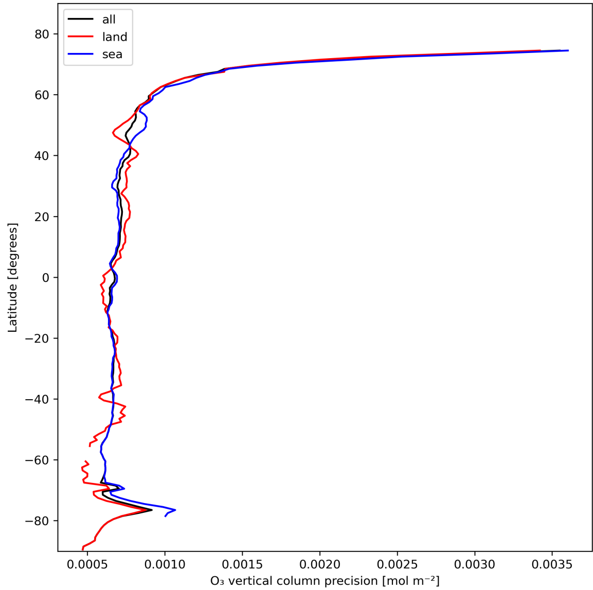
Figure 15: Zonal average of “O 3 vertical column precision” for 2024-02-08 to 2024-02-10.
