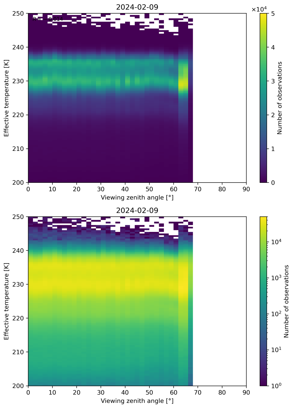
Figure 50: Scatter density plot of “Viewing zenith angle” against “Effective temperature” for 2024-02-08 to 2024-02-10.
