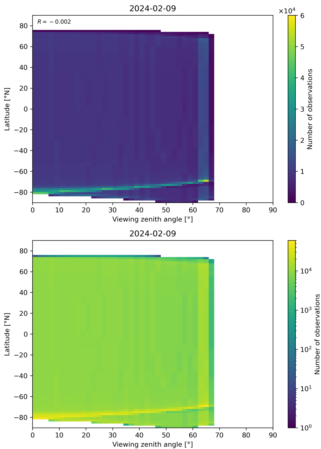
Figure 49: Scatter density plot of “Viewing zenith angle” against “Latitude” for 2024-02-08 to 2024-02-10.
