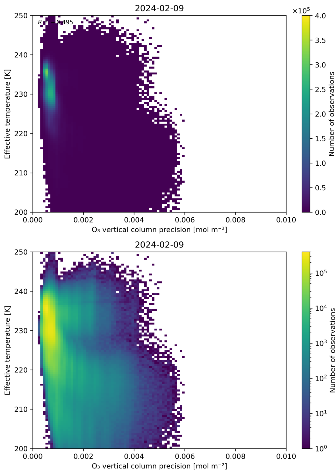
Figure 42: Scatter density plot of “O 3 vertical column precision” against “Effective temperature” for 2024-02-08 to 2024-02-10.
