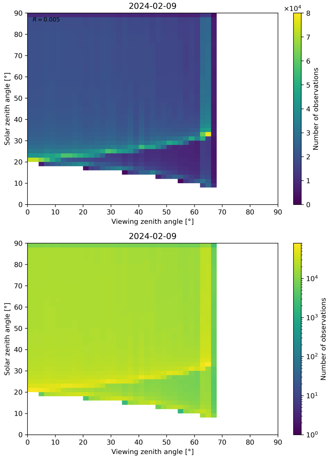
Figure 54: Scatter density plot of “Viewing zenith angle” against “Solar zenith angle” for 2024-02-08 to 2024-02-10.
