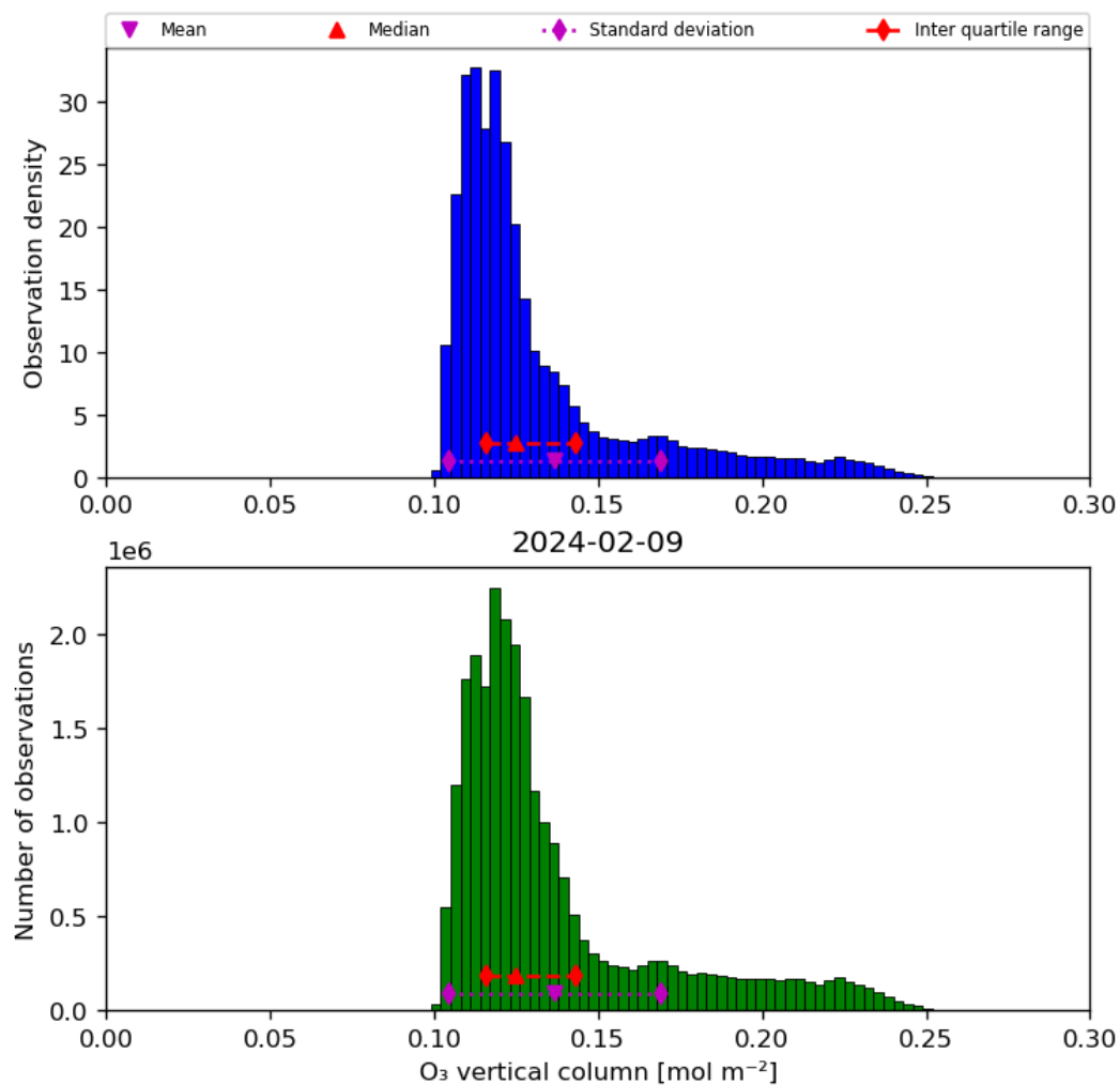
Figure 21: Histogram of “O 3 vertical column” for 2024-02-08 to 2024-02-10
