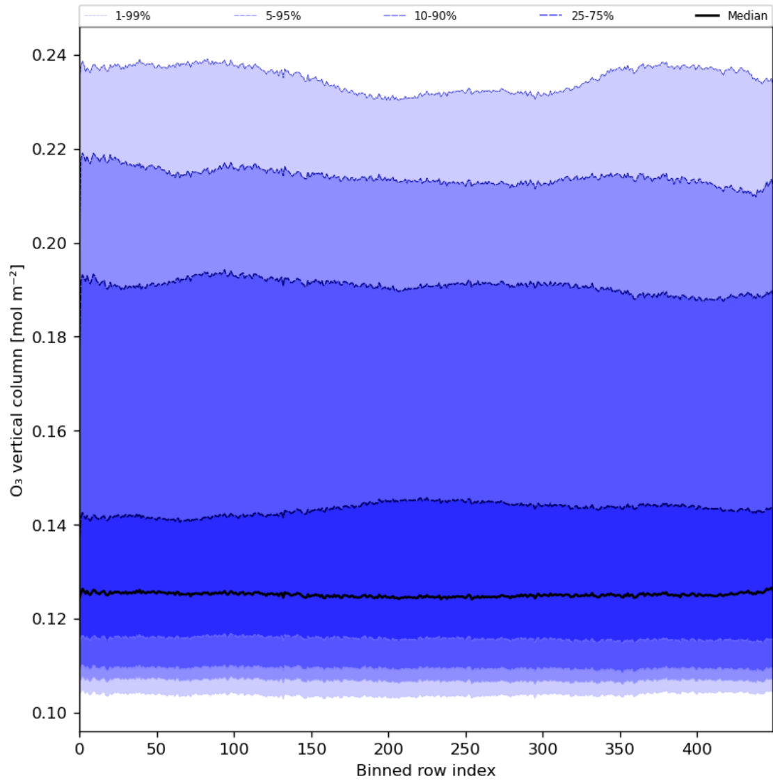
Figure 28: Along track statistics of “O 3 vertical column” for 2024-02-08 to 2024-02-10
