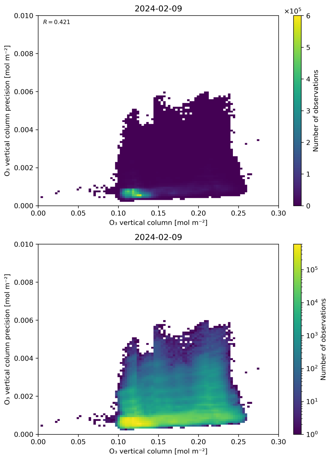
Figure 41: Scatter density plot of “O 3 vertical column” against “O 3 vertical column precision” for 2024-02-08 to 2024-02-10.
