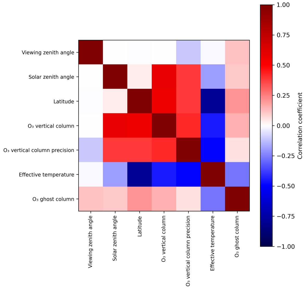
Figure 2: Map of correlation matrix for 2024-02-08 to 2024-02-10.
