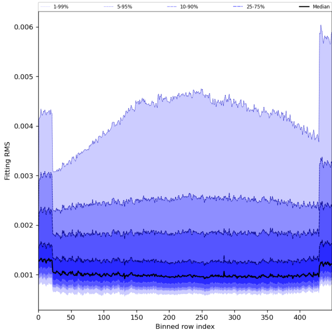
Figure 30: Along track statistics of “Fitting RMS” for 2024-02-08 to 2024-02-10
