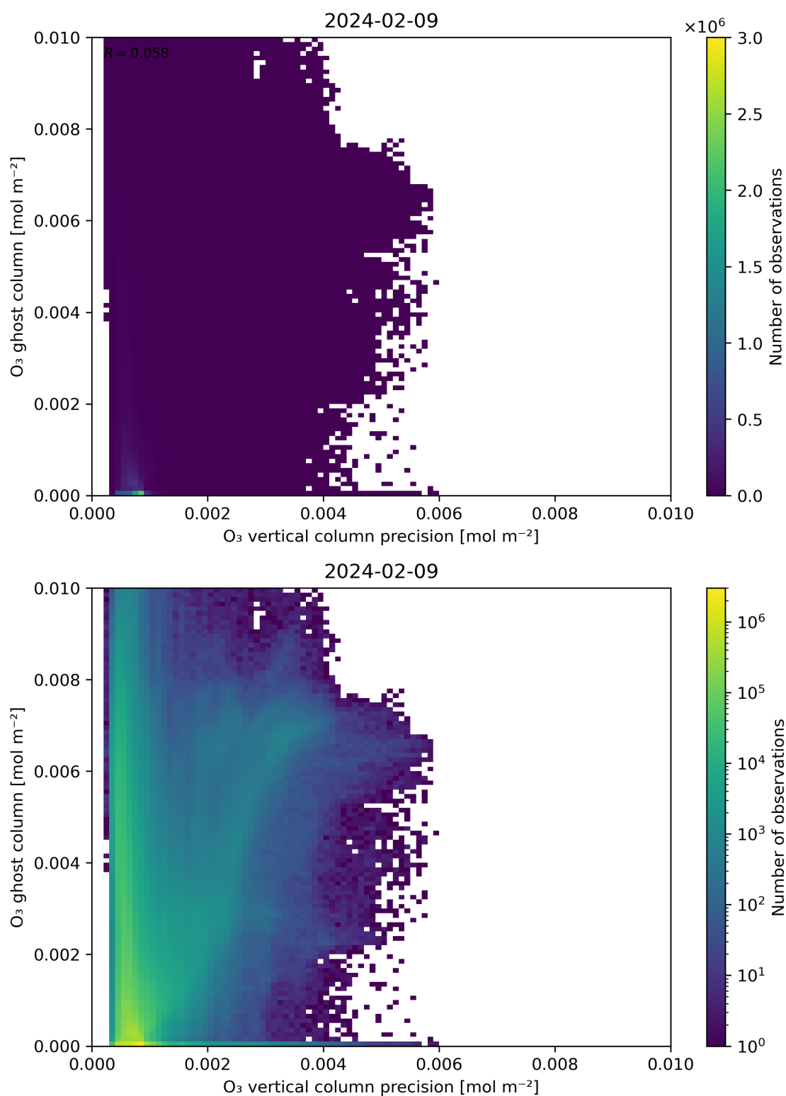
Figure 43: Scatter density plot of “ \text{O}_3 vertical column precision” against “ \text{O}_3 ghost column” for 2024-02-08 to 2024-02-10.
