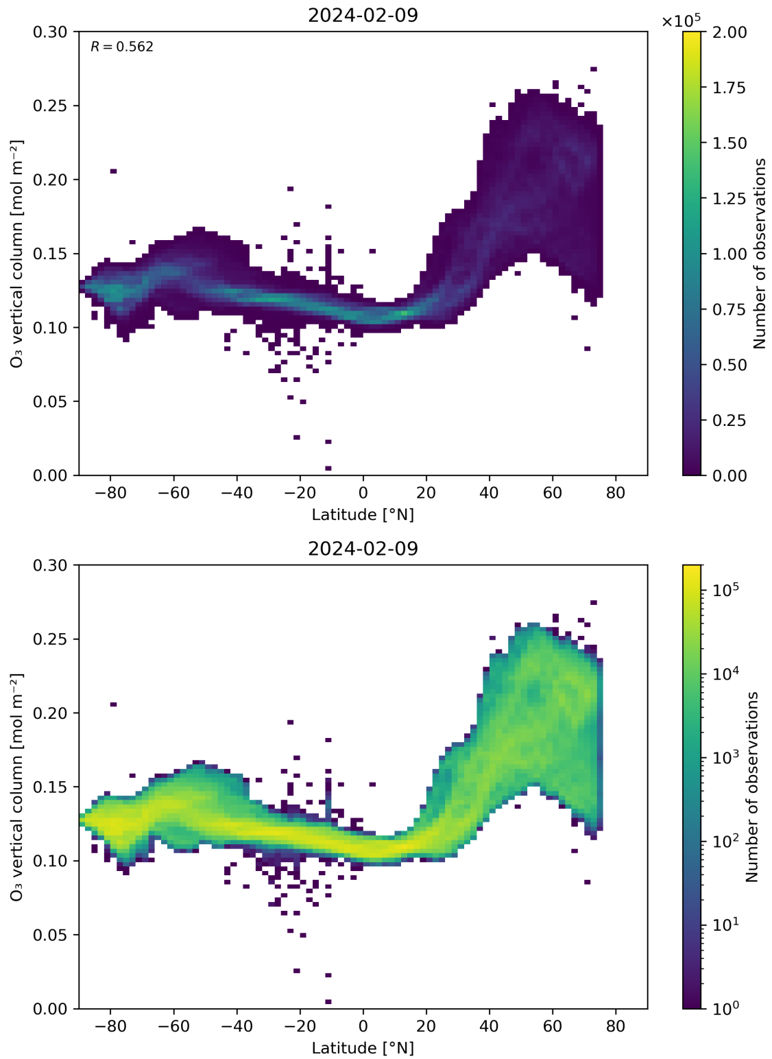
Figure 36: Scatter density plot of “Latitude” against “O 3 vertical column” for 2024-02-08 to 2024-02-10.
