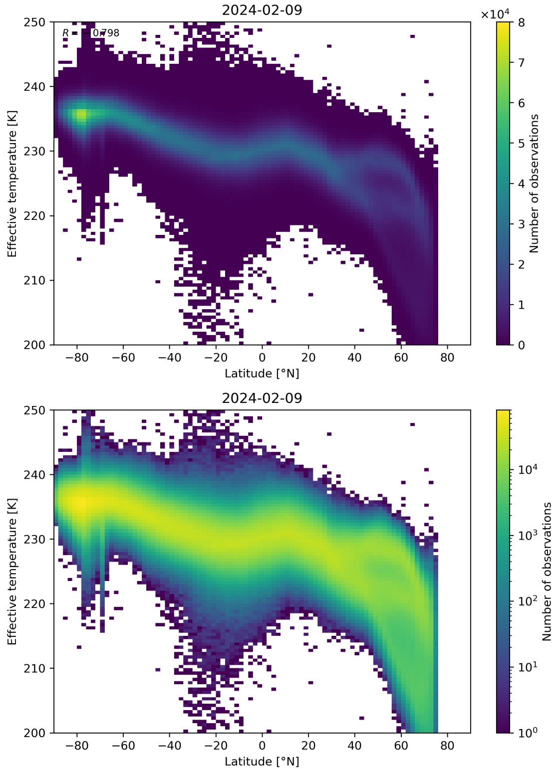
Figure 34: Scatter density plot of “Latitude” against “Effective temperature” for 2024-02-08 to 2024-02-10.
