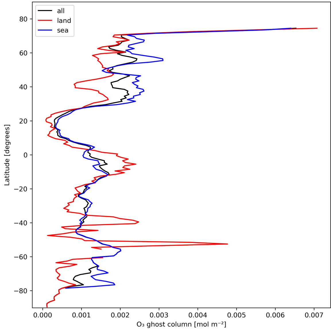
Figure 18: Zonal average of "O 3 ghost column" for 2024-02-08 to 2024-02-10.
