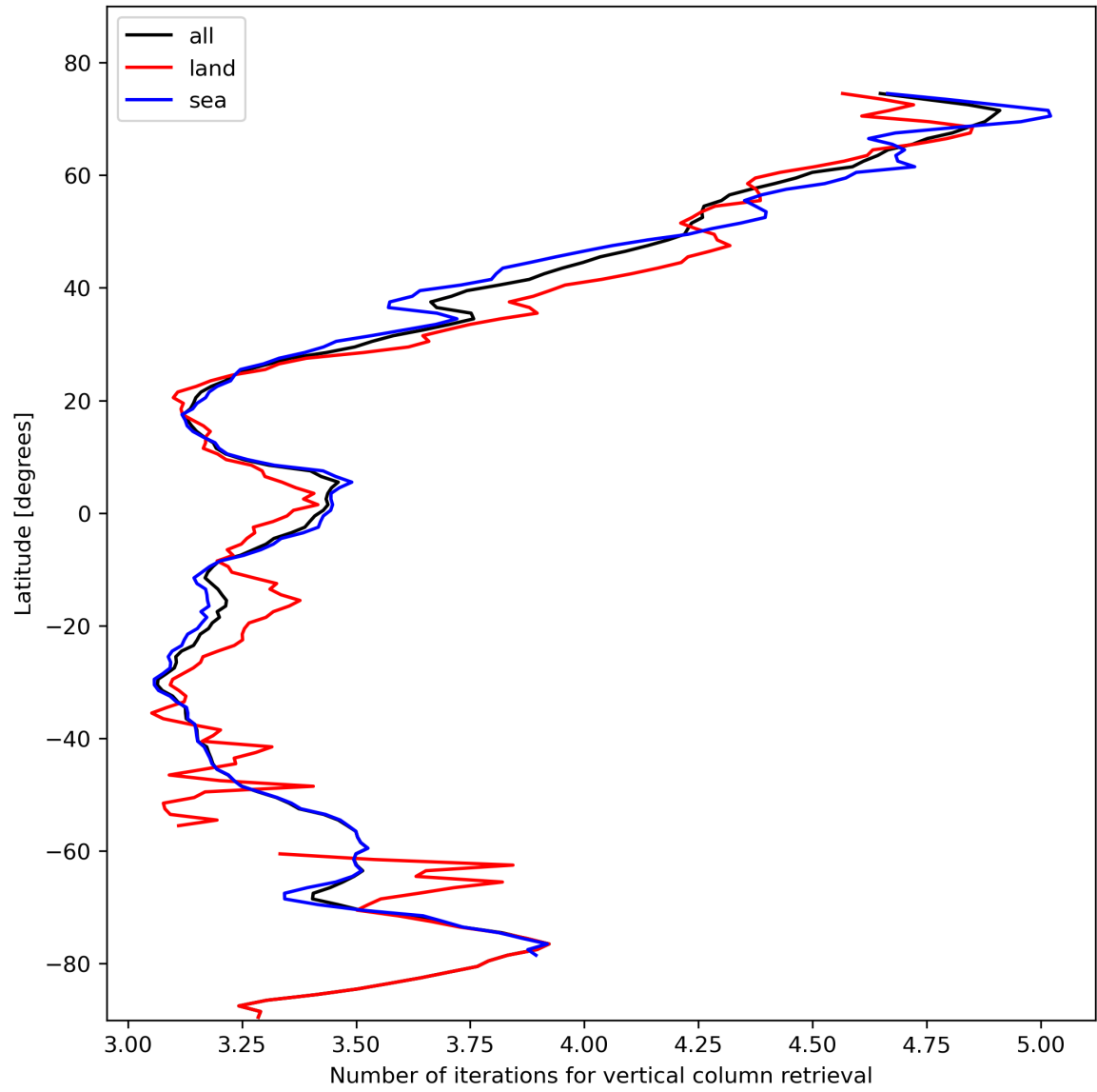
Figure 19: Zonal average of “Number of iterations for vertical column retrieval” for 2024-02-08 to 2024-02-10.
