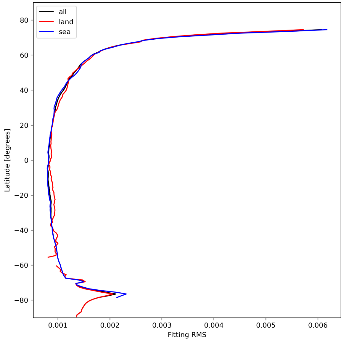
Figure 16: Zonal average of “Fitting RMS” for 2024-02-08 to 2024-02-10.
