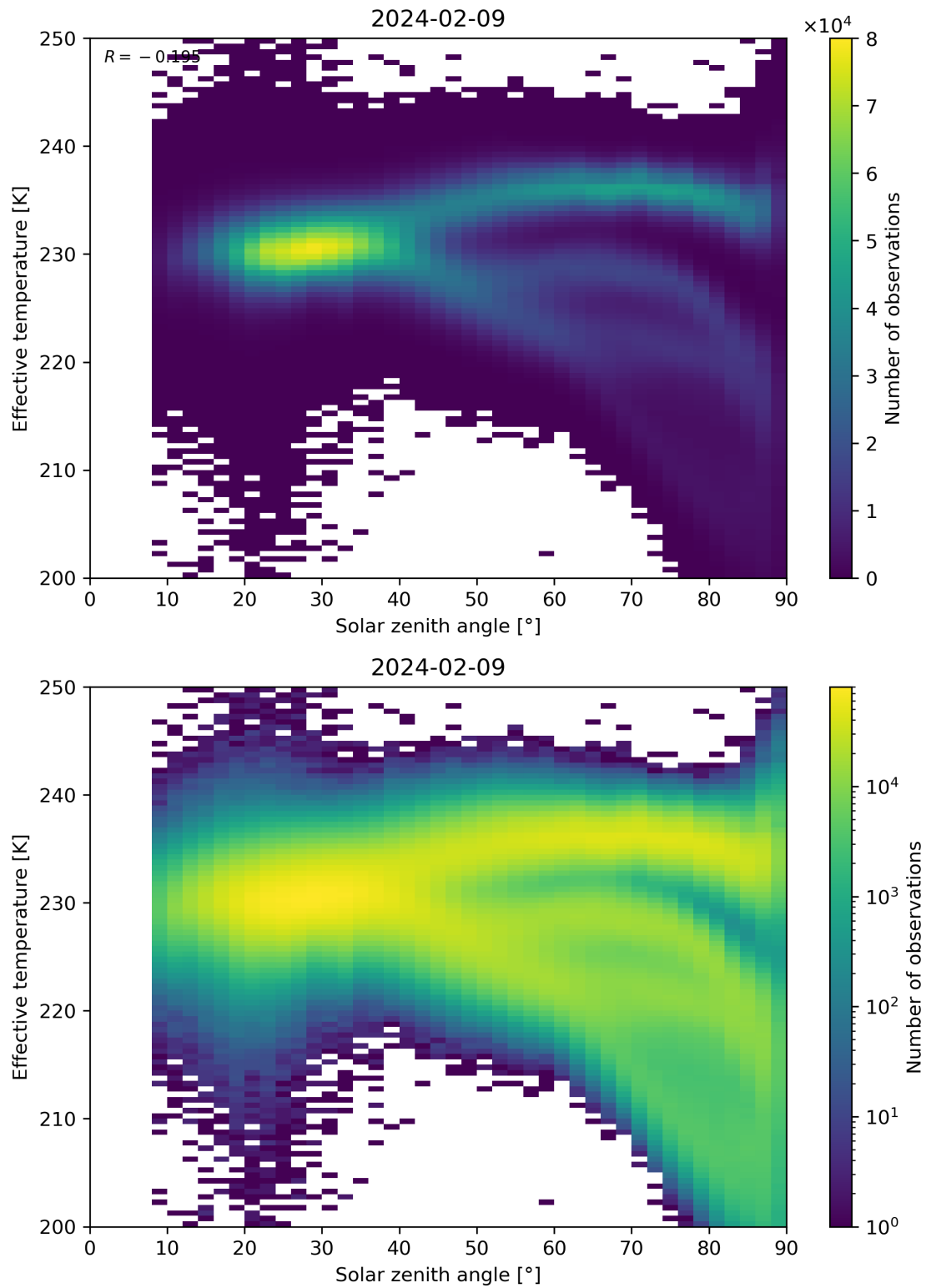
Figure 45: Scatter density plot of “Solar zenith angle” against “Effective temperature” for 2024-02-08 to 2024-02-10.
