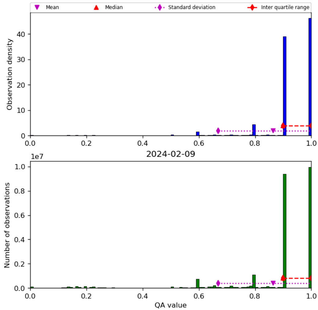
Figure 20: Histogram of “QA value” for 2024-02-08 to 2024-02-10
