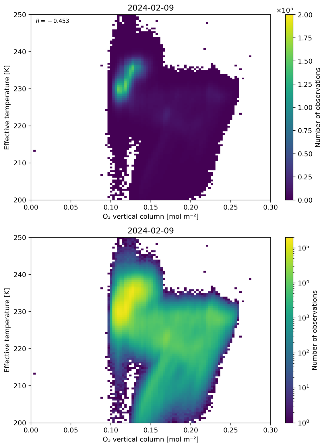
Figure 39: Scatter density plot of “O 3 vertical column” against “Effective temperature” for 2024-02-08 to 2024-02-10.
