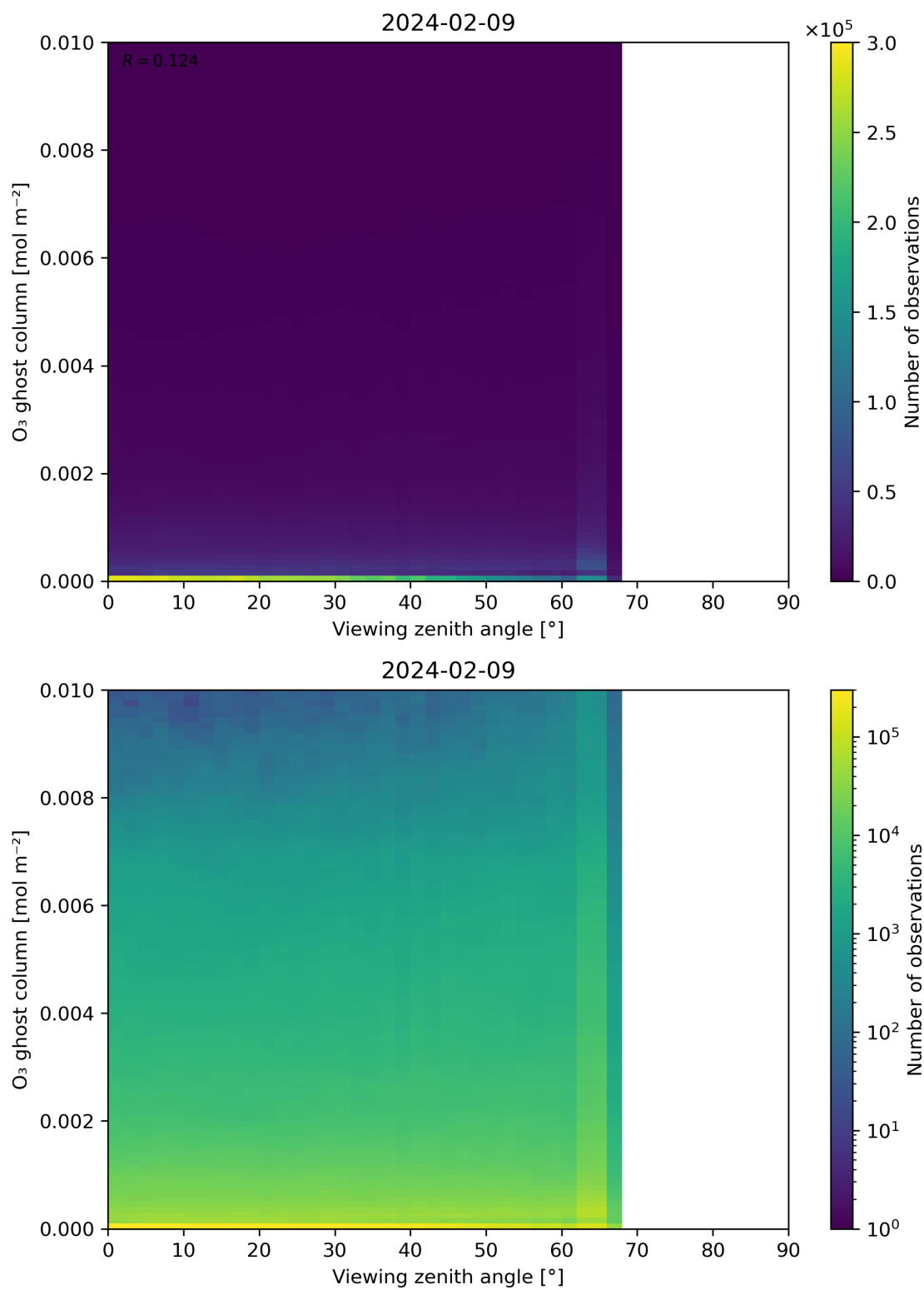
Figure 51: Scatter density plot of “Viewing zenith angle” against “O 3 ghost column” for 2024-02-08 to 2024-02-10.
