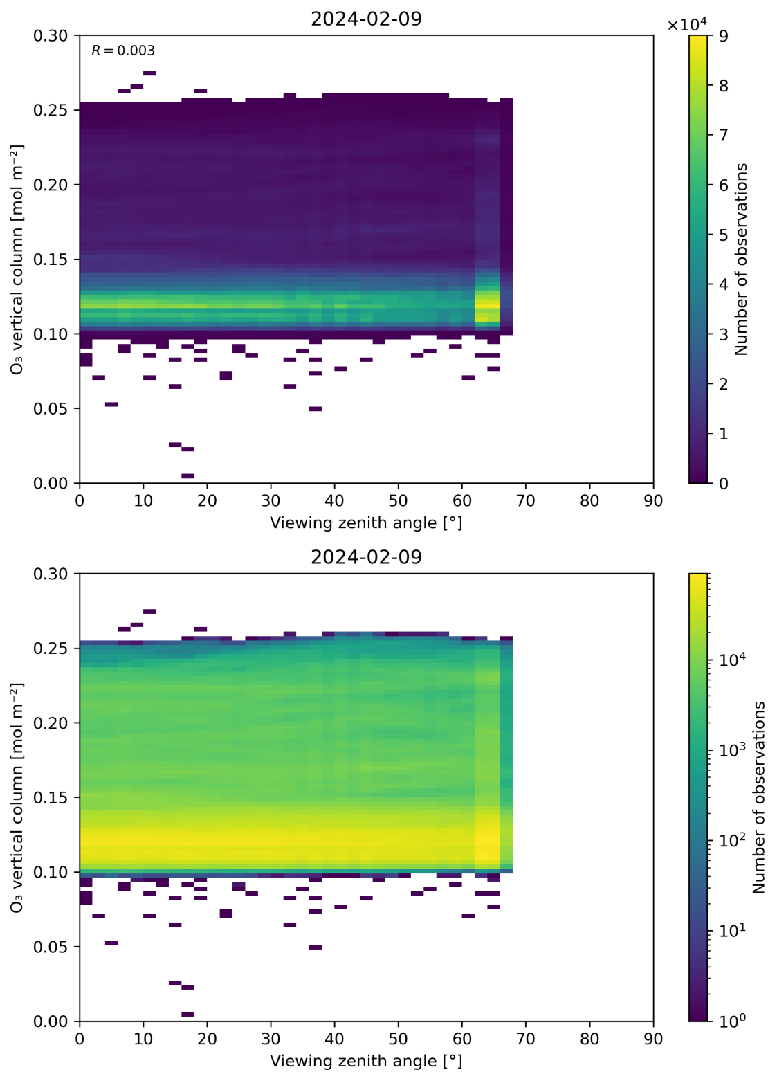
Figure 52: Scatter density plot of “Viewing zenith angle” against “O 3 vertical column” for 2024-02-08 to 2024-02-10.
