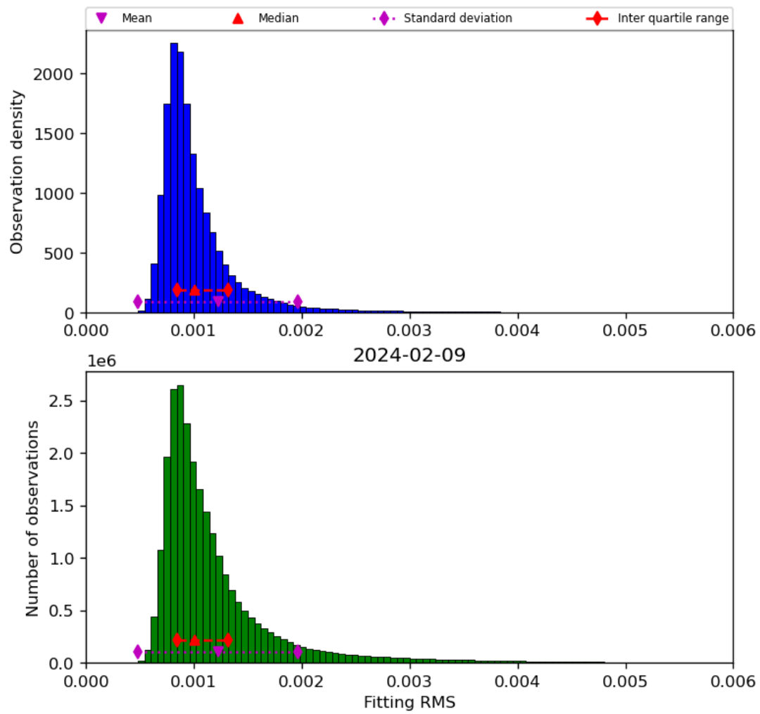
Figure 23: Histogram of “Fitting RMS” for 2024-02-08 to 2024-02-10
