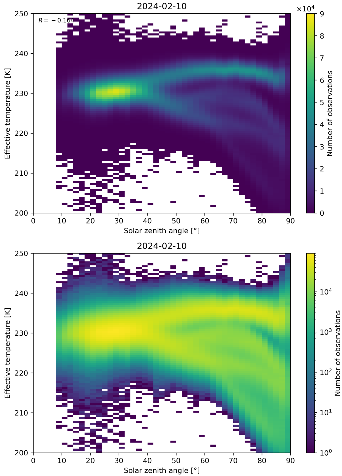
Figure 45: Scatter density plot of “Solar zenith angle” against “Effective temperature” for 2024-02-09 to 2024-02-11.
