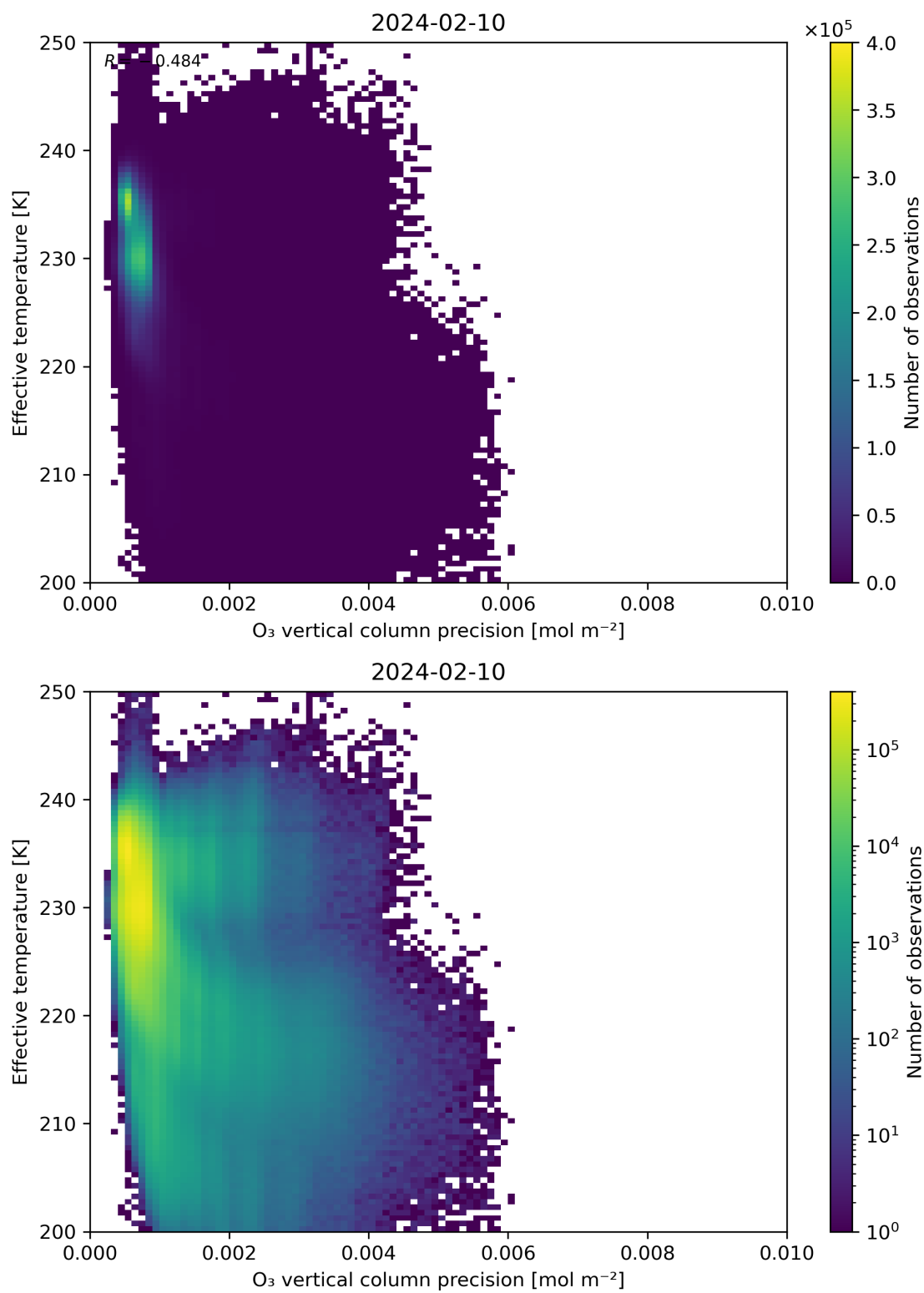
Figure 42: Scatter density plot of “O 3 vertical column precision” against “Effective temperature” for 2024-02-09 to 2024-02-11.
