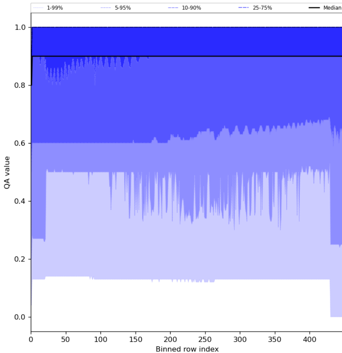
Figure 27: Along track statistics of “QA value” for 2024-02-09 to 2024-02-11
