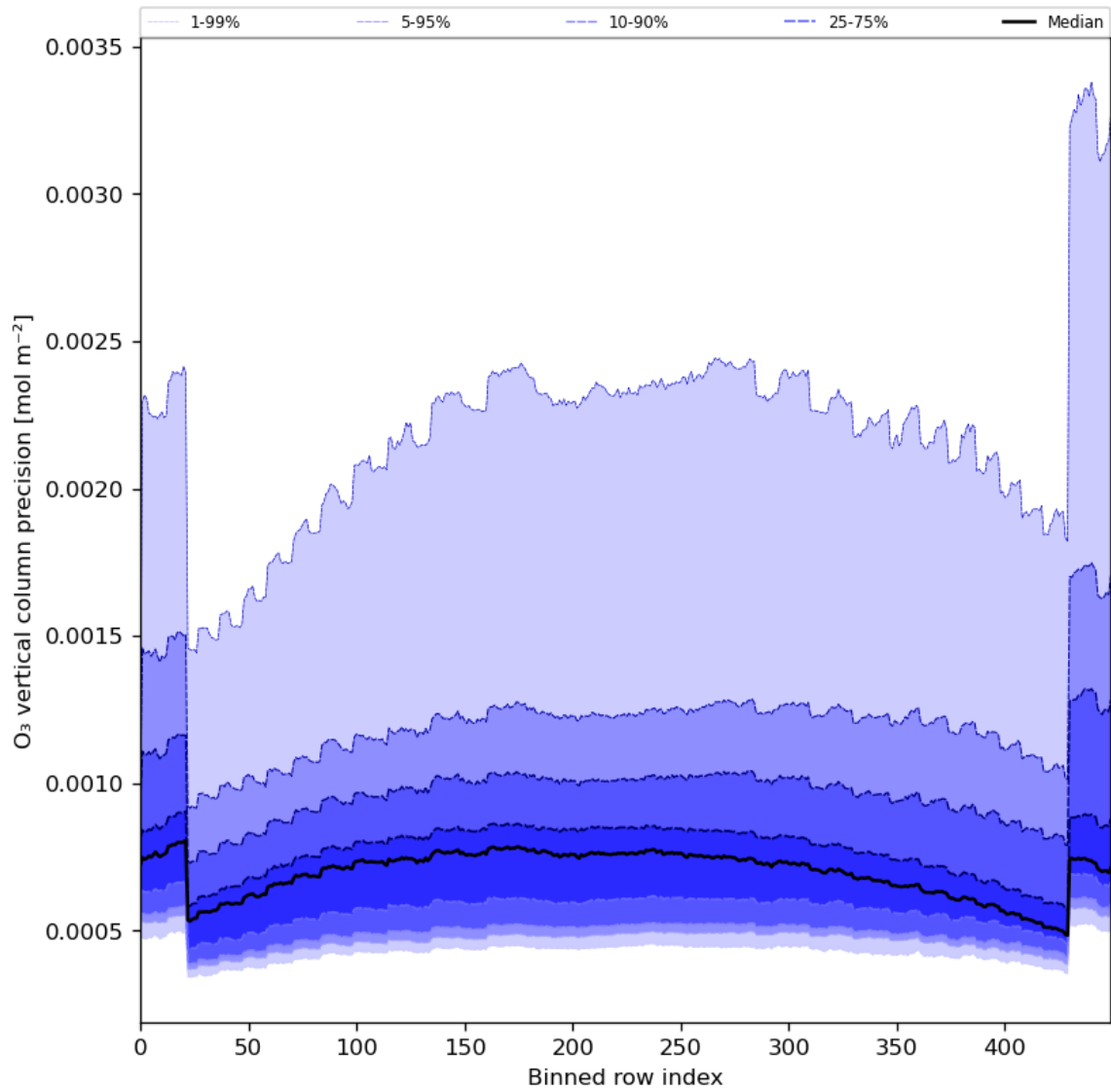
Figure 29: Along track statistics of “O 3 vertical column precision” for 2024-02-09 to 2024-02-11
