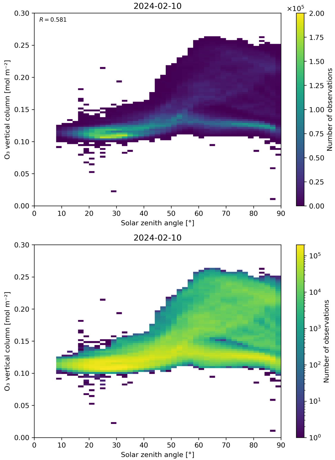
Figure 47: Scatter density plot of “Solar zenith angle” against “O 3 vertical column” for 2024-02-09 to 2024-02-11.
