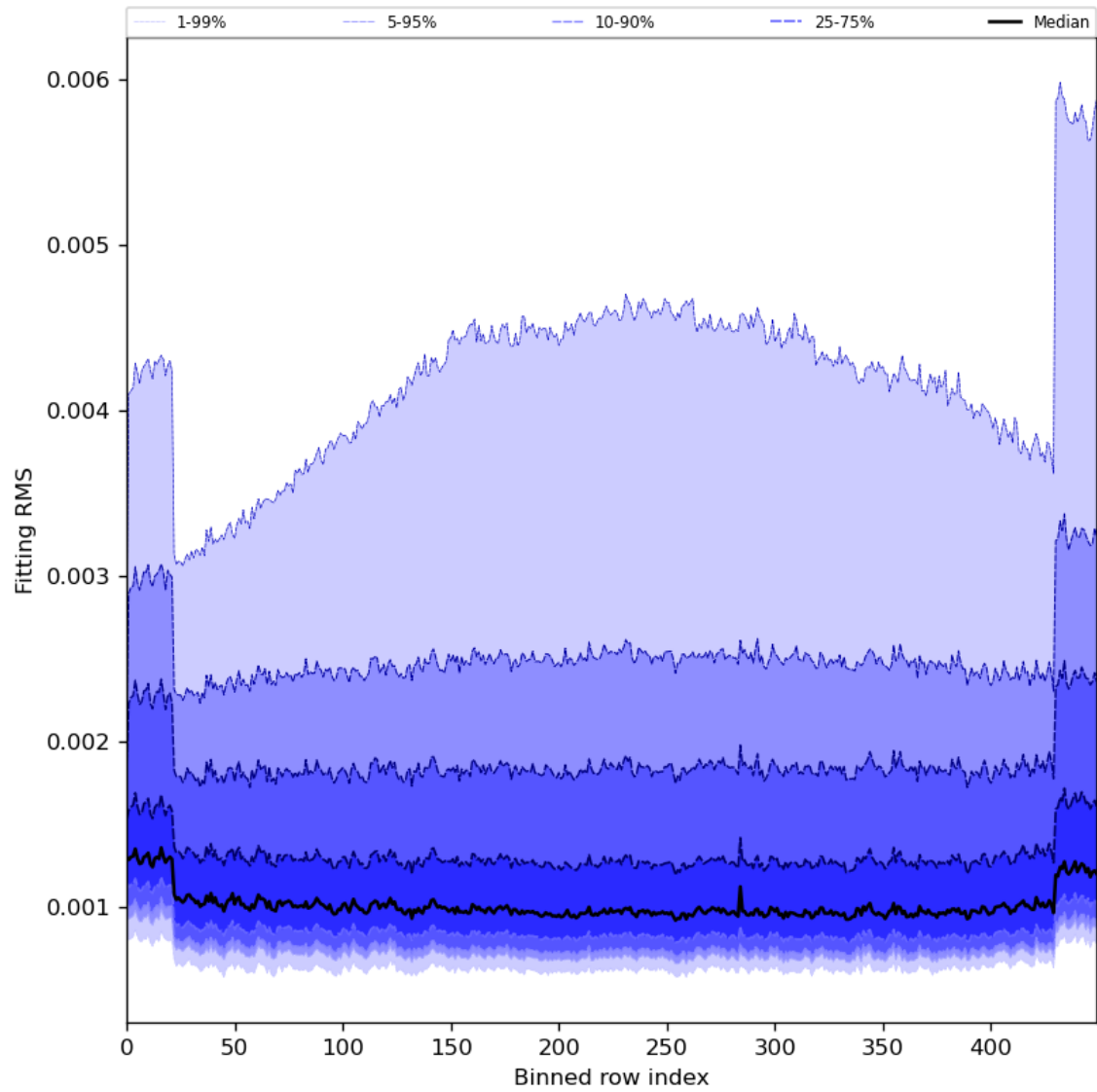
Figure 30: Along track statistics of “Fitting RMS” for 2024-02-09 to 2024-02-11
