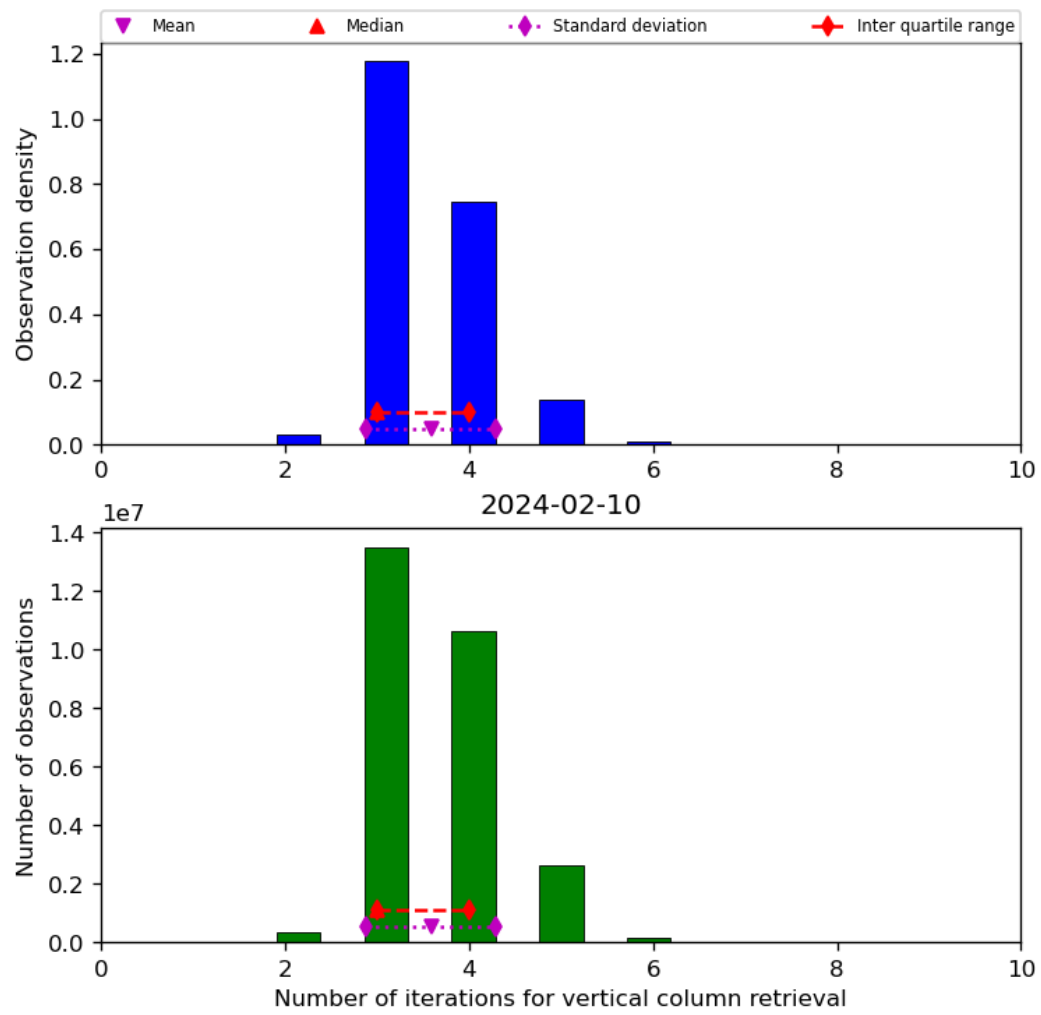
Figure 26: Histogram of “Number of iterations for vertical column retrieval” for 2024-02-09 to 2024-02-11
