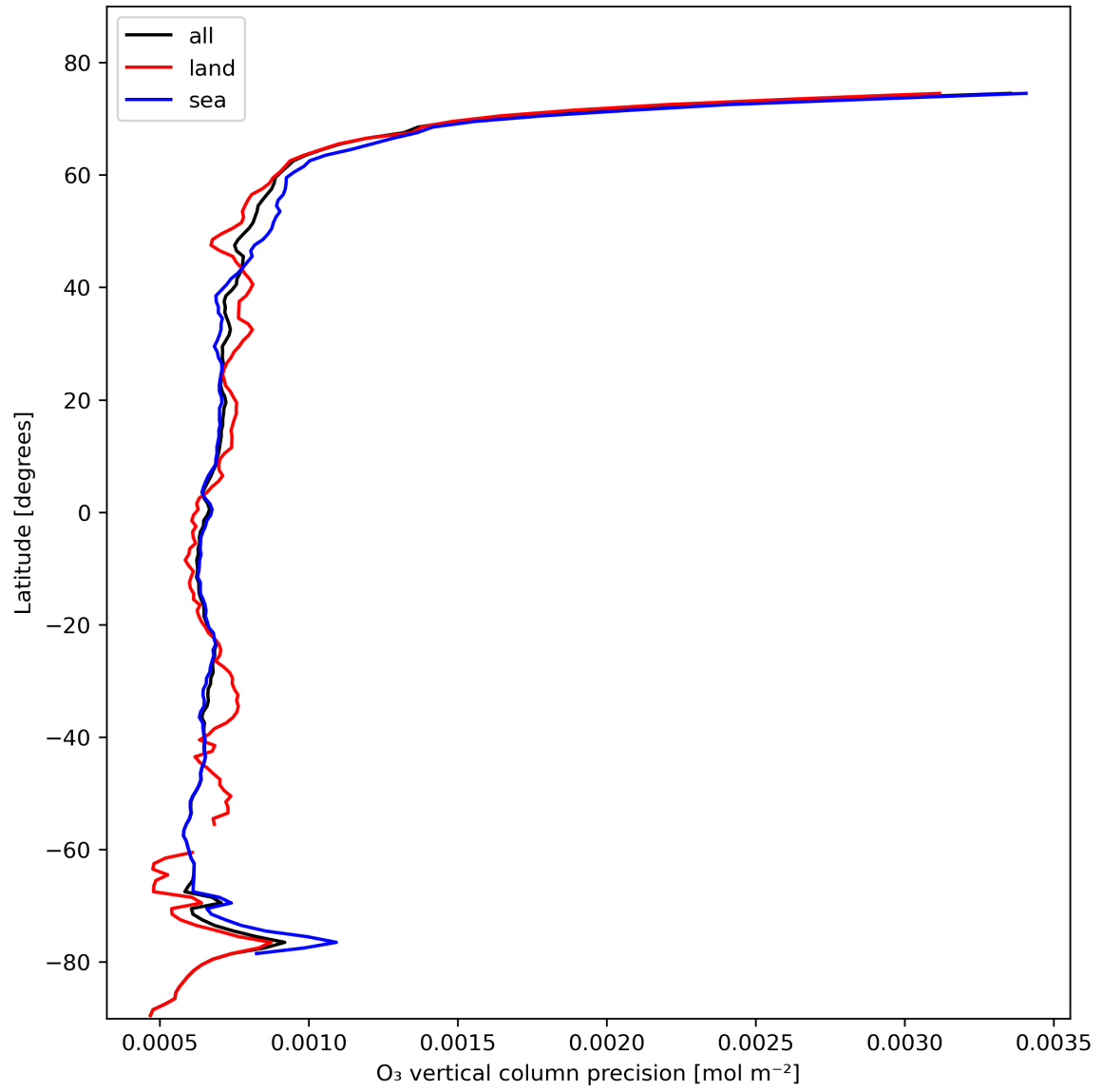
Figure 15: Zonal average of “O 3 vertical column precision” for 2024-02-09 to 2024-02-11.
