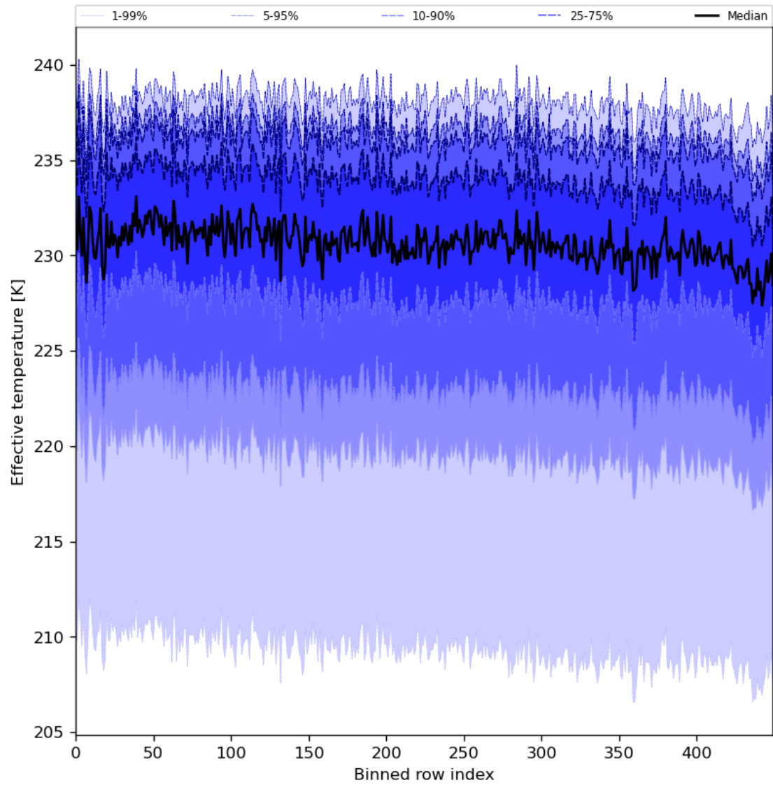
Figure 31: Along track statistics of “Effective temperature” for 2024-02-09 to 2024-02-11
