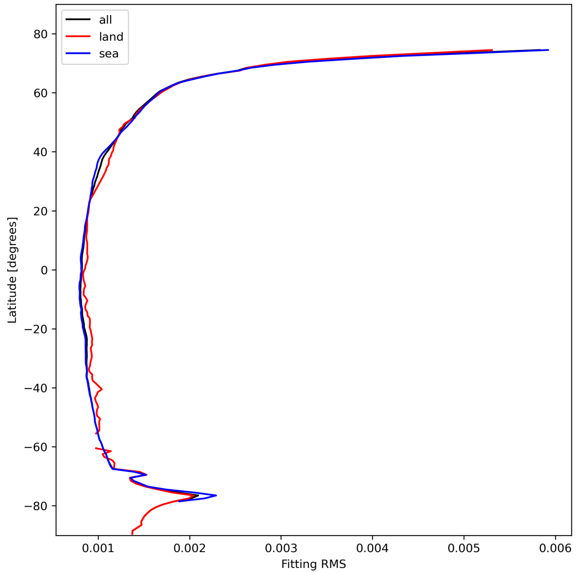
Figure 16: Zonal average of “Fitting RMS” for 2024-02-09 to 2024-02-11.
