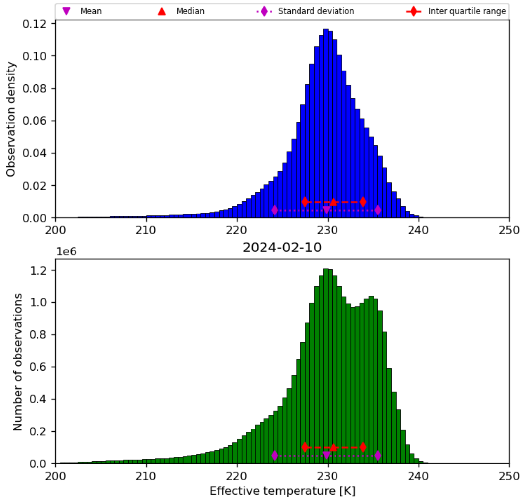
Figure 24: Histogram of “Effective temperature” for 2024-02-09 to 2024-02-11
