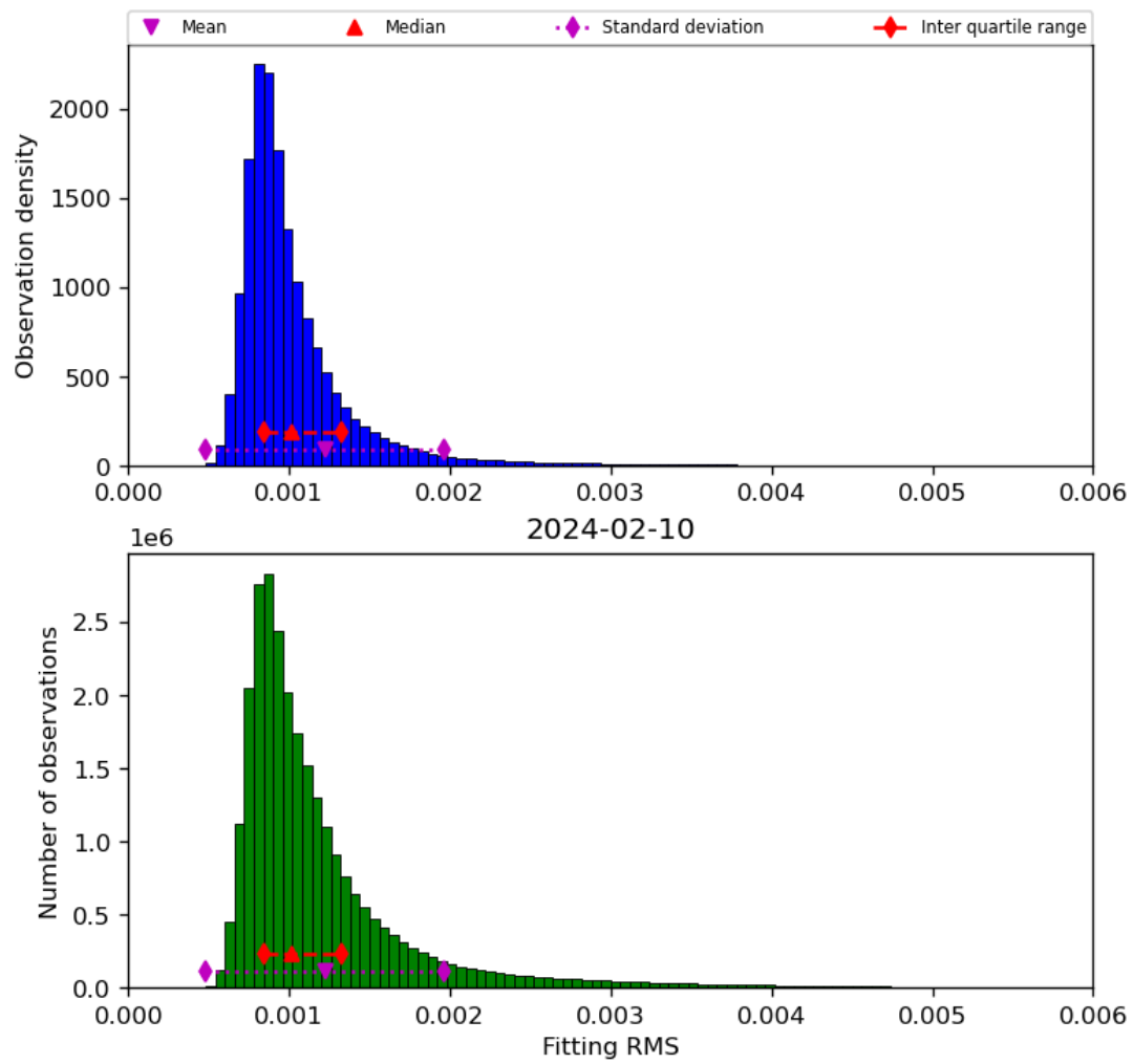
Figure 23: Histogram of “Fitting RMS” for 2024-02-09 to 2024-02-11
