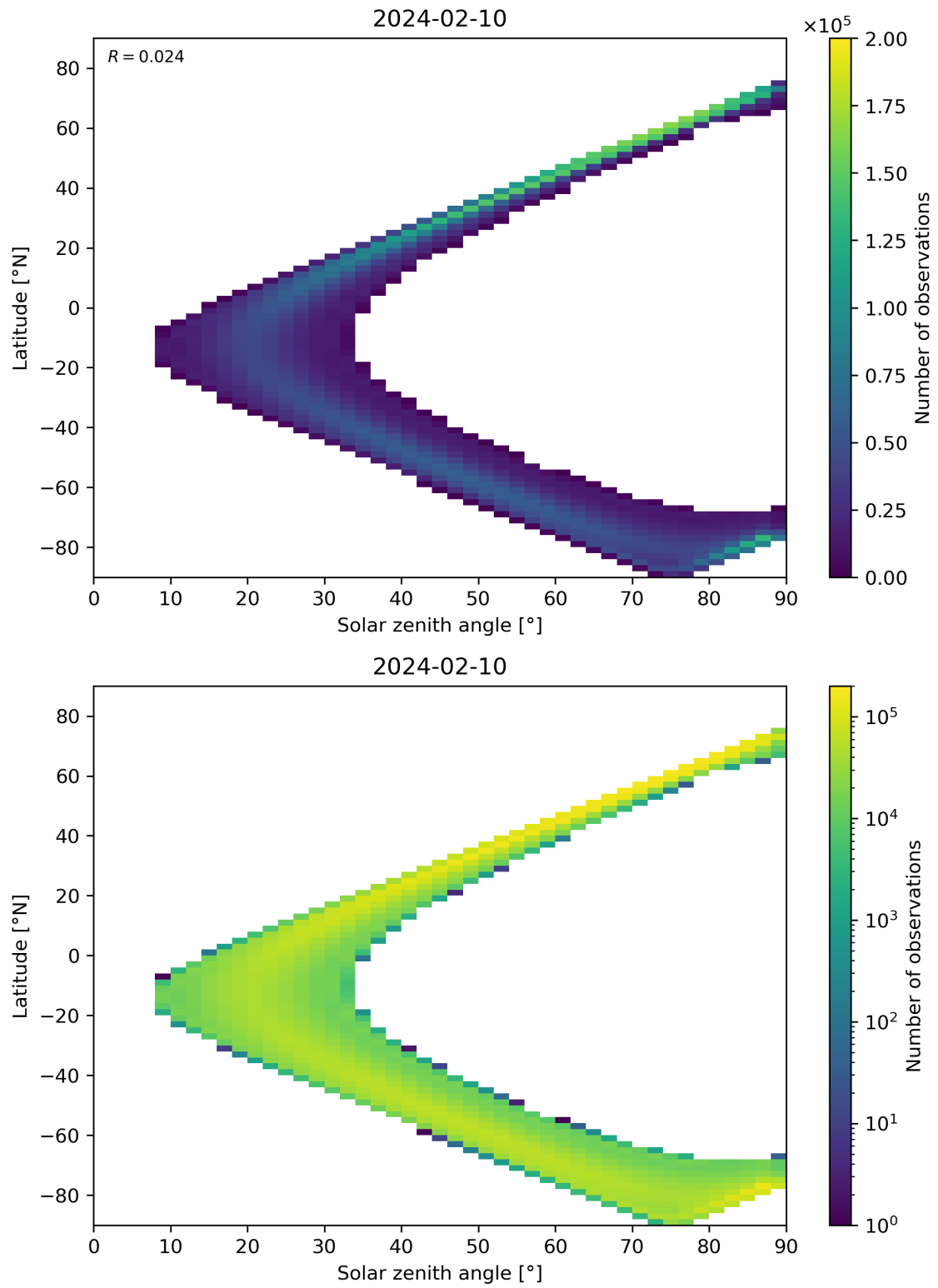
Figure 44: Scatter density plot of “Solar zenith angle” against “Latitude” for 2024-02-09 to 2024-02-11.
