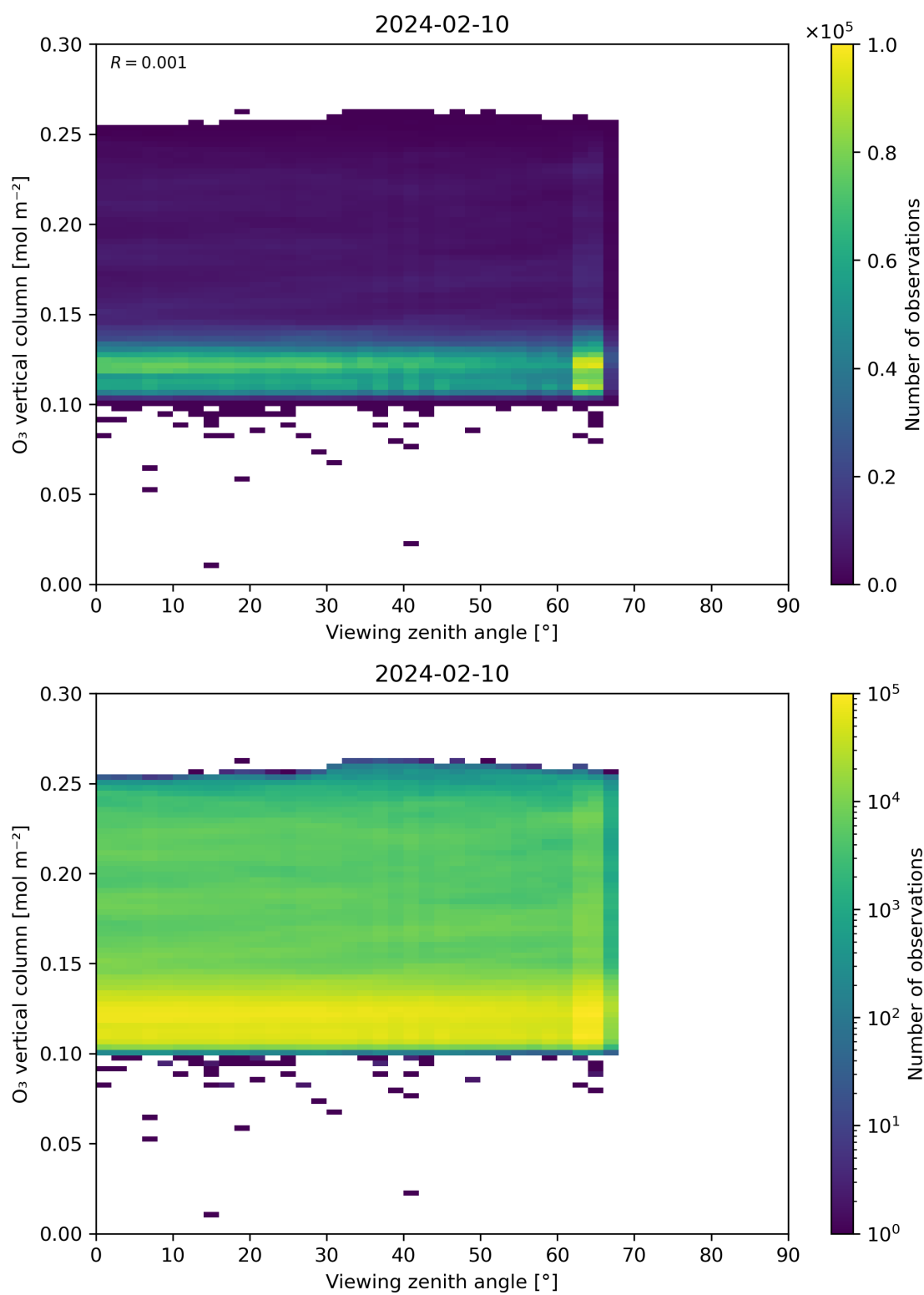
Figure 52: Scatter density plot of “Viewing zenith angle” against “O 3 vertical column” for 2024-02-09 to 2024-02-11.
