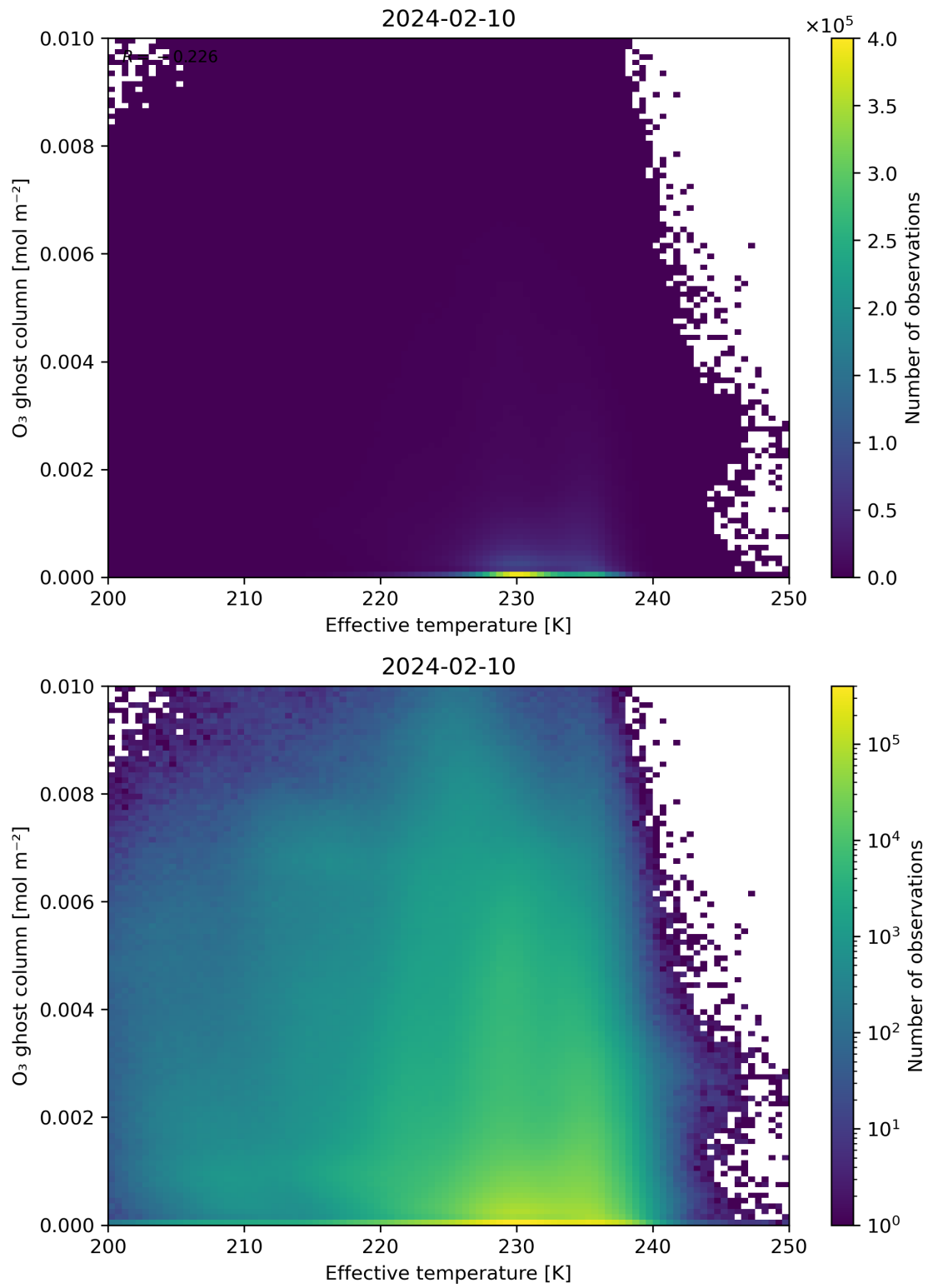
Figure 38: Scatter density plot of “Effective temperature” against “O 3 ghost column” for 2024-02-09 to 2024-02-11.
