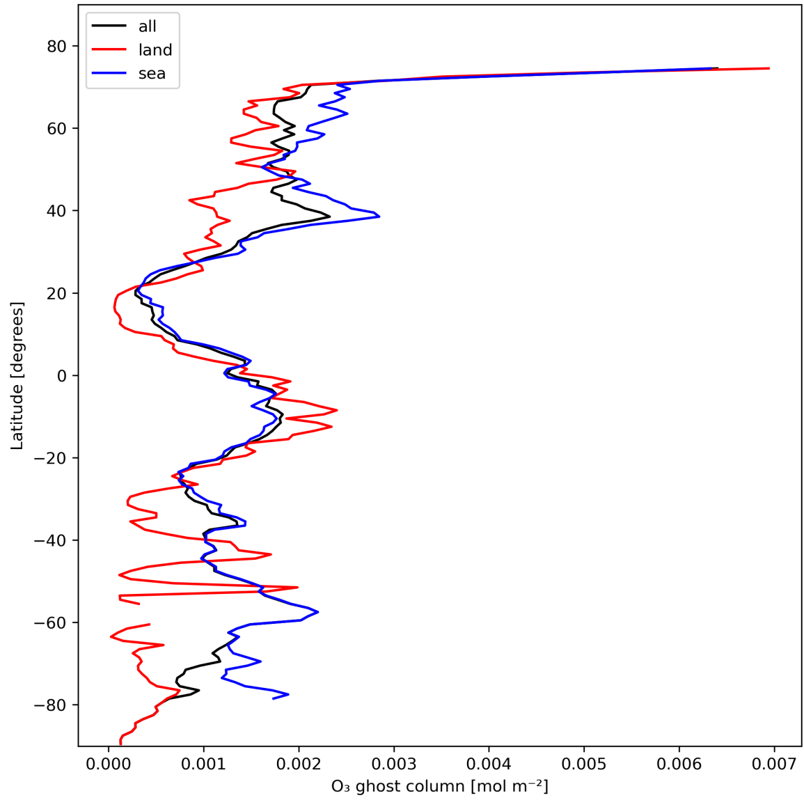
Figure 18: Zonal average of “O 3 ghost column” for 2024-02-09 to 2024-02-11.
