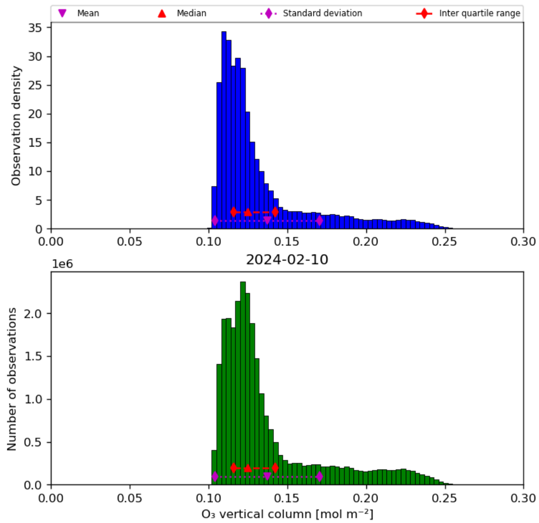
Figure 21: Histogram of “O 3 vertical column” for 2024-02-09 to 2024-02-11
