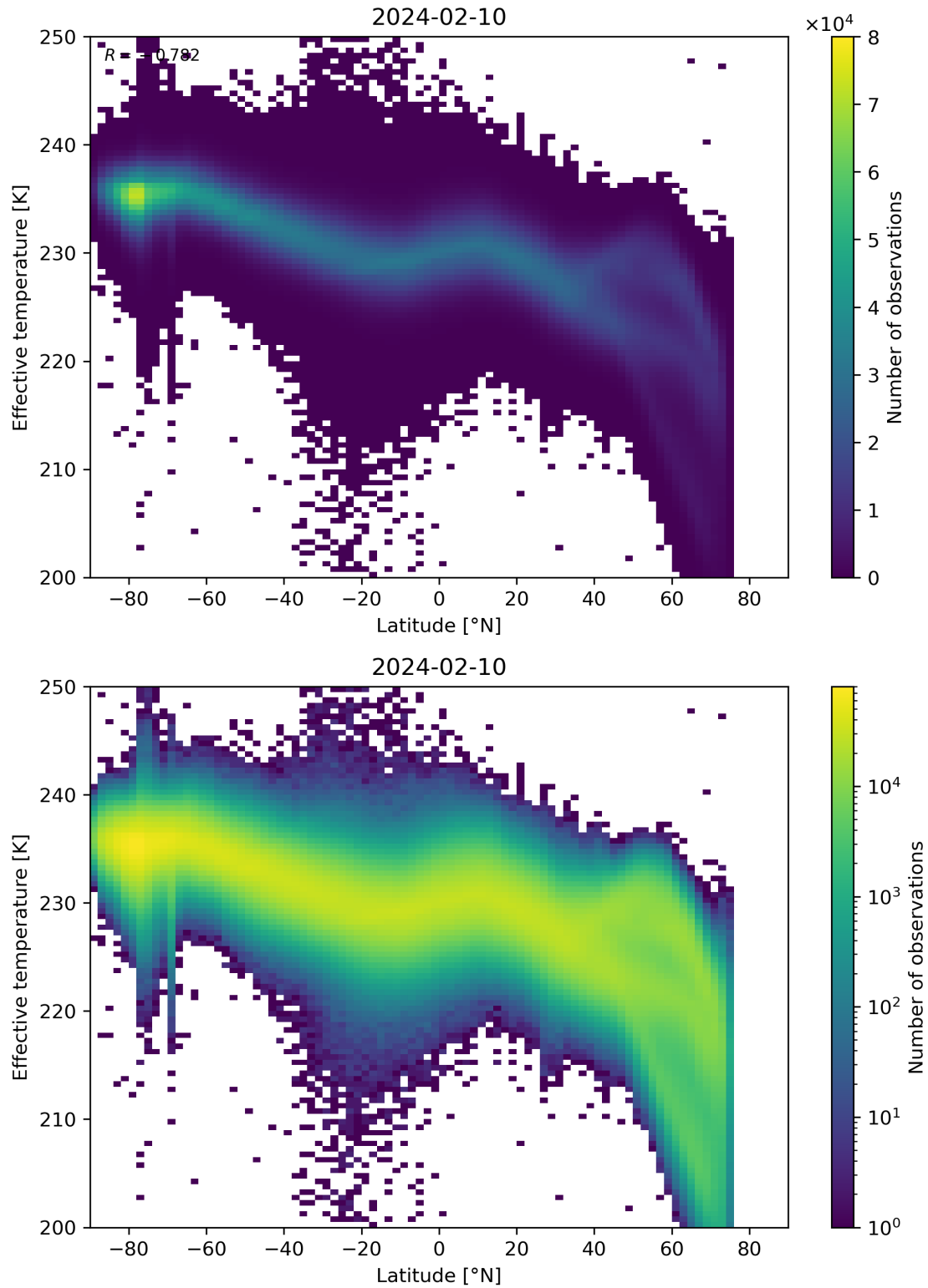
Figure 34: Scatter density plot of “Latitude” against “Effective temperature” for 2024-02-09 to 2024-02-11.
