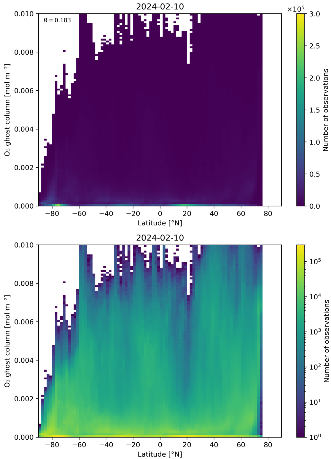
Figure 35: Scatter density plot of “Latitude” against “O 3 ghost column” for 2024-02-09 to 2024-02-11.
