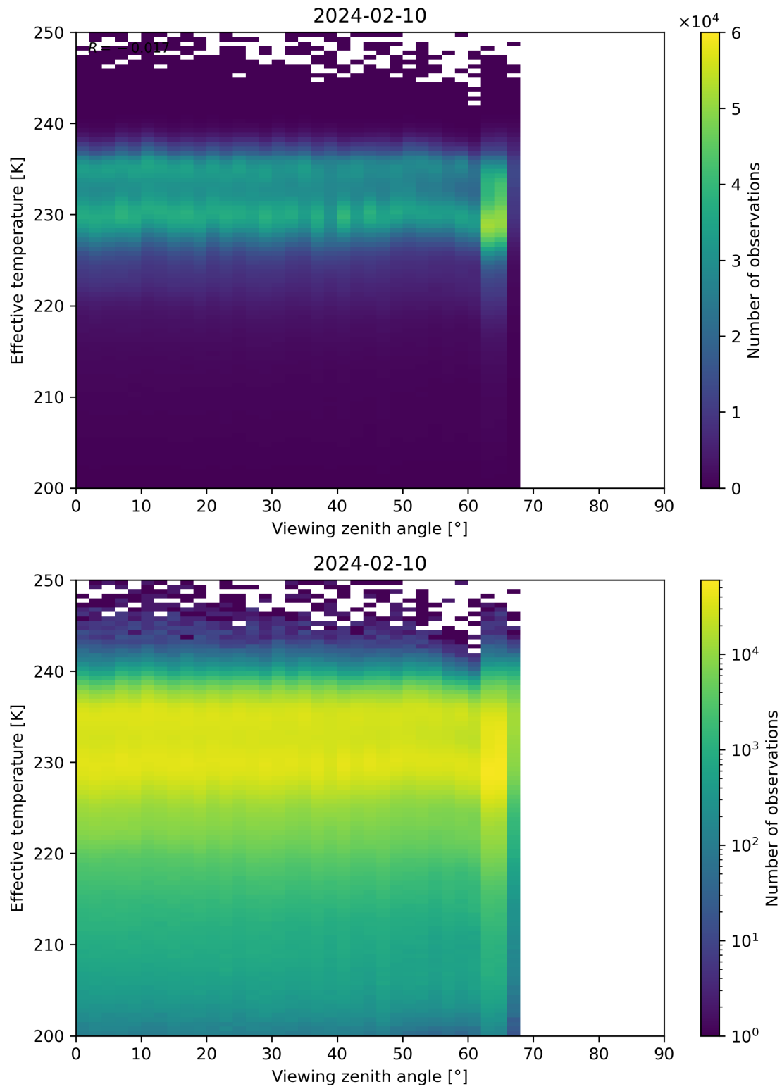
Figure 50: Scatter density plot of “Viewing zenith angle” against “Effective temperature” for 2024-02-09 to 2024-02-11.
