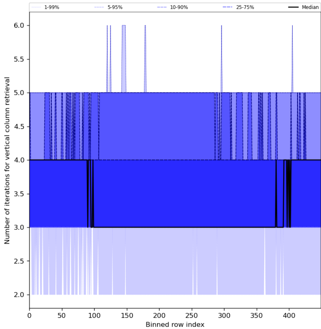
Figure 33: Along track statistics of “Number of iterations for vertical column retrieval” for 2024-02-09 to 2024-02-11
