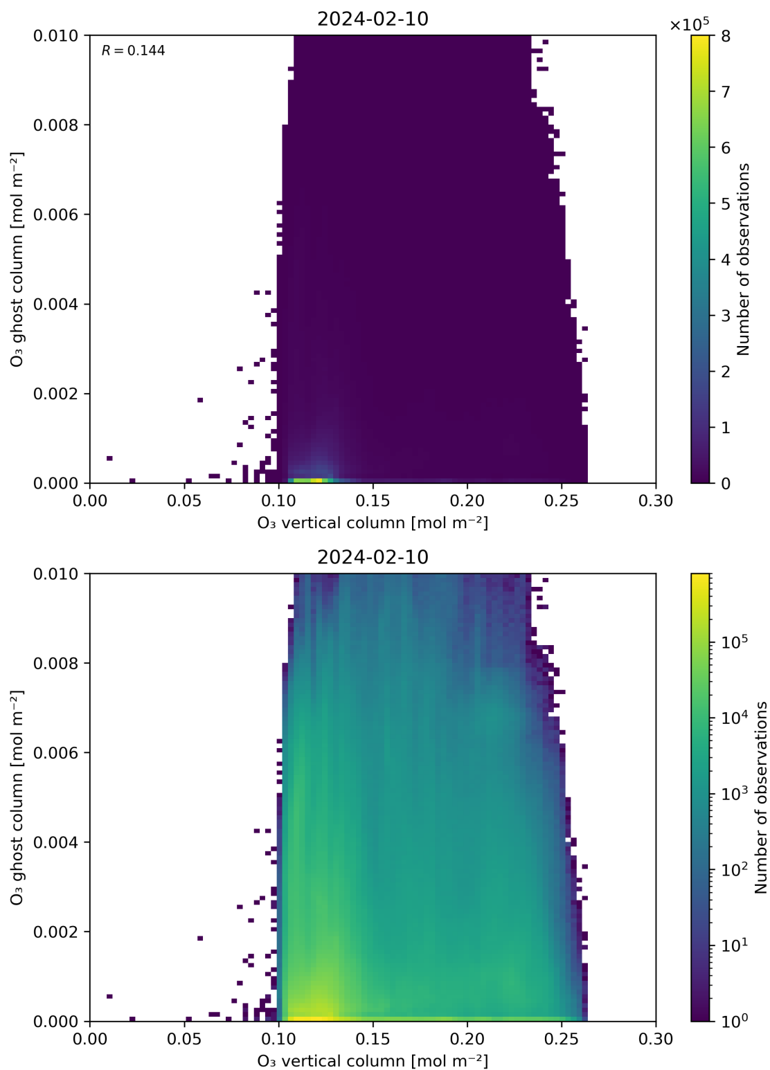
Figure 40: Scatter density plot of “O 3 vertical column” against “O 3 ghost column” for 2024-02-09 to 2024-02-11.
