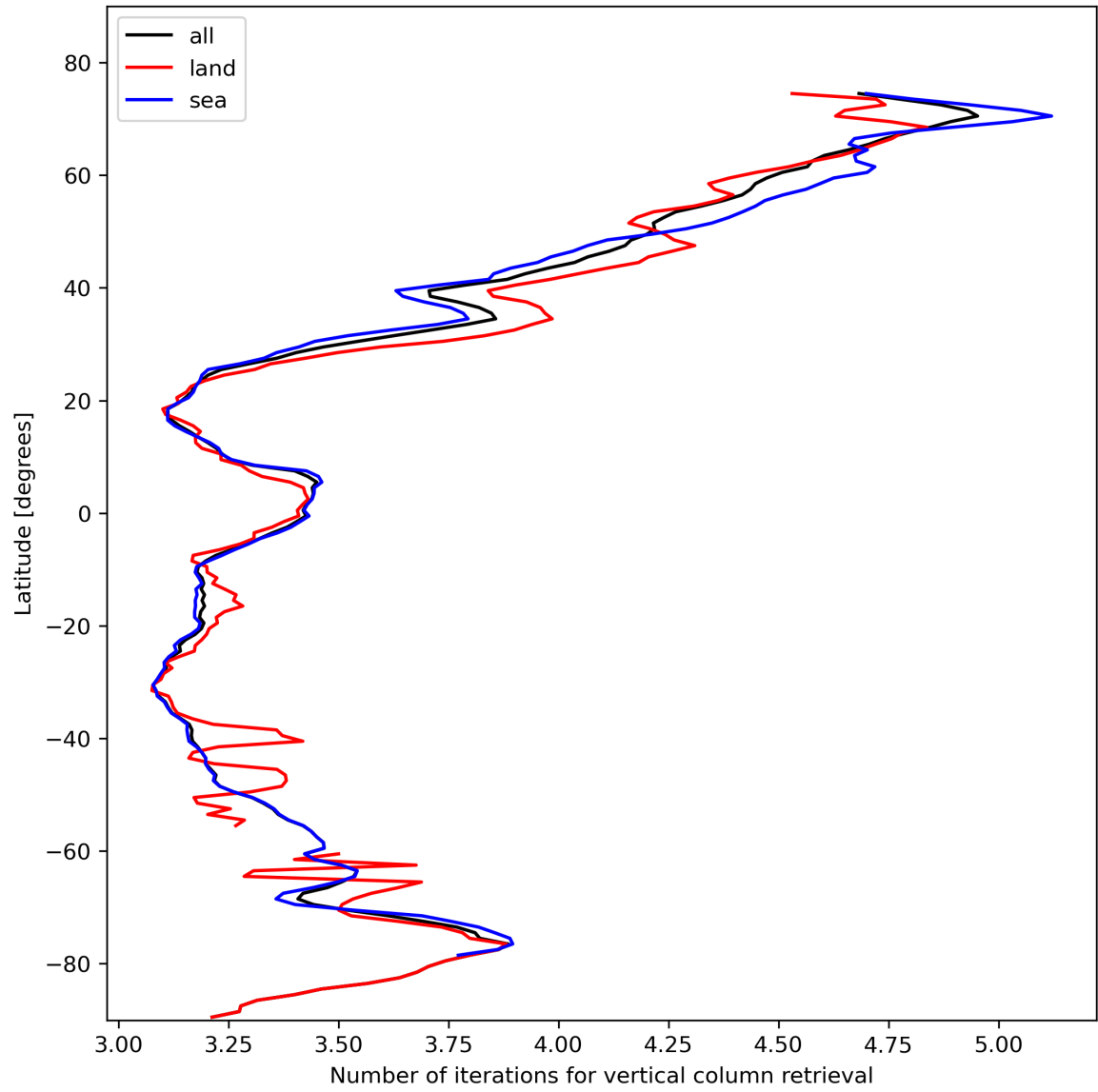
Figure 19: Zonal average of “Number of iterations for vertical column retrieval” for 2024-02-09 to 2024-02-11.
