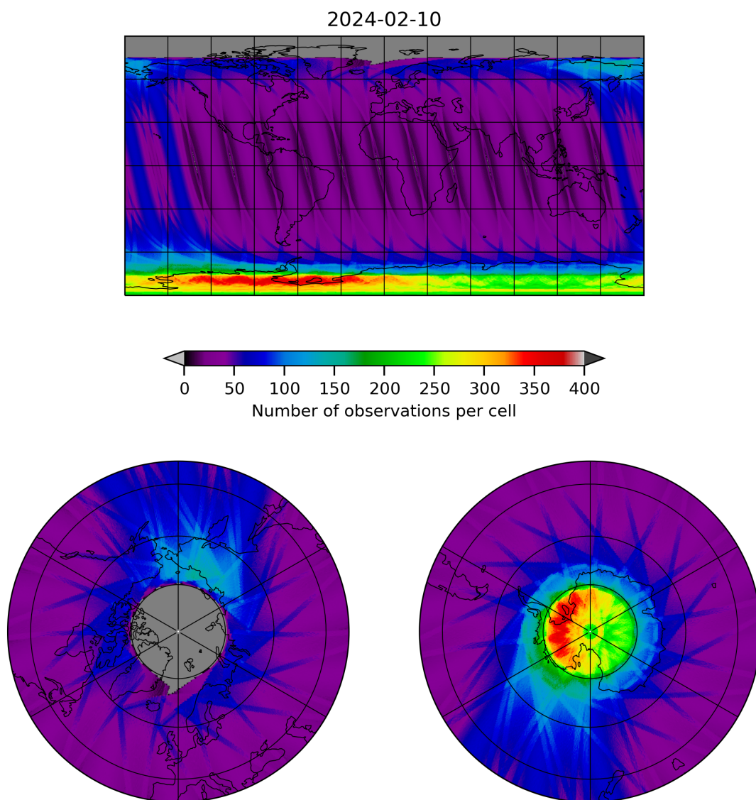
Figure 12: Map of the number of observations for 2024-02-09 to 2024-02-11
