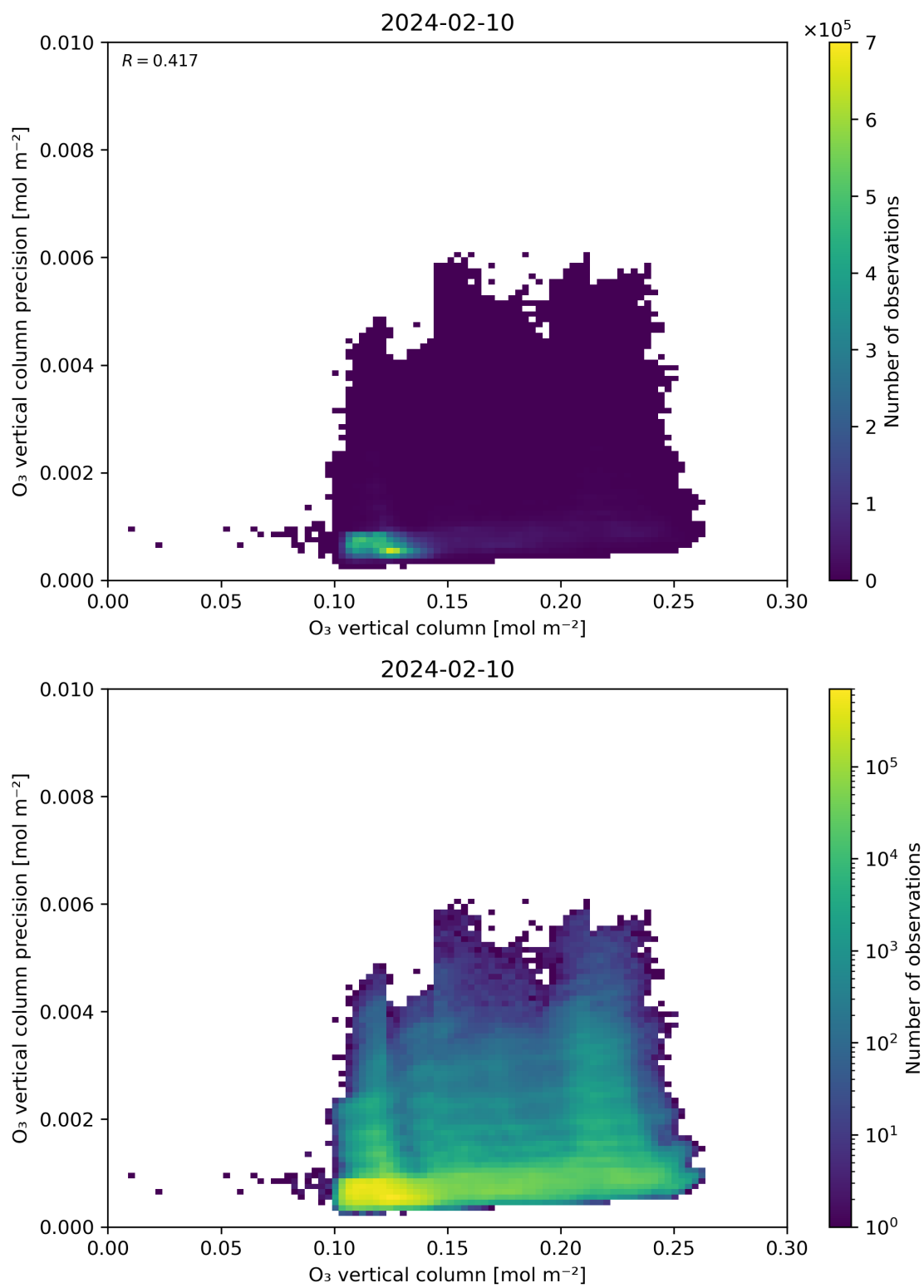
Figure 41: Scatter density plot of “O 3 vertical column” against “O 3 vertical column precision” for 2024-02-09 to 2024-02-11.
