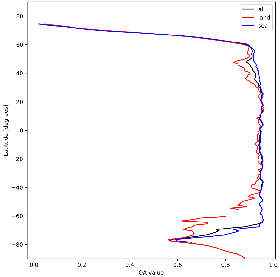
Figure 13: Zonal average of “QA value” for 2024-02-09 to 2024-02-11.
