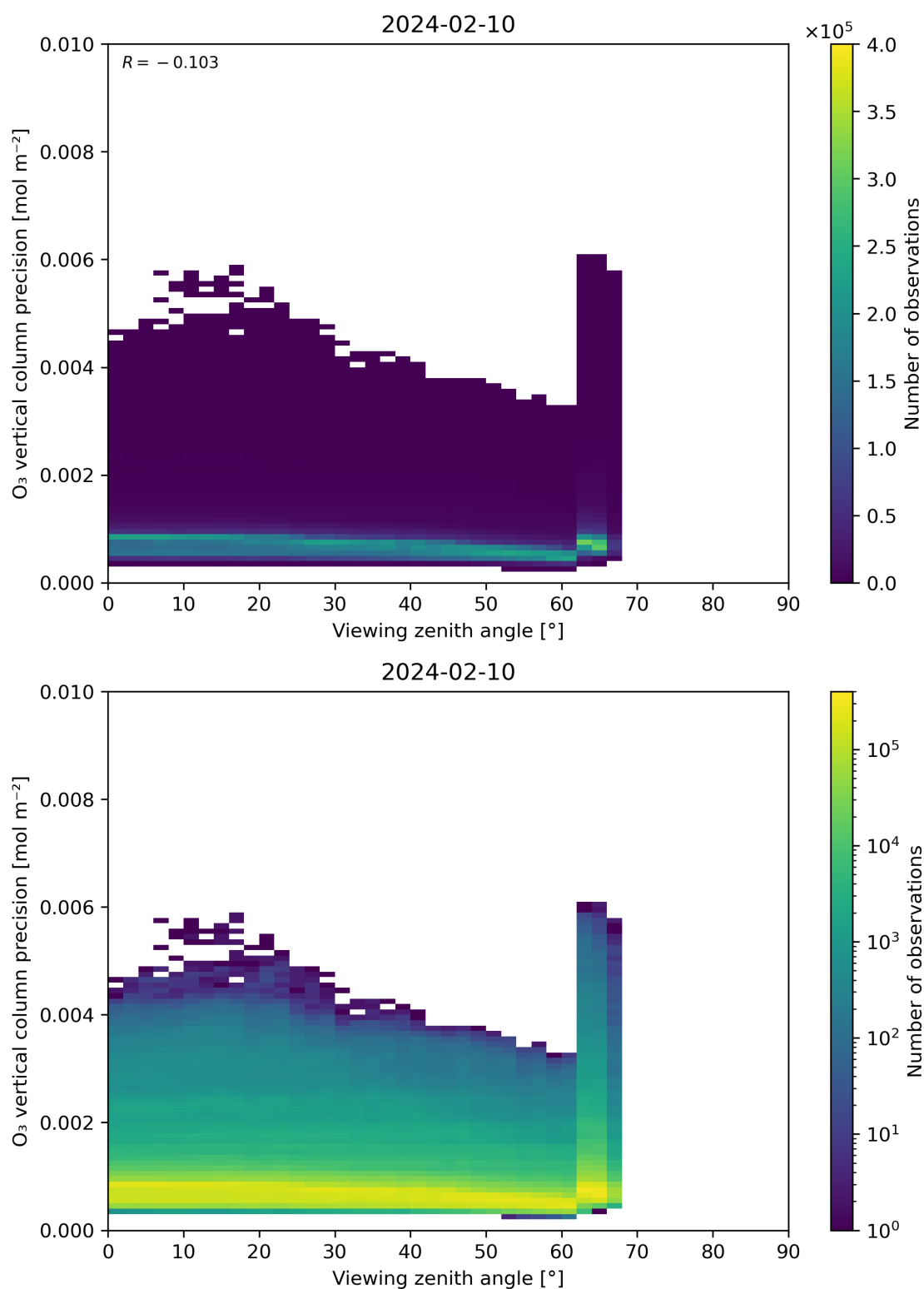
Figure 53: Scatter density plot of “Viewing zenith angle” against “O 3 vertical column precision” for 2024-02-09 to 2024-02-11.
