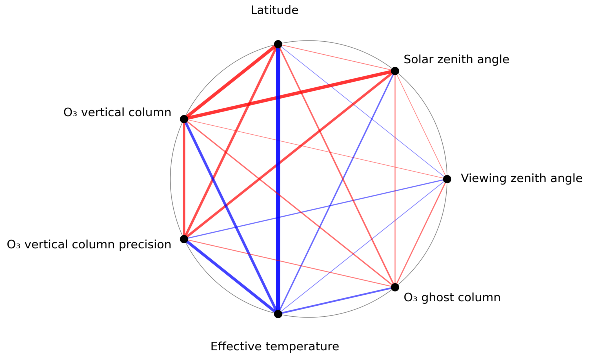
Figure 1: Map of correlation graph for 2024-02-09 to 2024-02-11.
