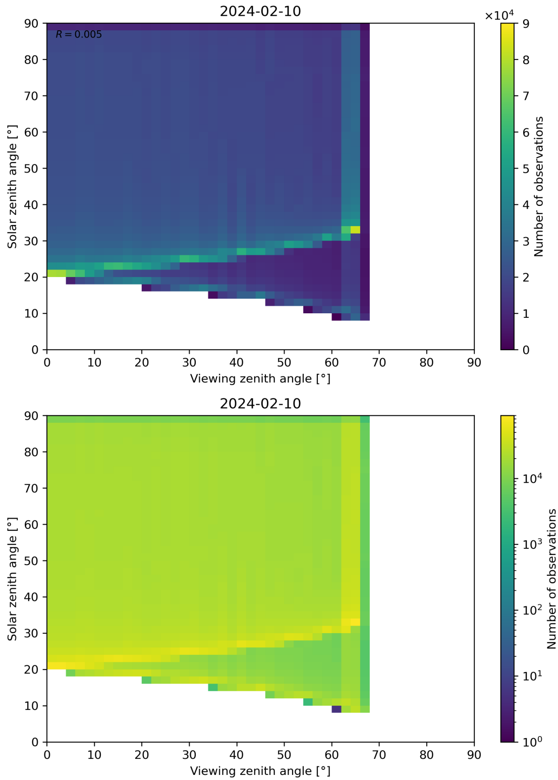
Figure 54: Scatter density plot of “Viewing zenith angle” against “Solar zenith angle” for 2024-02-09 to 2024-02-11.
