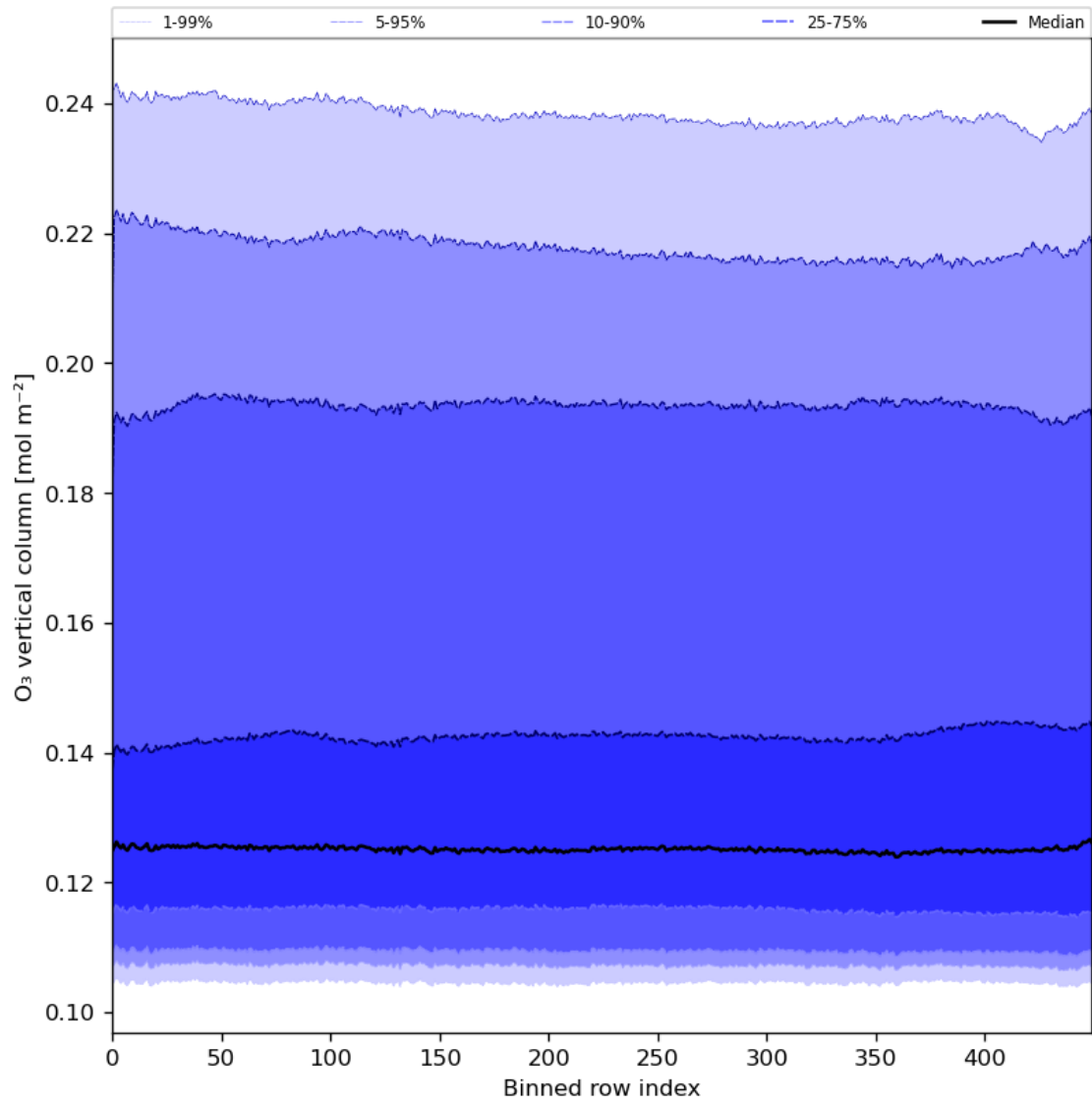
Figure 28: Along track statistics of “O 3 vertical column” for 2024-02-09 to 2024-02-11
