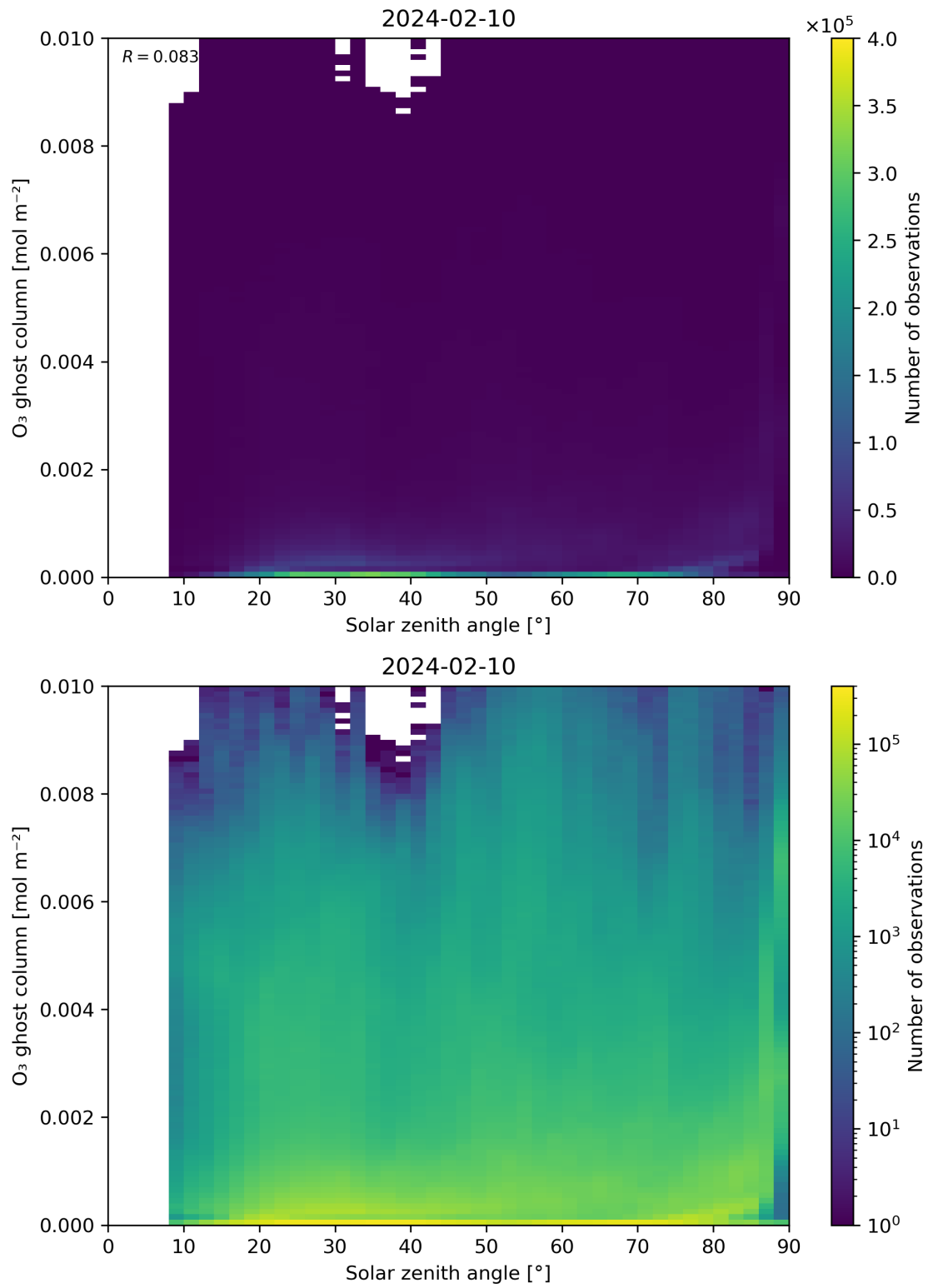
Figure 46: Scatter density plot of “Solar zenith angle” against “O 3 ghost column” for 2024-02-09 to 2024-02-11.
