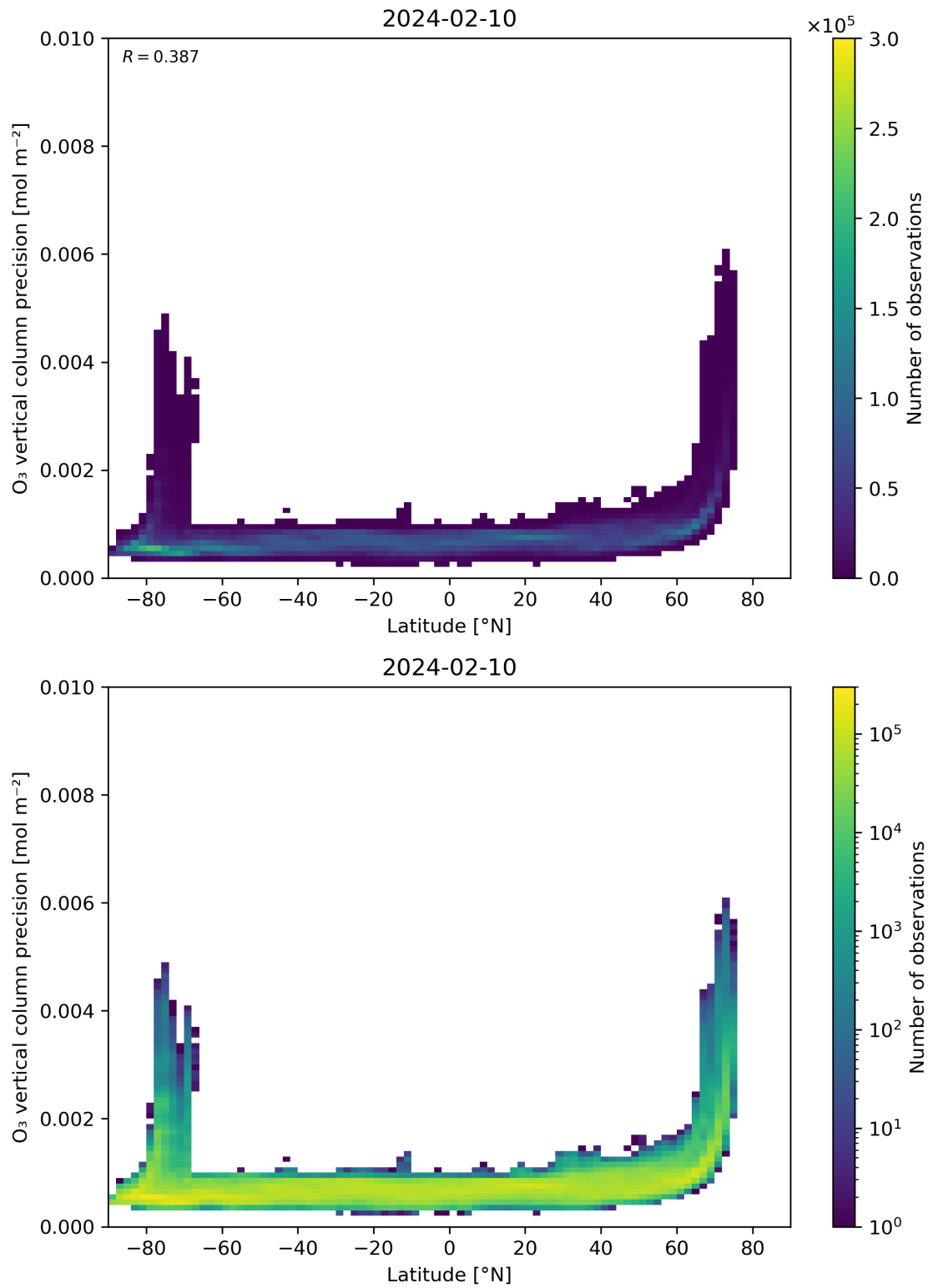
Figure 37: Scatter density plot of “Latitude” against “O 3 vertical column precision” for 2024-02-09 to 2024-02-11.
