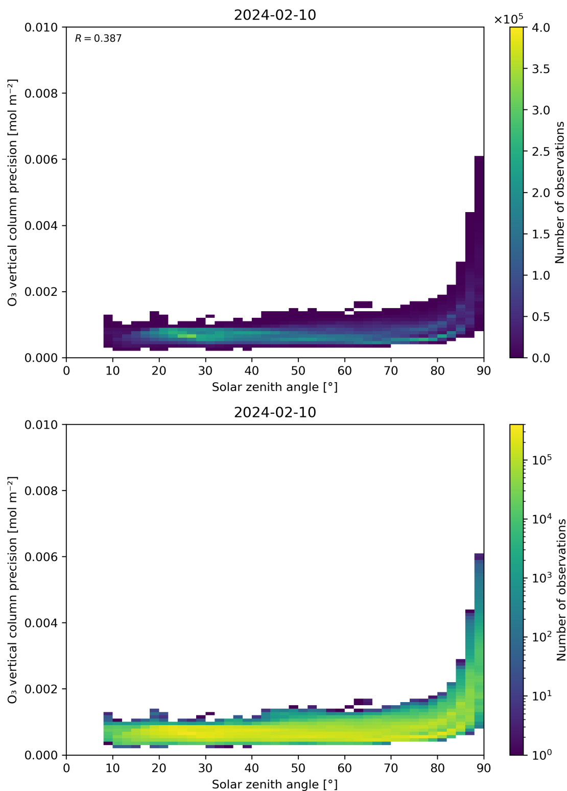
Figure 48: Scatter density plot of “Solar zenith angle” against “O 3 vertical column precision” for 2024-02-09 to 2024-02-11.
