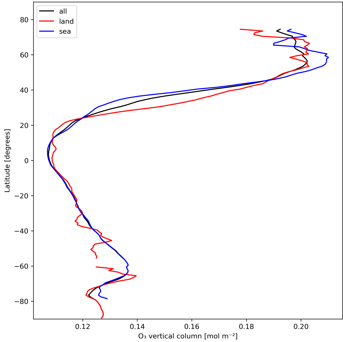
Figure 14: Zonal average of “O 3 vertical column” for 2024-02-09 to 2024-02-11.
