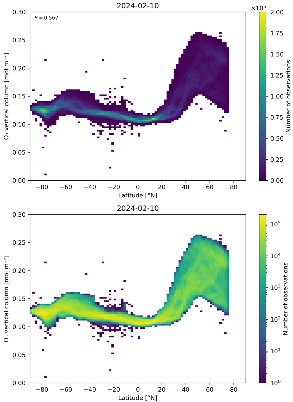
Figure 36: Scatter density plot of “Latitude” against “O 3 vertical column” for 2024-02-09 to 2024-02-11.
