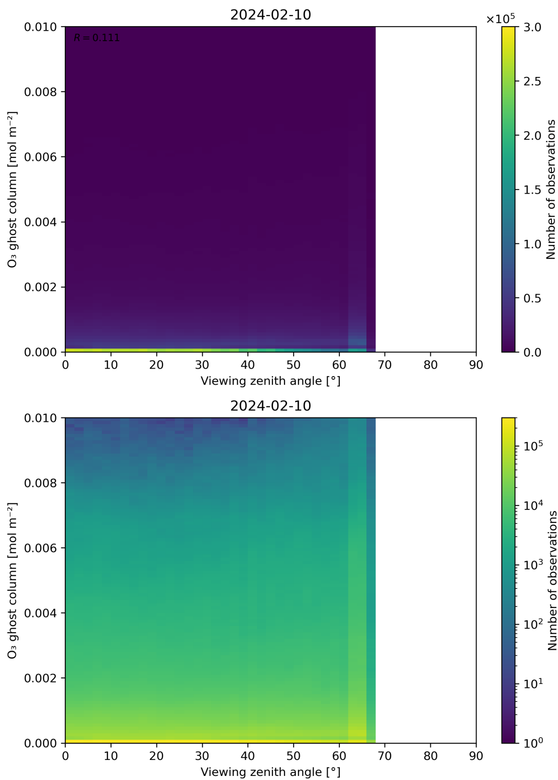
Figure 51: Scatter density plot of “Viewing zenith angle” against “O 3 ghost column” for 2024-02-09 to 2024-02-11.
