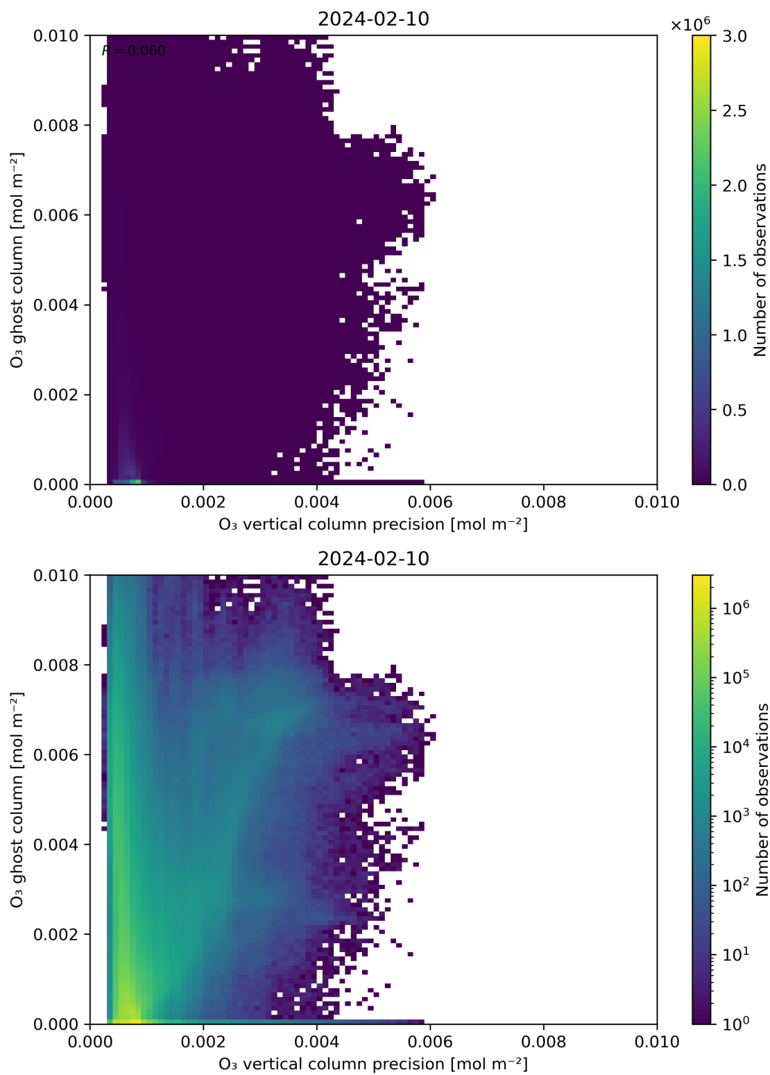
Figure 43: Scatter density plot of “O 3 vertical column precision” against “O 3 ghost column” for 2024-02-09 to 2024-02-11.
