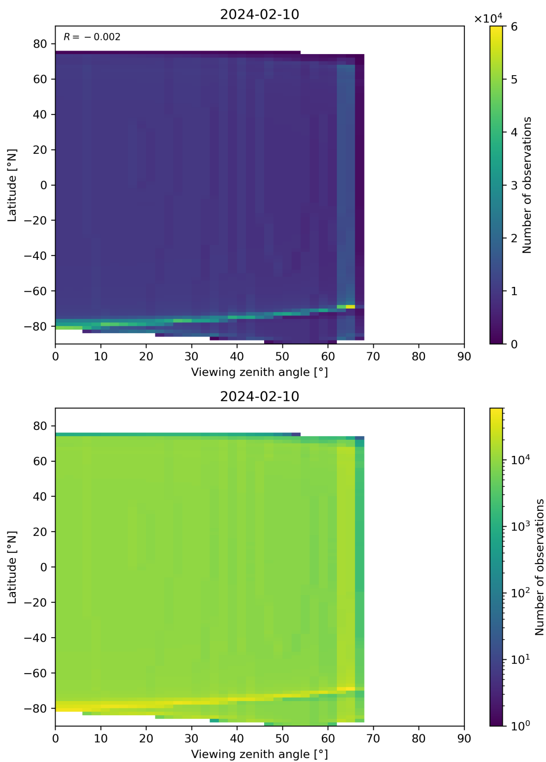
Figure 49: Scatter density plot of “Viewing zenith angle” against “Latitude” for 2024-02-09 to 2024-02-11.
