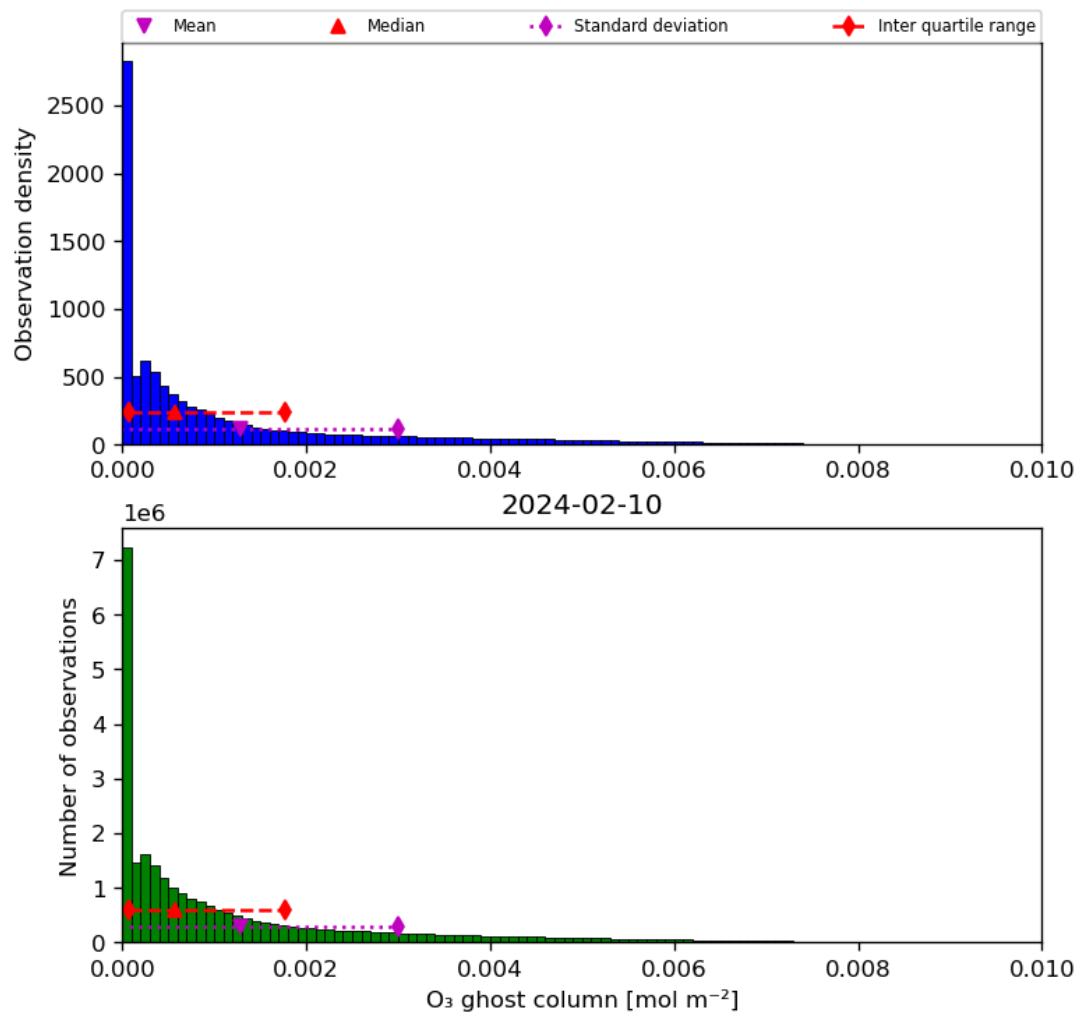
Figure 25: Histogram of “O 3 ghost column” for 2024-02-09 to 2024-02-11
