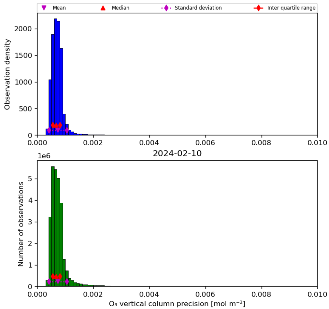
Figure 22: Histogram of “O 3 vertical column precision” for 2024-02-09 to 2024-02-11
