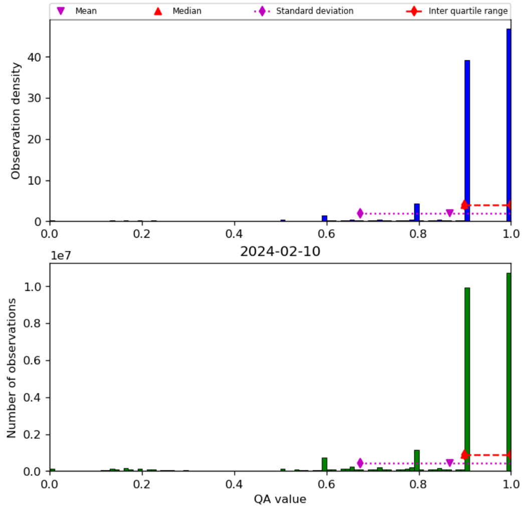
Figure 20: Histogram of “QA value” for 2024-02-09 to 2024-02-11
