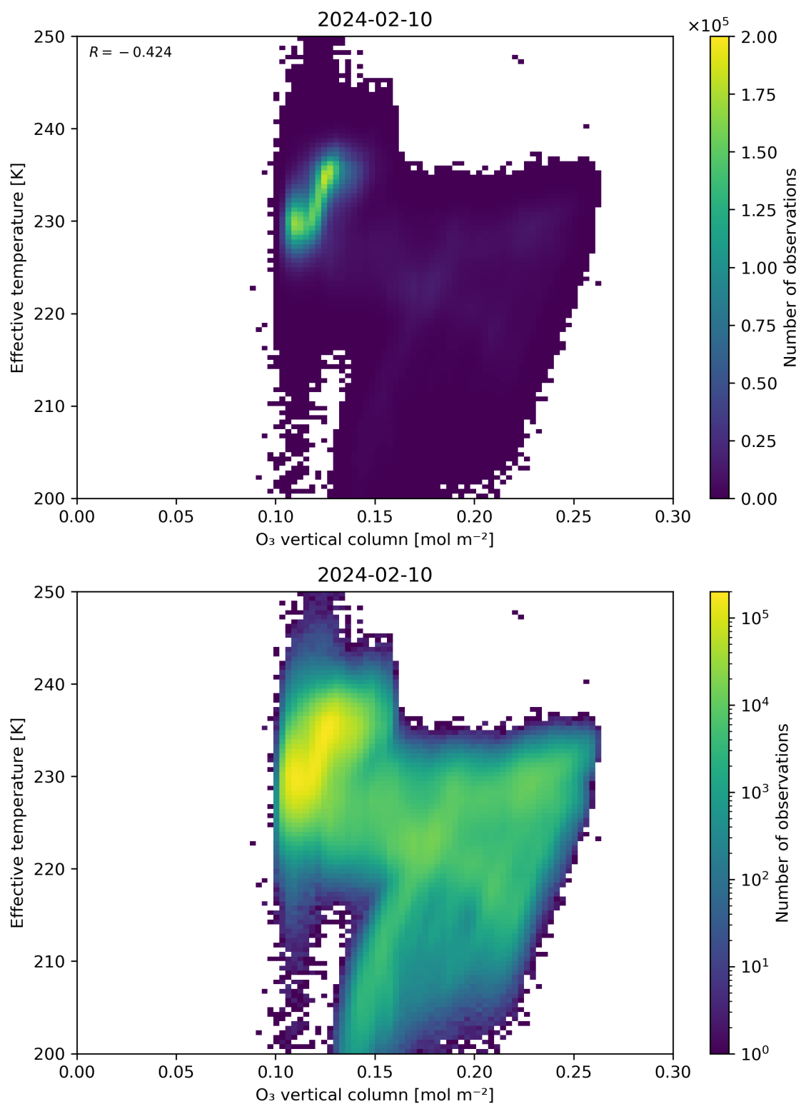
Figure 39: Scatter density plot of “O 3 vertical column” against “Effective temperature” for 2024-02-09 to 2024-02-11.
