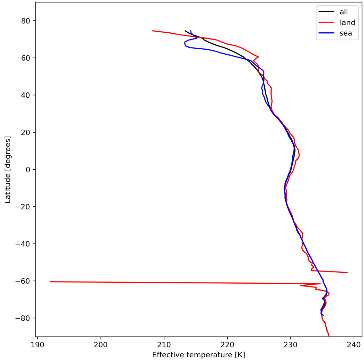
Figure 17: Zonal average of “Effective temperature” for 2024-02-09 to 2024-02-11.
