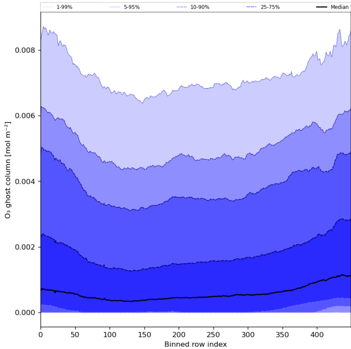
Figure 32: Along track statistics of “O 3 ghost column” for 2024-02-09 to 2024-02-11
