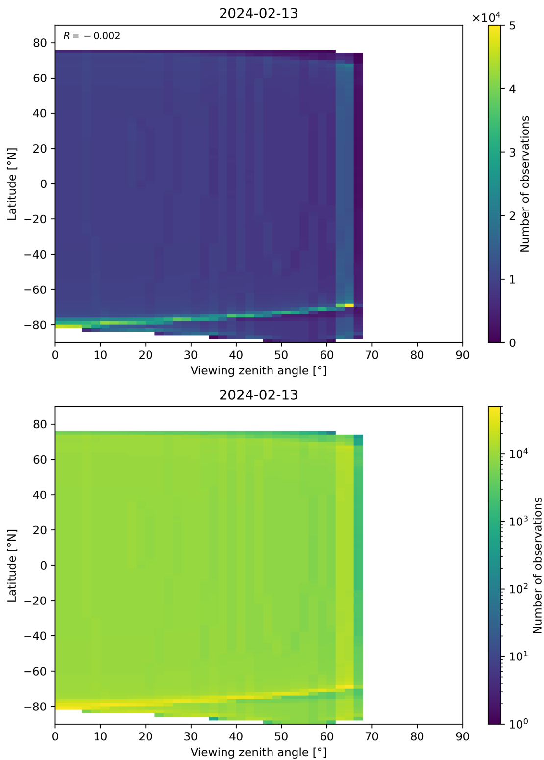
Figure 49: Scatter density plot of “Viewing zenith angle” against “Latitude” for 2024-02-12 to 2024-02-14.
