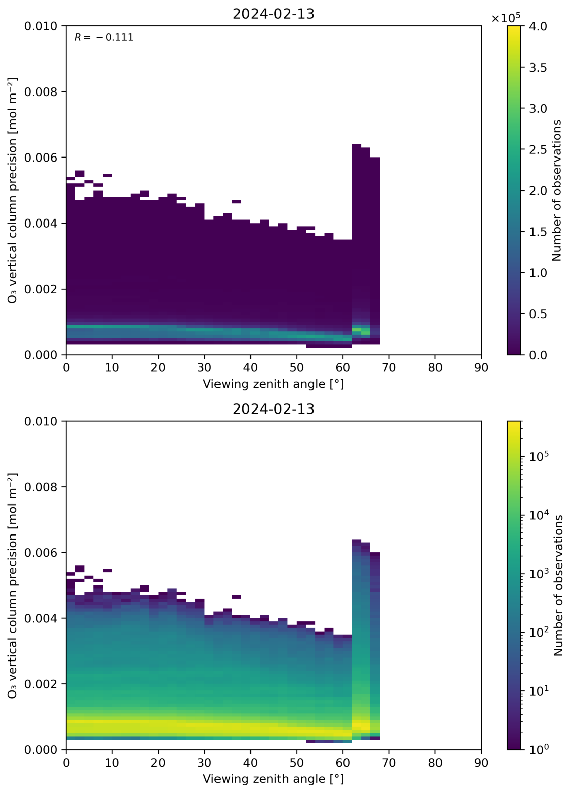
Figure 53: Scatter density plot of “Viewing zenith angle” against “O 3 vertical column precision” for 2024-02-12 to 2024-02-14.
