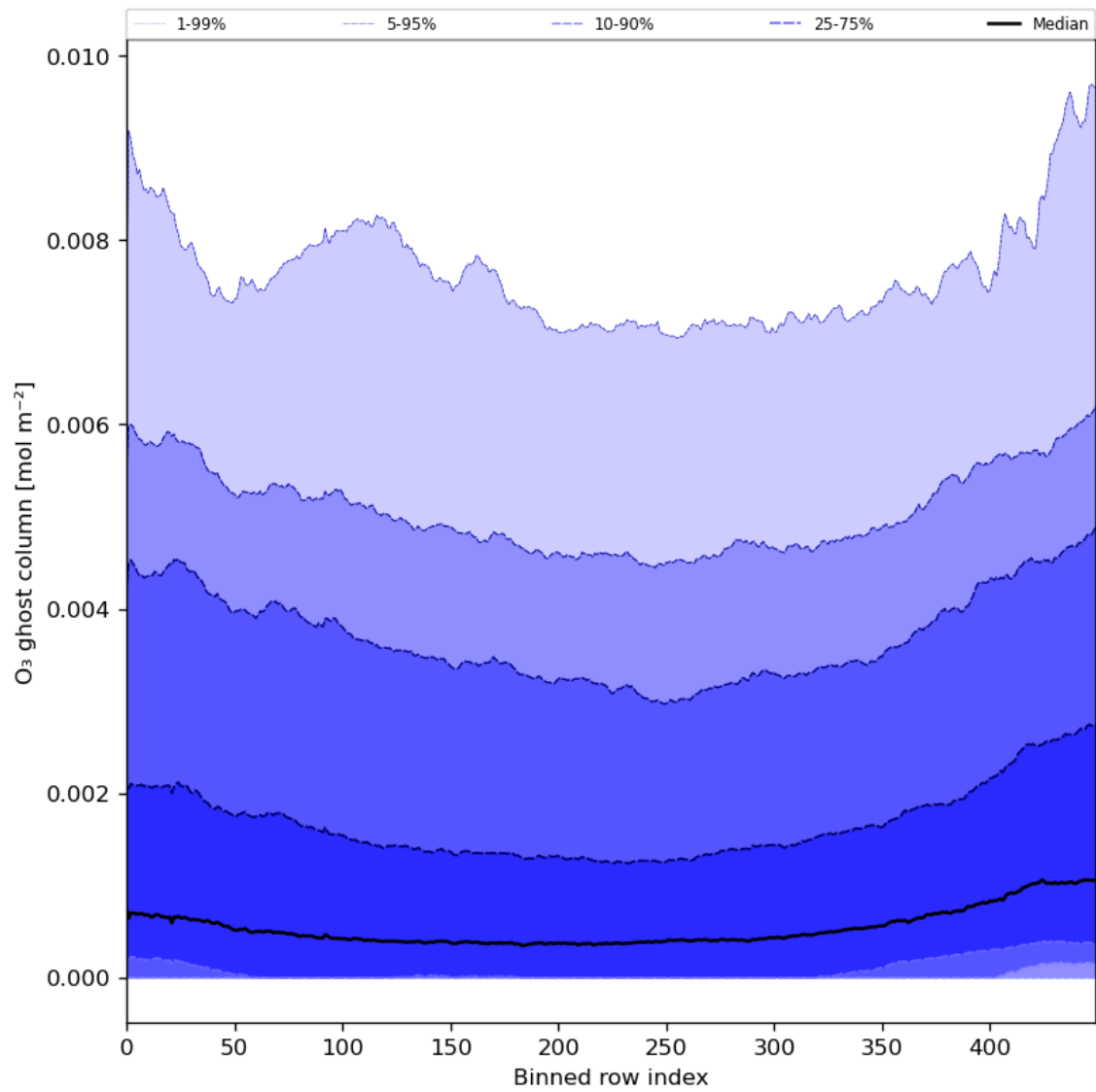
Figure 32: Along track statistics of “O 3 ghost column” for 2024-02-12 to 2024-02-14
