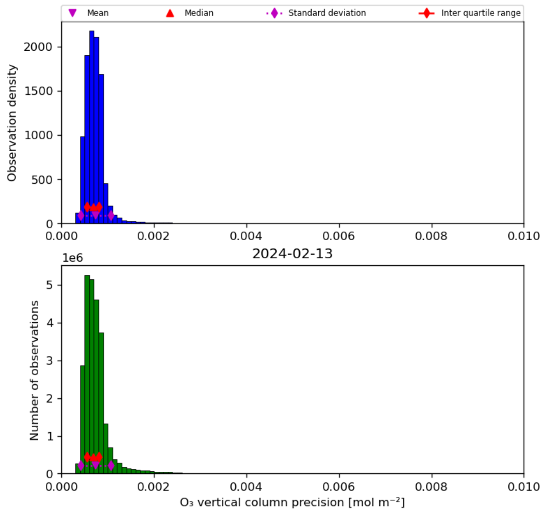
Figure 22: Histogram of “O 3 vertical column precision” for 2024-02-12 to 2024-02-14
