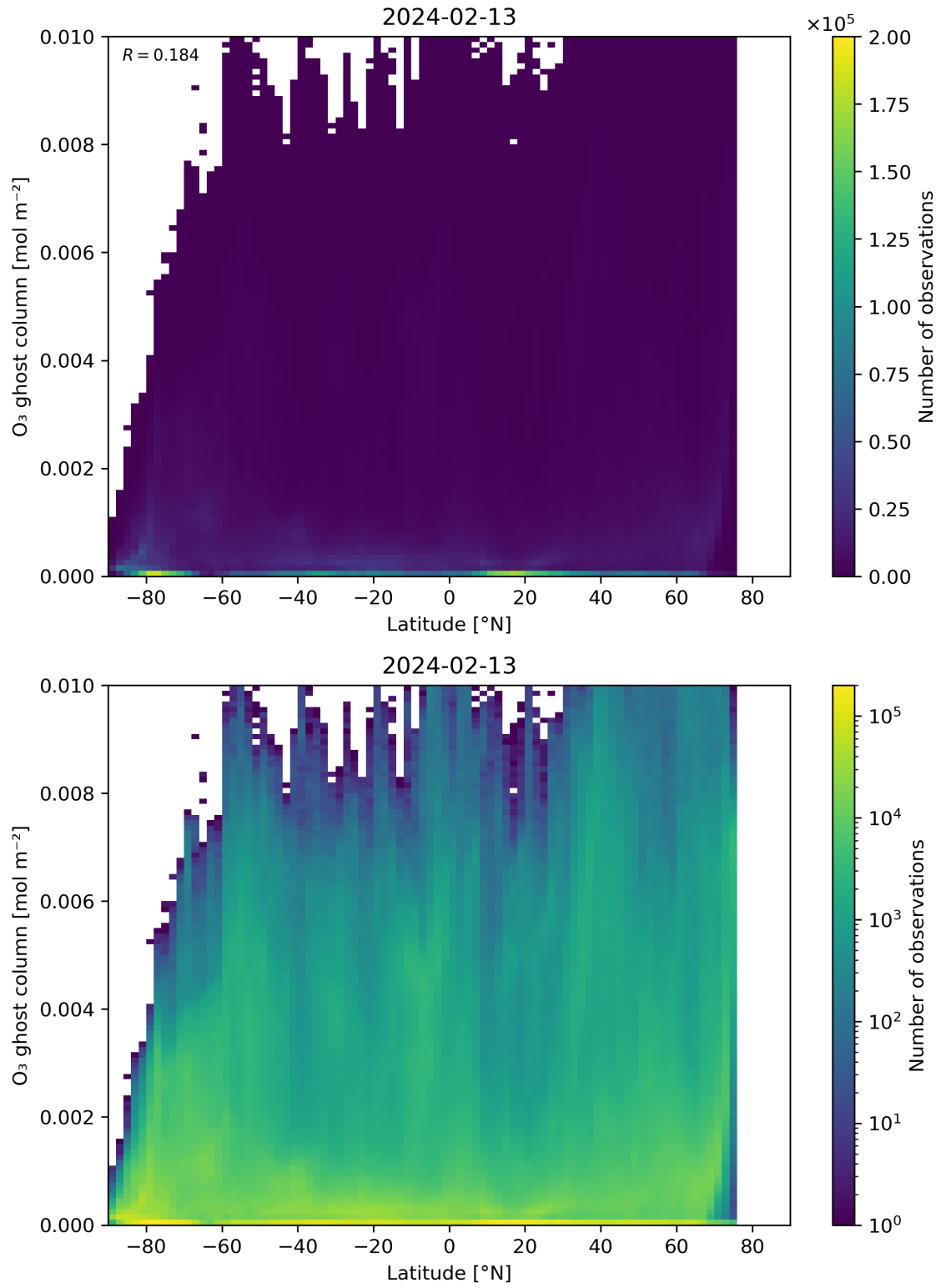
Figure 35: Scatter density plot of “Latitude” against “O 3 ghost column” for 2024-02-12 to 2024-02-14.
