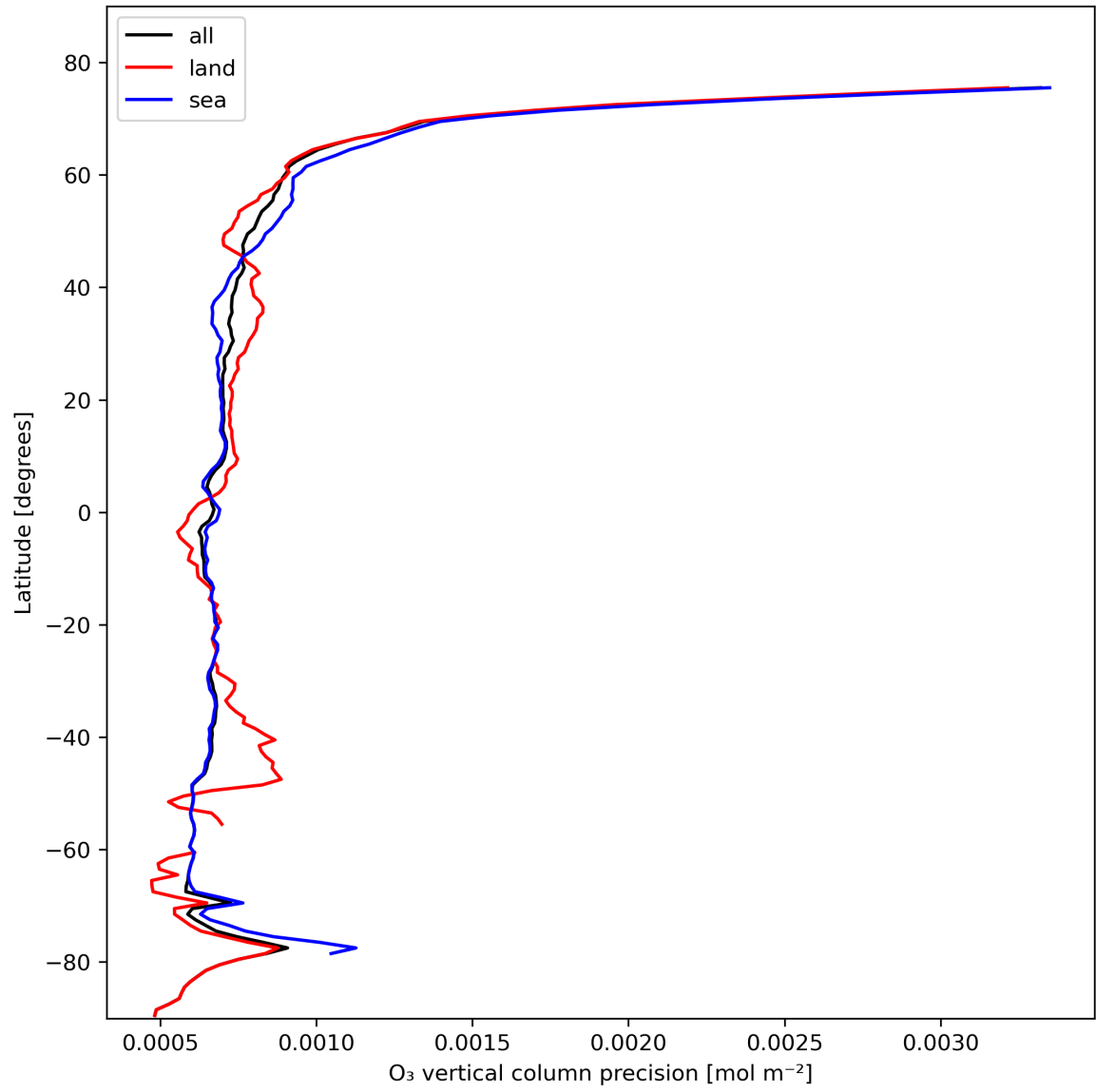
Figure 15: Zonal average of “O 3 vertical column precision” for 2024-02-12 to 2024-02-14.
