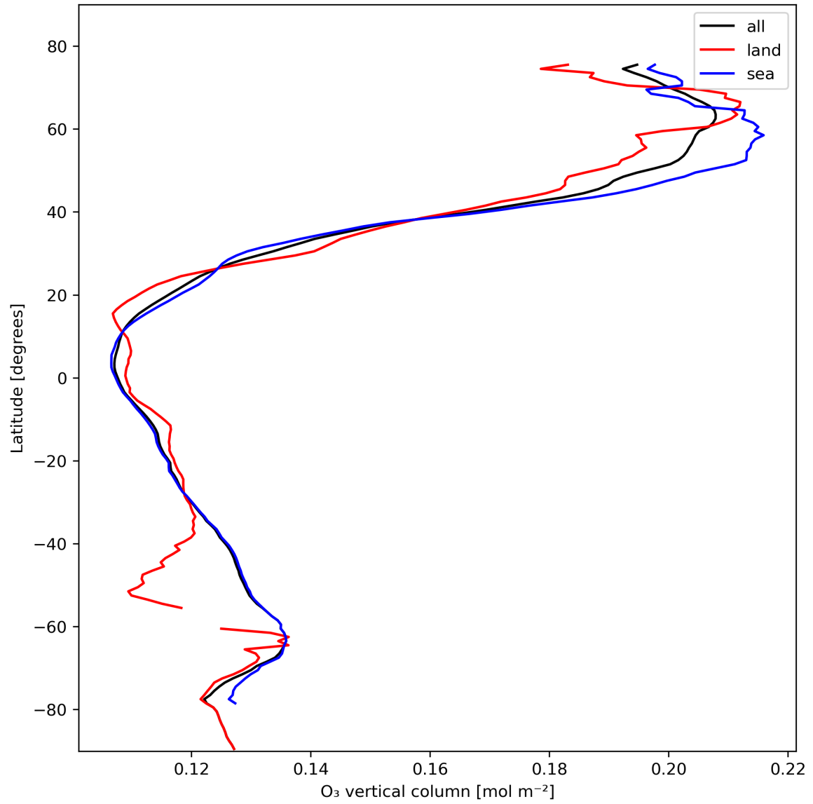
Figure 14: Zonal average of “O 3 vertical column” for 2024-02-12 to 2024-02-14.
