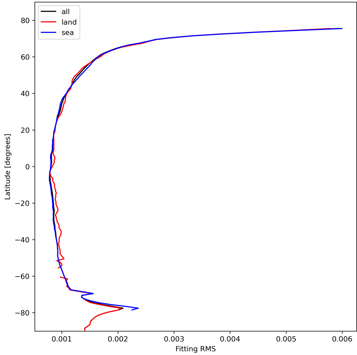
Figure 16: Zonal average of “Fitting RMS” for 2024-02-12 to 2024-02-14.
