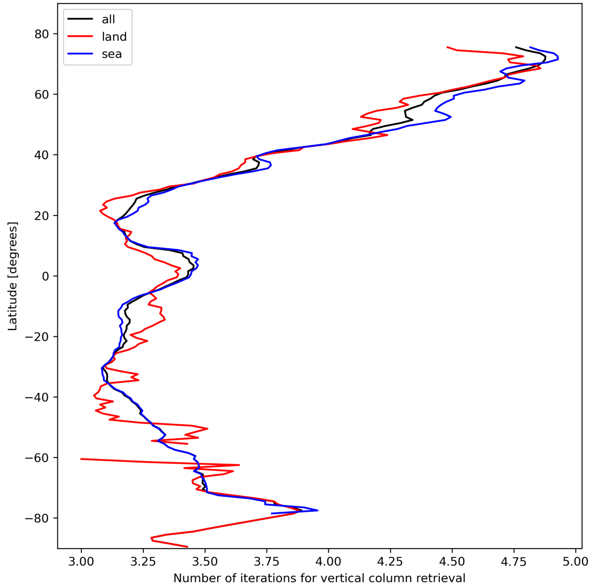
Figure 19: Zonal average of “Number of iterations for vertical column retrieval” for 2024-02-12 to 2024-02-14.
