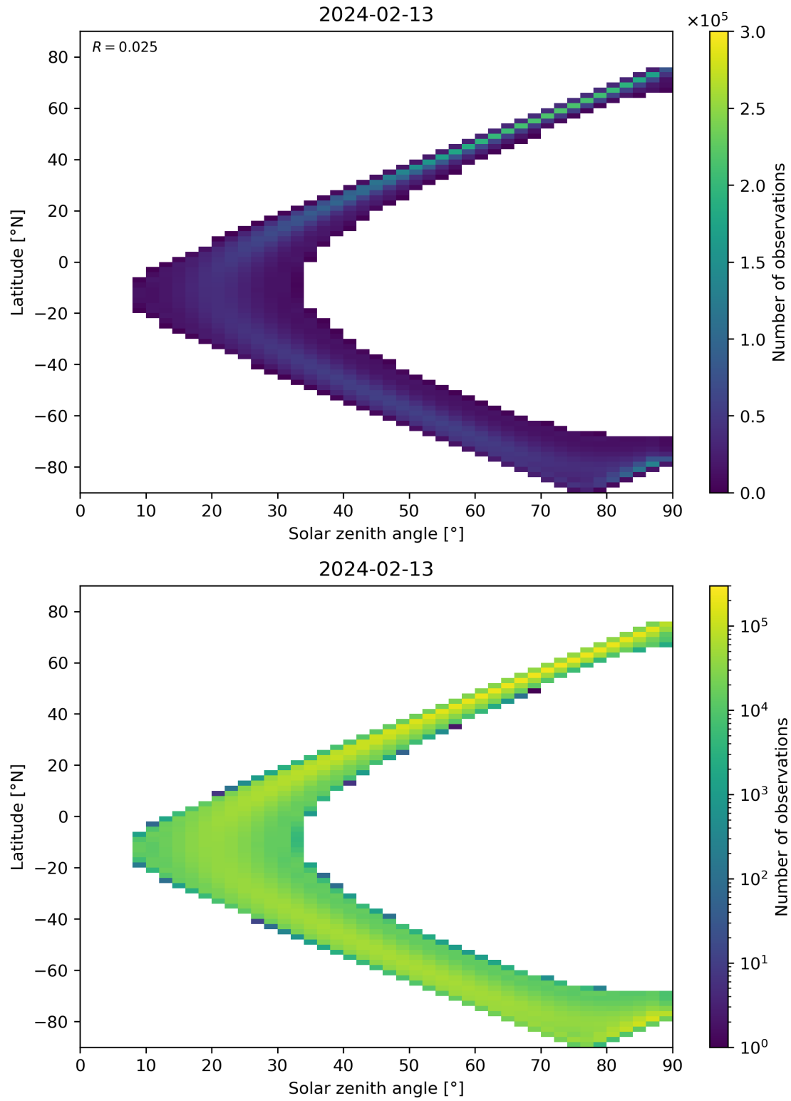
Figure 44: Scatter density plot of “Solar zenith angle” against “Latitude” for 2024-02-12 to 2024-02-14.
