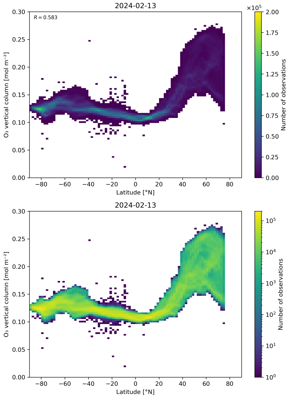
Figure 36: Scatter density plot of “Latitude” against “O 3 vertical column” for 2024-02-12 to 2024-02-14.
