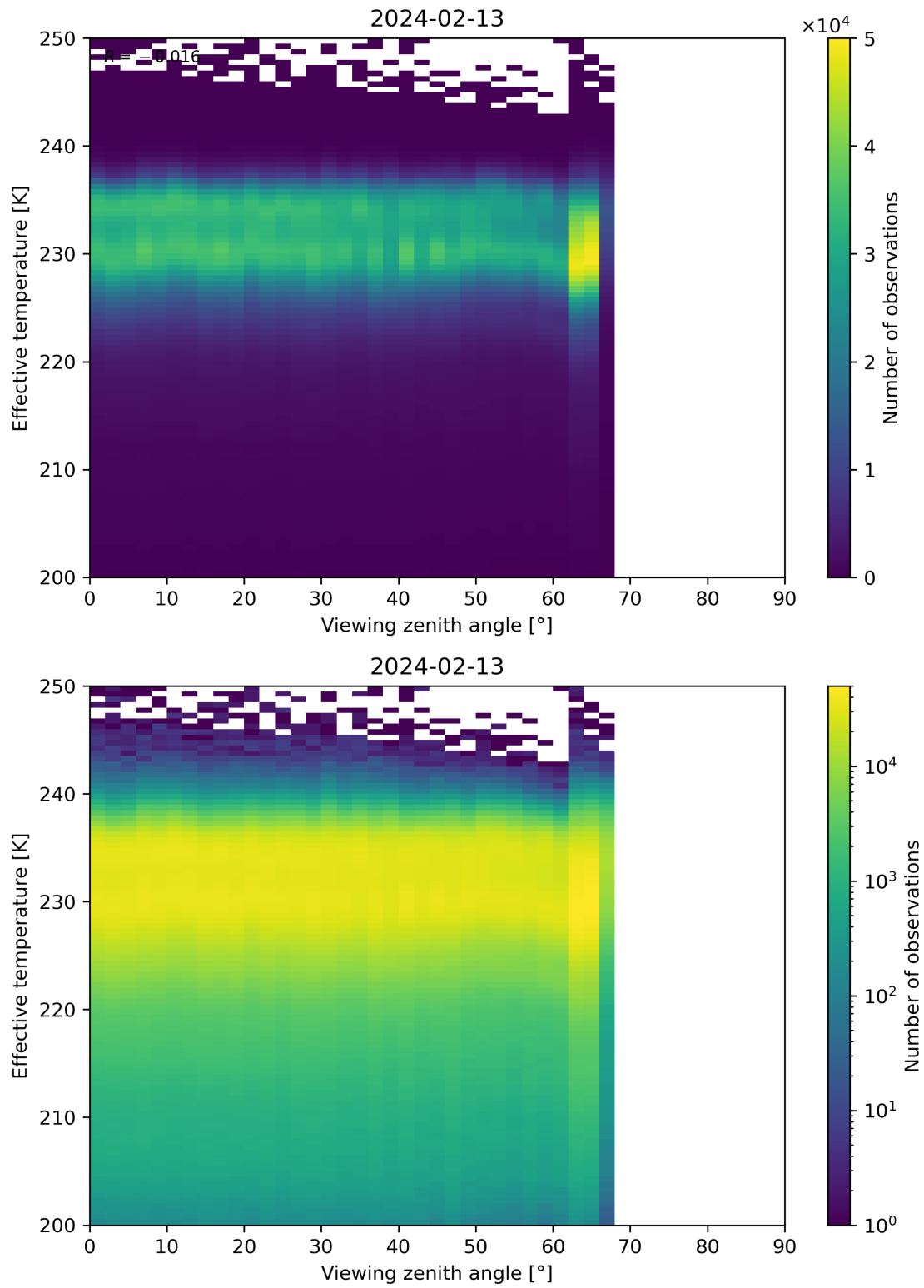
Figure 50: Scatter density plot of “Viewing zenith angle” against “Effective temperature” for 2024-02-12 to 2024-02-14.
