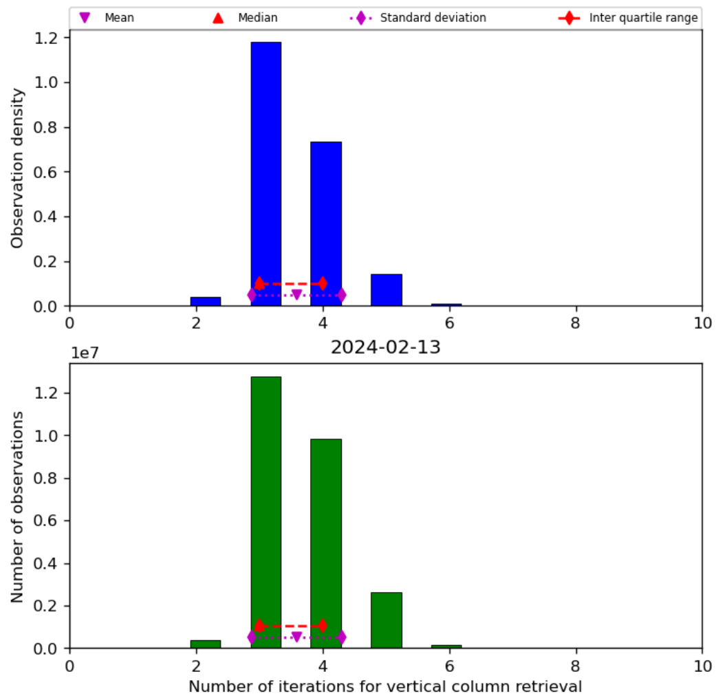
Figure 26: Histogram of “Number of iterations for vertical column retrieval” for 2024-02-12 to 2024-02-14
