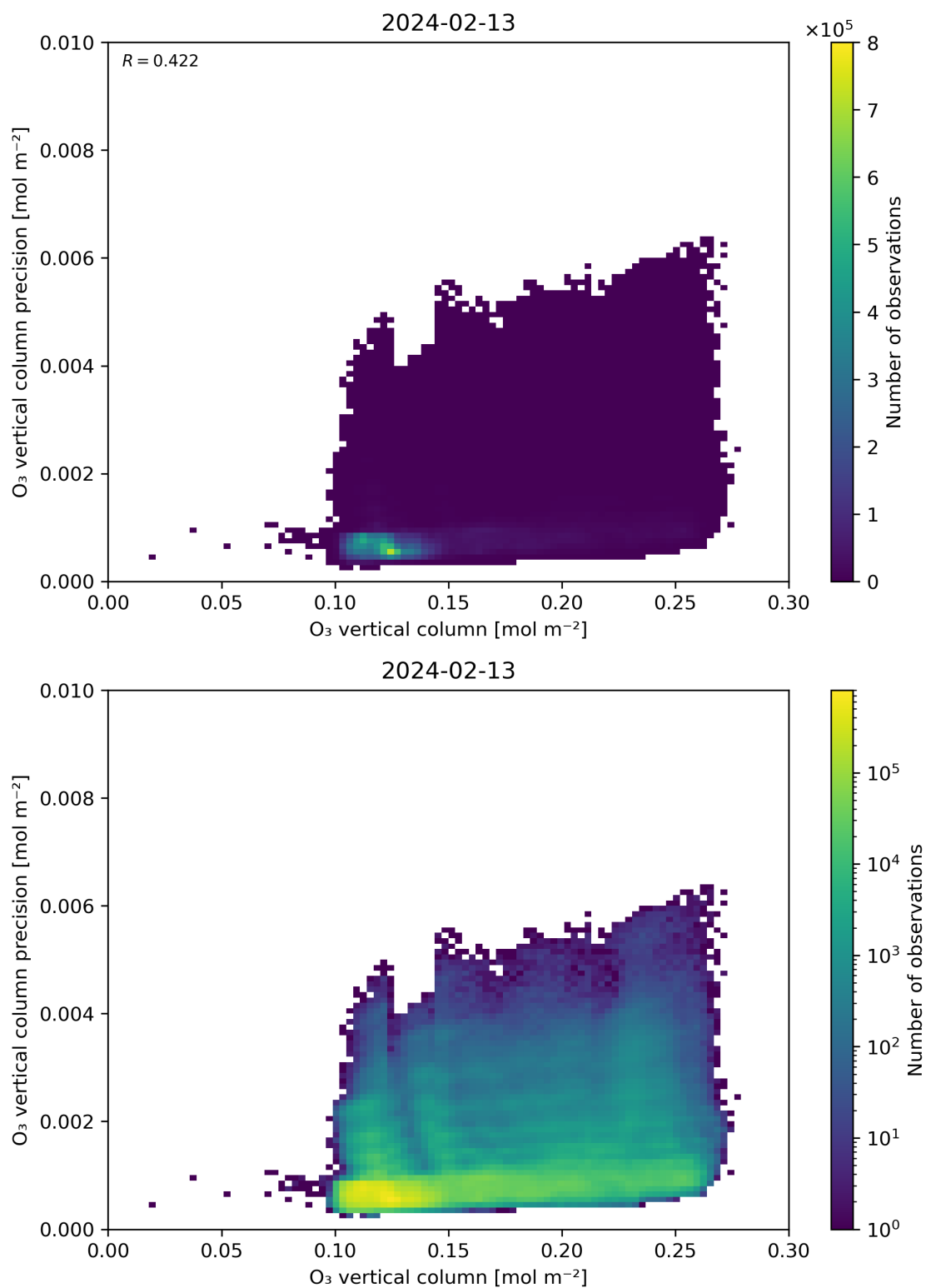
Figure 41: Scatter density plot of “O 3 vertical column” against “O 3 vertical column precision” for 2024-02-12 to 2024-02-14.
