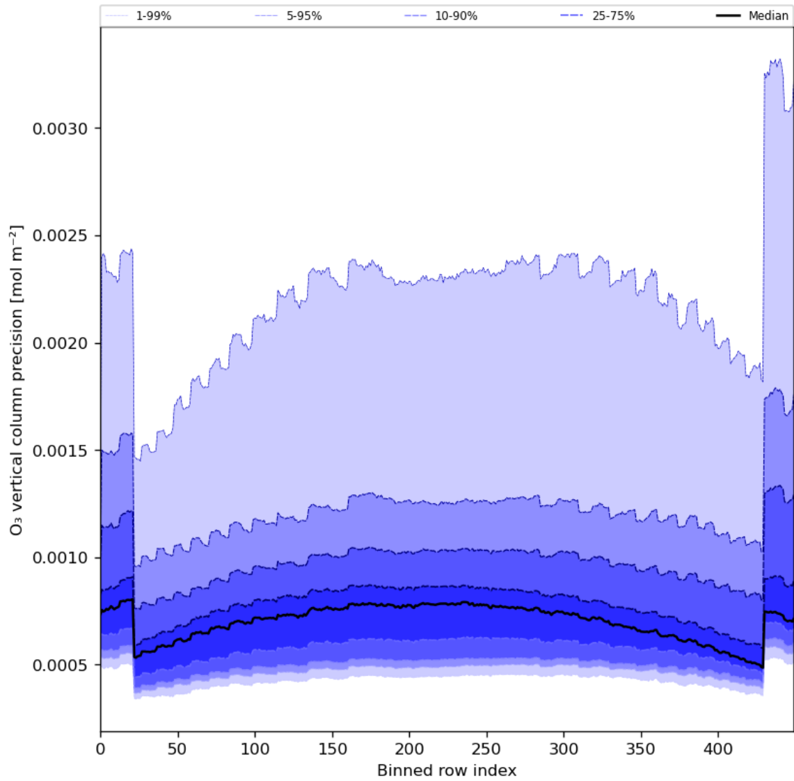
Figure 29: Along track statistics of “O 3 vertical column precision” for 2024-02-12 to 2024-02-14
