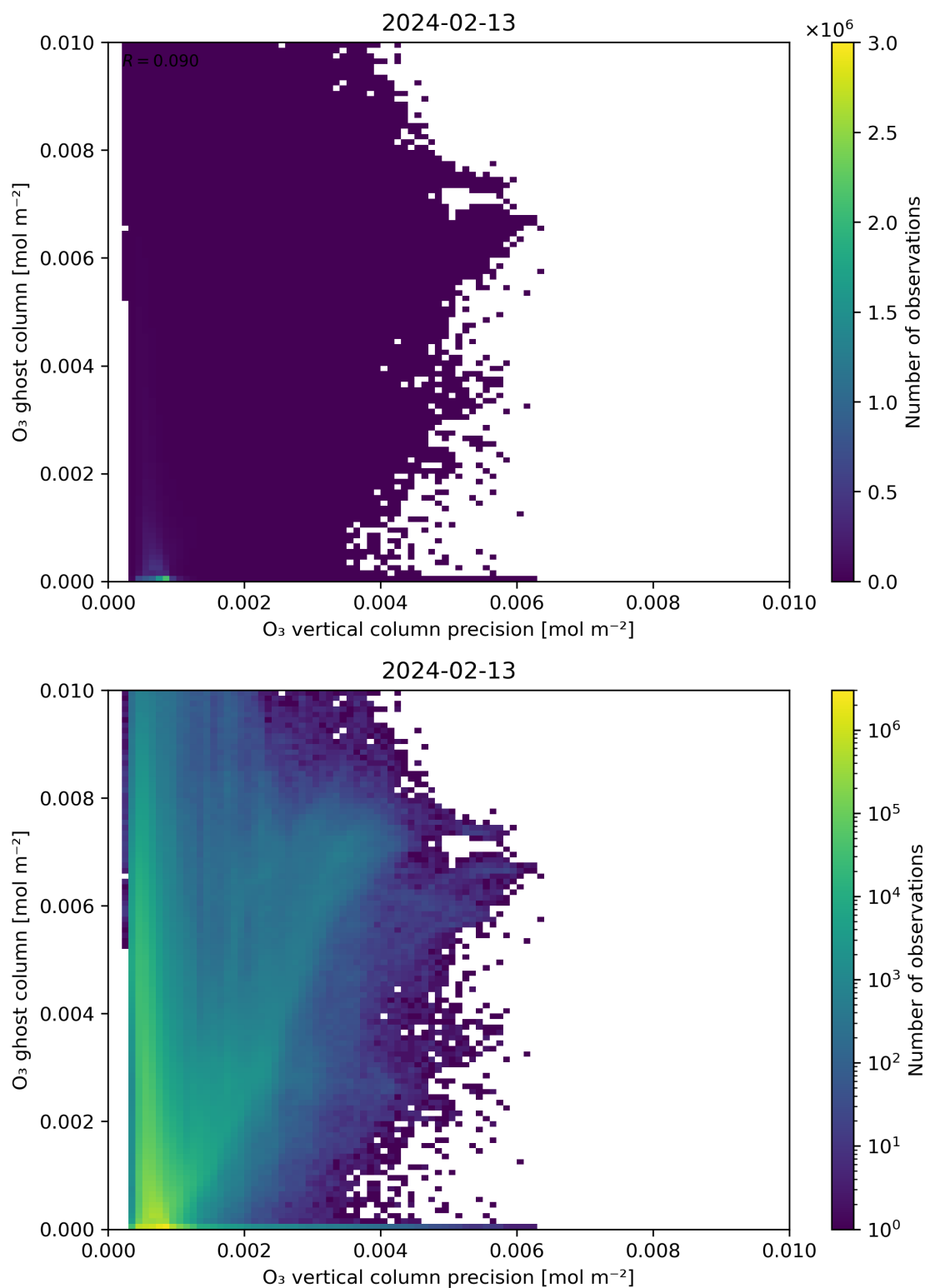
Figure 43: Scatter density plot of “O 3 vertical column precision” against “O 3 ghost column” for 2024-02-12 to 2024-02-14.
