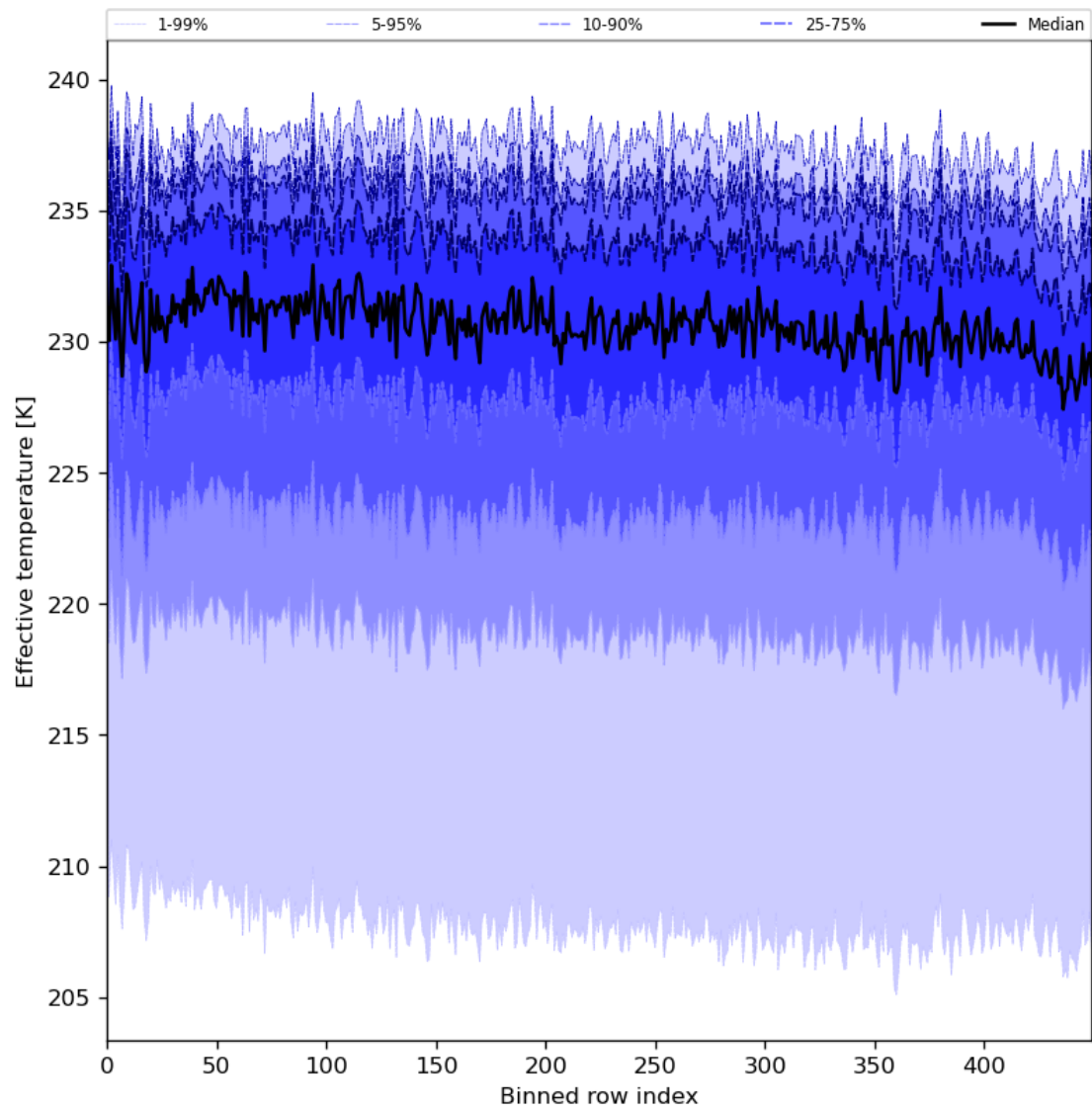
Figure 31: Along track statistics of “Effective temperature” for 2024-02-12 to 2024-02-14
