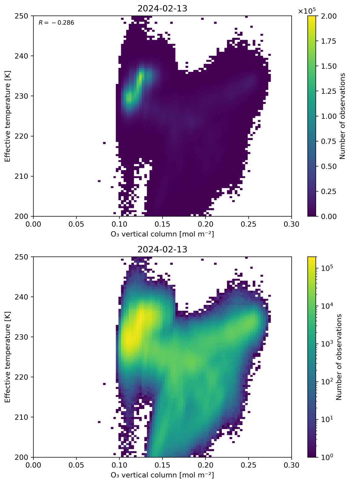
Figure 39: Scatter density plot of “O 3 vertical column” against “Effective temperature” for 2024-02-12 to 2024-02-14.
