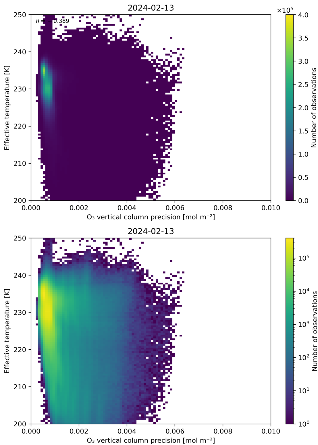
Figure 42: Scatter density plot of “O 3 vertical column precision” against “Effective temperature” for 2024-02-12 to 2024-02-14.
