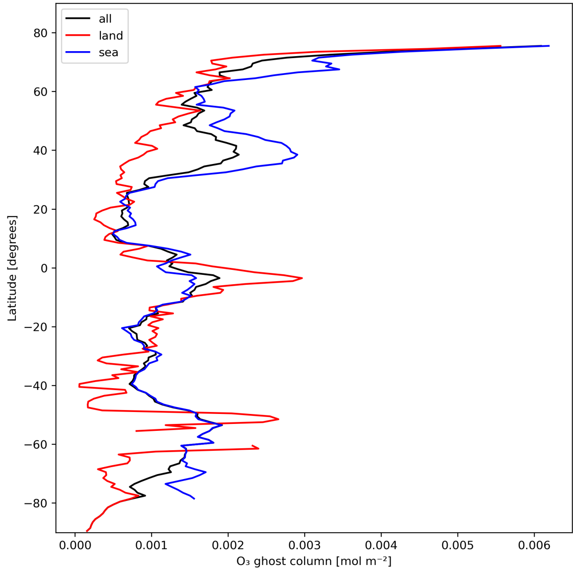
Figure 18: Zonal average of “O 3 ghost column” for 2024-02-12 to 2024-02-14.
