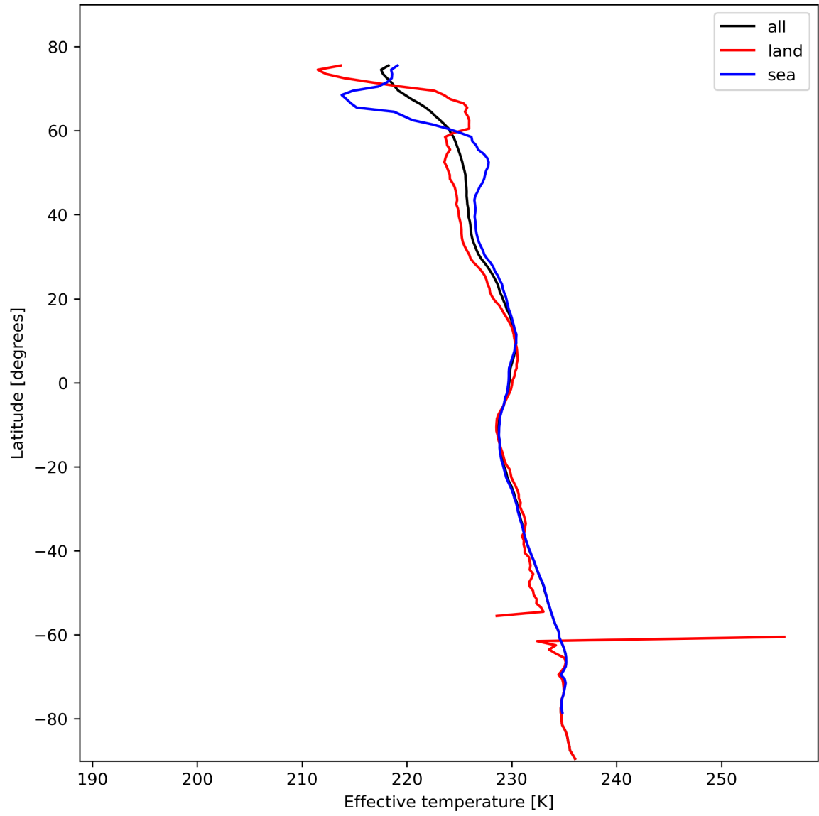
Figure 17: Zonal average of "Effective temperature" for 2024-02-12 to 2024-02-14.
