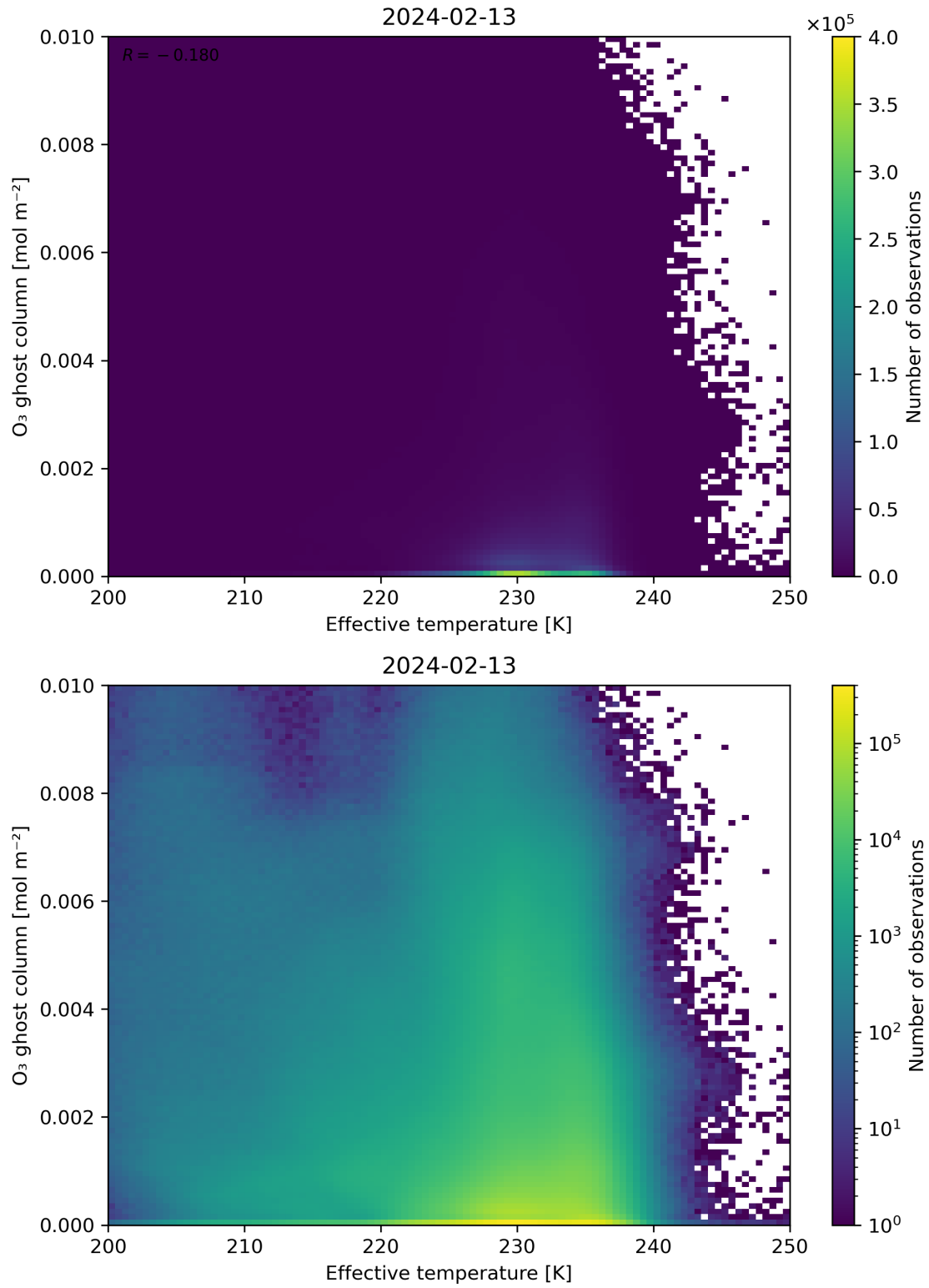
Figure 38: Scatter density plot of “Effective temperature” against “O 3 ghost column” for 2024-02-12 to 2024-02-14.
