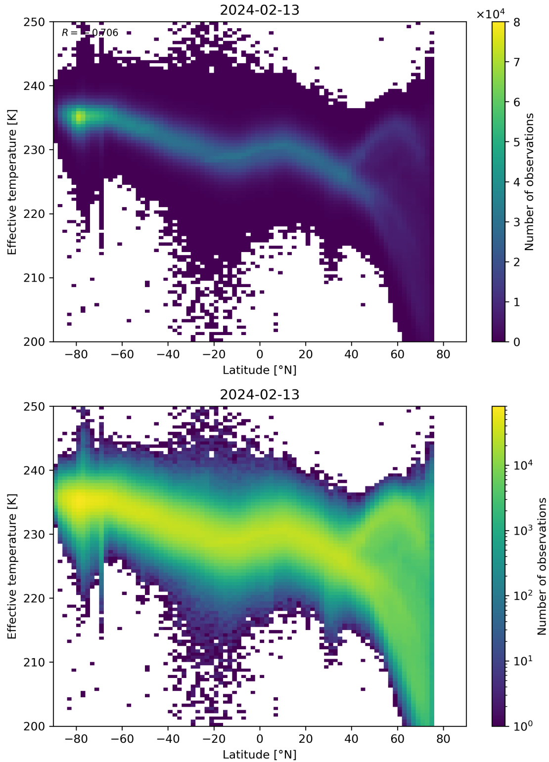
Figure 34: Scatter density plot of “Latitude” against “Effective temperature” for 2024-02-12 to 2024-02-14.
