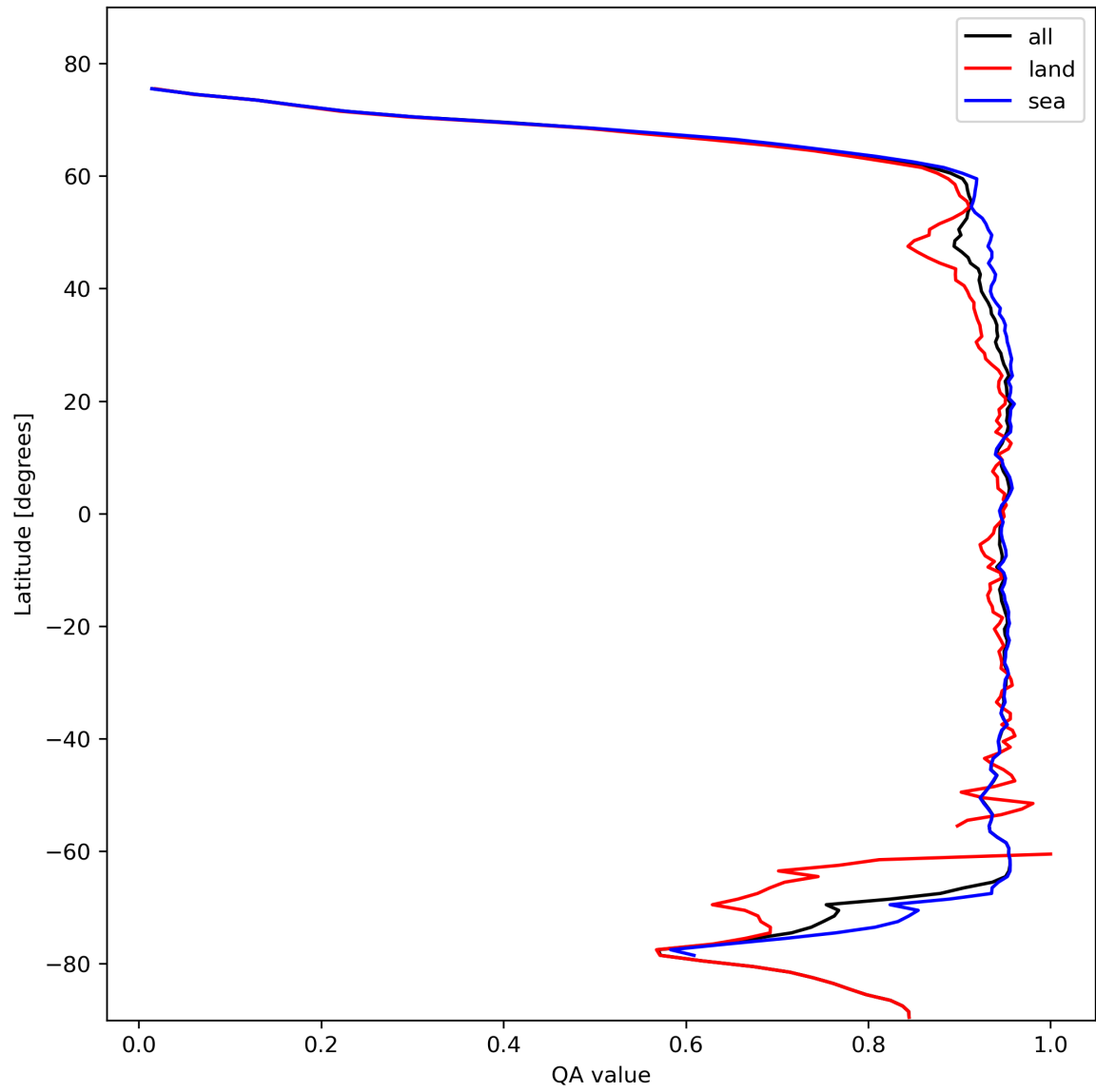
Figure 13: Zonal average of “QA value” for 2024-02-12 to 2024-02-14.
