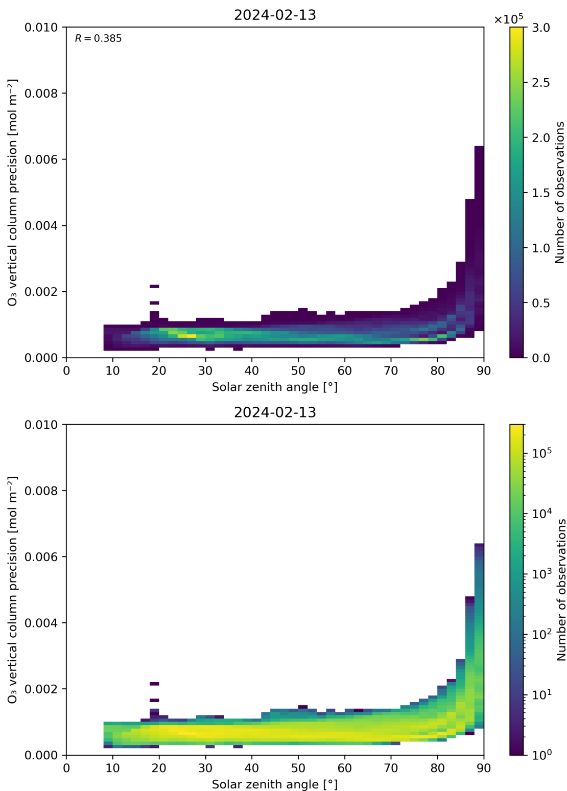
Figure 48: Scatter density plot of “Solar zenith angle” against “O 3 vertical column precision” for 2024-02-12 to 2024-02-14.
