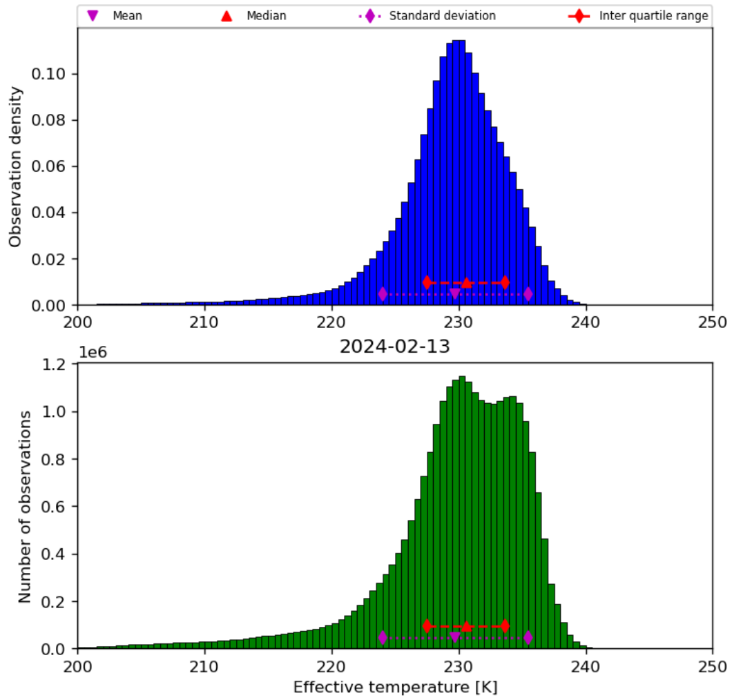
Figure 24: Histogram of “Effective temperature” for 2024-02-12 to 2024-02-14
