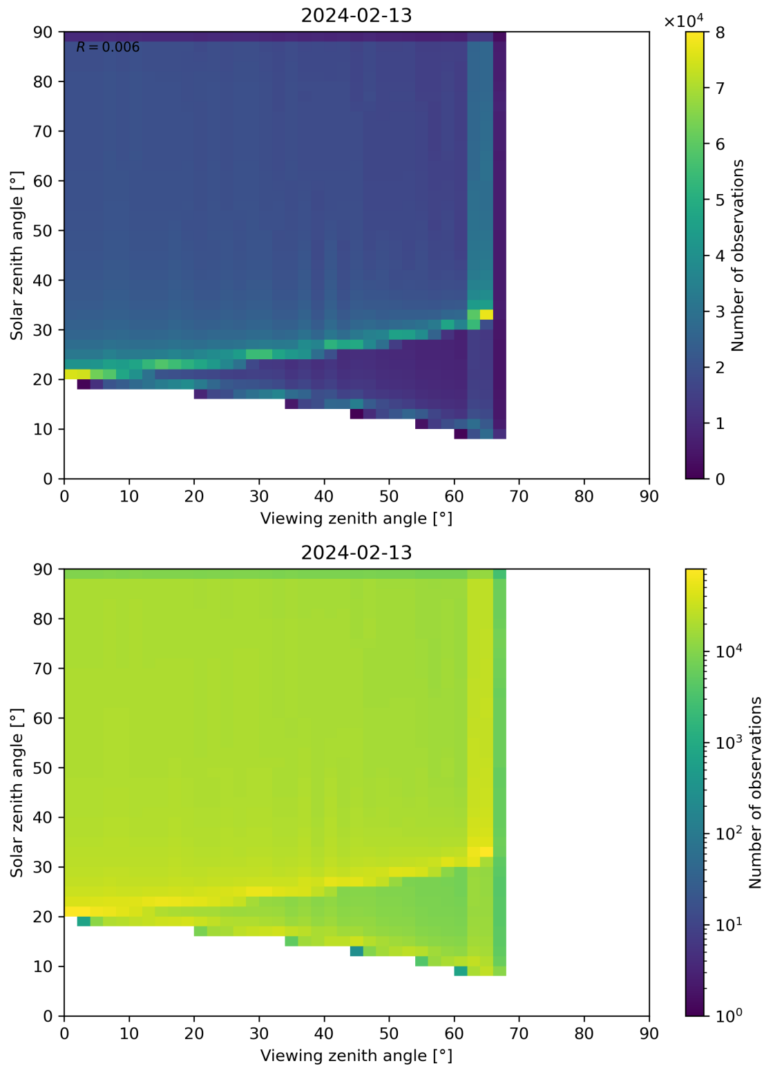
Figure 54: Scatter density plot of “Viewing zenith angle” against “Solar zenith angle” for 2024-02-12 to 2024-02-14.
