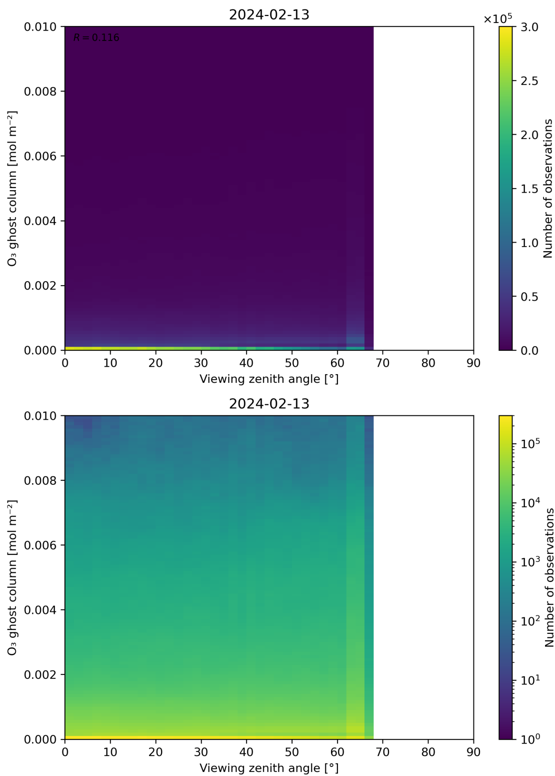
Figure 51: Scatter density plot of “Viewing zenith angle” against “O 3 ghost column” for 2024-02-12 to 2024-02-14.
