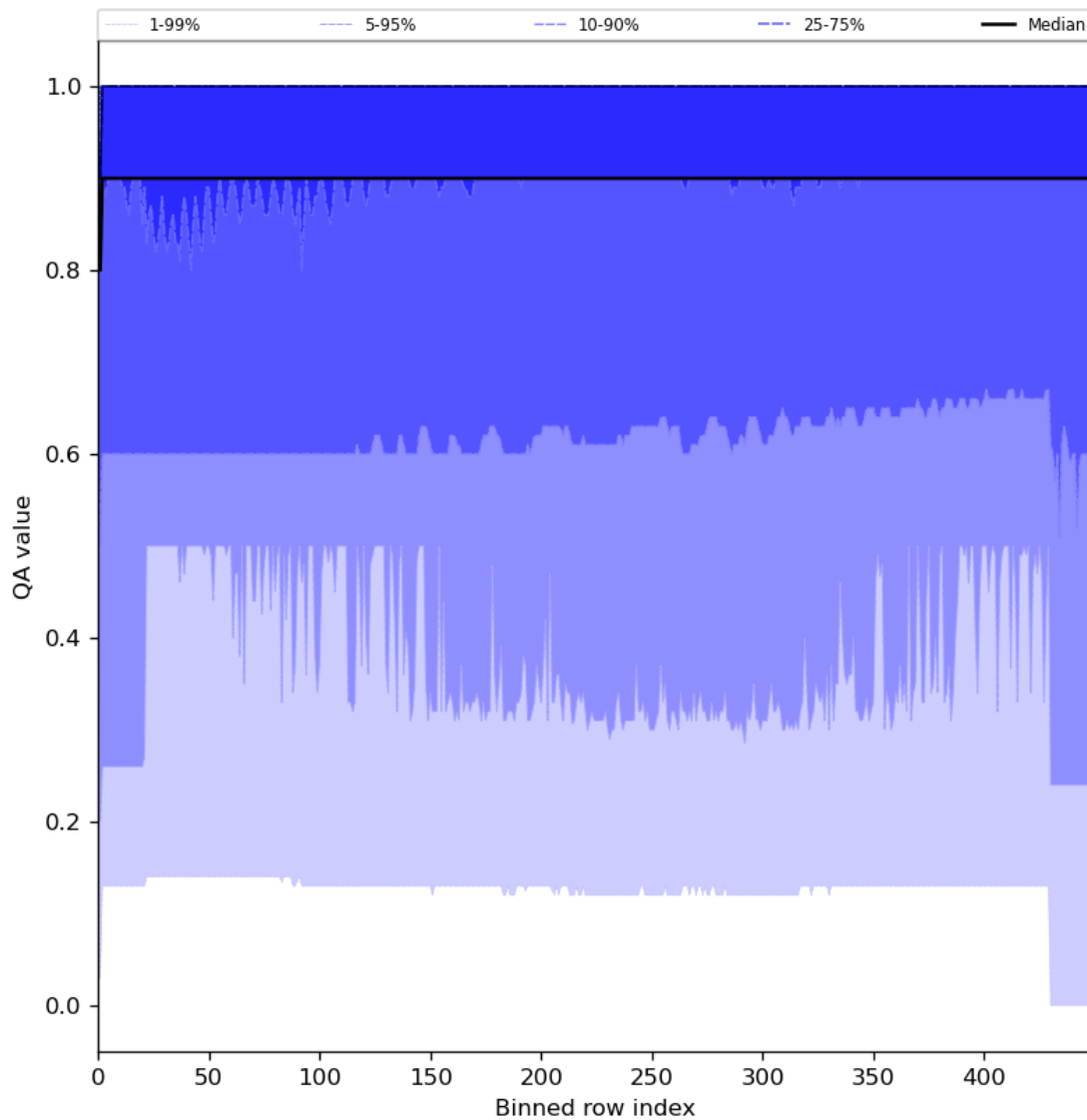
Figure 27: Along track statistics of “QA value” for 2024-02-12 to 2024-02-14
