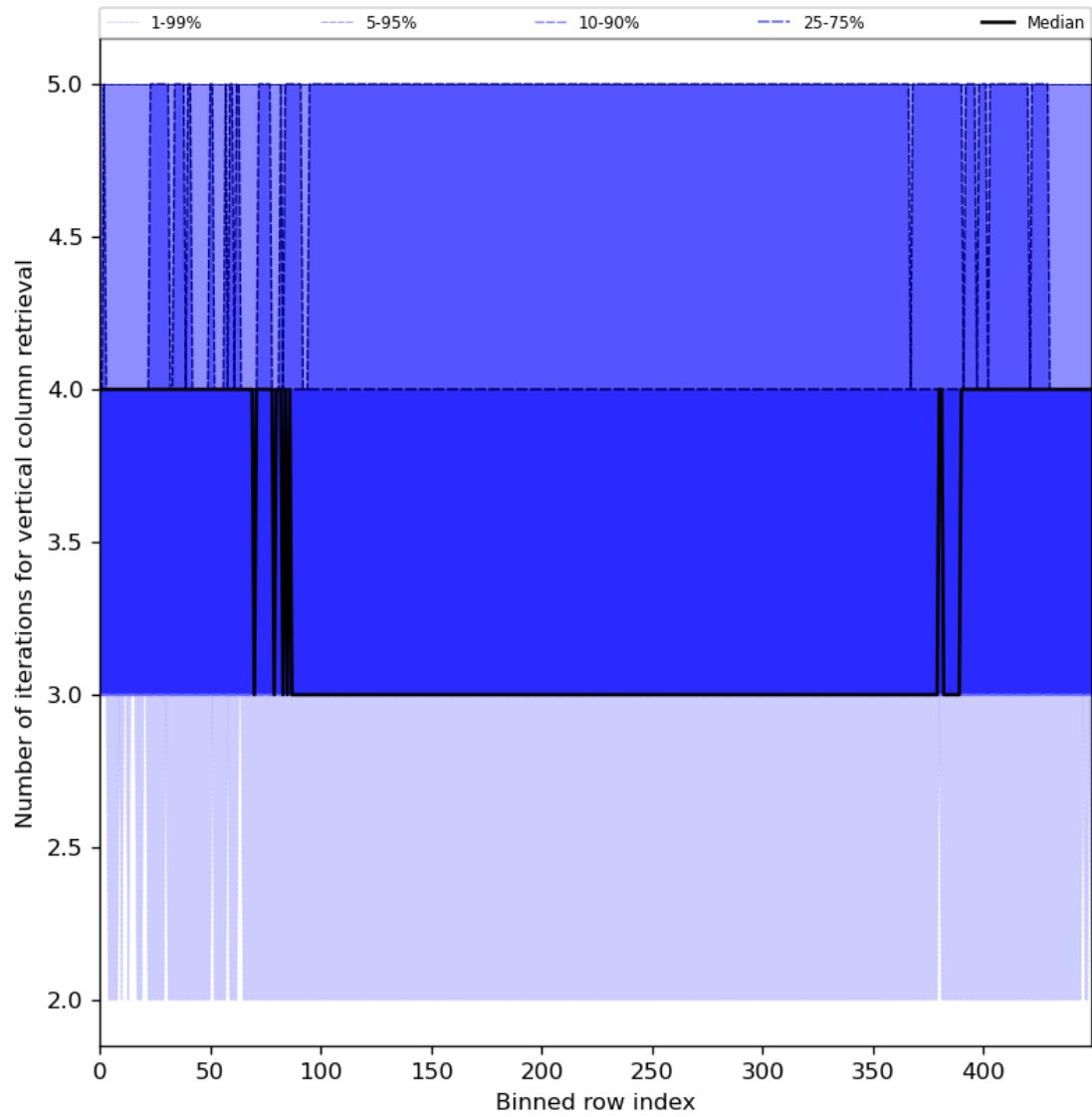
Figure 33: Along track statistics of “Number of iterations for vertical column retrieval” for 2024-02-12 to 2024-02-14
