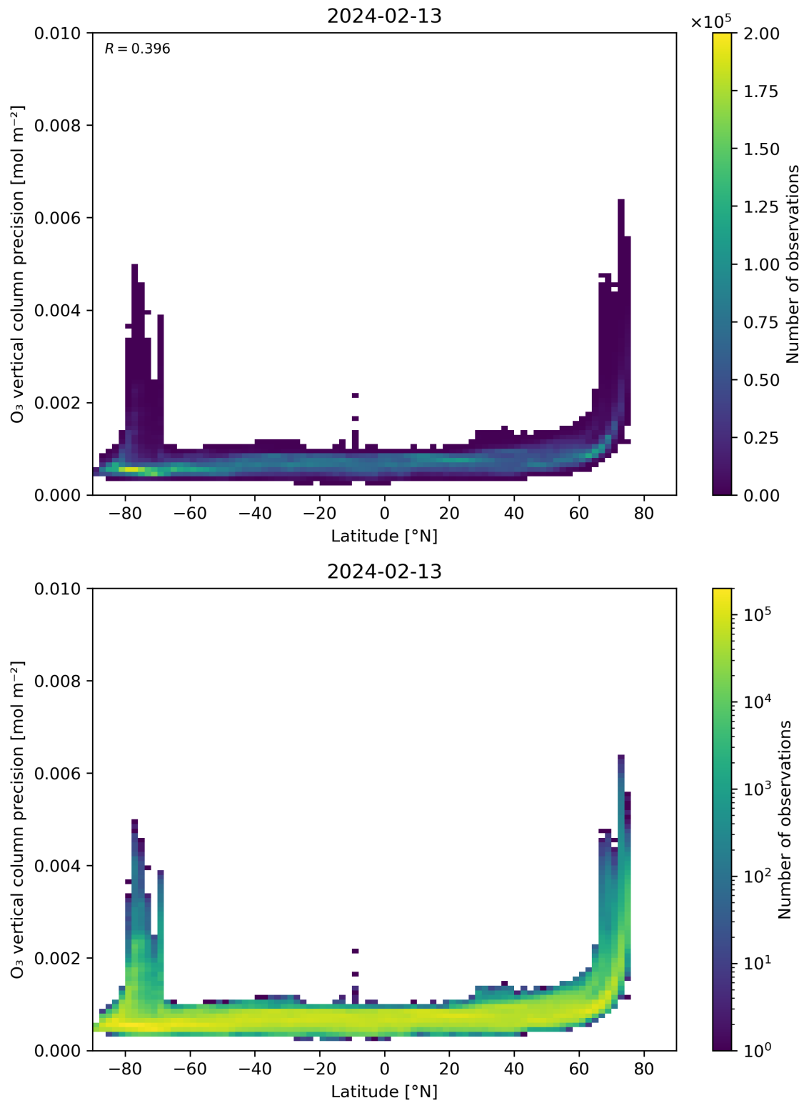
Figure 37: Scatter density plot of “Latitude” against “O 3 vertical column precision” for 2024-02-12 to 2024-02-14.
