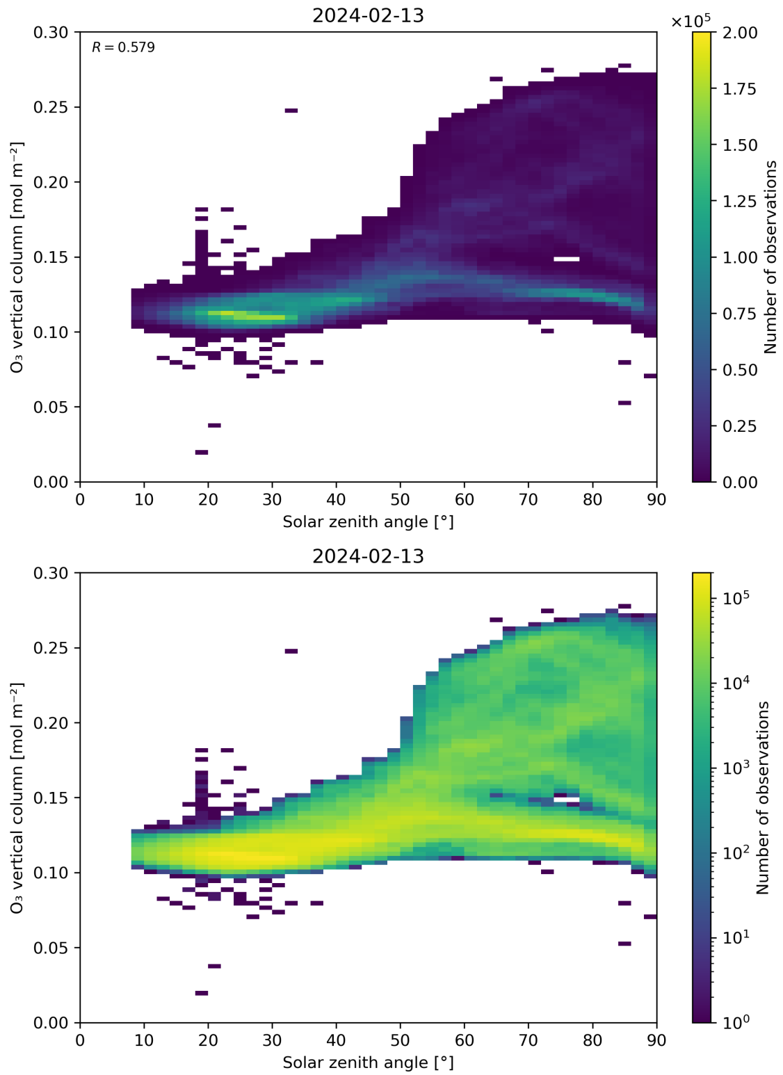
Figure 47: Scatter density plot of “Solar zenith angle” against “O 3 vertical column” for 2024-02-12 to 2024-02-14.
