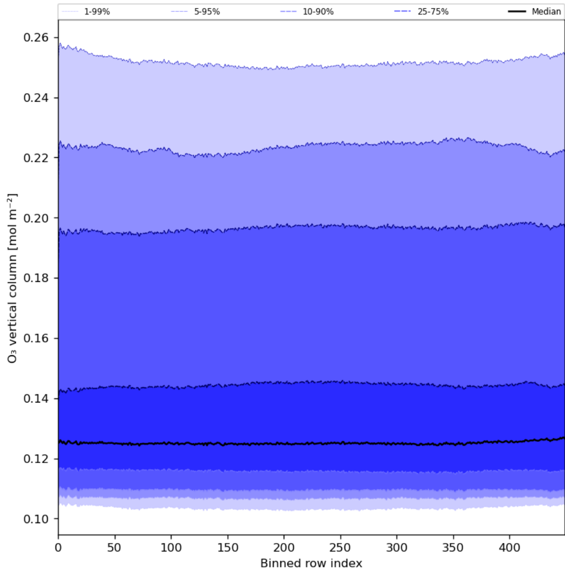
Figure 28: Along track statistics of “O 3 vertical column” for 2024-02-12 to 2024-02-14
