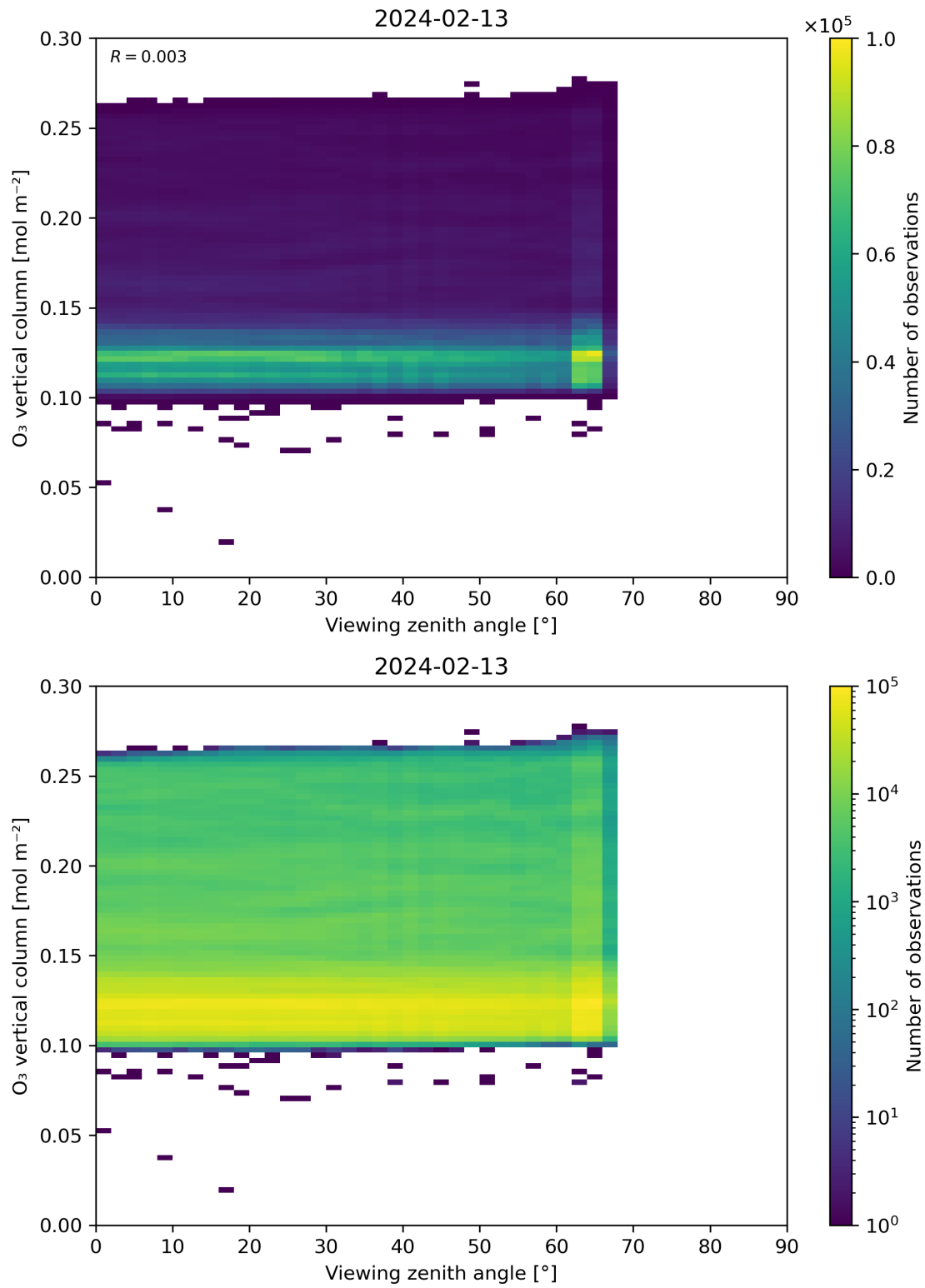
Figure 52: Scatter density plot of “Viewing zenith angle” against “O 3 vertical column” for 2024-02-12 to 2024-02-14.
