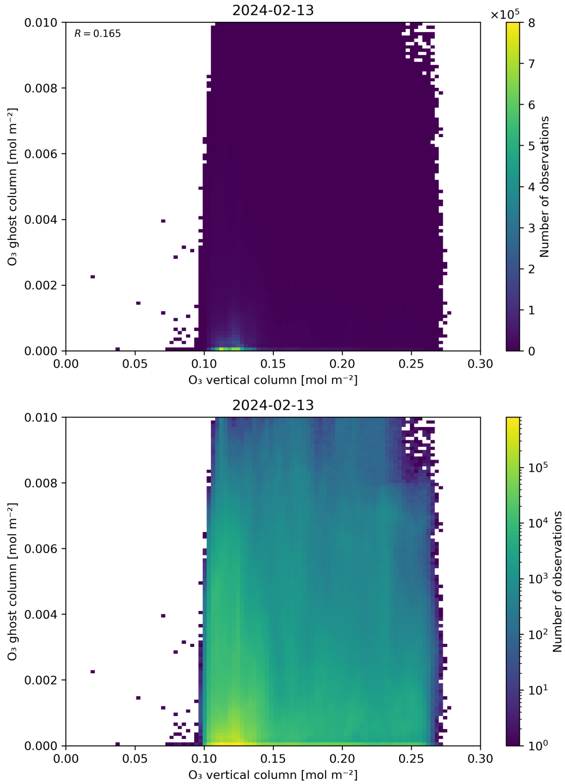
Figure 40: Scatter density plot of “O 3 vertical column” against “O 3 ghost column” for 2024-02-12 to 2024-02-14.
