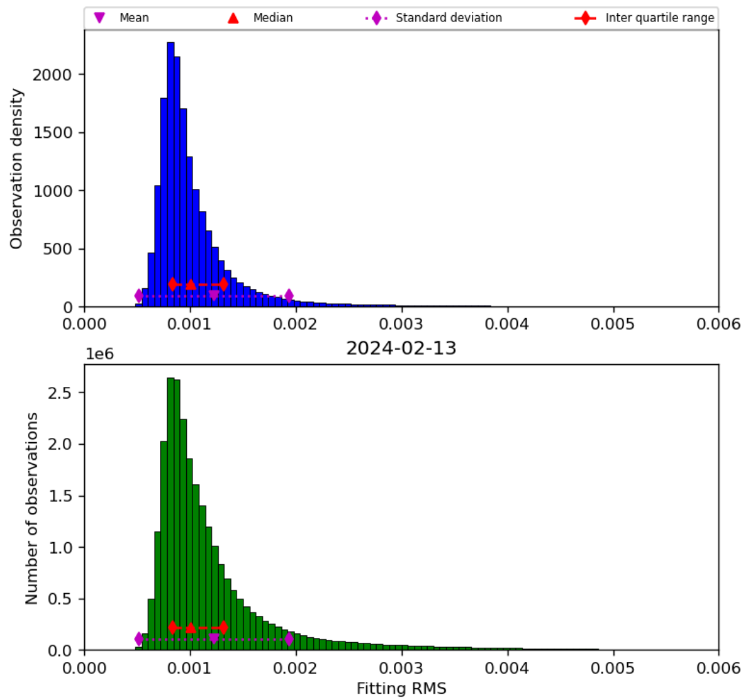
Figure 23: Histogram of “Fitting RMS” for 2024-02-12 to 2024-02-14
