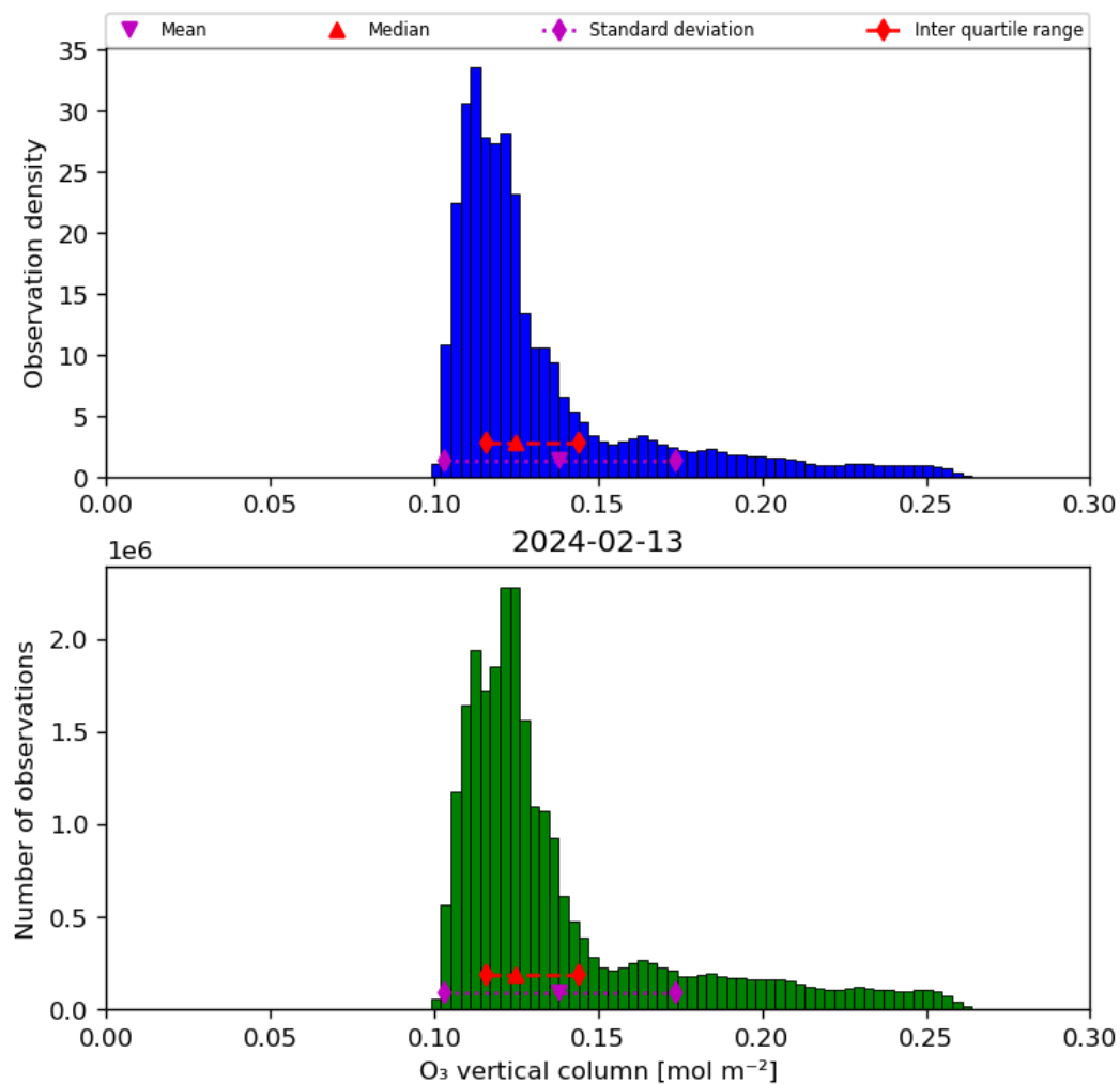
Figure 21: Histogram of “O 3 vertical column” for 2024-02-12 to 2024-02-14
