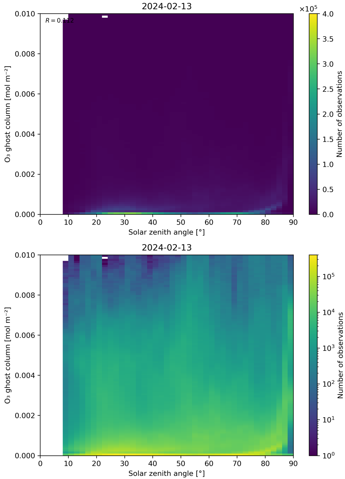
Figure 46: Scatter density plot of “Solar zenith angle” against “O 3 ghost column” for 2024-02-12 to 2024-02-14.
