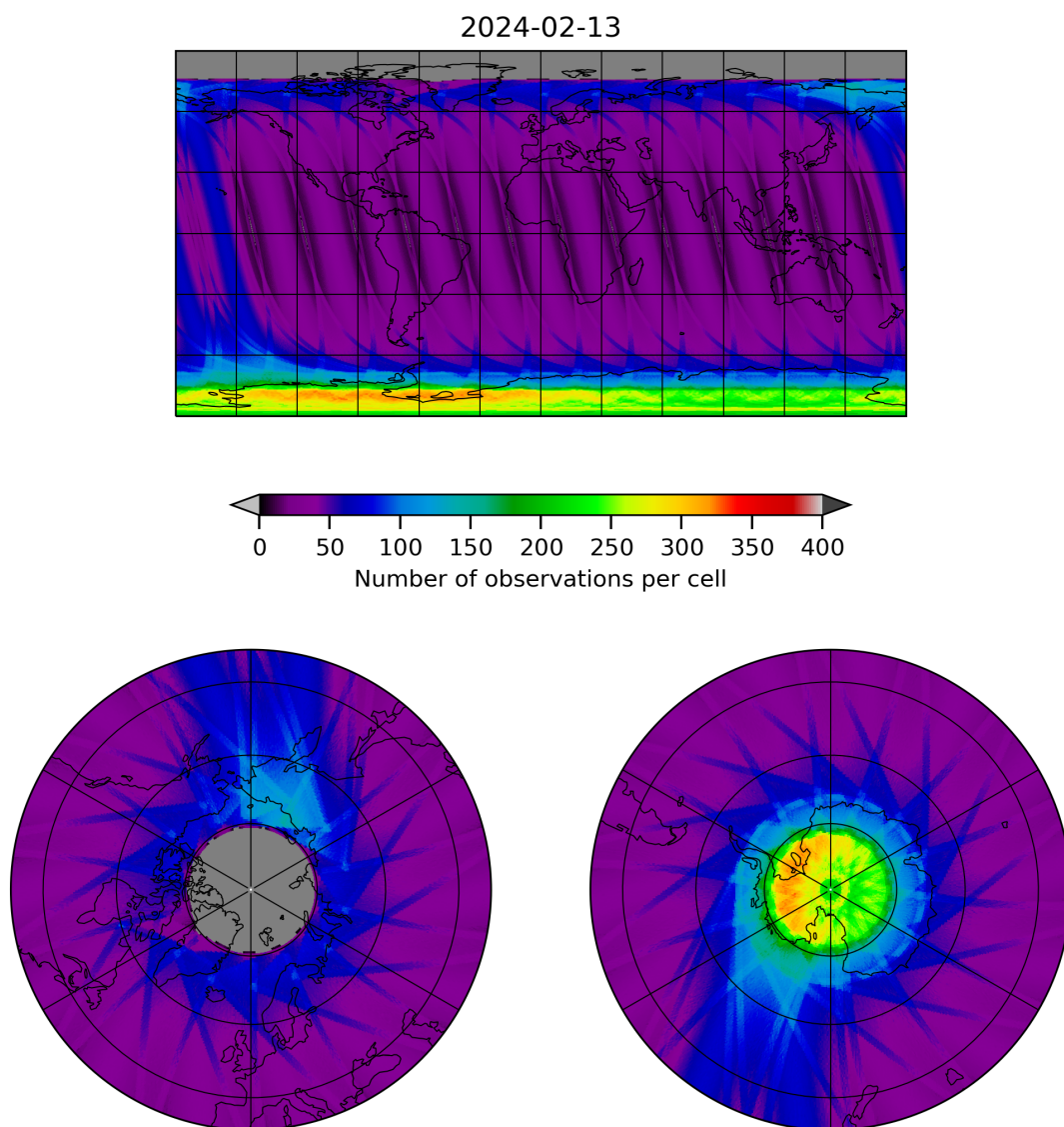
Figure 12: Map of the number of observations for 2024-02-12 to 2024-02-14
