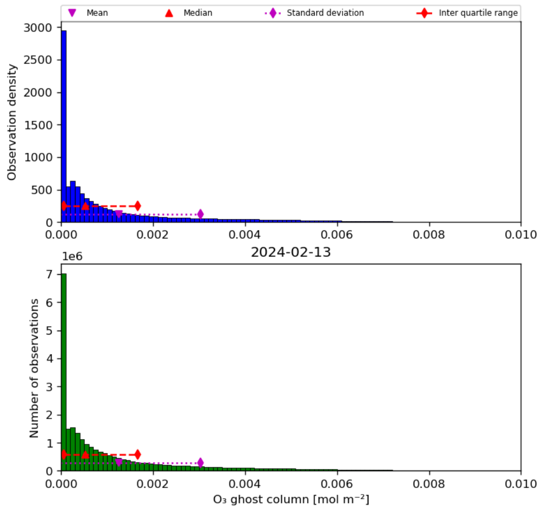
Figure 25: Histogram of “O 3 ghost column” for 2024-02-12 to 2024-02-14
