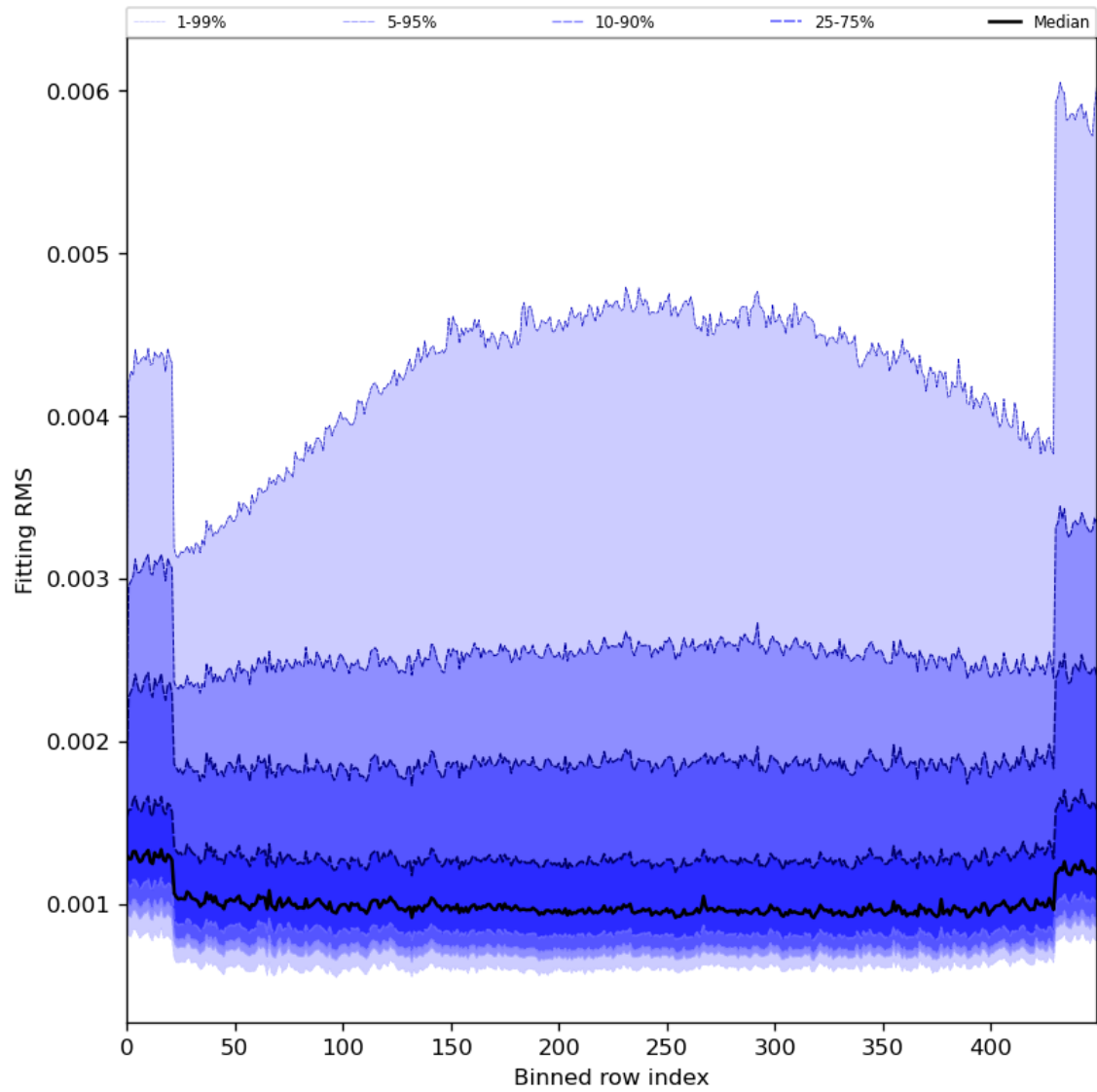
Figure 30: Along track statistics of “Fitting RMS” for 2024-02-12 to 2024-02-14
