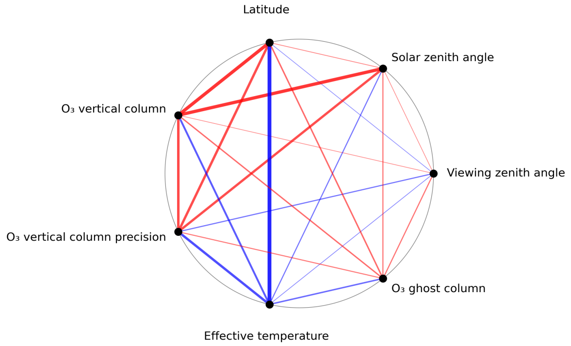
Figure 1: Map of correlation graph for 2024-02-12 to 2024-02-14.
