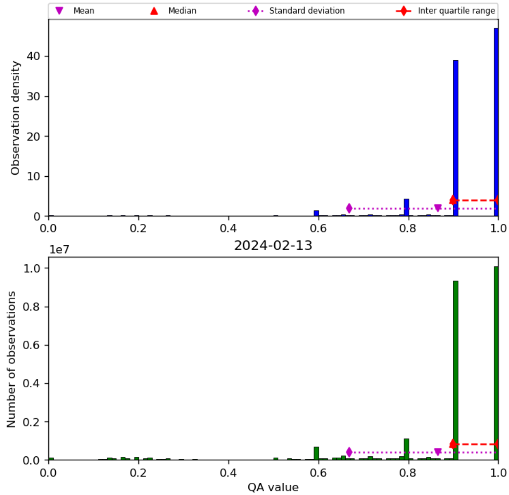
Figure 20: Histogram of “QA value” for 2024-02-12 to 2024-02-14
