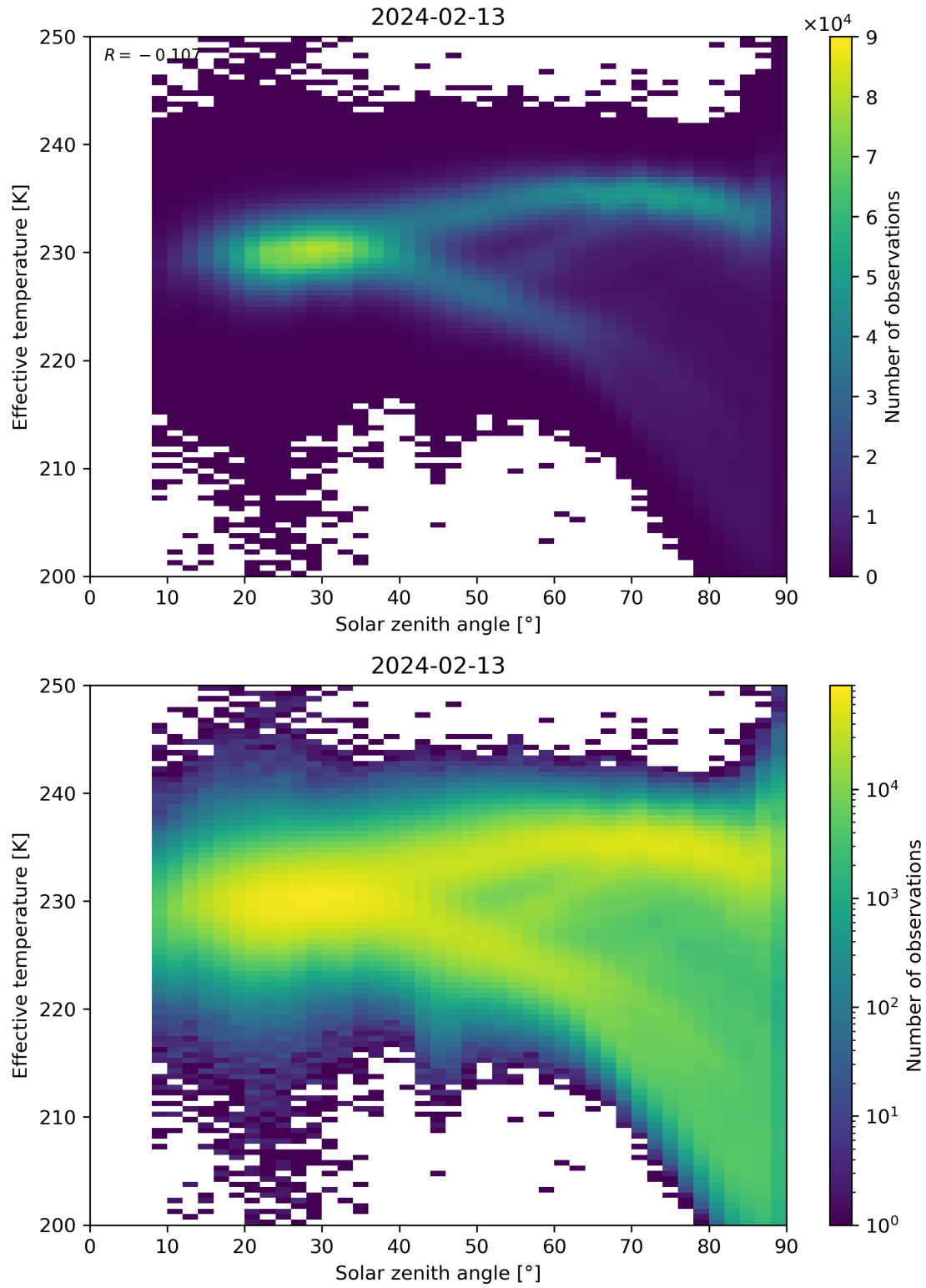
Figure 45: Scatter density plot of “Solar zenith angle” against “Effective temperature” for 2024-02-12 to 2024-02-14.
