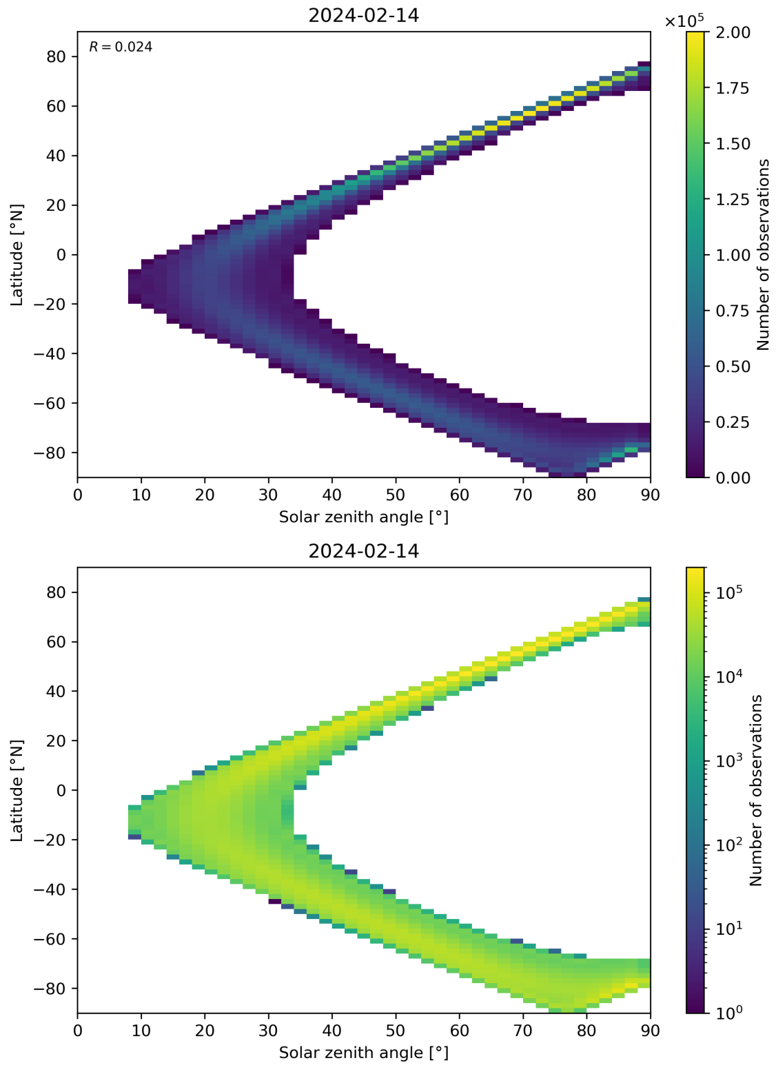
Figure 44: Scatter density plot of “Solar zenith angle” against “Latitude” for 2024-02-13 to 2024-02-15.
