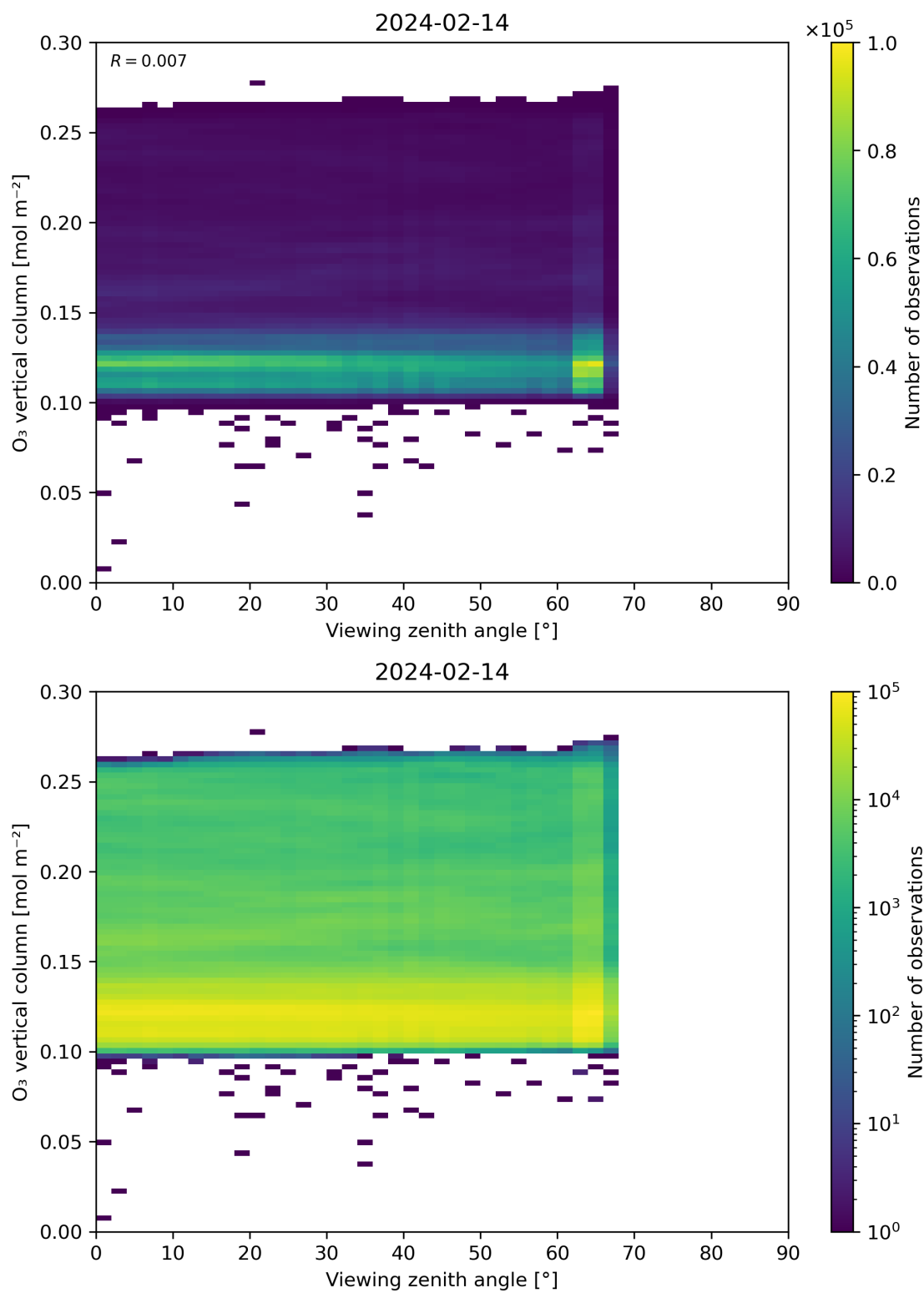
Figure 52: Scatter density plot of “Viewing zenith angle” against “O 3 vertical column” for 2024-02-13 to 2024-02-15.
