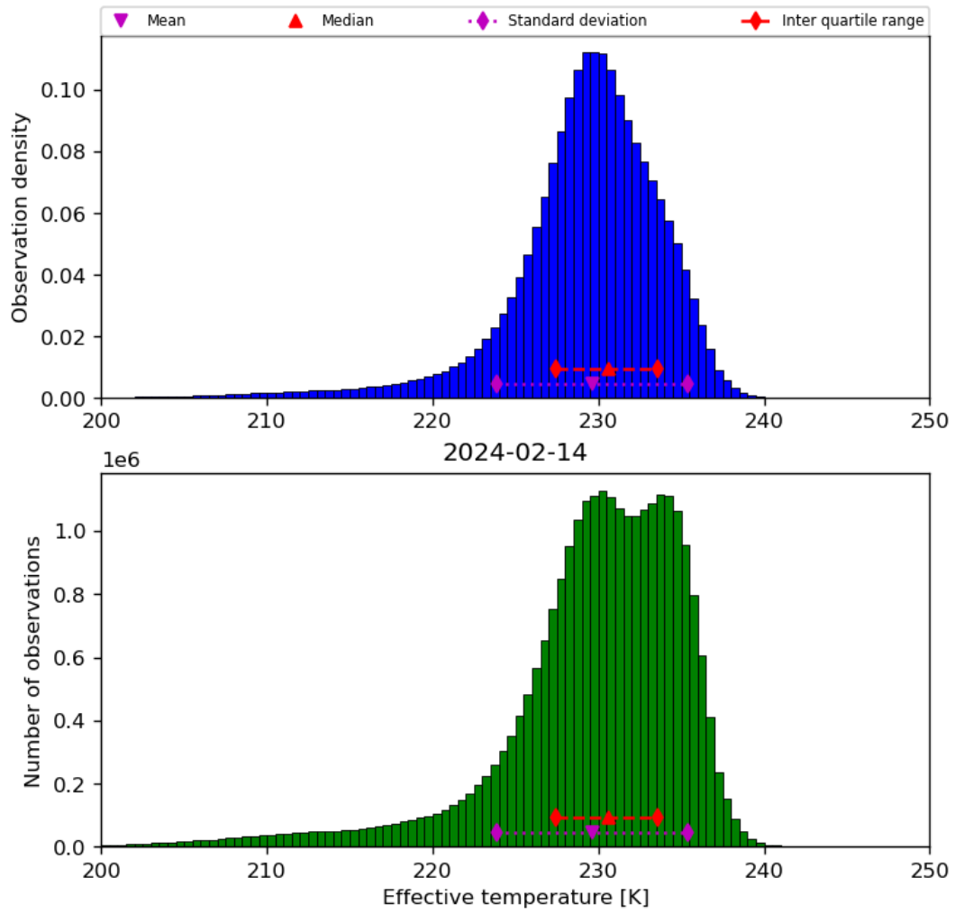
Figure 24: Histogram of “Effective temperature” for 2024-02-13 to 2024-02-15
