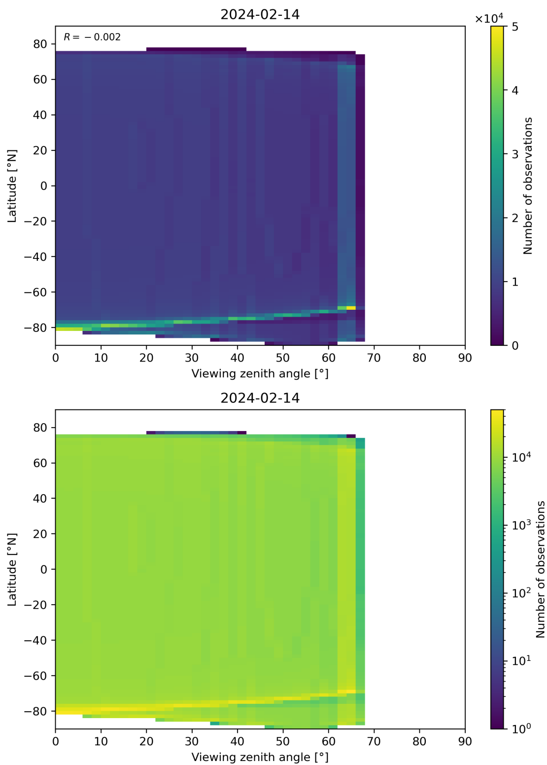
Figure 49: Scatter density plot of “Viewing zenith angle” against “Latitude” for 2024-02-13 to 2024-02-15.
