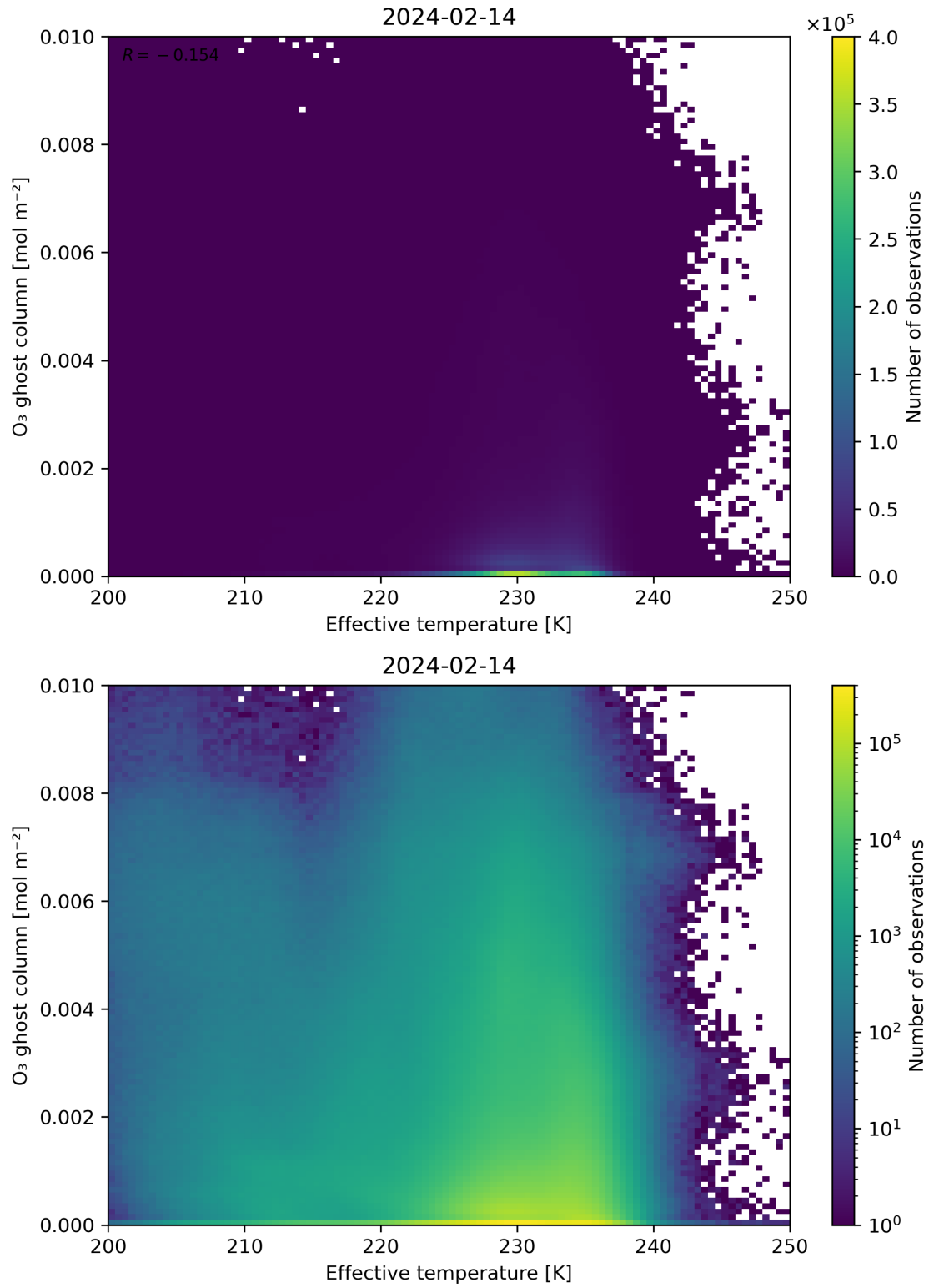
Figure 38: Scatter density plot of “Effective temperature” against “O 3 ghost column” for 2024-02-13 to 2024-02-15.
