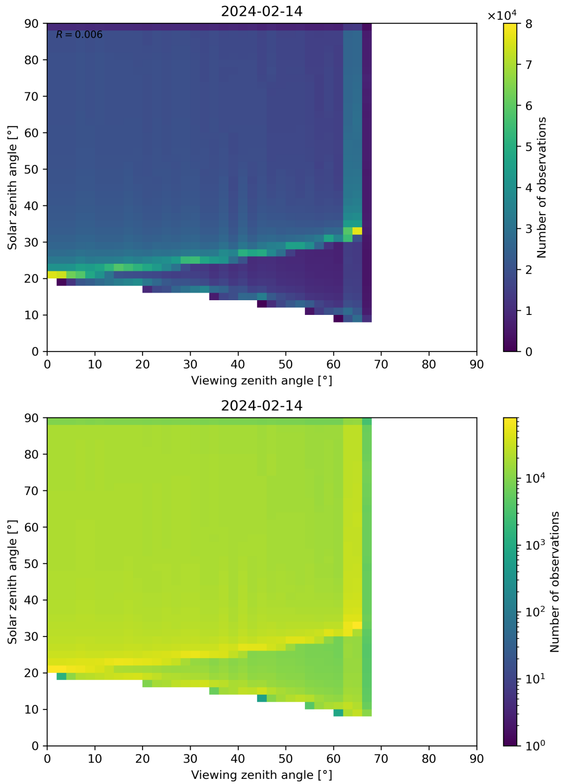
Figure 54: Scatter density plot of “Viewing zenith angle” against “Solar zenith angle” for 2024-02-13 to 2024-02-15.
