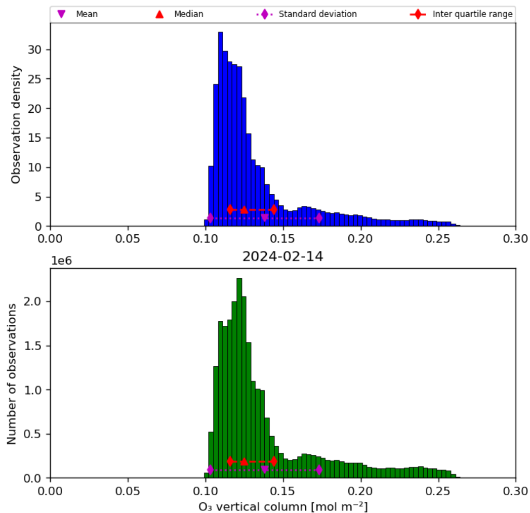
Figure 21: Histogram of “O 3 vertical column” for 2024-02-13 to 2024-02-15
