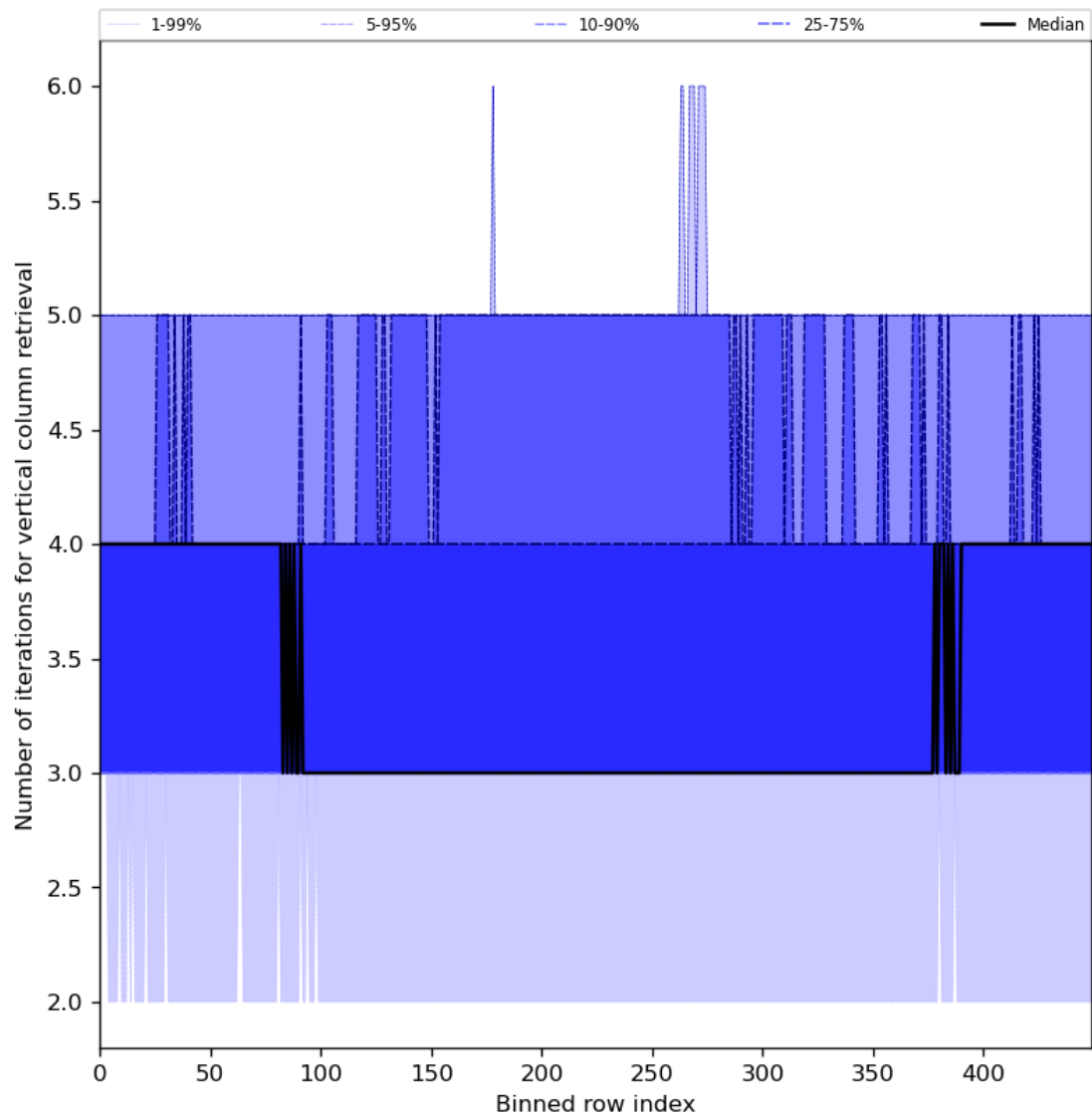
Figure 33: Along track statistics of “Number of iterations for vertical column retrieval” for 2024-02-13 to 2024-02-15
