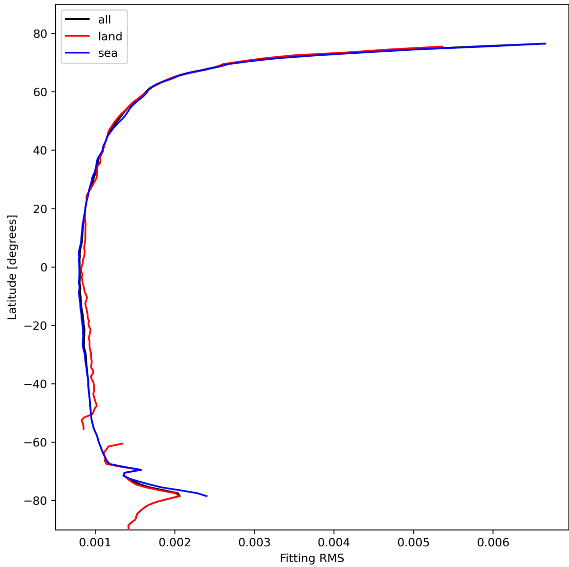
Figure 16: Zonal average of “Fitting RMS” for 2024-02-13 to 2024-02-15.
