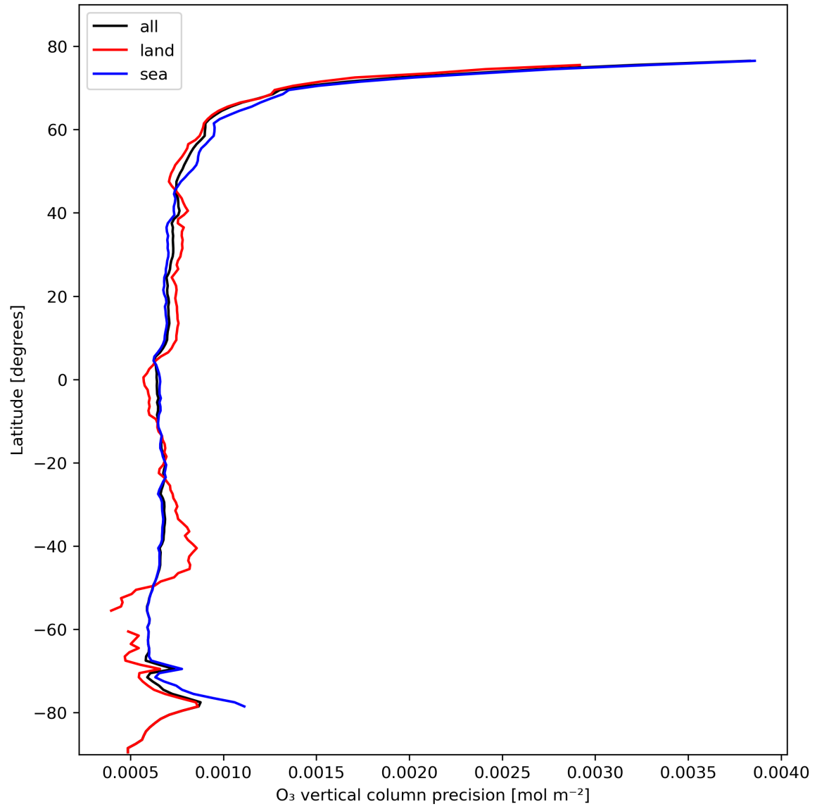
Figure 15: Zonal average of “O 3 vertical column precision” for 2024-02-13 to 2024-02-15.
