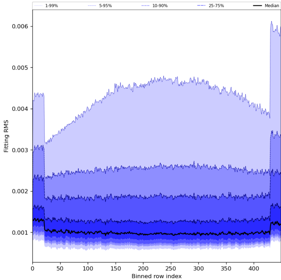
Figure 30: Along track statistics of “Fitting RMS” for 2024-02-13 to 2024-02-15
