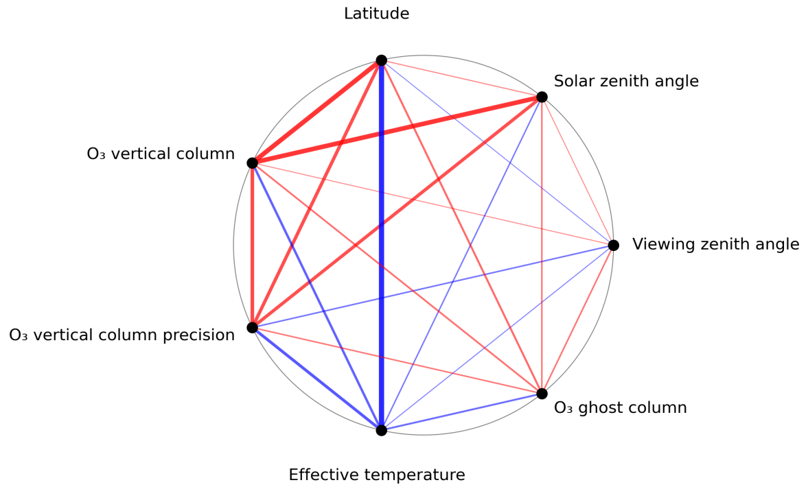
Figure 1: Map of correlation graph for 2024-02-13 to 2024-02-15.
