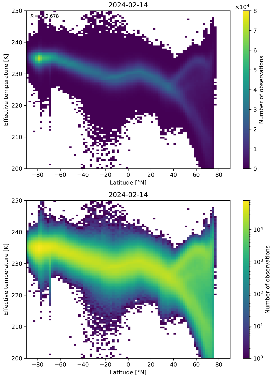
Figure 34: Scatter density plot of “Latitude” against “Effective temperature” for 2024-02-13 to 2024-02-15.
