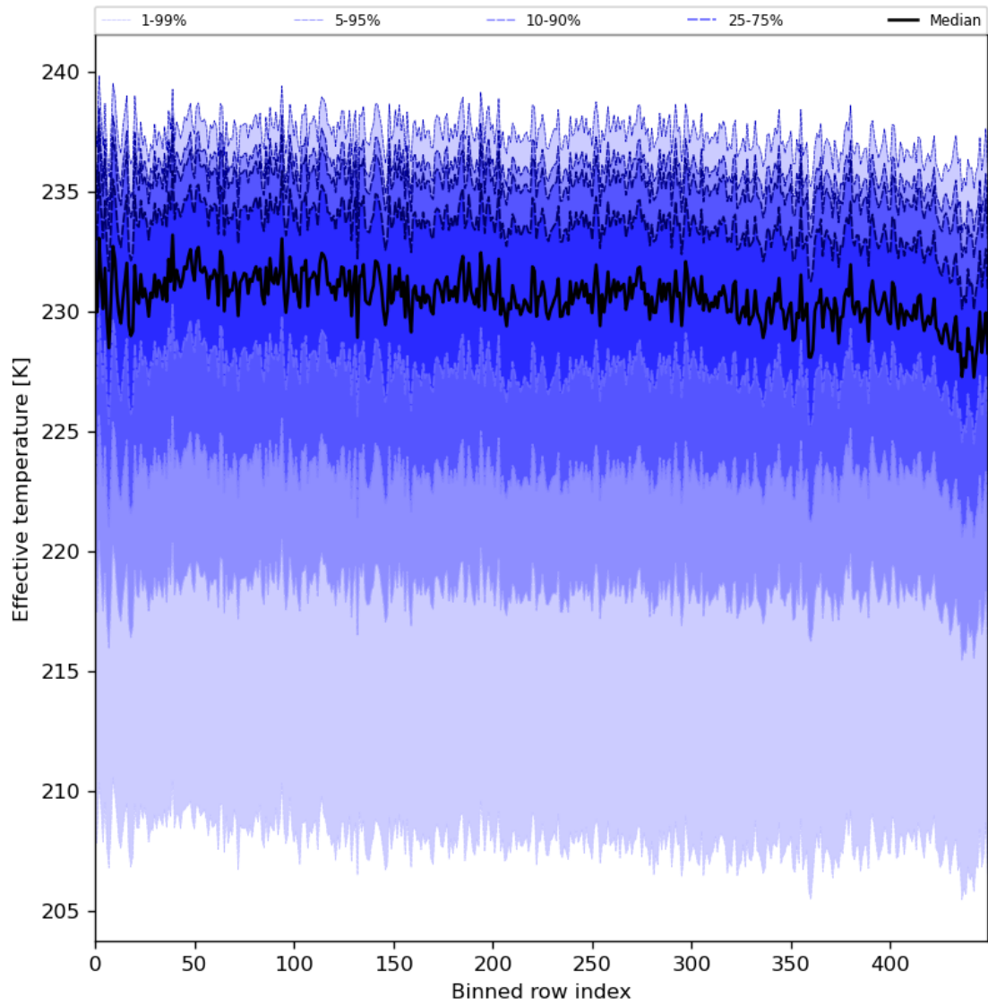
Figure 31: Along track statistics of “Effective temperature” for 2024-02-13 to 2024-02-15
