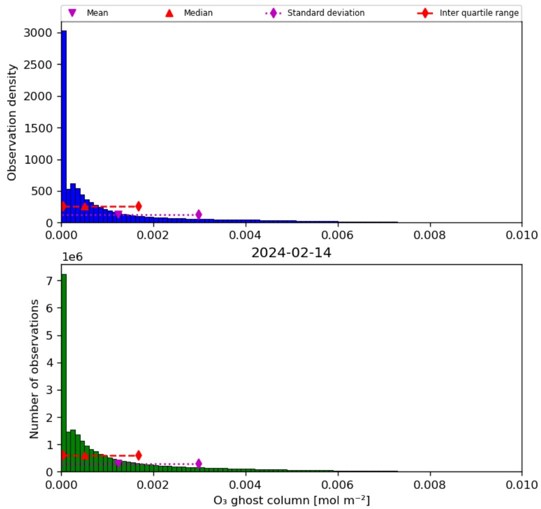
Figure 25: Histogram of “O 3 ghost column” for 2024-02-13 to 2024-02-15
