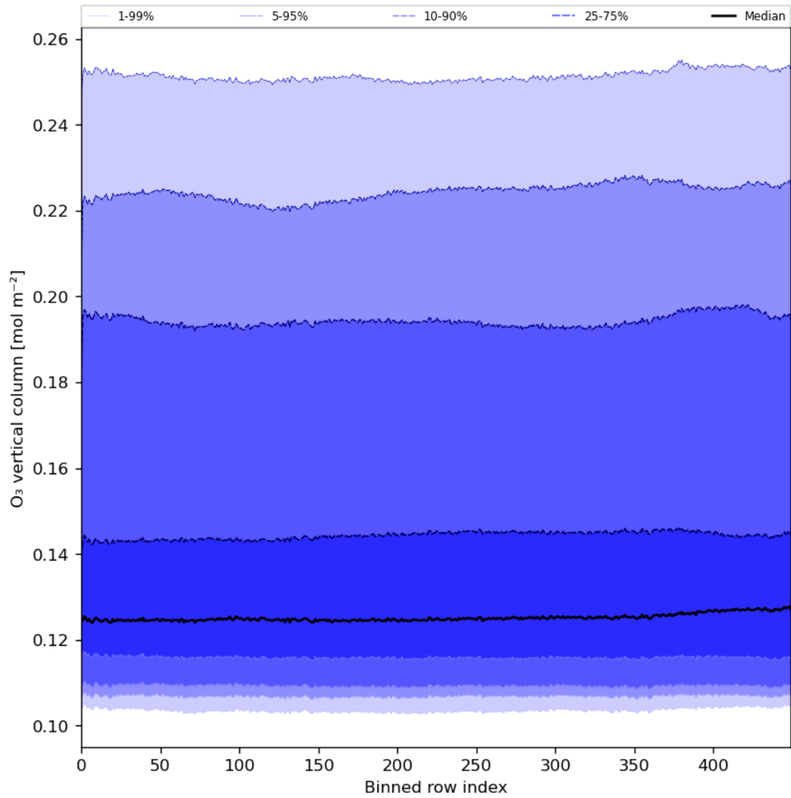
Figure 28: Along track statistics of “O 3 vertical column” for 2024-02-13 to 2024-02-15
