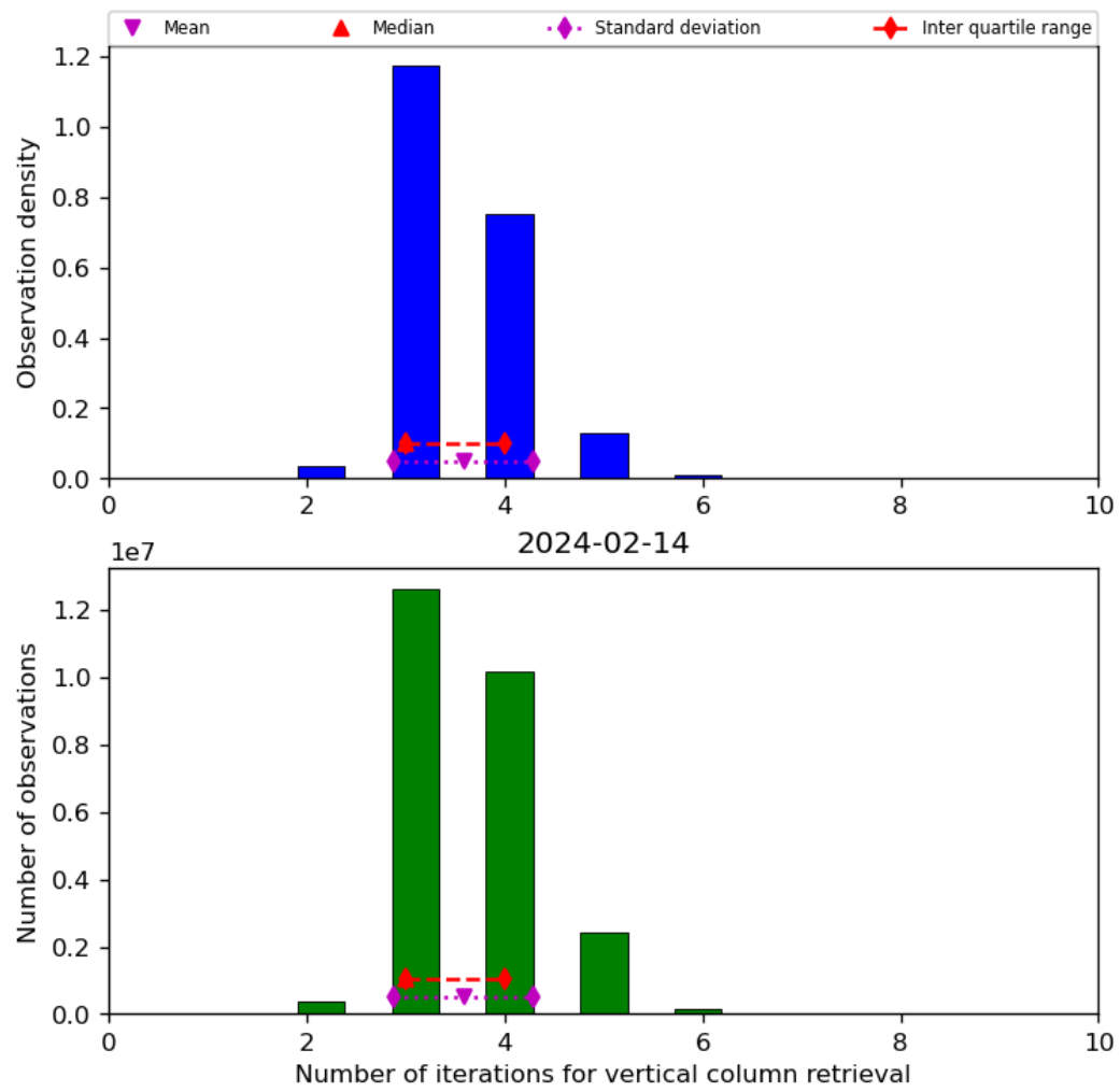
Figure 26: Histogram of “Number of iterations for vertical column retrieval” for 2024-02-13 to 2024-02-15
