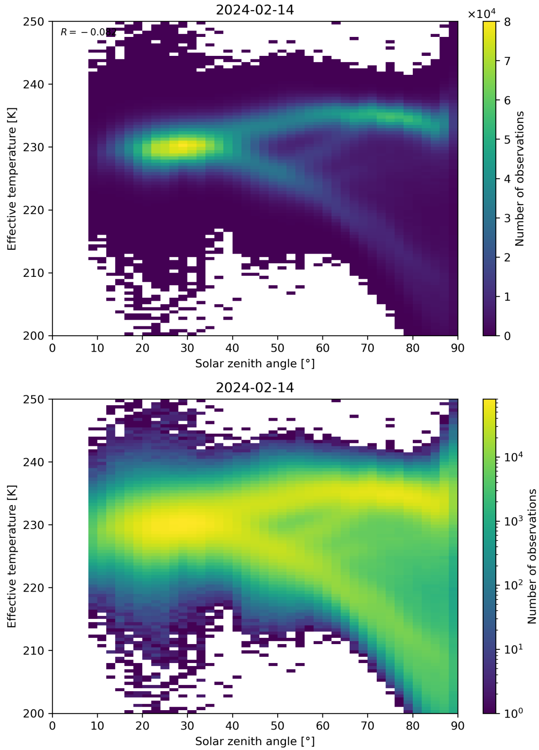
Figure 45: Scatter density plot of “Solar zenith angle” against “Effective temperature” for 2024-02-13 to 2024-02-15.
