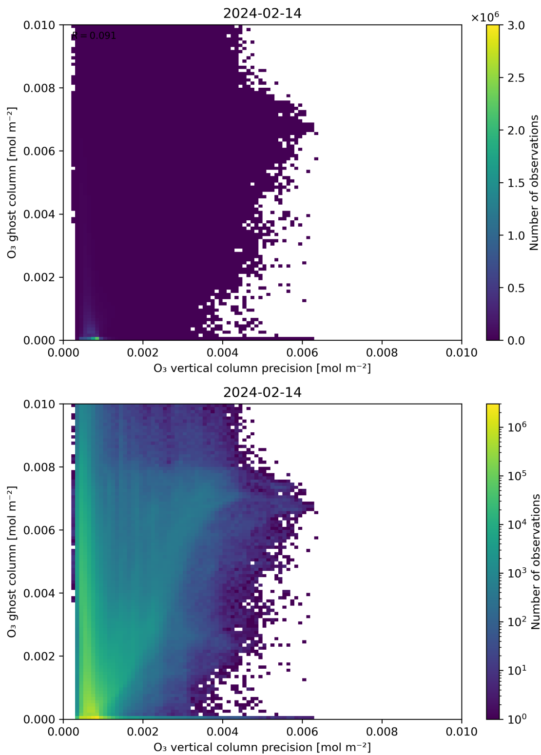
Figure 43: Scatter density plot of “O 3 vertical column precision” against “O 3 ghost column” for 2024-02-13 to 2024-02-15.
