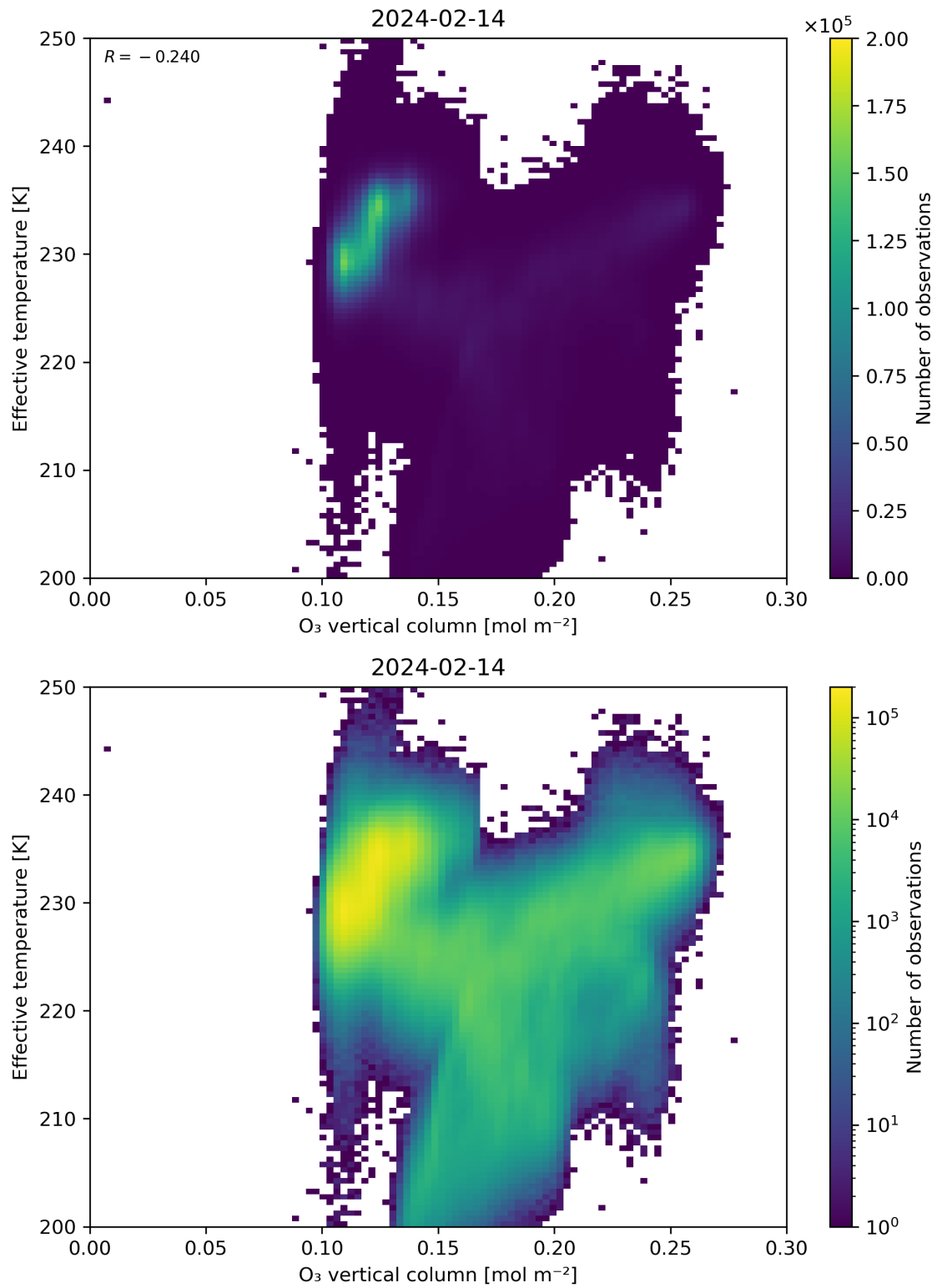
Figure 39: Scatter density plot of “O 3 vertical column” against “Effective temperature” for 2024-02-13 to 2024-02-15.
