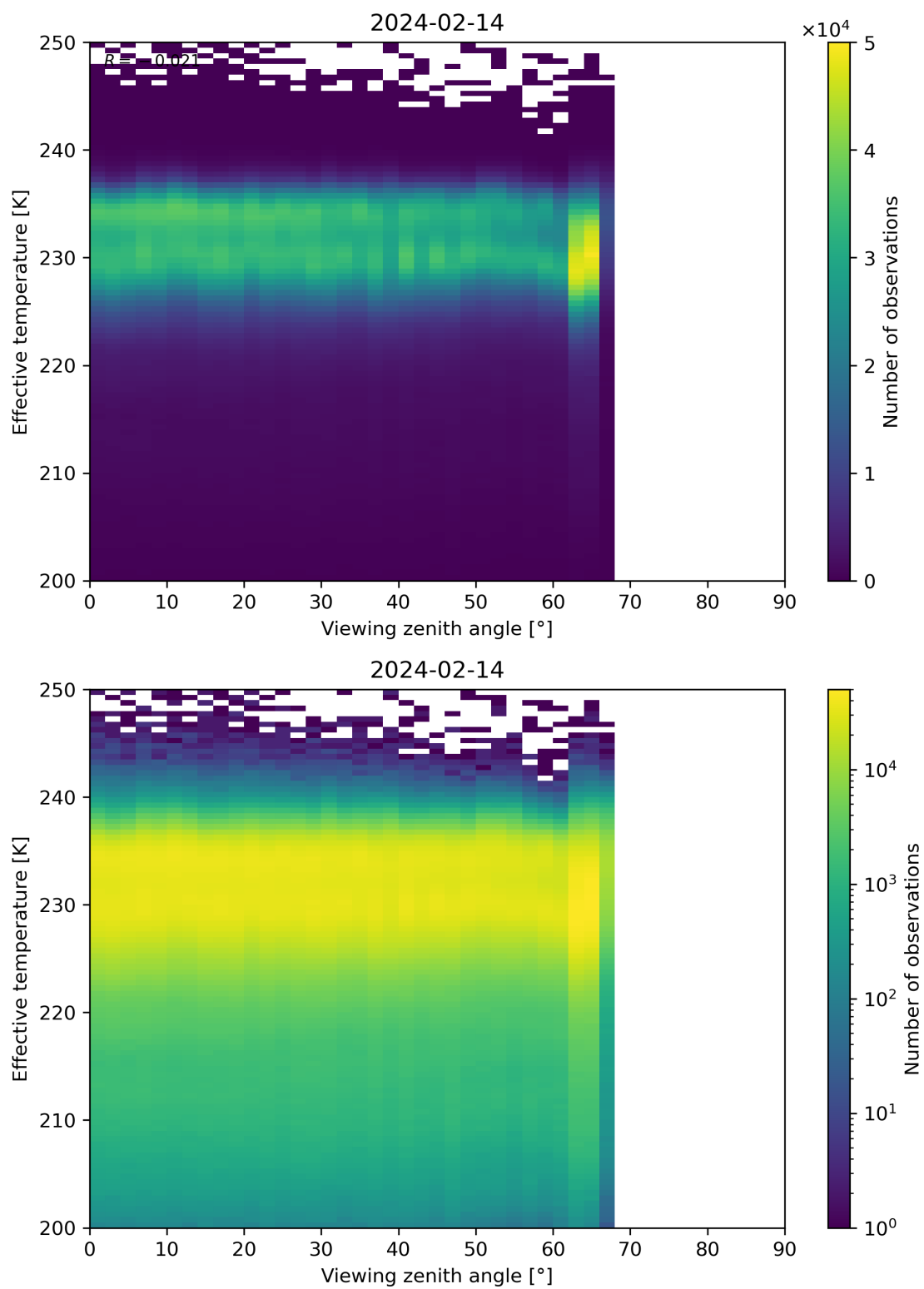
Figure 50: Scatter density plot of “Viewing zenith angle” against “Effective temperature” for 2024-02-13 to 2024-02-15.
