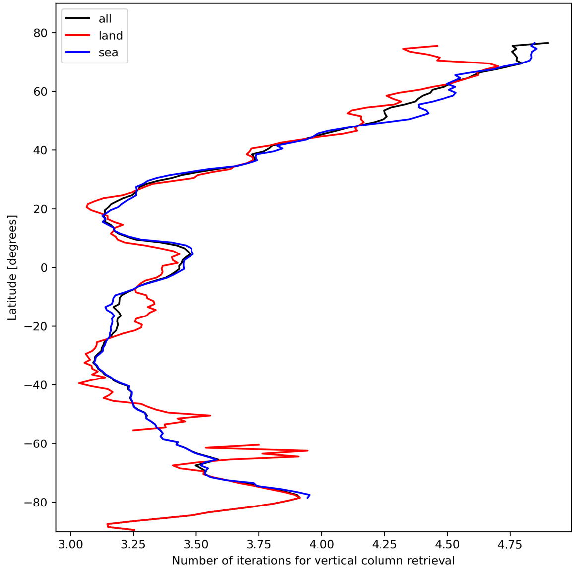
Figure 19: Zonal average of “Number of iterations for vertical column retrieval” for 2024-02-13 to 2024-02-15.
