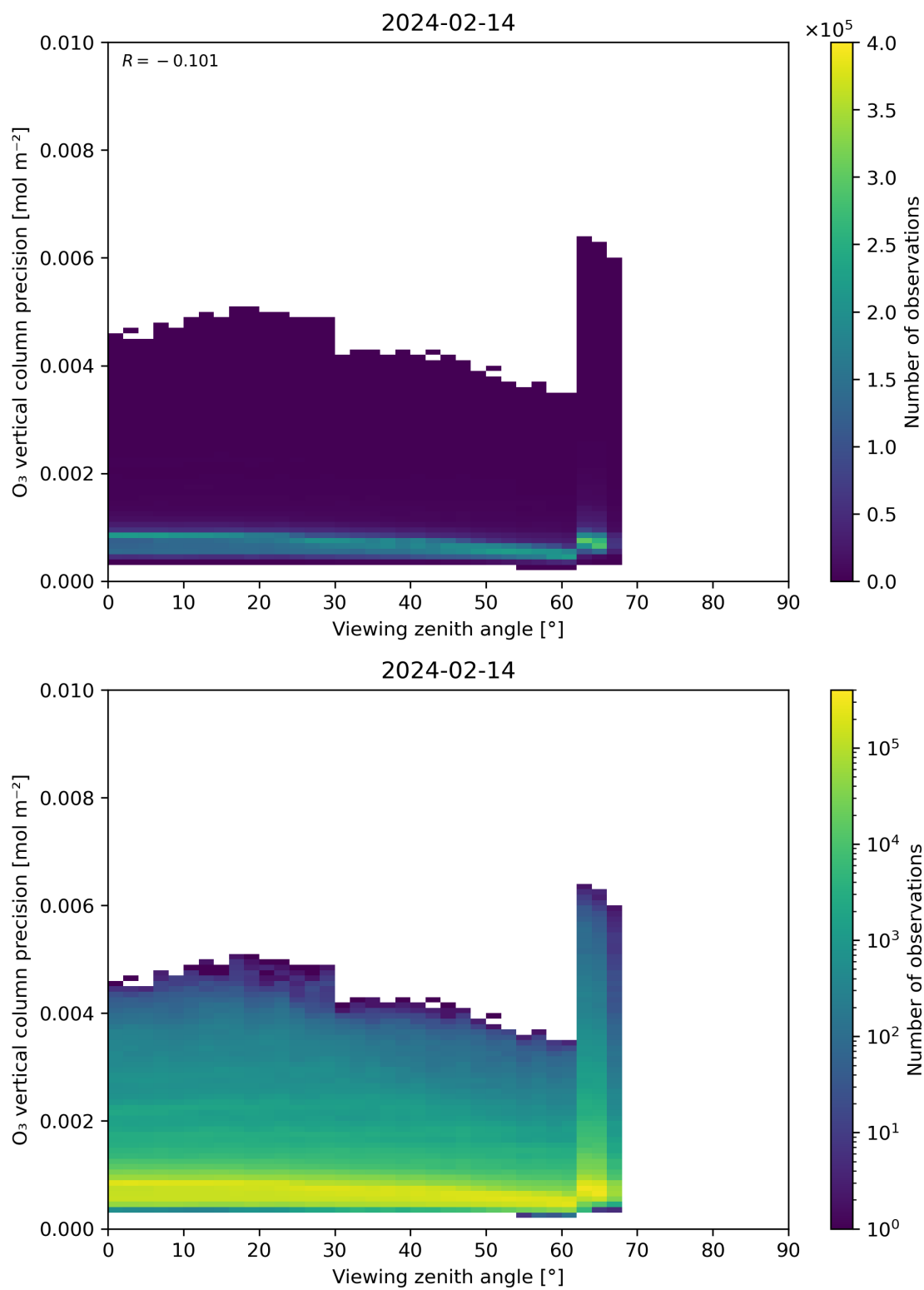
Figure 53: Scatter density plot of “Viewing zenith angle” against “O 3 vertical column precision” for 2024-02-13 to 2024-02-15.
