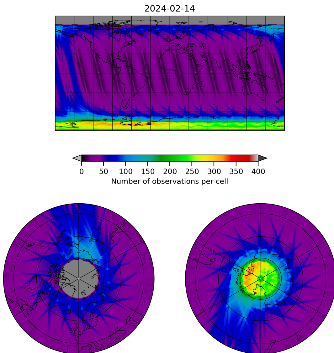
Figure 12: Map of the number of observations for 2024-02-13 to 2024-02-15
