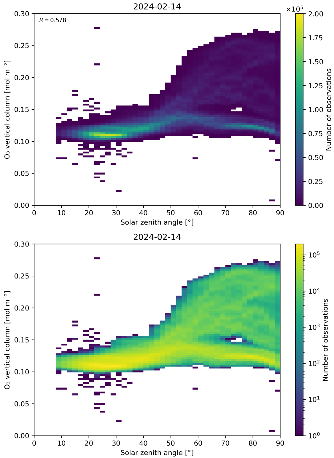
Figure 47: Scatter density plot of “Solar zenith angle” against “O 3 vertical column” for 2024-02-13 to 2024-02-15.
