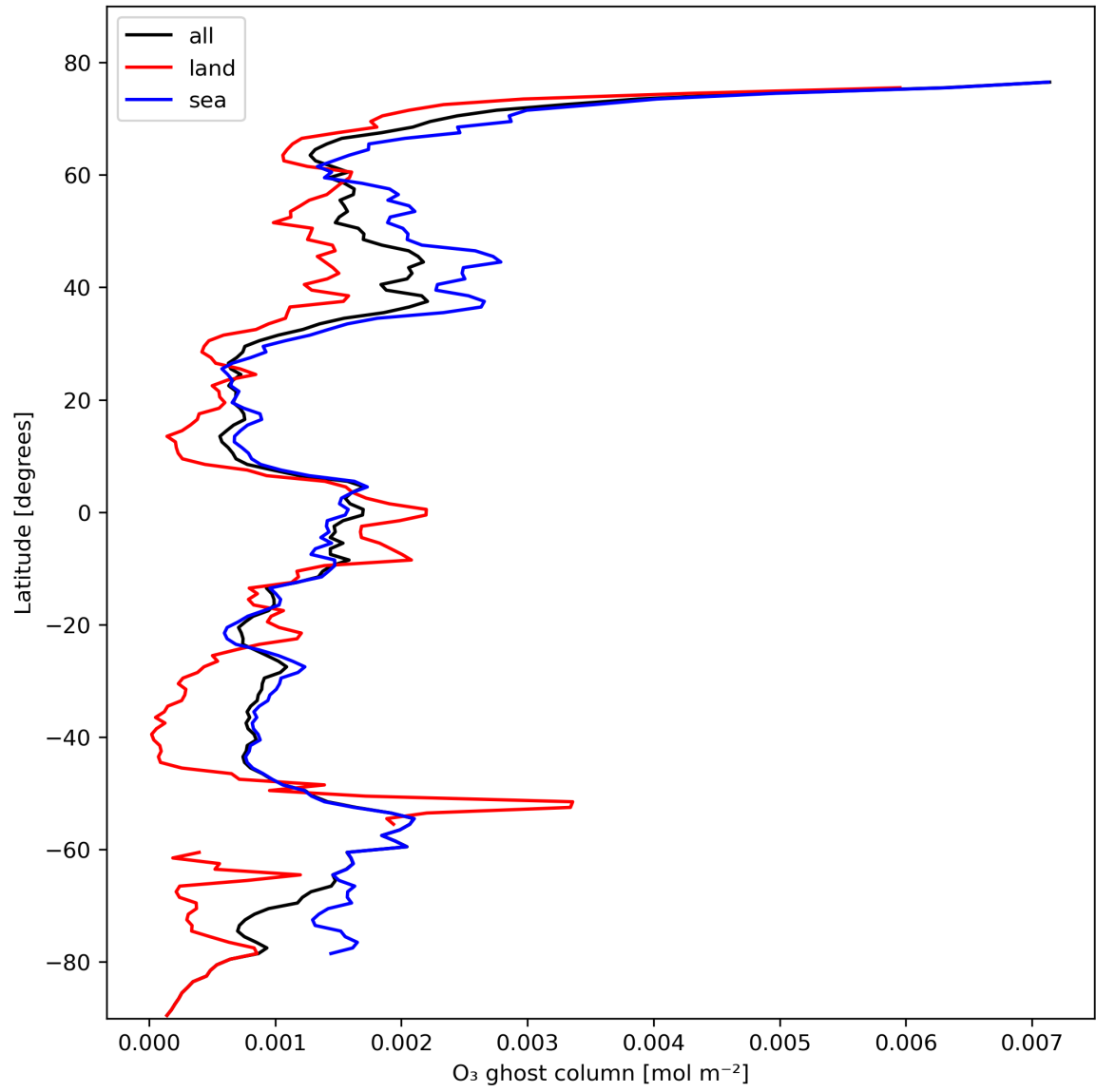
Figure 18: Zonal average of “O 3 ghost column” for 2024-02-13 to 2024-02-15.
