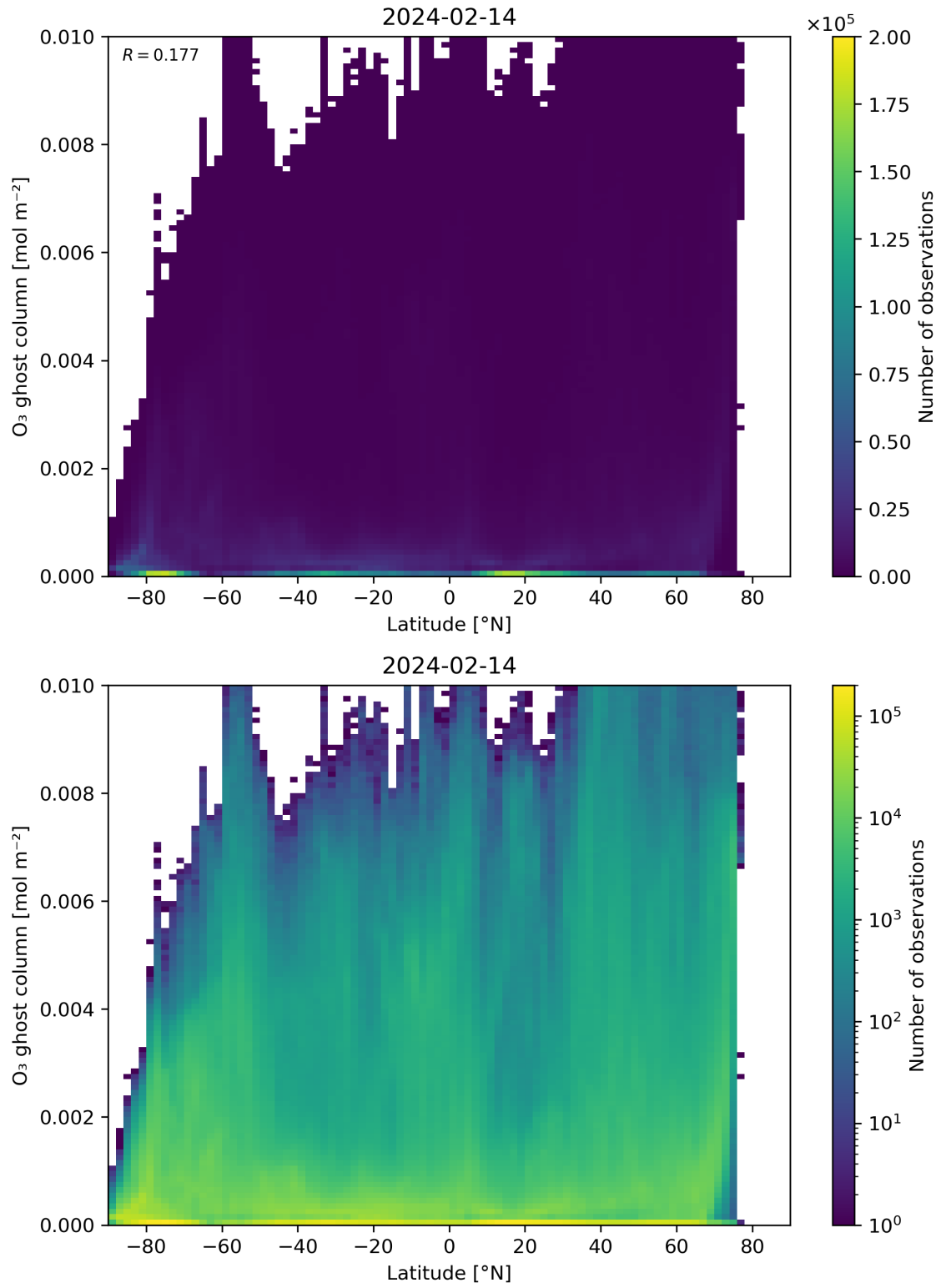
Figure 35: Scatter density plot of “Latitude” against “O 3 ghost column” for 2024-02-13 to 2024-02-15.
