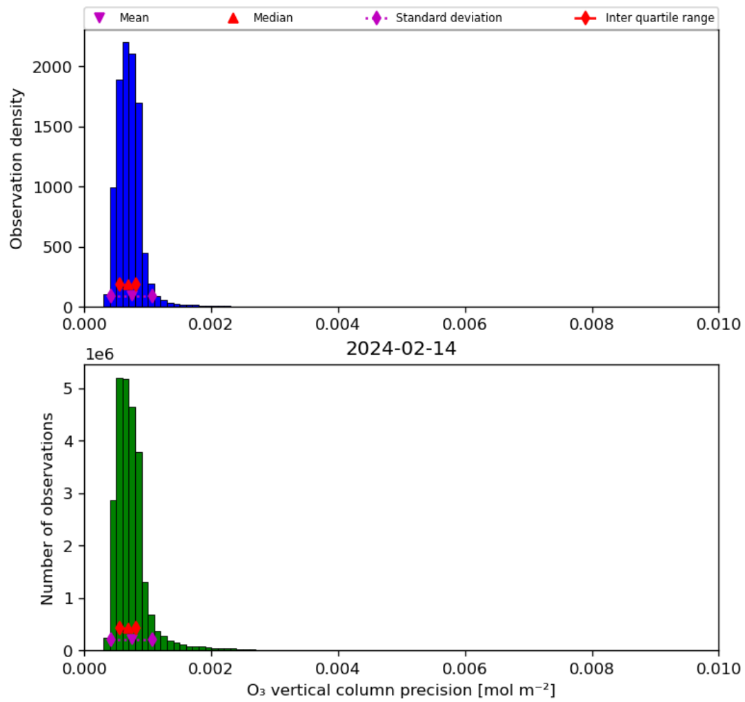
Figure 22: Histogram of “O 3 vertical column precision” for 2024-02-13 to 2024-02-15
