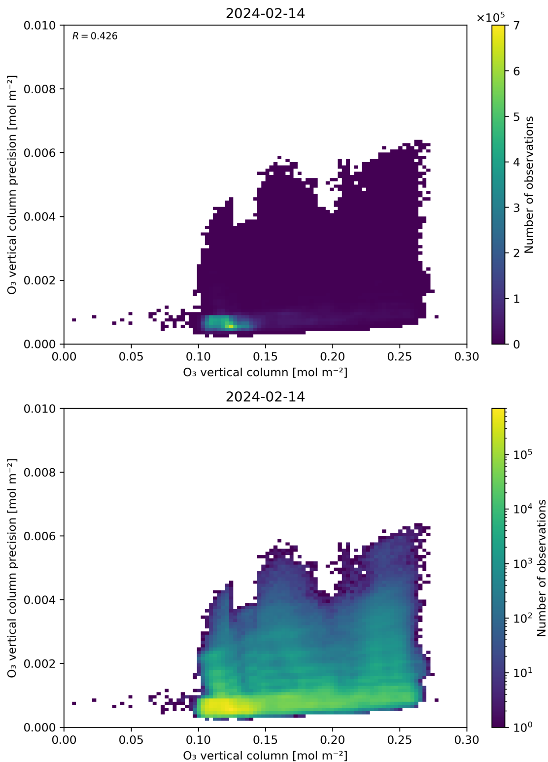
Figure 41: Scatter density plot of “O 3 vertical column” against “O 3 vertical column precision” for 2024-02-13 to 2024-02-15.
