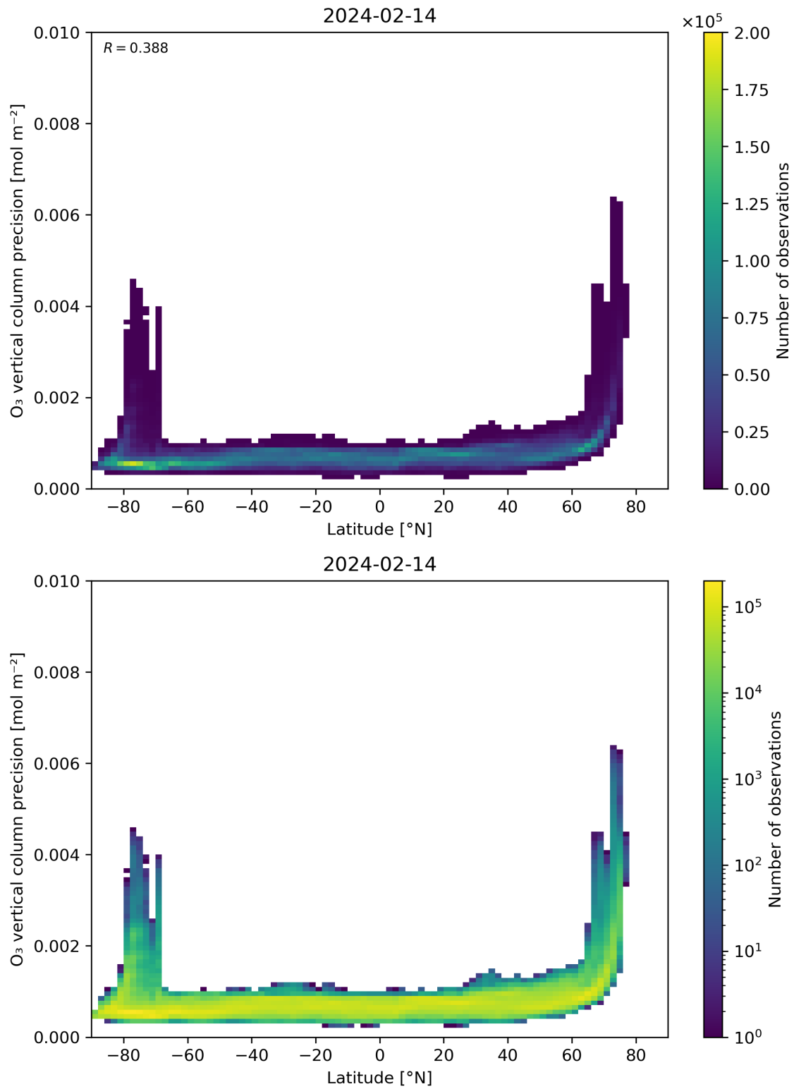
Figure 37: Scatter density plot of “Latitude” against “O 3 vertical column precision” for 2024-02-13 to 2024-02-15.
