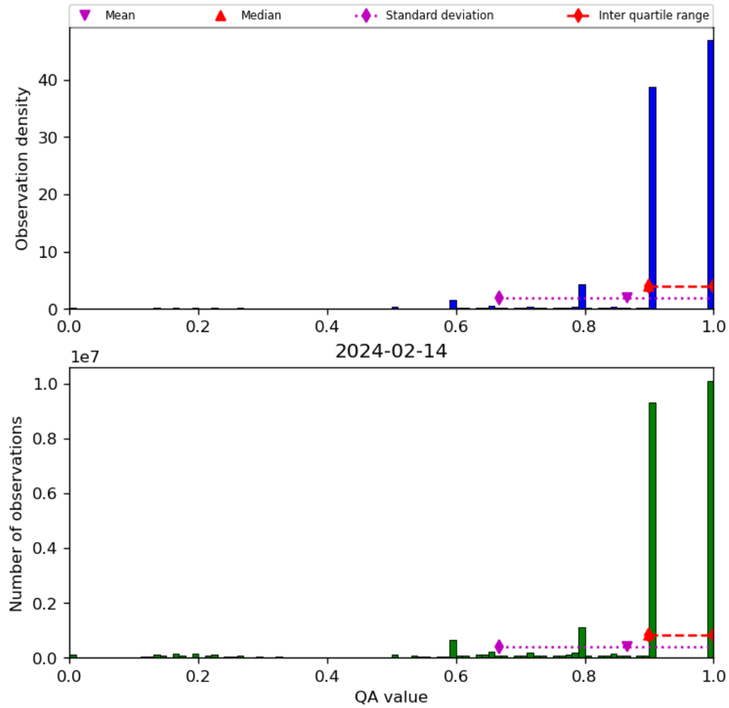
Figure 20: Histogram of “QA value” for 2024-02-13 to 2024-02-15
