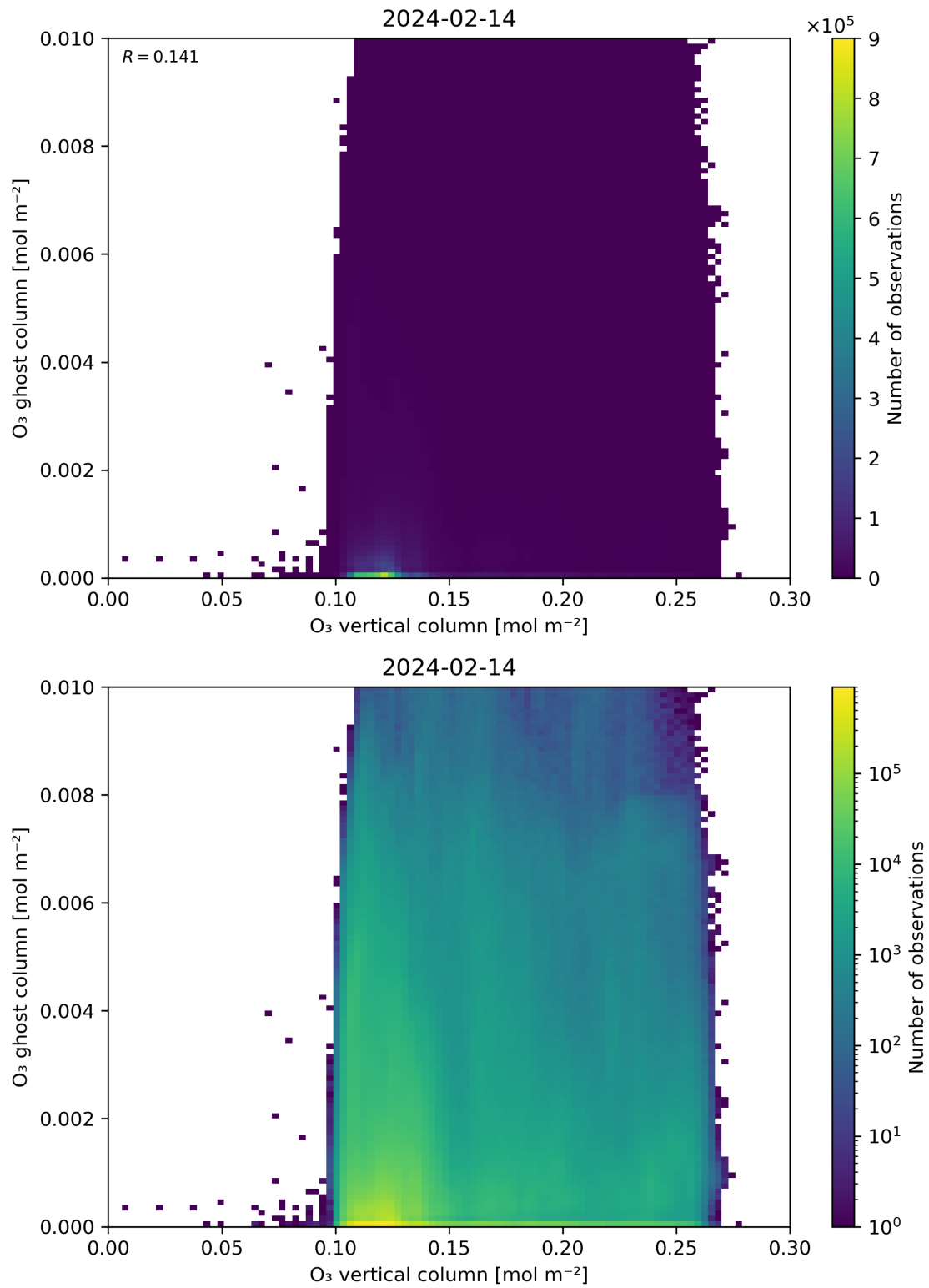
Figure 40: Scatter density plot of “O 3 vertical column” against “O 3 ghost column” for 2024-02-13 to 2024-02-15.
