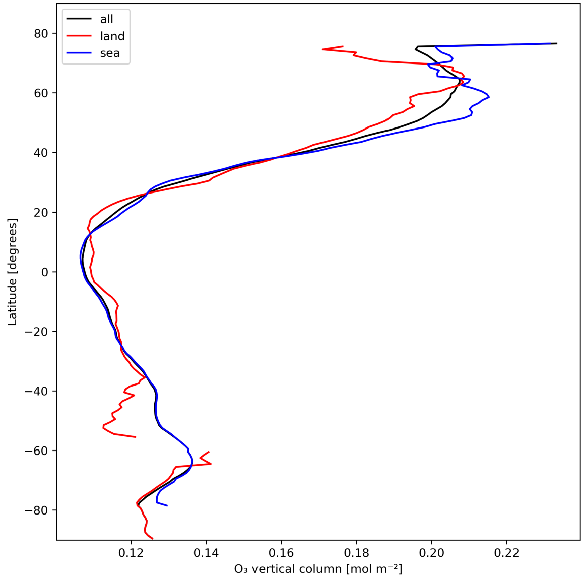
Figure 14: Zonal average of “O 3 vertical column” for 2024-02-13 to 2024-02-15.
