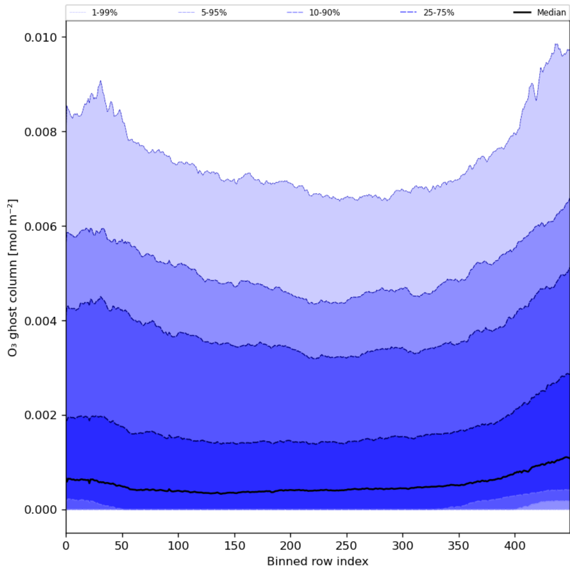
Figure 32: Along track statistics of “O 3 ghost column” for 2024-02-13 to 2024-02-15
