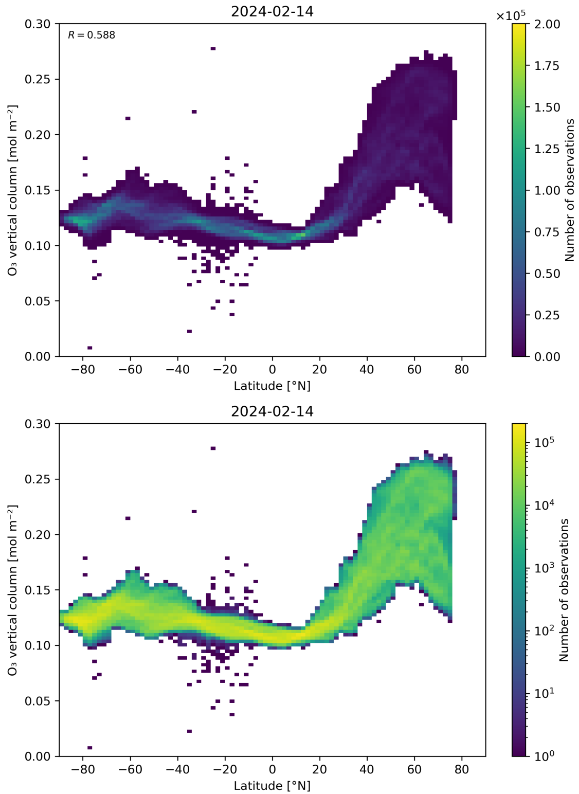
Figure 36: Scatter density plot of “Latitude” against “O 3 vertical column” for 2024-02-13 to 2024-02-15.
