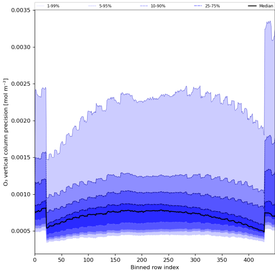
Figure 29: Along track statistics of “O 3 vertical column precision” for 2024-02-13 to 2024-02-15
