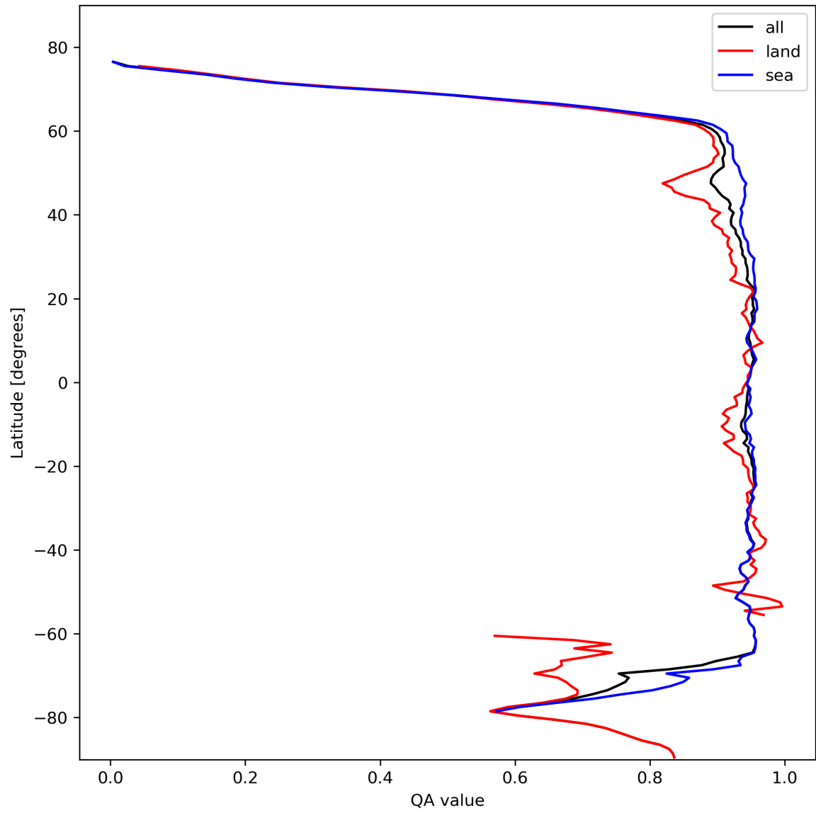
Figure 13: Zonal average of “QA value” for 2024-02-13 to 2024-02-15.
