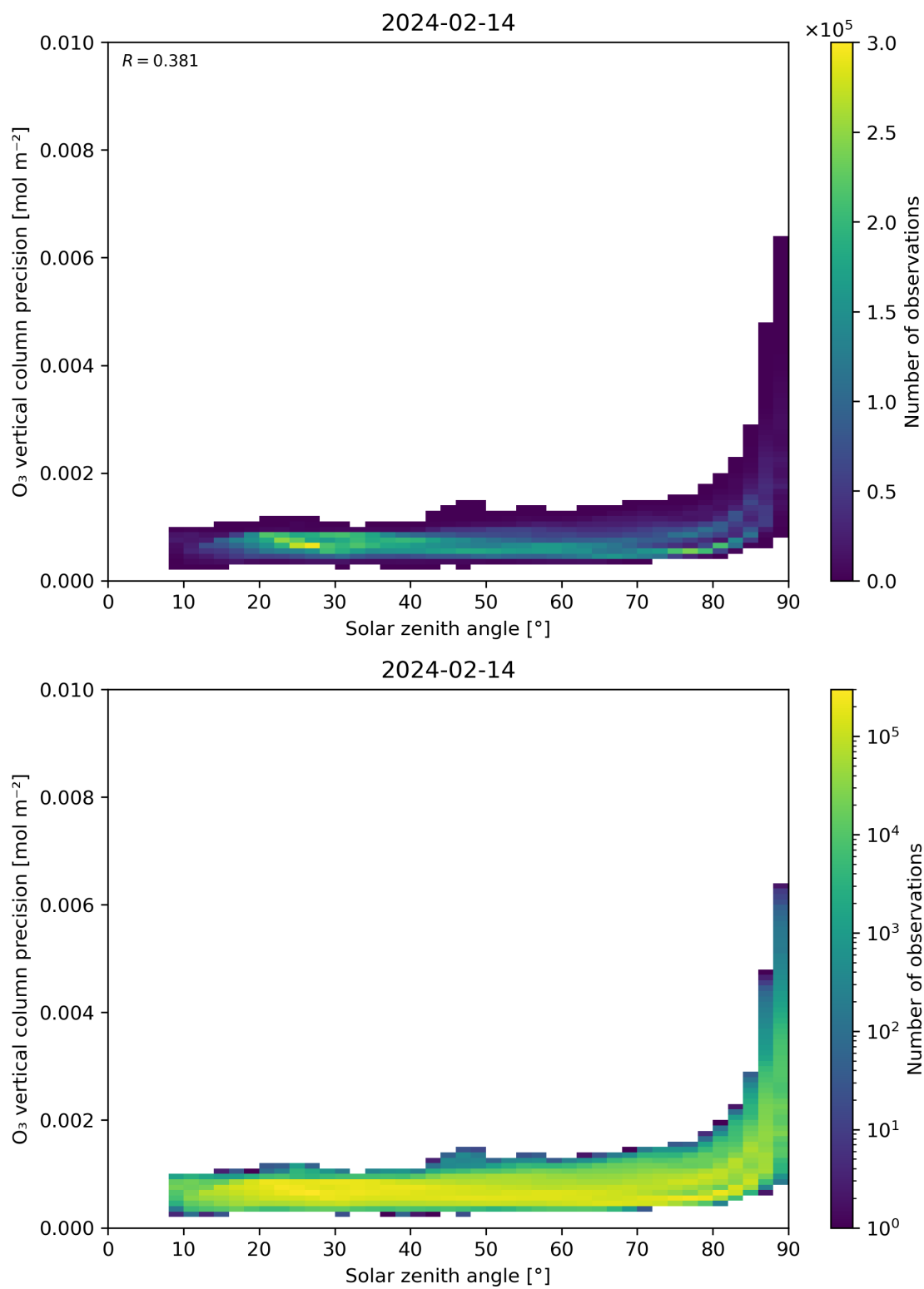
Figure 48: Scatter density plot of “Solar zenith angle” against “O 3 vertical column precision” for 2024-02-13 to 2024-02-15.
