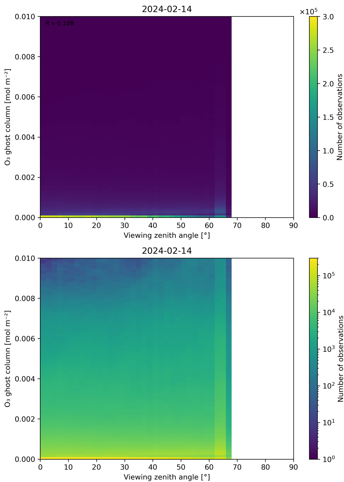
Figure 51: Scatter density plot of “Viewing zenith angle” against “O 3 ghost column” for 2024-02-13 to 2024-02-15.
