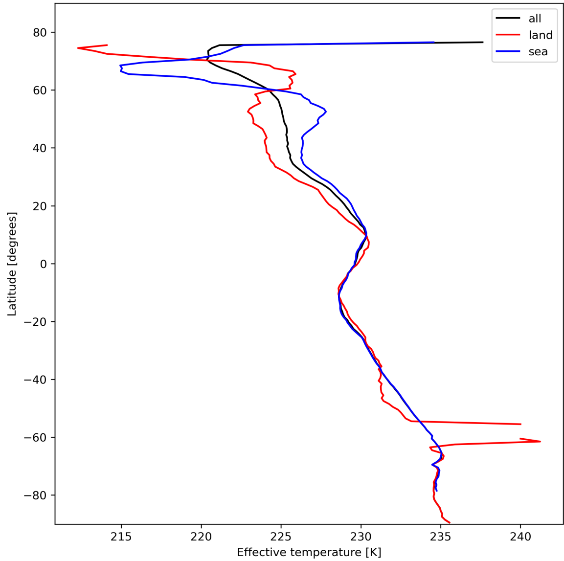
Figure 17: Zonal average of “Effective temperature” for 2024-02-13 to 2024-02-15.
