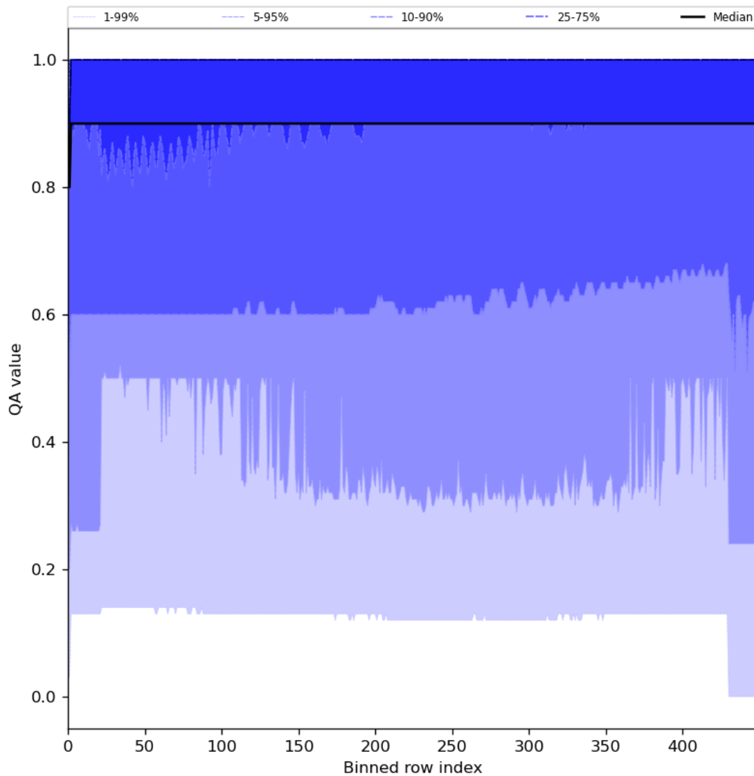
Figure 27: Along track statistics of “QA value” for 2024-02-13 to 2024-02-15
