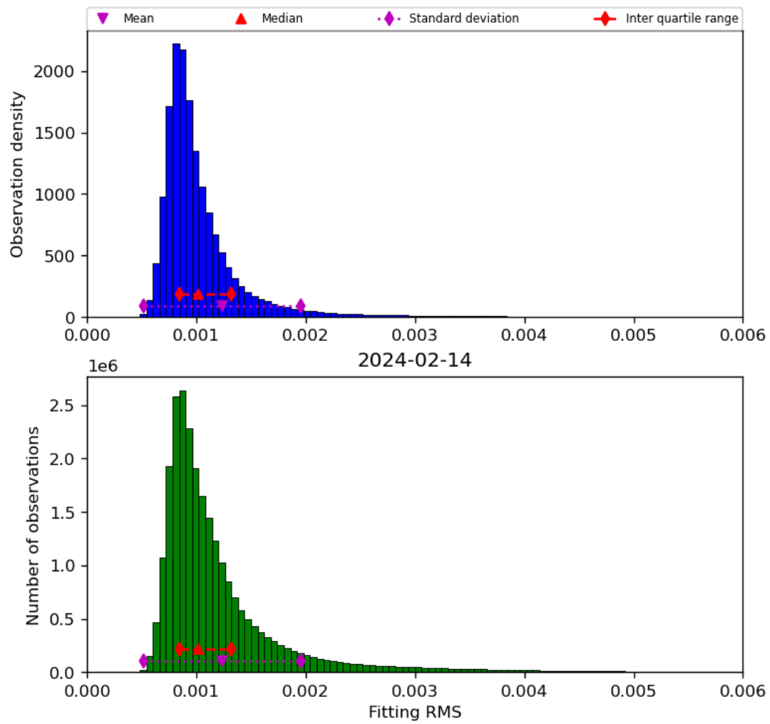
Figure 23: Histogram of “Fitting RMS” for 2024-02-13 to 2024-02-15
