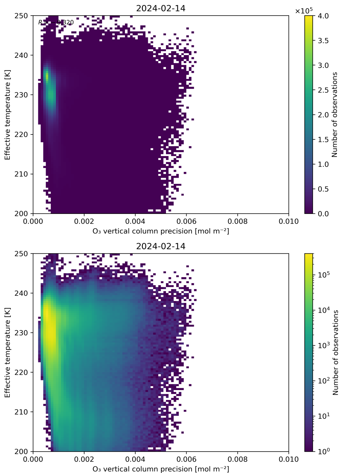
Figure 42: Scatter density plot of “O 3 vertical column precision” against “Effective temperature” for 2024-02-13 to 2024-02-15.
