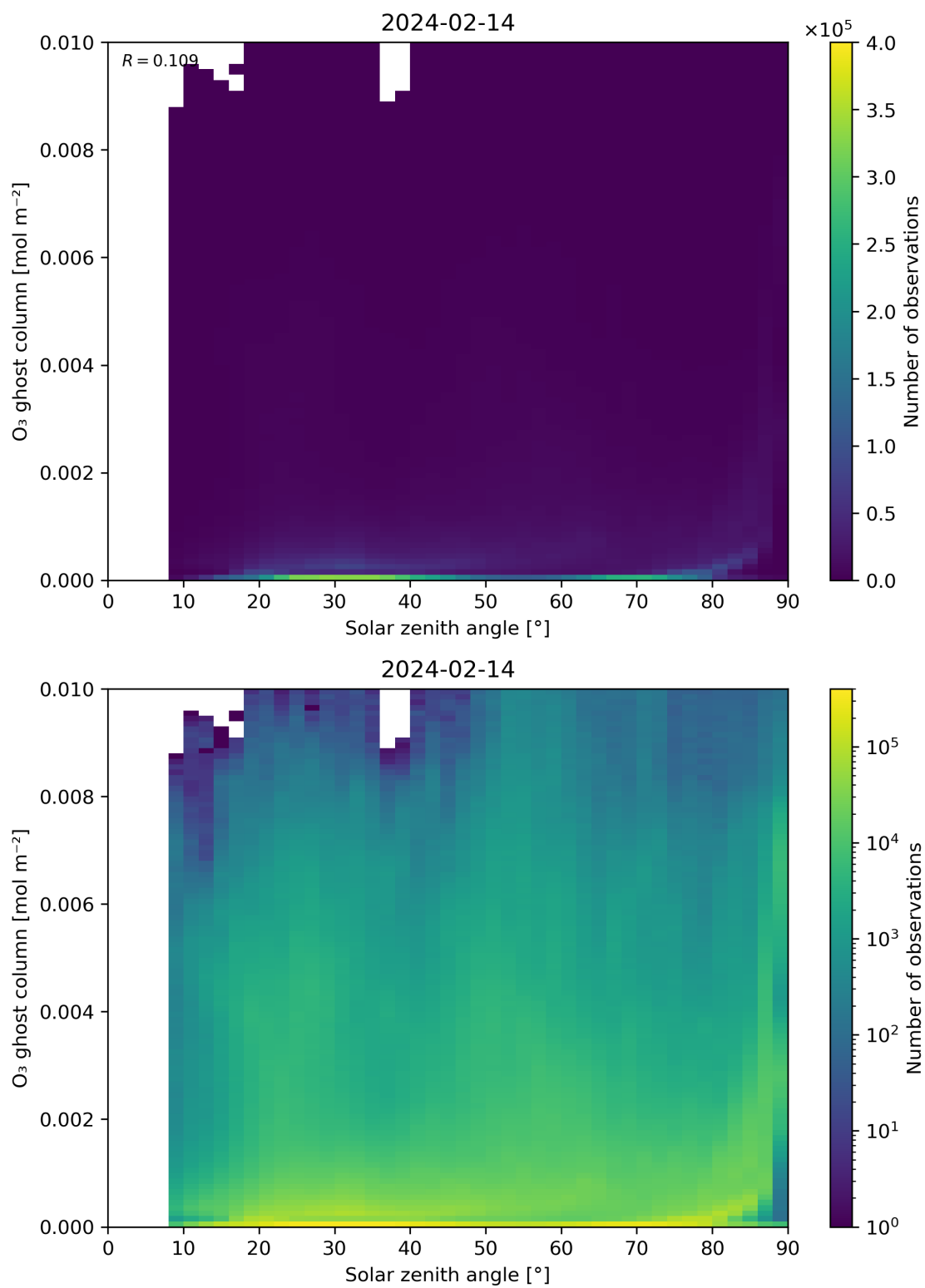
Figure 46: Scatter density plot of “Solar zenith angle” against “O 3 ghost column” for 2024-02-13 to 2024-02-15.
