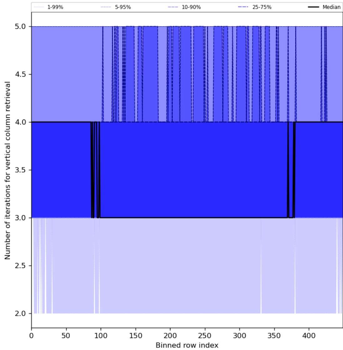
Figure 33: Along track statistics of “Number of iterations for vertical column retrieval” for 2024-02-16 to 2024-02-17
