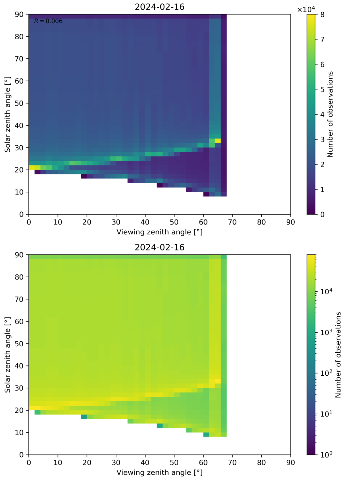
Figure 54: Scatter density plot of “Viewing zenith angle” against “Solar zenith angle” for 2024-02-16 to 2024-02-17.
