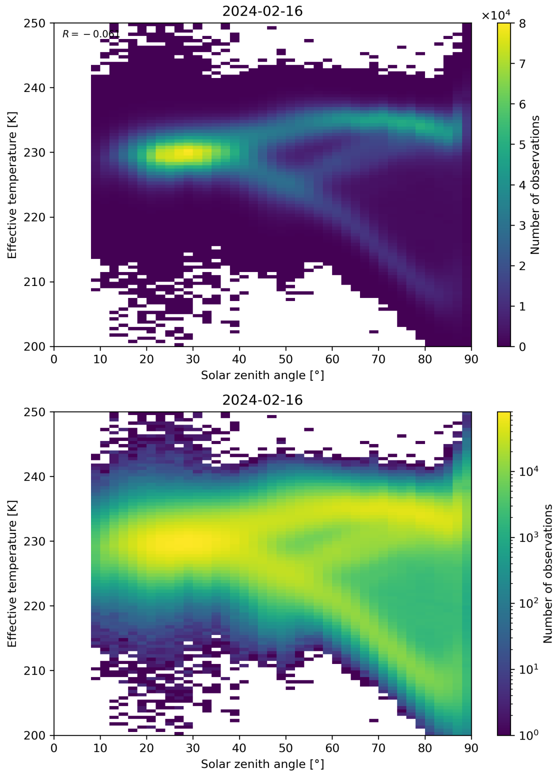
Figure 45: Scatter density plot of “Solar zenith angle” against “Effective temperature” for 2024-02-16 to 2024-02-17.
