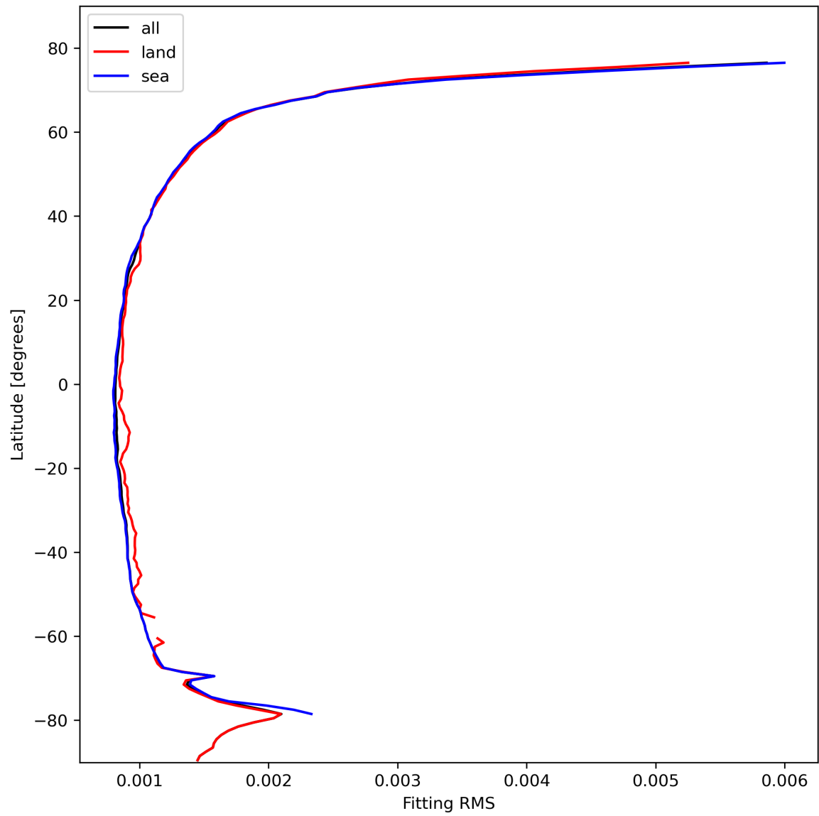
Figure 16: Zonal average of “Fitting RMS” for 2024-02-16 to 2024-02-17.
