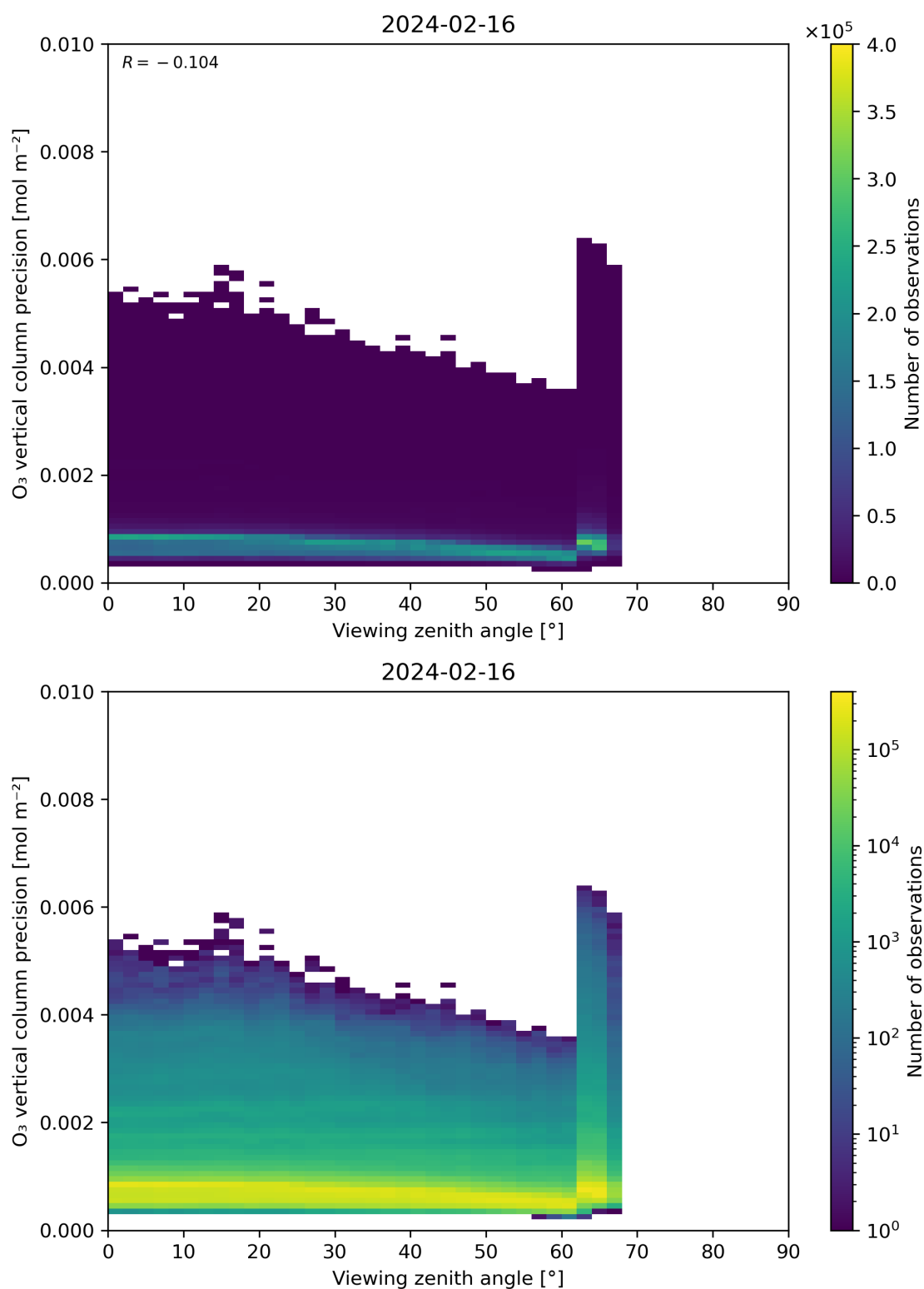
Figure 53: Scatter density plot of “Viewing zenith angle” against “O 3 vertical column precision” for 2024-02-16 to 2024-02-17.
