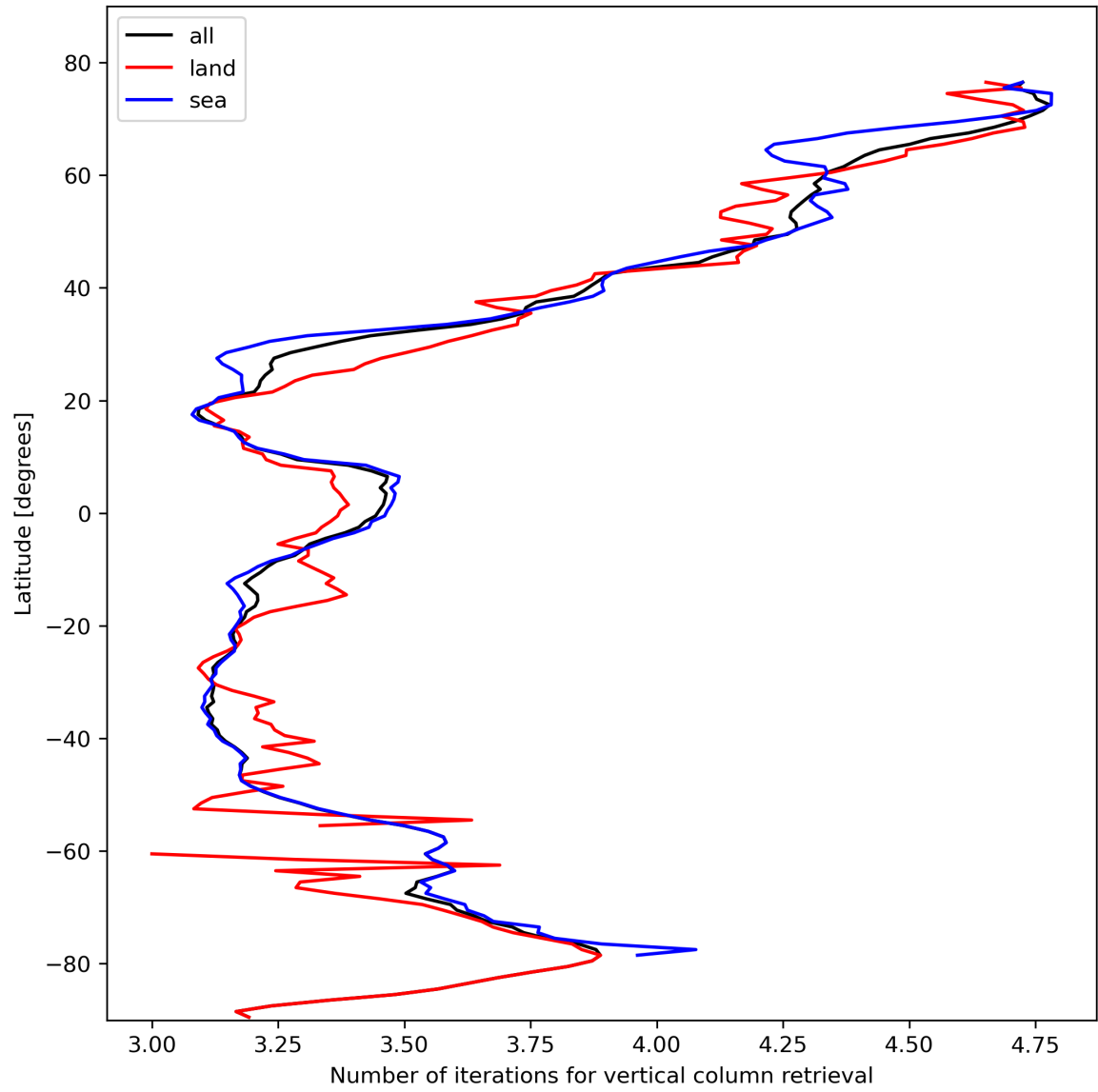
Figure 19: Zonal average of “Number of iterations for vertical column retrieval” for 2024-02-16 to 2024-02-17.
