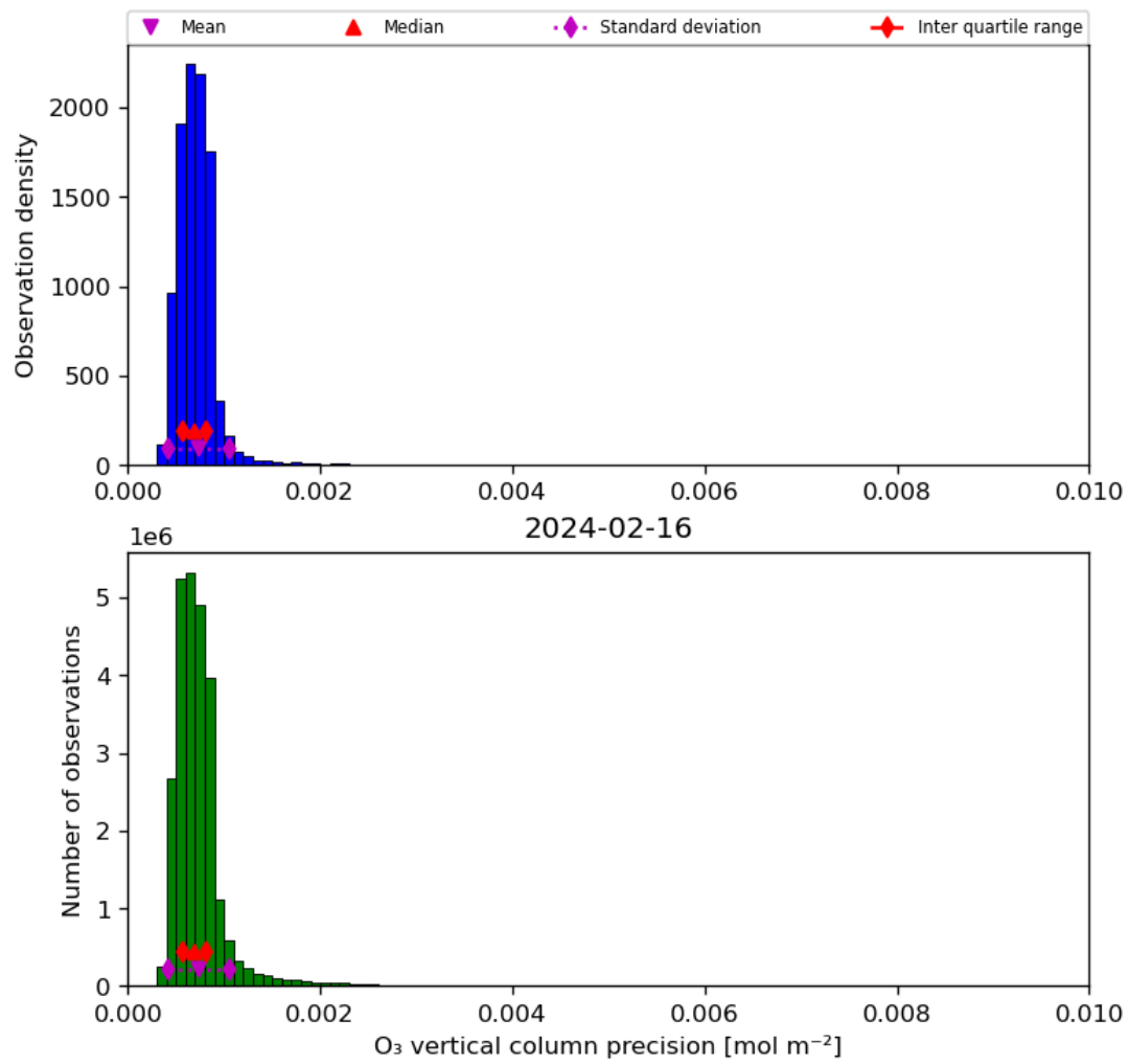
Figure 22: Histogram of “O 3 vertical column precision” for 2024-02-16 to 2024-02-17
