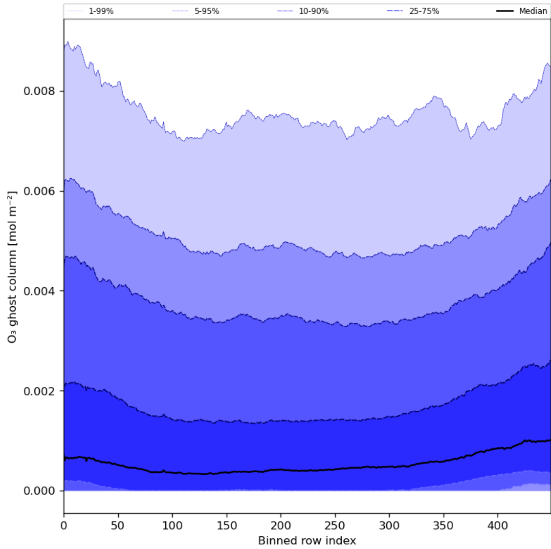
Figure 32: Along track statistics of “O 3 ghost column” for 2024-02-16 to 2024-02-17
