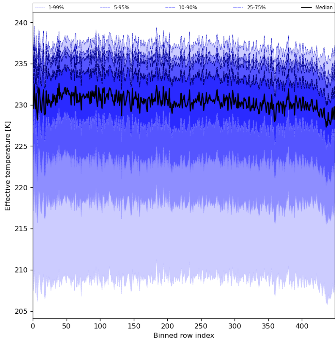
Figure 31: Along track statistics of “Effective temperature” for 2024-02-16 to 2024-02-17
