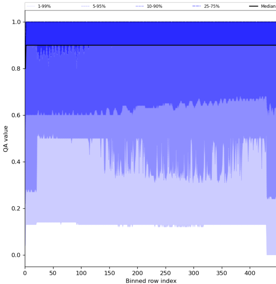
Figure 27: Along track statistics of “QA value” for 2024-02-16 to 2024-02-17
