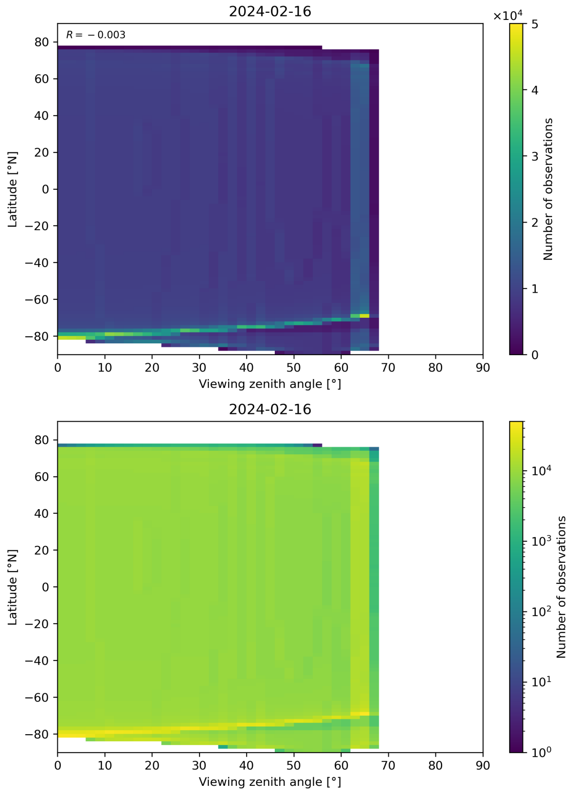
Figure 49: Scatter density plot of “Viewing zenith angle” against “Latitude” for 2024-02-16 to 2024-02-17.
