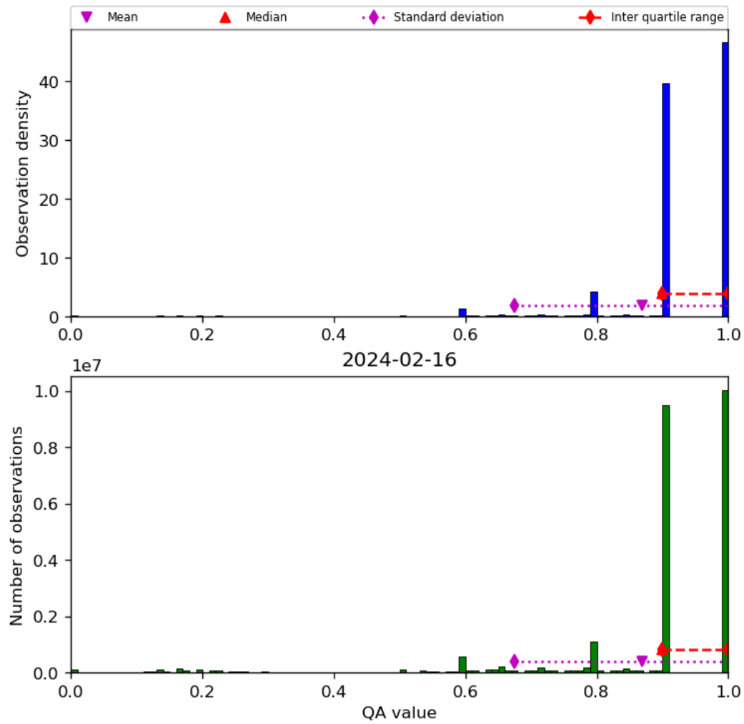
Figure 20: Histogram of “QA value” for 2024-02-16 to 2024-02-17
