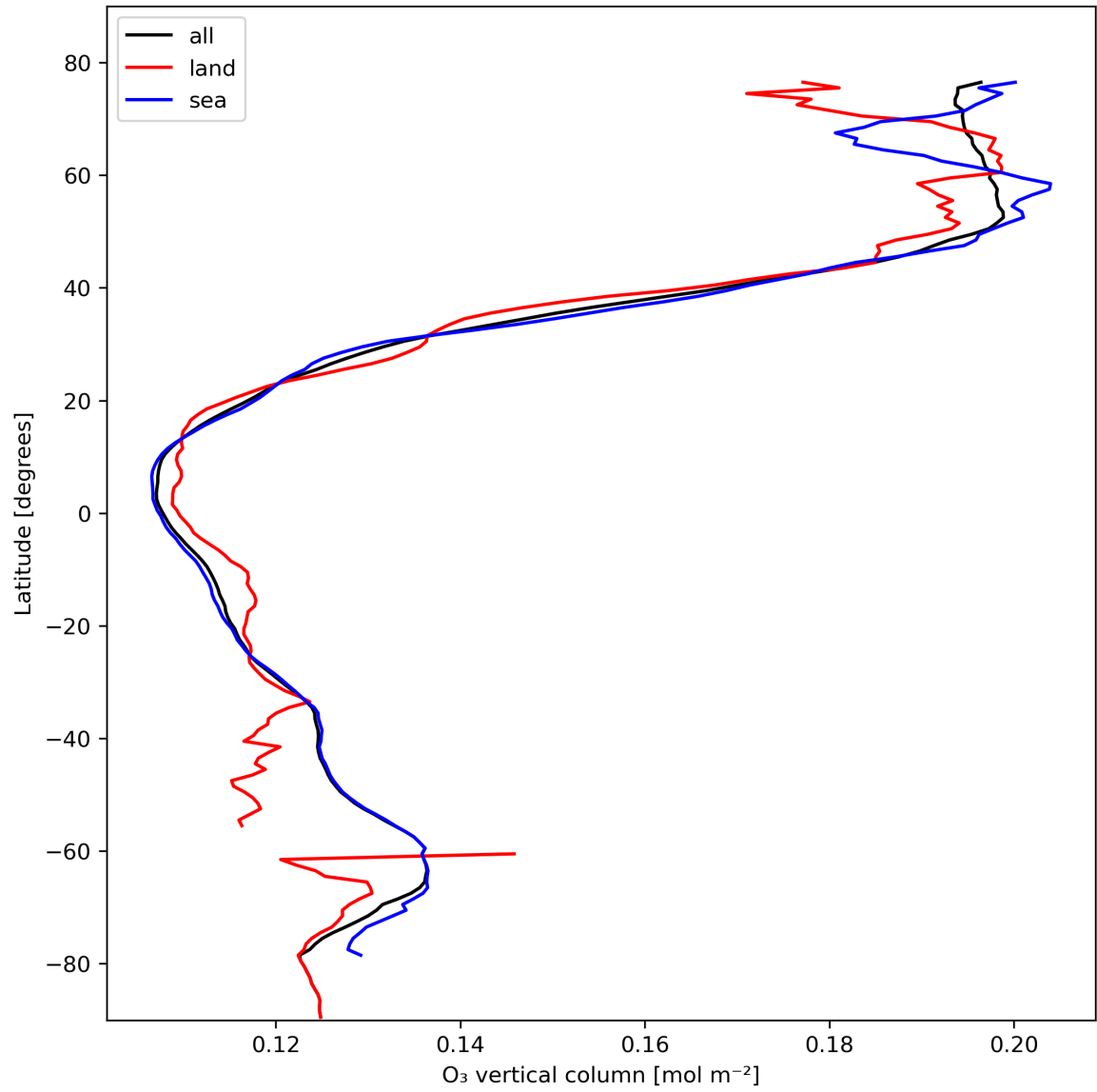
Figure 14: Zonal average of “O 3 vertical column” for 2024-02-16 to 2024-02-17.
