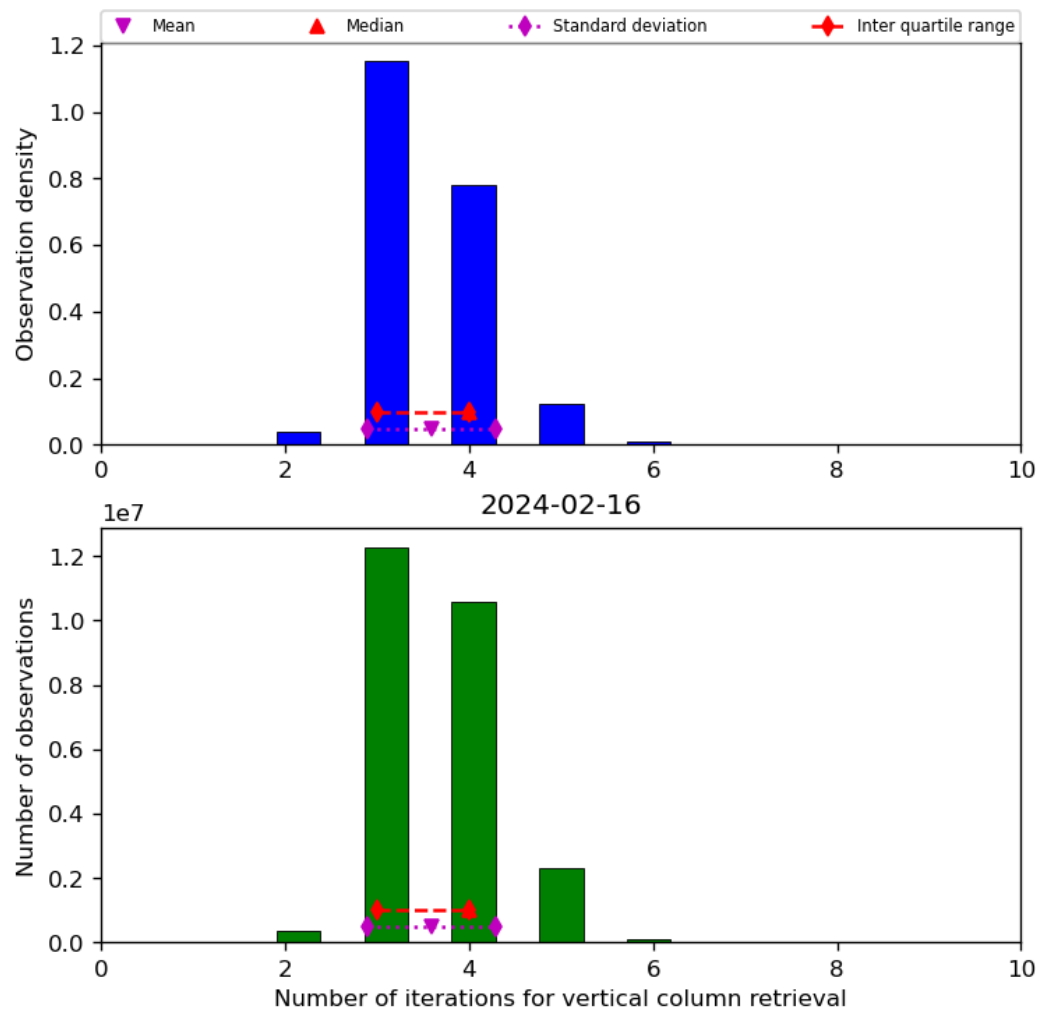
Figure 26: Histogram of “Number of iterations for vertical column retrieval” for 2024-02-16 to 2024-02-17
