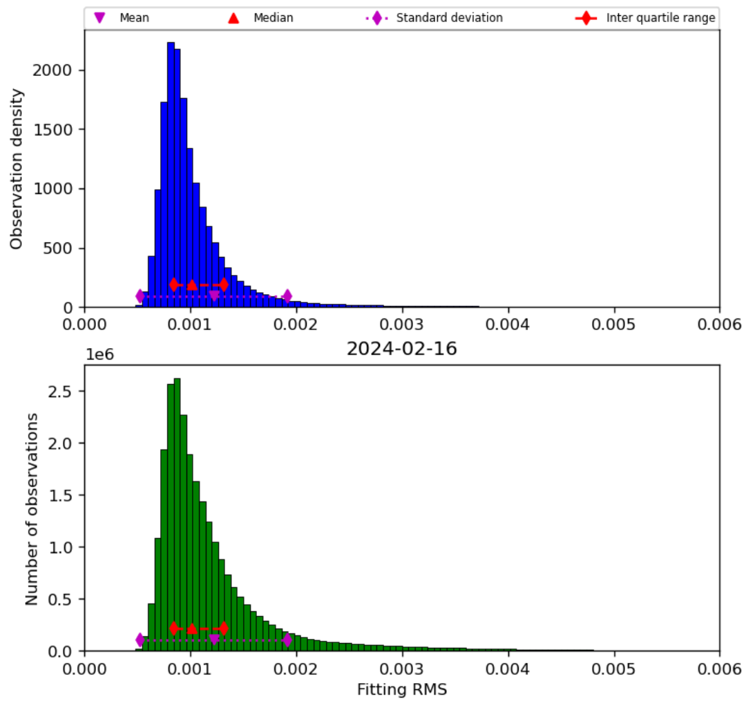
Figure 23: Histogram of “Fitting RMS” for 2024-02-16 to 2024-02-17
