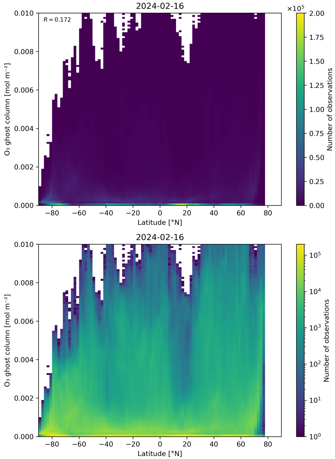
Figure 35: Scatter density plot of “Latitude” against “O 3 ghost column” for 2024-02-16 to 2024-02-17.
