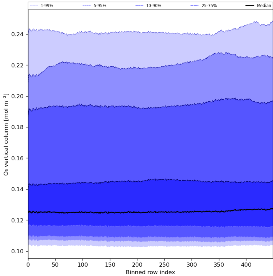
Figure 28: Along track statistics of “O 3 vertical column” for 2024-02-16 to 2024-02-17
