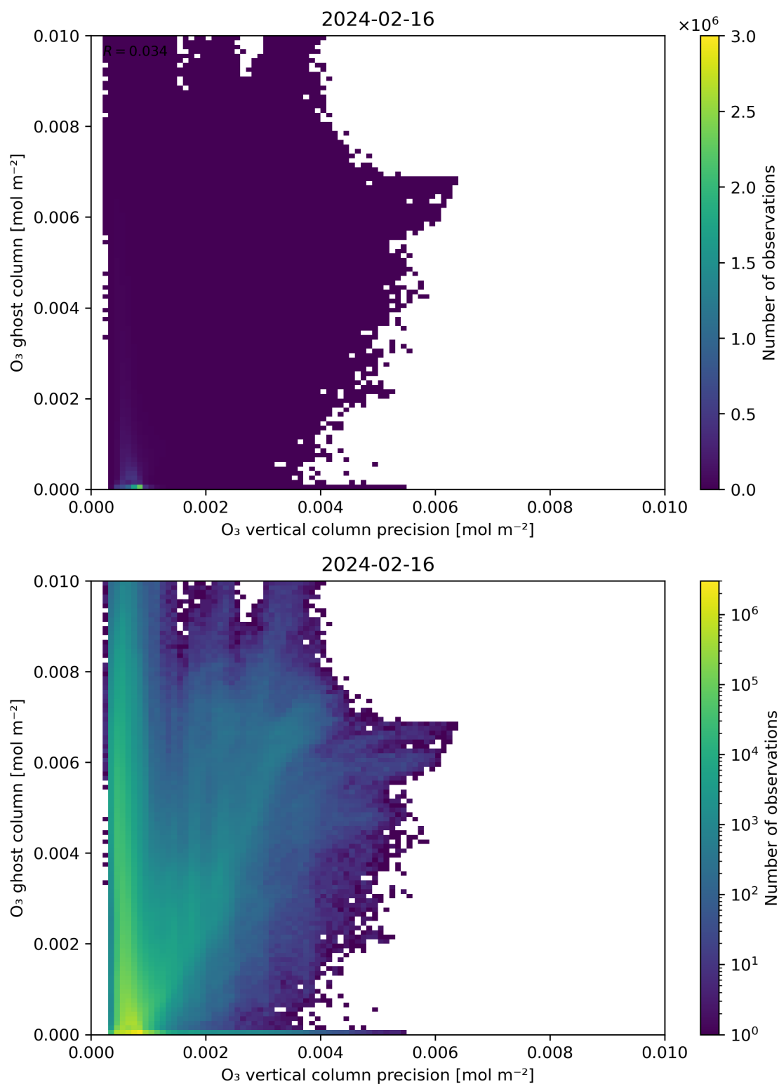
Figure 43: Scatter density plot of “ \text{O}_3 vertical column precision” against “ \text{O}_3 ghost column” for 2024-02-16 to 2024-02-17.
