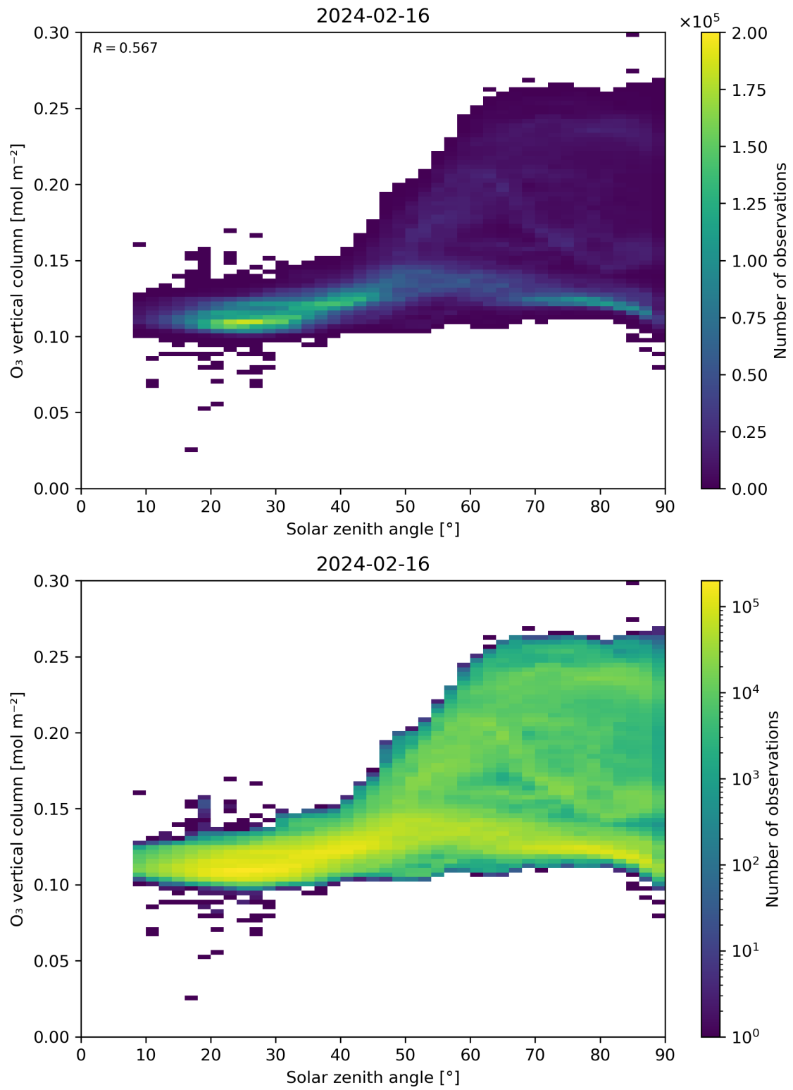
Figure 47: Scatter density plot of “Solar zenith angle” against “O 3 vertical column” for 2024-02-16 to 2024-02-17.
