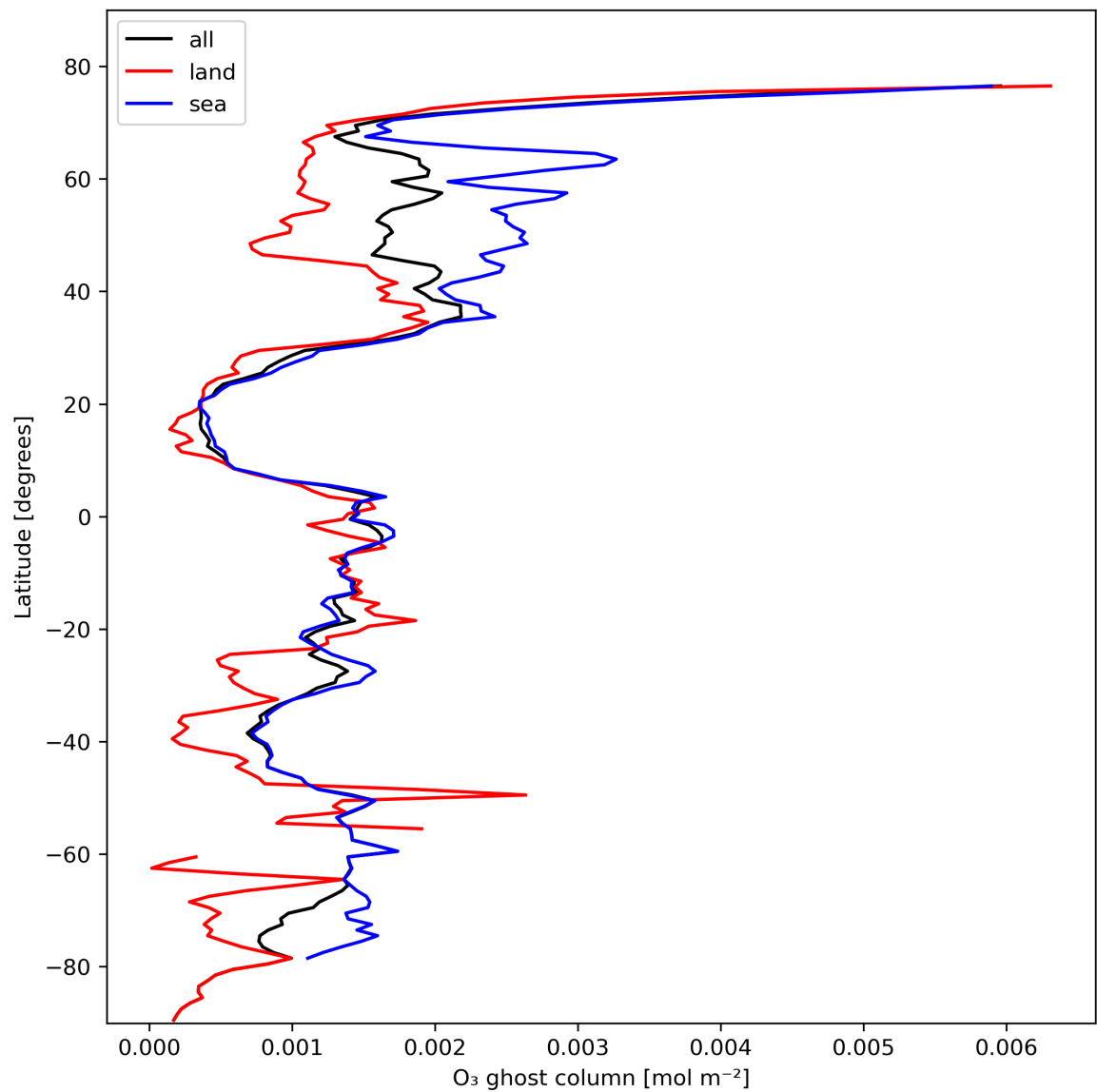
Figure 18: Zonal average of “O 3 ghost column” for 2024-02-16 to 2024-02-17.
