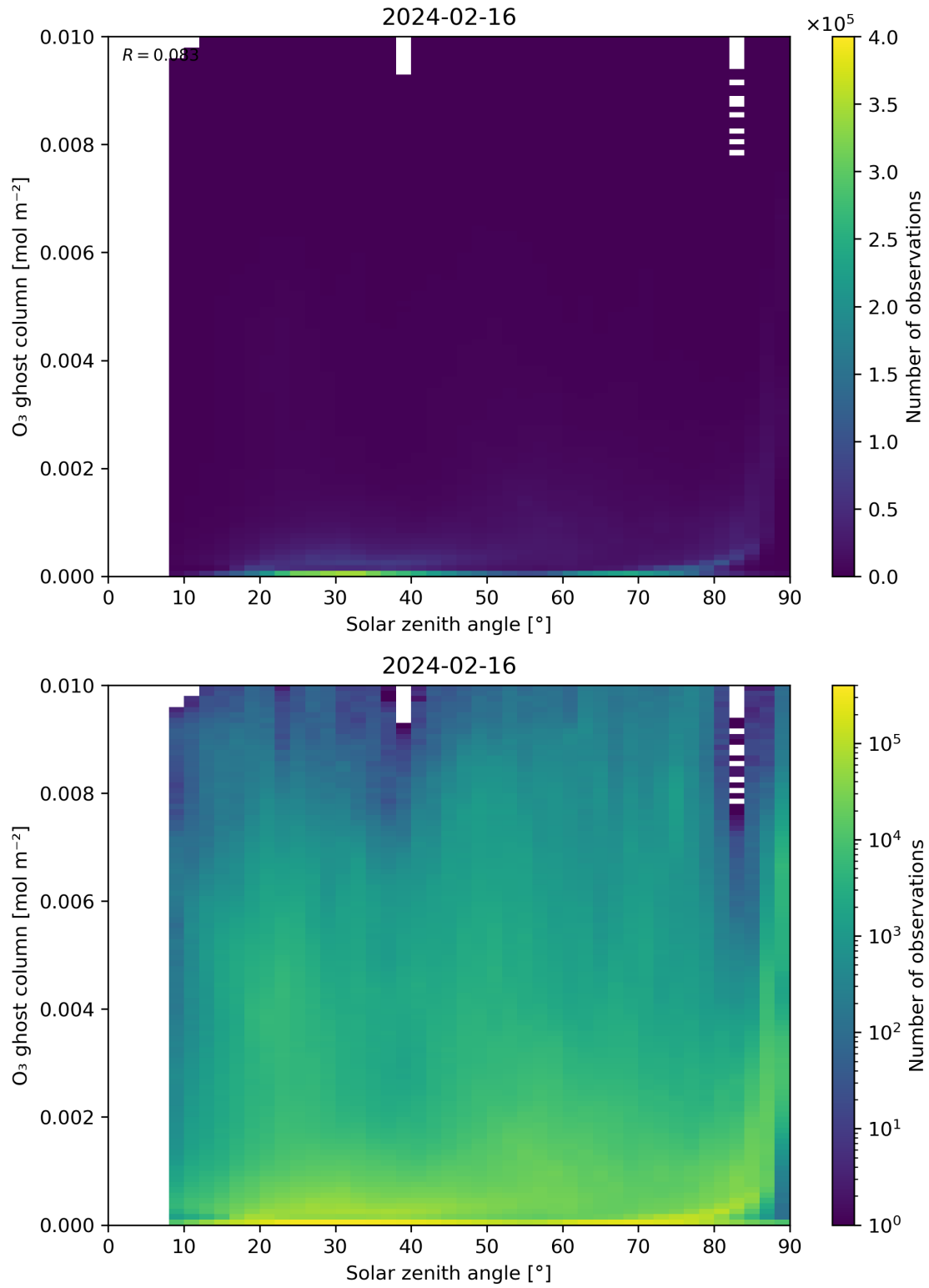
Figure 46: Scatter density plot of “Solar zenith angle” against “O 3 ghost column” for 2024-02-16 to 2024-02-17.
