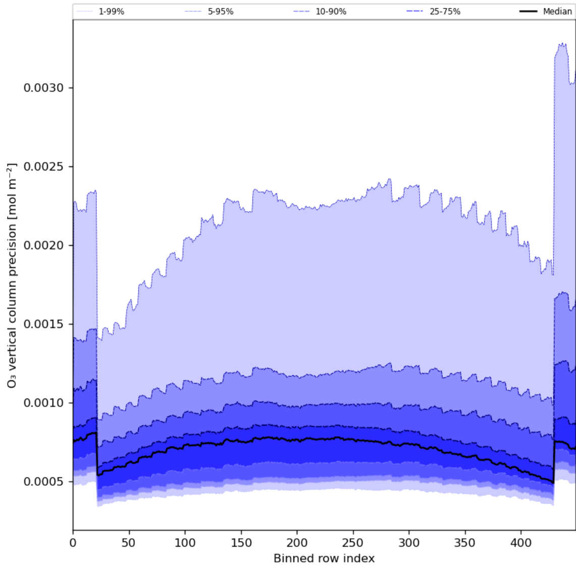
Figure 29: Along track statistics of “O 3 vertical column precision” for 2024-02-16 to 2024-02-17
