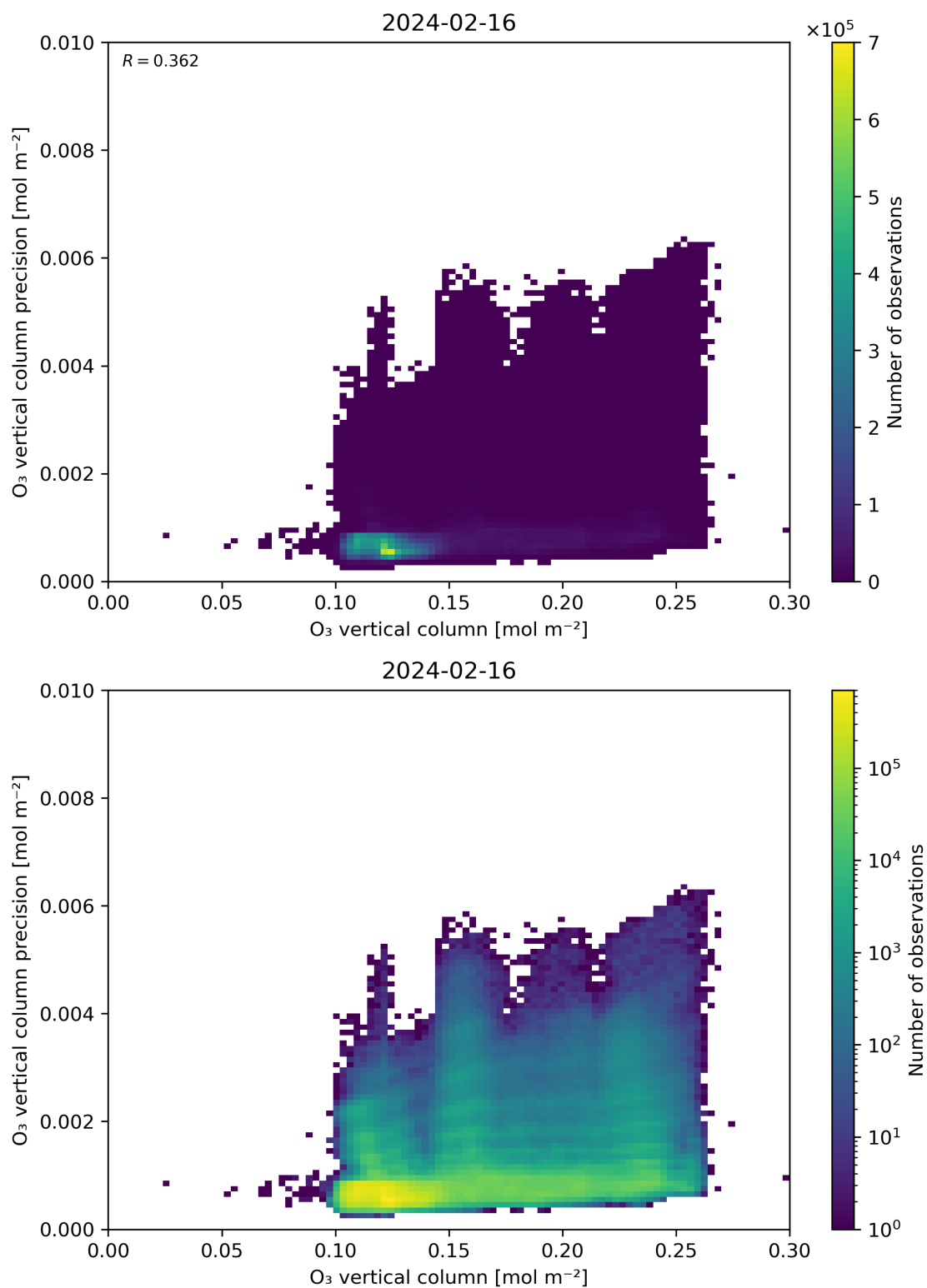
Figure 41: Scatter density plot of “O 3 vertical column” against “O 3 vertical column precision” for 2024-02-16 to 2024-02-17.
