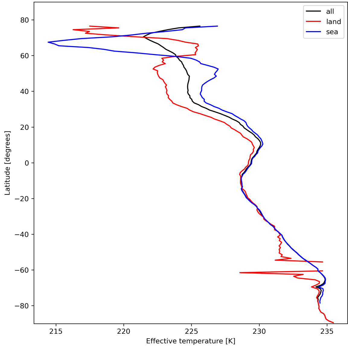
Figure 17: Zonal average of “Effective temperature” for 2024-02-16 to 2024-02-17.
