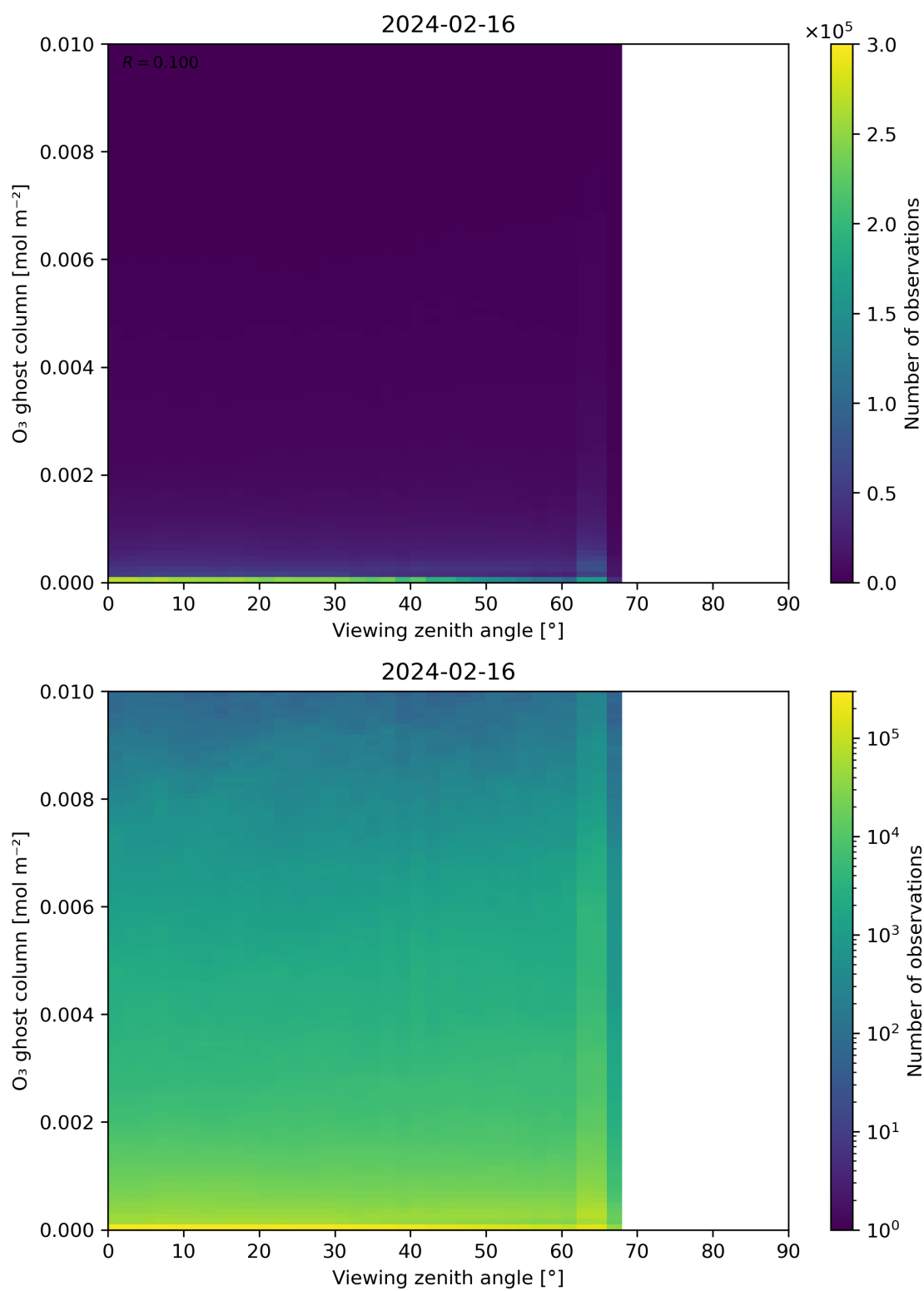
Figure 51: Scatter density plot of “Viewing zenith angle” against “O 3 ghost column” for 2024-02-16 to 2024-02-17.
