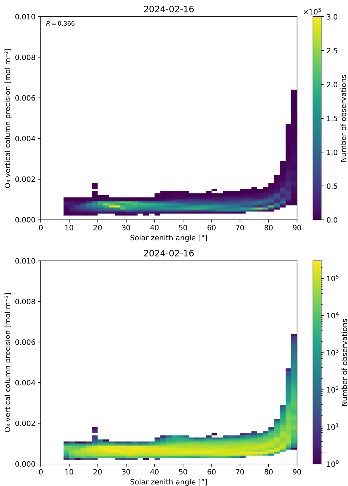
Figure 48: Scatter density plot of “Solar zenith angle” against “O 3 vertical column precision” for 2024-02-16 to 2024-02-17.
