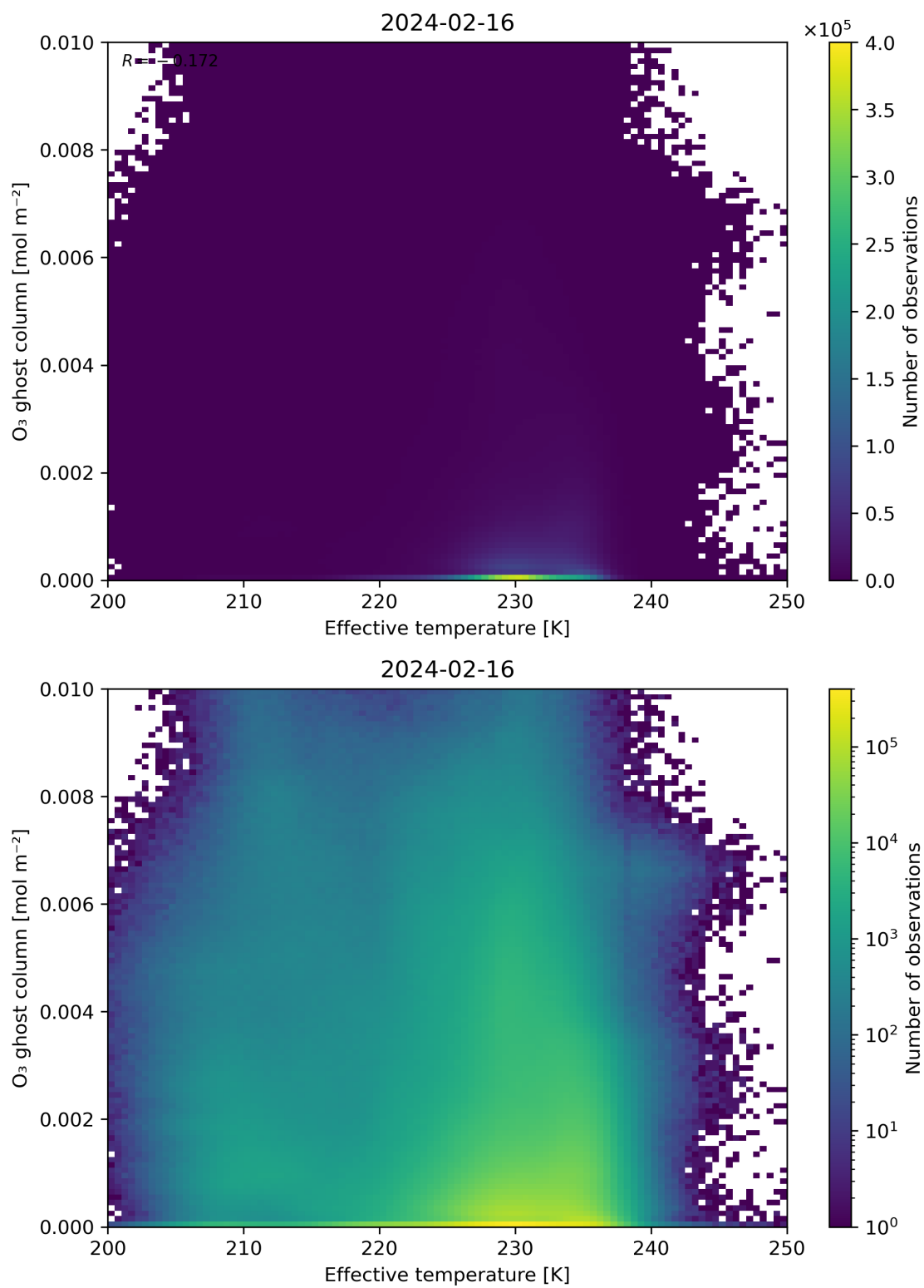
Figure 38: Scatter density plot of “Effective temperature” against “O 3 ghost column” for 2024-02-16 to 2024-02-17.
