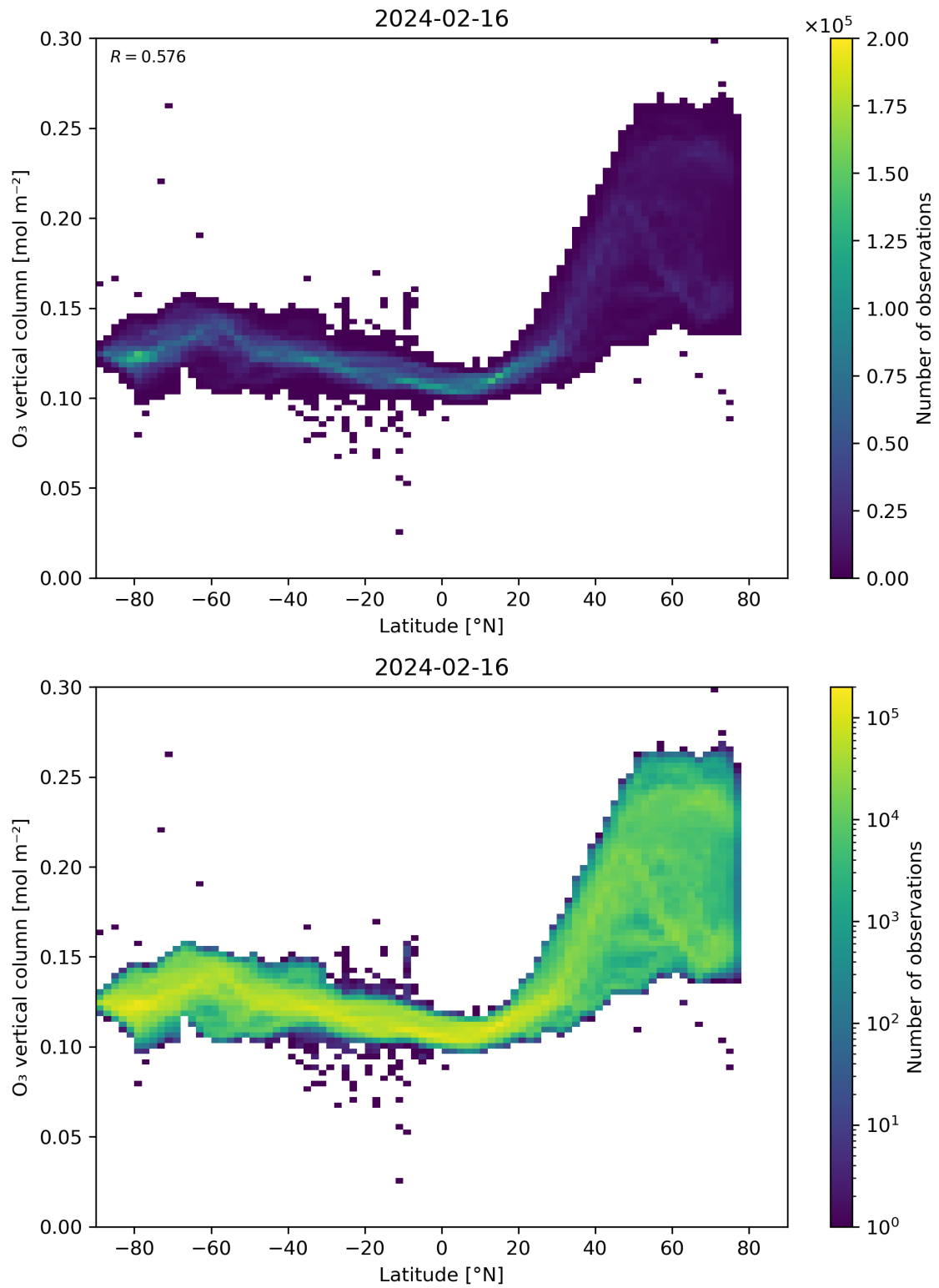
Figure 36: Scatter density plot of “Latitude” against “O 3 vertical column” for 2024-02-16 to 2024-02-17.
