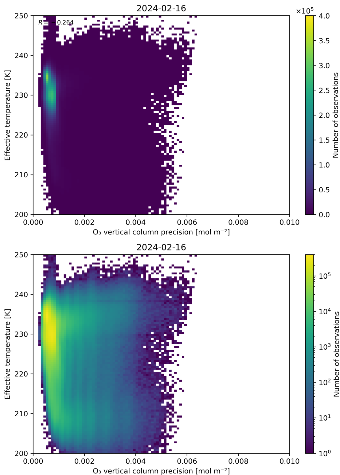
Figure 42: Scatter density plot of “O 3 vertical column precision” against “Effective temperature” for 2024-02-16 to 2024-02-17.
