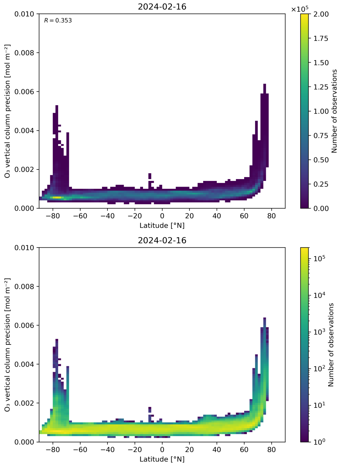
Figure 37: Scatter density plot of “Latitude” against “O 3 vertical column precision” for 2024-02-16 to 2024-02-17.
