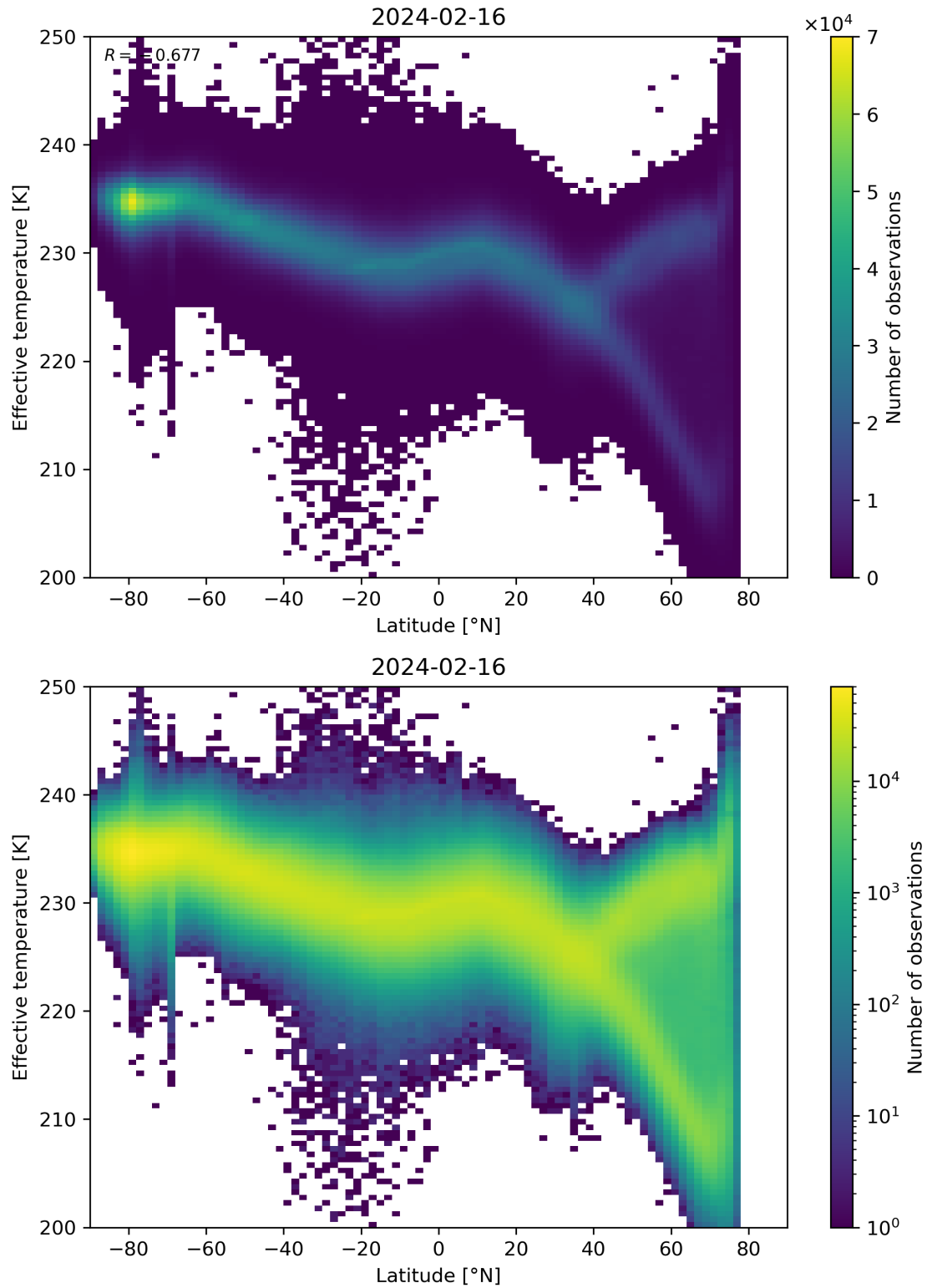
Figure 34: Scatter density plot of “Latitude” against “Effective temperature” for 2024-02-16 to 2024-02-17.
