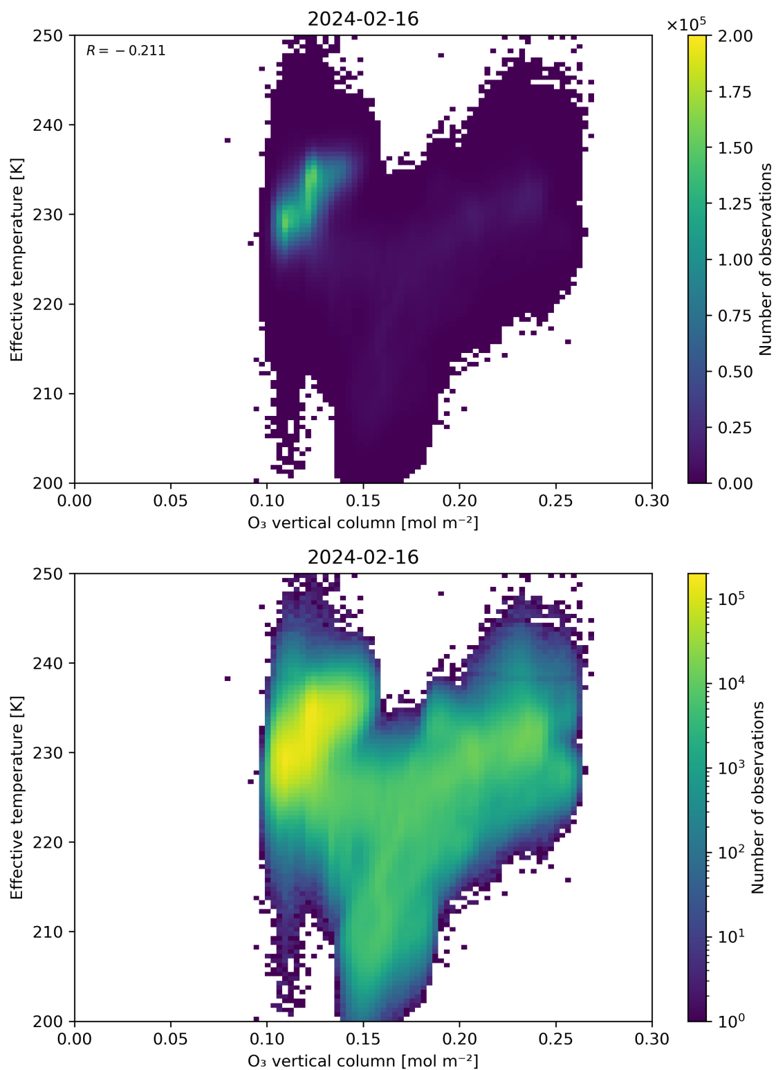
Figure 39: Scatter density plot of “O 3 vertical column” against “Effective temperature” for 2024-02-16 to 2024-02-17.
