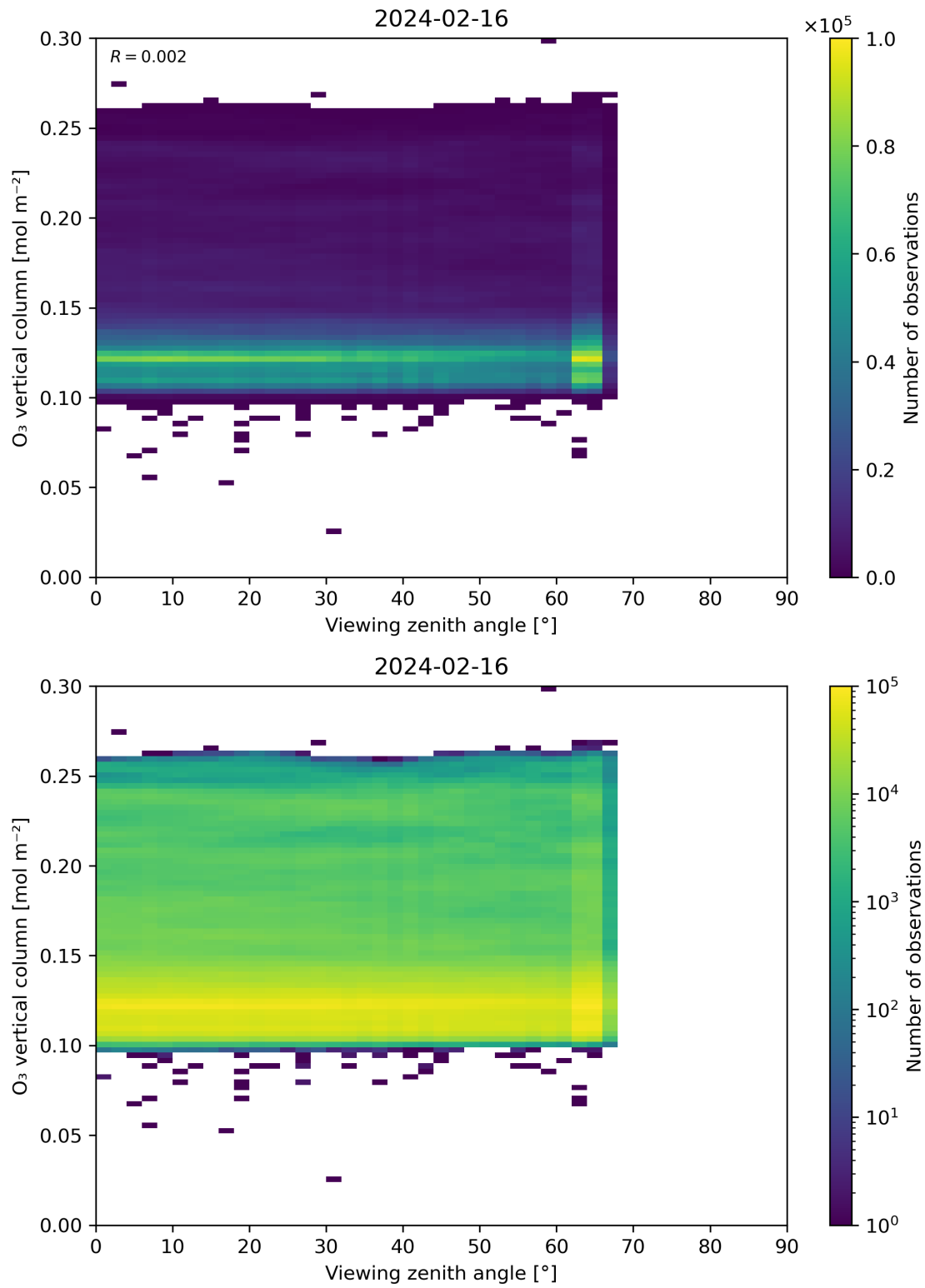
Figure 52: Scatter density plot of “Viewing zenith angle” against “O 3 vertical column” for 2024-02-16 to 2024-02-17.
