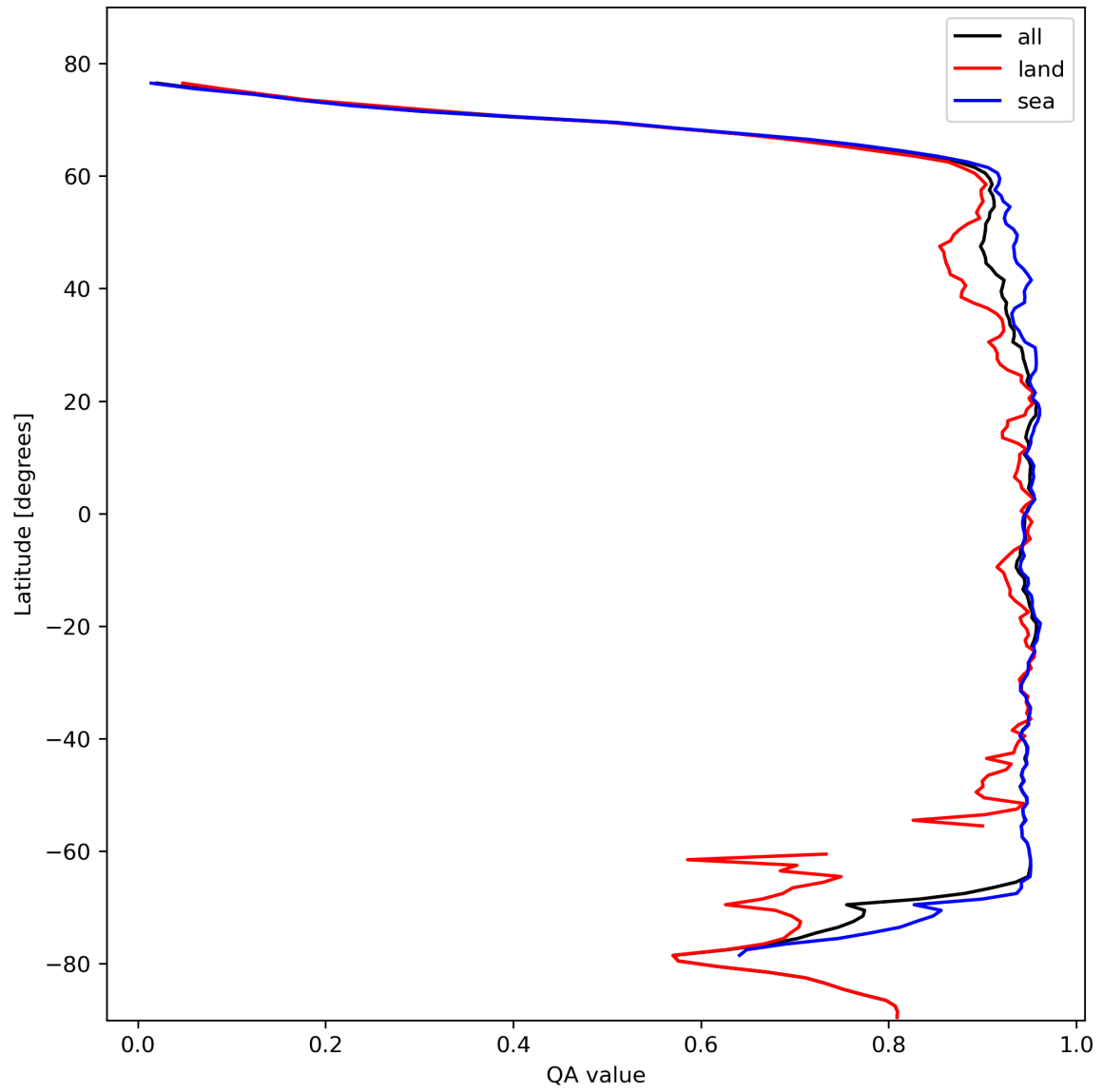
Figure 13: Zonal average of “QA value” for 2024-02-16 to 2024-02-17.
