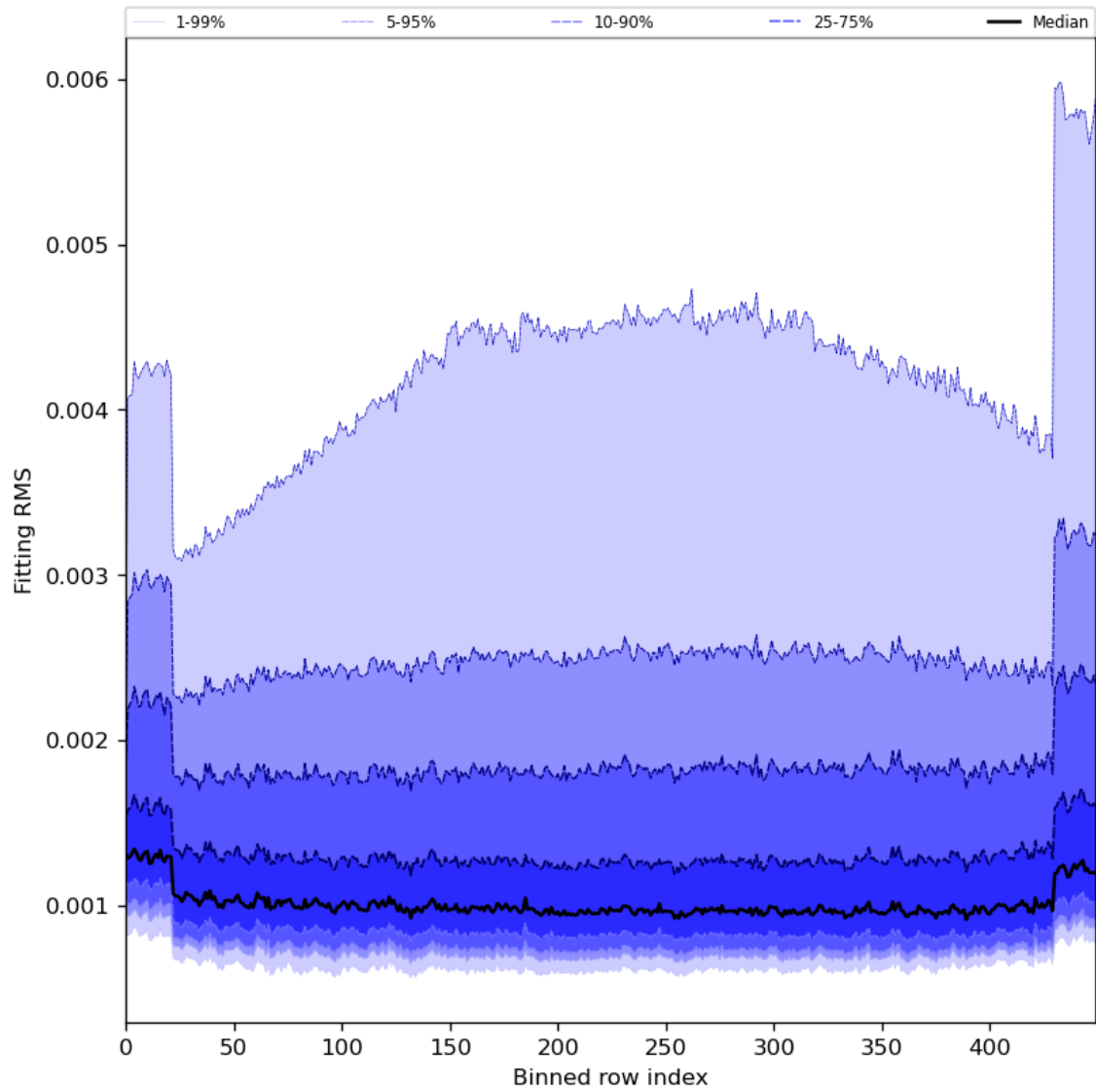
Figure 30: Along track statistics of “Fitting RMS” for 2024-02-16 to 2024-02-17
