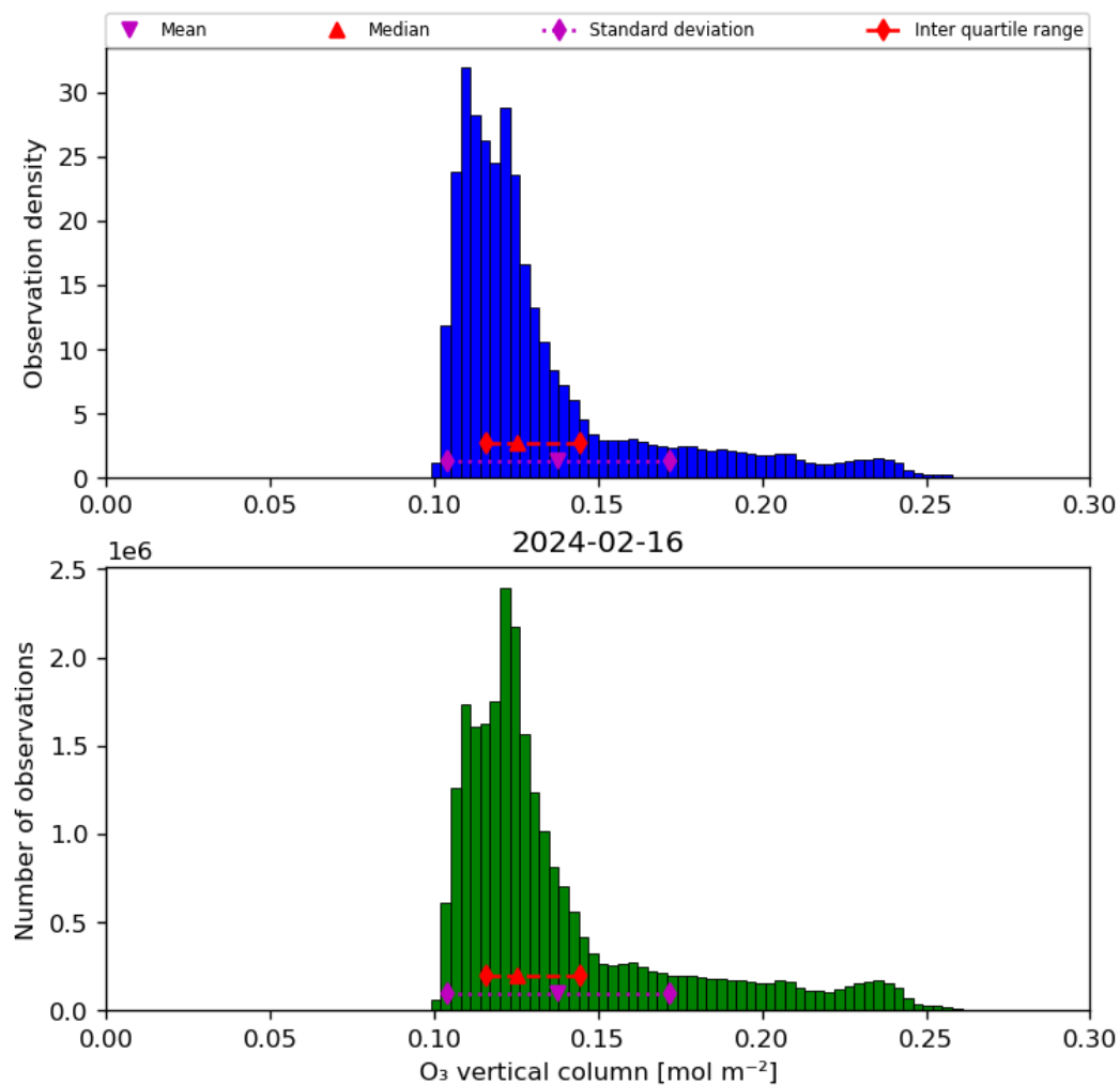
Figure 21: Histogram of “O 3 vertical column” for 2024-02-16 to 2024-02-17
