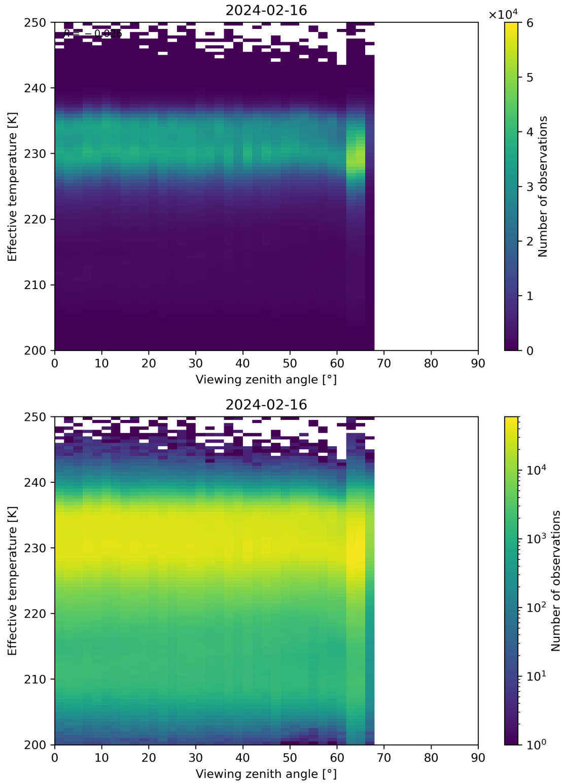
Figure 50: Scatter density plot of “Viewing zenith angle” against “Effective temperature” for 2024-02-16 to 2024-02-17.
