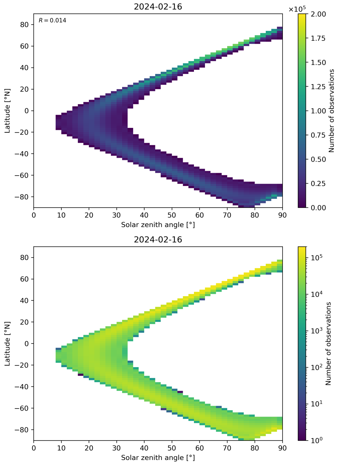
Figure 44: Scatter density plot of “Solar zenith angle” against “Latitude” for 2024-02-16 to 2024-02-17.
