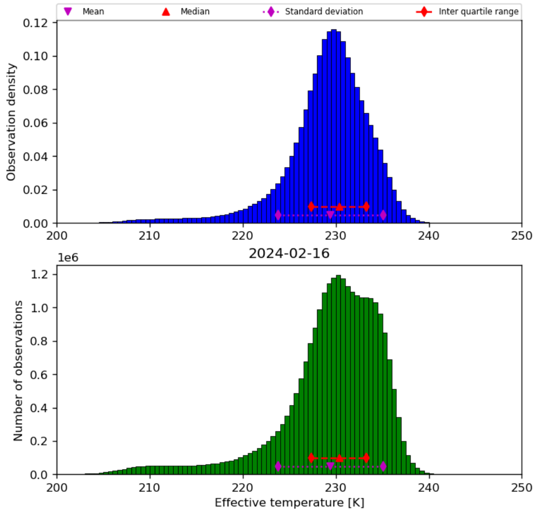
Figure 24: Histogram of “Effective temperature” for 2024-02-16 to 2024-02-17
