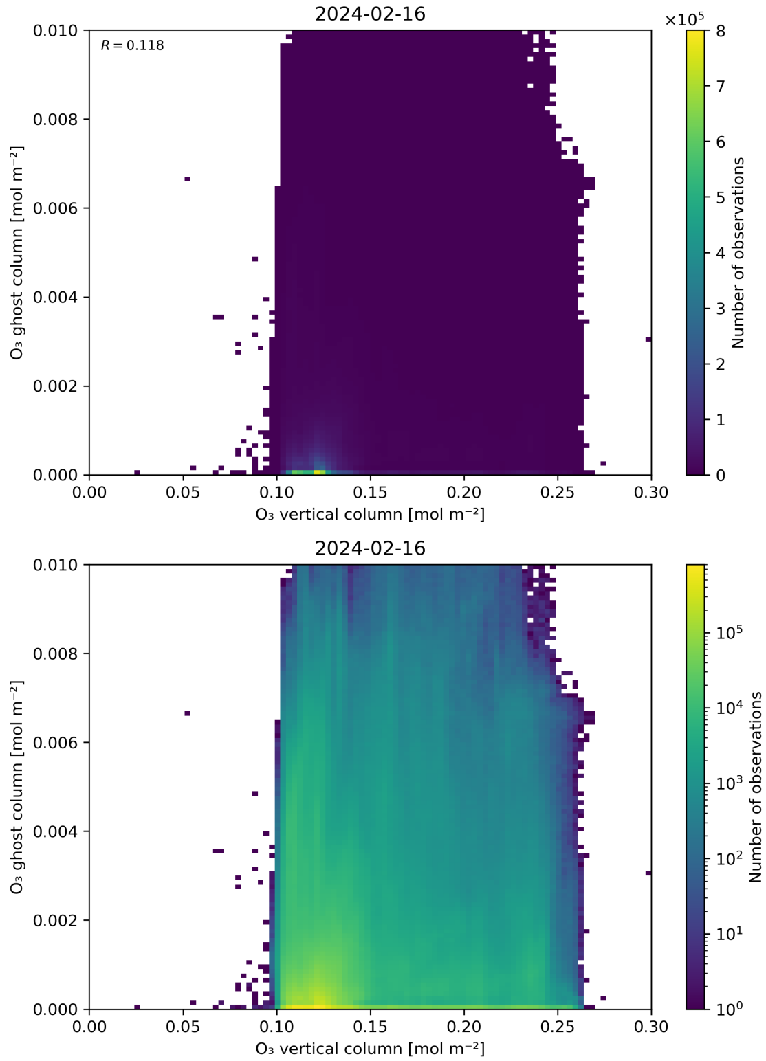
Figure 40: Scatter density plot of “O 3 vertical column” against “O 3 ghost column” for 2024-02-16 to 2024-02-17.
