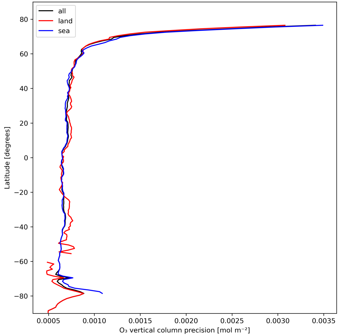
Figure 15: Zonal average of "O 3 vertical column precision" for 2024-02-16 to 2024-02-17.
