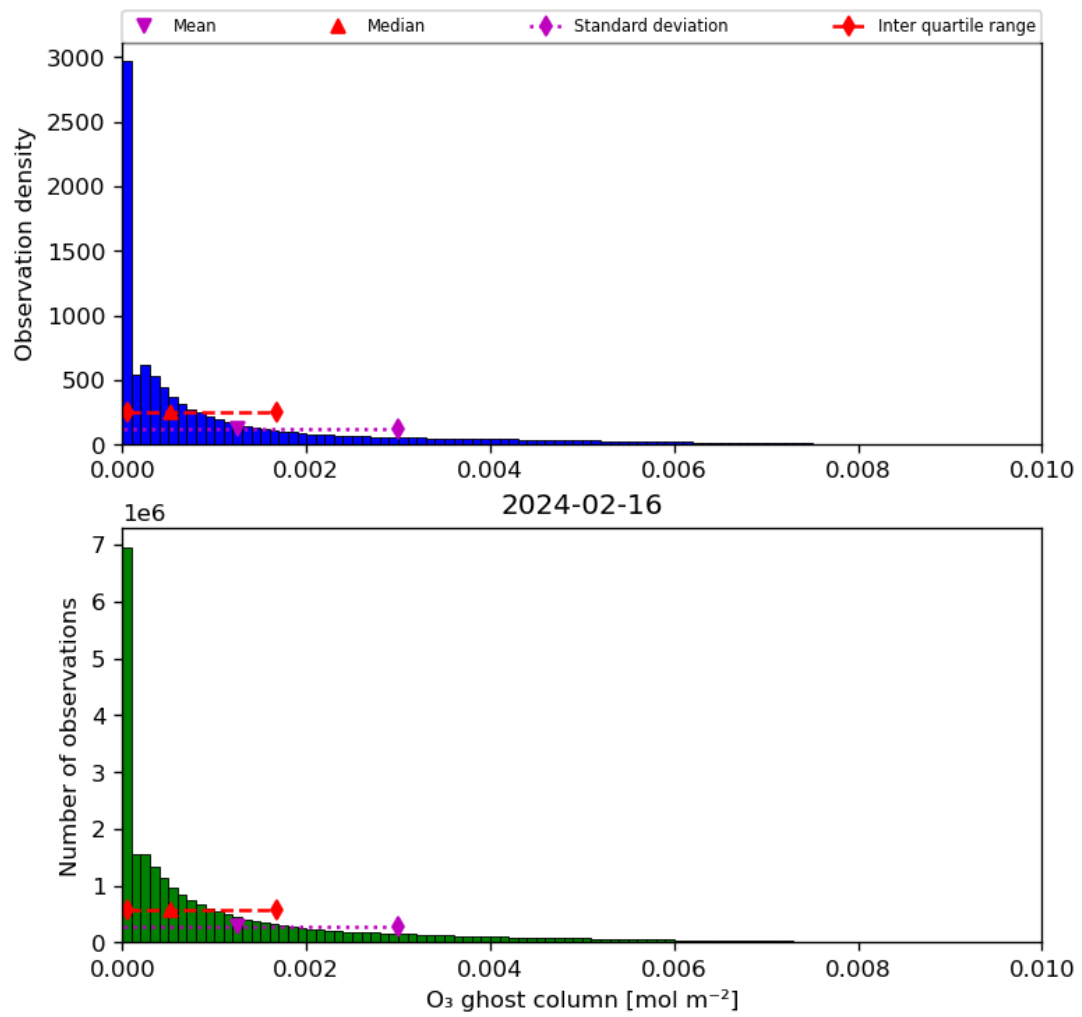
Figure 25: Histogram of “O 3 ghost column” for 2024-02-16 to 2024-02-17
