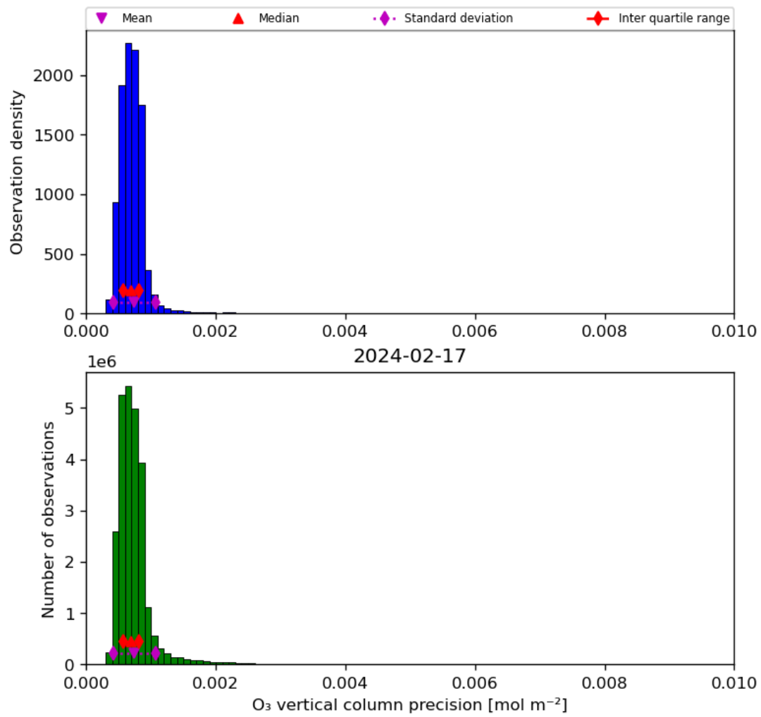
Figure 22: Histogram of “O 3 vertical column precision” for 2024-02-17 to 2024-02-18
