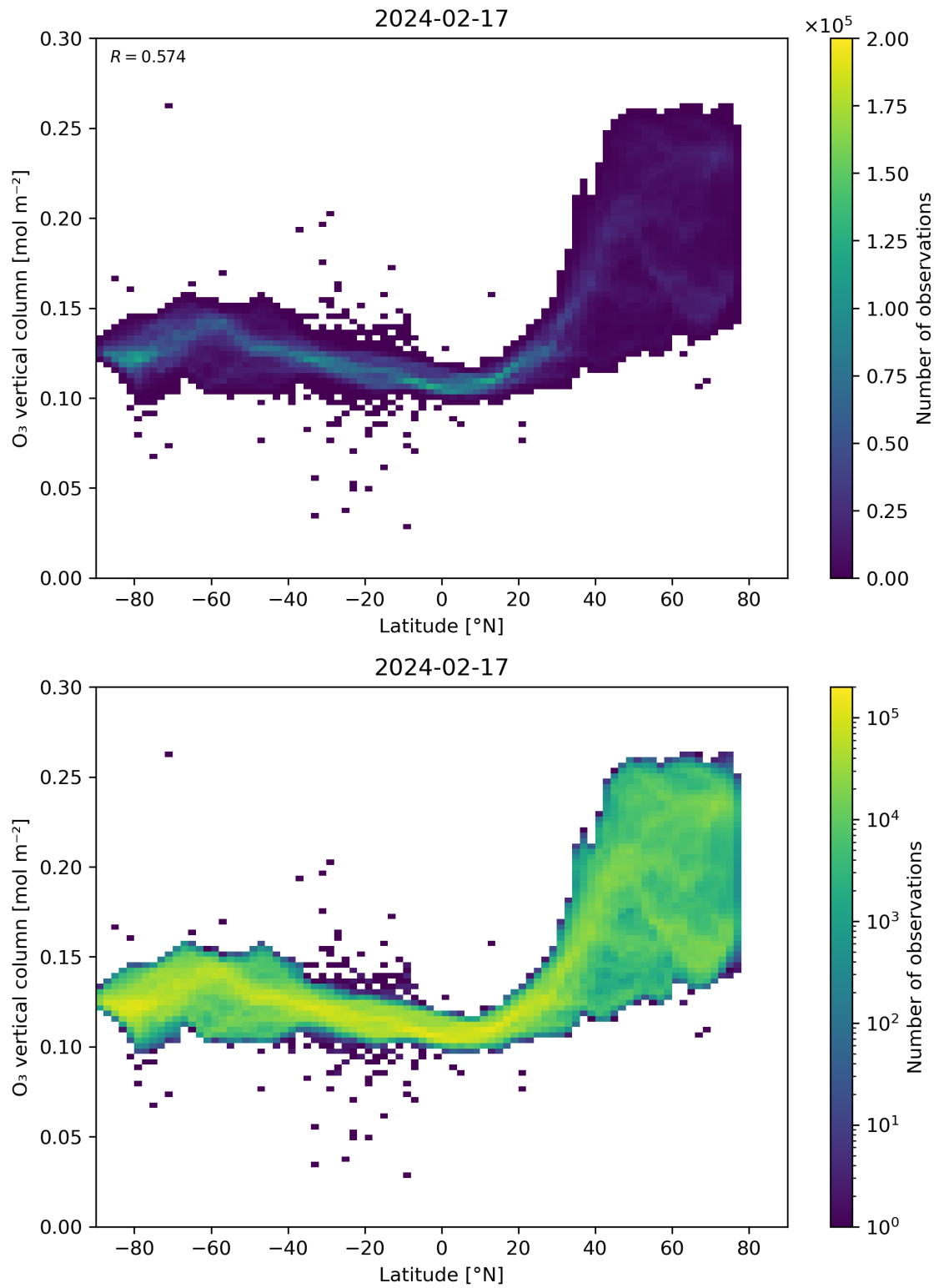
Figure 36: Scatter density plot of “Latitude” against “O 3 vertical column” for 2024-02-17 to 2024-02-18.
