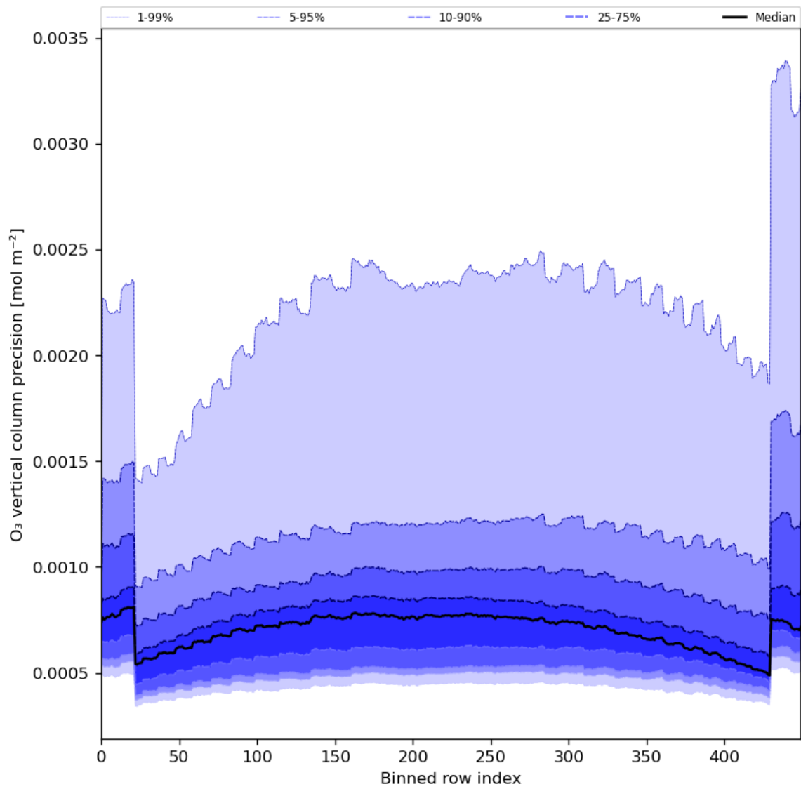
Figure 29: Along track statistics of “O 3 vertical column precision” for 2024-02-17 to 2024-02-18
