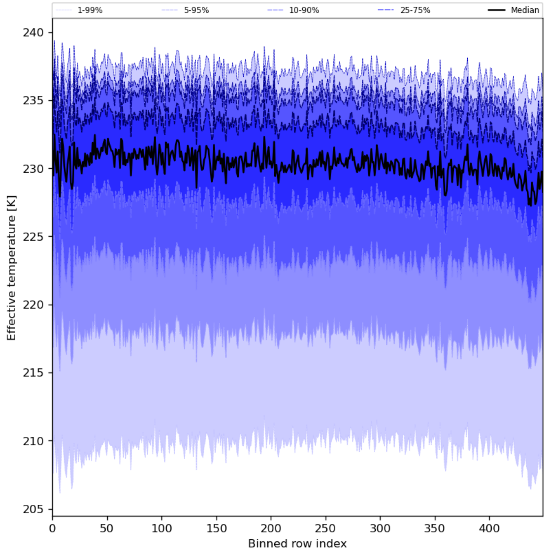
Figure 31: Along track statistics of “Effective temperature” for 2024-02-17 to 2024-02-18
