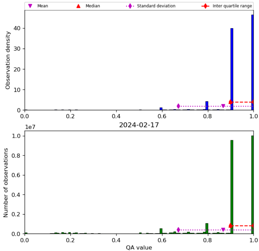
Figure 20: Histogram of “QA value” for 2024-02-17 to 2024-02-18
