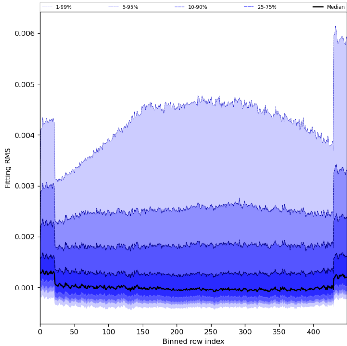
Figure 30: Along track statistics of “Fitting RMS” for 2024-02-17 to 2024-02-18
