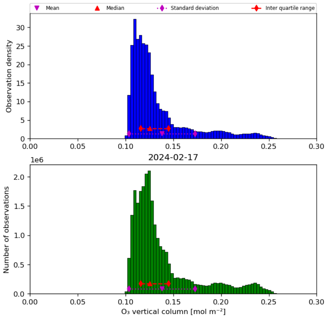
Figure 21: Histogram of “O 3 vertical column” for 2024-02-17 to 2024-02-18
