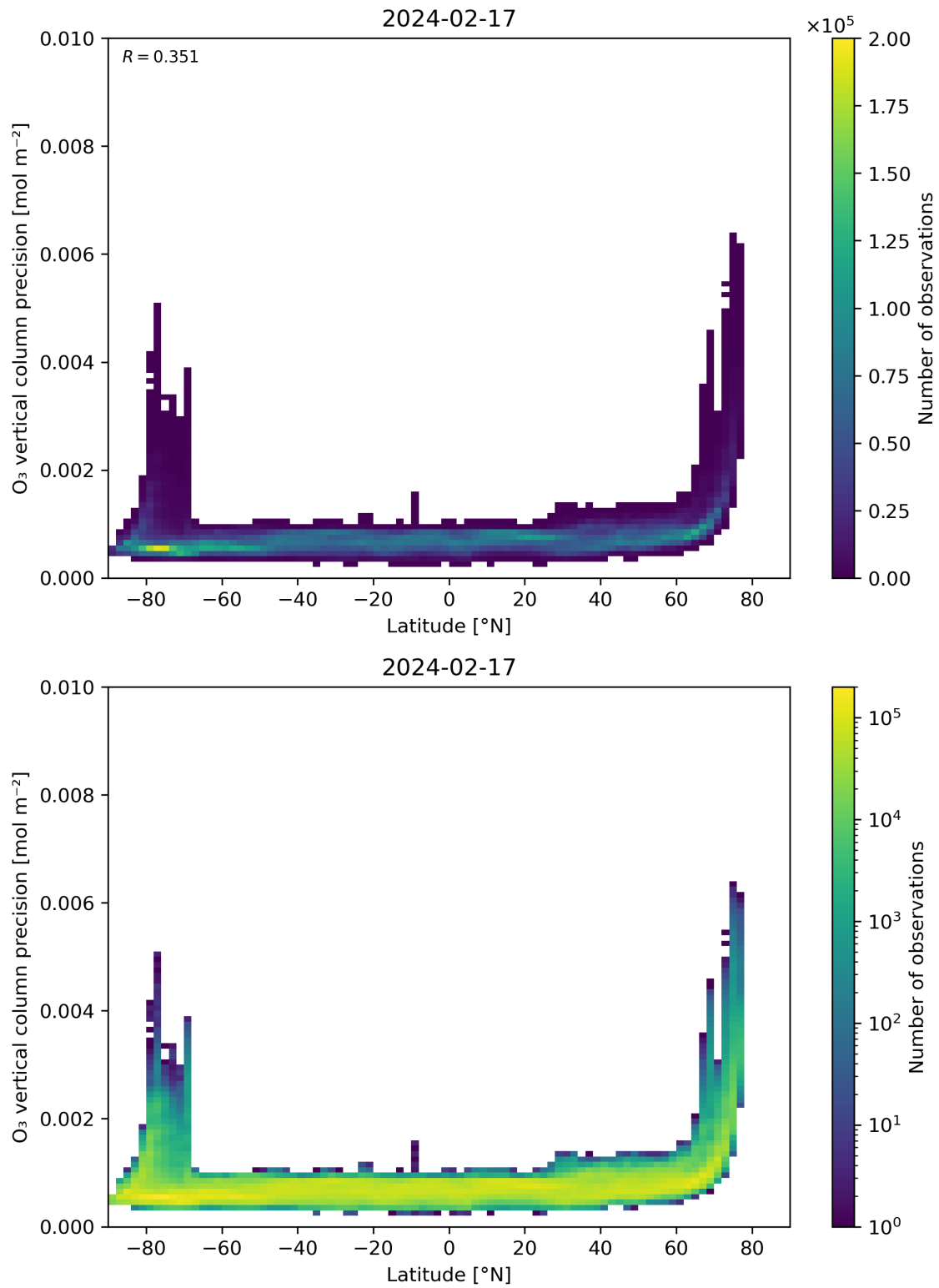
Figure 37: Scatter density plot of “Latitude” against “O 3 vertical column precision” for 2024-02-17 to 2024-02-18.
