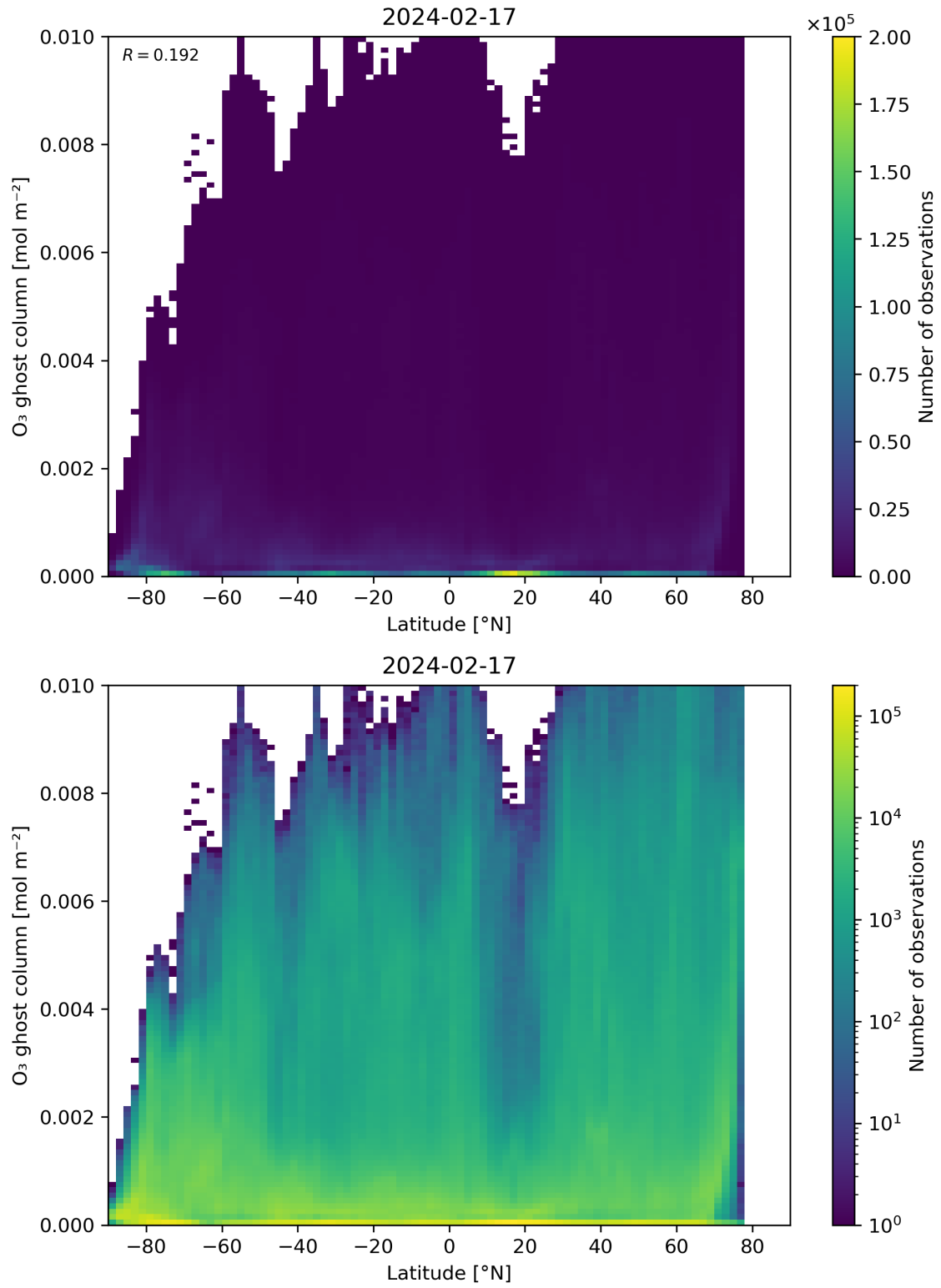
Figure 35: Scatter density plot of “Latitude” against “O 3 ghost column” for 2024-02-17 to 2024-02-18.
