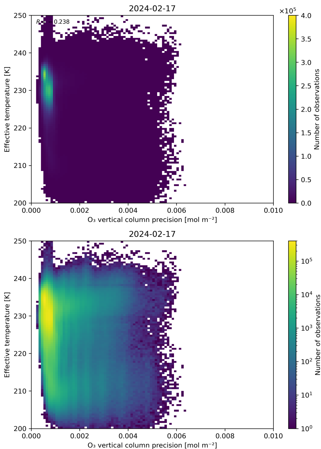
Figure 42: Scatter density plot of “O 3 vertical column precision” against “Effective temperature” for 2024-02-17 to 2024-02-18.
