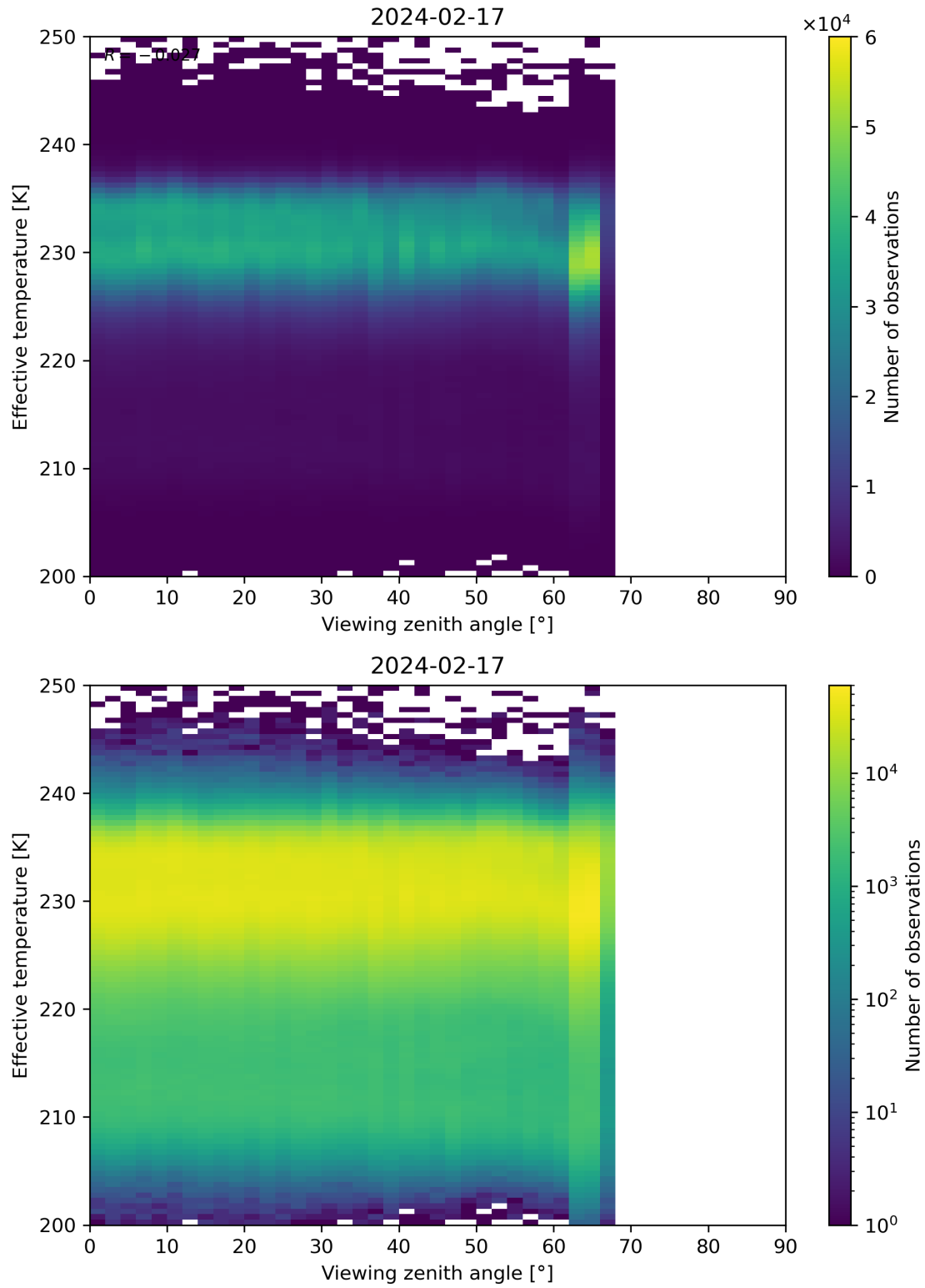
Figure 50: Scatter density plot of “Viewing zenith angle” against “Effective temperature” for 2024-02-17 to 2024-02-18.
