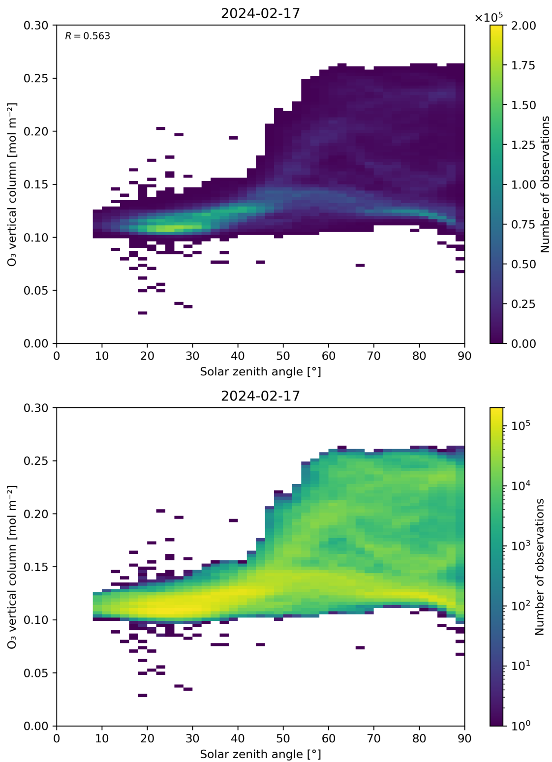
Figure 47: Scatter density plot of “Solar zenith angle” against “O 3 vertical column” for 2024-02-17 to 2024-02-18.
