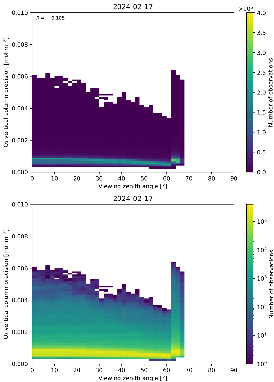
Figure 53: Scatter density plot of “Viewing zenith angle” against “O 3 vertical column precision” for 2024-02-17 to 2024-02-18.
