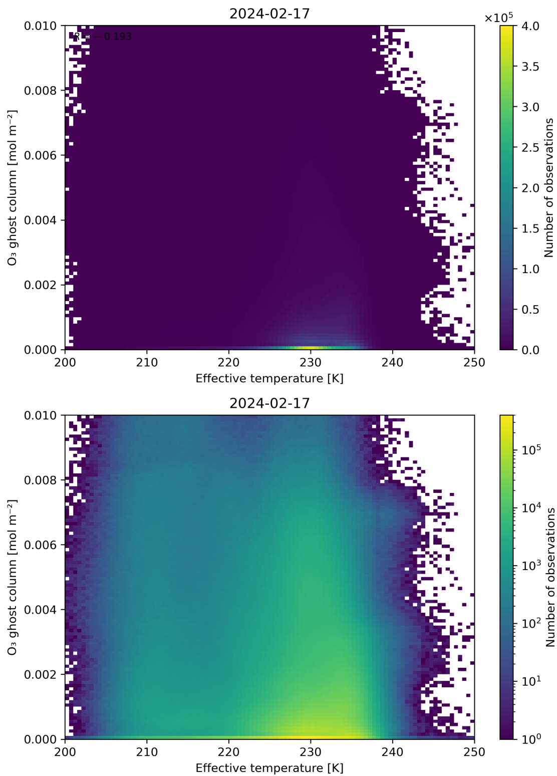
Figure 38: Scatter density plot of “Effective temperature” against “O 3 ghost column” for 2024-02-17 to 2024-02-18.
