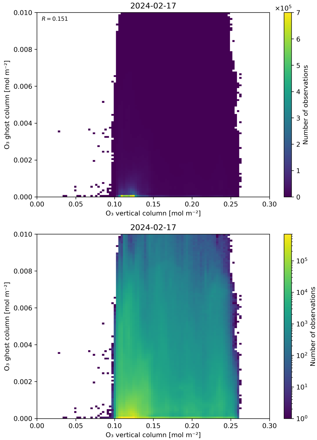
Figure 40: Scatter density plot of “O 3 vertical column” against “O 3 ghost column” for 2024-02-17 to 2024-02-18.
