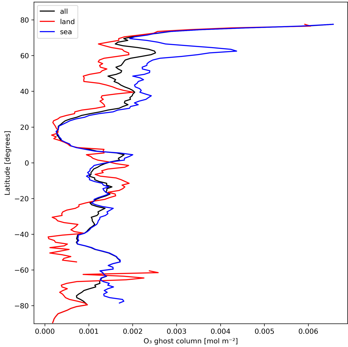
Figure 18: Zonal average of “O 3 ghost column” for 2024-02-17 to 2024-02-18.
