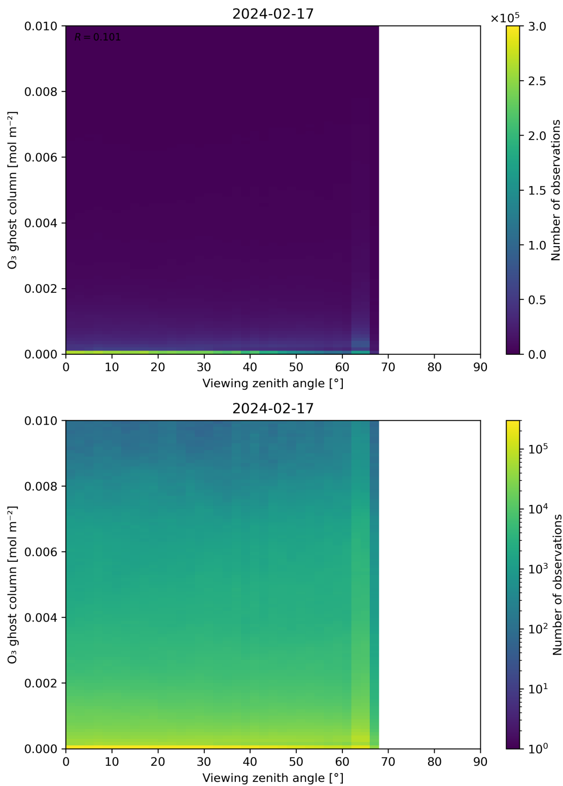
Figure 51: Scatter density plot of “Viewing zenith angle” against “O 3 ghost column” for 2024-02-17 to 2024-02-18.
