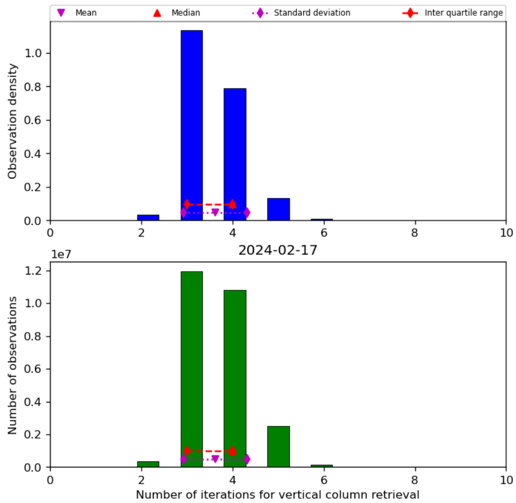
Figure 26: Histogram of “Number of iterations for vertical column retrieval” for 2024-02-17 to 2024-02-18
