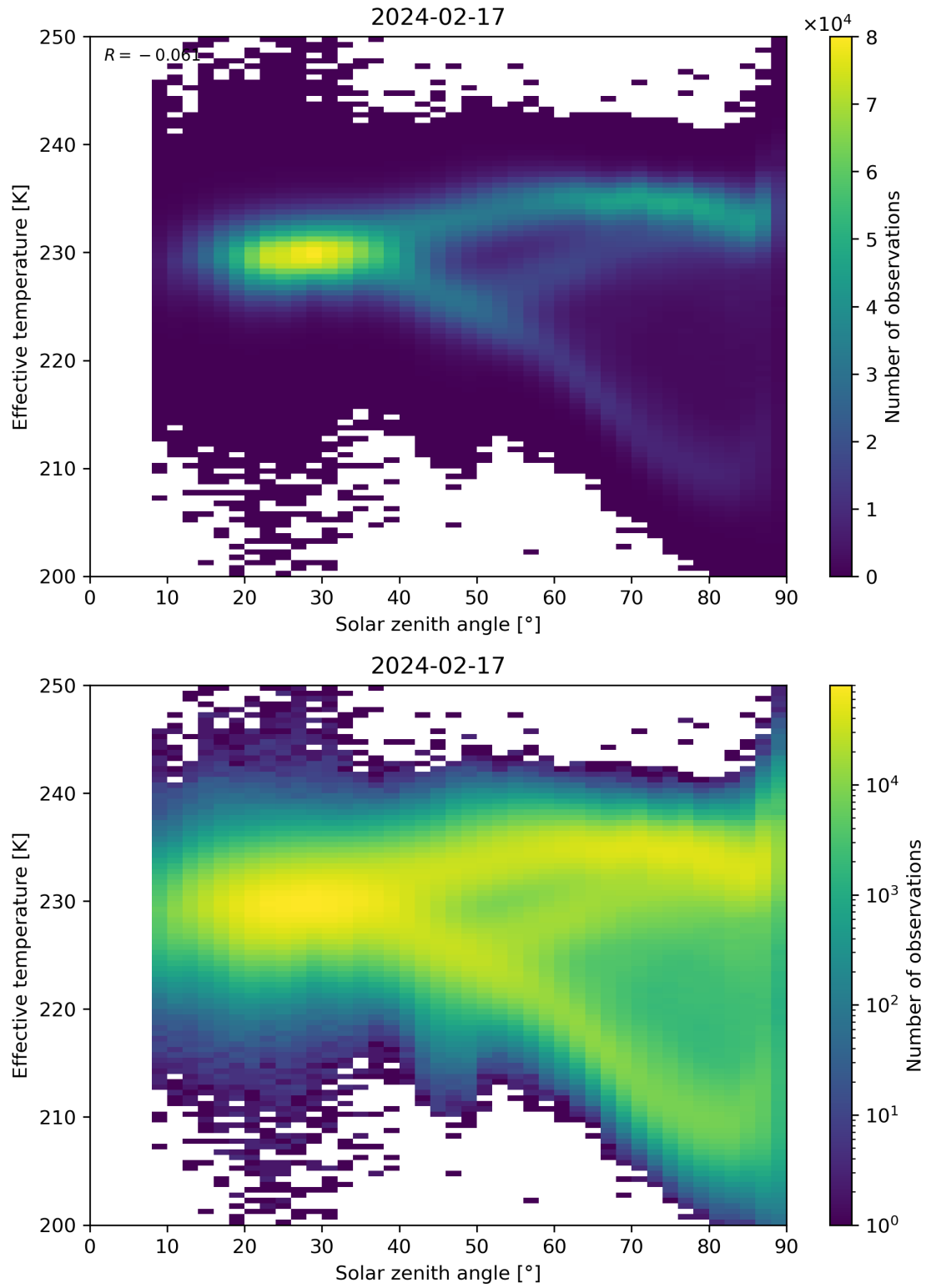
Figure 45: Scatter density plot of “Solar zenith angle” against “Effective temperature” for 2024-02-17 to 2024-02-18.
