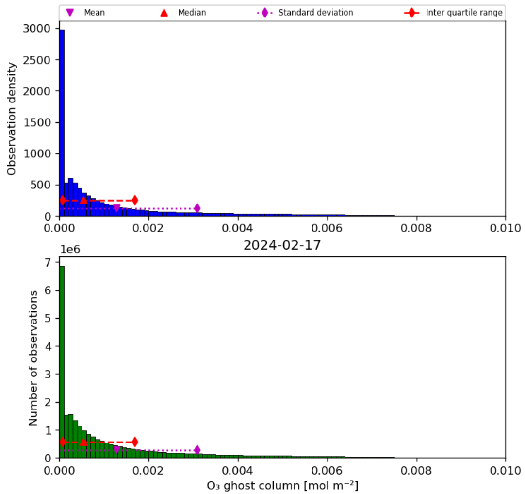
Figure 25: Histogram of “O 3 ghost column” for 2024-02-17 to 2024-02-18
