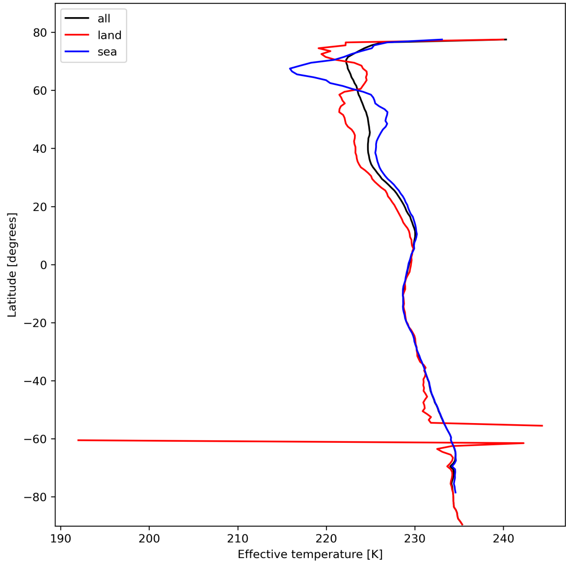
Figure 17: Zonal average of “Effective temperature” for 2024-02-17 to 2024-02-18.
