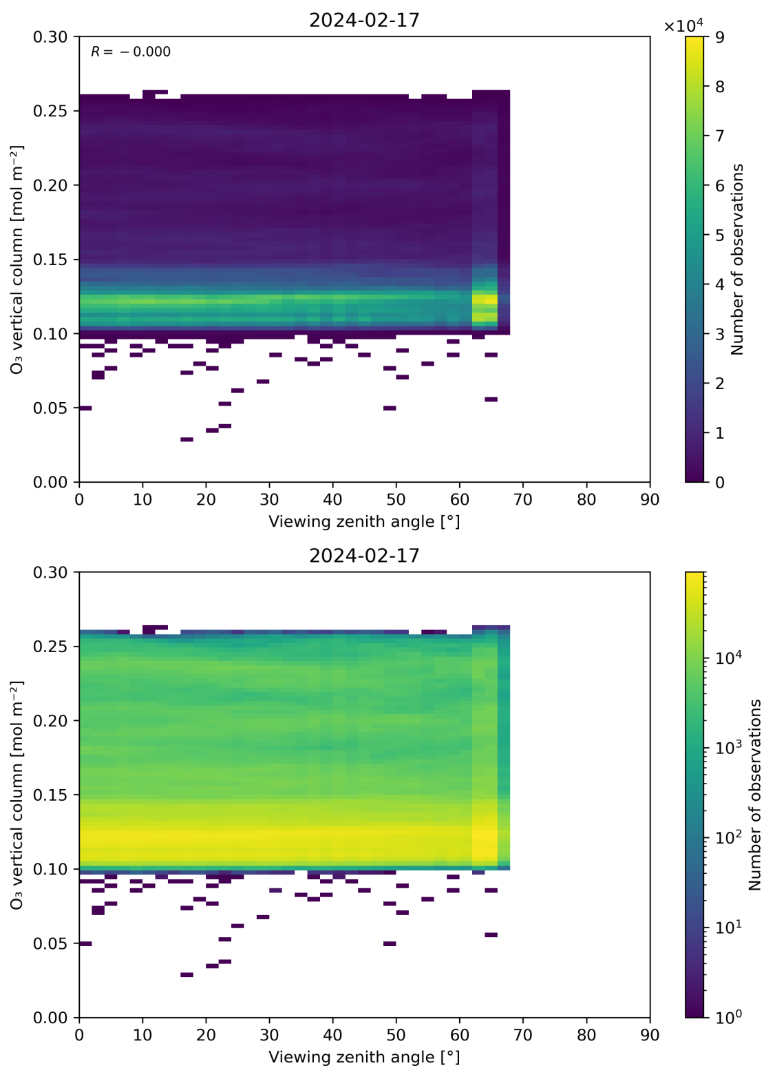
Figure 52: Scatter density plot of “Viewing zenith angle” against “O 3 vertical column” for 2024-02-17 to 2024-02-18.
