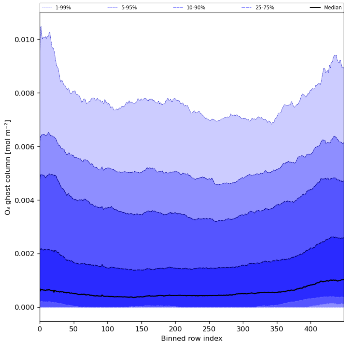
Figure 32: Along track statistics of “O 3 ghost column” for 2024-02-17 to 2024-02-18
