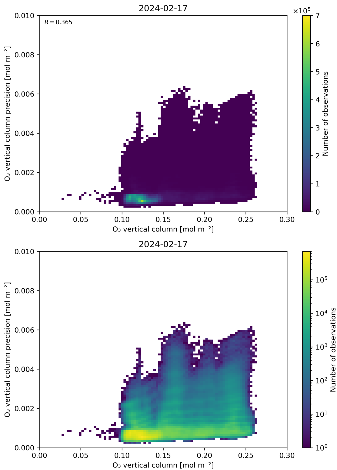
Figure 41: Scatter density plot of “O 3 vertical column” against “O 3 vertical column precision” for 2024-02-17 to 2024-02-18.
