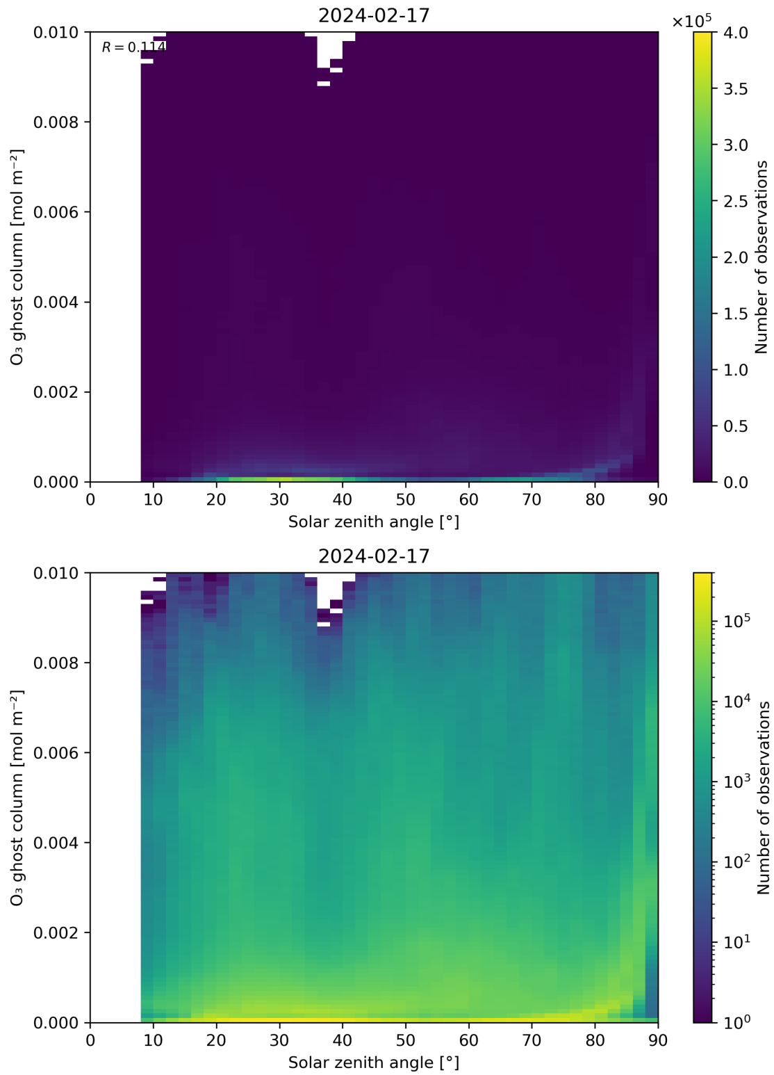
Figure 46: Scatter density plot of “Solar zenith angle” against “O 3 ghost column” for 2024-02-17 to 2024-02-18.
