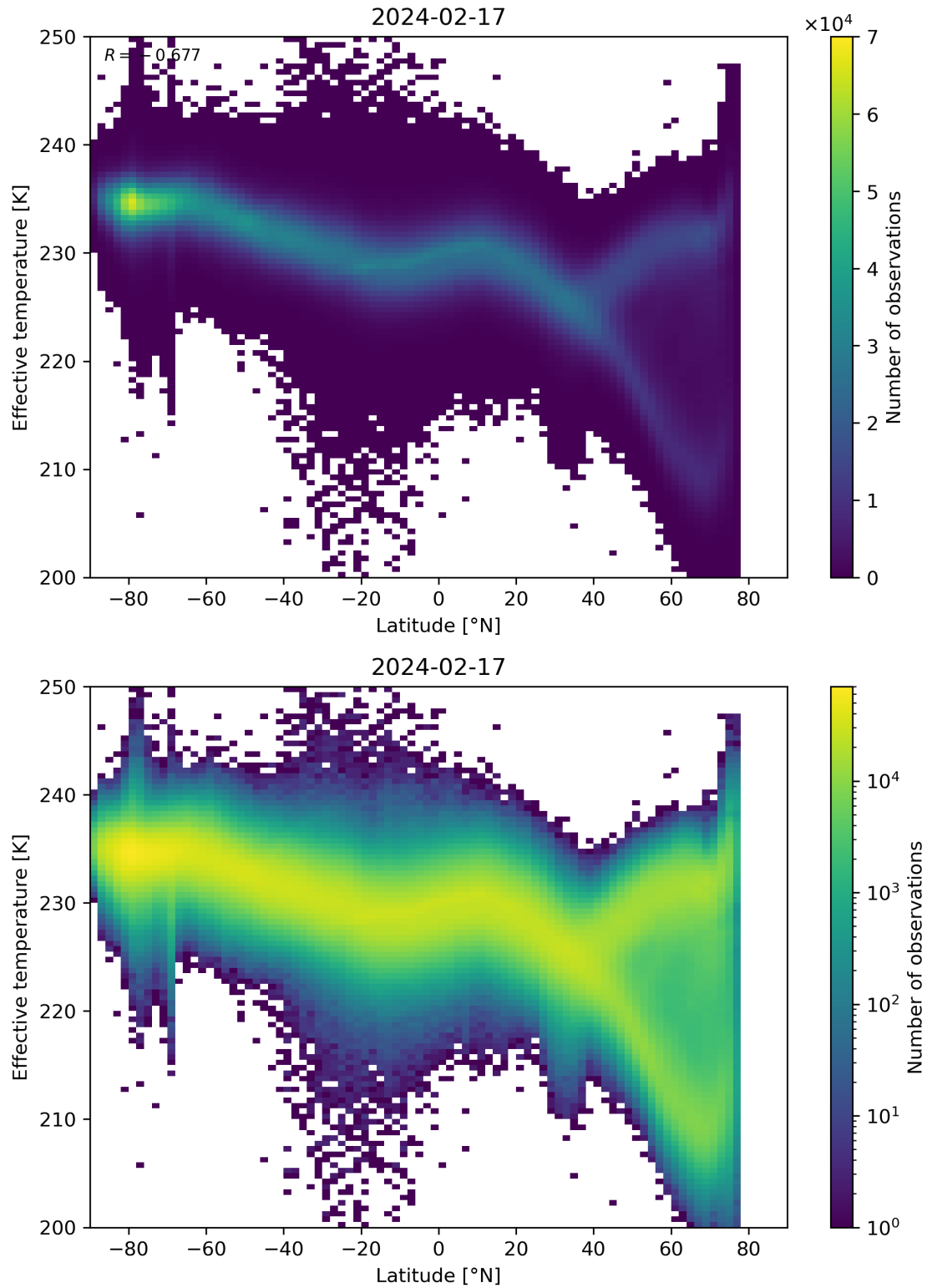
Figure 34: Scatter density plot of “Latitude” against “Effective temperature” for 2024-02-17 to 2024-02-18.
