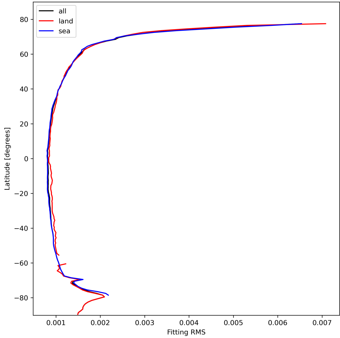
Figure 16: Zonal average of “Fitting RMS” for 2024-02-17 to 2024-02-18.
