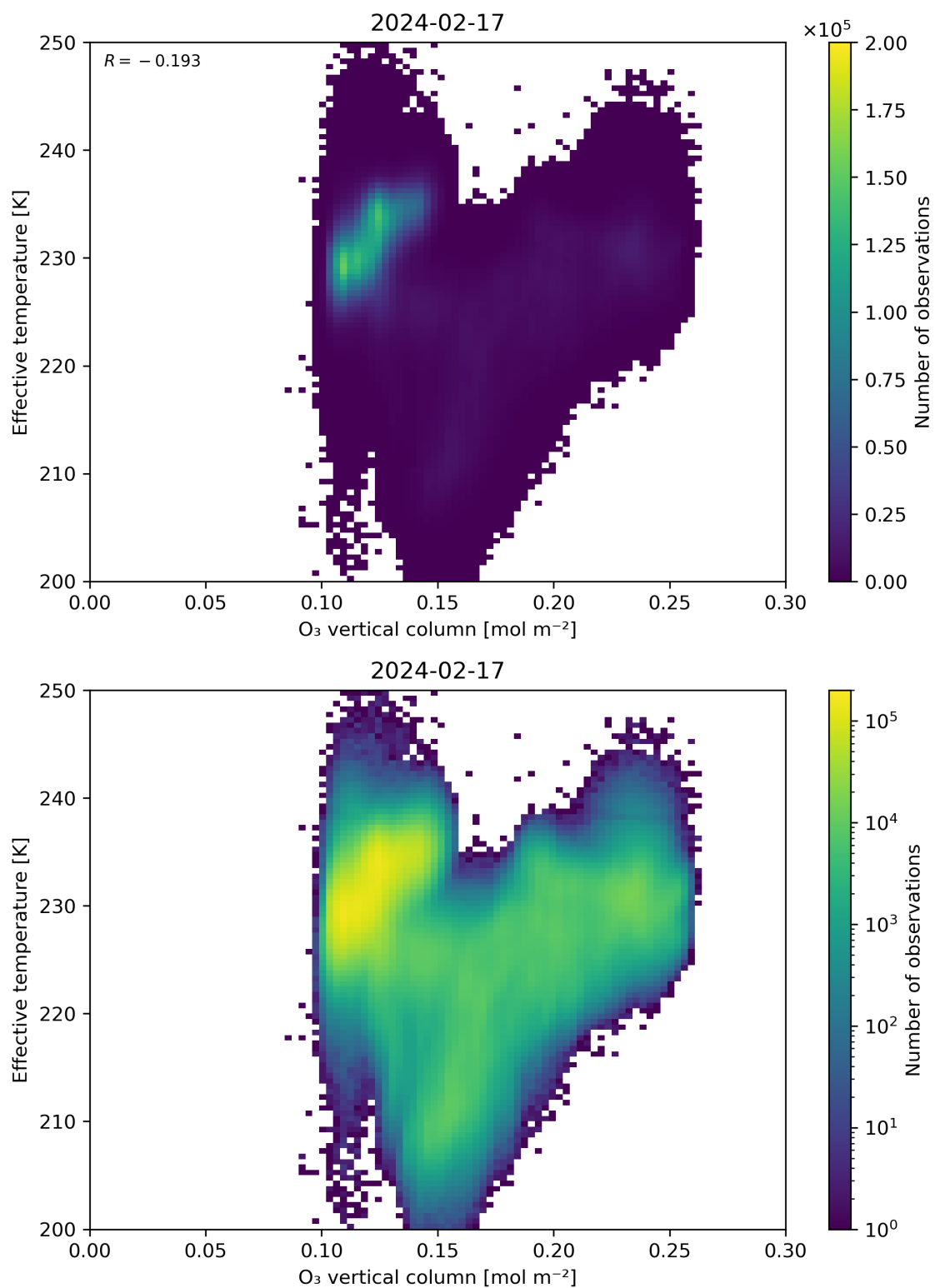
Figure 39: Scatter density plot of “O 3 vertical column” against “Effective temperature” for 2024-02-17 to 2024-02-18.
