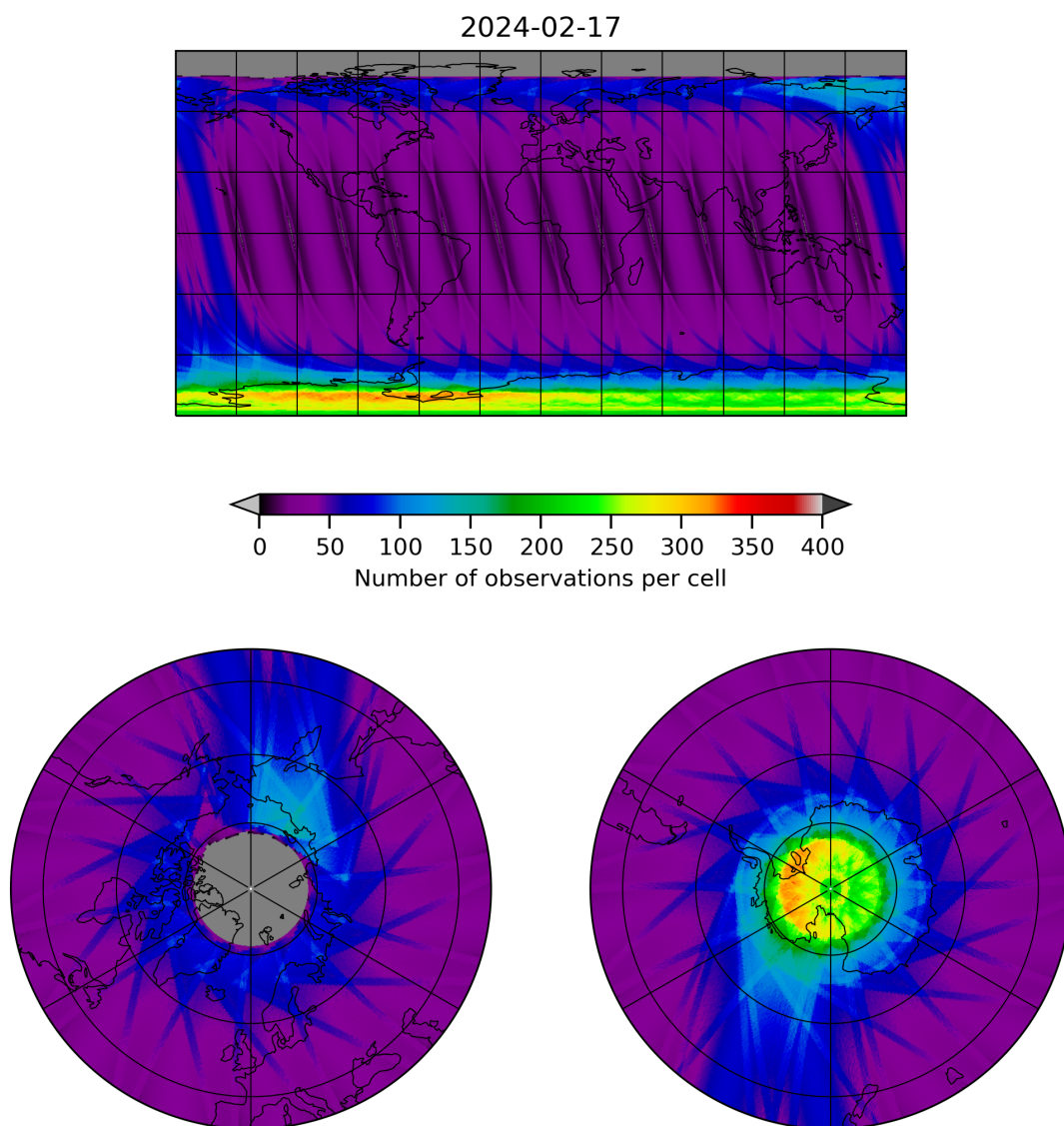
Figure 12: Map of the number of observations for 2024-02-17 to 2024-02-18
