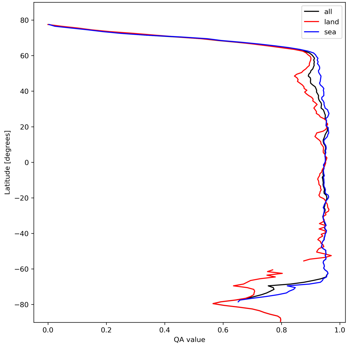
Figure 13: Zonal average of “QA value” for 2024-02-17 to 2024-02-18.
