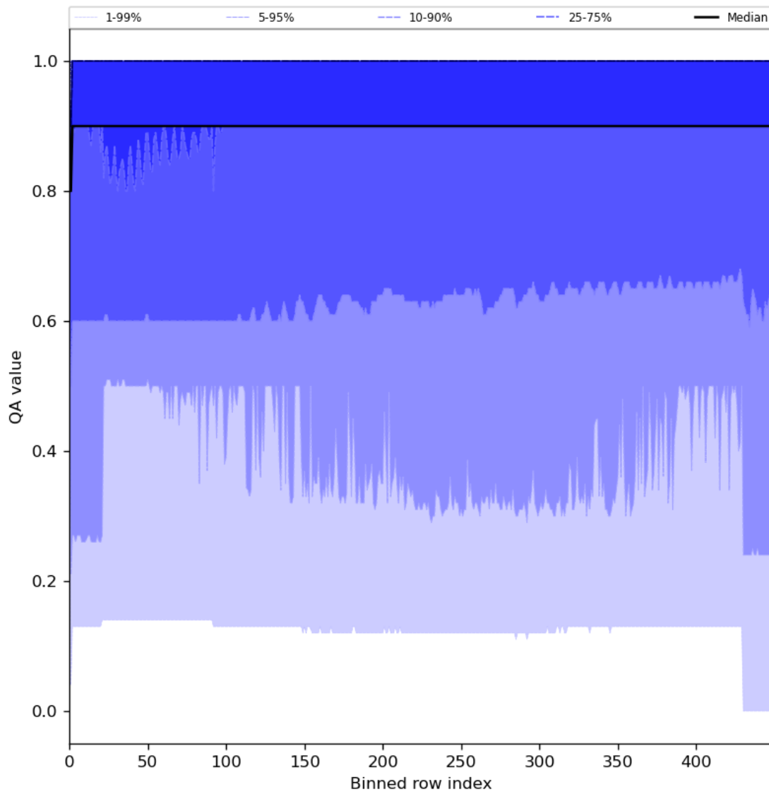
Figure 27: Along track statistics of “QA value” for 2024-02-17 to 2024-02-18
