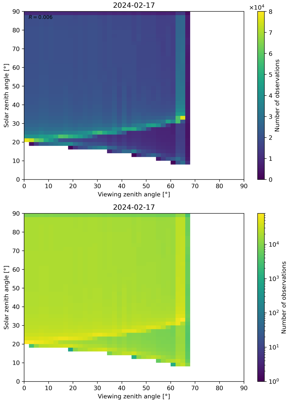
Figure 54: Scatter density plot of “Viewing zenith angle” against “Solar zenith angle” for 2024-02-17 to 2024-02-18.
