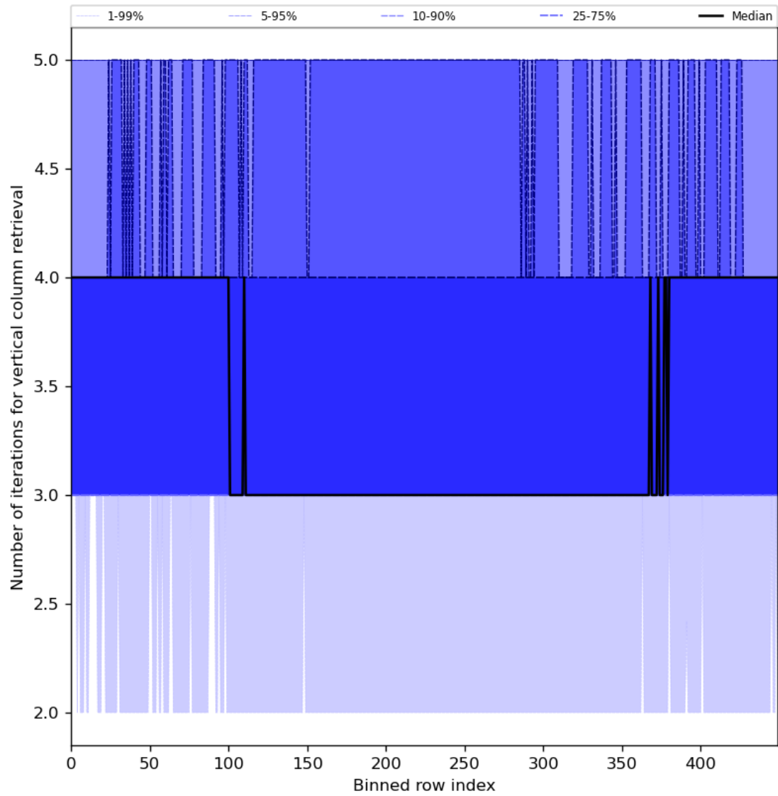
Figure 33: Along track statistics of “Number of iterations for vertical column retrieval” for 2024-02-17 to 2024-02-18
