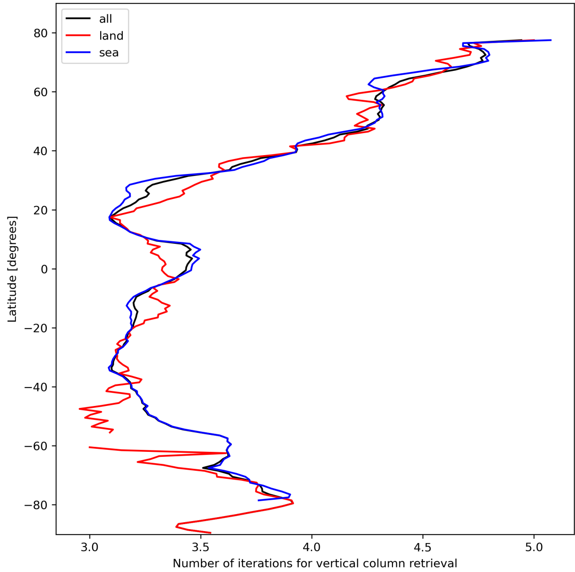
Figure 19: Zonal average of “Number of iterations for vertical column retrieval” for 2024-02-17 to 2024-02-18.
