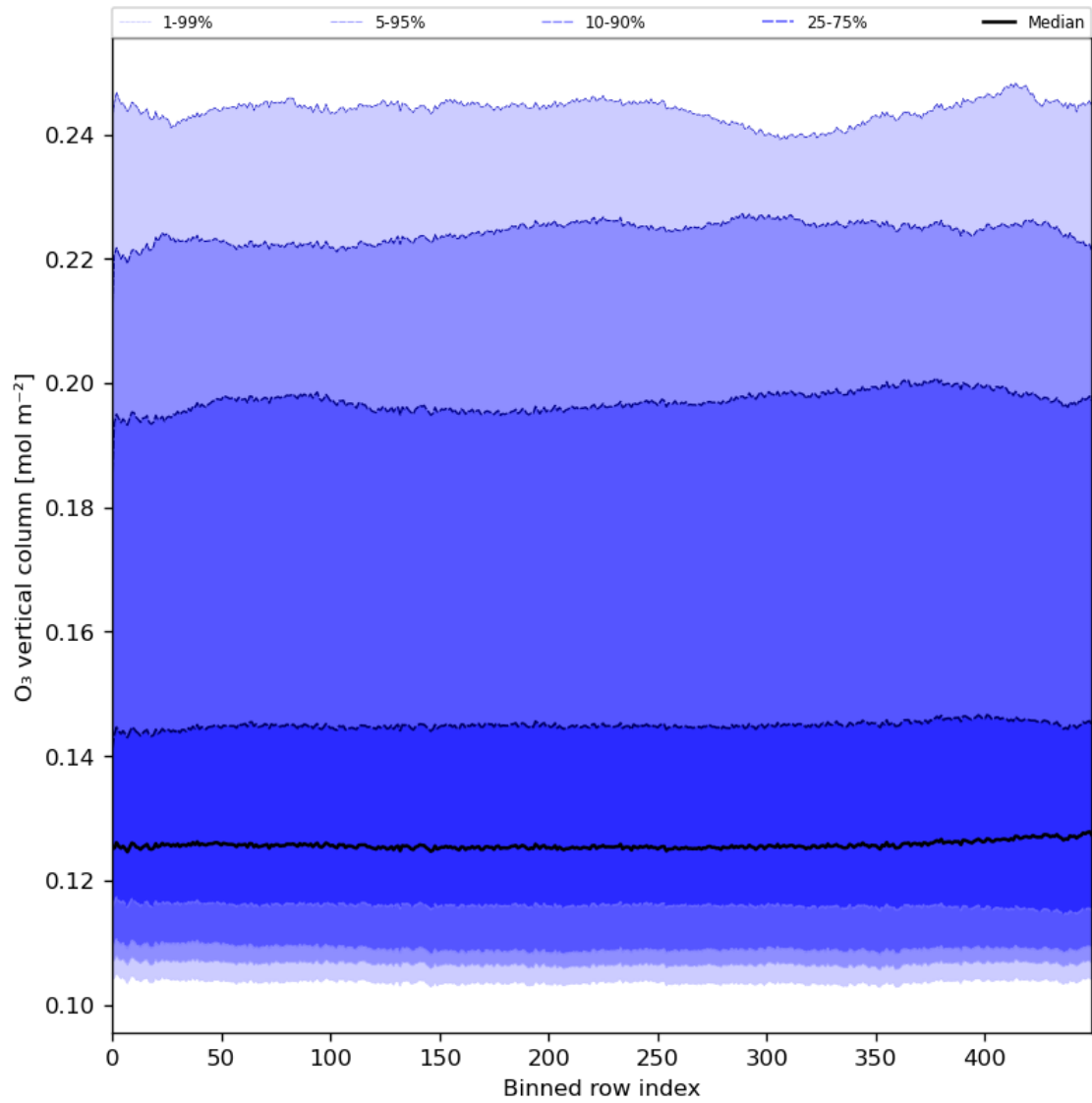
Figure 28: Along track statistics of “O 3 vertical column” for 2024-02-17 to 2024-02-18
