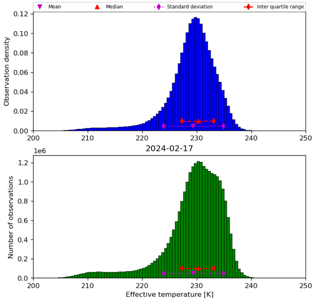
Figure 24: Histogram of “Effective temperature” for 2024-02-17 to 2024-02-18
