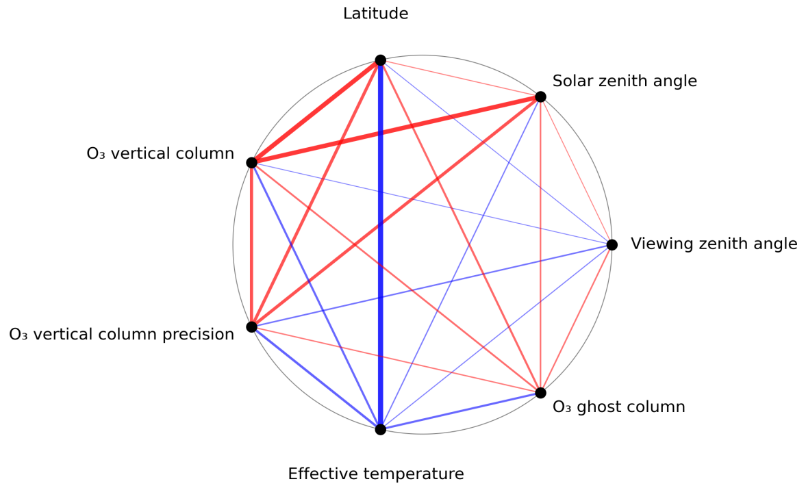
Figure 1: Map of correlation graph for 2024-02-17 to 2024-02-18.
