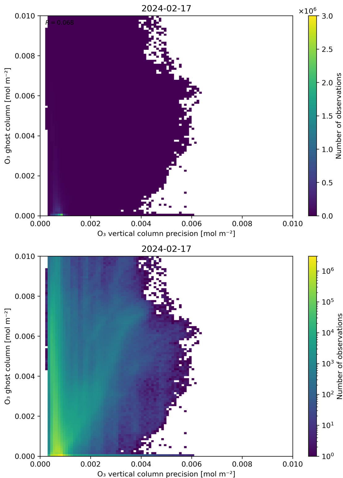
Figure 43: Scatter density plot of “ \text{O}_3 vertical column precision” against “ \text{O}_3 ghost column” for 2024-02-17 to 2024-02-18.
