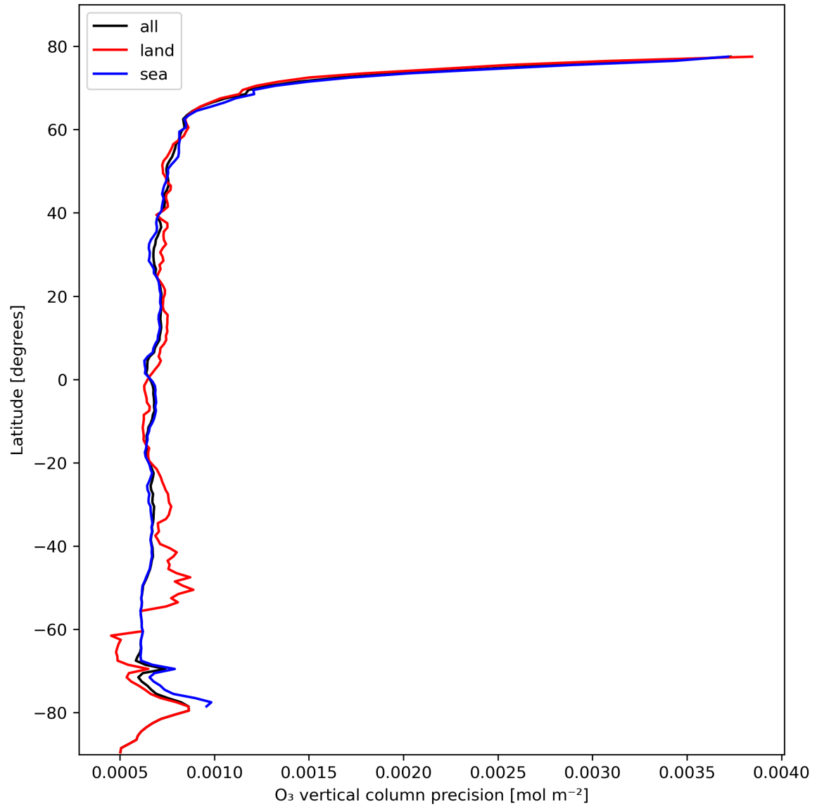
Figure 15: Zonal average of “O 3 vertical column precision” for 2024-02-17 to 2024-02-18.
