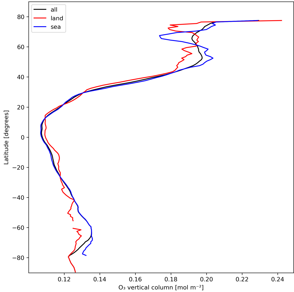
Figure 14: Zonal average of “O 3 vertical column” for 2024-02-17 to 2024-02-18.
