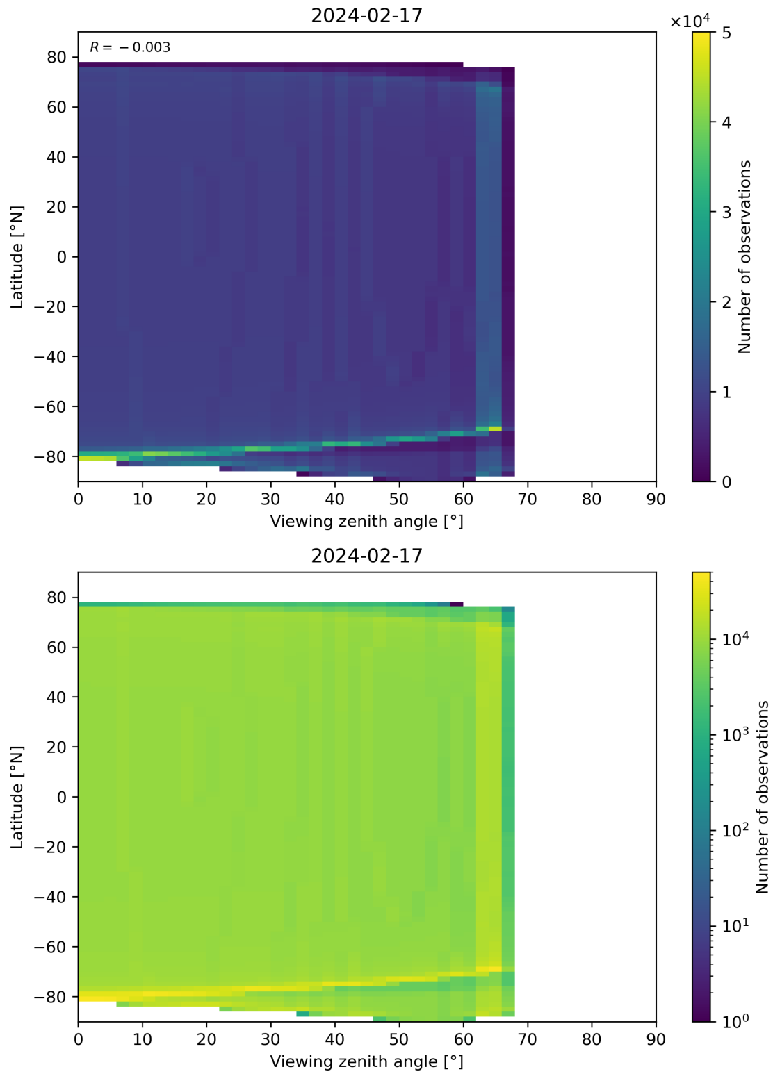
Figure 49: Scatter density plot of “Viewing zenith angle” against “Latitude” for 2024-02-17 to 2024-02-18.
