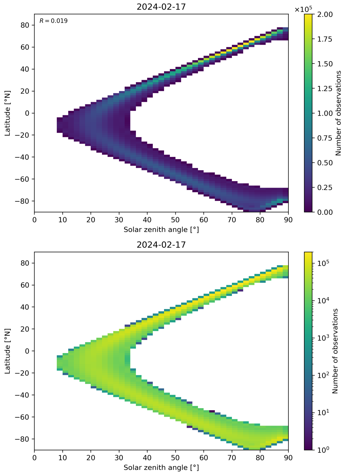
Figure 44: Scatter density plot of “Solar zenith angle” against “Latitude” for 2024-02-17 to 2024-02-18.
