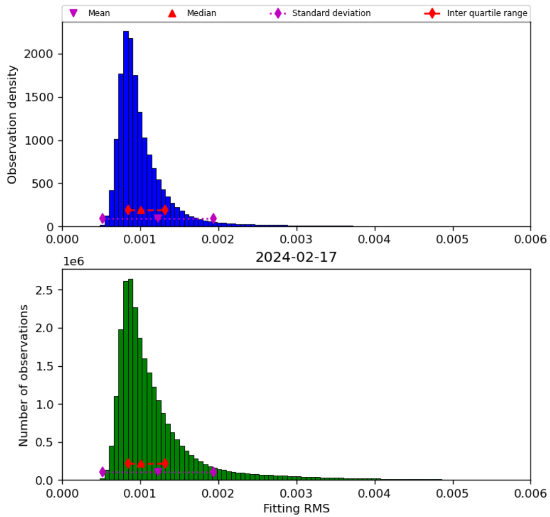
Figure 23: Histogram of “Fitting RMS” for 2024-02-17 to 2024-02-18
