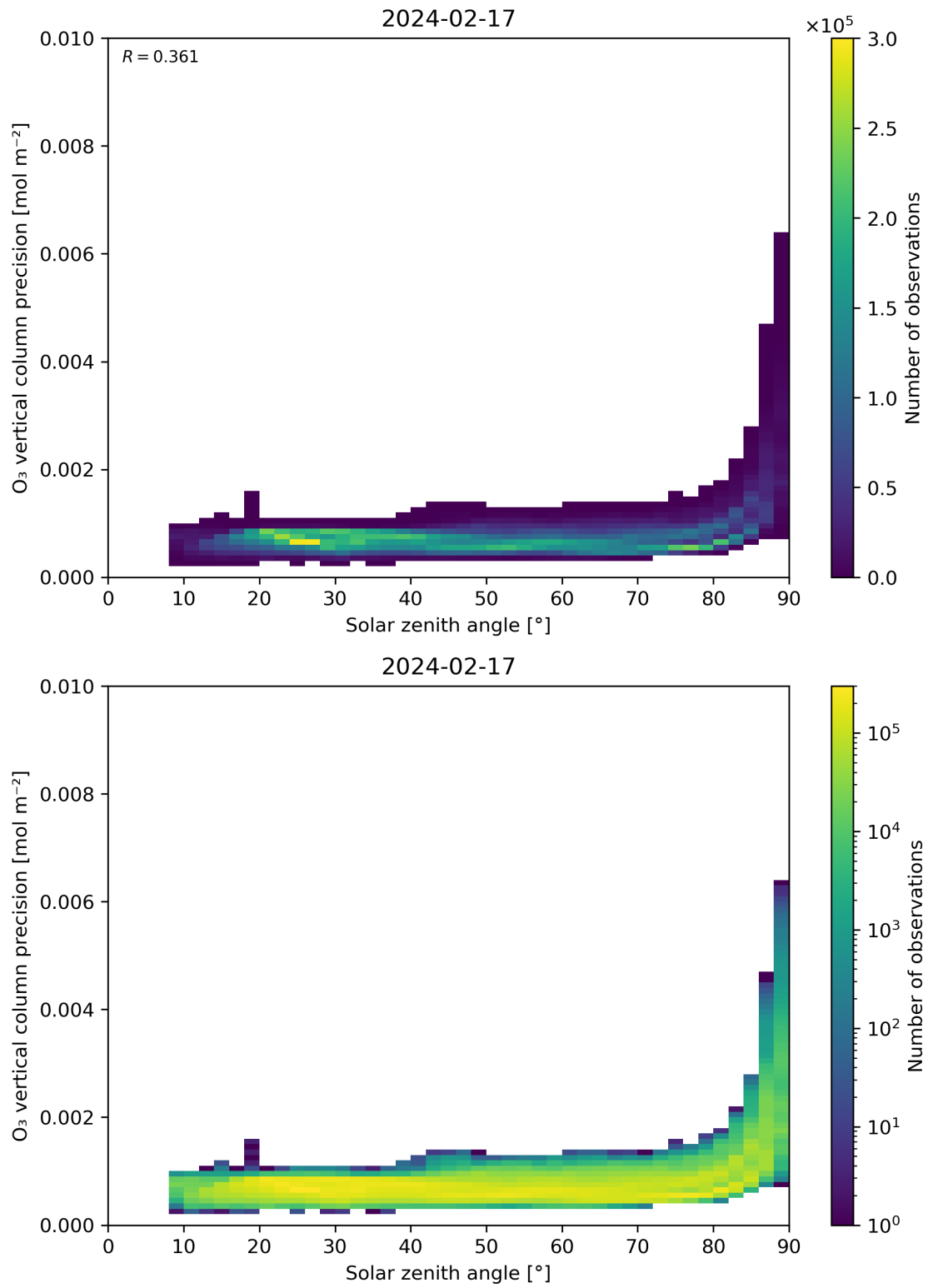
Figure 48: Scatter density plot of “Solar zenith angle” against “O 3 vertical column precision” for 2024-02-17 to 2024-02-18.
