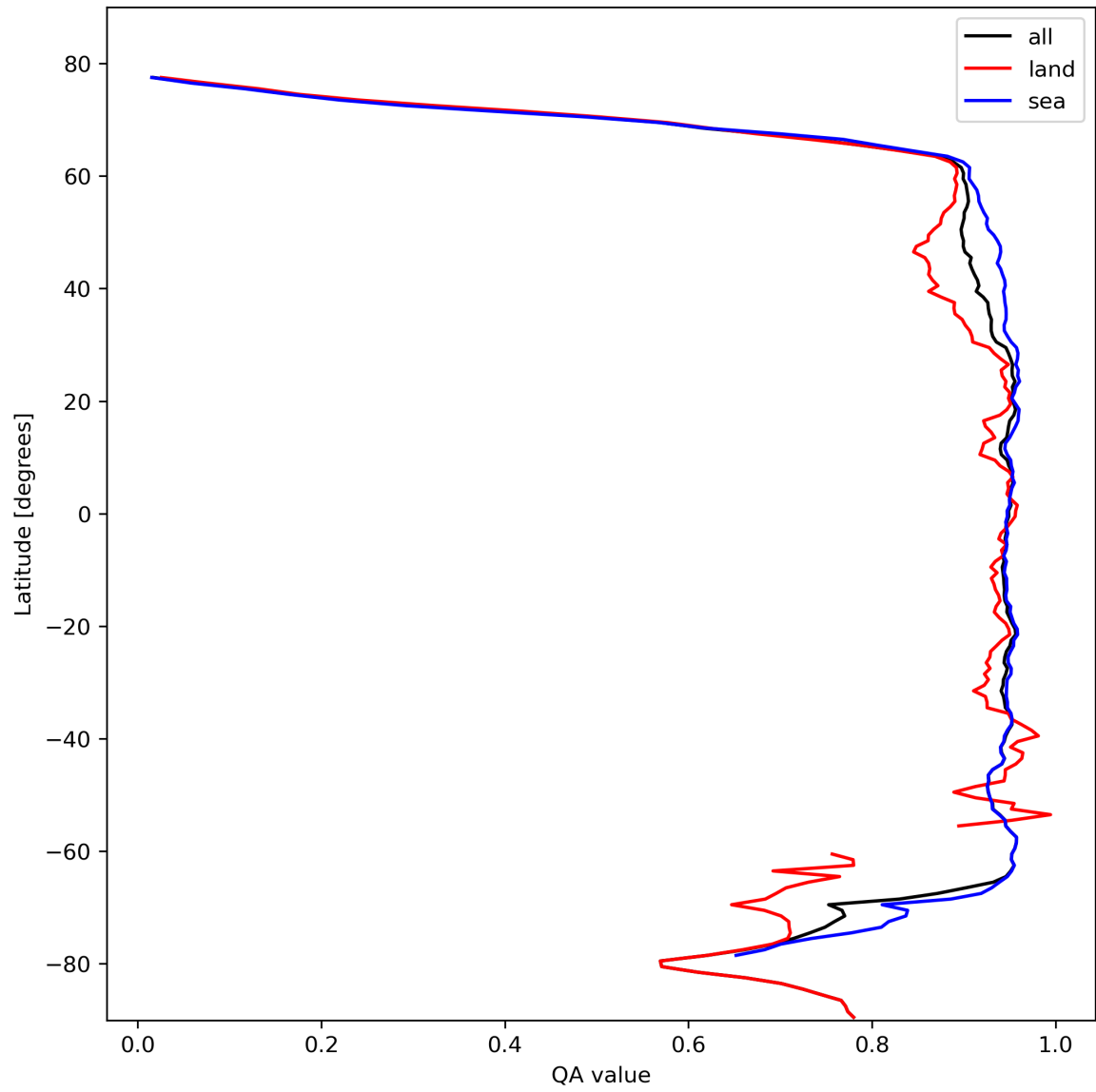
Figure 13: Zonal average of “QA value” for 2024-02-18 to 2024-02-20.
