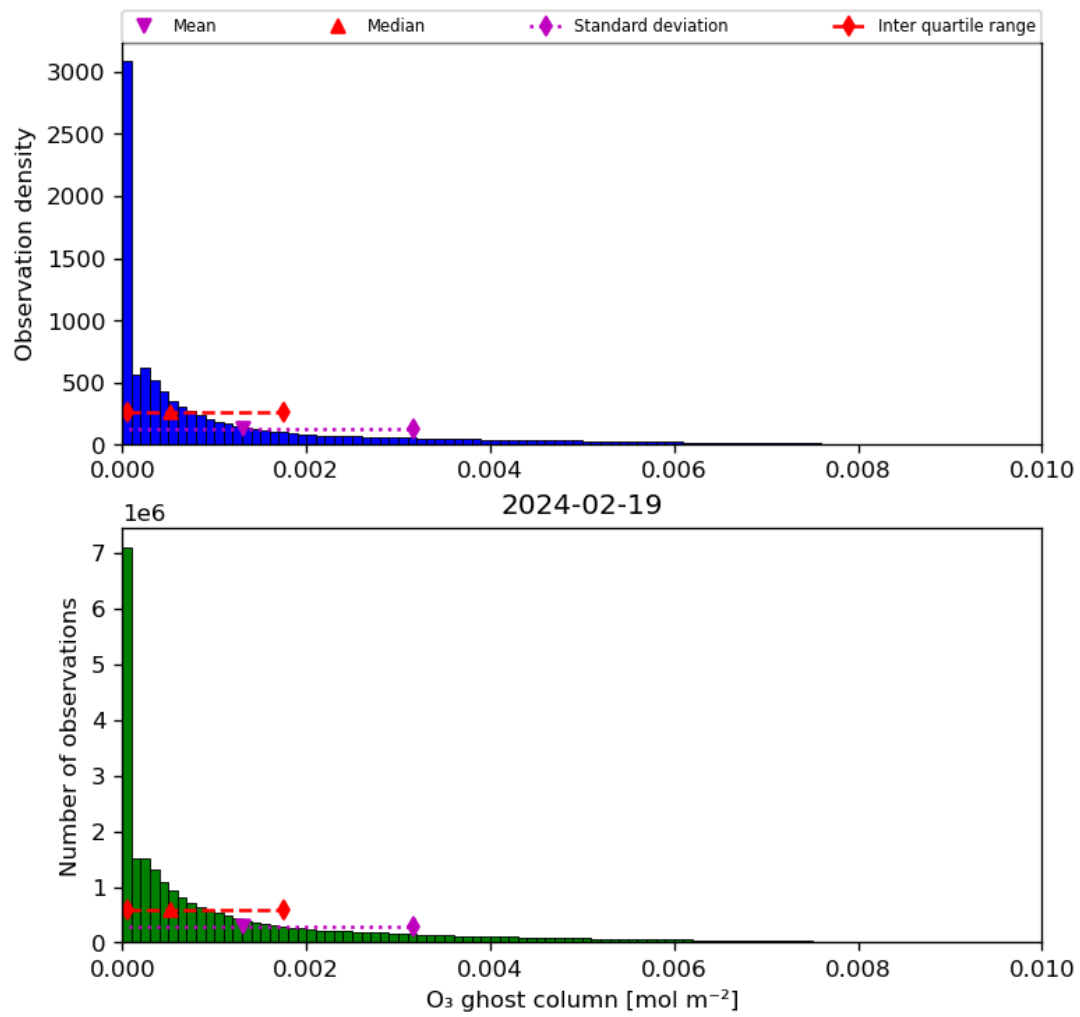
Figure 25: Histogram of “O 3 ghost column” for 2024-02-18 to 2024-02-20
