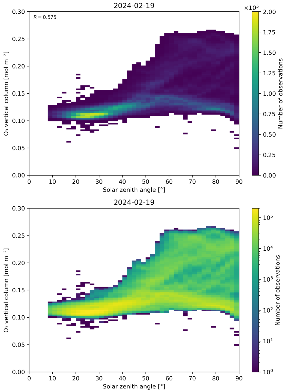
Figure 47: Scatter density plot of “Solar zenith angle” against “O 3 vertical column” for 2024-02-18 to 2024-02-20.
