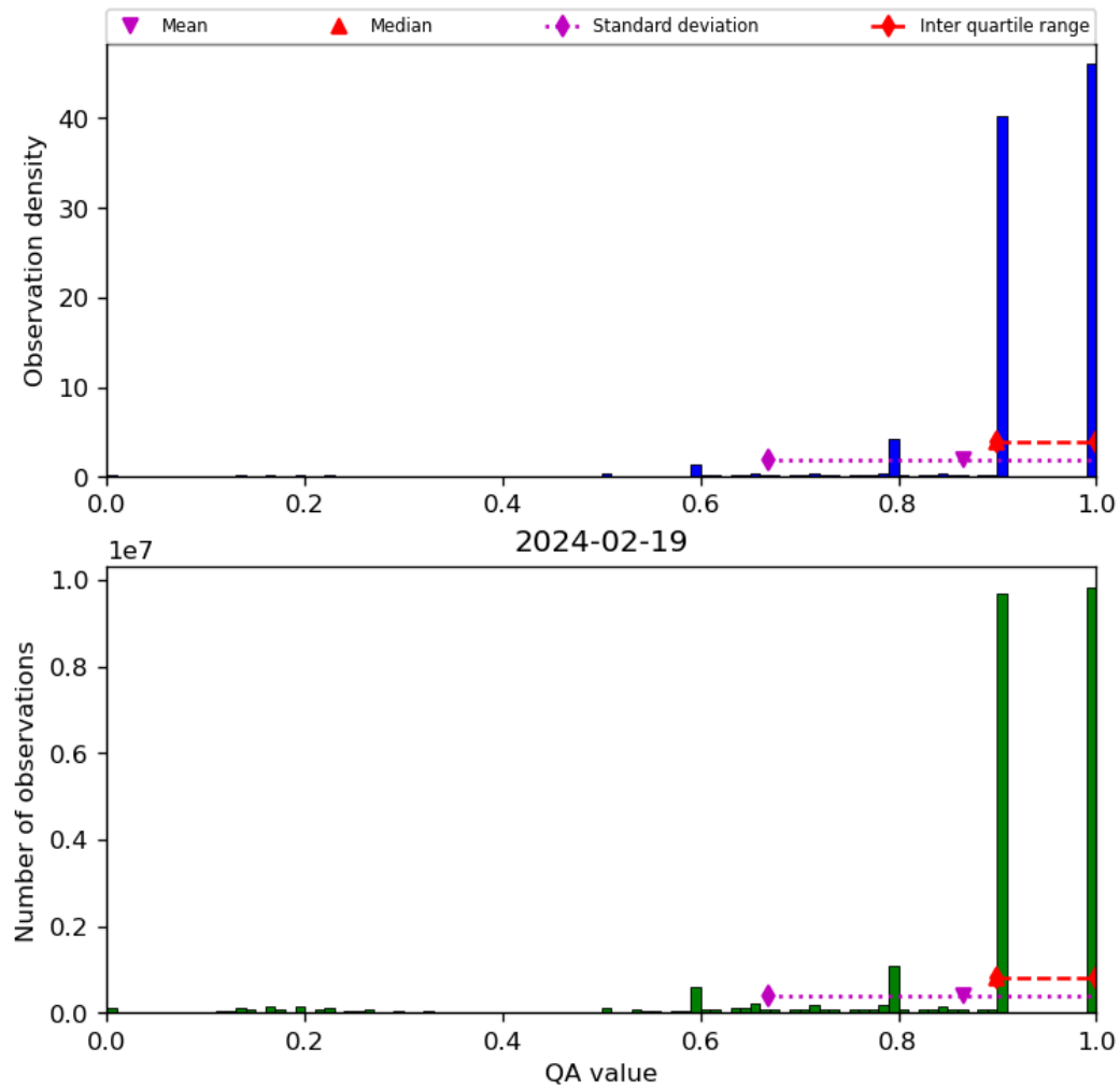
Figure 20: Histogram of “QA value” for 2024-02-18 to 2024-02-20
