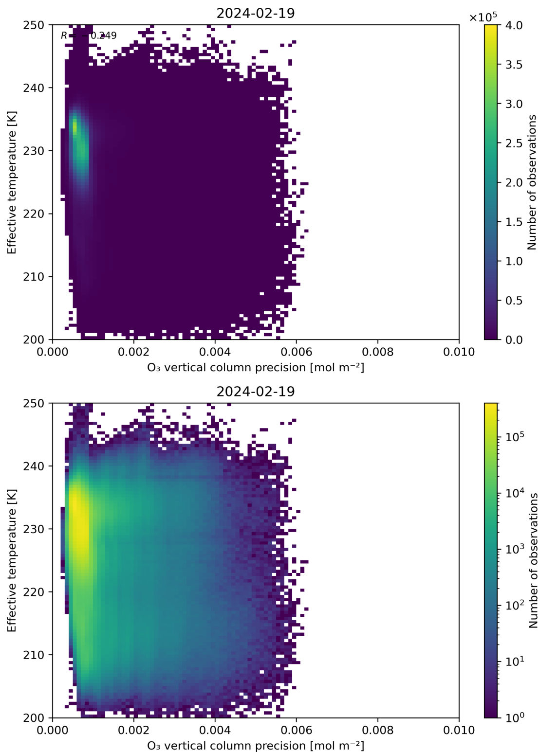
Figure 42: Scatter density plot of “O 3 vertical column precision” against “Effective temperature” for 2024-02-18 to 2024-02-20.
