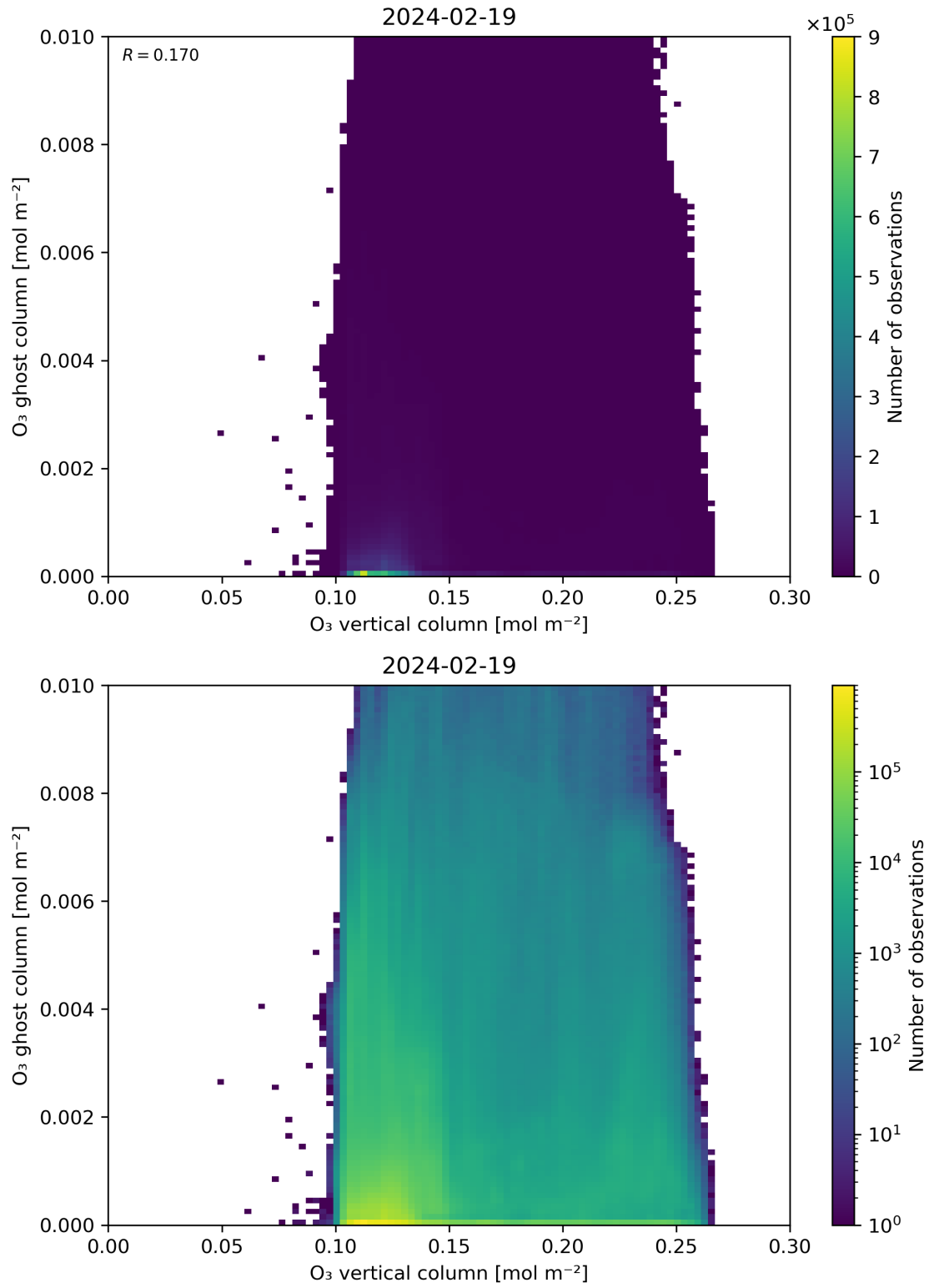
Figure 40: Scatter density plot of “O 3 vertical column” against “O 3 ghost column” for 2024-02-18 to 2024-02-20.
