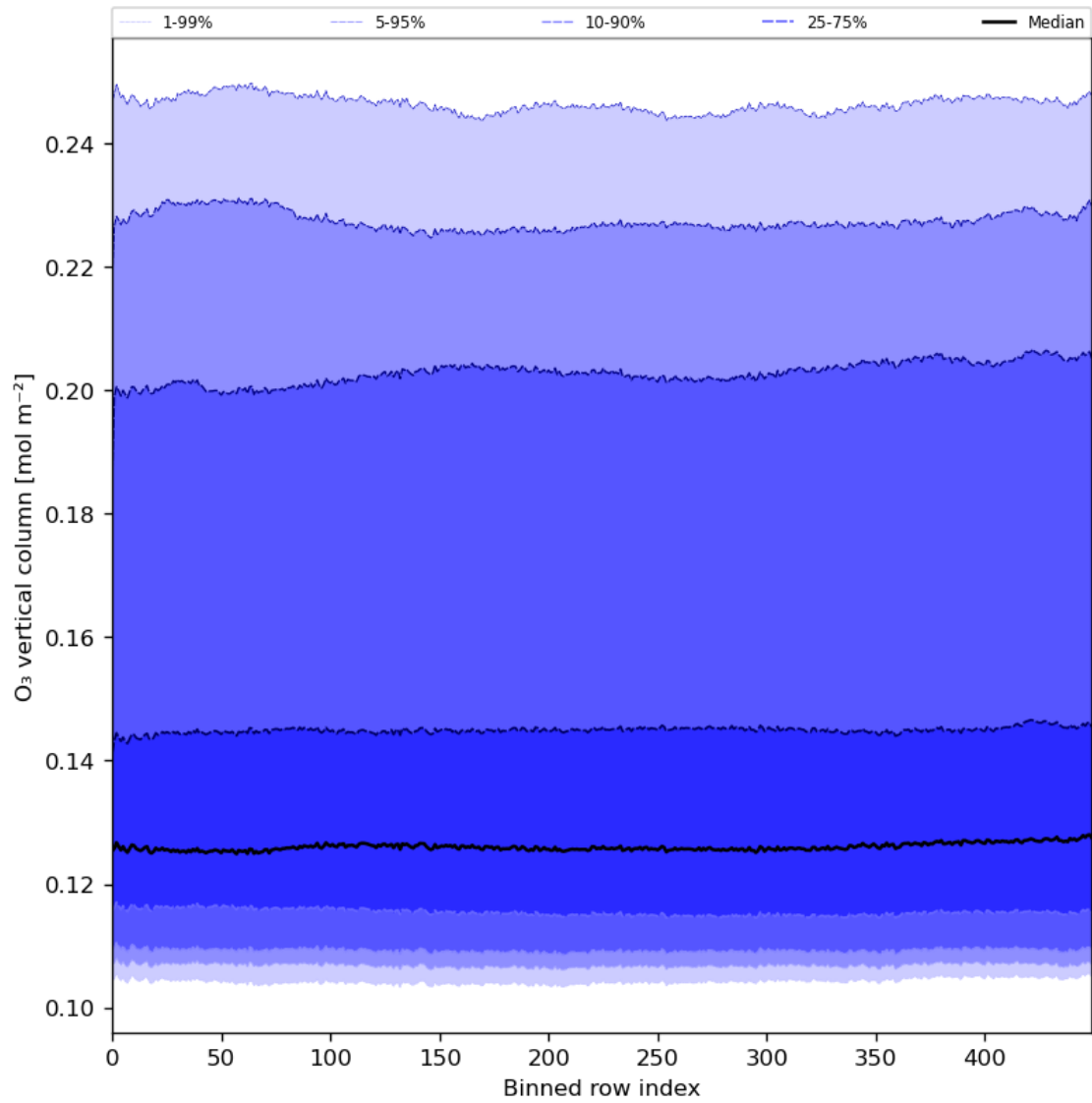
Figure 28: Along track statistics of “O 3 vertical column” for 2024-02-18 to 2024-02-20
