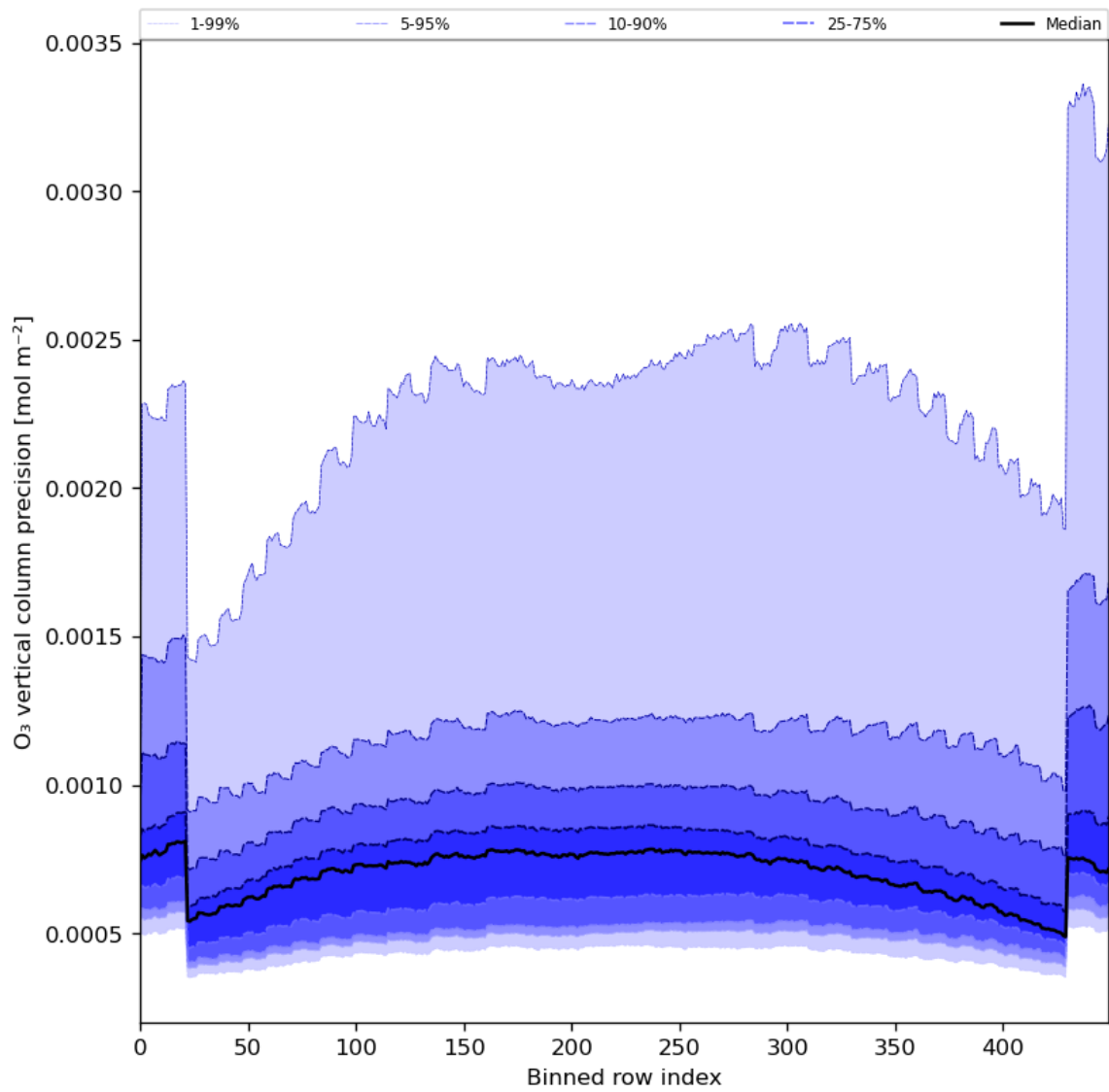
Figure 29: Along track statistics of “O 3 vertical column precision” for 2024-02-18 to 2024-02-20
