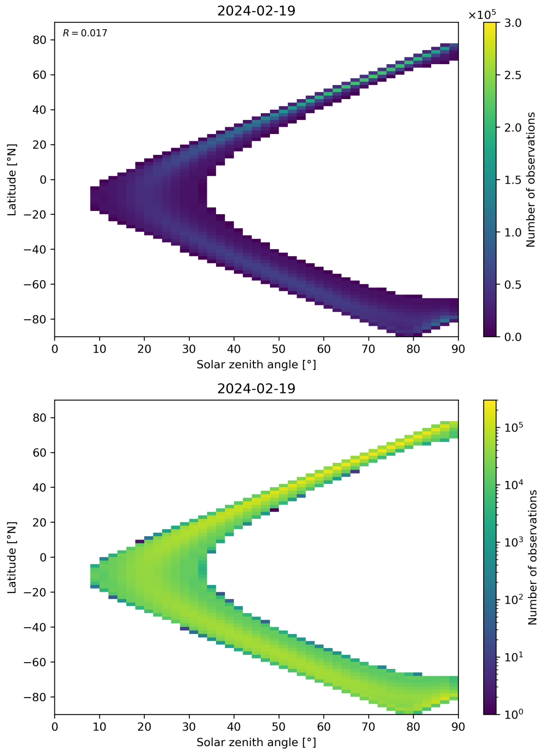
Figure 44: Scatter density plot of “Solar zenith angle” against “Latitude” for 2024-02-18 to 2024-02-20.
