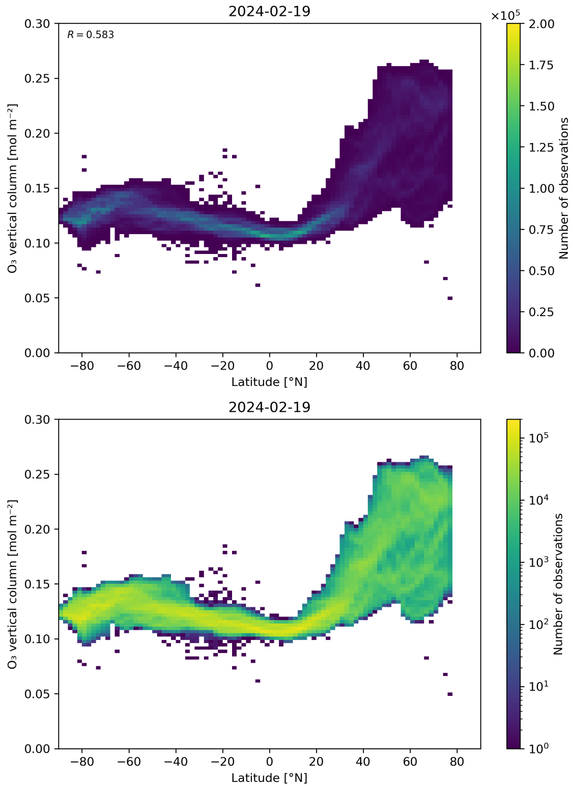
Figure 36: Scatter density plot of “Latitude” against “O 3 vertical column” for 2024-02-18 to 2024-02-20.
