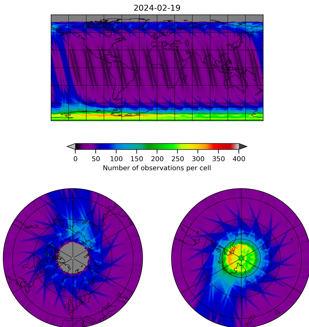
Figure 12: Map of the number of observations for 2024-02-18 to 2024-02-20
