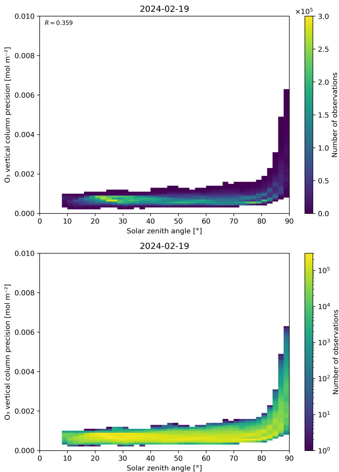
Figure 48: Scatter density plot of “Solar zenith angle” against “O 3 vertical column precision” for 2024-02-18 to 2024-02-20.
