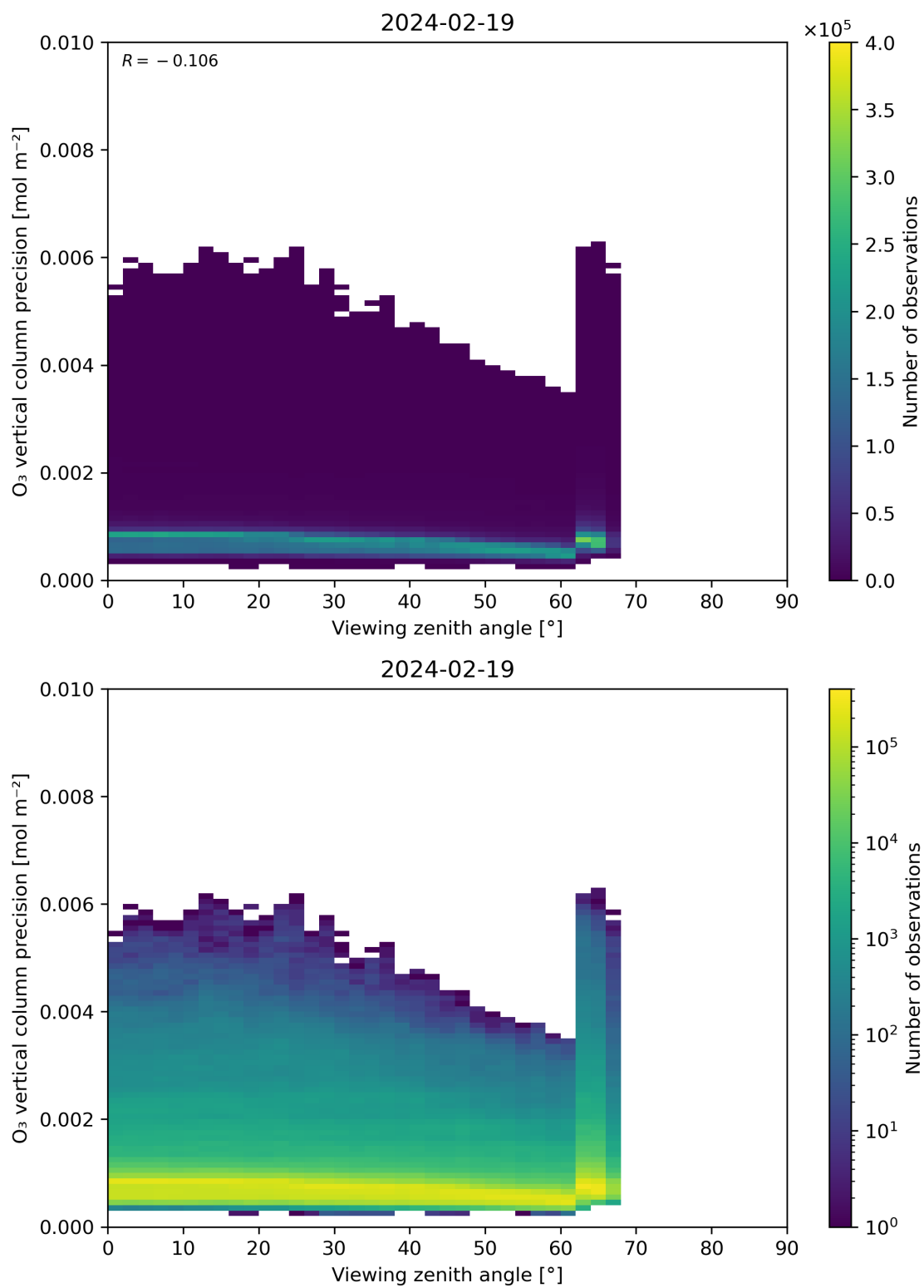
Figure 53: Scatter density plot of “Viewing zenith angle” against “O 3 vertical column precision” for 2024-02-18 to 2024-02-20.
