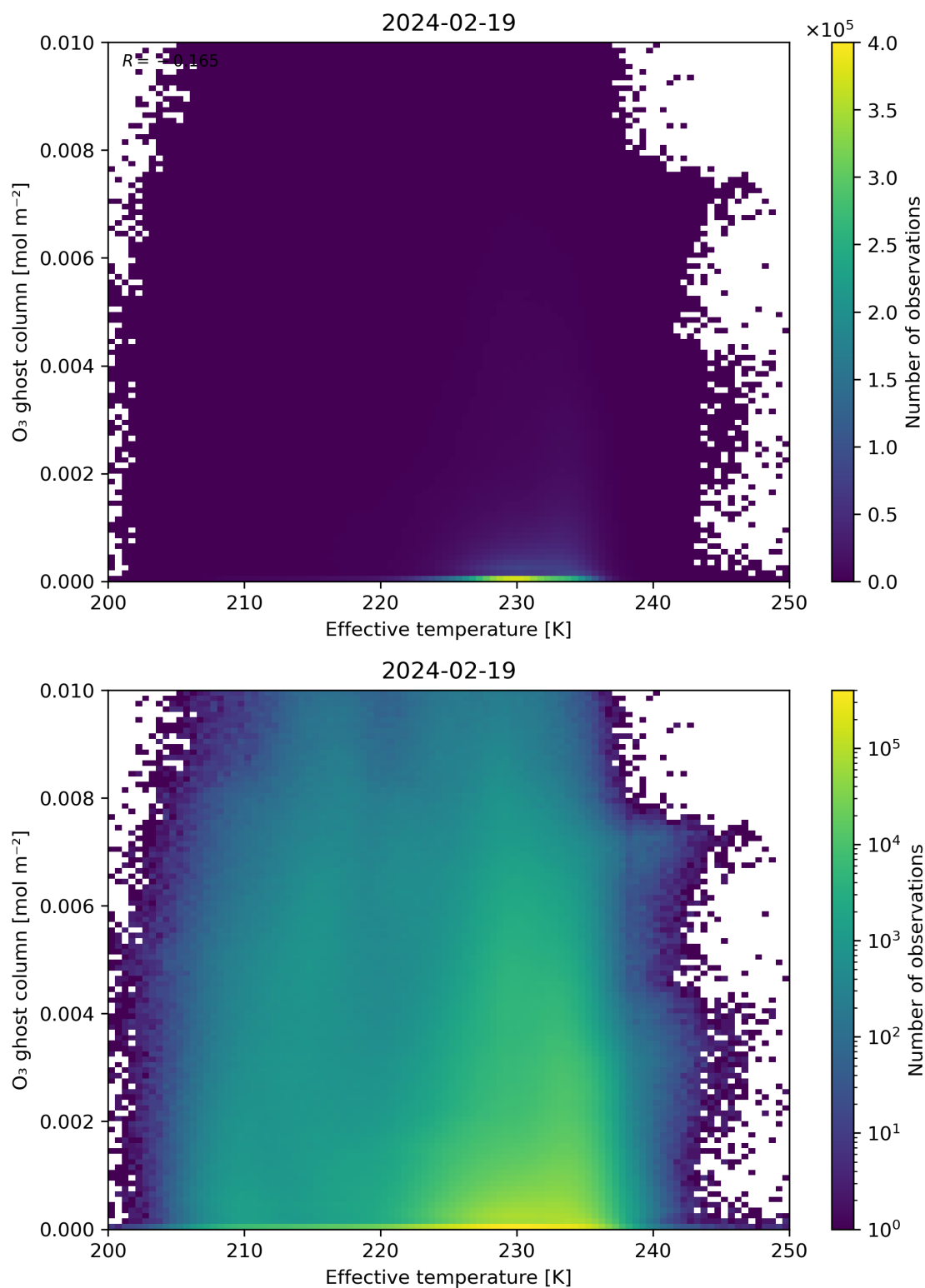
Figure 38: Scatter density plot of “Effective temperature” against “O 3 ghost column” for 2024-02-18 to 2024-02-20.
