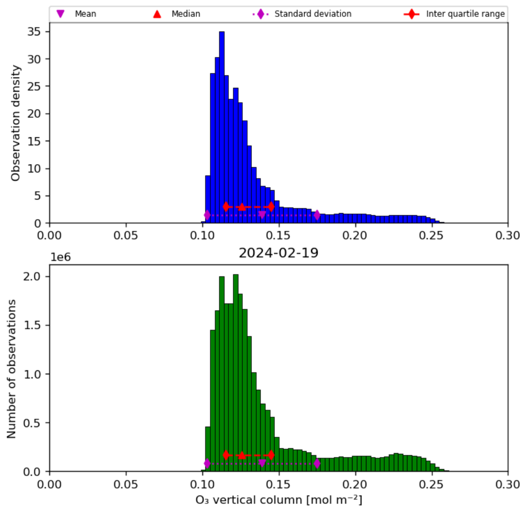
Figure 21: Histogram of “O 3 vertical column” for 2024-02-18 to 2024-02-20
