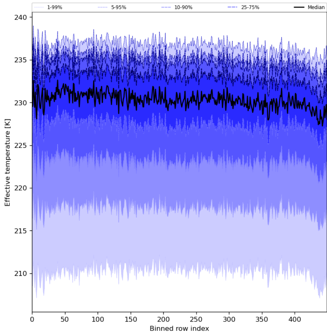
Figure 31: Along track statistics of “Effective temperature” for 2024-02-18 to 2024-02-20
