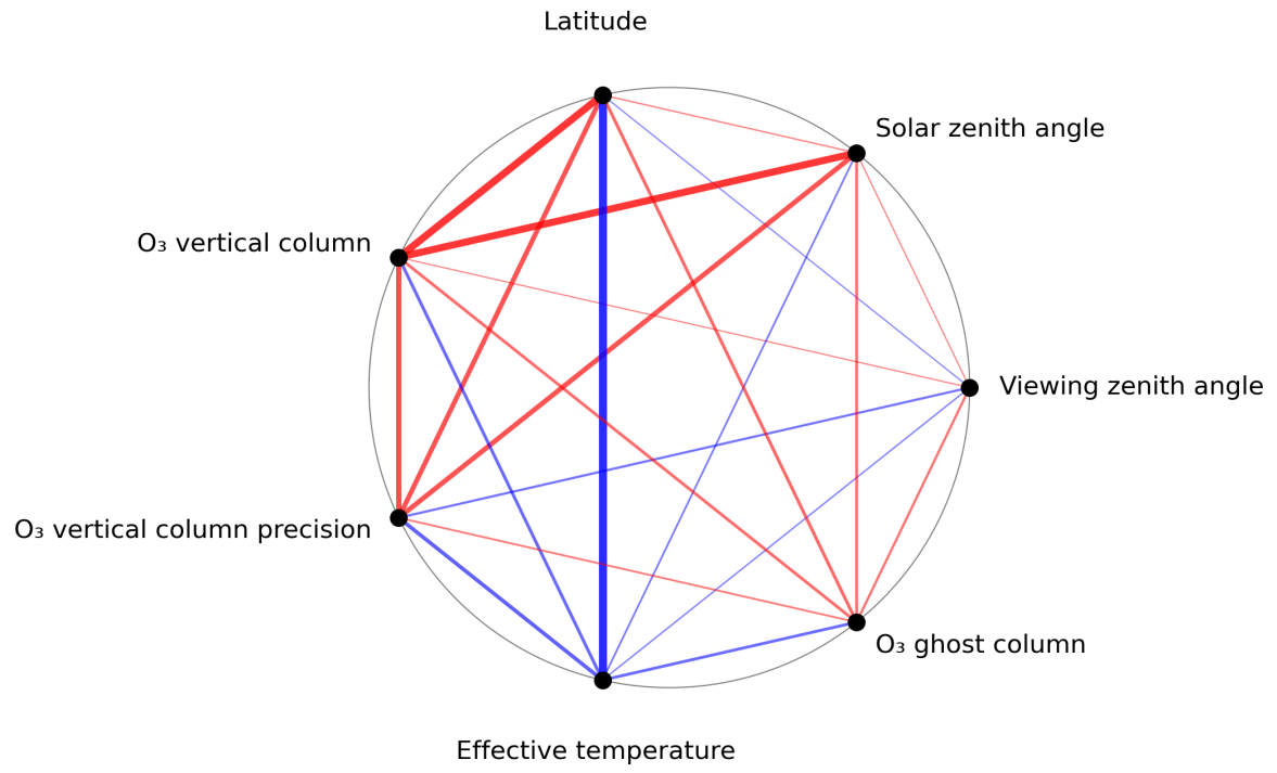
Figure 1: Map of correlation graph for 2024-02-18 to 2024-02-20.
