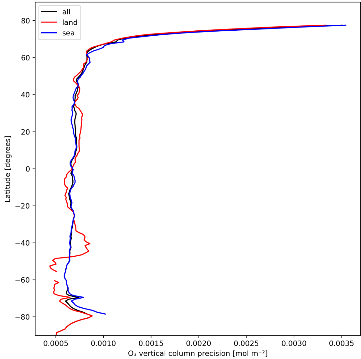
Figure 15: Zonal average of “O 3 vertical column precision” for 2024-02-18 to 2024-02-20.
