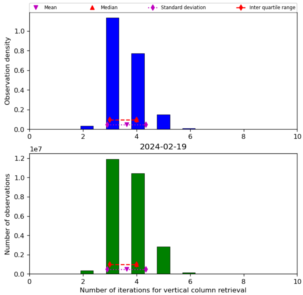
Figure 26: Histogram of “Number of iterations for vertical column retrieval” for 2024-02-18 to 2024-02-20
