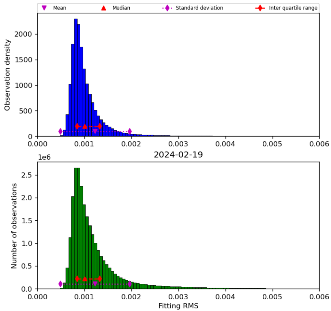
Figure 23: Histogram of “Fitting RMS” for 2024-02-18 to 2024-02-20
