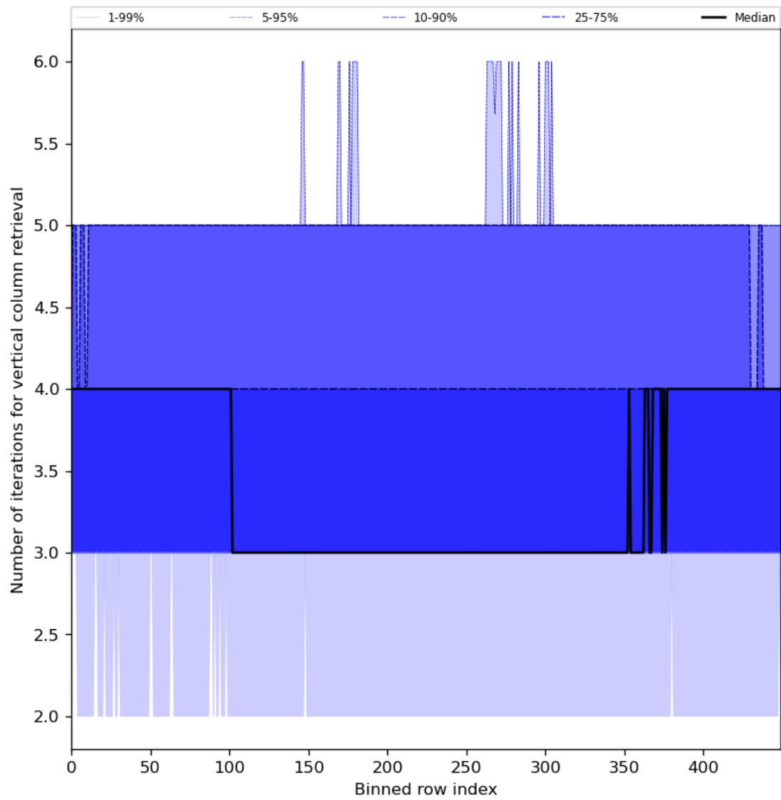
Figure 33: Along track statistics of “Number of iterations for vertical column retrieval” for 2024-02-18 to 2024-02-20
