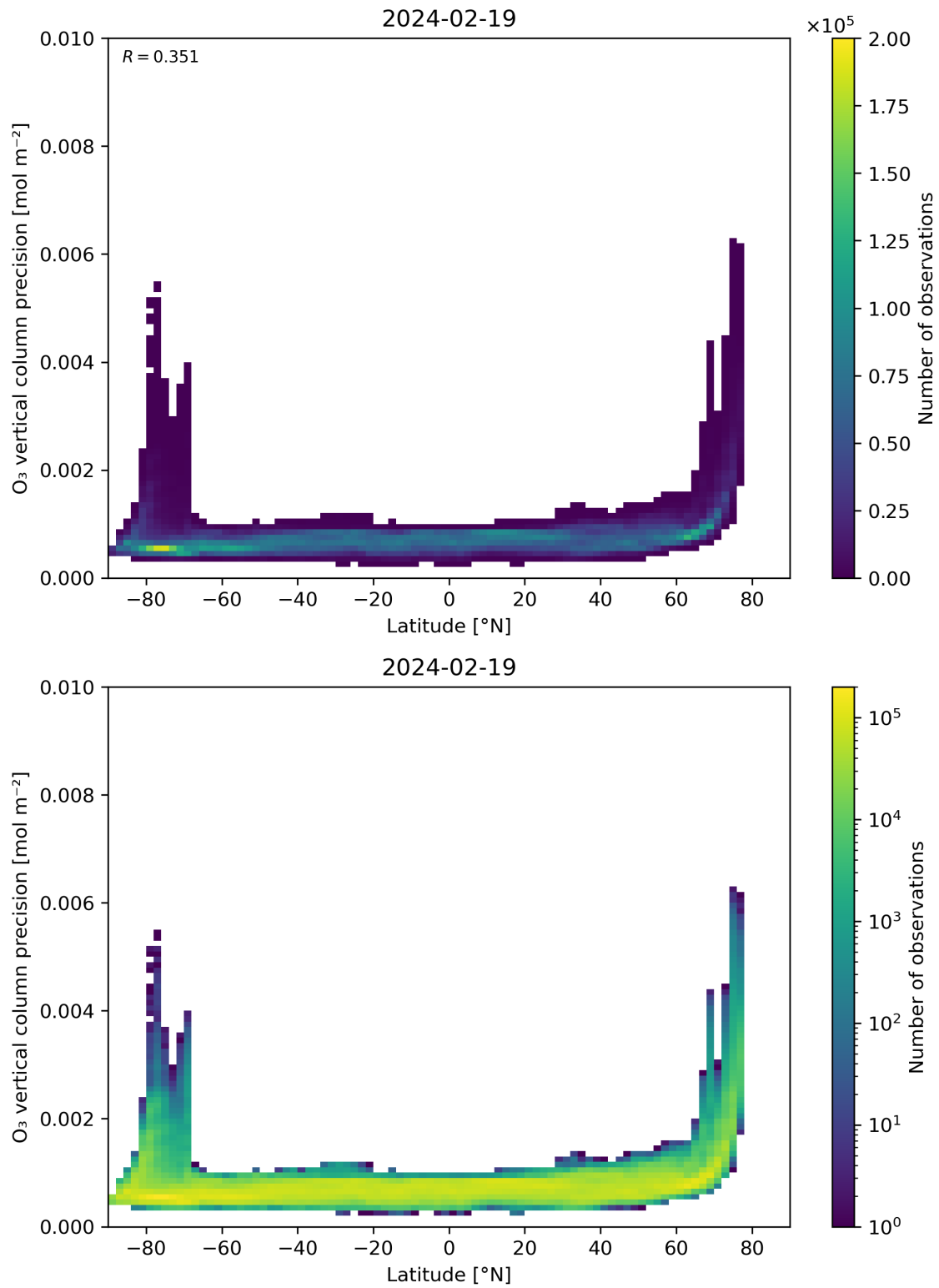
Figure 37: Scatter density plot of “Latitude” against “O 3 vertical column precision” for 2024-02-18 to 2024-02-20.
