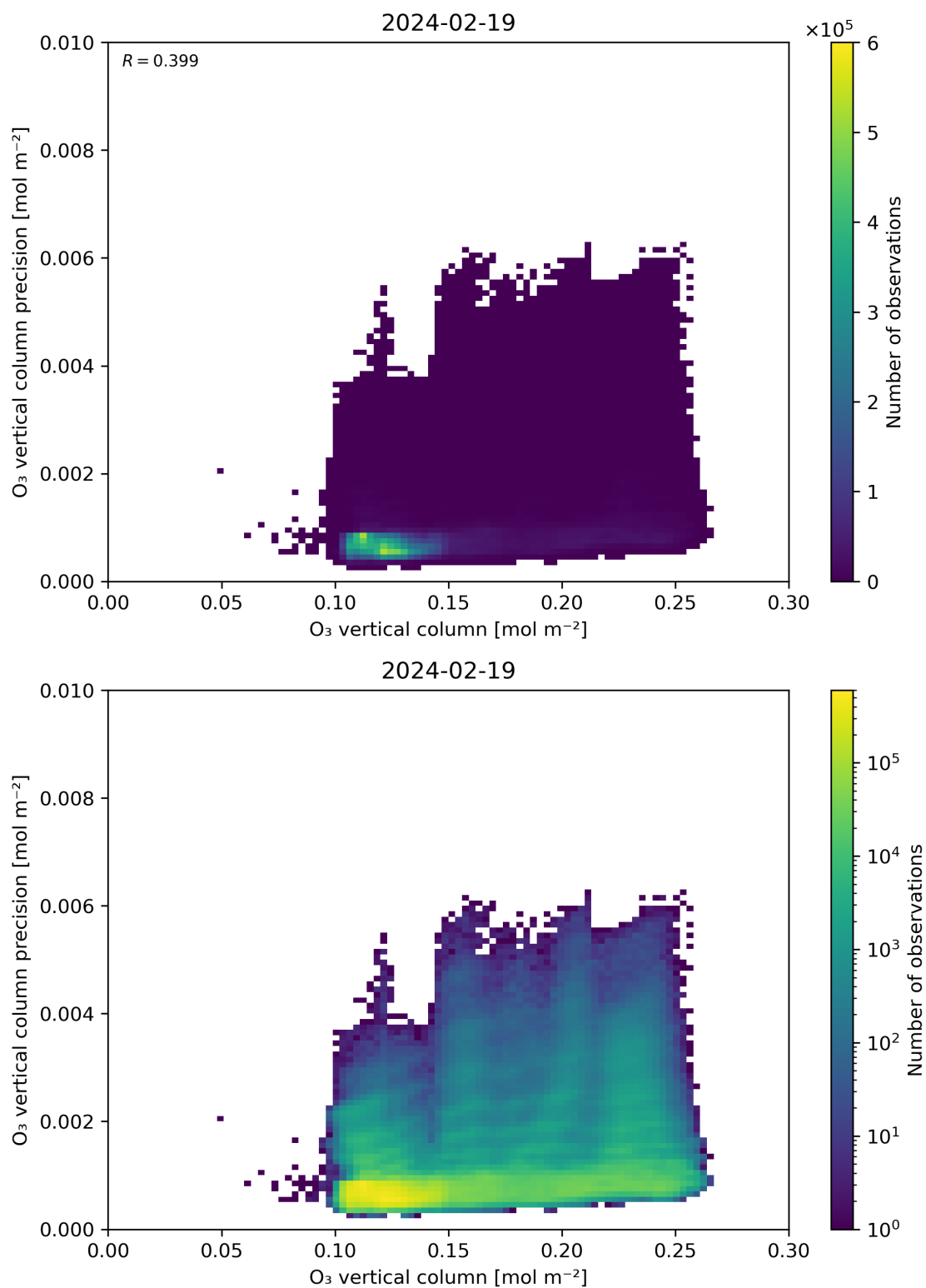
Figure 41: Scatter density plot of “O 3 vertical column” against “O 3 vertical column precision” for 2024-02-18 to 2024-02-20.
