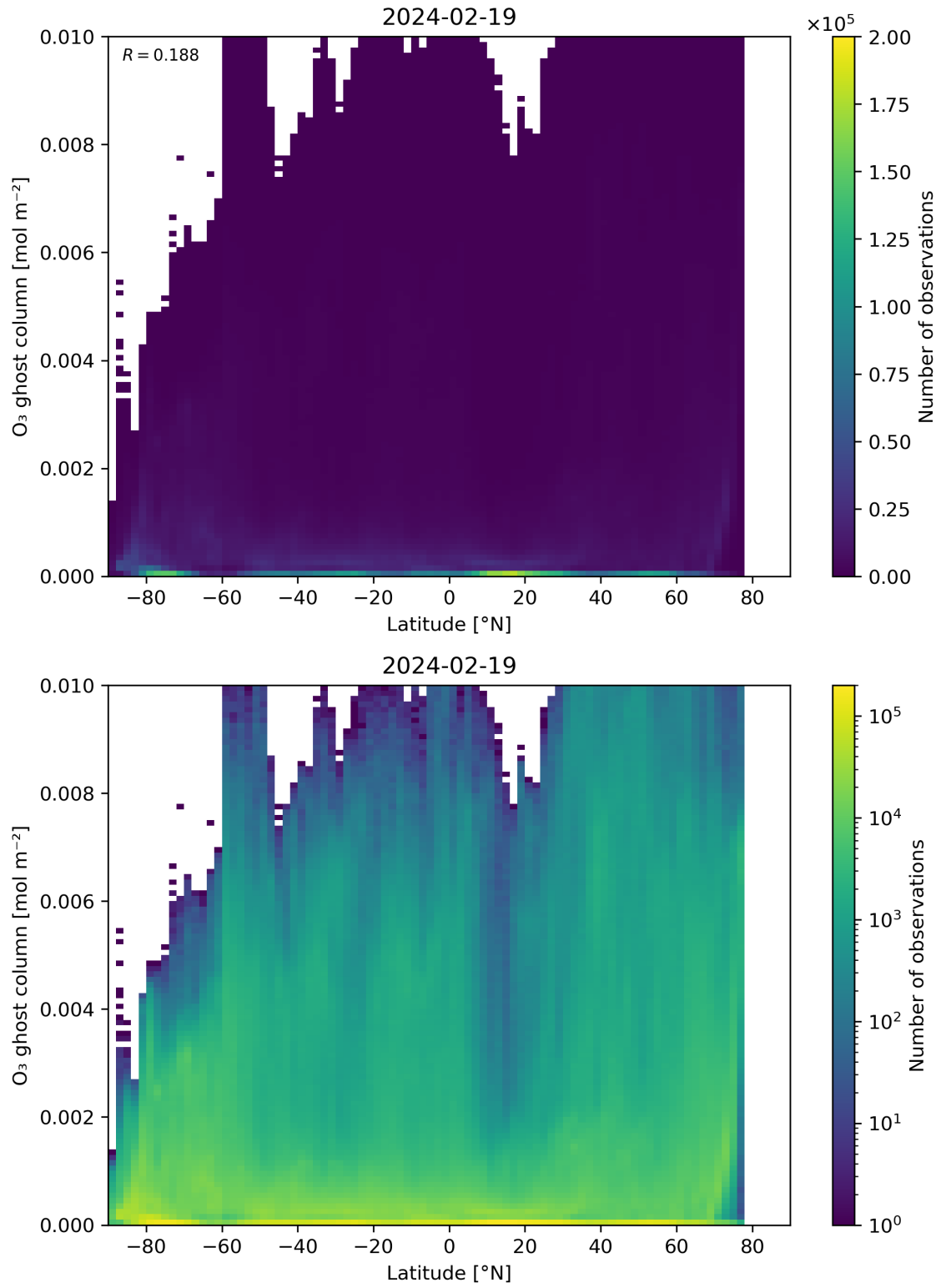
Figure 35: Scatter density plot of “Latitude” against “O 3 ghost column” for 2024-02-18 to 2024-02-20.
