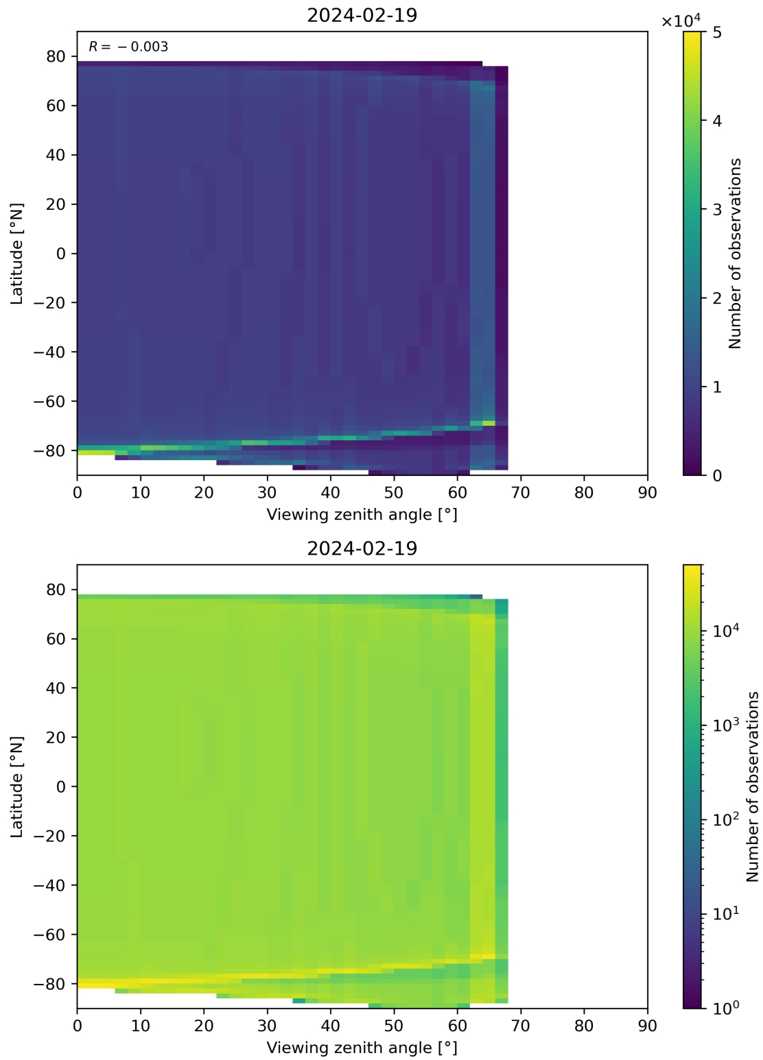
Figure 49: Scatter density plot of “Viewing zenith angle” against “Latitude” for 2024-02-18 to 2024-02-20.
