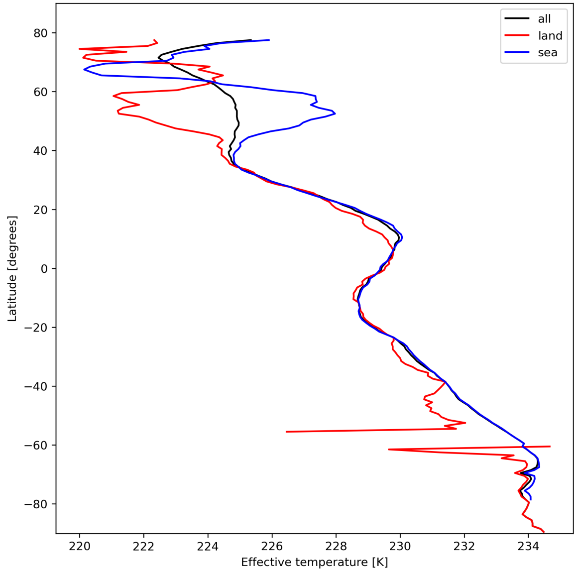
Figure 17: Zonal average of “Effective temperature” for 2024-02-18 to 2024-02-20.
