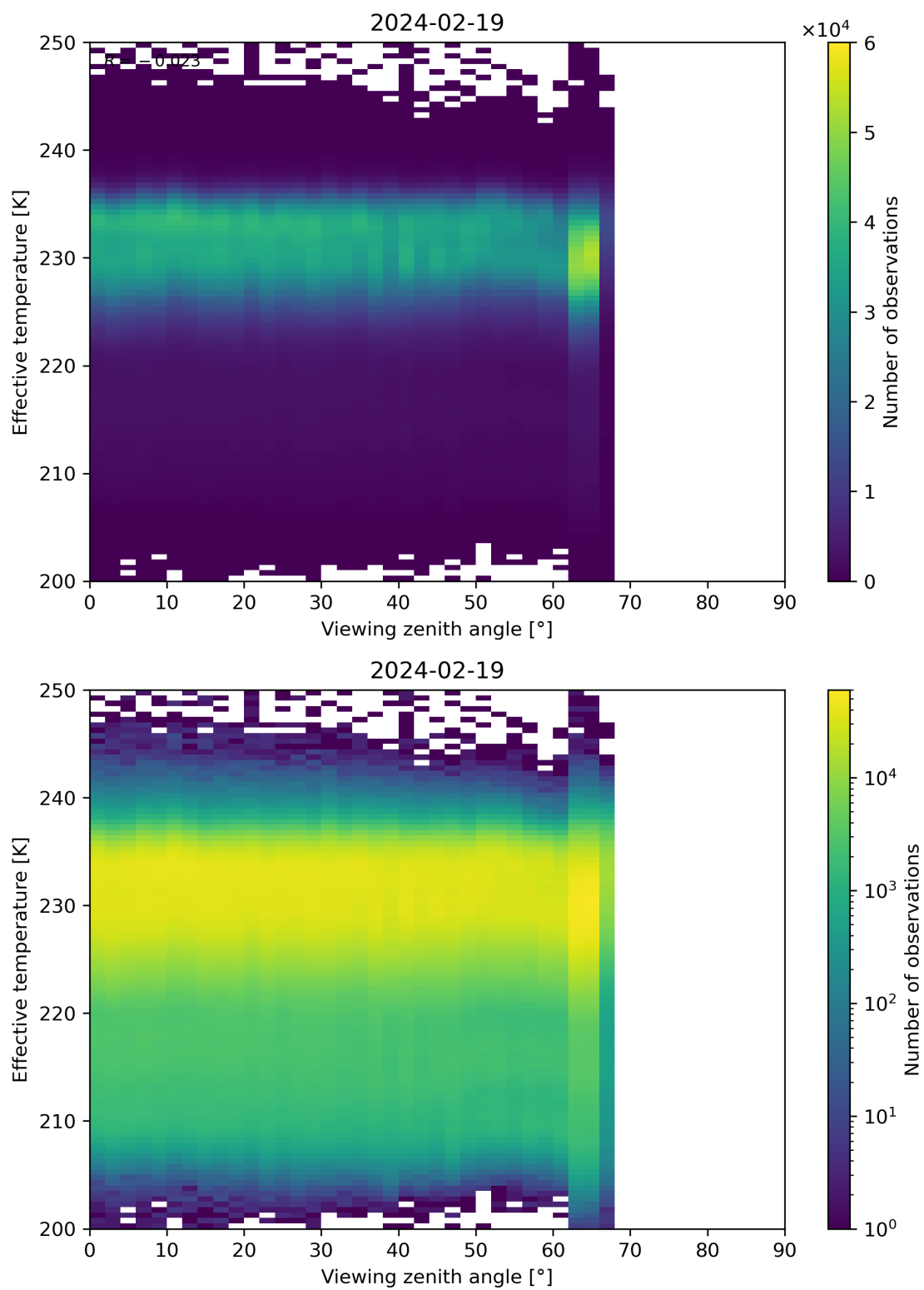
Figure 50: Scatter density plot of “Viewing zenith angle” against “Effective temperature” for 2024-02-18 to 2024-02-20.
