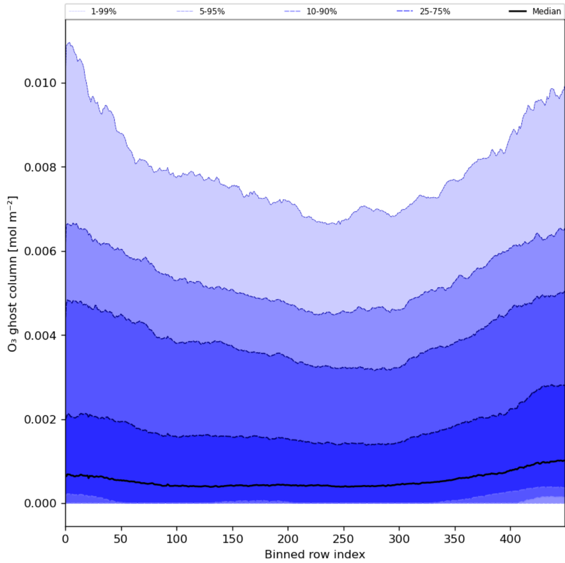
Figure 32: Along track statistics of “O 3 ghost column” for 2024-02-18 to 2024-02-20
