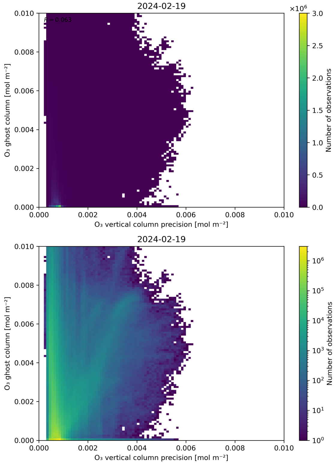
Figure 43: Scatter density plot of “O 3 vertical column precision” against “O 3 ghost column” for 2024-02-18 to 2024-02-20.
