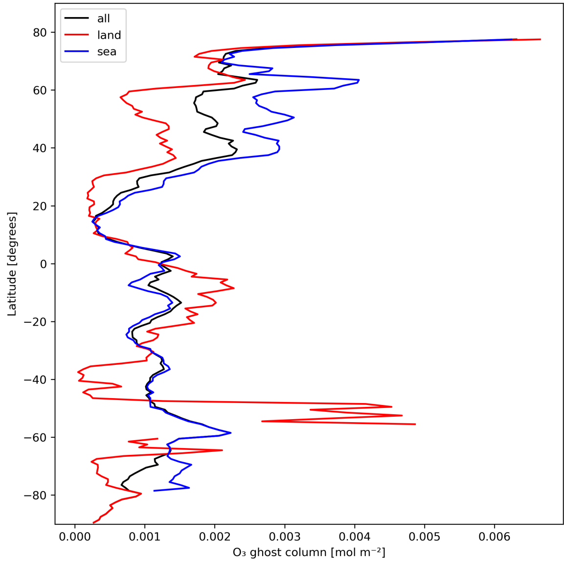
Figure 18: Zonal average of "O 3 ghost column" for 2024-02-18 to 2024-02-20.
