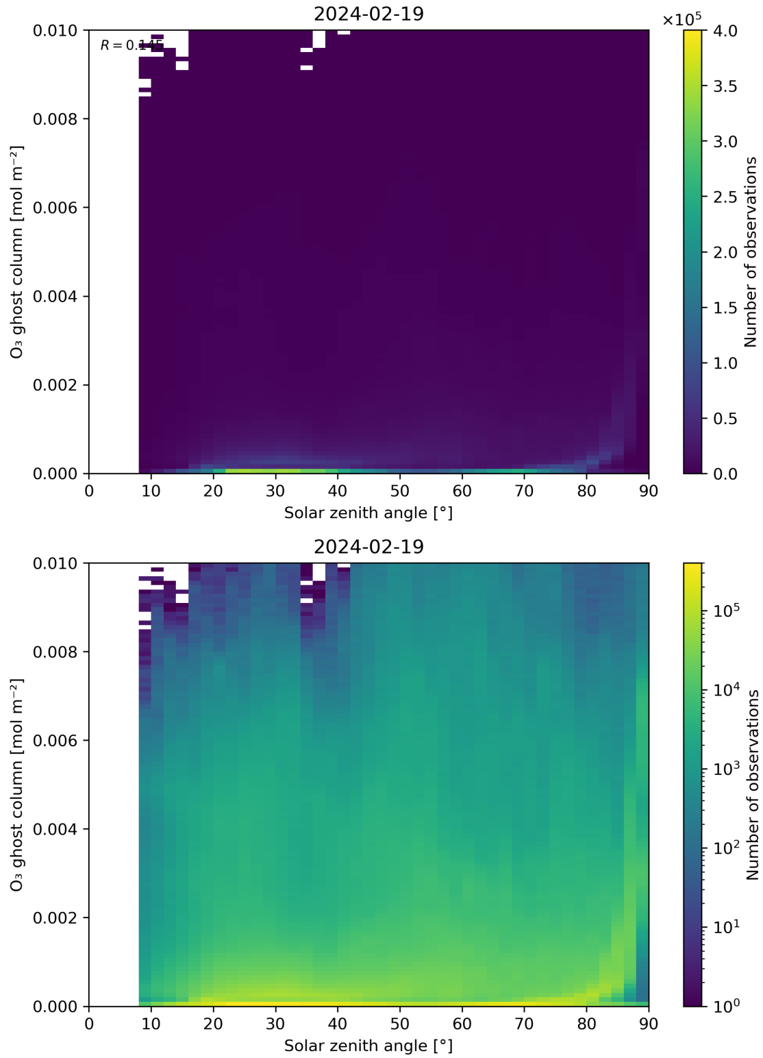
Figure 46: Scatter density plot of “Solar zenith angle” against “O 3 ghost column” for 2024-02-18 to 2024-02-20.
