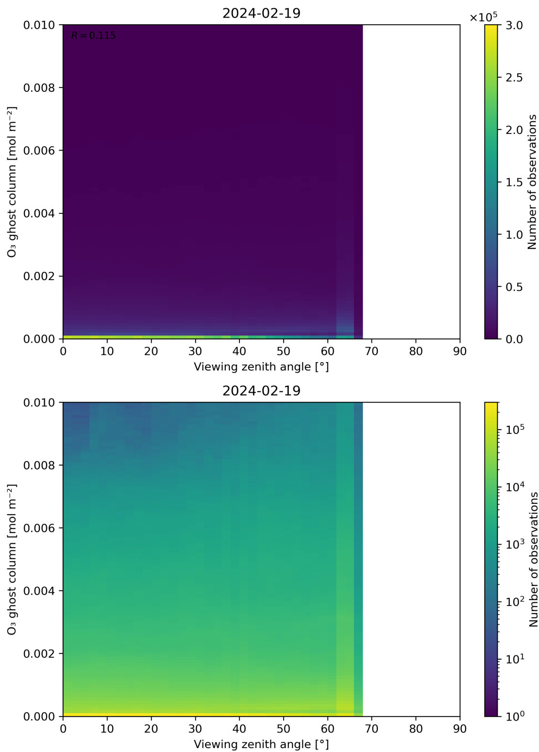
Figure 51: Scatter density plot of “Viewing zenith angle” against “O 3 ghost column” for 2024-02-18 to 2024-02-20.
