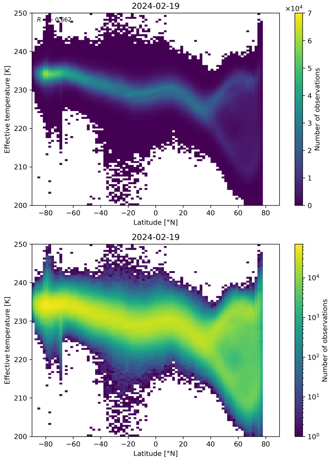
Figure 34: Scatter density plot of “Latitude” against “Effective temperature” for 2024-02-18 to 2024-02-20.
