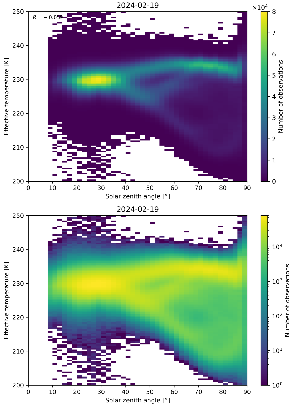
Figure 45: Scatter density plot of “Solar zenith angle” against “Effective temperature” for 2024-02-18 to 2024-02-20.
