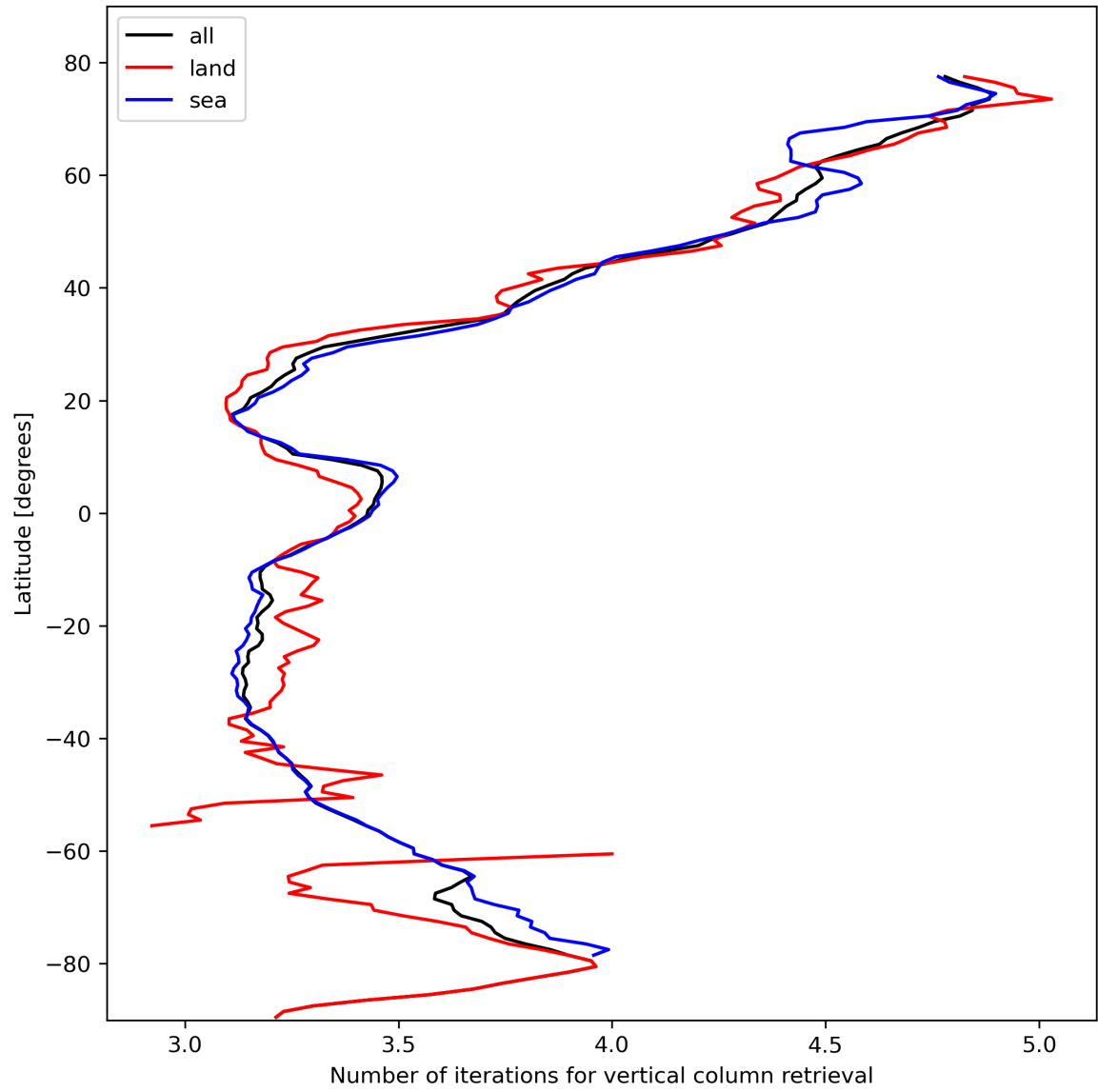
Figure 19: Zonal average of “Number of iterations for vertical column retrieval” for 2024-02-18 to 2024-02-20.
