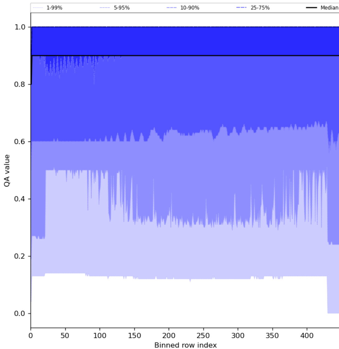
Figure 27: Along track statistics of “QA value” for 2024-02-18 to 2024-02-20
