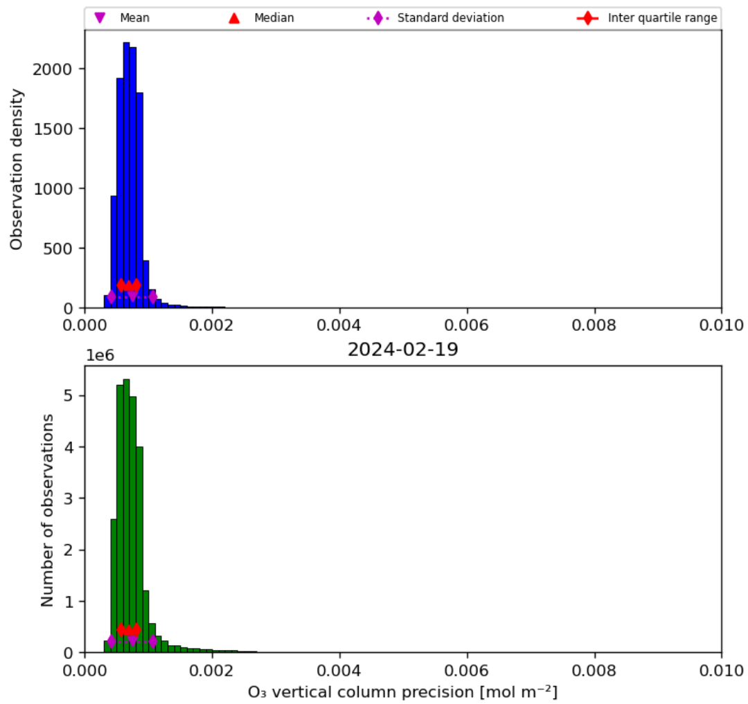
Figure 22: Histogram of “O 3 vertical column precision” for 2024-02-18 to 2024-02-20
