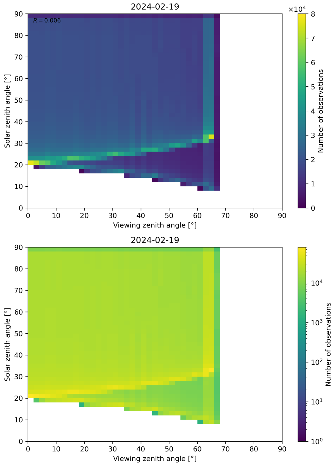
Figure 54: Scatter density plot of “Viewing zenith angle” against “Solar zenith angle” for 2024-02-18 to 2024-02-20.
