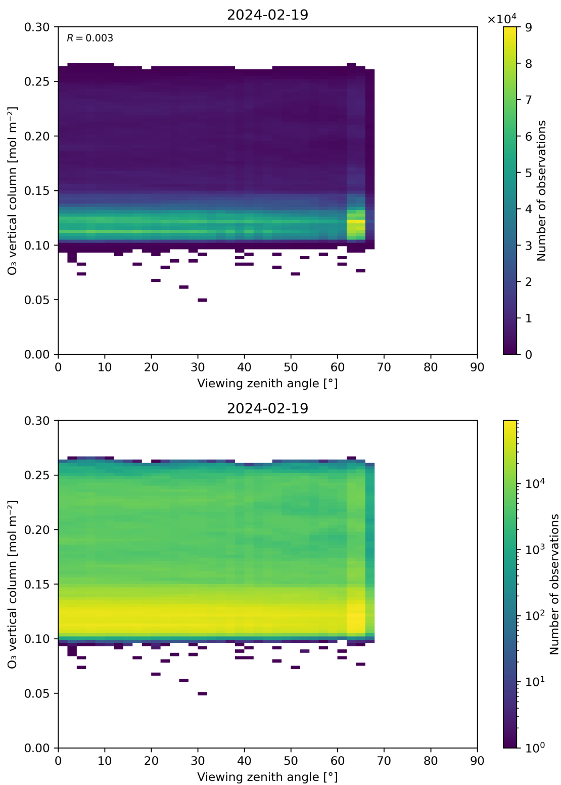
Figure 52: Scatter density plot of “Viewing zenith angle” against “O 3 vertical column” for 2024-02-18 to 2024-02-20.
