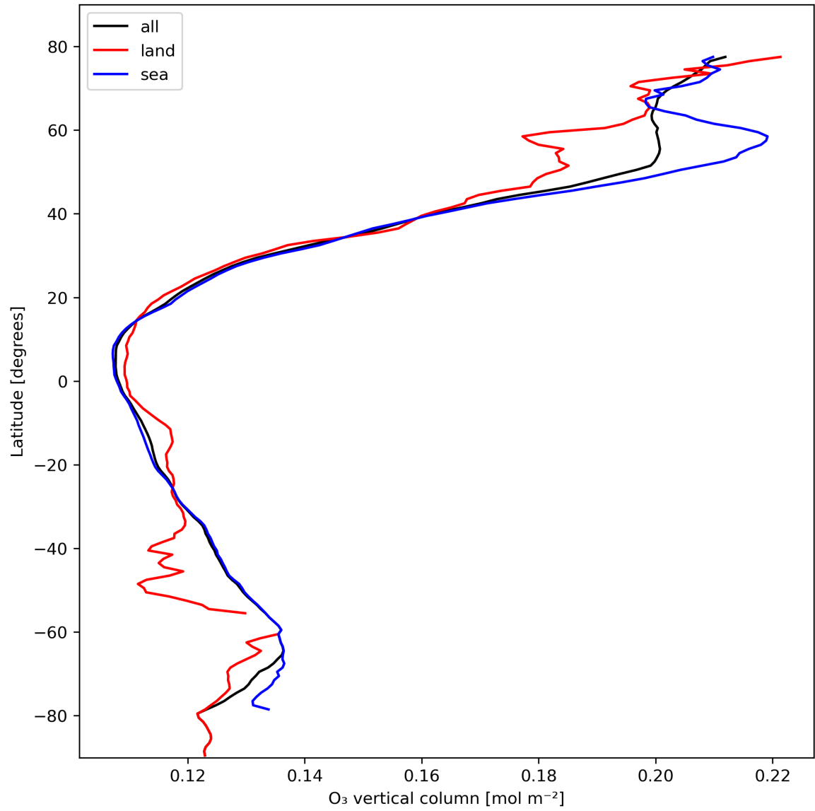
Figure 14: Zonal average of “O 3 vertical column” for 2024-02-18 to 2024-02-20.
