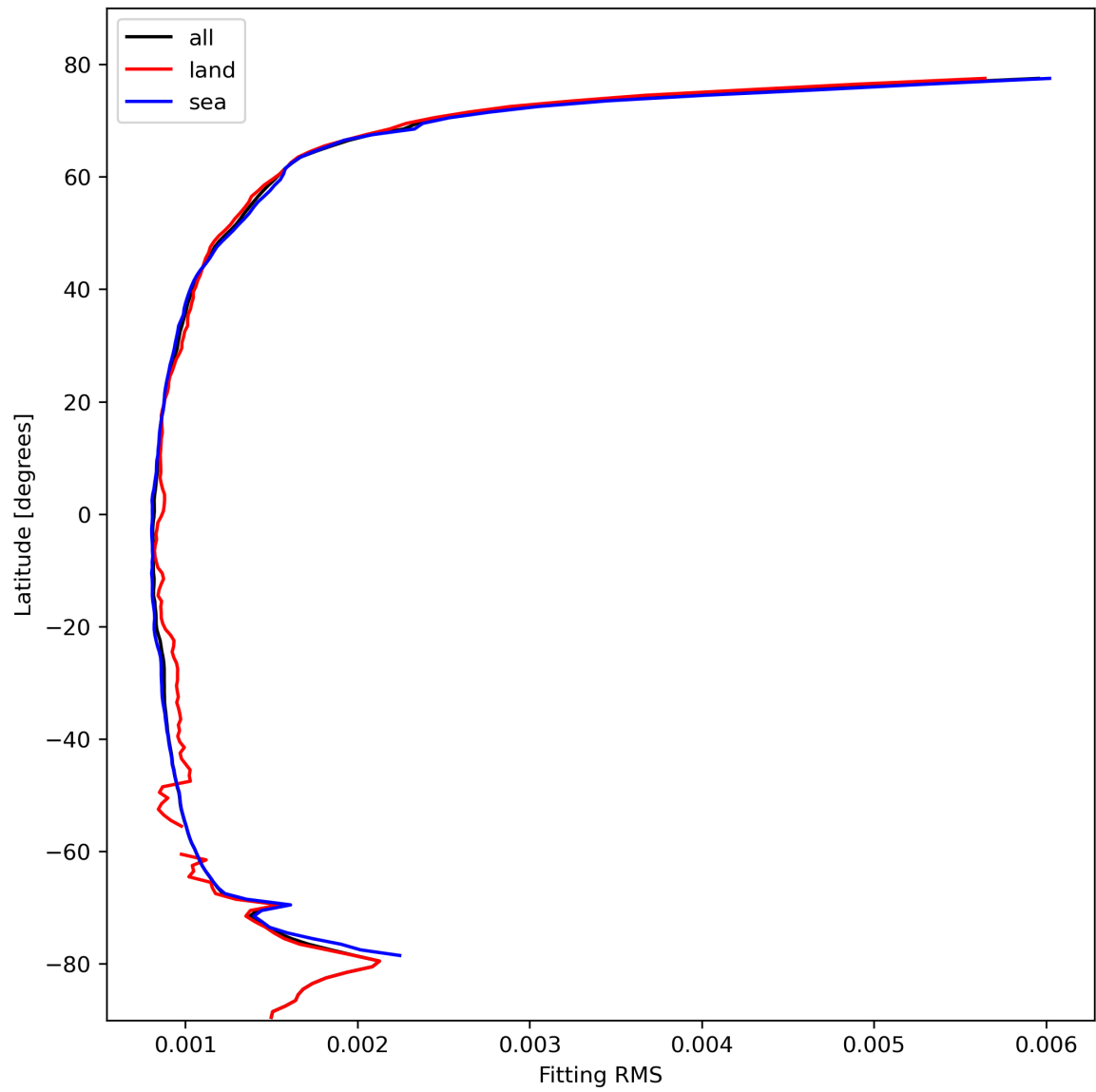
Figure 16: Zonal average of “Fitting RMS” for 2024-02-18 to 2024-02-20.
