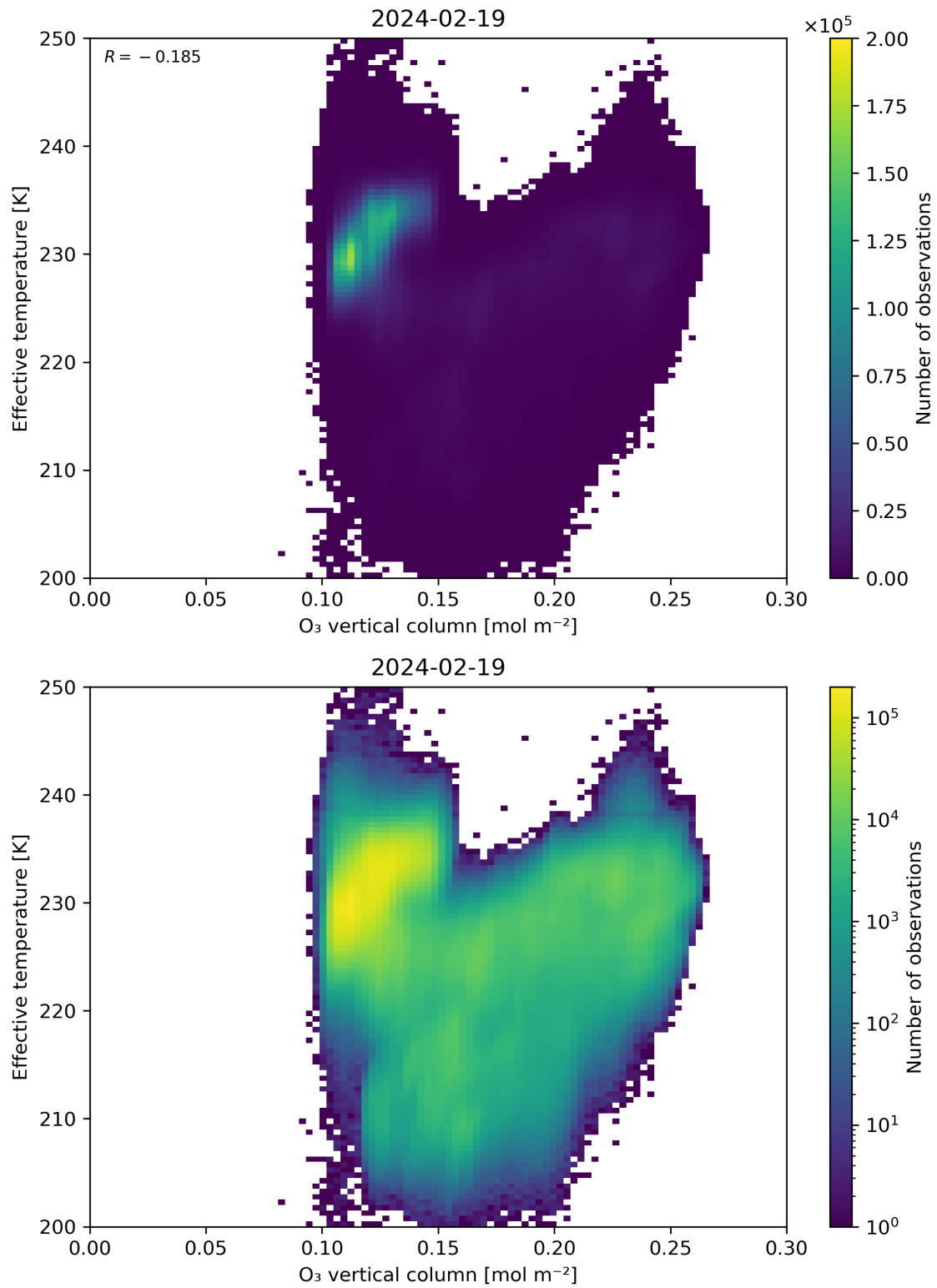
Figure 39: Scatter density plot of “O 3 vertical column” against “Effective temperature” for 2024-02-18 to 2024-02-20.
