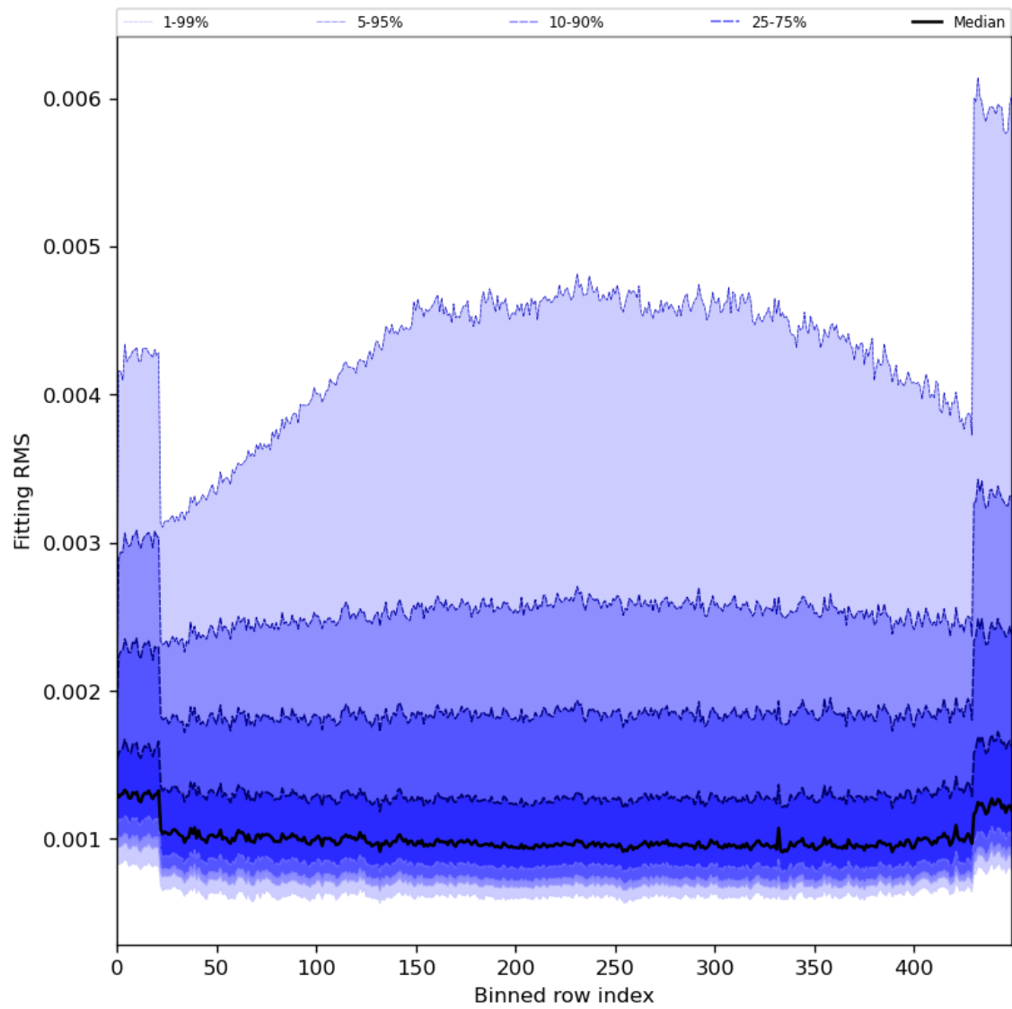
Figure 30: Along track statistics of “Fitting RMS” for 2024-02-18 to 2024-02-20
