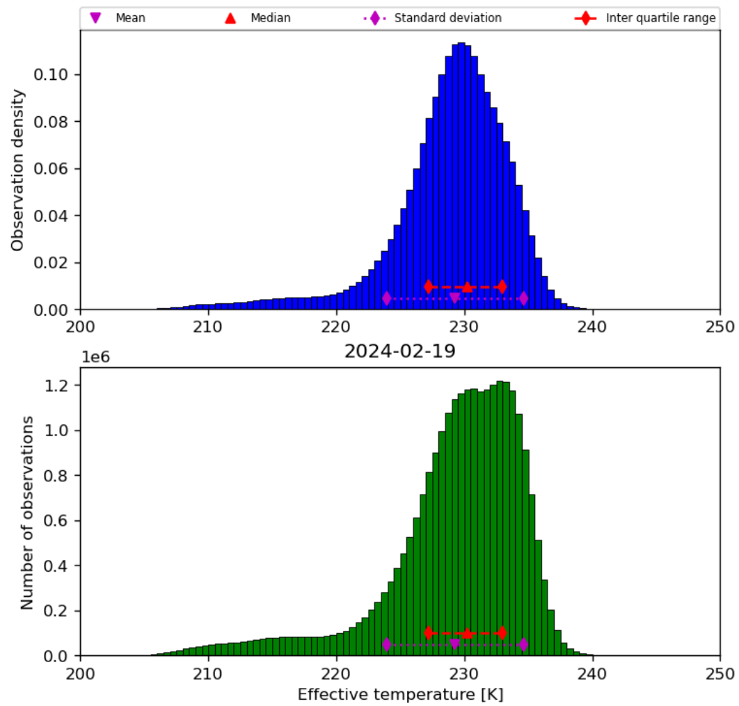
Figure 24: Histogram of “Effective temperature” for 2024-02-18 to 2024-02-20
