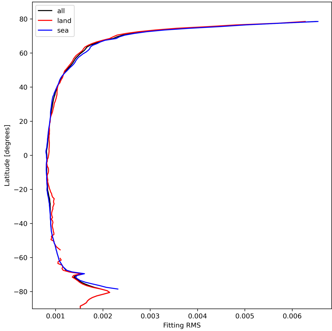
Figure 16: Zonal average of “Fitting RMS” for 2024-02-19 to 2024-02-21.
