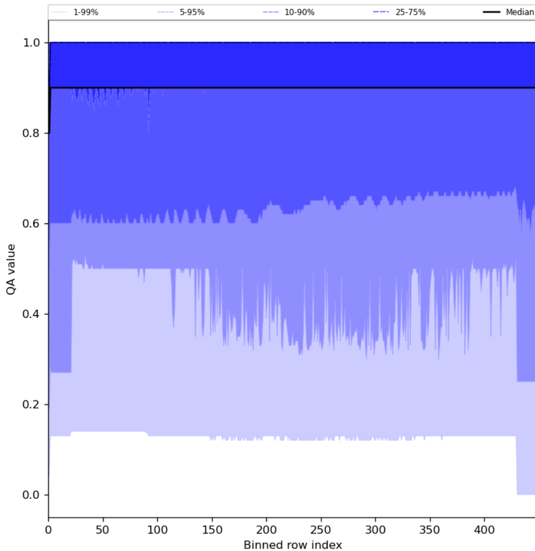
Figure 27: Along track statistics of “QA value” for 2024-02-19 to 2024-02-21
