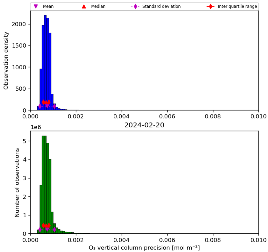
Figure 22: Histogram of “O 3 vertical column precision” for 2024-02-19 to 2024-02-21
