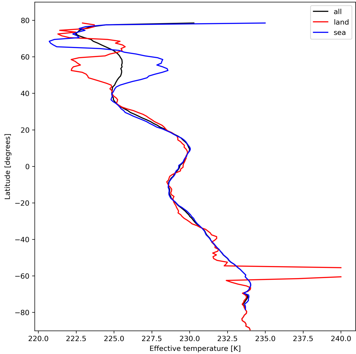
Figure 17: Zonal average of “Effective temperature” for 2024-02-19 to 2024-02-21.
