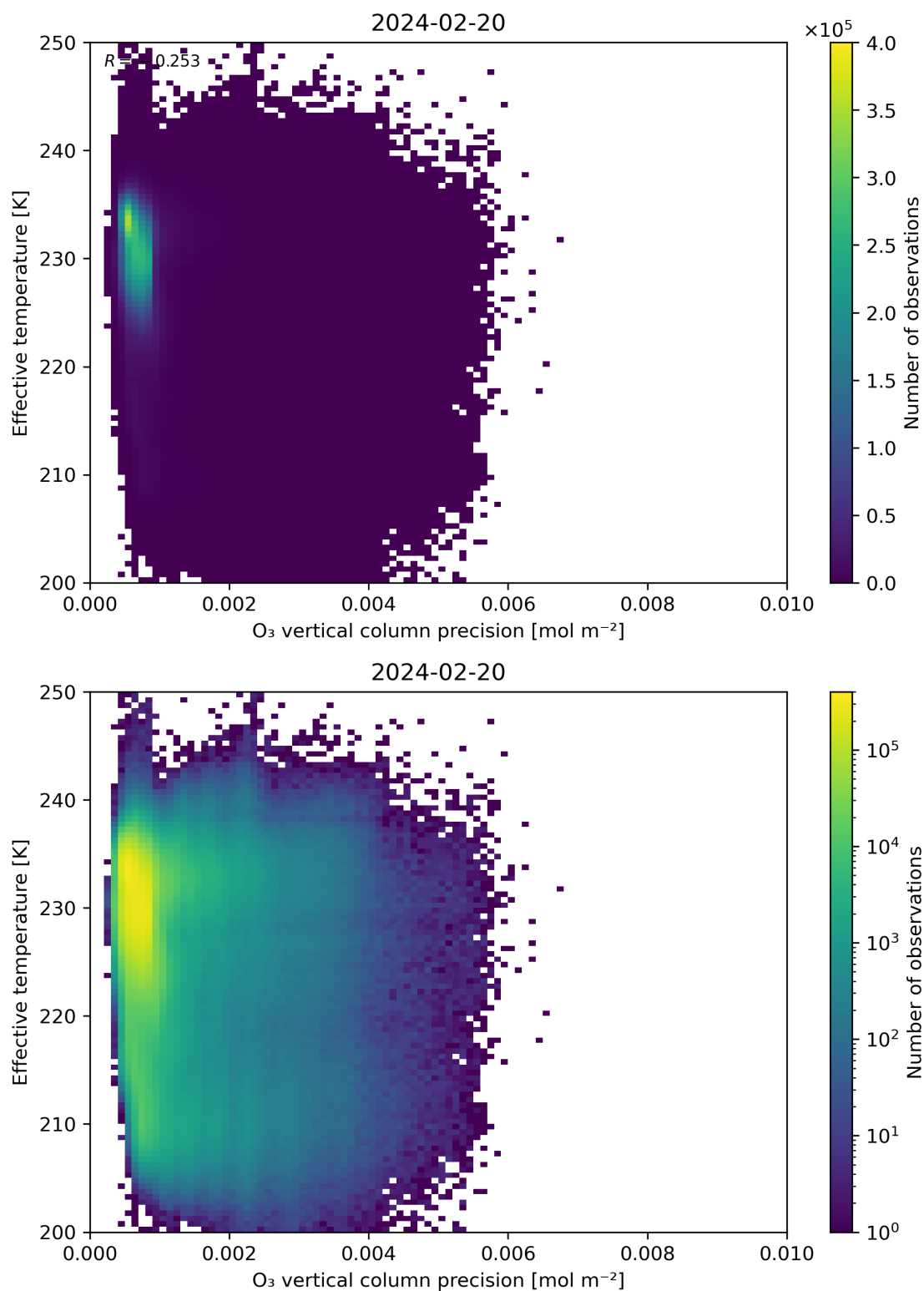
Figure 42: Scatter density plot of “O 3 vertical column precision” against “Effective temperature” for 2024-02-19 to 2024-02-21.
