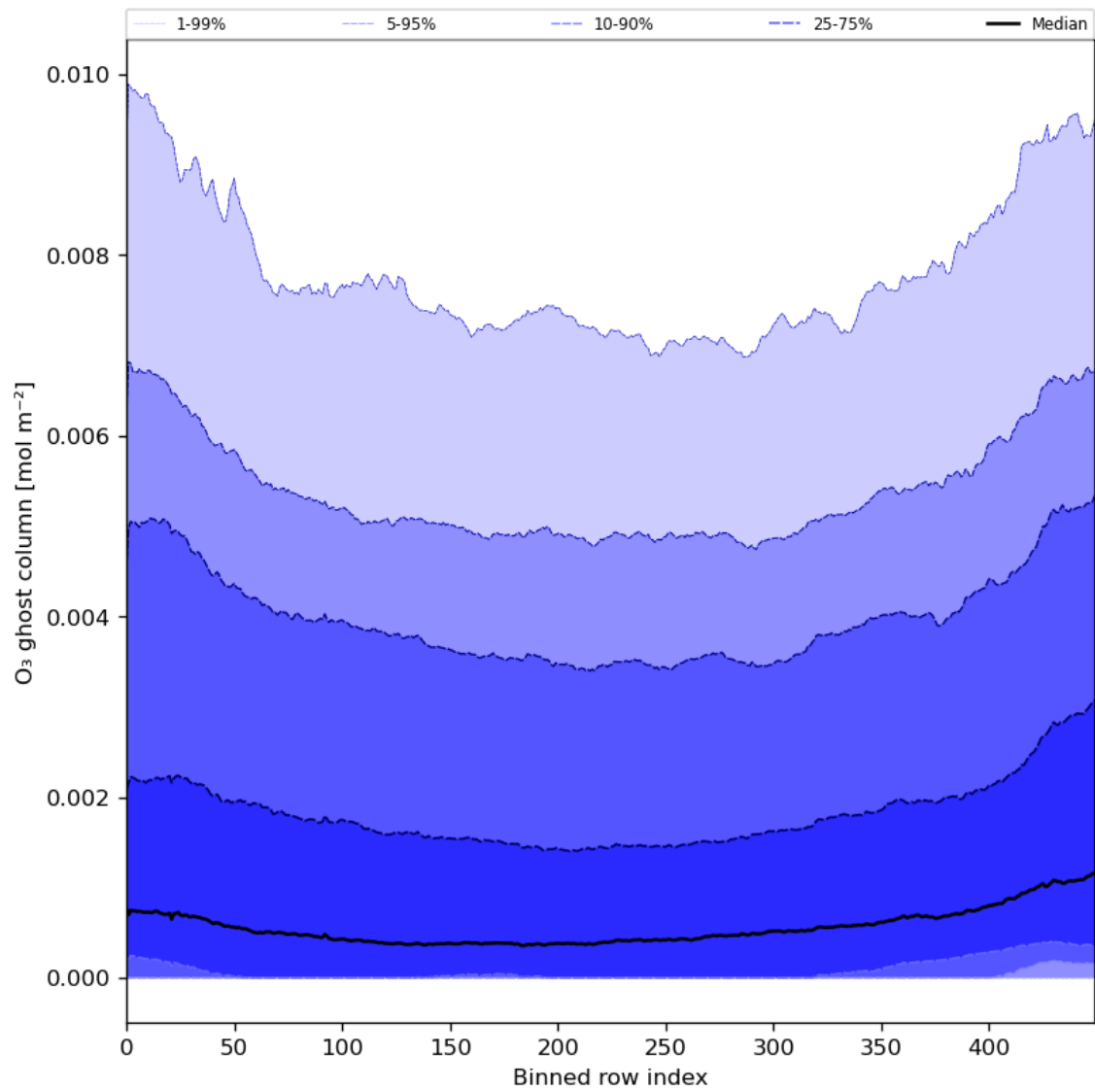
Figure 32: Along track statistics of "O 3 ghost column" for 2024-02-19 to 2024-02-21
