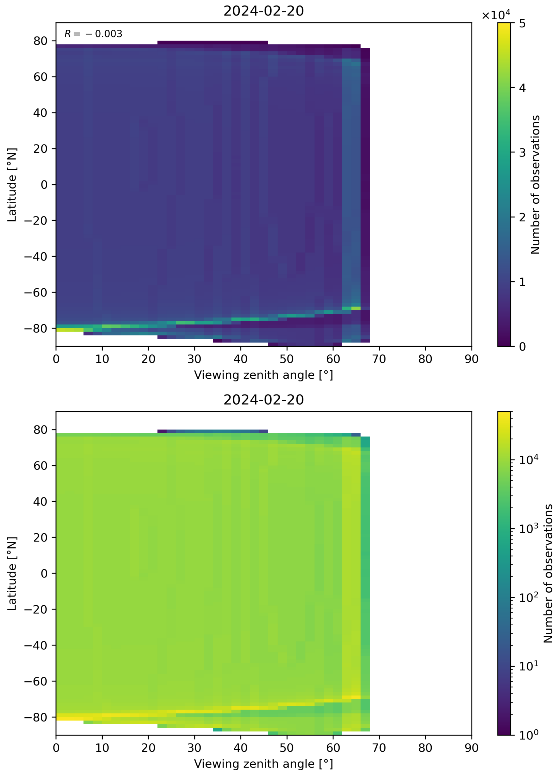
Figure 49: Scatter density plot of “Viewing zenith angle” against “Latitude” for 2024-02-19 to 2024-02-21.
