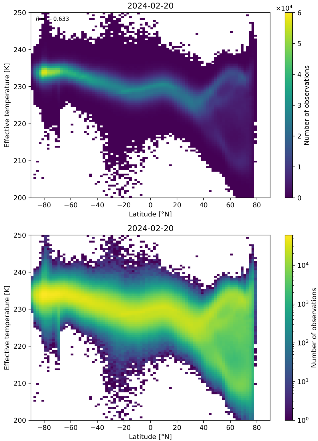
Figure 34: Scatter density plot of “Latitude” against “Effective temperature” for 2024-02-19 to 2024-02-21.
