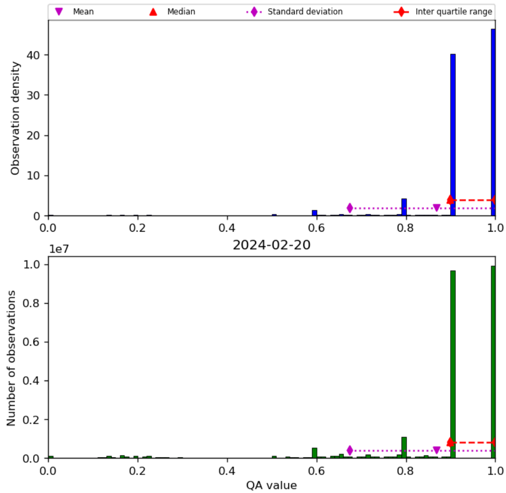
Figure 20: Histogram of “QA value” for 2024-02-19 to 2024-02-21
