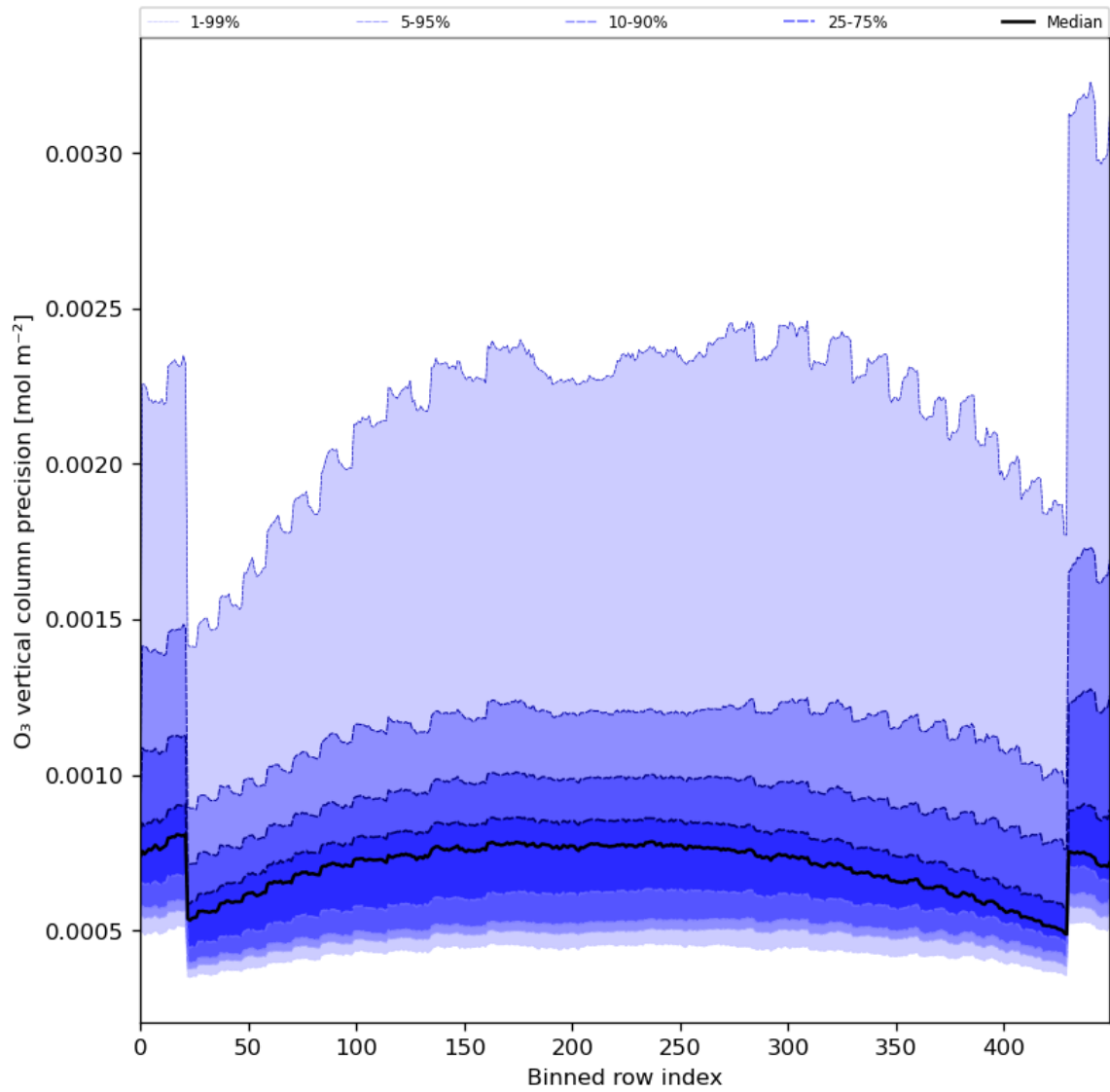
Figure 29: Along track statistics of “O 3 vertical column precision” for 2024-02-19 to 2024-02-21
