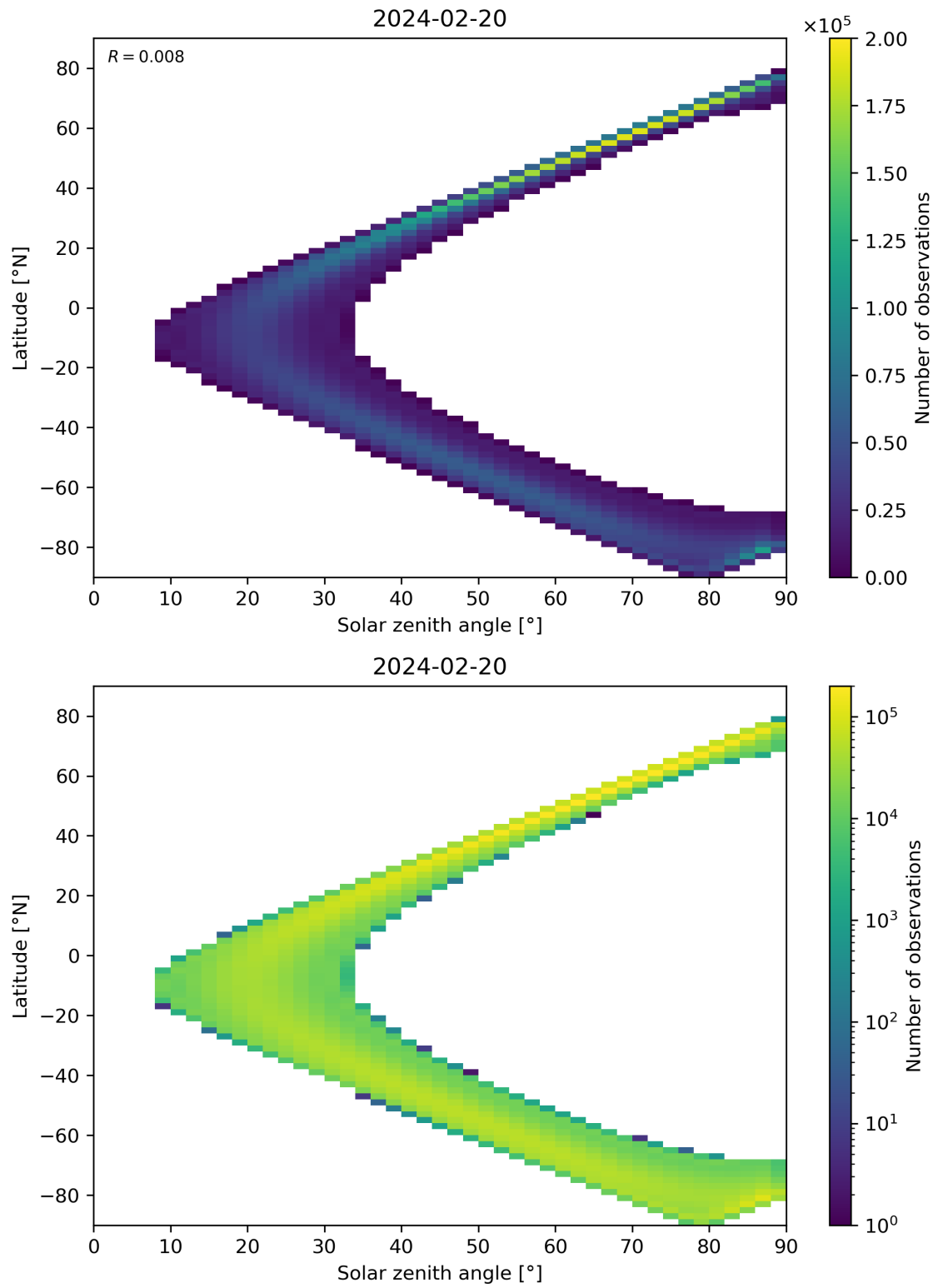
Figure 44: Scatter density plot of “Solar zenith angle” against “Latitude” for 2024-02-19 to 2024-02-21.
