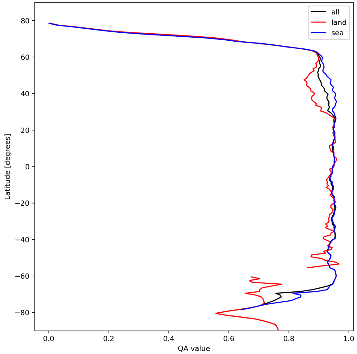
Figure 13: Zonal average of “QA value” for 2024-02-19 to 2024-02-21.
