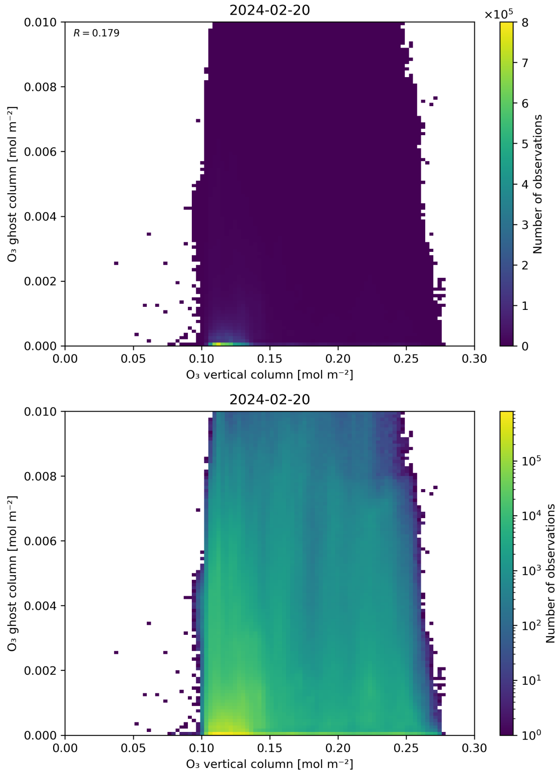
Figure 40: Scatter density plot of “O 3 vertical column” against “O 3 ghost column” for 2024-02-19 to 2024-02-21.
