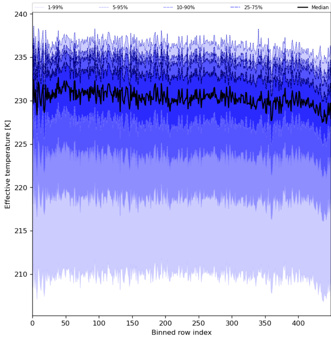
Figure 31: Along track statistics of “Effective temperature” for 2024-02-19 to 2024-02-21
