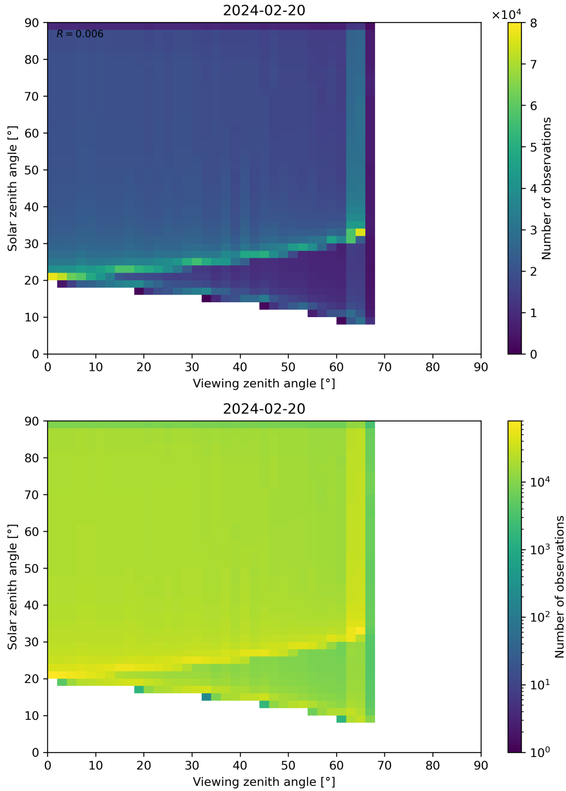
Figure 54: Scatter density plot of “Viewing zenith angle” against “Solar zenith angle” for 2024-02-19 to 2024-02-21.
