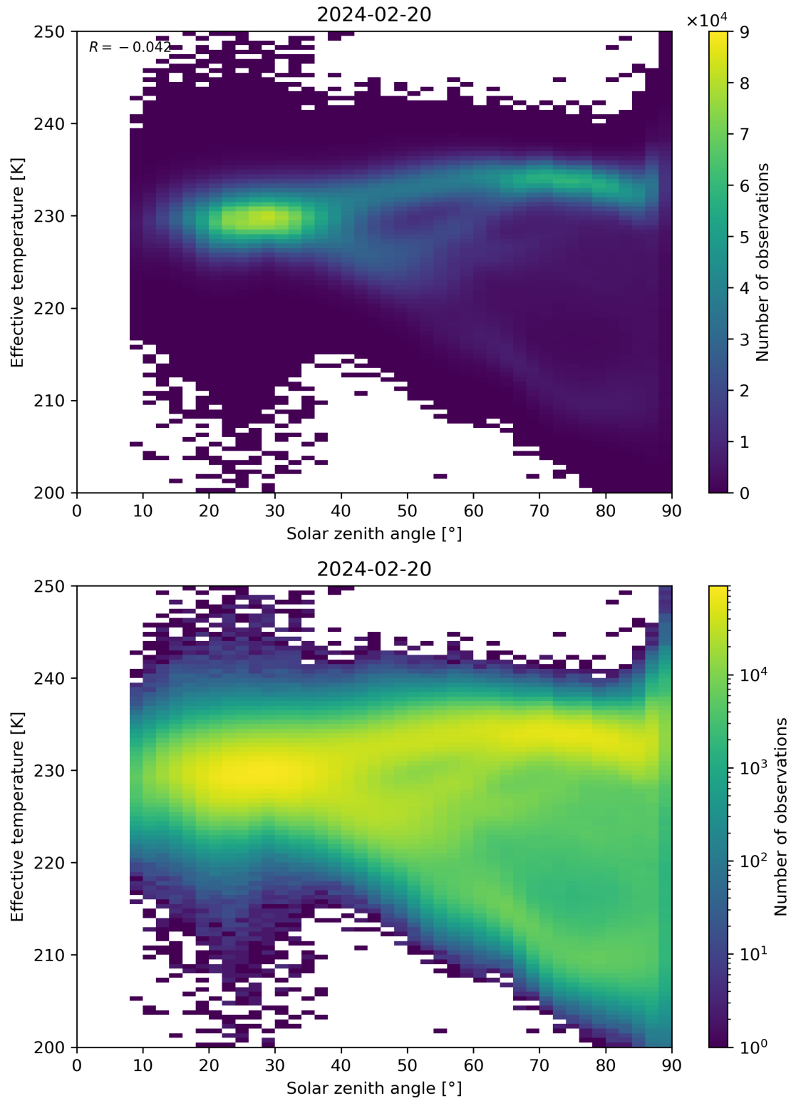
Figure 45: Scatter density plot of “Solar zenith angle” against “Effective temperature” for 2024-02-19 to 2024-02-21.
