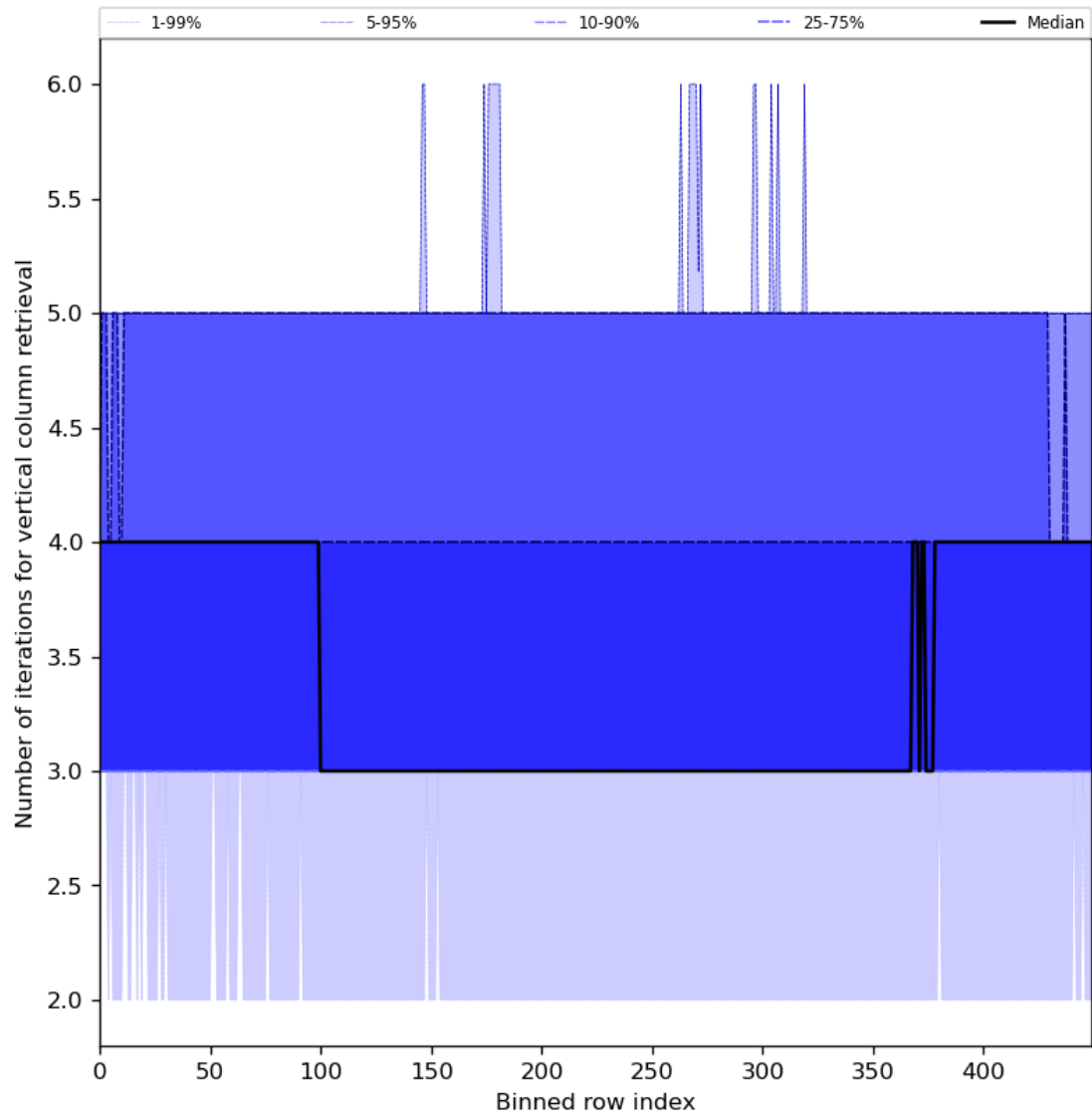
Figure 33: Along track statistics of “Number of iterations for vertical column retrieval” for 2024-02-19 to 2024-02-21
