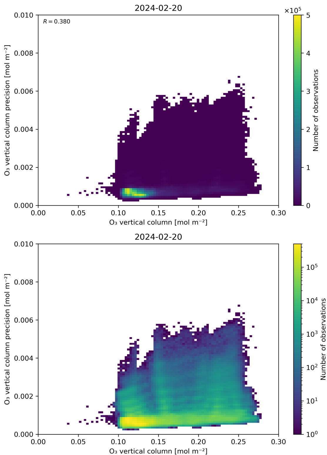
Figure 41: Scatter density plot of “O 3 vertical column” against “O 3 vertical column precision” for 2024-02-19 to 2024-02-21.
