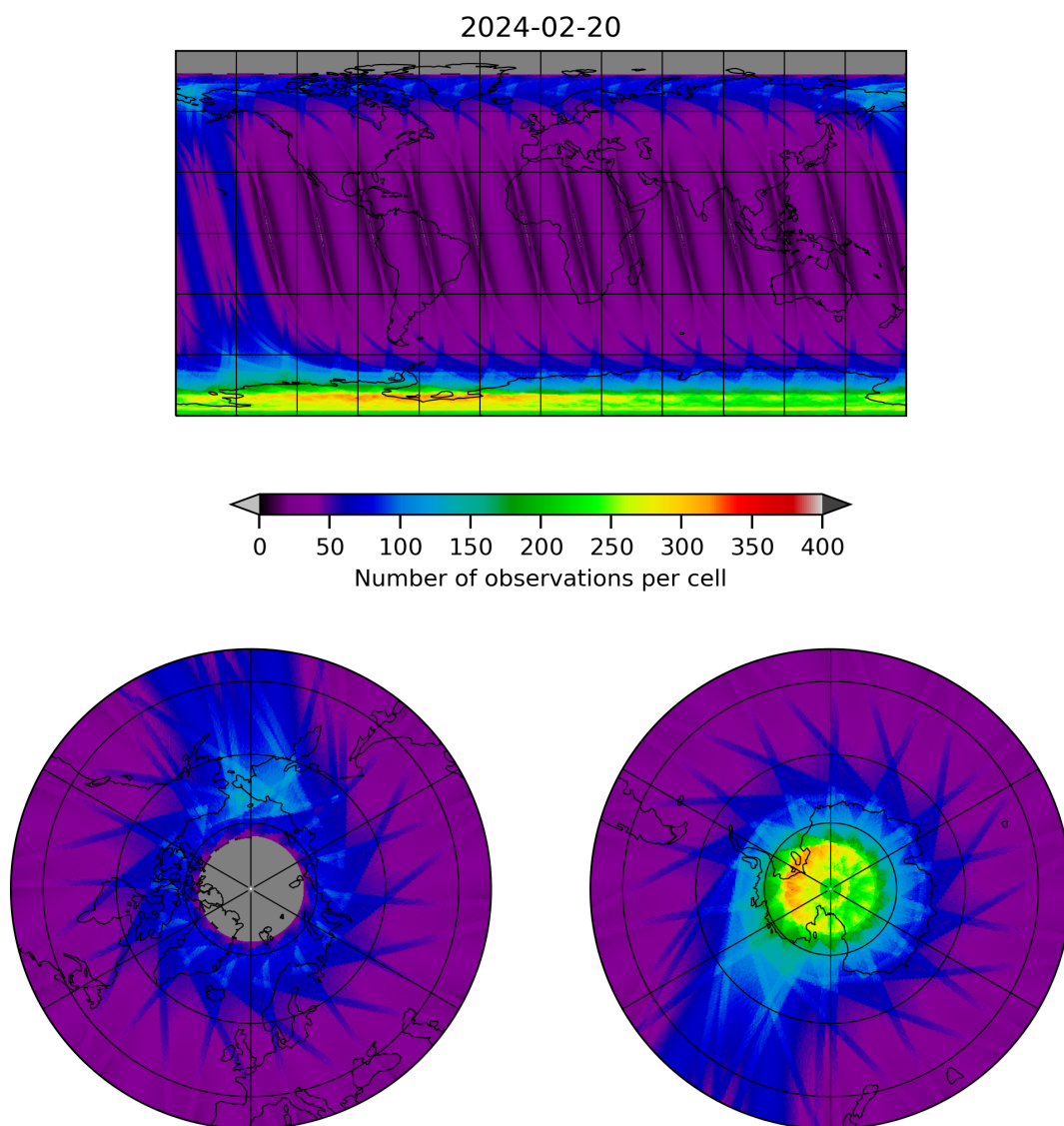
Figure 12: Map of the number of observations for 2024-02-19 to 2024-02-21
