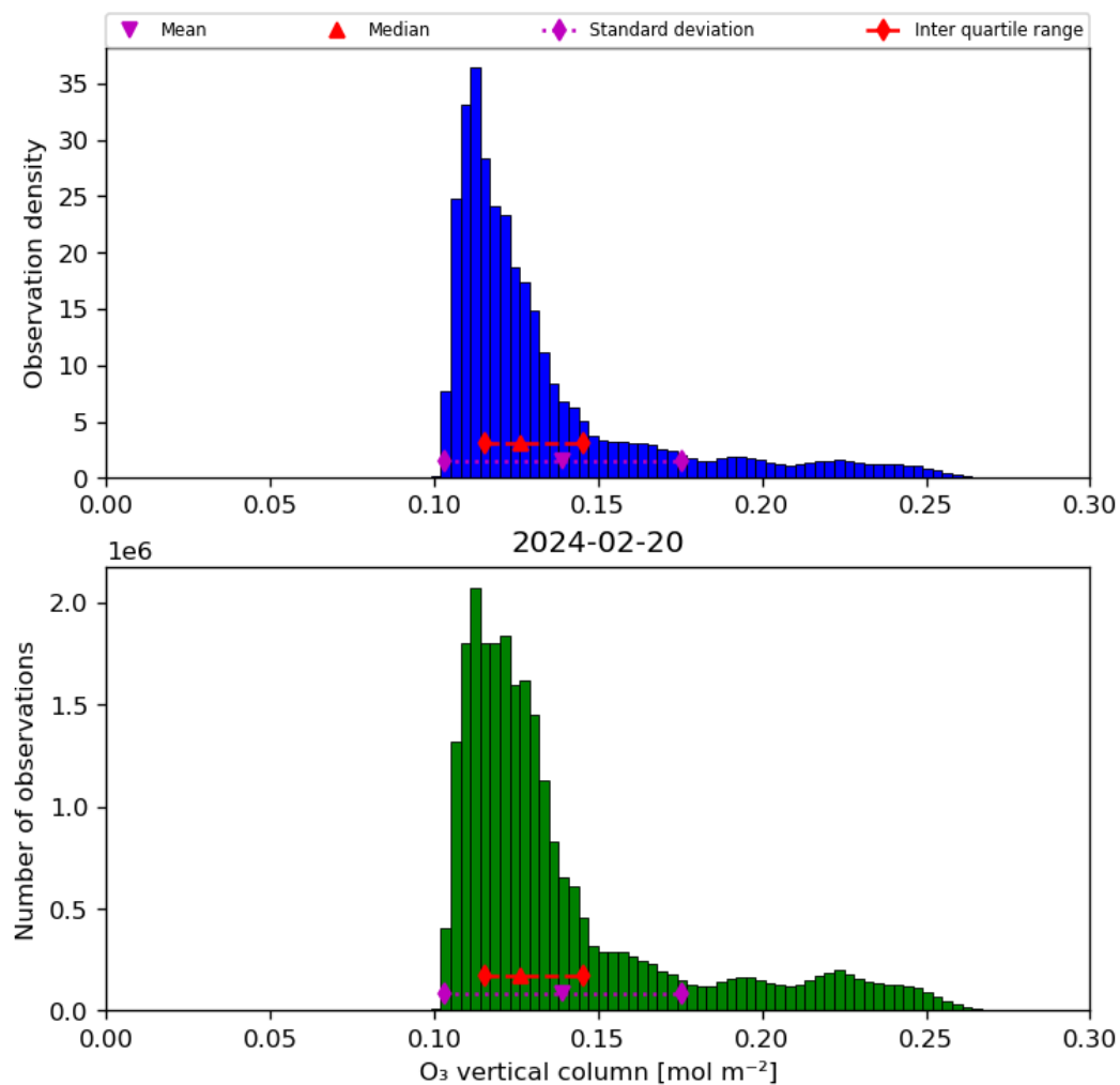
Figure 21: Histogram of “O 3 vertical column” for 2024-02-19 to 2024-02-21
