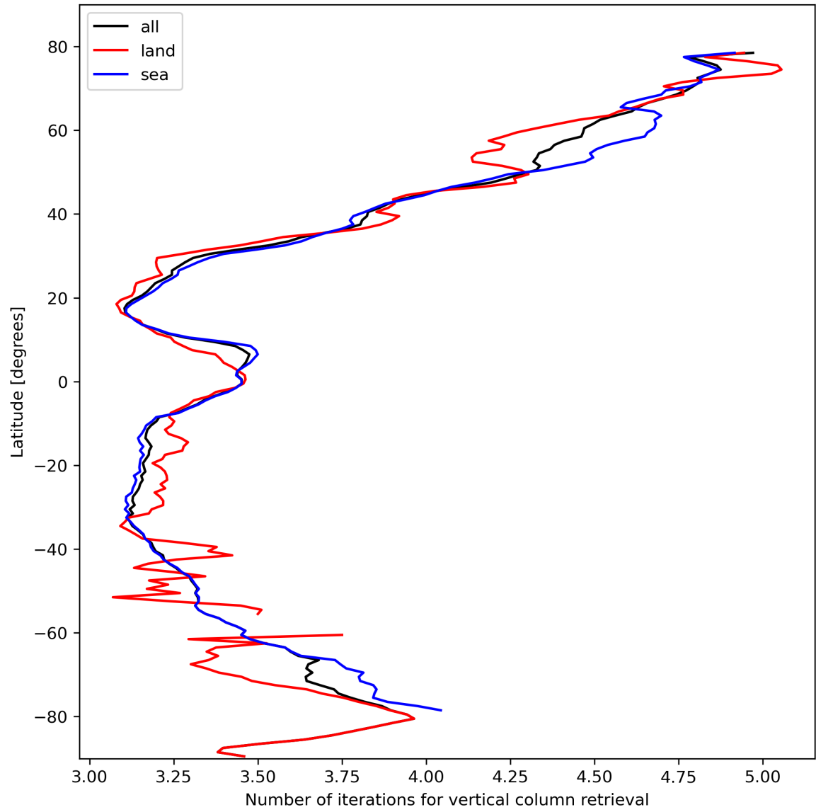
Figure 19: Zonal average of “Number of iterations for vertical column retrieval” for 2024-02-19 to 2024-02-21.
