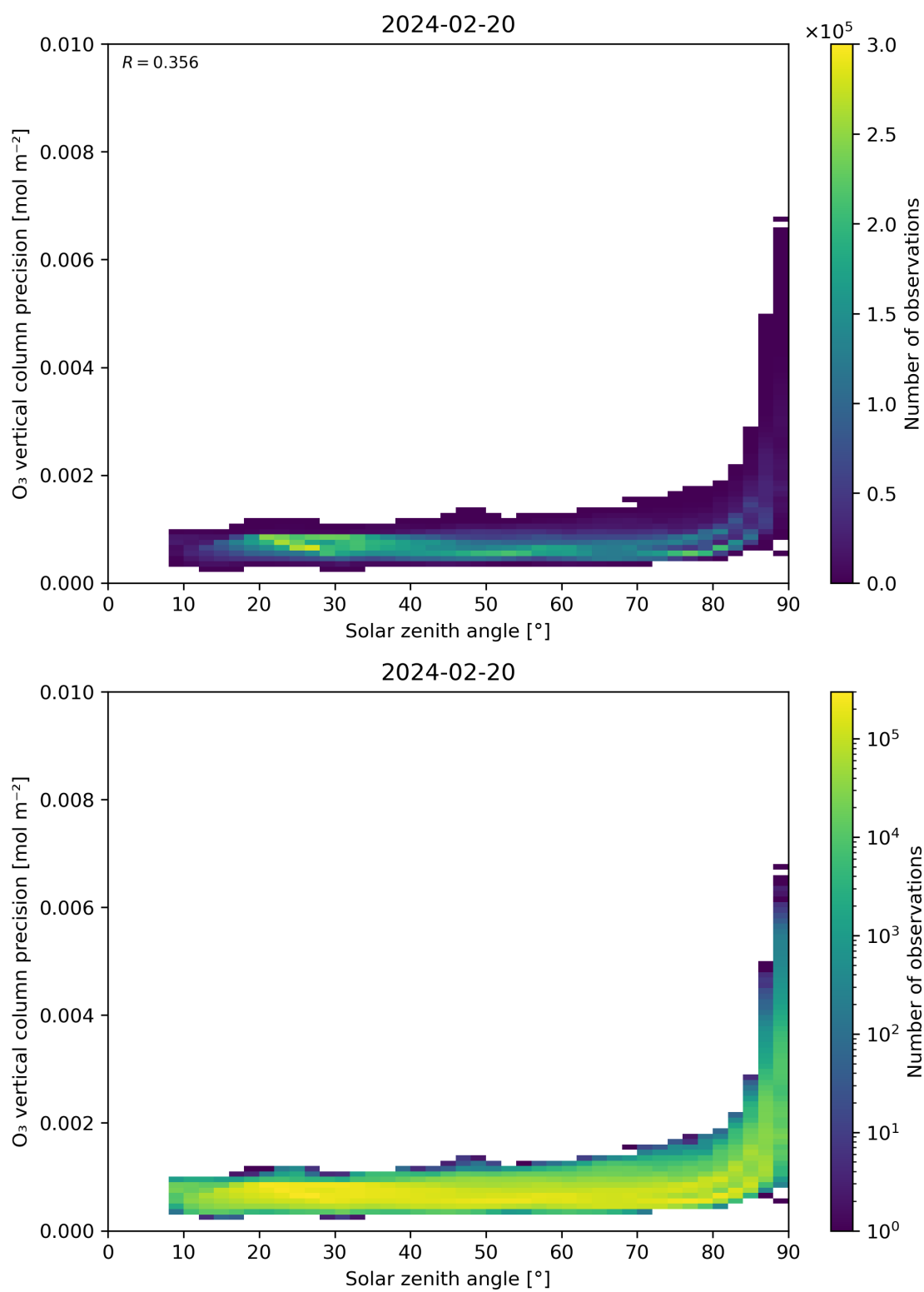
Figure 48: Scatter density plot of “Solar zenith angle” against “O 3 vertical column precision” for 2024-02-19 to 2024-02-21.
