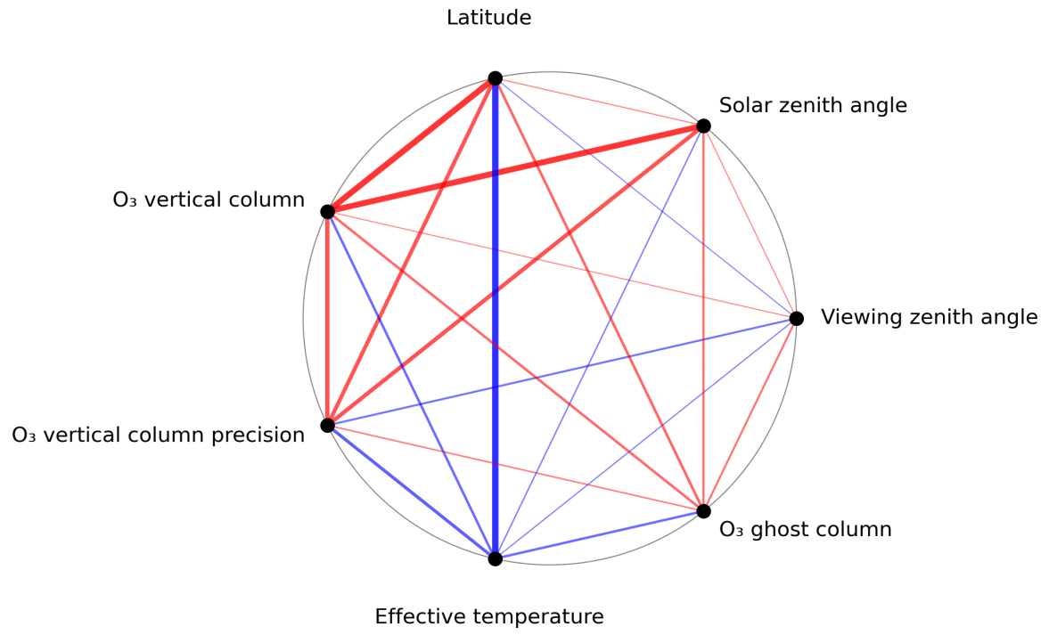
Figure 1: Map of correlation graph for 2024-02-19 to 2024-02-21.
