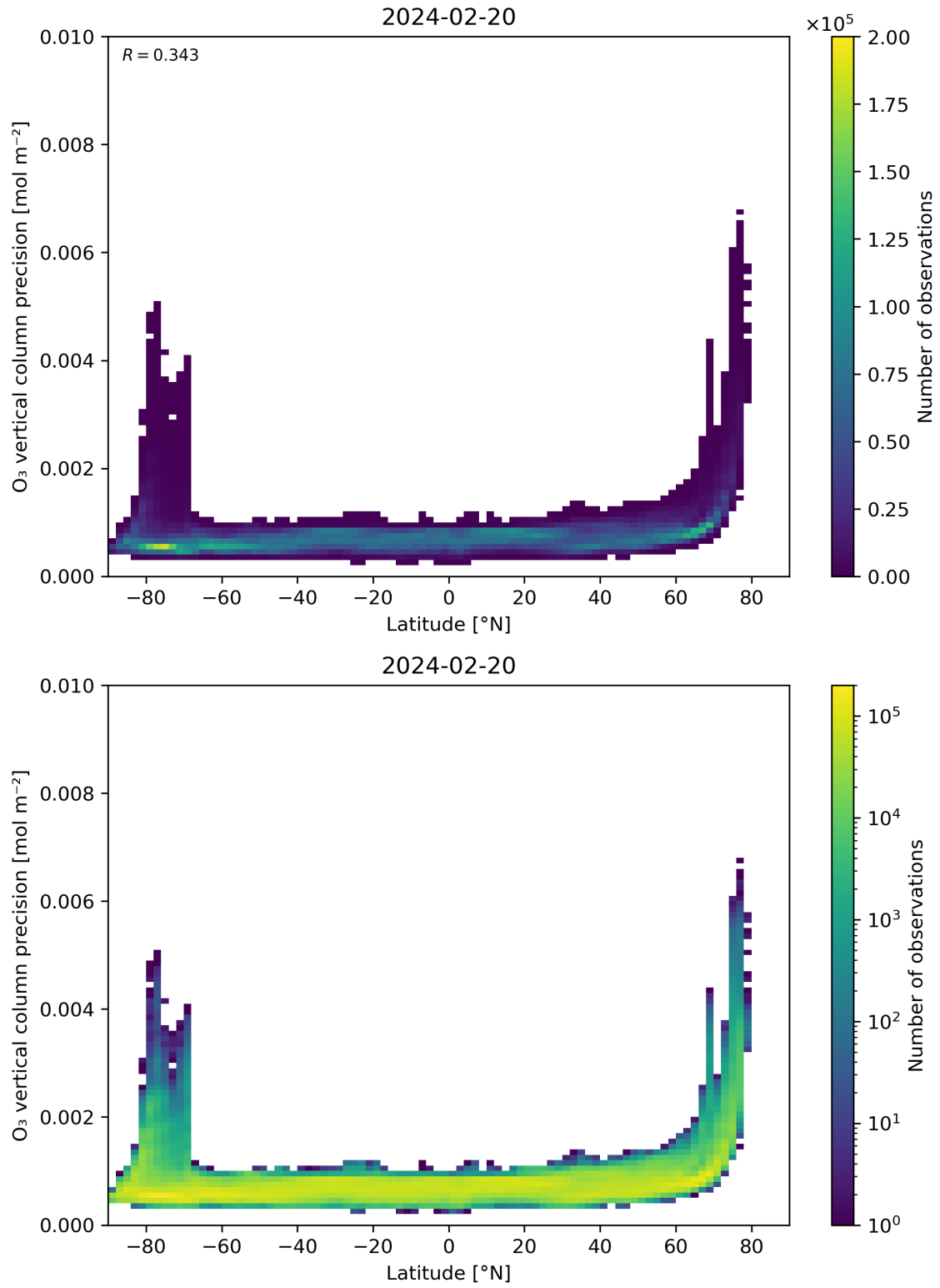
Figure 37: Scatter density plot of “Latitude” against “O 3 vertical column precision” for 2024-02-19 to 2024-02-21.
