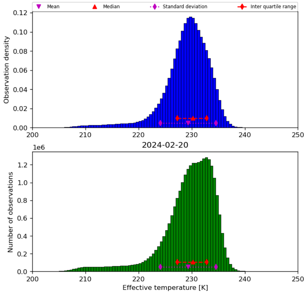
Figure 24: Histogram of “Effective temperature” for 2024-02-19 to 2024-02-21
