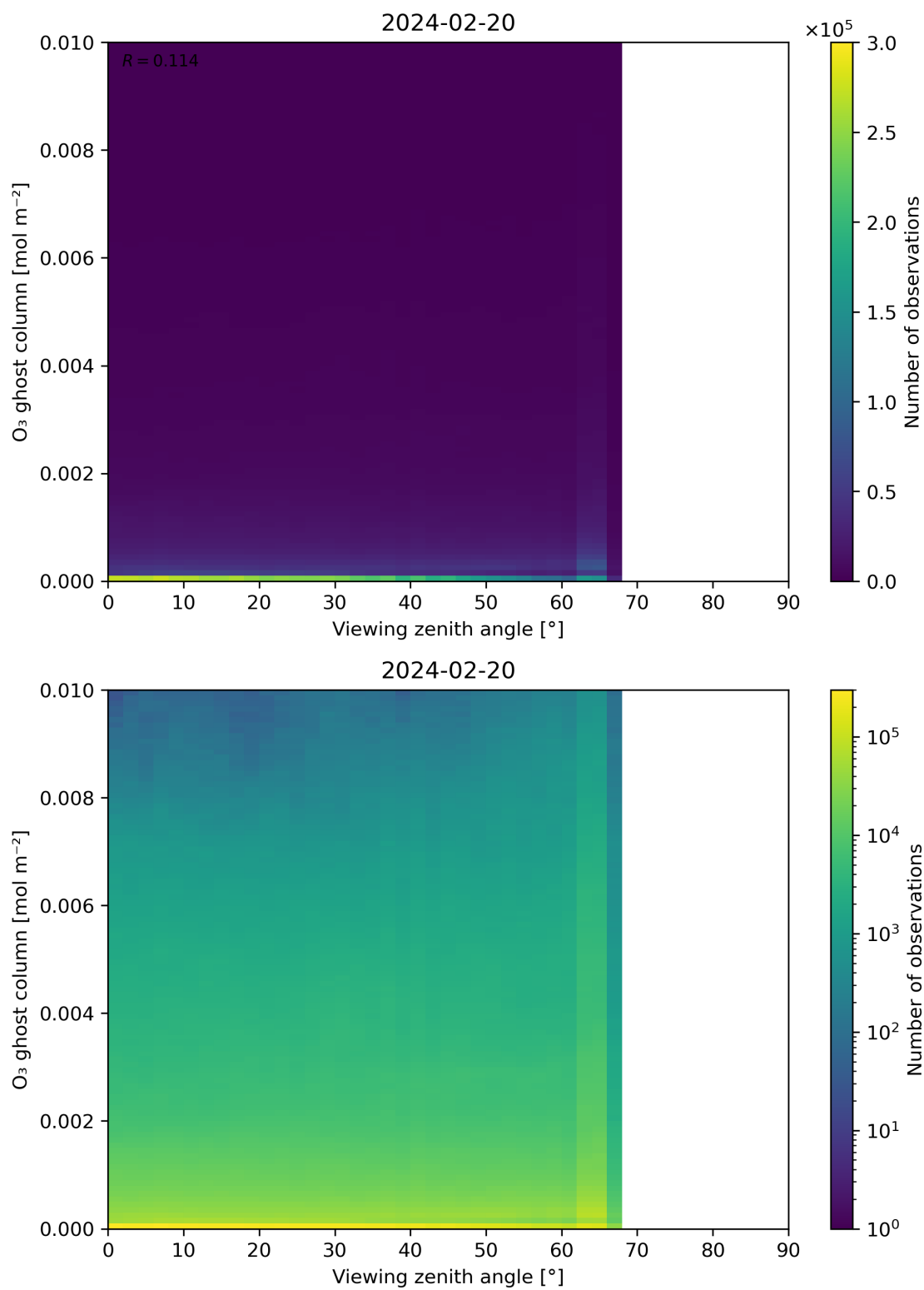
Figure 51: Scatter density plot of “Viewing zenith angle” against “O 3 ghost column” for 2024-02-19 to 2024-02-21.
