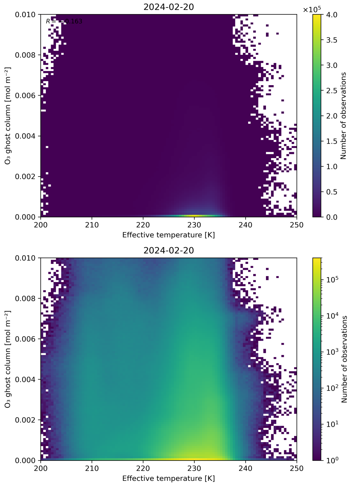
Figure 38: Scatter density plot of “Effective temperature” against “O 3 ghost column” for 2024-02-19 to 2024-02-21.
