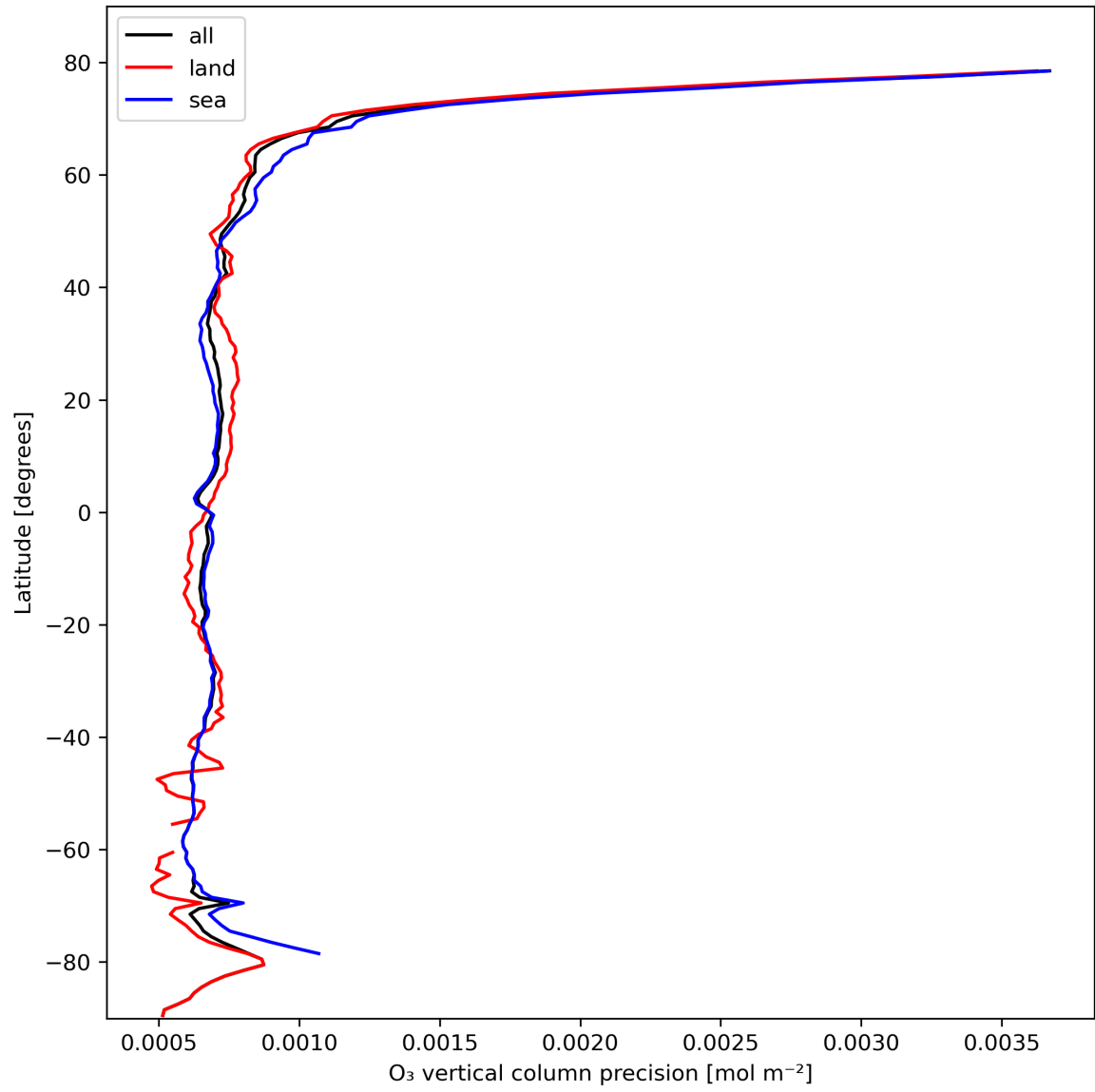
Figure 15: Zonal average of “O 3 vertical column precision” for 2024-02-19 to 2024-02-21.
