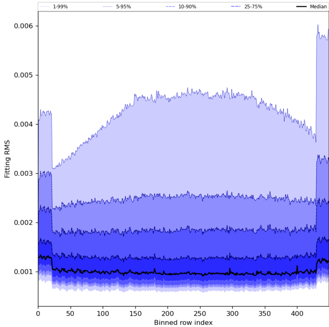
Figure 30: Along track statistics of “Fitting RMS” for 2024-02-19 to 2024-02-21
