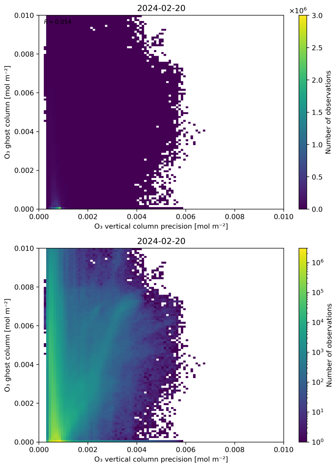
Figure 43: Scatter density plot of “ O_3 vertical column precision” against “ O_3 ghost column” for 2024-02-19 to 2024-02-21.
