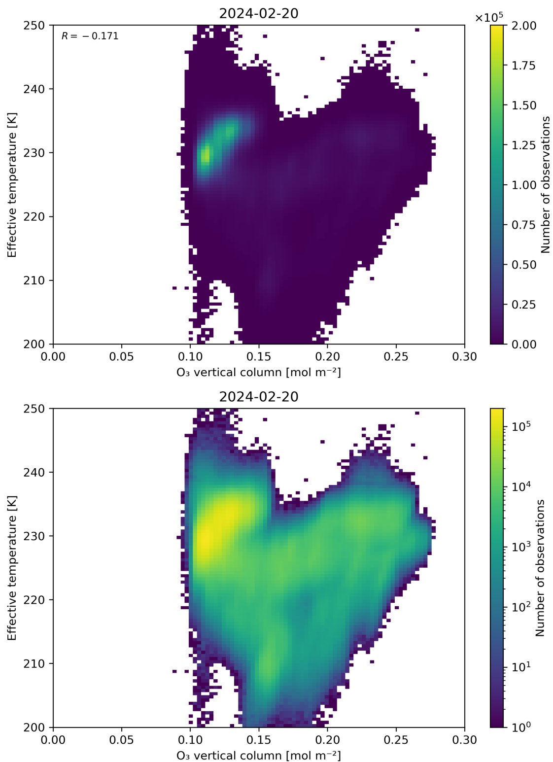
Figure 39: Scatter density plot of “O 3 vertical column” against “Effective temperature” for 2024-02-19 to 2024-02-21.
