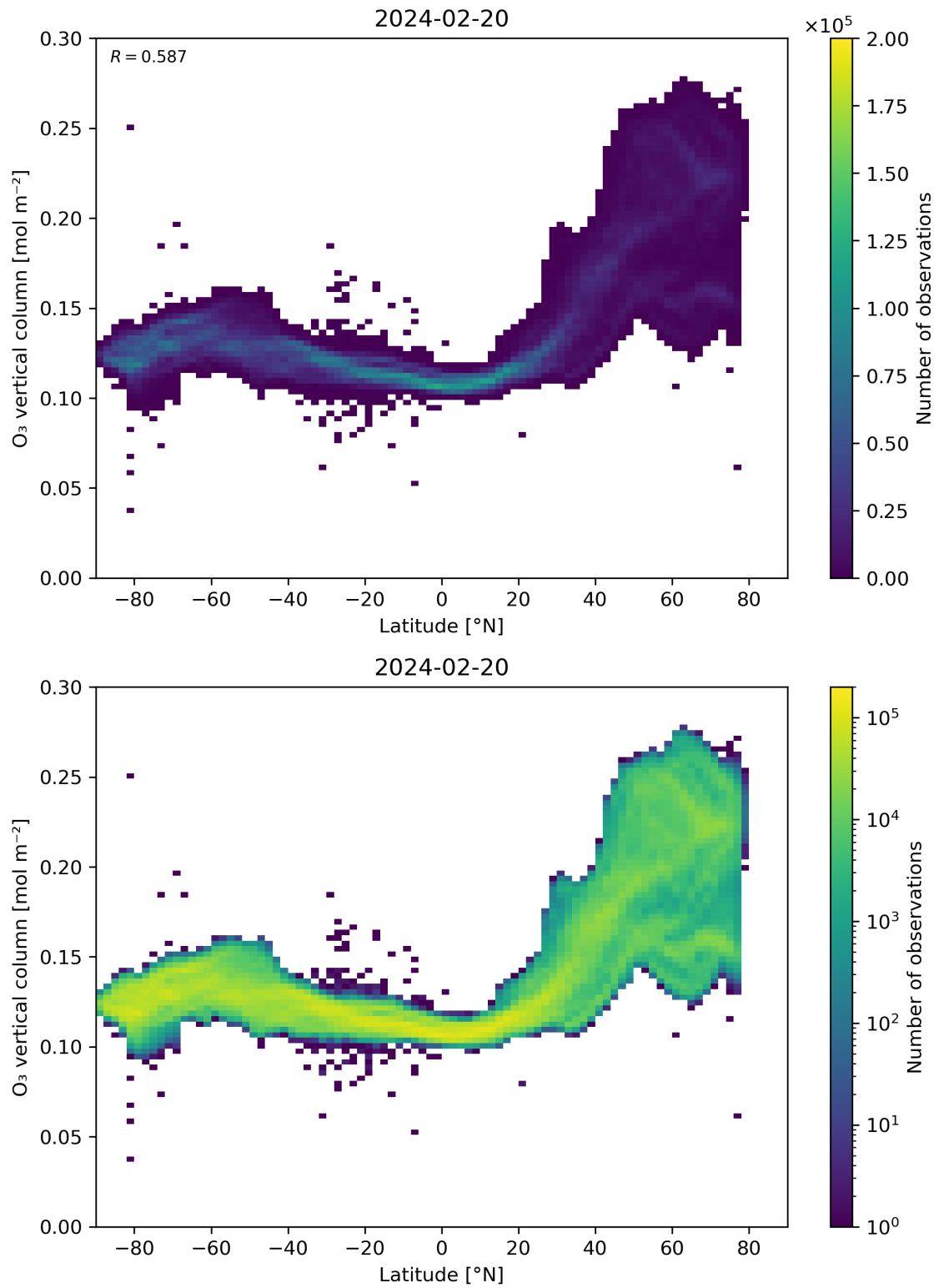
Figure 36: Scatter density plot of “Latitude” against “O 3 vertical column” for 2024-02-19 to 2024-02-21.
