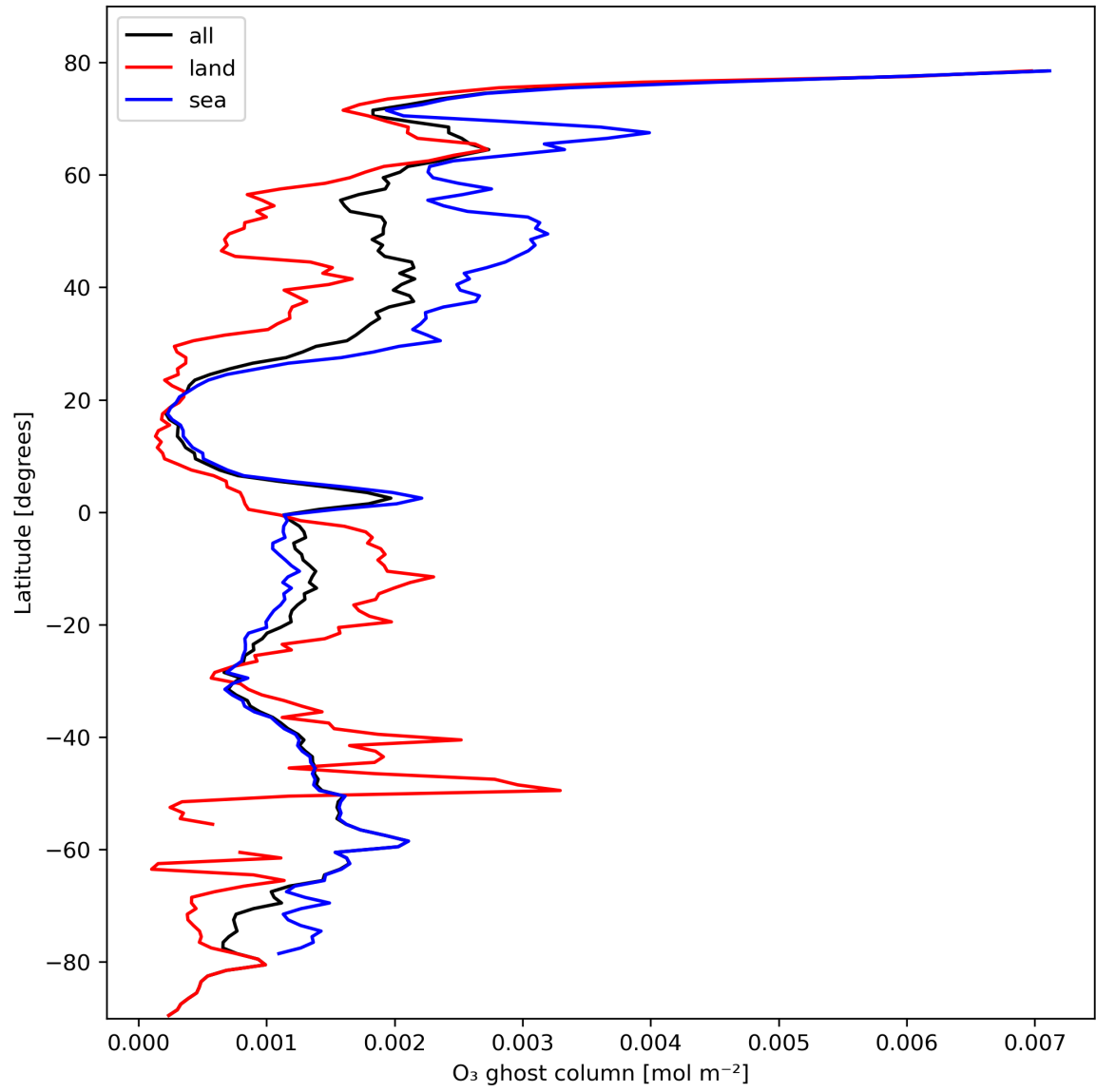
Figure 18: Zonal average of “O 3 ghost column” for 2024-02-19 to 2024-02-21.
