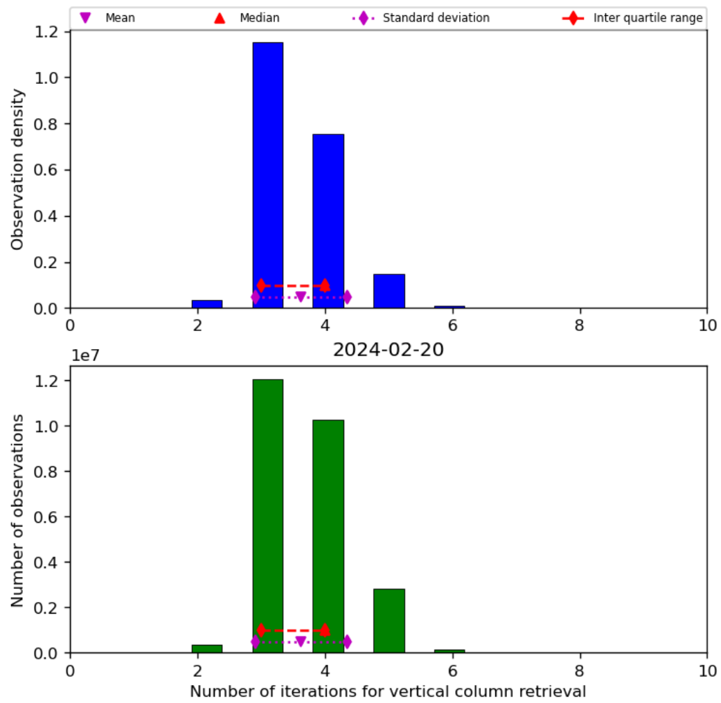
Figure 26: Histogram of “Number of iterations for vertical column retrieval” for 2024-02-19 to 2024-02-21
