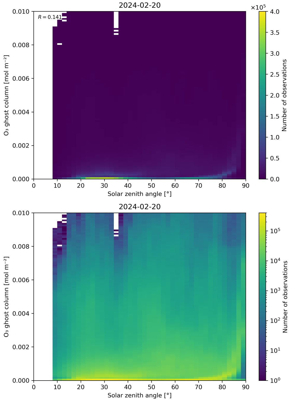
Figure 46: Scatter density plot of “Solar zenith angle” against “O 3 ghost column” for 2024-02-19 to 2024-02-21.
