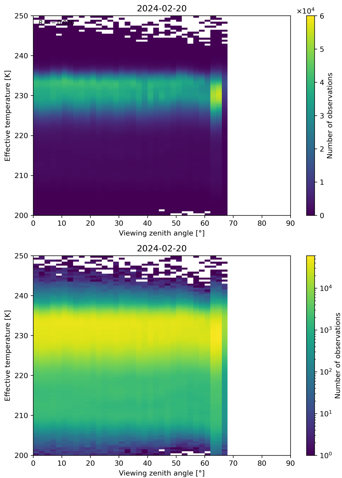
Figure 50: Scatter density plot of “Viewing zenith angle” against “Effective temperature” for 2024-02-19 to 2024-02-21.
