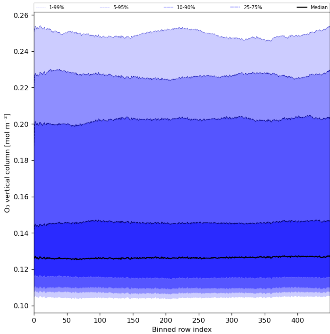
Figure 28: Along track statistics of “ \text{O}_3 vertical column” for 2024-02-19 to 2024-02-21
