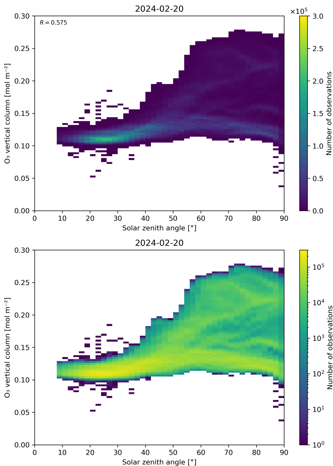
Figure 47: Scatter density plot of “Solar zenith angle” against “O 3 vertical column” for 2024-02-19 to 2024-02-21.
