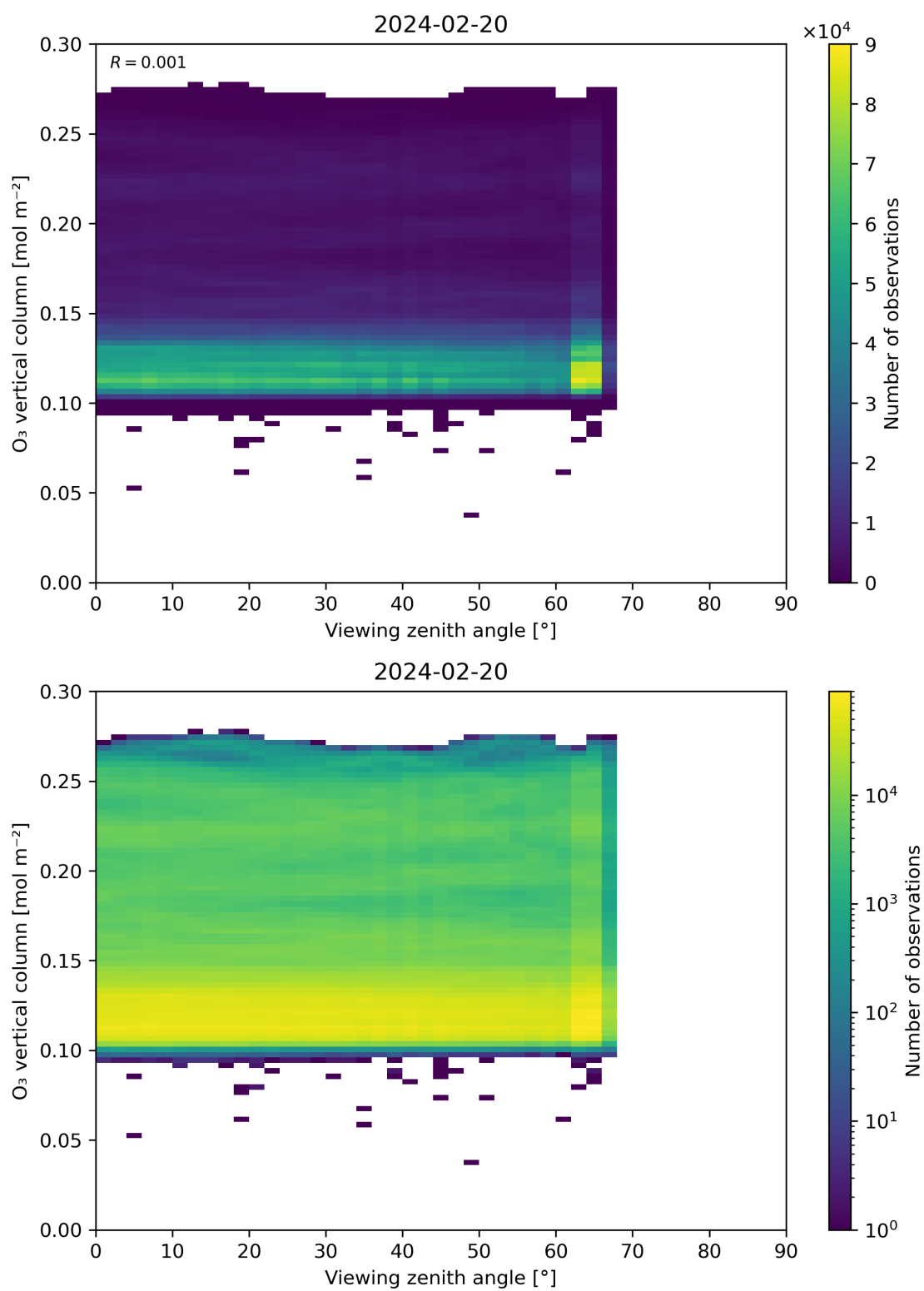
Figure 52: Scatter density plot of “Viewing zenith angle” against “O 3 vertical column” for 2024-02-19 to 2024-02-21.
