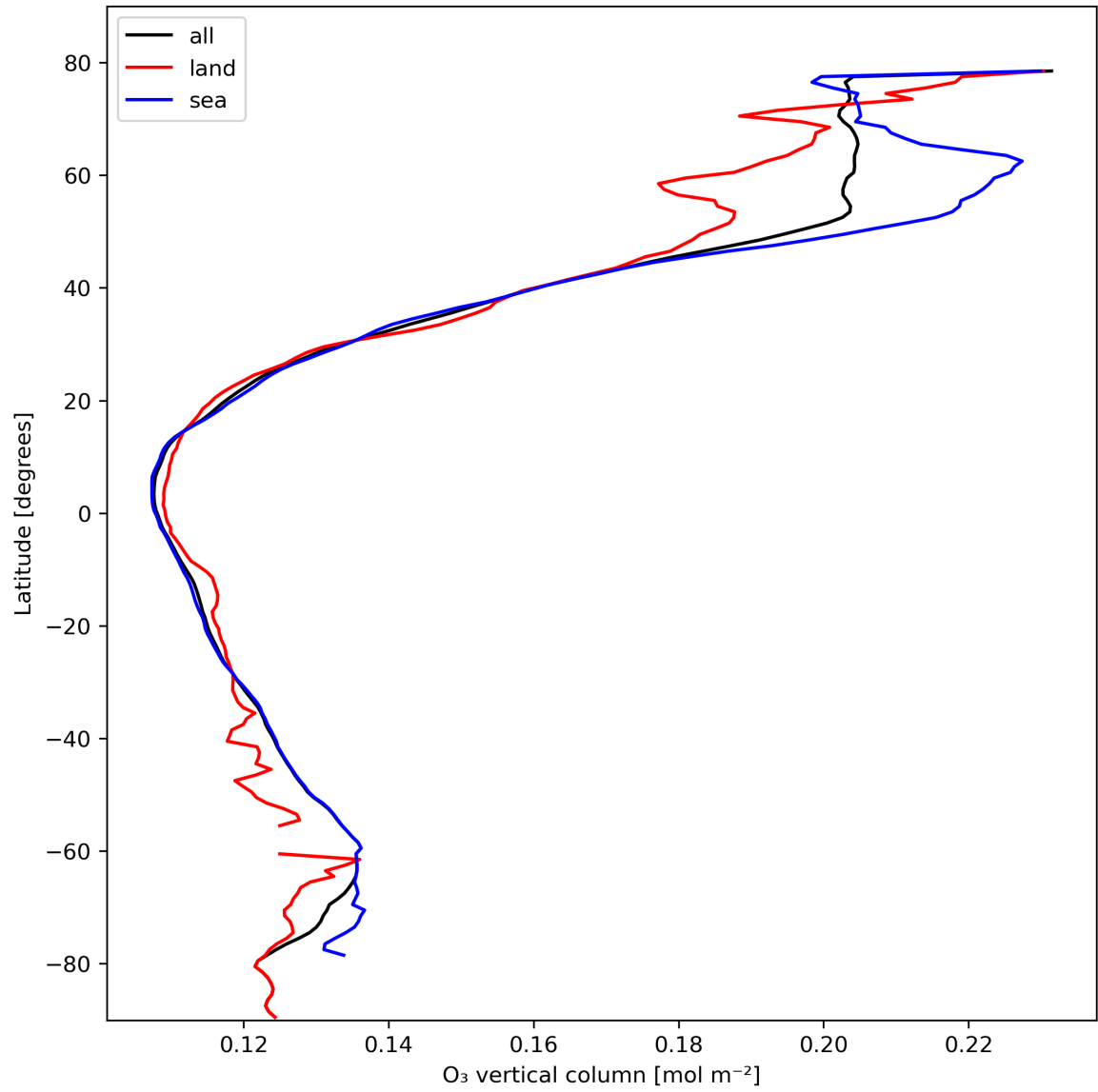
Figure 14: Zonal average of “O 3 vertical column” for 2024-02-19 to 2024-02-21.
