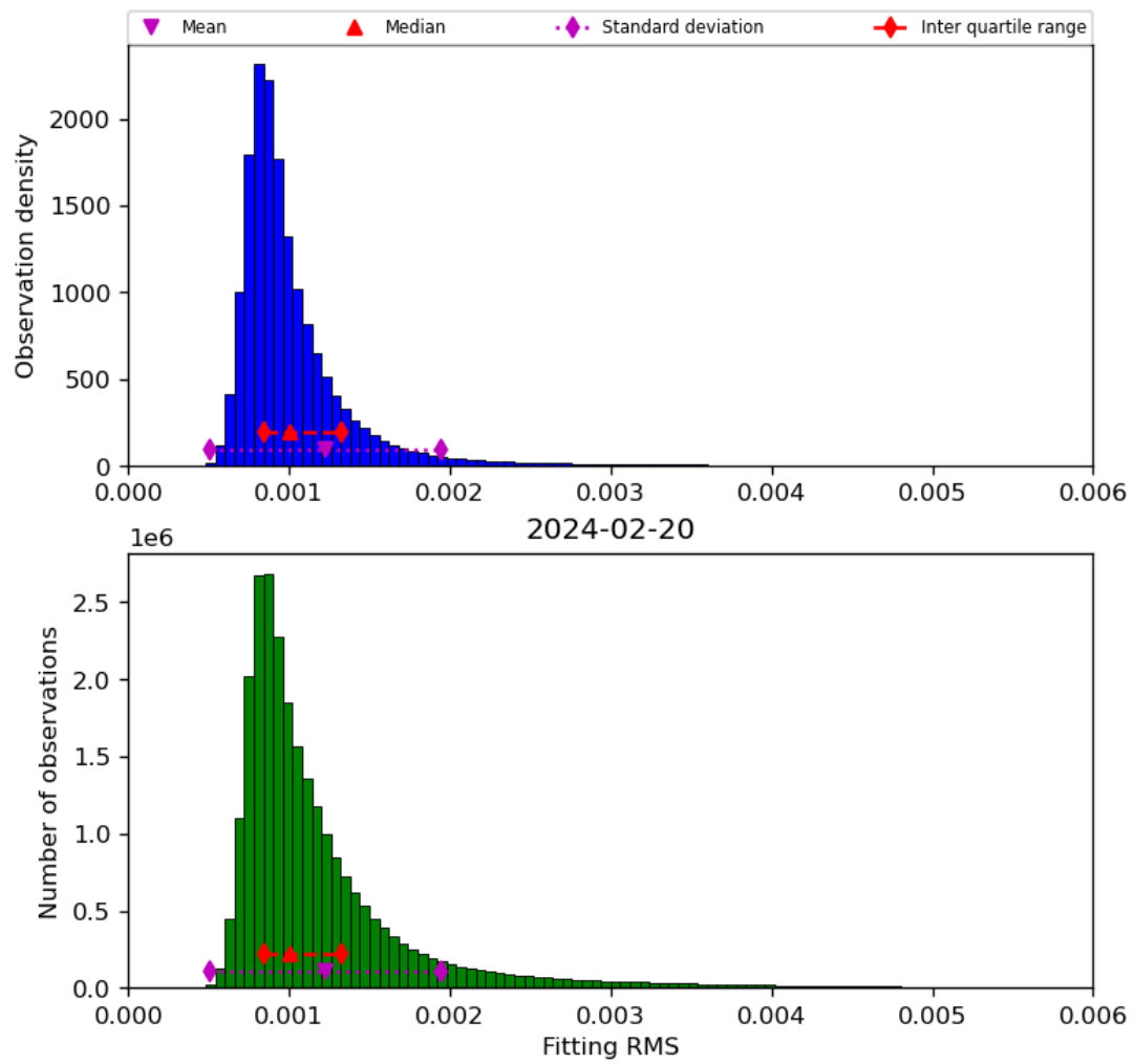
Figure 23: Histogram of “Fitting RMS” for 2024-02-19 to 2024-02-21
