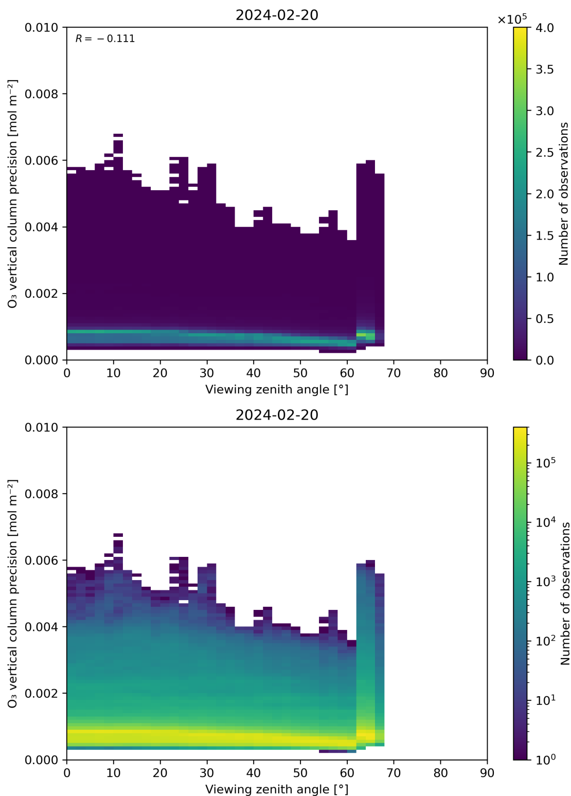
Figure 53: Scatter density plot of “Viewing zenith angle” against “O 3 vertical column precision” for 2024-02-19 to 2024-02-21.
