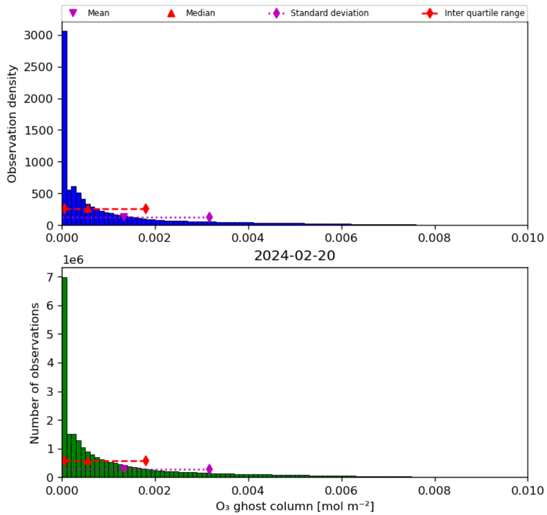
Figure 25: Histogram of “O 3 ghost column” for 2024-02-19 to 2024-02-21
