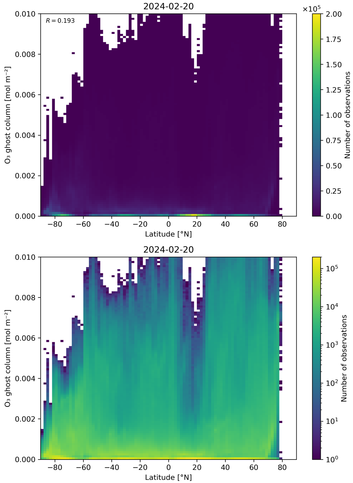
Figure 35: Scatter density plot of “Latitude” against “O 3 ghost column” for 2024-02-19 to 2024-02-21.
