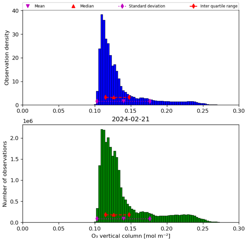
Figure 21: Histogram of “O 3 vertical column” for 2024-02-20 to 2024-02-22
