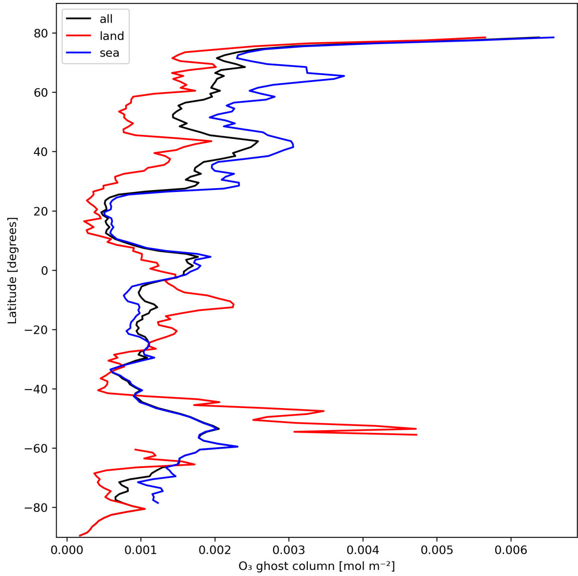
Figure 18: Zonal average of "O 3 ghost column" for 2024-02-20 to 2024-02-22.
