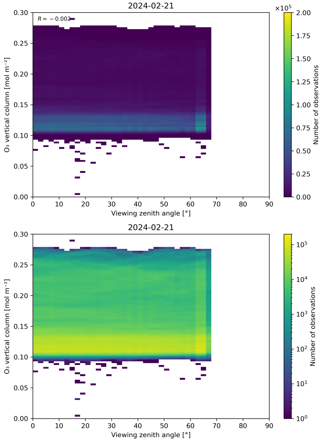
Figure 52: Scatter density plot of “Viewing zenith angle” against “O 3 vertical column” for 2024-02-20 to 2024-02-22.
