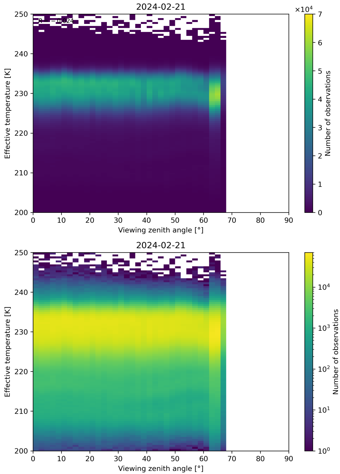
Figure 50: Scatter density plot of “Viewing zenith angle” against “Effective temperature” for 2024-02-20 to 2024-02-22.
