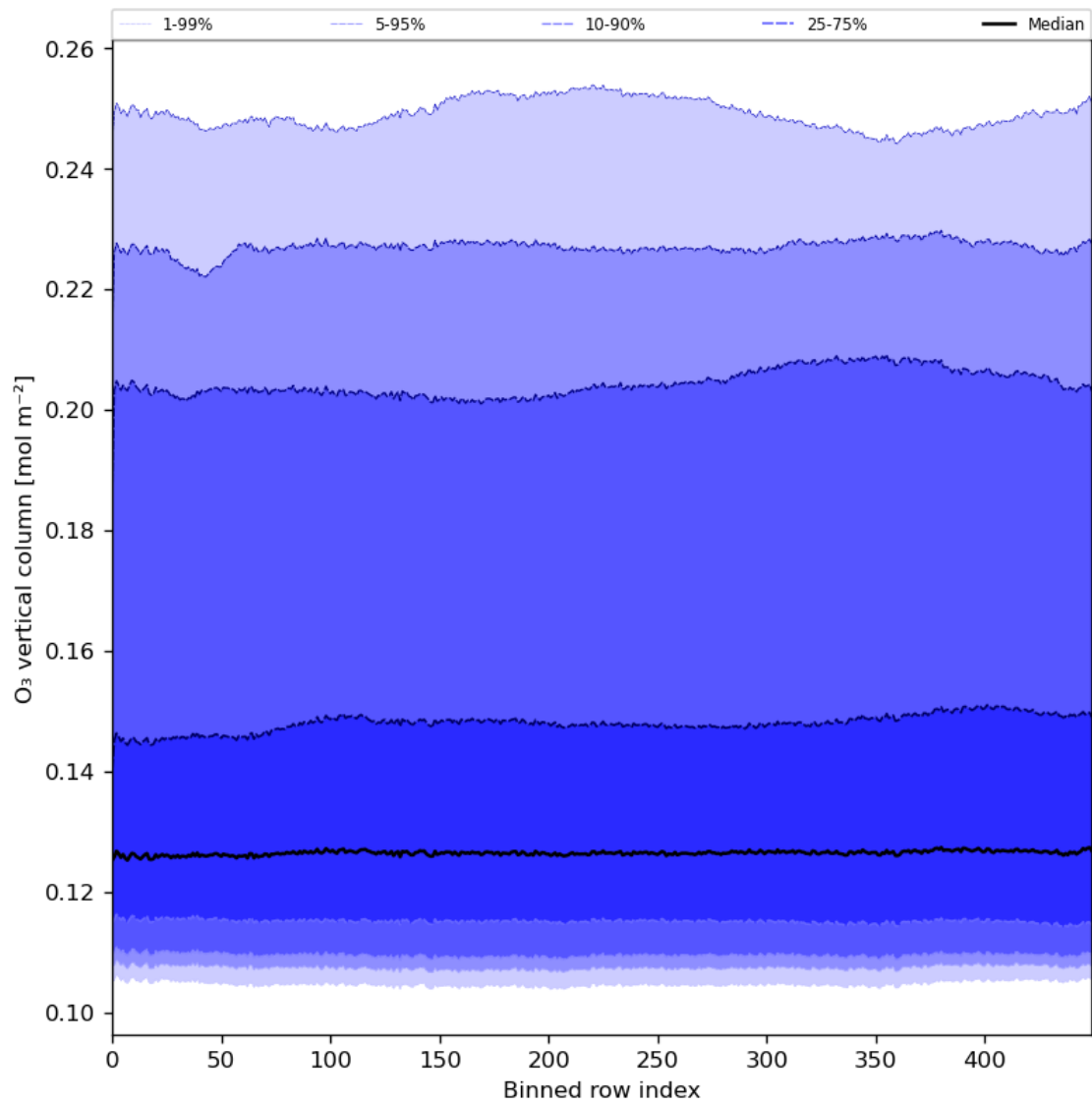
Figure 28: Along track statistics of “O 3 vertical column” for 2024-02-20 to 2024-02-22
