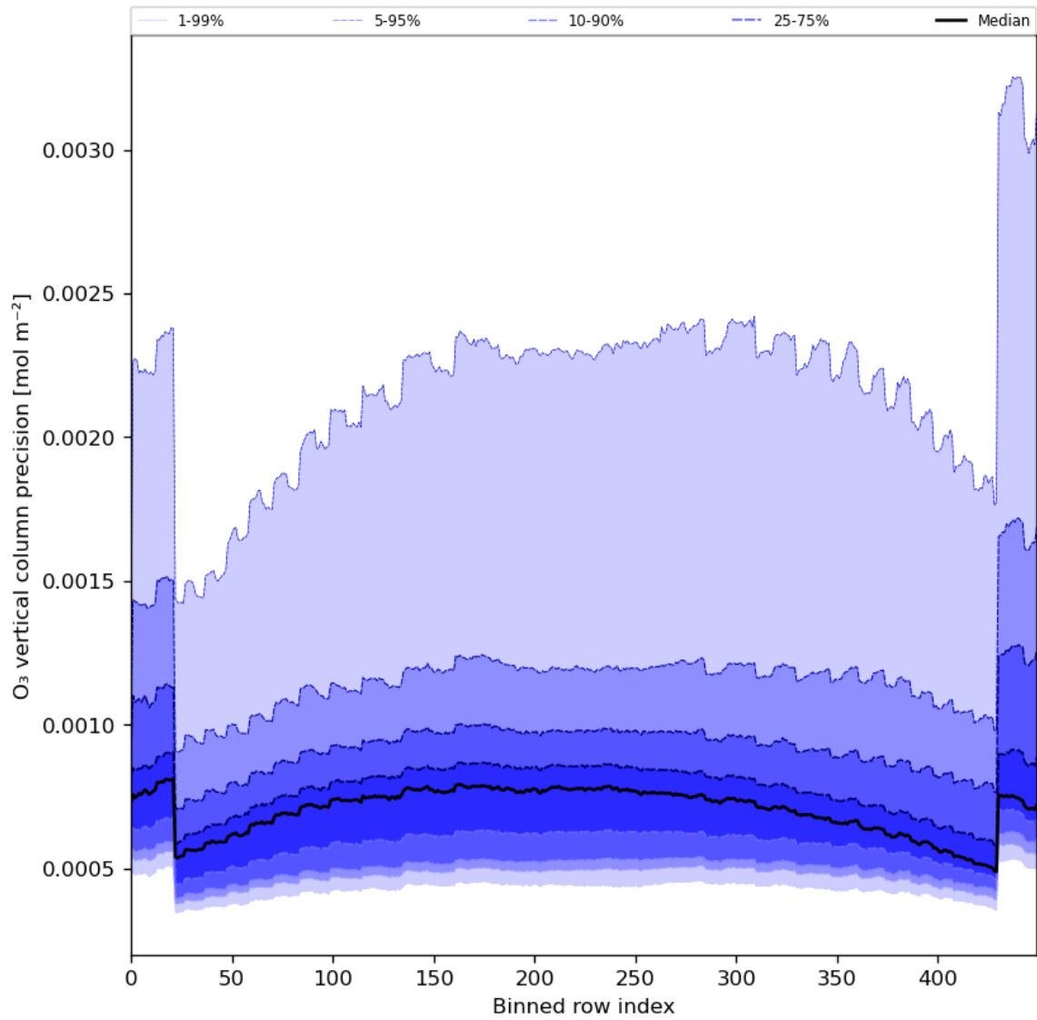
Figure 29: Along track statistics of “O 3 vertical column precision” for 2024-02-20 to 2024-02-22
