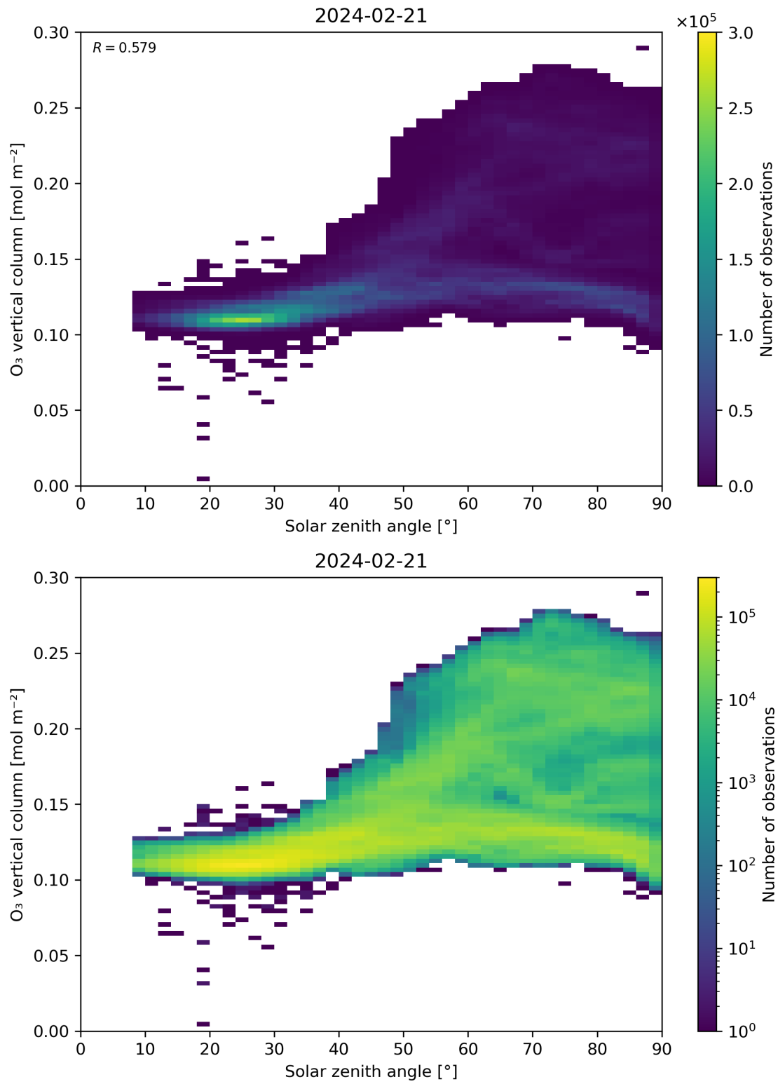
Figure 47: Scatter density plot of “Solar zenith angle” against “O 3 vertical column” for 2024-02-20 to 2024-02-22.
