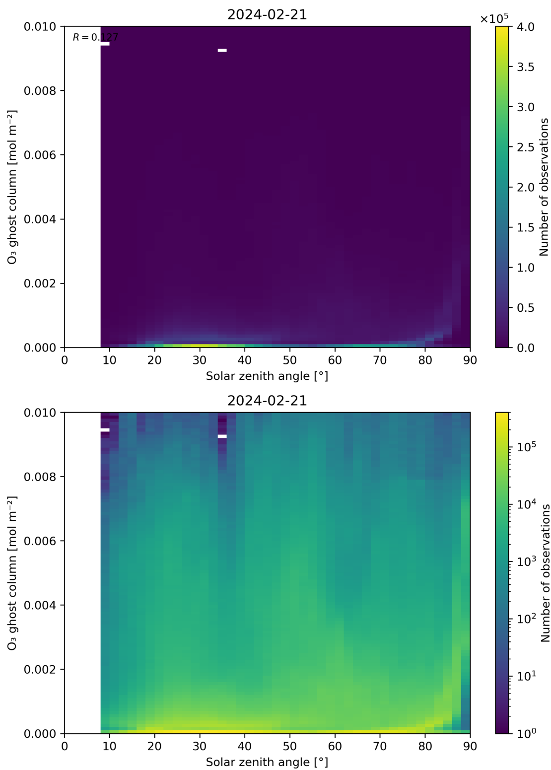
Figure 46: Scatter density plot of “Solar zenith angle” against “O 3 ghost column” for 2024-02-20 to 2024-02-22.
