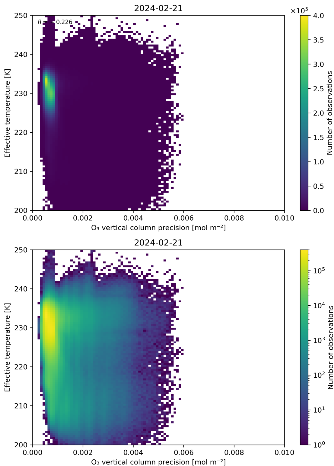
Figure 42: Scatter density plot of “O 3 vertical column precision” against “Effective temperature” for 2024-02-20 to 2024-02-22.
