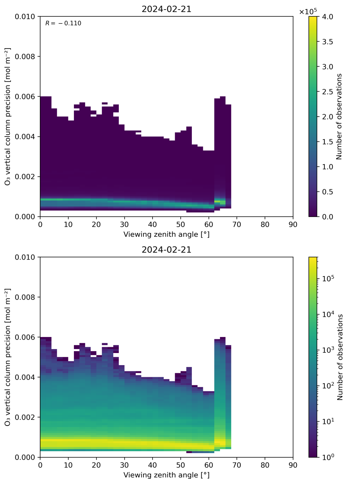
Figure 53: Scatter density plot of “Viewing zenith angle” against “O 3 vertical column precision” for 2024-02-20 to 2024-02-22.
