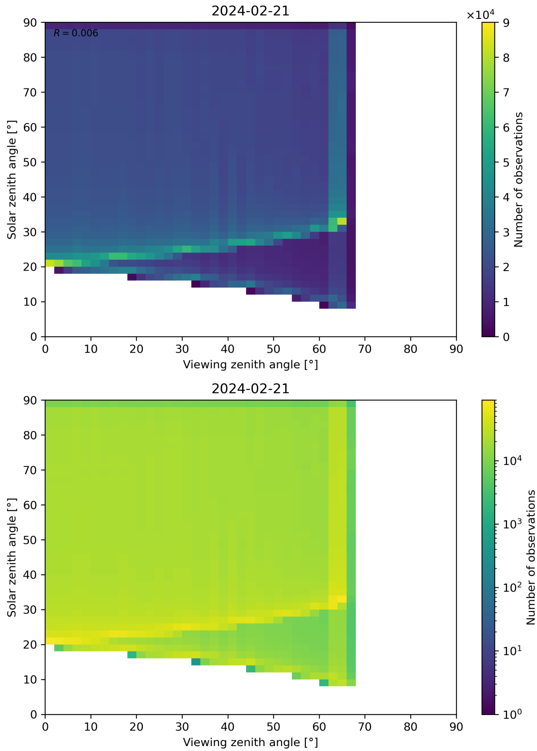
Figure 54: Scatter density plot of “Viewing zenith angle” against “Solar zenith angle” for 2024-02-20 to 2024-02-22.
