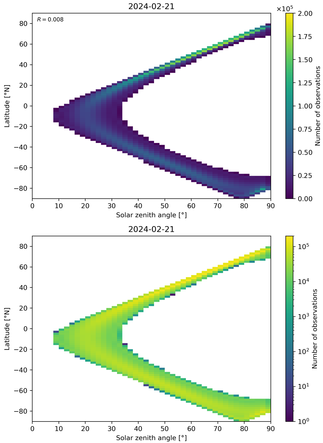
Figure 44: Scatter density plot of “Solar zenith angle” against “Latitude” for 2024-02-20 to 2024-02-22.
