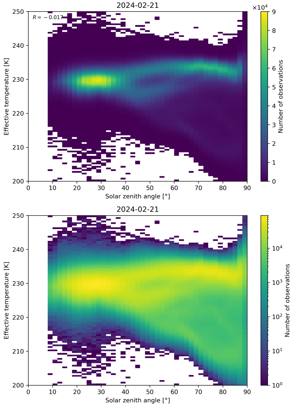
Figure 45: Scatter density plot of “Solar zenith angle” against “Effective temperature” for 2024-02-20 to 2024-02-22.
