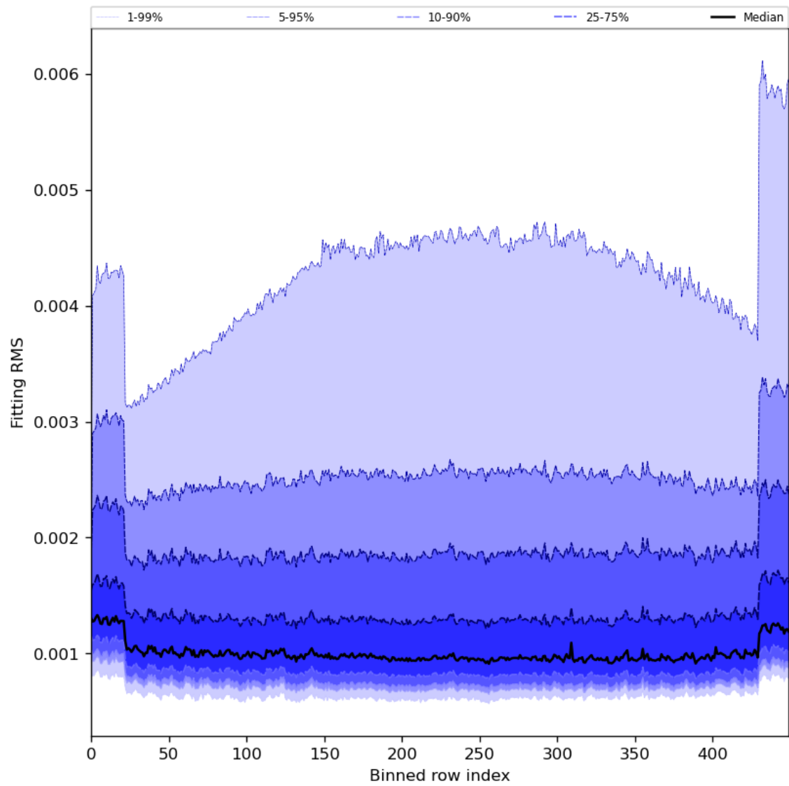
Figure 30: Along track statistics of “Fitting RMS” for 2024-02-20 to 2024-02-22
