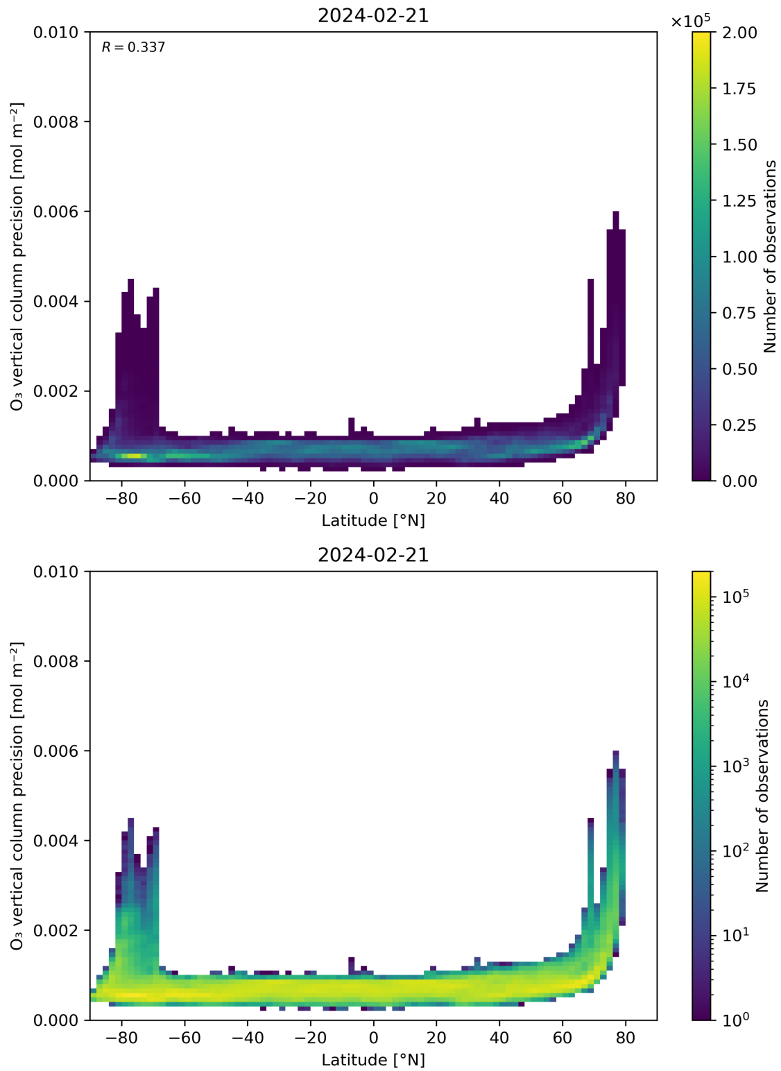
Figure 37: Scatter density plot of “Latitude” against “O 3 vertical column precision” for 2024-02-20 to 2024-02-22.
