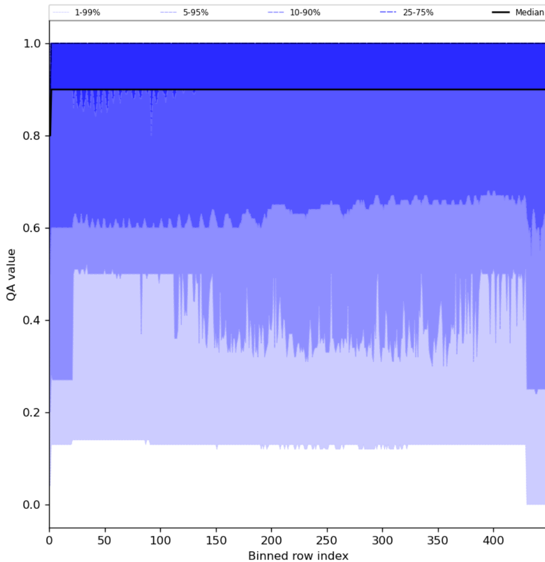
Figure 27: Along track statistics of “QA value” for 2024-02-20 to 2024-02-22
