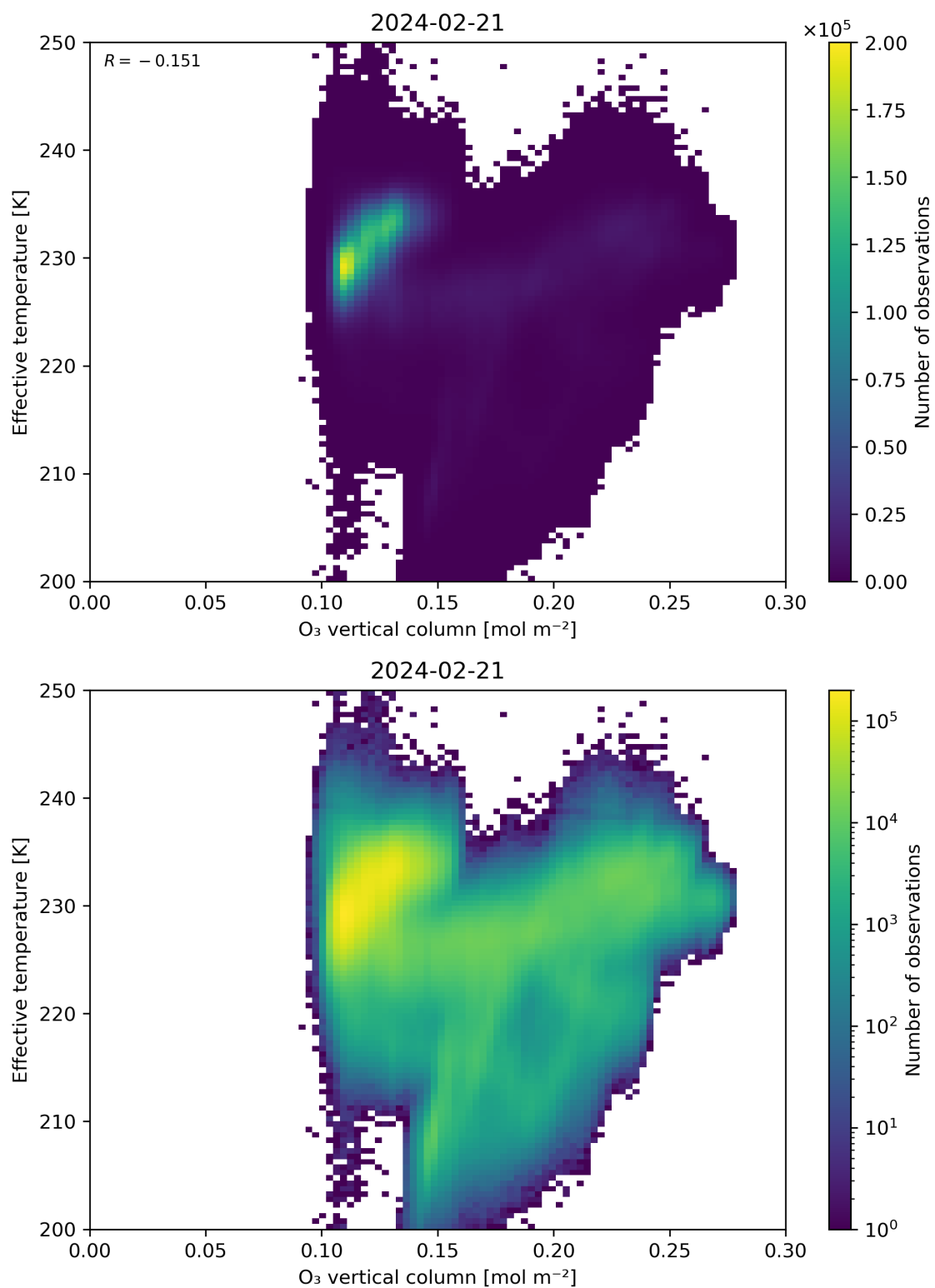
Figure 39: Scatter density plot of “O 3 vertical column” against “Effective temperature” for 2024-02-20 to 2024-02-22.
