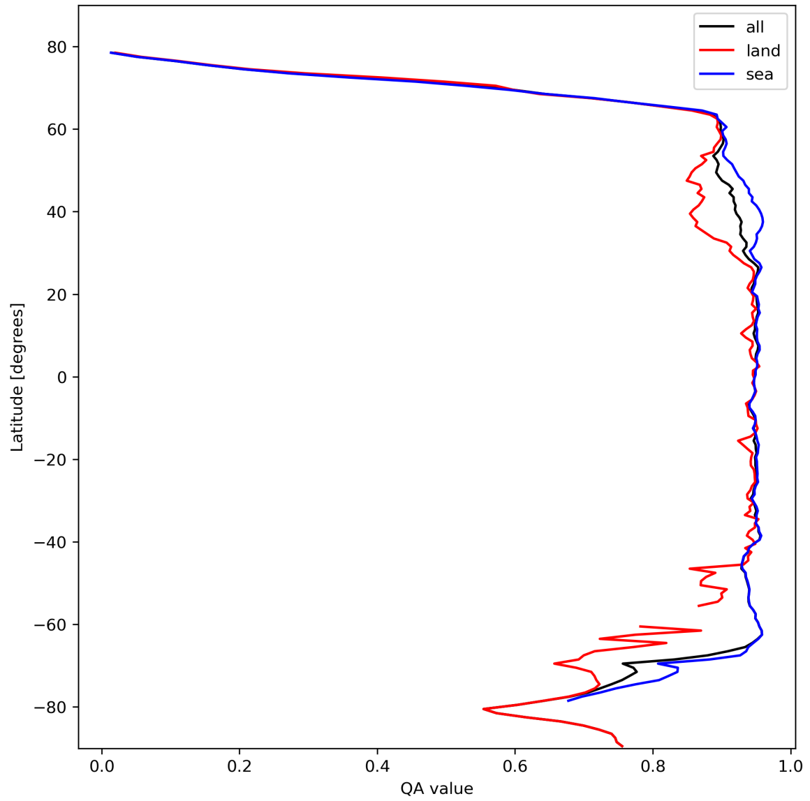
Figure 13: Zonal average of “QA value” for 2024-02-20 to 2024-02-22.
