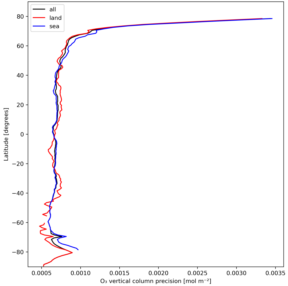
Figure 15: Zonal average of “O 3 vertical column precision” for 2024-02-20 to 2024-02-22.
