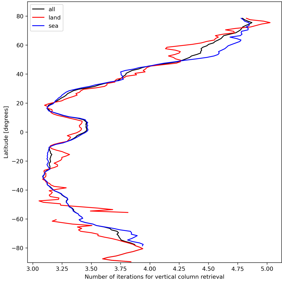
Figure 19: Zonal average of “Number of iterations for vertical column retrieval” for 2024-02-20 to 2024-02-22.
