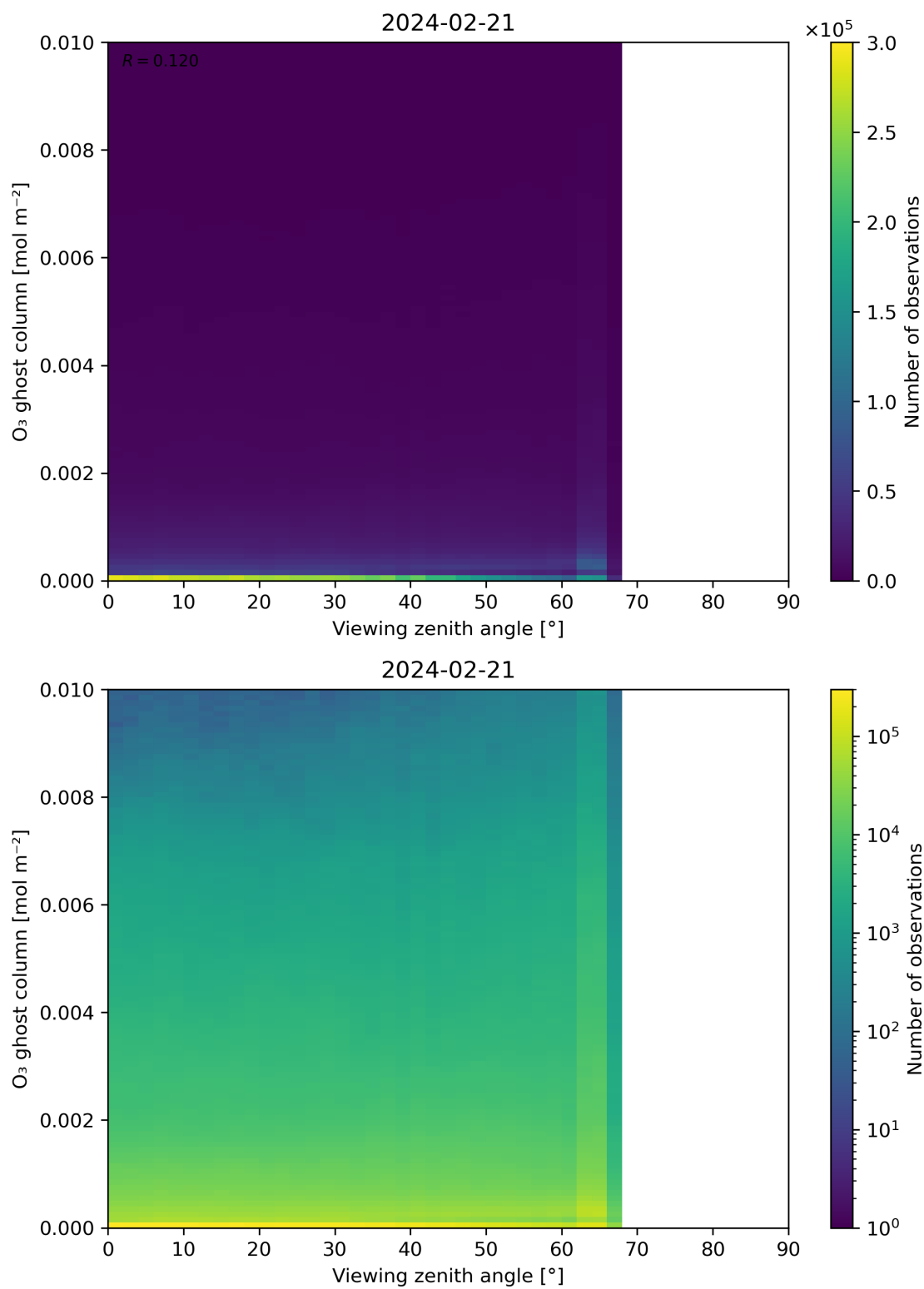
Figure 51: Scatter density plot of “Viewing zenith angle” against “O 3 ghost column” for 2024-02-20 to 2024-02-22.
