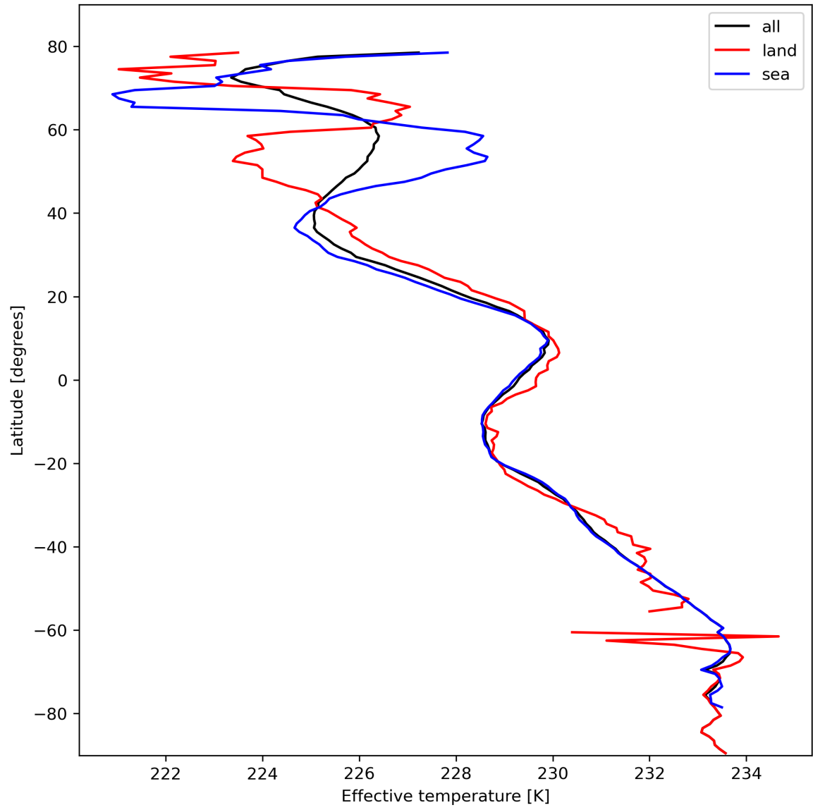
Figure 17: Zonal average of “Effective temperature” for 2024-02-20 to 2024-02-22.
