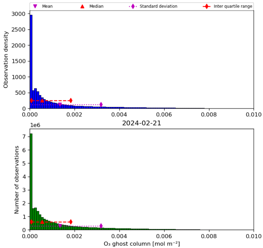
Figure 25: Histogram of "O 3 ghost column" for 2024-02-20 to 2024-02-22
