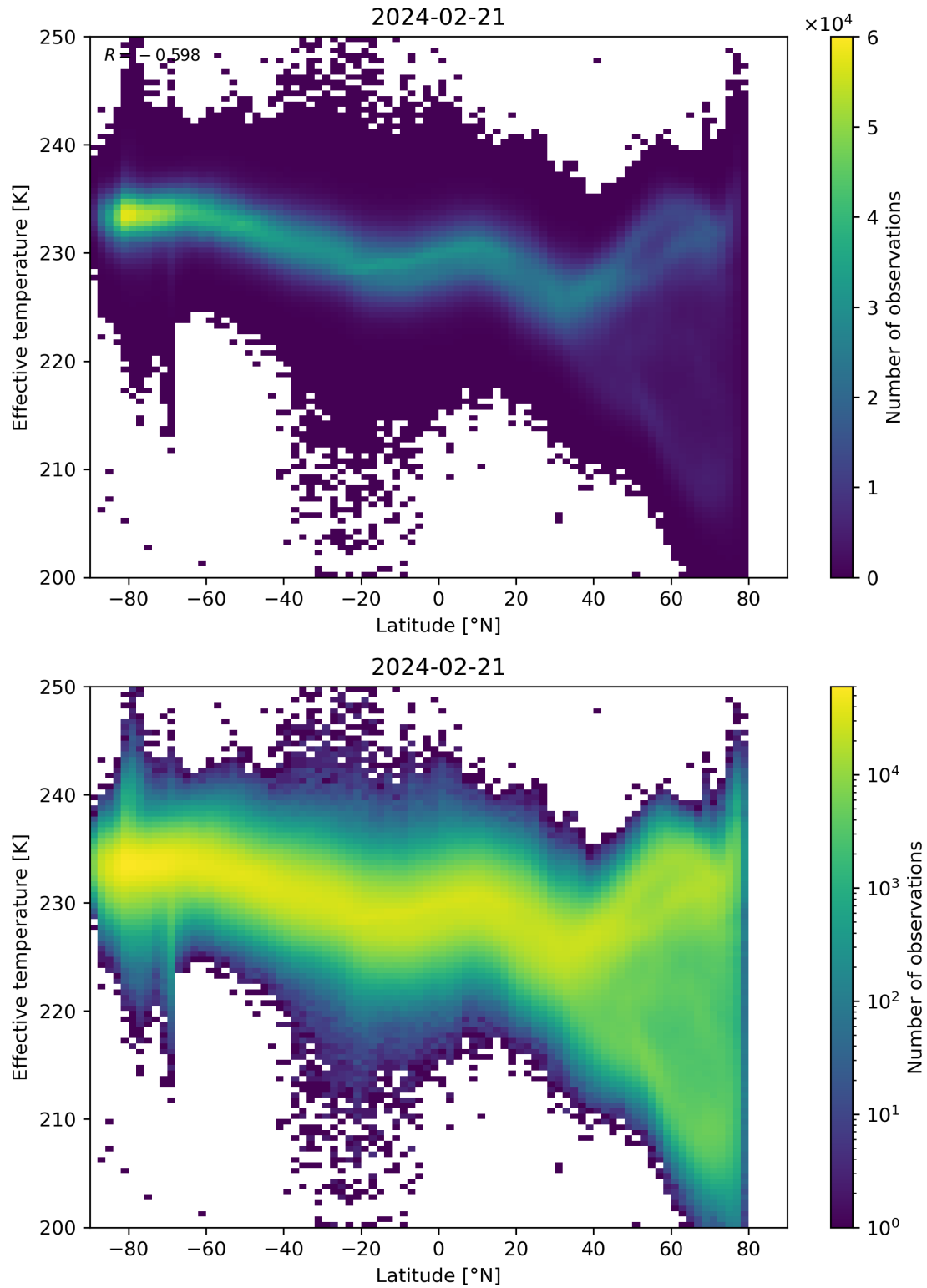
Figure 34: Scatter density plot of “Latitude” against “Effective temperature” for 2024-02-20 to 2024-02-22.
