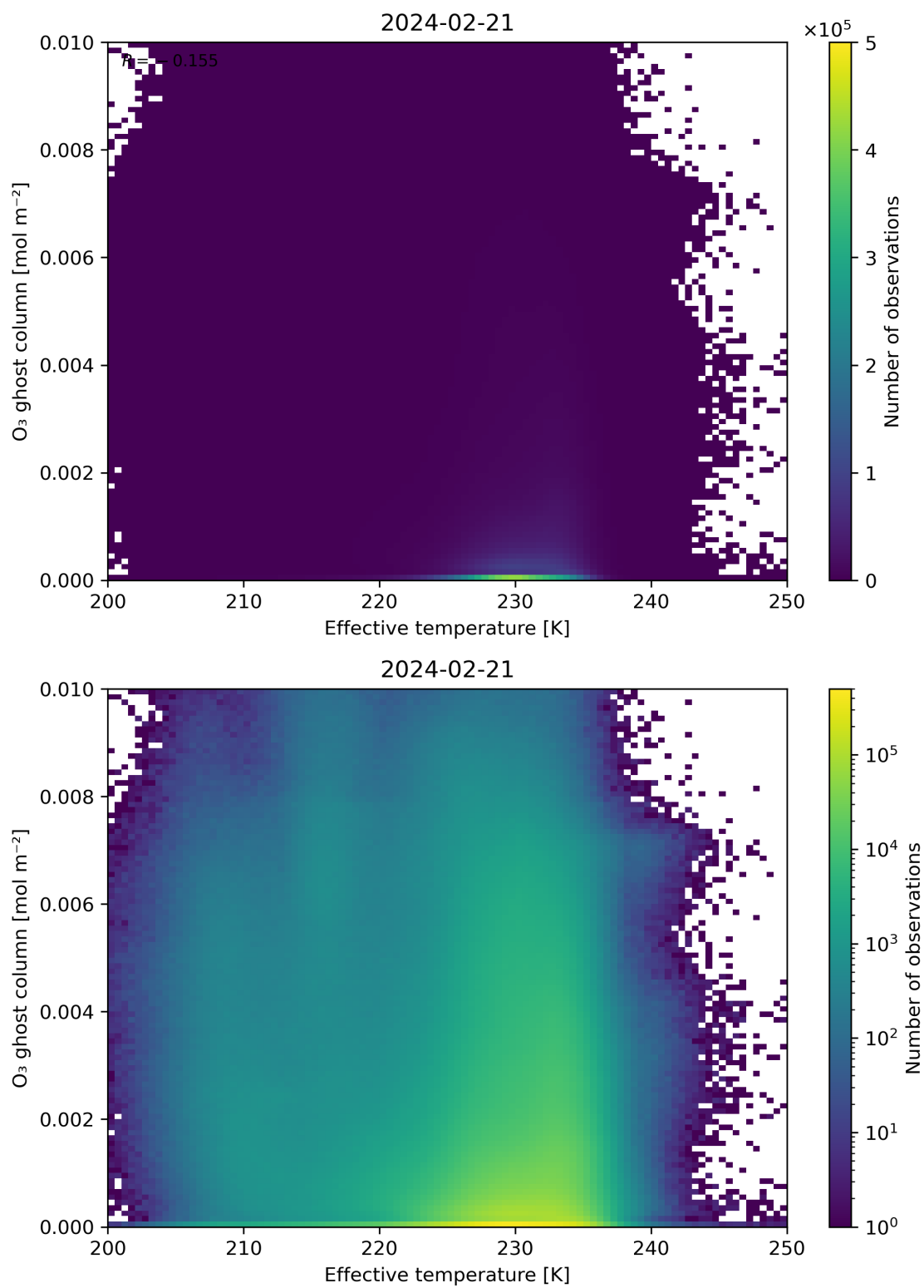
Figure 38: Scatter density plot of “Effective temperature” against “O 3 ghost column” for 2024-02-20 to 2024-02-22.
