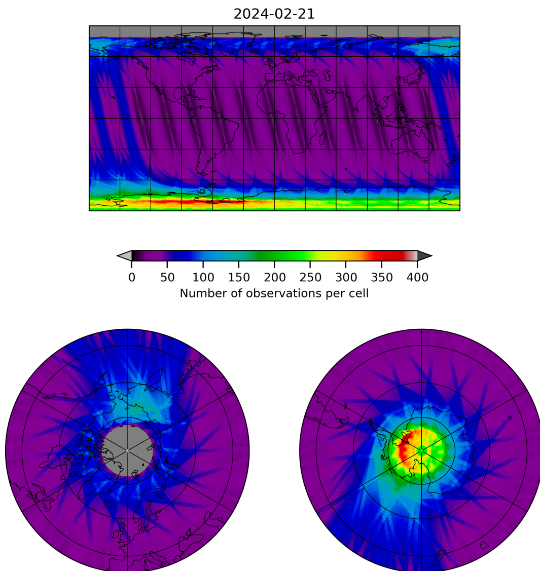
Figure 12: Map of the number of observations for 2024-02-20 to 2024-02-22
