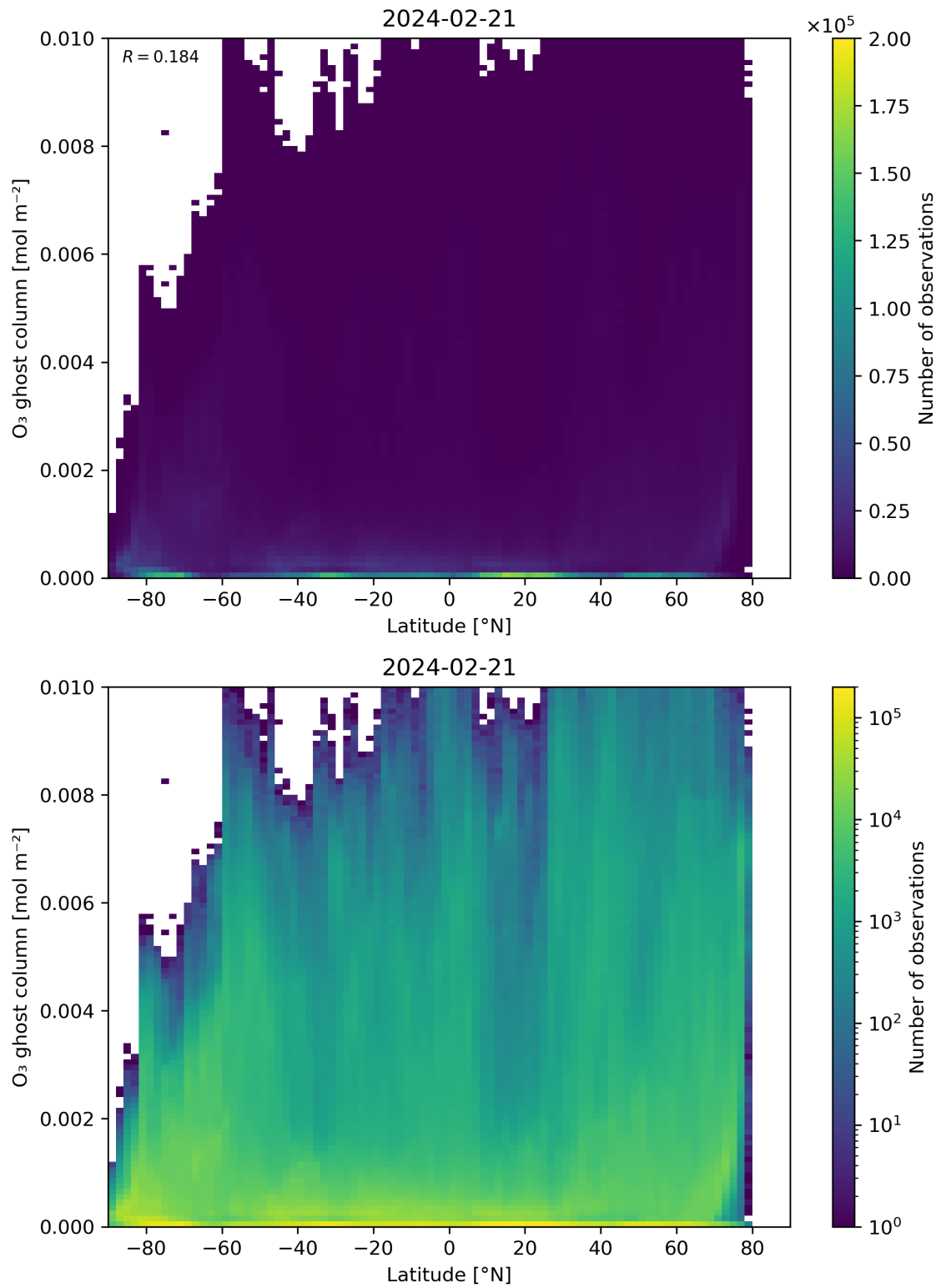
Figure 35: Scatter density plot of “Latitude” against “O 3 ghost column” for 2024-02-20 to 2024-02-22.
