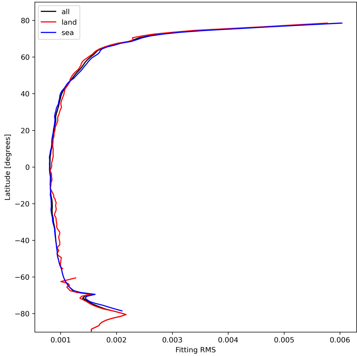
Figure 16: Zonal average of “Fitting RMS” for 2024-02-20 to 2024-02-22.
