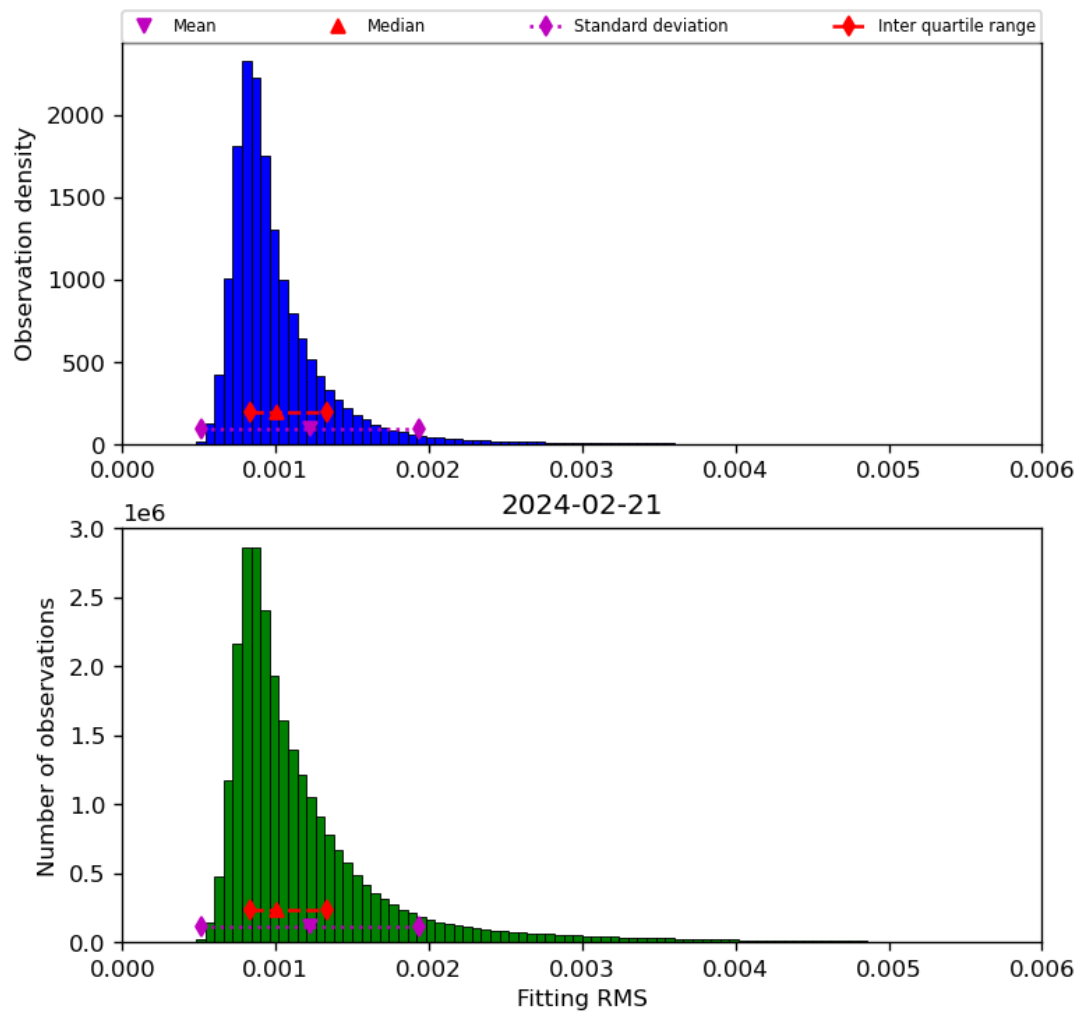
Figure 23: Histogram of “Fitting RMS” for 2024-02-20 to 2024-02-22
