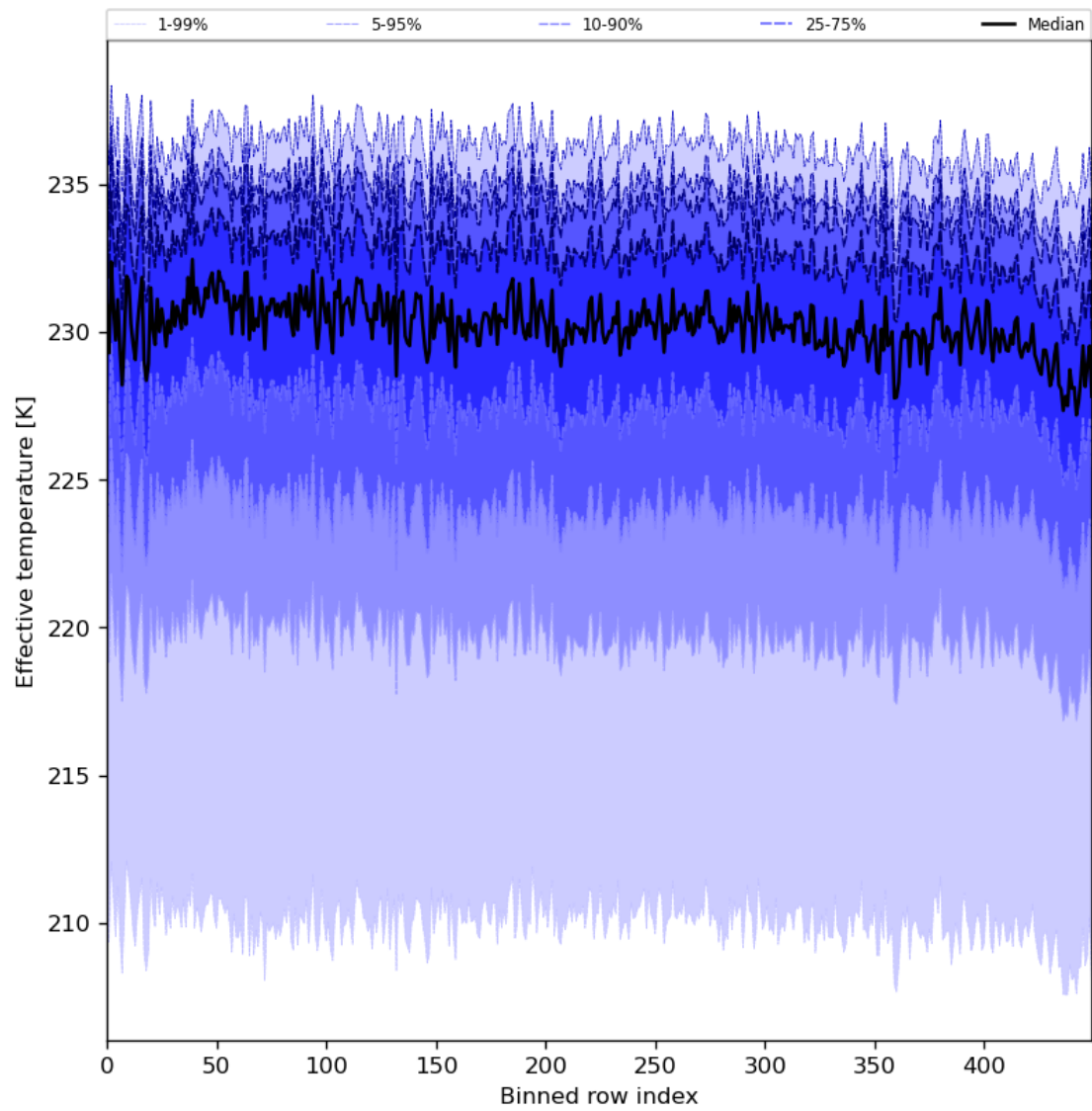
Figure 31: Along track statistics of “Effective temperature” for 2024-02-20 to 2024-02-22
