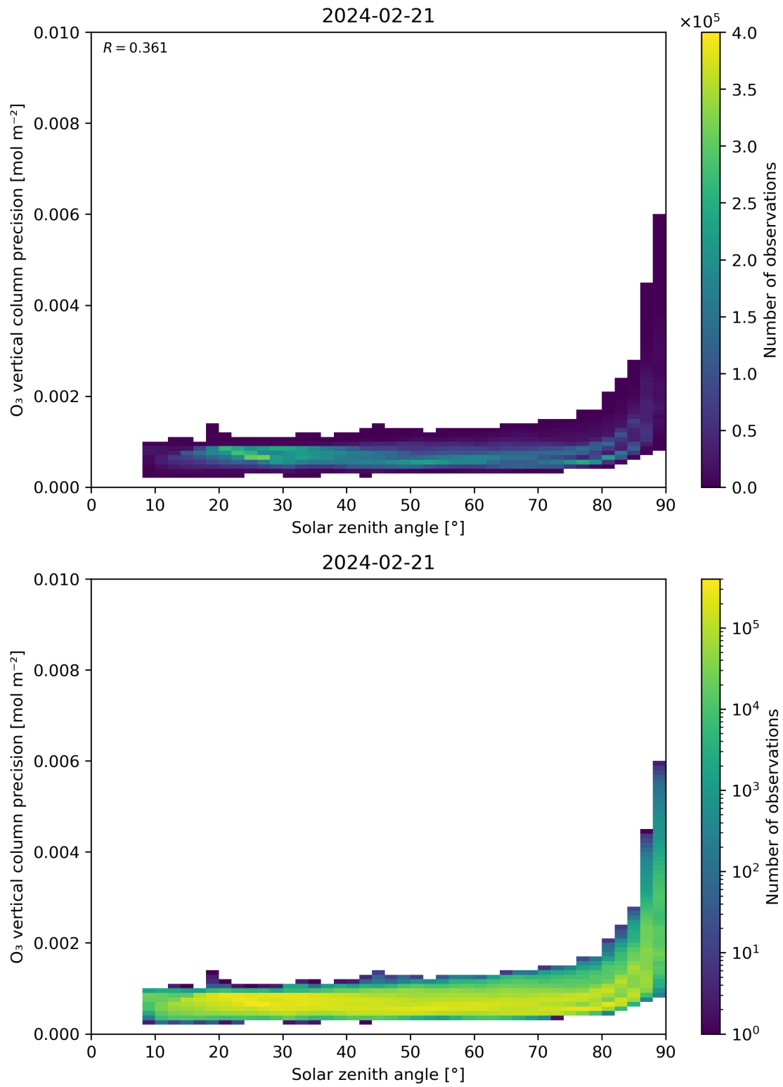
Figure 48: Scatter density plot of “Solar zenith angle” against “O 3 vertical column precision” for 2024-02-20 to 2024-02-22.
