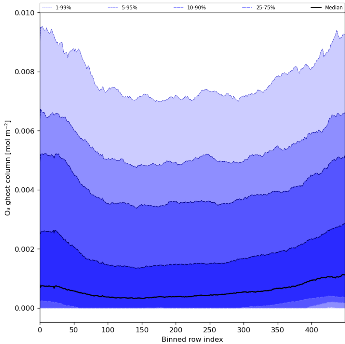
Figure 32: Along track statistics of “O 3 ghost column” for 2024-02-20 to 2024-02-22
