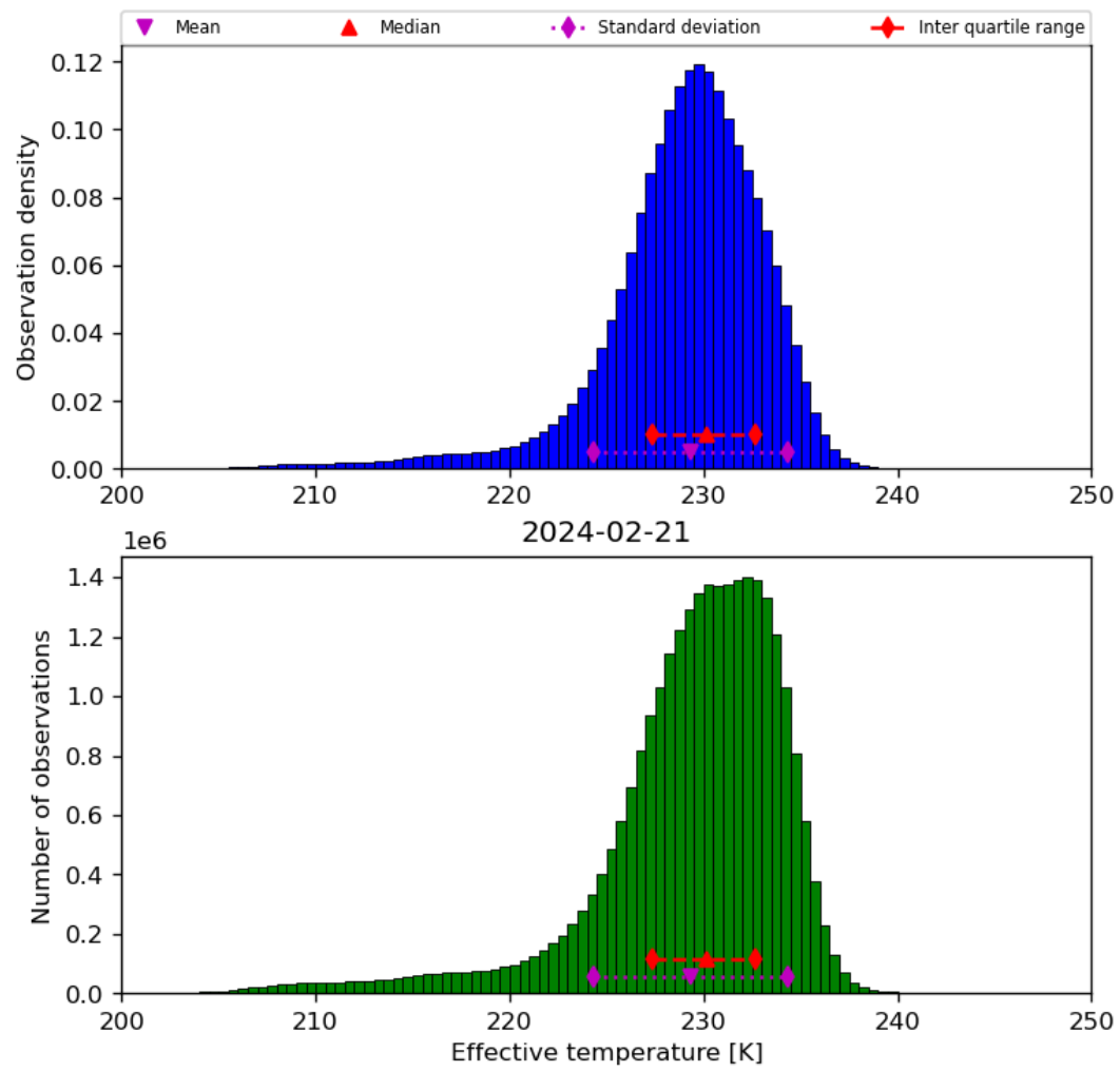
Figure 24: Histogram of “Effective temperature” for 2024-02-20 to 2024-02-22
