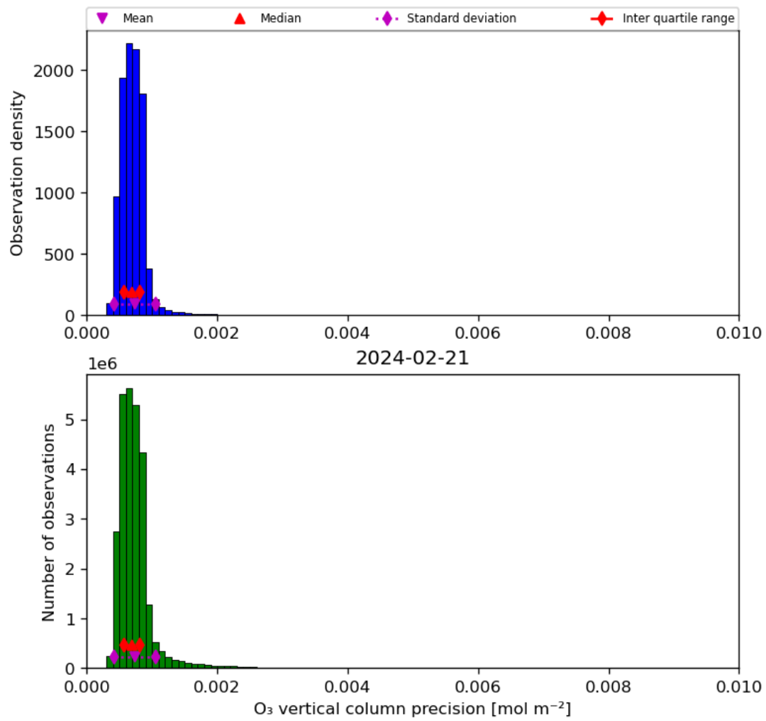
Figure 22: Histogram of “O 3 vertical column precision” for 2024-02-20 to 2024-02-22
