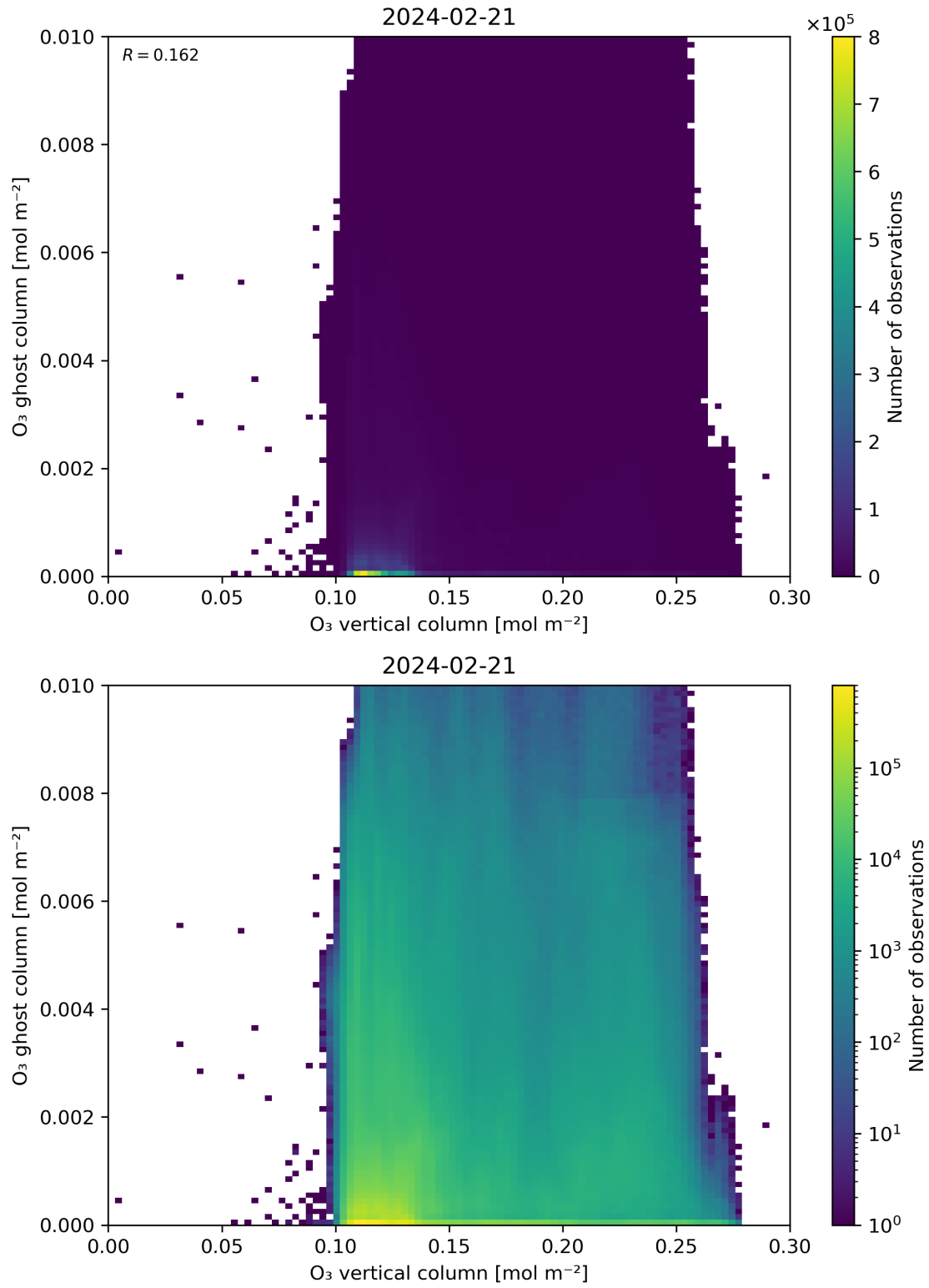
Figure 40: Scatter density plot of “O 3 vertical column” against “O 3 ghost column” for 2024-02-20 to 2024-02-22.
