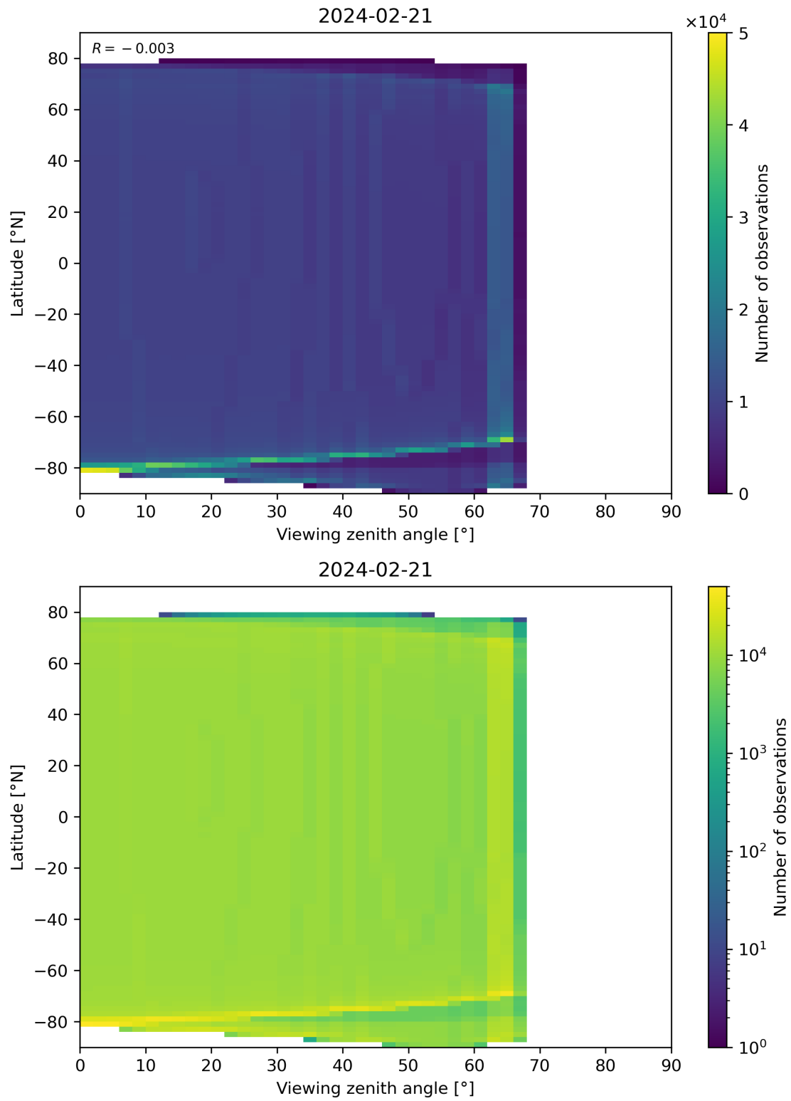
Figure 49: Scatter density plot of “Viewing zenith angle” against “Latitude” for 2024-02-20 to 2024-02-22.
