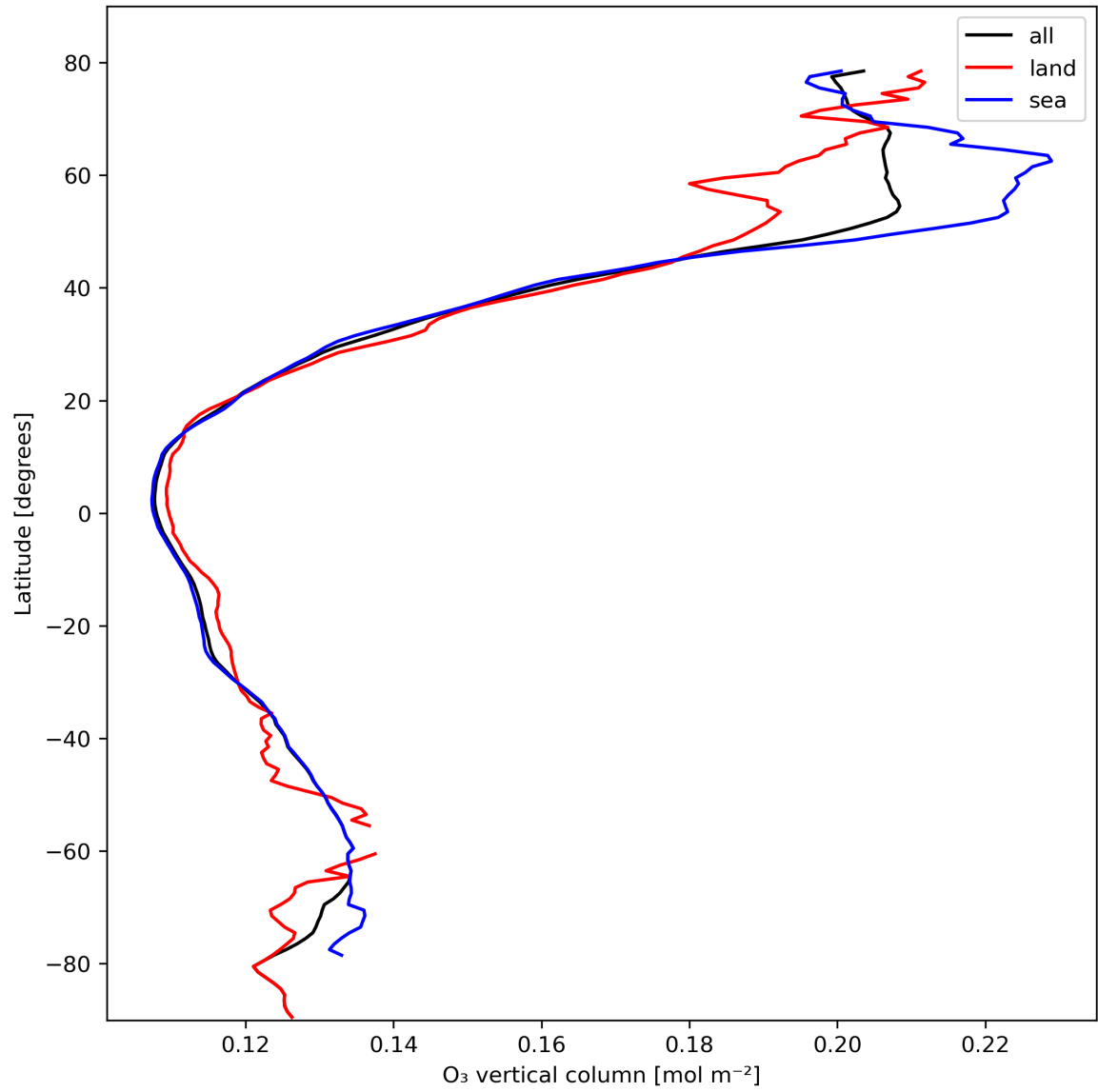
Figure 14: Zonal average of “O 3 vertical column” for 2024-02-20 to 2024-02-22.
