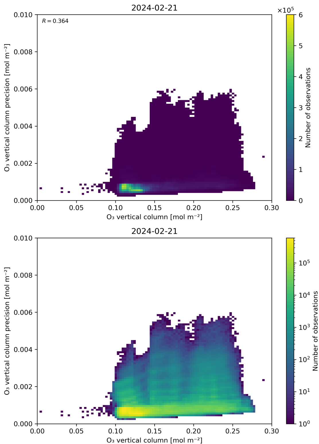
Figure 41: Scatter density plot of “O 3 vertical column” against “O 3 vertical column precision” for 2024-02-20 to 2024-02-22.
