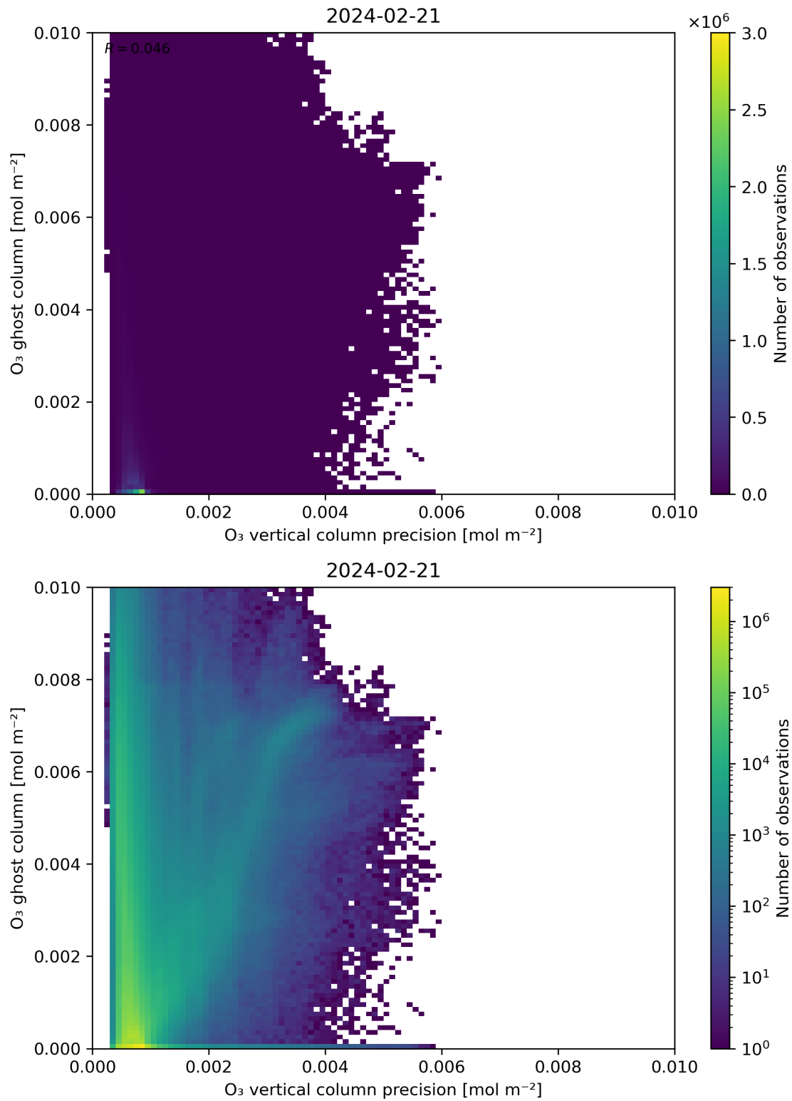
Figure 43: Scatter density plot of “ \text{O}_3 vertical column precision” against “ \text{O}_3 ghost column” for 2024-02-20 to 2024-02-22.
