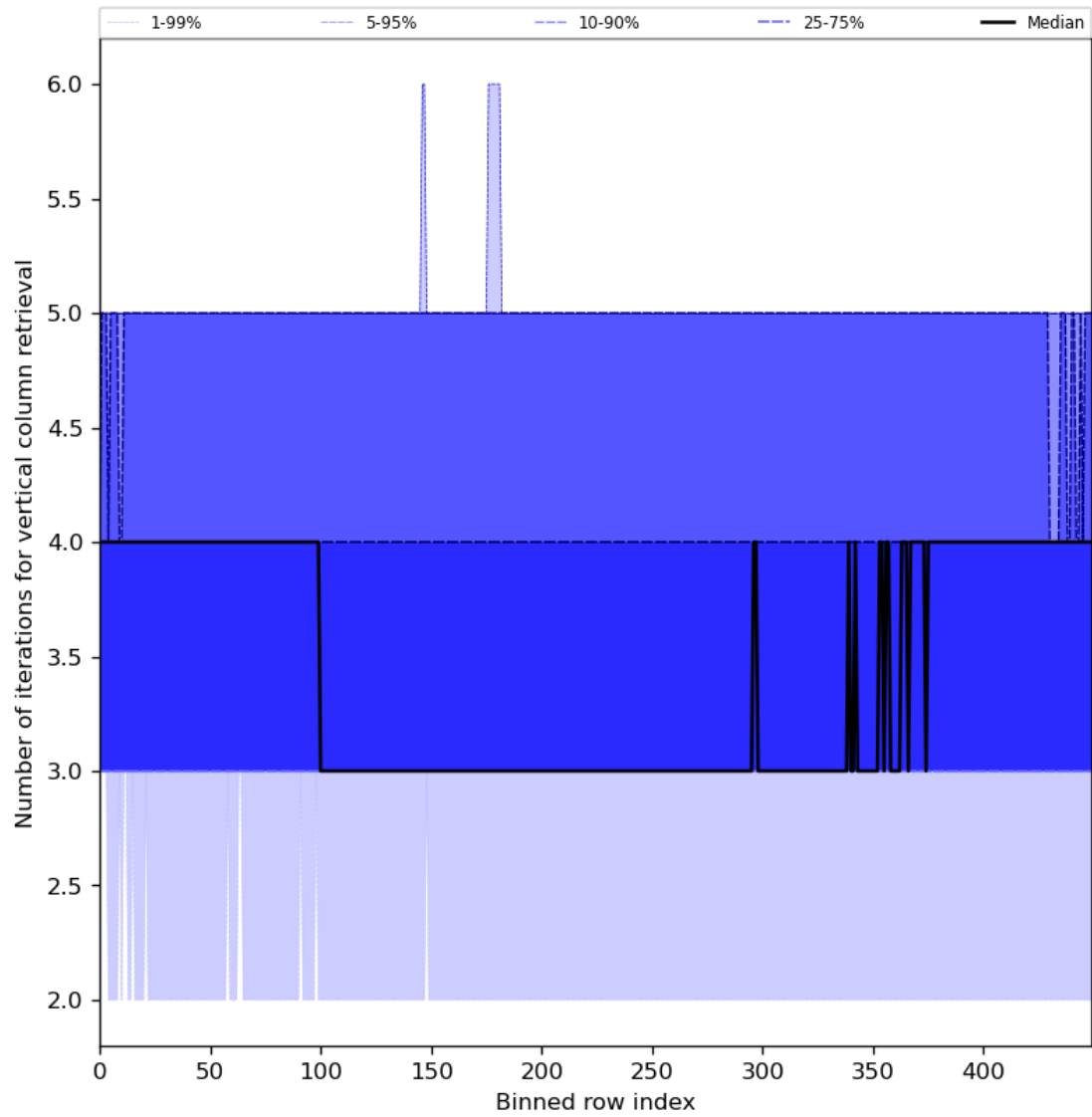
Figure 33: Along track statistics of “Number of iterations for vertical column retrieval” for 2024-02-20 to 2024-02-22
