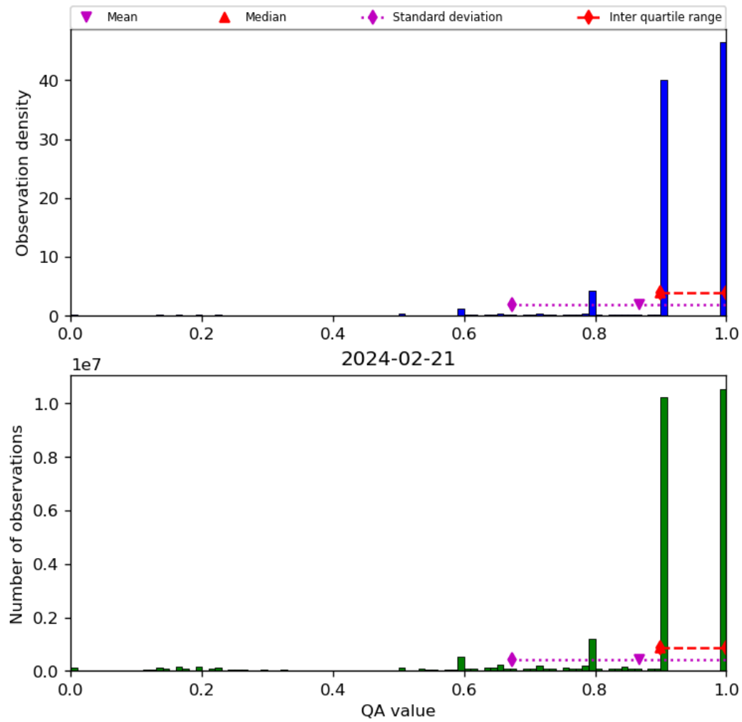
Figure 20: Histogram of “QA value” for 2024-02-20 to 2024-02-22
