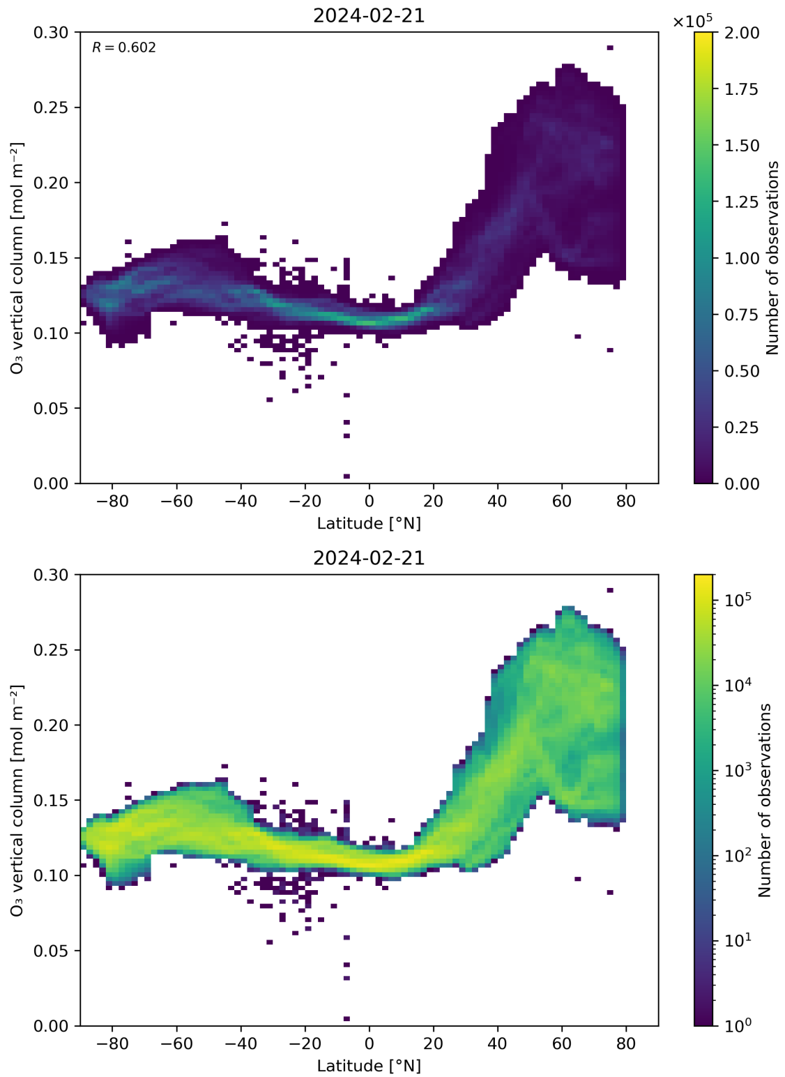
Figure 36: Scatter density plot of “Latitude” against “O 3 vertical column” for 2024-02-20 to 2024-02-22.
