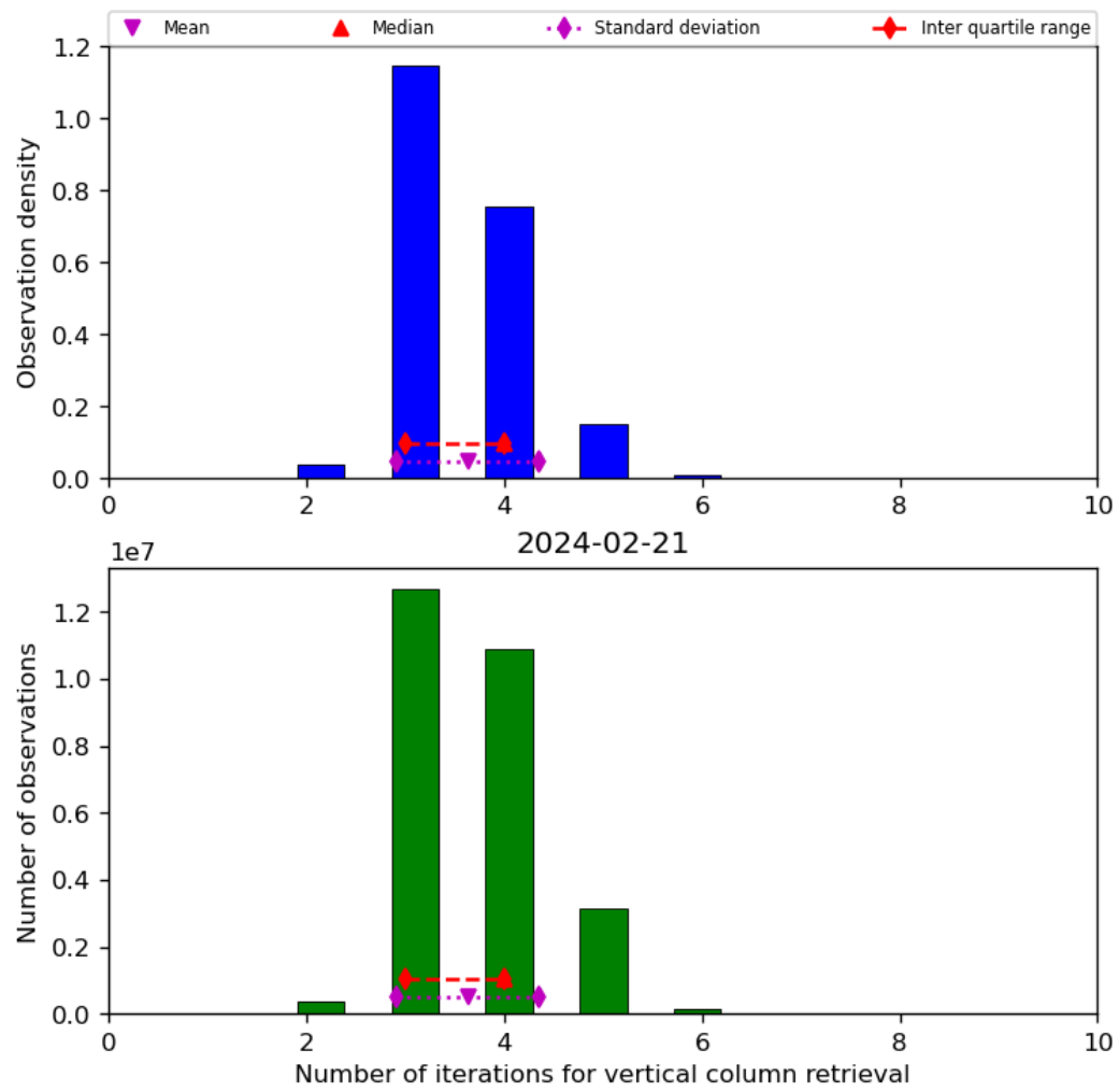
Figure 26: Histogram of "Number of iterations for vertical column retrieval" for 2024-02-20 to 2024-02-22
