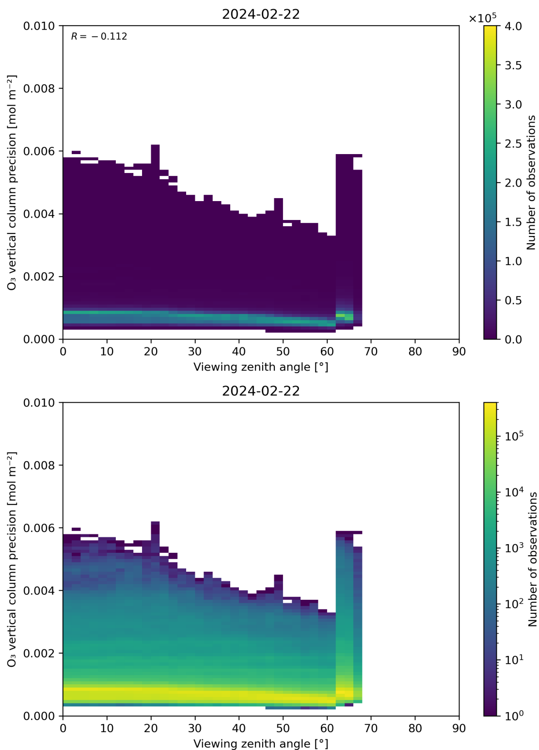
Figure 53: Scatter density plot of “Viewing zenith angle” against “O 3 vertical column precision” for 2024-02-22 to 2024-02-23.
