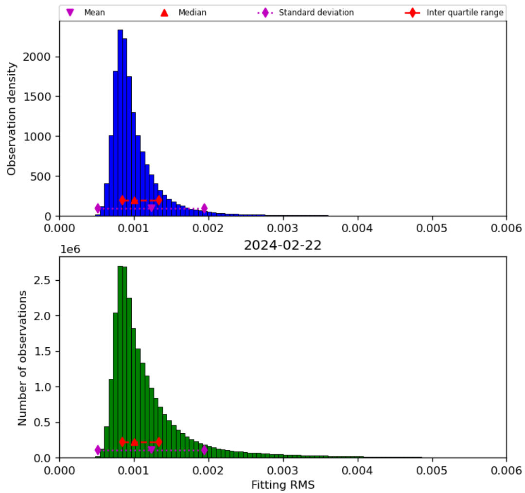
Figure 23: Histogram of “Fitting RMS” for 2024-02-22 to 2024-02-23
