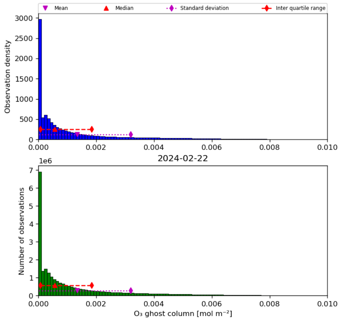
Figure 25: Histogram of “O 3 ghost column” for 2024-02-22 to 2024-02-23
