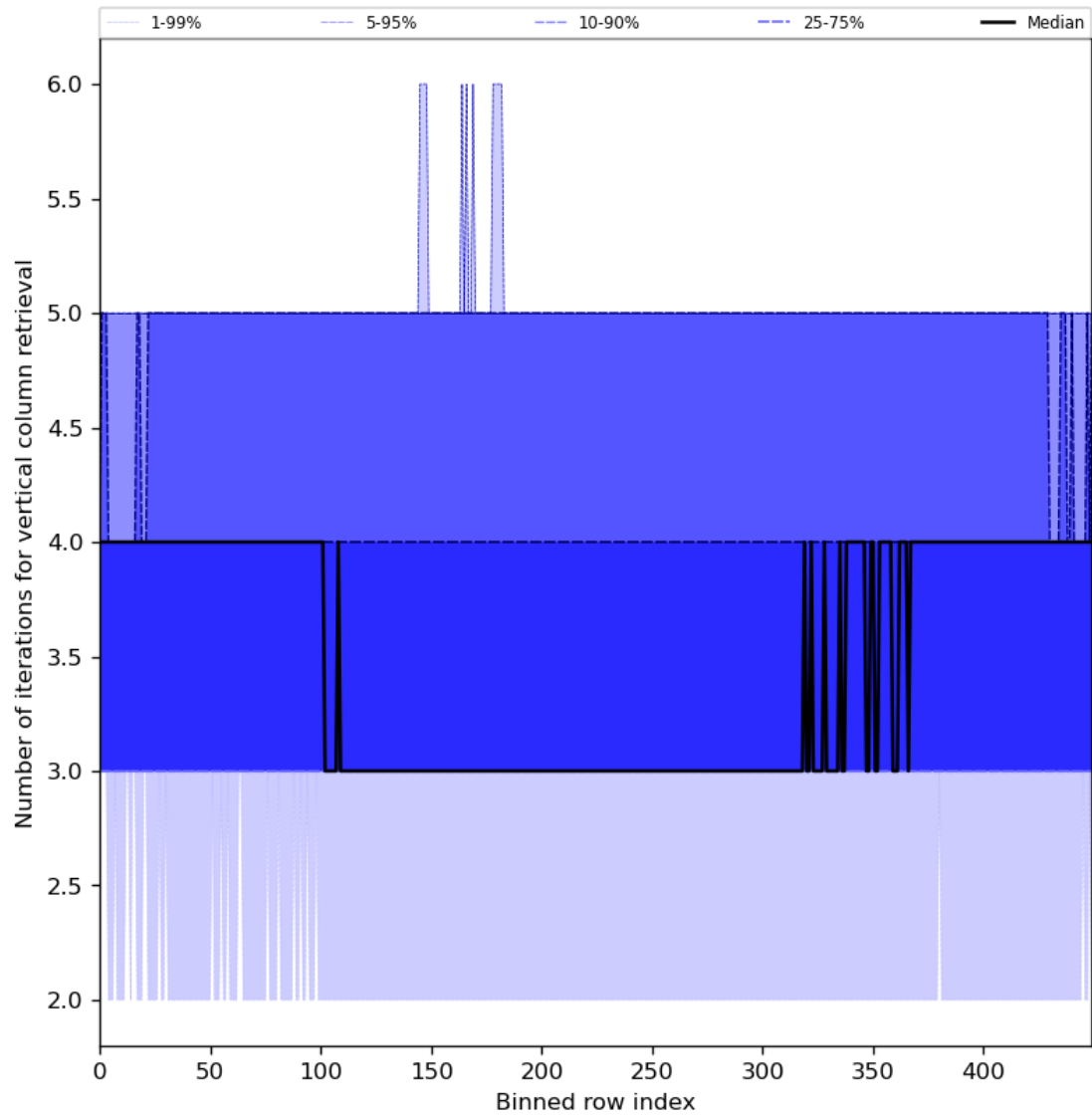
Figure 33: Along track statistics of “Number of iterations for vertical column retrieval” for 2024-02-22 to 2024-02-23
