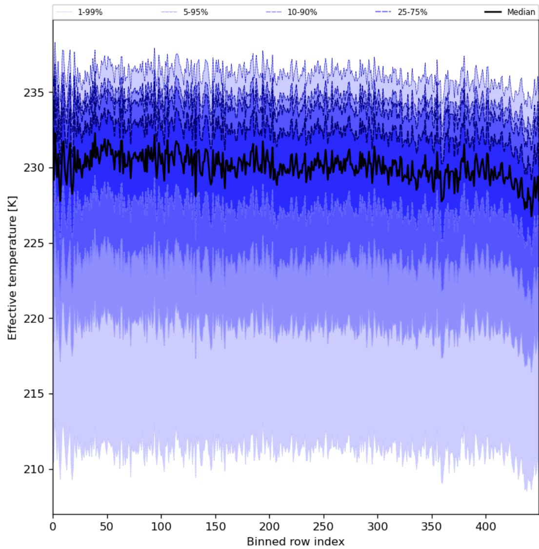
Figure 31: Along track statistics of “Effective temperature” for 2024-02-22 to 2024-02-23
