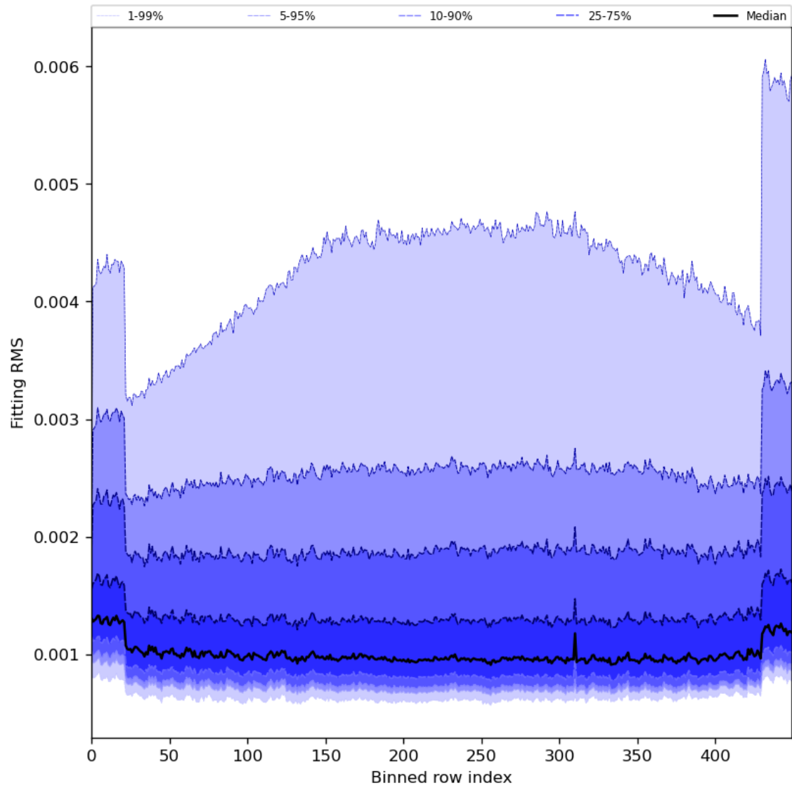
Figure 30: Along track statistics of “Fitting RMS” for 2024-02-22 to 2024-02-23
