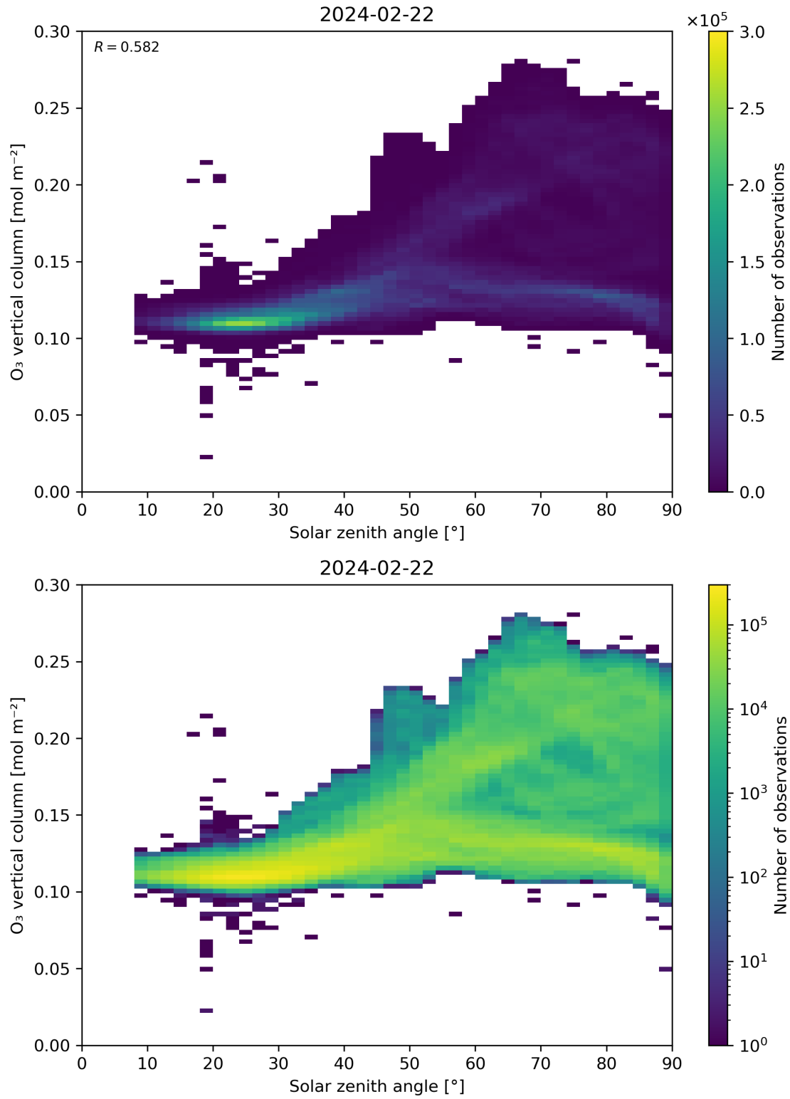
Figure 47: Scatter density plot of “Solar zenith angle” against “O 3 vertical column” for 2024-02-22 to 2024-02-23.
