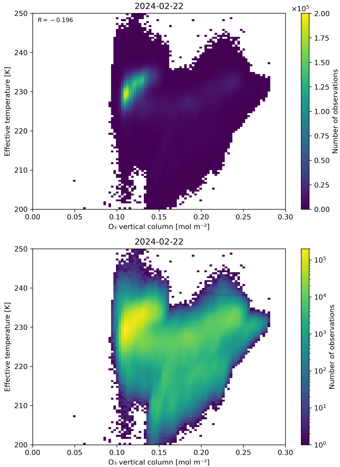
Figure 39: Scatter density plot of “O 3 vertical column” against “Effective temperature” for 2024-02-22 to 2024-02-23.
