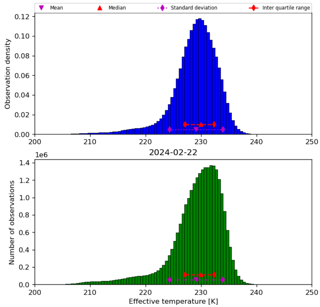
Figure 24: Histogram of “Effective temperature” for 2024-02-22 to 2024-02-23
