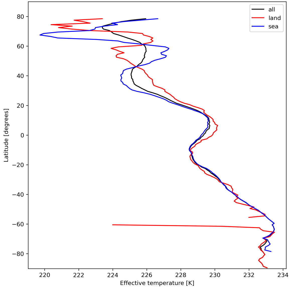
Figure 17: Zonal average of “Effective temperature” for 2024-02-22 to 2024-02-23.
