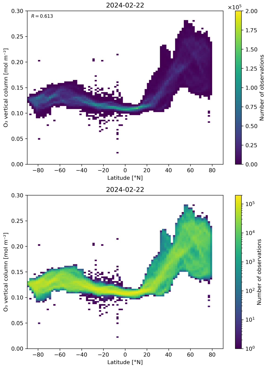
Figure 36: Scatter density plot of “Latitude” against “O 3 vertical column” for 2024-02-22 to 2024-02-23.
