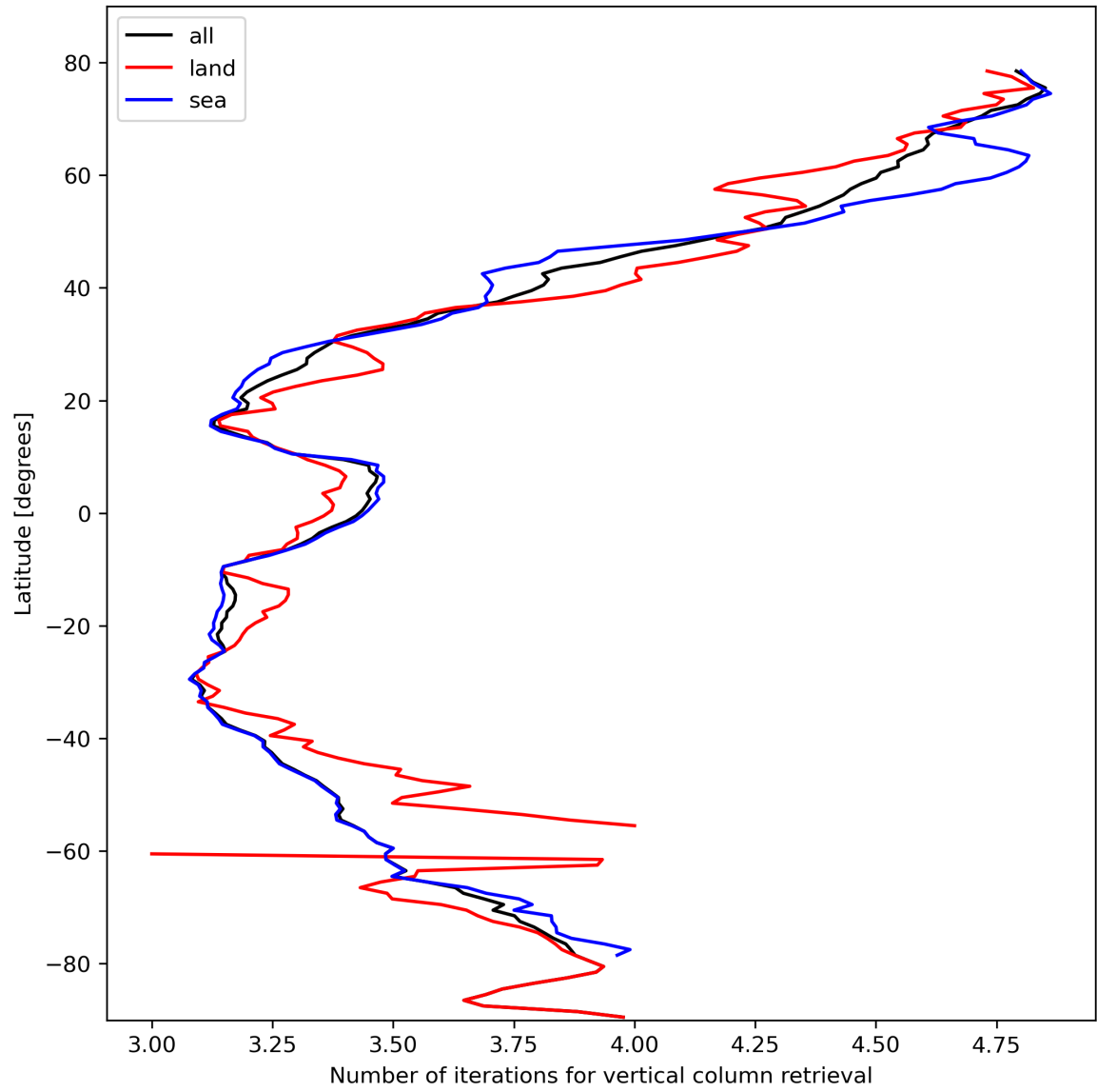
Figure 19: Zonal average of “Number of iterations for vertical column retrieval” for 2024-02-22 to 2024-02-23.
