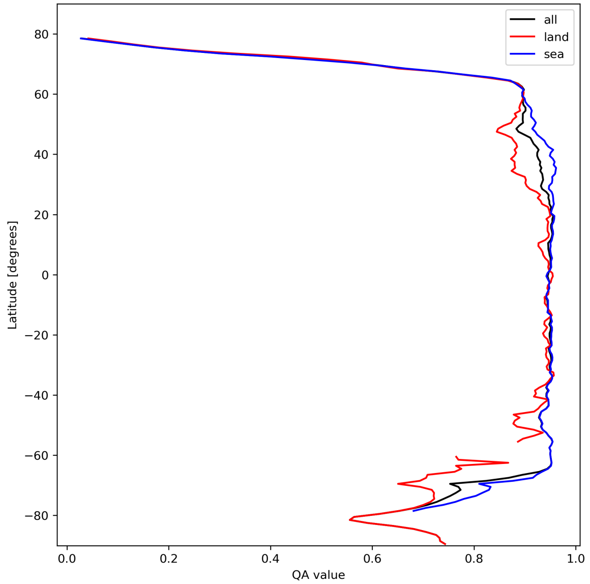
Figure 13: Zonal average of “QA value” for 2024-02-22 to 2024-02-23.
