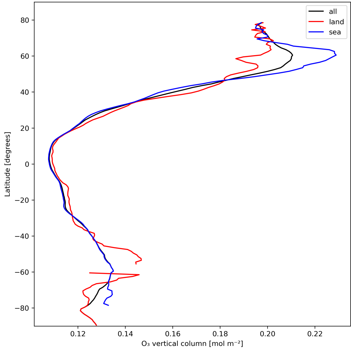
Figure 14: Zonal average of “O 3 vertical column” for 2024-02-22 to 2024-02-23.
