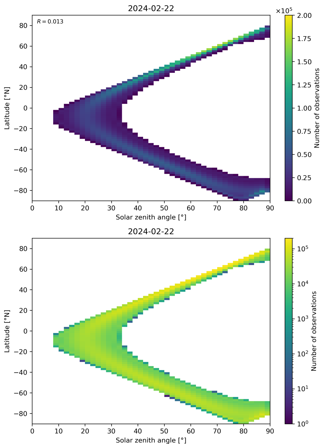
Figure 44: Scatter density plot of “Solar zenith angle” against “Latitude” for 2024-02-22 to 2024-02-23.
