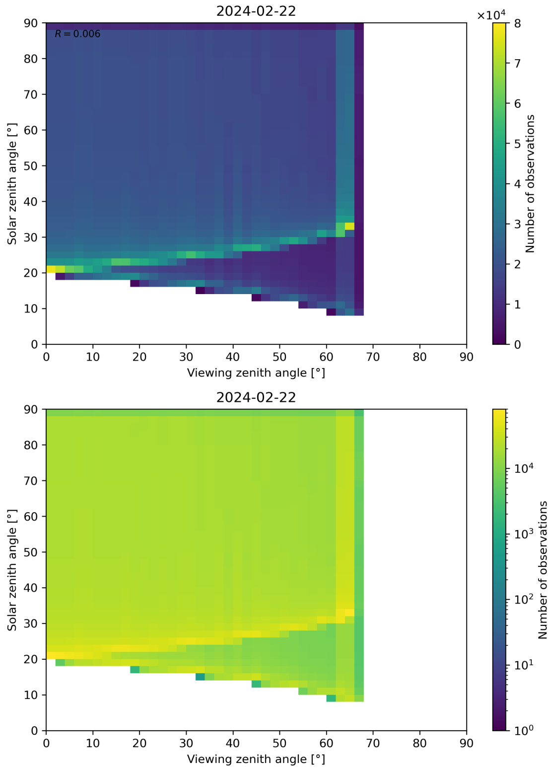
Figure 54: Scatter density plot of “Viewing zenith angle” against “Solar zenith angle” for 2024-02-22 to 2024-02-23.
