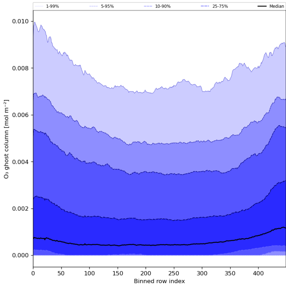
Figure 32: Along track statistics of “O 3 ghost column” for 2024-02-22 to 2024-02-23
