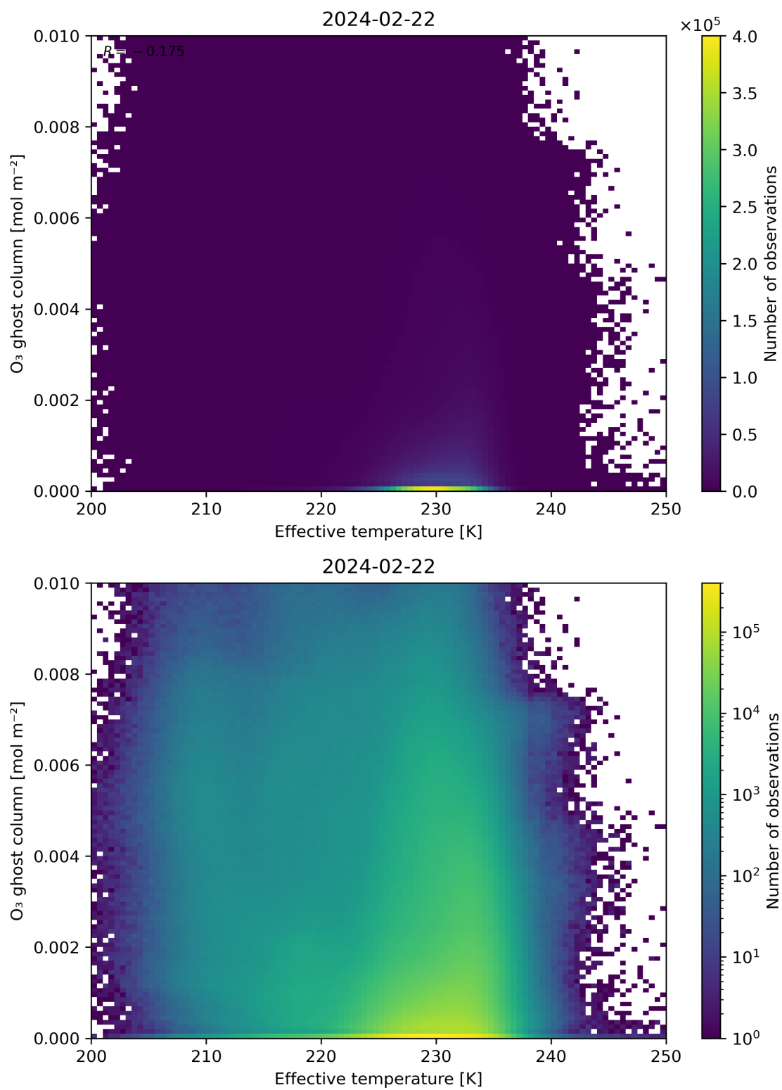
Figure 38: Scatter density plot of “Effective temperature” against “O 3 ghost column” for 2024-02-22 to 2024-02-23.
