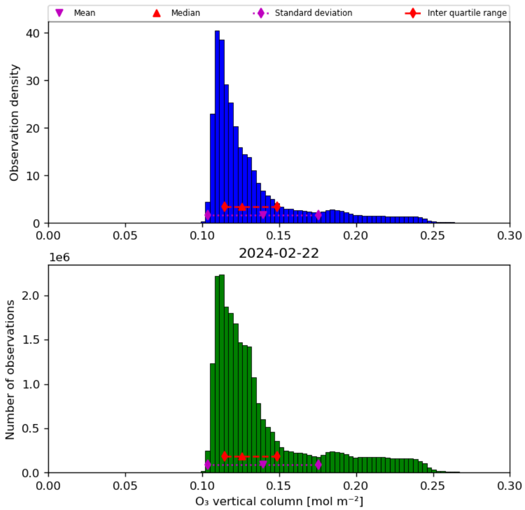
Figure 21: Histogram of “O 3 vertical column” for 2024-02-22 to 2024-02-23
