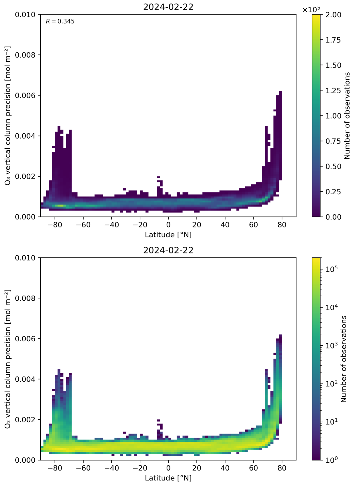
Figure 37: Scatter density plot of “Latitude” against “O 3 vertical column precision” for 2024-02-22 to 2024-02-23.
