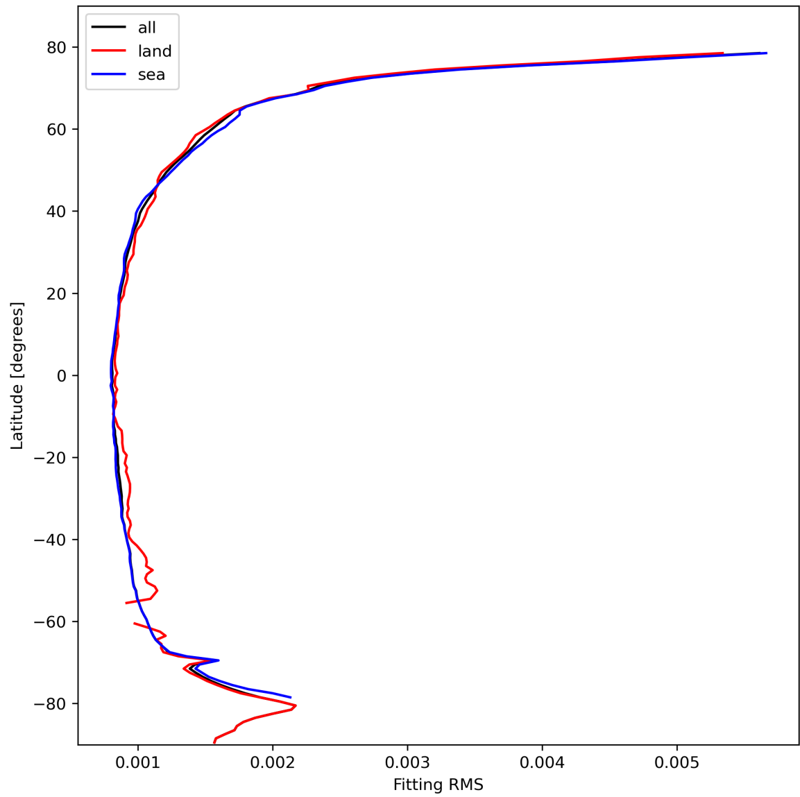
Figure 16: Zonal average of “Fitting RMS” for 2024-02-22 to 2024-02-23.
