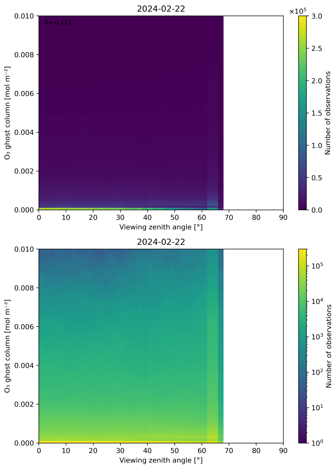
Figure 51: Scatter density plot of “Viewing zenith angle” against “O 3 ghost column” for 2024-02-22 to 2024-02-23.
