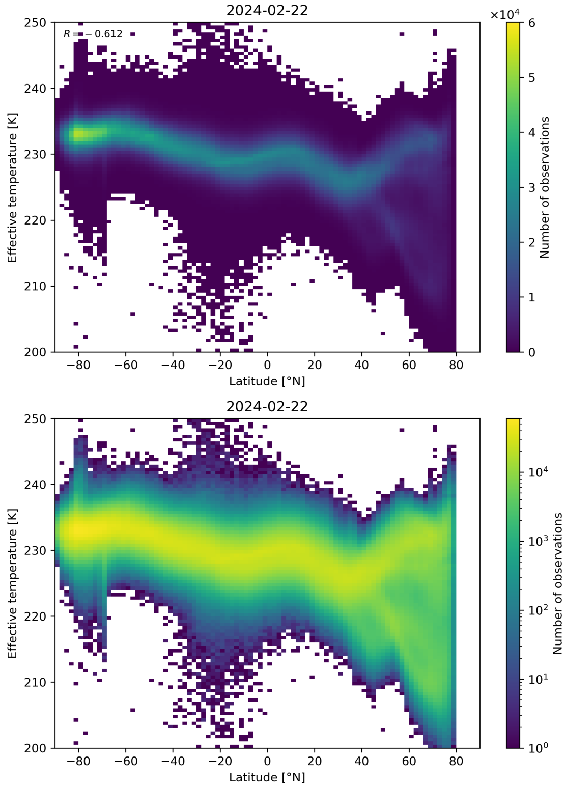
Figure 34: Scatter density plot of “Latitude” against “Effective temperature” for 2024-02-22 to 2024-02-23.
