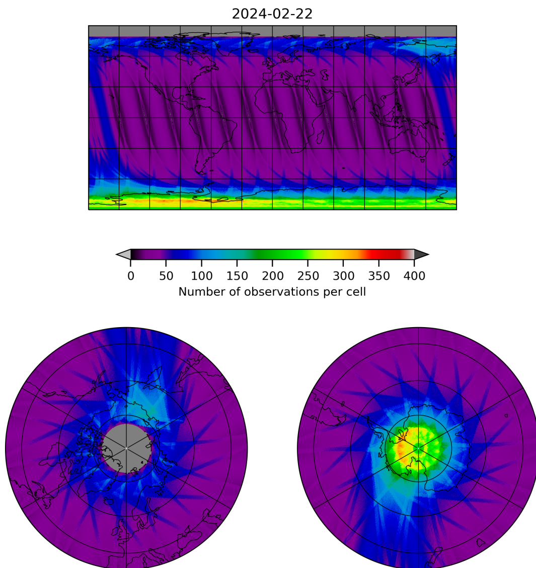
Figure 12: Map of the number of observations for 2024-02-22 to 2024-02-23
