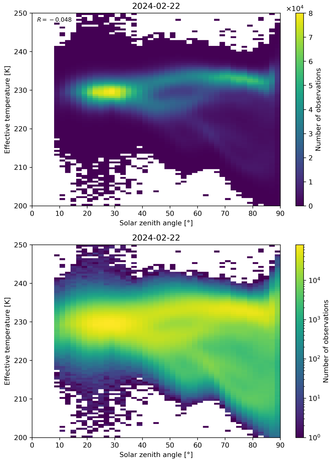
Figure 45: Scatter density plot of “Solar zenith angle” against “Effective temperature” for 2024-02-22 to 2024-02-23.
