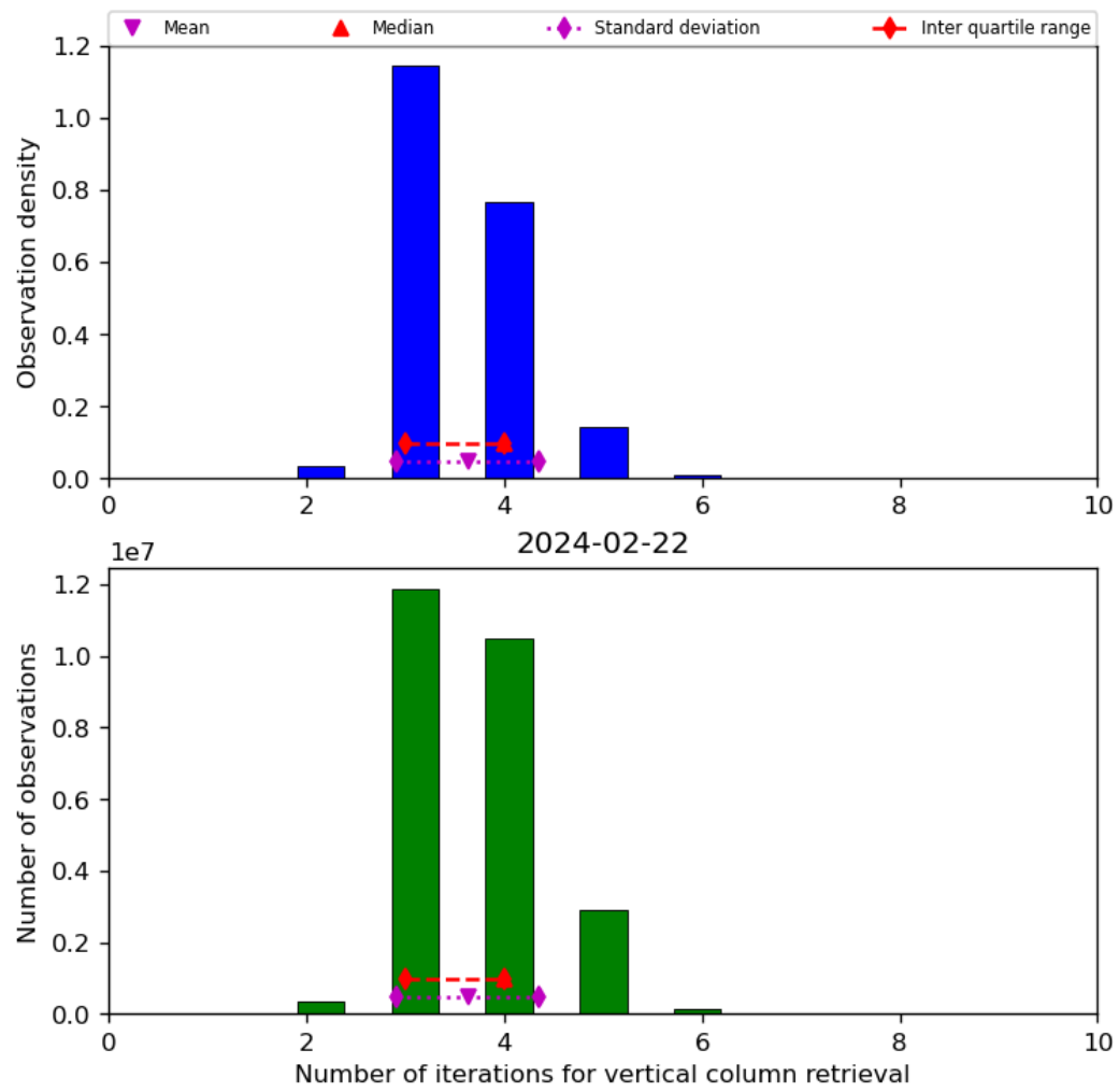
Figure 26: Histogram of “Number of iterations for vertical column retrieval” for 2024-02-22 to 2024-02-23
