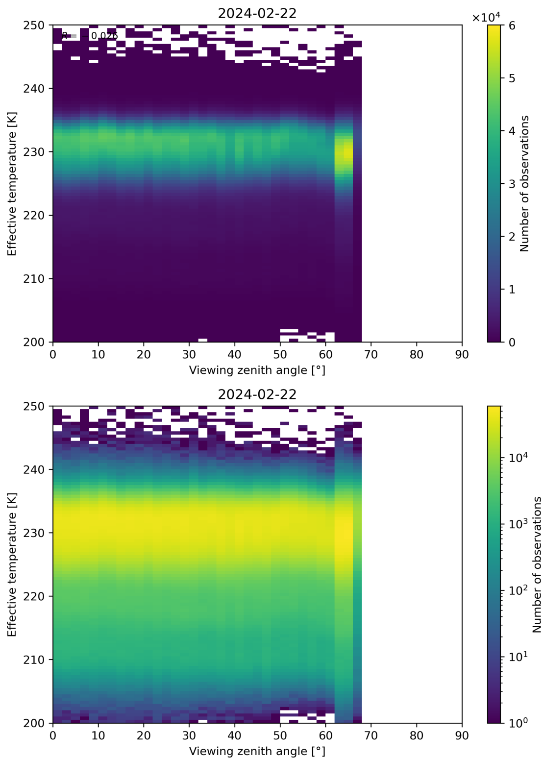
Figure 50: Scatter density plot of “Viewing zenith angle” against “Effective temperature” for 2024-02-22 to 2024-02-23.
