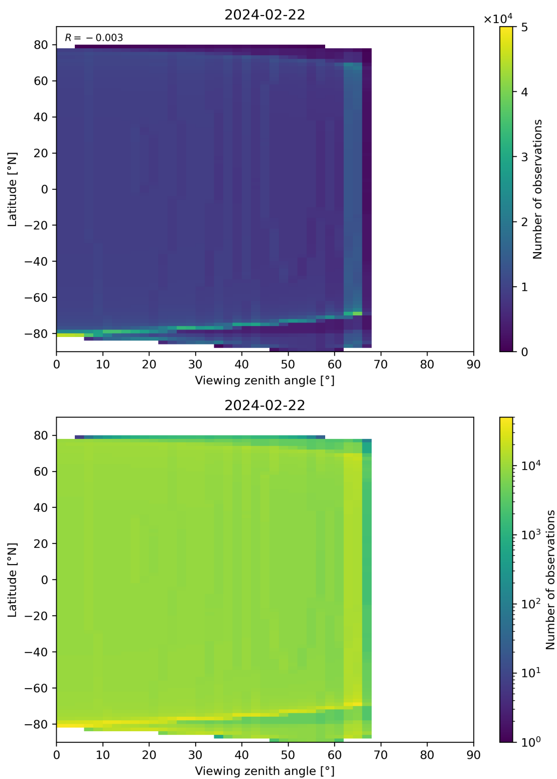
Figure 49: Scatter density plot of “Viewing zenith angle” against “Latitude” for 2024-02-22 to 2024-02-23.
