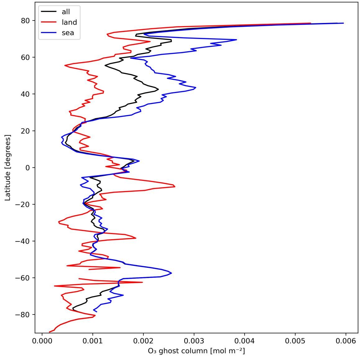
Figure 18: Zonal average of “O 3 ghost column” for 2024-02-22 to 2024-02-23.
