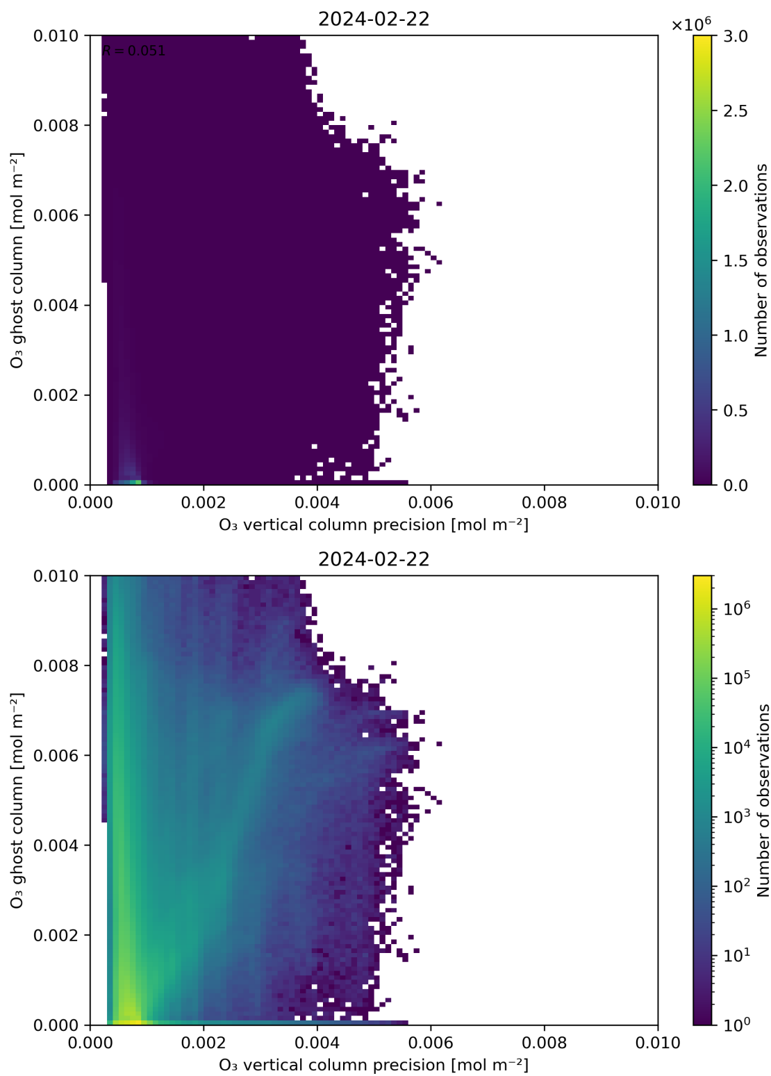
Figure 43: Scatter density plot of “ O_3 vertical column precision” against “ O_3 ghost column” for 2024-02-22 to 2024-02-23.
