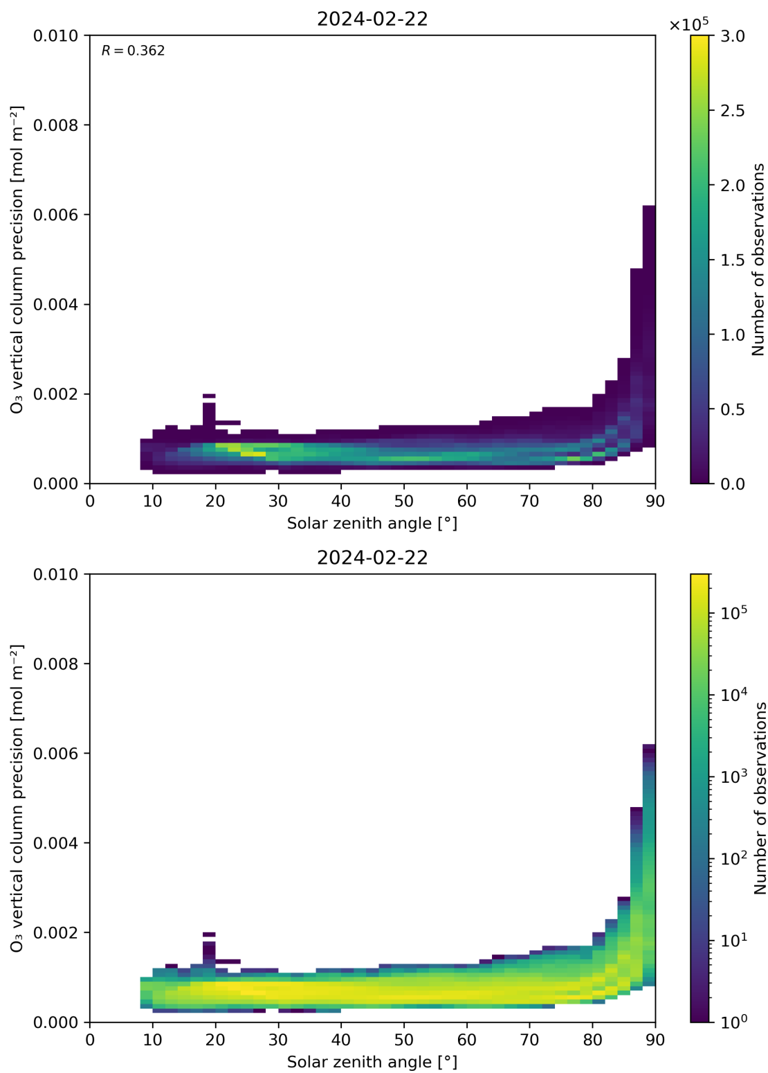
Figure 48: Scatter density plot of “Solar zenith angle” against “O 3 vertical column precision” for 2024-02-22 to 2024-02-23.
