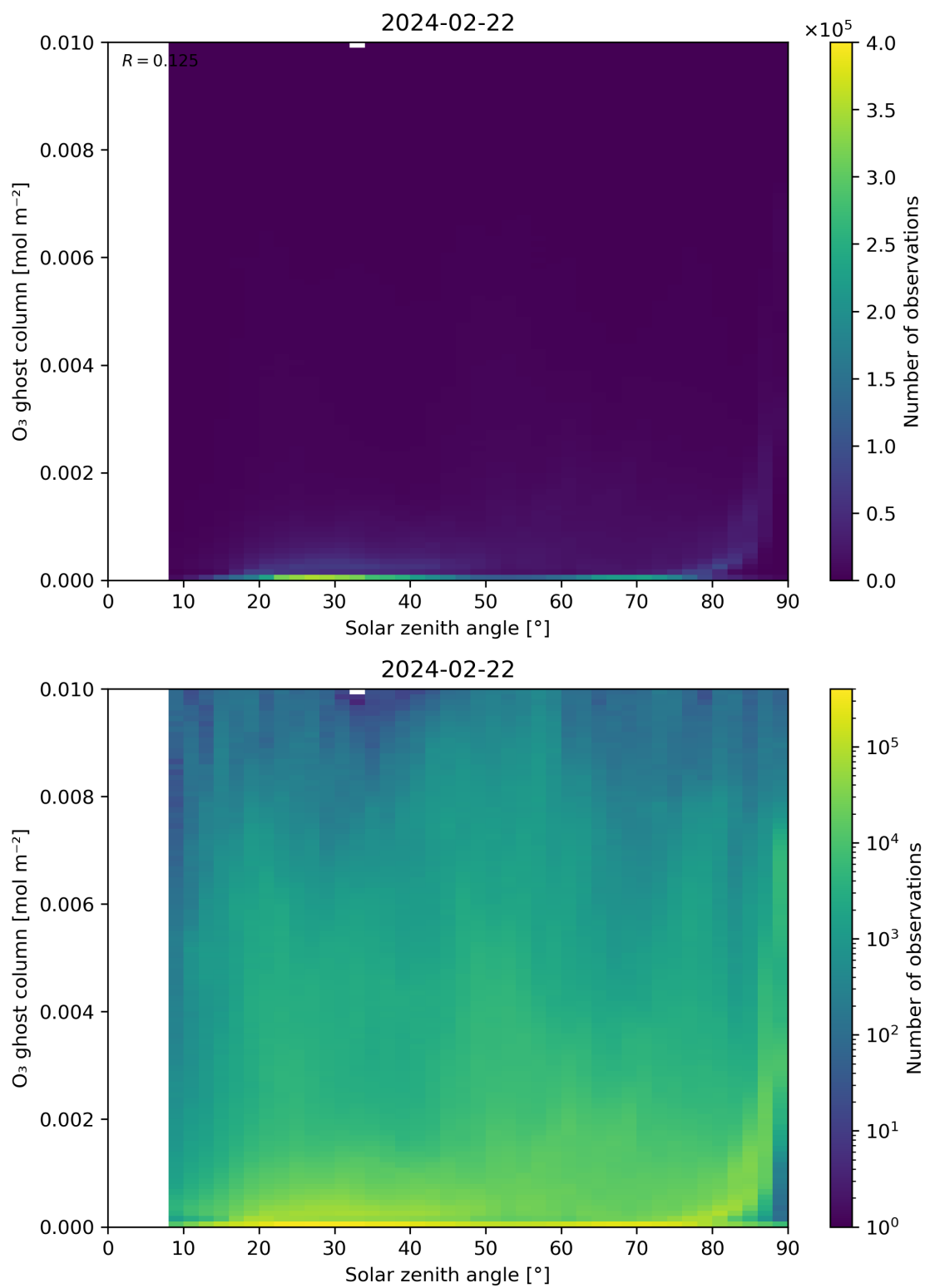
Figure 46: Scatter density plot of “Solar zenith angle” against “O 3 ghost column” for 2024-02-22 to 2024-02-23.
