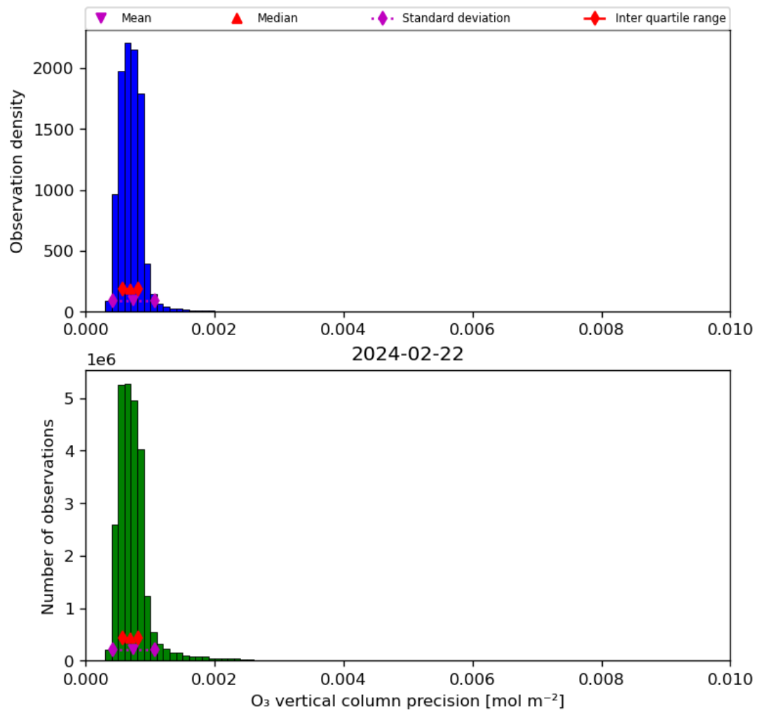
Figure 22: Histogram of “O 3 vertical column precision” for 2024-02-22 to 2024-02-23
