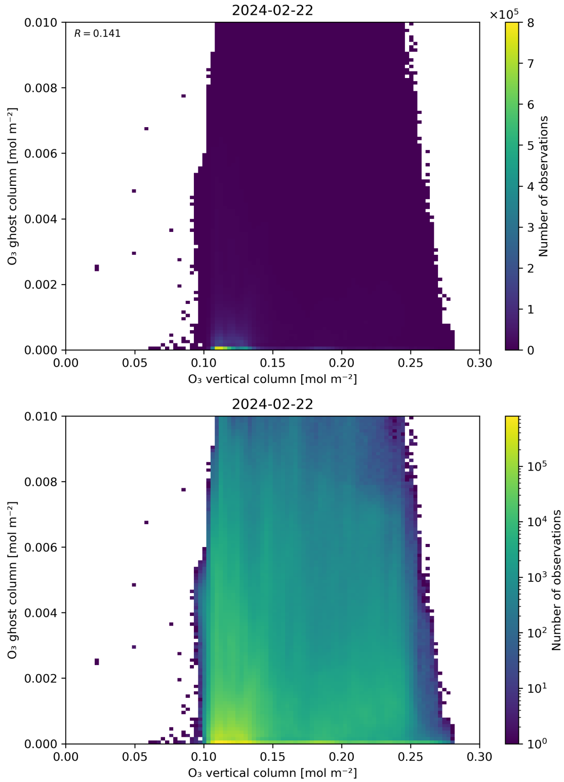
Figure 40: Scatter density plot of “O 3 vertical column” against “O 3 ghost column” for 2024-02-22 to 2024-02-23.
