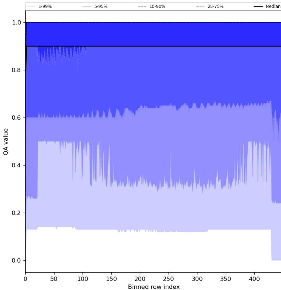
Figure 27: Along track statistics of “QA value” for 2024-02-22 to 2024-02-23
