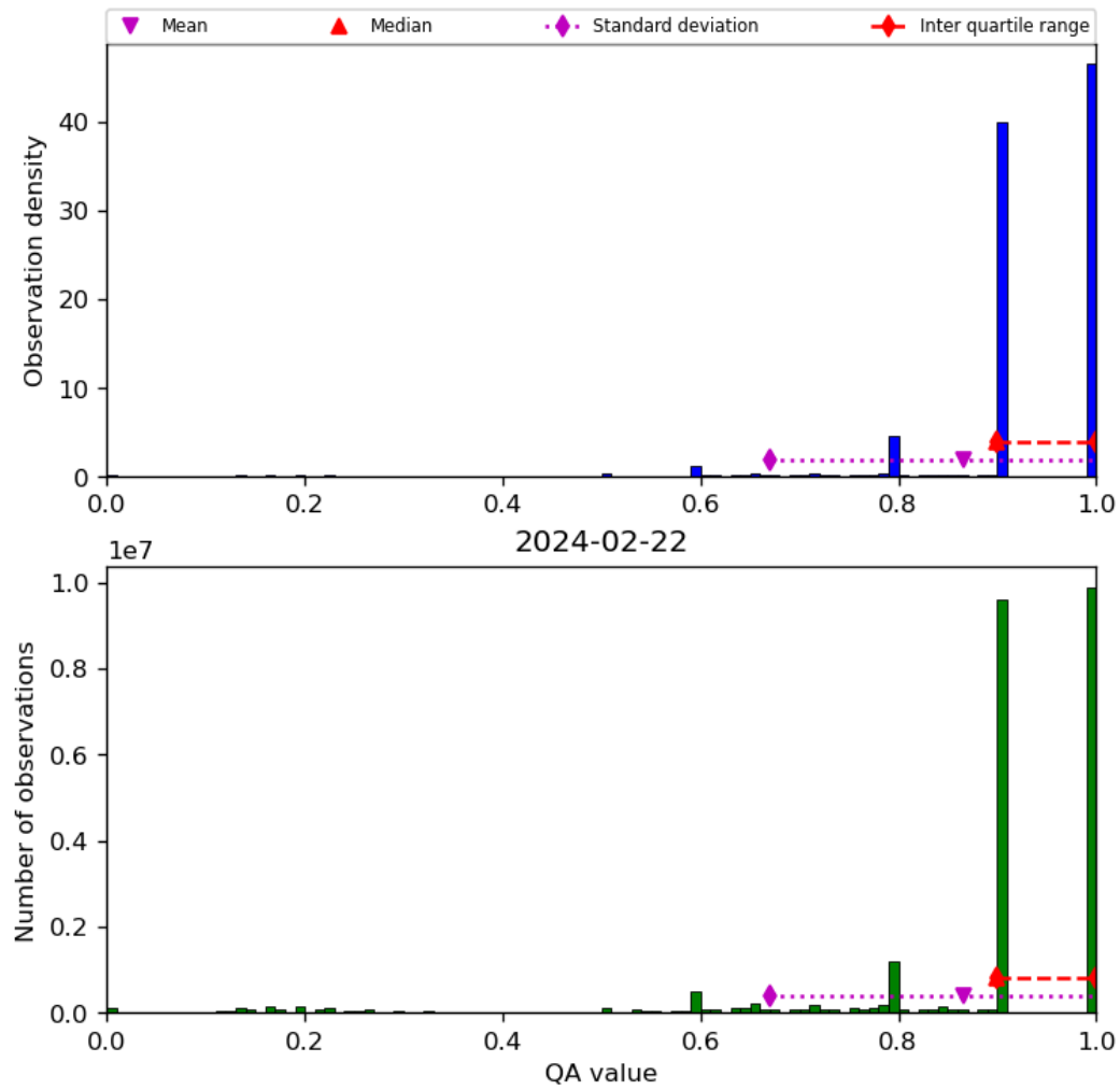
Figure 20: Histogram of “QA value” for 2024-02-22 to 2024-02-23
