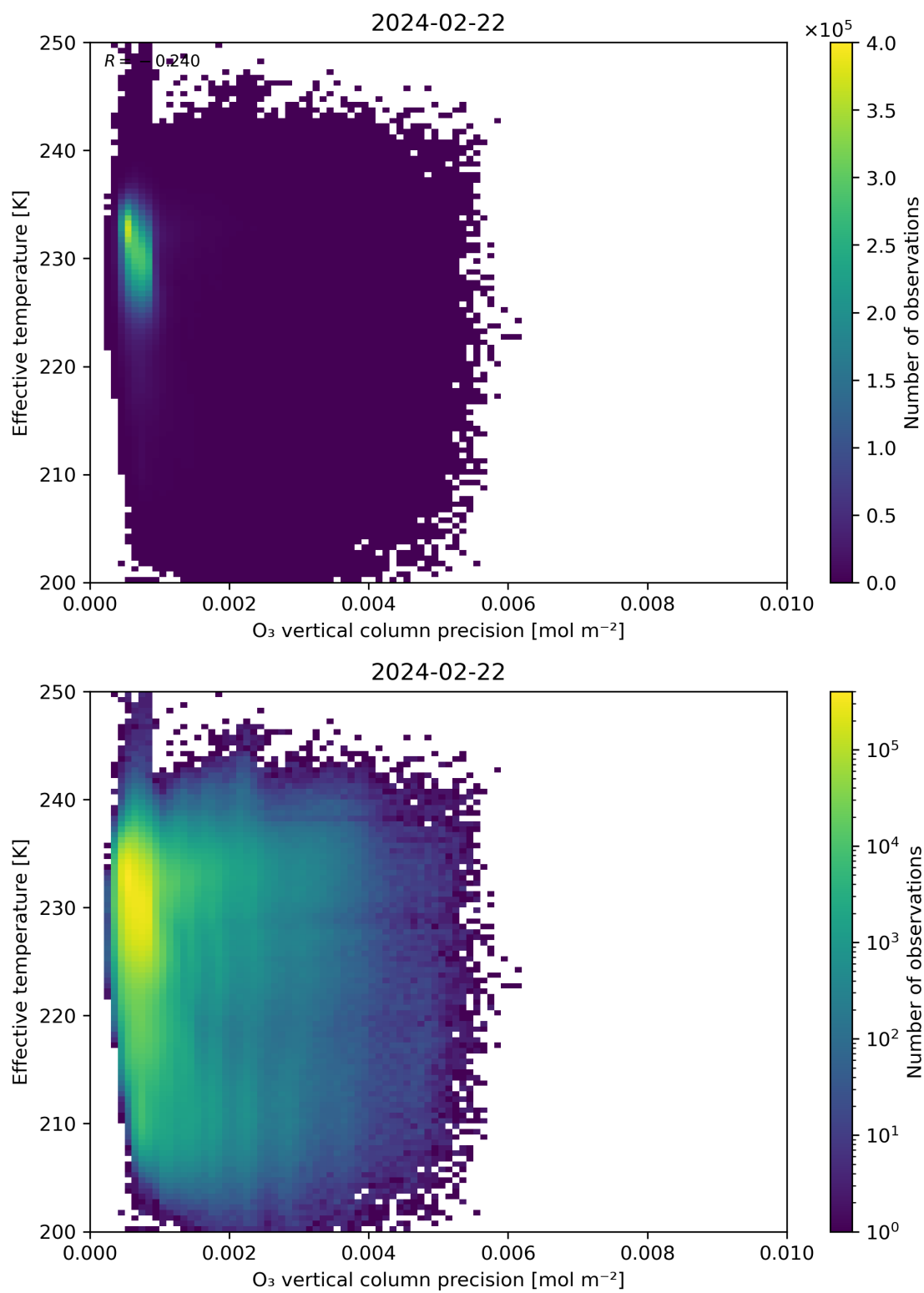
Figure 42: Scatter density plot of “ O_3 vertical column precision” against “Effective temperature” for 2024-02-22 to 2024-02-23.
