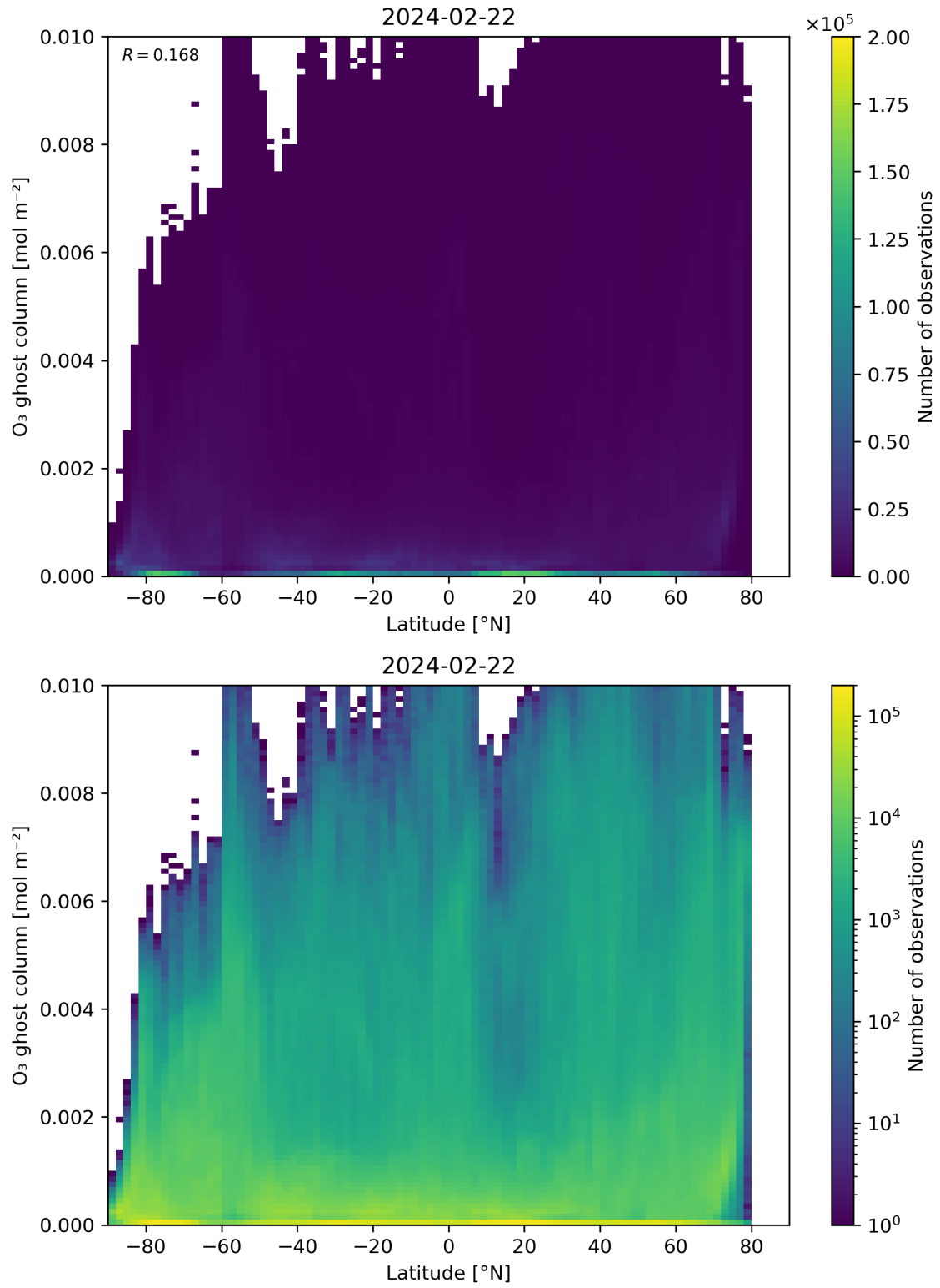
Figure 35: Scatter density plot of “Latitude” against “O 3 ghost column” for 2024-02-22 to 2024-02-23.
