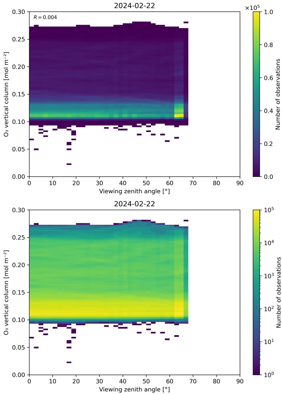
Figure 52: Scatter density plot of “Viewing zenith angle” against “O 3 vertical column” for 2024-02-22 to 2024-02-23.
