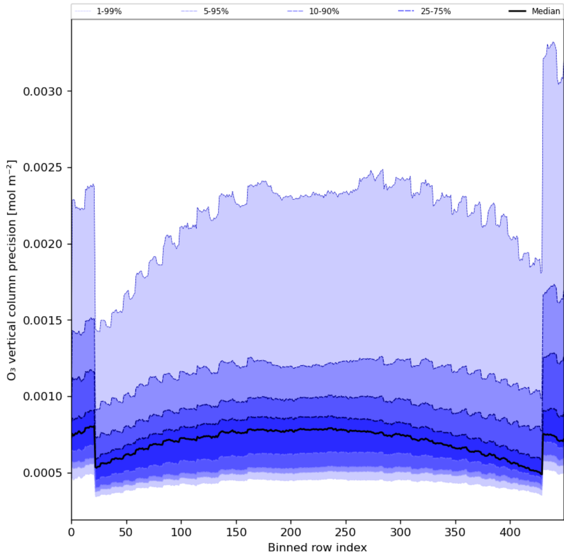
Figure 29: Along track statistics of “O 3 vertical column precision” for 2024-02-22 to 2024-02-23
