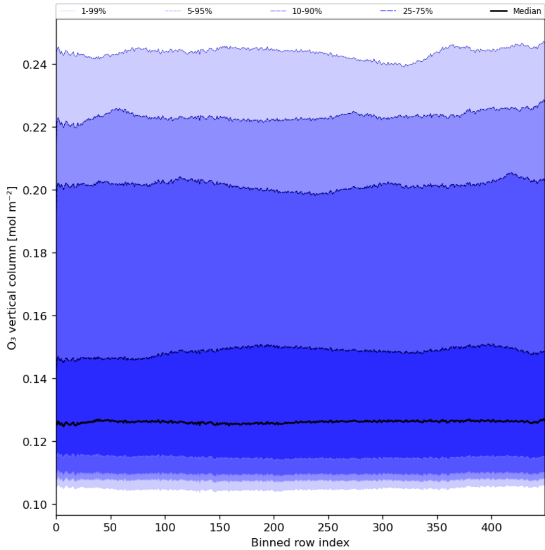
Figure 28: Along track statistics of “ O_3 vertical column” for 2024-02-22 to 2024-02-23
