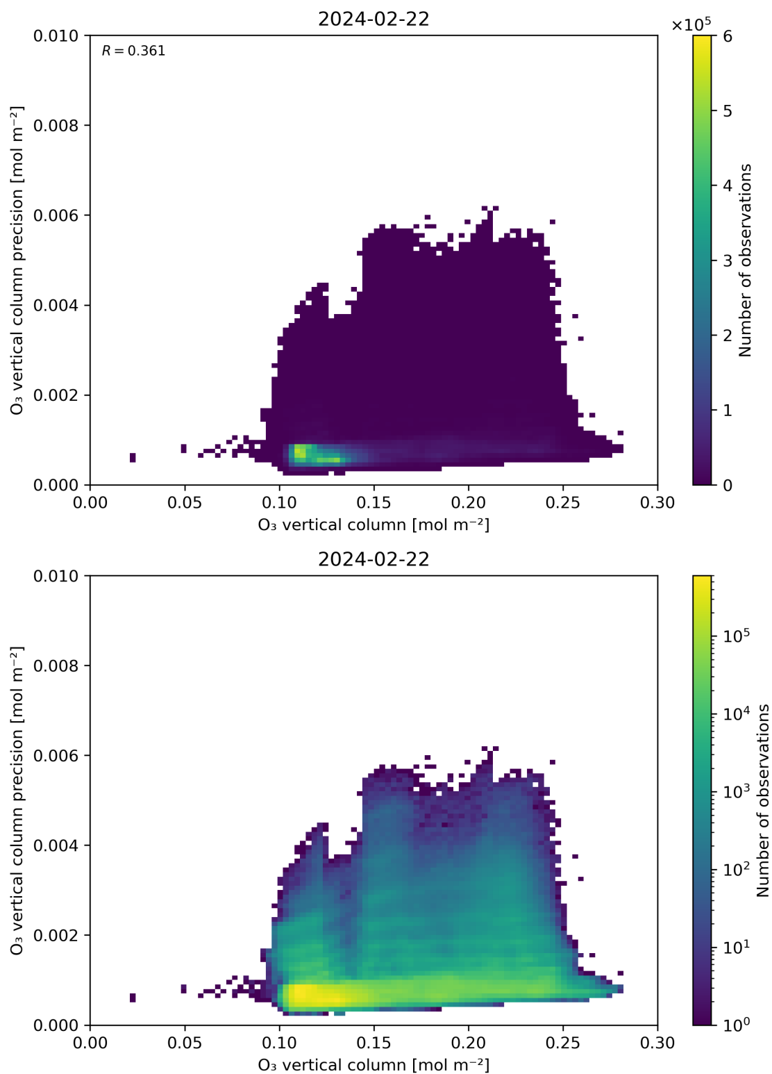
Figure 41: Scatter density plot of “O 3 vertical column” against “O 3 vertical column precision” for 2024-02-22 to 2024-02-23.
