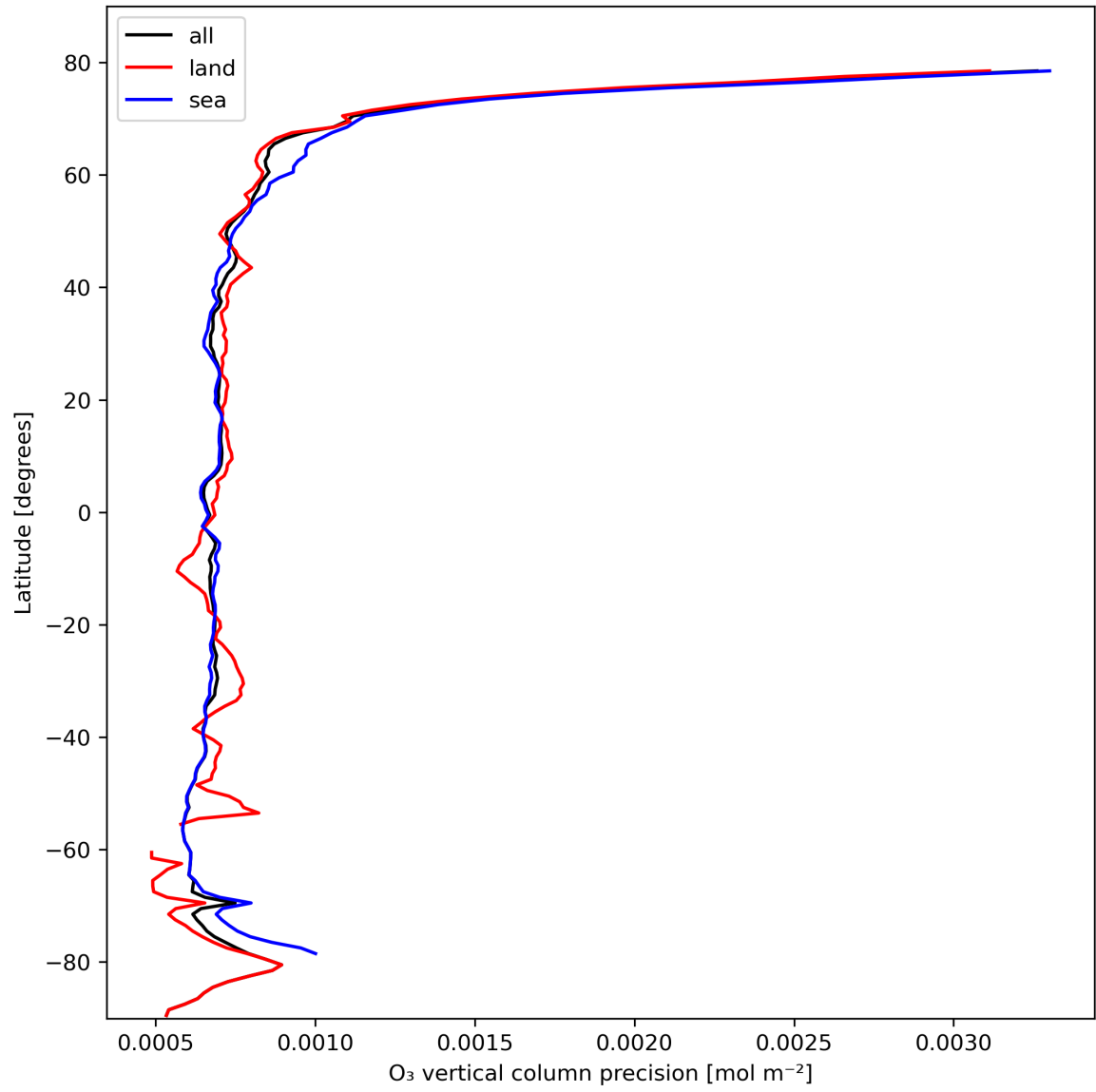
Figure 15: Zonal average of "O 3 vertical column precision" for 2024-02-22 to 2024-02-23.
