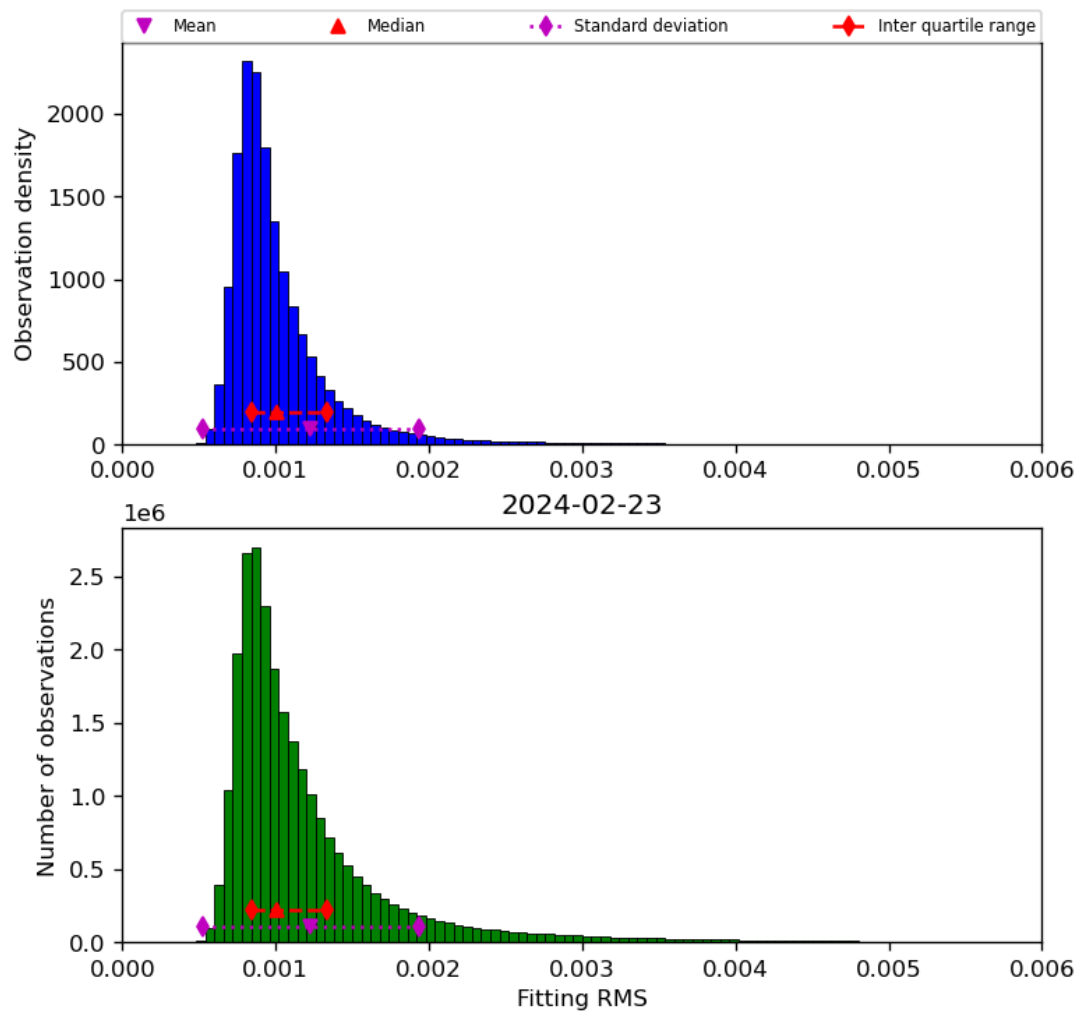
Figure 23: Histogram of “Fitting RMS” for 2024-02-22 to 2024-02-24
