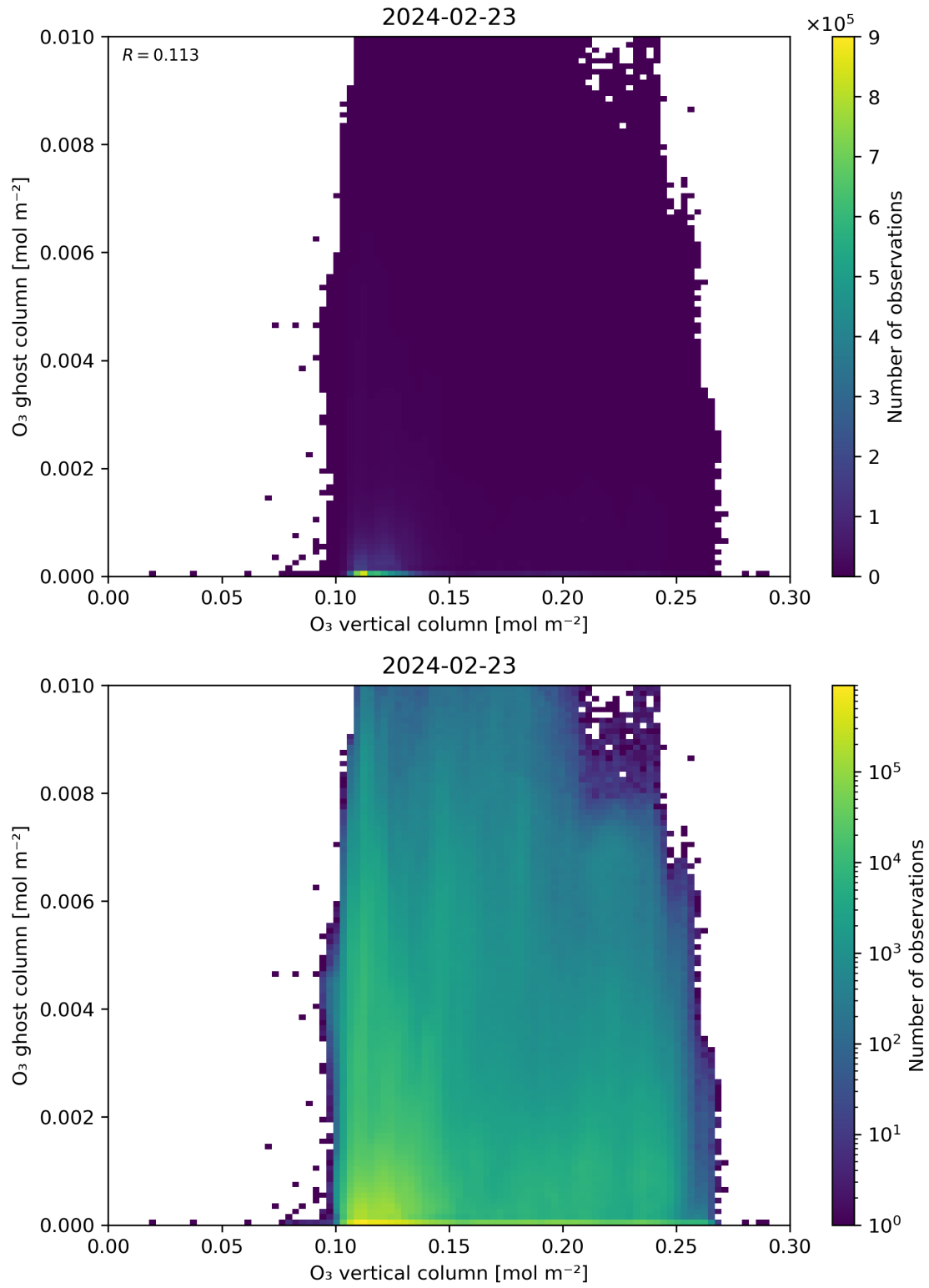
Figure 40: Scatter density plot of “O 3 vertical column” against “O 3 ghost column” for 2024-02-22 to 2024-02-24.
