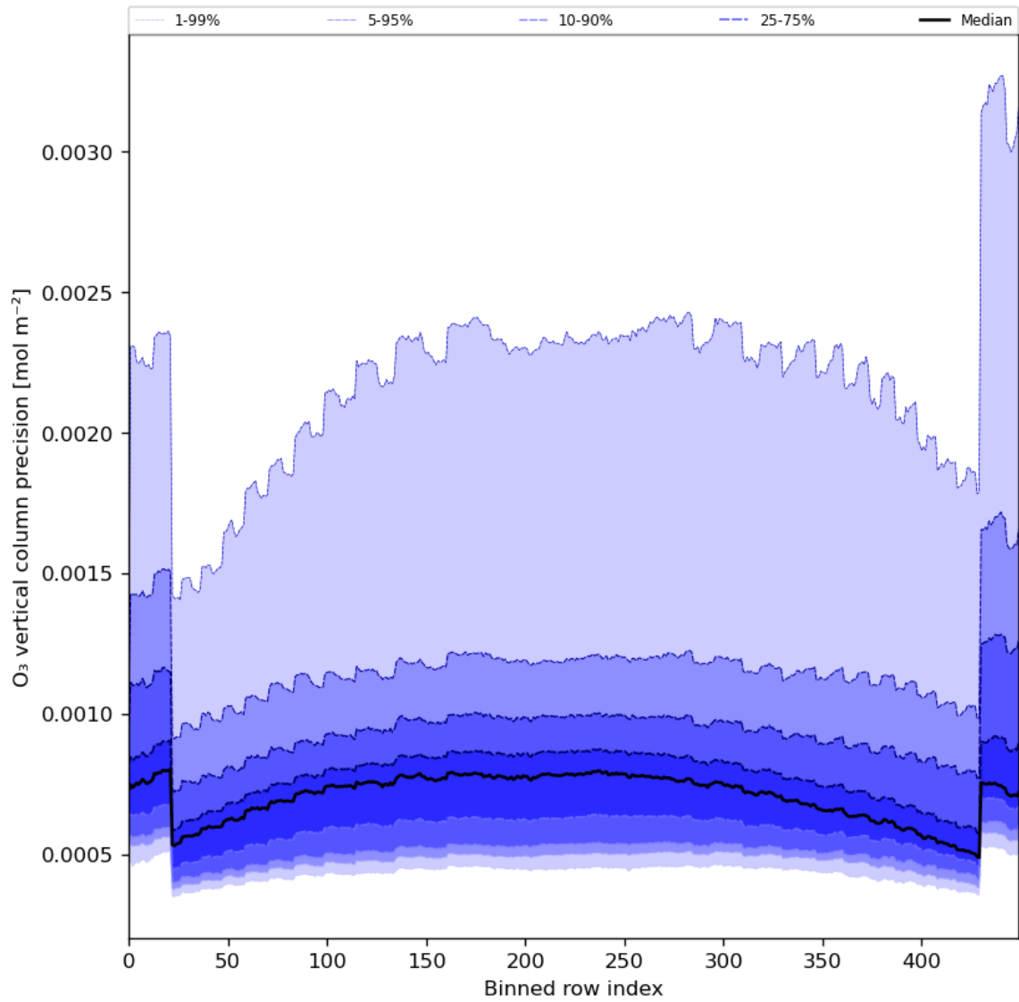
Figure 29: Along track statistics of “O 3 vertical column precision” for 2024-02-22 to 2024-02-24
