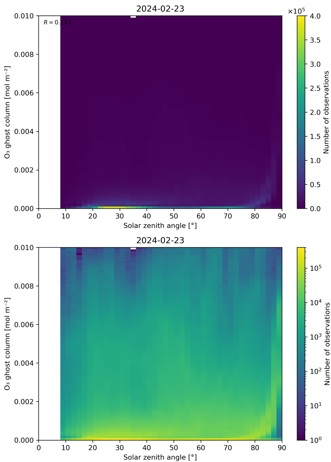
Figure 46: Scatter density plot of “Solar zenith angle” against “O 3 ghost column” for 2024-02-22 to 2024-02-24.
