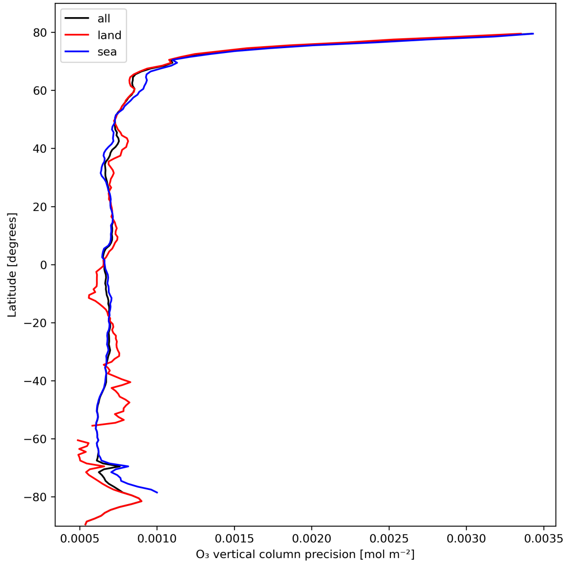
Figure 15: Zonal average of "O 3 vertical column precision" for 2024-02-22 to 2024-02-24.
