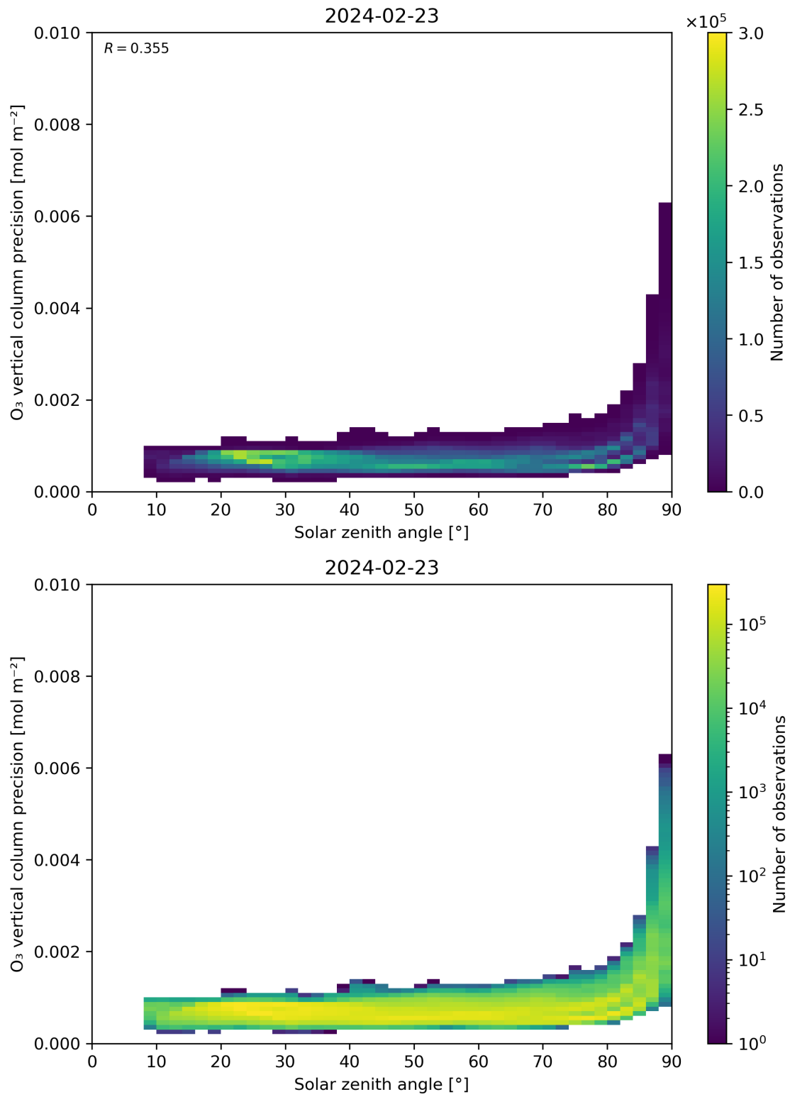
Figure 48: Scatter density plot of “Solar zenith angle” against “O 3 vertical column precision” for 2024-02-22 to 2024-02-24.
