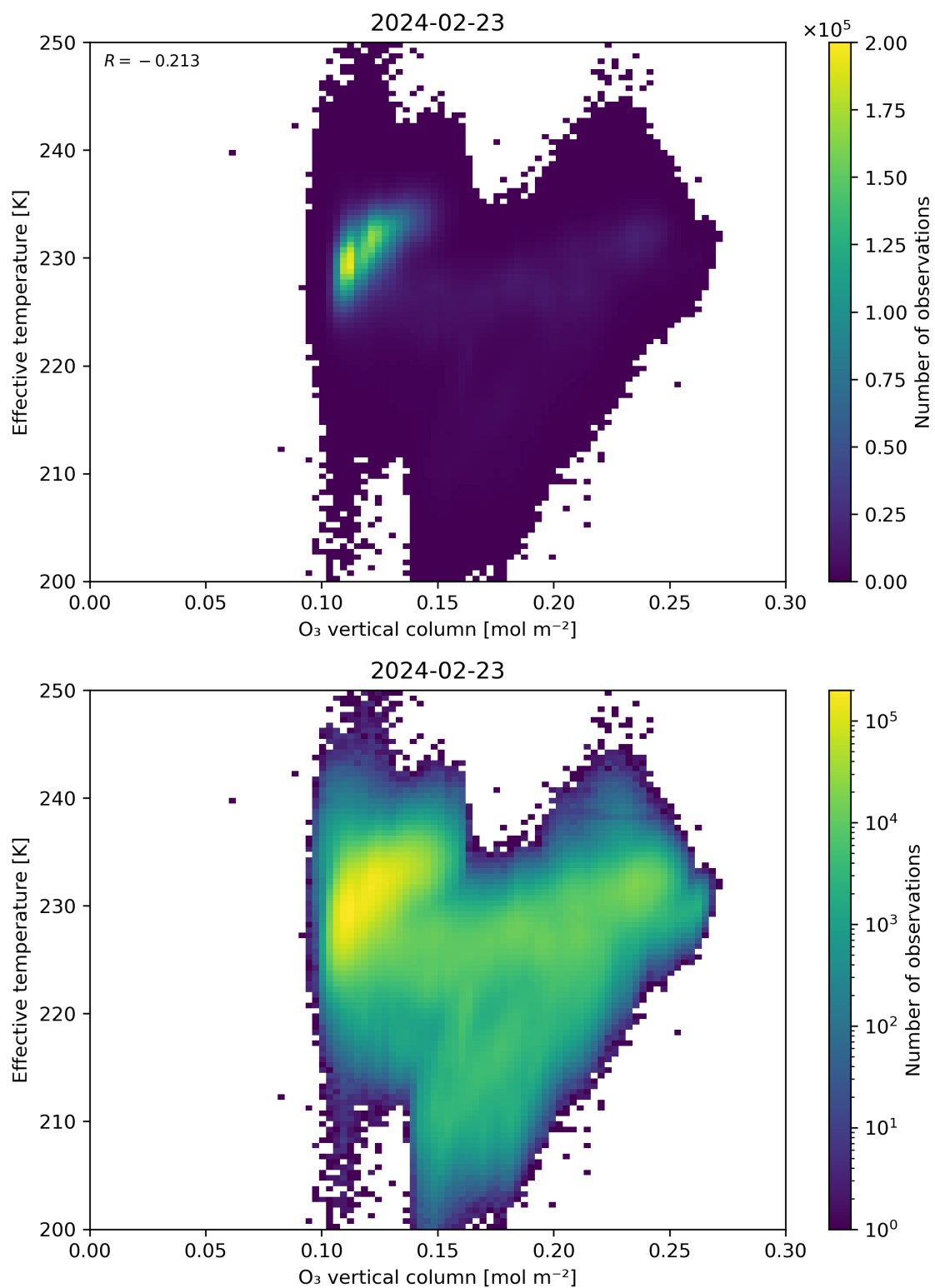
Figure 39: Scatter density plot of “O 3 vertical column” against “Effective temperature” for 2024-02-22 to 2024-02-24.
