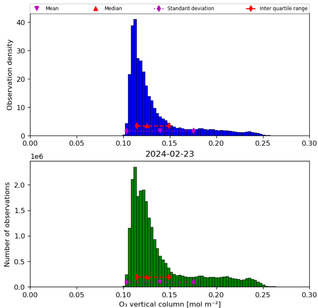
Figure 21: Histogram of “O 3 vertical column” for 2024-02-22 to 2024-02-24
