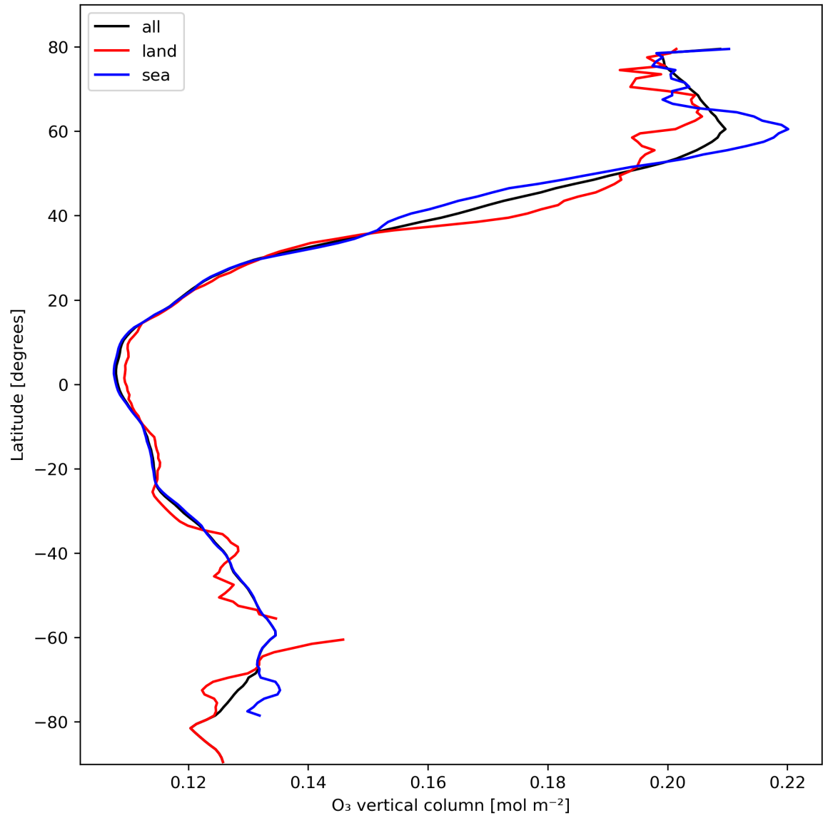
Figure 14: Zonal average of “O 3 vertical column” for 2024-02-22 to 2024-02-24.
