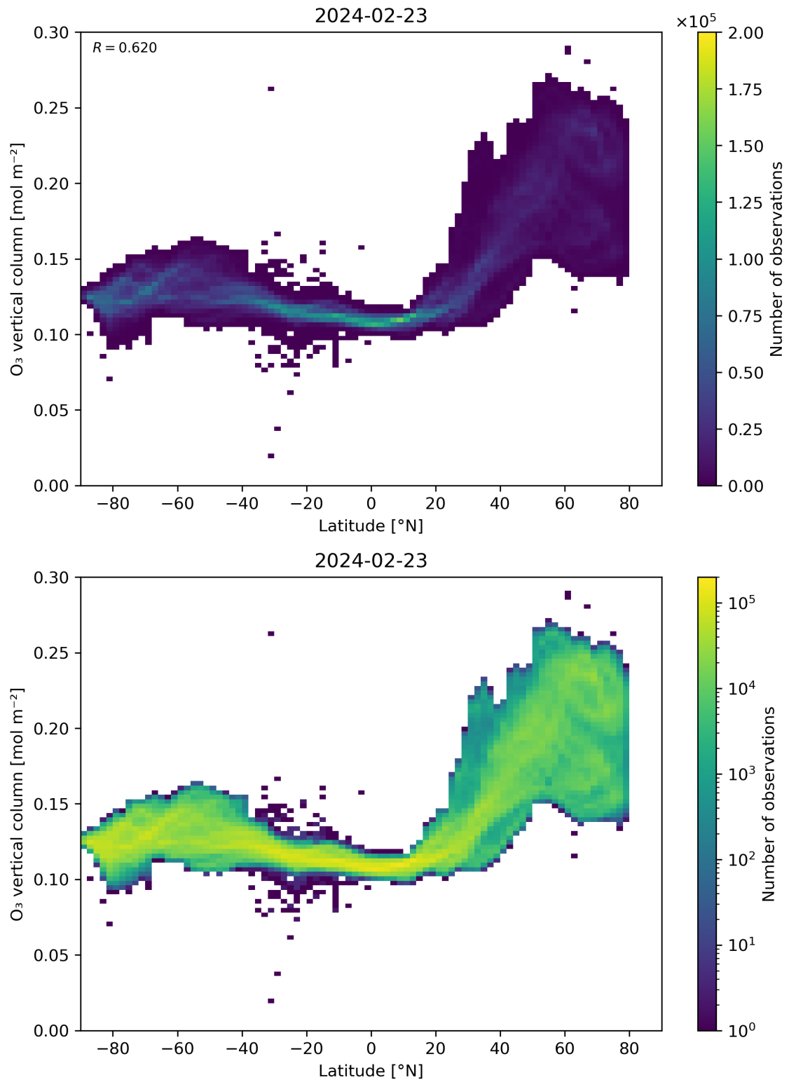
Figure 36: Scatter density plot of “Latitude” against “O 3 vertical column” for 2024-02-22 to 2024-02-24.
