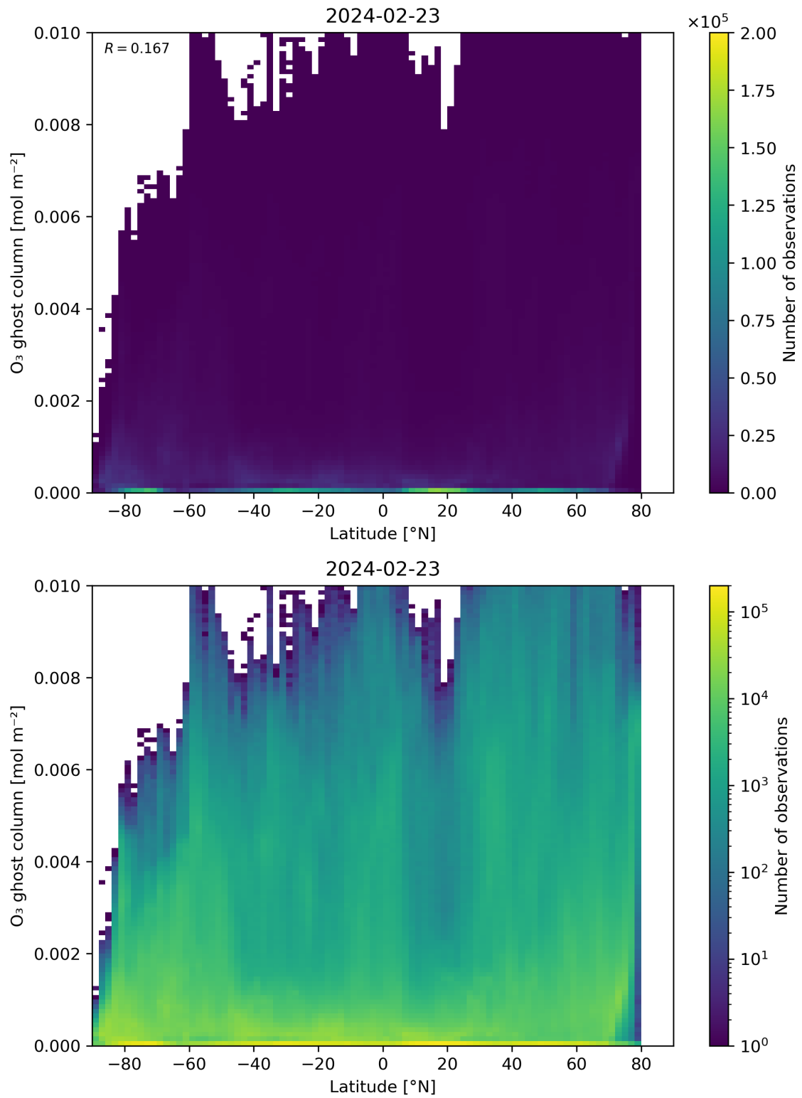
Figure 35: Scatter density plot of “Latitude” against “O 3 ghost column” for 2024-02-22 to 2024-02-24.
