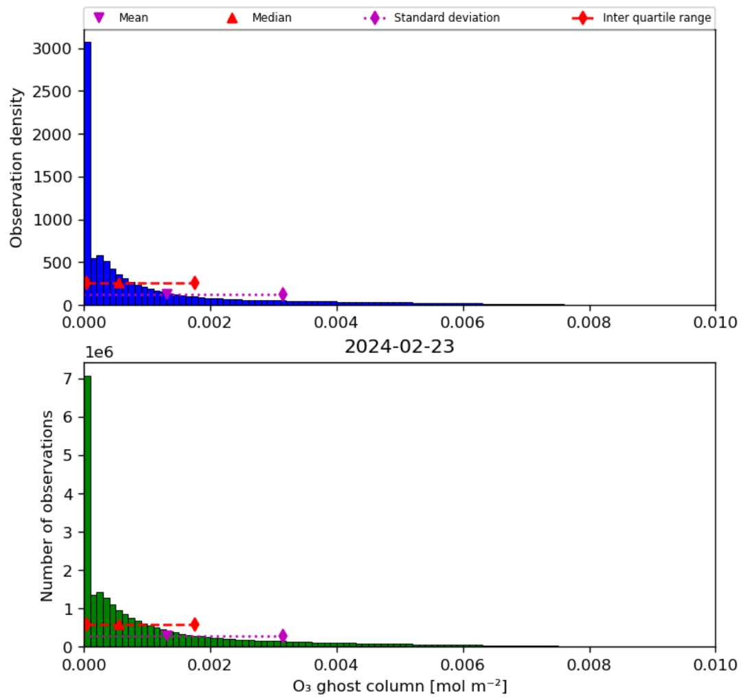
Figure 25: Histogram of “O 3 ghost column” for 2024-02-22 to 2024-02-24
