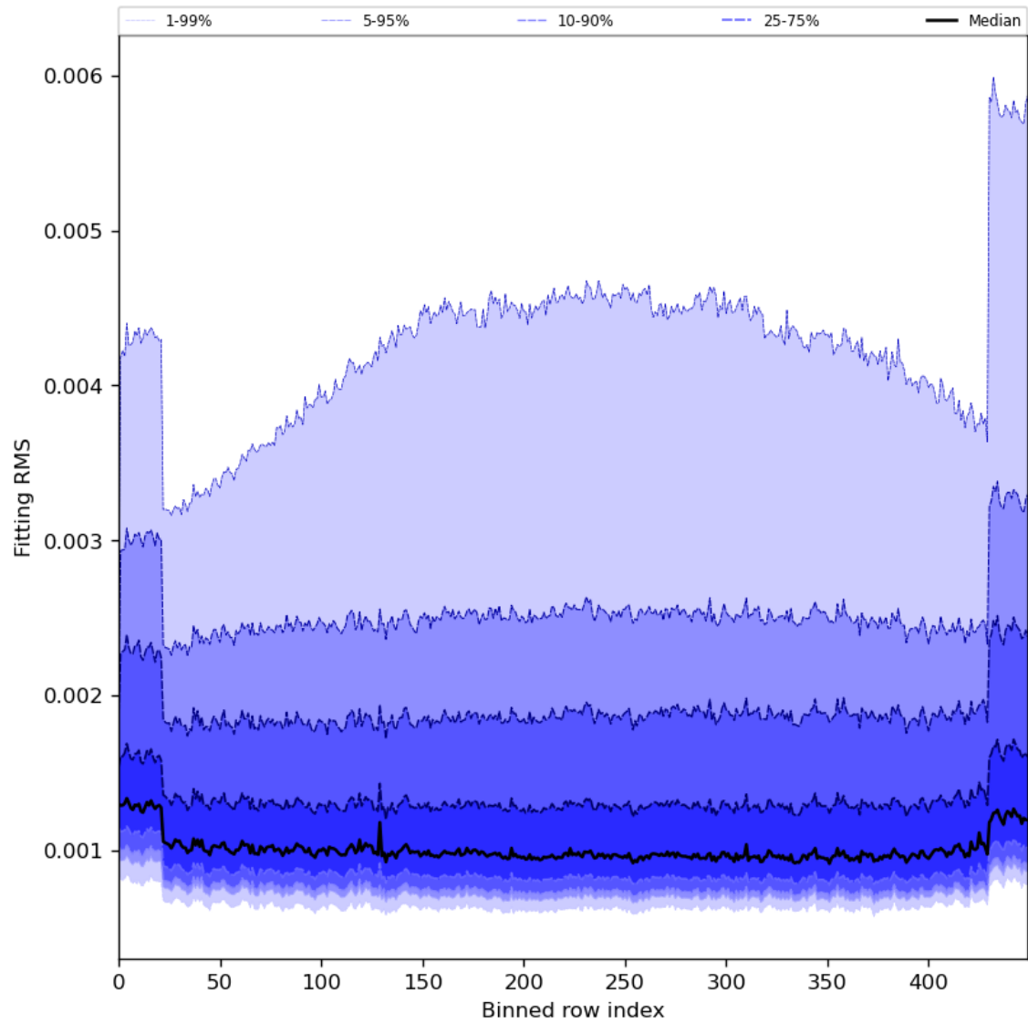
Figure 30: Along track statistics of “Fitting RMS” for 2024-02-22 to 2024-02-24
