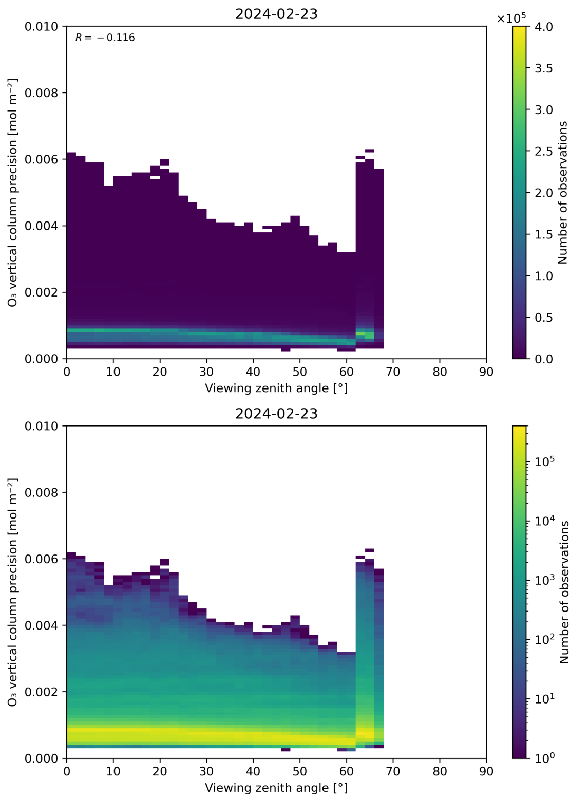
Figure 53: Scatter density plot of “Viewing zenith angle” against “O 3 vertical column precision” for 2024-02-22 to 2024-02-24.
