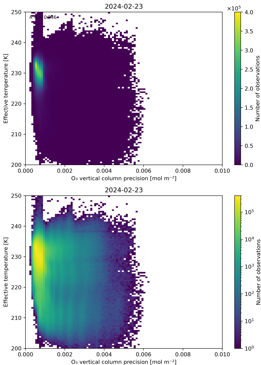
Figure 42: Scatter density plot of “ O_3 vertical column precision” against “Effective temperature” for 2024-02-22 to 2024-02-24.
