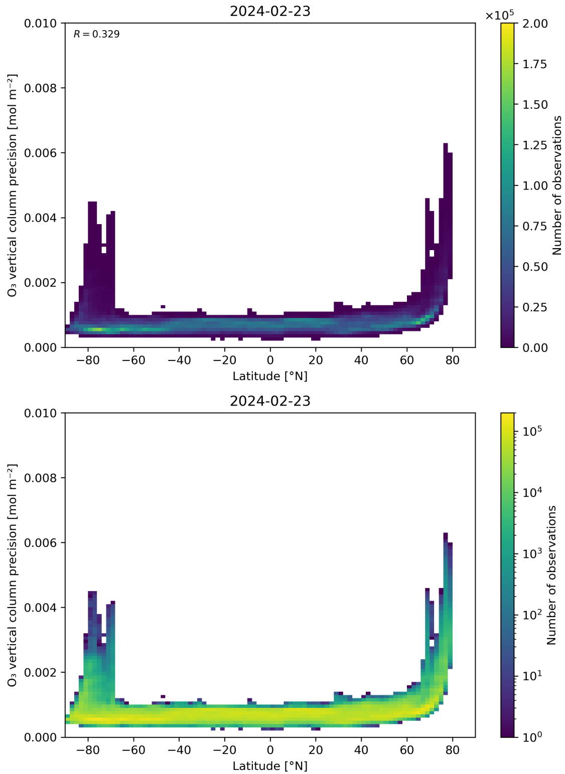
Figure 37: Scatter density plot of “Latitude” against “O 3 vertical column precision” for 2024-02-22 to 2024-02-24.
