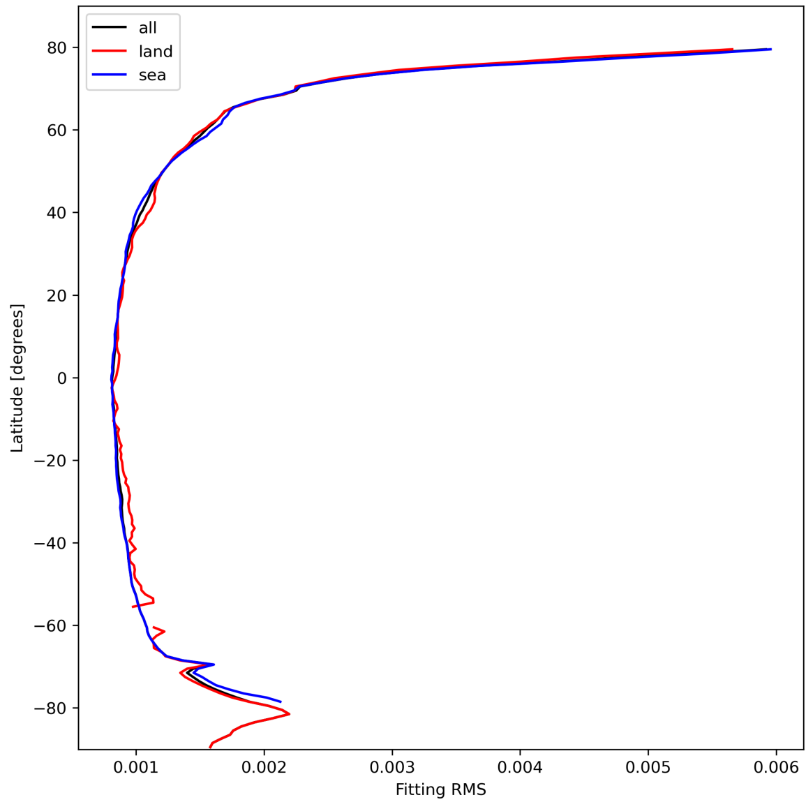
Figure 16: Zonal average of “Fitting RMS” for 2024-02-22 to 2024-02-24.
