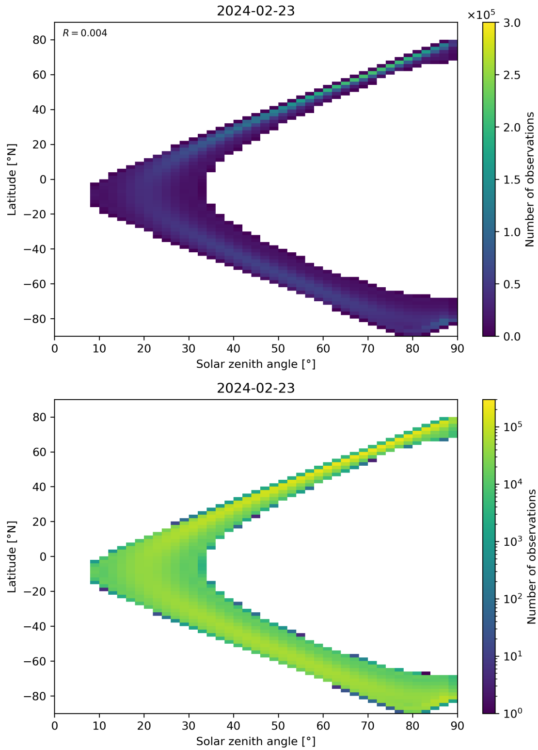
Figure 44: Scatter density plot of “Solar zenith angle” against “Latitude” for 2024-02-22 to 2024-02-24.
