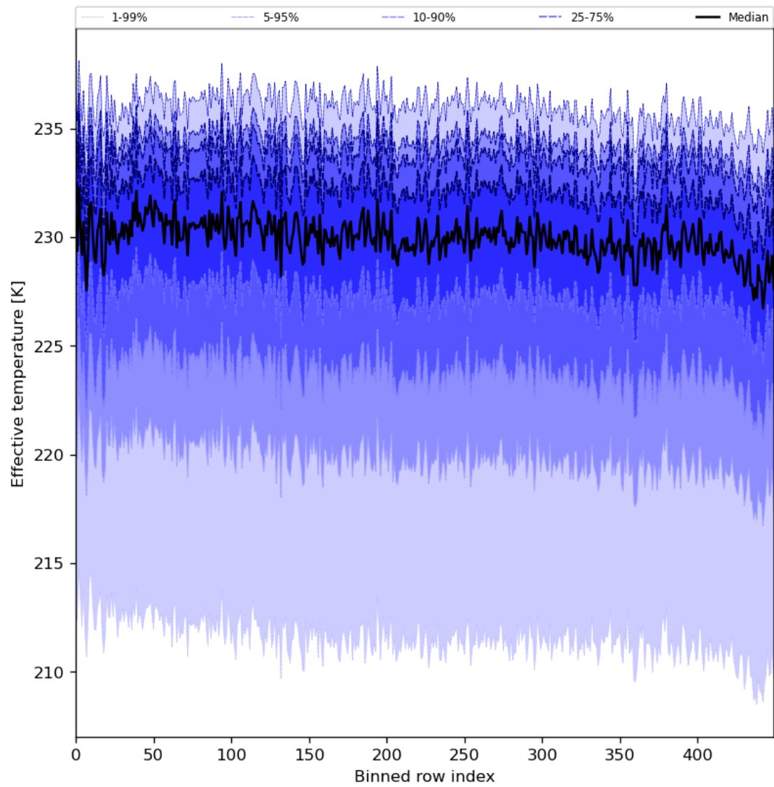
Figure 31: Along track statistics of “Effective temperature” for 2024-02-22 to 2024-02-24
