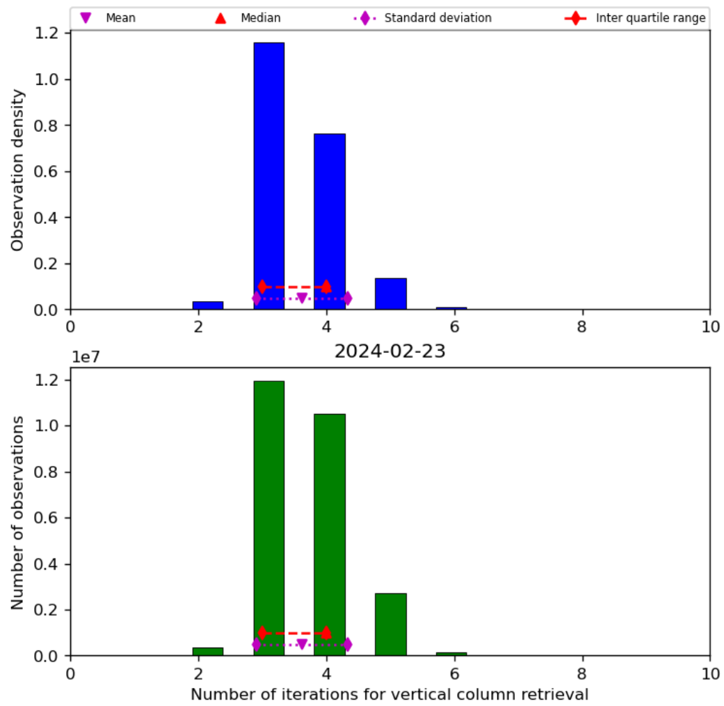
Figure 26: Histogram of “Number of iterations for vertical column retrieval” for 2024-02-22 to 2024-02-24
