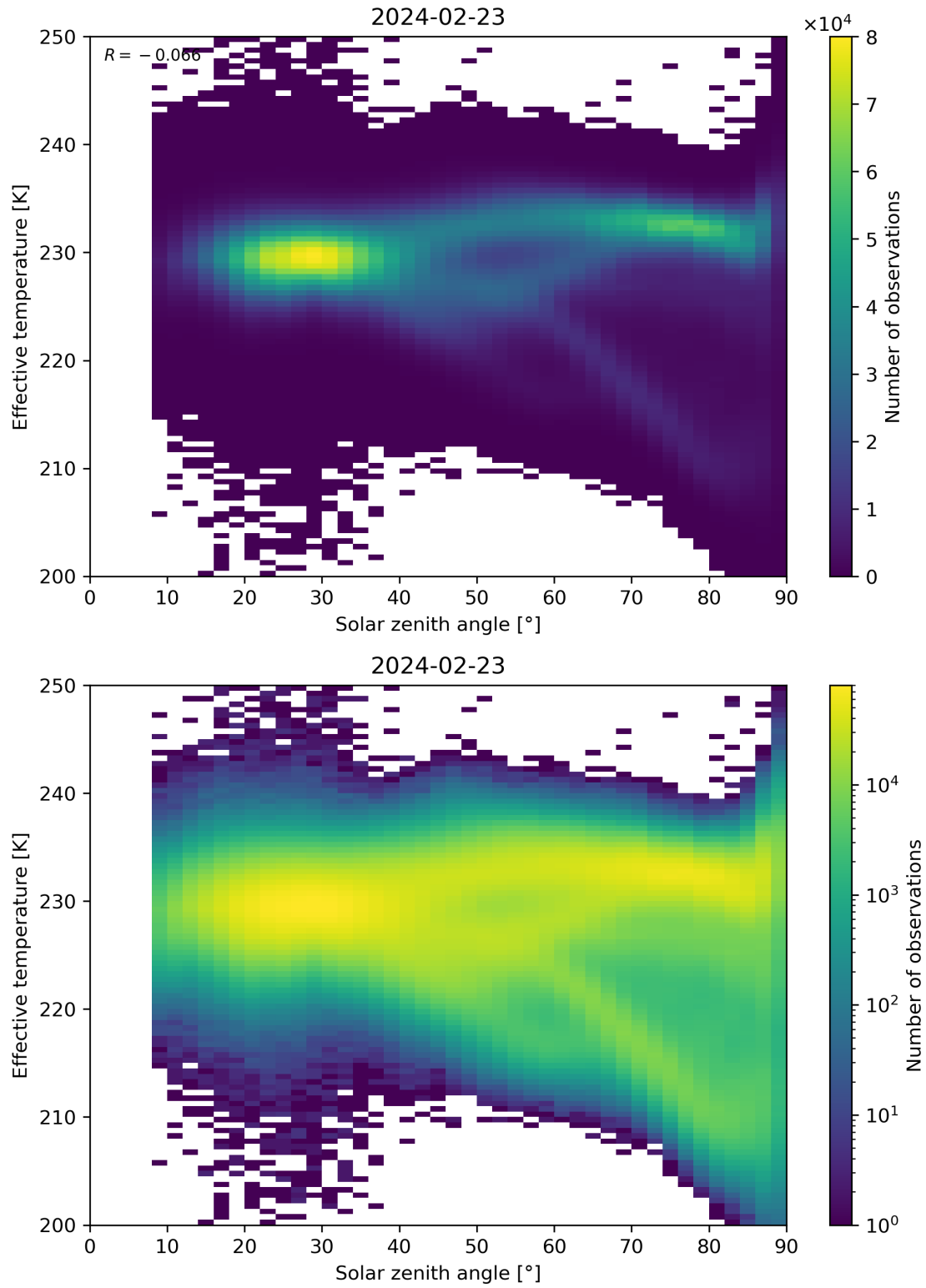
Figure 45: Scatter density plot of “Solar zenith angle” against “Effective temperature” for 2024-02-22 to 2024-02-24.
