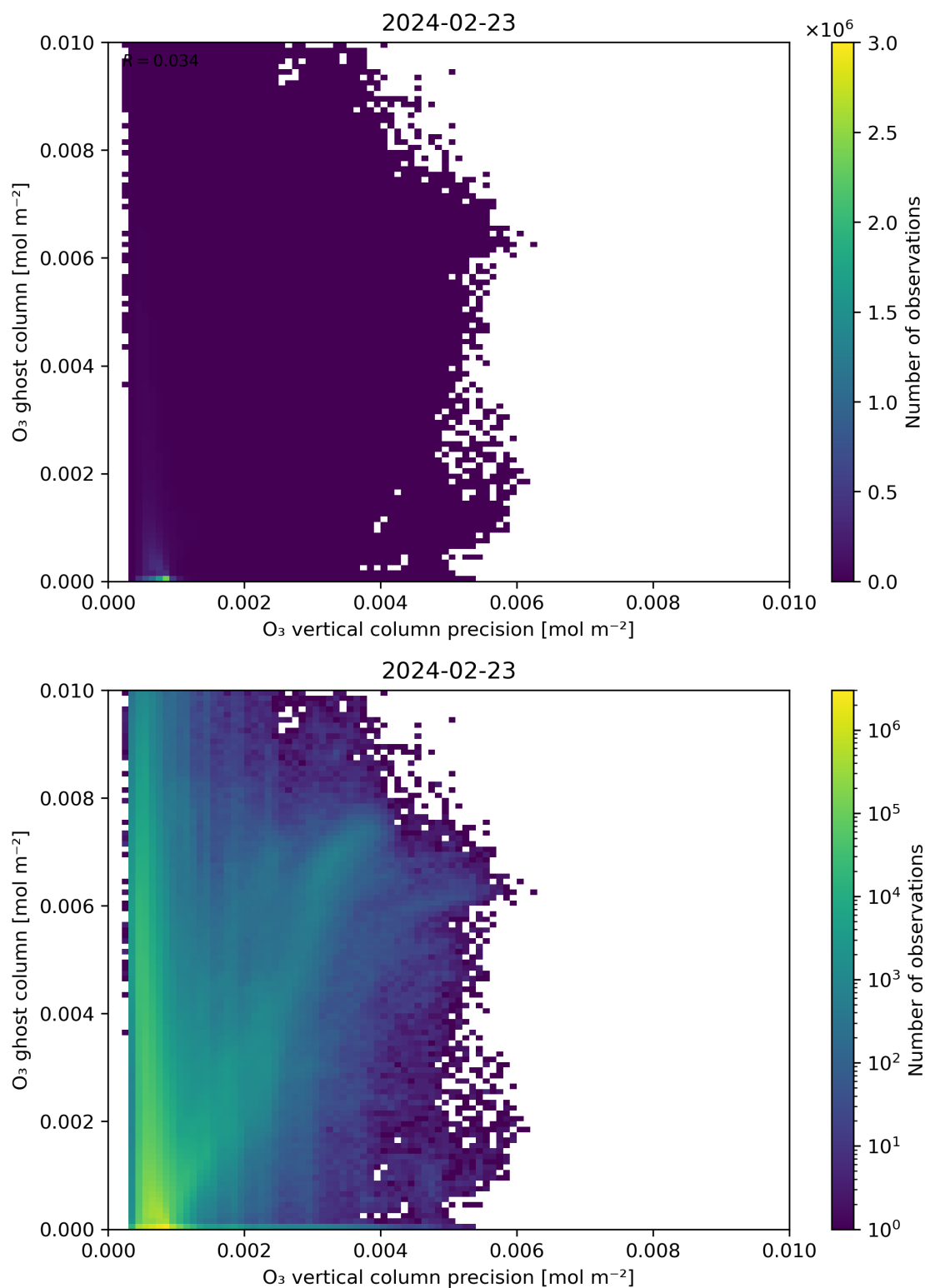
Figure 43: Scatter density plot of “ \text{O}_3 vertical column precision” against “ \text{O}_3 ghost column” for 2024-02-22 to 2024-02-24.
