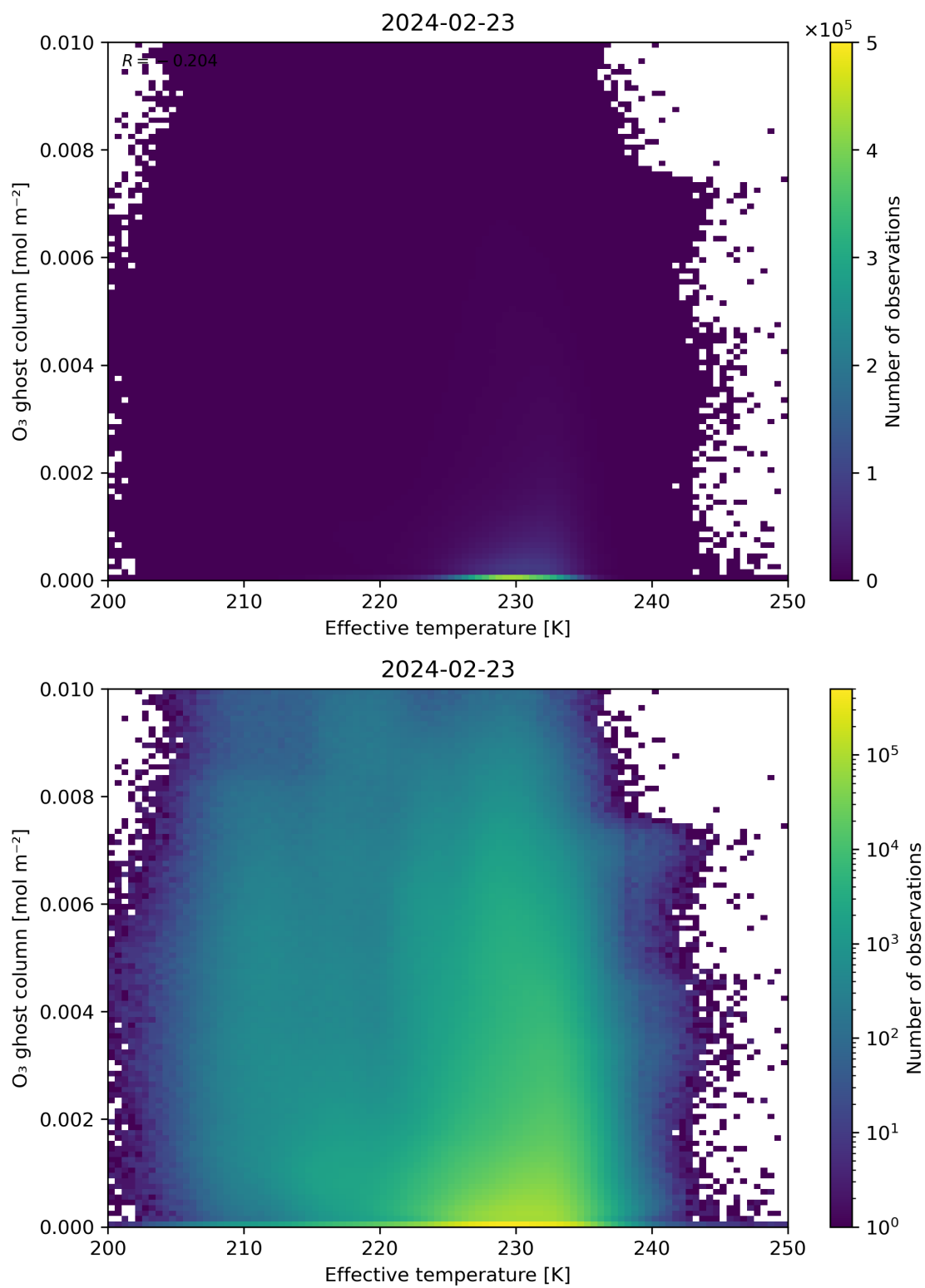
Figure 38: Scatter density plot of “Effective temperature” against “O 3 ghost column” for 2024-02-22 to 2024-02-24.
