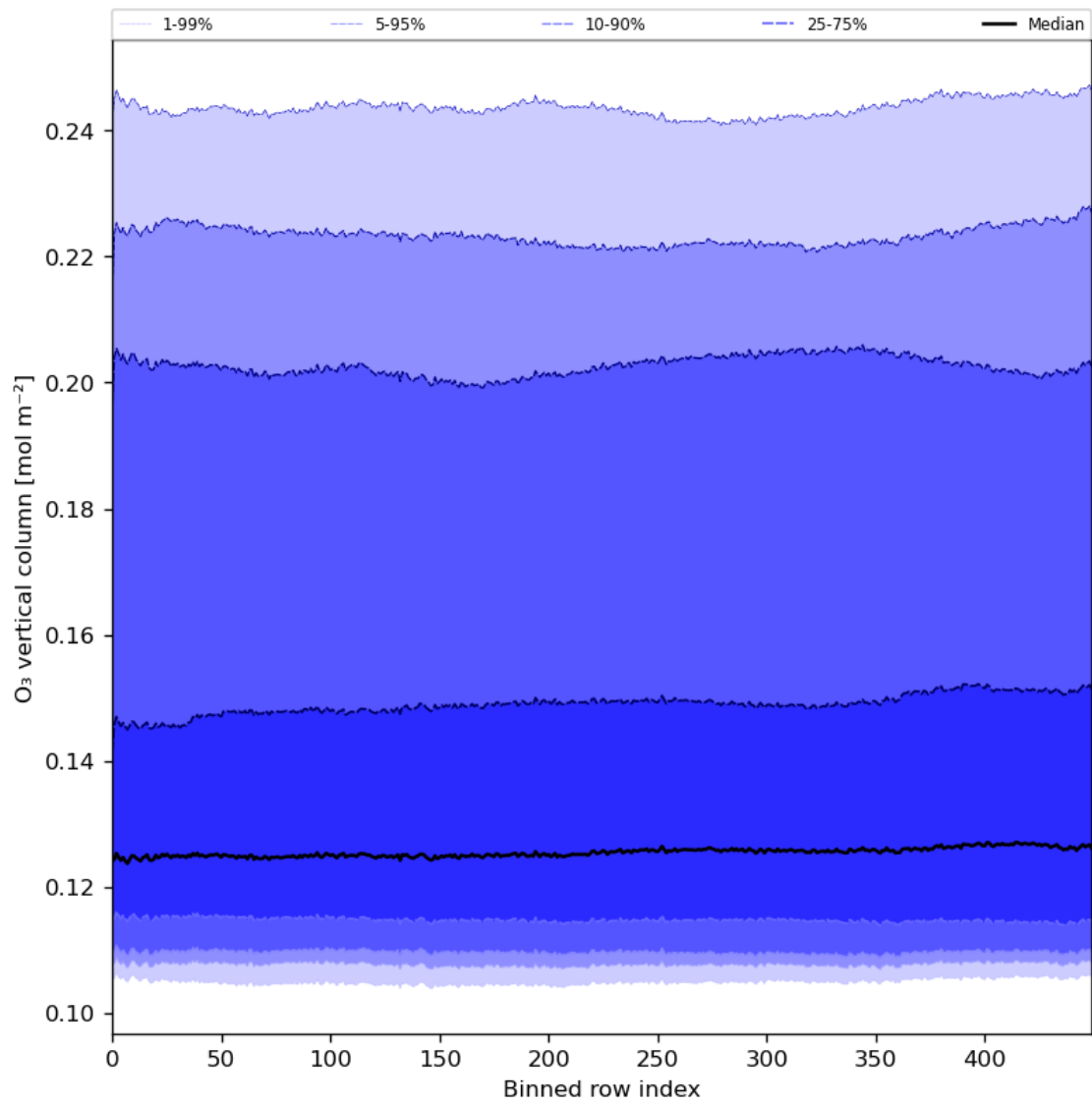
Figure 28: Along track statistics of “O 3 vertical column” for 2024-02-22 to 2024-02-24
