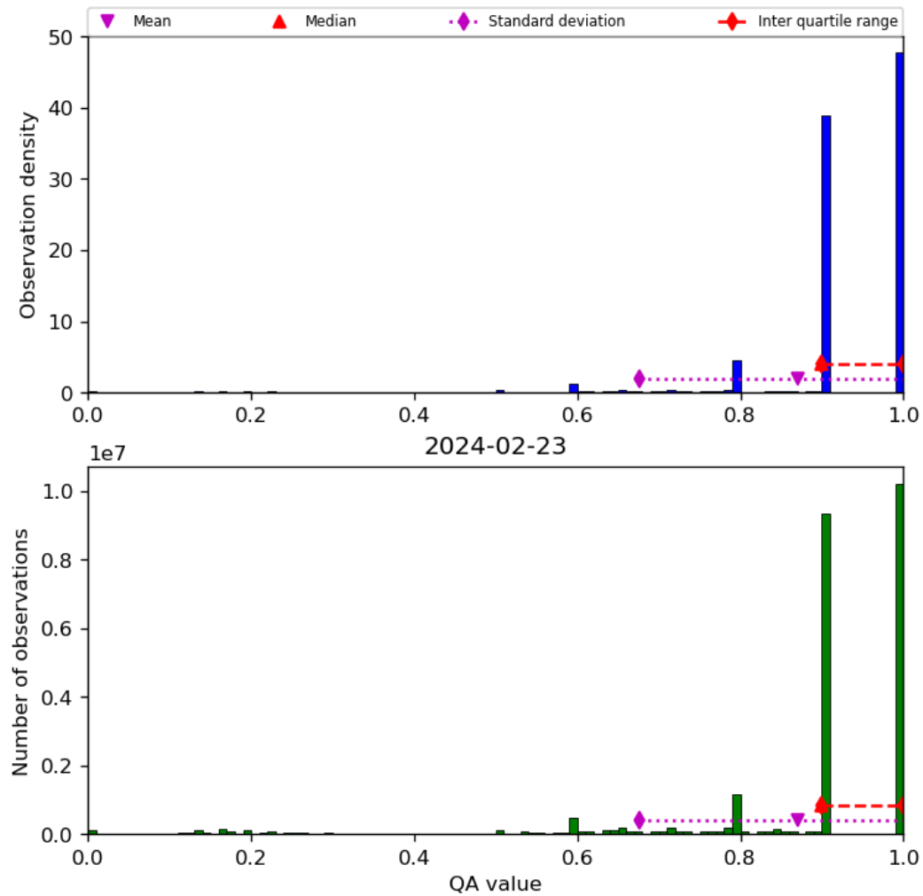
Figure 20: Histogram of “QA value” for 2024-02-22 to 2024-02-24
