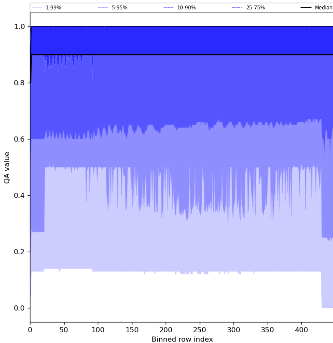
Figure 27: Along track statistics of “QA value” for 2024-02-22 to 2024-02-24
