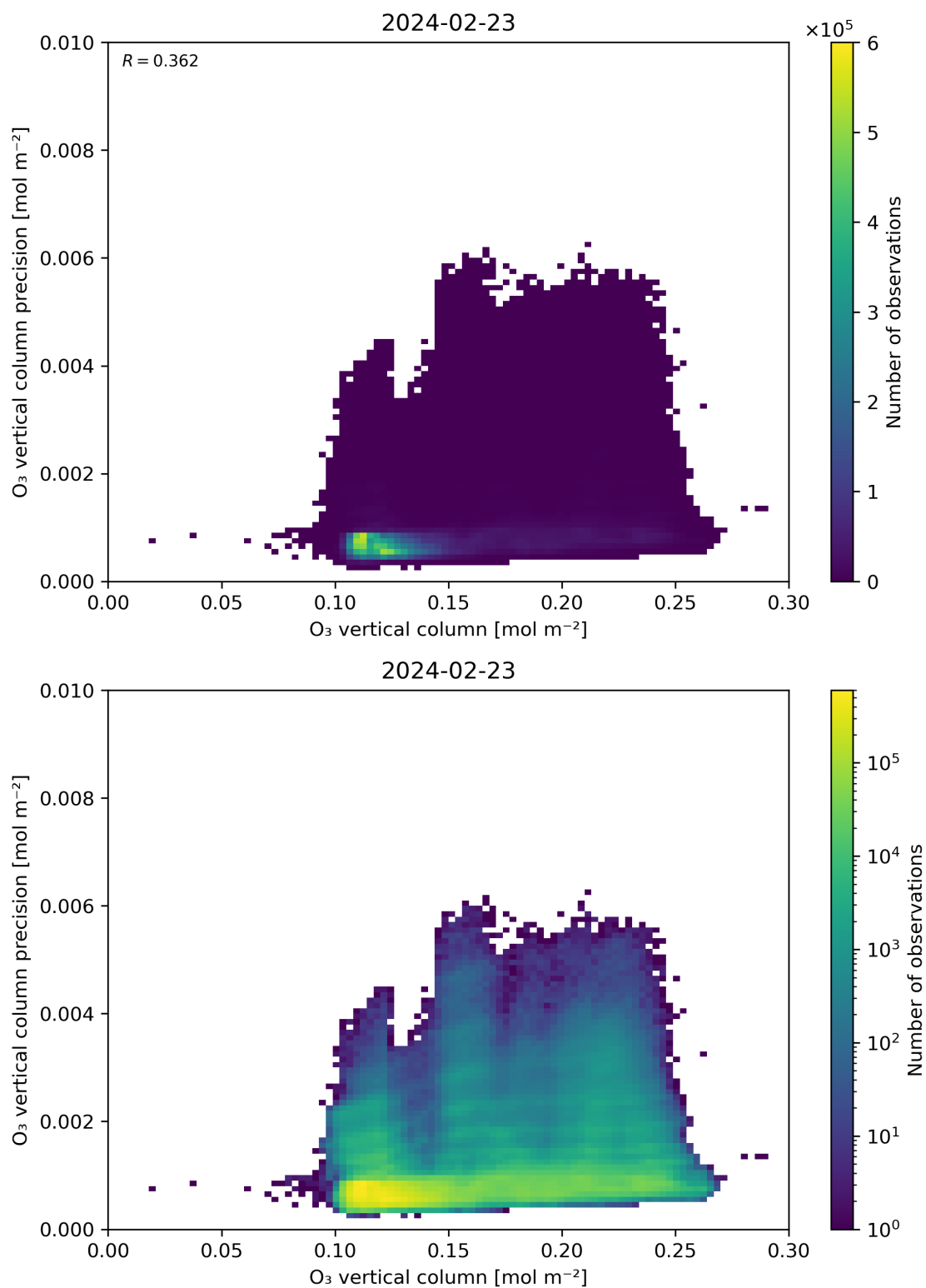
Figure 41: Scatter density plot of “O 3 vertical column” against “O 3 vertical column precision” for 2024-02-22 to 2024-02-24.
