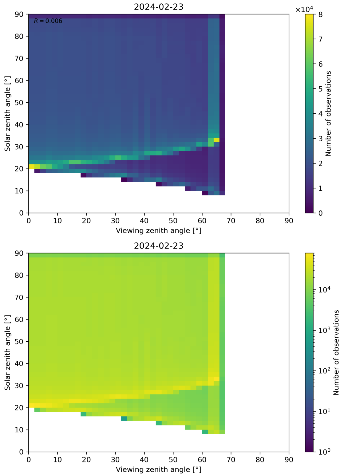
Figure 54: Scatter density plot of “Viewing zenith angle” against “Solar zenith angle” for 2024-02-22 to 2024-02-24.
