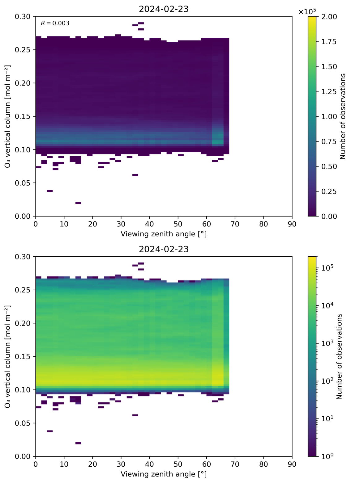
Figure 52: Scatter density plot of “Viewing zenith angle” against “O 3 vertical column” for 2024-02-22 to 2024-02-24.
