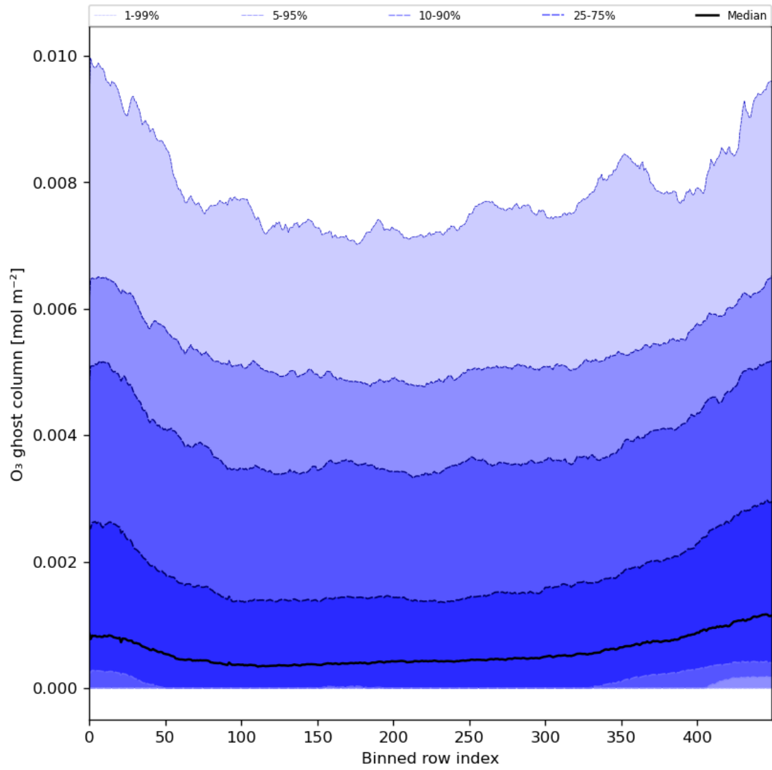
Figure 32: Along track statistics of “O 3 ghost column” for 2024-02-22 to 2024-02-24
