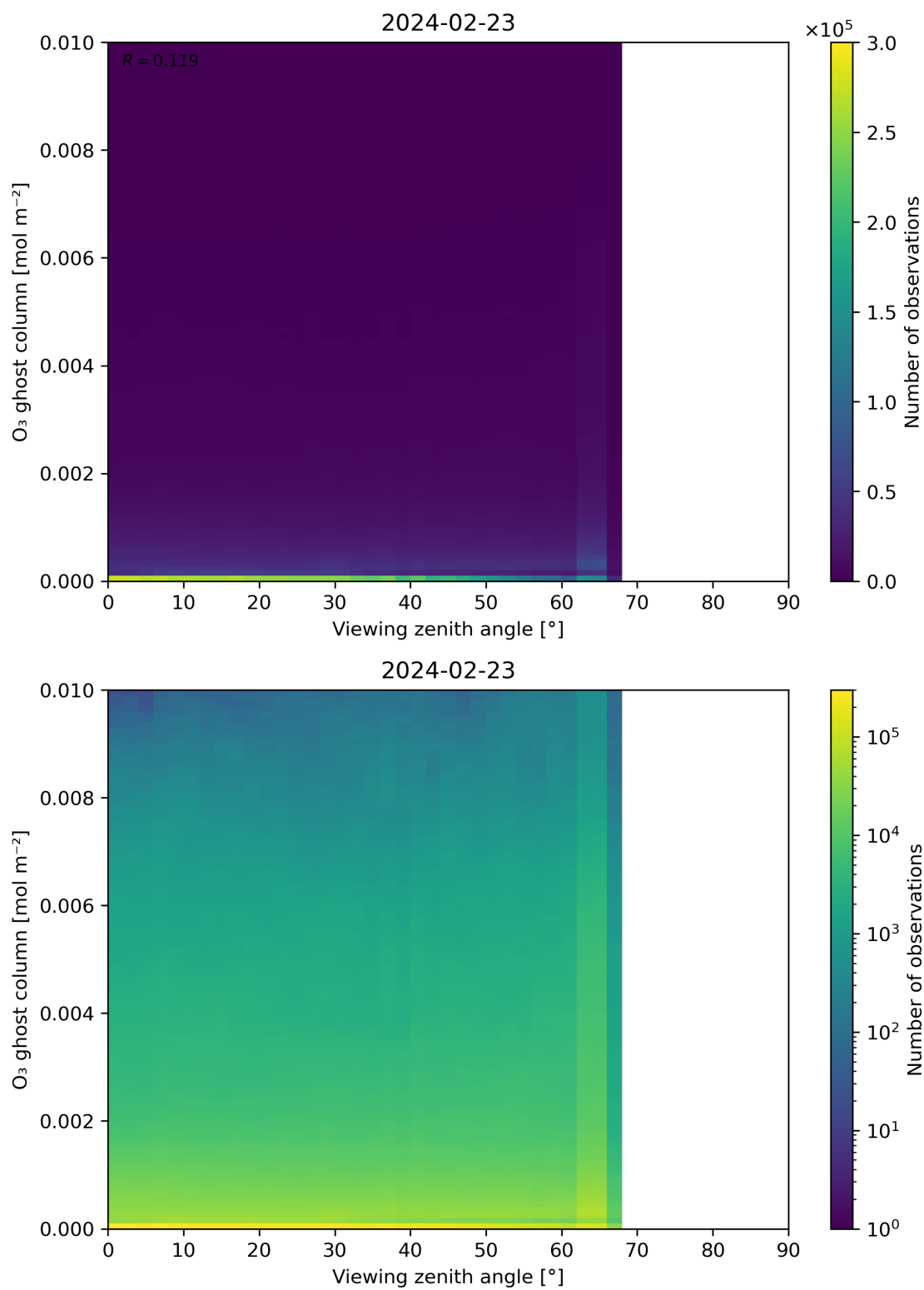
Figure 51: Scatter density plot of “Viewing zenith angle” against “O 3 ghost column” for 2024-02-22 to 2024-02-24.
