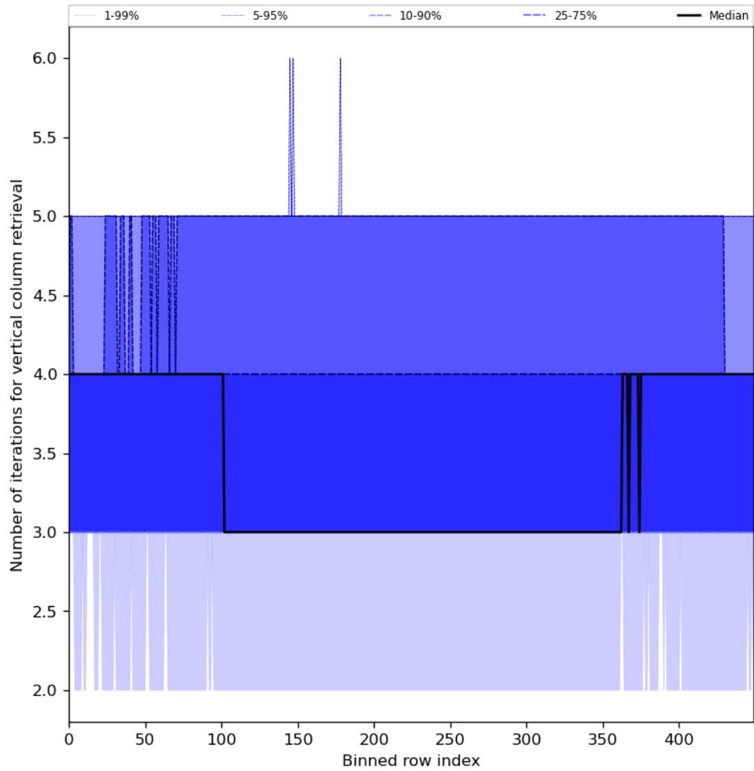
Figure 33: Along track statistics of “Number of iterations for vertical column retrieval” for 2024-02-22 to 2024-02-24
