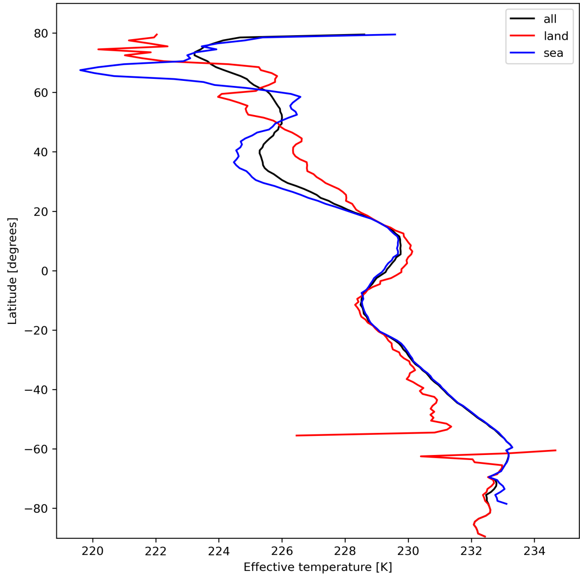
Figure 17: Zonal average of “Effective temperature” for 2024-02-22 to 2024-02-24.
