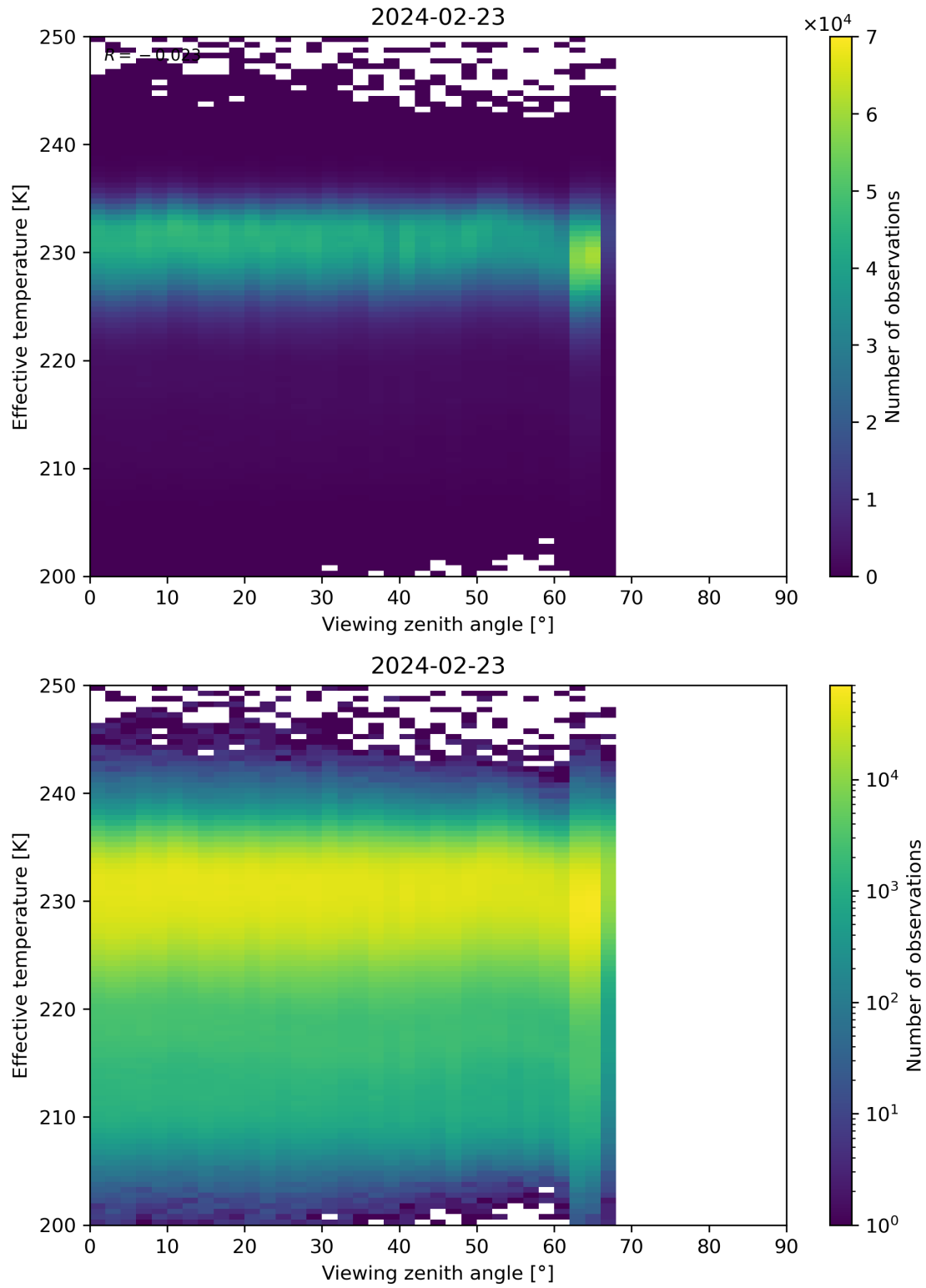
Figure 50: Scatter density plot of “Viewing zenith angle” against “Effective temperature” for 2024-02-22 to 2024-02-24.
