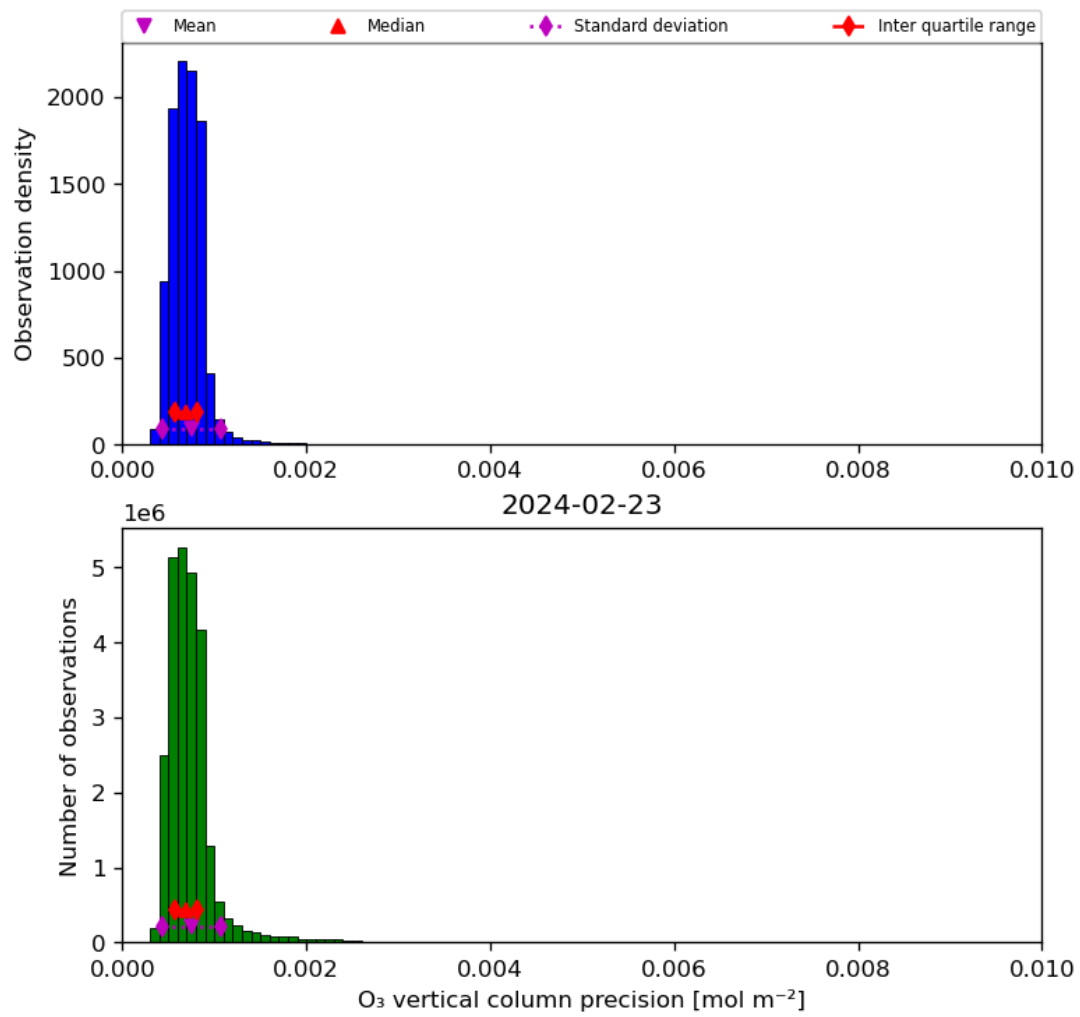
Figure 22: Histogram of “O 3 vertical column precision” for 2024-02-22 to 2024-02-24
