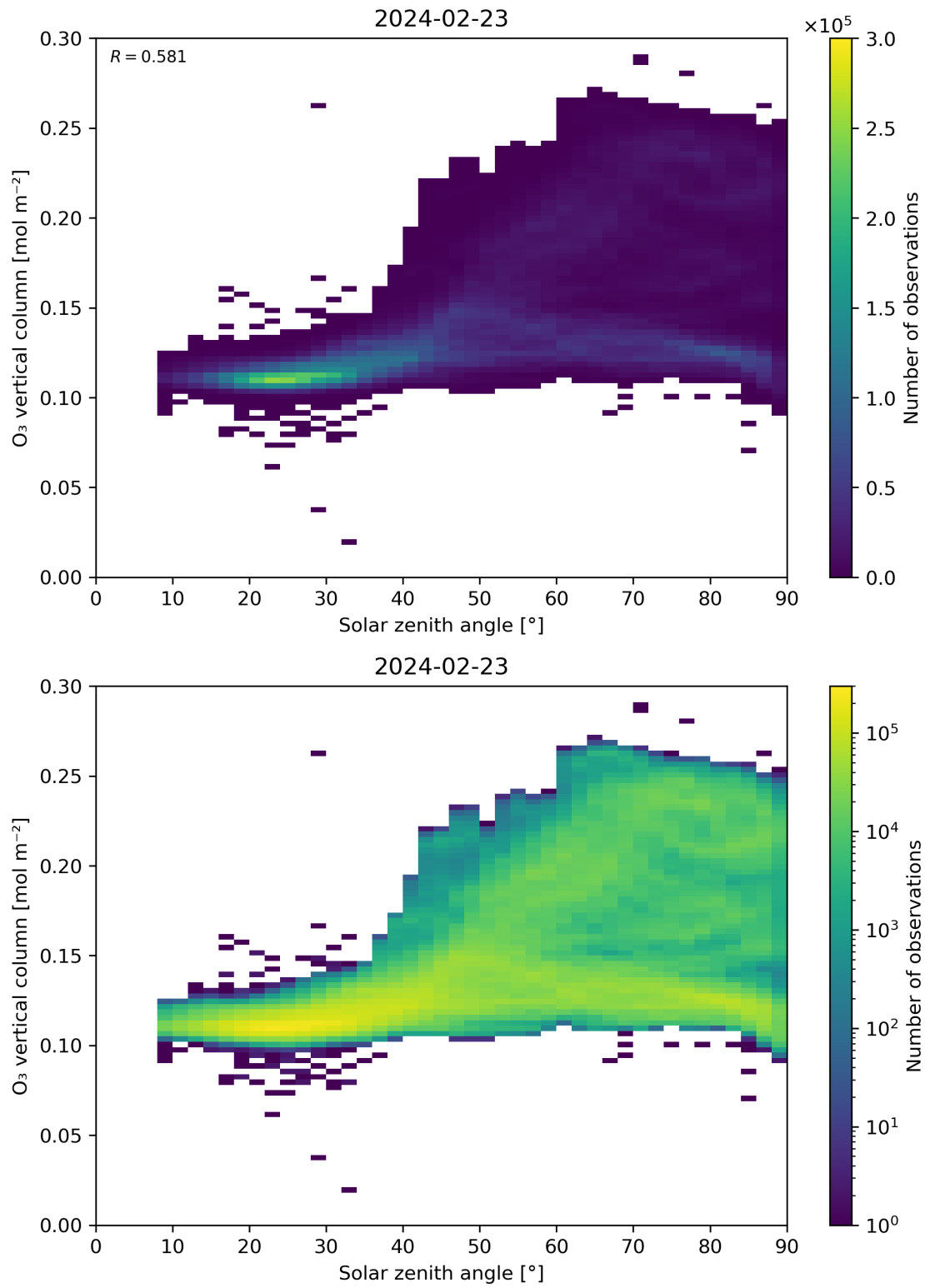
Figure 47: Scatter density plot of “Solar zenith angle” against “O 3 vertical column” for 2024-02-22 to 2024-02-24.
