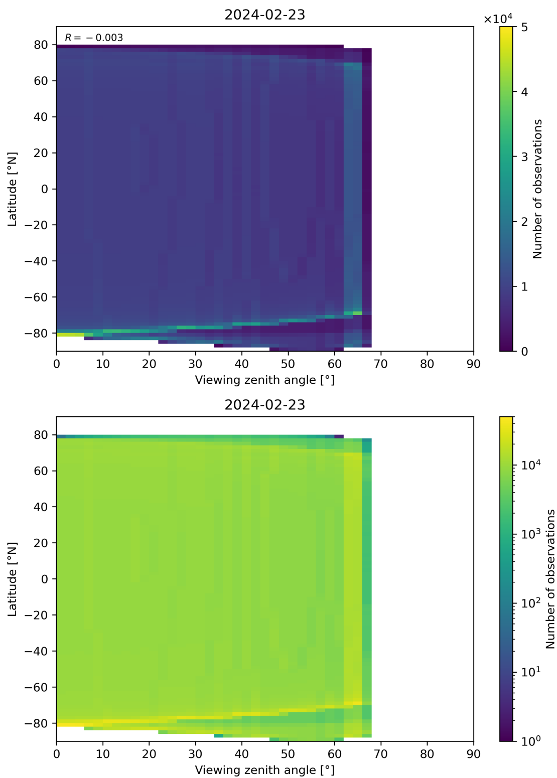
Figure 49: Scatter density plot of “Viewing zenith angle” against “Latitude” for 2024-02-22 to 2024-02-24.
