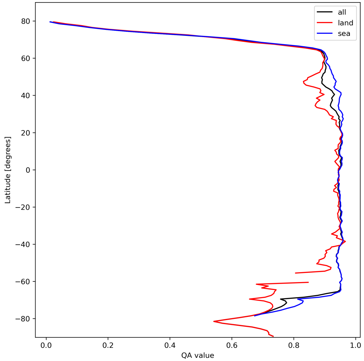
Figure 13: Zonal average of “QA value” for 2024-02-22 to 2024-02-24.
