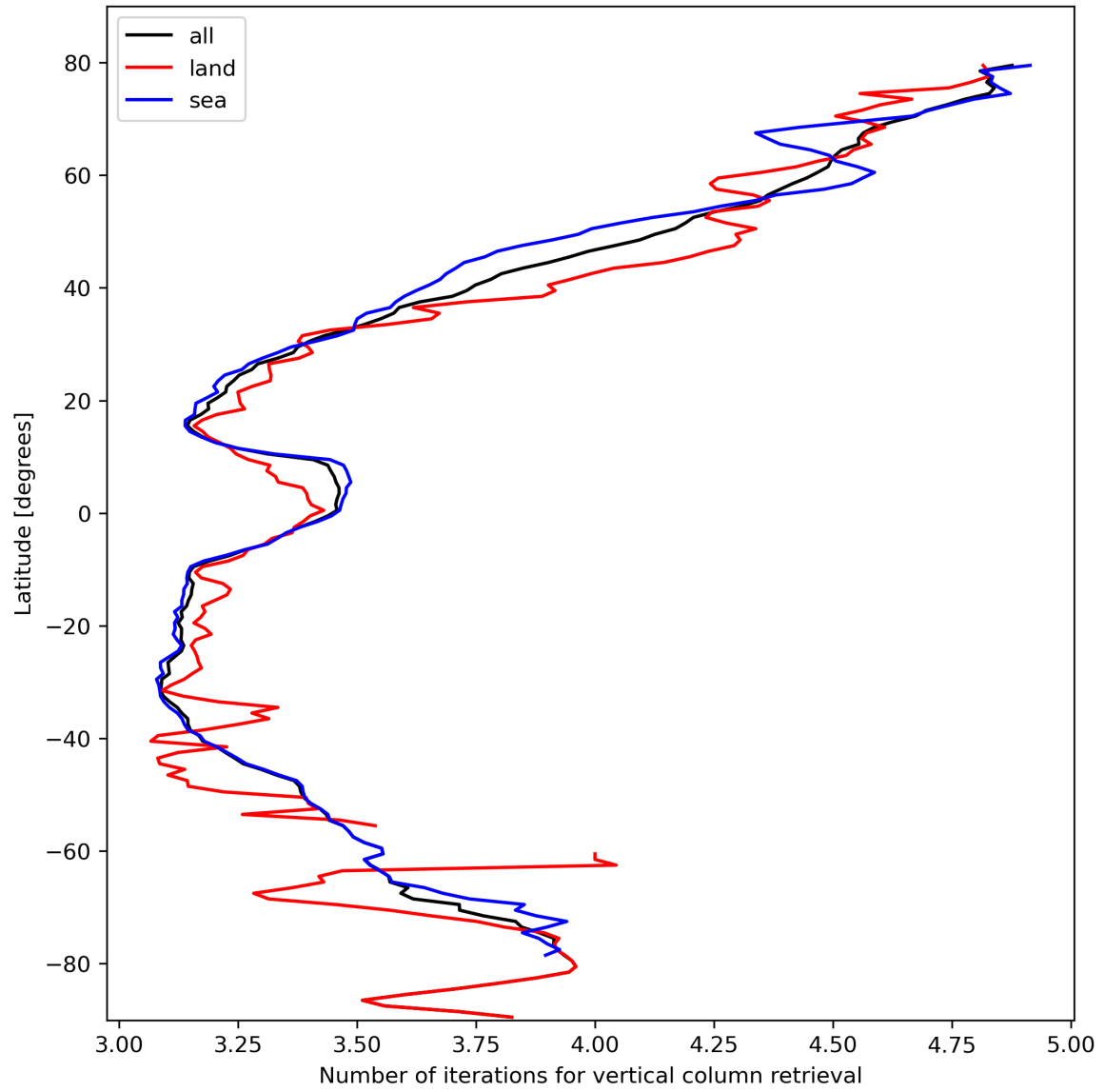
Figure 19: Zonal average of “Number of iterations for vertical column retrieval” for 2024-02-22 to 2024-02-24.
