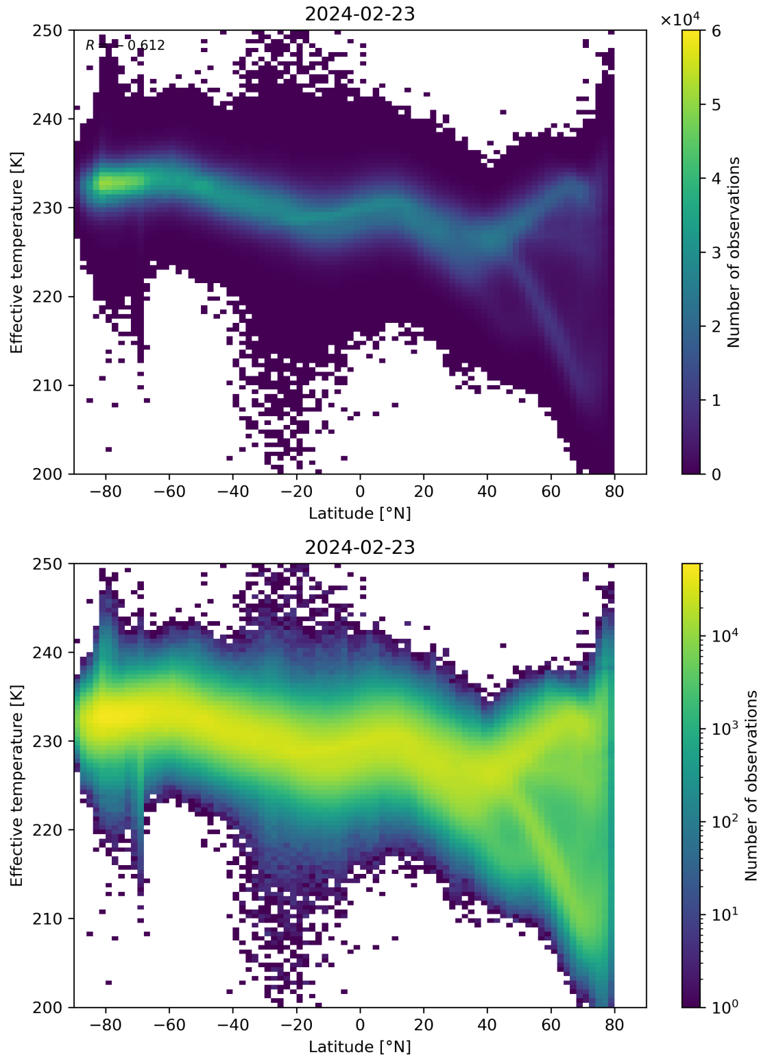
Figure 34: Scatter density plot of “Latitude” against “Effective temperature” for 2024-02-22 to 2024-02-24.
