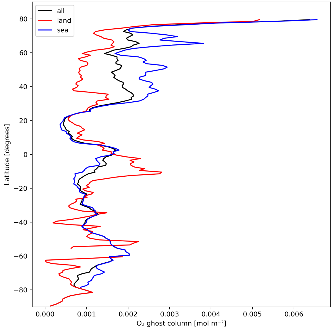
Figure 18: Zonal average of "O 3 ghost column" for 2024-02-22 to 2024-02-24.
